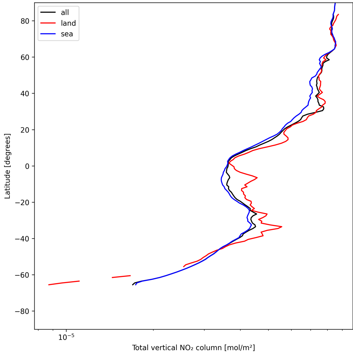
Figure 19: Zonal average of “Total vertical NO 2 column” for 2025-06-01 to 2025-06-02.
