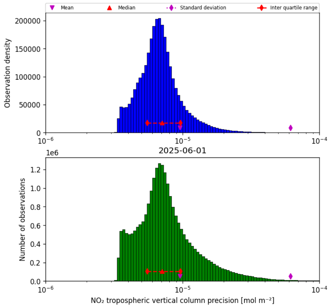
Figure 28: Histogram of “NO 2 tropospheric vertical column precision” for 2025-06-01 to 2025-06-02
