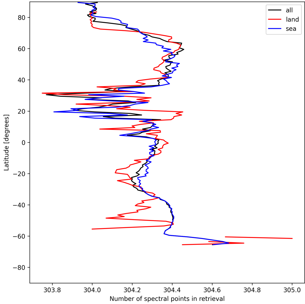
Figure 14: Zonal average of “Number of spectral points in retrieval” for 2025-06-01 to 2025-06-02.
