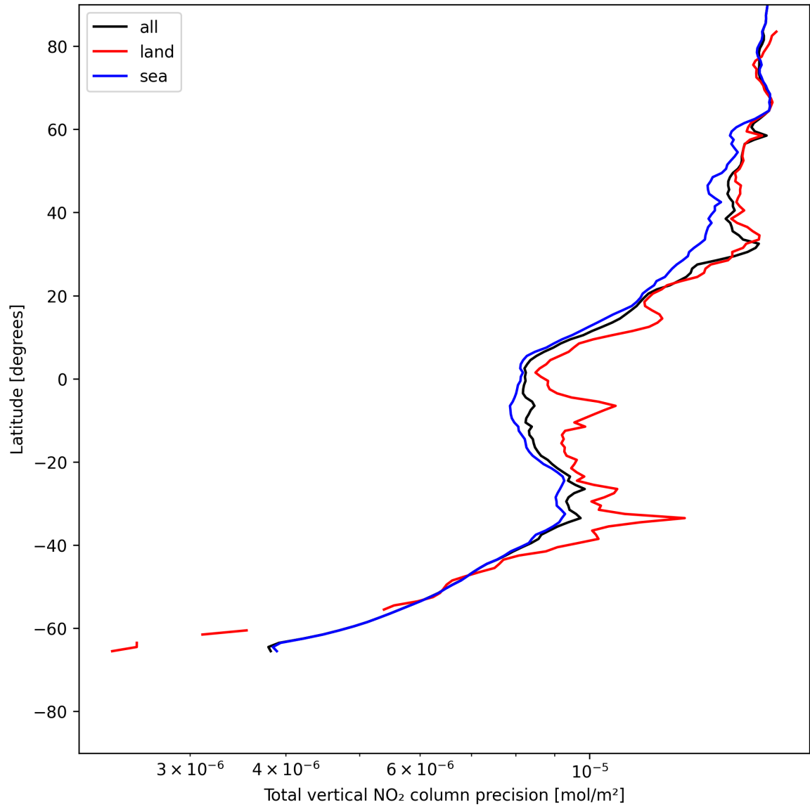
Figure 20: Zonal average of “Total vertical NO 2 column precision” for 2025-06-01 to 2025-06-02.
