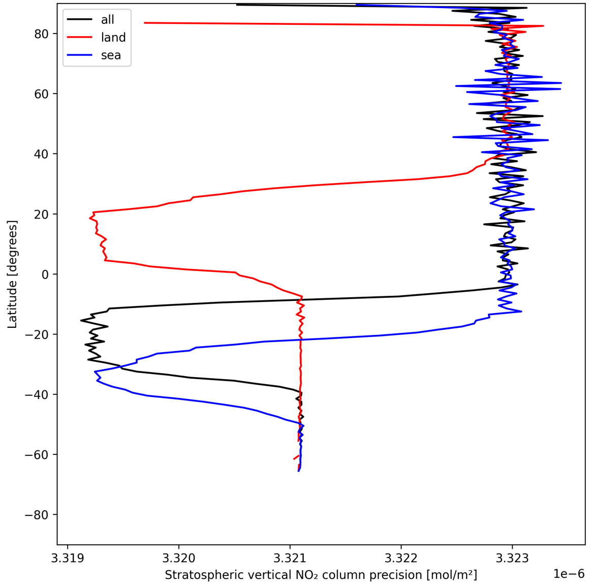
Figure 18: Zonal average of “Stratospheric vertical NO 2 column precision” for 2025-06-01 to 2025-06-02.
