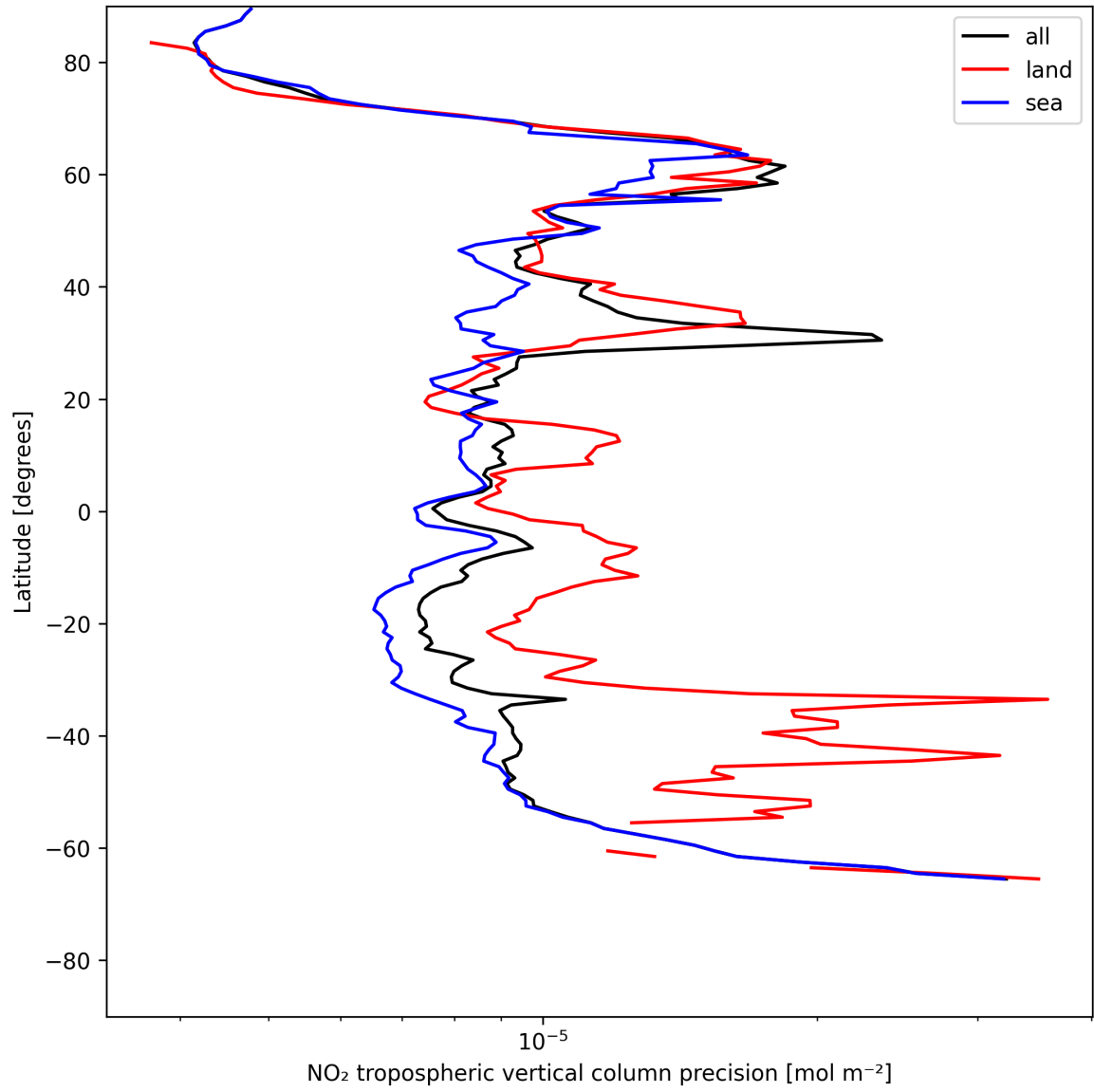
Figure 11: Zonal average of “NO 2 tropospheric vertical column precision” for 2025-06-01 to 2025-06-02.
