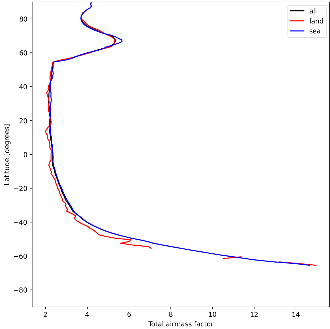
Figure 13: Zonal average of “Total airmass factor” for 2025-06-01 to 2025-06-02.
