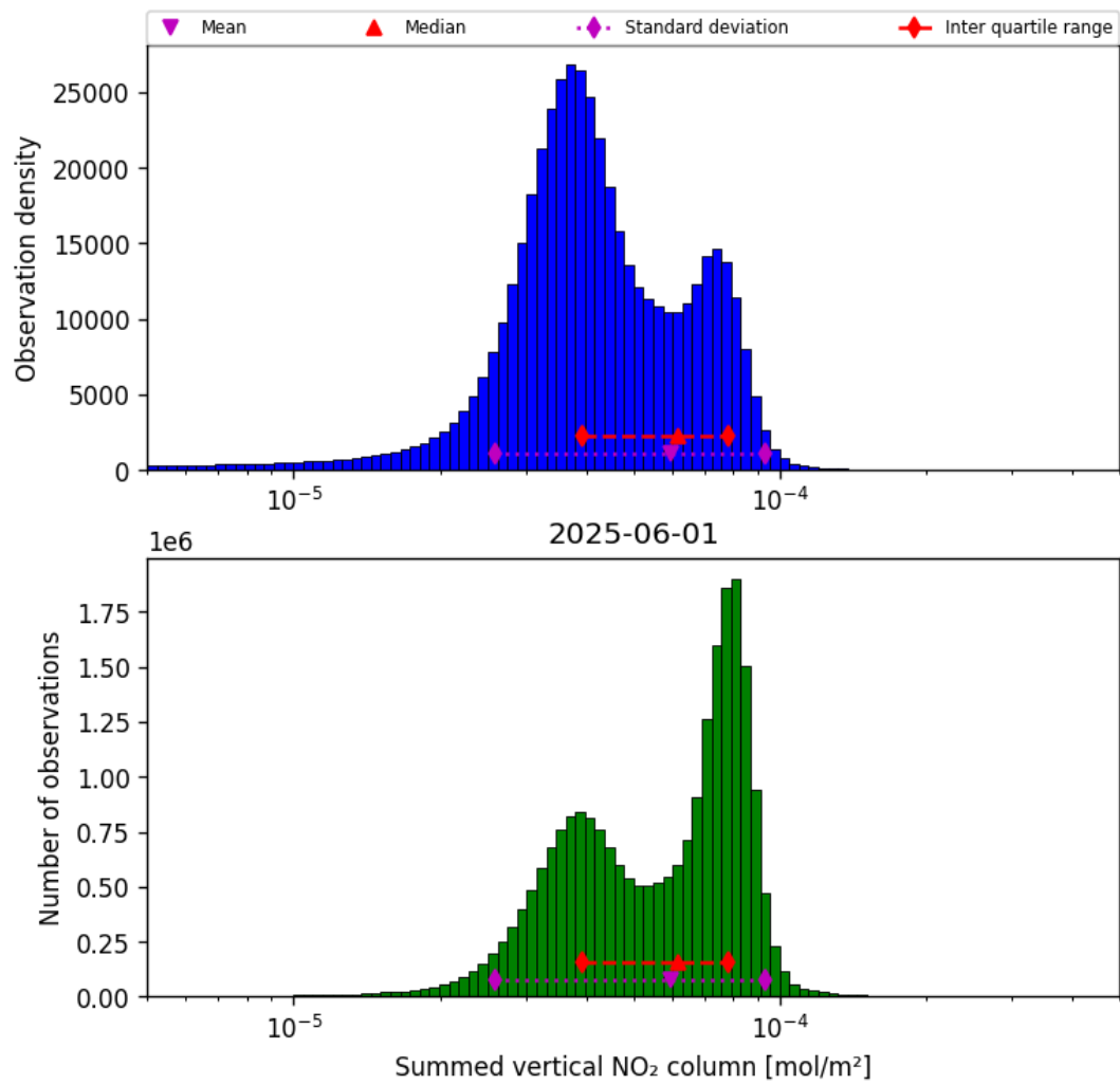
Figure 38: Histogram of “Summed vertical NO 2 column” for 2025-06-01 to 2025-06-02
