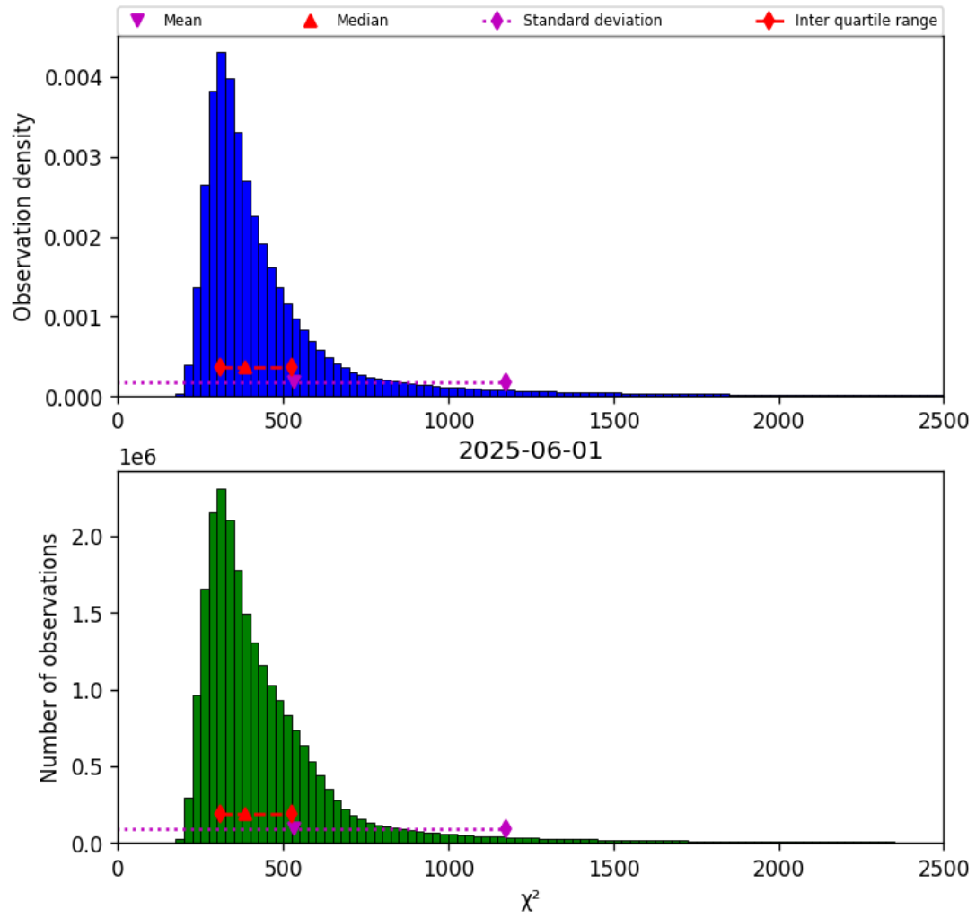
Figure 40: Histogram of “ \chi^2 ” for 2025-06-01 to 2025-06-02
