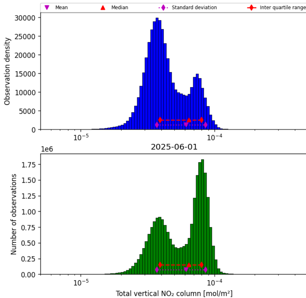
Figure 36: Histogram of “Total vertical NO 2 column” for 2025-06-01 to 2025-06-02
