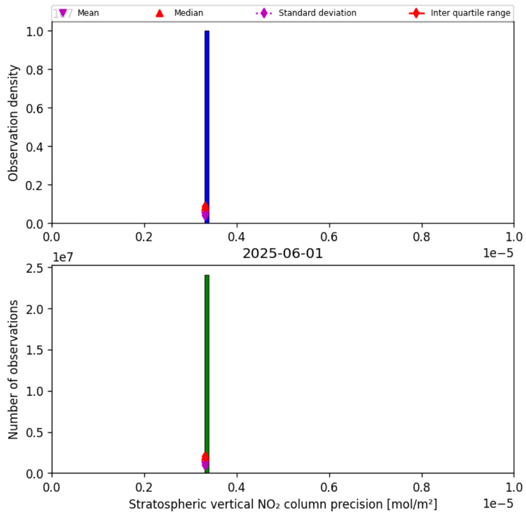
Figure 35: Histogram of “Stratospheric vertical NO 2 column precision” for 2025-06-01 to 2025-06-02
