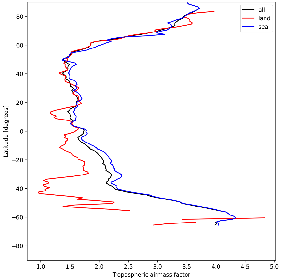
Figure 12: Zonal average of “Tropospheric airmass factor” for 2025-06-01 to 2025-06-02.
