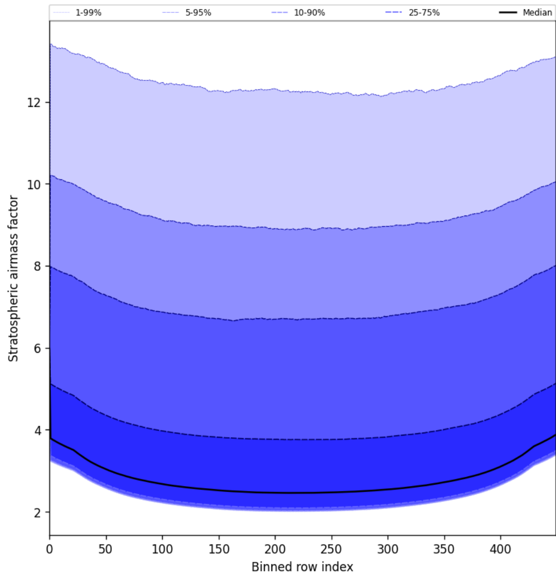
Figure 59: Along track statistics of “Stratospheric airmass factor” for 2025-06-01 to 2025-06-02
