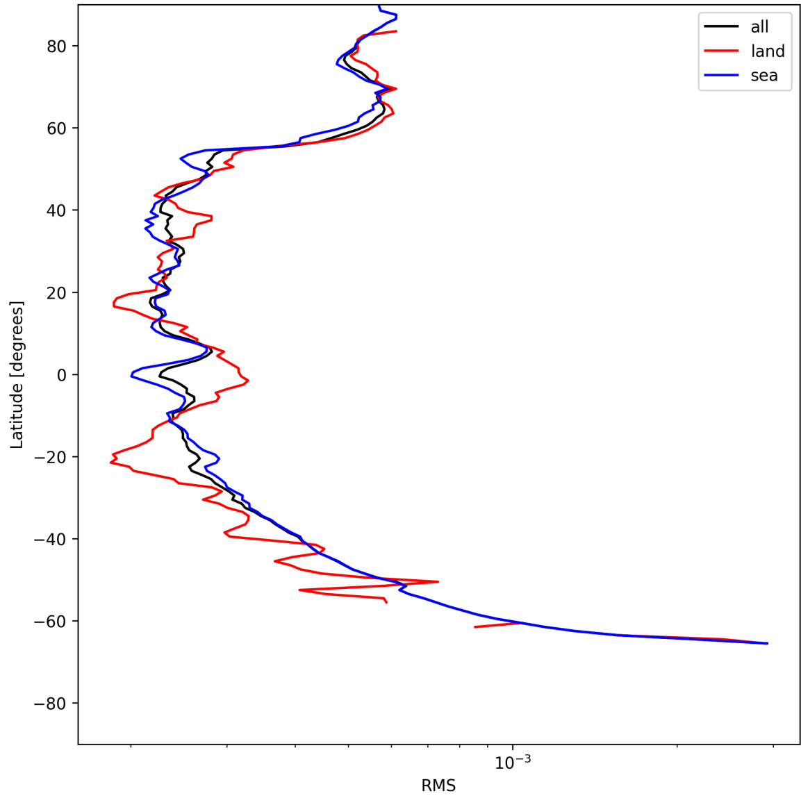
Figure 24: Zonal average of “RMS” for 2025-06-01 to 2025-06-02.
