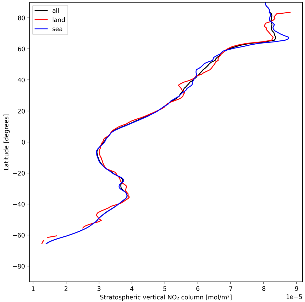
Figure 17: Zonal average of “Stratospheric vertical NO 2 column” for 2025-06-01 to 2025-06-02.
