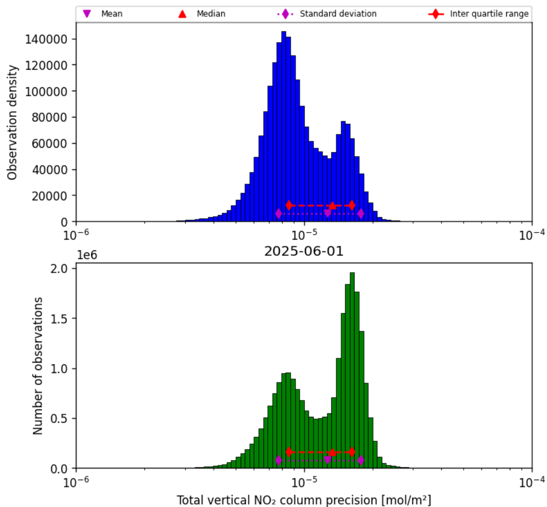
Figure 37: Histogram of “Total vertical NO 2 column precision” for 2025-06-01 to 2025-06-02
