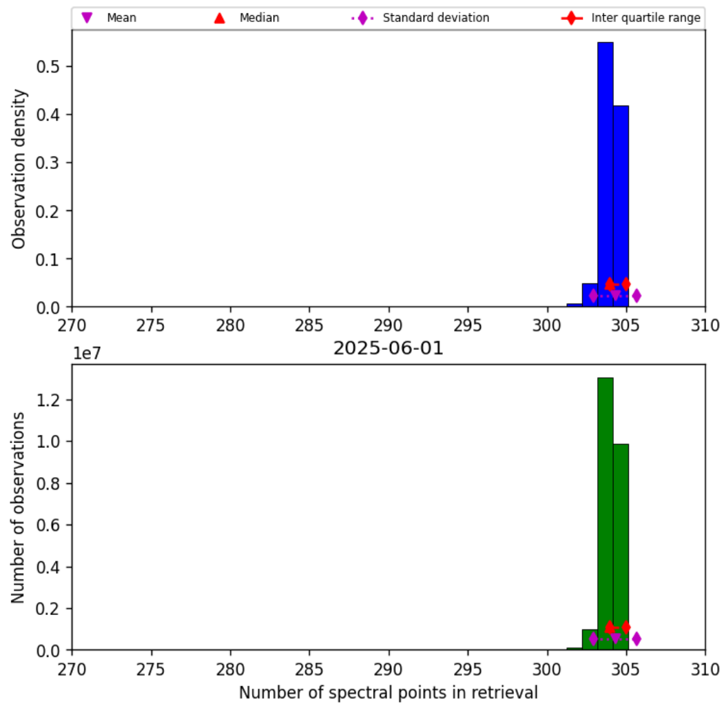
Figure 31: Histogram of “Number of spectral points in retrieval” for 2025-06-01 to 2025-06-02
