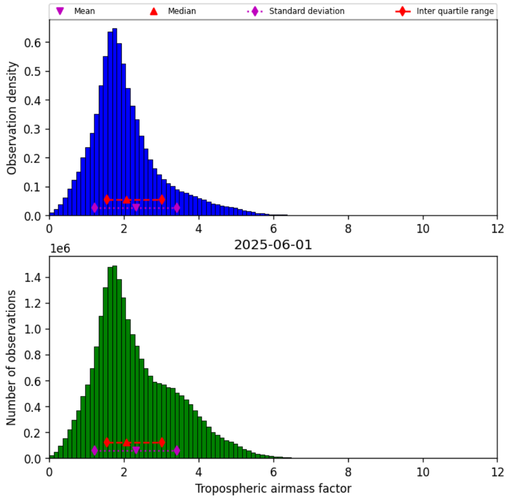
Figure 29: Histogram of “Tropospheric airmass factor” for 2025-06-01 to 2025-06-02
