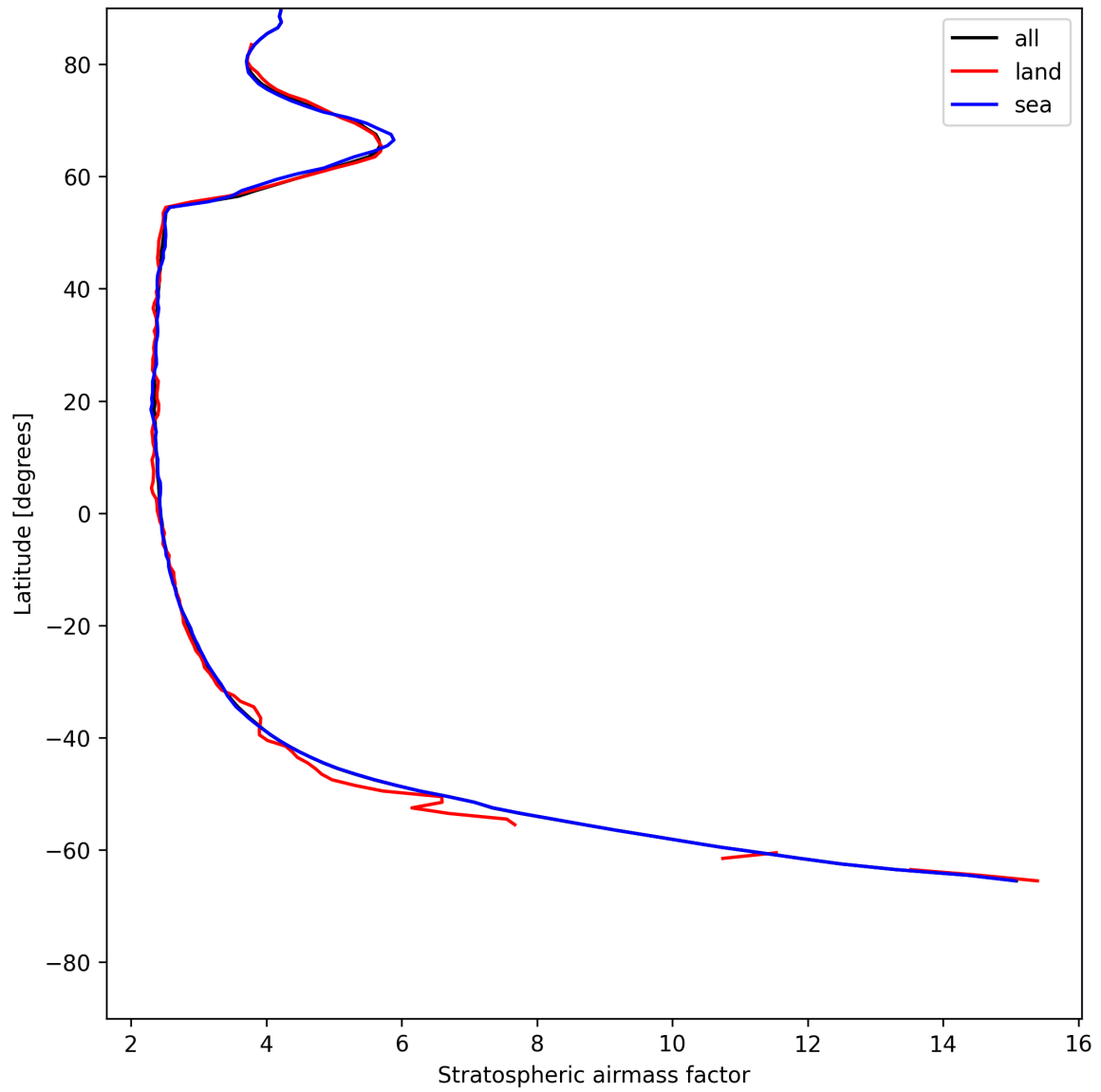
Figure 25: Zonal average of “Stratospheric airmass factor” for 2025-06-01 to 2025-06-02.
