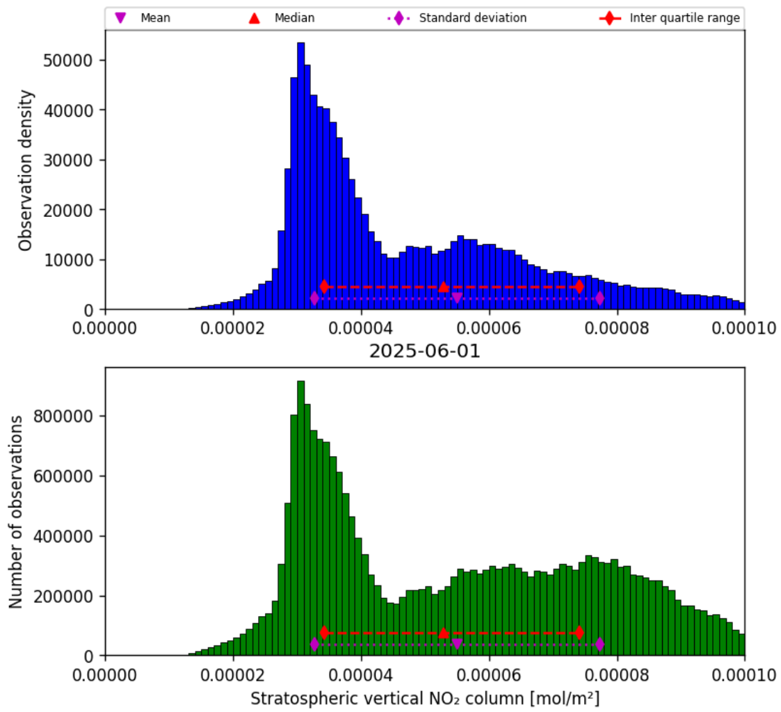
Figure 34: Histogram of “Stratospheric vertical NO 2 column” for 2025-06-01 to 2025-06-02
