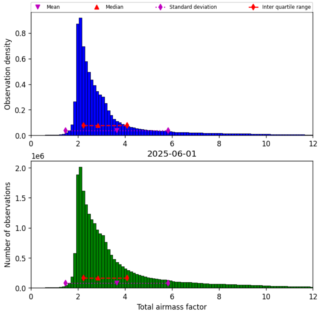
Figure 30: Histogram of “Total airmass factor” for 2025-06-01 to 2025-06-02
