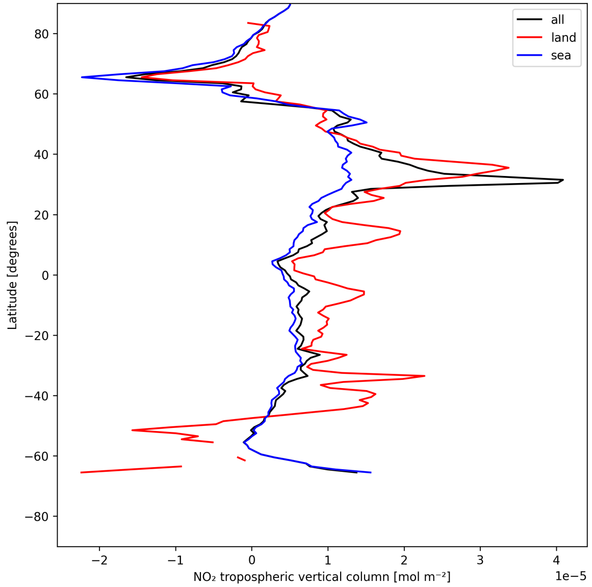
Figure 10: Zonal average of “NO 2 tropospheric vertical column” for 2025-06-01 to 2025-06-02.
