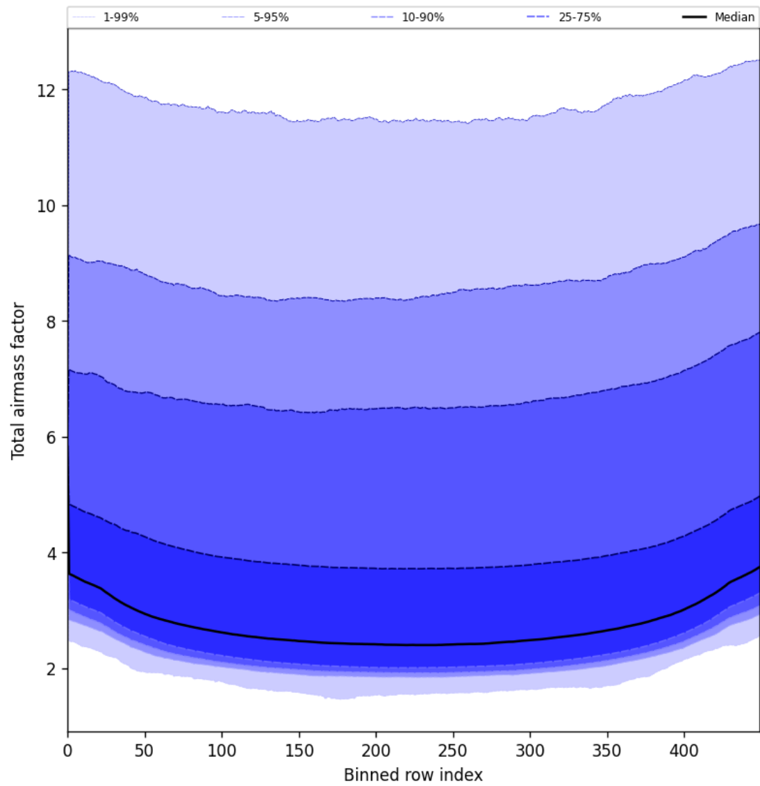
Figure 47: Along track statistics of “Total airmass factor” for 2025-06-01 to 2025-06-02
