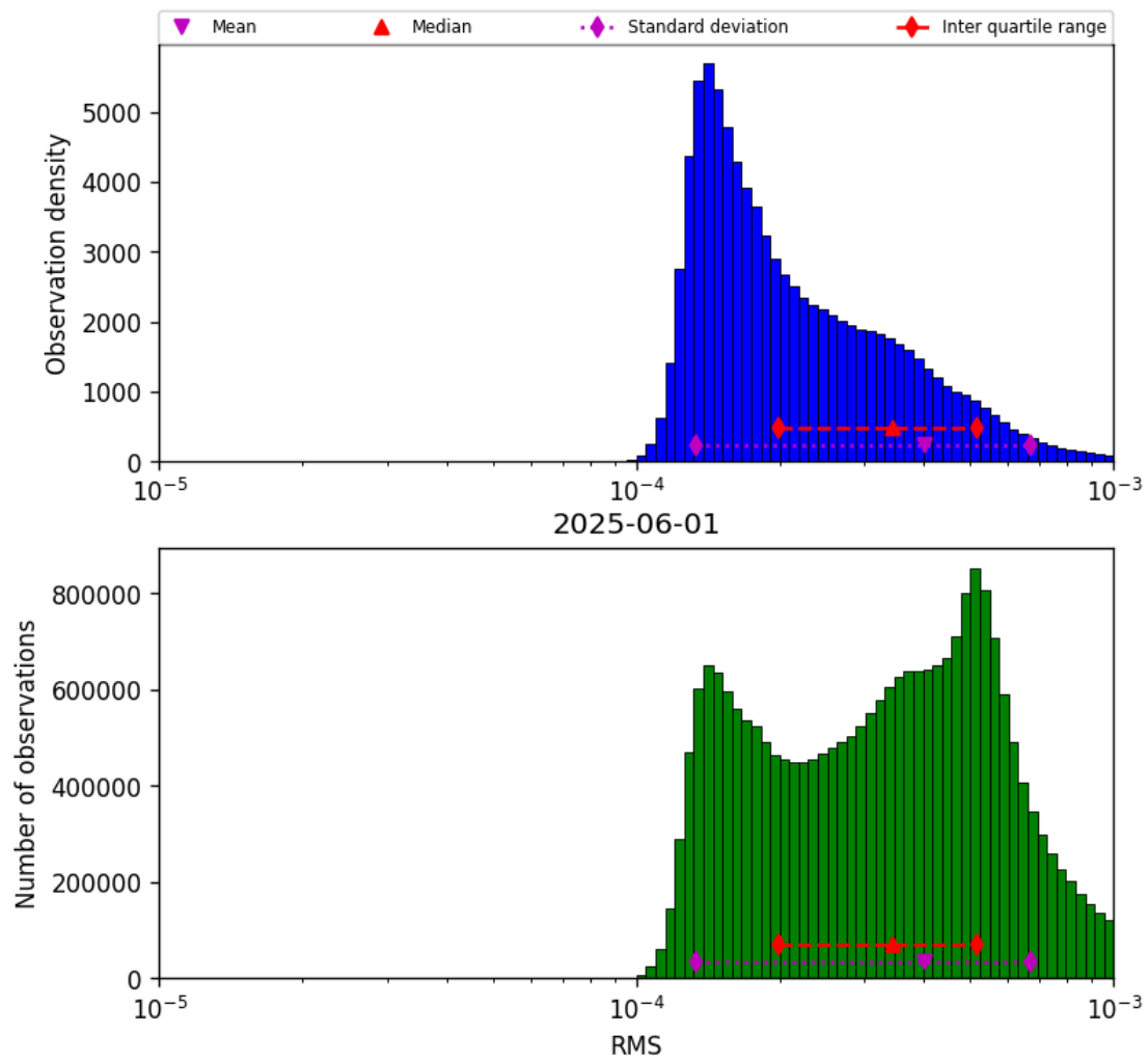
Figure 41: Histogram of “RMS” for 2025-06-01 to 2025-06-02
