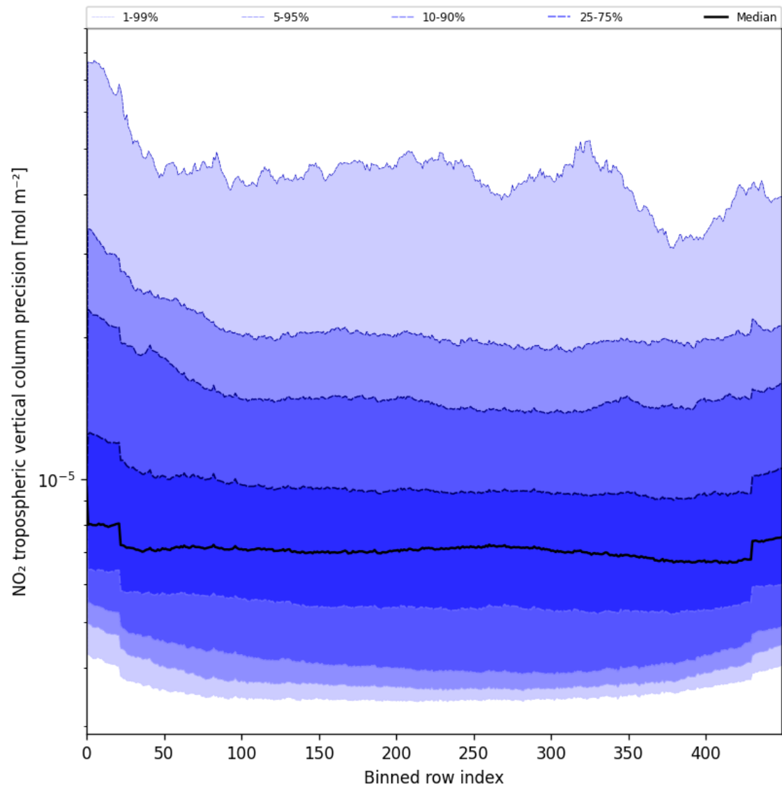
Figure 45: Along track statistics of “NO 2 tropospheric vertical column precision” for 2025-06-01 to 2025-06-02
