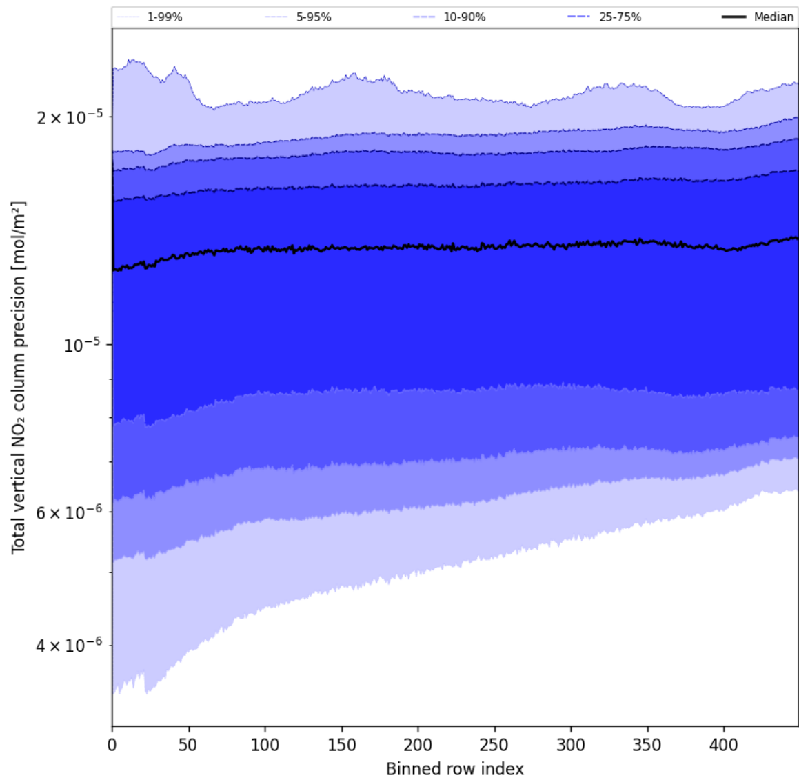
Figure 54: Along track statistics of “Total vertical NO 2 column precision” for 2025-06-01 to 2025-06-02
