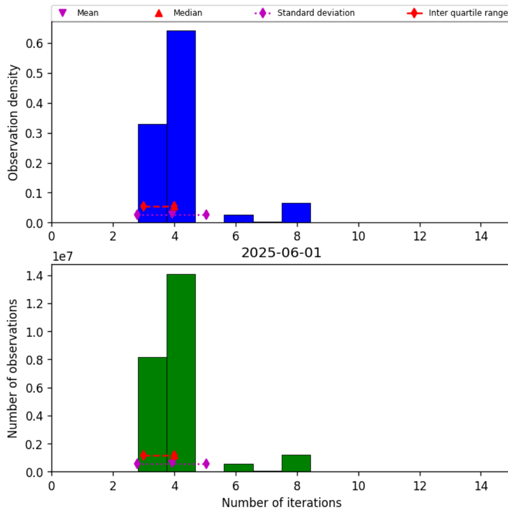
Figure 32: Histogram of “Number of iterations” for 2025-06-01 to 2025-06-02
