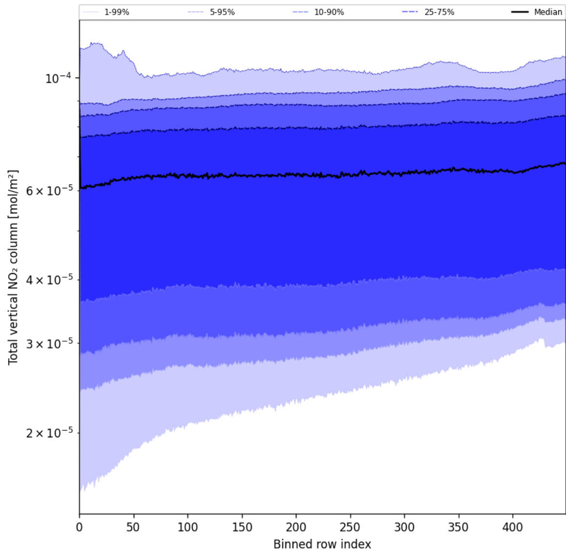
Figure 53: Along track statistics of “Total vertical NO 2 column” for 2025-06-01 to 2025-06-02
