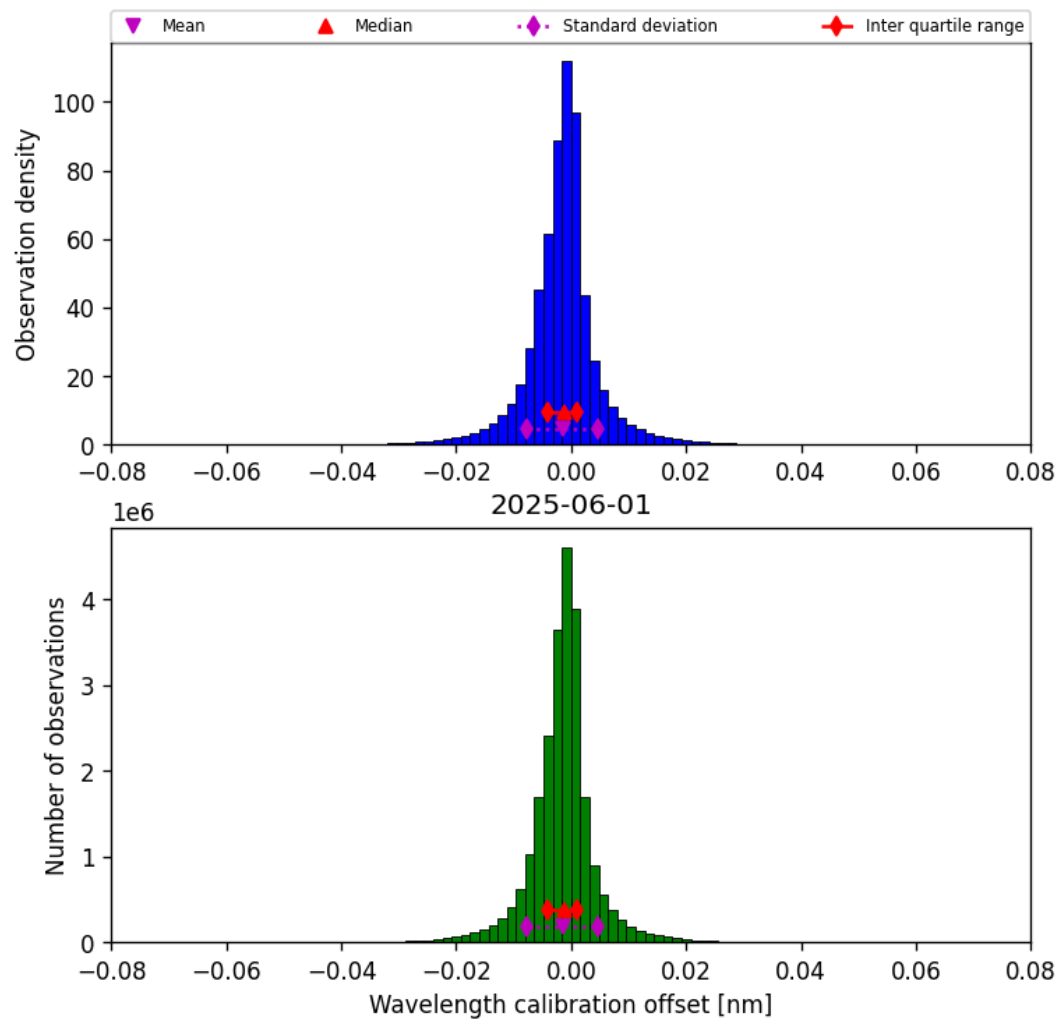
Figure 33: Histogram of “Wavelength calibration offset” for 2025-06-01 to 2025-06-02
