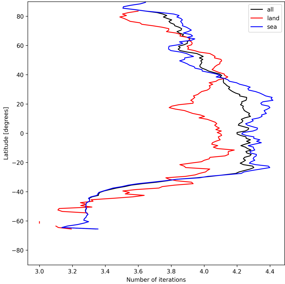
Figure 15: Zonal average of “Number of iterations” for 2025-06-01 to 2025-06-02.
