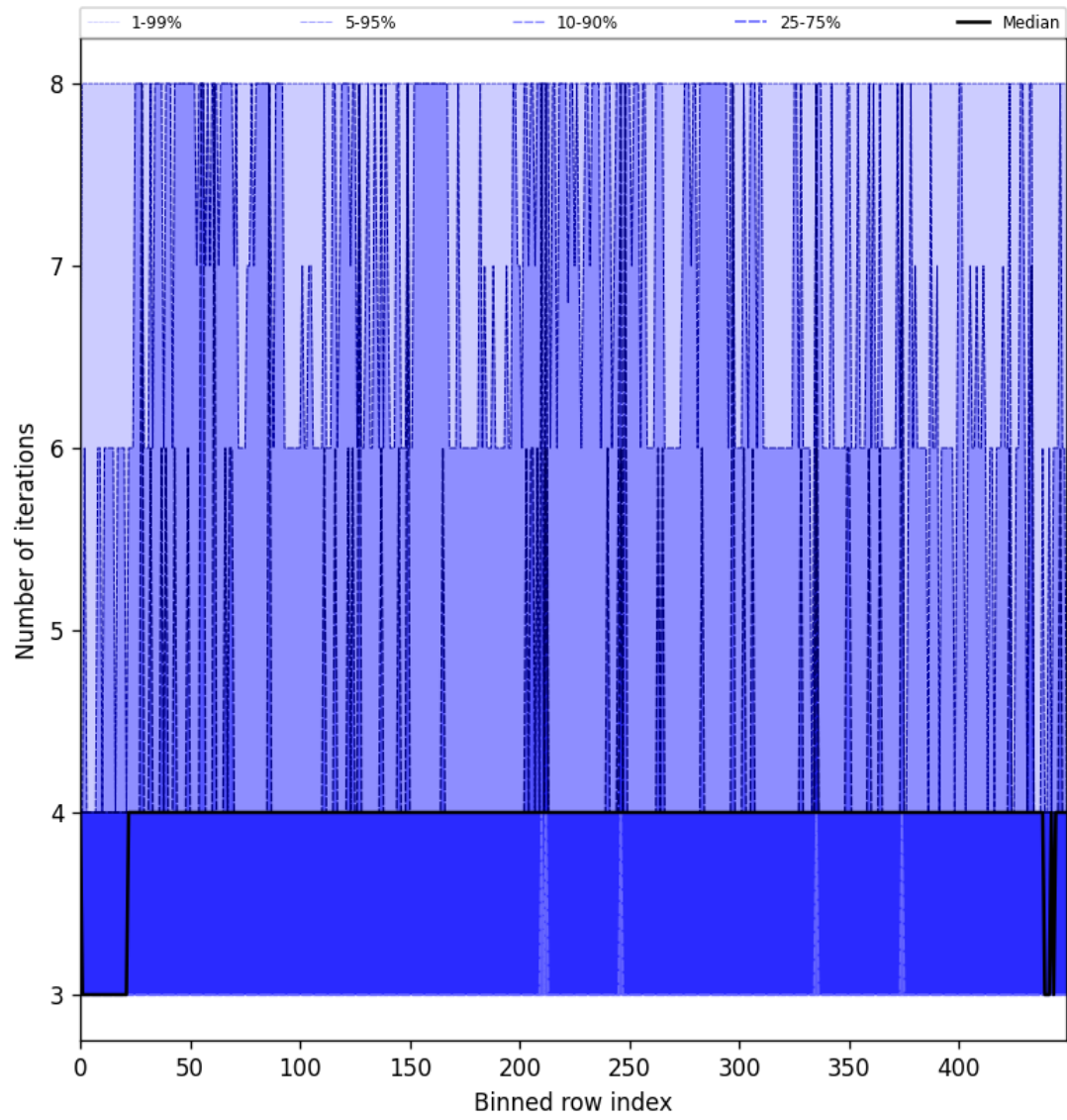
Figure 49: Along track statistics of “Number of iterations” for 2025-06-01 to 2025-06-02
