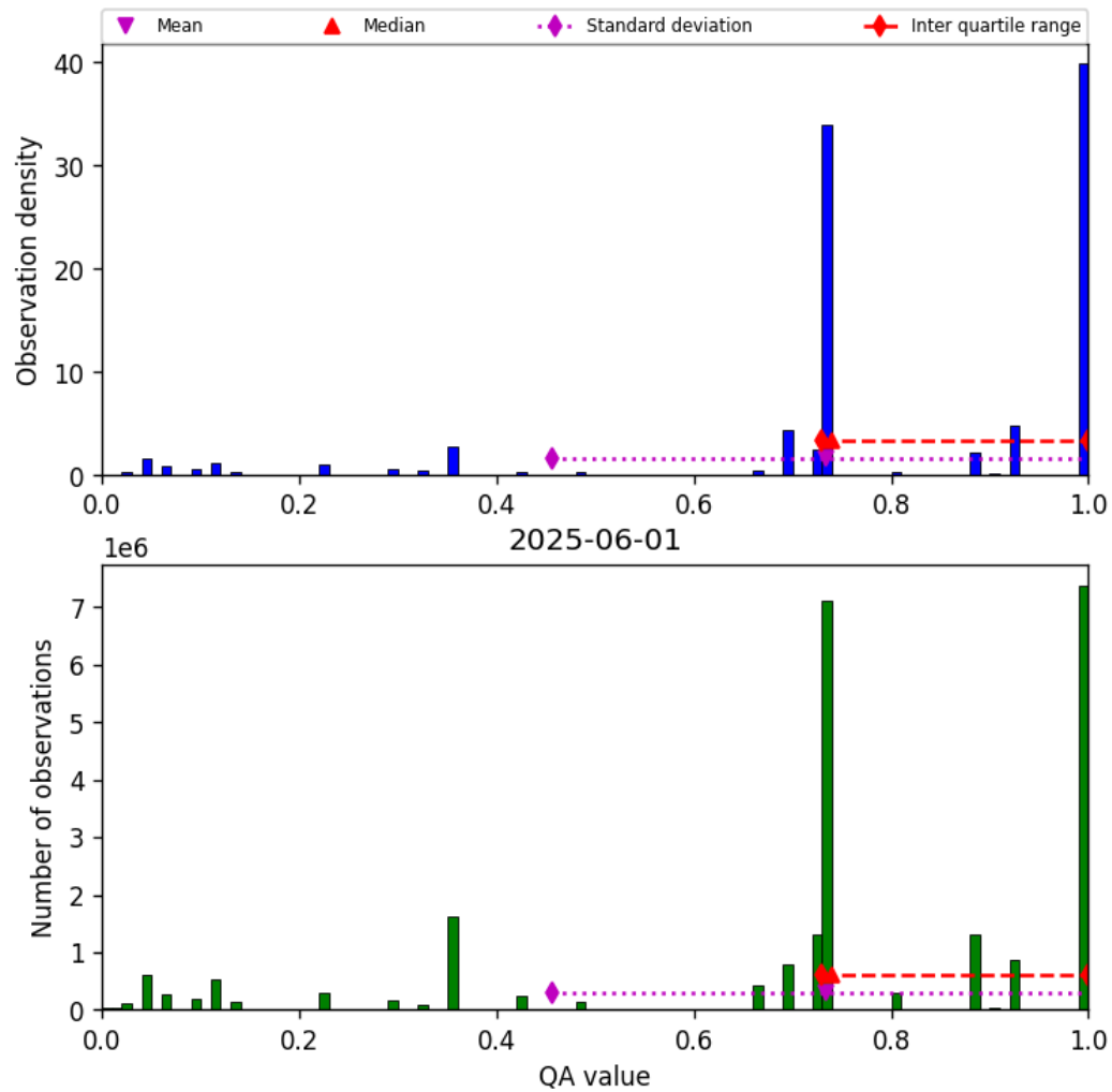
Figure 26: Histogram of “QA value” for 2025-06-01 to 2025-06-02
