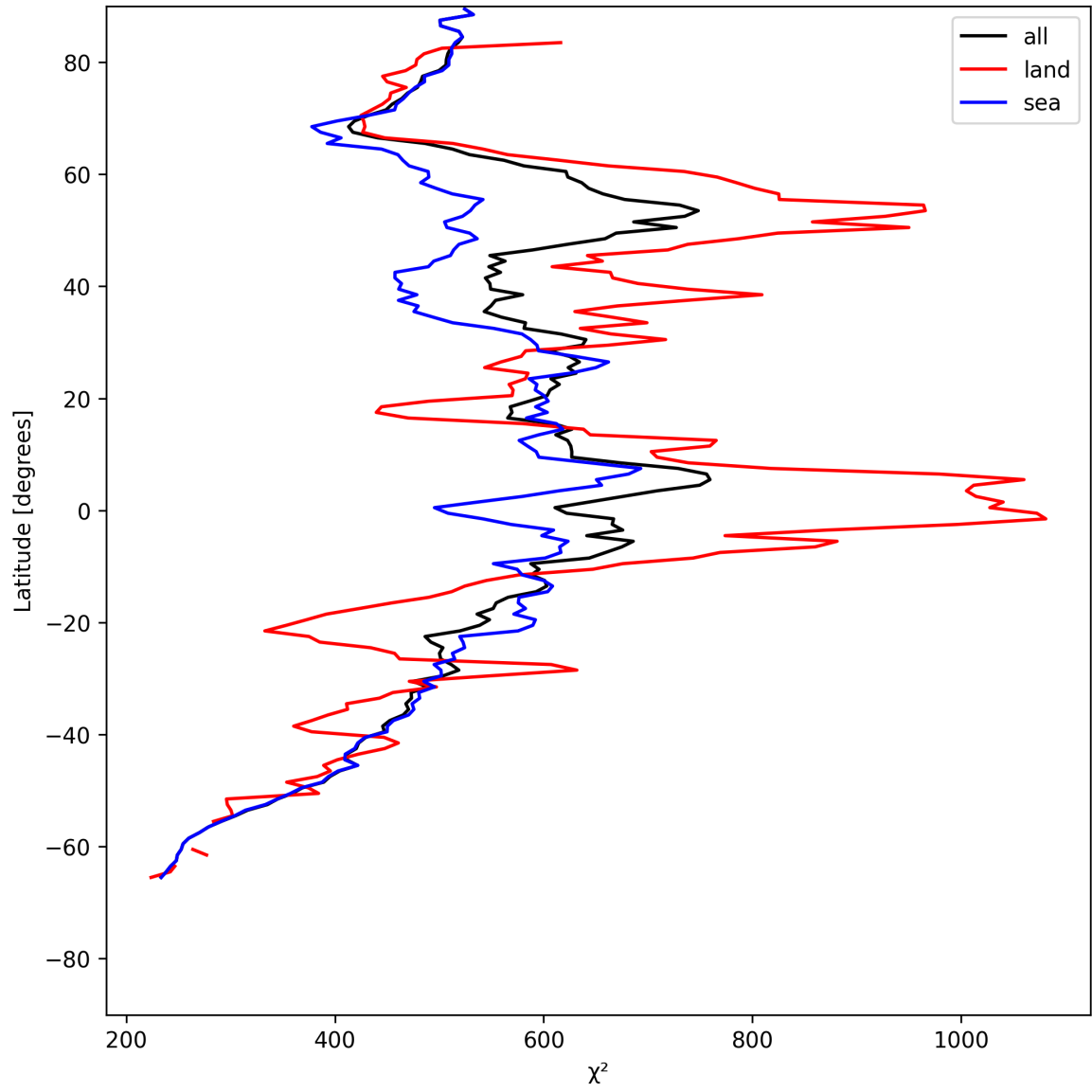
Figure 23: Zonal average of “ \chi^2 ” for 2025-06-01 to 2025-06-02.
