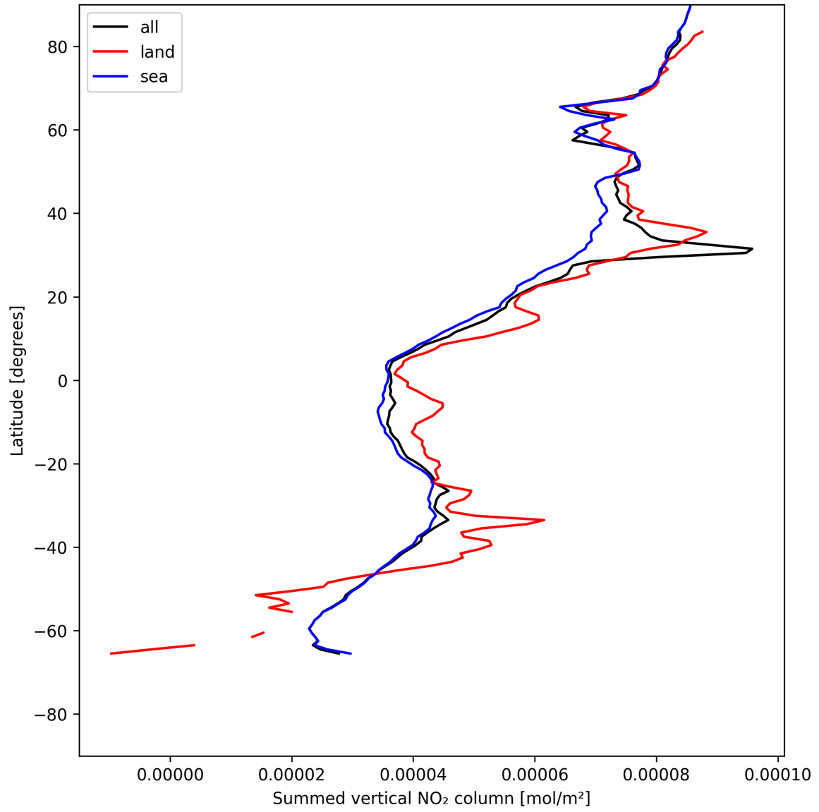
Figure 21: Zonal average of “Summed vertical NO 2 column” for 2025-06-01 to 2025-06-02.
