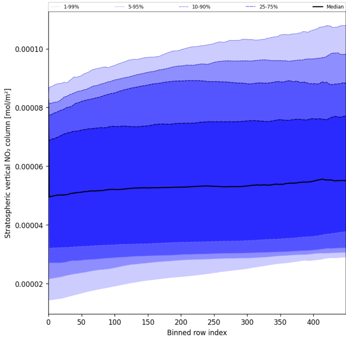
Figure 51: Along track statistics of “Stratospheric vertical NO 2 column” for 2025-06-01 to 2025-06-02
