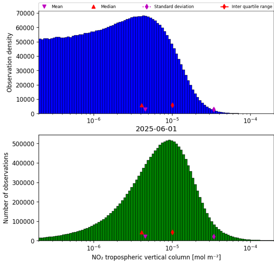
Figure 27: Histogram of “NO 2 tropospheric vertical column” for 2025-06-01 to 2025-06-02
