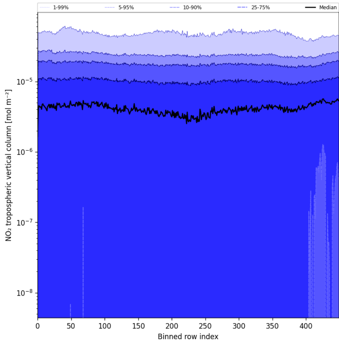
Figure 44: Along track statistics of “NO 2 tropospheric vertical column” for 2025-06-01 to 2025-06-02
