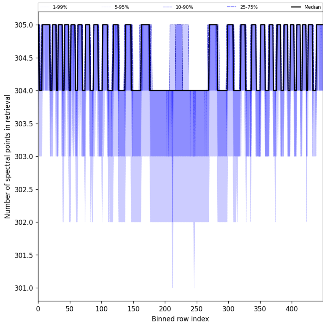
Figure 48: Along track statistics of “Number of spectral points in retrieval” for 2025-06-01 to 2025-06-02
