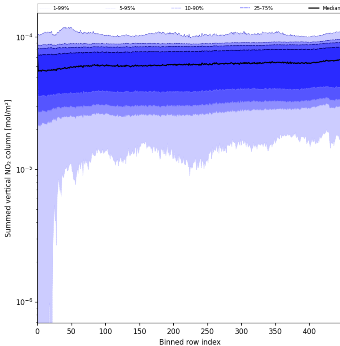
Figure 55: Along track statistics of “Summed vertical NO 2 column” for 2025-06-01 to 2025-06-02
