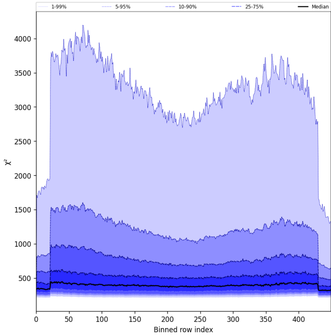
Figure 57: Along track statistics of “ \chi^2 ” for 2025-06-01 to 2025-06-02
