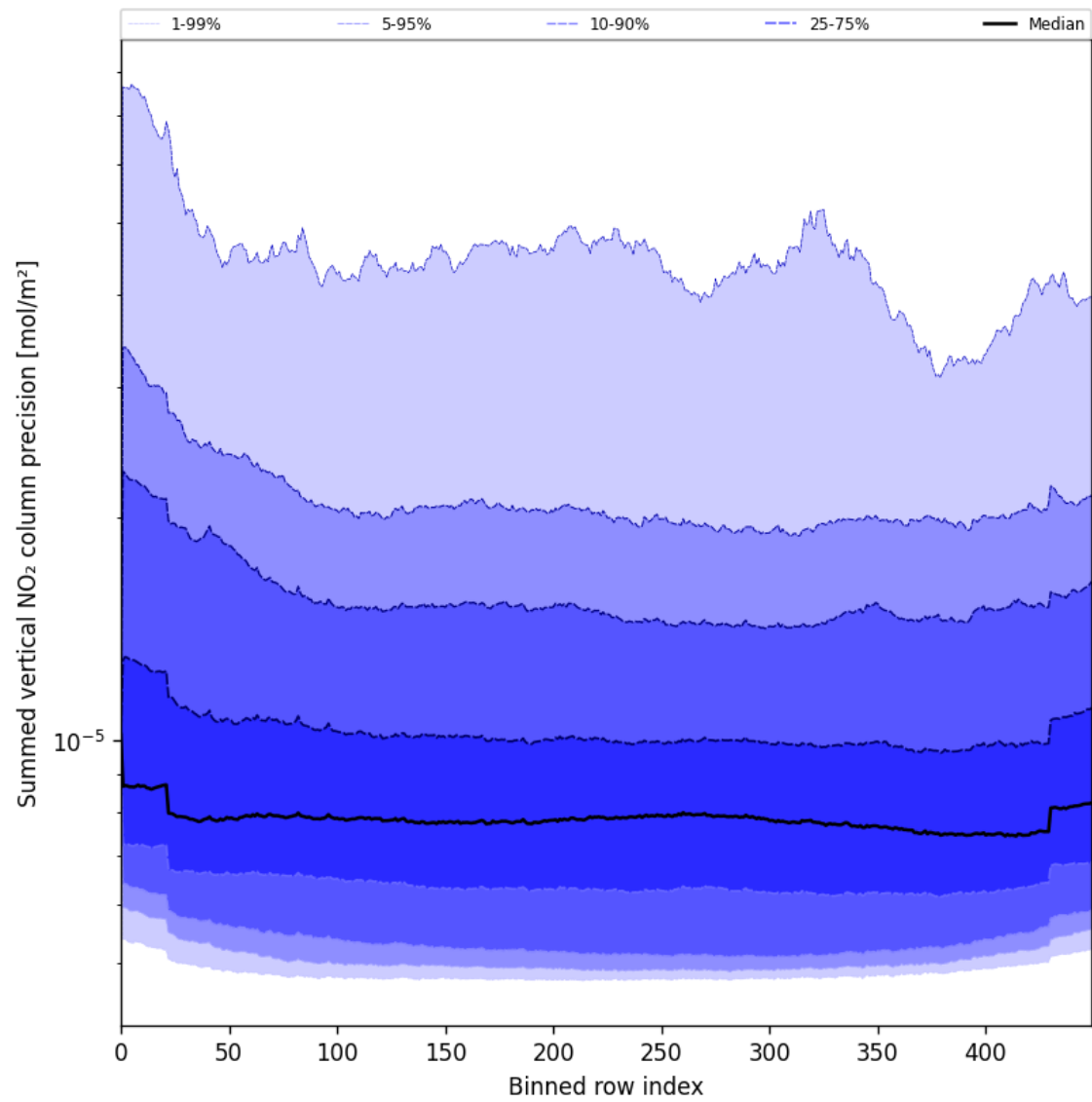
Figure 56: Along track statistics of “Summed vertical NO 2 column precision” for 2025-06-01 to 2025-06-02
