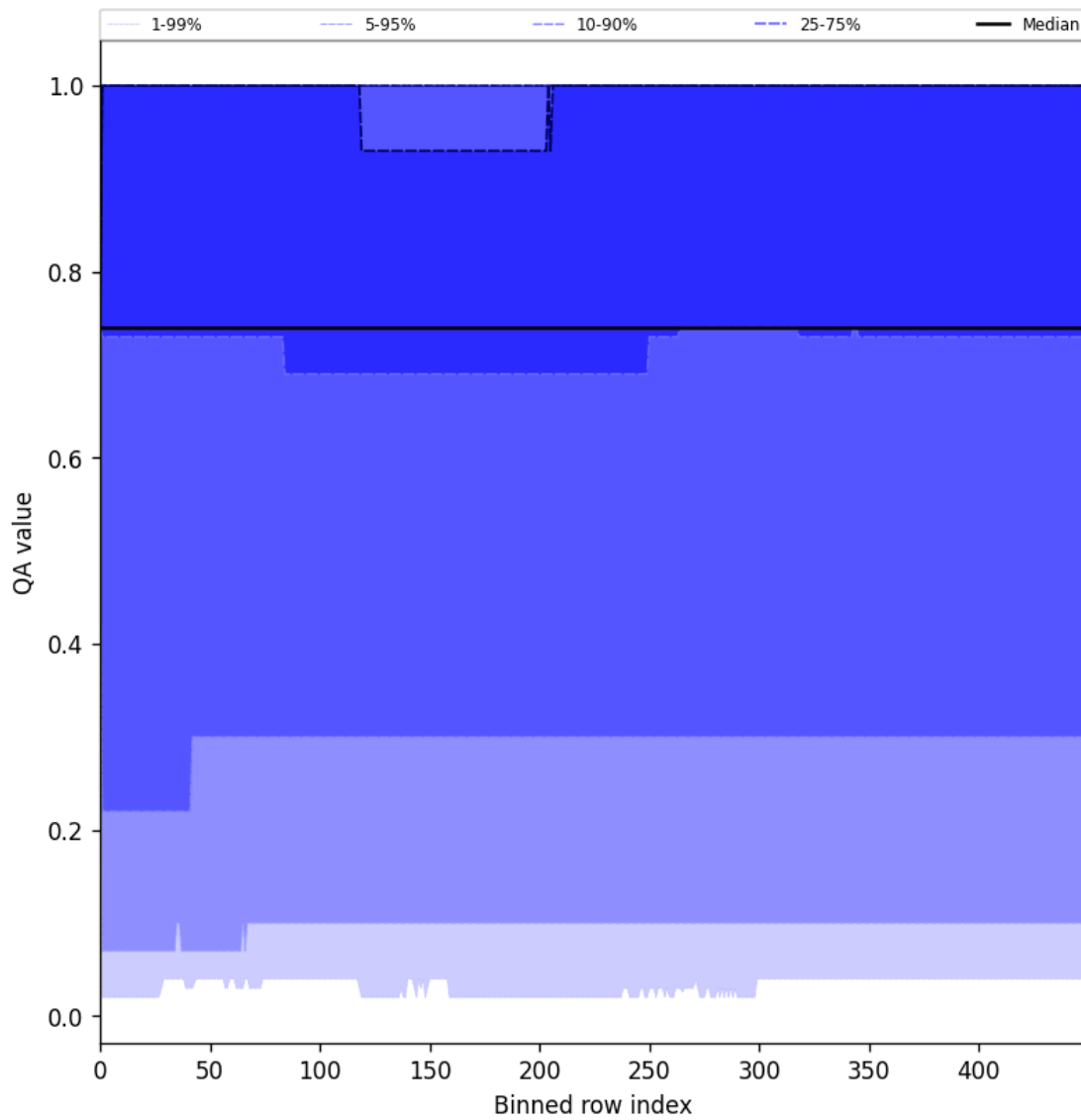
Figure 43: Along track statistics of “QA value” for 2025-06-01 to 2025-06-02
