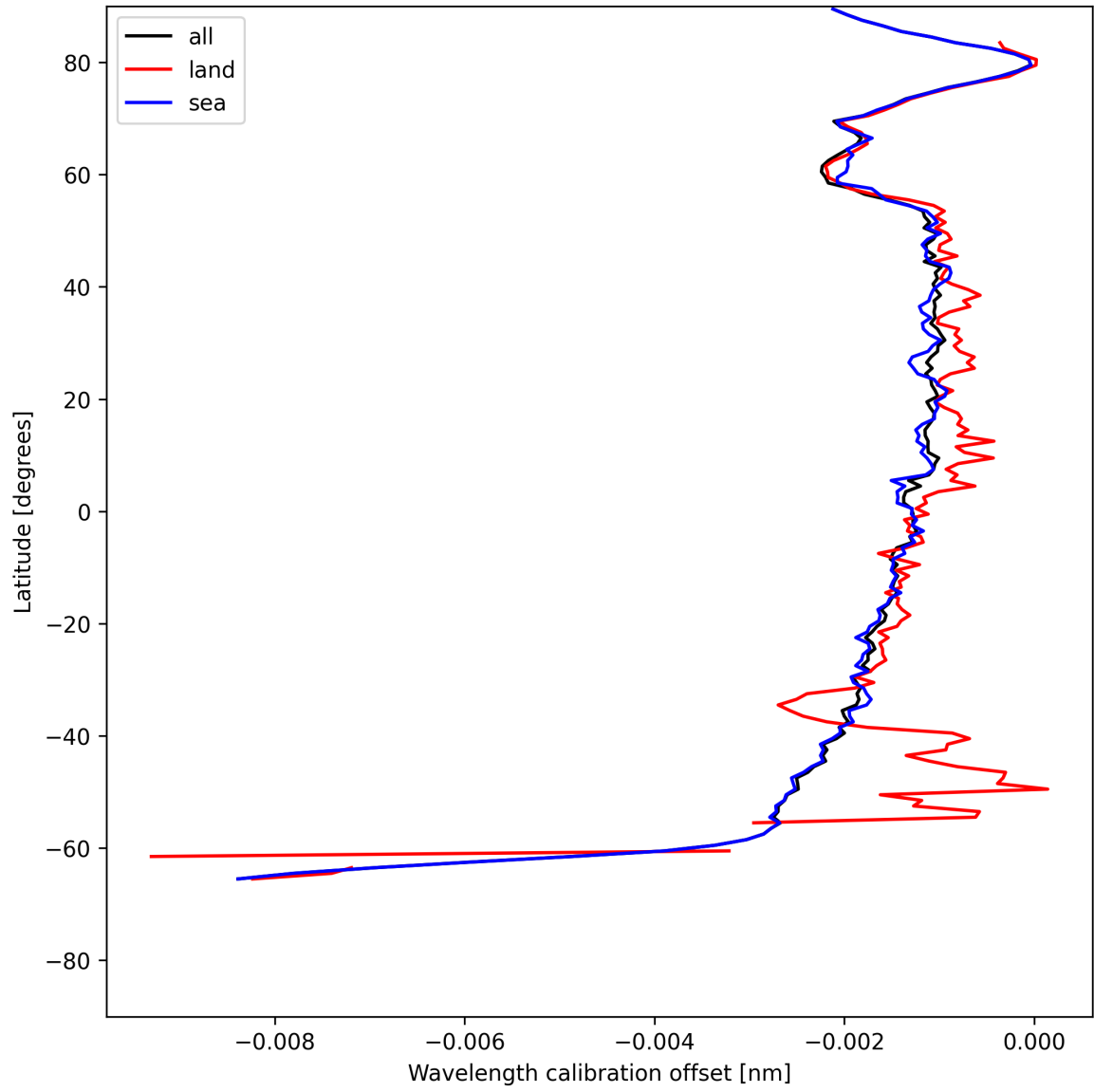
Figure 16: Zonal average of “Wavelength calibration offset” for 2025-06-01 to 2025-06-02.
