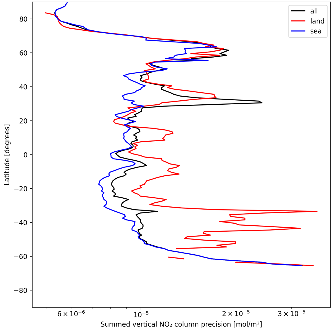
Figure 22: Zonal average of “Summed vertical NO 2 column precision” for 2025-06-01 to 2025-06-02.
