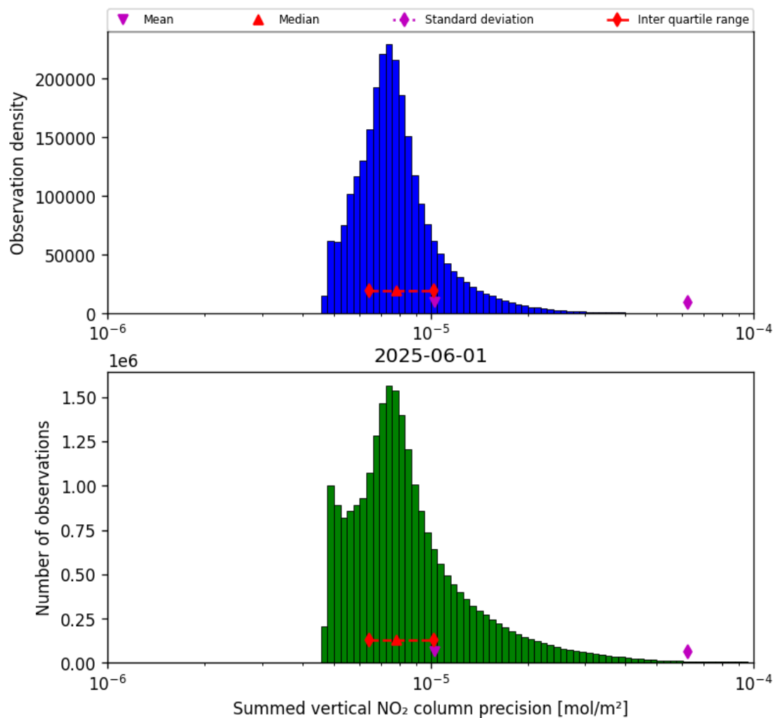
Figure 39: Histogram of "Summed vertical NO 2 column precision" for 2025-06-01 to 2025-06-02
