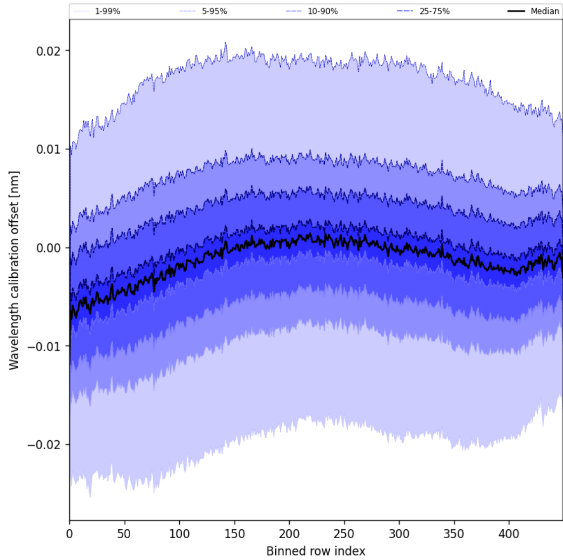
Figure 50: Along track statistics of “Wavelength calibration offset” for 2025-06-01 to 2025-06-02
