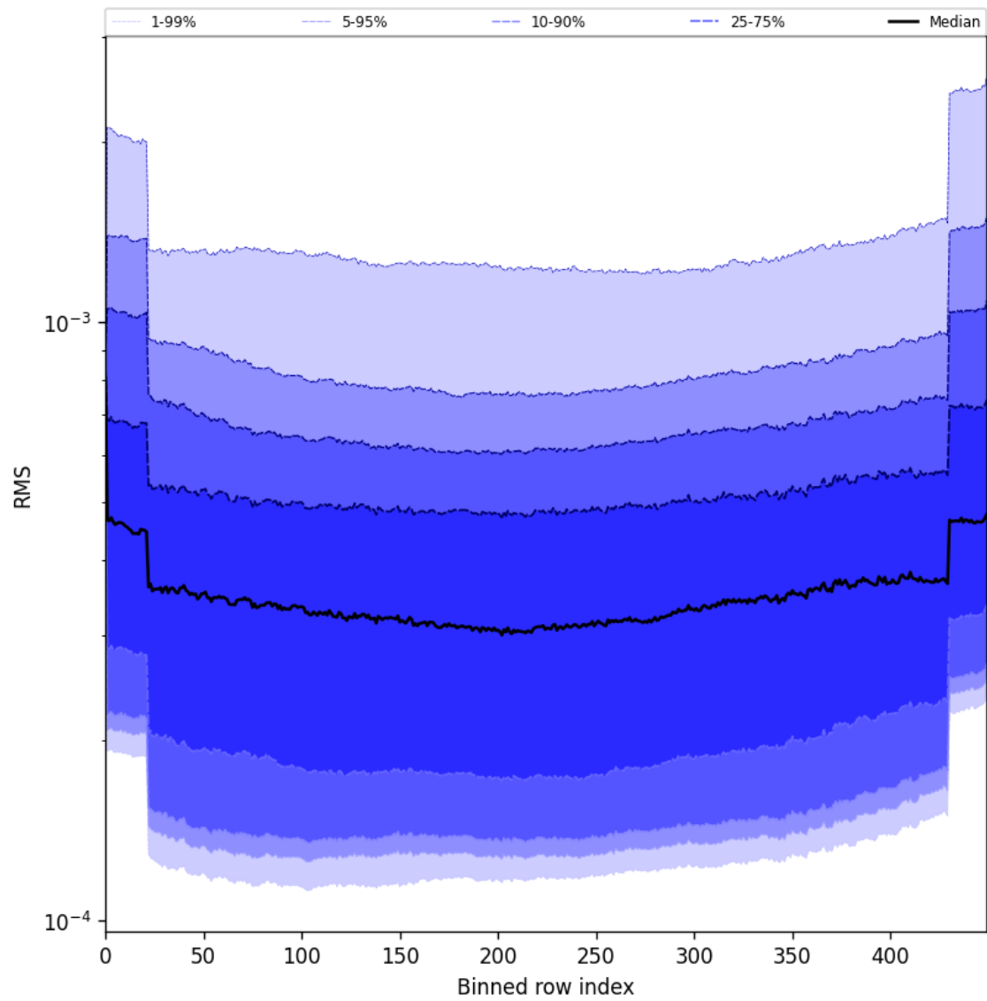
Figure 58: Along track statistics of “RMS” for 2025-06-01 to 2025-06-02
