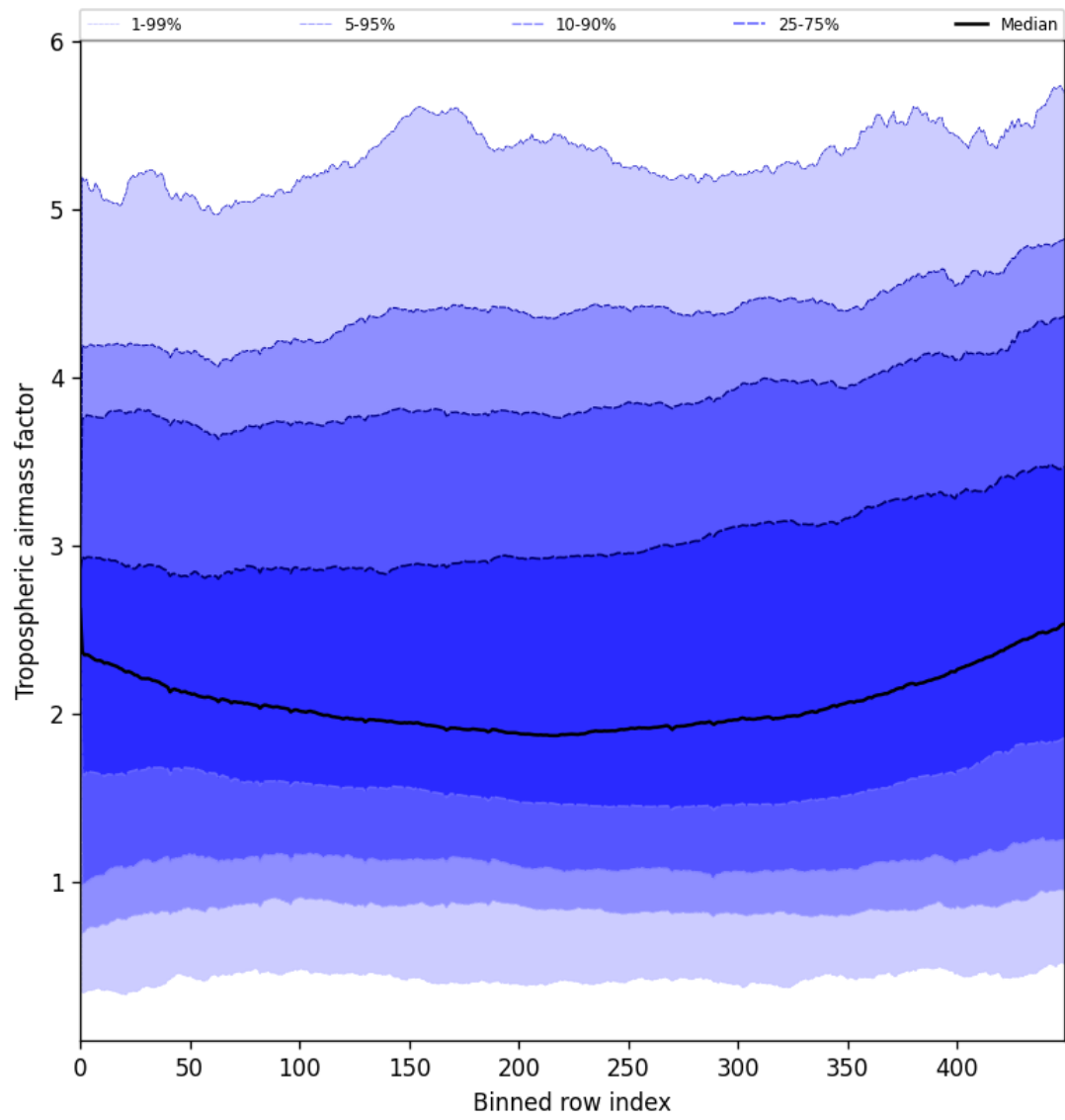
Figure 46: Along track statistics of “Tropospheric airmass factor” for 2025-06-01 to 2025-06-02
