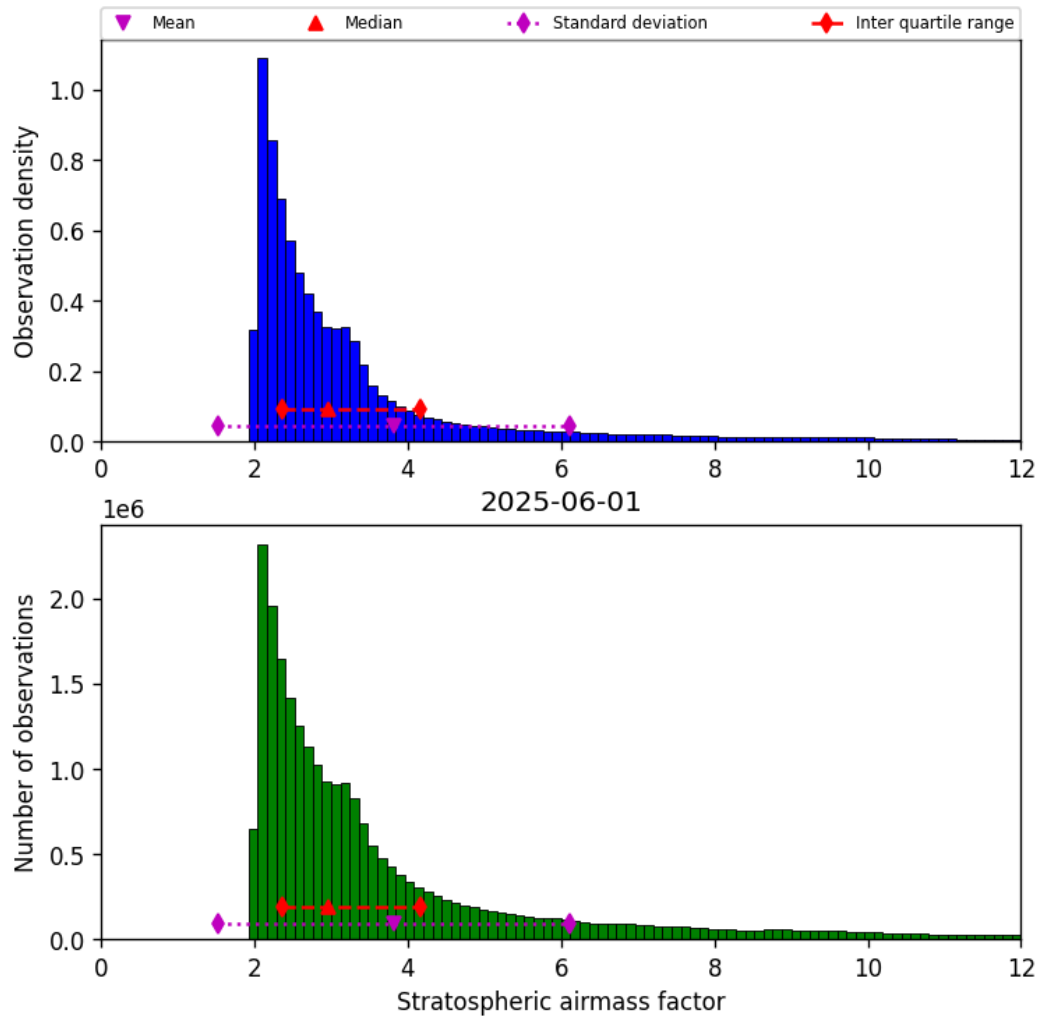
Figure 42: Histogram of “Stratospheric airmass factor” for 2025-06-01 to 2025-06-02
