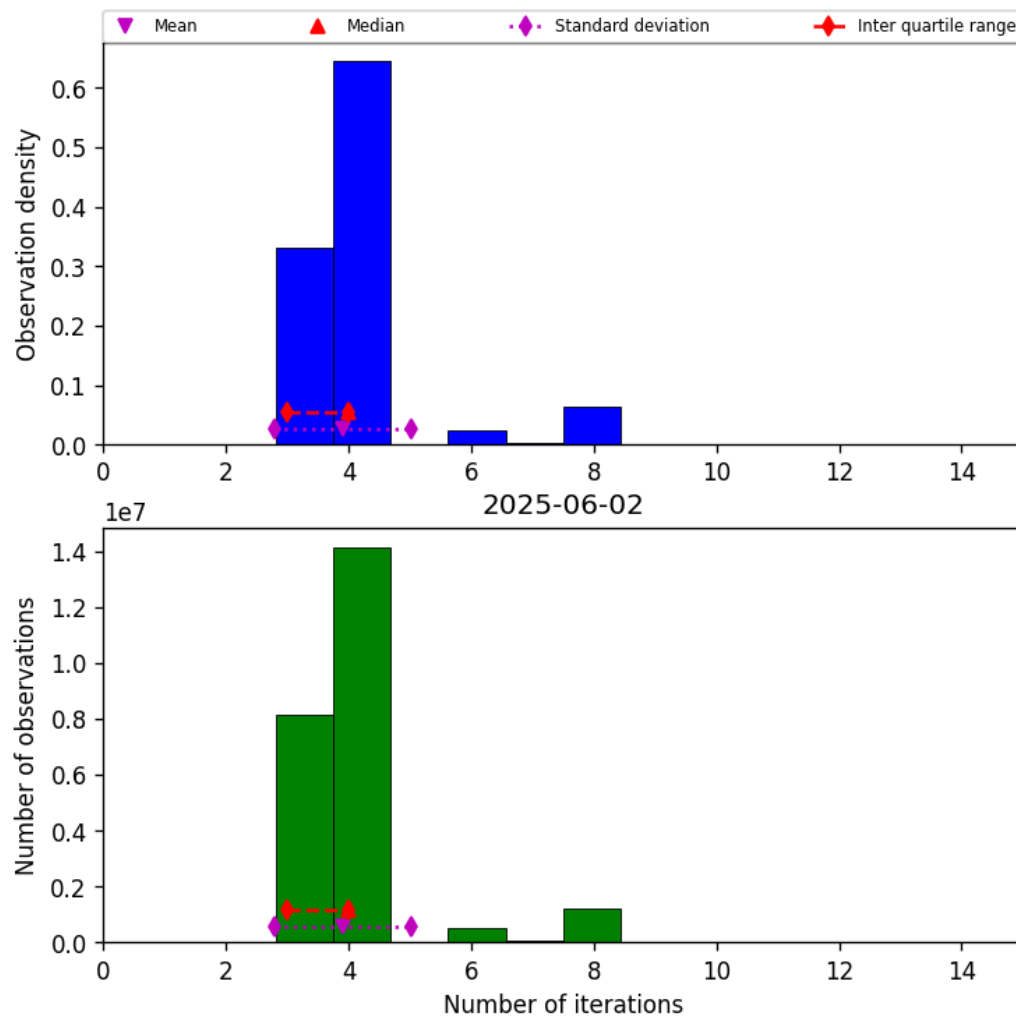
Figure 32: Histogram of “Number of iterations” for 2025-06-02 to 2025-06-03
