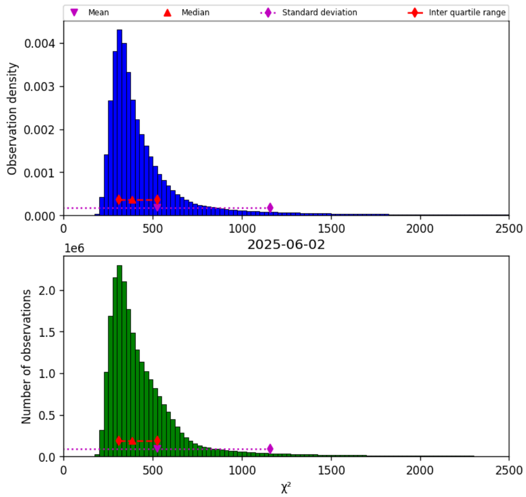
Figure 40: Histogram of “ \chi^2 ” for 2025-06-02 to 2025-06-03
