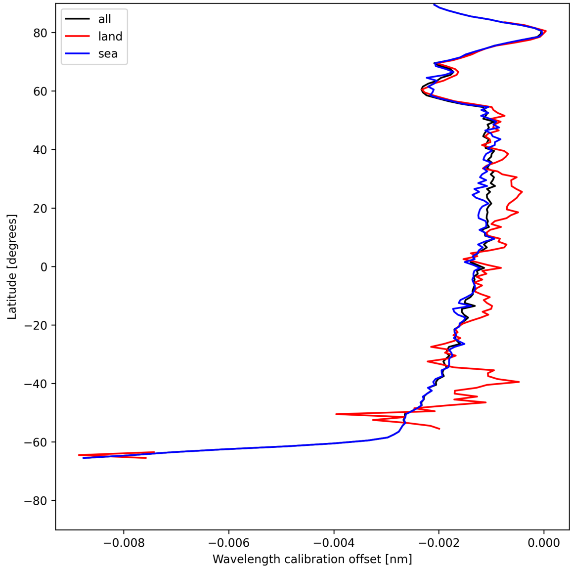
Figure 16: Zonal average of “Wavelength calibration offset” for 2025-06-02 to 2025-06-03.
