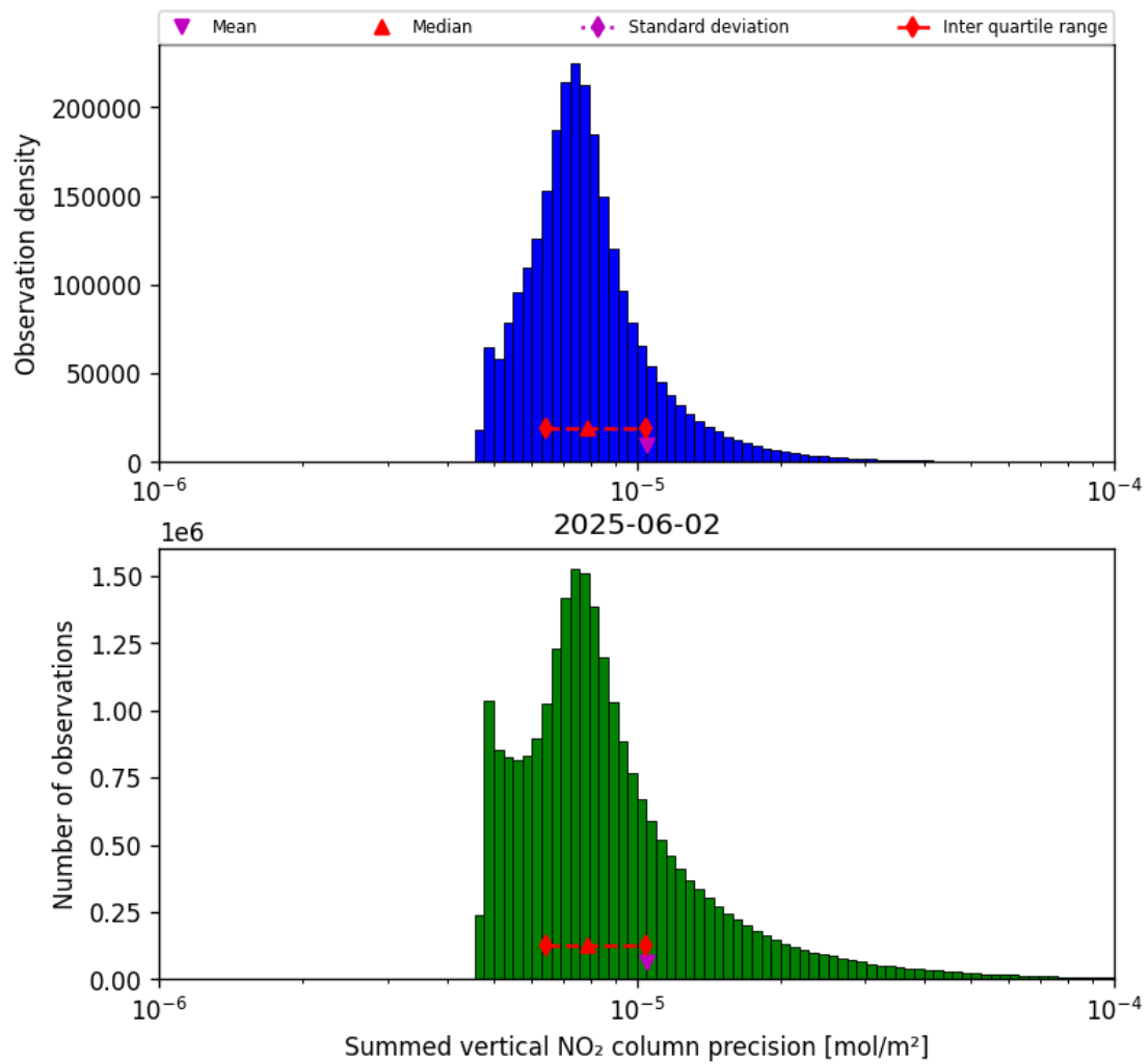
Figure 39: Histogram of "Summed vertical NO 2 column precision" for 2025-06-02 to 2025-06-03
