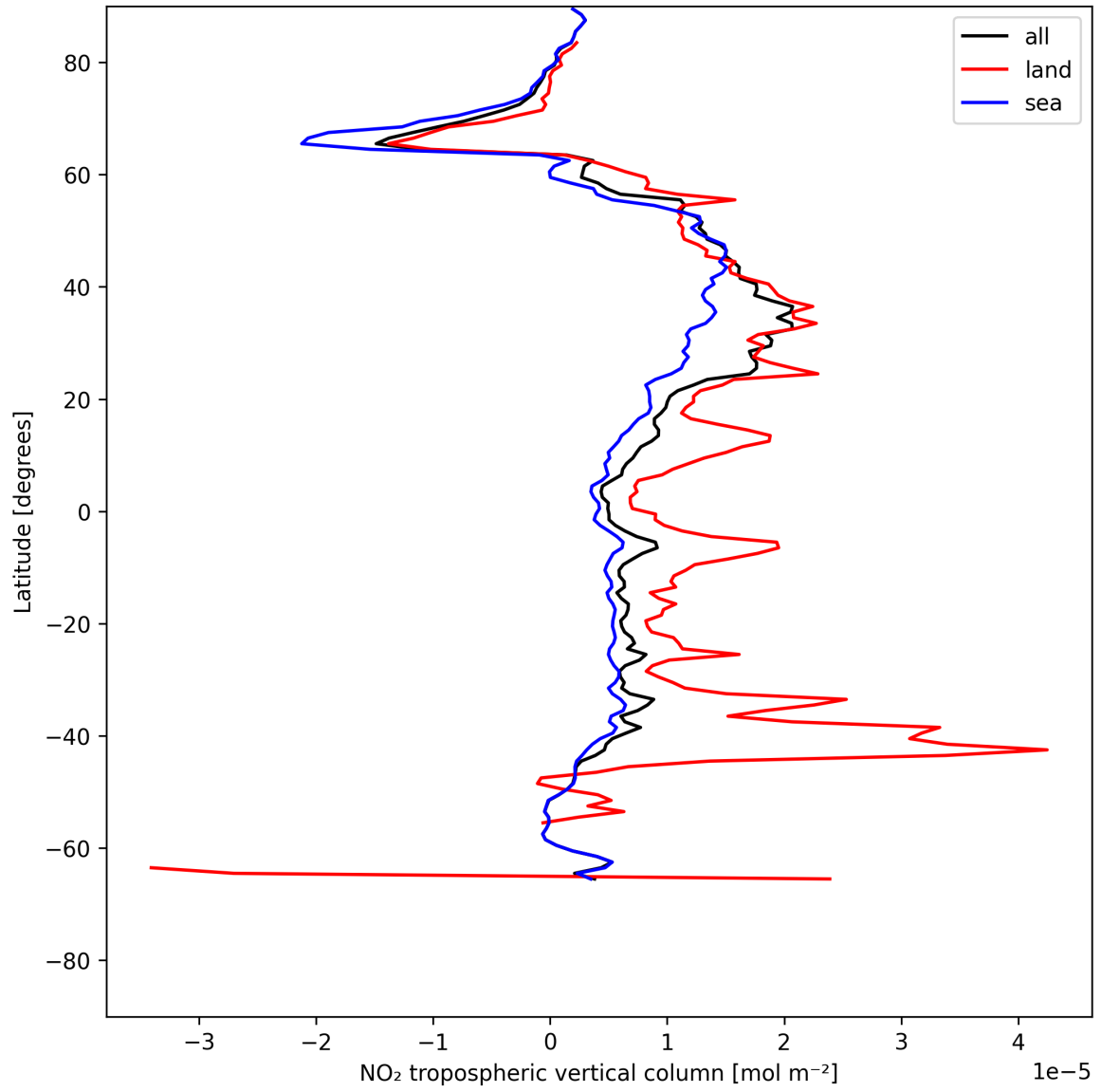
Figure 10: Zonal average of “NO 2 tropospheric vertical column” for 2025-06-02 to 2025-06-03.
