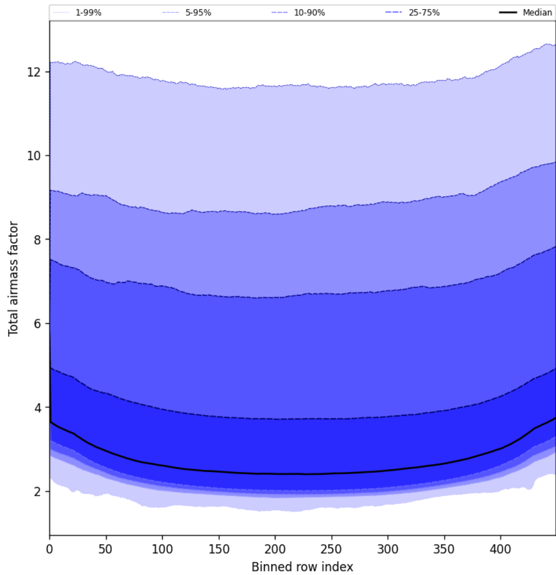
Figure 47: Along track statistics of “Total airmass factor” for 2025-06-02 to 2025-06-03
