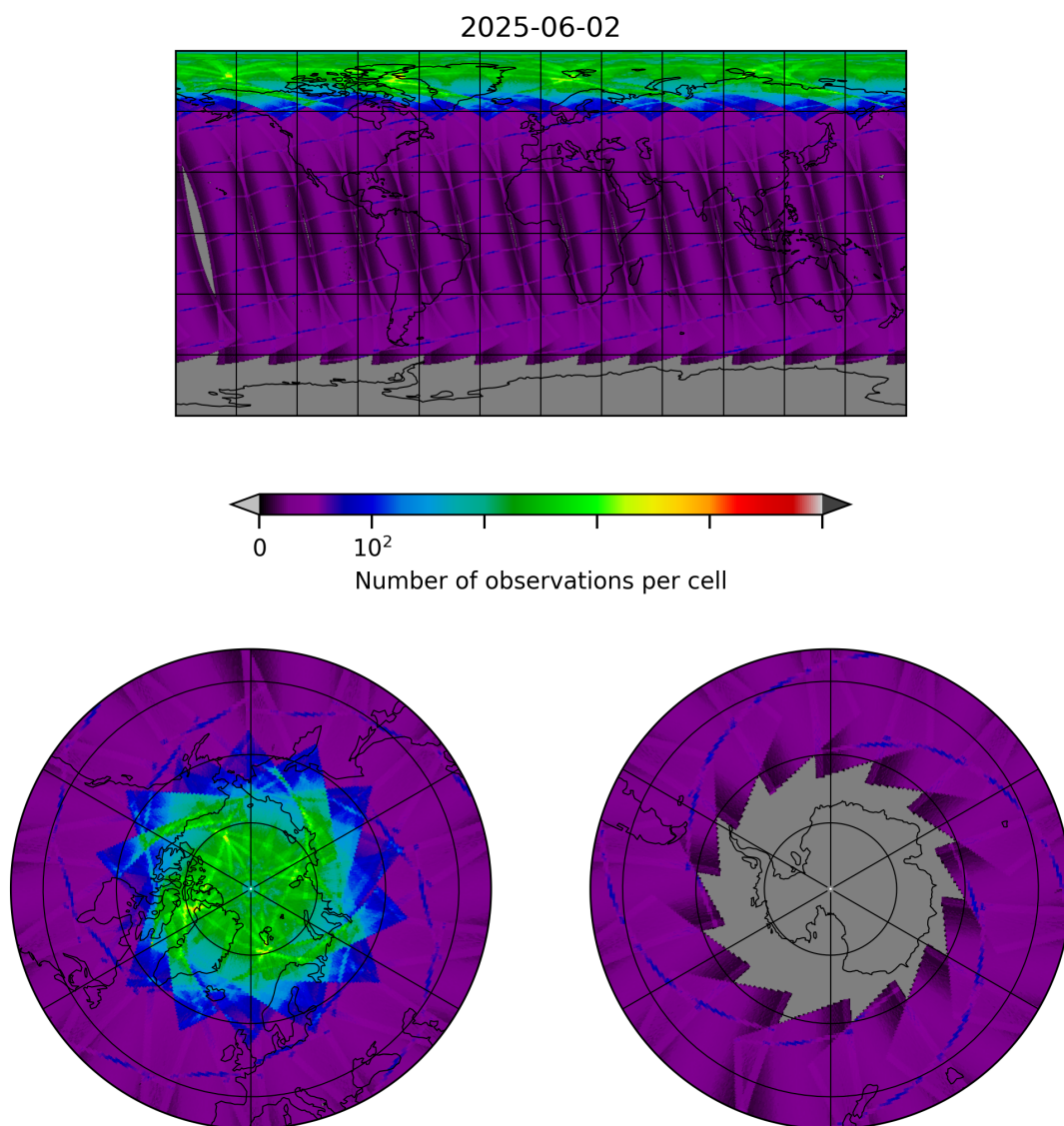
Figure 8: Map of the number of observations for 2025-06-02 to 2025-06-03
