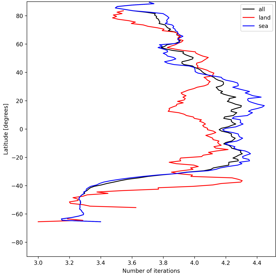
Figure 15: Zonal average of “Number of iterations” for 2025-06-02 to 2025-06-03.
