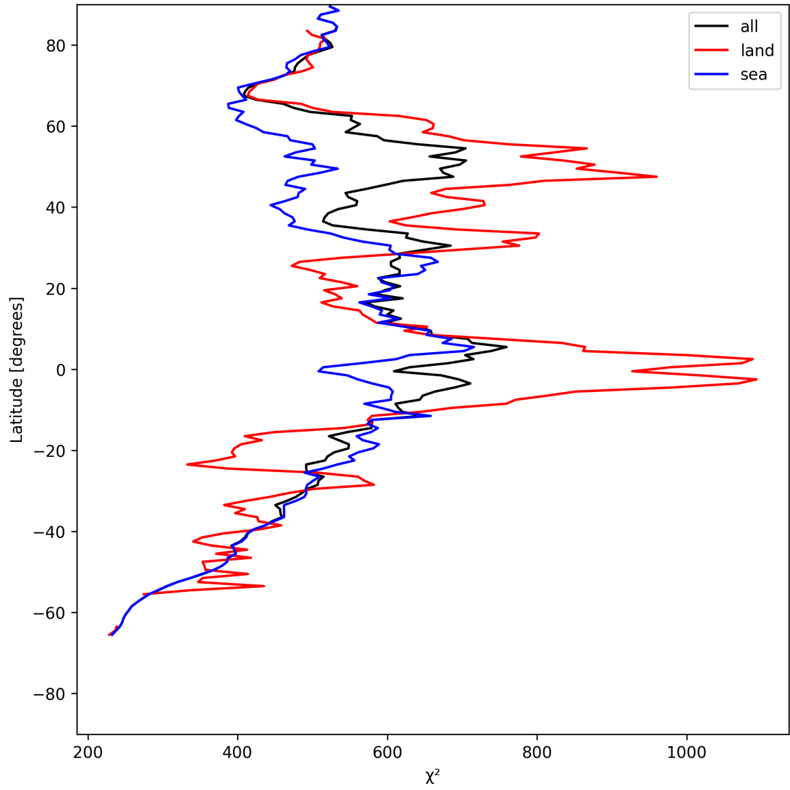
Figure 23: Zonal average of “ \chi^2 ” for 2025-06-02 to 2025-06-03.
