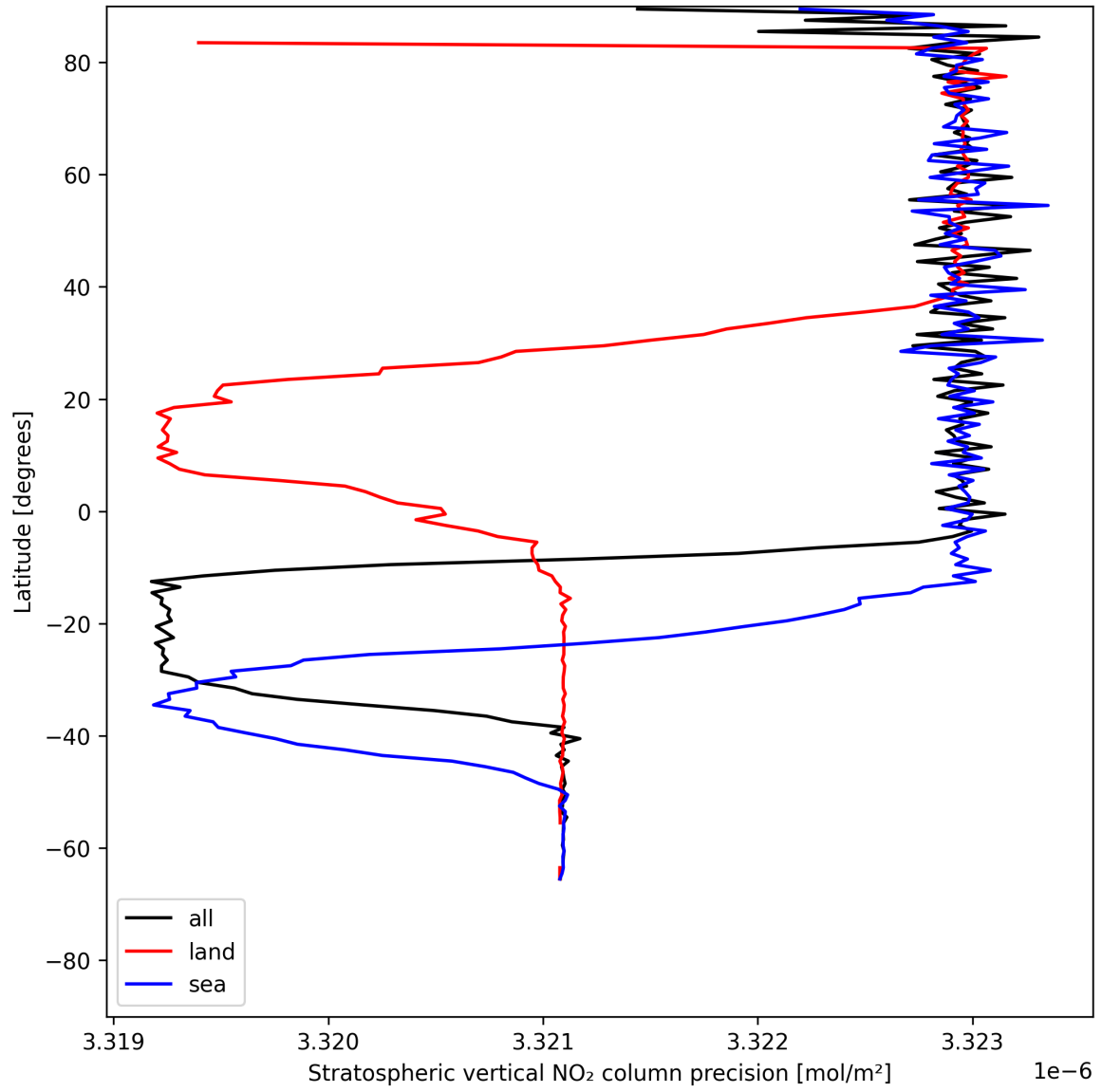
Figure 18: Zonal average of “Stratospheric vertical NO 2 column precision” for 2025-06-02 to 2025-06-03.
