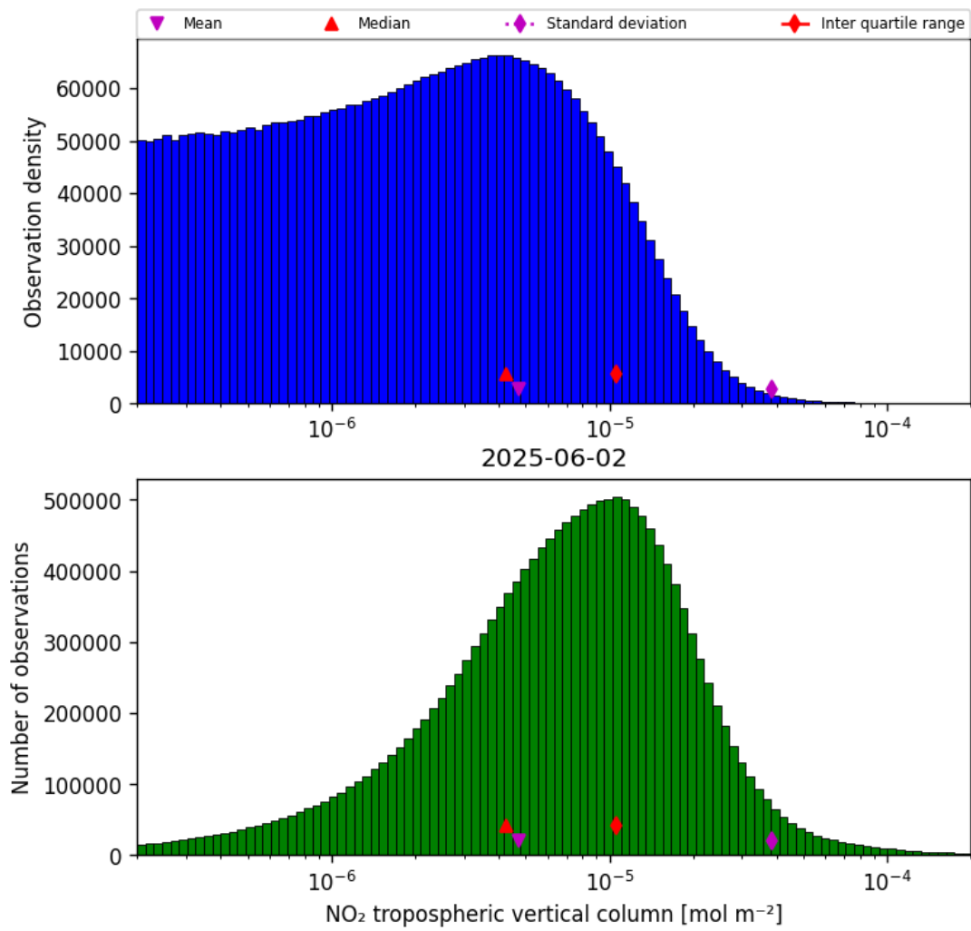
Figure 27: Histogram of “NO 2 tropospheric vertical column” for 2025-06-02 to 2025-06-03
