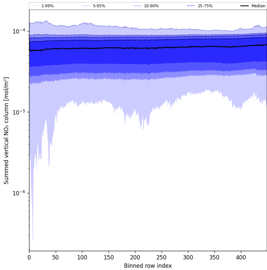
Figure 55: Along track statistics of “Summed vertical NO 2 column” for 2025-06-02 to 2025-06-03
