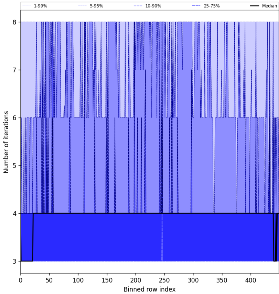
Figure 49: Along track statistics of “Number of iterations” for 2025-06-02 to 2025-06-03
