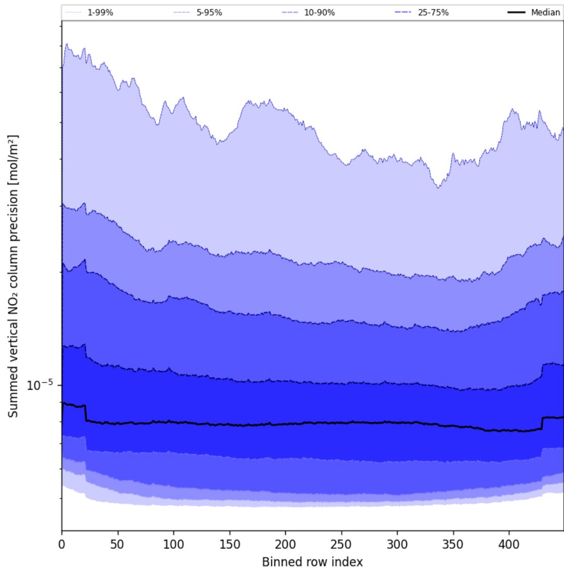
Figure 56: Along track statistics of “Summed vertical NO 2 column precision” for 2025-06-02 to 2025-06-03
