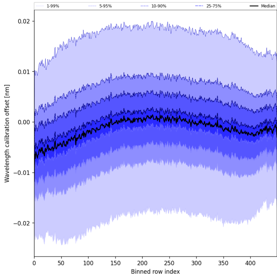
Figure 50: Along track statistics of “Wavelength calibration offset” for 2025-06-02 to 2025-06-03
