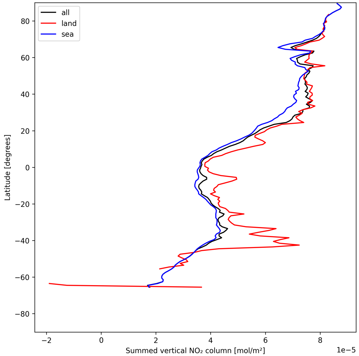
Figure 21: Zonal average of “Summed vertical NO 2 column” for 2025-06-02 to 2025-06-03.
