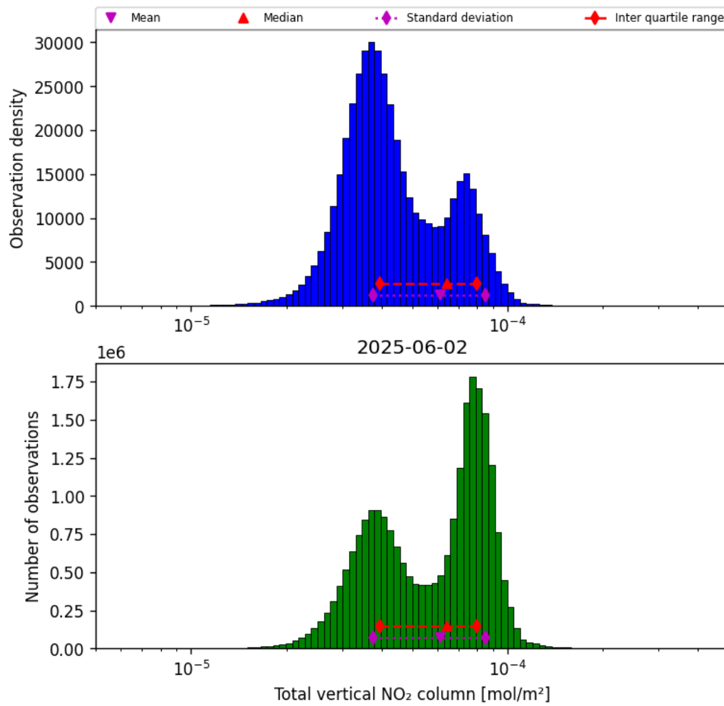
Figure 36: Histogram of “Total vertical NO 2 column” for 2025-06-02 to 2025-06-03
