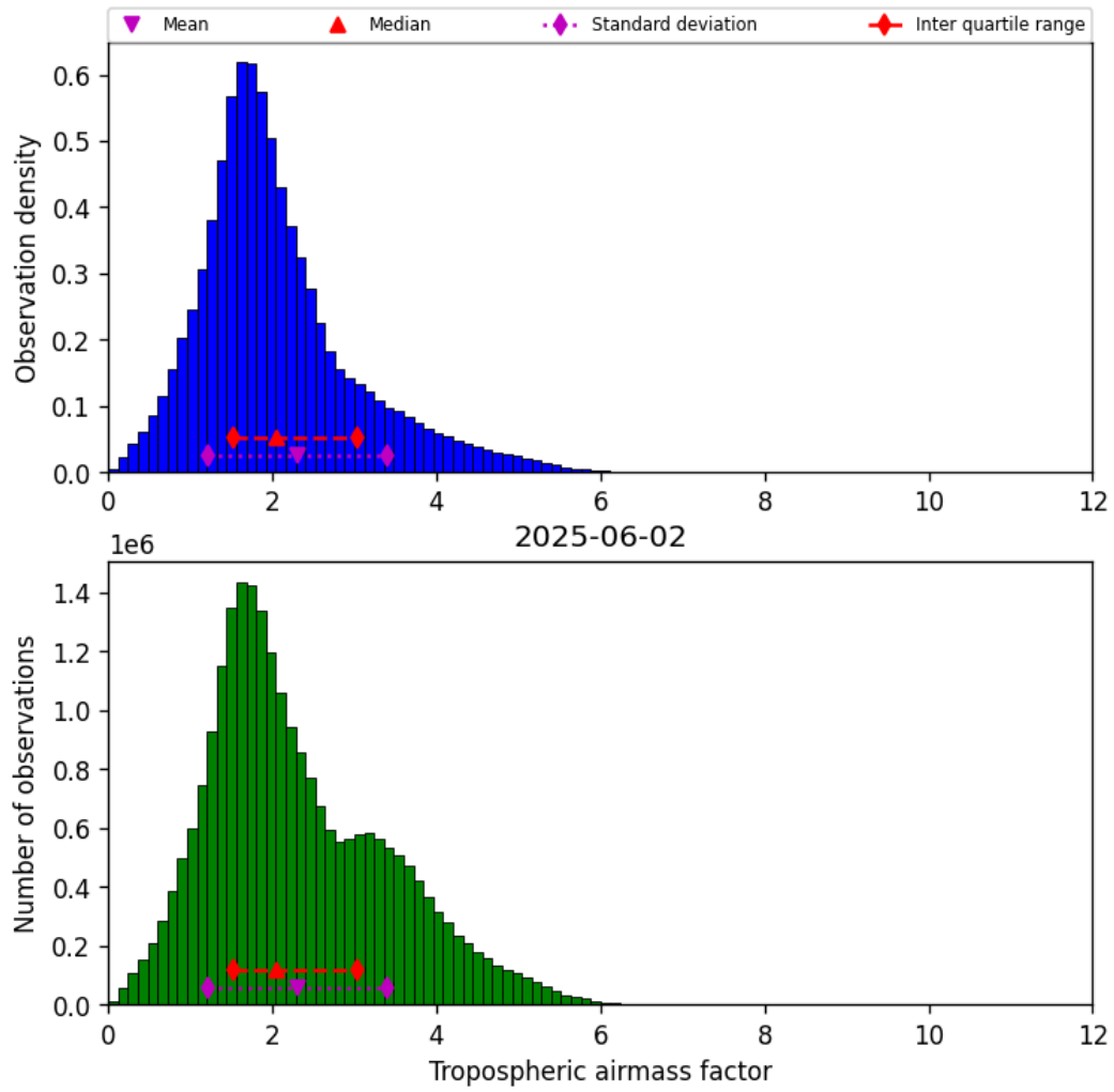
Figure 29: Histogram of “Tropospheric airmass factor” for 2025-06-02 to 2025-06-03
