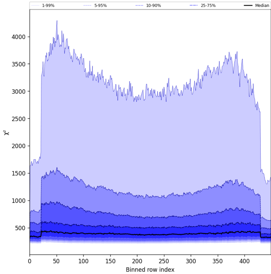
Figure 57: Along track statistics of “ \chi^2 ” for 2025-06-02 to 2025-06-03
