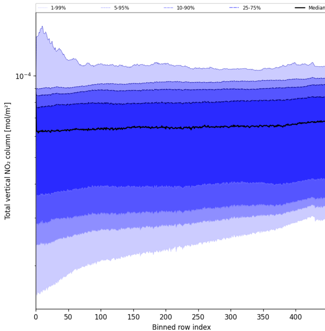
Figure 53: Along track statistics of “Total vertical NO 2 column” for 2025-06-02 to 2025-06-03
