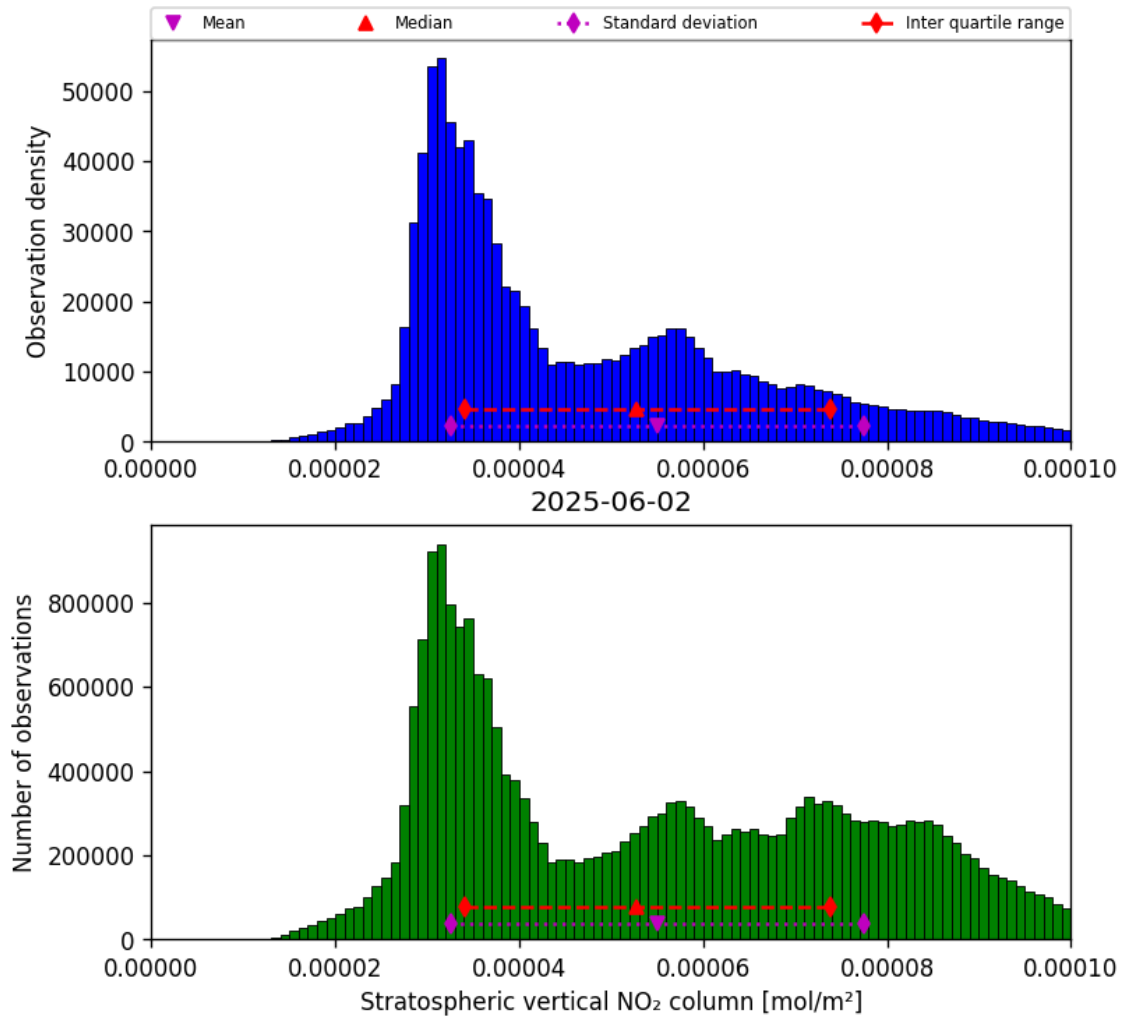
Figure 34: Histogram of “Stratospheric vertical NO 2 column” for 2025-06-02 to 2025-06-03
