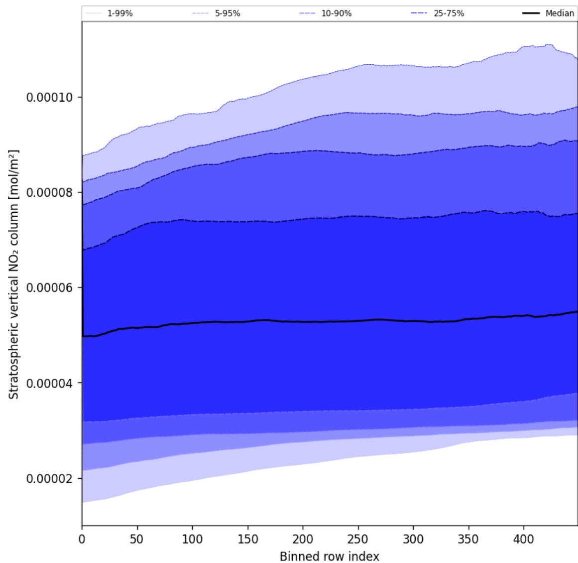
Figure 51: Along track statistics of “Stratospheric vertical NO 2 column” for 2025-06-02 to 2025-06-03
