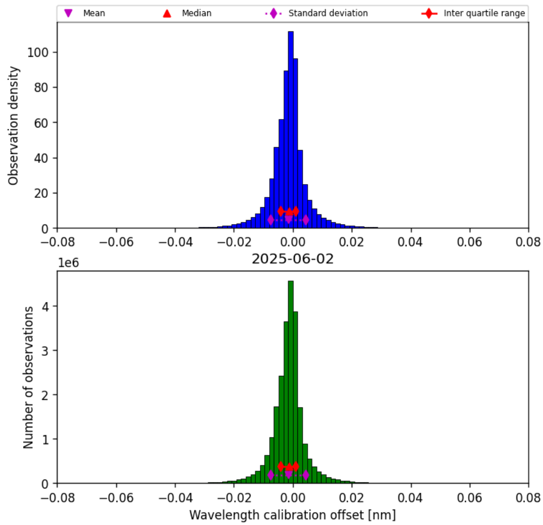
Figure 33: Histogram of “Wavelength calibration offset” for 2025-06-02 to 2025-06-03
