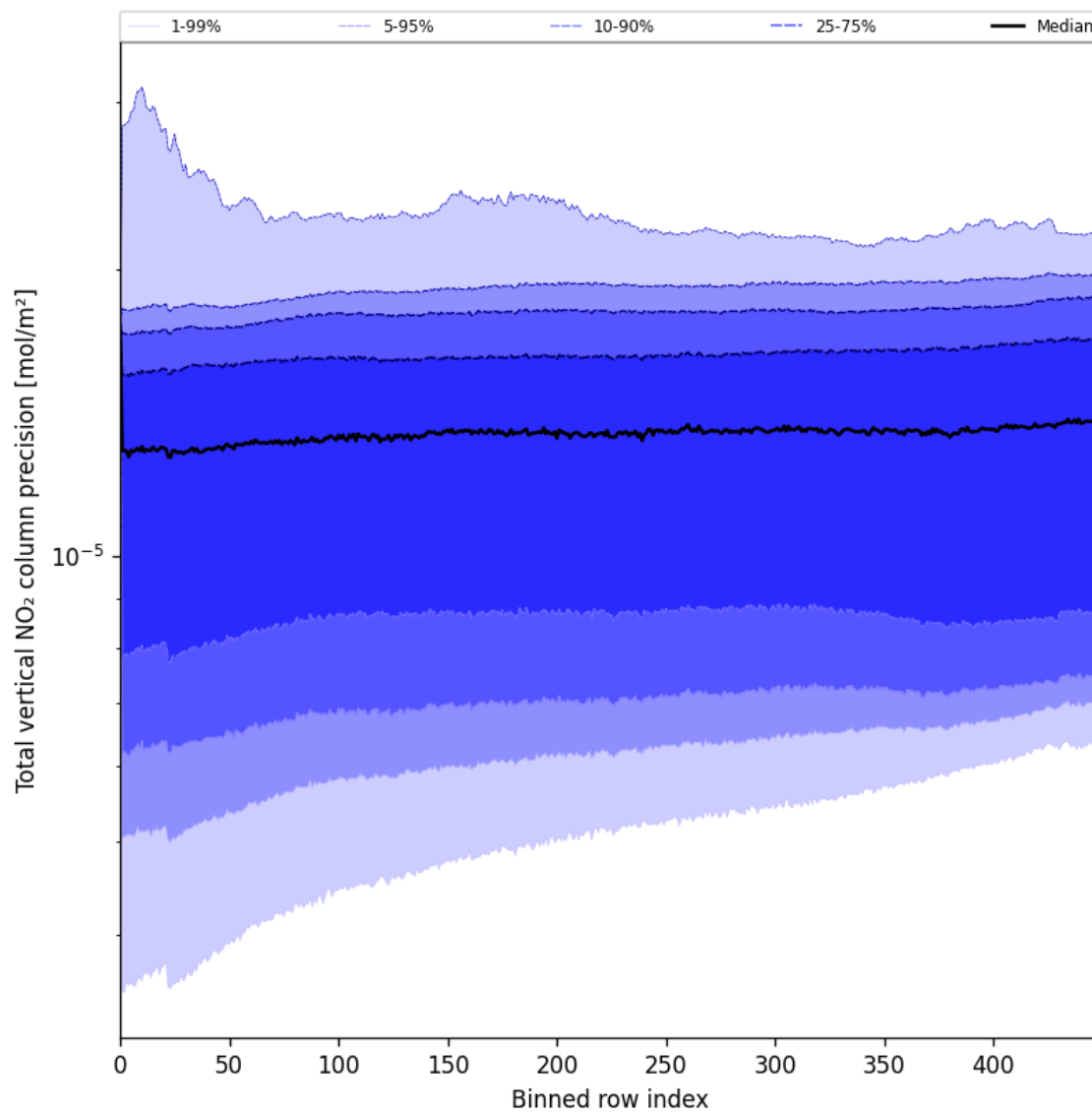
Figure 54: Along track statistics of “Total vertical NO 2 column precision” for 2025-06-02 to 2025-06-03
