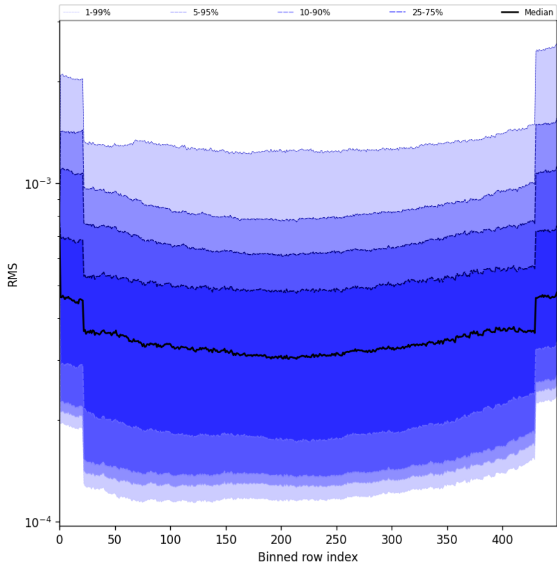
Figure 58: Along track statistics of “RMS” for 2025-06-02 to 2025-06-03
