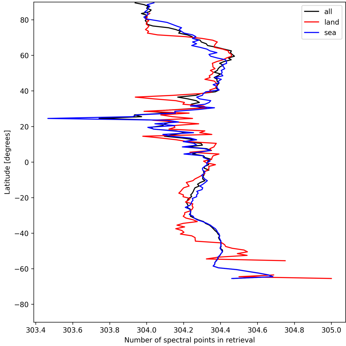
Figure 14: Zonal average of “Number of spectral points in retrieval” for 2025-06-02 to 2025-06-03.
