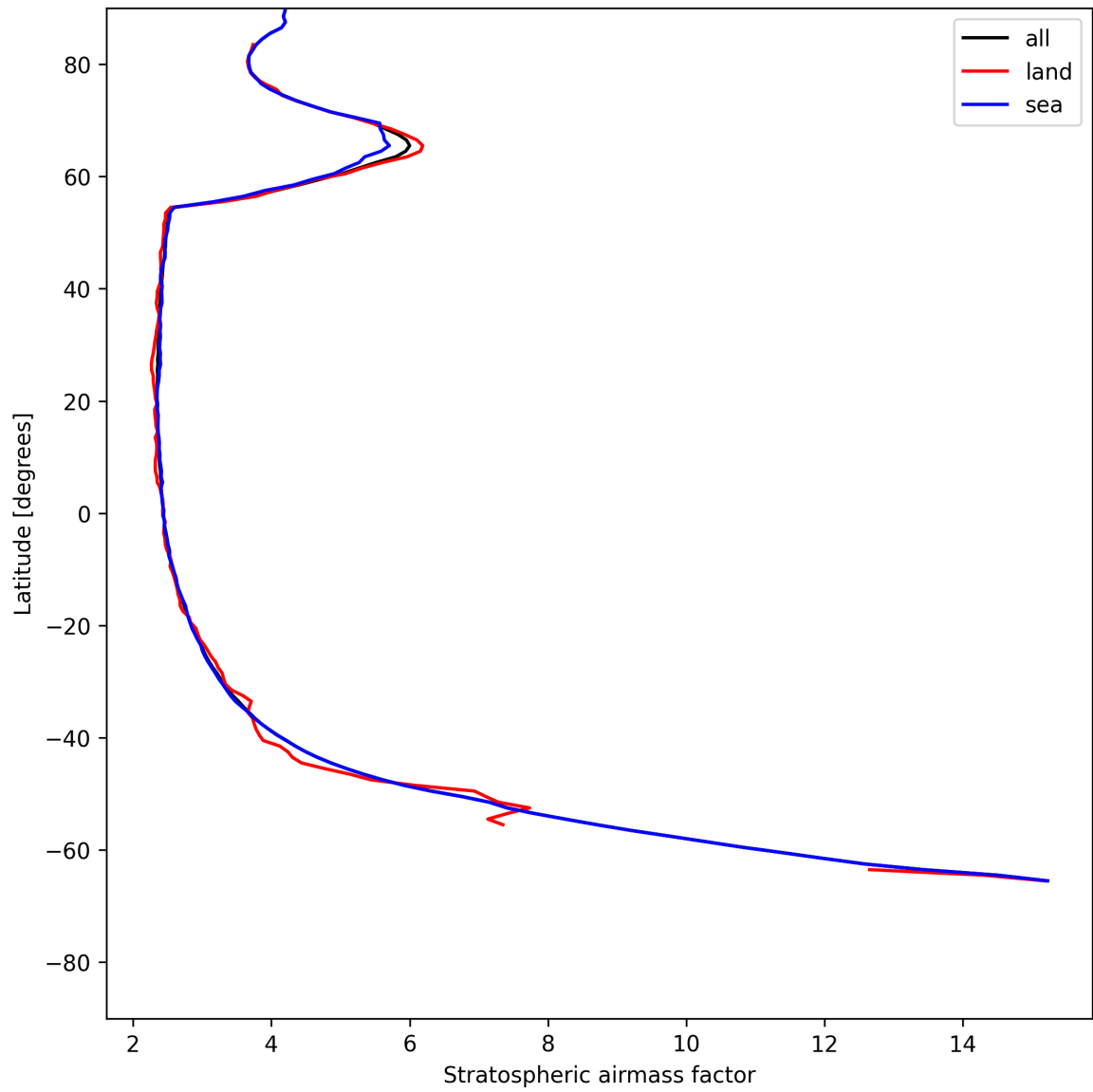
Figure 25: Zonal average of “Stratospheric air mass factor” for 2025-06-02 to 2025-06-03.
