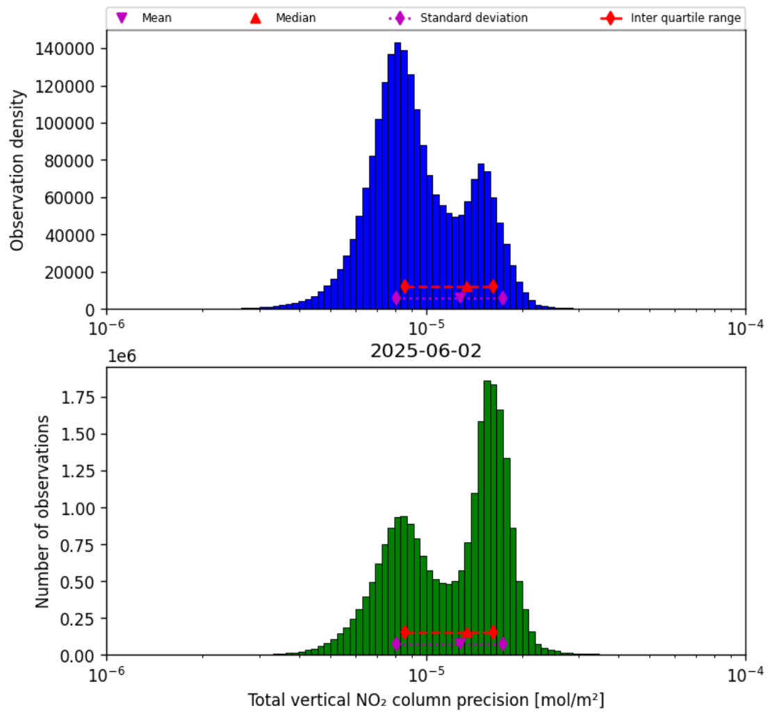
Figure 37: Histogram of “Total vertical NO 2 column precision” for 2025-06-02 to 2025-06-03
