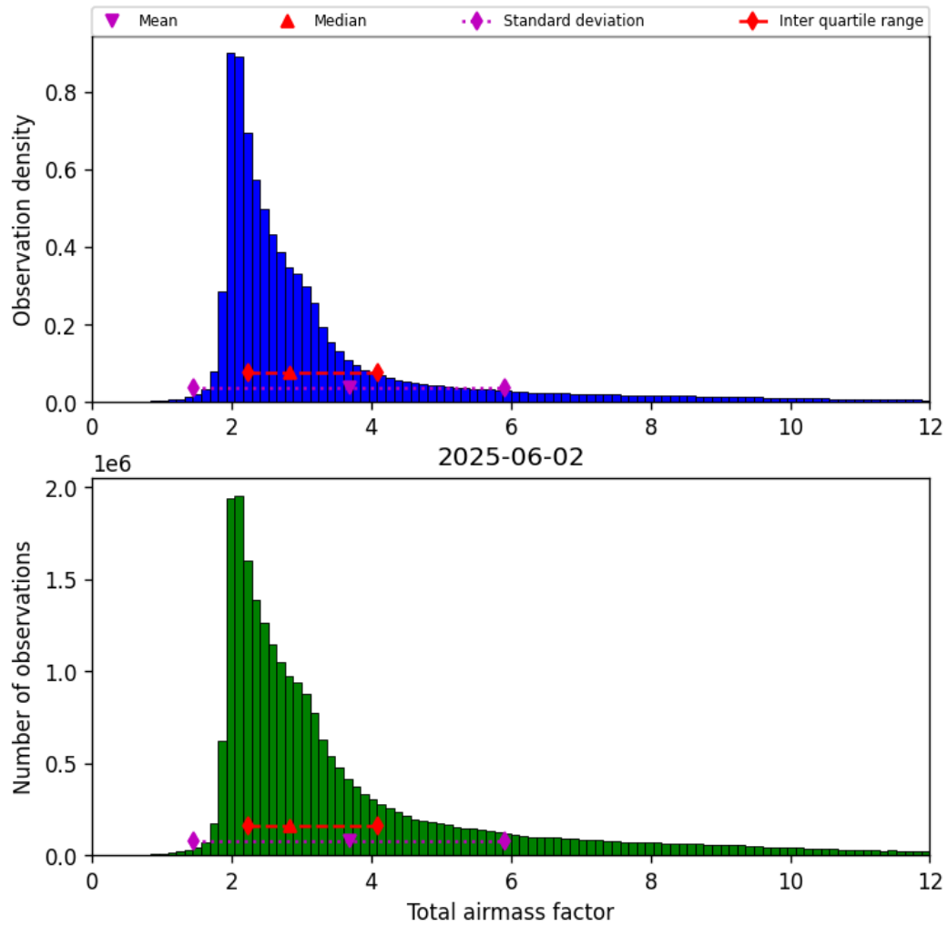
Figure 30: Histogram of “Total airmass factor” for 2025-06-02 to 2025-06-03
