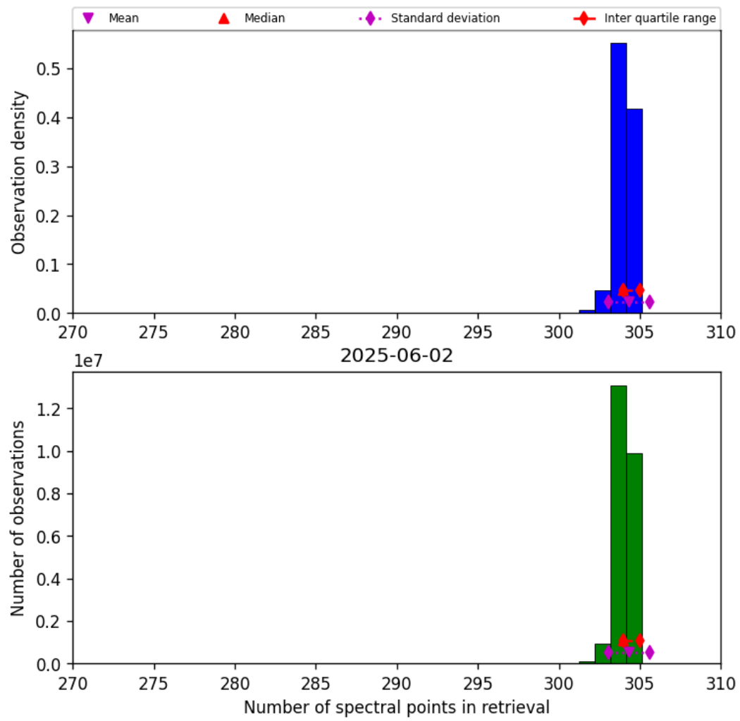
Figure 31: Histogram of “Number of spectral points in retrieval” for 2025-06-02 to 2025-06-03
