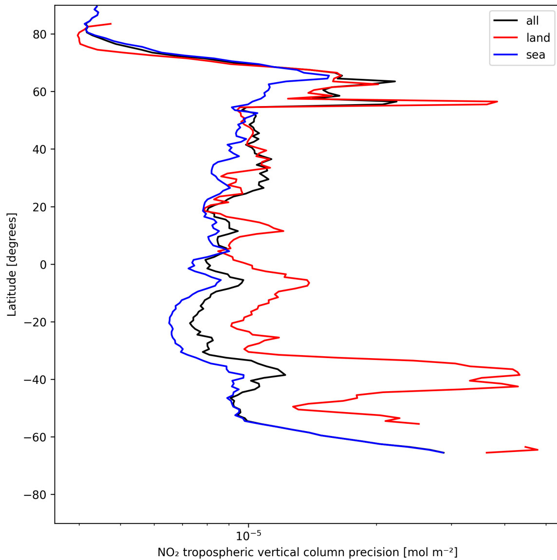
Figure 11: Zonal average of “NO 2 tropospheric vertical column precision” for 2025-06-02 to 2025-06-03.
