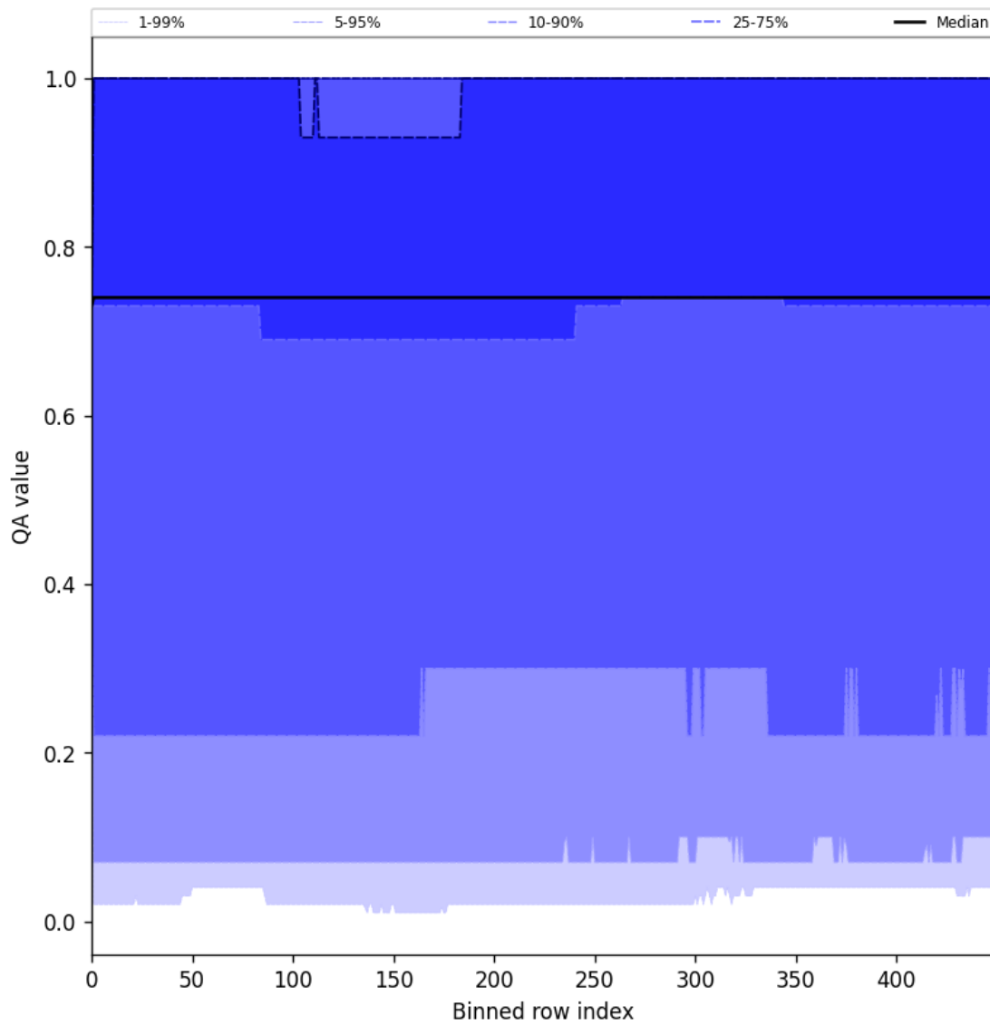
Figure 43: Along track statistics of “QA value” for 2025-06-02 to 2025-06-03
