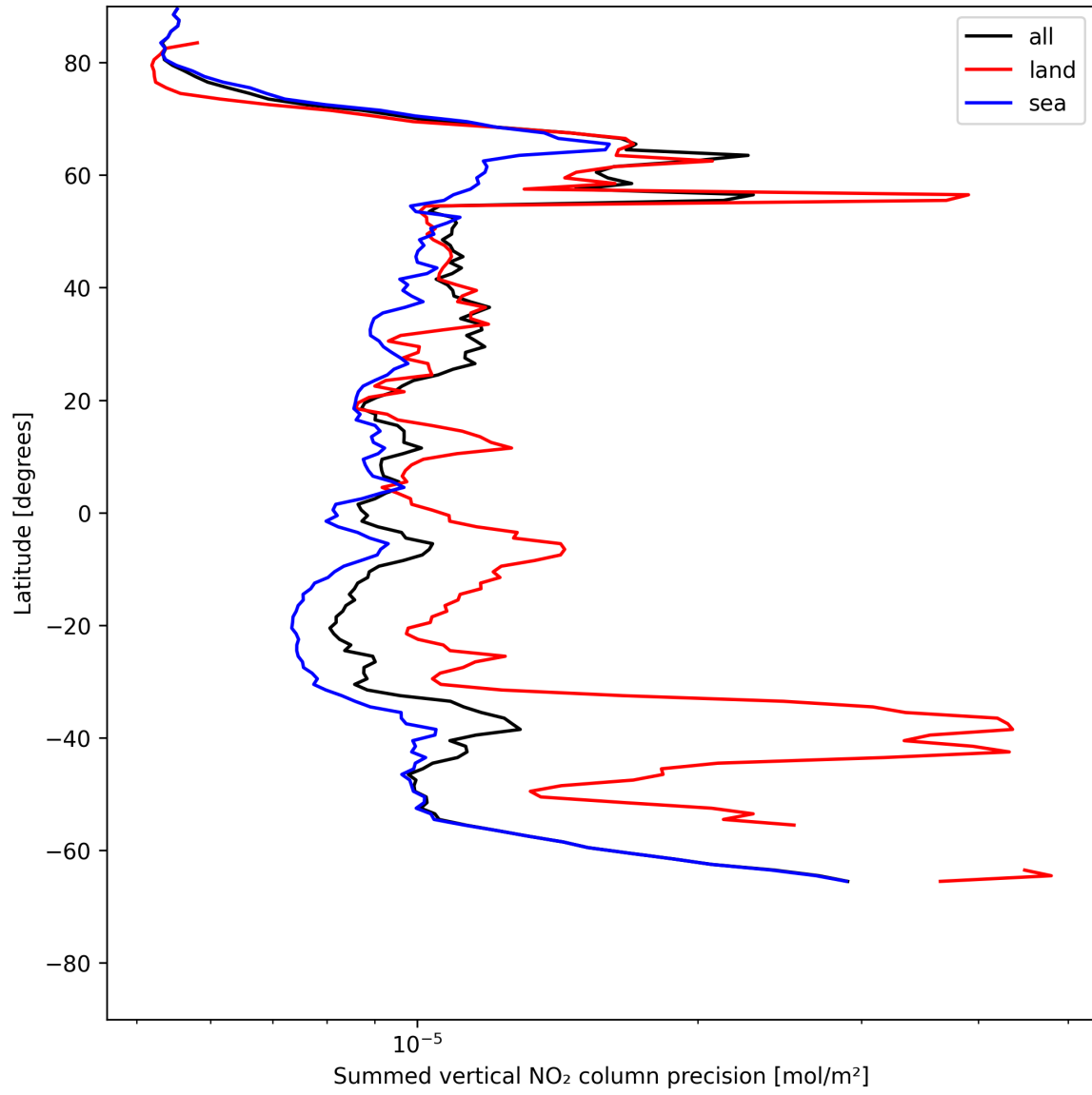
Figure 22: Zonal average of “Summed vertical NO 2 column precision” for 2025-06-02 to 2025-06-03.
