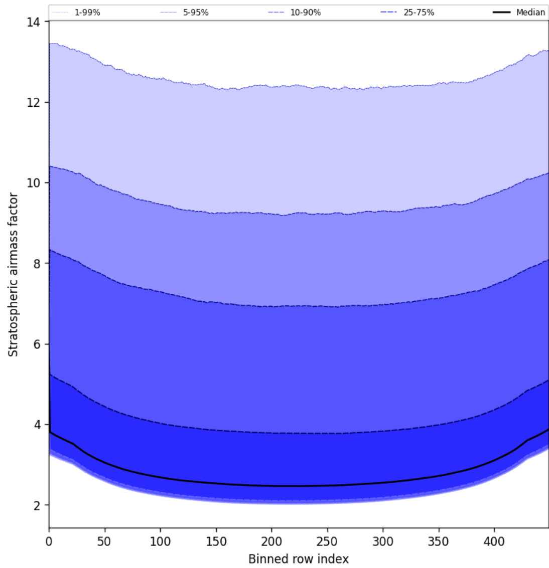
Figure 59: Along track statistics of “Stratospheric airmass factor” for 2025-06-02 to 2025-06-03
