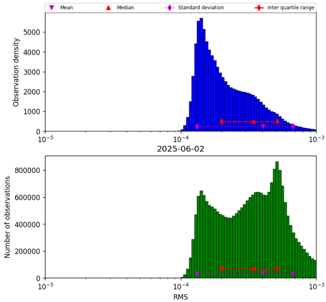
Figure 41: Histogram of “RMS” for 2025-06-02 to 2025-06-03
