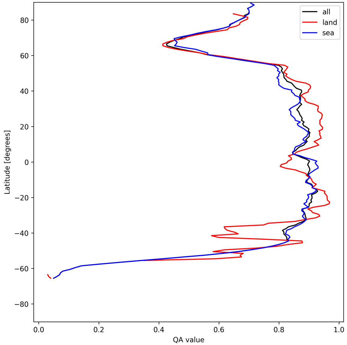
Figure 9: Zonal average of “QA value” for 2025-06-02 to 2025-06-03.
