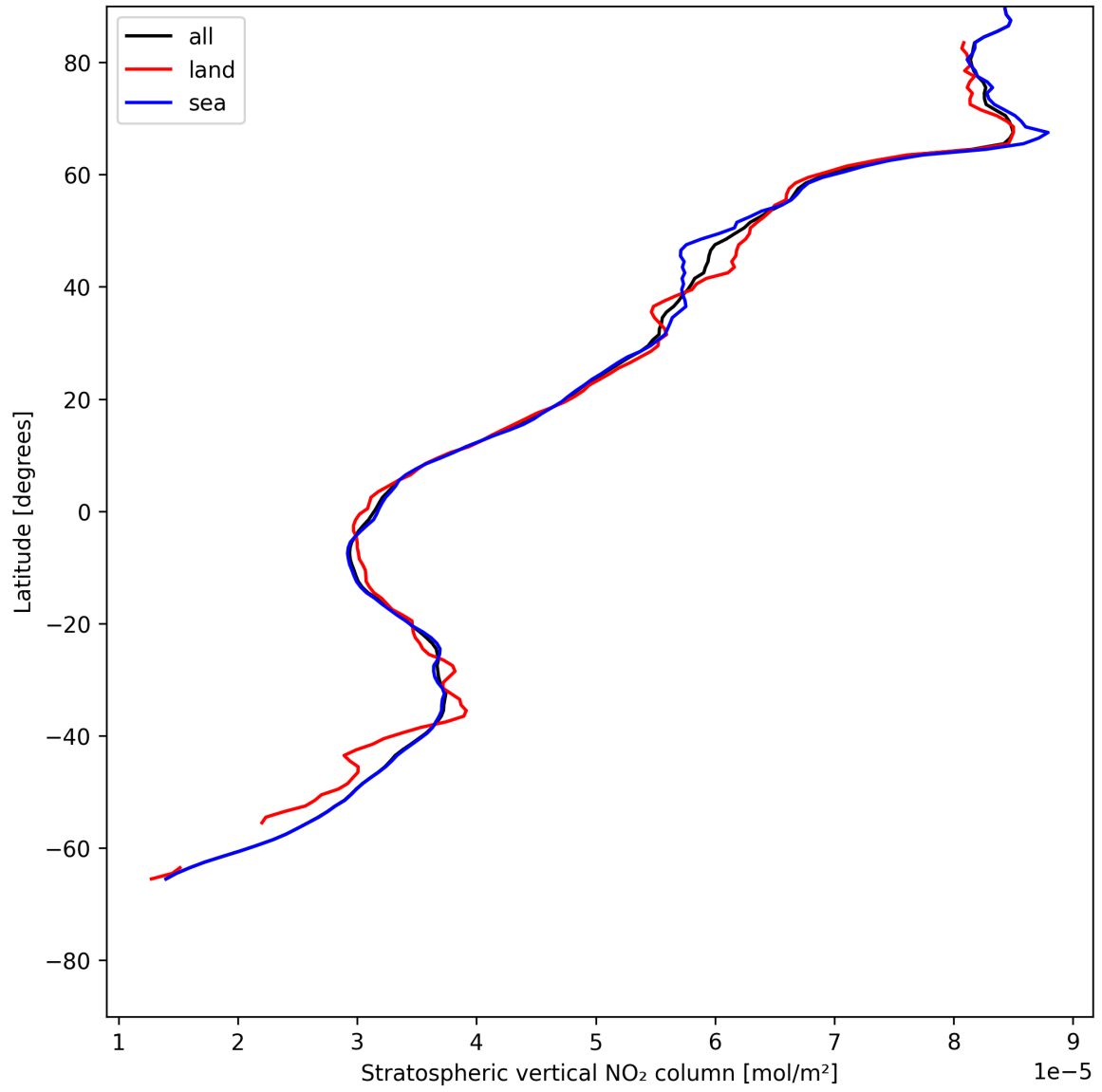
Figure 17: Zonal average of “Stratospheric vertical NO 2 column” for 2025-06-02 to 2025-06-03.
