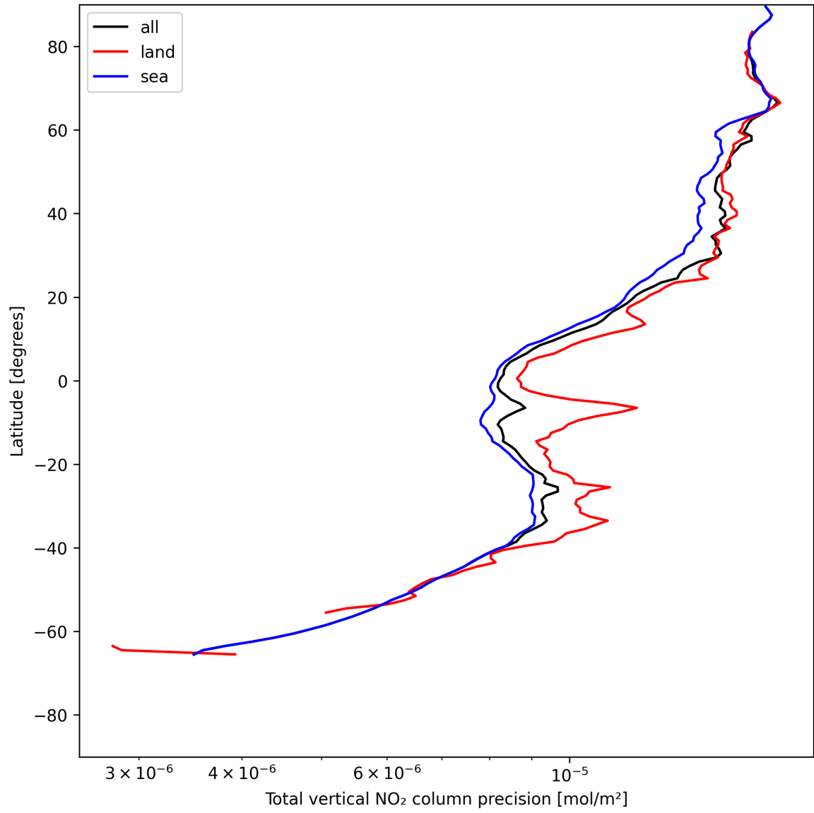
Figure 20: Zonal average of “Total vertical NO 2 column precision” for 2025-06-02 to 2025-06-03.
