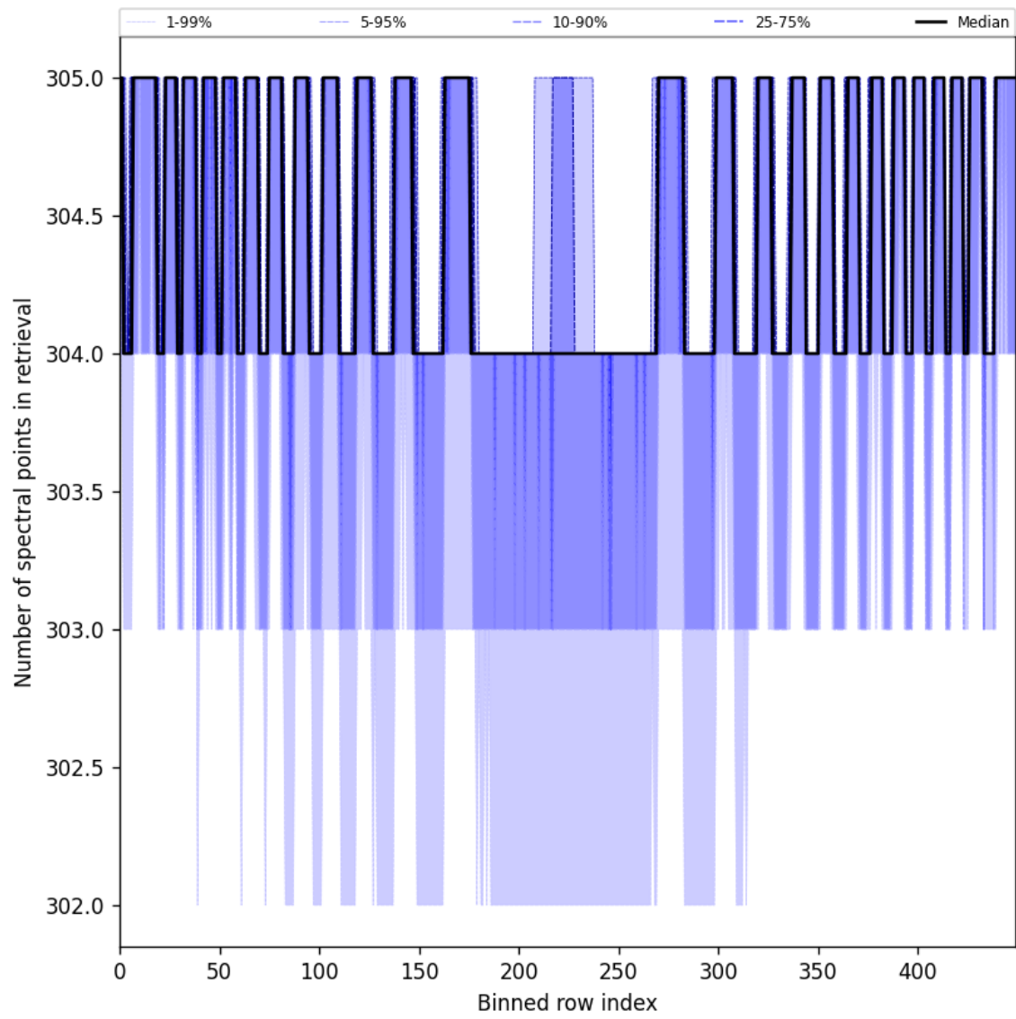
Figure 48: Along track statistics of “Number of spectral points in retrieval” for 2025-06-02 to 2025-06-03
