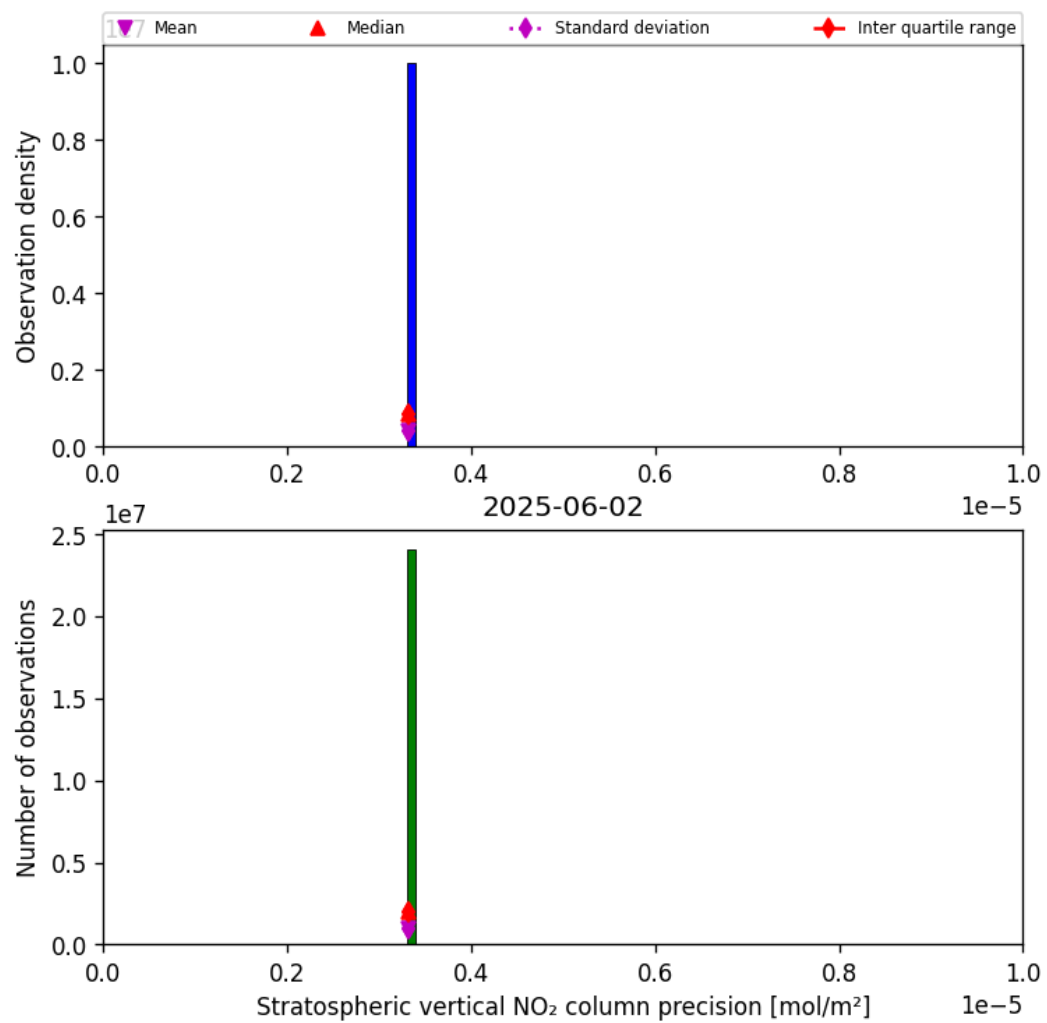
Figure 35: Histogram of “Stratospheric vertical NO 2 column precision” for 2025-06-02 to 2025-06-03
