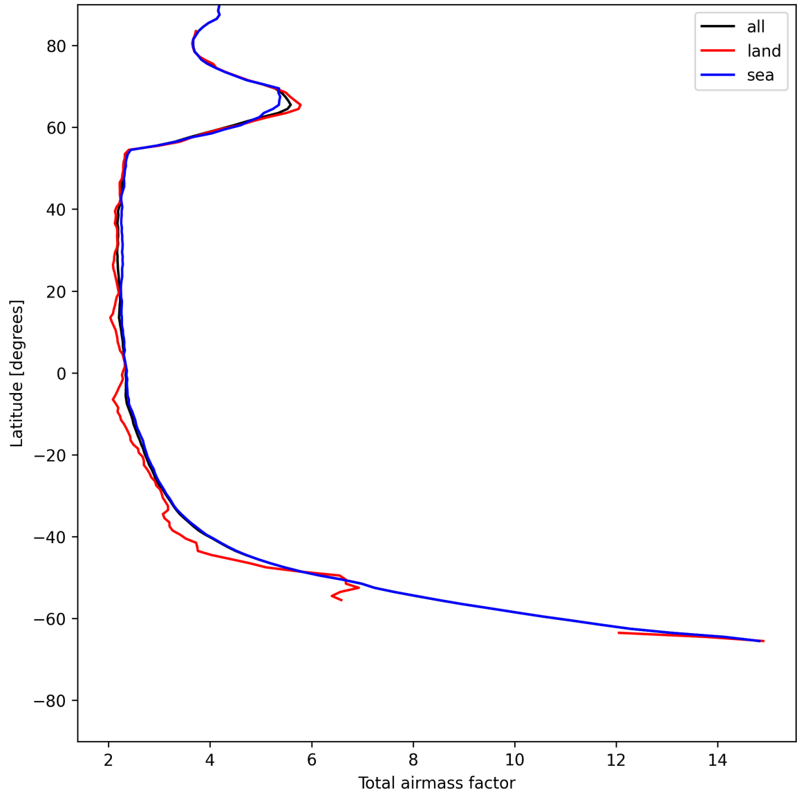
Figure 13: Zonal average of “Total airmass factor” for 2025-06-02 to 2025-06-03.
