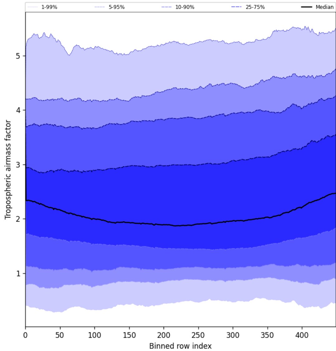
Figure 46: Along track statistics of “Tropospheric airmass factor” for 2025-06-02 to 2025-06-03
