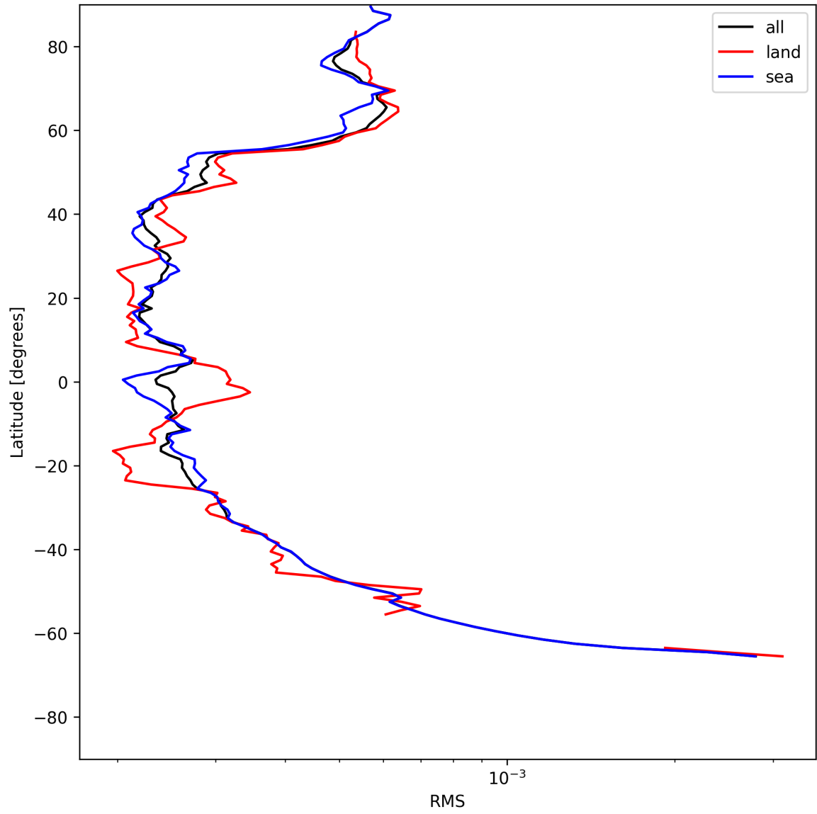
Figure 24: Zonal average of “RMS” for 2025-06-02 to 2025-06-03.
