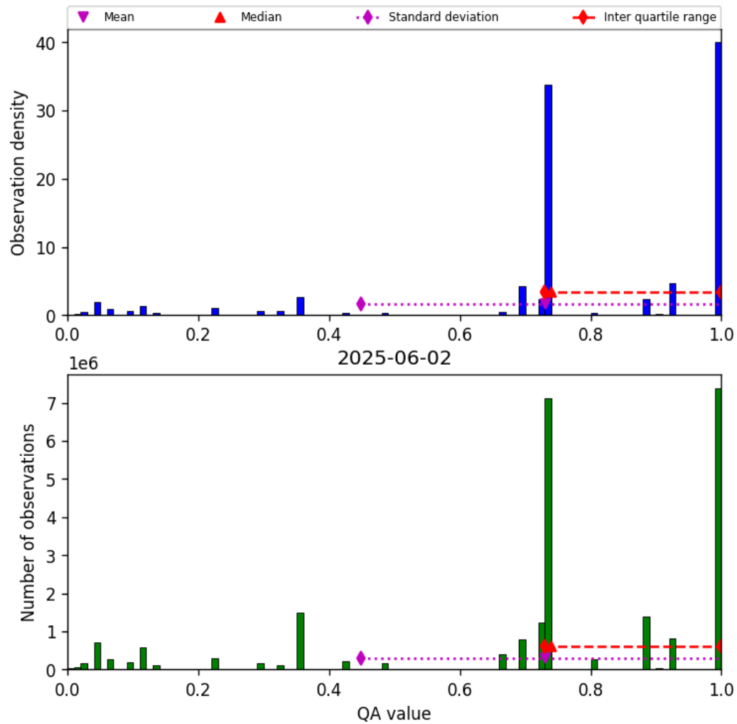
Figure 26: Histogram of “QA value” for 2025-06-02 to 2025-06-03
