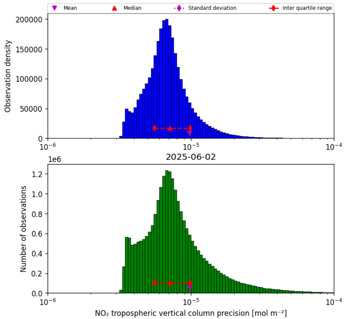
Figure 28: Histogram of “NO 2 tropospheric vertical column precision” for 2025-06-02 to 2025-06-03
