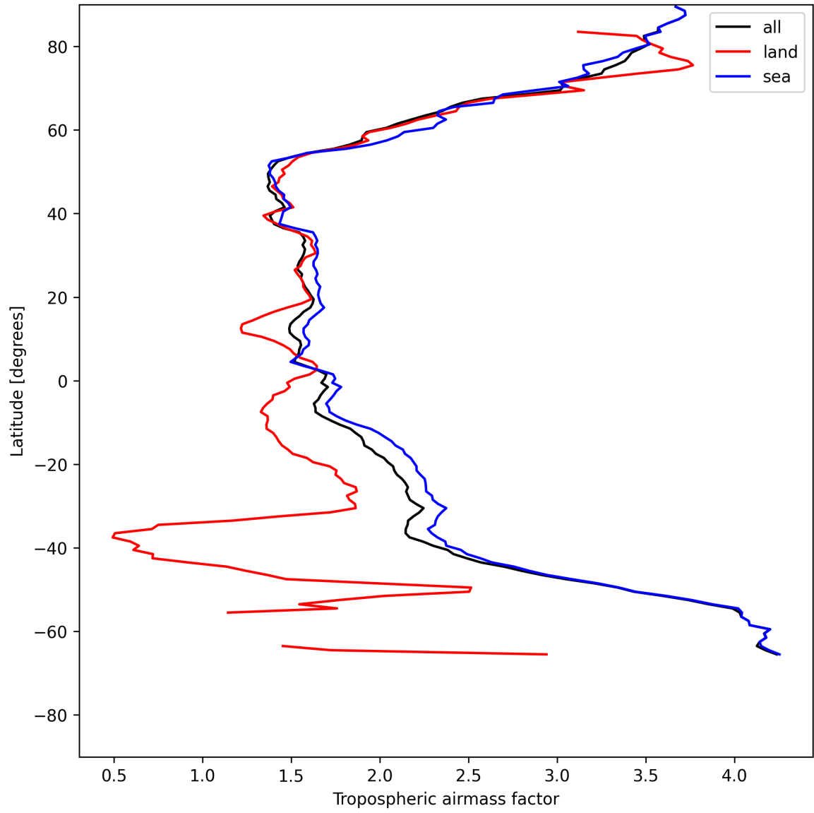
Figure 12: Zonal average of “Tropospheric air mass factor” for 2025-06-02 to 2025-06-03.
