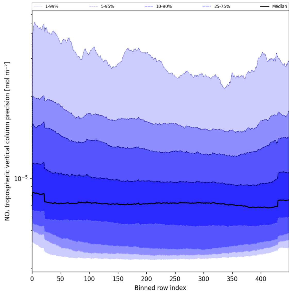
Figure 45: Along track statistics of “NO 2 tropospheric vertical column precision” for 2025-06-02 to 2025-06-03
