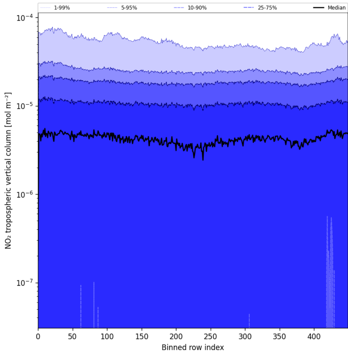
Figure 44: Along track statistics of “NO 2 tropospheric vertical column” for 2025-06-02 to 2025-06-03
