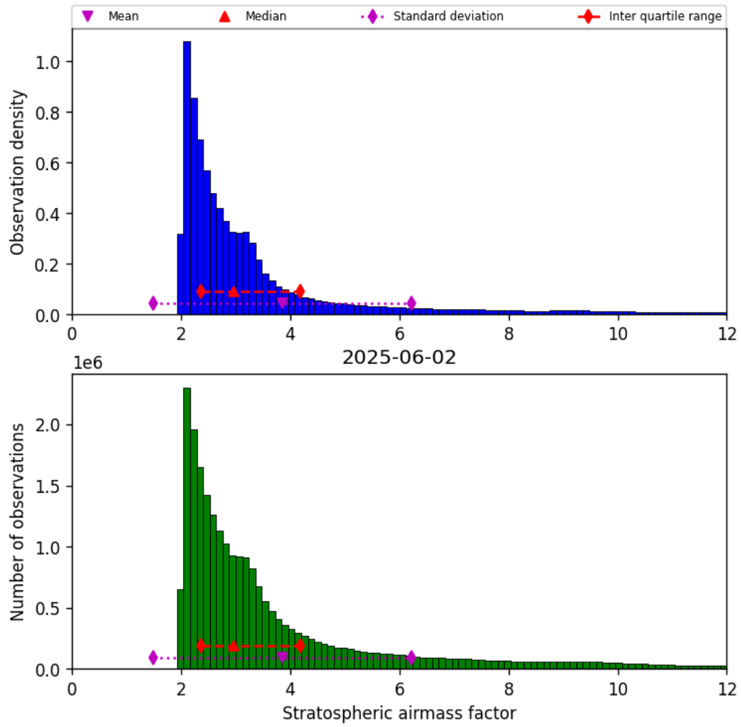
Figure 42: Histogram of “Stratospheric airmass factor” for 2025-06-02 to 2025-06-03
