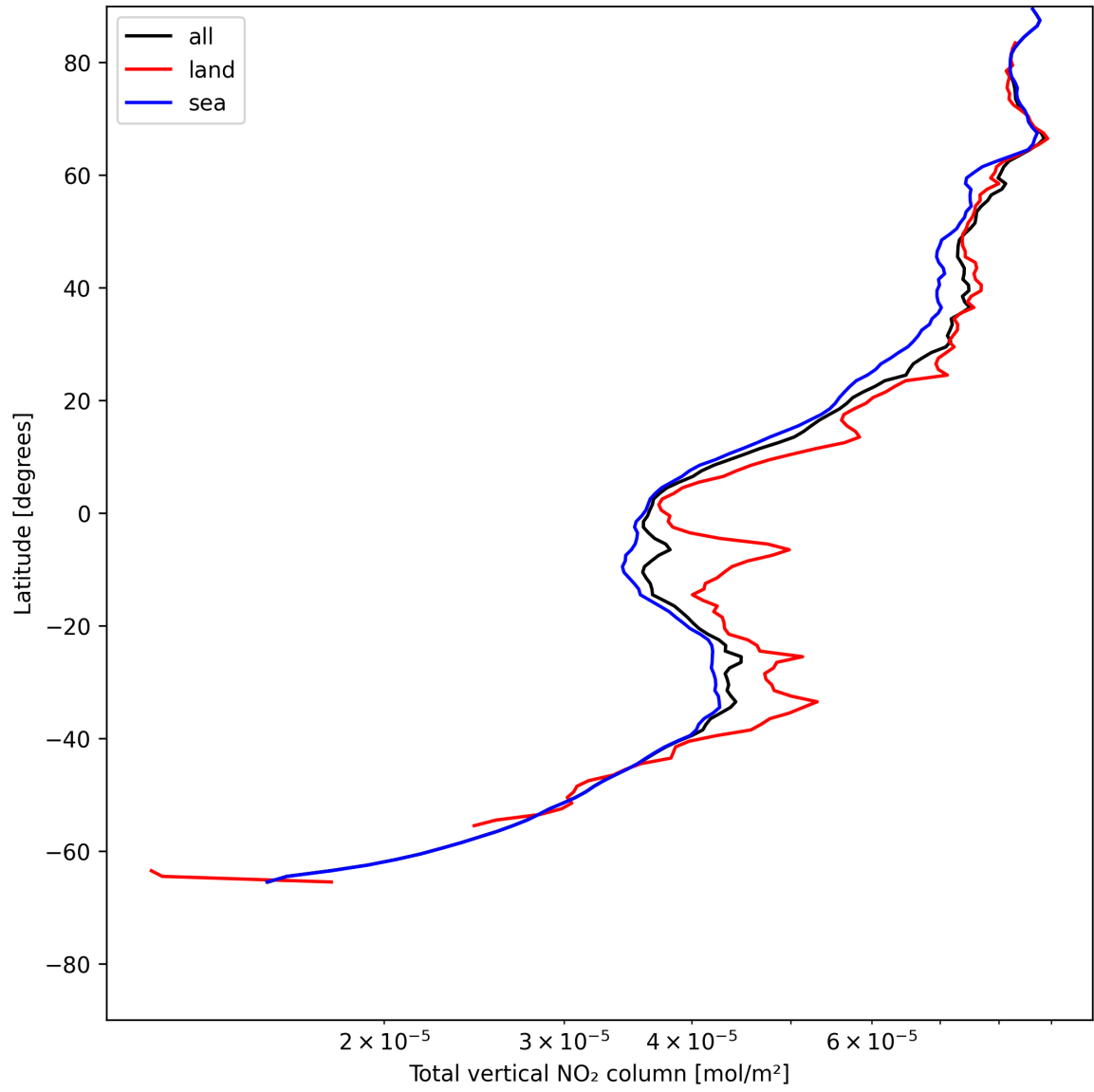
Figure 19: Zonal average of “Total vertical NO 2 column” for 2025-06-02 to 2025-06-03.
