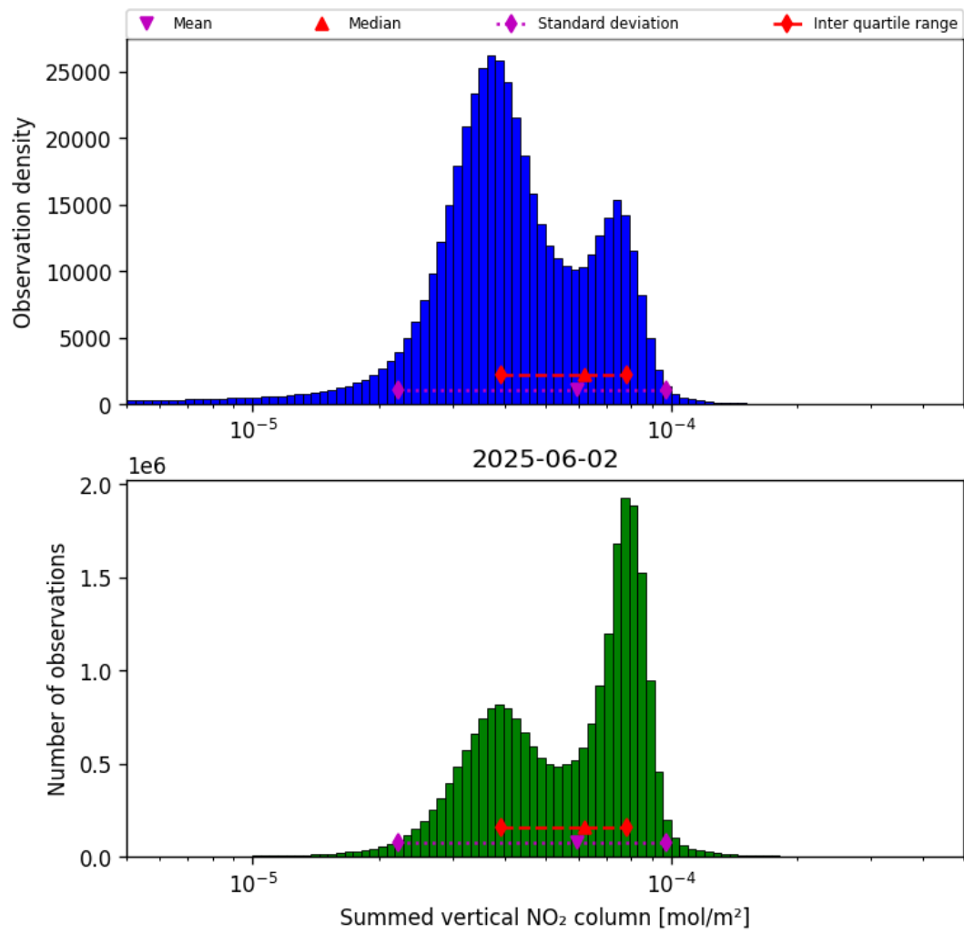
Figure 38: Histogram of "Summed vertical NO 2 column" for 2025-06-02 to 2025-06-03
