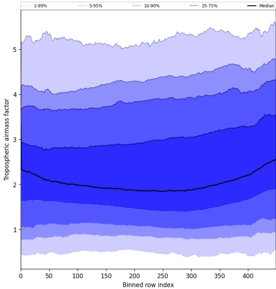
Figure 46: Along track statistics of “Tropospheric airmass factor” for 2025-06-04 to 2025-06-04
