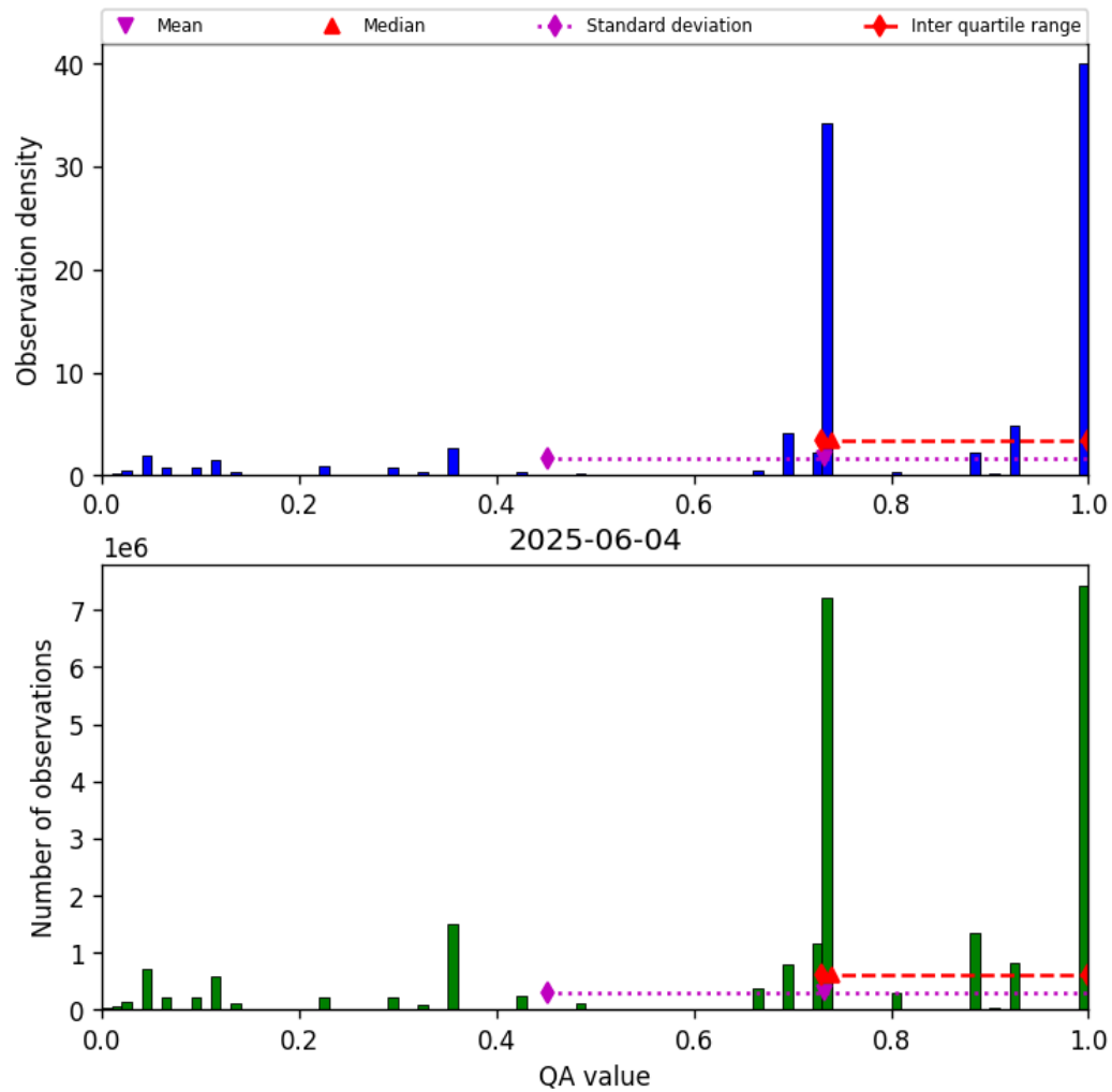
Figure 26: Histogram of “QA value” for 2025-06-04 to 2025-06-04
