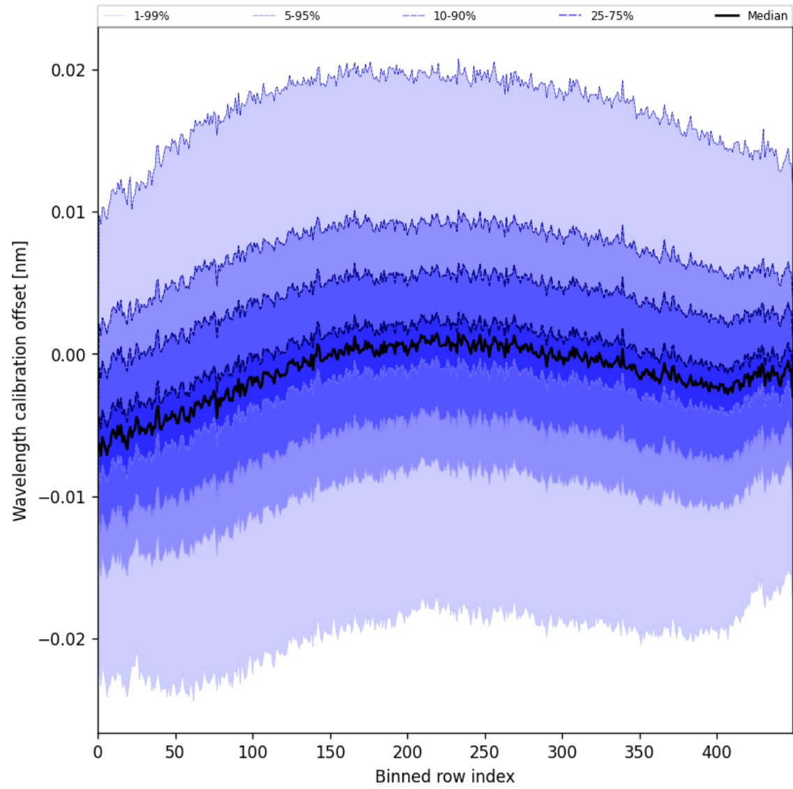
Figure 50: Along track statistics of “Wavelength calibration offset” for 2025-06-04 to 2025-06-04
