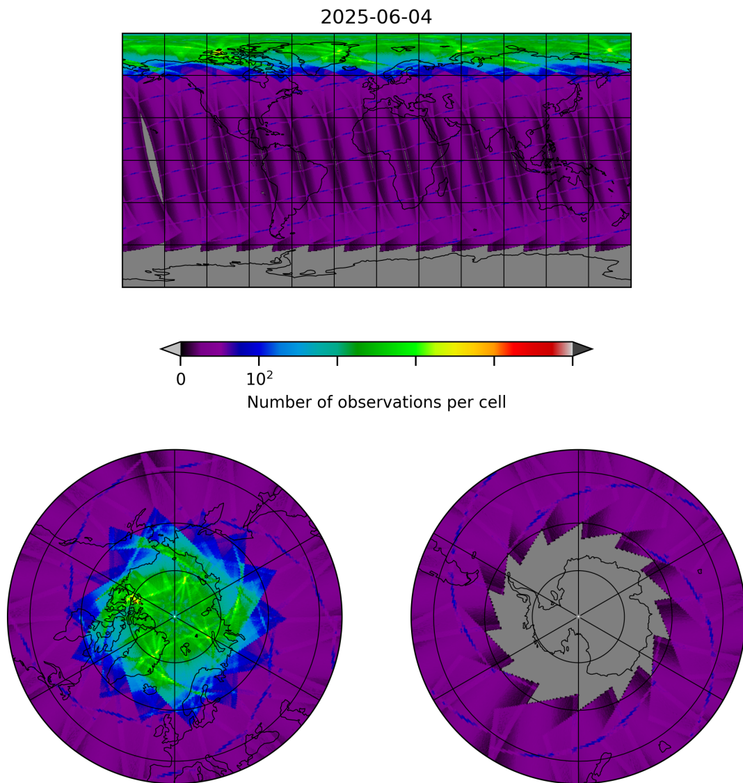
Figure 8: Map of the number of observations for 2025-06-04 to 2025-06-04
