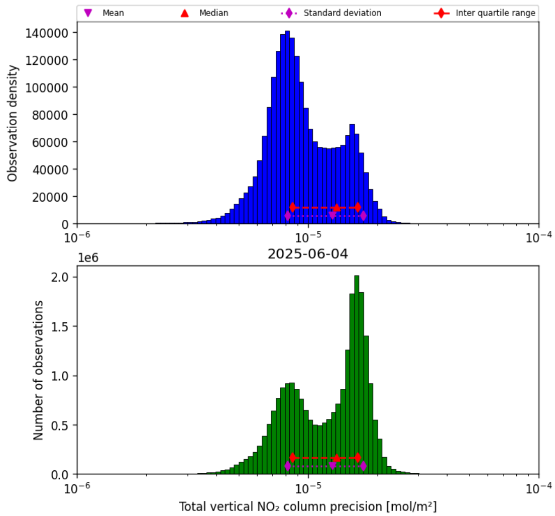
Figure 37: Histogram of “Total vertical NO 2 column precision” for 2025-06-04 to 2025-06-04
