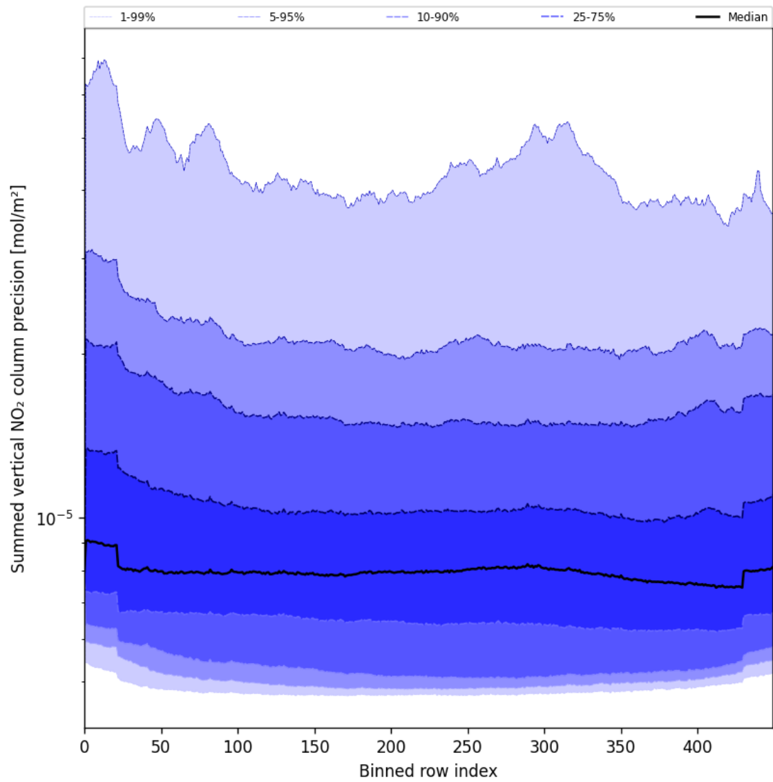
Figure 56: Along track statistics of “Summed vertical NO 2 column precision” for 2025-06-04 to 2025-06-04
