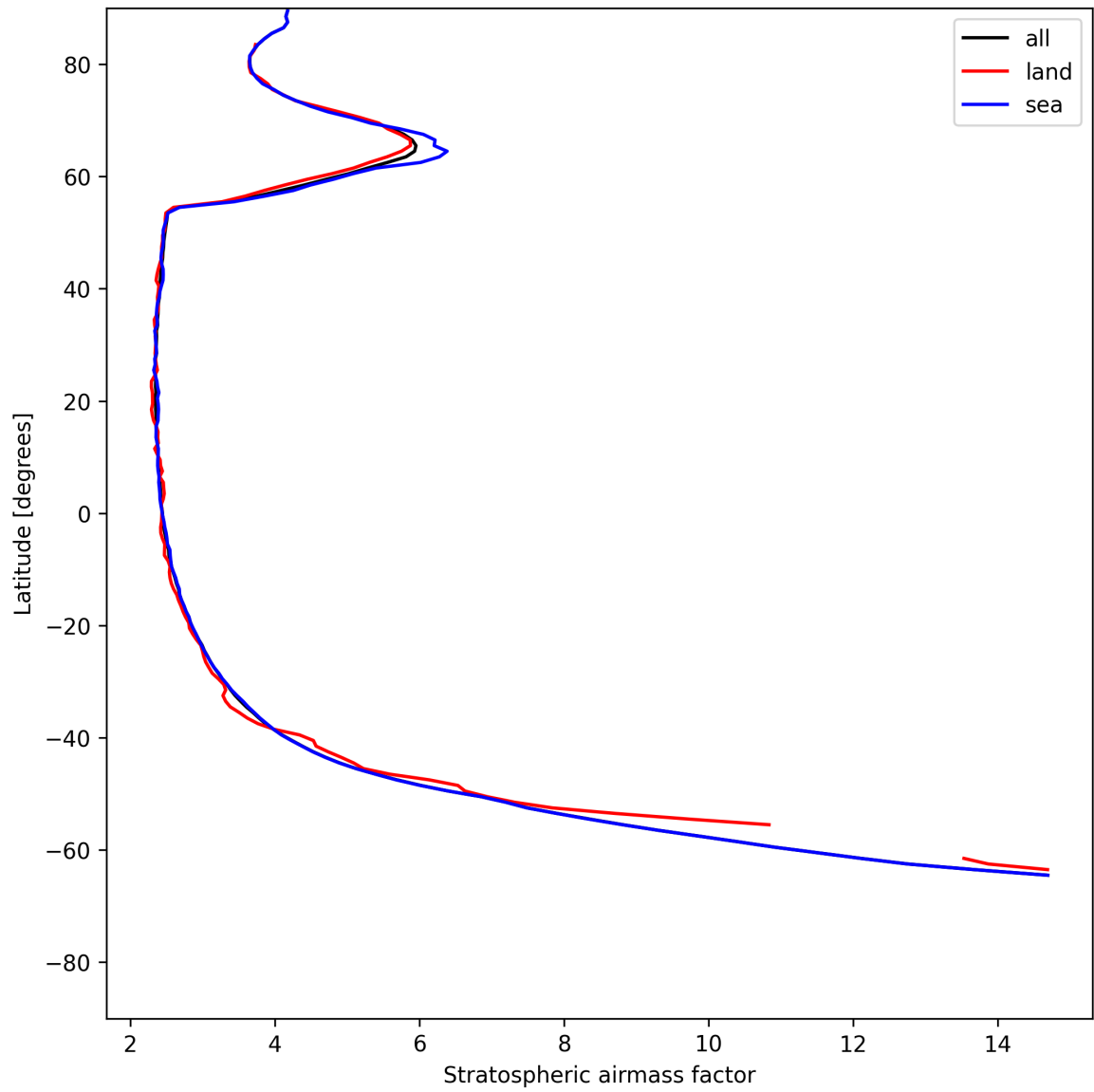
Figure 25: Zonal average of “Stratospheric air mass factor” for 2025-06-04 to 2025-06-04.
