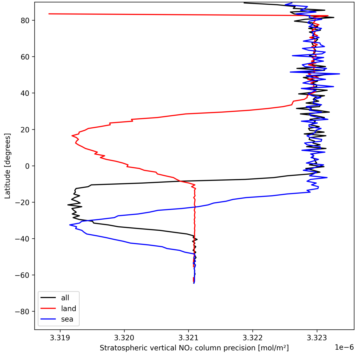
Figure 18: Zonal average of “Stratospheric vertical NO 2 column precision” for 2025-06-04 to 2025-06-04.
