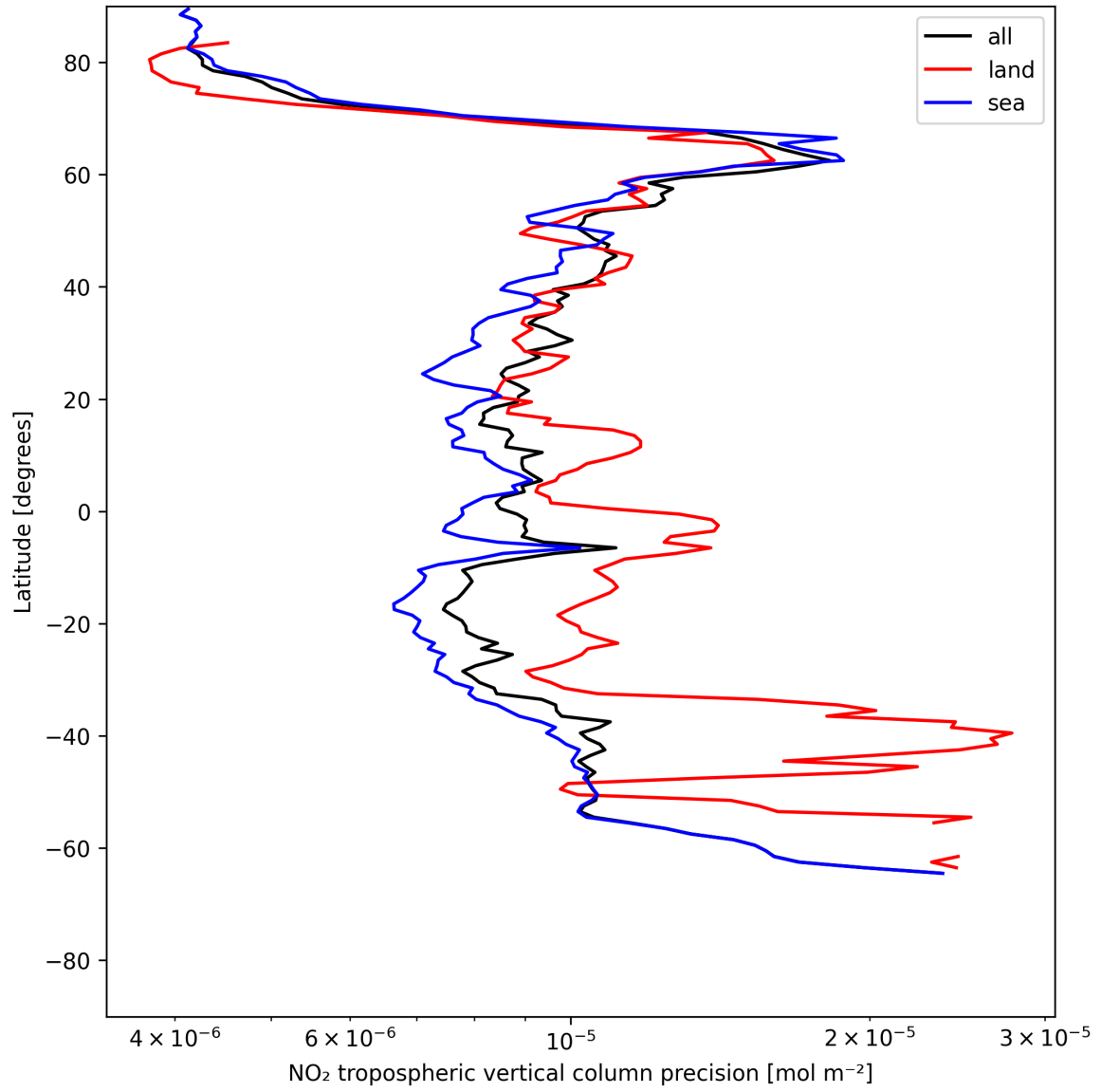
Figure 11: Zonal average of “NO 2 tropospheric vertical column precision” for 2025-06-04 to 2025-06-04.
