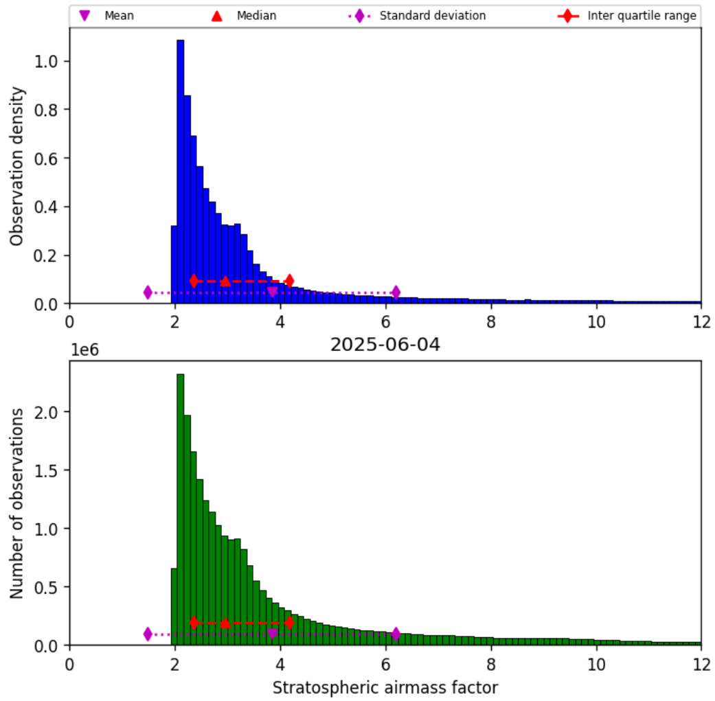
Figure 42: Histogram of “Stratospheric airmass factor” for 2025-06-04 to 2025-06-04
