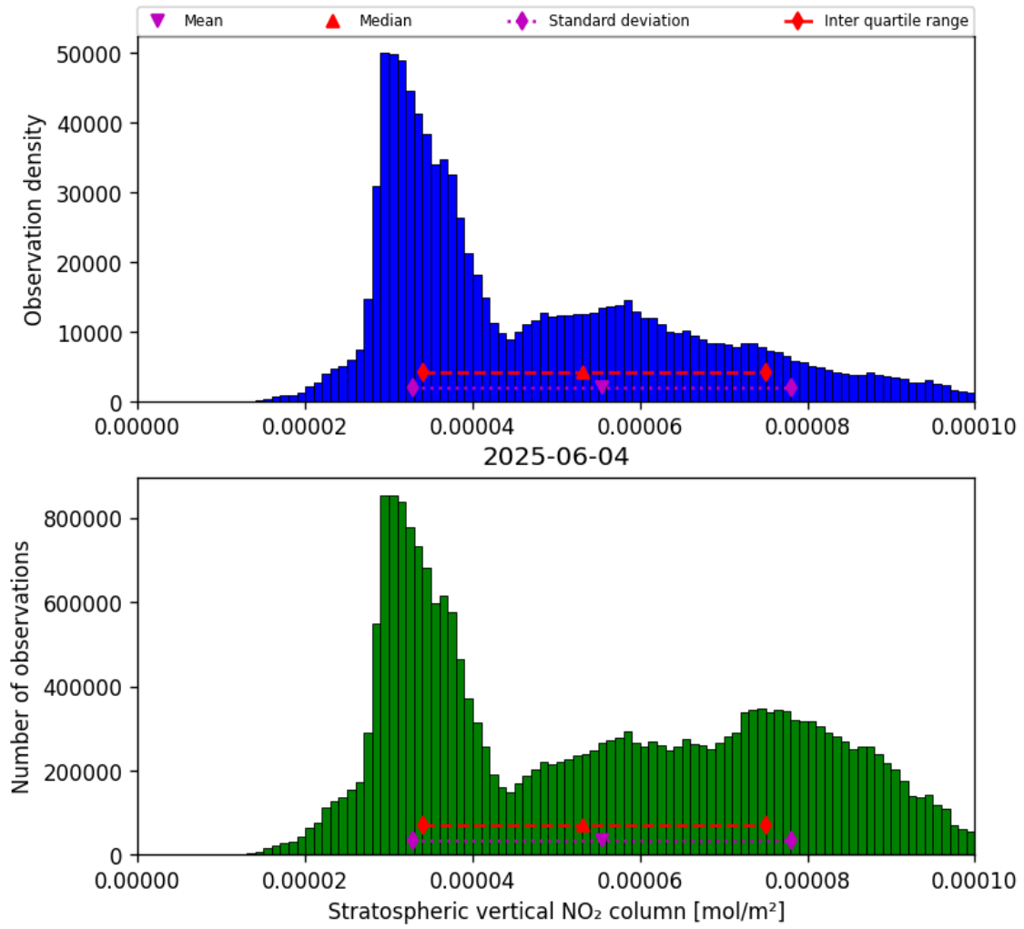
Figure 34: Histogram of “Stratospheric vertical NO 2 column” for 2025-06-04 to 2025-06-04
