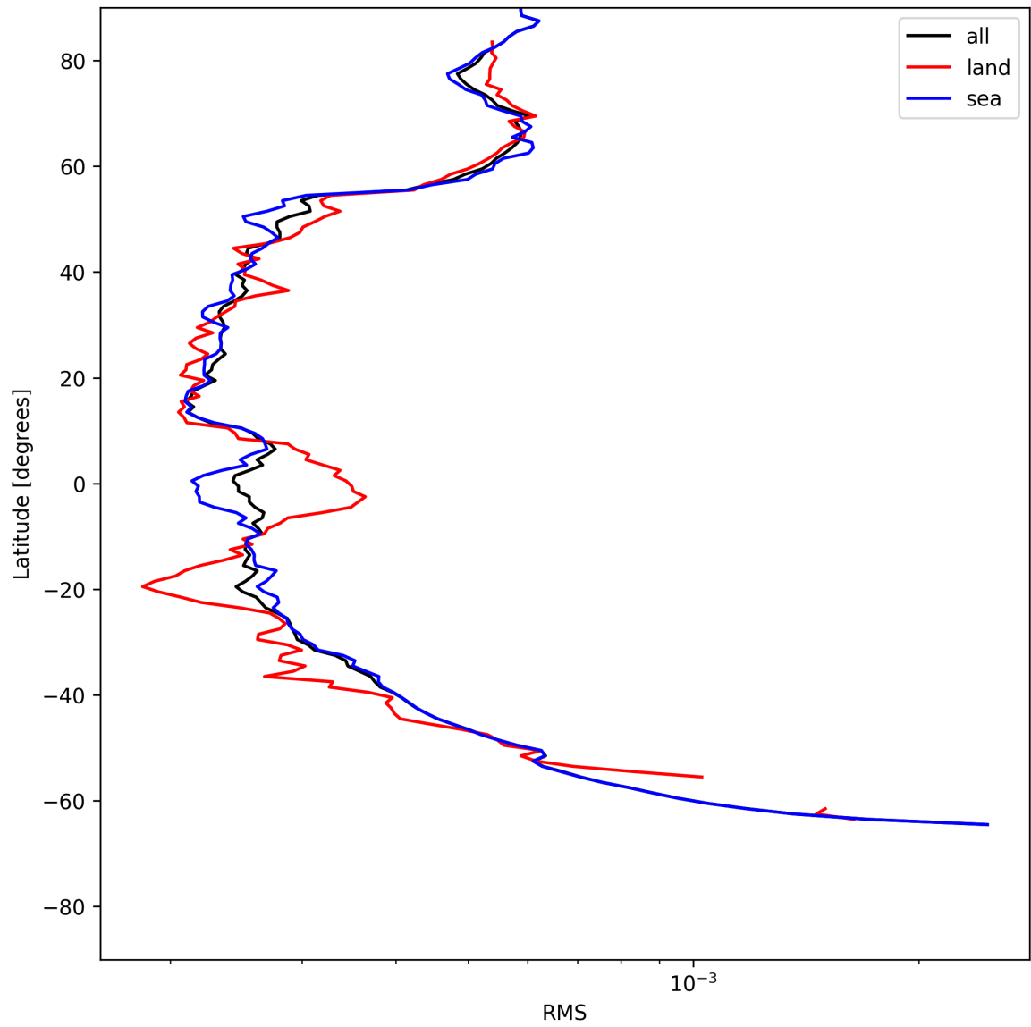
Figure 24: Zonal average of “RMS” for 2025-06-04 to 2025-06-04.
