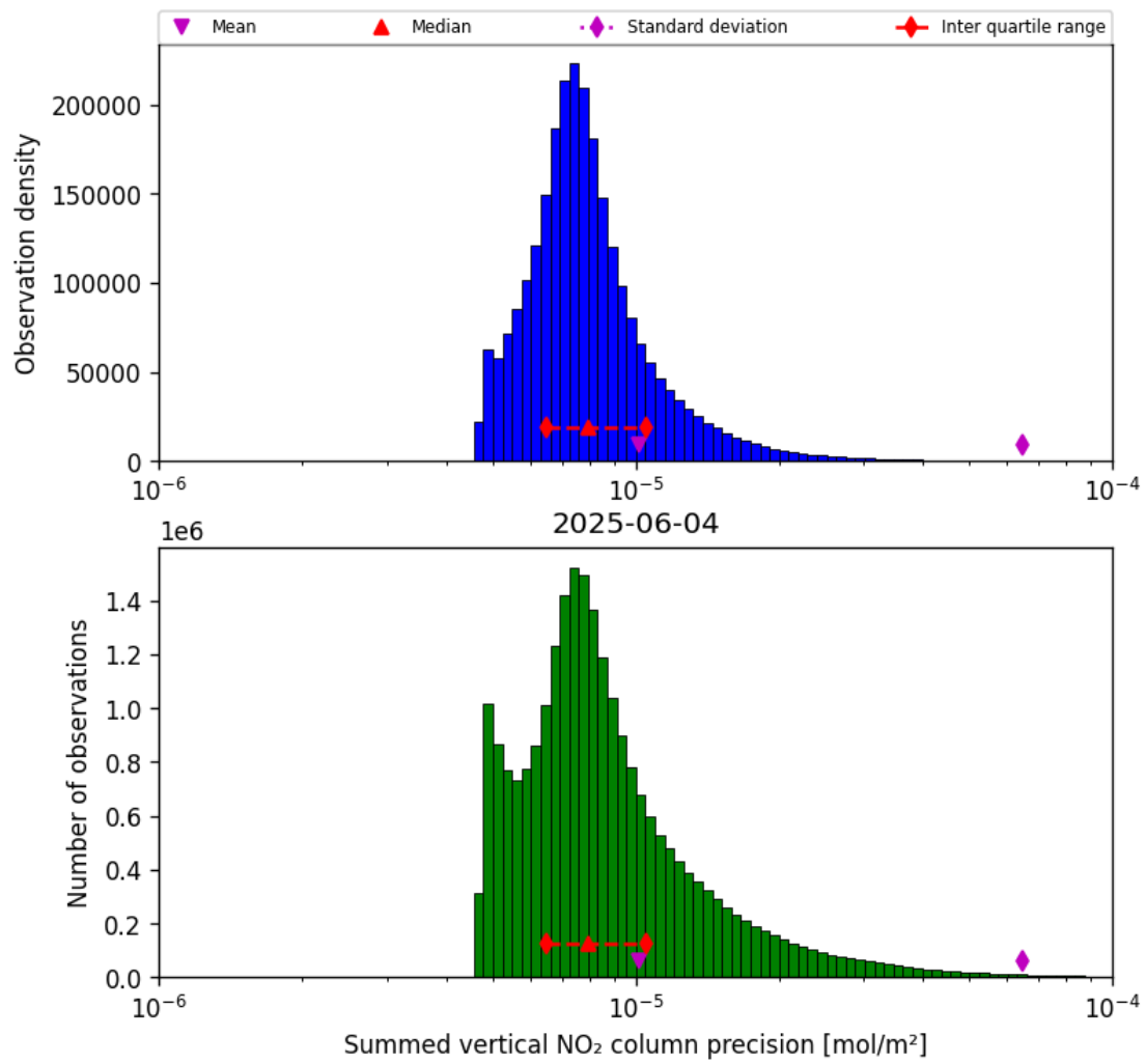
Figure 39: Histogram of "Summed vertical NO 2 column precision" for 2025-06-04 to 2025-06-04
