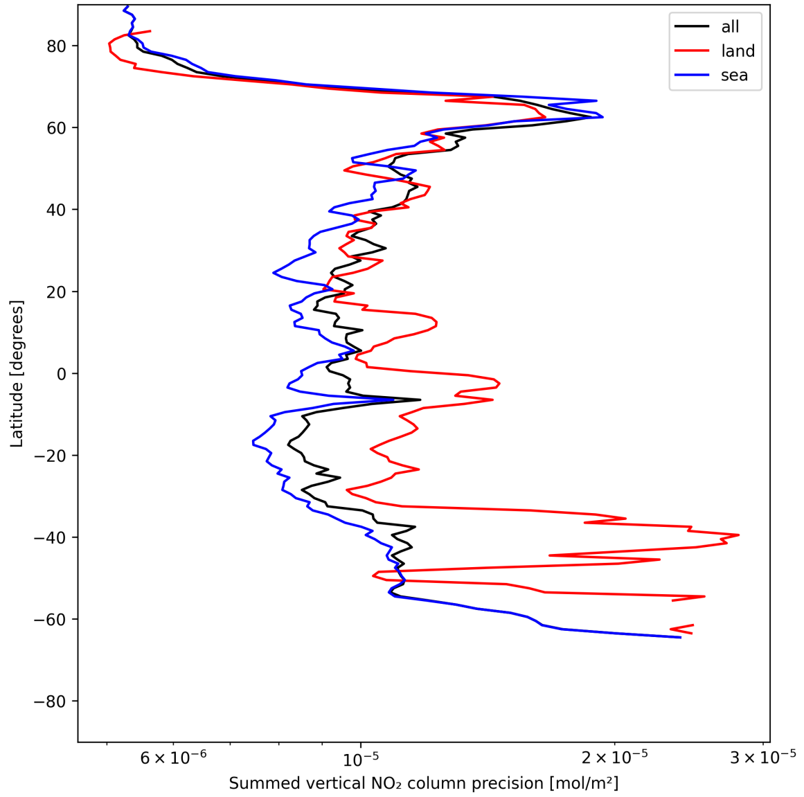
Figure 22: Zonal average of “Summed vertical NO 2 column precision” for 2025-06-04 to 2025-06-04.
