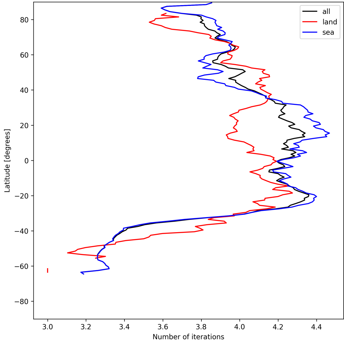
Figure 15: Zonal average of “Number of iterations” for 2025-06-04 to 2025-06-04.
