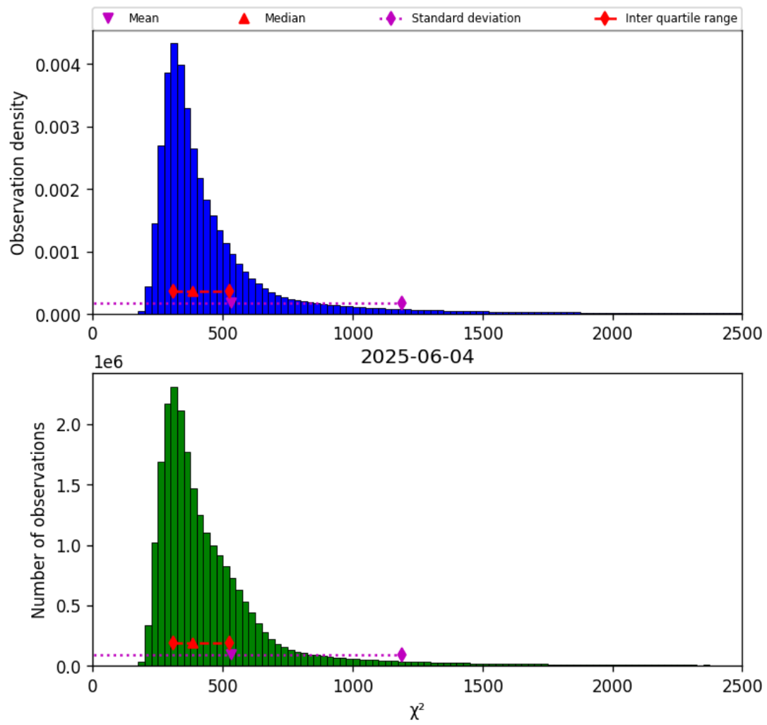
Figure 40: Histogram of " \chi^2 " for 2025-06-04 to 2025-06-04
