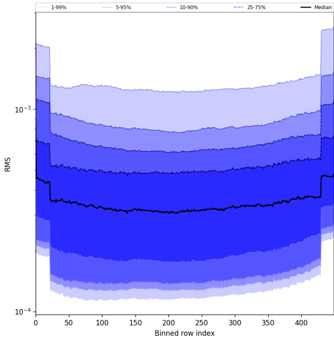
Figure 58: Along track statistics of “RMS” for 2025-06-04 to 2025-06-04
