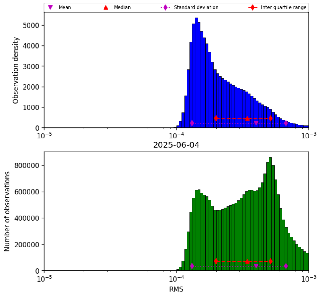
Figure 41: Histogram of “RMS” for 2025-06-04 to 2025-06-04
