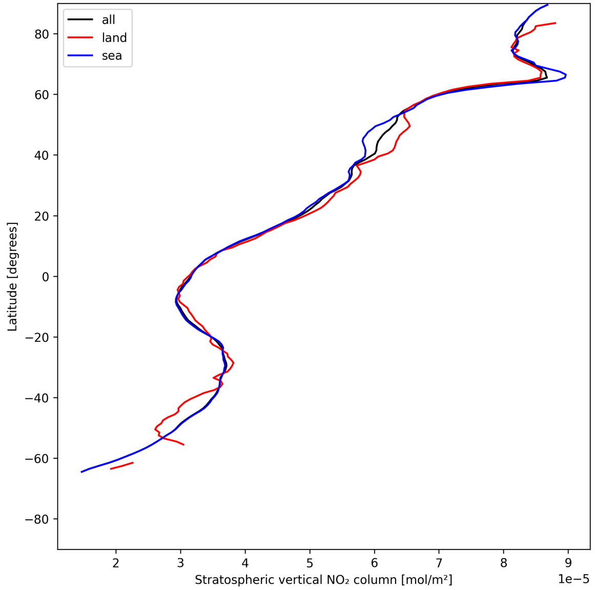
Figure 17: Zonal average of “Stratospheric vertical NO 2 column” for 2025-06-04 to 2025-06-04.
