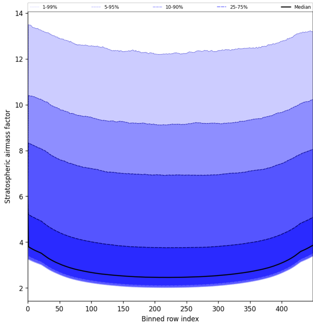
Figure 59: Along track statistics of “Stratospheric airmass factor” for 2025-06-04 to 2025-06-04
