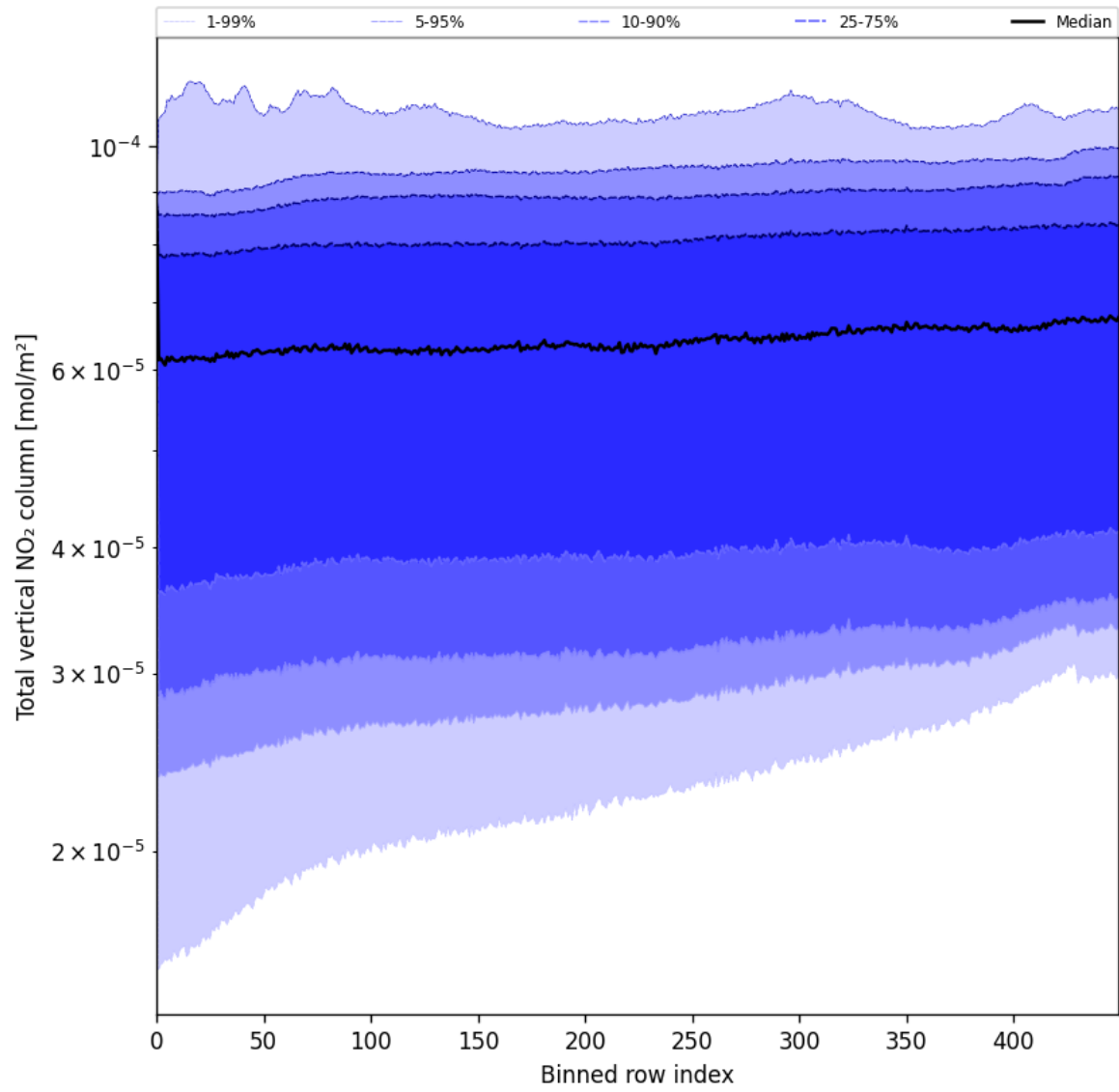
Figure 53: Along track statistics of “Total vertical NO 2 column” for 2025-06-04 to 2025-06-04
