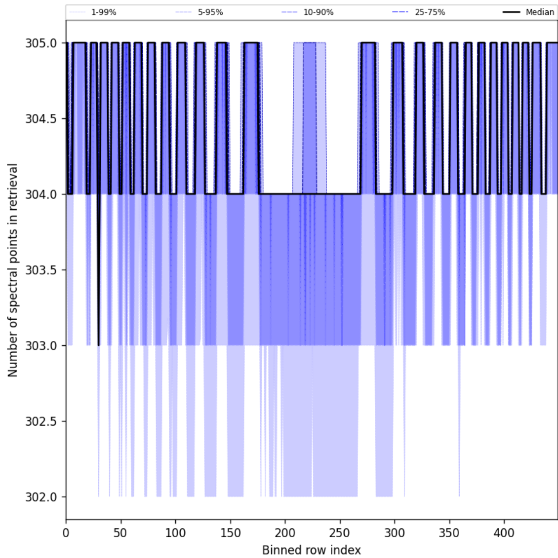
Figure 48: Along track statistics of “Number of spectral points in retrieval” for 2025-06-04 to 2025-06-04
