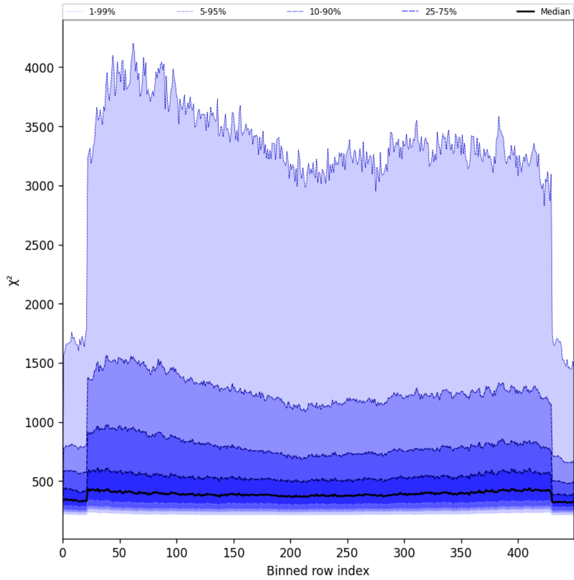
Figure 57: Along track statistics of “ \chi^2 ” for 2025-06-04 to 2025-06-04
