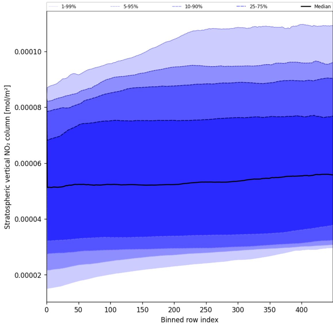
Figure 51: Along track statistics of “Stratospheric vertical NO 2 column” for 2025-06-04 to 2025-06-04
