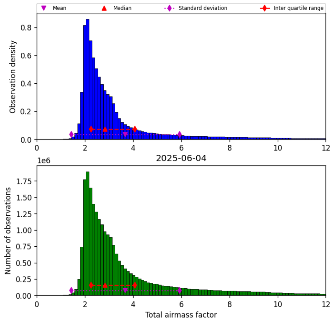
Figure 30: Histogram of “Total airmass factor” for 2025-06-04 to 2025-06-04
