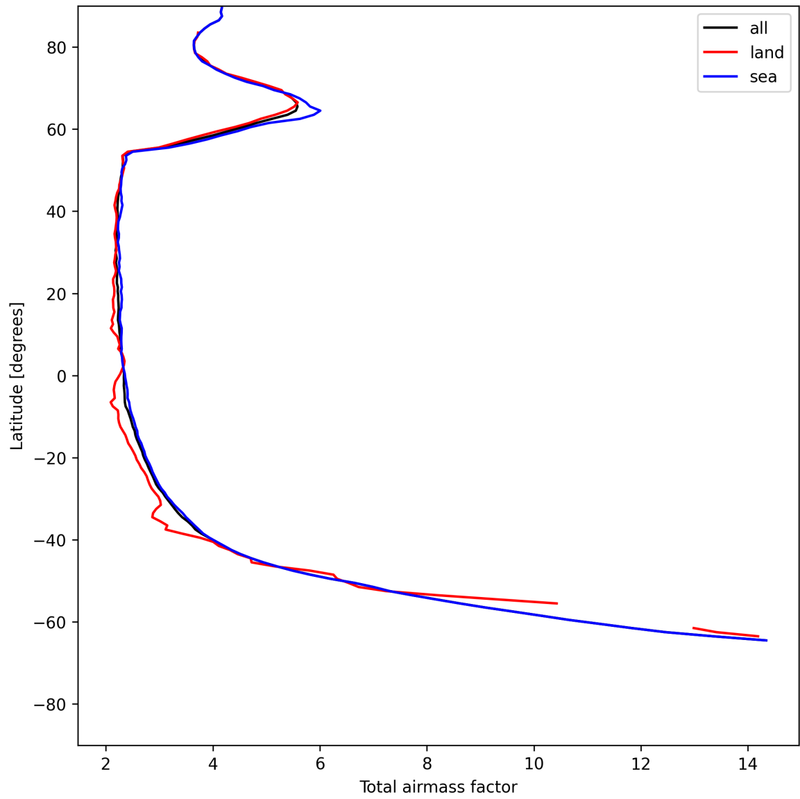
Figure 13: Zonal average of “Total airmass factor” for 2025-06-04 to 2025-06-04.
