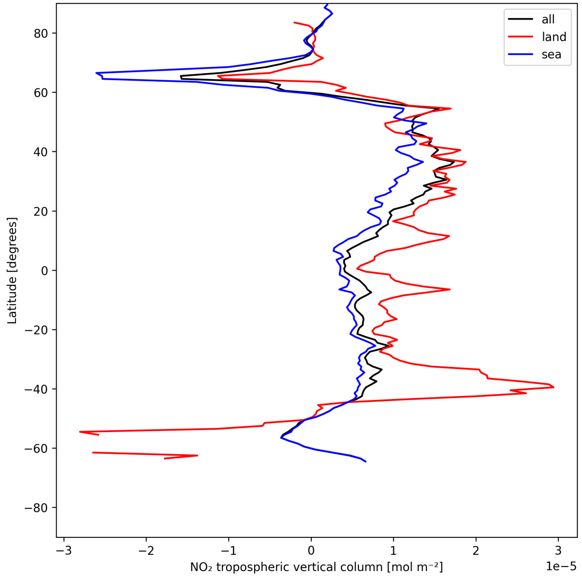
Figure 10: Zonal average of “NO 2 tropospheric vertical column” for 2025-06-04 to 2025-06-04.
