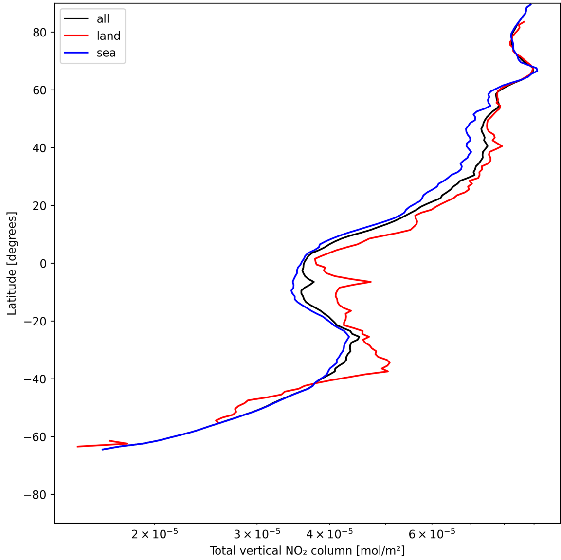
Figure 19: Zonal average of “Total vertical NO 2 column” for 2025-06-04 to 2025-06-04.
