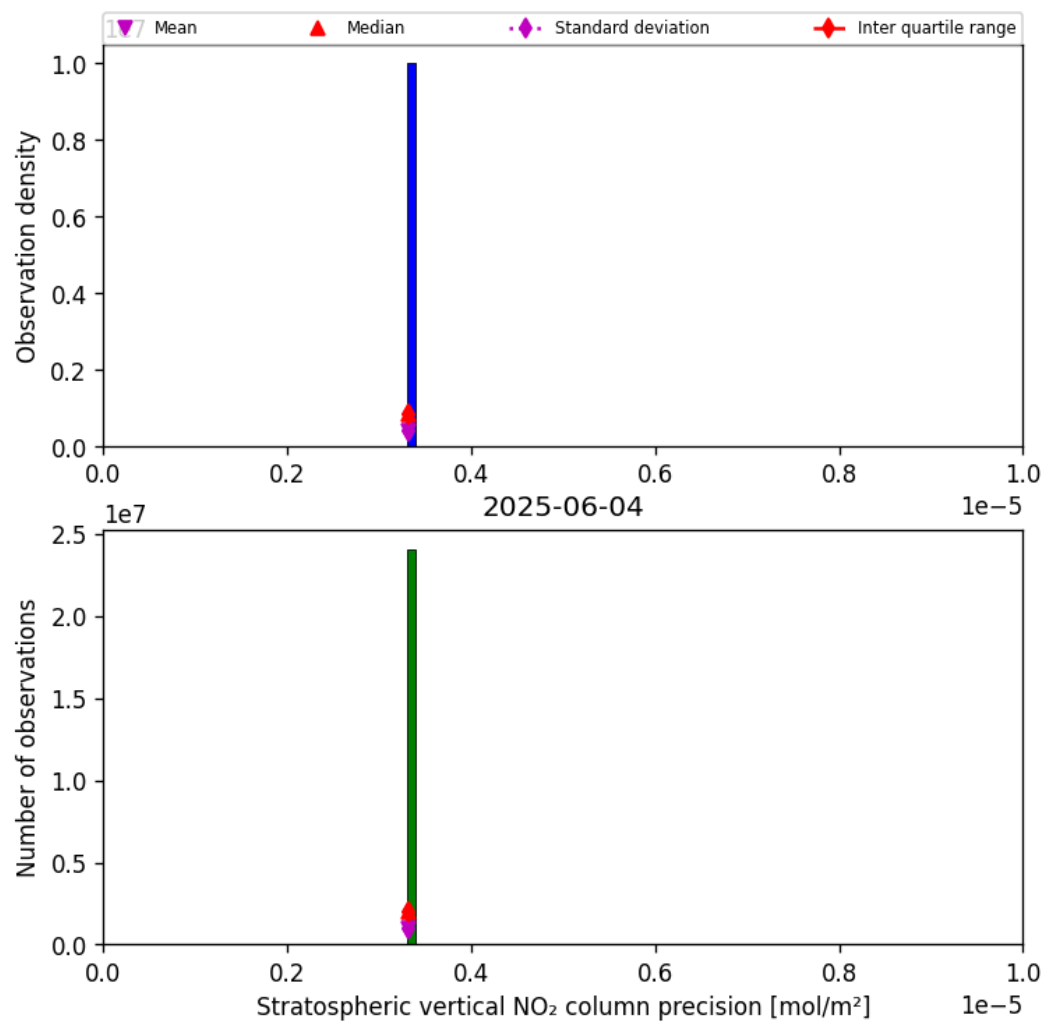
Figure 35: Histogram of “Stratospheric vertical NO 2 column precision” for 2025-06-04 to 2025-06-04
