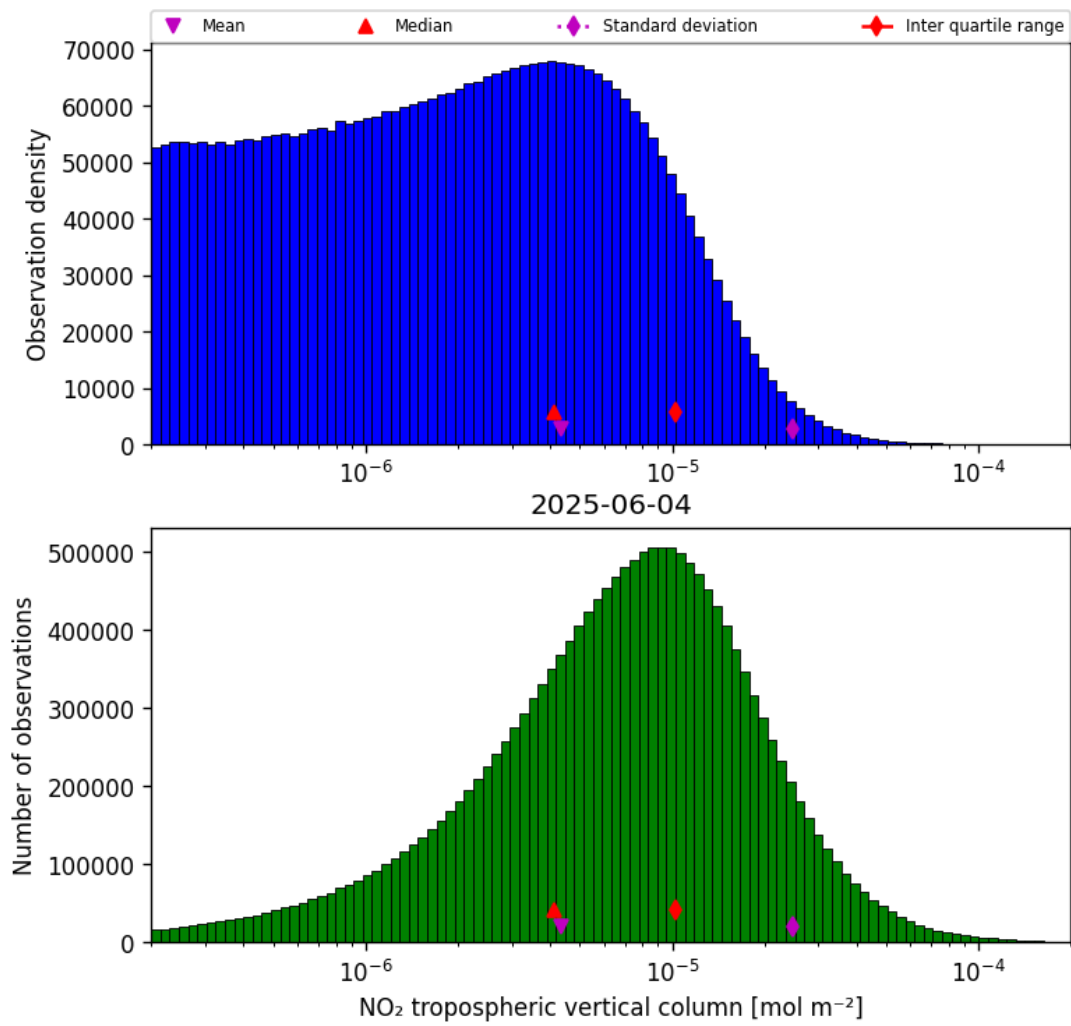
Figure 27: Histogram of “NO 2 tropospheric vertical column” for 2025-06-04 to 2025-06-04
