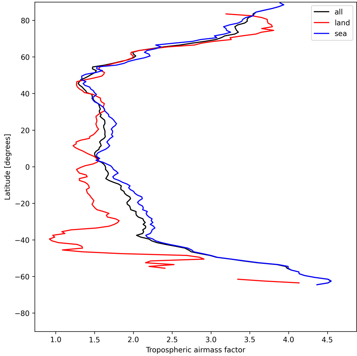
Figure 12: Zonal average of “Tropospheric air mass factor” for 2025-06-04 to 2025-06-04.
