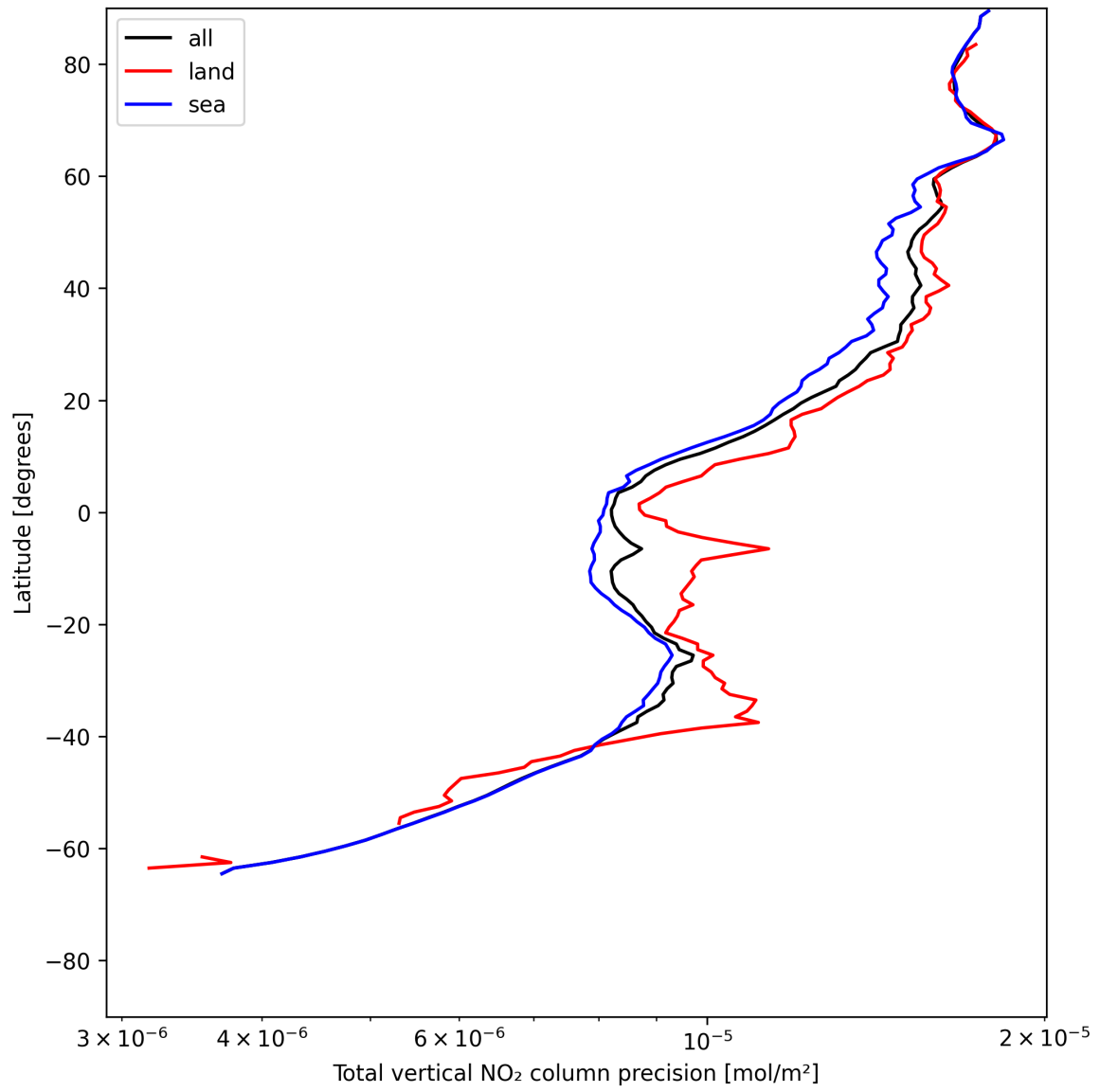
Figure 20: Zonal average of “Total vertical NO 2 column precision” for 2025-06-04 to 2025-06-04.
