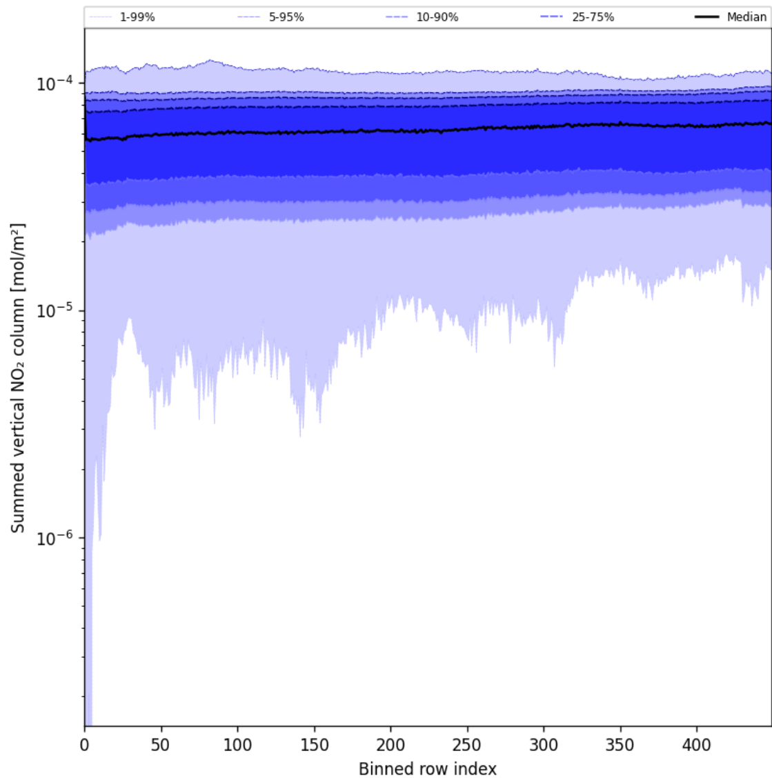
Figure 55: Along track statistics of “Summed vertical NO 2 column” for 2025-06-04 to 2025-06-04
