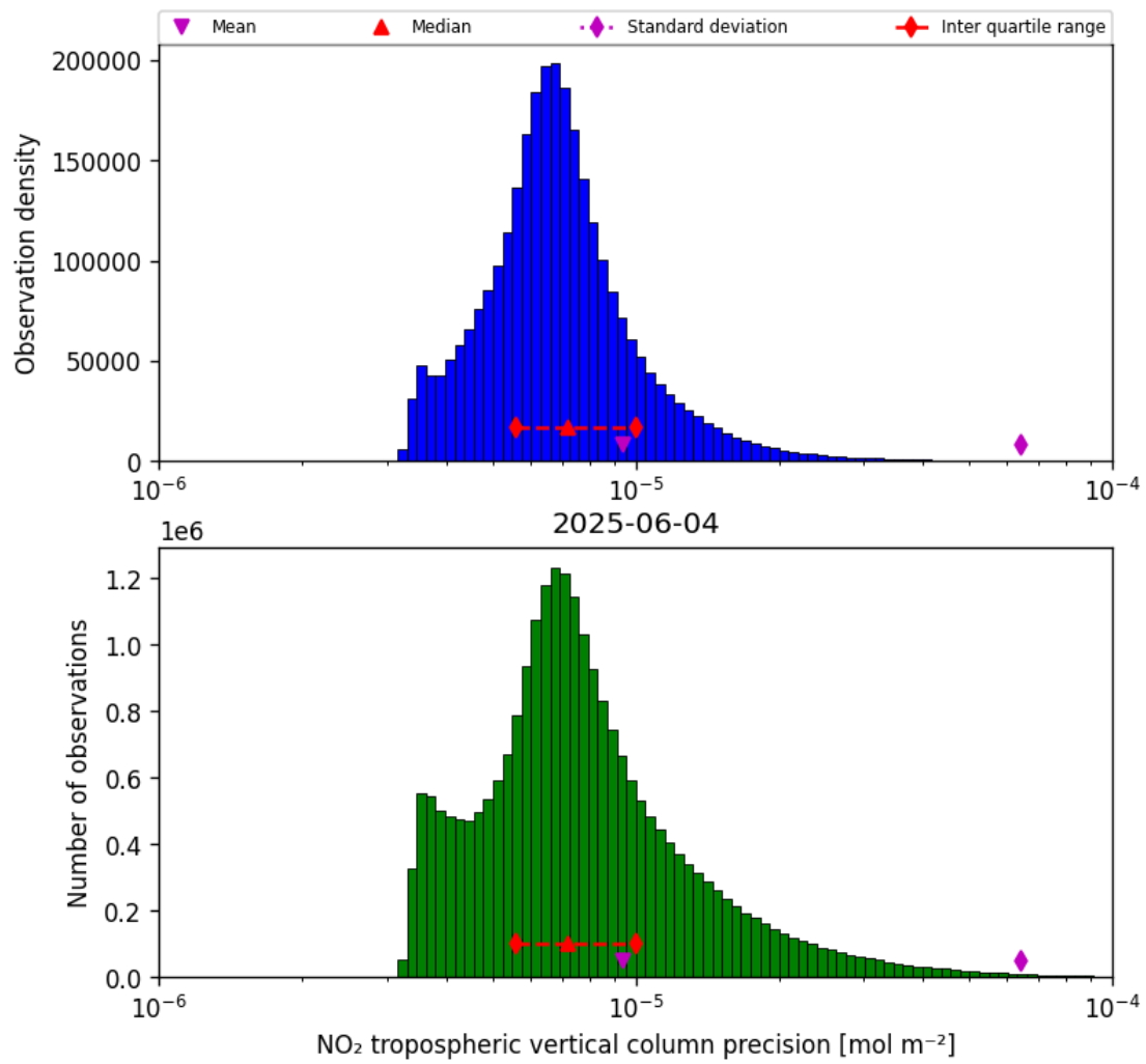
Figure 28: Histogram of “NO 2 tropospheric vertical column precision” for 2025-06-04 to 2025-06-04
