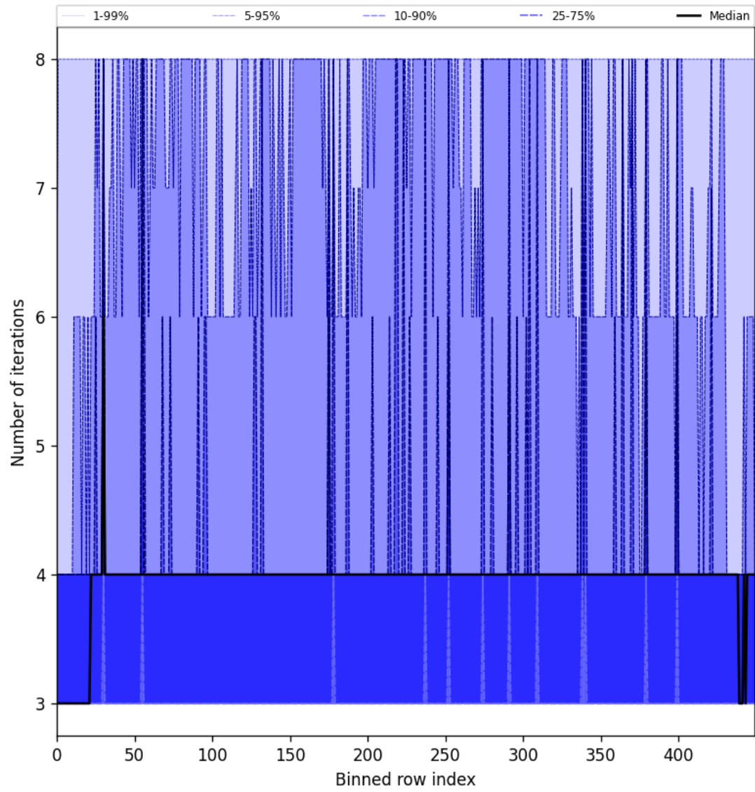
Figure 49: Along track statistics of “Number of iterations” for 2025-06-04 to 2025-06-04
