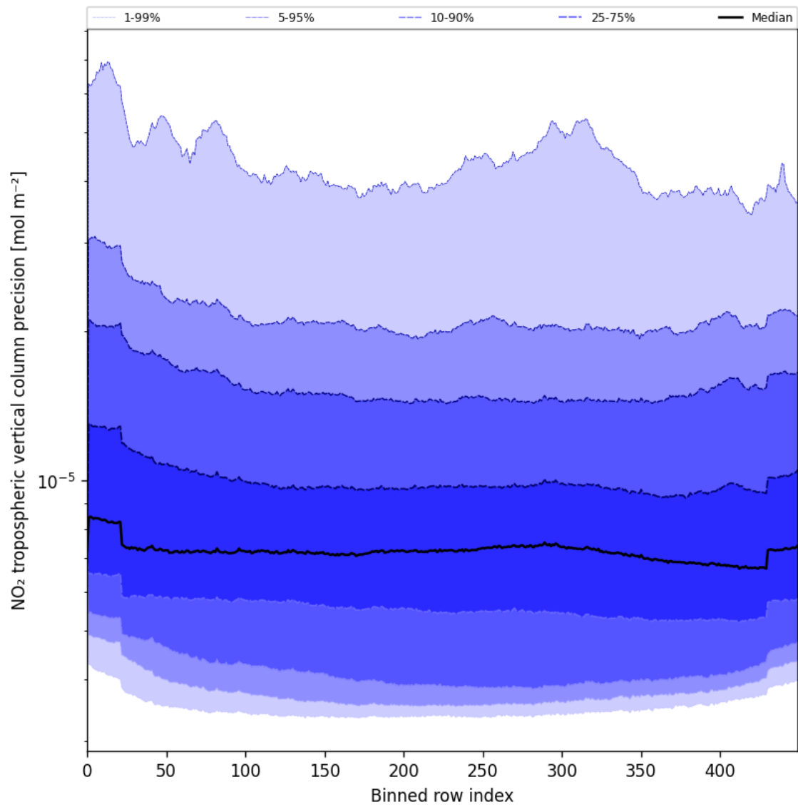
Figure 45: Along track statistics of “NO 2 tropospheric vertical column precision” for 2025-06-04 to 2025-06-04
