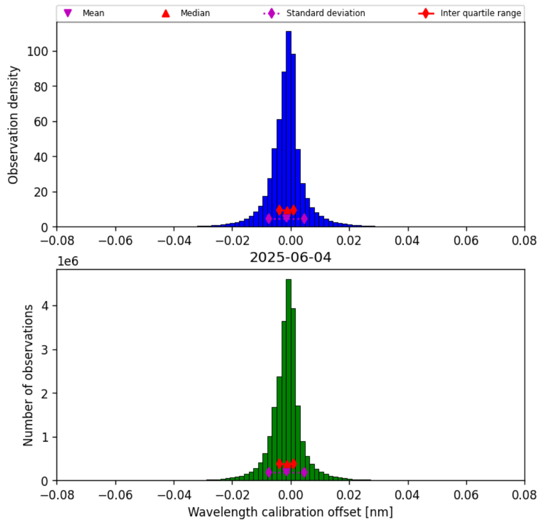
Figure 33: Histogram of “Wavelength calibration offset” for 2025-06-04 to 2025-06-04
