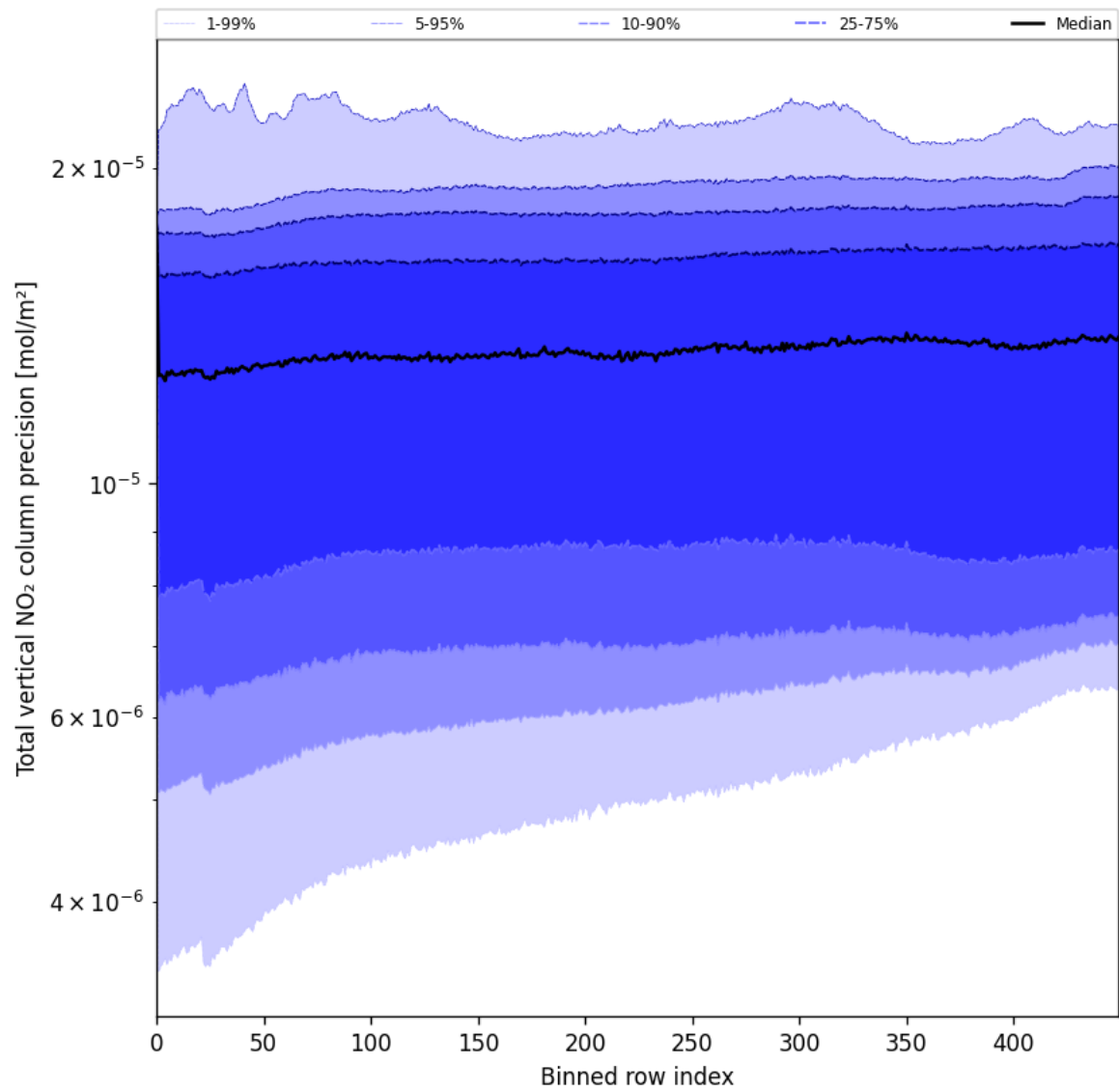
Figure 54: Along track statistics of “Total vertical NO 2 column precision” for 2025-06-04 to 2025-06-04
