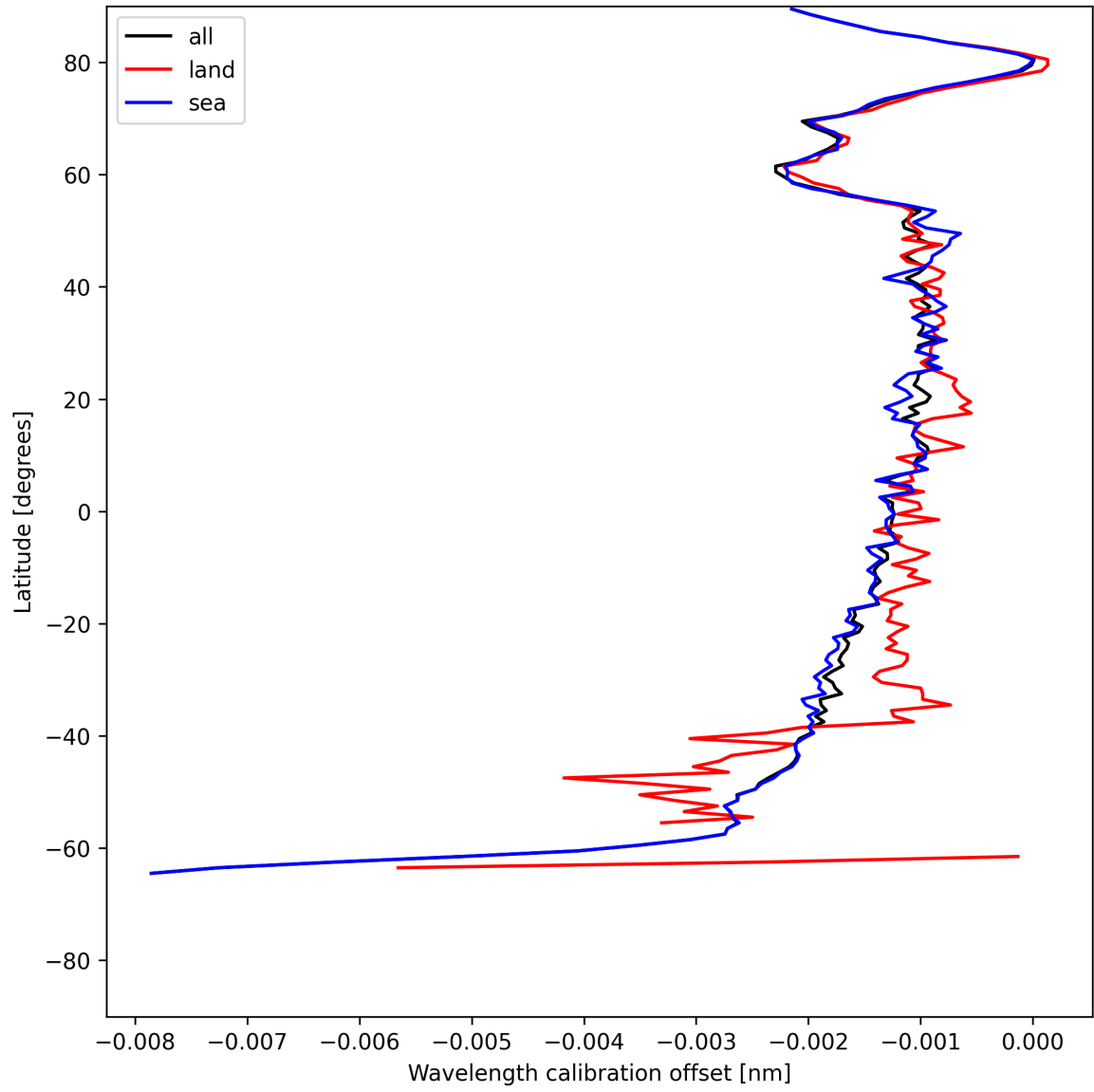
Figure 16: Zonal average of “Wavelength calibration offset” for 2025-06-04 to 2025-06-04.
