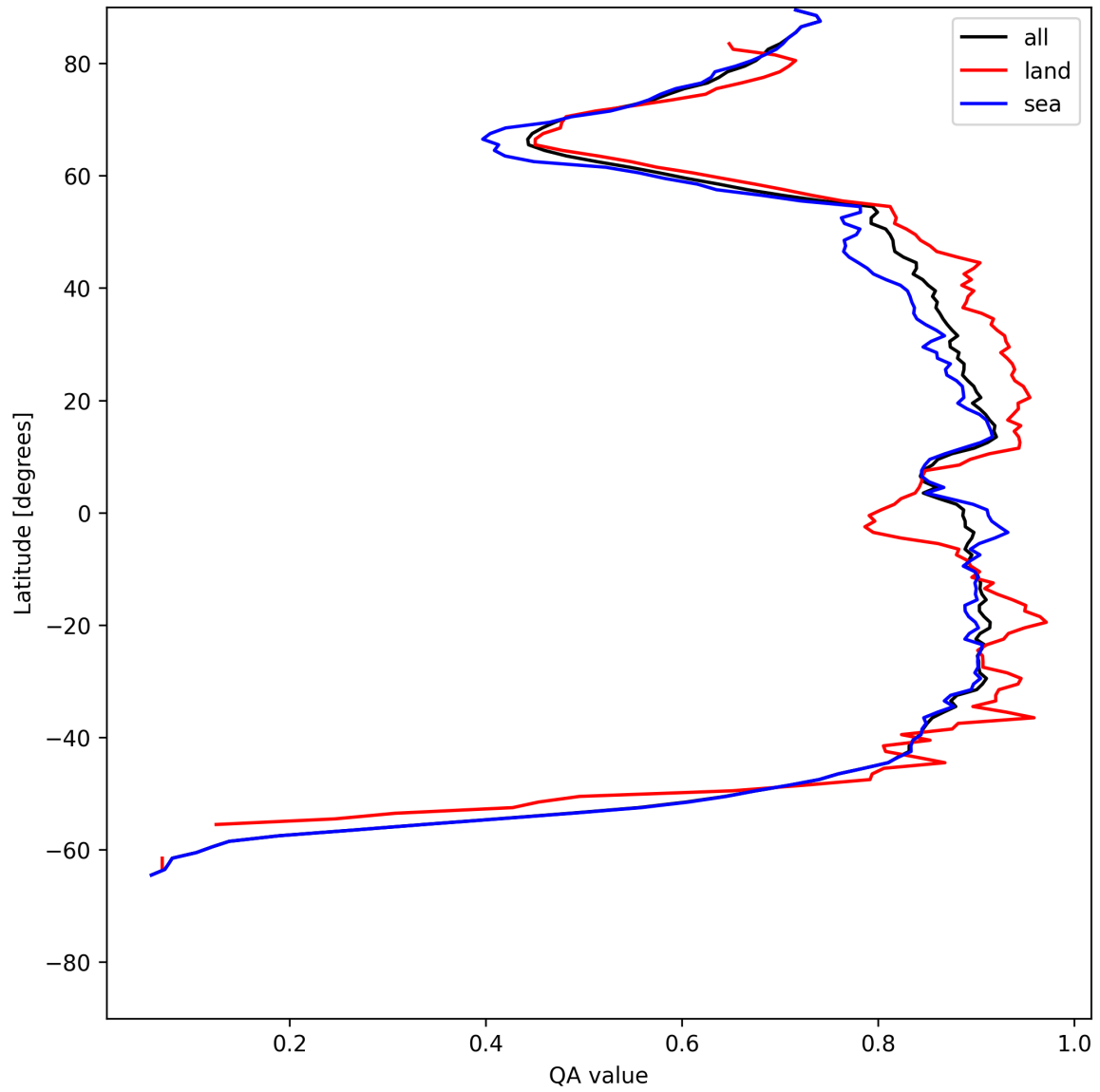
Figure 9: Zonal average of “QA value” for 2025-06-04 to 2025-06-04.
