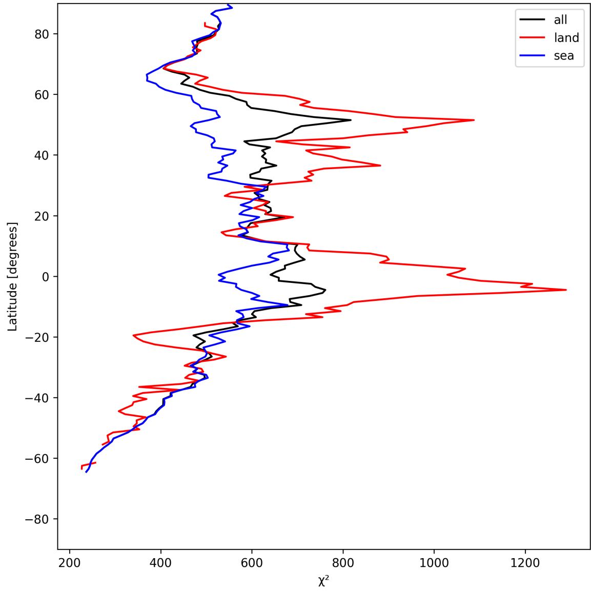
Figure 23: Zonal average of “ \chi^2 ” for 2025-06-04 to 2025-06-04.
