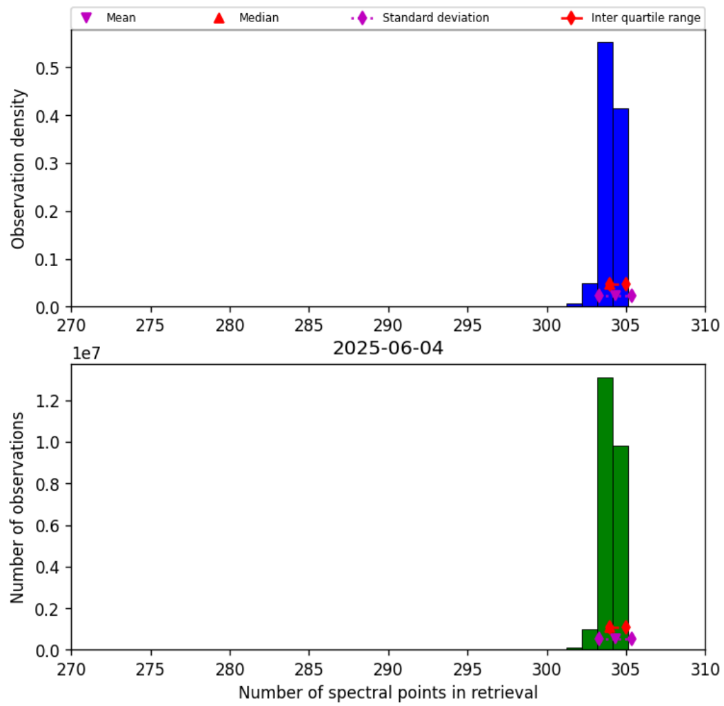
Figure 31: Histogram of “Number of spectral points in retrieval” for 2025-06-04 to 2025-06-04
