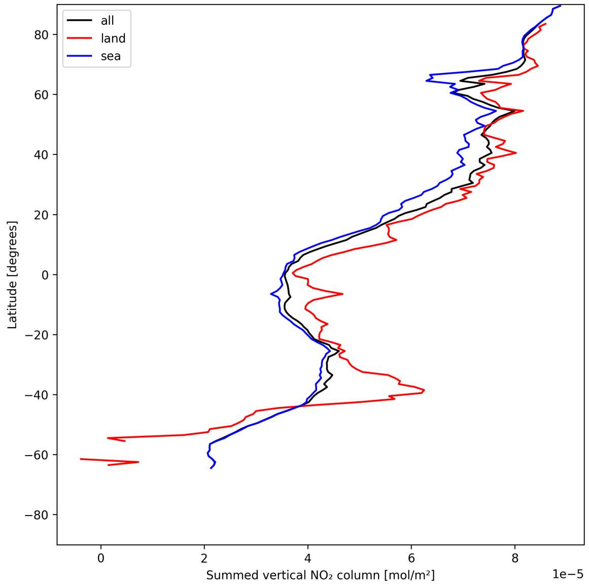
Figure 21: Zonal average of “Summed vertical NO 2 column” for 2025-06-04 to 2025-06-04.
