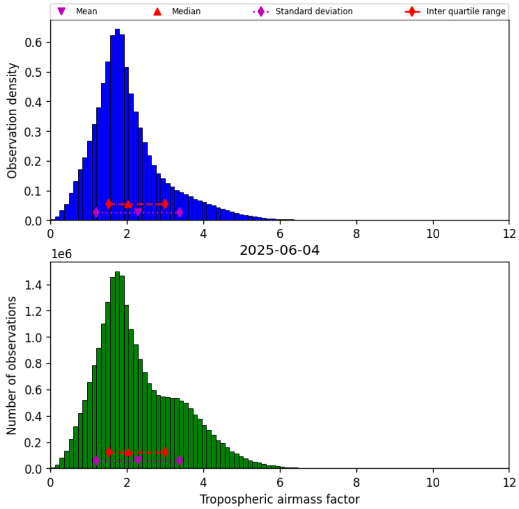
Figure 29: Histogram of “Tropospheric airmass factor” for 2025-06-04 to 2025-06-04
