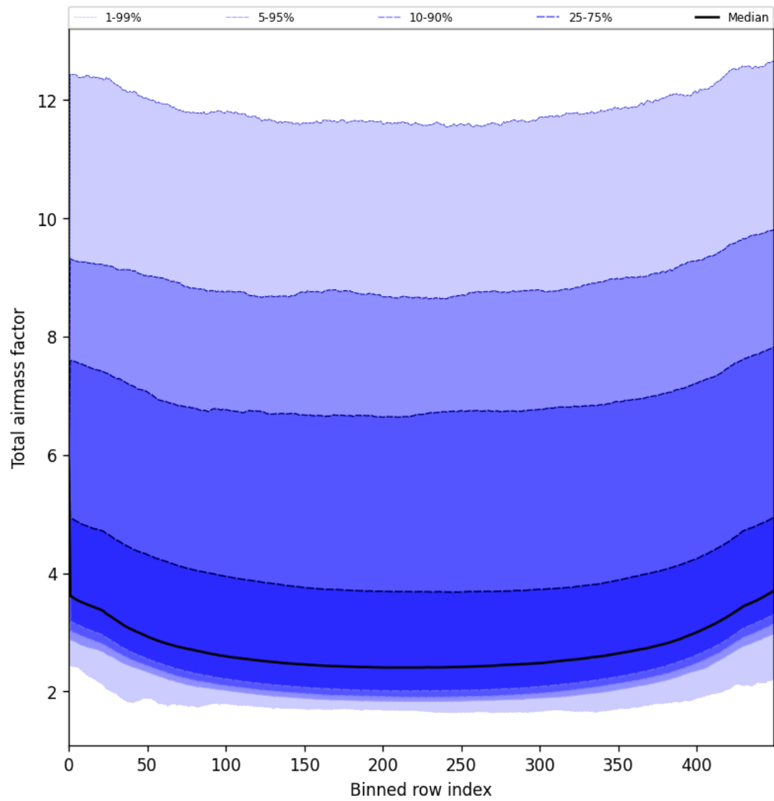
Figure 47: Along track statistics of “Total airmass factor” for 2025-06-04 to 2025-06-04
