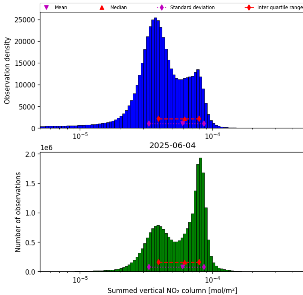
Figure 38: Histogram of “Summed vertical NO 2 column” for 2025-06-04 to 2025-06-04
