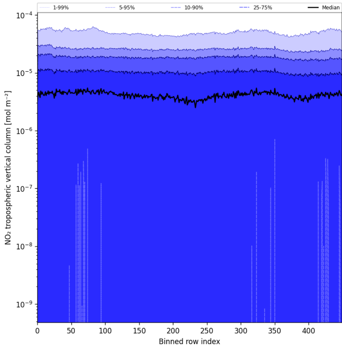
Figure 44: Along track statistics of “NO 2 tropospheric vertical column” for 2025-06-04 to 2025-06-04
