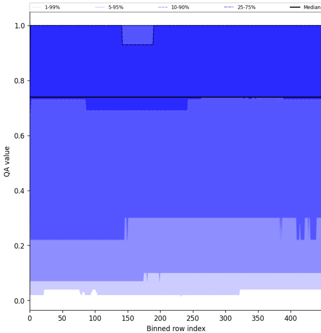
Figure 43: Along track statistics of “QA value” for 2025-06-04 to 2025-06-04
