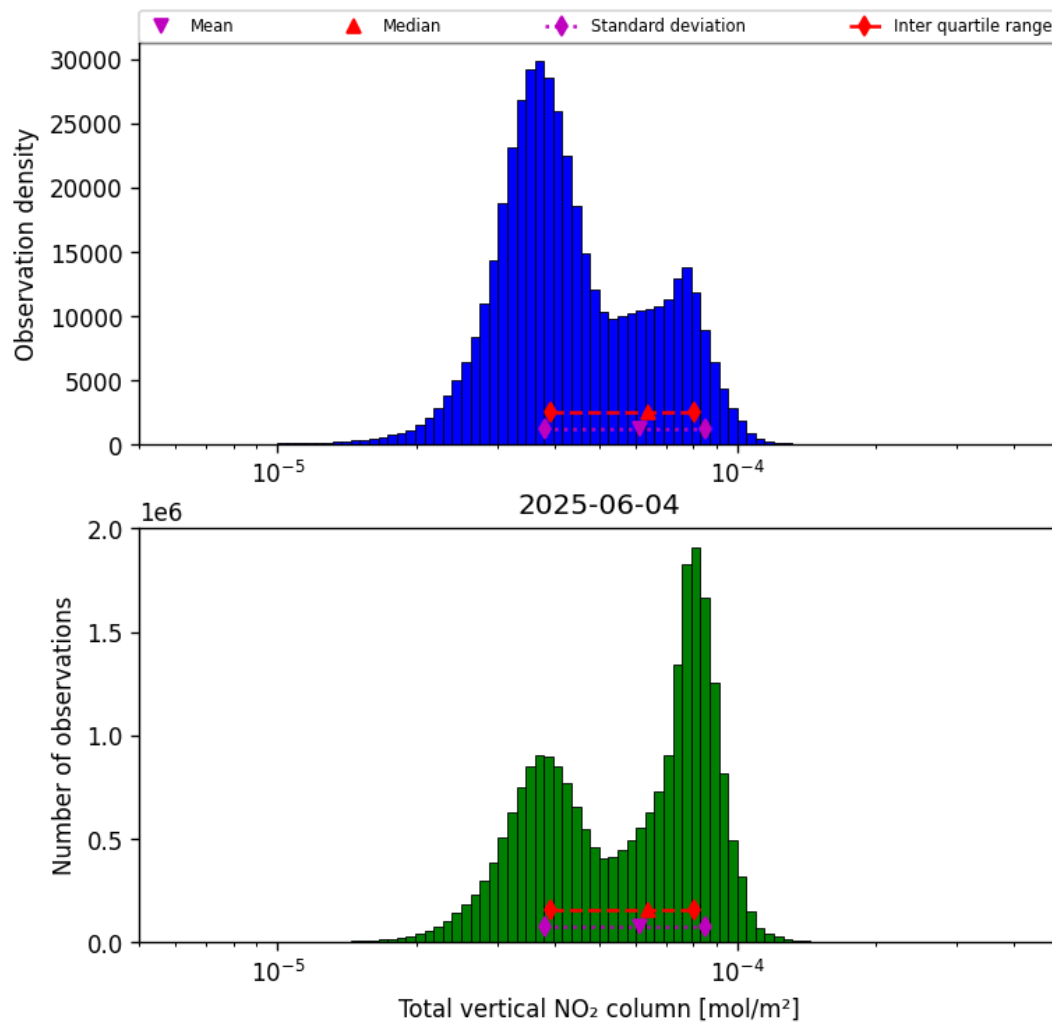
Figure 36: Histogram of "Total vertical NO 2 column" for 2025-06-04 to 2025-06-04
