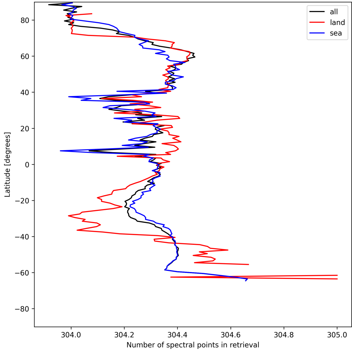
Figure 14: Zonal average of “Number of spectral points in retrieval” for 2025-06-04 to 2025-06-04.
