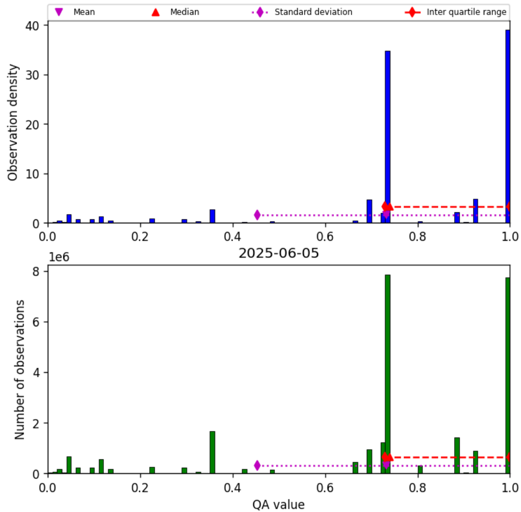
Figure 26: Histogram of “QA value” for 2025-06-05 to 2025-06-06
