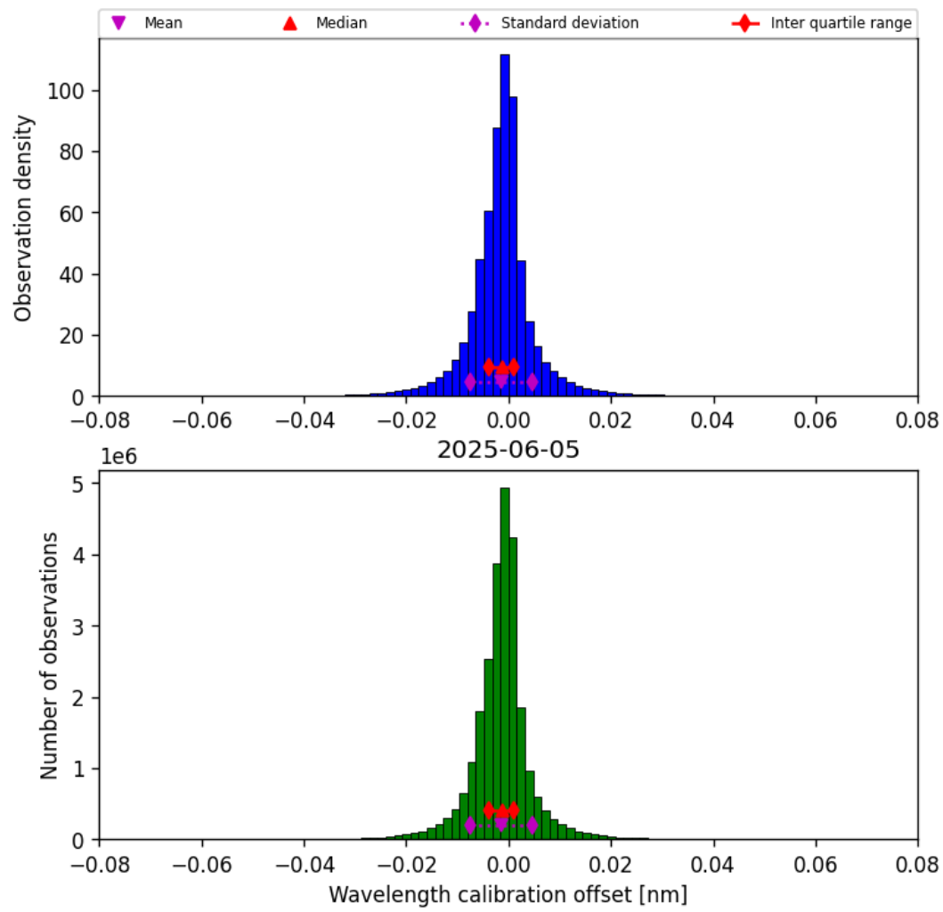
Figure 33: Histogram of “Wavelength calibration offset” for 2025-06-05 to 2025-06-06
