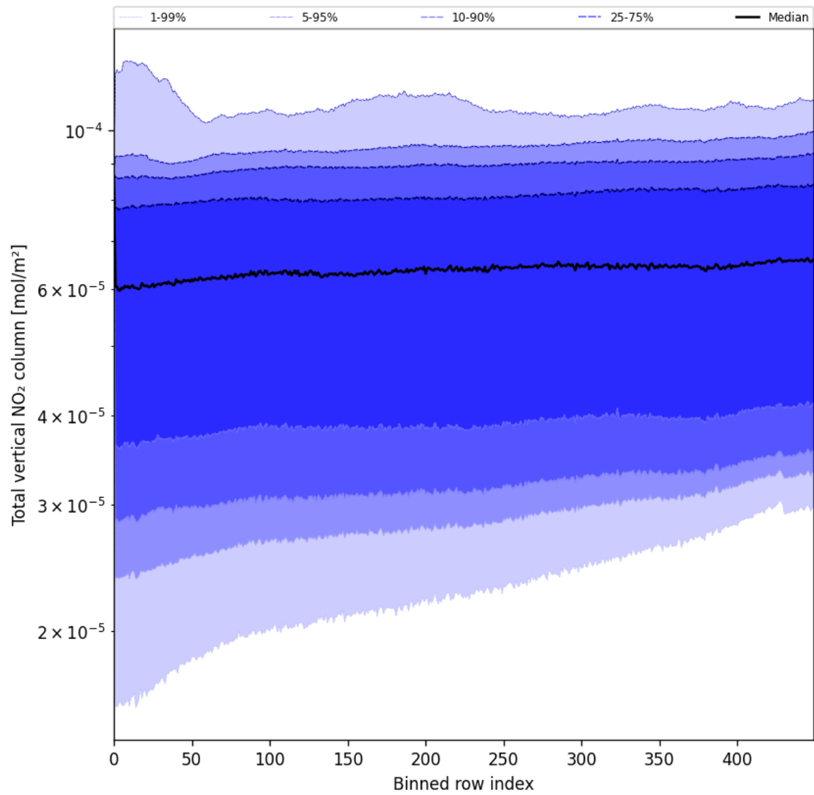
Figure 53: Along track statistics of “Total vertical NO 2 column” for 2025-06-05 to 2025-06-06
