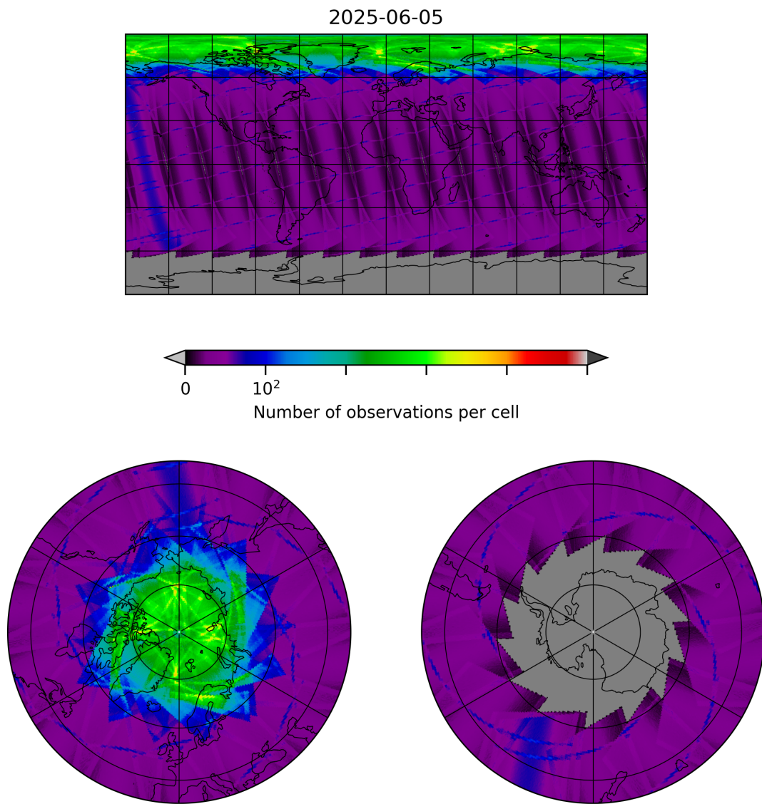
Figure 8: Map of the number of observations for 2025-06-05 to 2025-06-06
