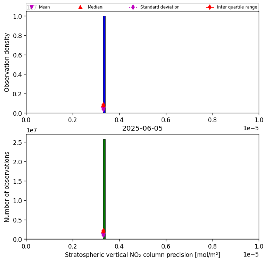
Figure 35: Histogram of “Stratospheric vertical NO 2 column precision” for 2025-06-05 to 2025-06-06
