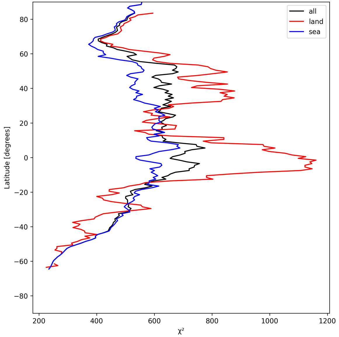
Figure 23: Zonal average of “ \chi^2 ” for 2025-06-05 to 2025-06-06.
