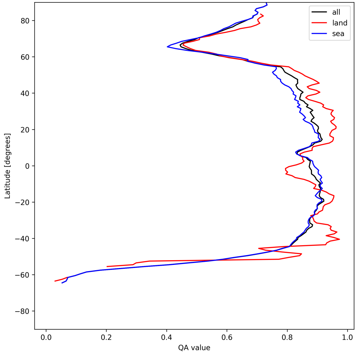
Figure 9: Zonal average of “QA value” for 2025-06-05 to 2025-06-06.
