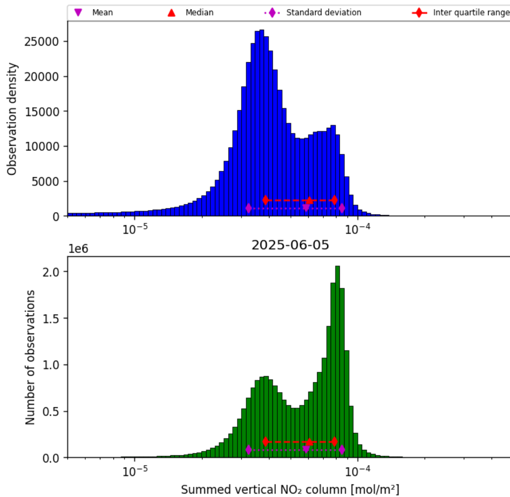
Figure 38: Histogram of “Summed vertical NO 2 column” for 2025-06-05 to 2025-06-06
