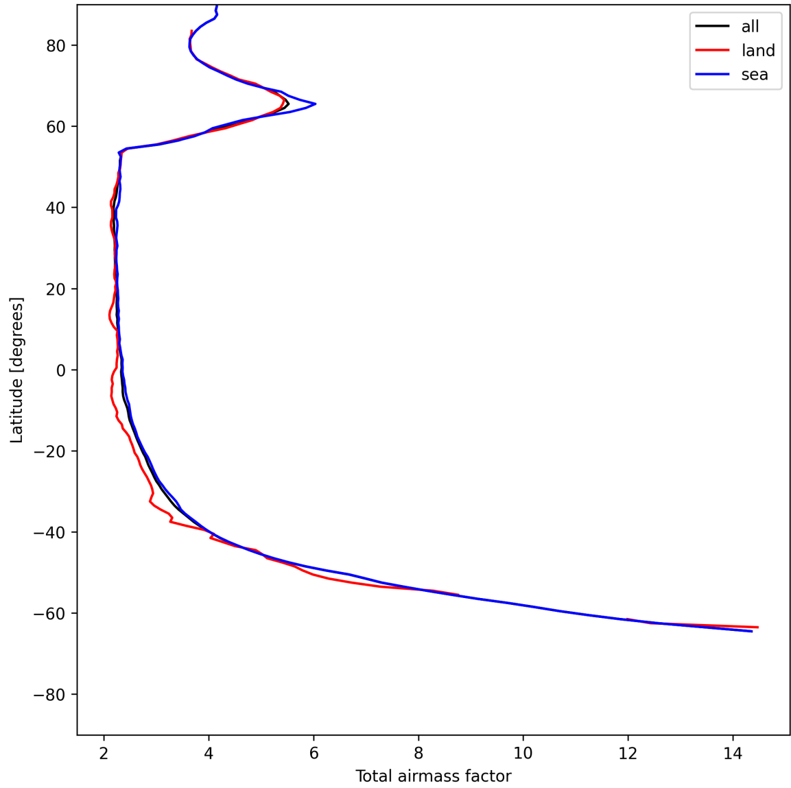
Figure 13: Zonal average of “Total airmass factor” for 2025-06-05 to 2025-06-06.
