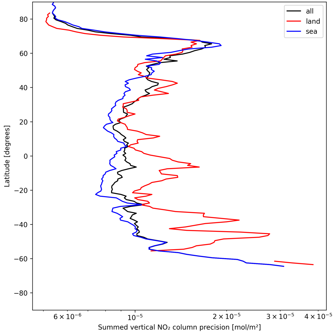
Figure 22: Zonal average of “Summed vertical NO 2 column precision” for 2025-06-05 to 2025-06-06.
