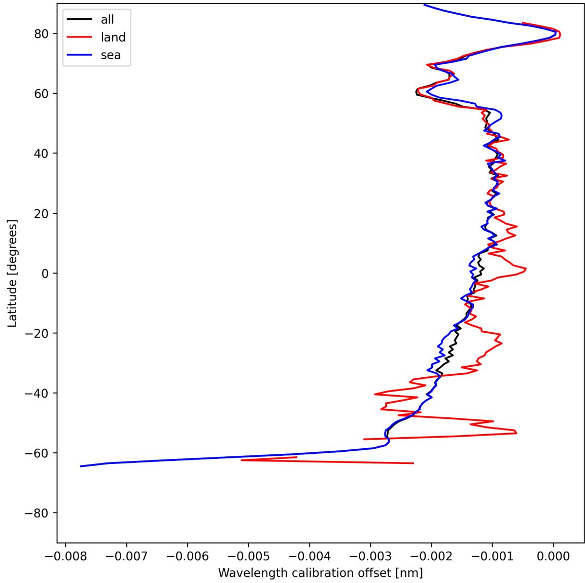
Figure 16: Zonal average of “Wavelength calibration offset” for 2025-06-05 to 2025-06-06.
