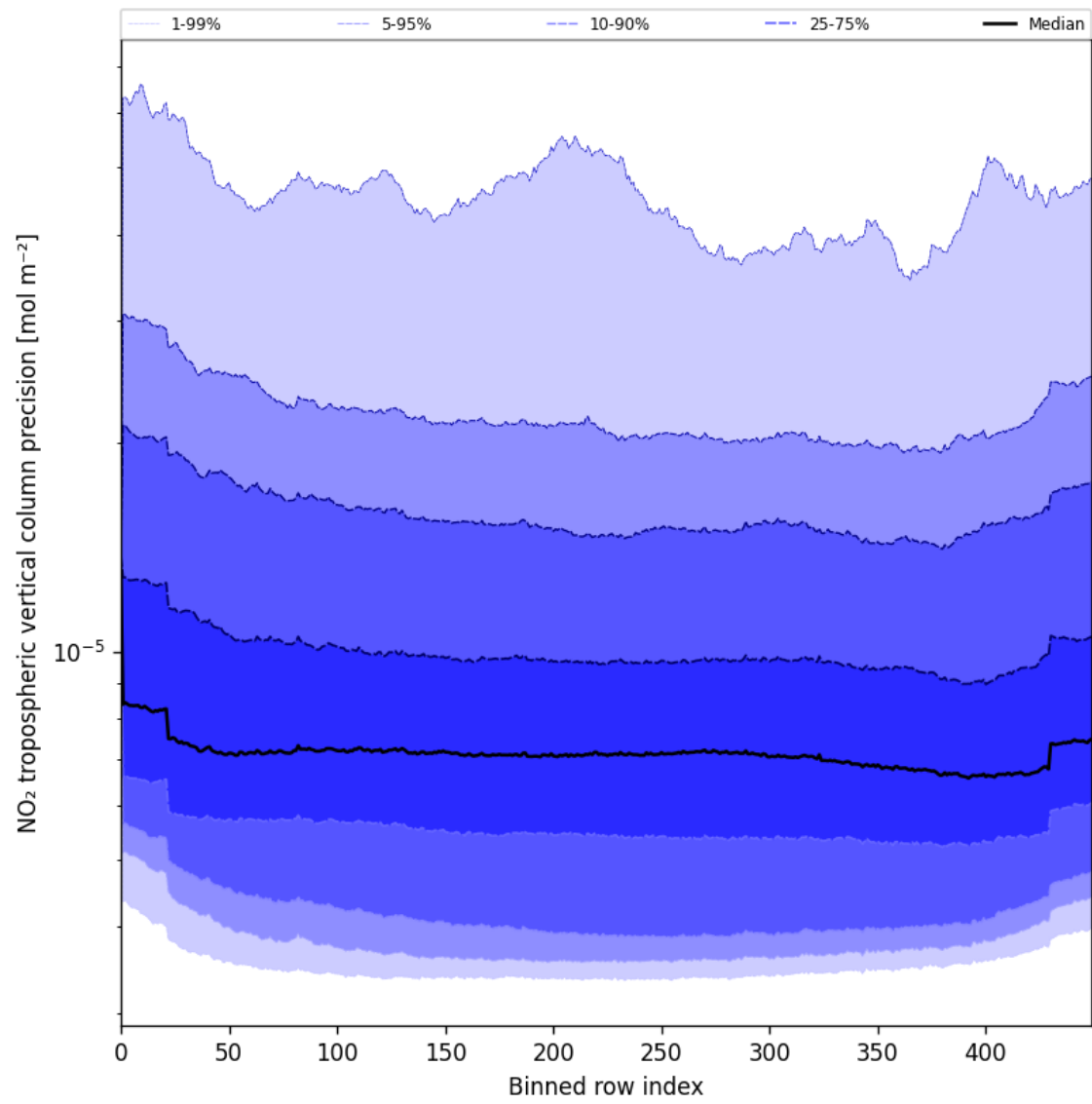
Figure 45: Along track statistics of “NO 2 tropospheric vertical column precision” for 2025-06-05 to 2025-06-06
