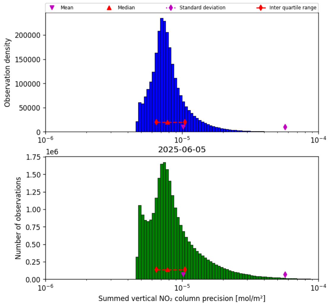
Figure 39: Histogram of “Summed vertical NO 2 column precision” for 2025-06-05 to 2025-06-06
