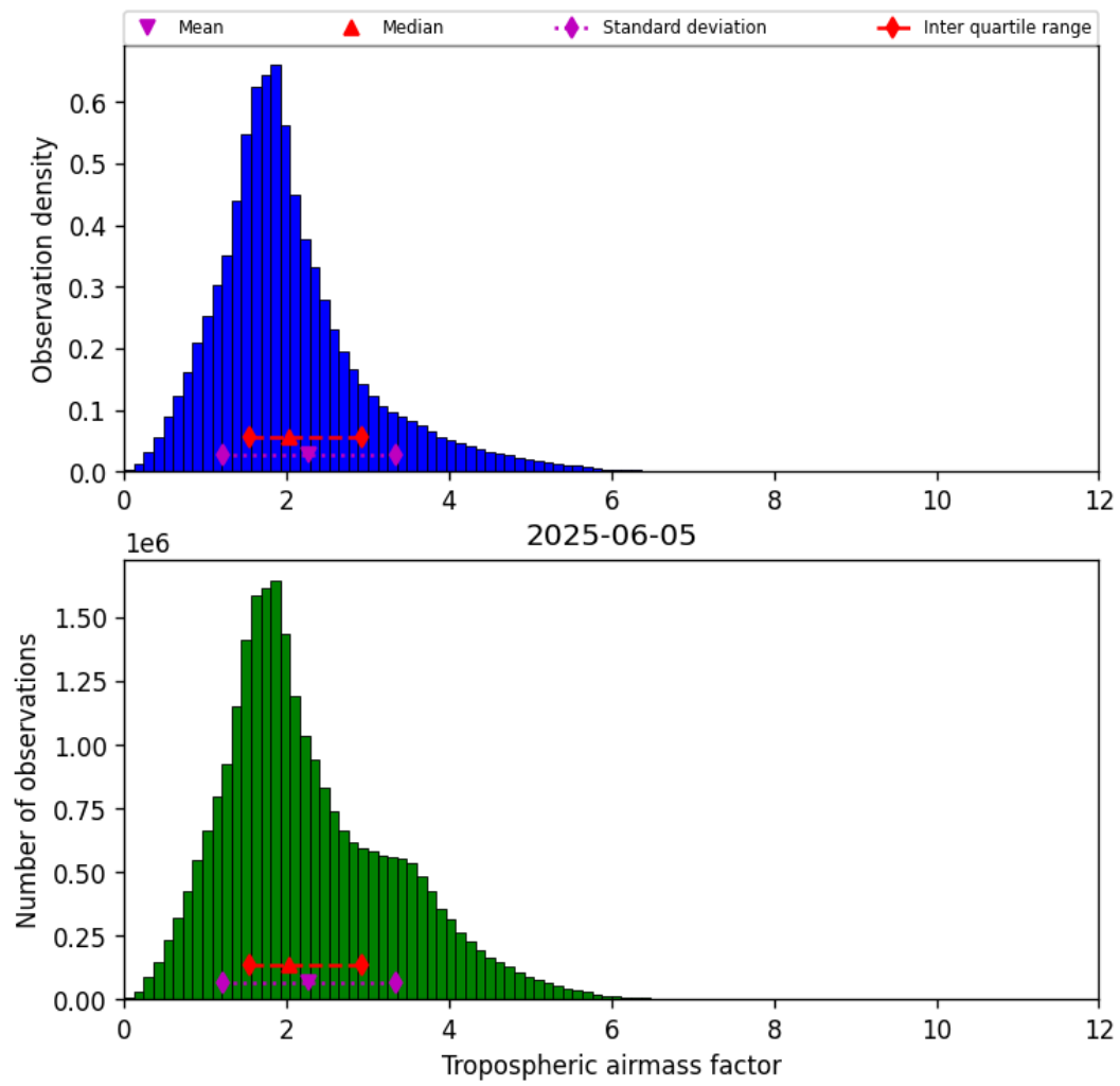
Figure 29: Histogram of “Tropospheric airmass factor” for 2025-06-05 to 2025-06-06
