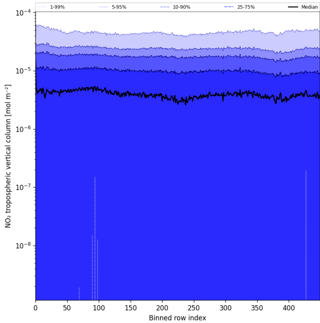
Figure 44: Along track statistics of “NO 2 tropospheric vertical column” for 2025-06-05 to 2025-06-06
