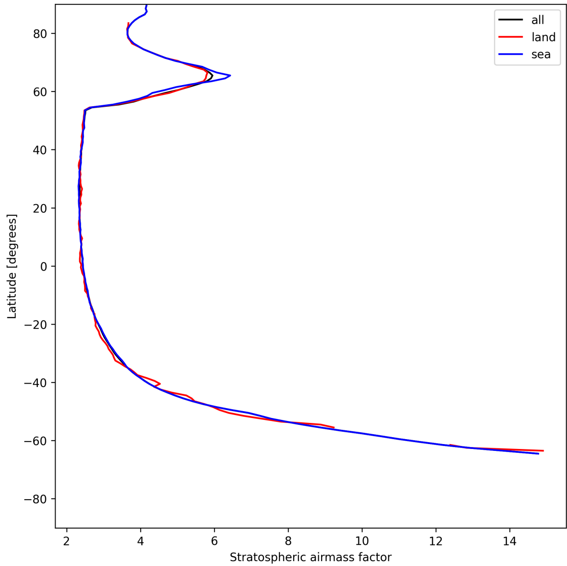
Figure 25: Zonal average of “Stratospheric air mass factor” for 2025-06-05 to 2025-06-06.
