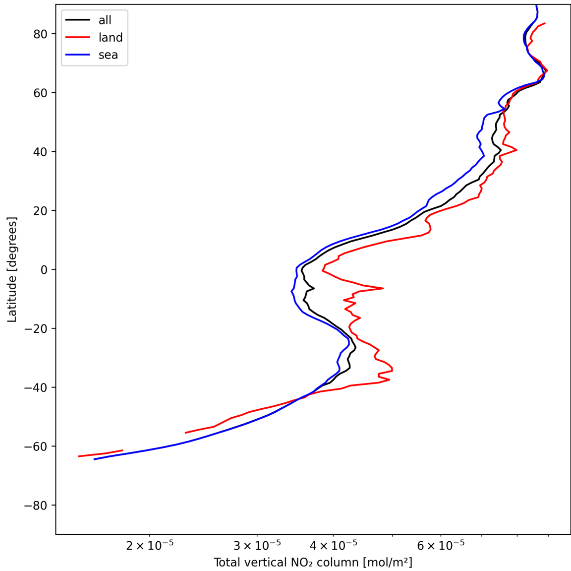
Figure 19: Zonal average of “Total vertical NO 2 column” for 2025-06-05 to 2025-06-06.
