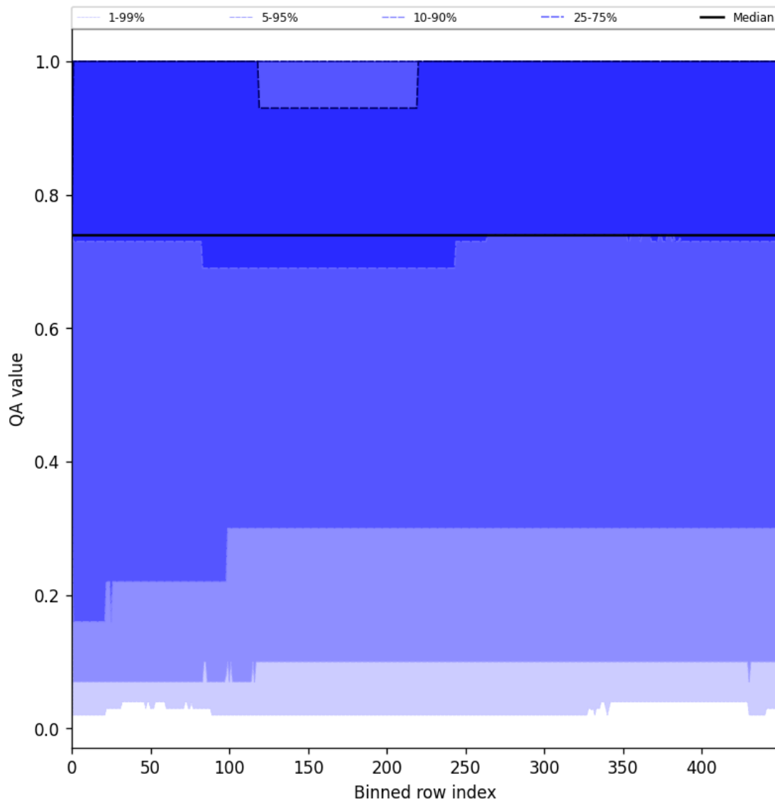
Figure 43: Along track statistics of “QA value” for 2025-06-05 to 2025-06-06
