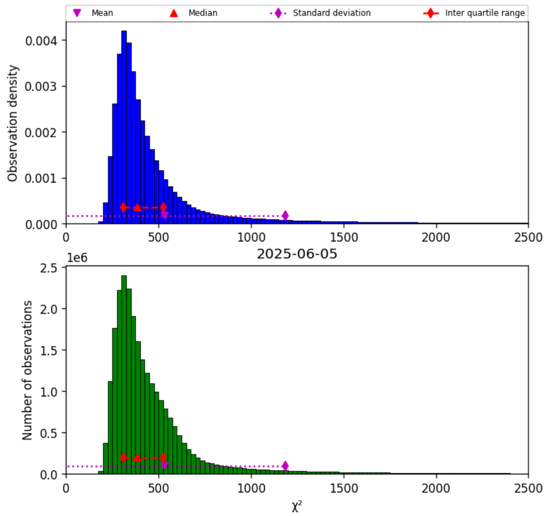
Figure 40: Histogram of " \chi^2 " for 2025-06-05 to 2025-06-06
