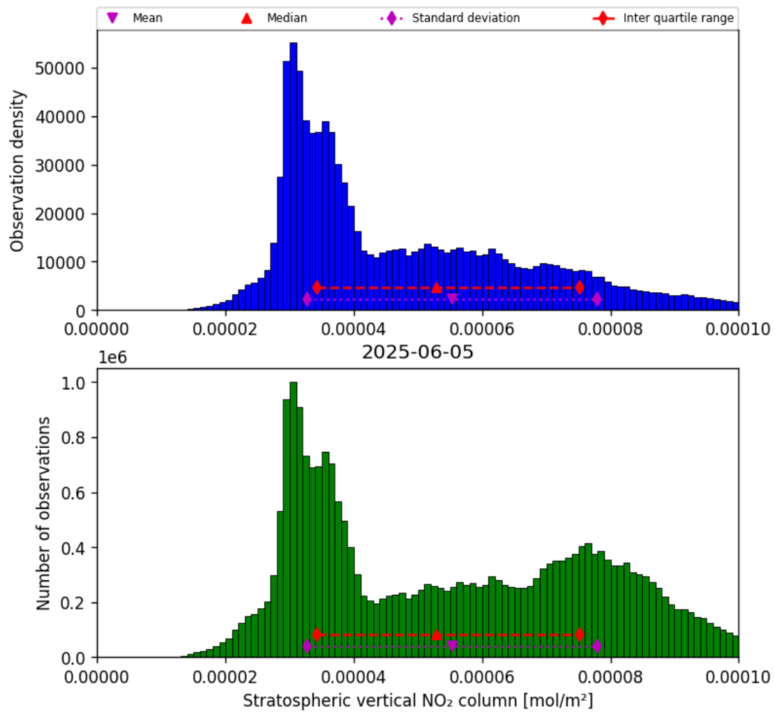
Figure 34: Histogram of “Stratospheric vertical NO 2 column” for 2025-06-05 to 2025-06-06
