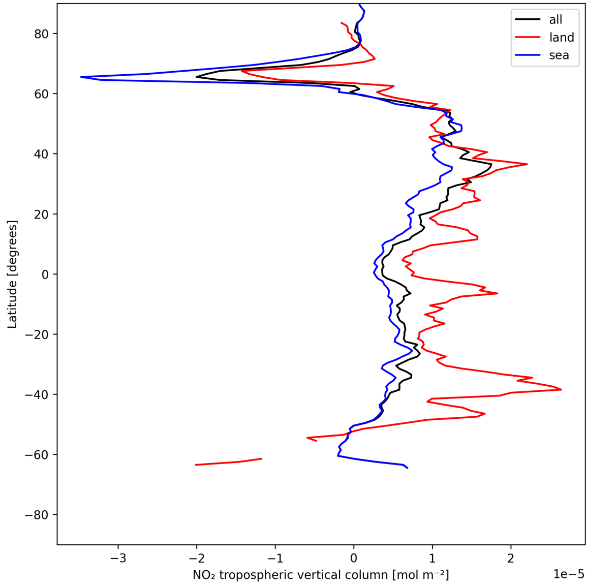
Figure 10: Zonal average of “NO 2 tropospheric vertical column” for 2025-06-05 to 2025-06-06.
