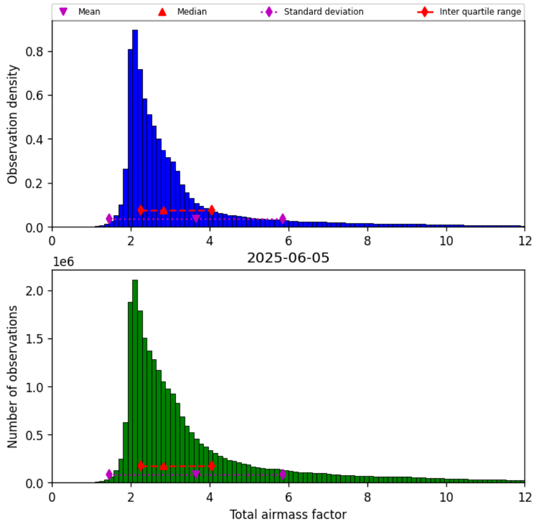
Figure 30: Histogram of “Total airmass factor” for 2025-06-05 to 2025-06-06
