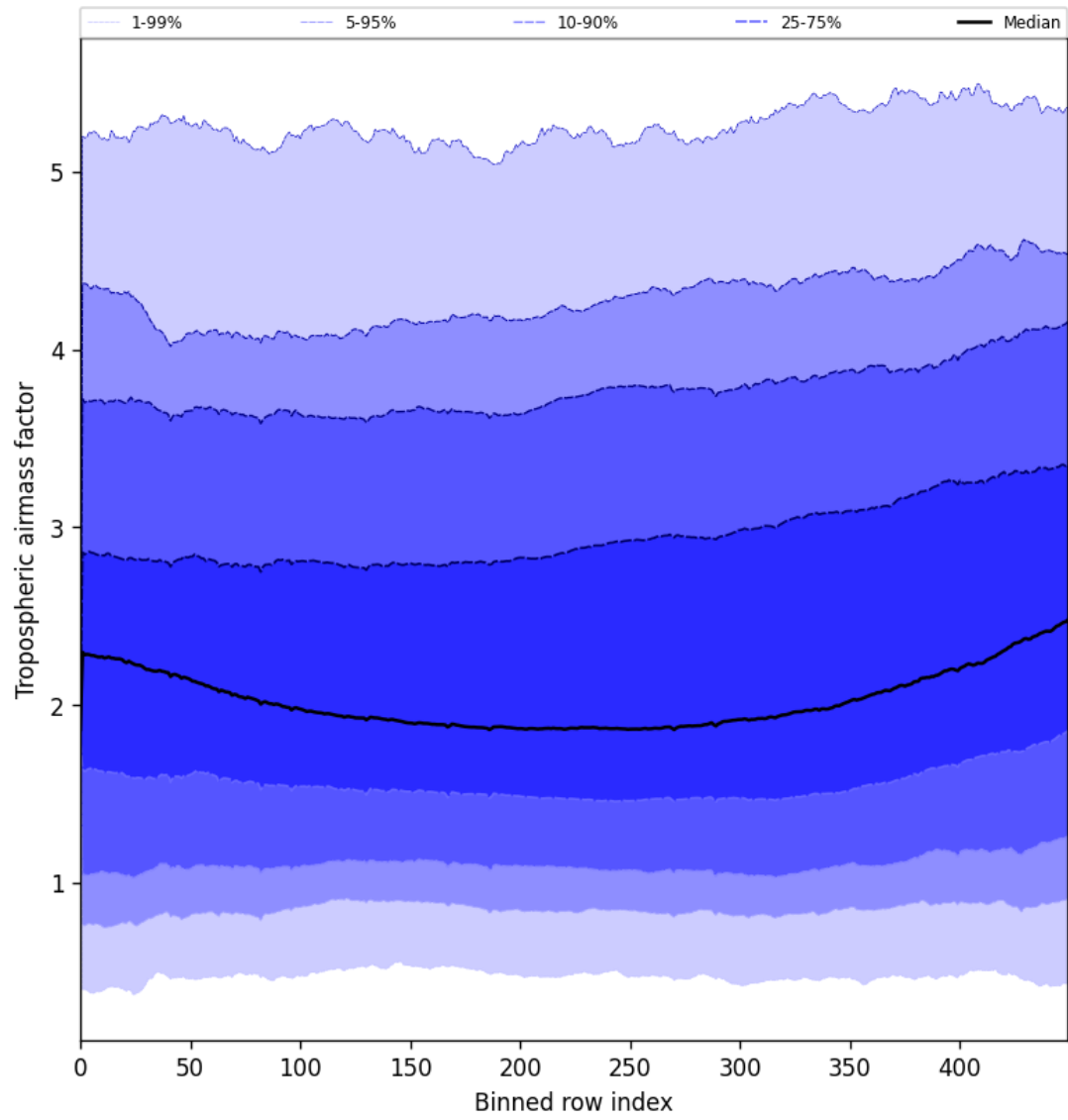
Figure 46: Along track statistics of “Tropospheric airmass factor” for 2025-06-05 to 2025-06-06
