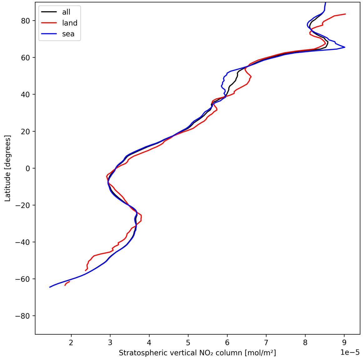
Figure 17: Zonal average of “Stratospheric vertical NO 2 column” for 2025-06-05 to 2025-06-06.
