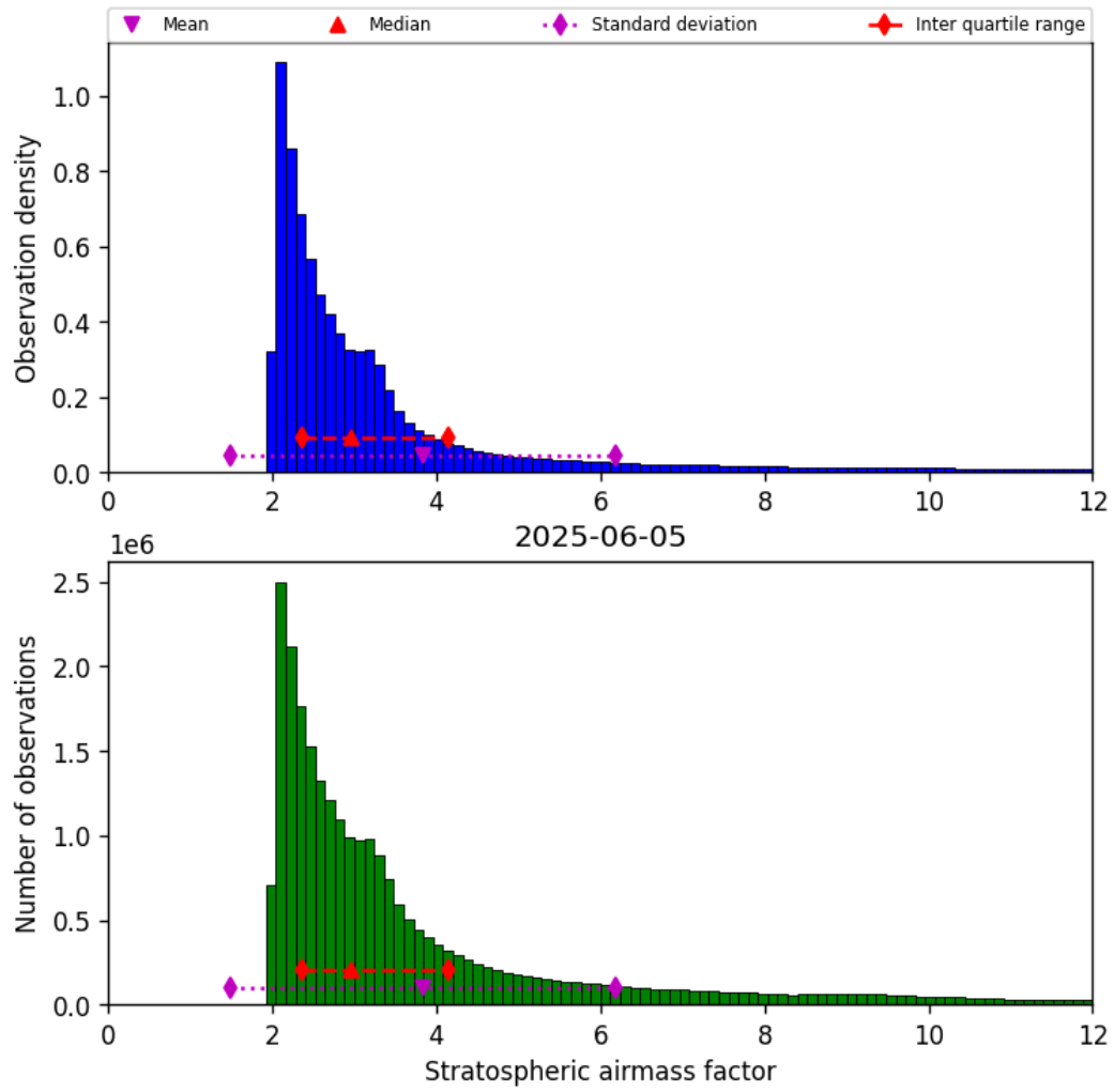
Figure 42: Histogram of “Stratospheric airmass factor” for 2025-06-05 to 2025-06-06
