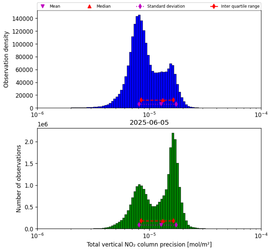
Figure 37: Histogram of “Total vertical NO 2 column precision” for 2025-06-05 to 2025-06-06
