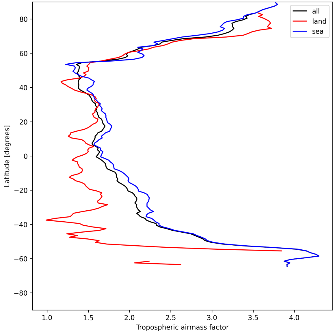
Figure 12: Zonal average of “Tropospheric air mass factor” for 2025-06-05 to 2025-06-06.
