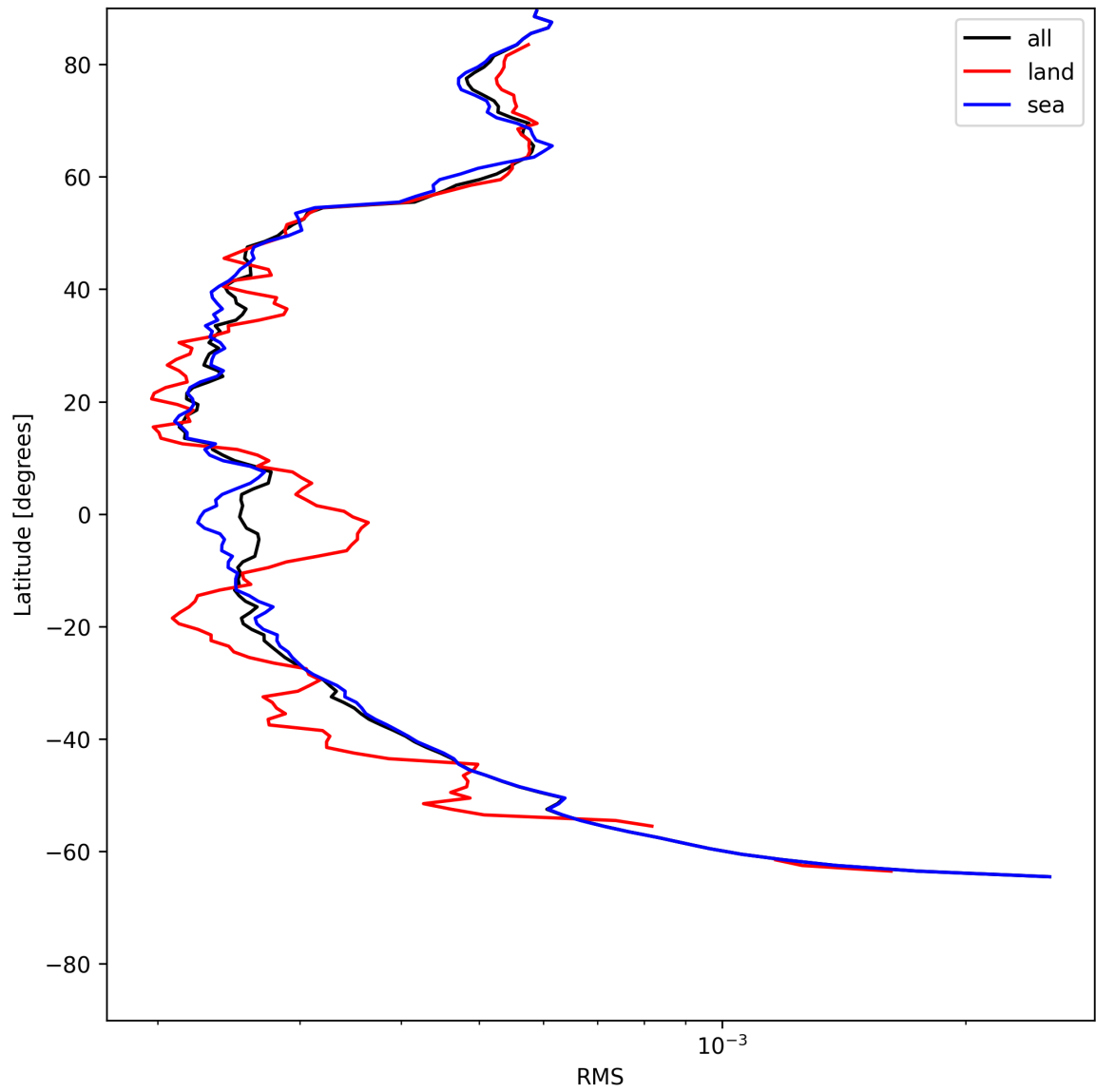
Figure 24: Zonal average of “RMS” for 2025-06-05 to 2025-06-06.
