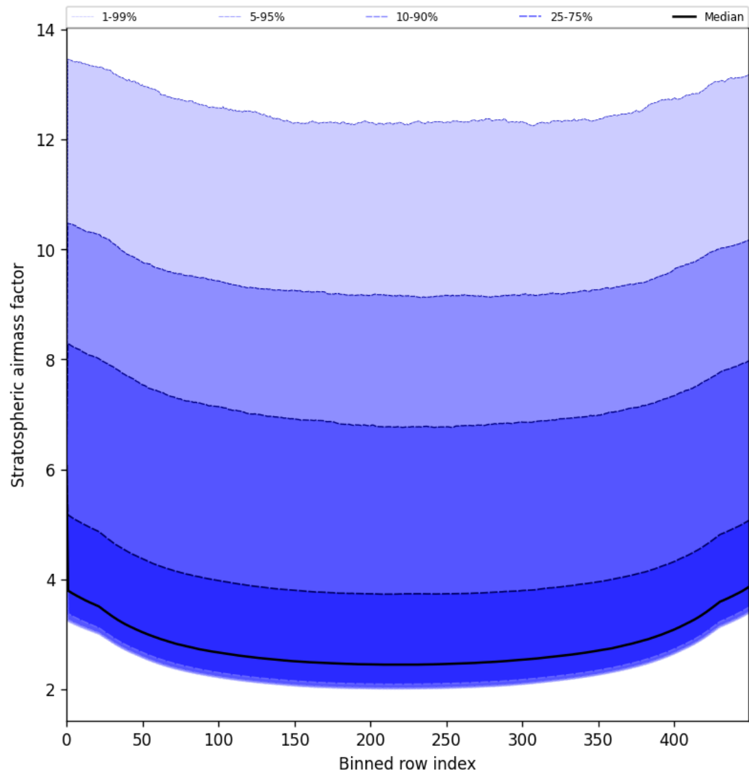
Figure 59: Along track statistics of “Stratospheric airmass factor” for 2025-06-05 to 2025-06-06
