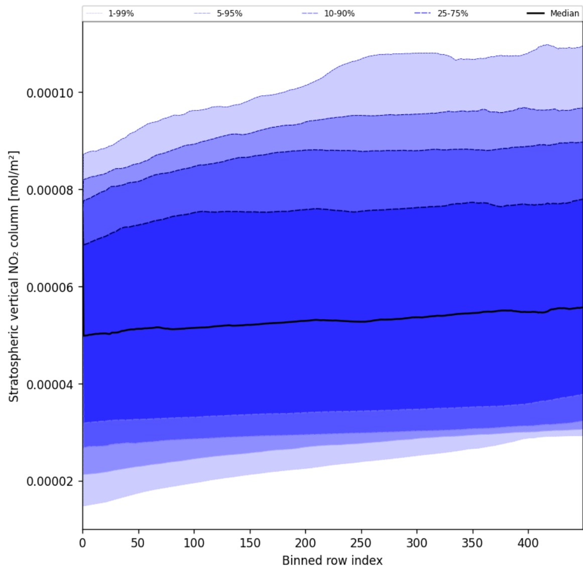
Figure 51: Along track statistics of “Stratospheric vertical NO 2 column” for 2025-06-05 to 2025-06-06
