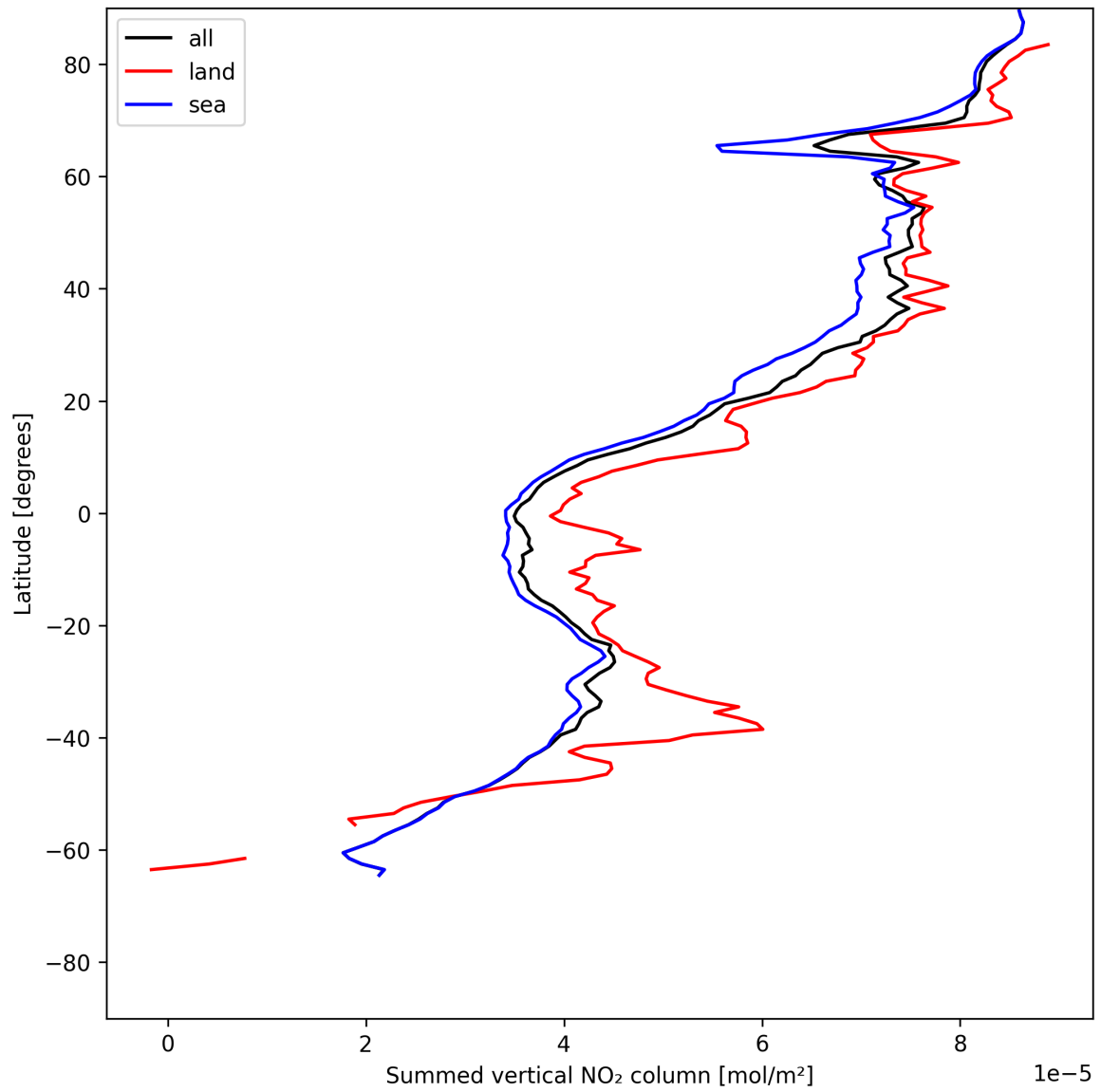
Figure 21: Zonal average of “Summed vertical NO 2 column” for 2025-06-05 to 2025-06-06.
