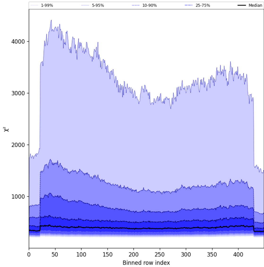
Figure 57: Along track statistics of “ \chi^2 ” for 2025-06-05 to 2025-06-06
