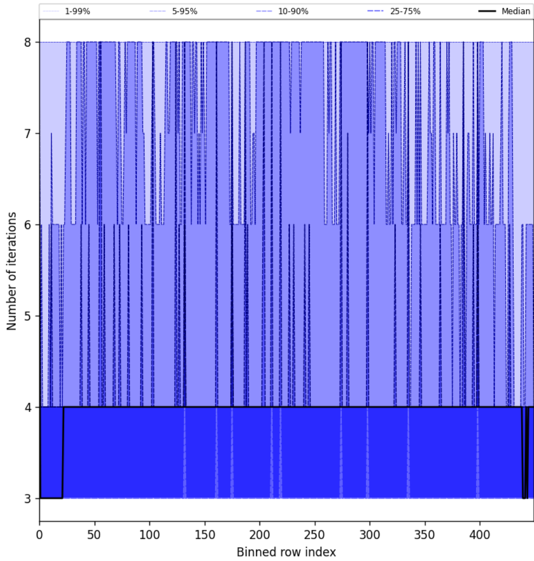
Figure 49: Along track statistics of “Number of iterations” for 2025-06-05 to 2025-06-06
