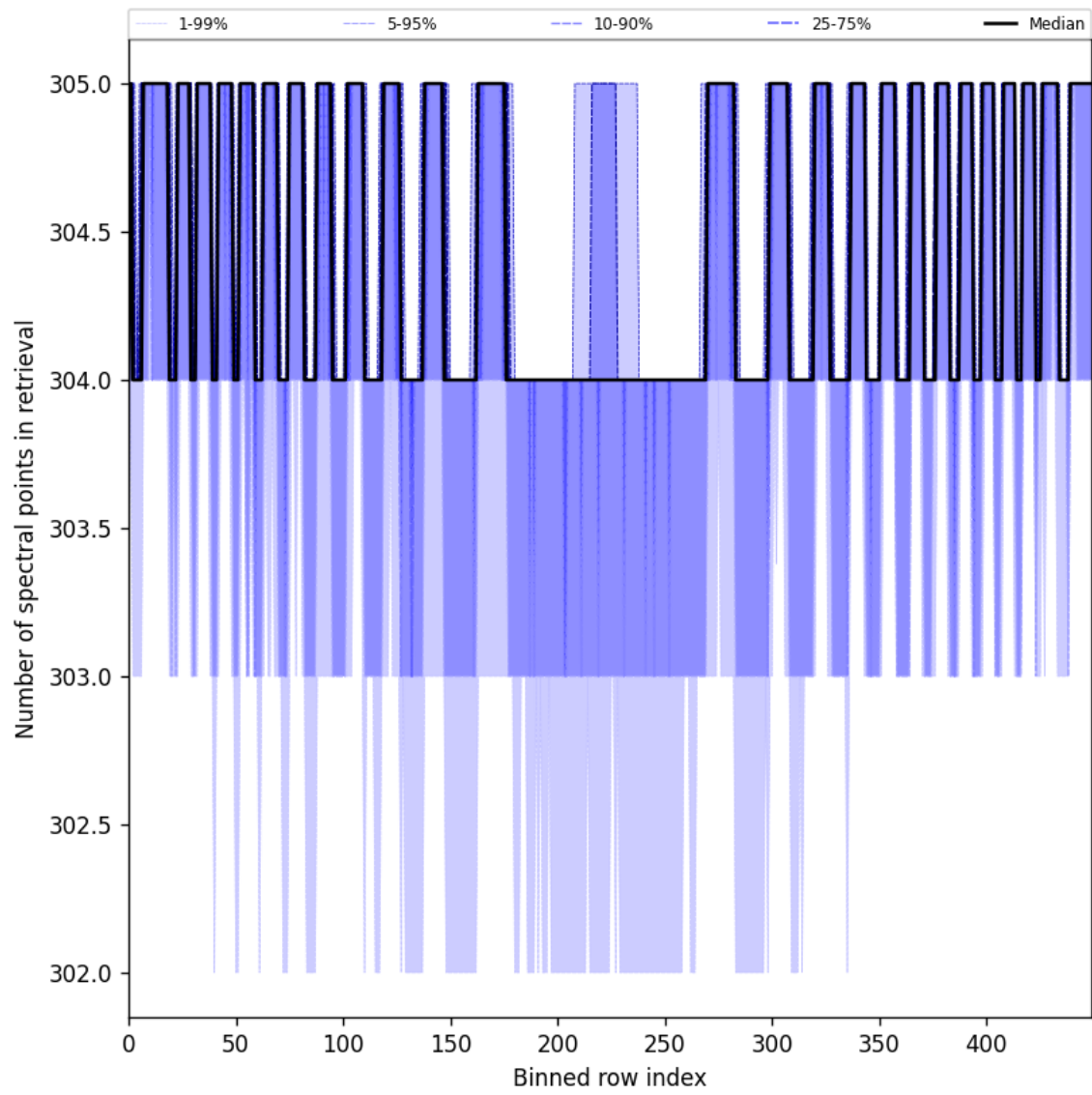
Figure 48: Along track statistics of “Number of spectral points in retrieval” for 2025-06-05 to 2025-06-06
