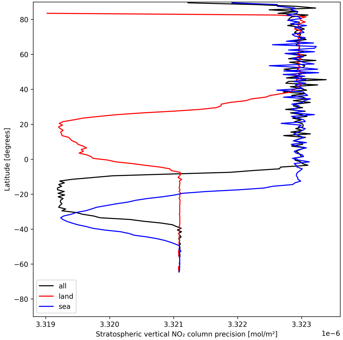
Figure 18: Zonal average of “Stratospheric vertical NO 2 column precision” for 2025-06-05 to 2025-06-06.
