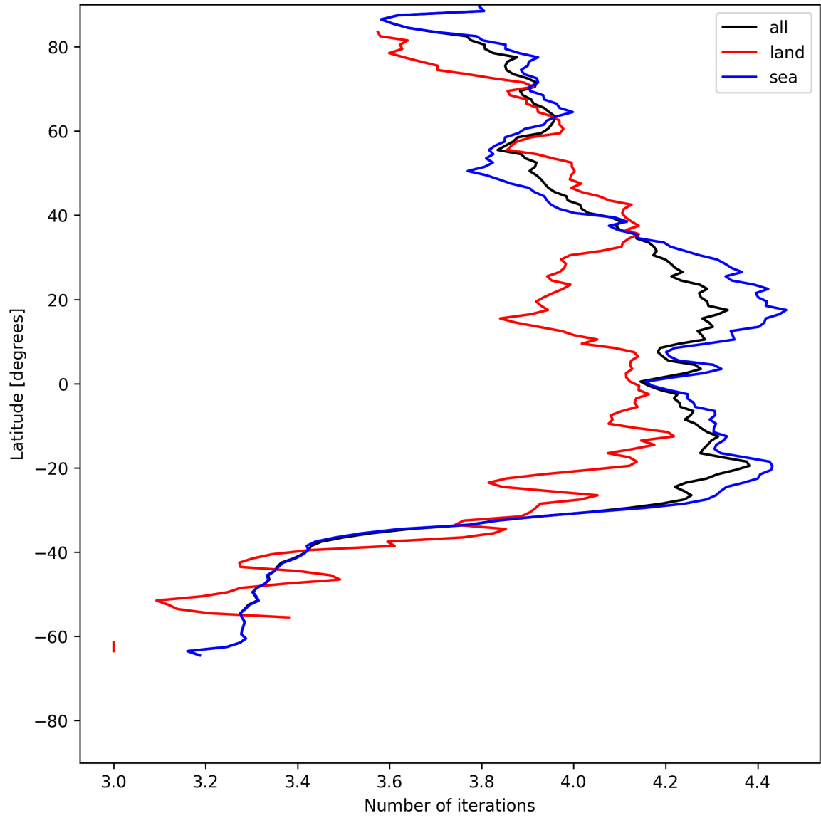
Figure 15: Zonal average of “Number of iterations” for 2025-06-05 to 2025-06-06.
