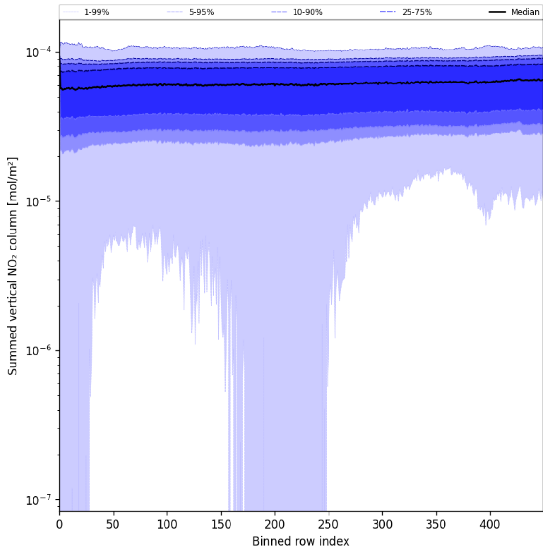
Figure 55: Along track statistics of “Summed vertical NO 2 column” for 2025-06-05 to 2025-06-06
