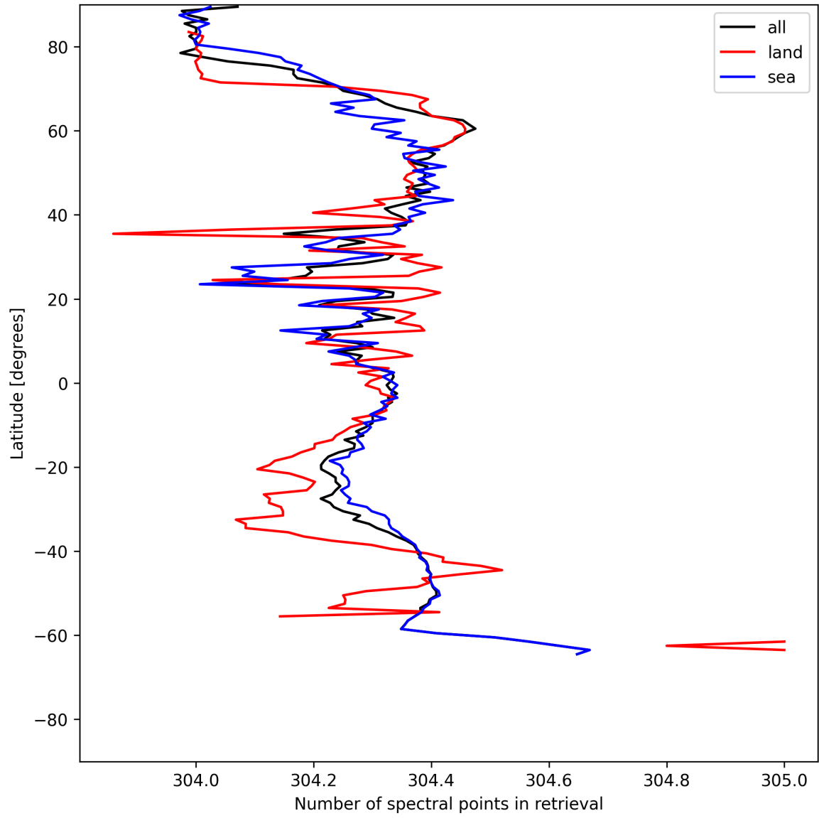
Figure 14: Zonal average of “Number of spectral points in retrieval” for 2025-06-05 to 2025-06-06.
