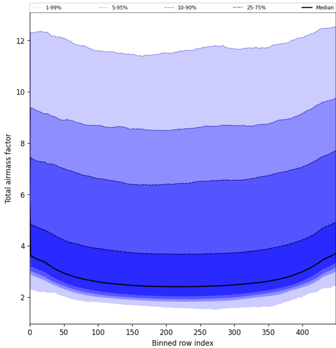
Figure 47: Along track statistics of “Total airmass factor” for 2025-06-05 to 2025-06-06
