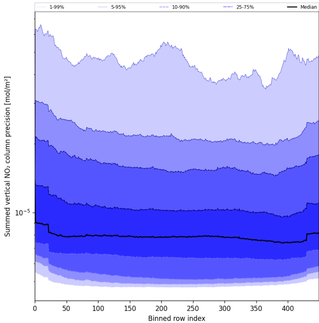
Figure 56: Along track statistics of “Summed vertical NO 2 column precision” for 2025-06-05 to 2025-06-06
