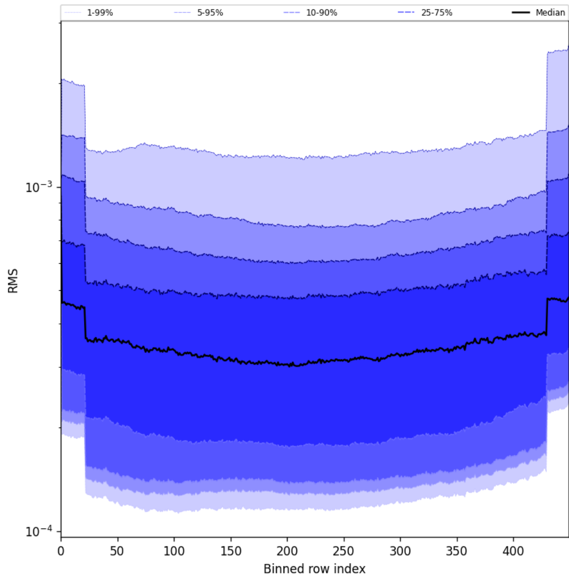
Figure 58: Along track statistics of “RMS” for 2025-06-05 to 2025-06-06
