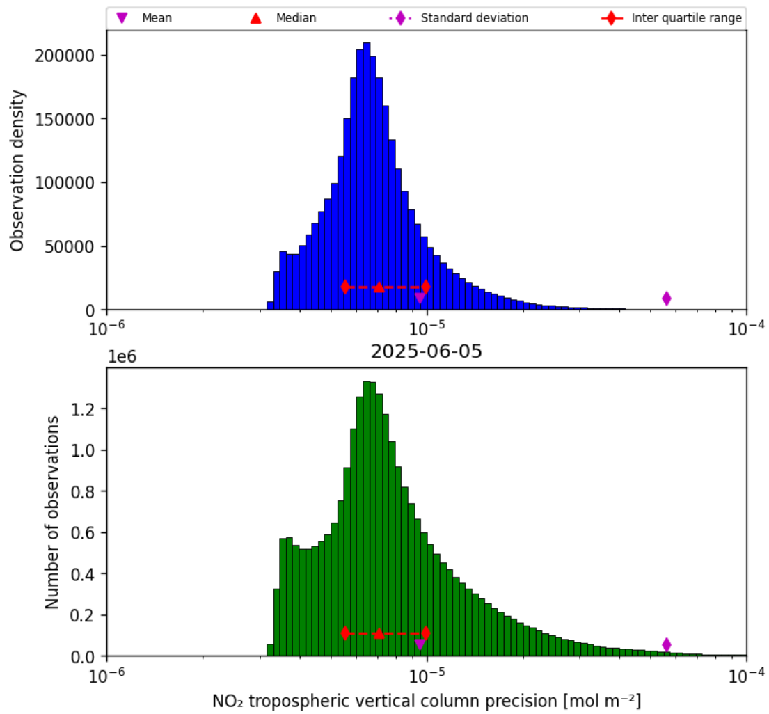
Figure 28: Histogram of “NO 2 tropospheric vertical column precision” for 2025-06-05 to 2025-06-06
