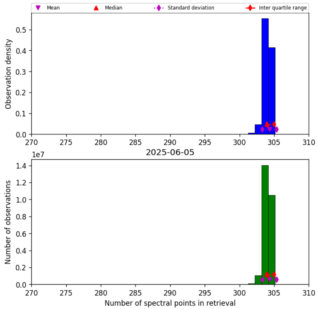
Figure 31: Histogram of “Number of spectral points in retrieval” for 2025-06-05 to 2025-06-06
