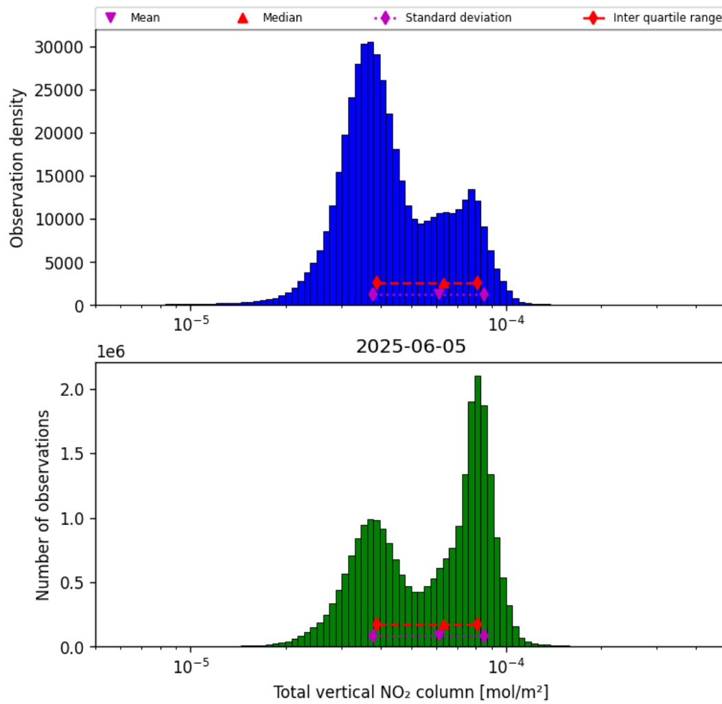
Figure 36: Histogram of “Total vertical NO 2 column” for 2025-06-05 to 2025-06-06
