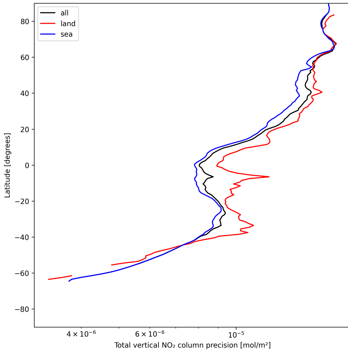
Figure 20: Zonal average of “Total vertical NO 2 column precision” for 2025-06-05 to 2025-06-06.
