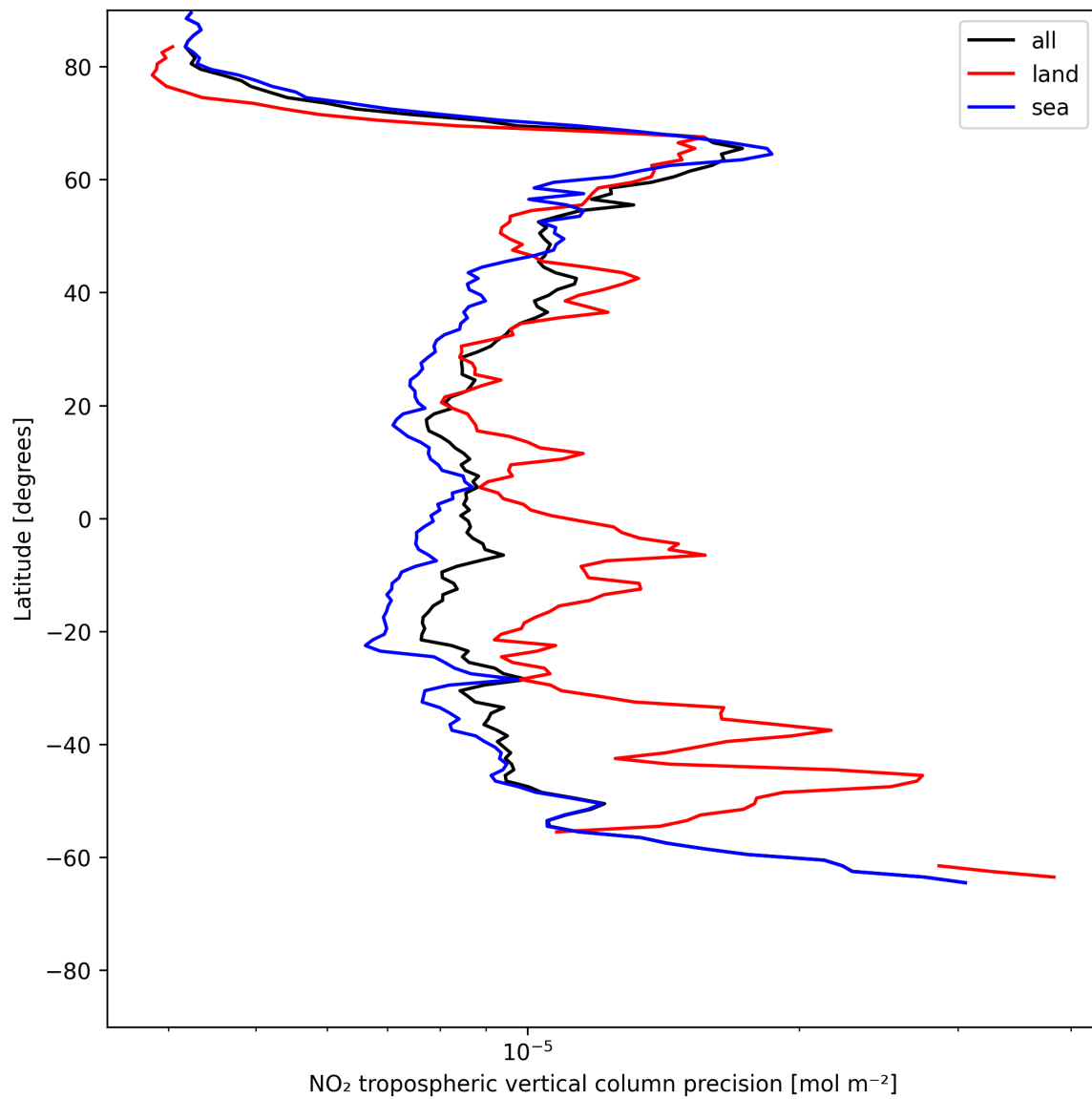
Figure 11: Zonal average of “NO 2 tropospheric vertical column precision” for 2025-06-05 to 2025-06-06.
