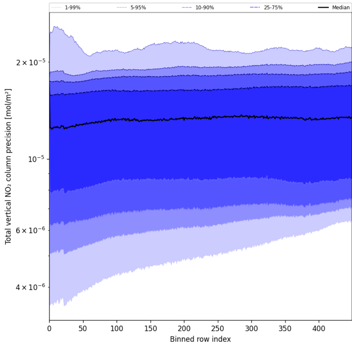
Figure 54: Along track statistics of “Total vertical NO 2 column precision” for 2025-06-05 to 2025-06-06
