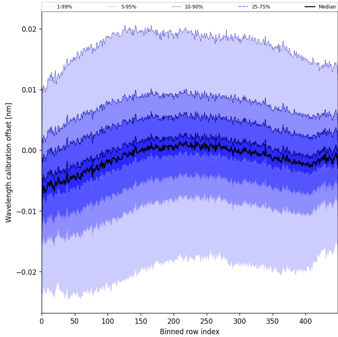
Figure 50: Along track statistics of “Wavelength calibration offset” for 2025-06-05 to 2025-06-06
