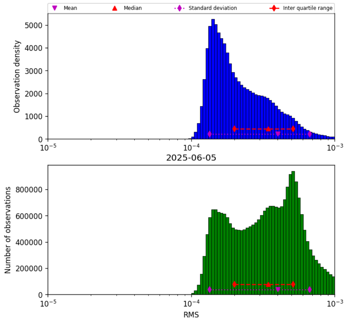
Figure 41: Histogram of “RMS” for 2025-06-05 to 2025-06-06
