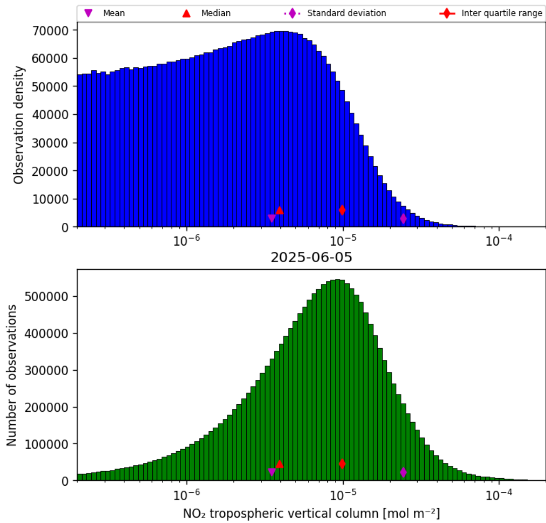
Figure 27: Histogram of “NO 2 tropospheric vertical column” for 2025-06-05 to 2025-06-06
