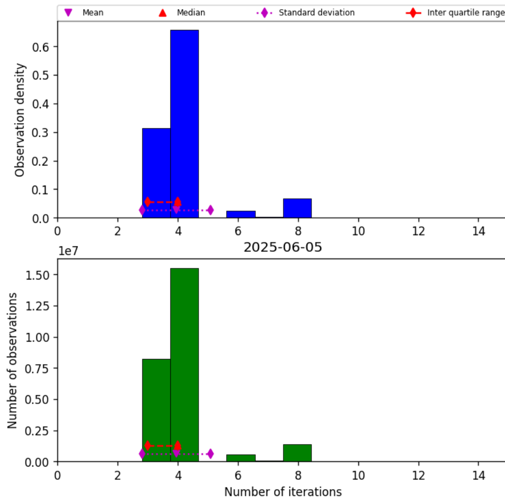
Figure 32: Histogram of “Number of iterations” for 2025-06-05 to 2025-06-06
