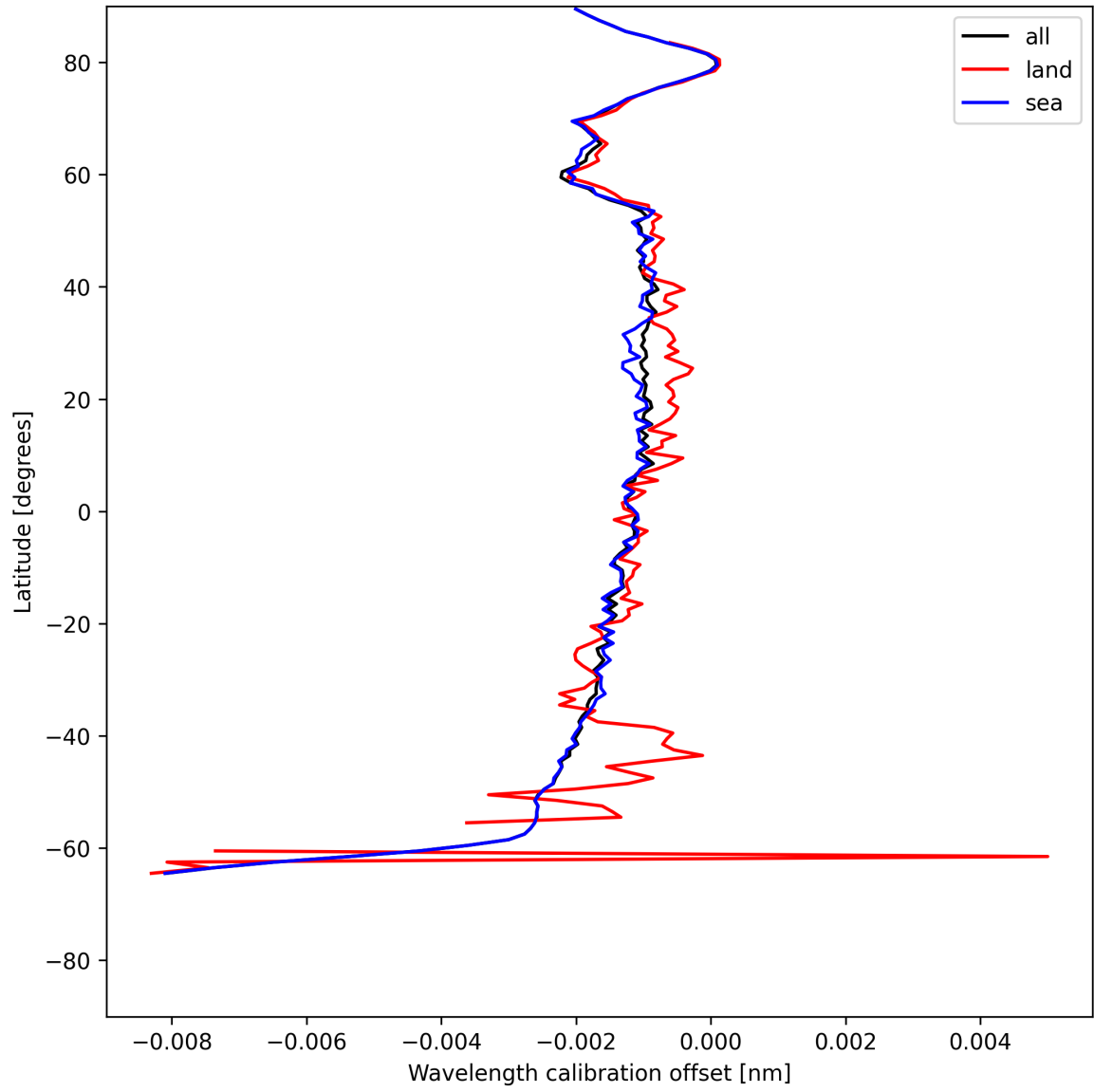
Figure 16: Zonal average of “Wavelength calibration offset” for 2025-06-07 to 2025-06-08.
