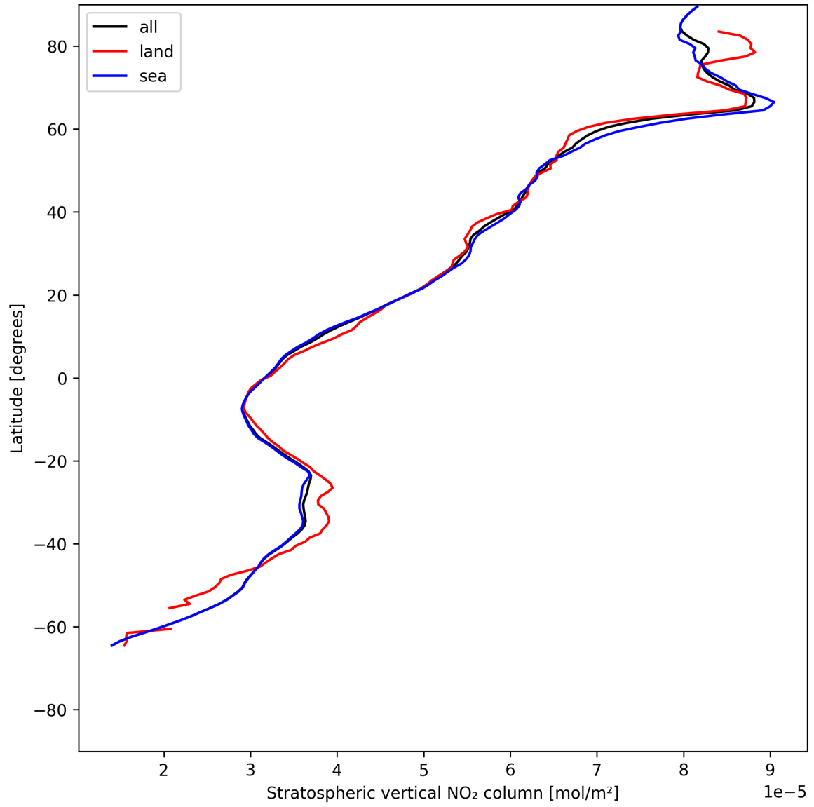
Figure 17: Zonal average of “Stratospheric vertical NO 2 column” for 2025-06-07 to 2025-06-08.
