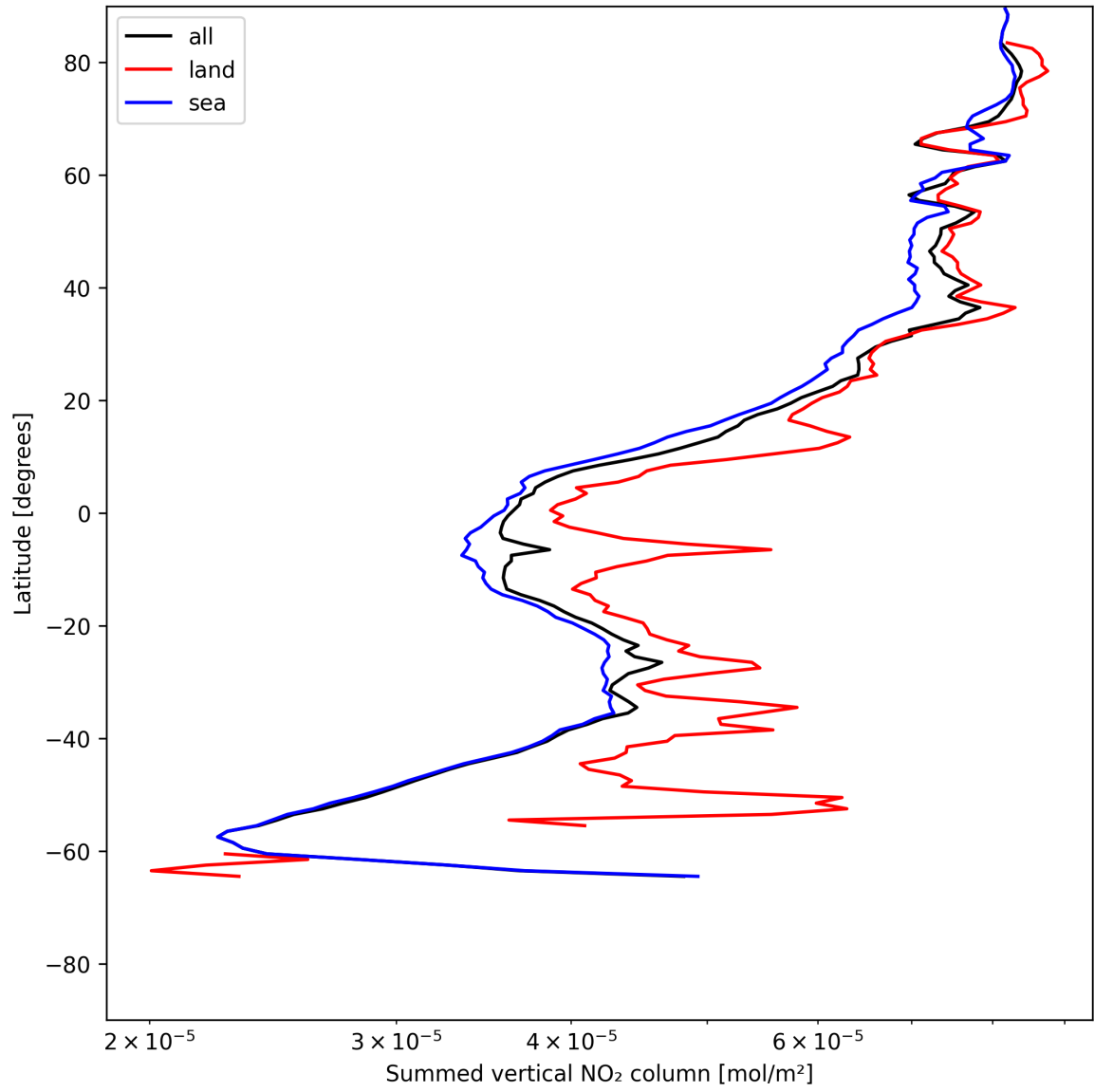
Figure 21: Zonal average of “Summed vertical NO 2 column” for 2025-06-07 to 2025-06-08.
