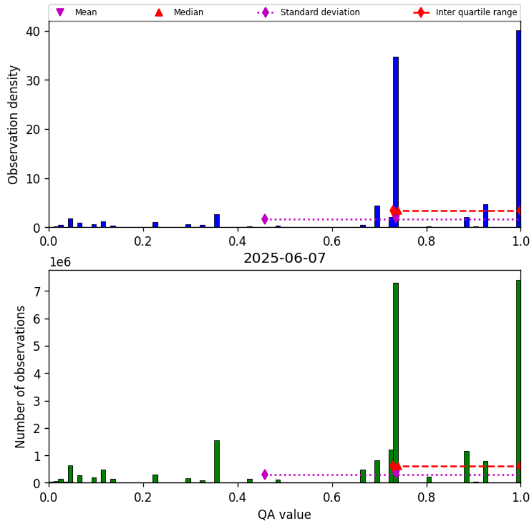
Figure 26: Histogram of “QA value” for 2025-06-07 to 2025-06-08
