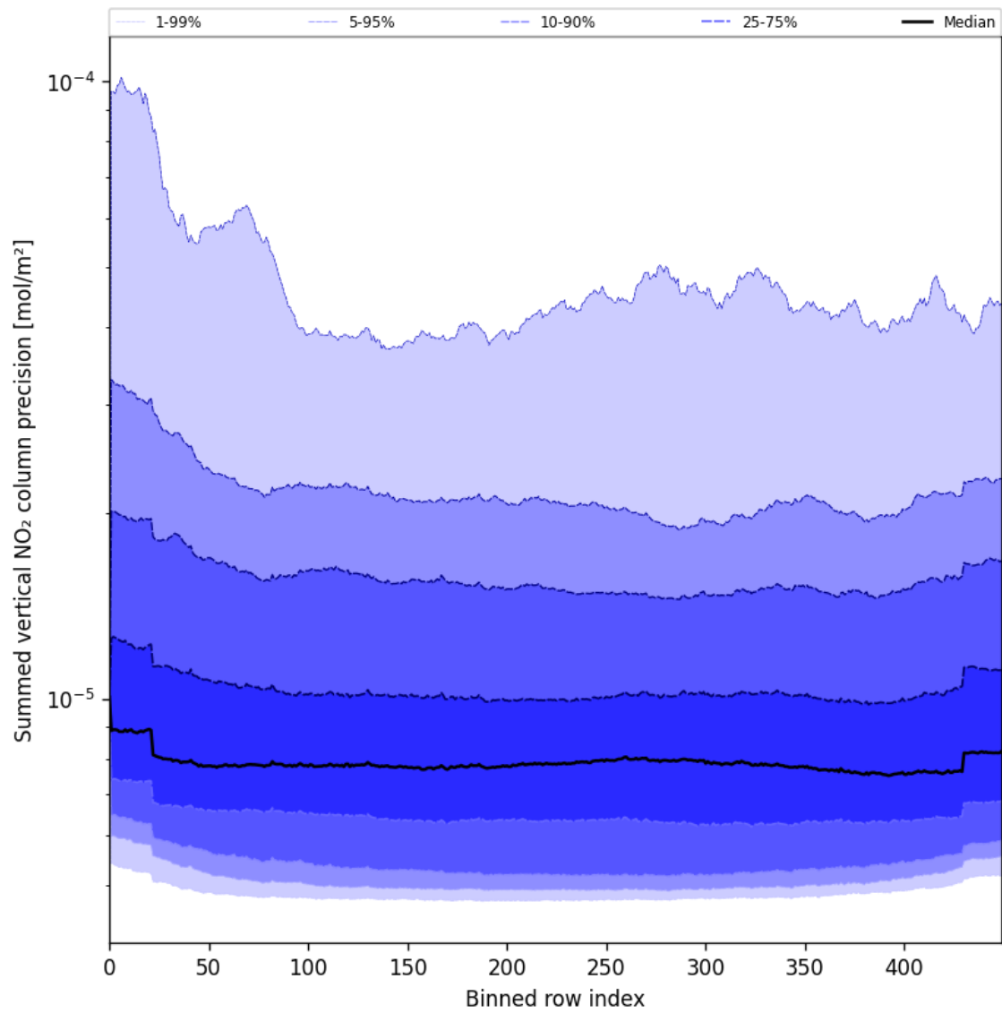
Figure 56: Along track statistics of “Summed vertical NO 2 column precision” for 2025-06-07 to 2025-06-08
