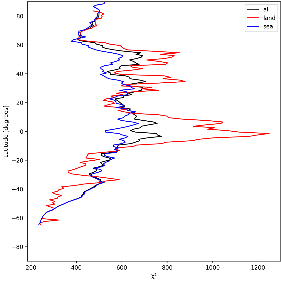
Figure 23: Zonal average of “ \chi^2 ” for 2025-06-07 to 2025-06-08.
