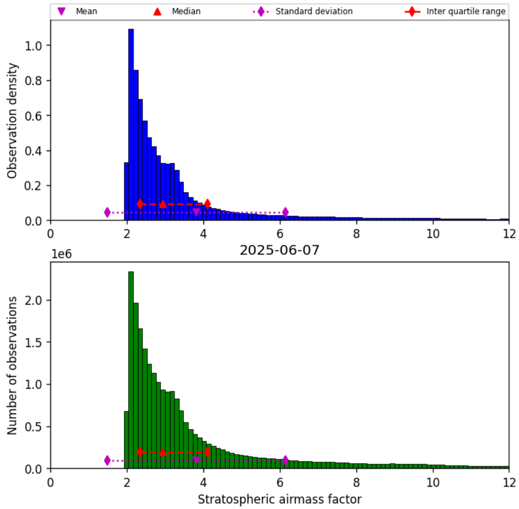
Figure 42: Histogram of “Stratospheric airmass factor” for 2025-06-07 to 2025-06-08
