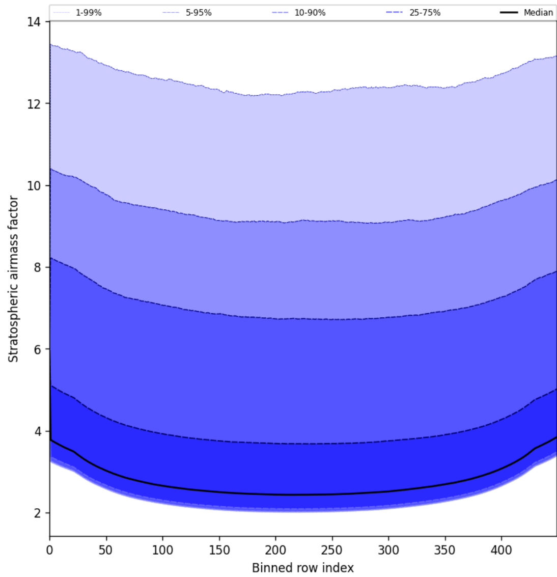
Figure 59: Along track statistics of “Stratospheric airmass factor” for 2025-06-07 to 2025-06-08
