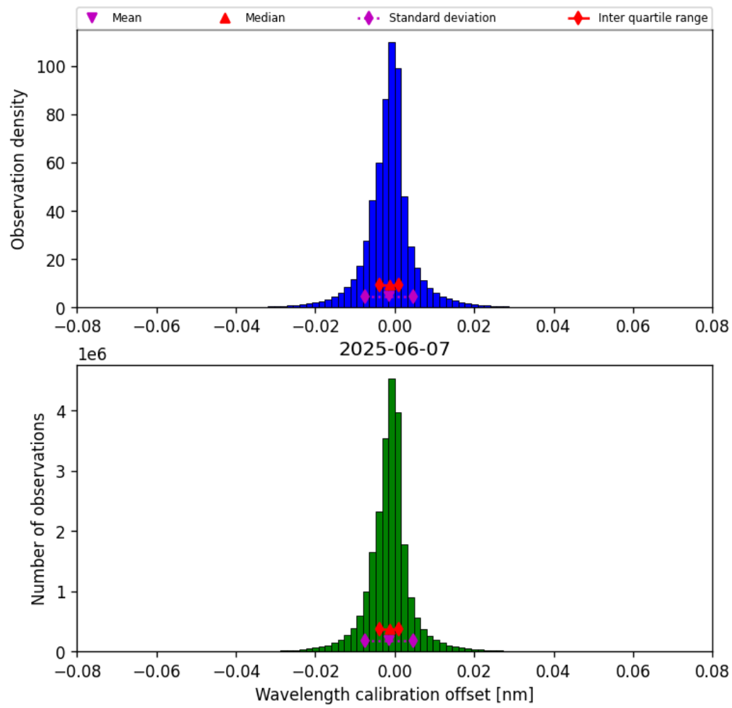
Figure 33: Histogram of “Wavelength calibration offset” for 2025-06-07 to 2025-06-08
