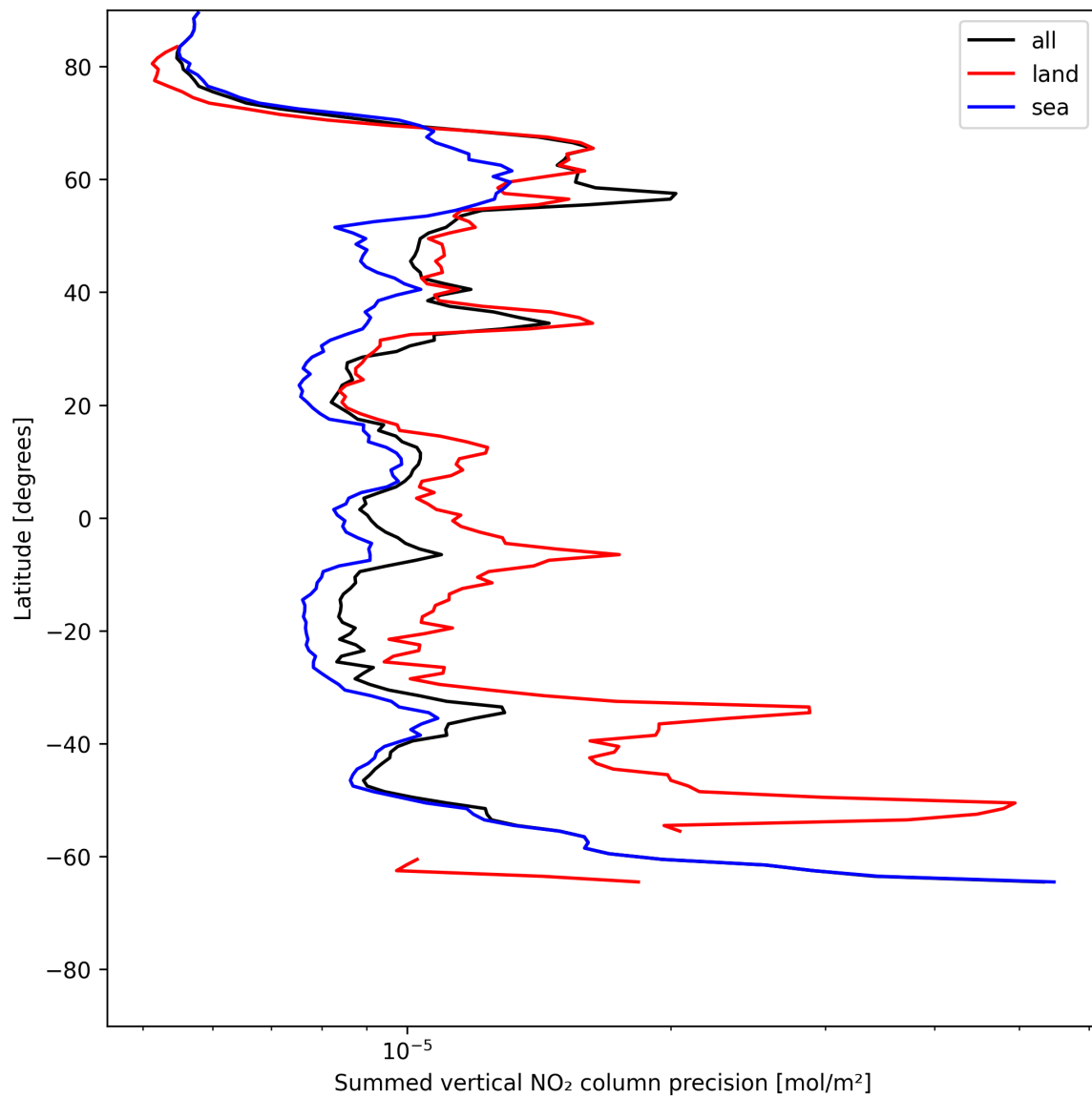
Figure 22: Zonal average of “Summed vertical NO 2 column precision” for 2025-06-07 to 2025-06-08.
