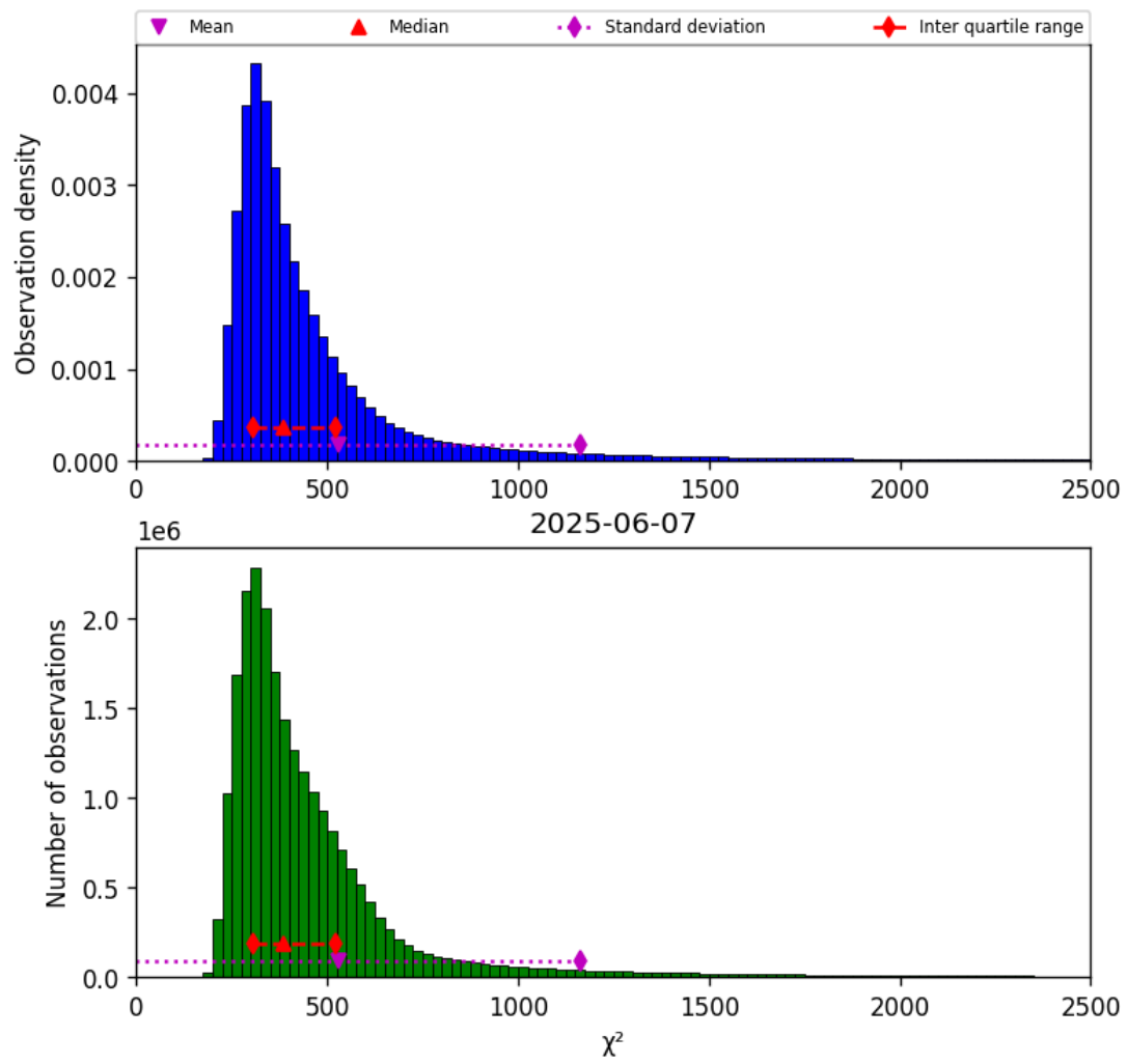
Figure 40: Histogram of " \chi^2 " for 2025-06-07 to 2025-06-08
