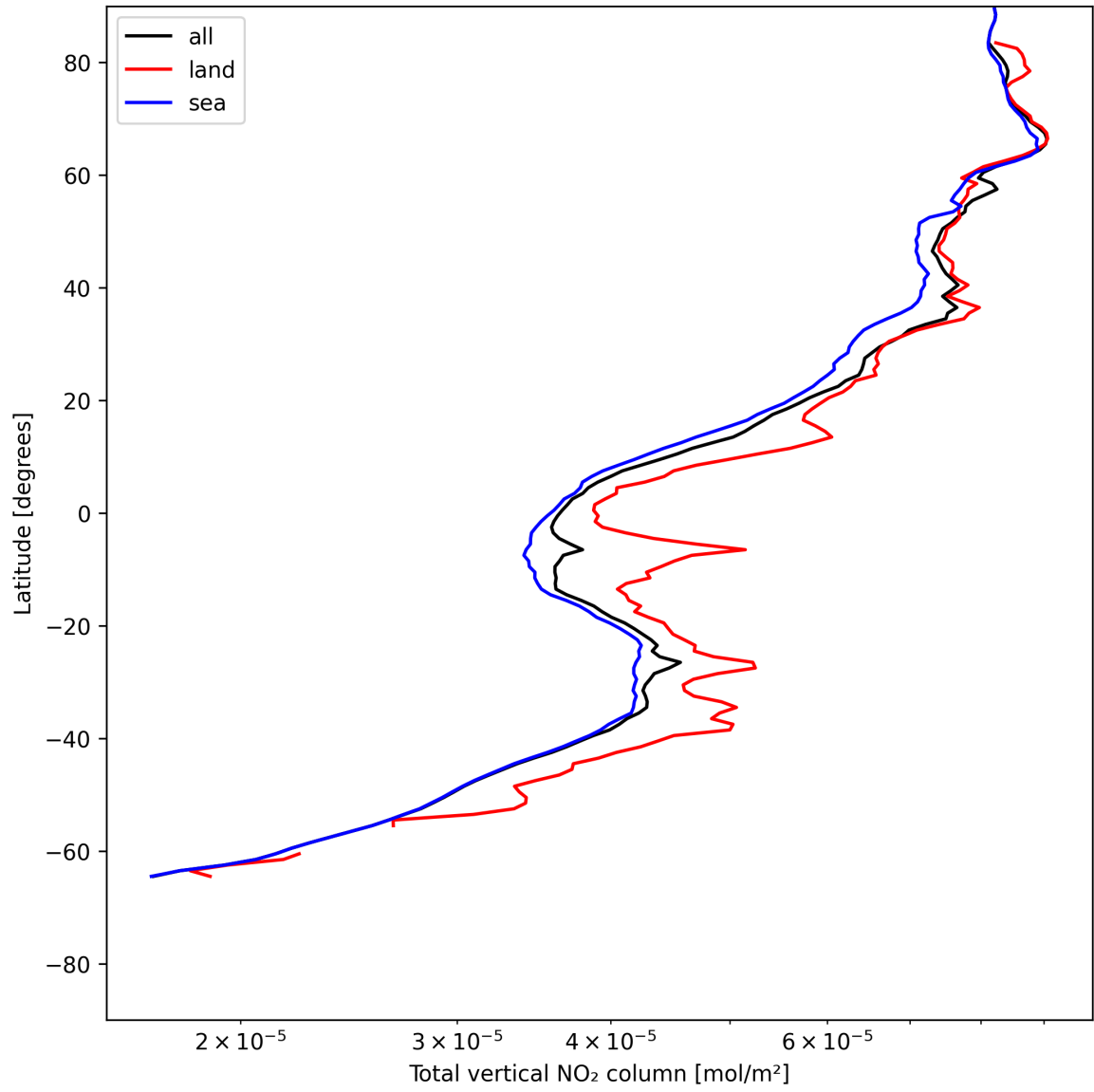
Figure 19: Zonal average of “Total vertical NO 2 column” for 2025-06-07 to 2025-06-08.
