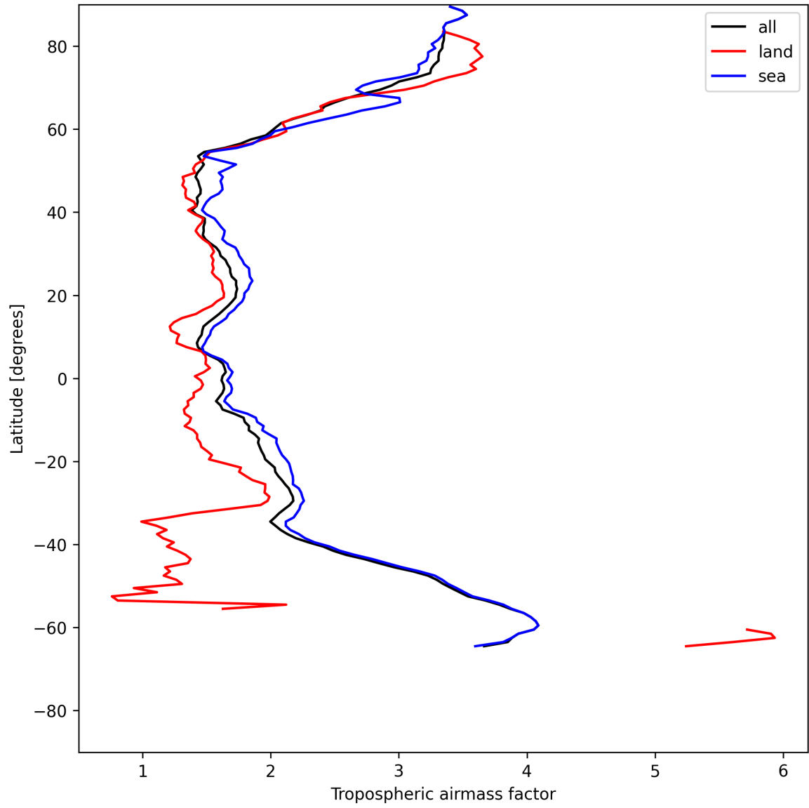
Figure 12: Zonal average of “Tropospheric airmass factor” for 2025-06-07 to 2025-06-08.
