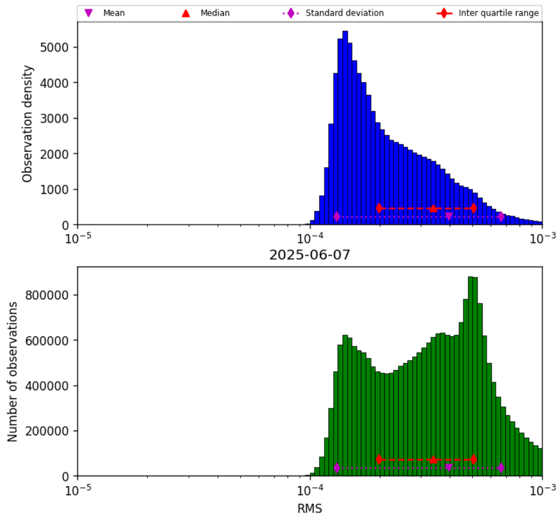
Figure 41: Histogram of “RMS” for 2025-06-07 to 2025-06-08
