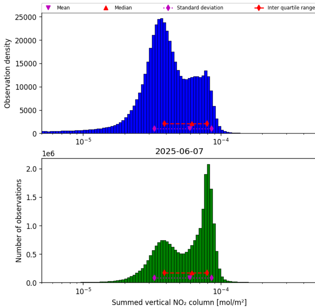
Figure 38: Histogram of “Summed vertical NO 2 column” for 2025-06-07 to 2025-06-08
