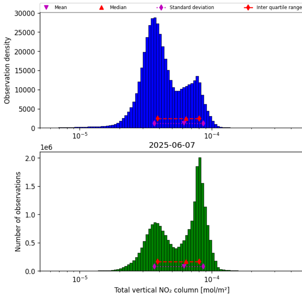
Figure 36: Histogram of “Total vertical NO 2 column” for 2025-06-07 to 2025-06-08
