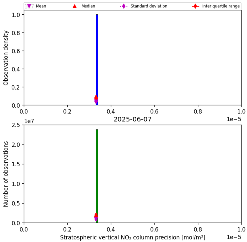
Figure 35: Histogram of “Stratospheric vertical NO 2 column precision” for 2025-06-07 to 2025-06-08
