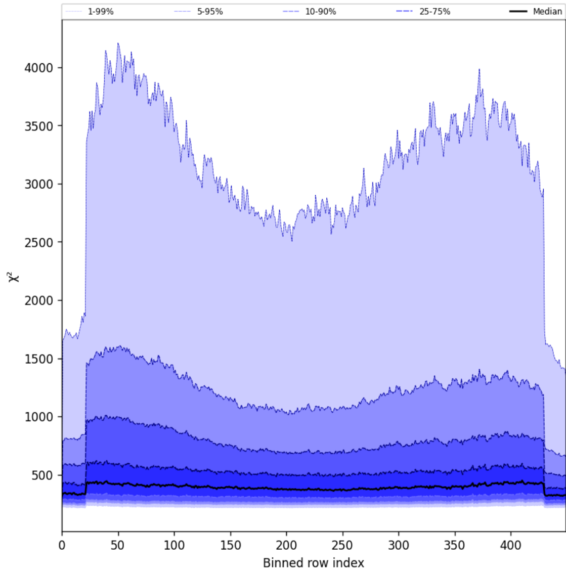
Figure 57: Along track statistics of “ \chi^2 ” for 2025-06-07 to 2025-06-08
