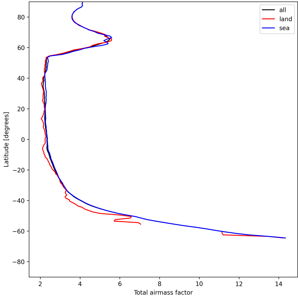
Figure 13: Zonal average of “Total airmass factor” for 2025-06-07 to 2025-06-08.
