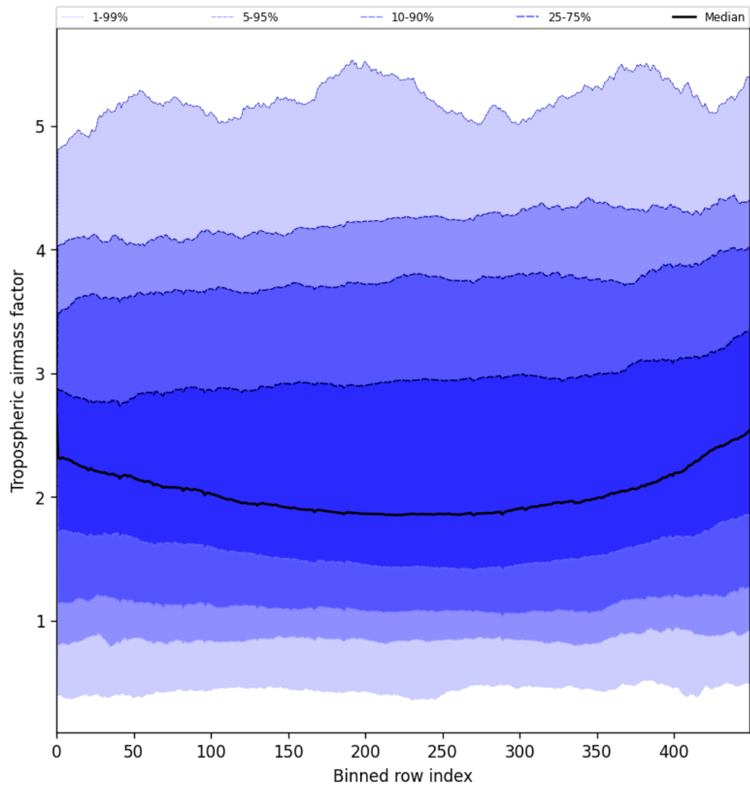
Figure 46: Along track statistics of “Tropospheric airmass factor” for 2025-06-07 to 2025-06-08
