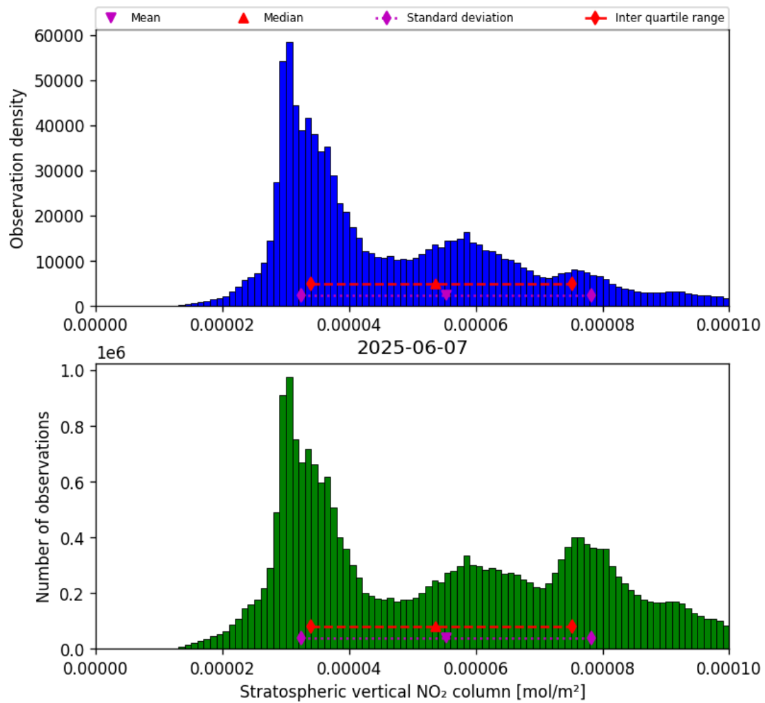
Figure 34: Histogram of “Stratospheric vertical NO 2 column” for 2025-06-07 to 2025-06-08
