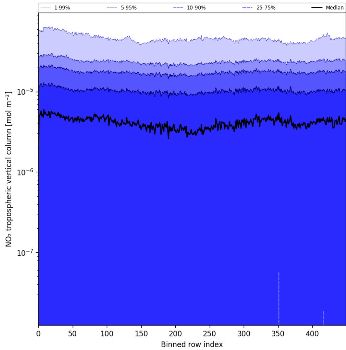
Figure 44: Along track statistics of "NO 2 tropospheric vertical column" for 2025-06-07 to 2025-06-08
