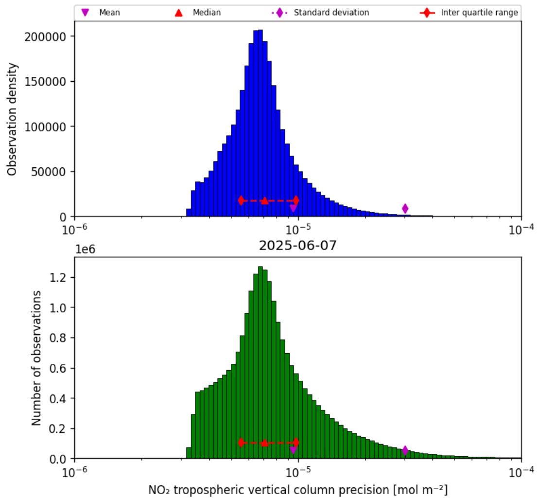
Figure 28: Histogram of “NO 2 tropospheric vertical column precision” for 2025-06-07 to 2025-06-08
