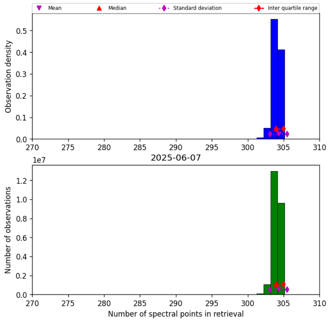
Figure 31: Histogram of “Number of spectral points in retrieval” for 2025-06-07 to 2025-06-08
