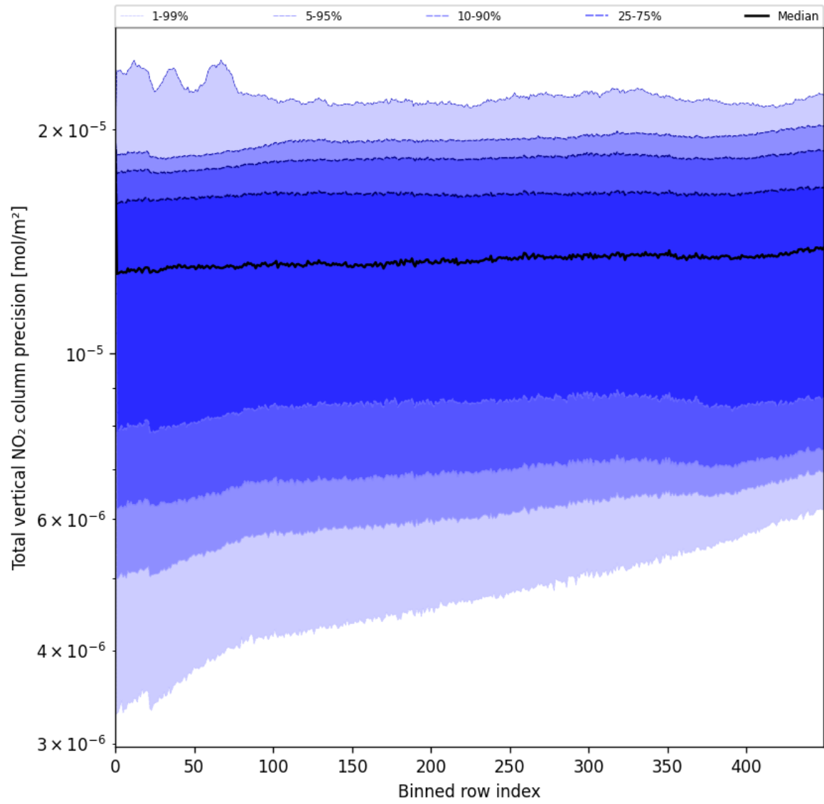
Figure 54: Along track statistics of “Total vertical NO 2 column precision” for 2025-06-07 to 2025-06-08
