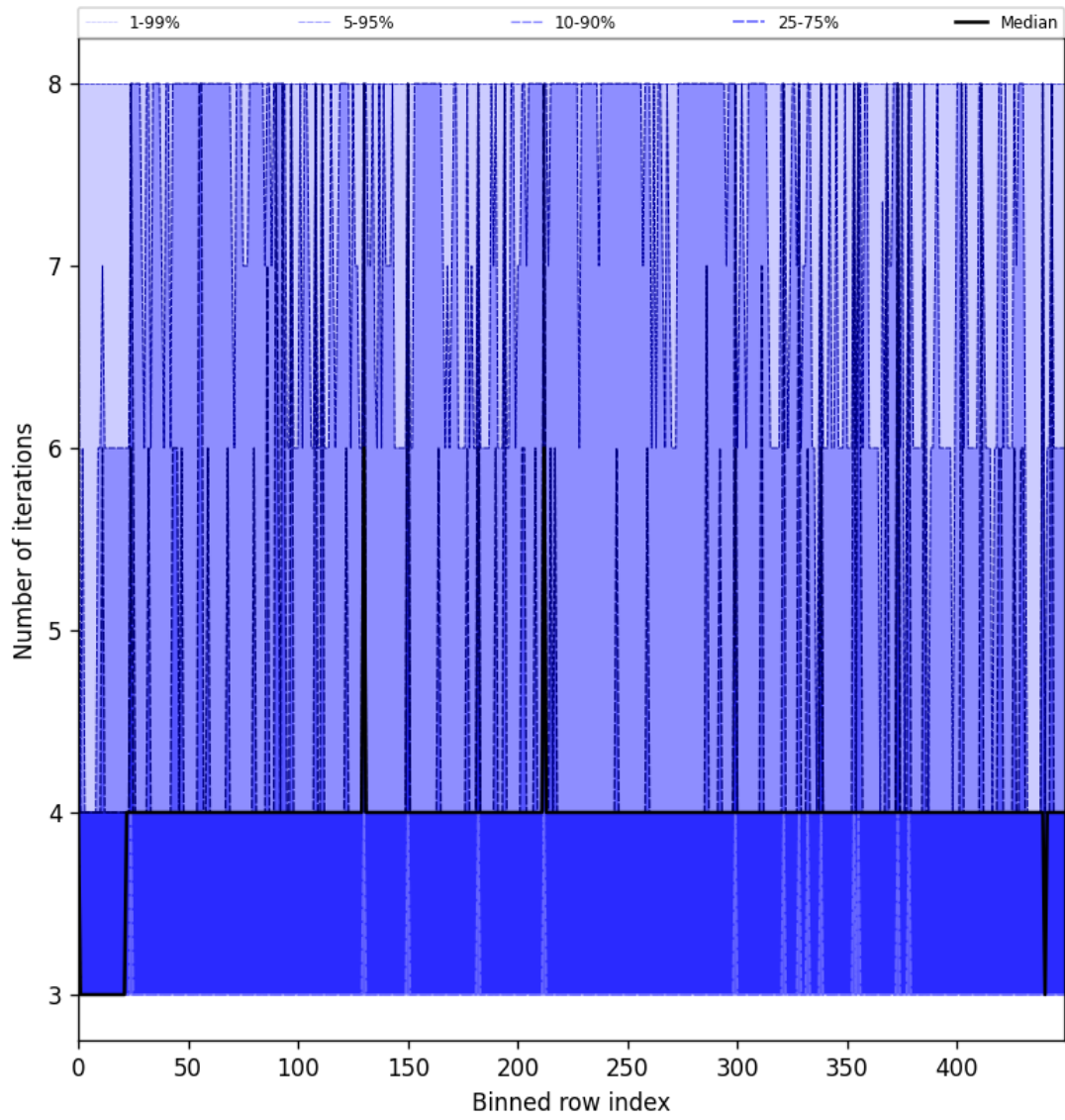
Figure 49: Along track statistics of “Number of iterations” for 2025-06-07 to 2025-06-08
