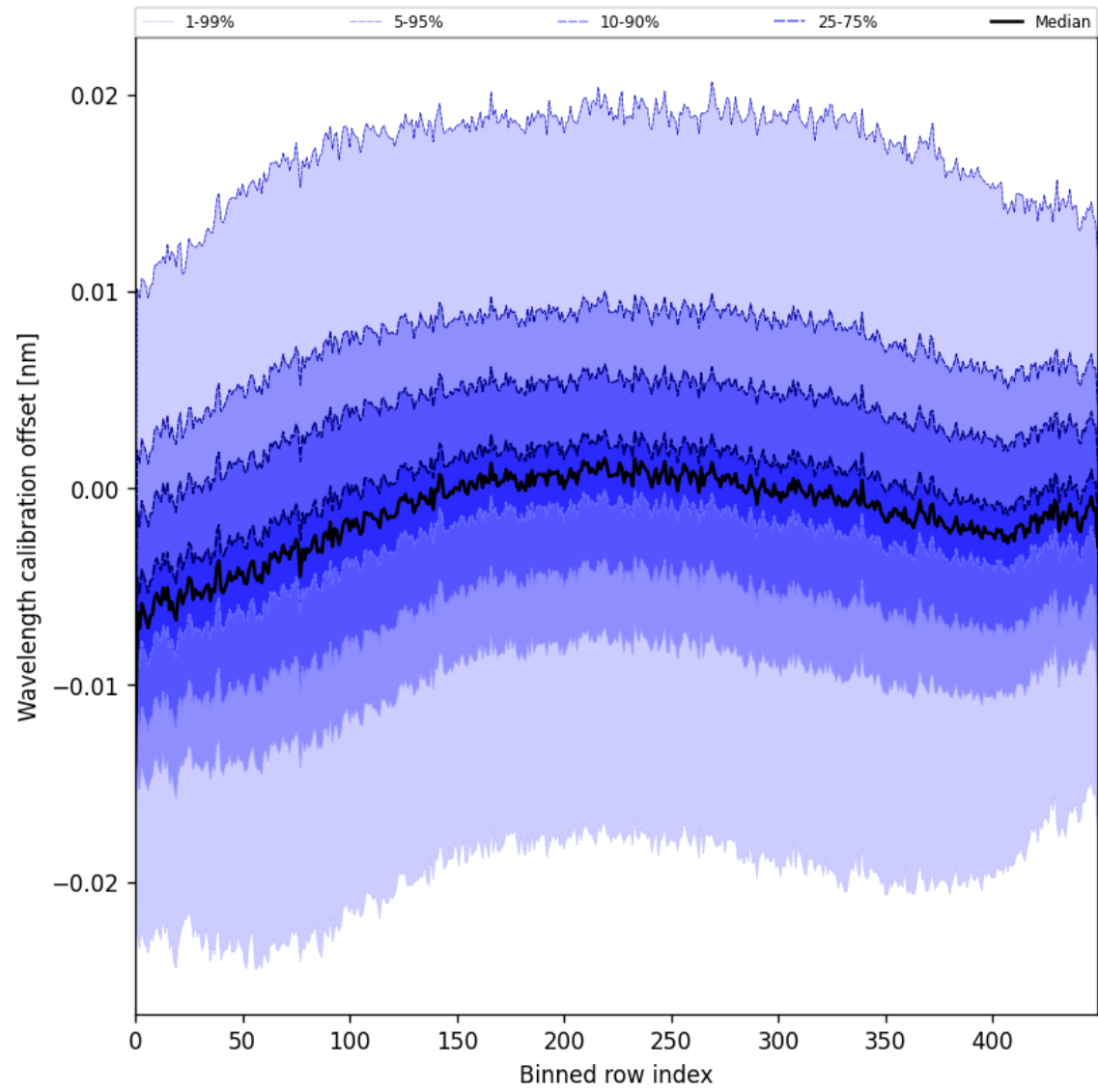
Figure 50: Along track statistics of “Wavelength calibration offset” for 2025-06-07 to 2025-06-08
