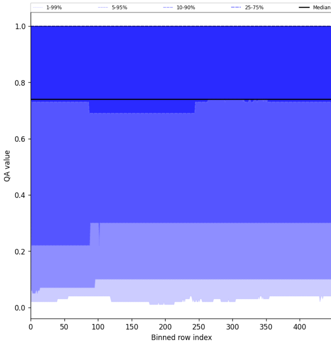
Figure 43: Along track statistics of “QA value” for 2025-06-07 to 2025-06-08
