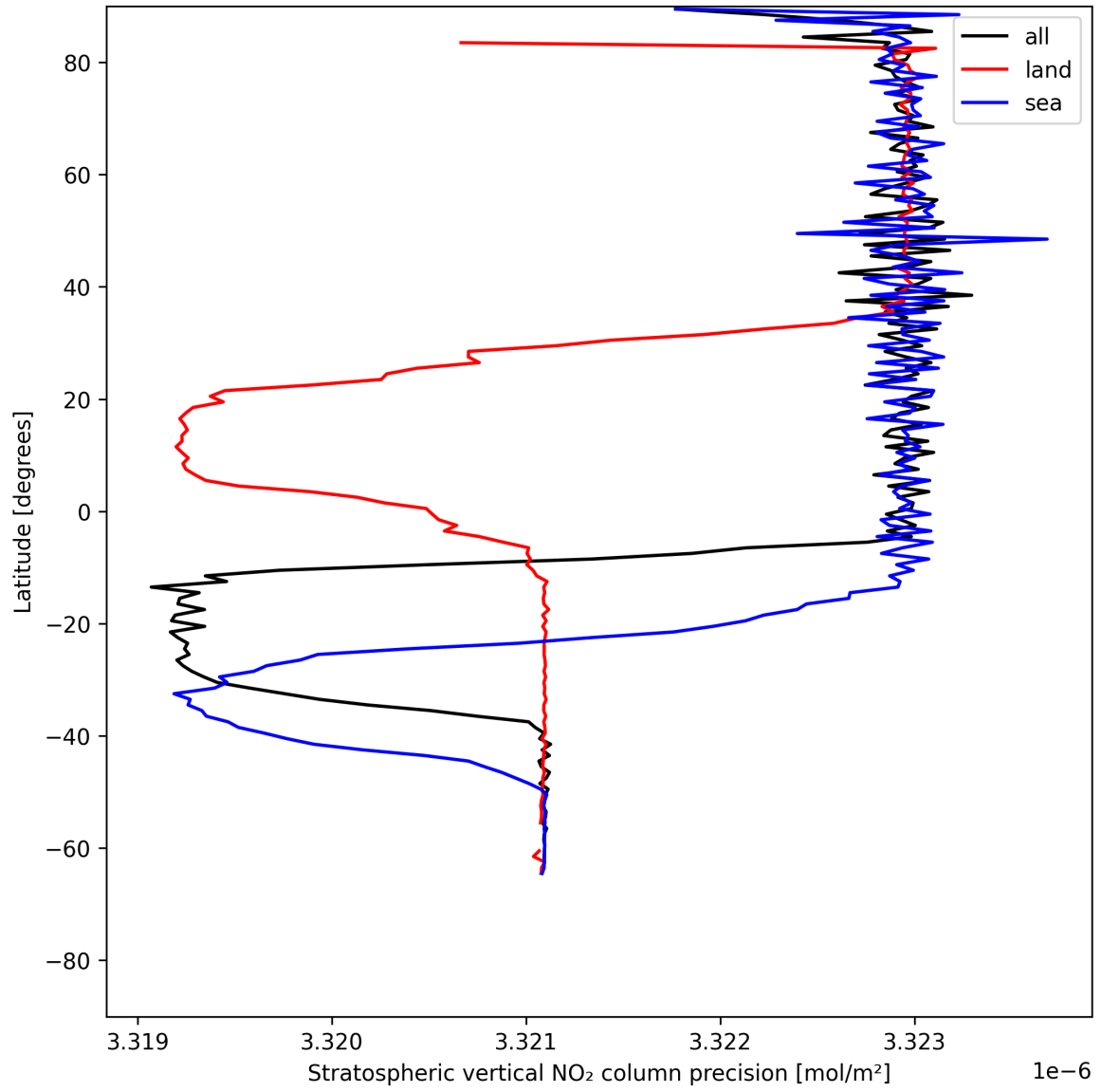
Figure 18: Zonal average of “Stratospheric vertical NO 2 column precision” for 2025-06-07 to 2025-06-08.
