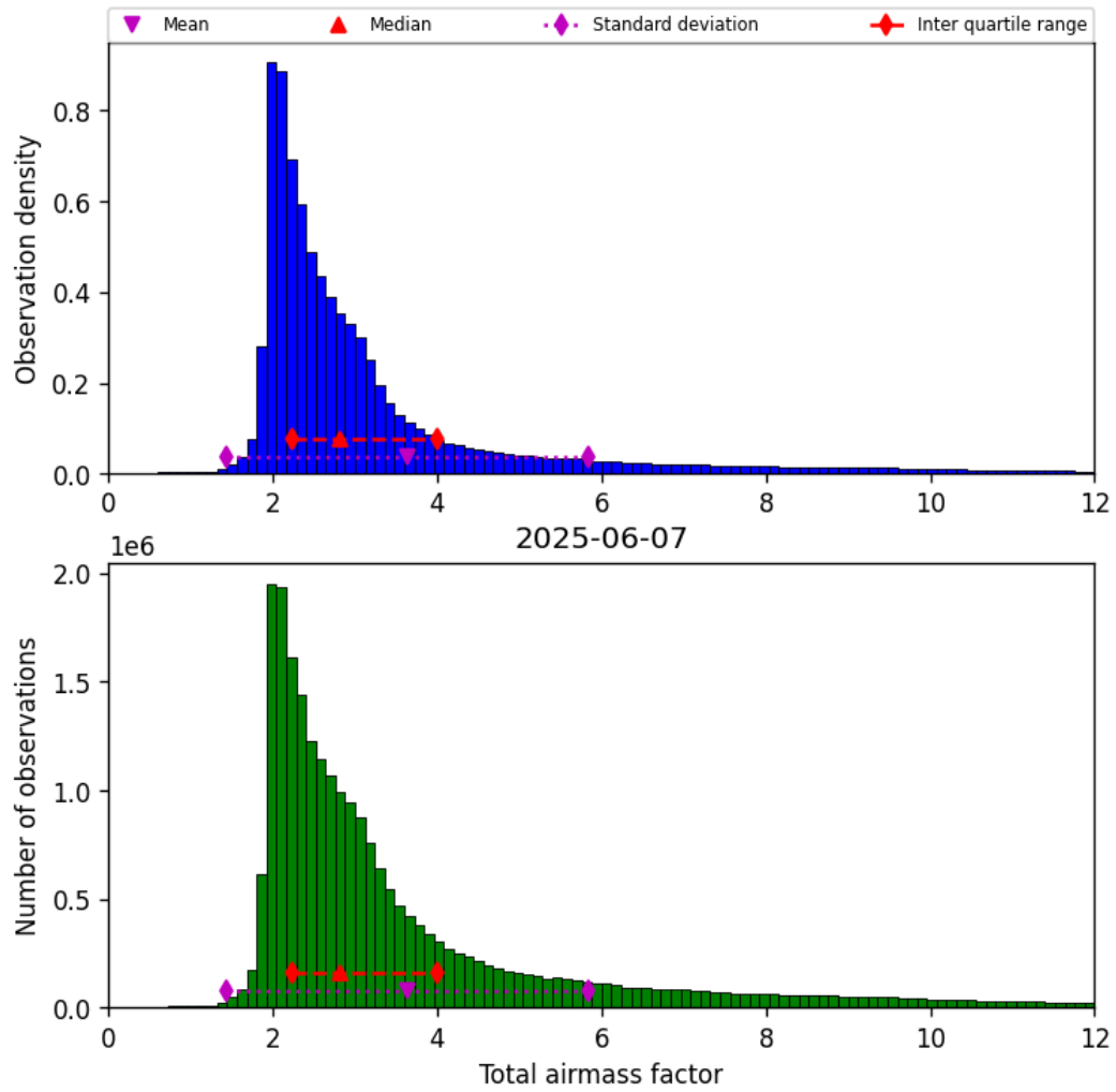
Figure 30: Histogram of “Total airmass factor” for 2025-06-07 to 2025-06-08
