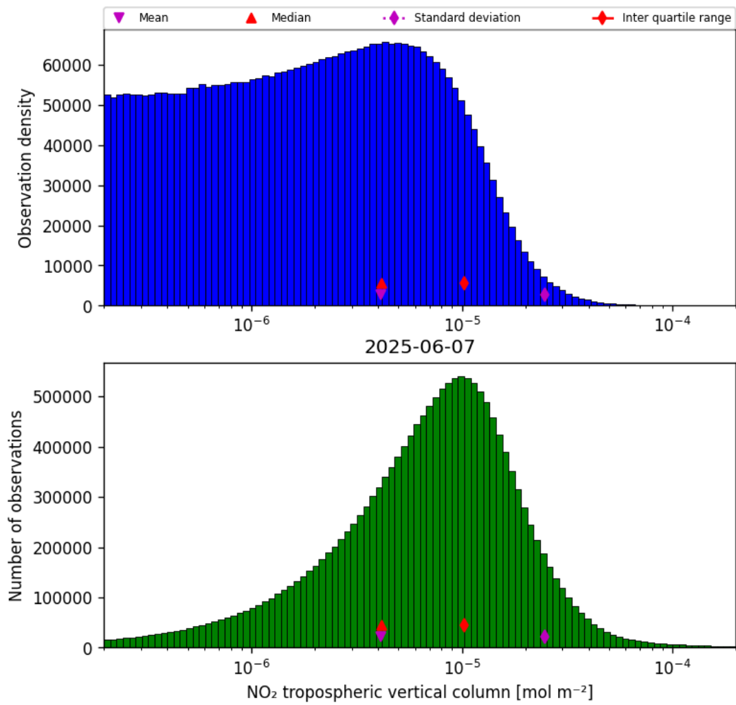
Figure 27: Histogram of “NO 2 tropospheric vertical column” for 2025-06-07 to 2025-06-08
