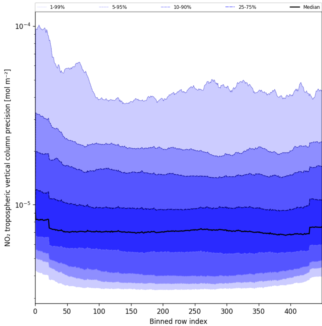
Figure 45: Along track statistics of “NO 2 tropospheric vertical column precision” for 2025-06-07 to 2025-06-08
