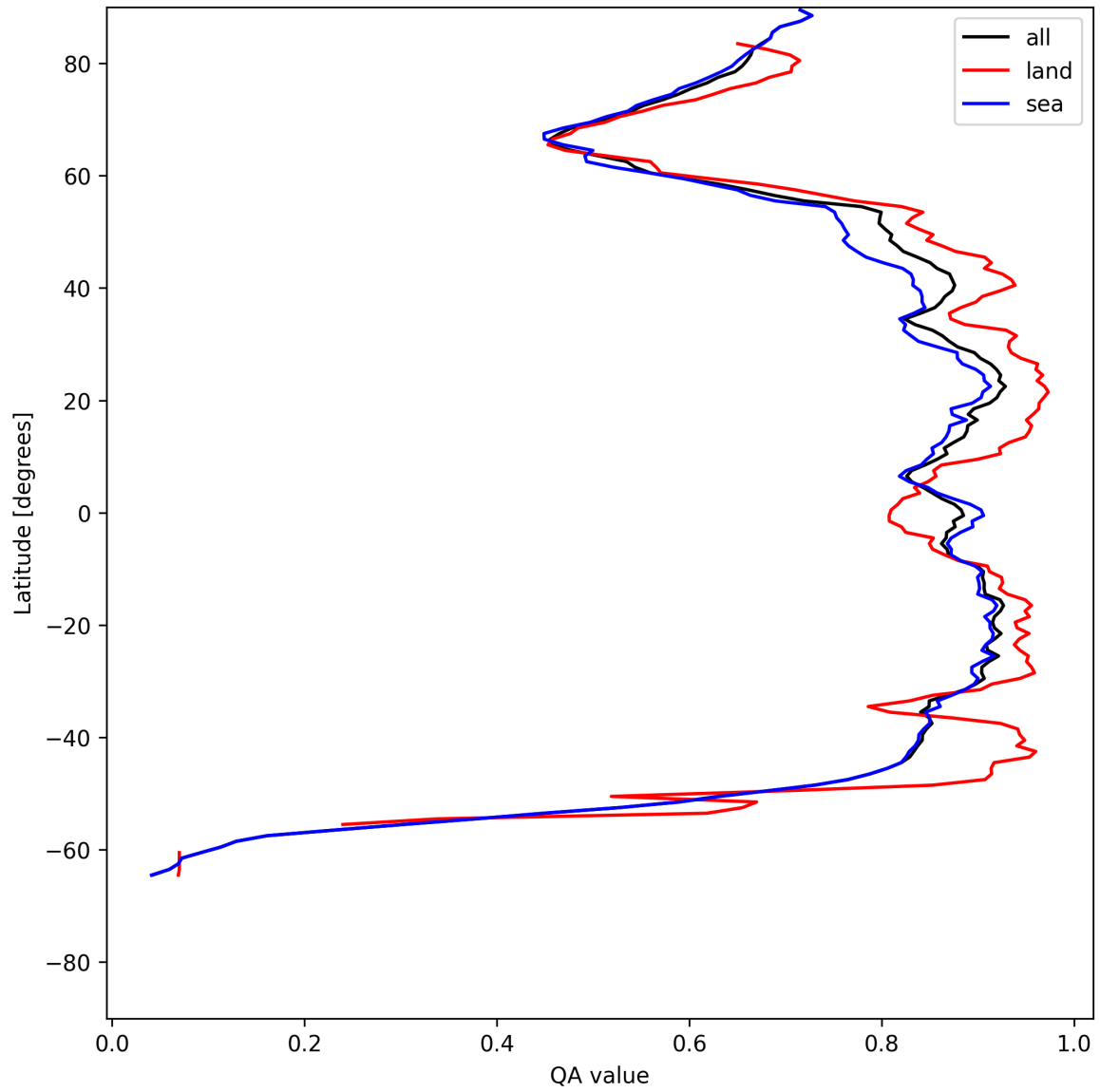
Figure 9: Zonal average of “QA value” for 2025-06-07 to 2025-06-08.
