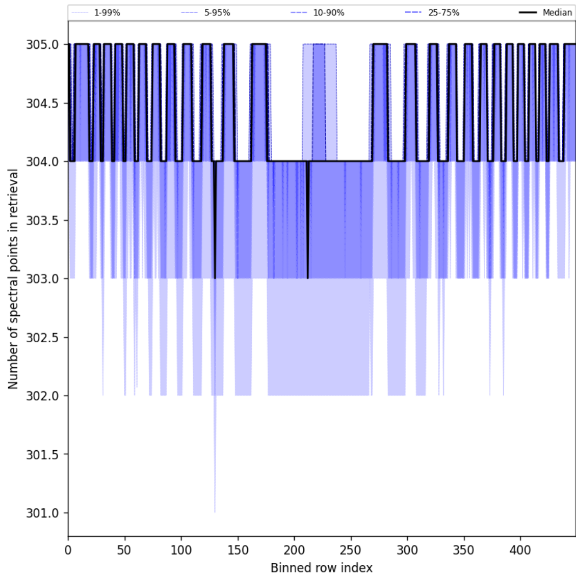
Figure 48: Along track statistics of “Number of spectral points in retrieval” for 2025-06-07 to 2025-06-08
