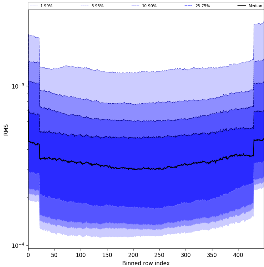
Figure 58: Along track statistics of “RMS” for 2025-06-07 to 2025-06-08
