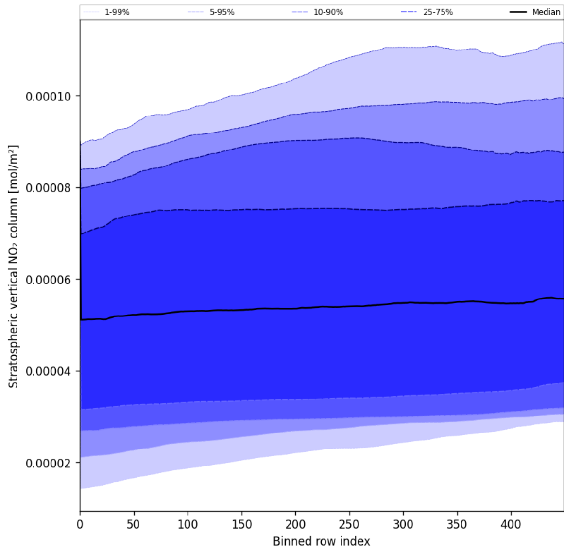
Figure 51: Along track statistics of “Stratospheric vertical NO 2 column” for 2025-06-07 to 2025-06-08
