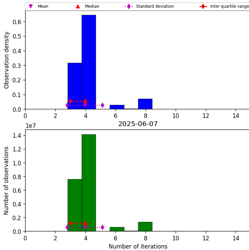
Figure 32: Histogram of “Number of iterations” for 2025-06-07 to 2025-06-08
