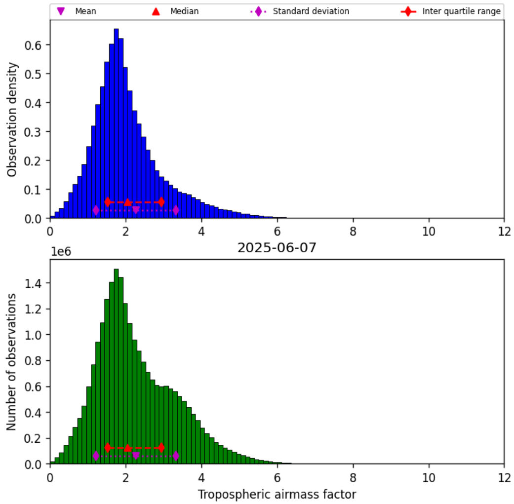
Figure 29: Histogram of “Tropospheric airmass factor” for 2025-06-07 to 2025-06-08
