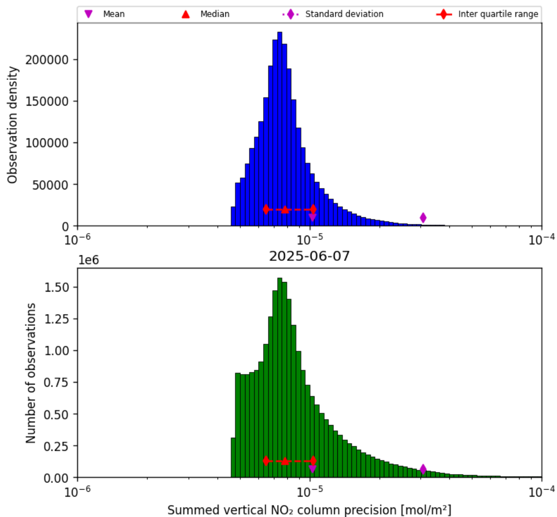
Figure 39: Histogram of “Summed vertical NO 2 column precision” for 2025-06-07 to 2025-06-08
