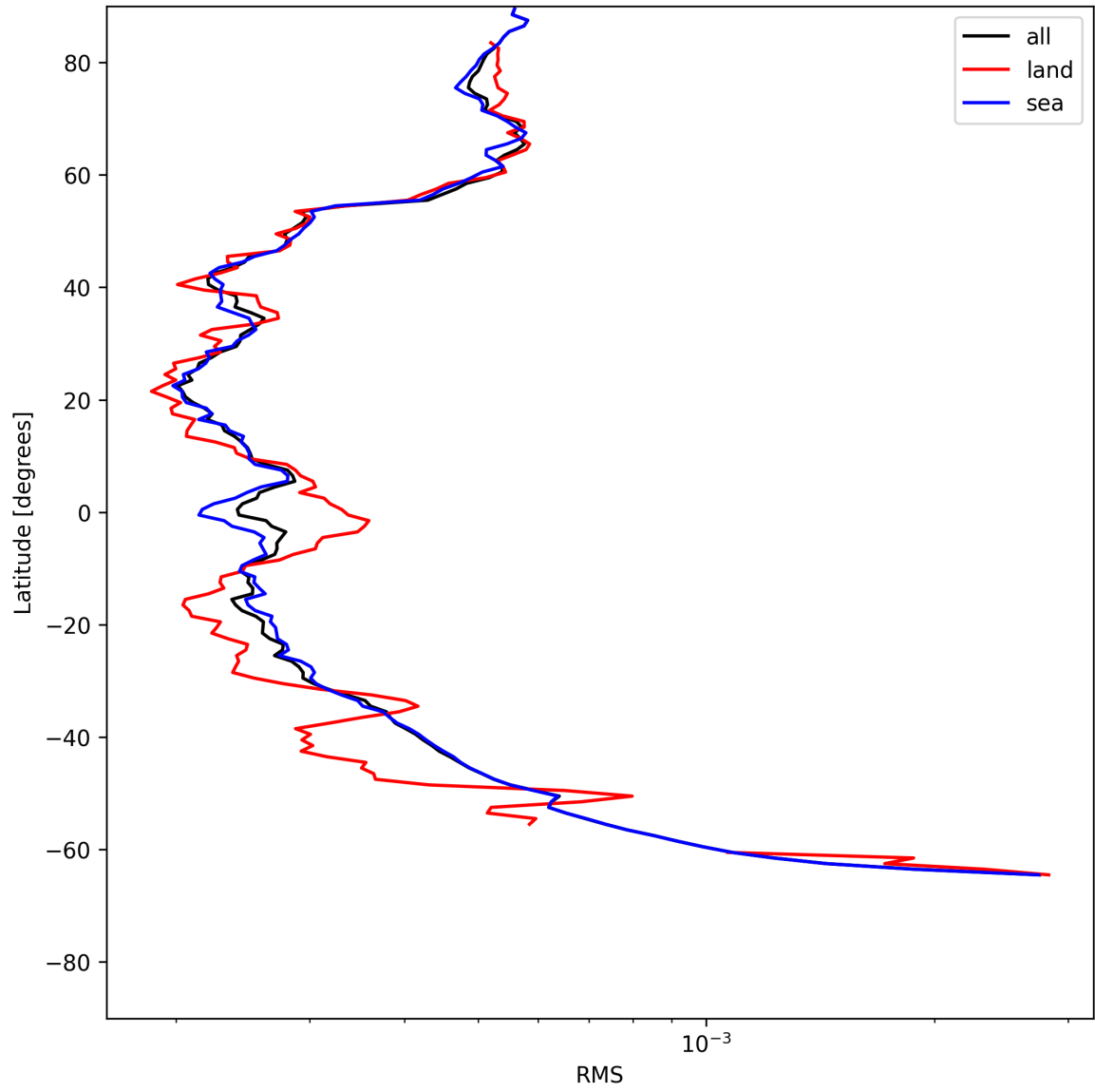
Figure 24: Zonal average of “RMS” for 2025-06-07 to 2025-06-08.
