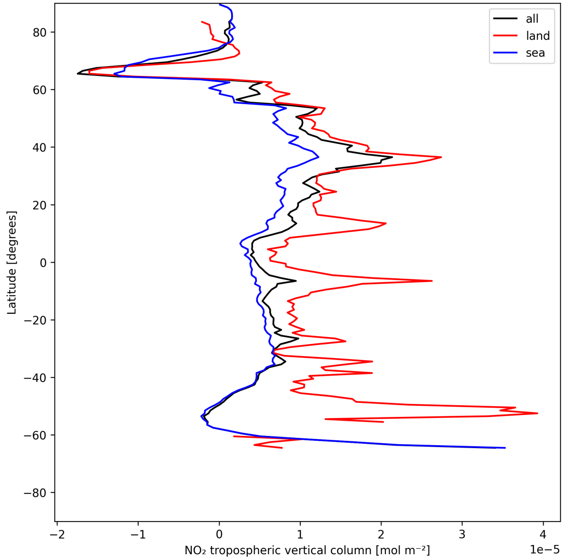
Figure 10: Zonal average of “NO 2 tropospheric vertical column” for 2025-06-07 to 2025-06-08.
