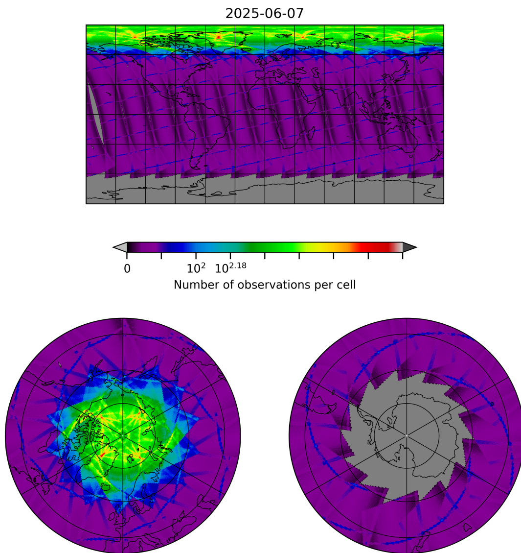
Figure 8: Map of the number of observations for 2025-06-07 to 2025-06-08
