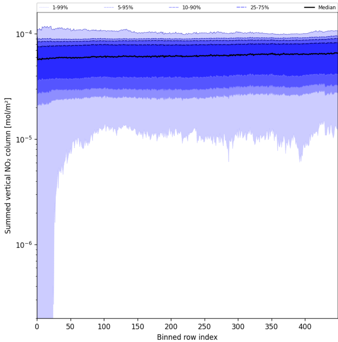
Figure 55: Along track statistics of “Summed vertical NO 2 column” for 2025-06-07 to 2025-06-08
