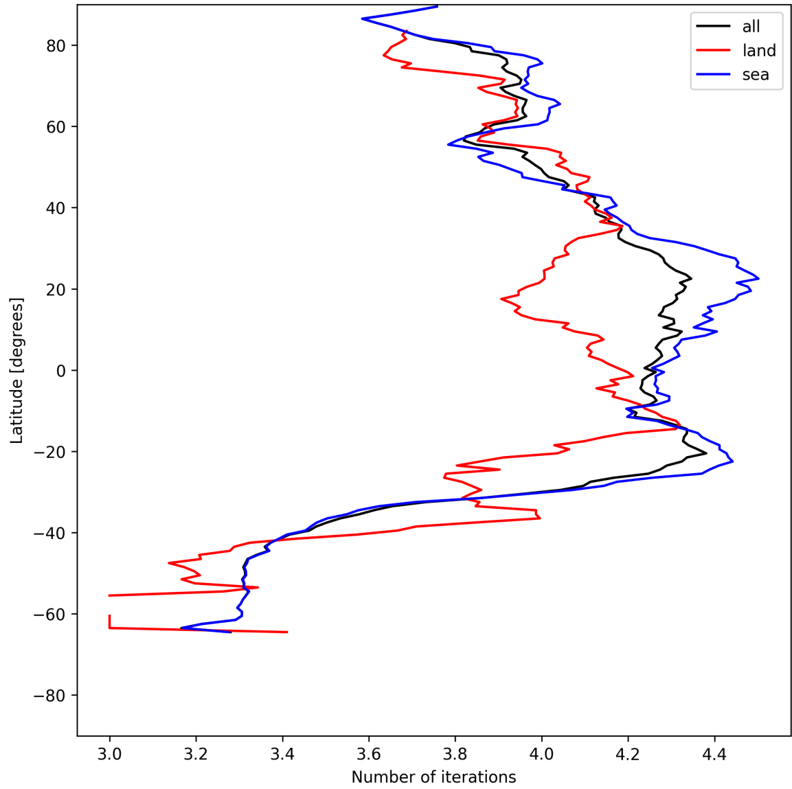
Figure 15: Zonal average of “Number of iterations” for 2025-06-07 to 2025-06-08.
