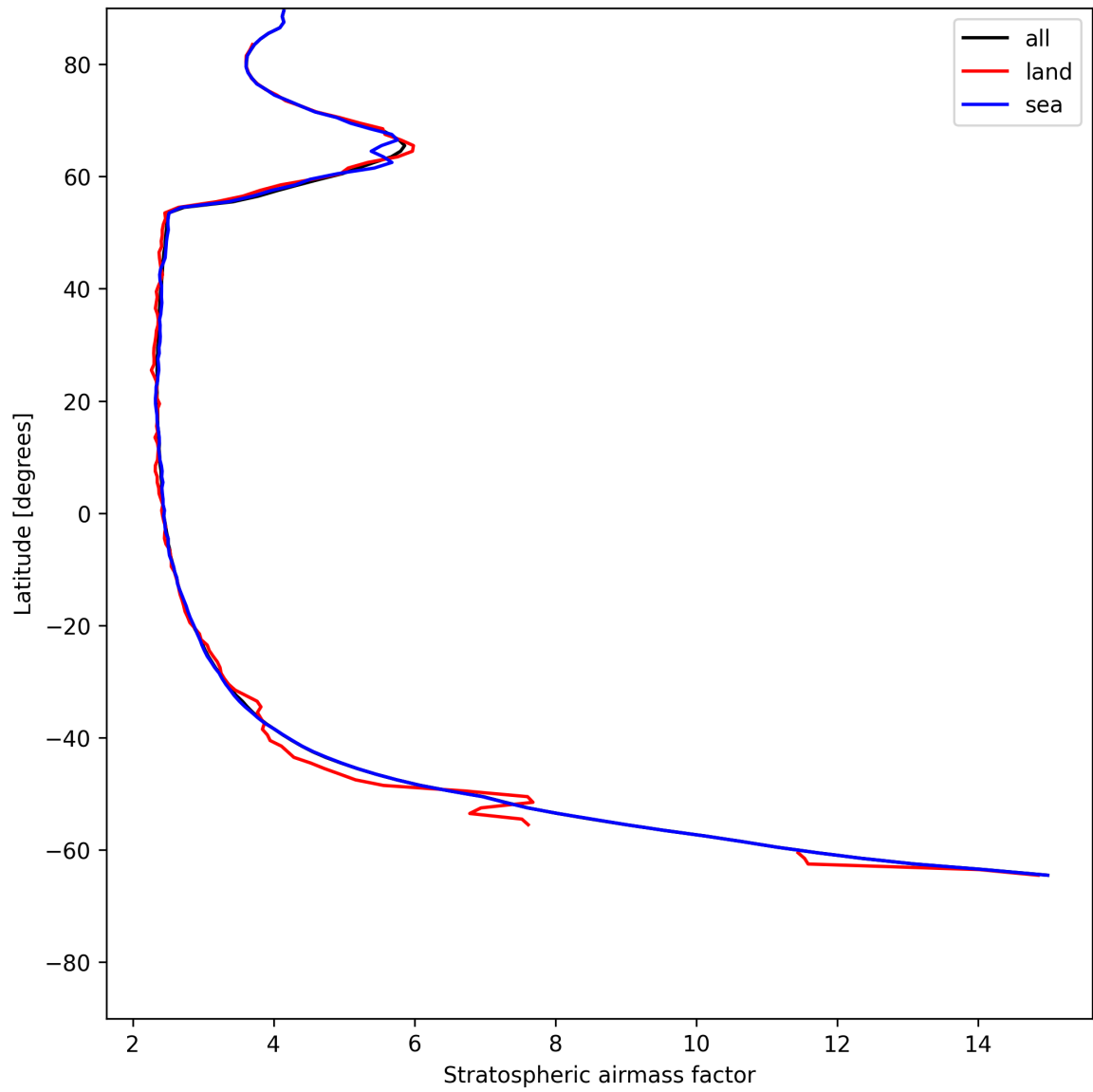
Figure 25: Zonal average of “Stratospheric air mass factor” for 2025-06-07 to 2025-06-08.
