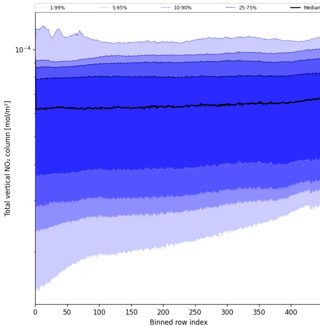
Figure 53: Along track statistics of “Total vertical NO 2 column” for 2025-06-07 to 2025-06-08
