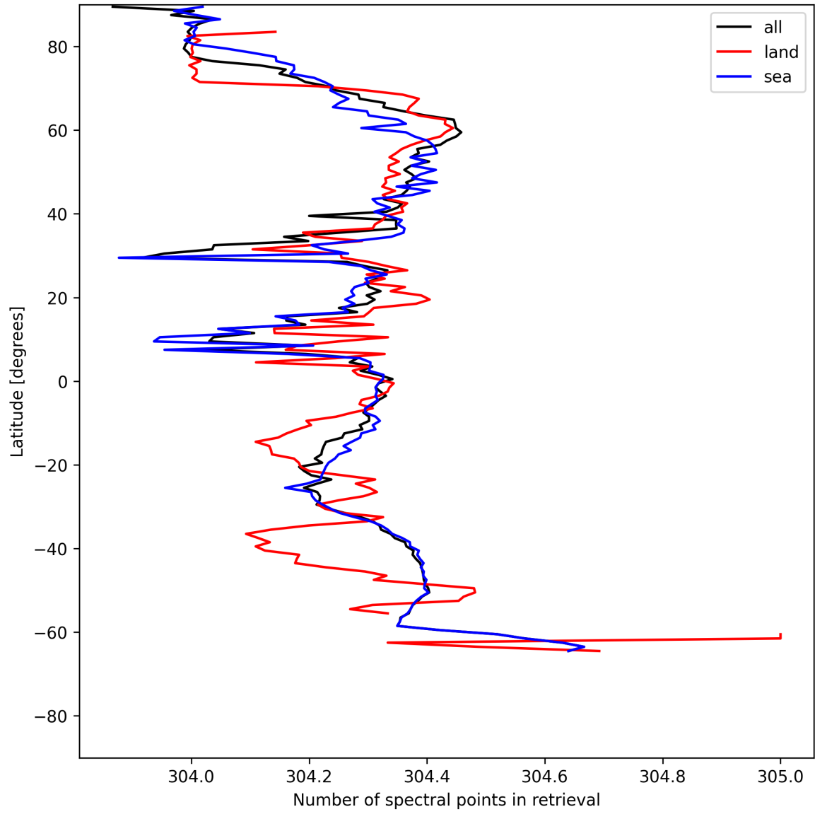
Figure 14: Zonal average of “Number of spectral points in retrieval” for 2025-06-07 to 2025-06-08.
