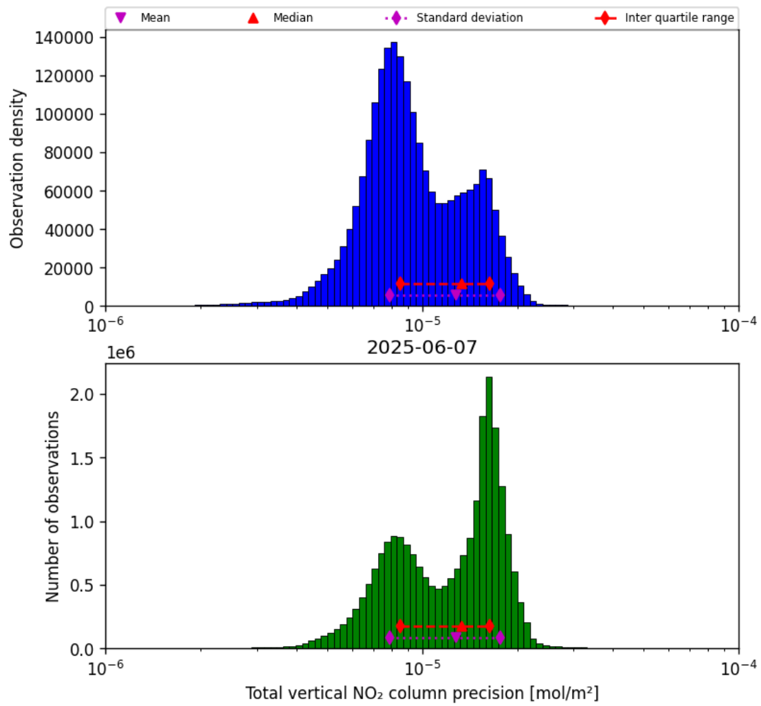
Figure 37: Histogram of “Total vertical NO 2 column precision” for 2025-06-07 to 2025-06-08
