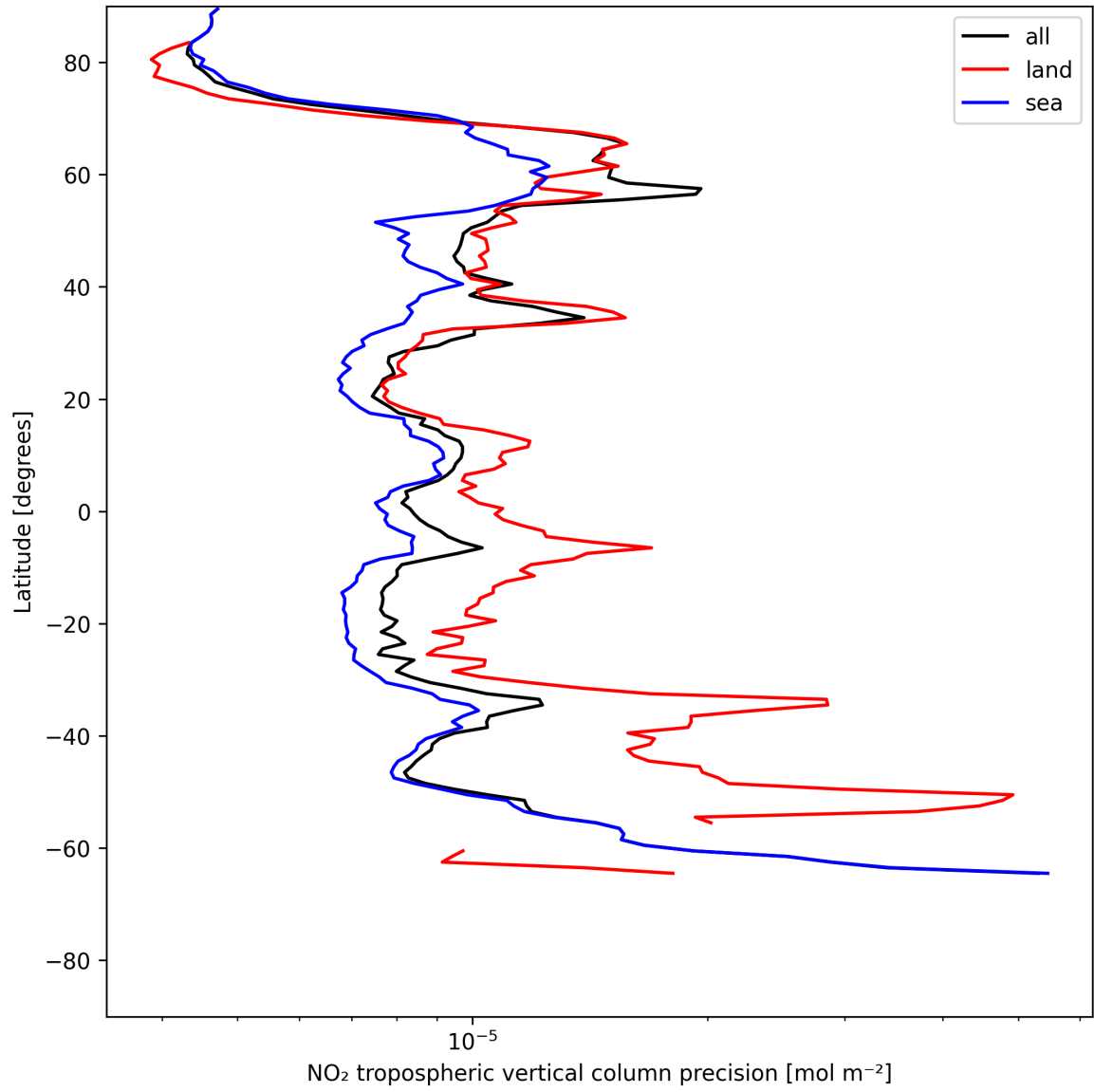
Figure 11: Zonal average of “NO 2 tropospheric vertical column precision” for 2025-06-07 to 2025-06-08.
