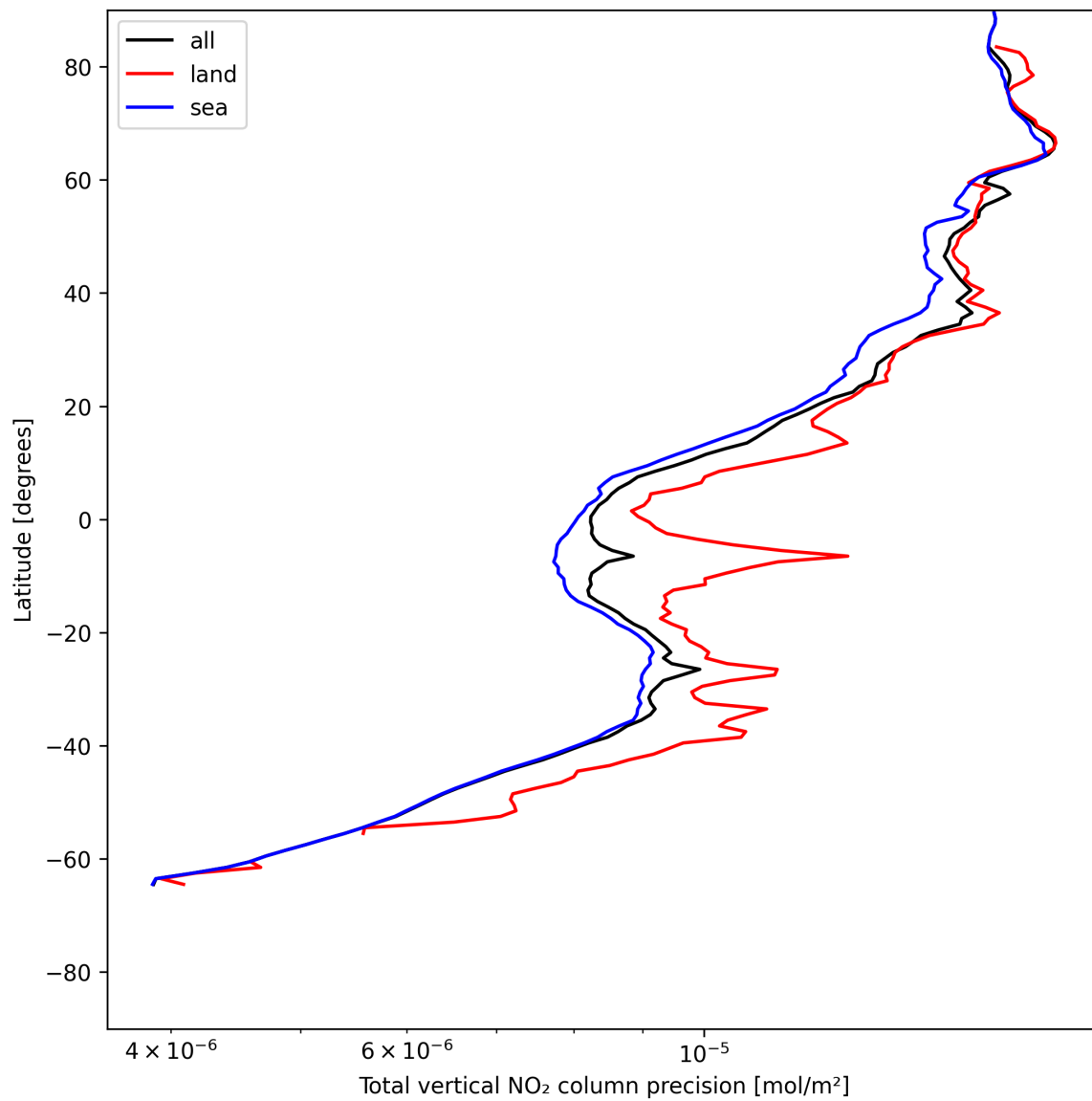
Figure 20: Zonal average of “Total vertical NO 2 column precision” for 2025-06-07 to 2025-06-08.
