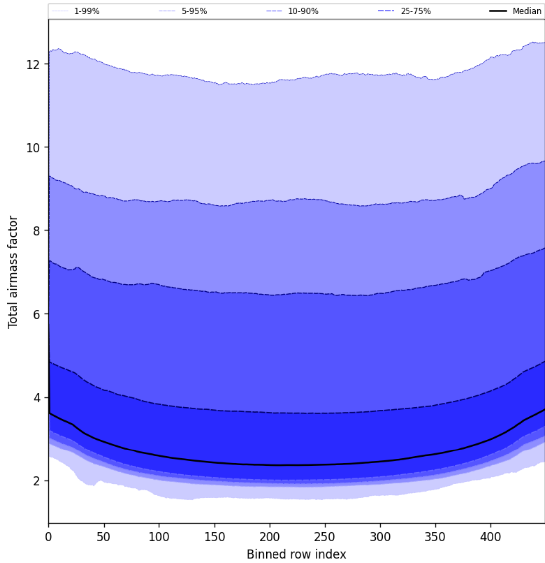
Figure 47: Along track statistics of “Total airmass factor” for 2025-06-07 to 2025-06-08
