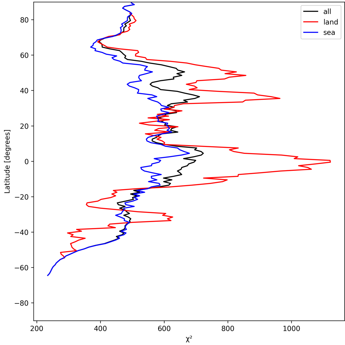
Figure 23: Zonal average of “ \chi^2 ” for 2025-06-08 to 2025-06-09.
