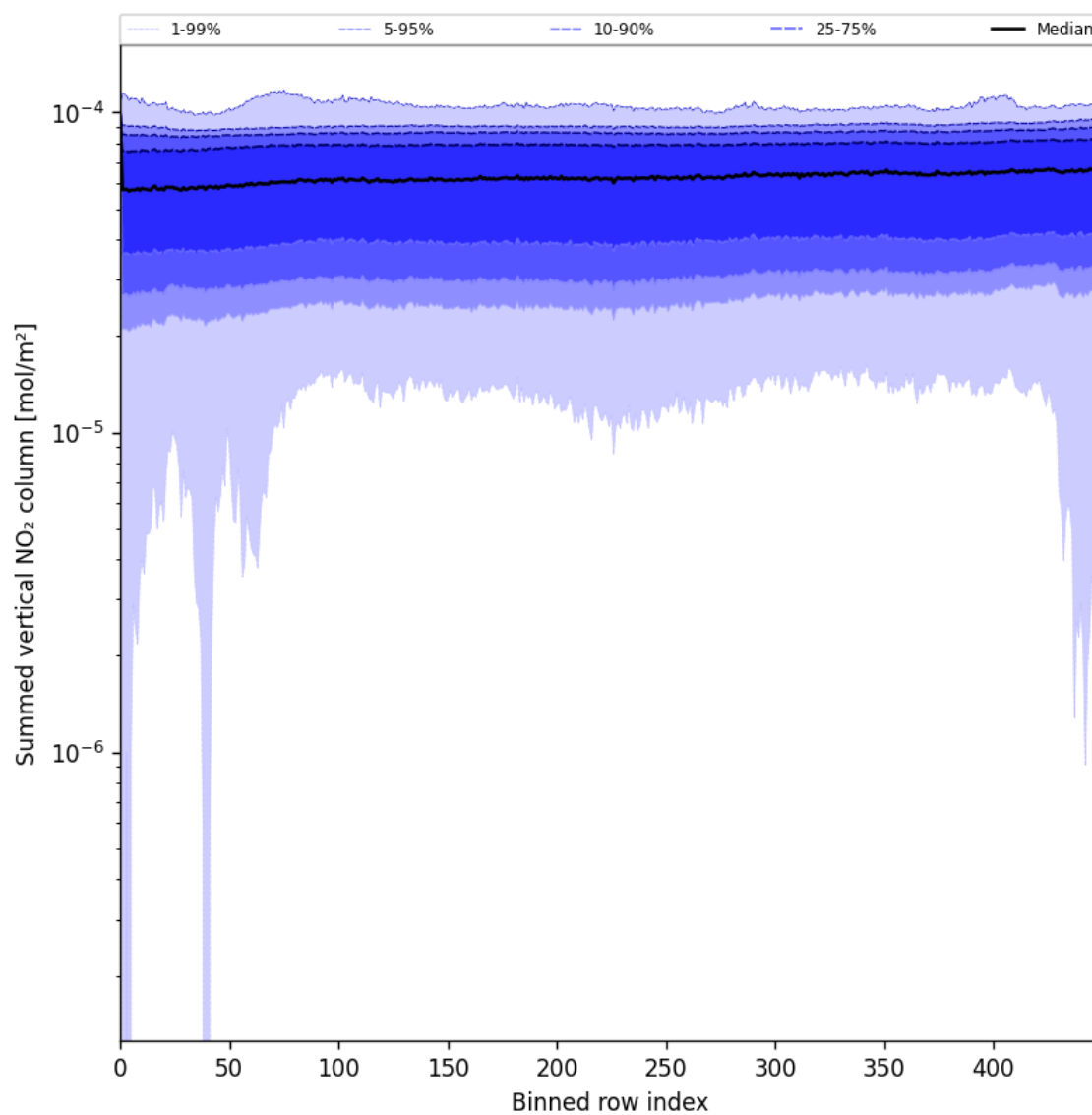
Figure 55: Along track statistics of “Summed vertical NO 2 column” for 2025-06-08 to 2025-06-09
