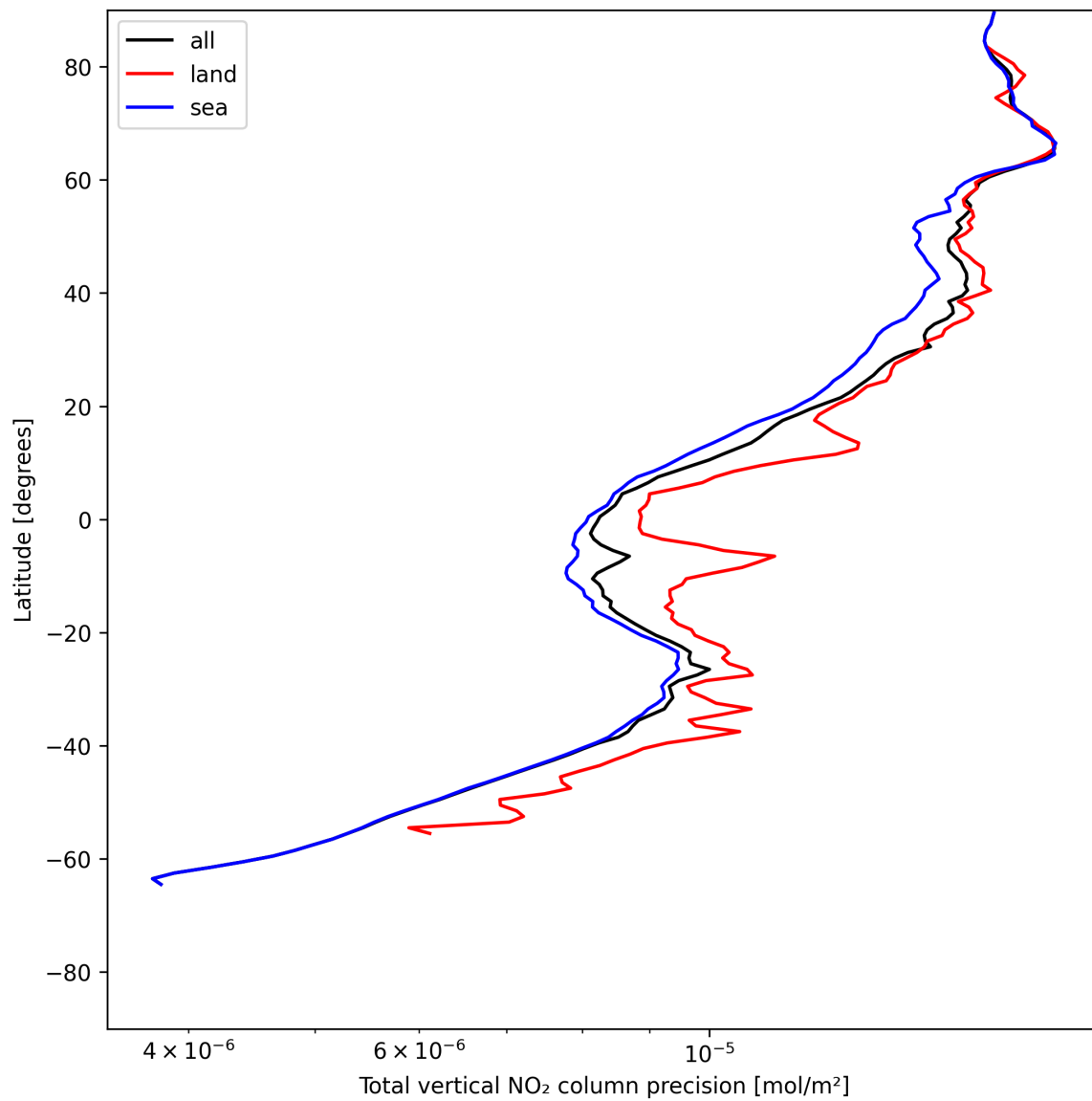
Figure 20: Zonal average of “Total vertical NO 2 column precision” for 2025-06-08 to 2025-06-09.
