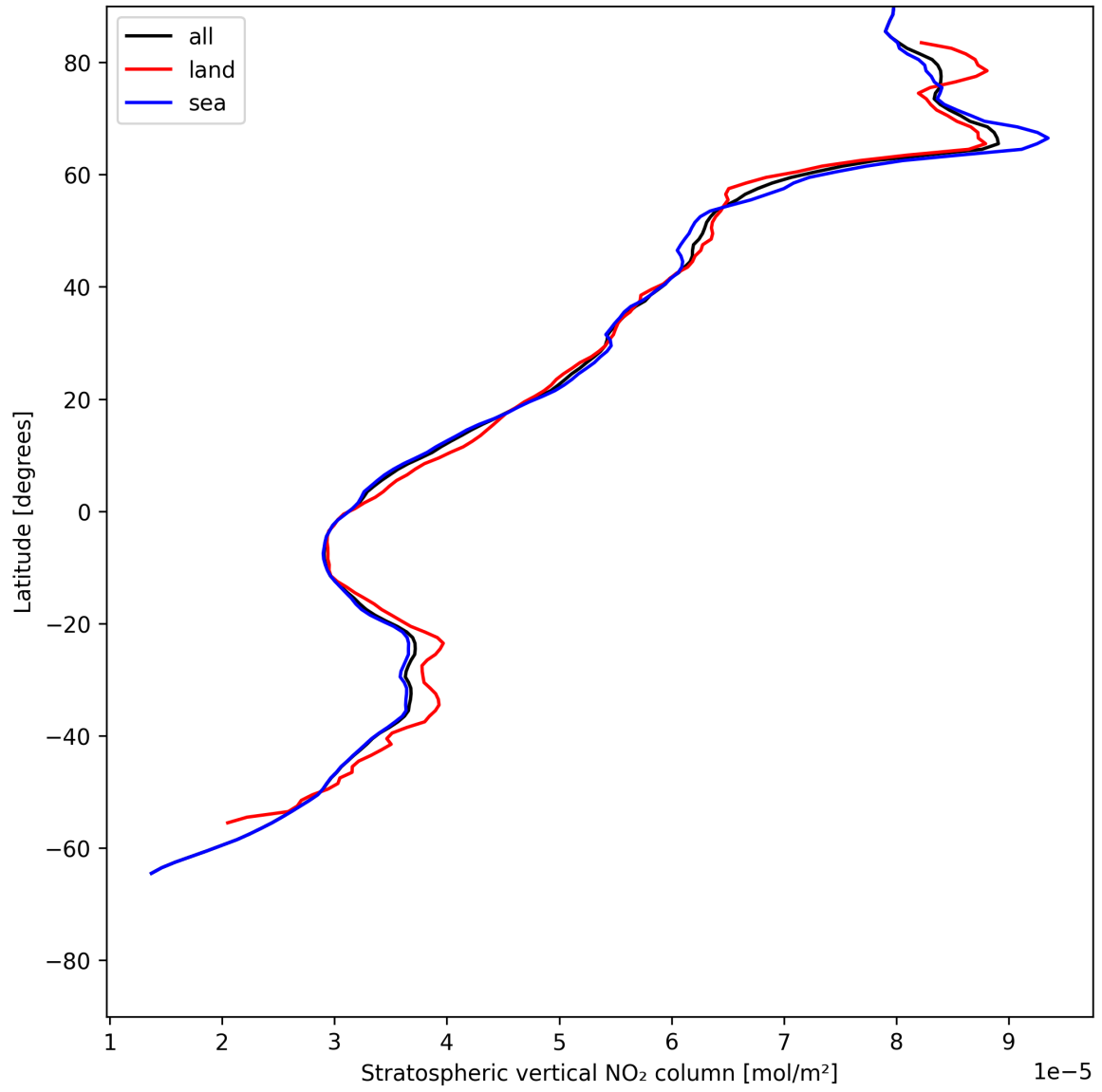
Figure 17: Zonal average of “Stratospheric vertical NO 2 column” for 2025-06-08 to 2025-06-09.
