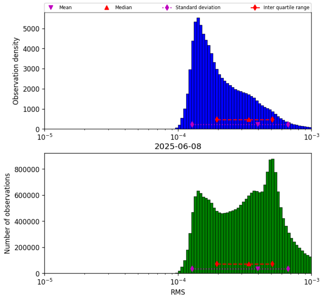
Figure 41: Histogram of “RMS” for 2025-06-08 to 2025-06-09
