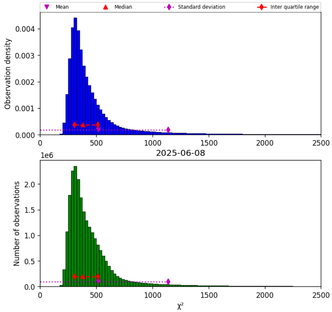
Figure 40: Histogram of “ \chi^2 ” for 2025-06-08 to 2025-06-09
