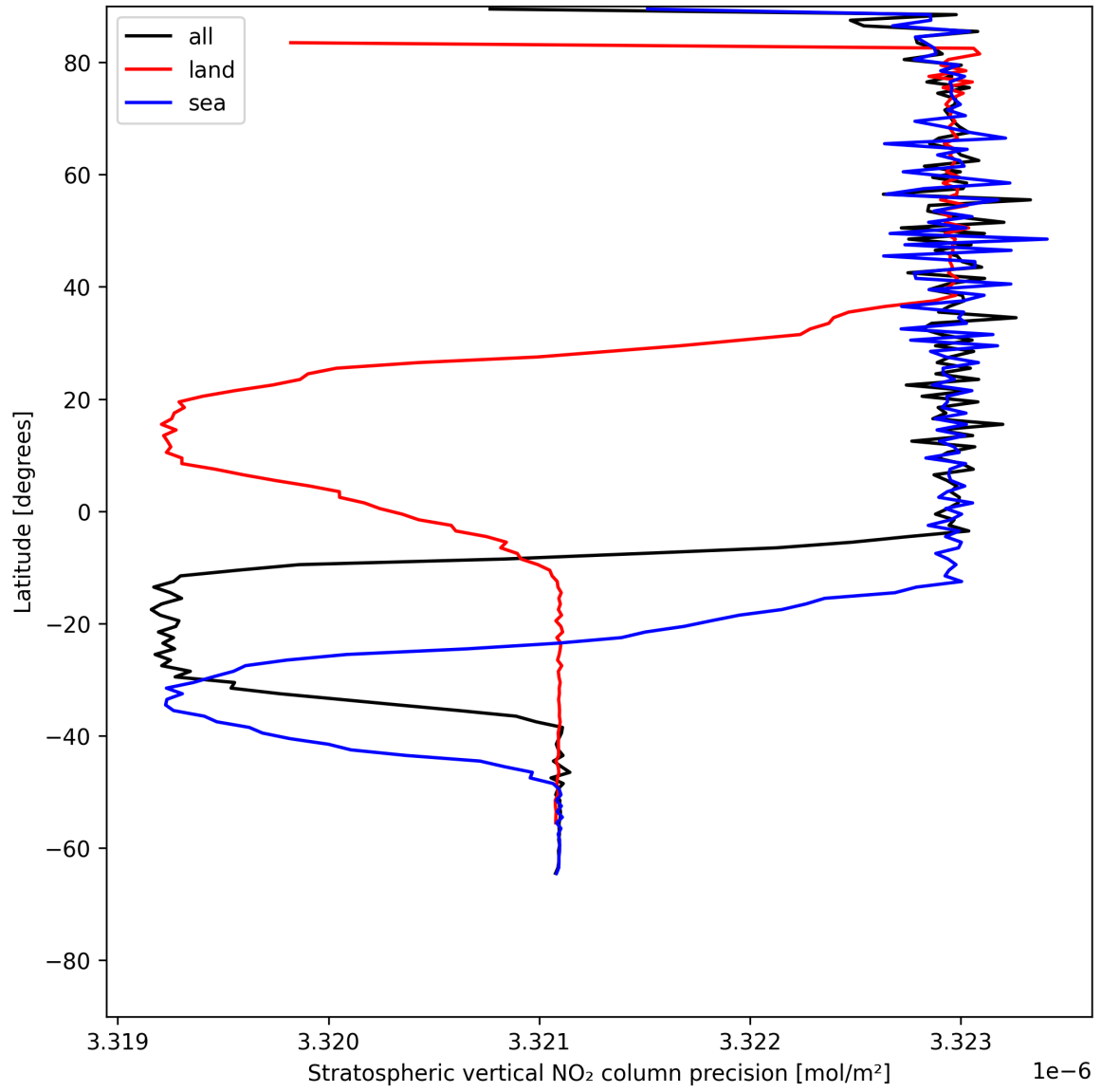
Figure 18: Zonal average of “Stratospheric vertical NO 2 column precision” for 2025-06-08 to 2025-06-09.
