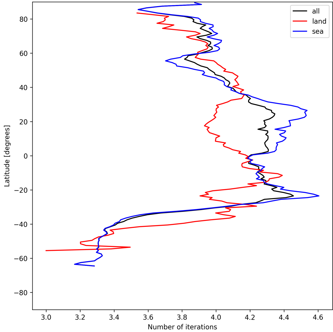
Figure 15: Zonal average of “Number of iterations” for 2025-06-08 to 2025-06-09.
