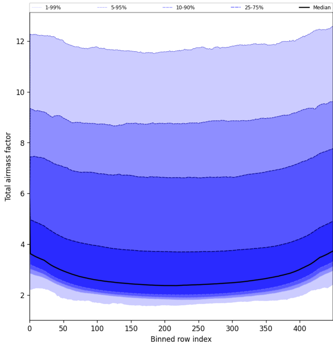
Figure 47: Along track statistics of “Total airmass factor” for 2025-06-08 to 2025-06-09
