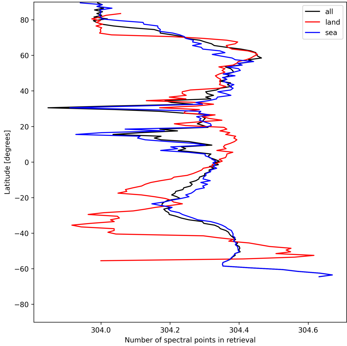
Figure 14: Zonal average of “Number of spectral points in retrieval” for 2025-06-08 to 2025-06-09.
