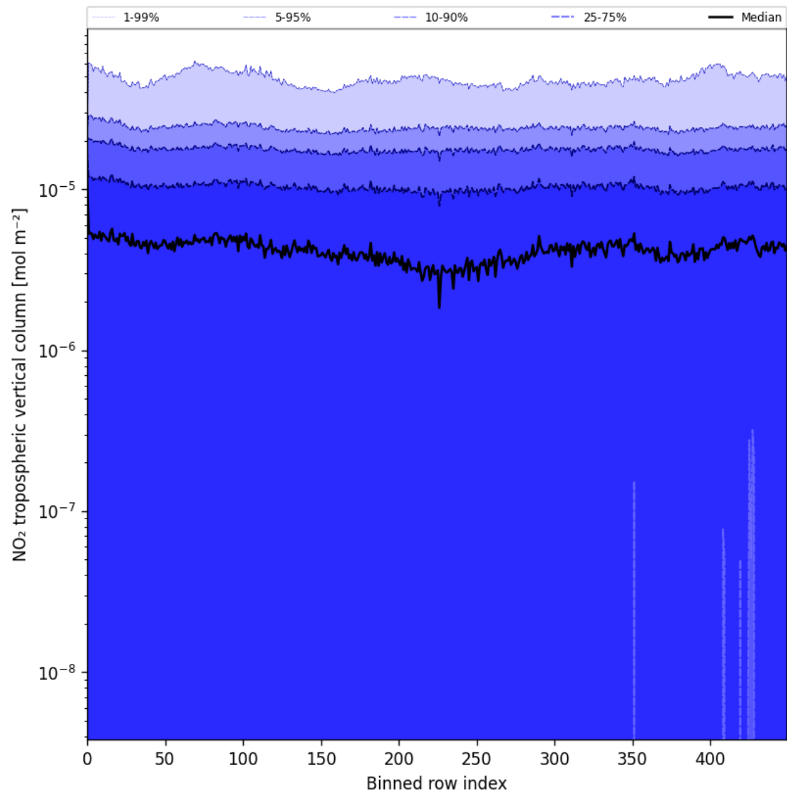
Figure 44: Along track statistics of "NO 2 tropospheric vertical column" for 2025-06-08 to 2025-06-09
