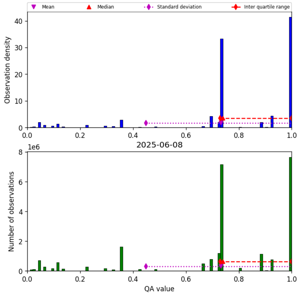
Figure 26: Histogram of “QA value” for 2025-06-08 to 2025-06-09
