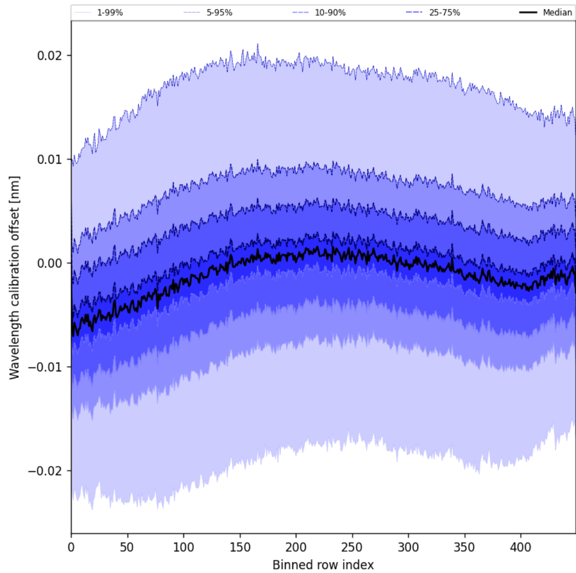
Figure 50: Along track statistics of “Wavelength calibration offset” for 2025-06-08 to 2025-06-09
