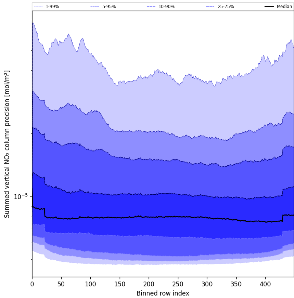
Figure 56: Along track statistics of “Summed vertical NO 2 column precision” for 2025-06-08 to 2025-06-09
