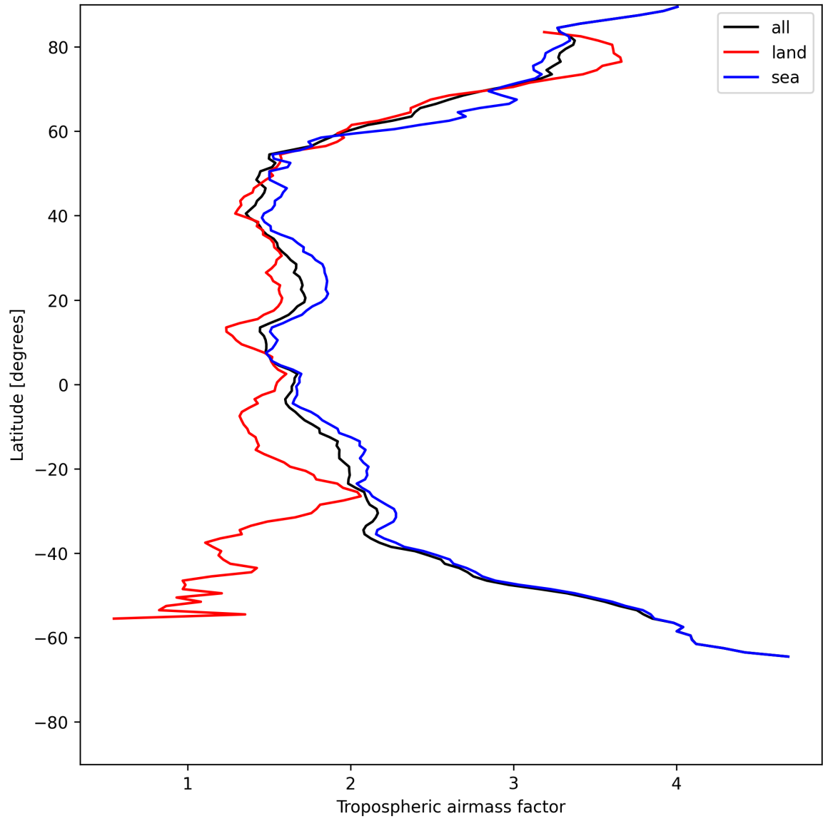
Figure 12: Zonal average of “Tropospheric airmass factor” for 2025-06-08 to 2025-06-09.
