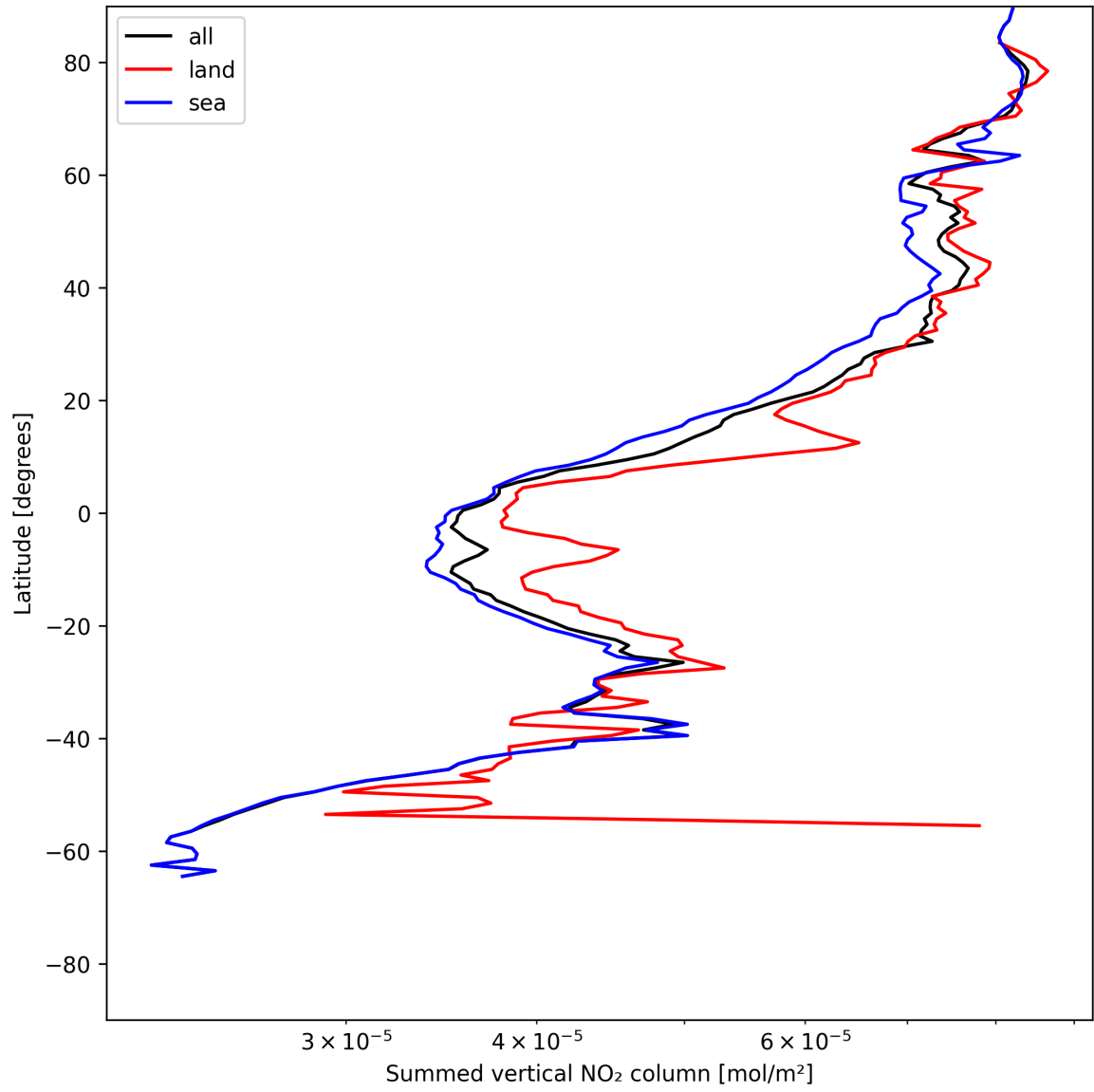
Figure 21: Zonal average of “Summed vertical NO 2 column” for 2025-06-08 to 2025-06-09.
