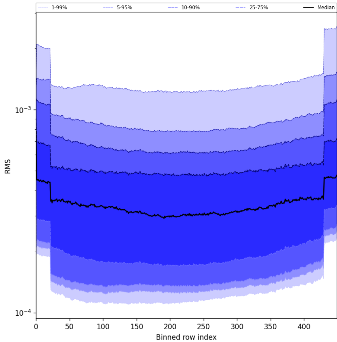
Figure 58: Along track statistics of “RMS” for 2025-06-08 to 2025-06-09
