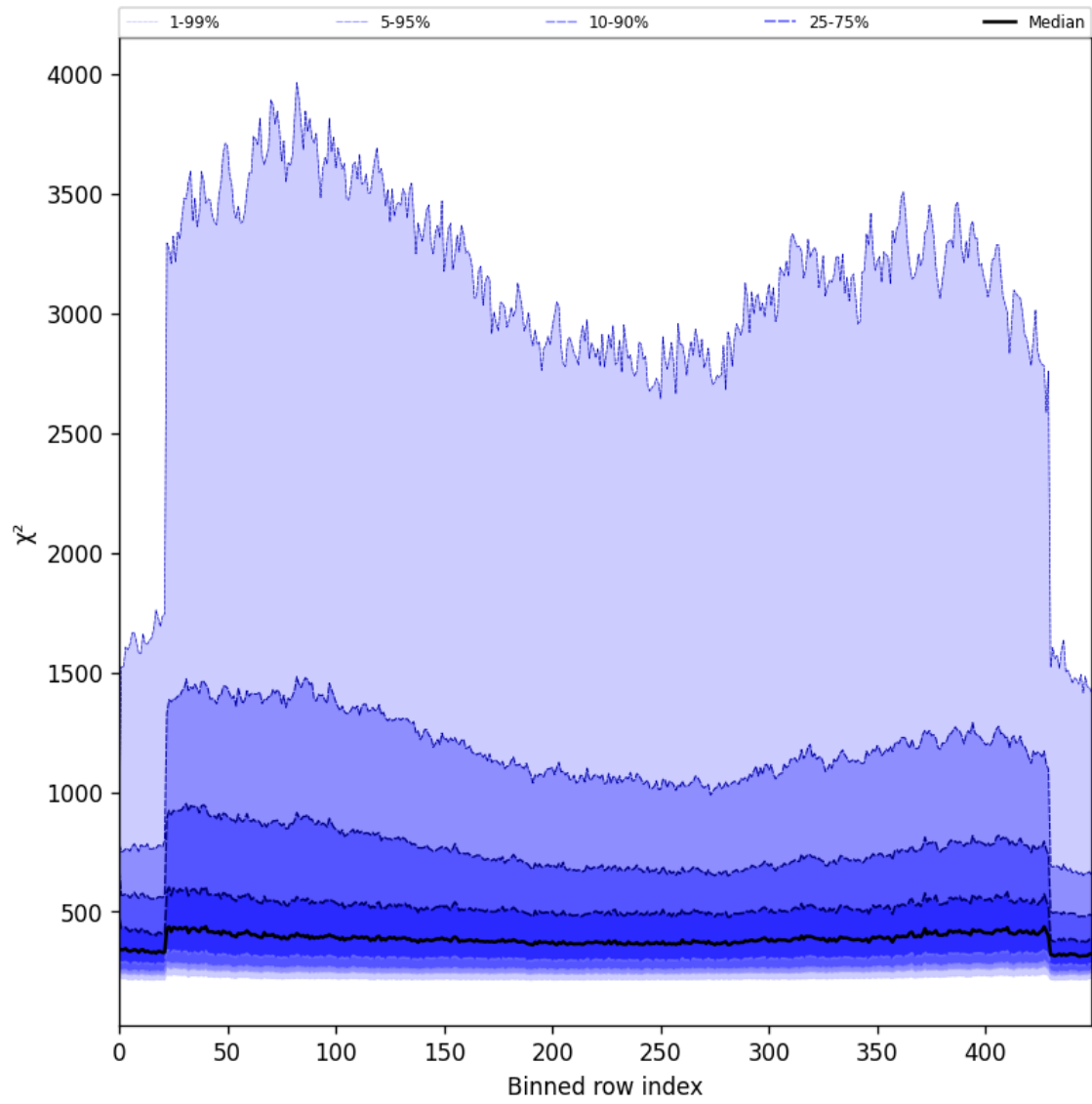
Figure 57: Along track statistics of “ \chi^2 ” for 2025-06-08 to 2025-06-09
