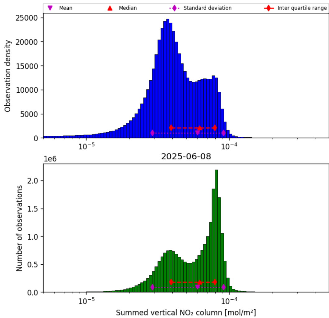
Figure 38: Histogram of “Summed vertical NO 2 column” for 2025-06-08 to 2025-06-09
