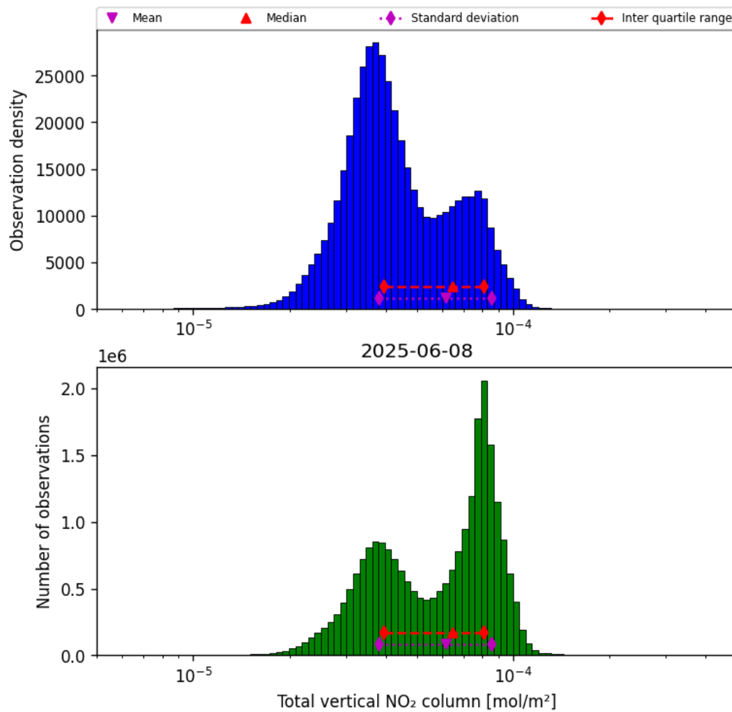
Figure 36: Histogram of “Total vertical NO 2 column” for 2025-06-08 to 2025-06-09
