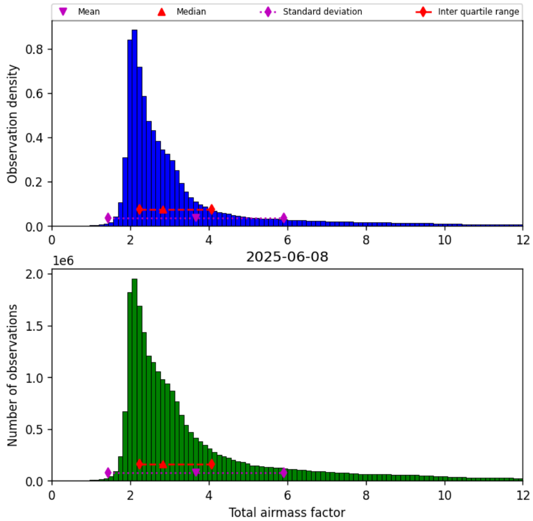
Figure 30: Histogram of “Total airmass factor” for 2025-06-08 to 2025-06-09
