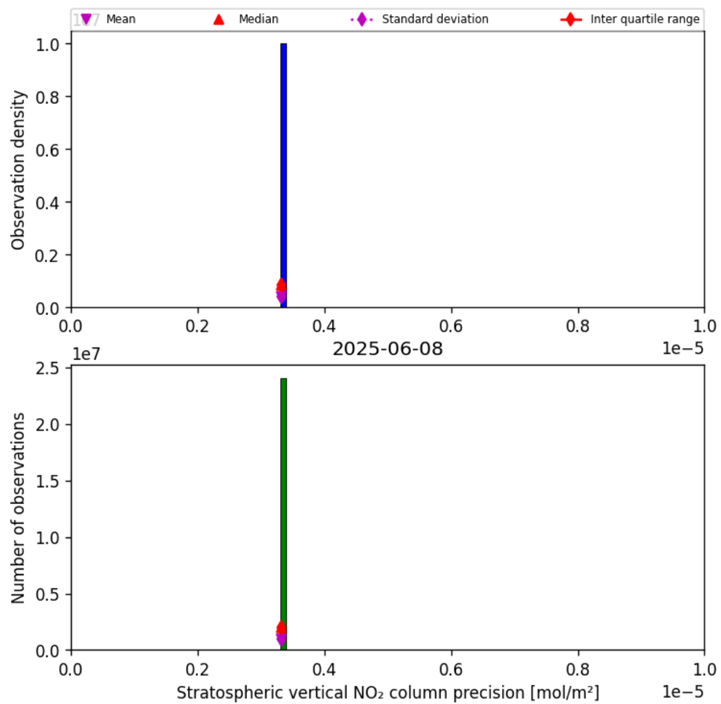
Figure 35: Histogram of “Stratospheric vertical NO 2 column precision” for 2025-06-08 to 2025-06-09
