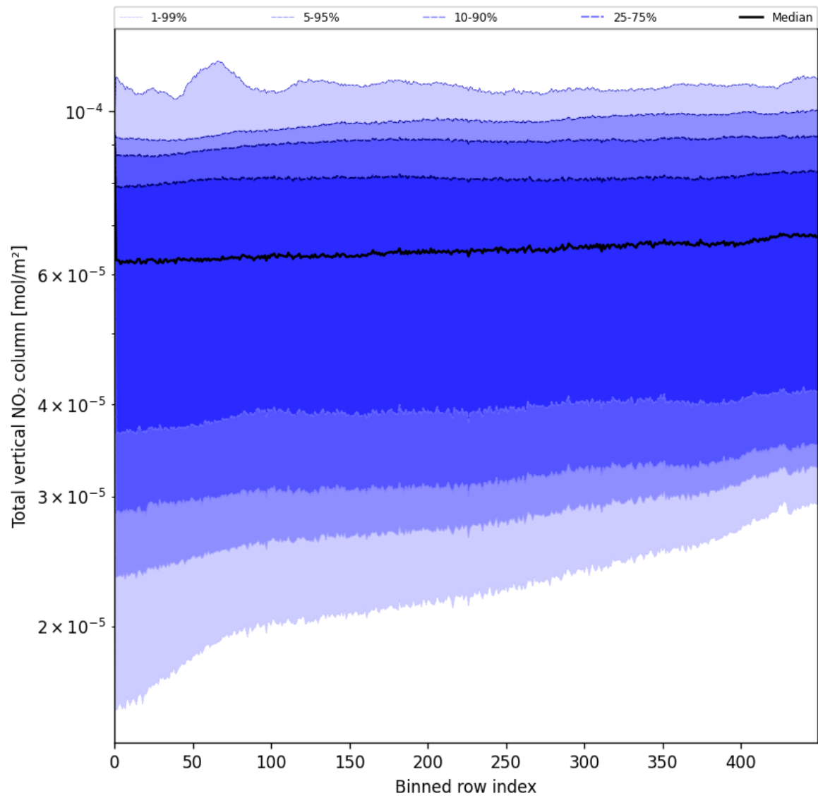
Figure 53: Along track statistics of “Total vertical NO 2 column” for 2025-06-08 to 2025-06-09
