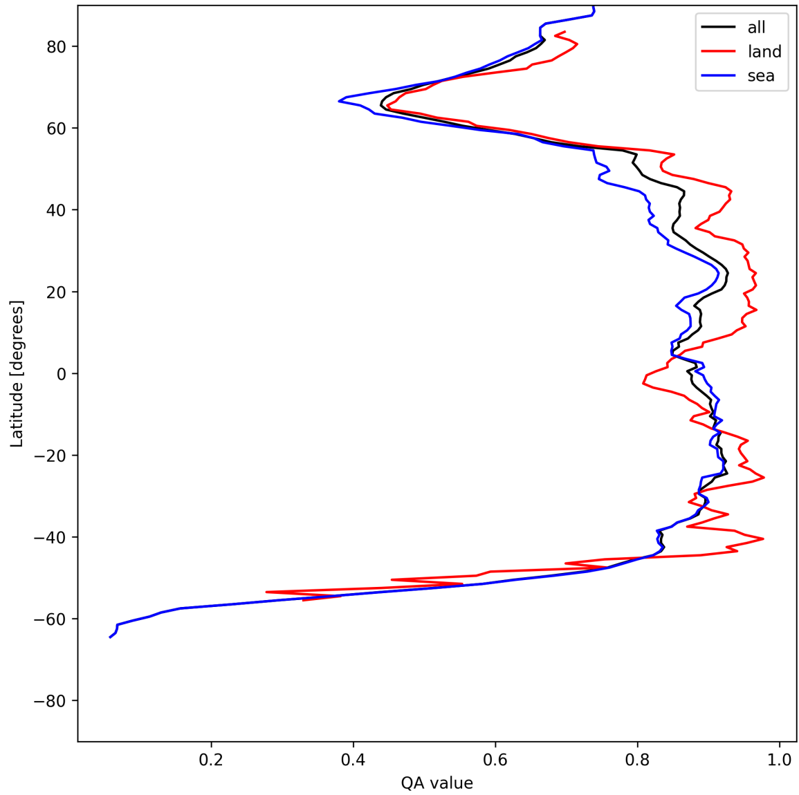
Figure 9: Zonal average of “QA value” for 2025-06-08 to 2025-06-09.
