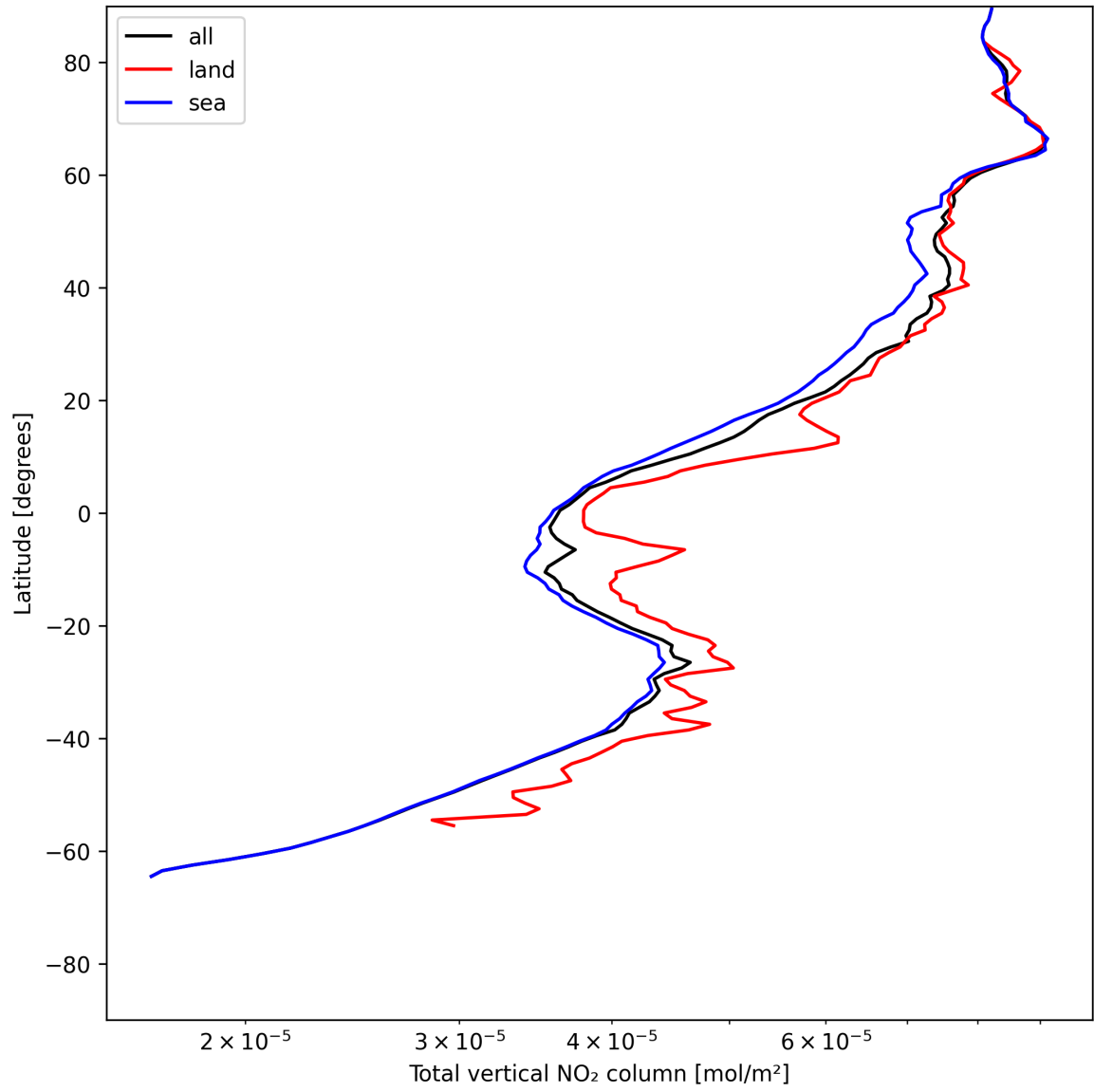
Figure 19: Zonal average of “Total vertical NO 2 column” for 2025-06-08 to 2025-06-09.
