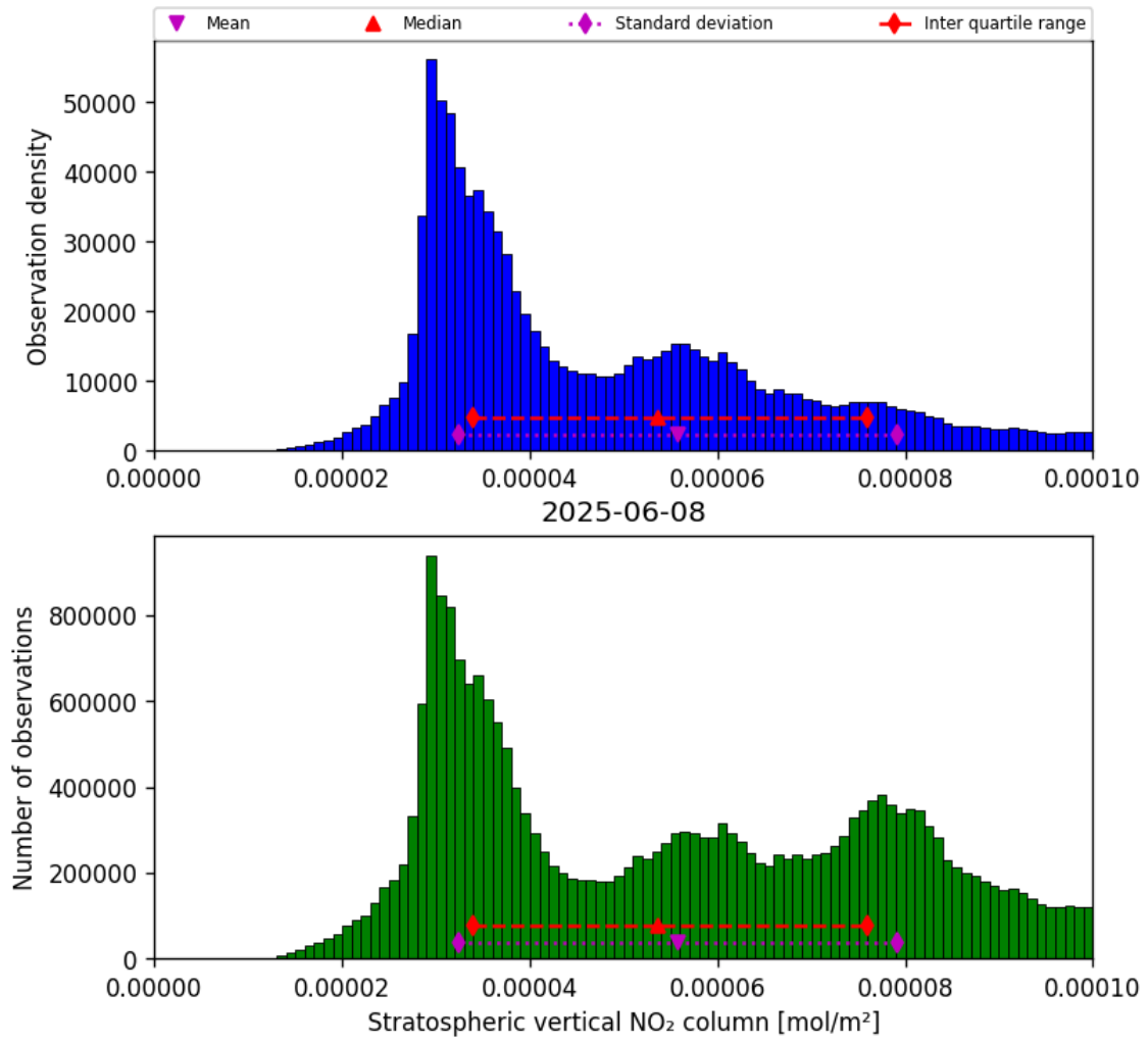
Figure 34: Histogram of “Stratospheric vertical NO 2 column” for 2025-06-08 to 2025-06-09
