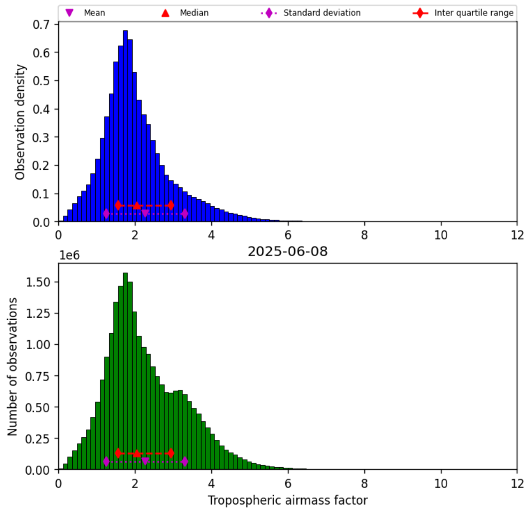
Figure 29: Histogram of “Tropospheric airmass factor” for 2025-06-08 to 2025-06-09
