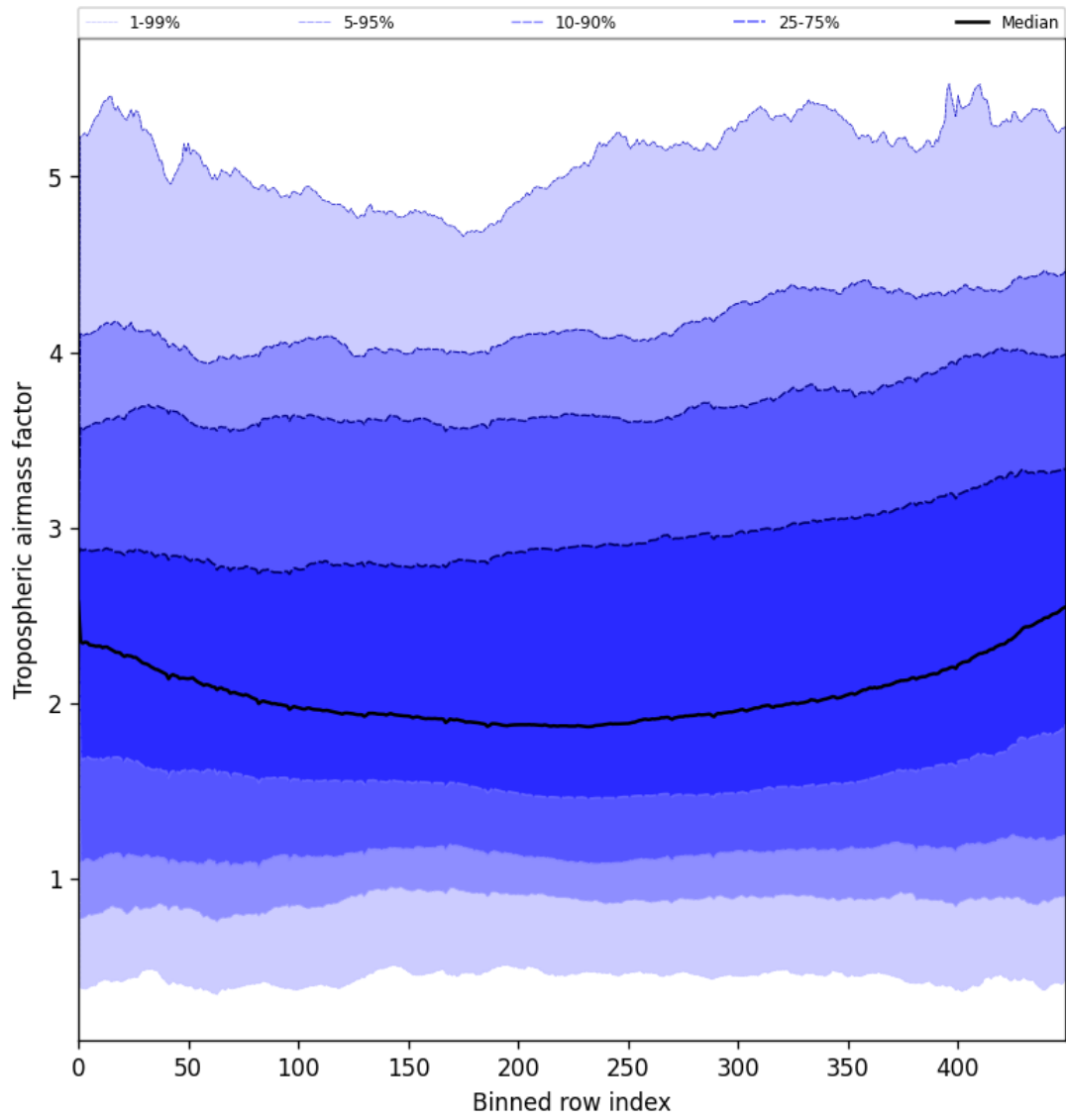
Figure 46: Along track statistics of “Tropospheric airmass factor” for 2025-06-08 to 2025-06-09
