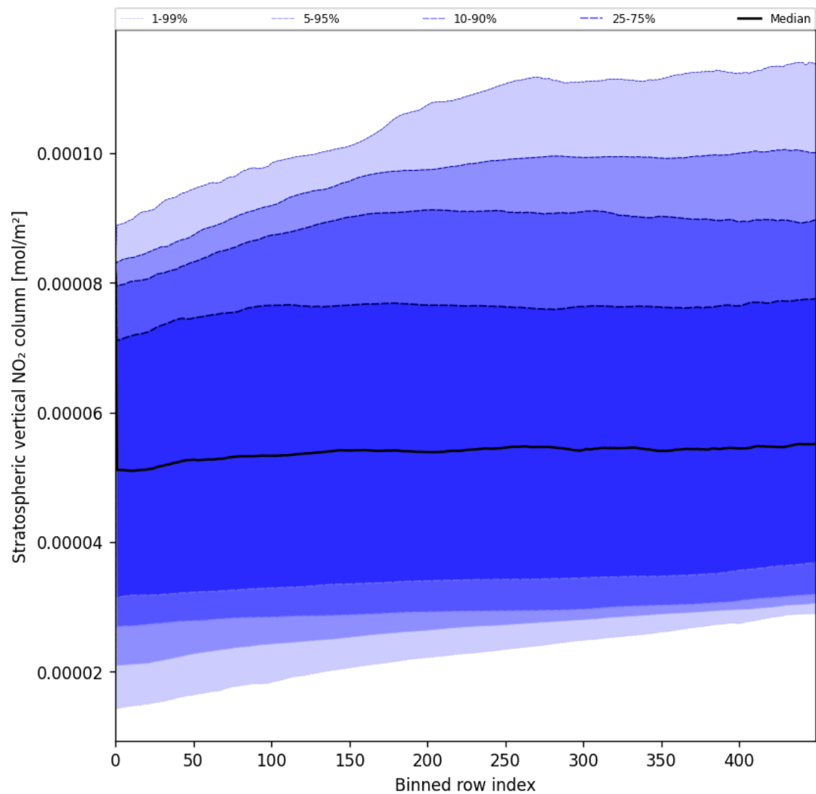
Figure 51: Along track statistics of “Stratospheric vertical NO 2 column” for 2025-06-08 to 2025-06-09
