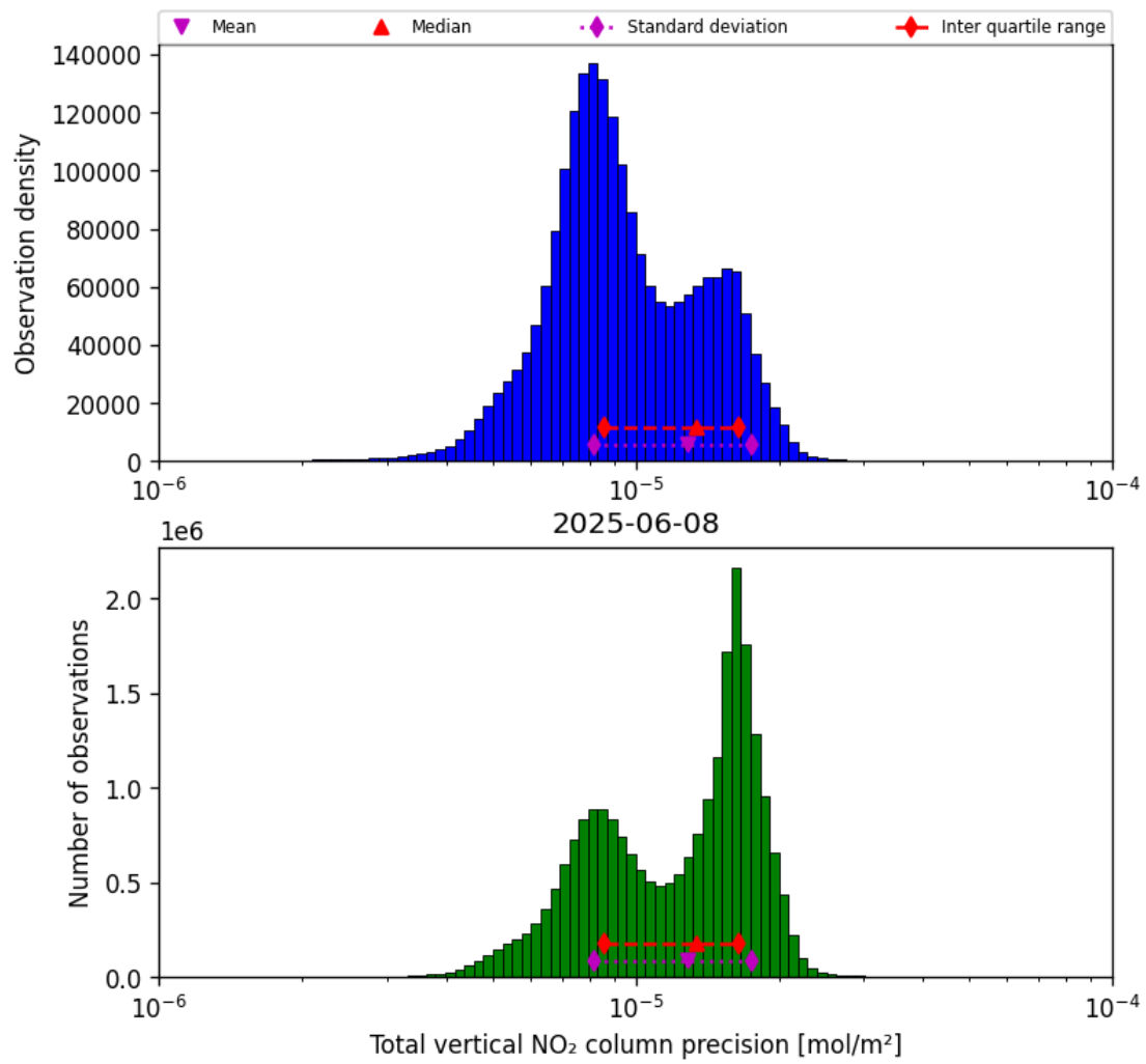
Figure 37: Histogram of “Total vertical NO 2 column precision” for 2025-06-08 to 2025-06-09
