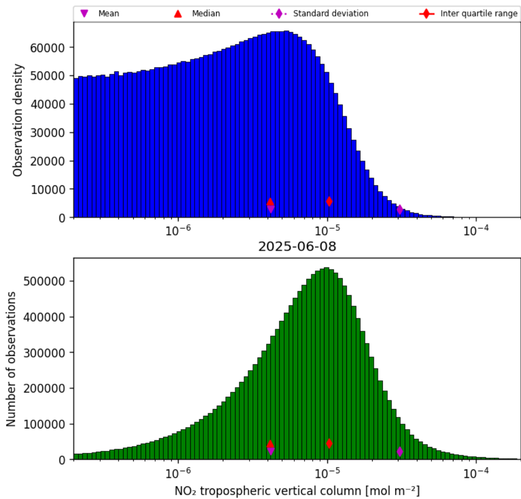
Figure 27: Histogram of “NO 2 tropospheric vertical column” for 2025-06-08 to 2025-06-09
