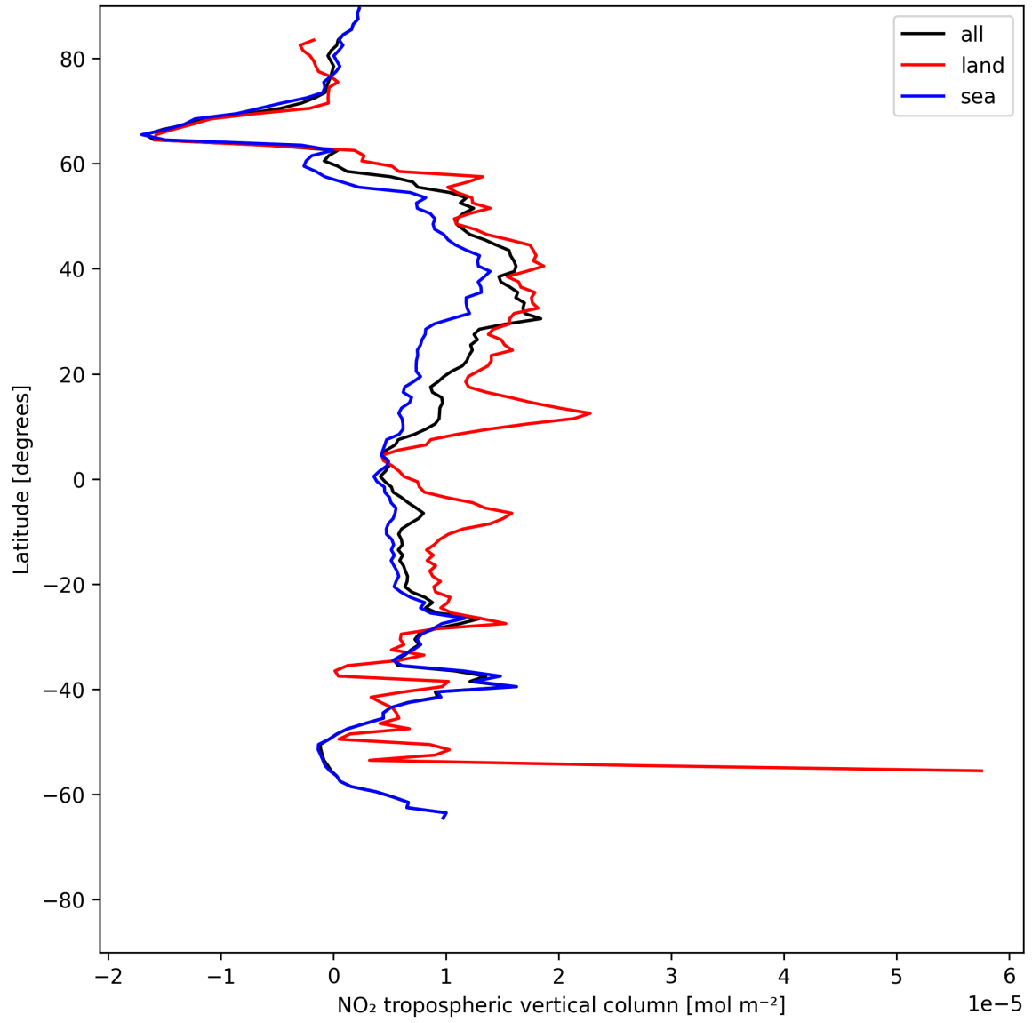
Figure 10: Zonal average of “NO 2 tropospheric vertical column” for 2025-06-08 to 2025-06-09.
