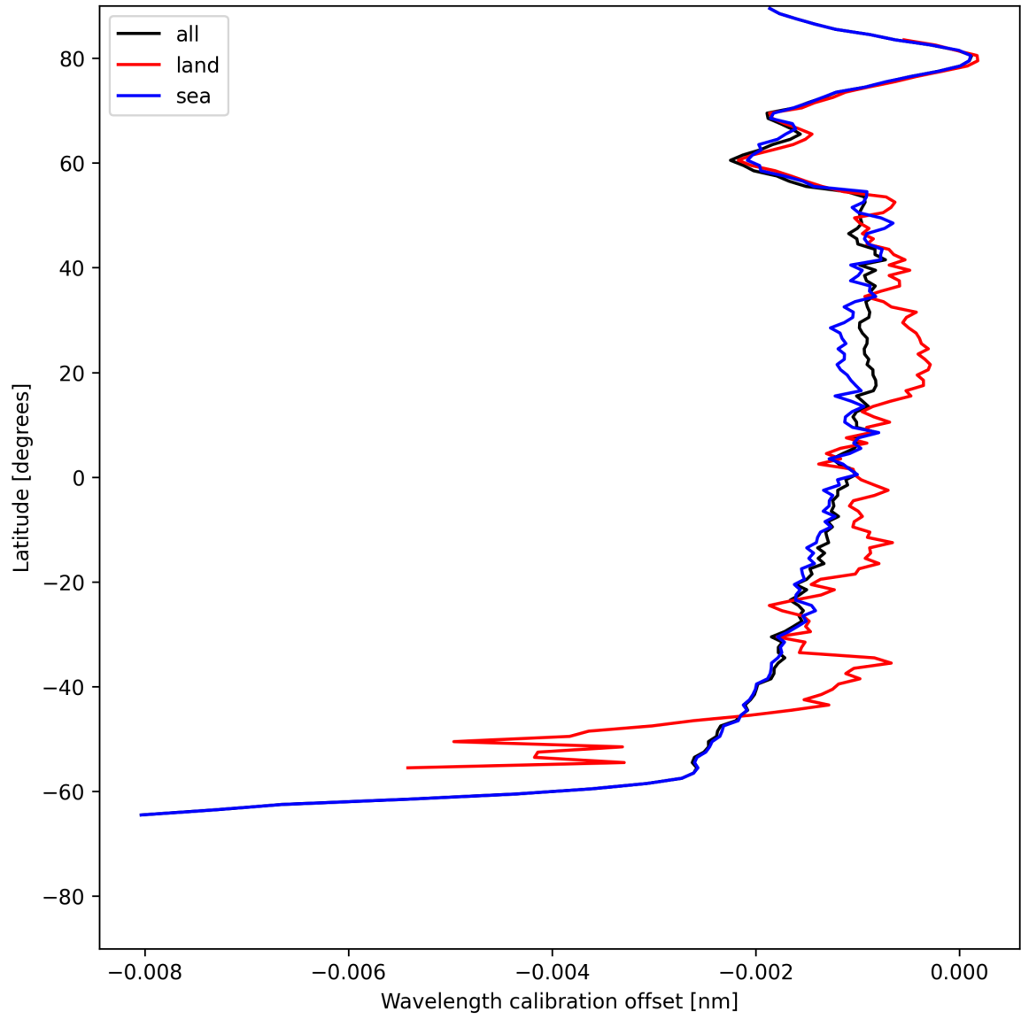
Figure 16: Zonal average of “Wavelength calibration offset” for 2025-06-08 to 2025-06-09.
