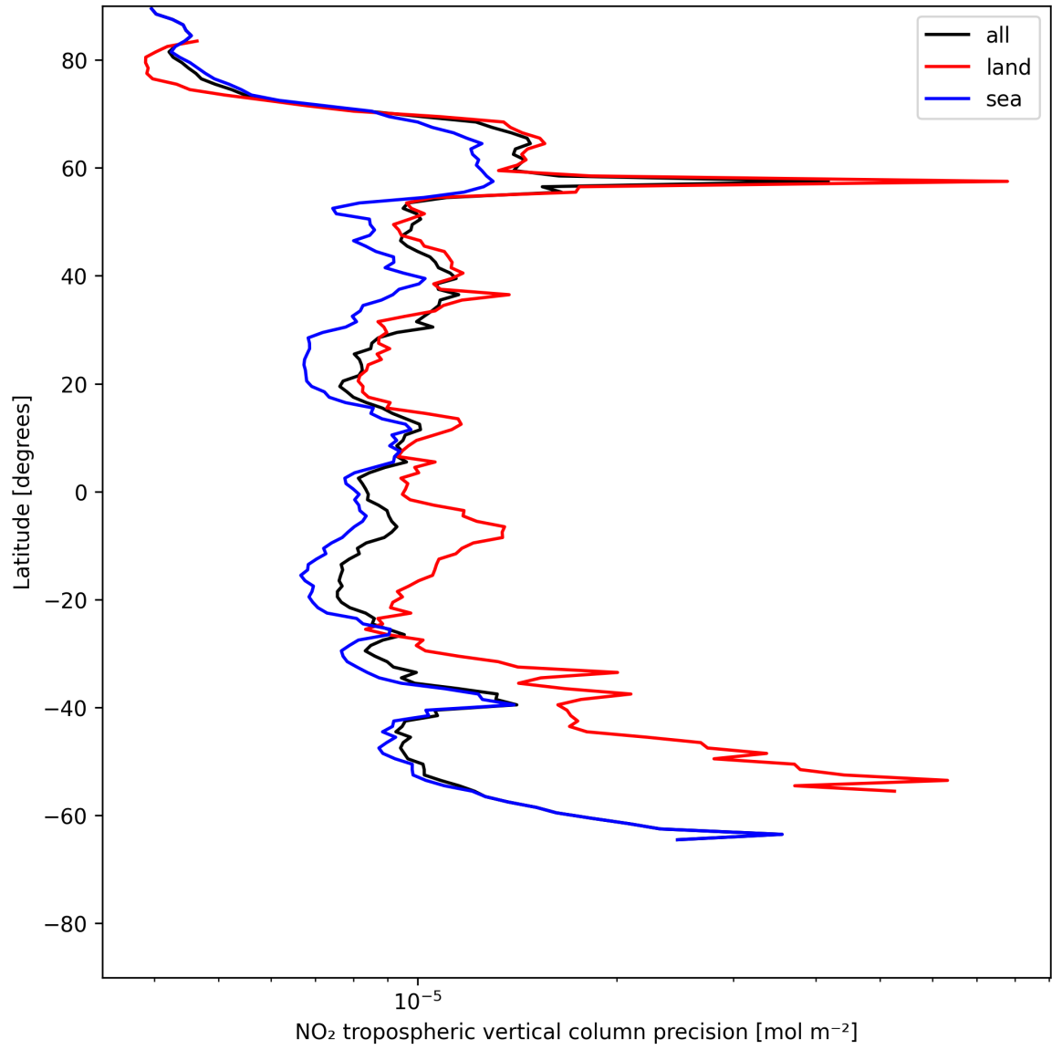
Figure 11: Zonal average of “NO 2 tropospheric vertical column precision” for 2025-06-08 to 2025-06-09.
