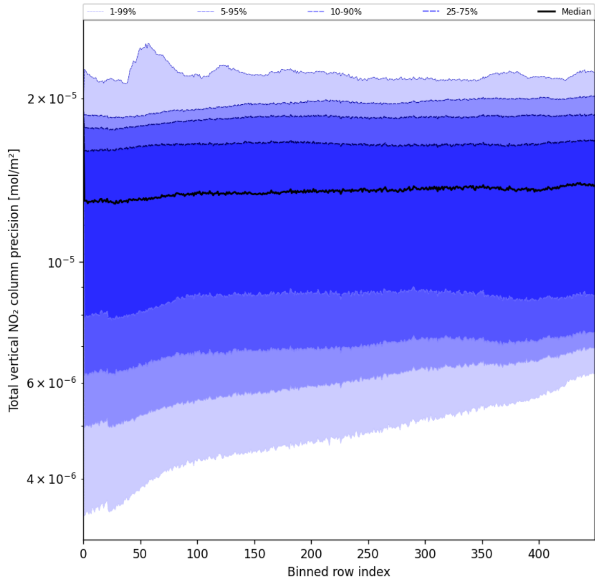
Figure 54: Along track statistics of “Total vertical NO 2 column precision” for 2025-06-08 to 2025-06-09
