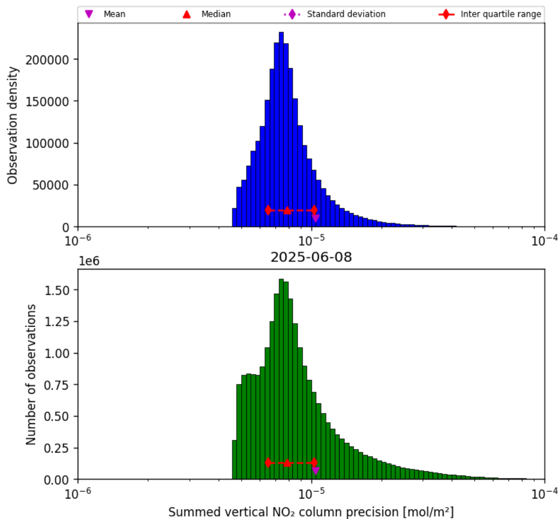
Figure 39: Histogram of “Summed vertical NO 2 column precision” for 2025-06-08 to 2025-06-09
