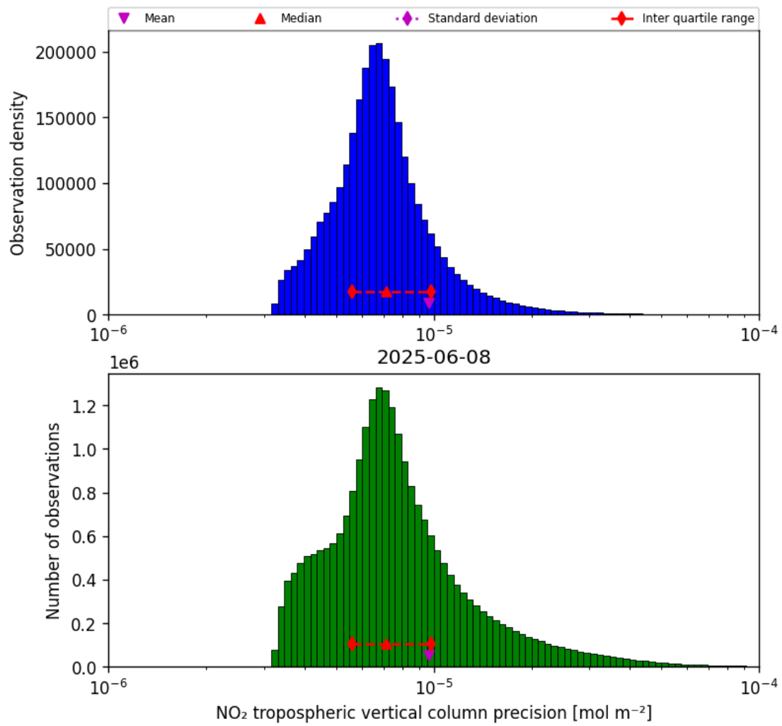
Figure 28: Histogram of “NO 2 tropospheric vertical column precision” for 2025-06-08 to 2025-06-09
