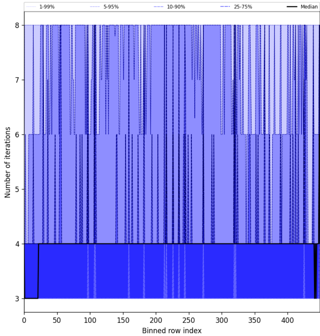
Figure 49: Along track statistics of “Number of iterations” for 2025-06-08 to 2025-06-09
