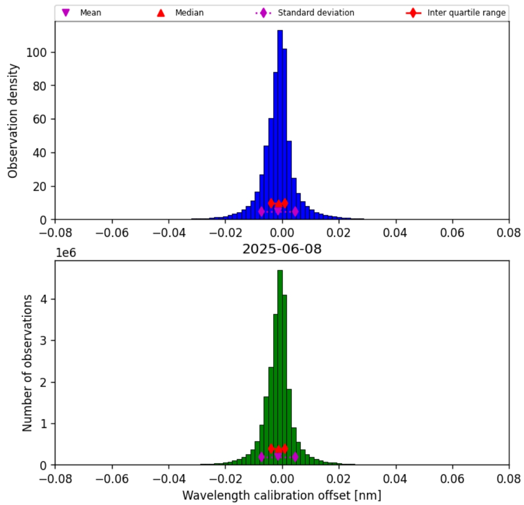
Figure 33: Histogram of “Wavelength calibration offset” for 2025-06-08 to 2025-06-09
