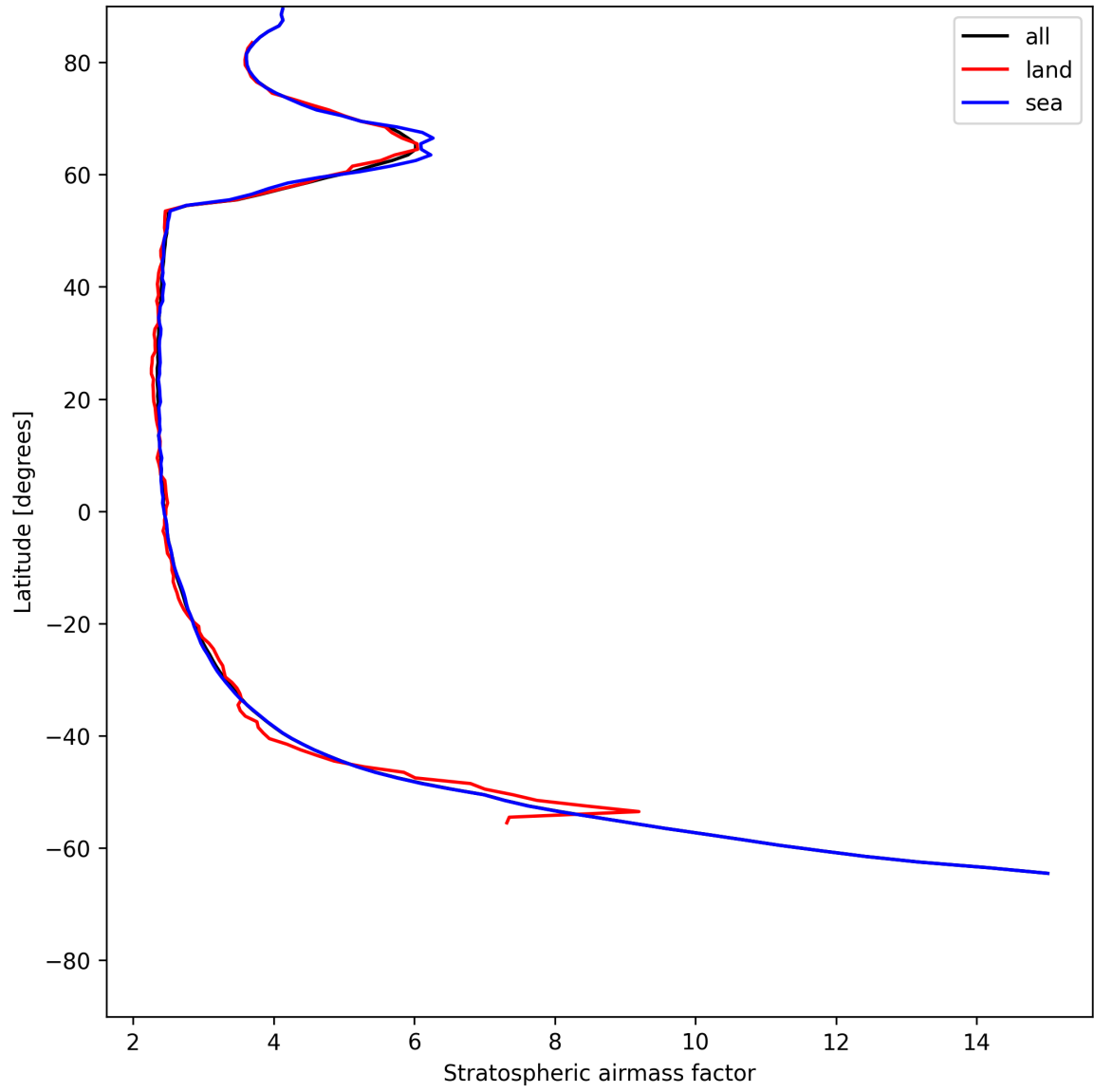
Figure 25: Zonal average of “Stratospheric air mass factor” for 2025-06-08 to 2025-06-09.
