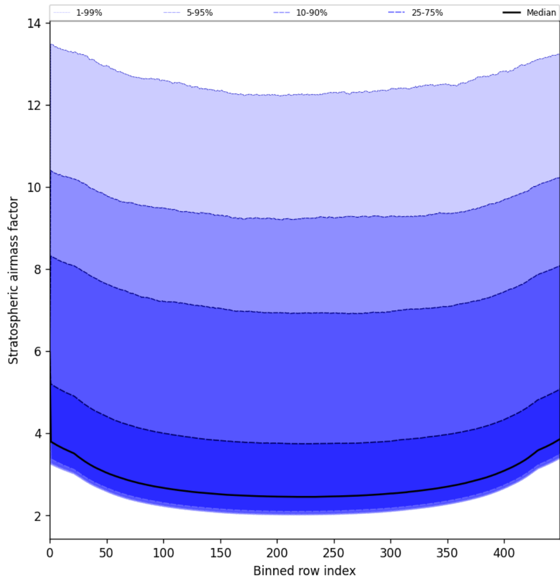
Figure 59: Along track statistics of “Stratospheric airmass factor” for 2025-06-08 to 2025-06-09
