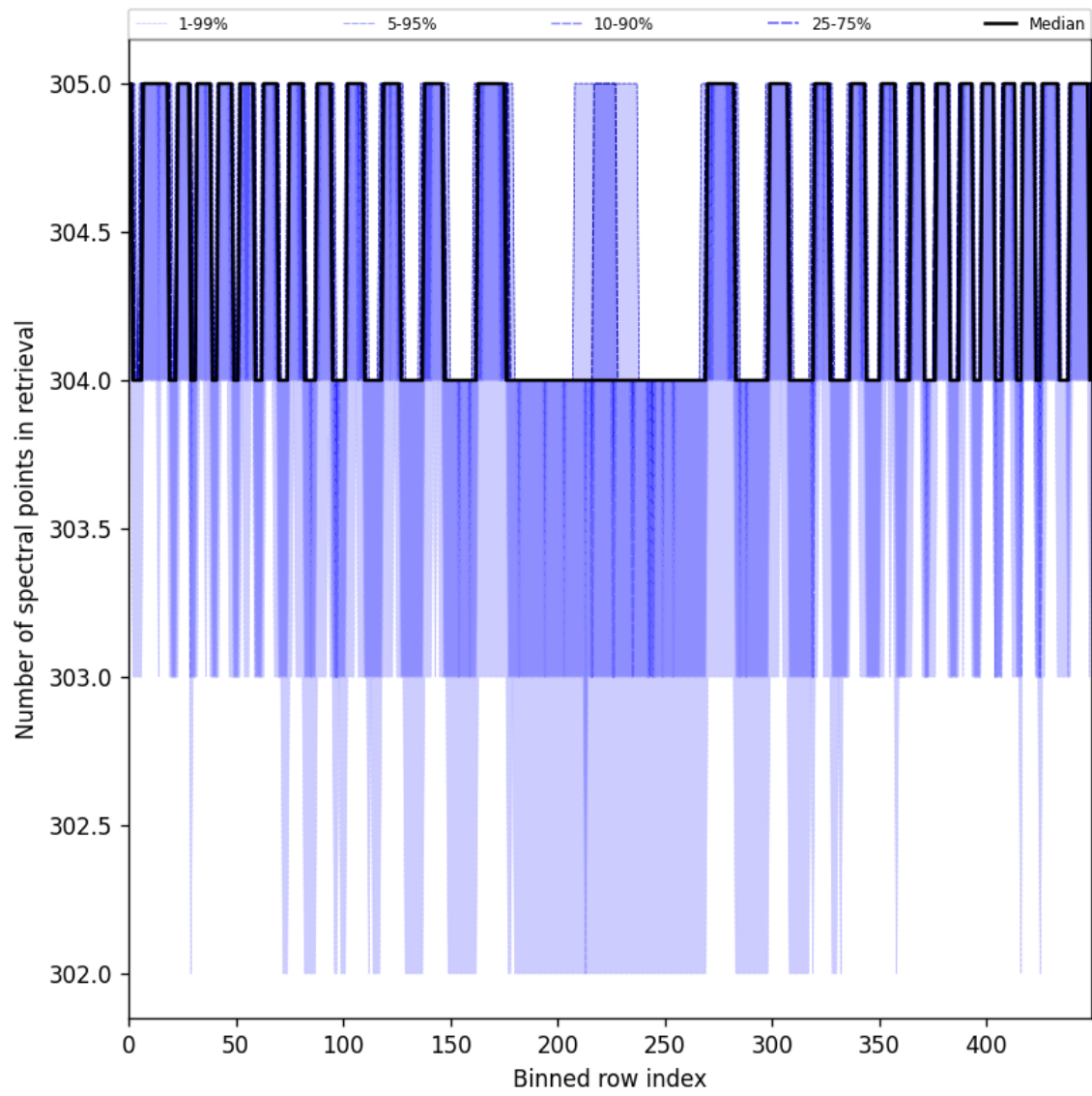
Figure 48: Along track statistics of “Number of spectral points in retrieval” for 2025-06-08 to 2025-06-09
