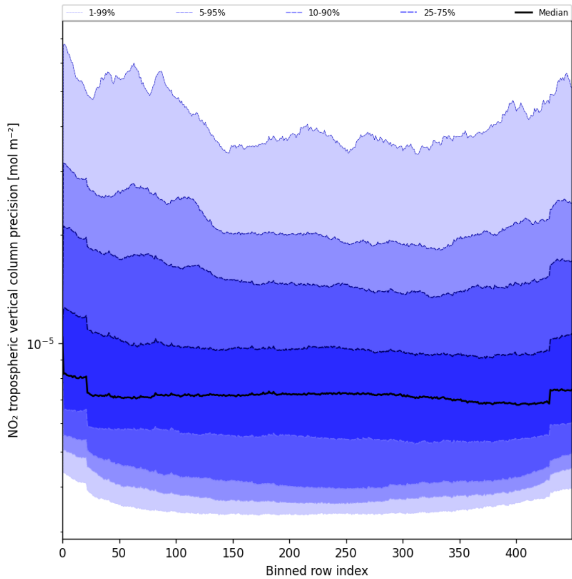
Figure 45: Along track statistics of “NO 2 tropospheric vertical column precision” for 2025-06-08 to 2025-06-09
