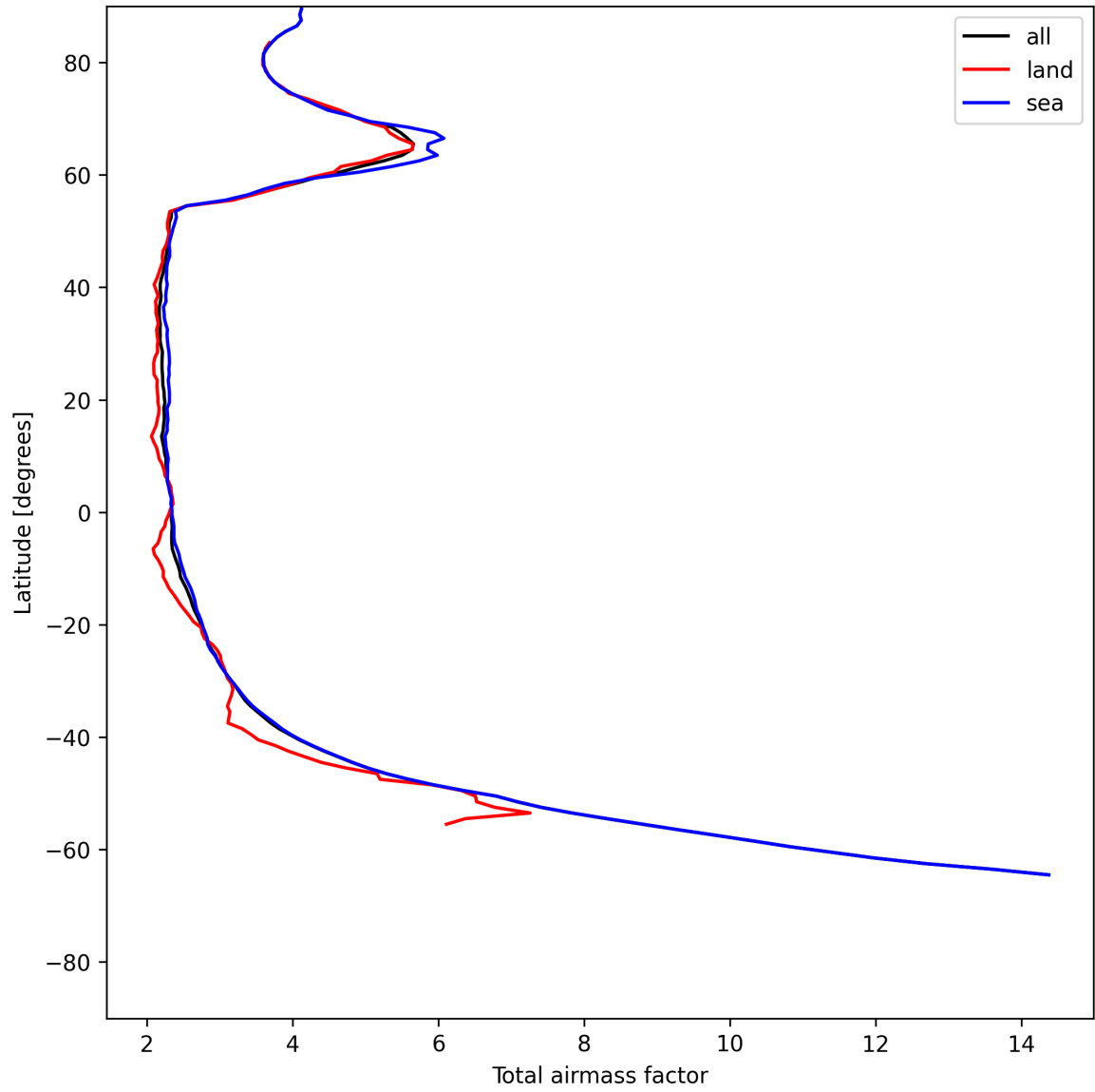
Figure 13: Zonal average of “Total airmass factor” for 2025-06-08 to 2025-06-09.
