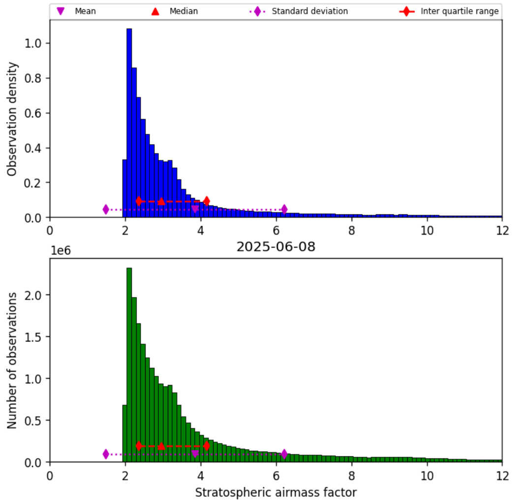
Figure 42: Histogram of “Stratospheric airmass factor” for 2025-06-08 to 2025-06-09
