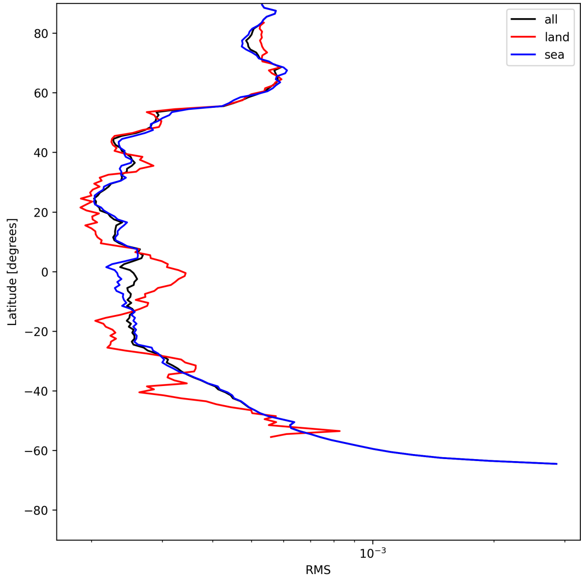
Figure 24: Zonal average of “RMS” for 2025-06-08 to 2025-06-09.
