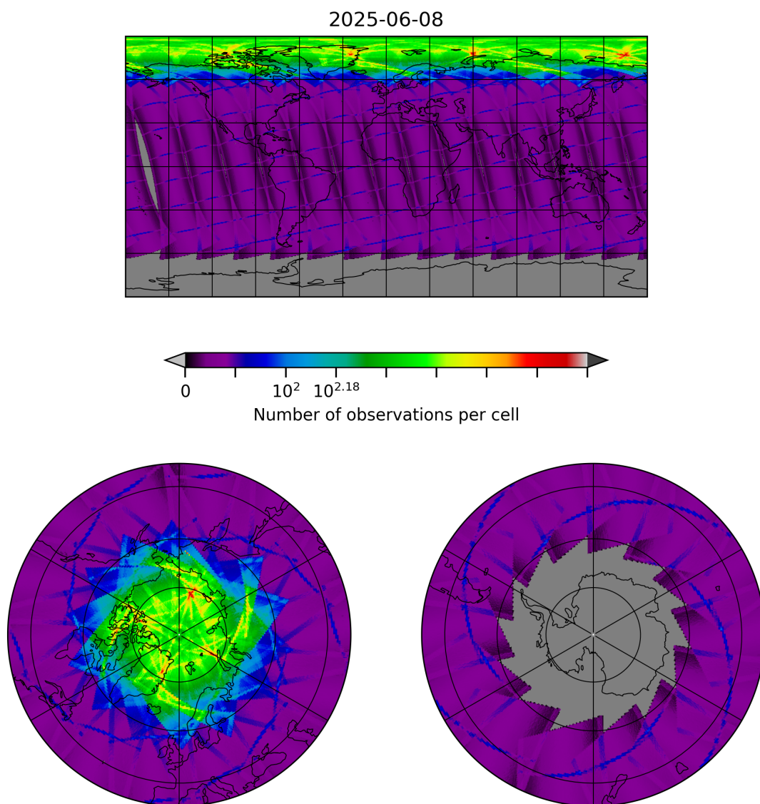
Figure 8: Map of the number of observations for 2025-06-08 to 2025-06-09
