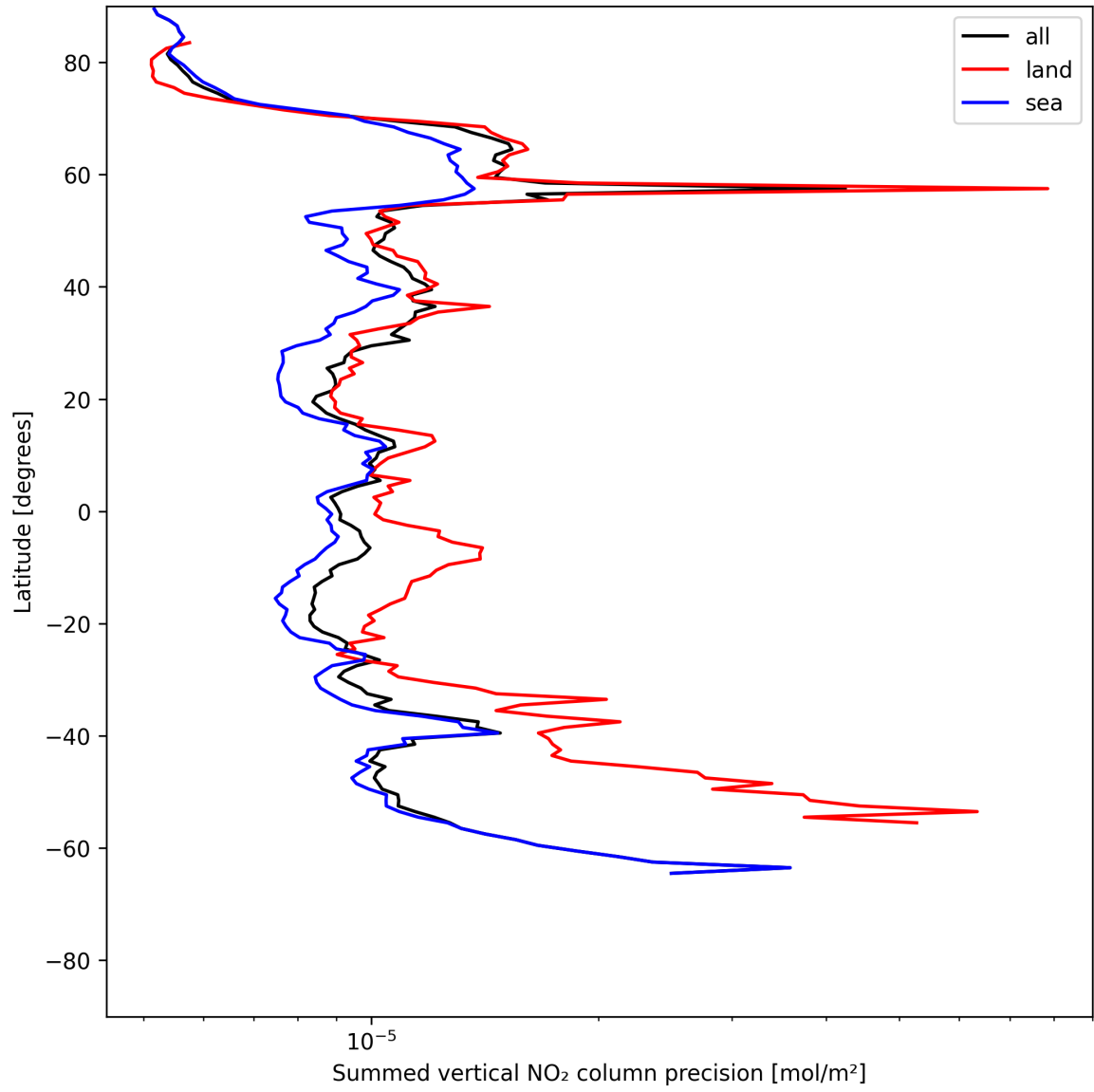
Figure 22: Zonal average of “Summed vertical NO 2 column precision” for 2025-06-08 to 2025-06-09.
