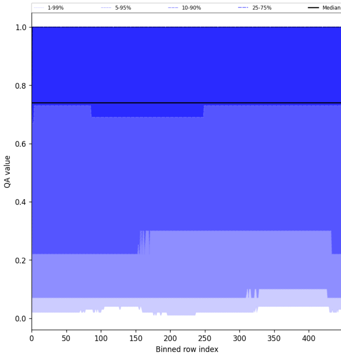
Figure 43: Along track statistics of “QA value” for 2025-06-08 to 2025-06-09
