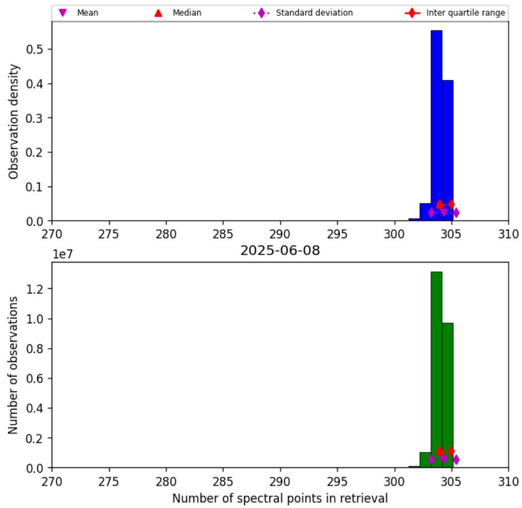
Figure 31: Histogram of “Number of spectral points in retrieval” for 2025-06-08 to 2025-06-09
