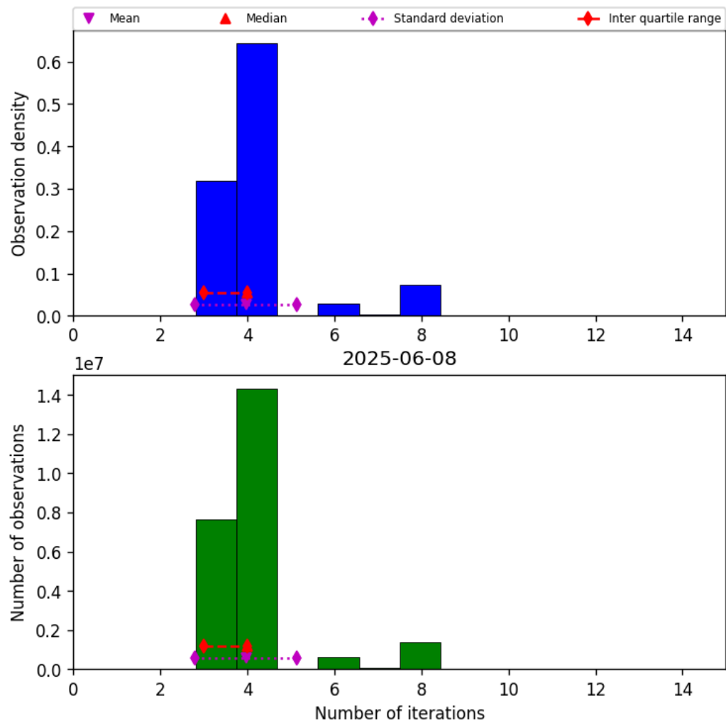
Figure 32: Histogram of “Number of iterations” for 2025-06-08 to 2025-06-09
