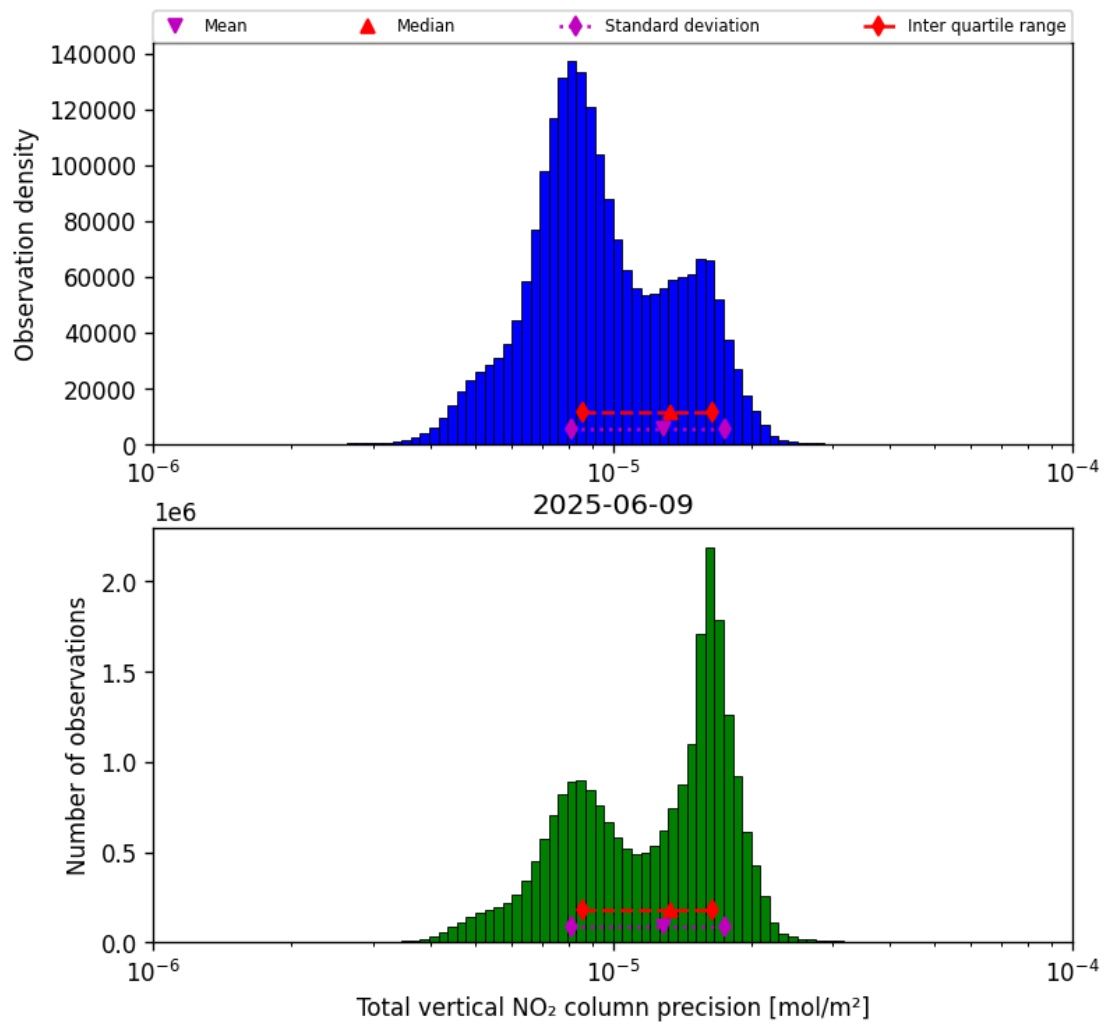
Figure 37: Histogram of “Total vertical NO 2 column precision” for 2025-06-09 to 2025-06-09
