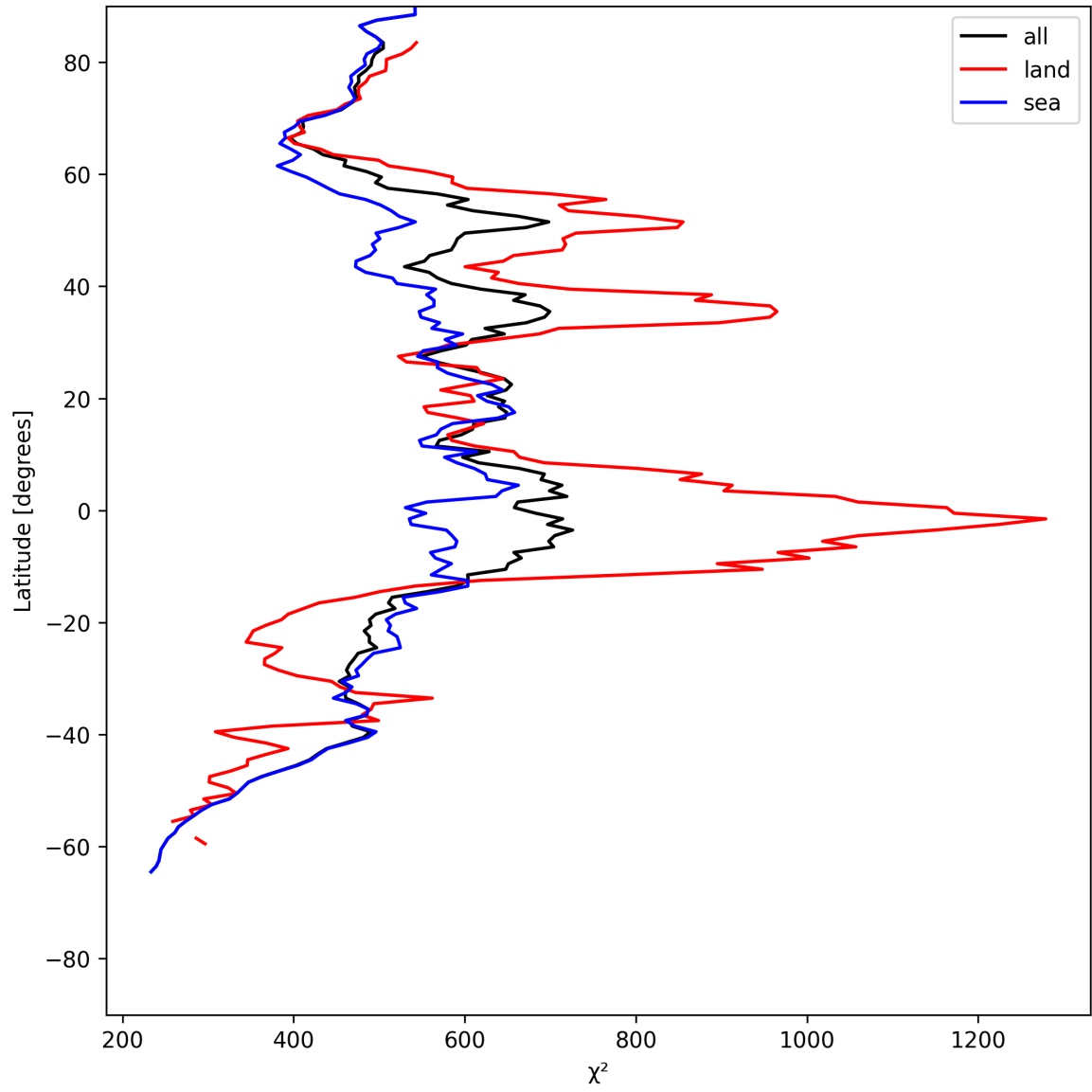
Figure 23: Zonal average of “ \chi^2 ” for 2025-06-09 to 2025-06-09.
