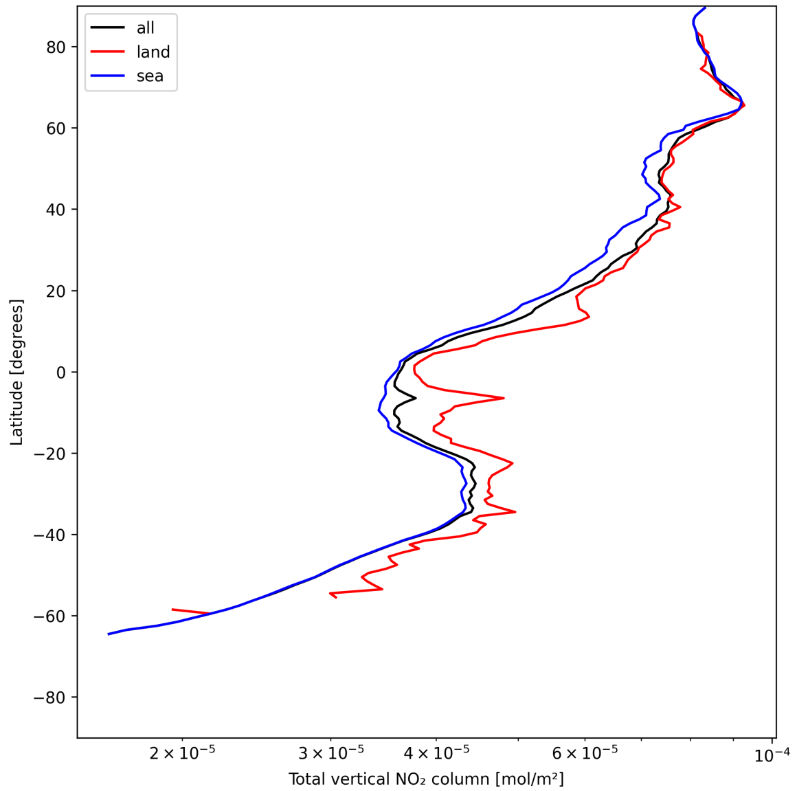
Figure 19: Zonal average of “Total vertical NO 2 column” for 2025-06-09 to 2025-06-09.
