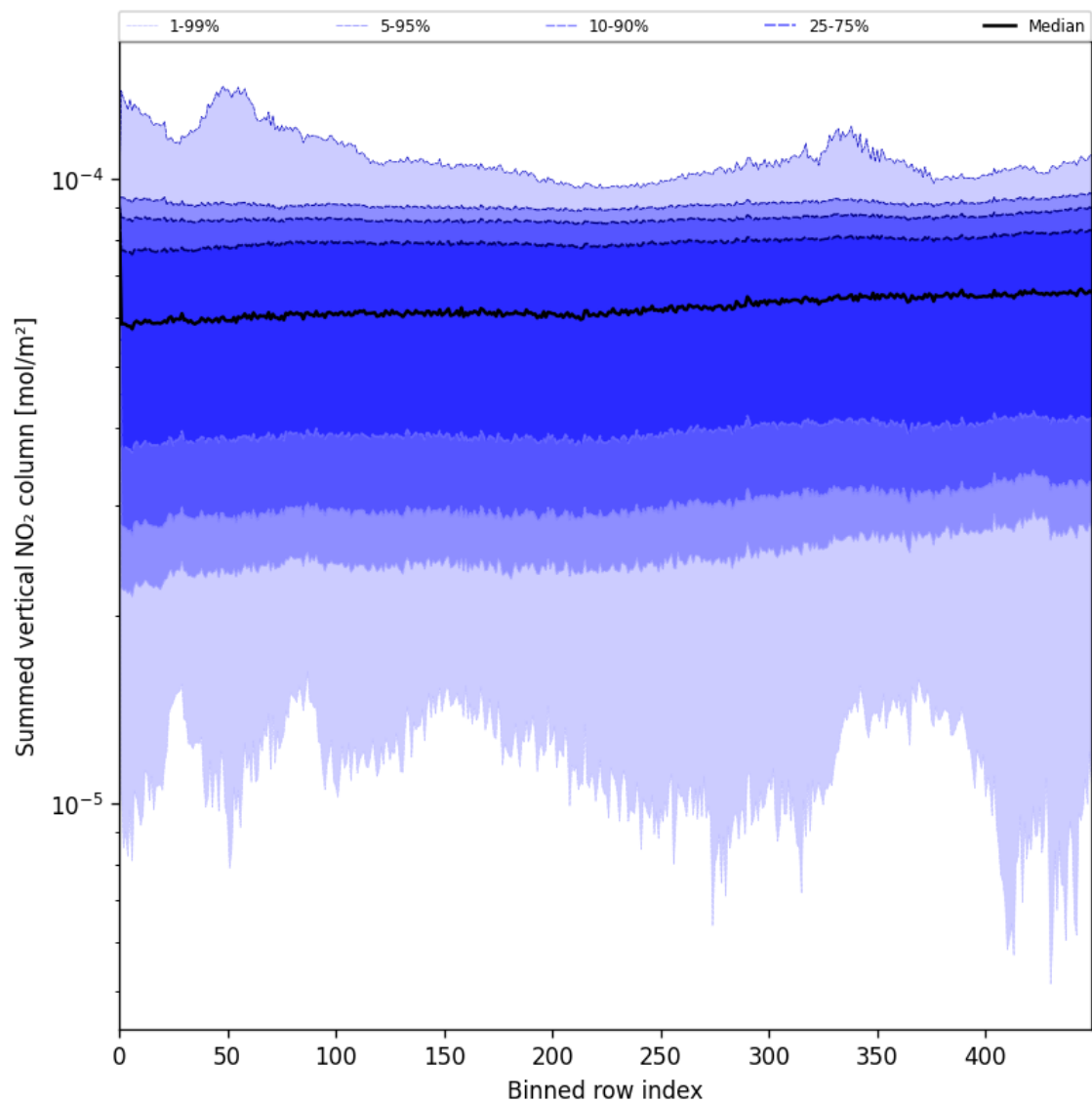
Figure 55: Along track statistics of “Summed vertical NO 2 column” for 2025-06-09 to 2025-06-09
