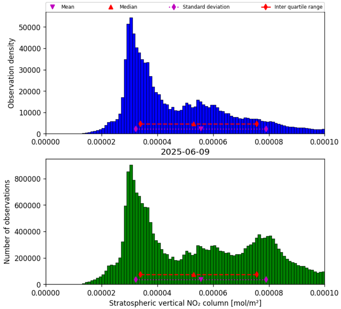
Figure 34: Histogram of “Stratospheric vertical NO 2 column” for 2025-06-09 to 2025-06-09
