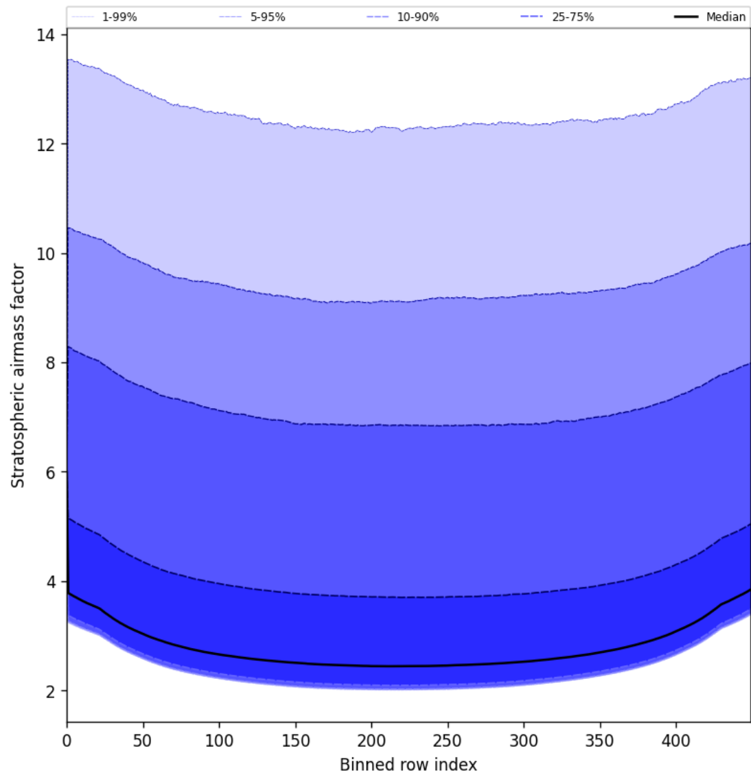
Figure 59: Along track statistics of “Stratospheric airmass factor” for 2025-06-09 to 2025-06-09
