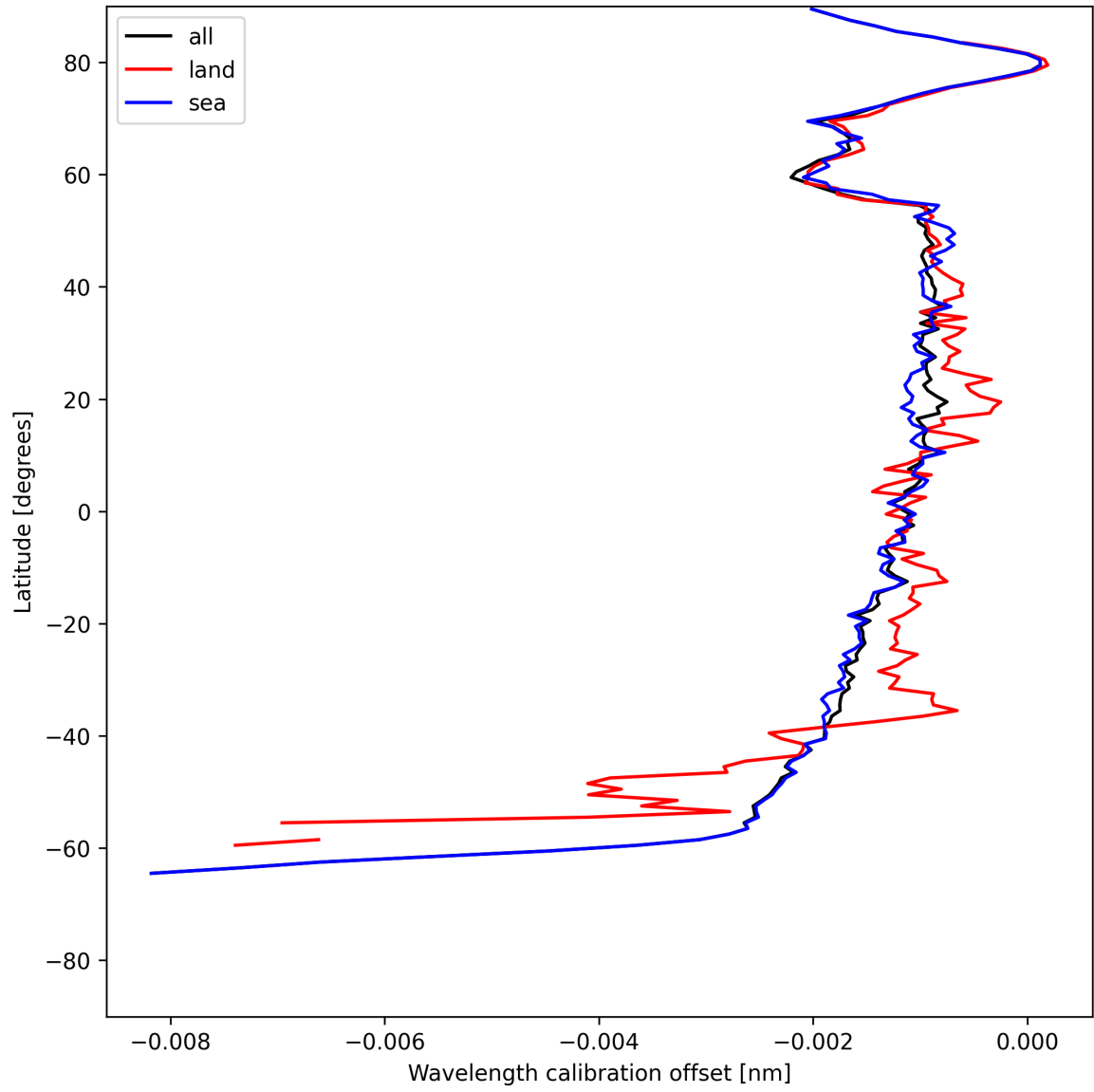
Figure 16: Zonal average of “Wavelength calibration offset” for 2025-06-09 to 2025-06-09.
