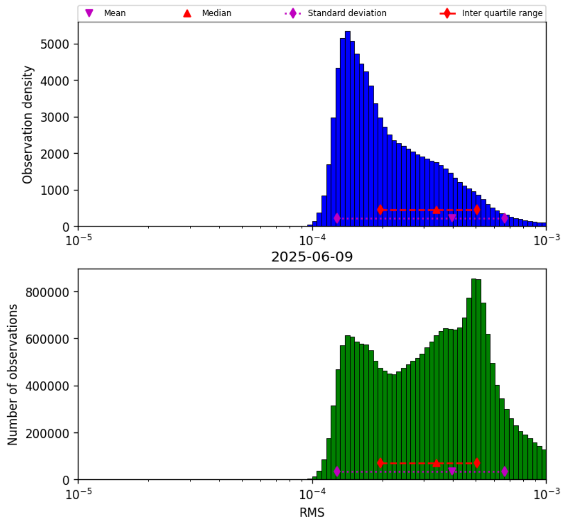
Figure 41: Histogram of “RMS” for 2025-06-09 to 2025-06-09
