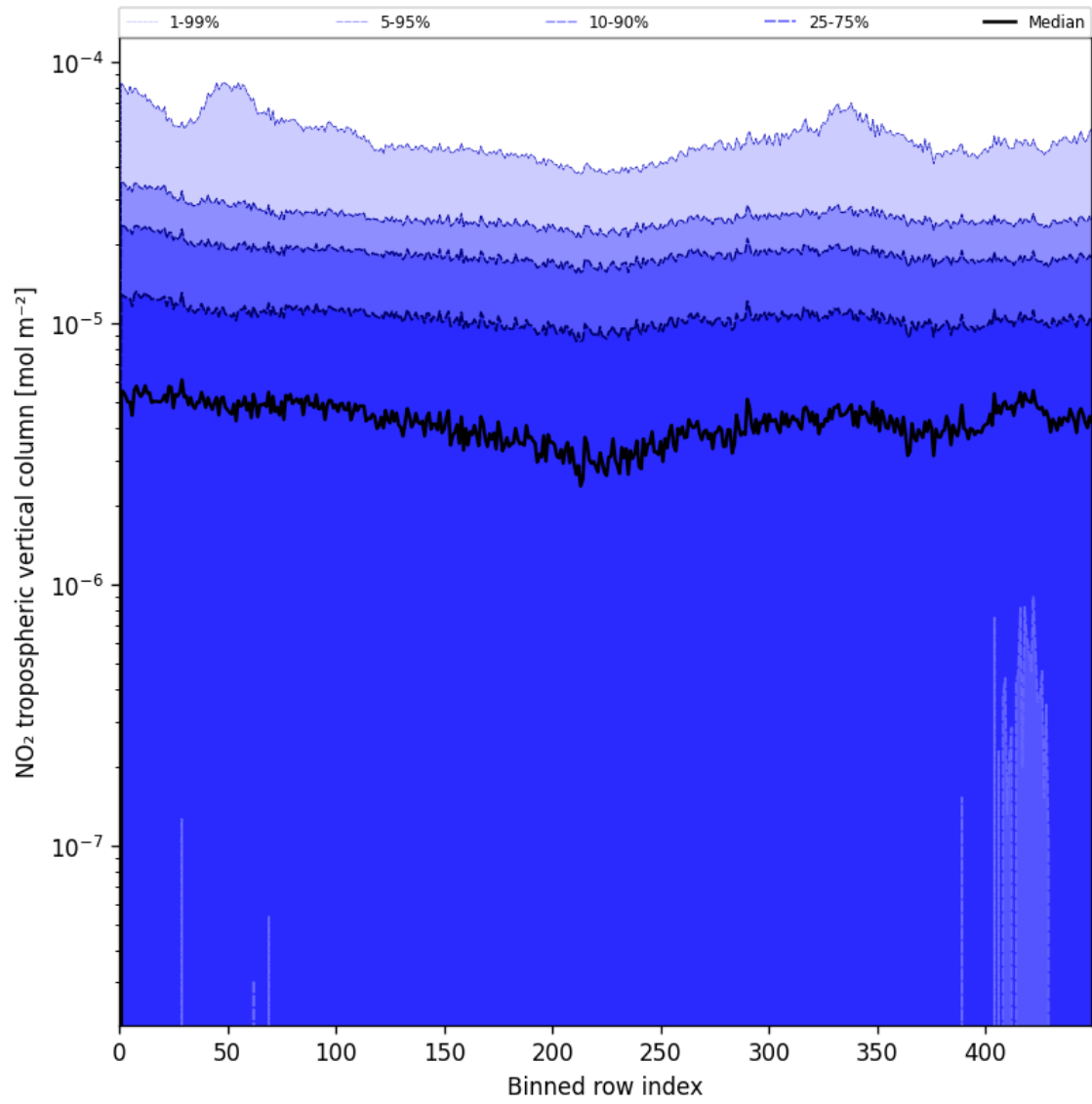
Figure 44: Along track statistics of “NO 2 tropospheric vertical column” for 2025-06-09 to 2025-06-09
