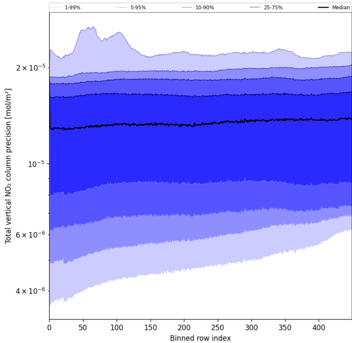
Figure 54: Along track statistics of “Total vertical NO 2 column precision” for 2025-06-09 to 2025-06-09
