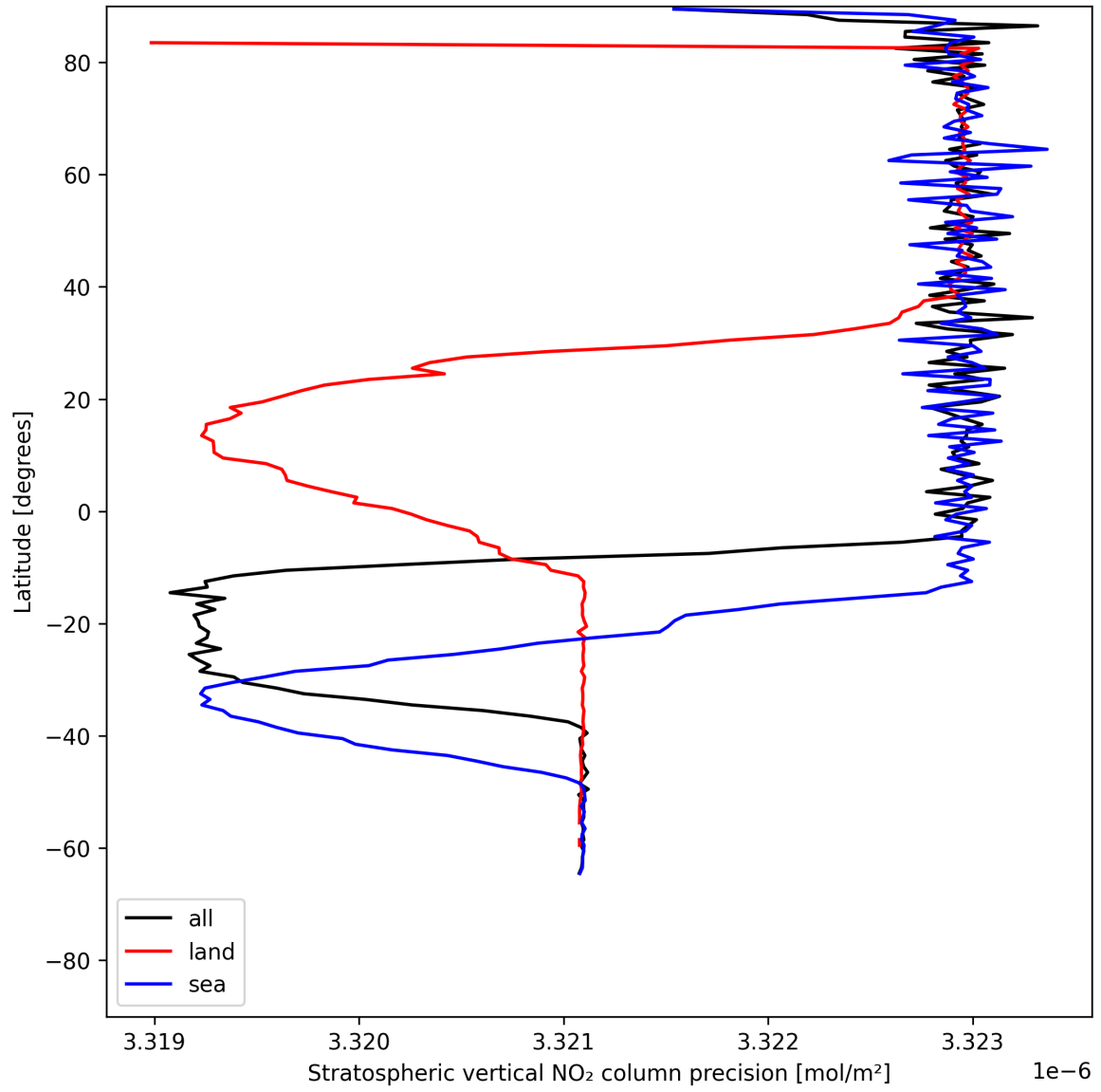
Figure 18: Zonal average of “Stratospheric vertical NO 2 column precision” for 2025-06-09 to 2025-06-09.
