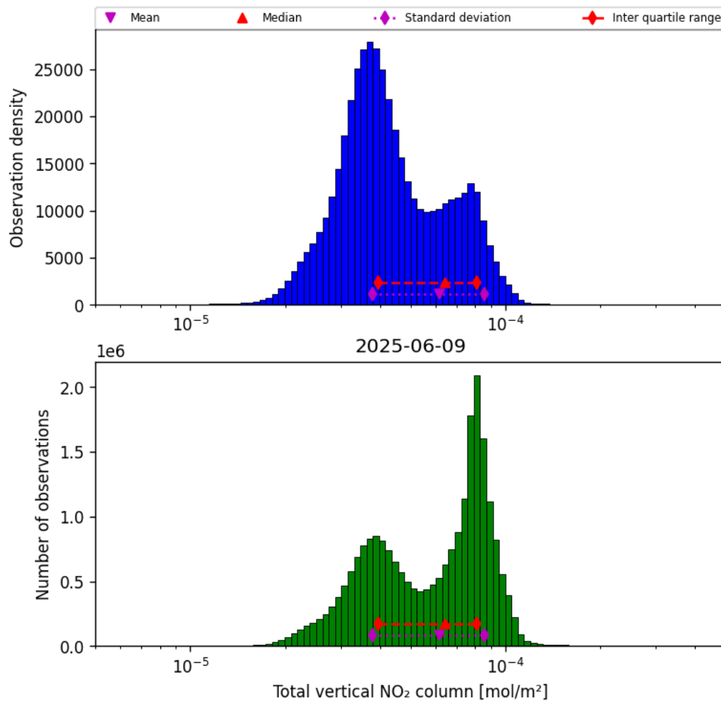
Figure 36: Histogram of “Total vertical NO 2 column” for 2025-06-09 to 2025-06-09
