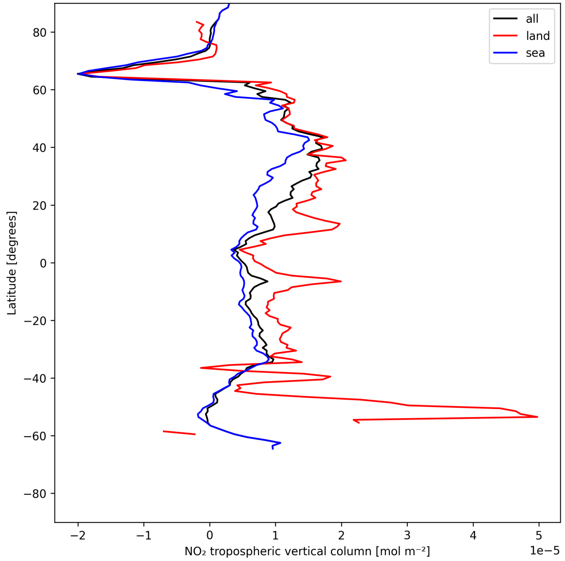
Figure 10: Zonal average of “NO 2 tropospheric vertical column” for 2025-06-09 to 2025-06-09.
