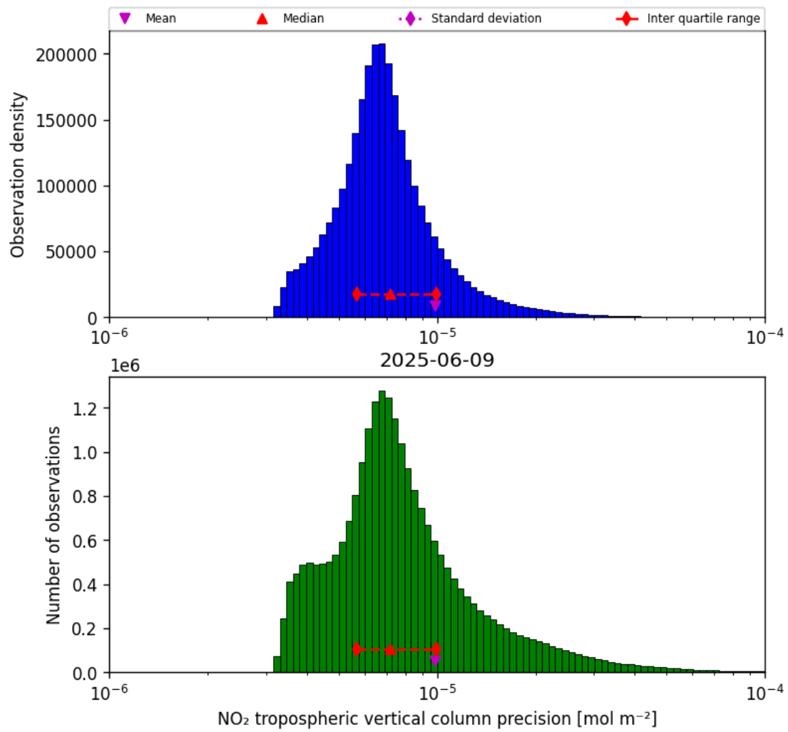
Figure 28: Histogram of "NO 2 tropospheric vertical column precision" for 2025-06-09 to 2025-06-09
