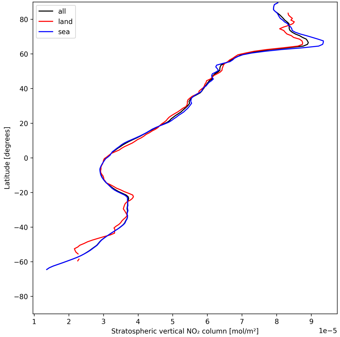
Figure 17: Zonal average of “Stratospheric vertical NO 2 column” for 2025-06-09 to 2025-06-09.
