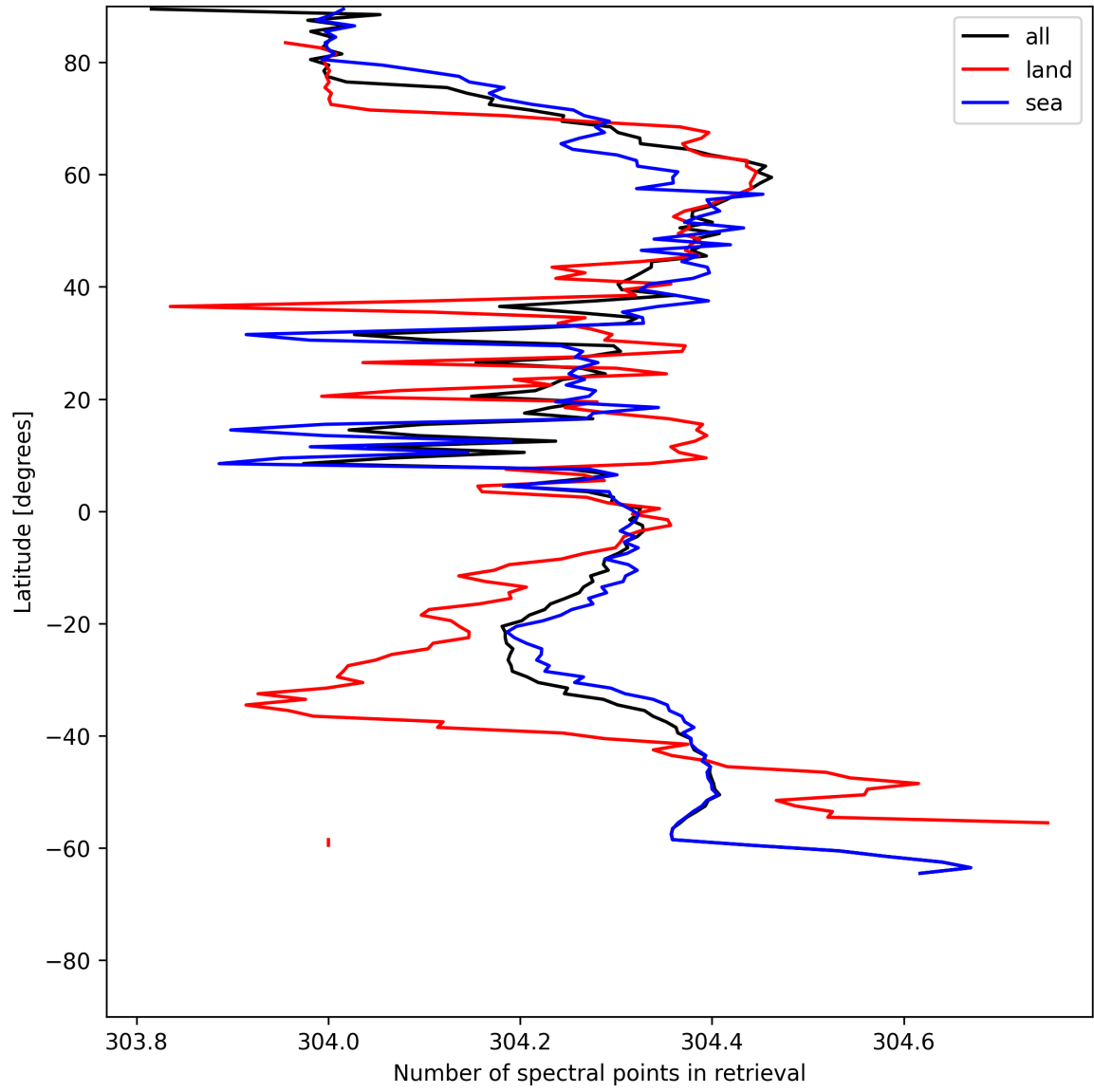
Figure 14: Zonal average of “Number of spectral points in retrieval” for 2025-06-09 to 2025-06-09.
