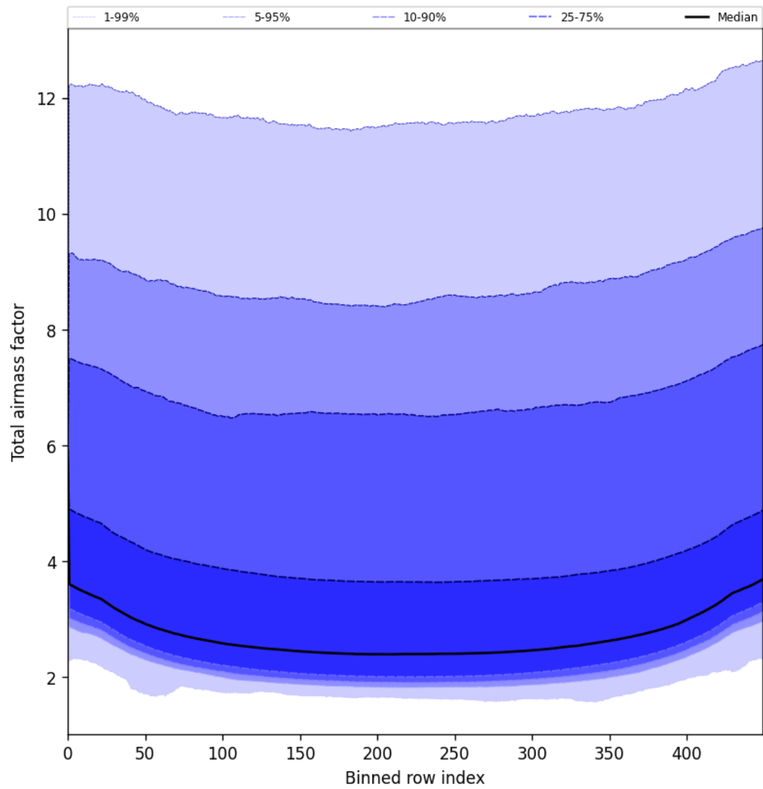
Figure 47: Along track statistics of “Total airmass factor” for 2025-06-09 to 2025-06-09
