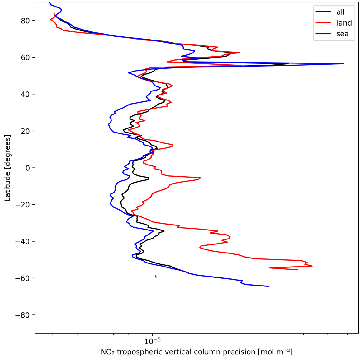
Figure 11: Zonal average of “NO 2 tropospheric vertical column precision” for 2025-06-09 to 2025-06-09.
