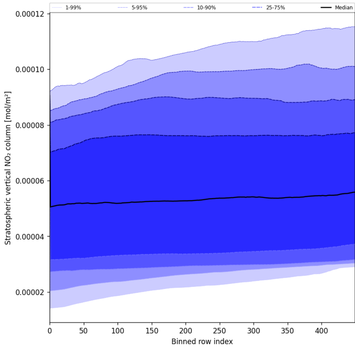
Figure 51: Along track statistics of “Stratospheric vertical NO 2 column” for 2025-06-09 to 2025-06-09
