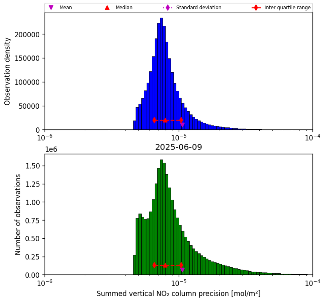
Figure 39: Histogram of "Summed vertical NO 2 column precision" for 2025-06-09 to 2025-06-09
