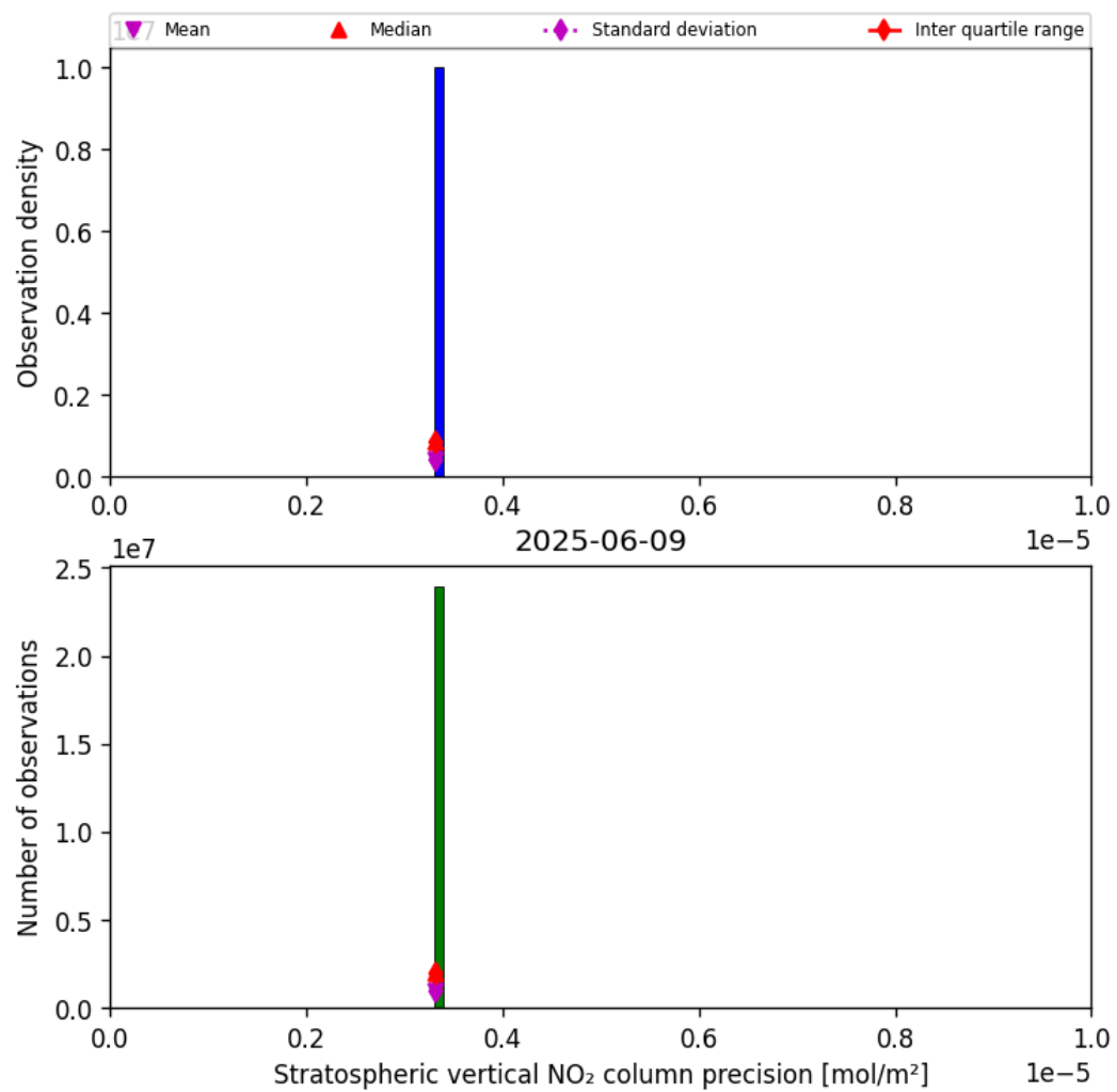
Figure 35: Histogram of “Stratospheric vertical NO 2 column precision” for 2025-06-09 to 2025-06-09
