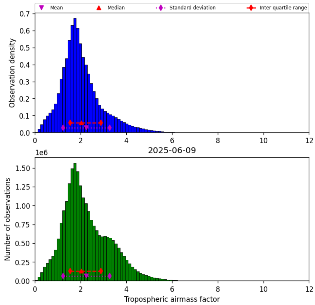
Figure 29: Histogram of “Tropospheric airmass factor” for 2025-06-09 to 2025-06-09
