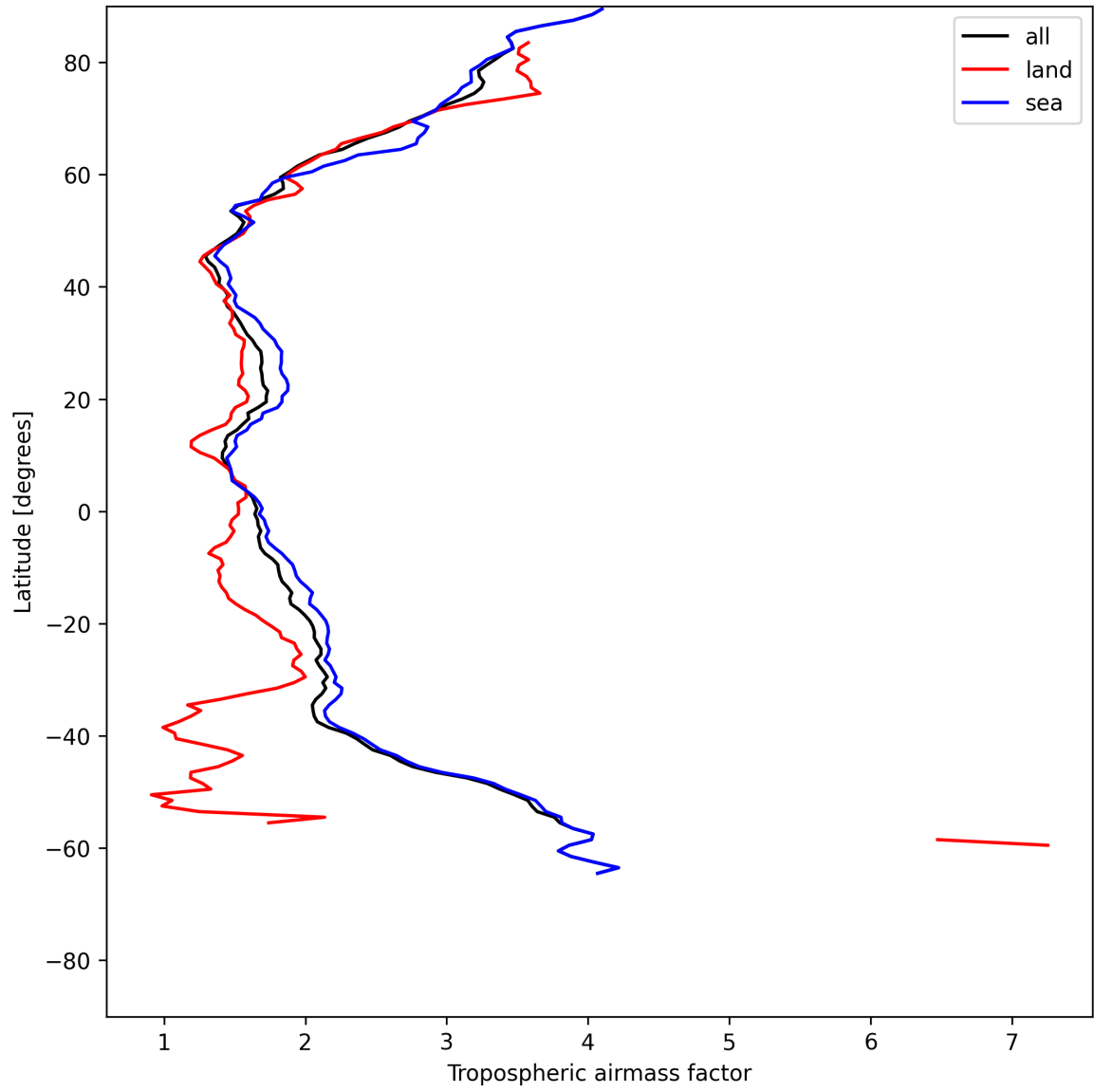
Figure 12: Zonal average of “Tropospheric airmass factor” for 2025-06-09 to 2025-06-09.
