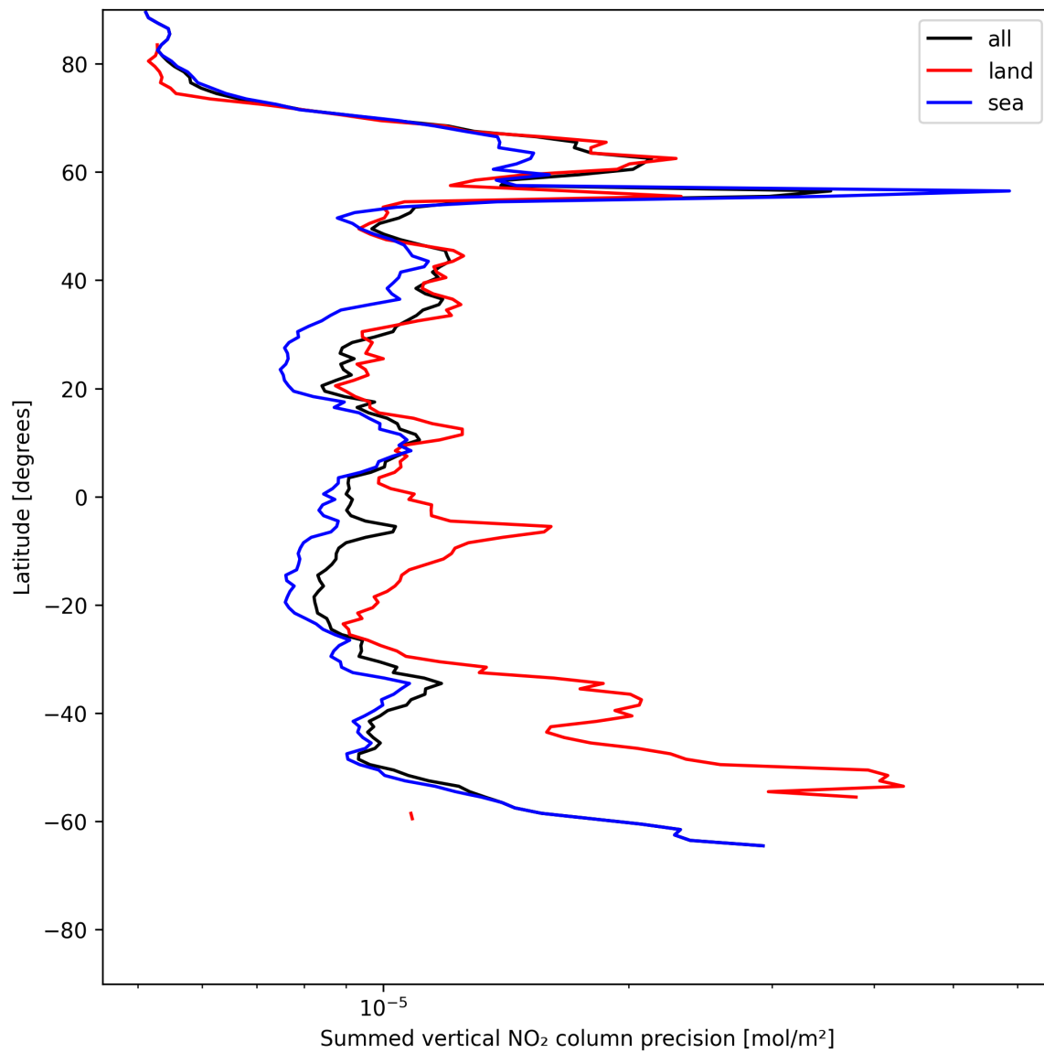
Figure 22: Zonal average of “Summed vertical NO 2 column precision” for 2025-06-09 to 2025-06-09.
