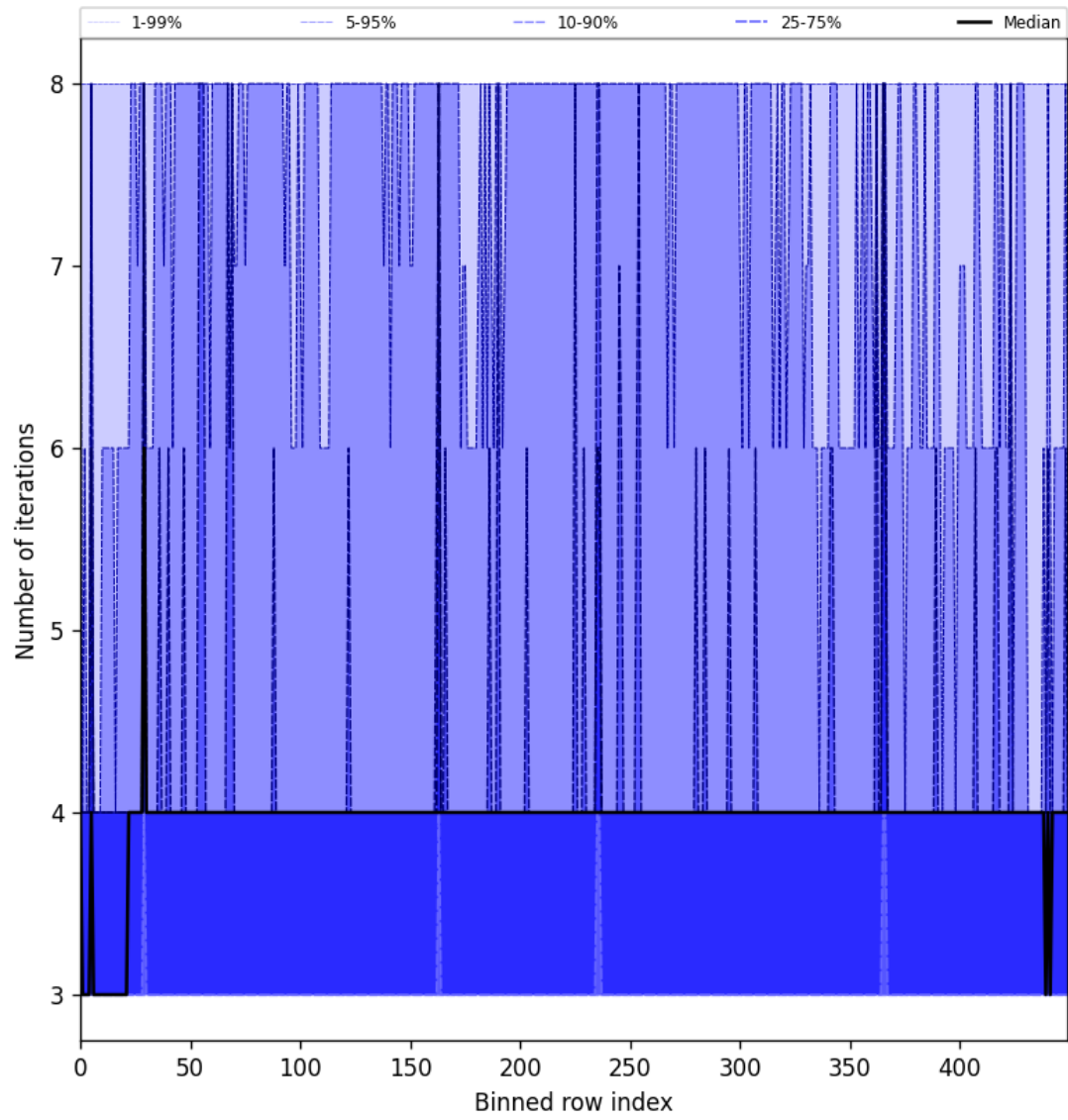
Figure 49: Along track statistics of “Number of iterations” for 2025-06-09 to 2025-06-09
