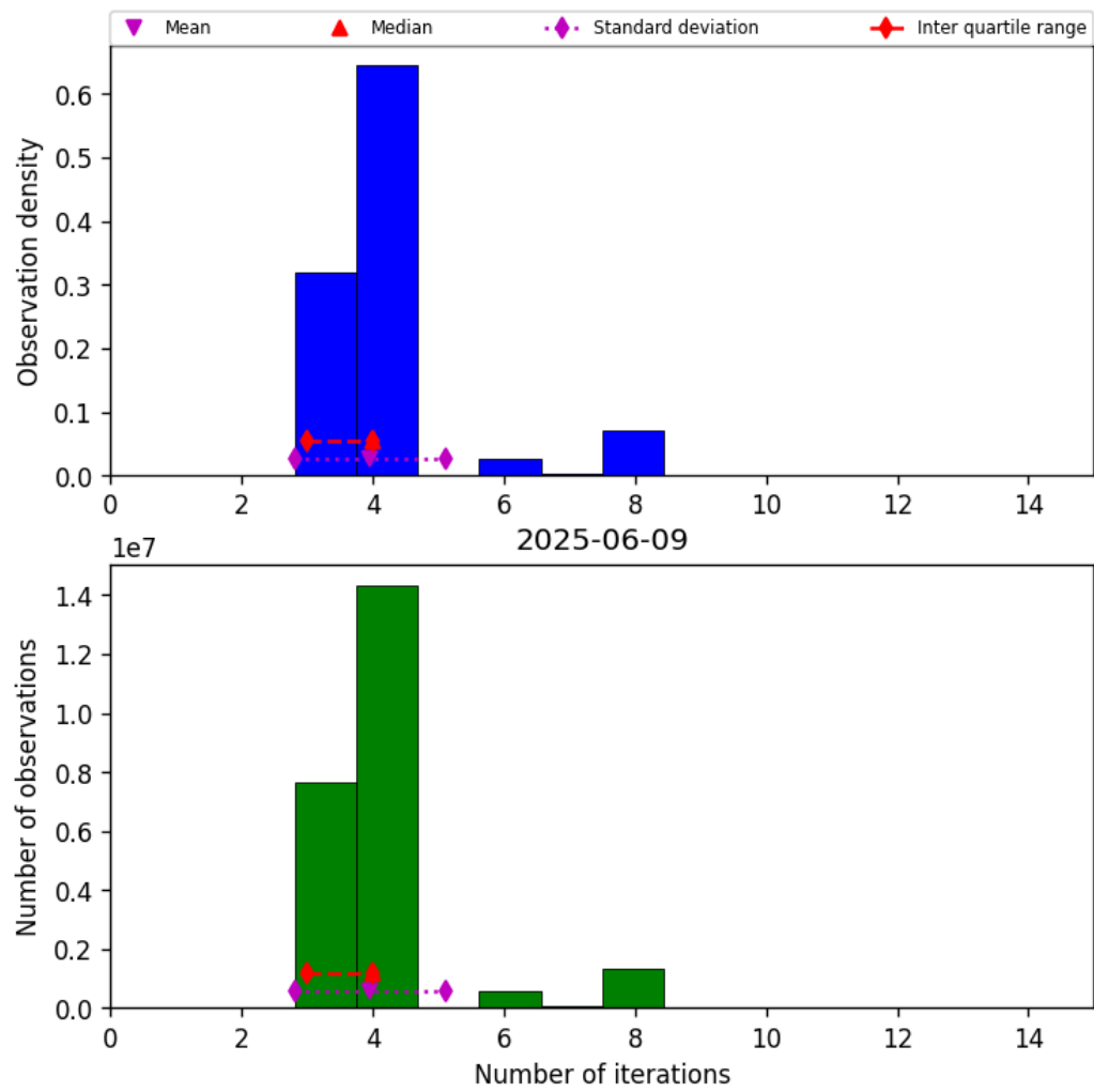
Figure 32: Histogram of “Number of iterations” for 2025-06-09 to 2025-06-09
