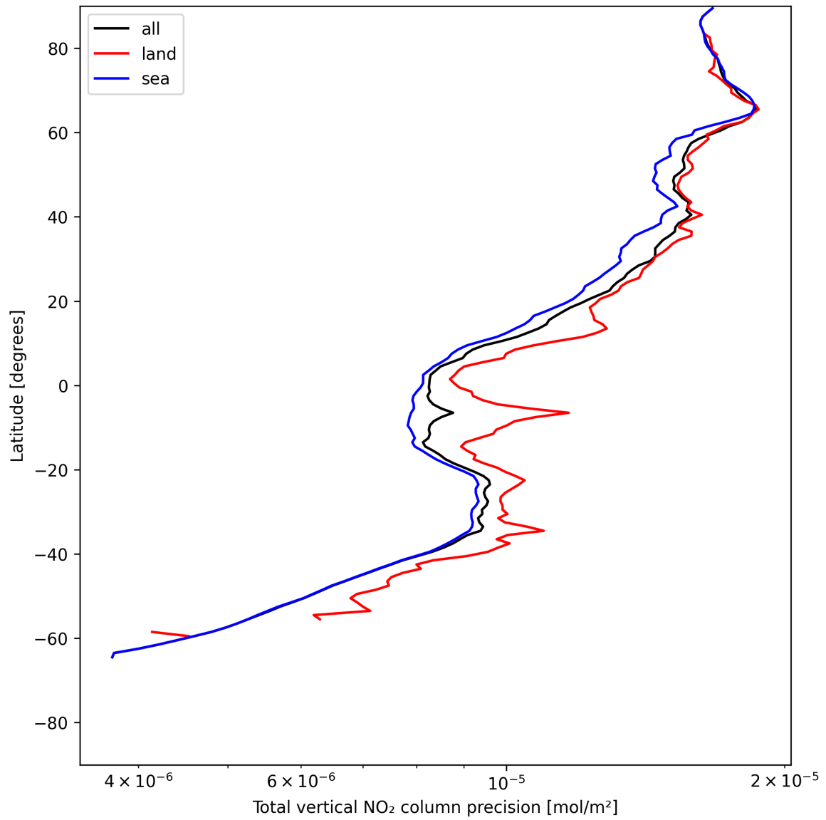
Figure 20: Zonal average of “Total vertical NO 2 column precision” for 2025-06-09 to 2025-06-09.
