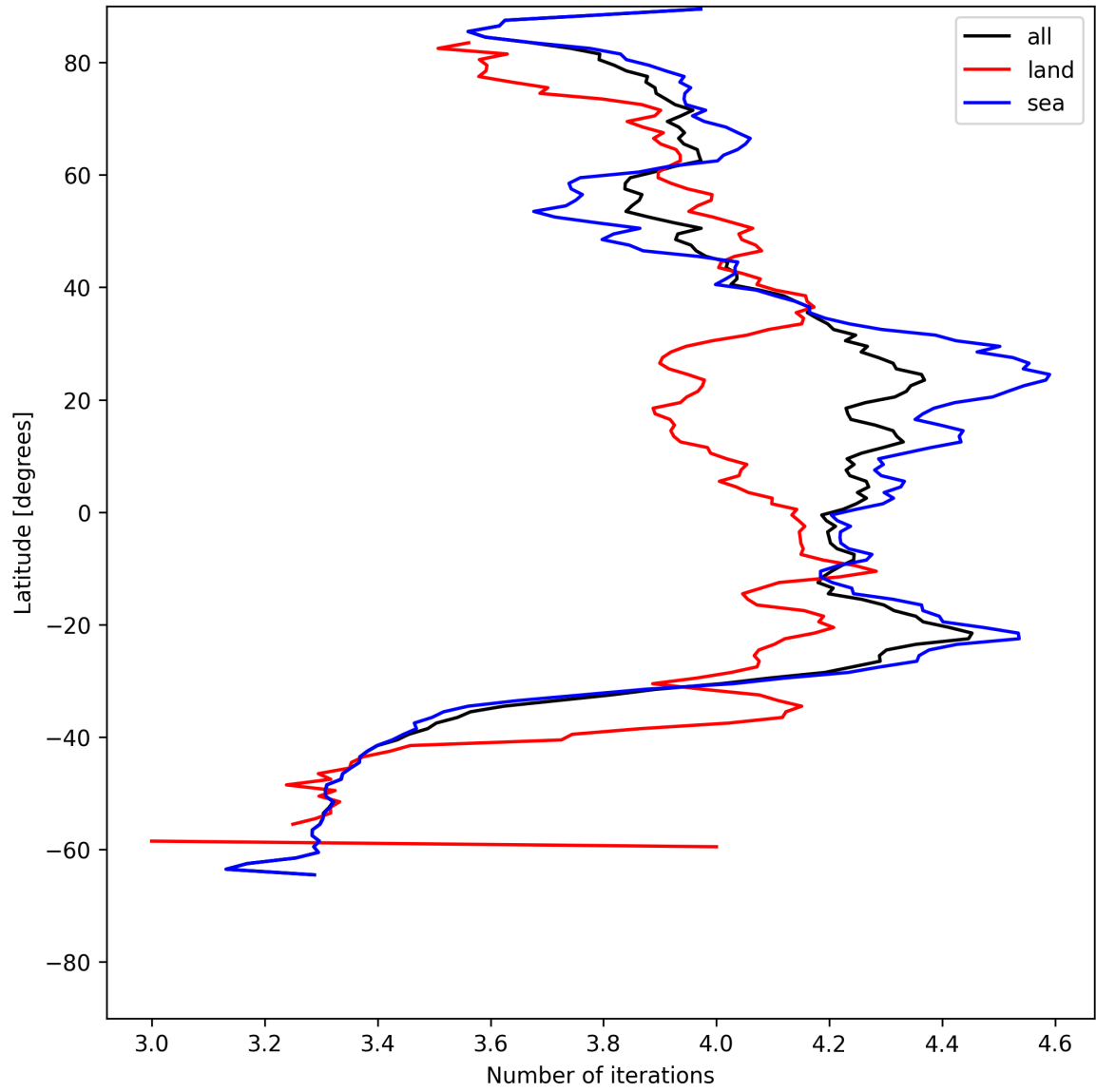
Figure 15: Zonal average of “Number of iterations” for 2025-06-09 to 2025-06-09.
