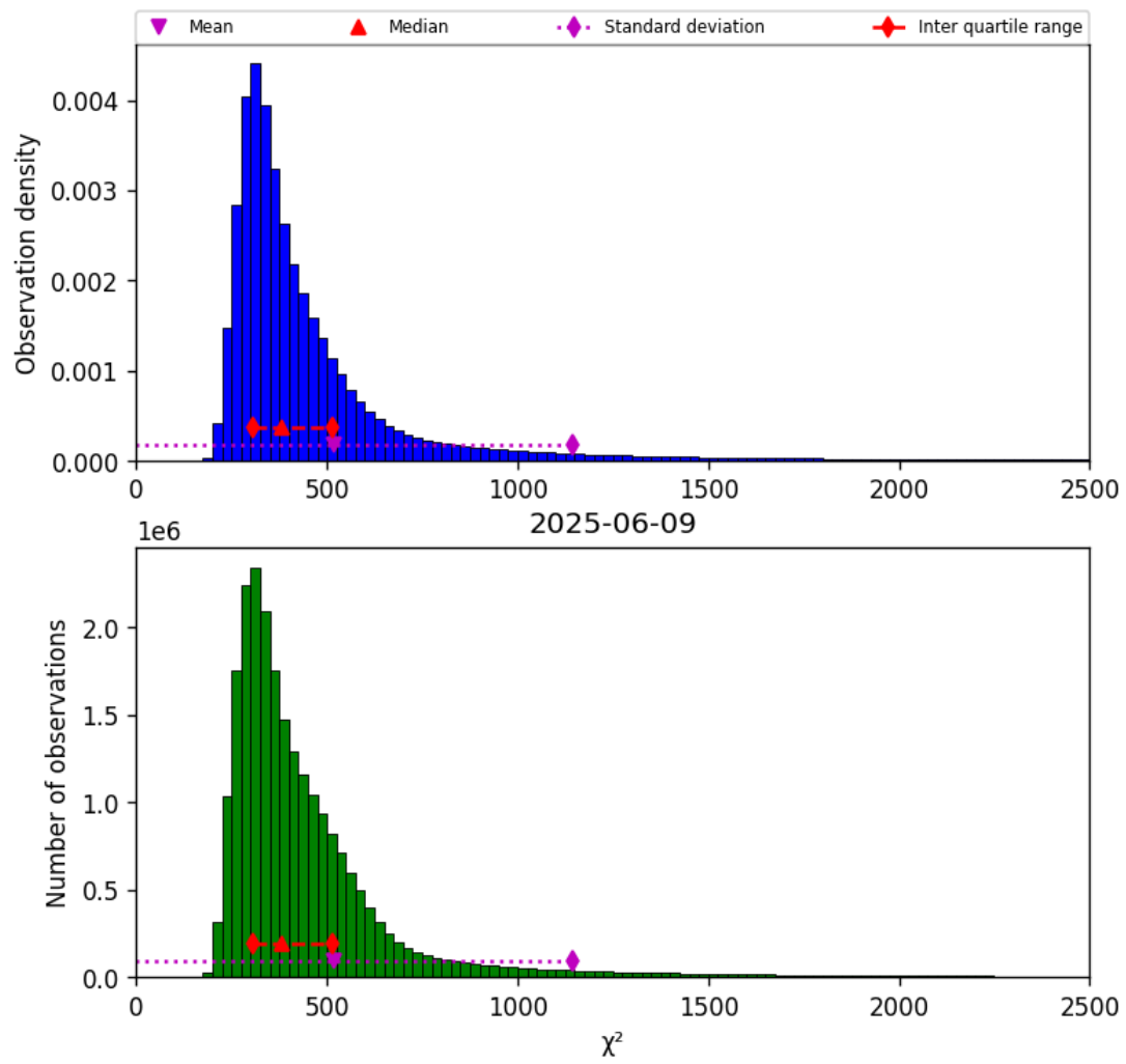
Figure 40: Histogram of “ \chi^2 ” for 2025-06-09 to 2025-06-09
