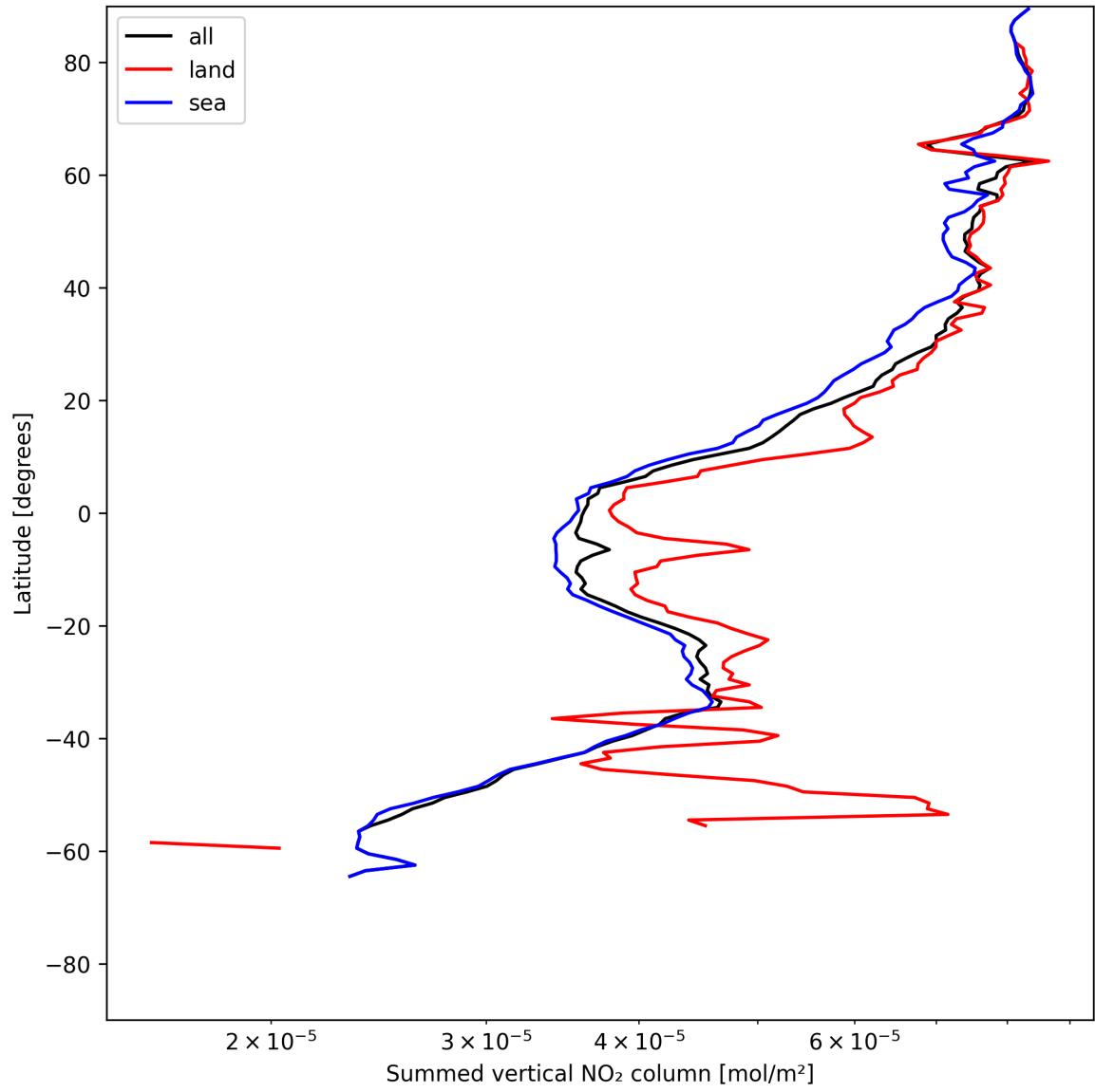
Figure 21: Zonal average of “Summed vertical NO 2 column” for 2025-06-09 to 2025-06-09.
