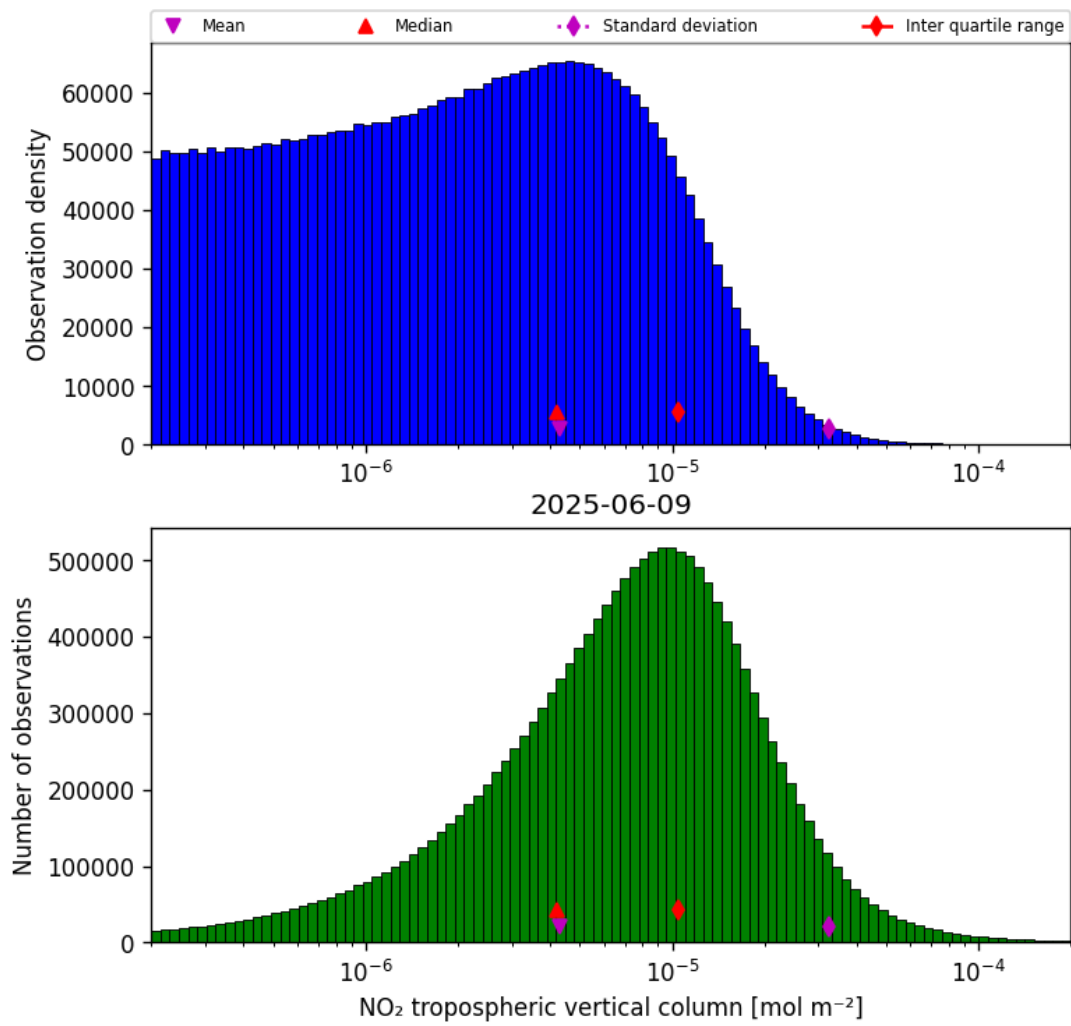
Figure 27: Histogram of “ \text{NO}_2 tropospheric vertical column” for 2025-06-09 to 2025-06-09
