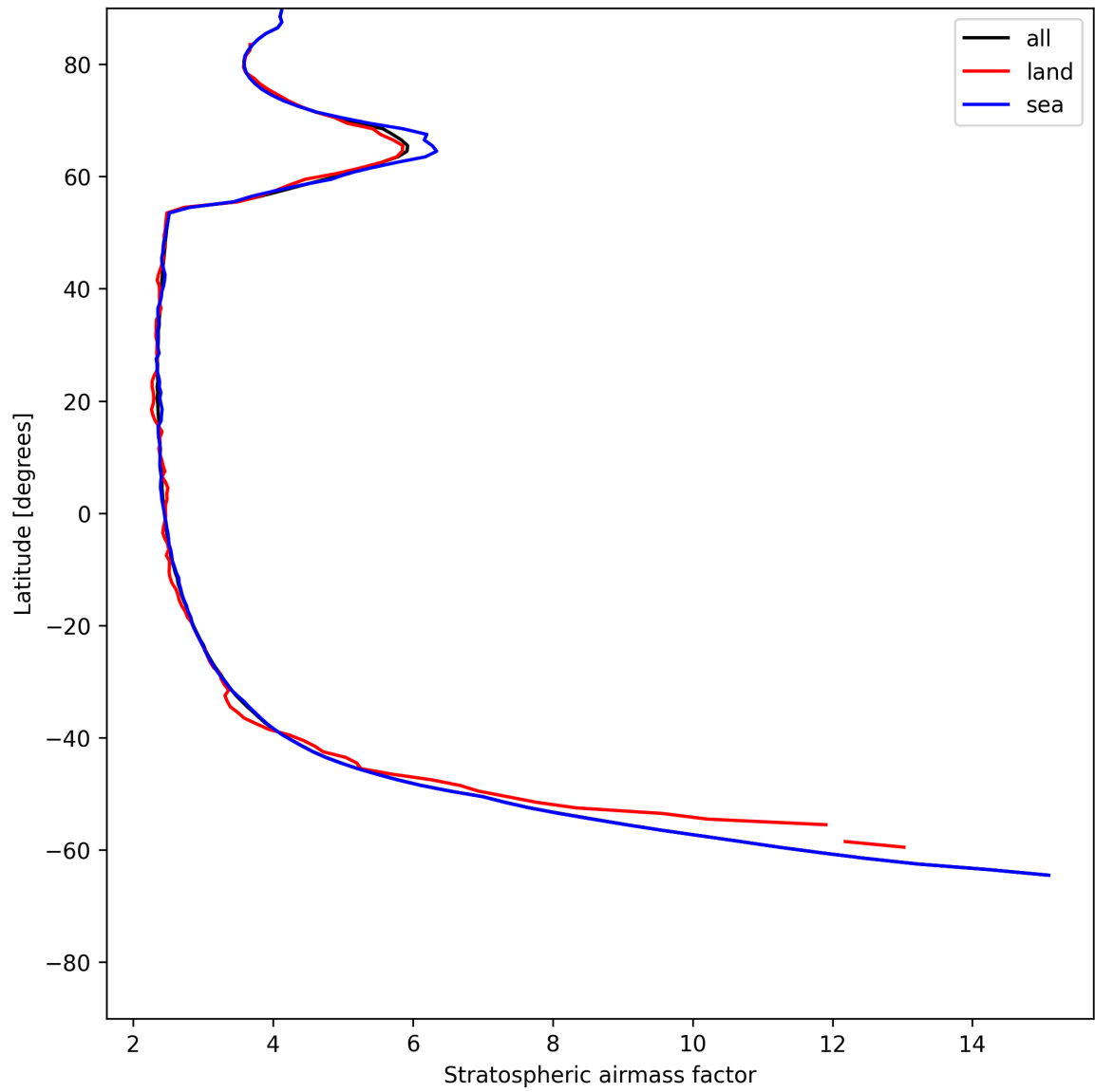
Figure 25: Zonal average of “Stratospheric air mass factor” for 2025-06-09 to 2025-06-09.
