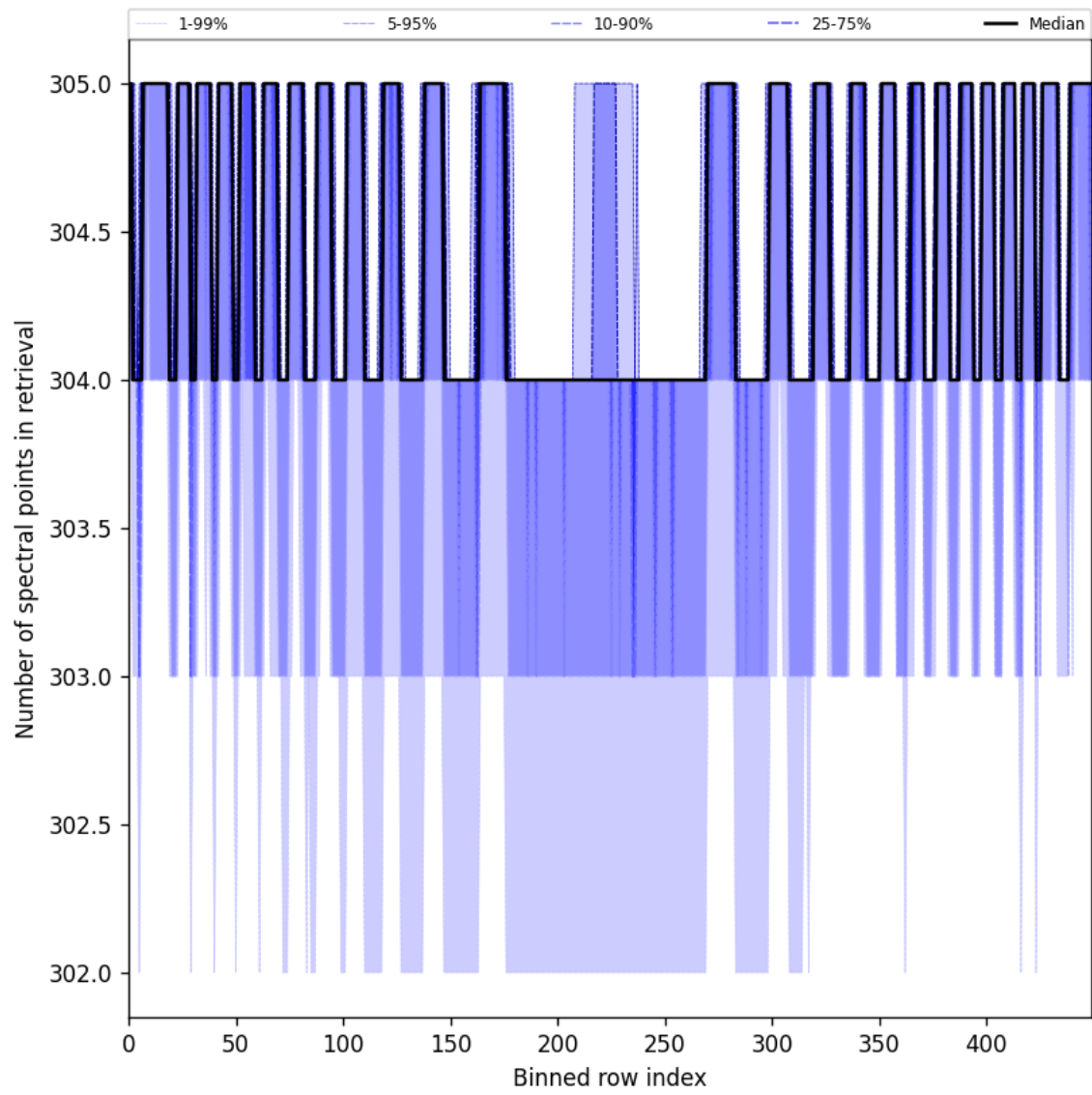
Figure 48: Along track statistics of “Number of spectral points in retrieval” for 2025-06-09 to 2025-06-09
