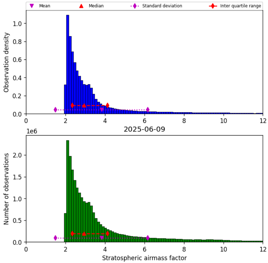
Figure 42: Histogram of “Stratospheric airmass factor” for 2025-06-09 to 2025-06-09
