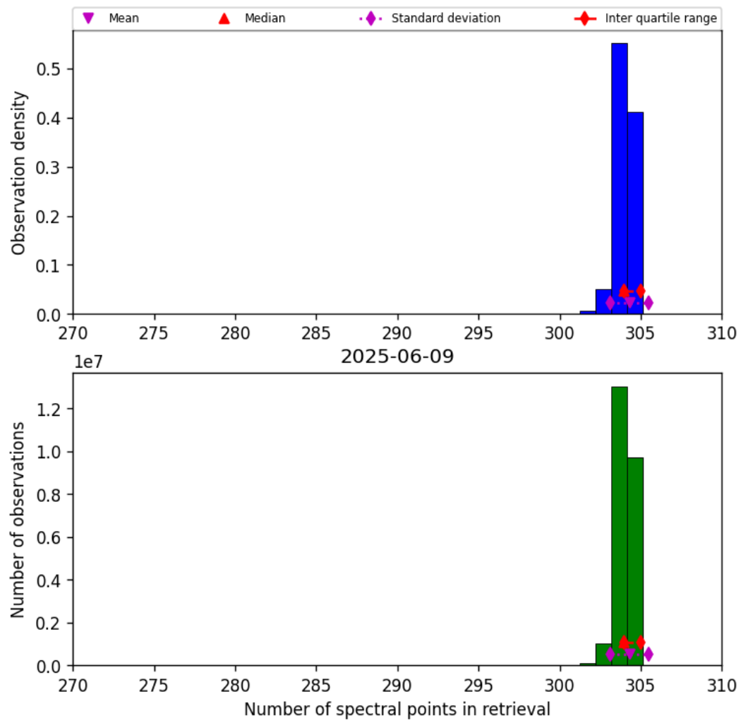
Figure 31: Histogram of “Number of spectral points in retrieval” for 2025-06-09 to 2025-06-09
