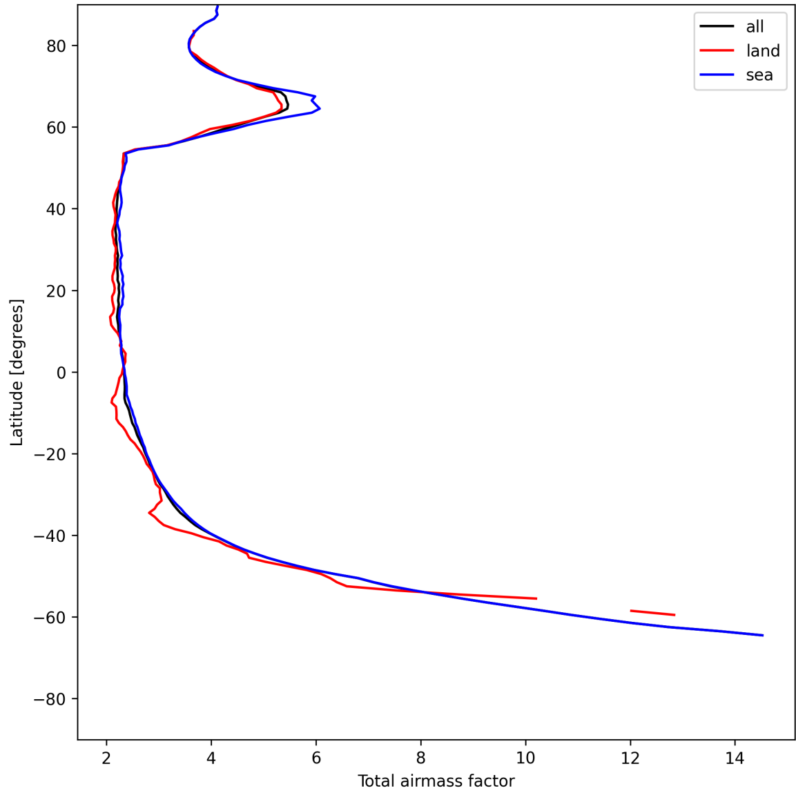
Figure 13: Zonal average of “Total airmass factor” for 2025-06-09 to 2025-06-09.
