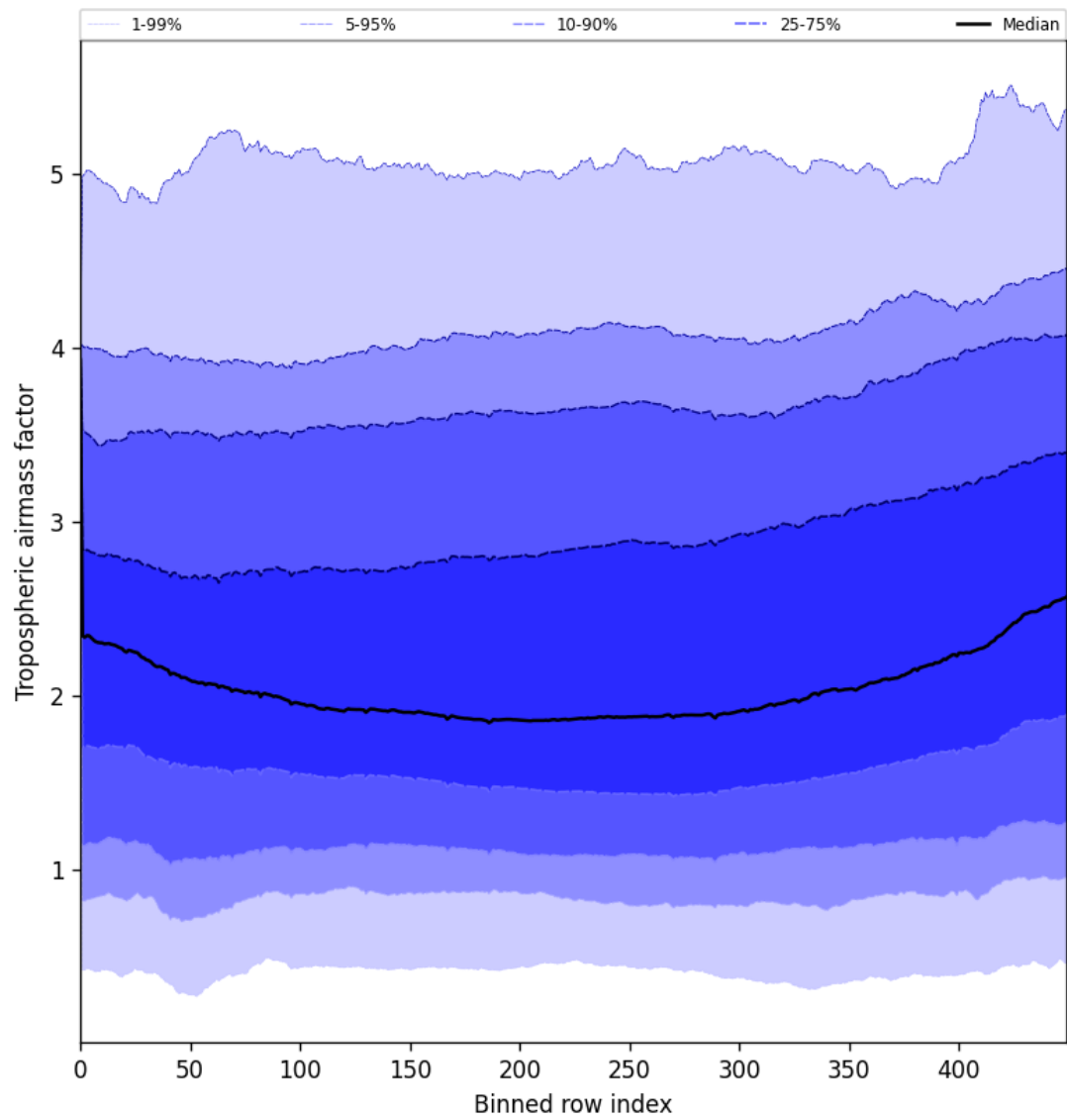
Figure 46: Along track statistics of “Tropospheric airmass factor” for 2025-06-09 to 2025-06-09
