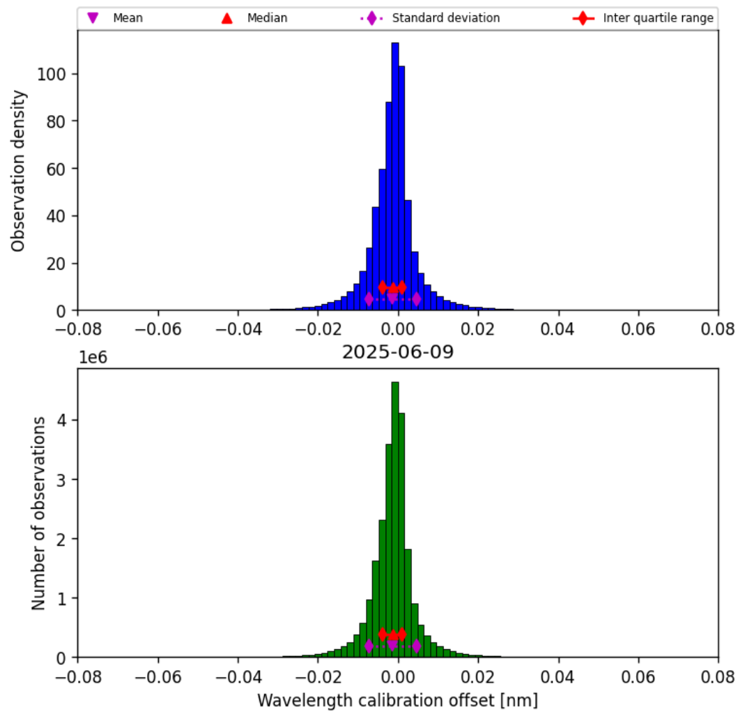
Figure 33: Histogram of “Wavelength calibration offset” for 2025-06-09 to 2025-06-09
