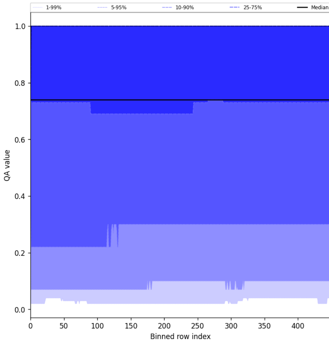
Figure 43: Along track statistics of “QA value” for 2025-06-09 to 2025-06-09
