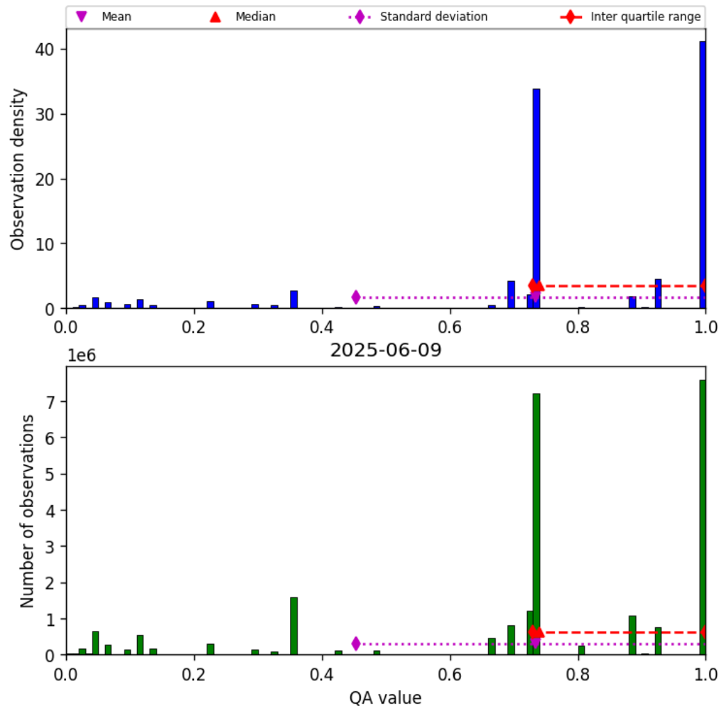
Figure 26: Histogram of “QA value” for 2025-06-09 to 2025-06-09
