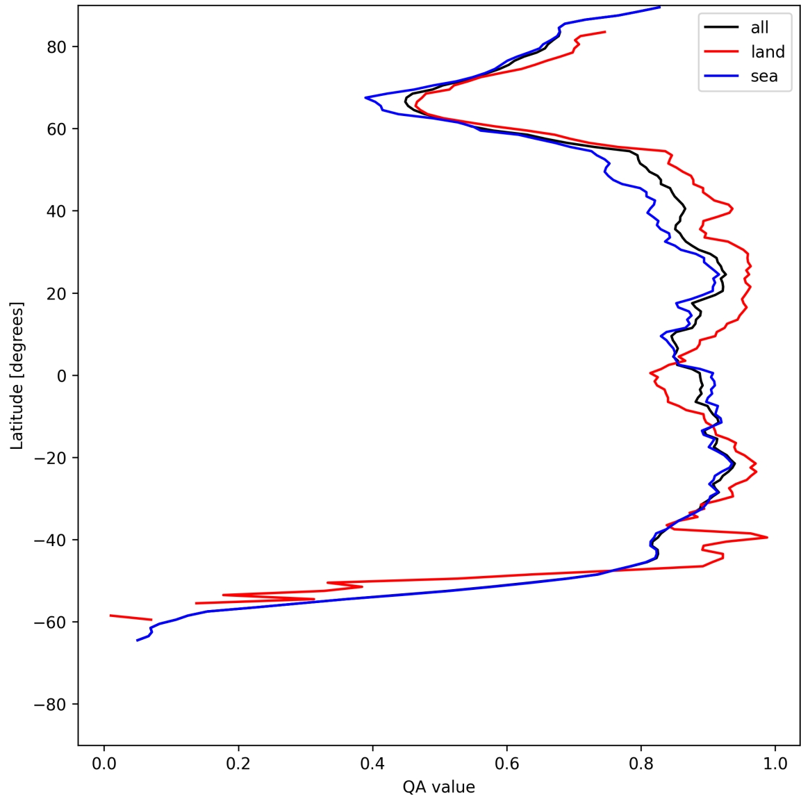
Figure 9: Zonal average of “QA value” for 2025-06-09 to 2025-06-09.
