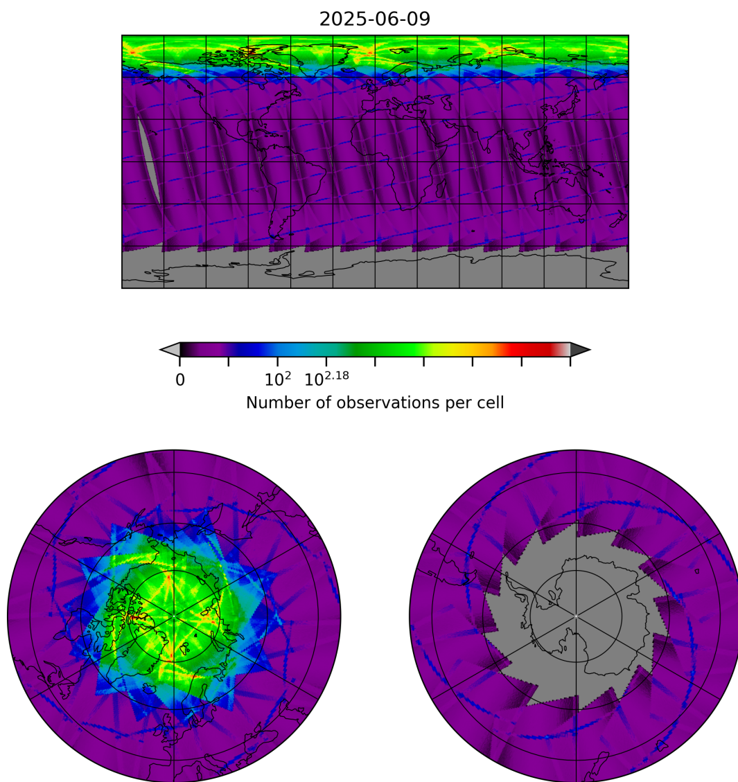
Figure 8: Map of the number of observations for 2025-06-09 to 2025-06-09
