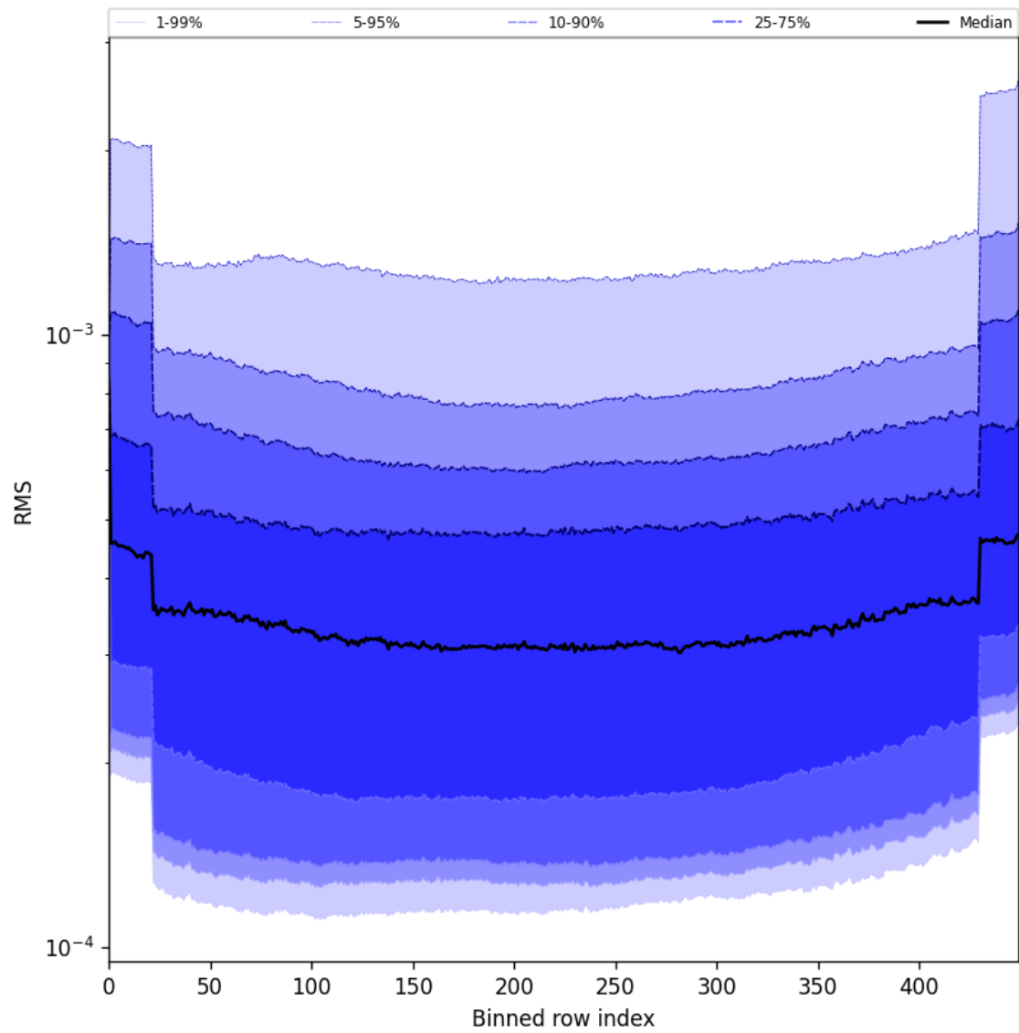
Figure 58: Along track statistics of “RMS” for 2025-06-09 to 2025-06-09
