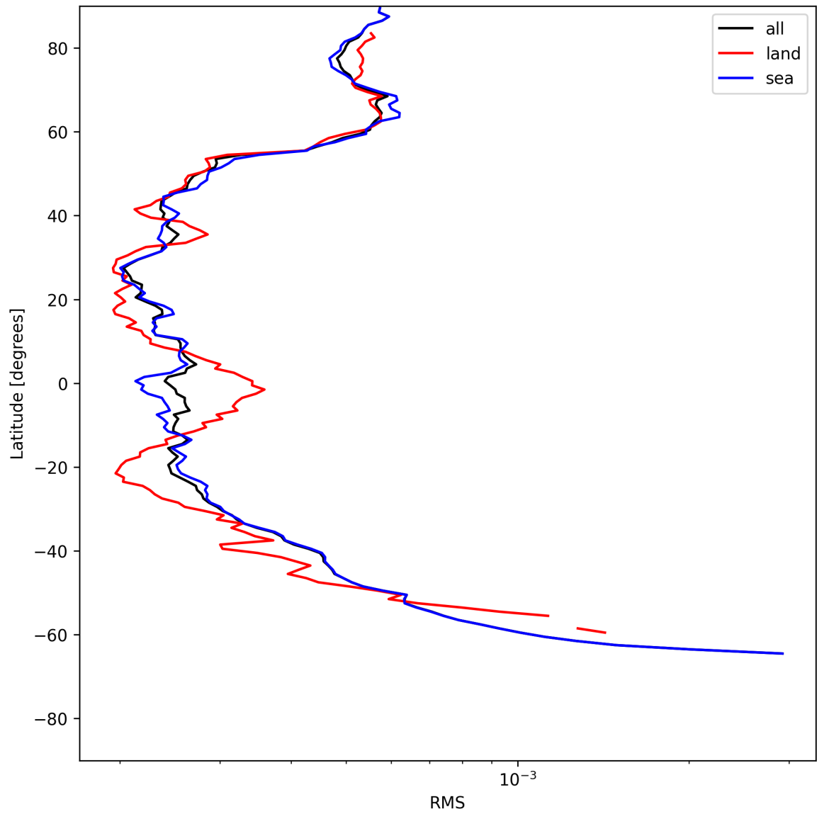
Figure 24: Zonal average of “RMS” for 2025-06-09 to 2025-06-09.
