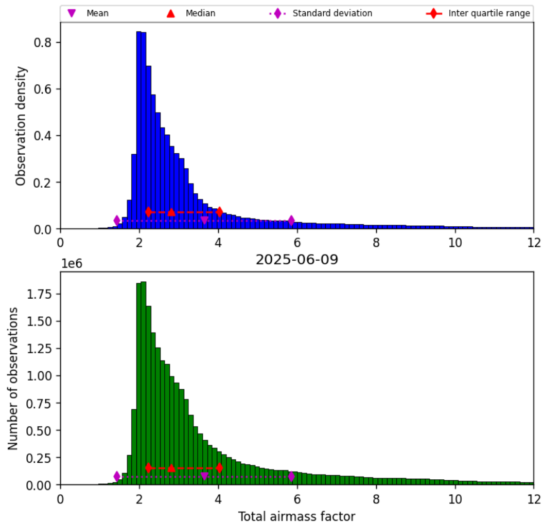
Figure 30: Histogram of “Total airmass factor” for 2025-06-09 to 2025-06-09
