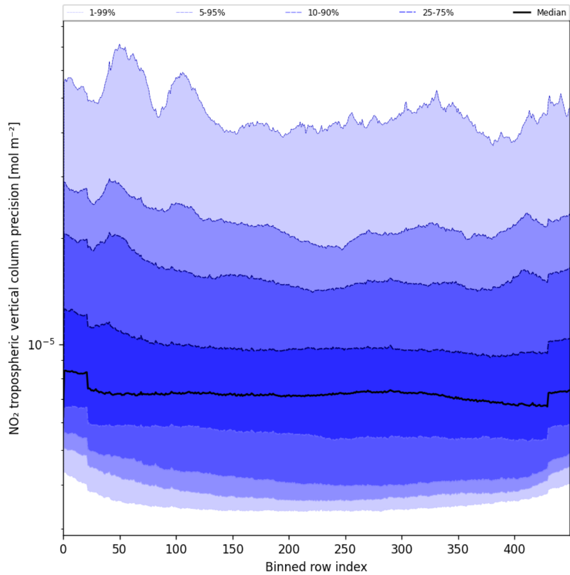
Figure 45: Along track statistics of “NO 2 tropospheric vertical column precision” for 2025-06-09 to 2025-06-09
