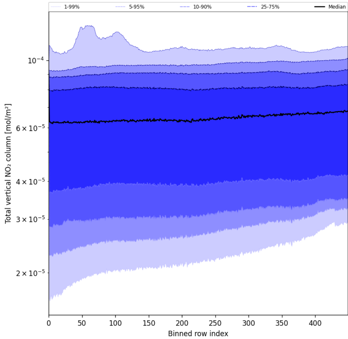
Figure 53: Along track statistics of “Total vertical NO 2 column” for 2025-06-09 to 2025-06-09
