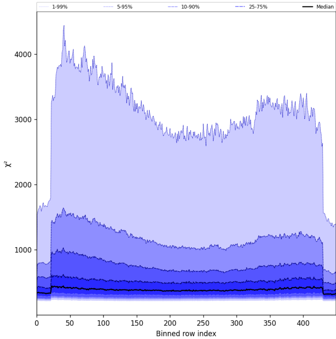
Figure 57: Along track statistics of “ \chi^2 ” for 2025-06-09 to 2025-06-09
