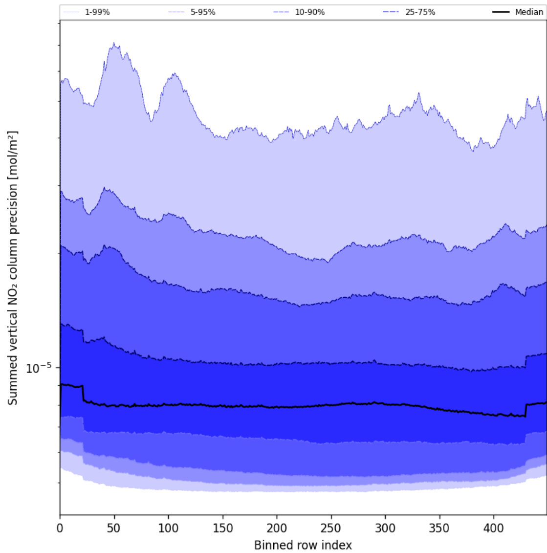
Figure 56: Along track statistics of “Summed vertical NO 2 column precision” for 2025-06-09 to 2025-06-09
