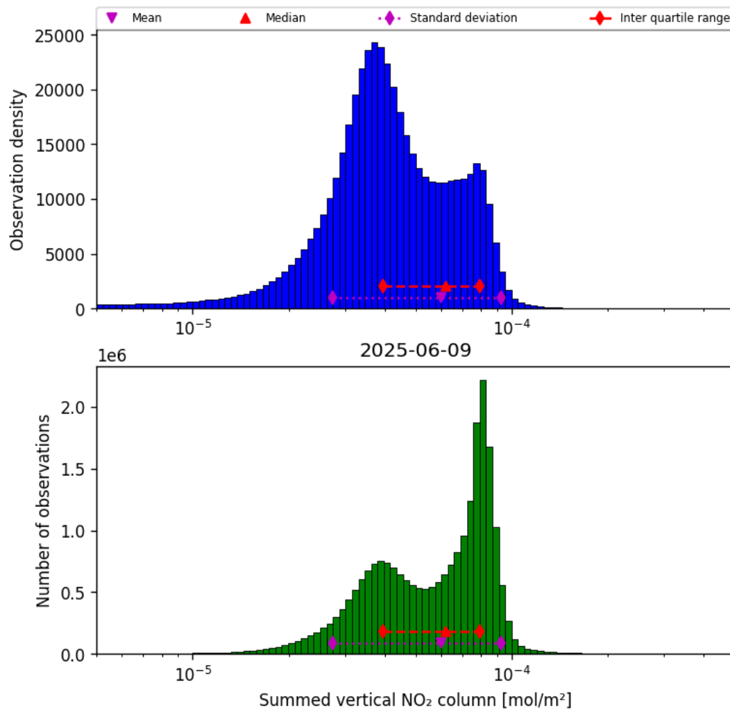
Figure 38: Histogram of “Summed vertical NO 2 column” for 2025-06-09 to 2025-06-09
