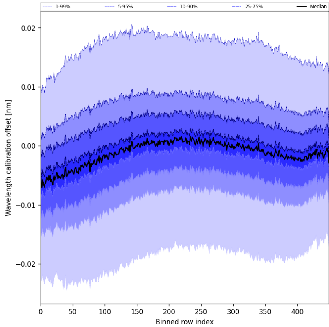
Figure 50: Along track statistics of “Wavelength calibration offset” for 2025-06-09 to 2025-06-09
