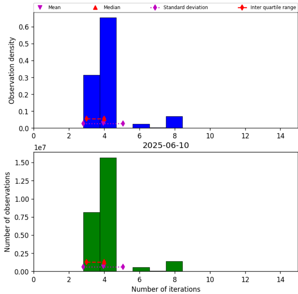
Figure 32: Histogram of “Number of iterations” for 2025-06-10 to 2025-06-11
