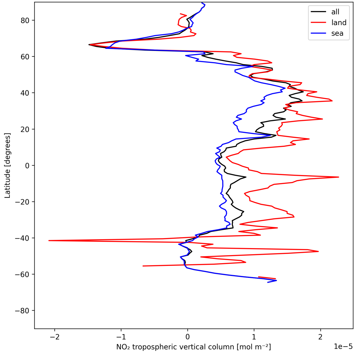
Figure 10: Zonal average of “NO 2 tropospheric vertical column” for 2025-06-10 to 2025-06-11.
