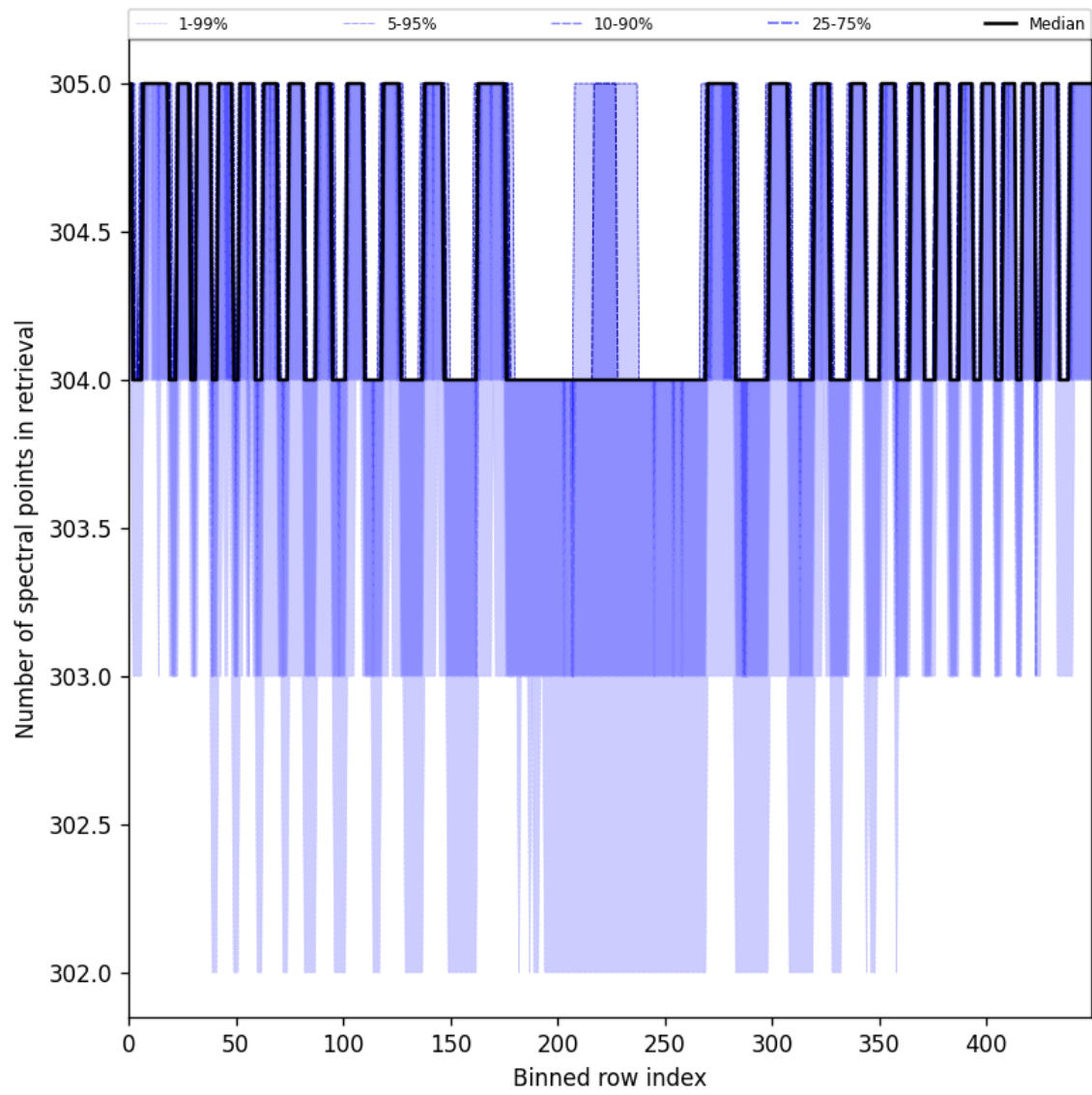
Figure 48: Along track statistics of “Number of spectral points in retrieval” for 2025-06-10 to 2025-06-11
