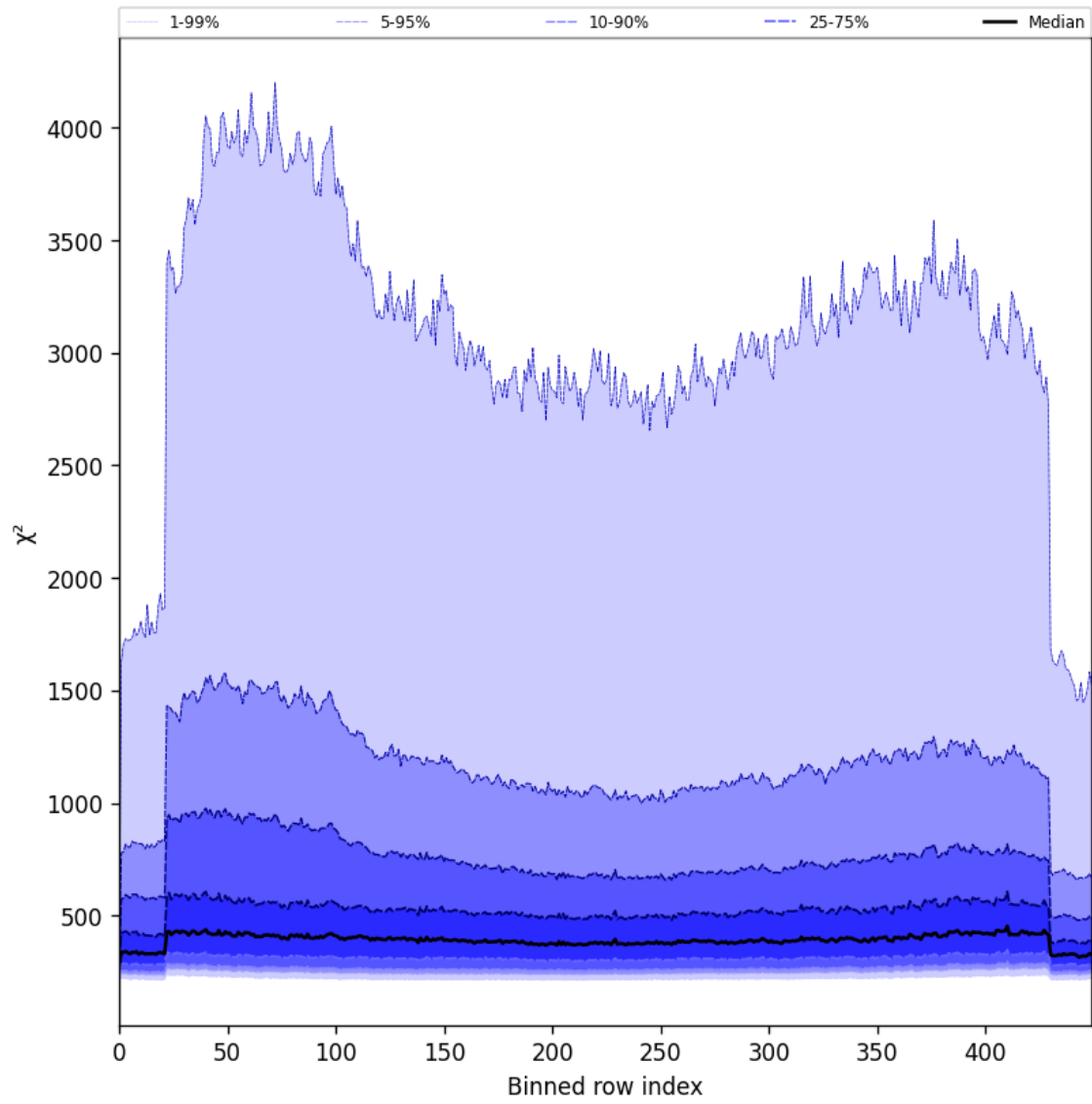
Figure 57: Along track statistics of “ \chi^2 ” for 2025-06-10 to 2025-06-11
