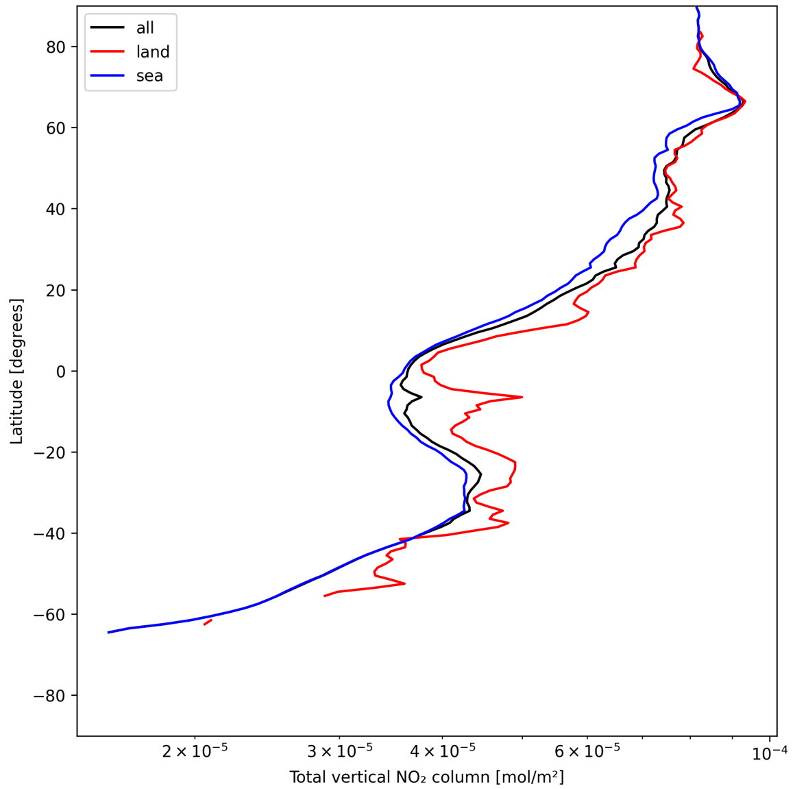
Figure 19: Zonal average of “Total vertical NO 2 column” for 2025-06-10 to 2025-06-11.
