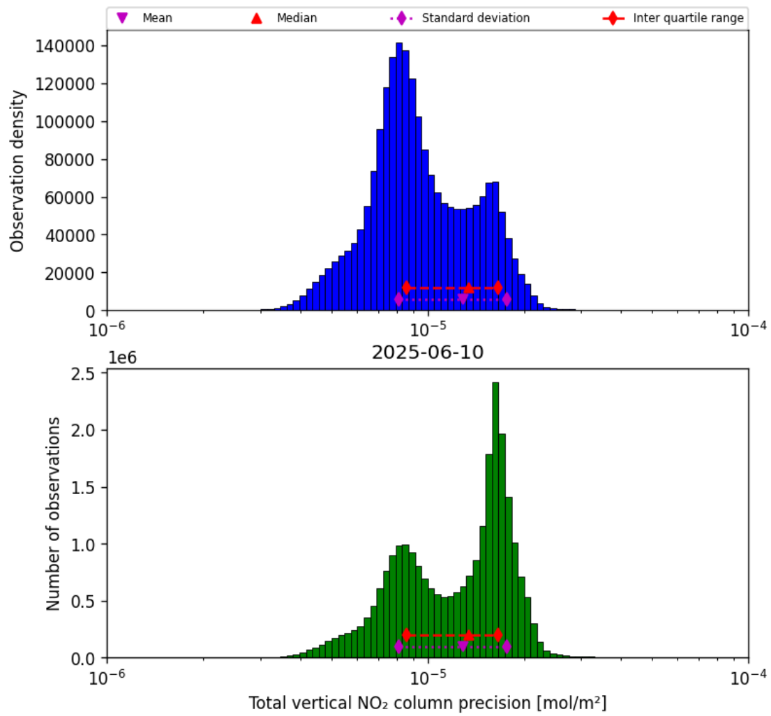
Figure 37: Histogram of “Total vertical NO 2 column precision” for 2025-06-10 to 2025-06-11
