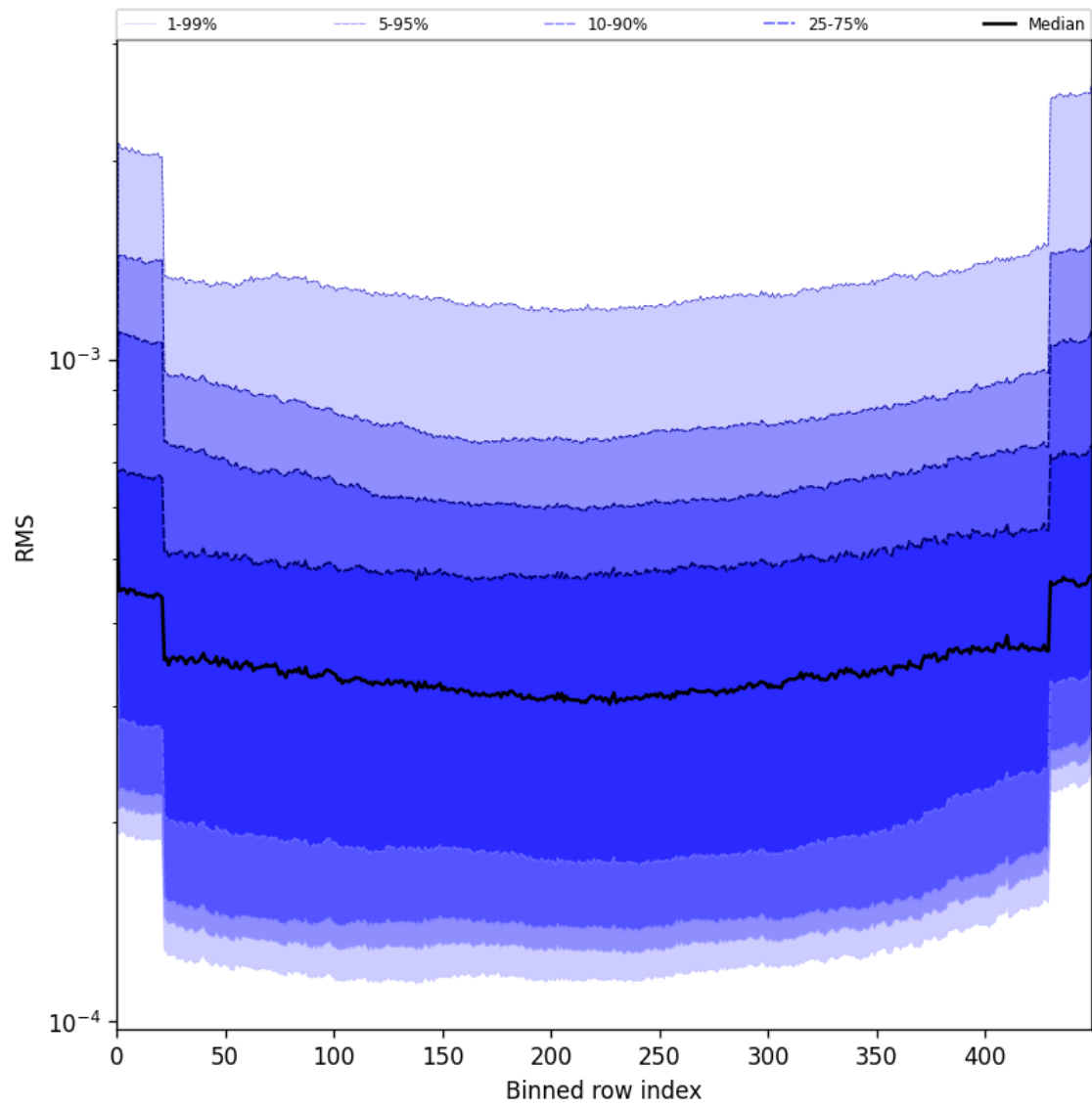
Figure 58: Along track statistics of “RMS” for 2025-06-10 to 2025-06-11
