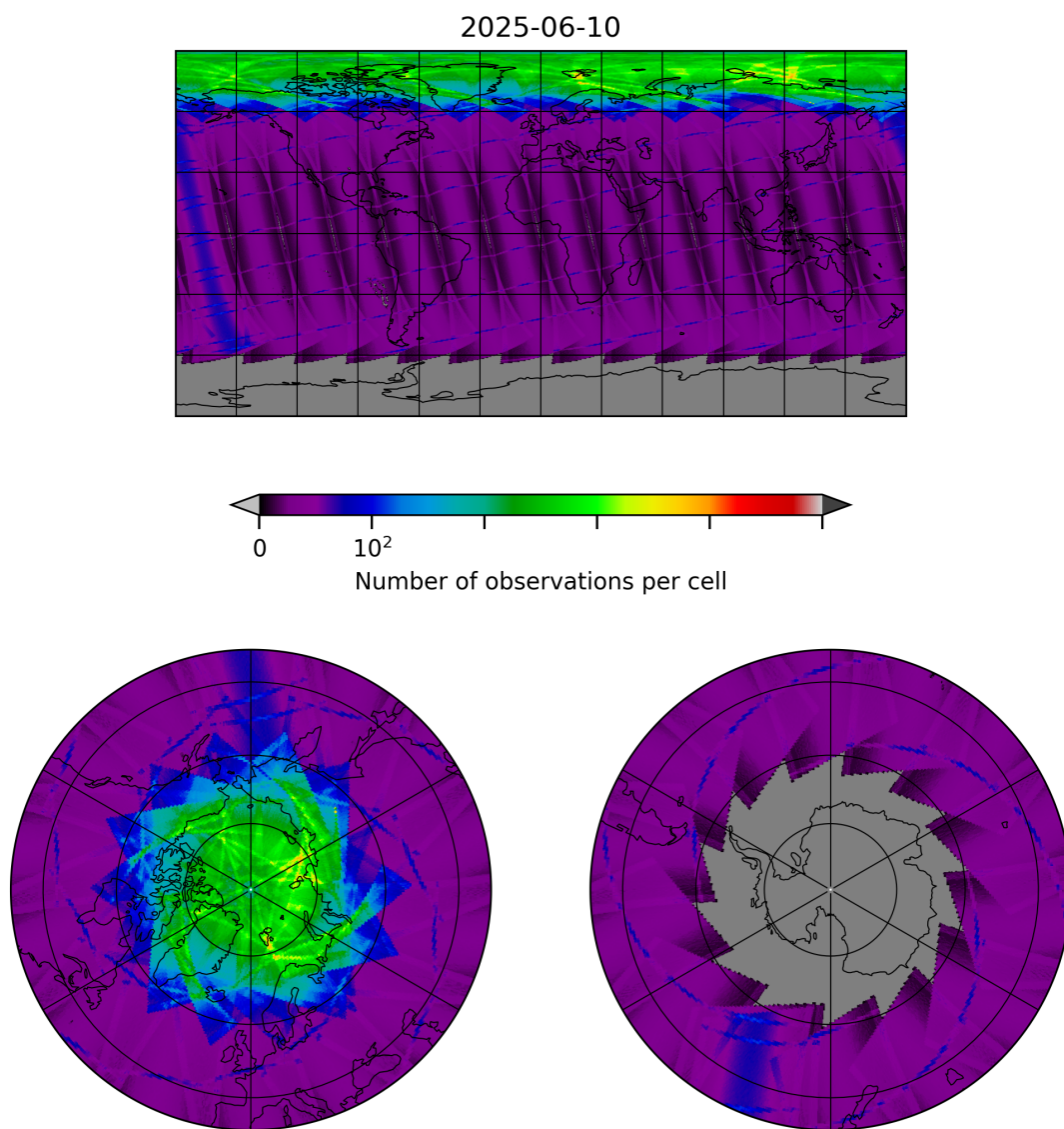
Figure 8: Map of the number of observations for 2025-06-10 to 2025-06-11
