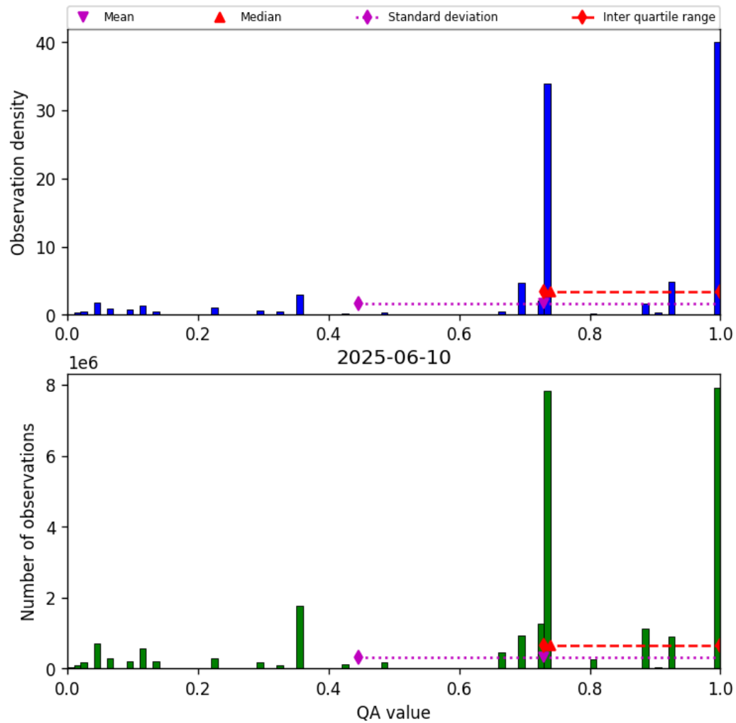
Figure 26: Histogram of “QA value” for 2025-06-10 to 2025-06-11
