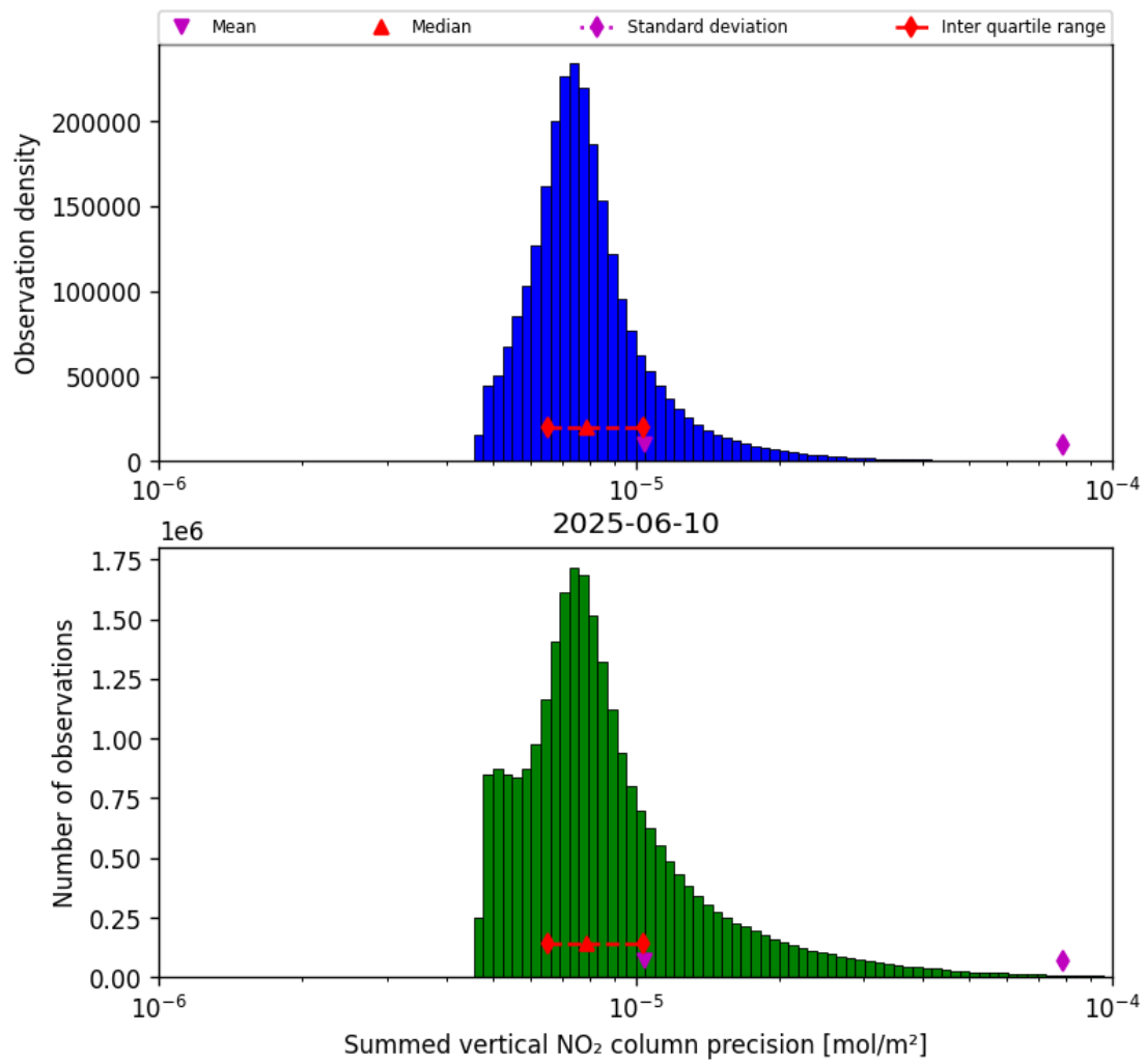
Figure 39: Histogram of “Summed vertical NO 2 column precision” for 2025-06-10 to 2025-06-11
