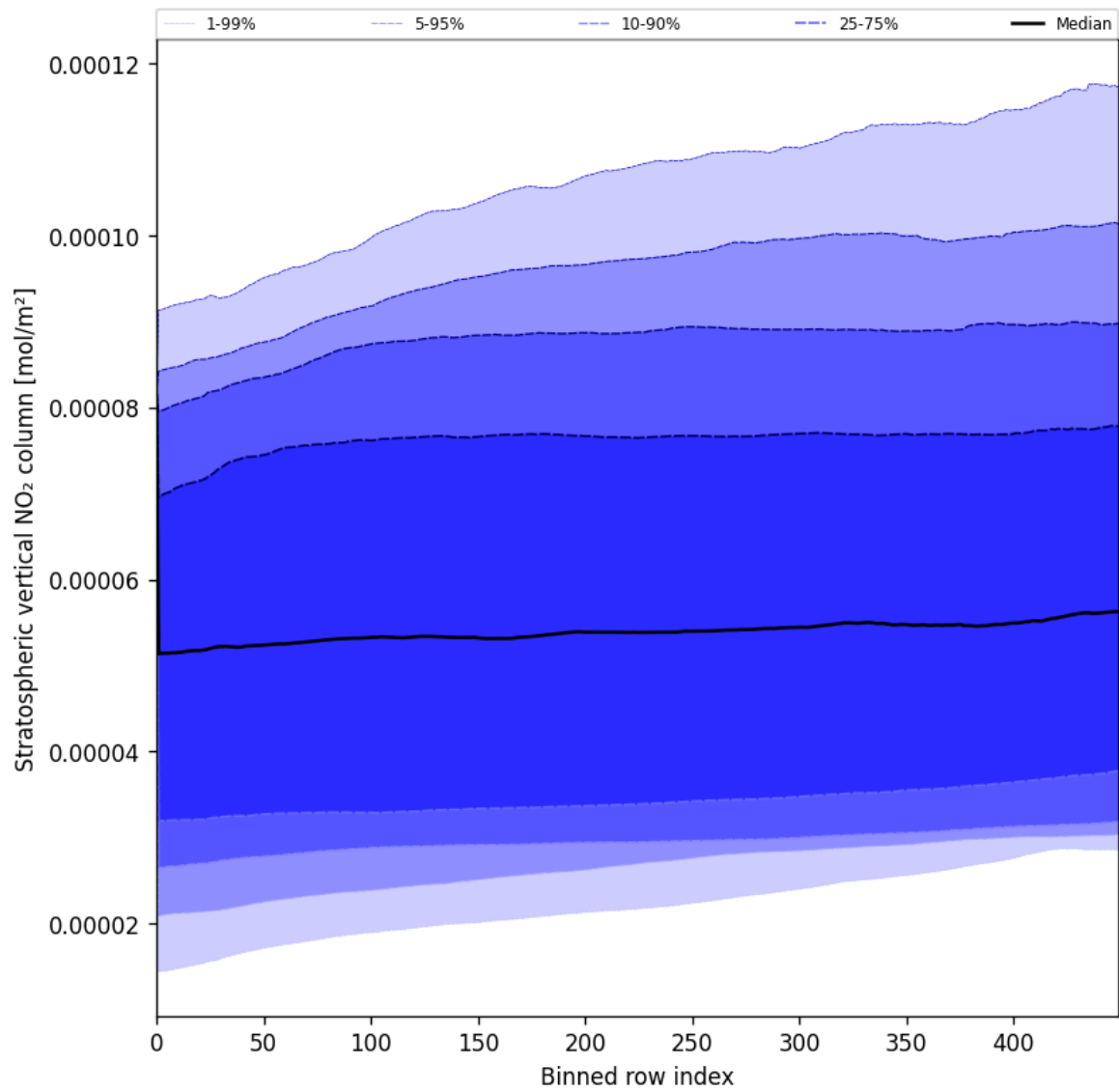
Figure 51: Along track statistics of “Stratospheric vertical NO 2 column” for 2025-06-10 to 2025-06-11
