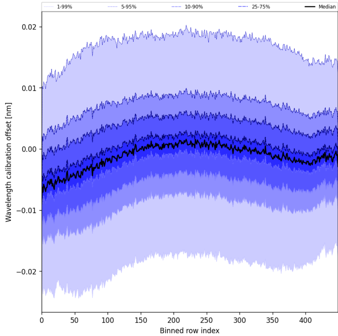
Figure 50: Along track statistics of “Wavelength calibration offset” for 2025-06-10 to 2025-06-11
