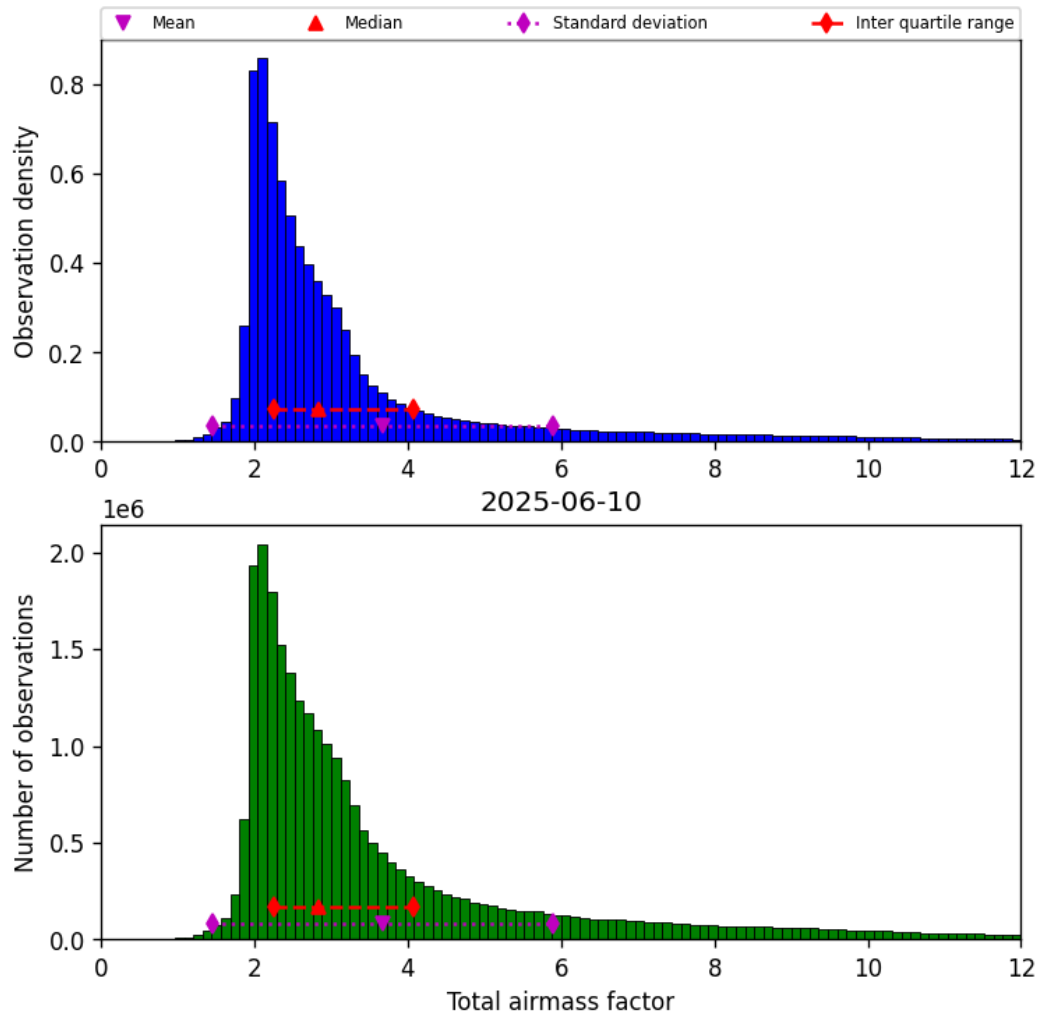
Figure 30: Histogram of “Total airmass factor” for 2025-06-10 to 2025-06-11
