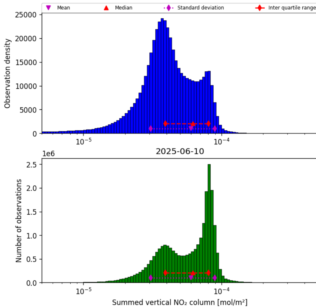
Figure 38: Histogram of “Summed vertical NO 2 column” for 2025-06-10 to 2025-06-11
