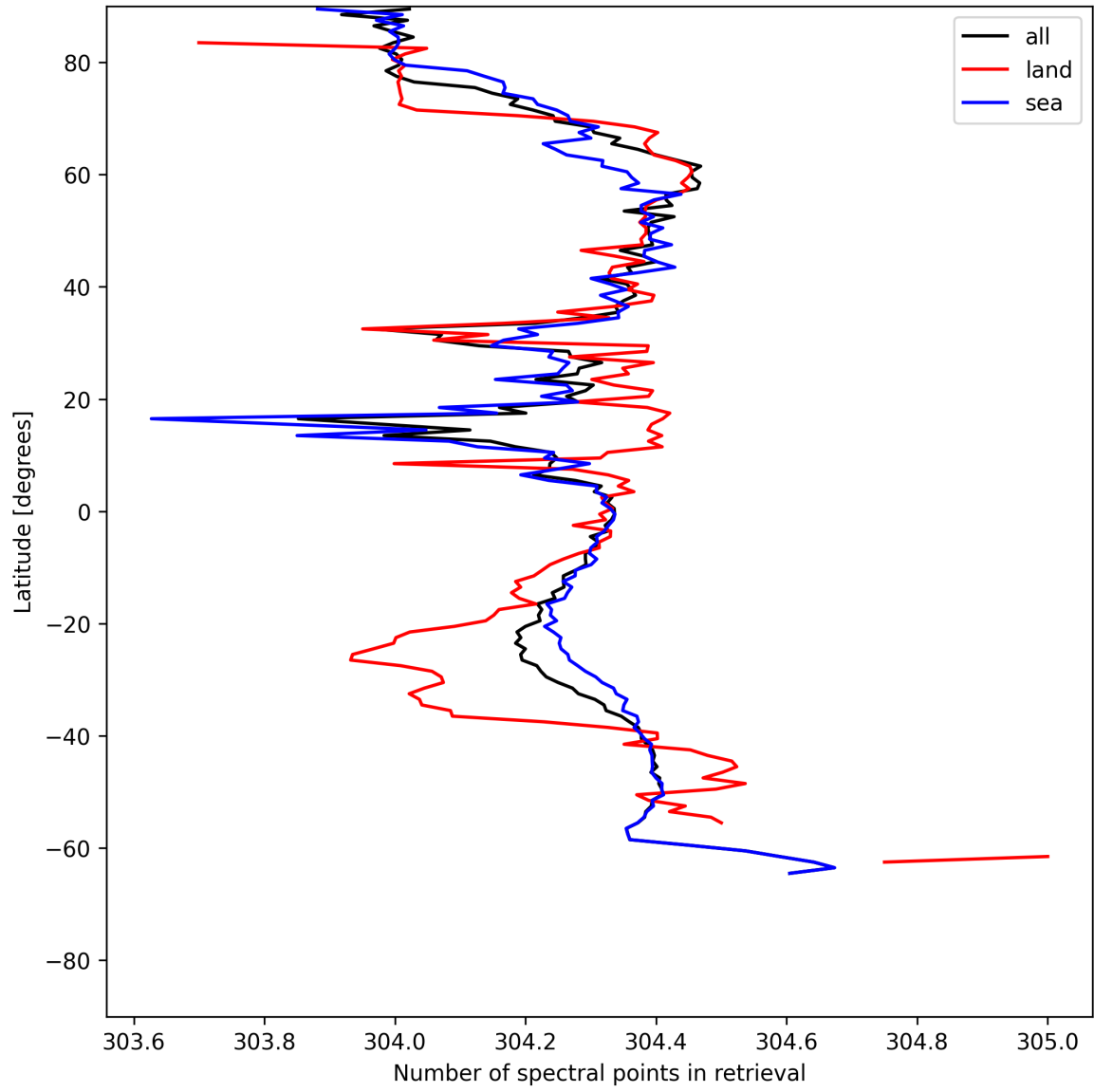
Figure 14: Zonal average of “Number of spectral points in retrieval” for 2025-06-10 to 2025-06-11.
