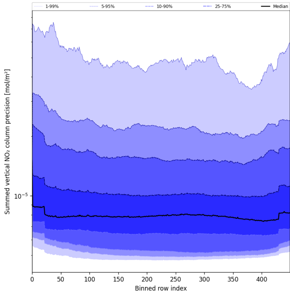
Figure 56: Along track statistics of “Summed vertical NO 2 column precision” for 2025-06-10 to 2025-06-11
