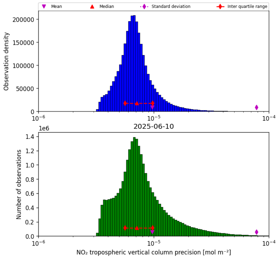
Figure 28: Histogram of “NO 2 tropospheric vertical column precision” for 2025-06-10 to 2025-06-11
