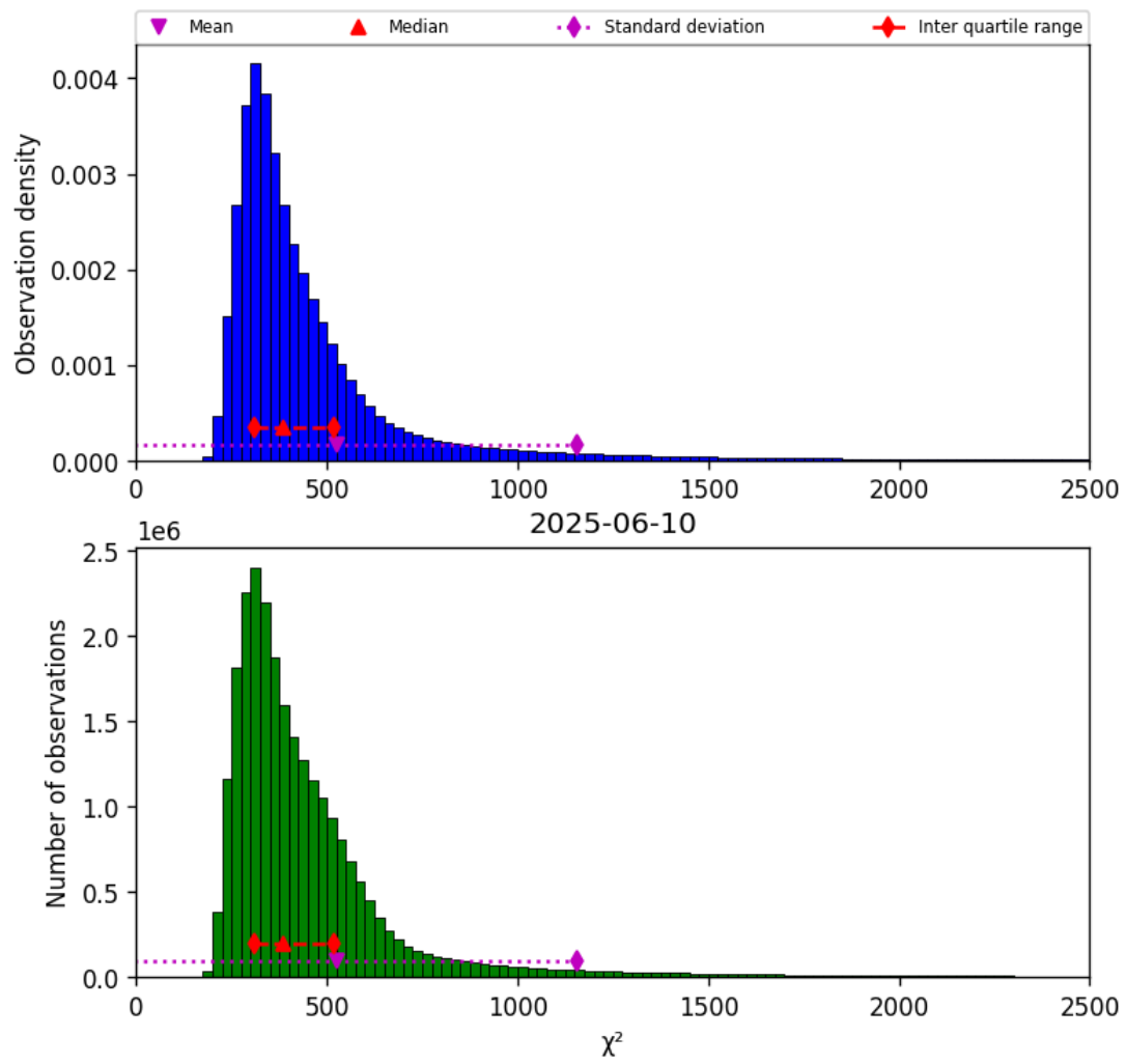
Figure 40: Histogram of “ \chi^2 ” for 2025-06-10 to 2025-06-11
