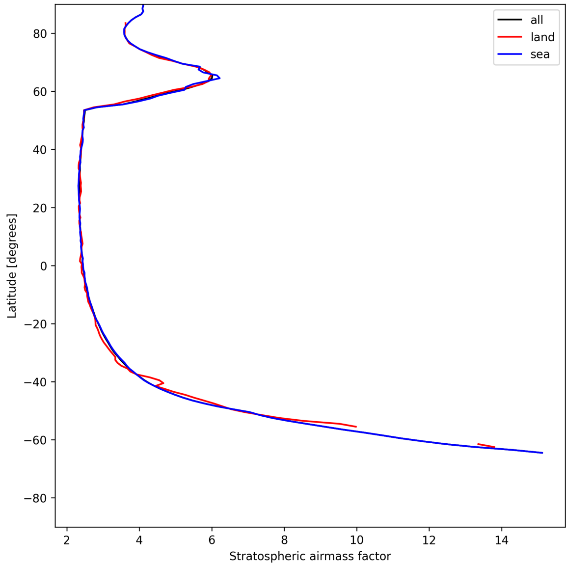
Figure 25: Zonal average of “Stratospheric air mass factor” for 2025-06-10 to 2025-06-11.
