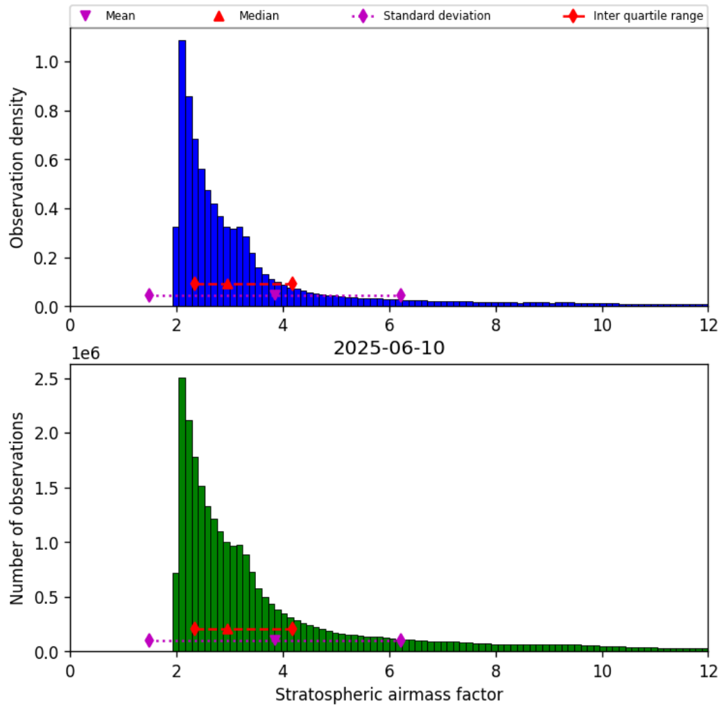
Figure 42: Histogram of “Stratospheric airmass factor” for 2025-06-10 to 2025-06-11
