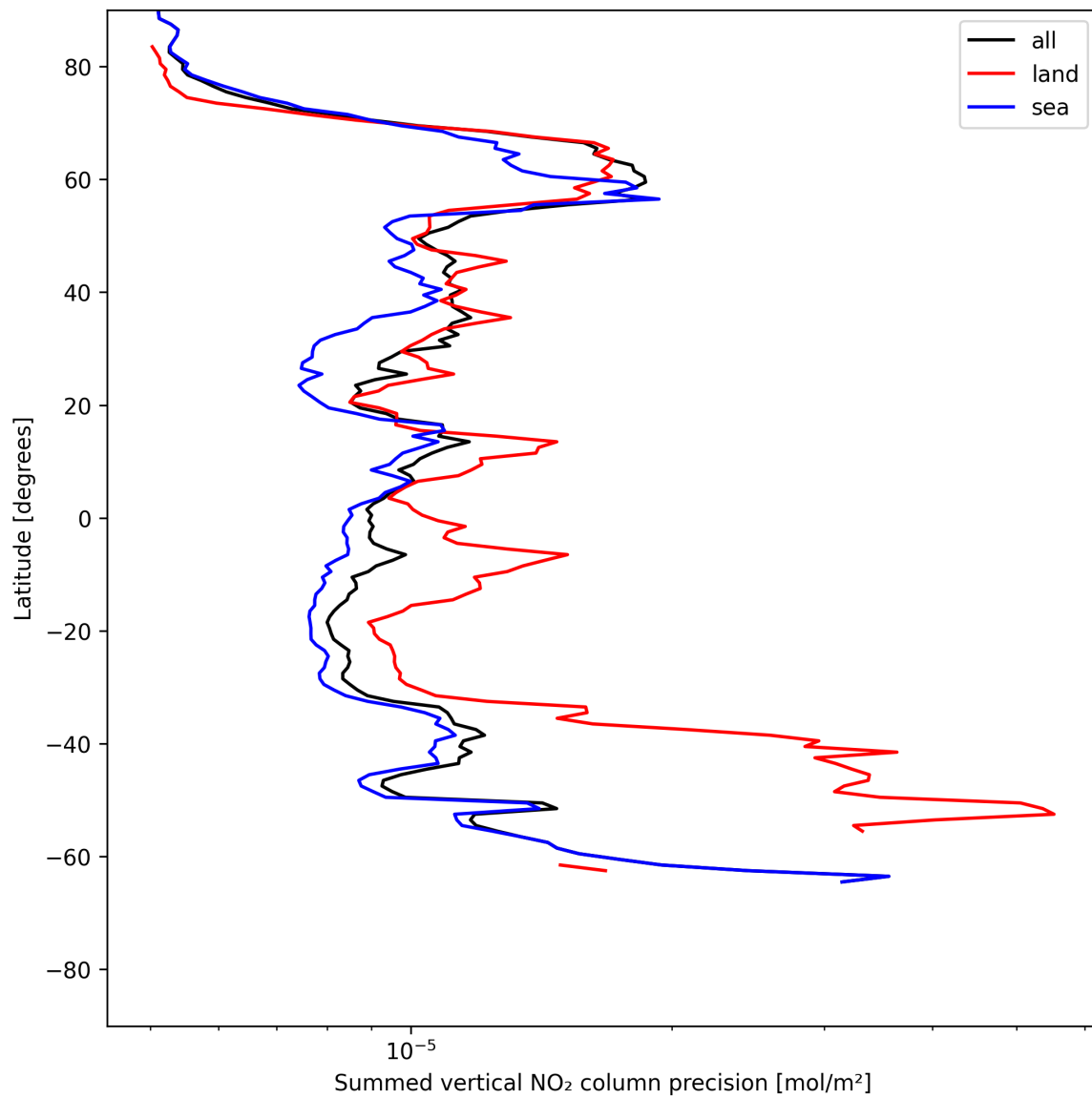
Figure 22: Zonal average of “Summed vertical NO 2 column precision” for 2025-06-10 to 2025-06-11.
