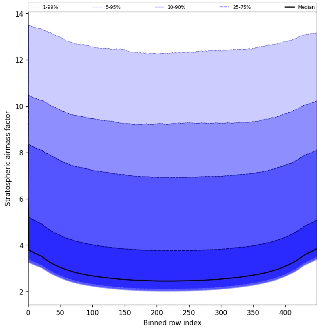
Figure 59: Along track statistics of “Stratospheric airmass factor” for 2025-06-10 to 2025-06-11
