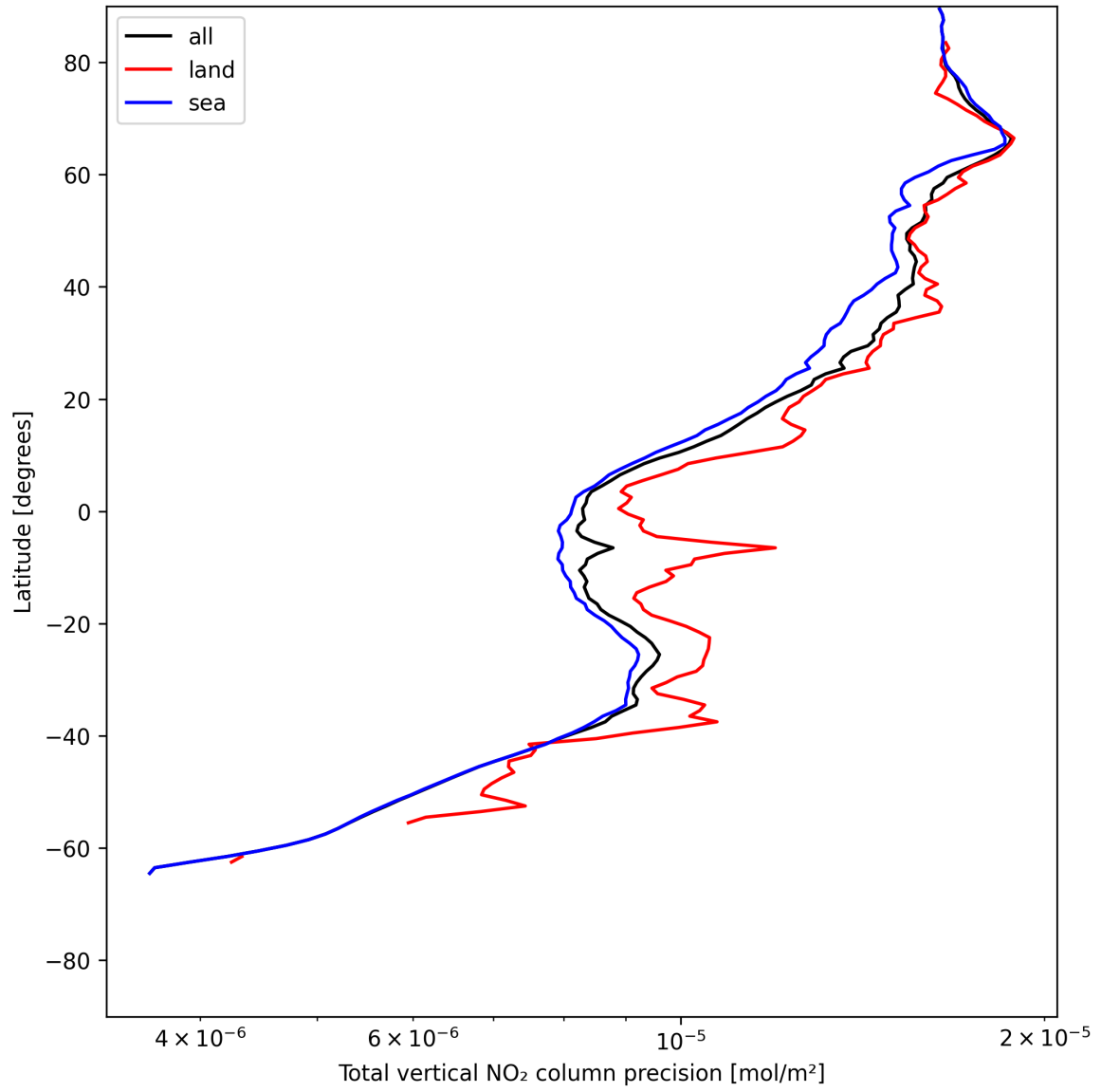
Figure 20: Zonal average of “Total vertical NO 2 column precision” for 2025-06-10 to 2025-06-11.
