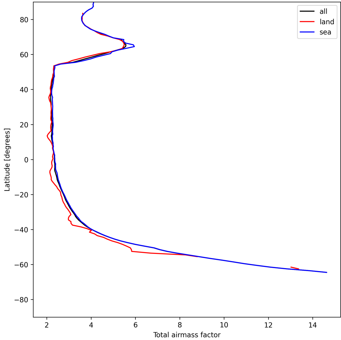
Figure 13: Zonal average of “Total airmass factor” for 2025-06-10 to 2025-06-11.
