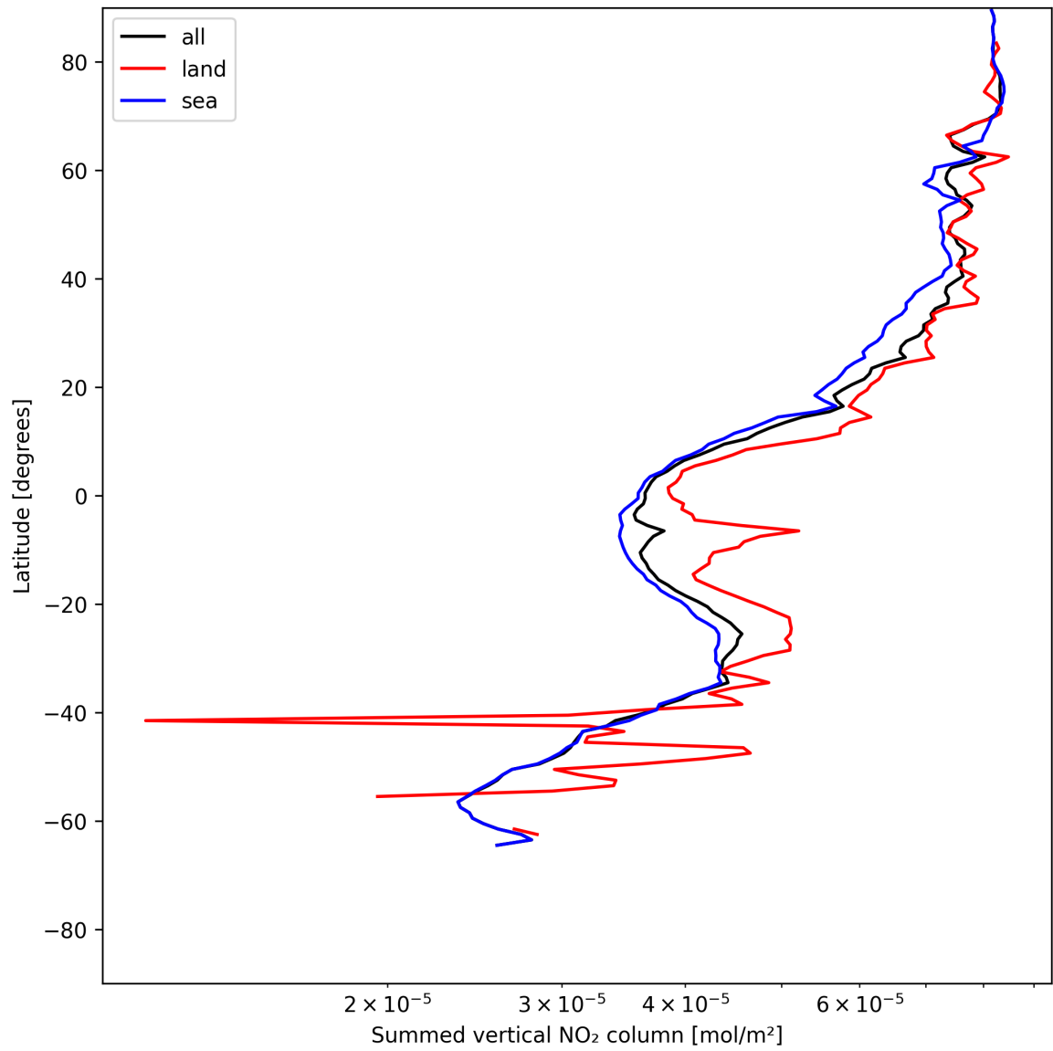
Figure 21: Zonal average of “Summed vertical NO 2 column” for 2025-06-10 to 2025-06-11.
