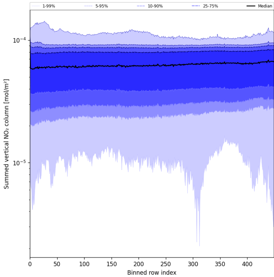
Figure 55: Along track statistics of “Summed vertical NO 2 column” for 2025-06-10 to 2025-06-11
