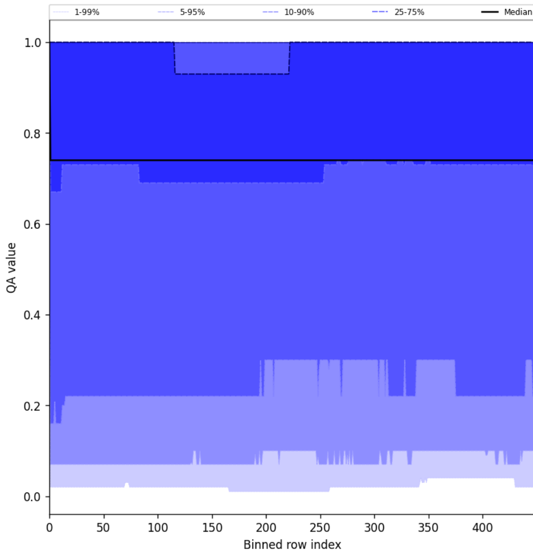
Figure 43: Along track statistics of “QA value” for 2025-06-10 to 2025-06-11
