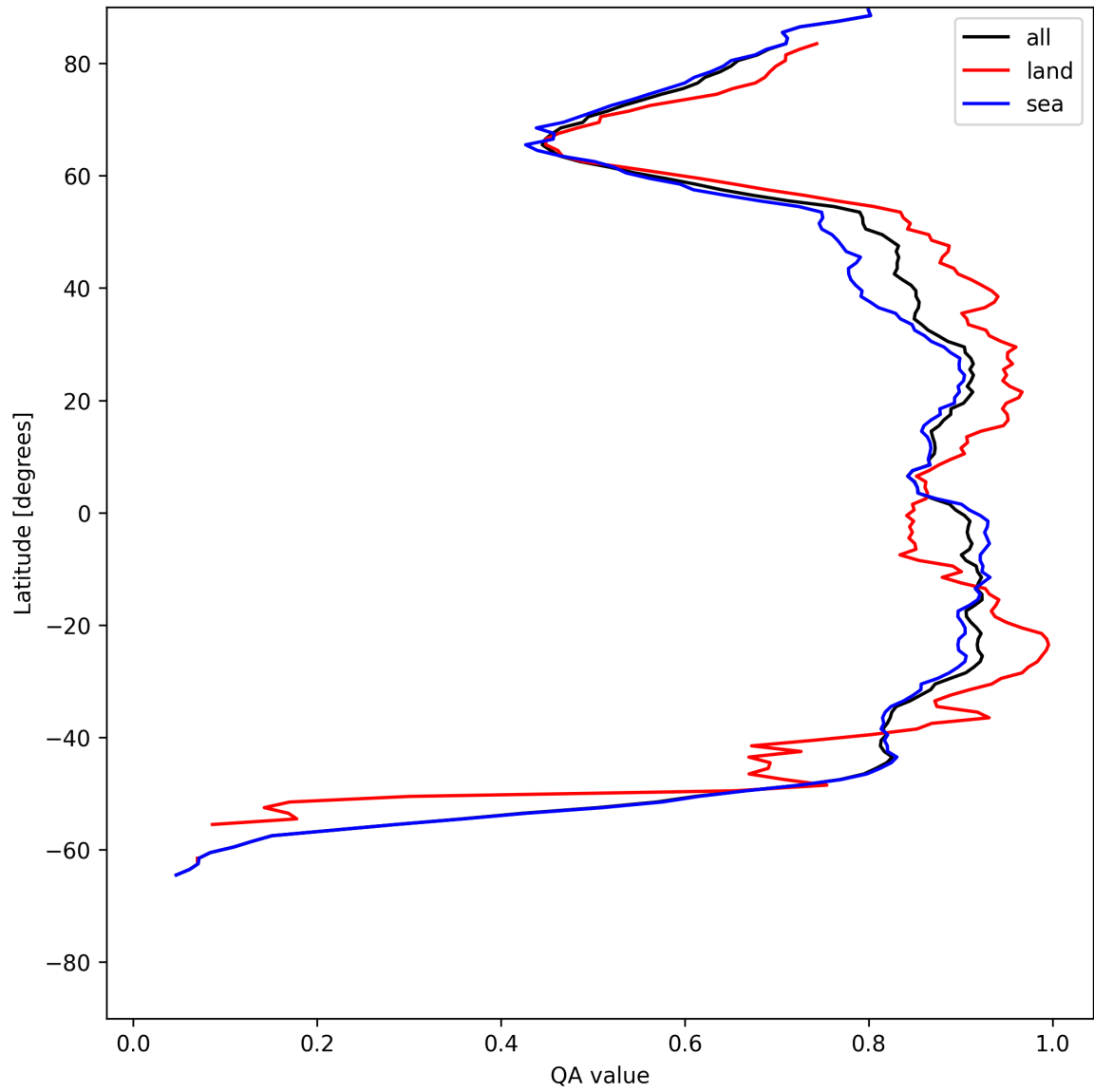
Figure 9: Zonal average of “QA value” for 2025-06-10 to 2025-06-11.
