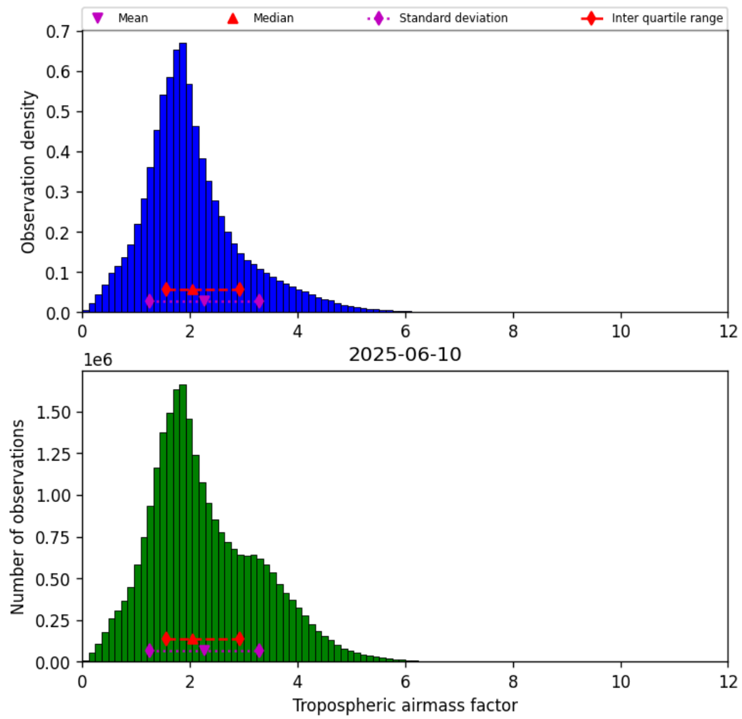
Figure 29: Histogram of “Tropospheric airmass factor” for 2025-06-10 to 2025-06-11
