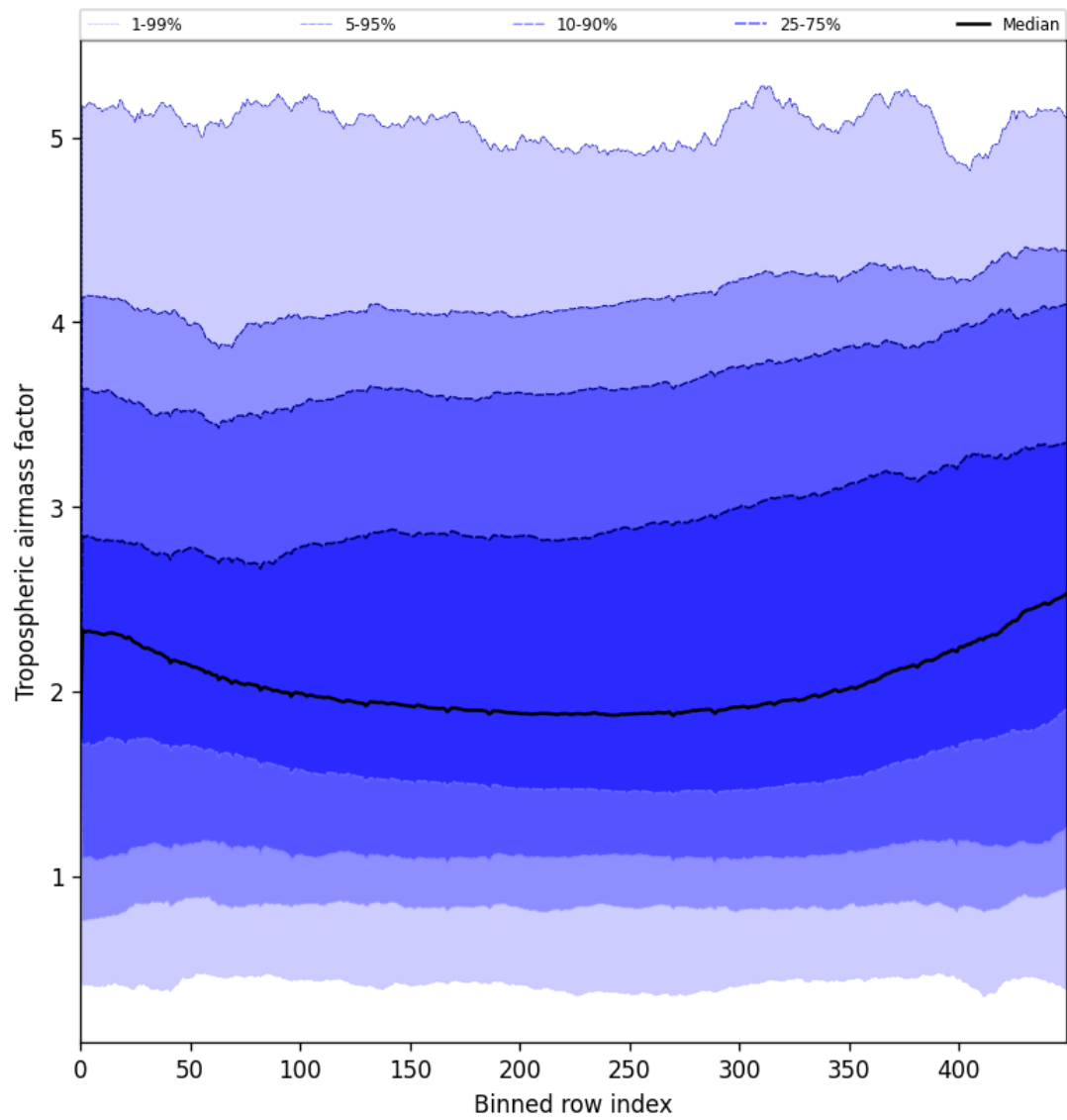
Figure 46: Along track statistics of “Tropospheric airmass factor” for 2025-06-10 to 2025-06-11
