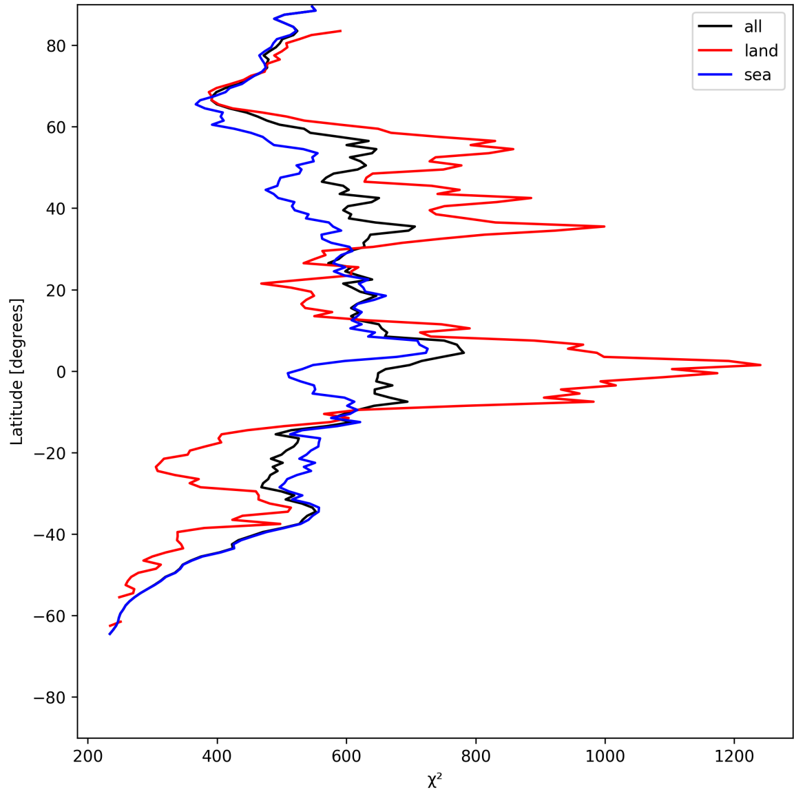
Figure 23: Zonal average of “ \chi^2 ” for 2025-06-10 to 2025-06-11.
