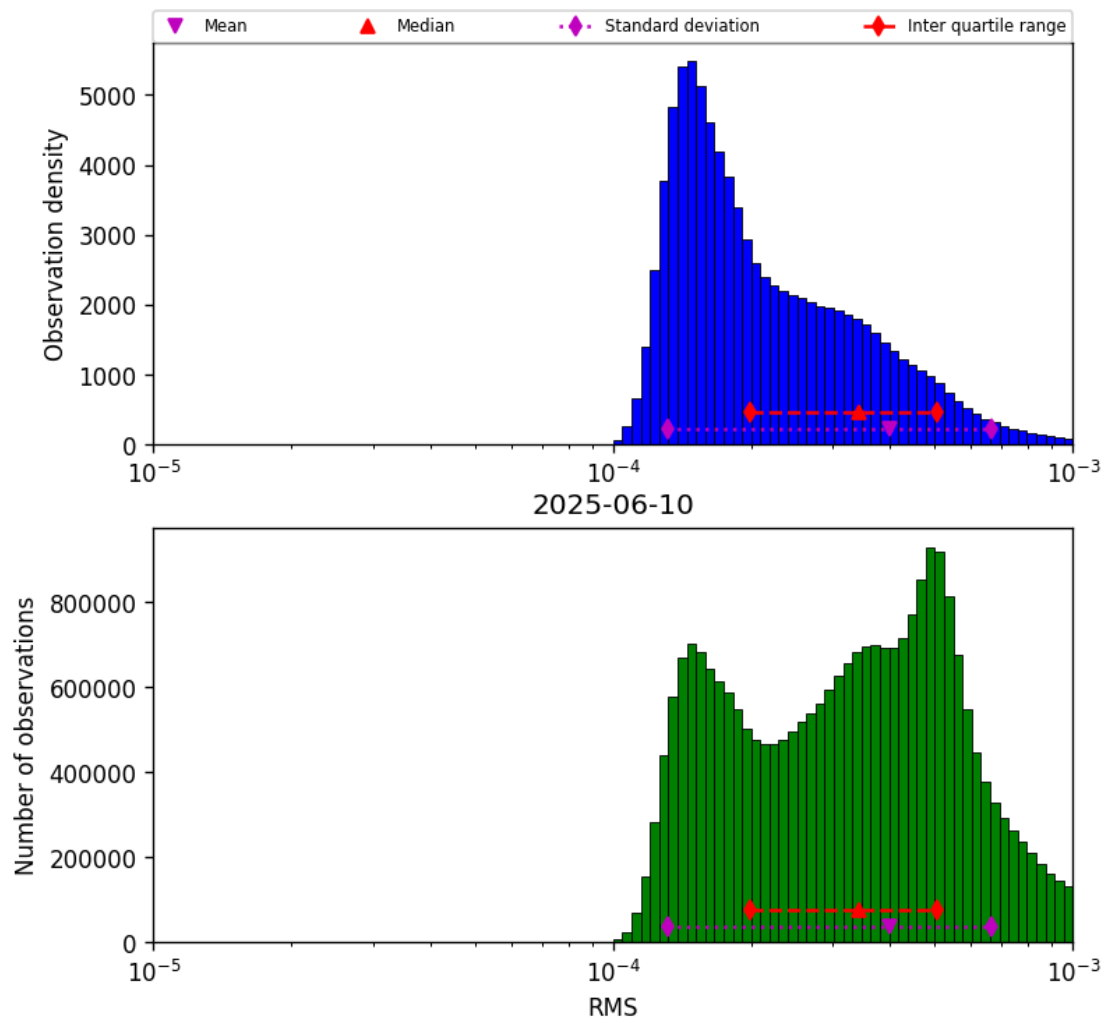
Figure 41: Histogram of “RMS” for 2025-06-10 to 2025-06-11
