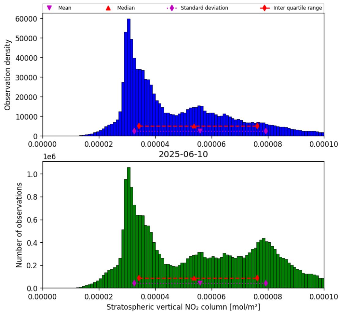
Figure 34: Histogram of “Stratospheric vertical NO 2 column” for 2025-06-10 to 2025-06-11
