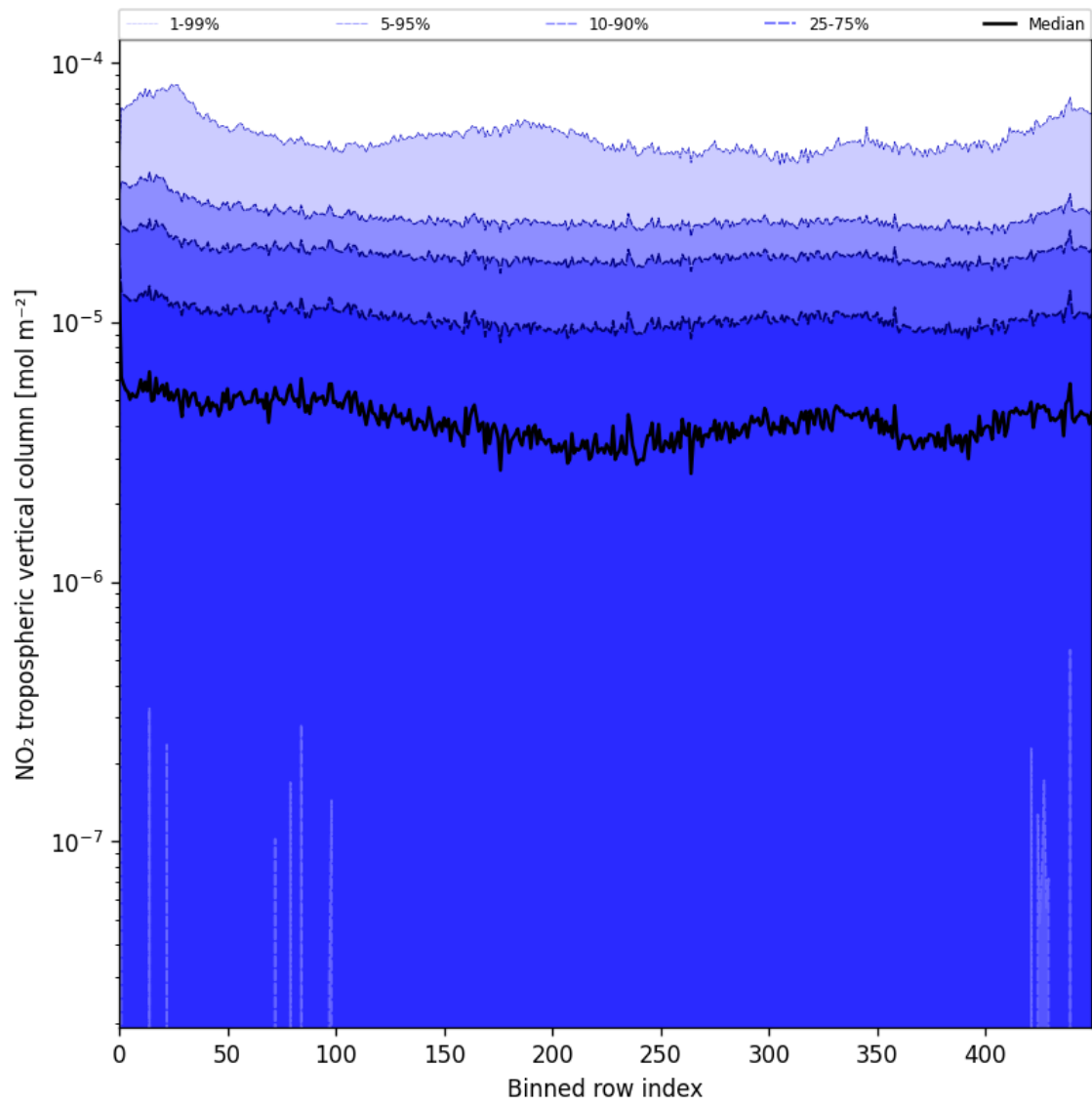
Figure 44: Along track statistics of “NO 2 tropospheric vertical column” for 2025-06-10 to 2025-06-11
