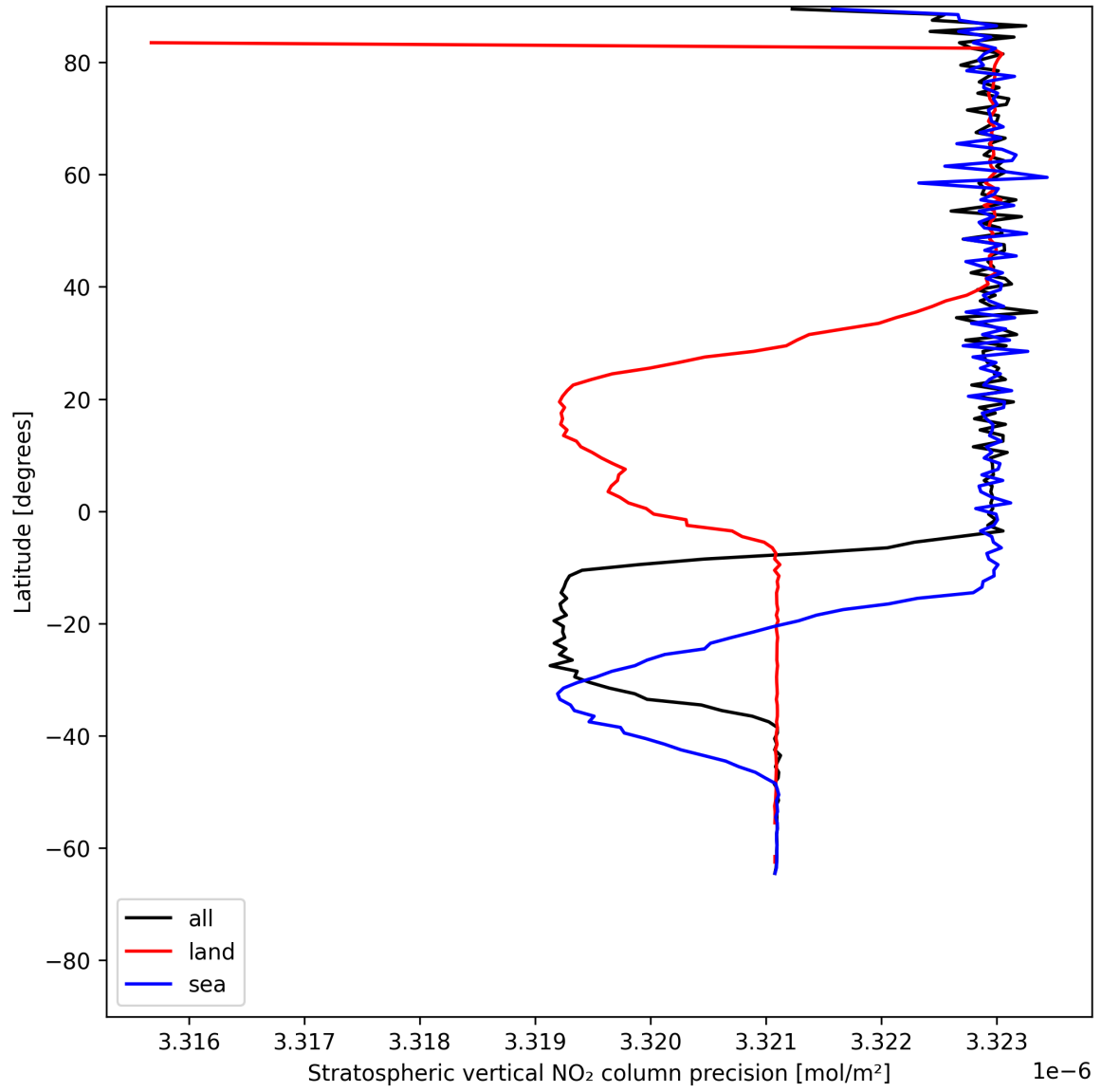
Figure 18: Zonal average of “Stratospheric vertical NO 2 column precision” for 2025-06-10 to 2025-06-11.
