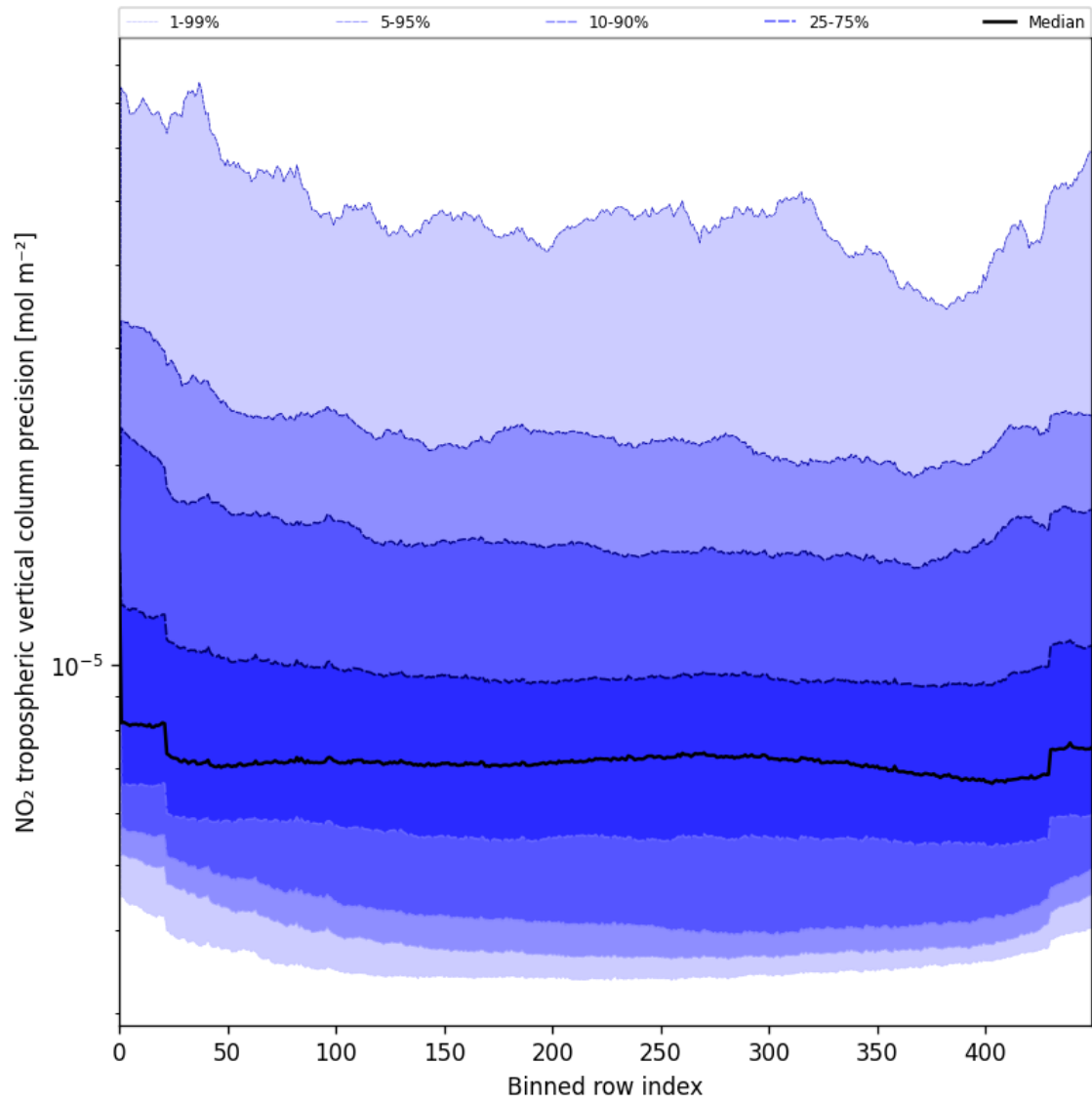
Figure 45: Along track statistics of “NO 2 tropospheric vertical column precision” for 2025-06-10 to 2025-06-11
