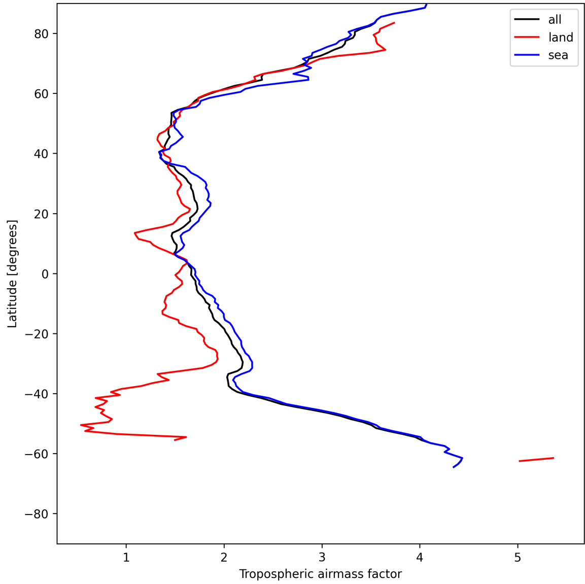
Figure 12: Zonal average of “Tropospheric air mass factor” for 2025-06-10 to 2025-06-11.
