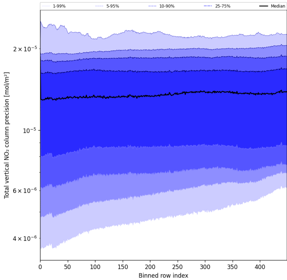
Figure 54: Along track statistics of “Total vertical NO 2 column precision” for 2025-06-10 to 2025-06-11
