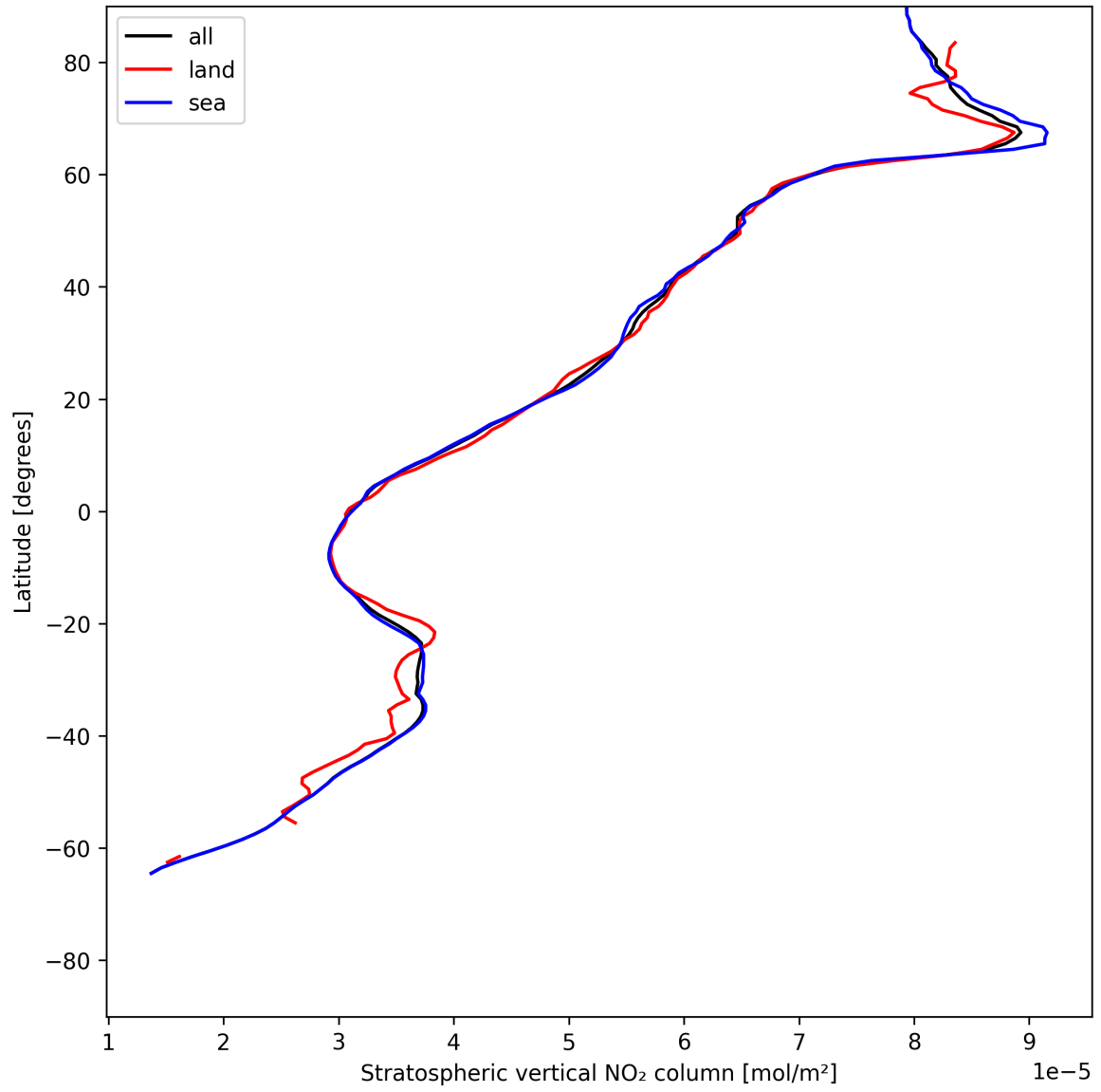
Figure 17: Zonal average of “Stratospheric vertical NO 2 column” for 2025-06-10 to 2025-06-11.
