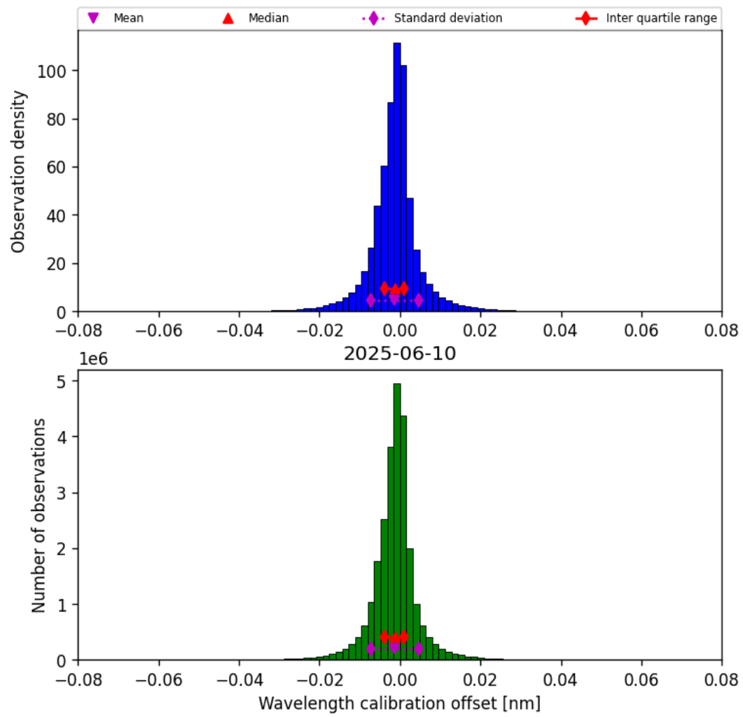
Figure 33: Histogram of “Wavelength calibration offset” for 2025-06-10 to 2025-06-11
