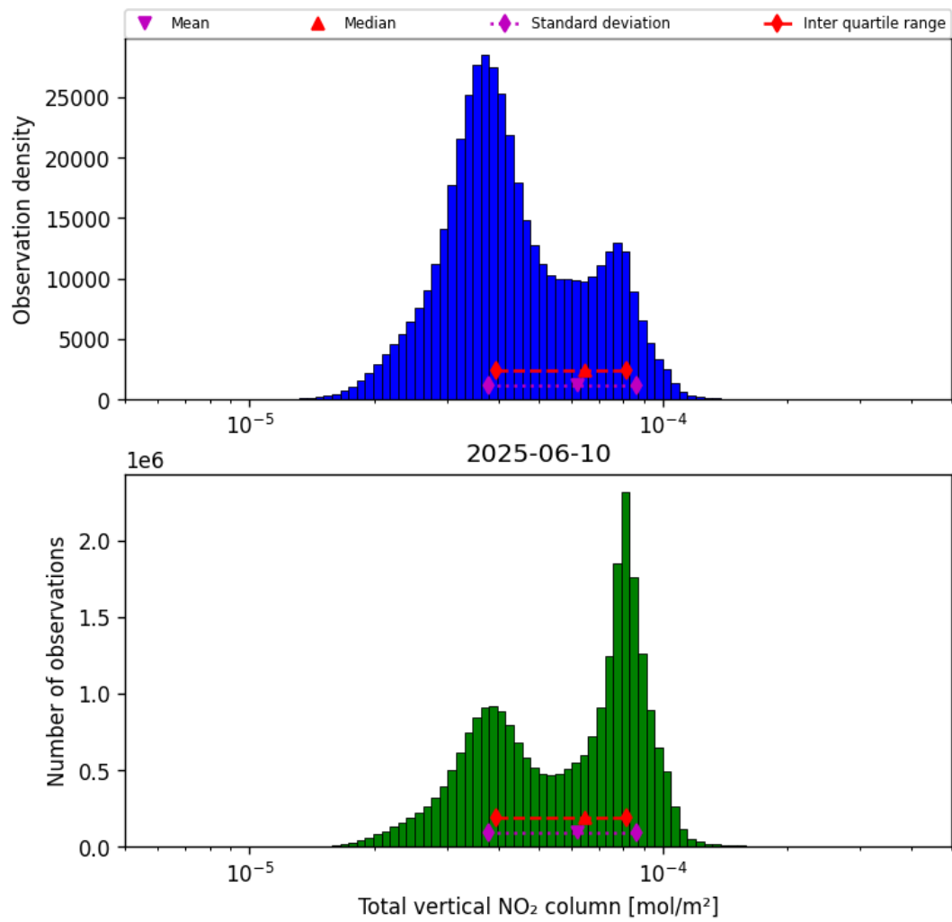
Figure 36: Histogram of “Total vertical NO 2 column” for 2025-06-10 to 2025-06-11
