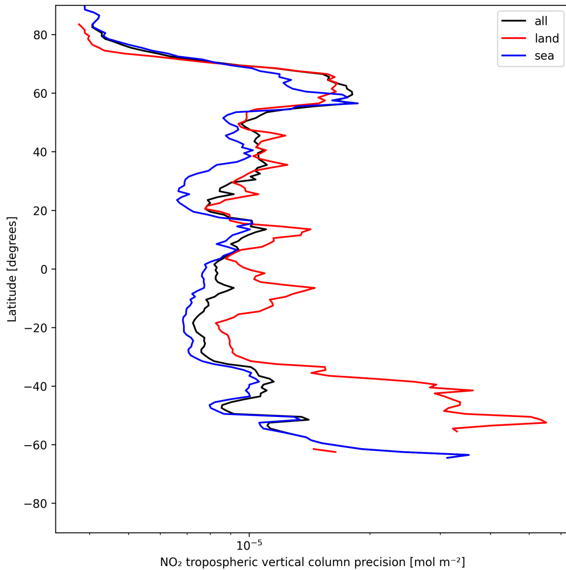
Figure 11: Zonal average of “NO 2 tropospheric vertical column precision” for 2025-06-10 to 2025-06-11.
