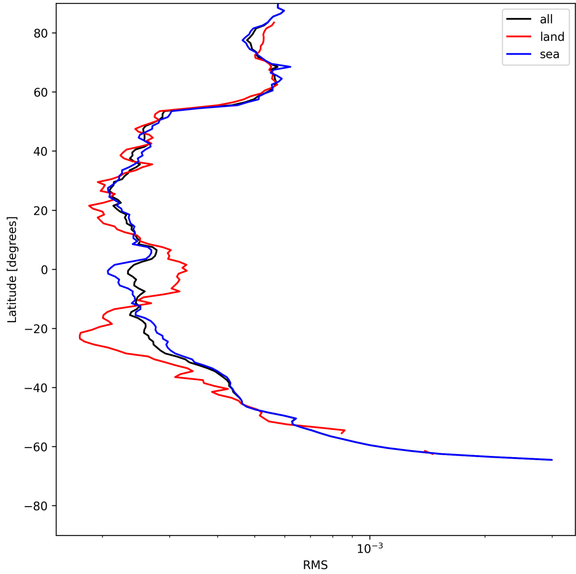
Figure 24: Zonal average of “RMS” for 2025-06-10 to 2025-06-11.
