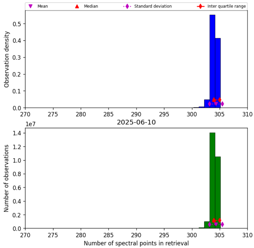
Figure 31: Histogram of “Number of spectral points in retrieval” for 2025-06-10 to 2025-06-11
