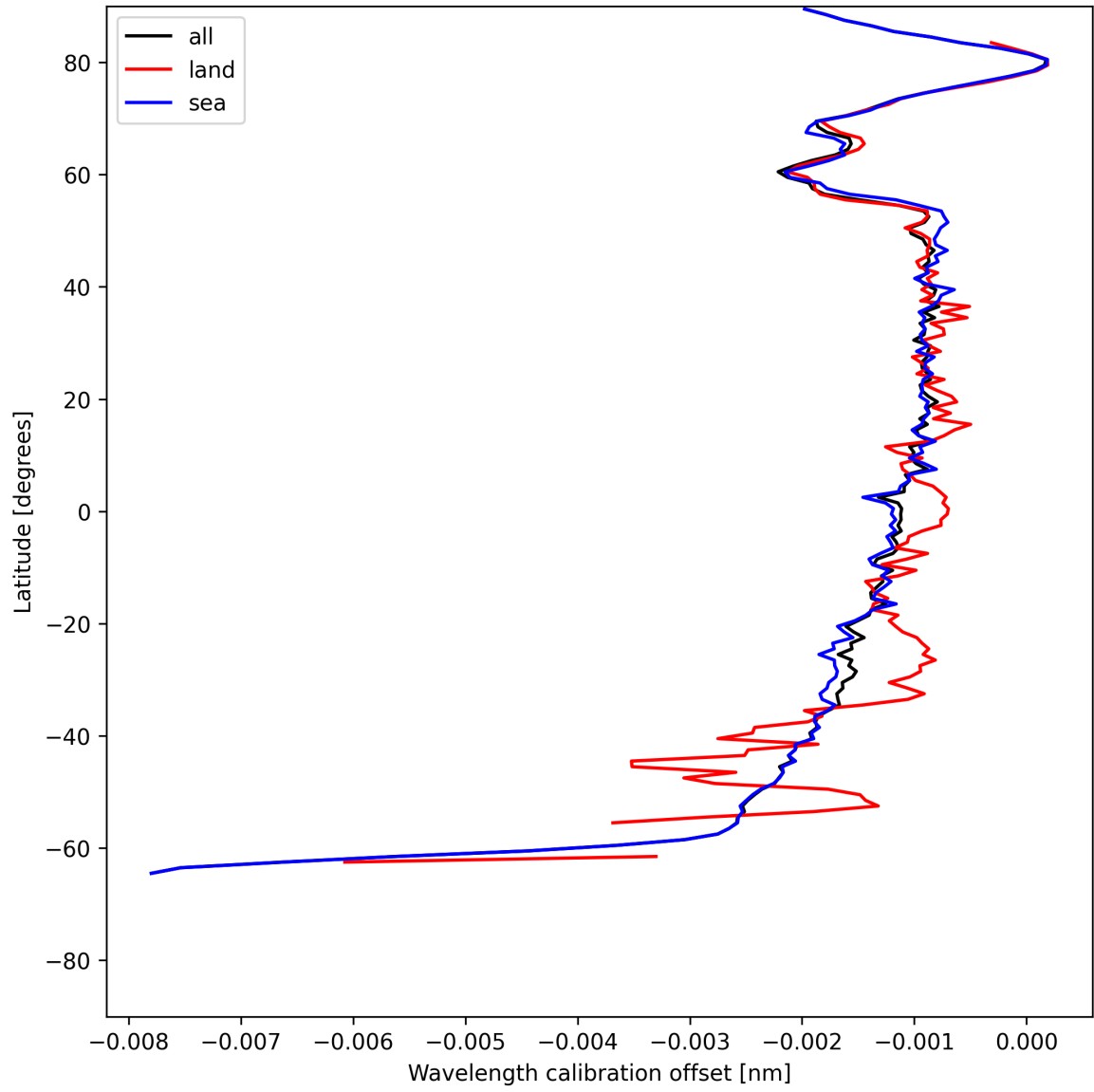
Figure 16: Zonal average of “Wavelength calibration offset” for 2025-06-10 to 2025-06-11.
