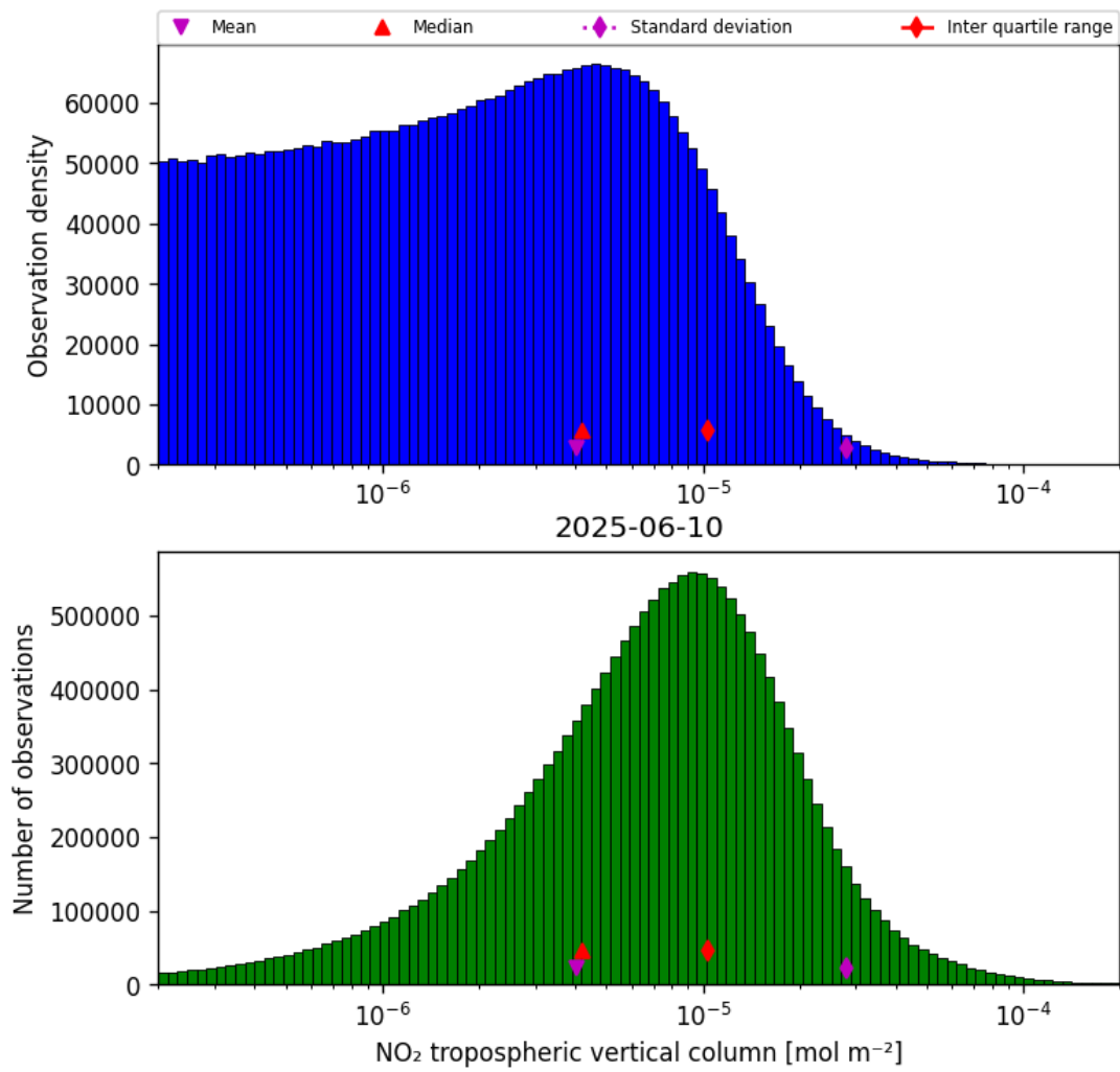
Figure 27: Histogram of “NO 2 tropospheric vertical column” for 2025-06-10 to 2025-06-11
