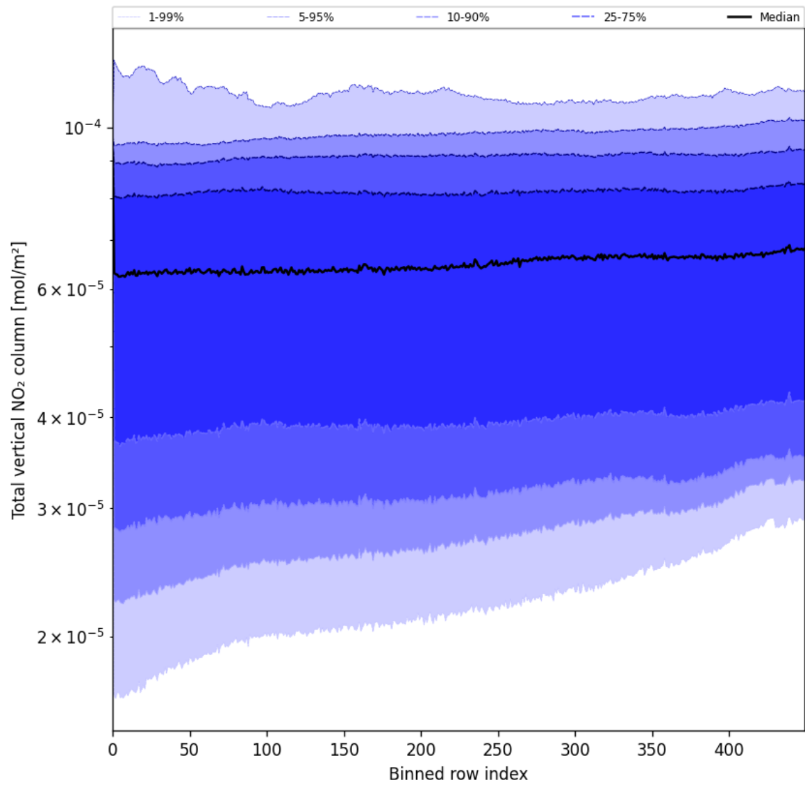
Figure 53: Along track statistics of “Total vertical NO 2 column” for 2025-06-10 to 2025-06-11
