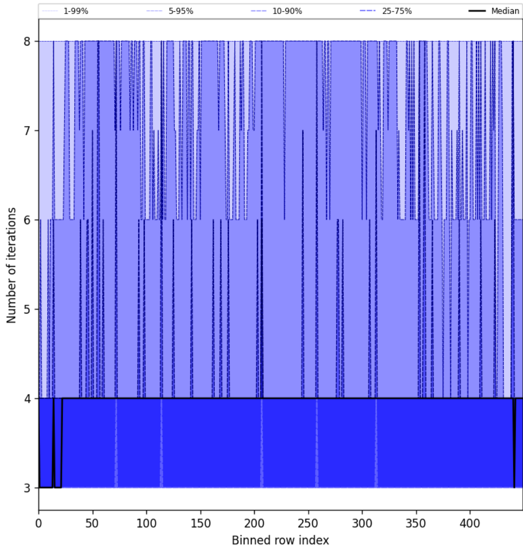
Figure 49: Along track statistics of “Number of iterations” for 2025-06-10 to 2025-06-11
