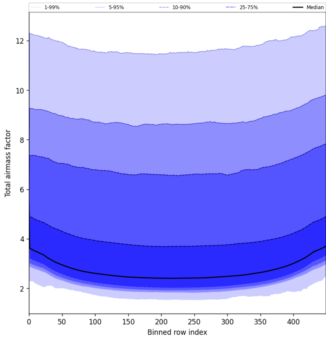
Figure 47: Along track statistics of “Total airmass factor” for 2025-06-10 to 2025-06-11
