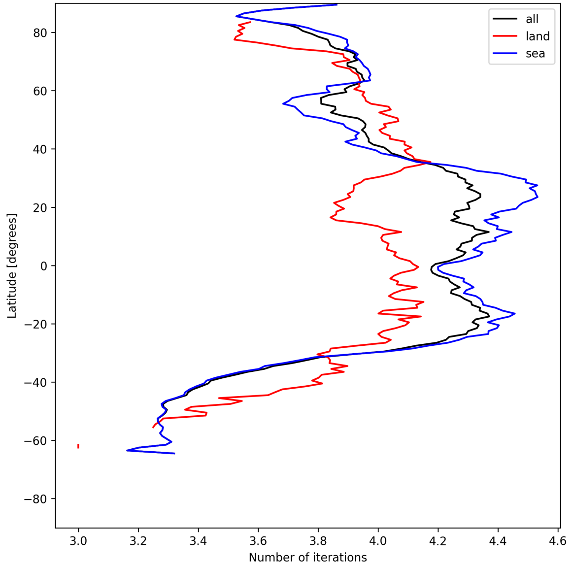
Figure 15: Zonal average of “Number of iterations” for 2025-06-10 to 2025-06-11.
