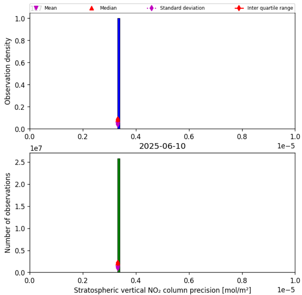
Figure 35: Histogram of “Stratospheric vertical NO 2 column precision” for 2025-06-10 to 2025-06-11
