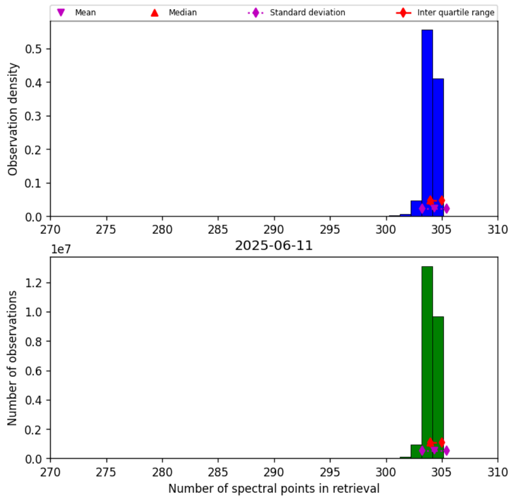
Figure 31: Histogram of “Number of spectral points in retrieval” for 2025-06-11 to 2025-06-12
