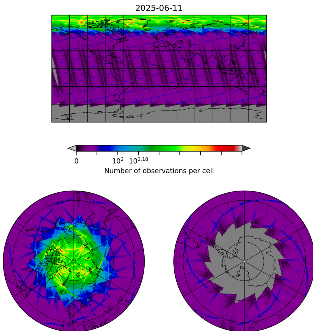
Figure 8: Map of the number of observations for 2025-06-11 to 2025-06-12
