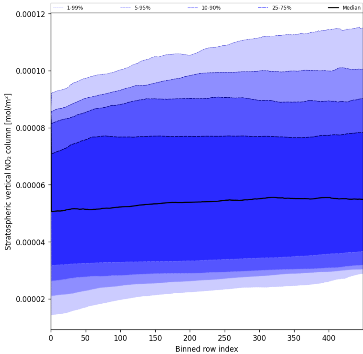
Figure 51: Along track statistics of “Stratospheric vertical NO 2 column” for 2025-06-11 to 2025-06-12
