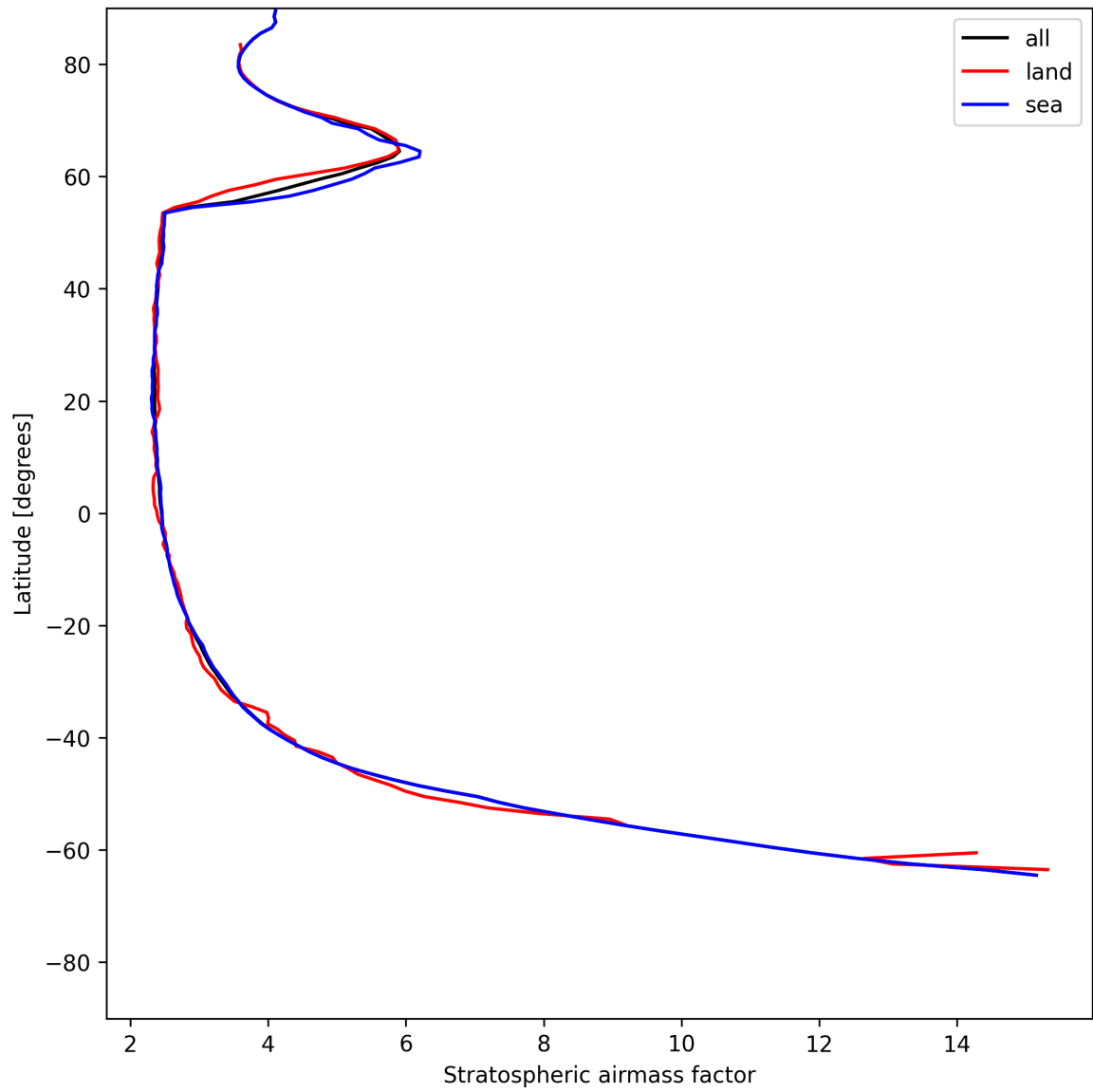
Figure 25: Zonal average of “Stratospheric airmass factor” for 2025-06-11 to 2025-06-12.
