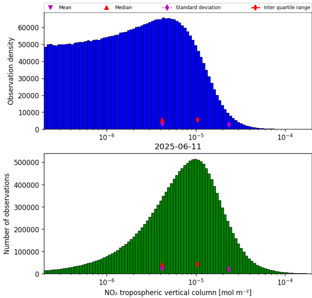
Figure 27: Histogram of “NO 2 tropospheric vertical column” for 2025-06-11 to 2025-06-12
