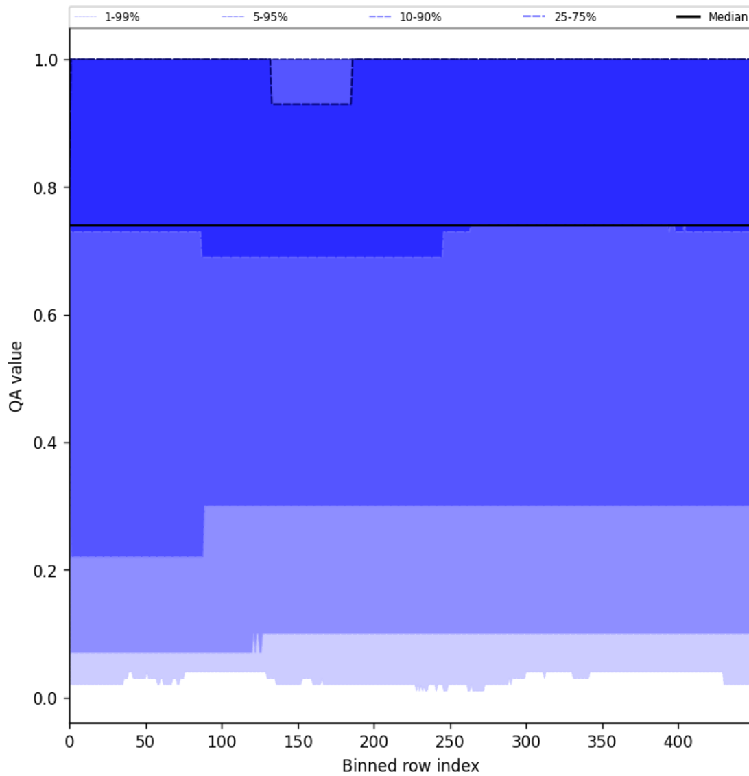
Figure 43: Along track statistics of “QA value” for 2025-06-11 to 2025-06-12
