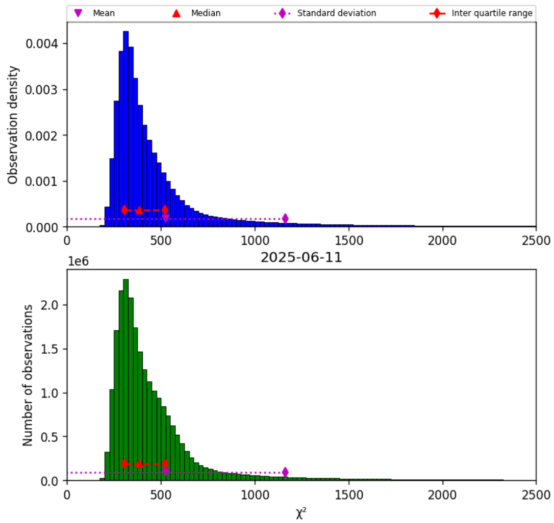
Figure 40: Histogram of “ \chi^2 ” for 2025-06-11 to 2025-06-12
