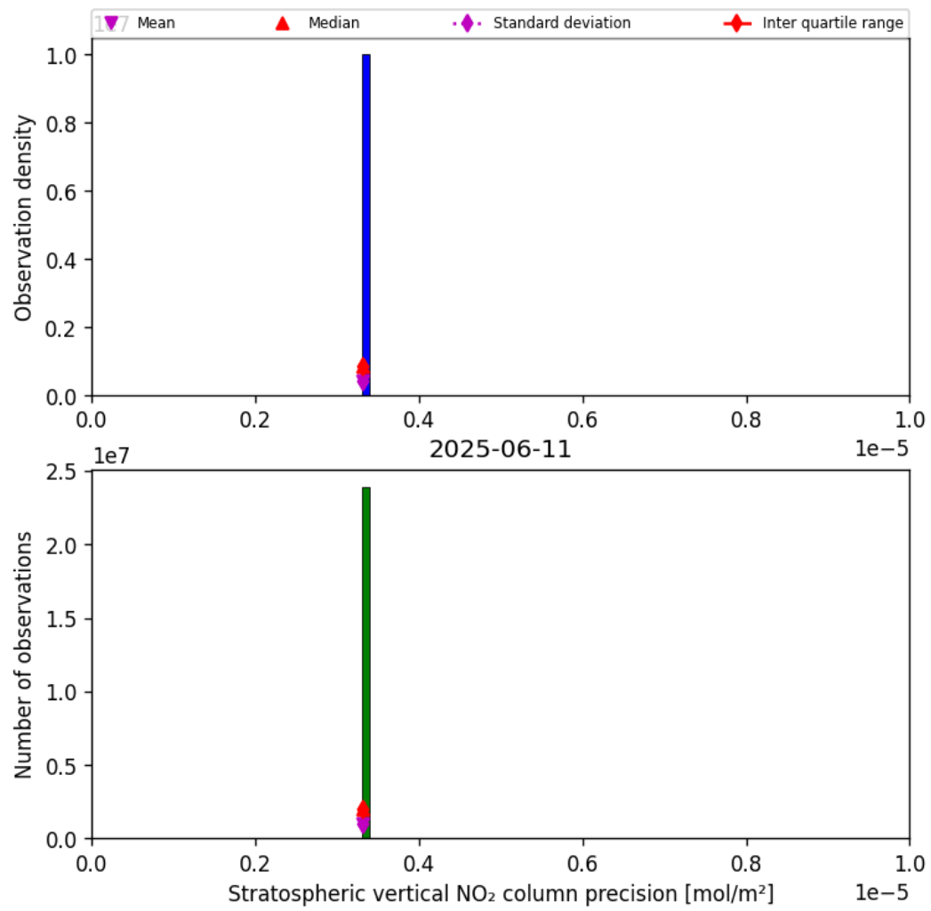
Figure 35: Histogram of “Stratospheric vertical NO 2 column precision” for 2025-06-11 to 2025-06-12
