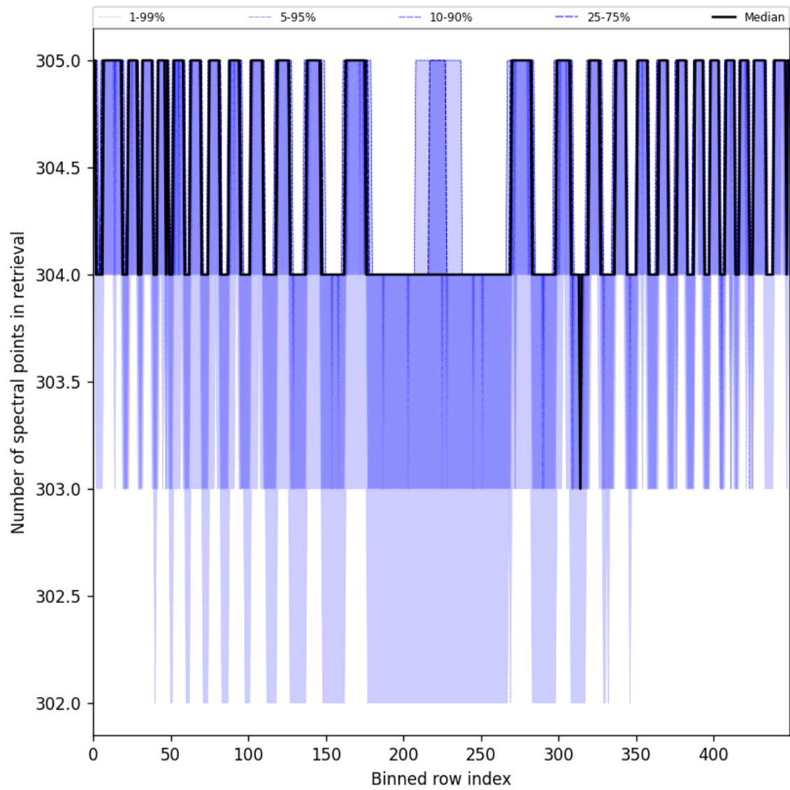
Figure 48: Along track statistics of “Number of spectral points in retrieval” for 2025-06-11 to 2025-06-12
