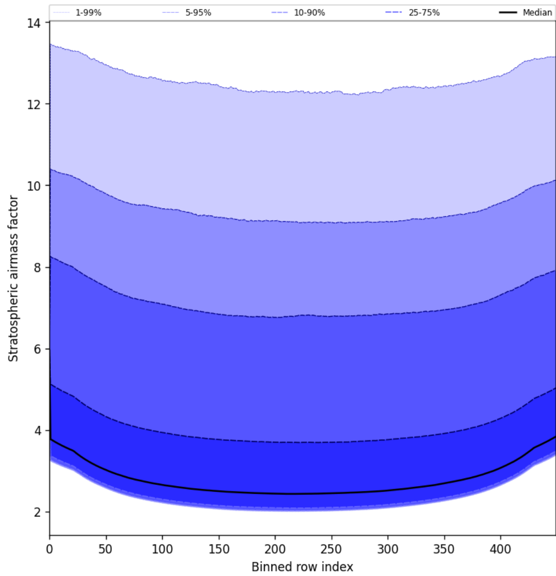
Figure 59: Along track statistics of “Stratospheric airmass factor” for 2025-06-11 to 2025-06-12
