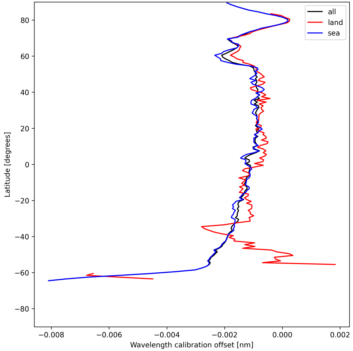
Figure 16: Zonal average of “Wavelength calibration offset” for 2025-06-11 to 2025-06-12.
