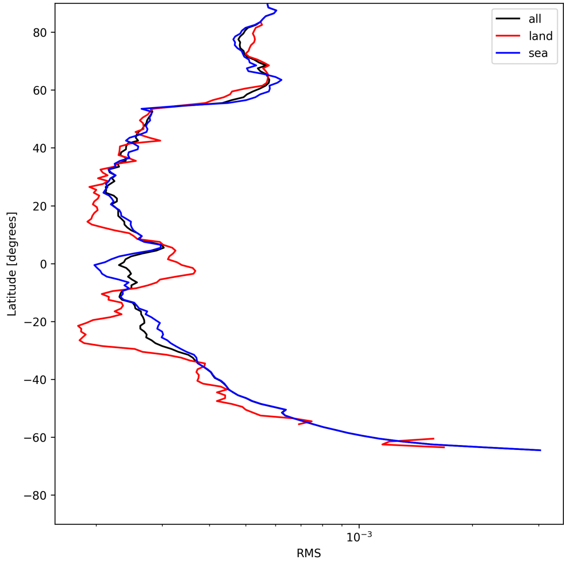
Figure 24: Zonal average of “RMS” for 2025-06-11 to 2025-06-12.
