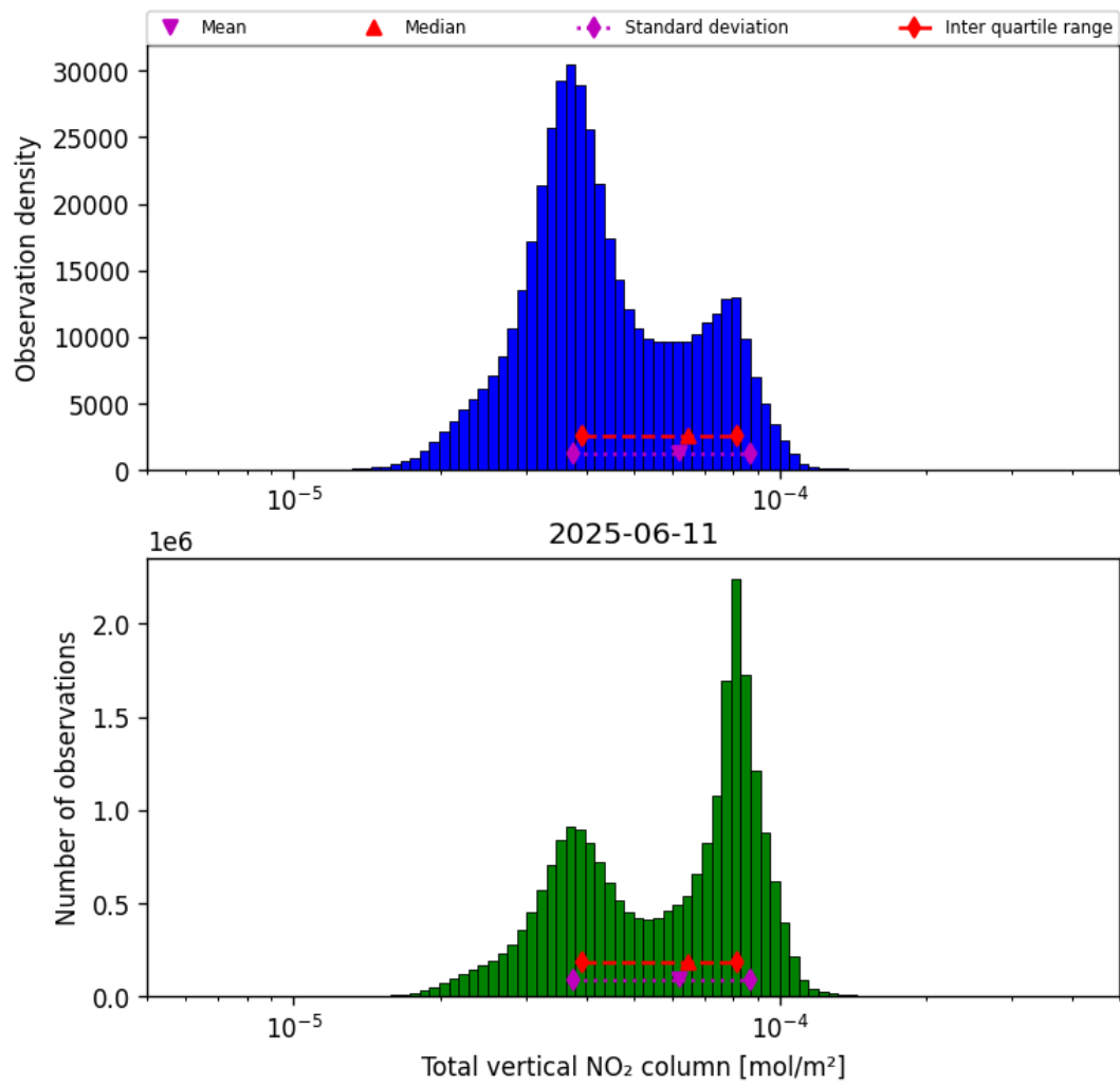
Figure 36: Histogram of “Total vertical NO 2 column” for 2025-06-11 to 2025-06-12
