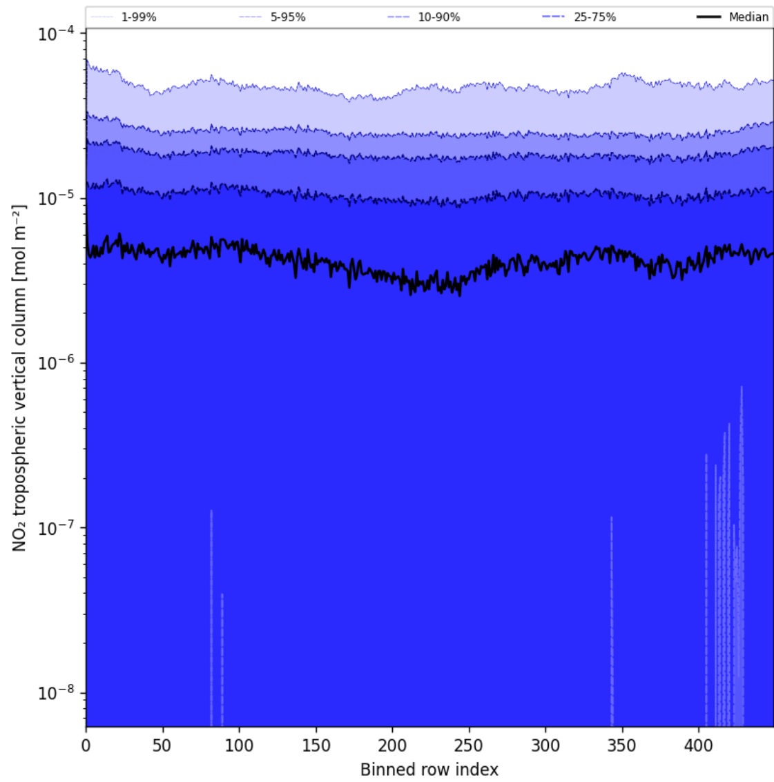
Figure 44: Along track statistics of “NO 2 tropospheric vertical column” for 2025-06-11 to 2025-06-12
