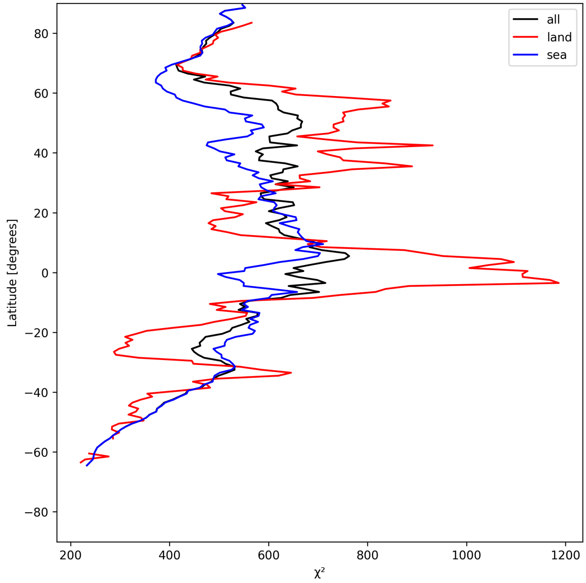
Figure 23: Zonal average of “ \chi^2 ” for 2025-06-11 to 2025-06-12.
