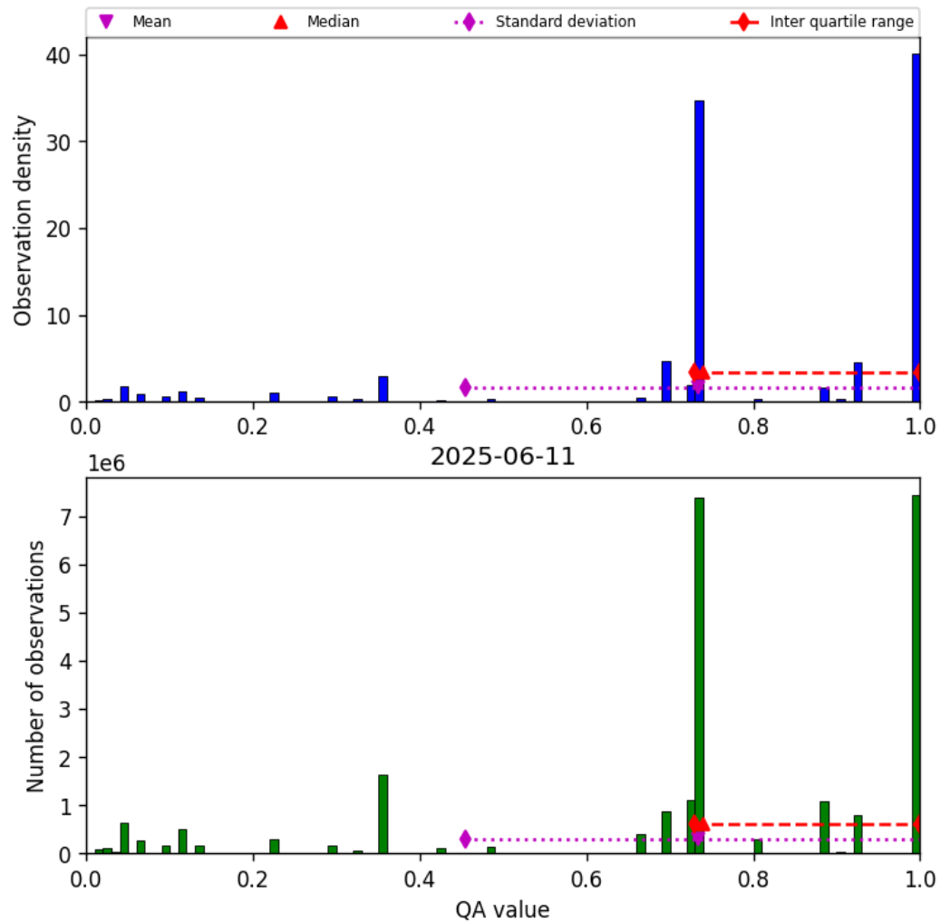
Figure 26: Histogram of “QA value” for 2025-06-11 to 2025-06-12
