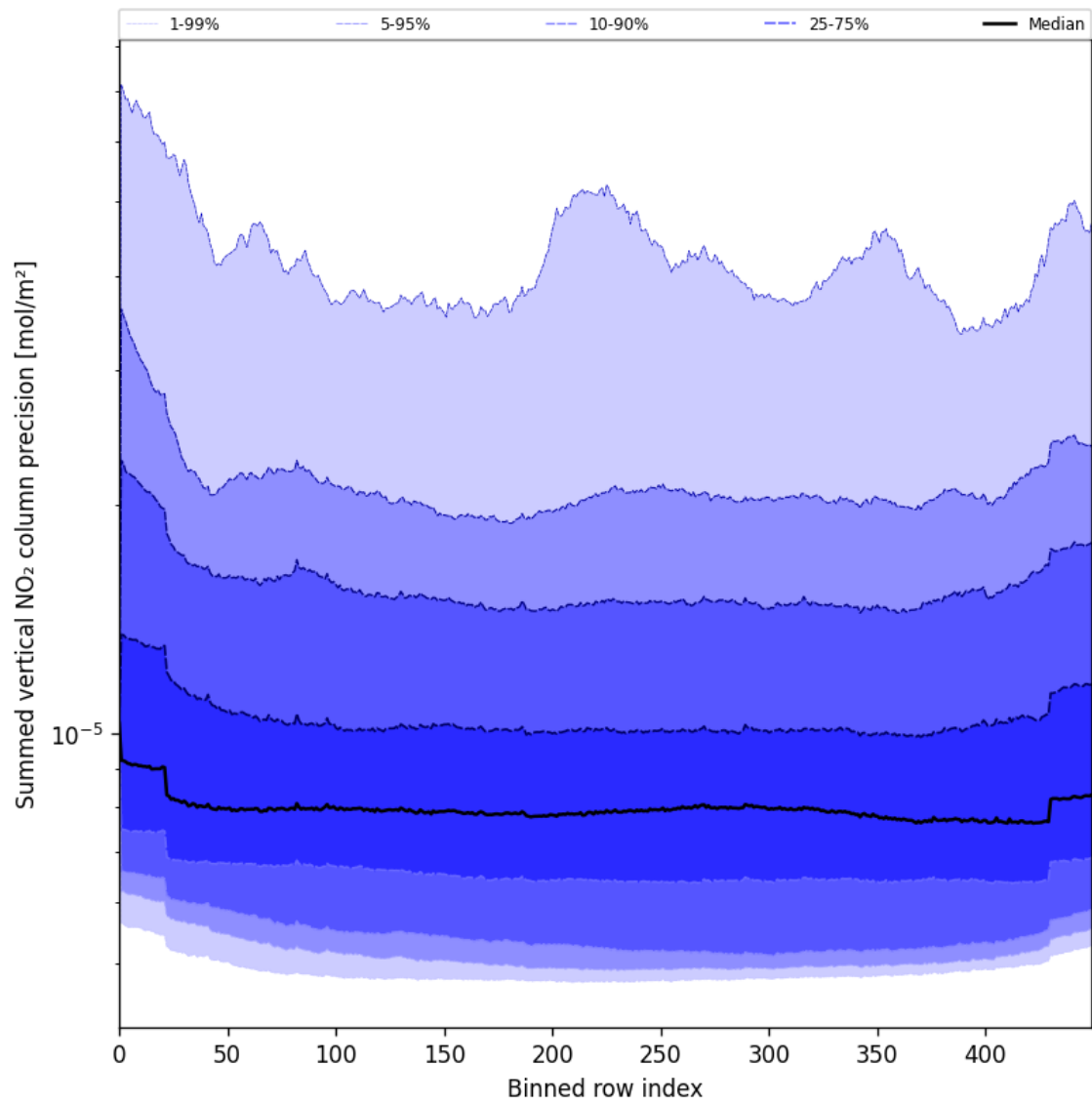
Figure 56: Along track statistics of “Summed vertical NO 2 column precision” for 2025-06-11 to 2025-06-12
