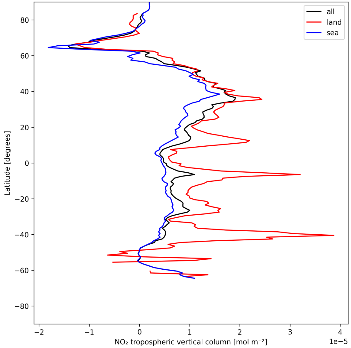
Figure 10: Zonal average of “NO 2 tropospheric vertical column” for 2025-06-11 to 2025-06-12.
