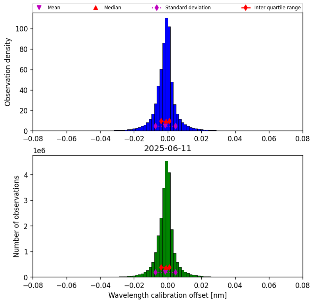
Figure 33: Histogram of “Wavelength calibration offset” for 2025-06-11 to 2025-06-12
