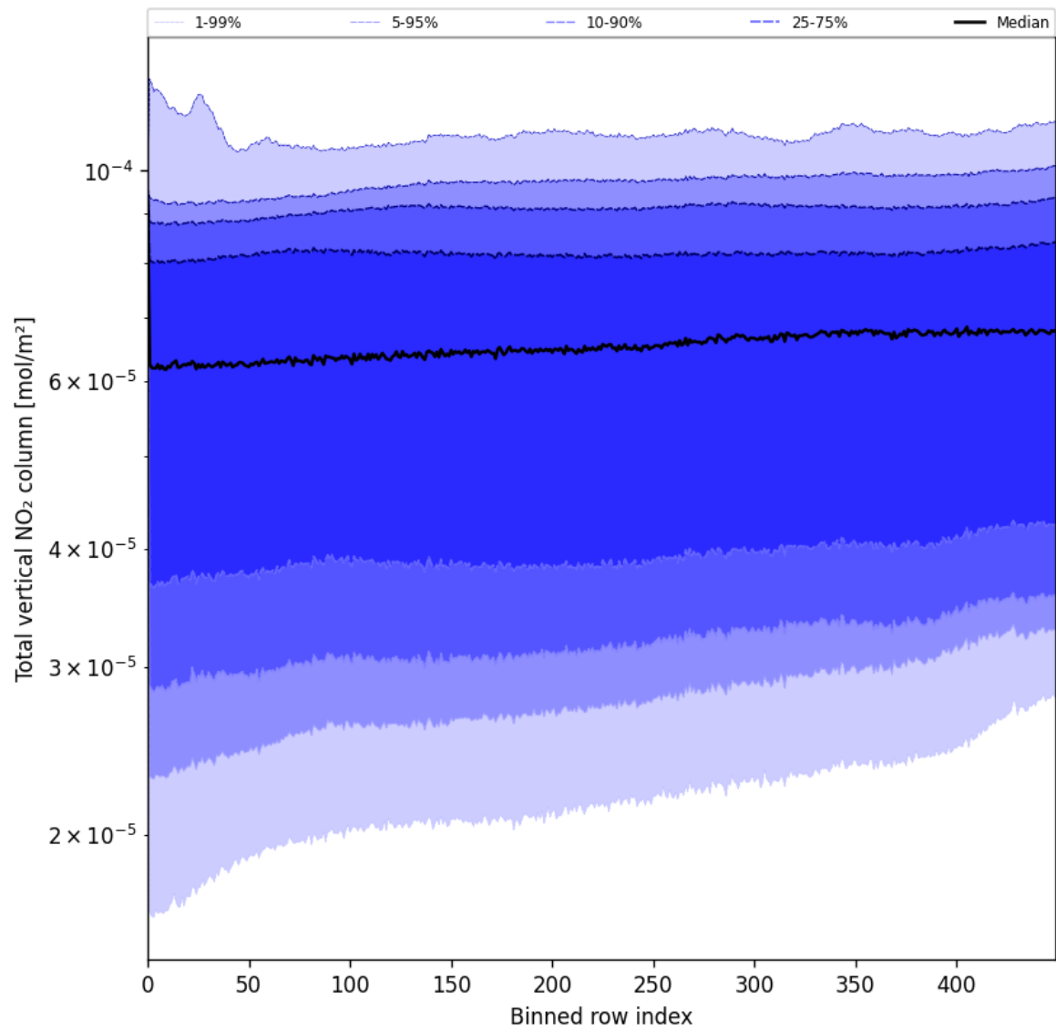
Figure 53: Along track statistics of “Total vertical NO 2 column” for 2025-06-11 to 2025-06-12
