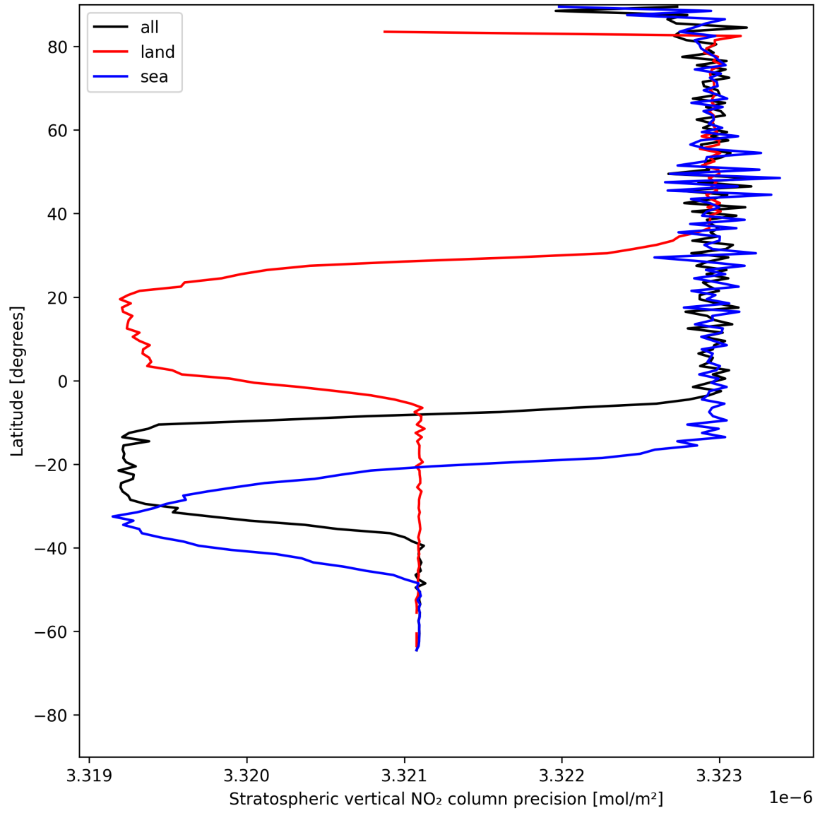
Figure 18: Zonal average of “Stratospheric vertical NO 2 column precision” for 2025-06-11 to 2025-06-12.
