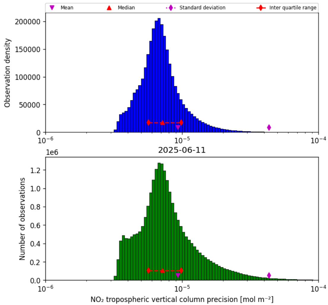
Figure 28: Histogram of “NO 2 tropospheric vertical column precision” for 2025-06-11 to 2025-06-12
