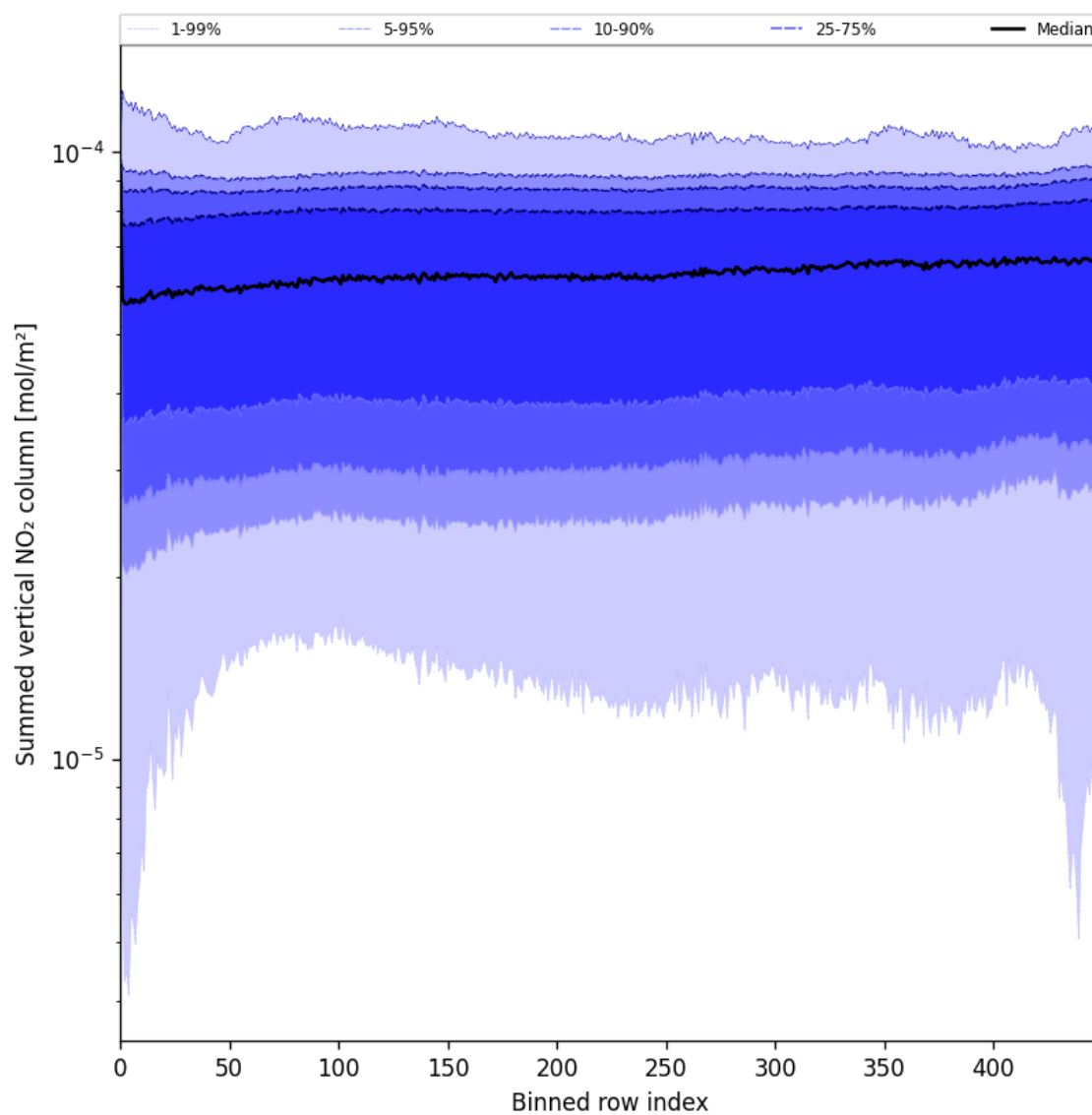
Figure 55: Along track statistics of “Summed vertical NO 2 column” for 2025-06-11 to 2025-06-12
