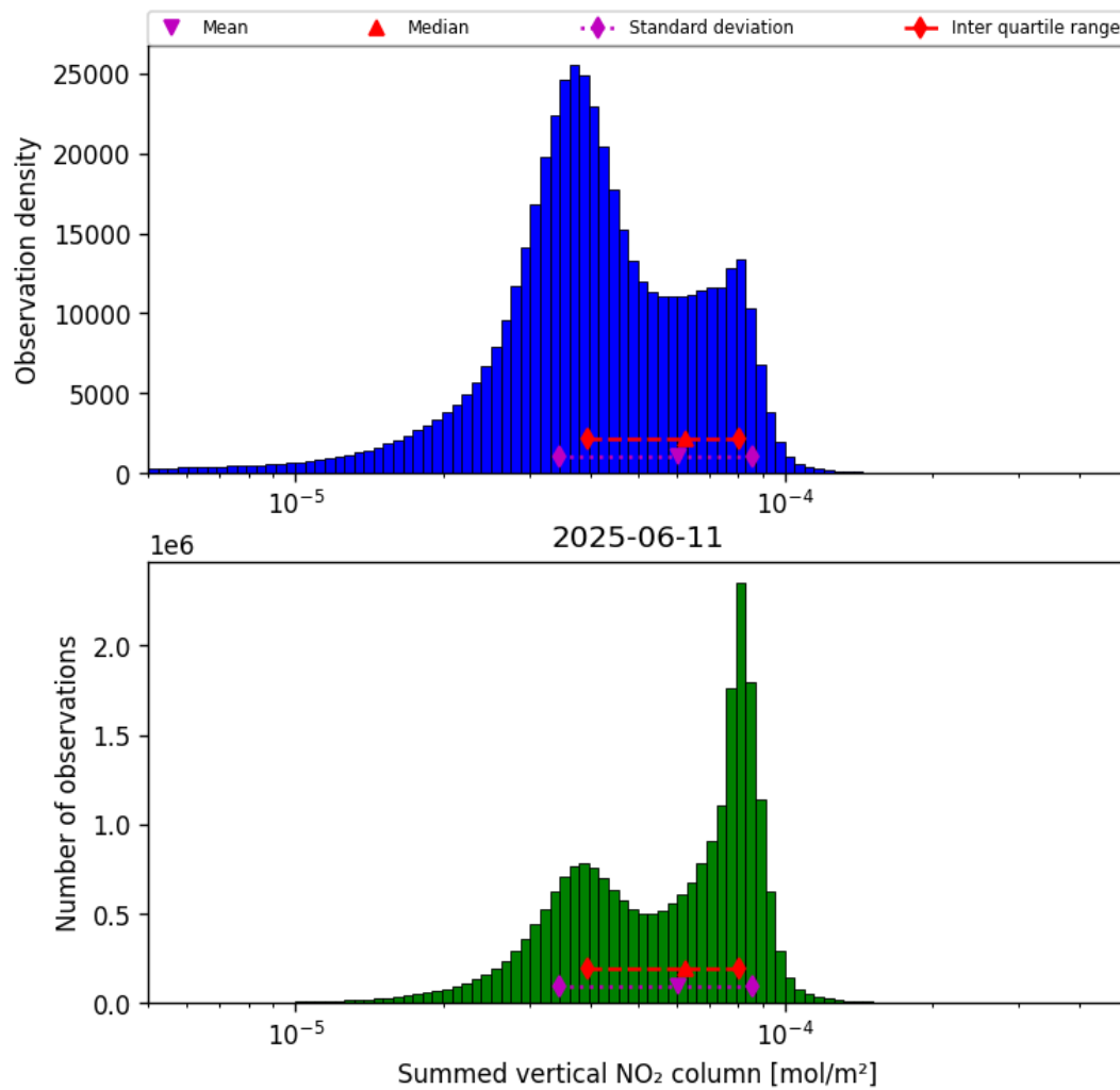
Figure 38: Histogram of “Summed vertical NO 2 column” for 2025-06-11 to 2025-06-12
