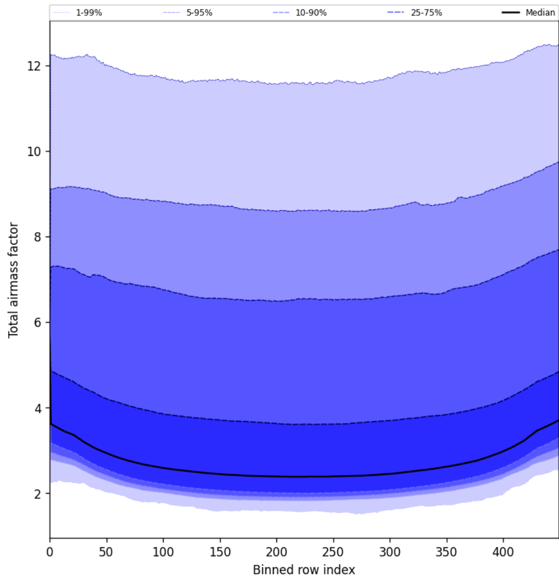
Figure 47: Along track statistics of “Total airmass factor” for 2025-06-11 to 2025-06-12
