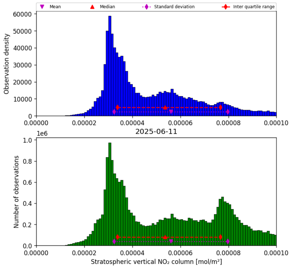
Figure 34: Histogram of “Stratospheric vertical NO 2 column” for 2025-06-11 to 2025-06-12
