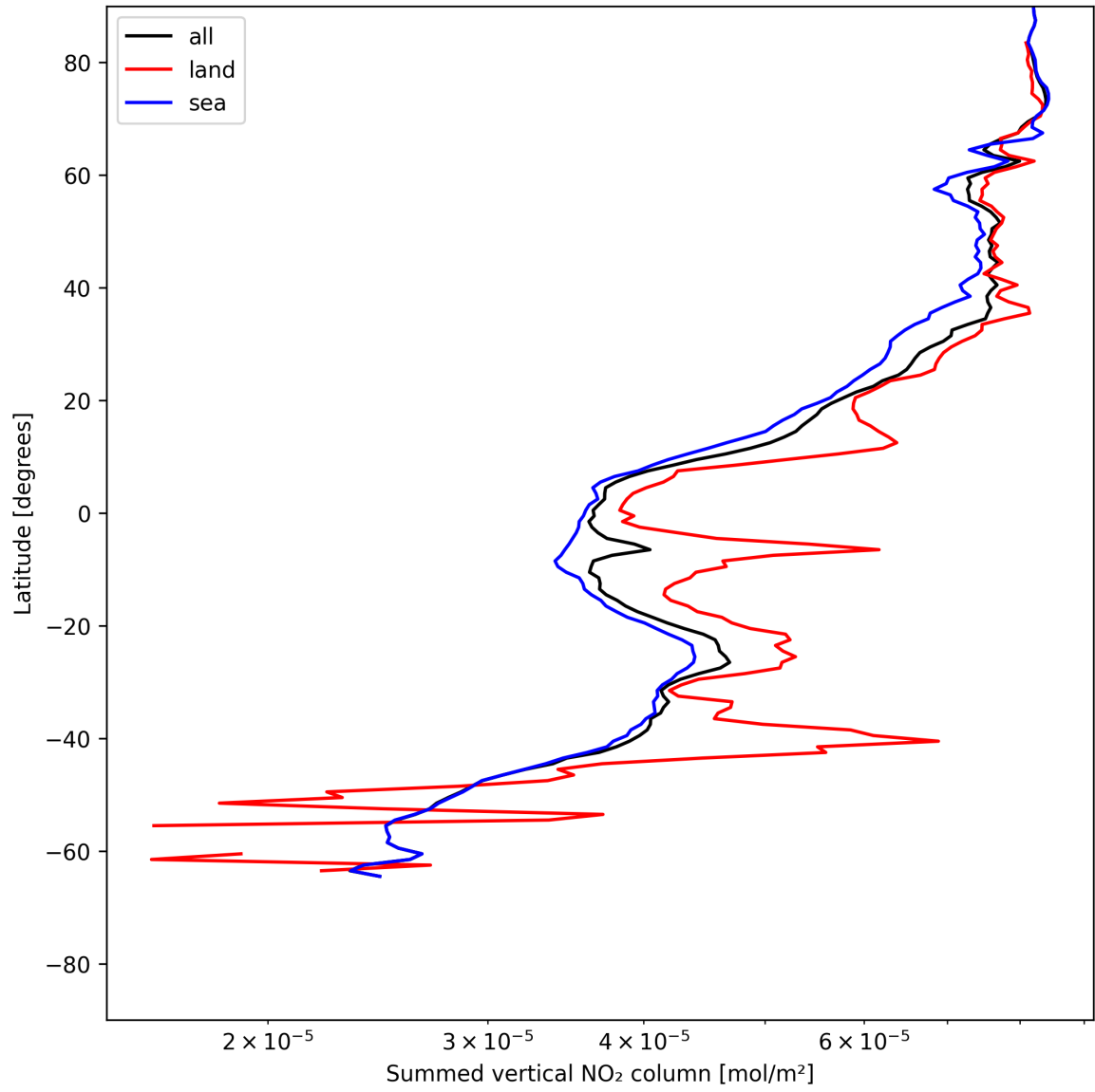
Figure 21: Zonal average of “Summed vertical NO 2 column” for 2025-06-11 to 2025-06-12.
