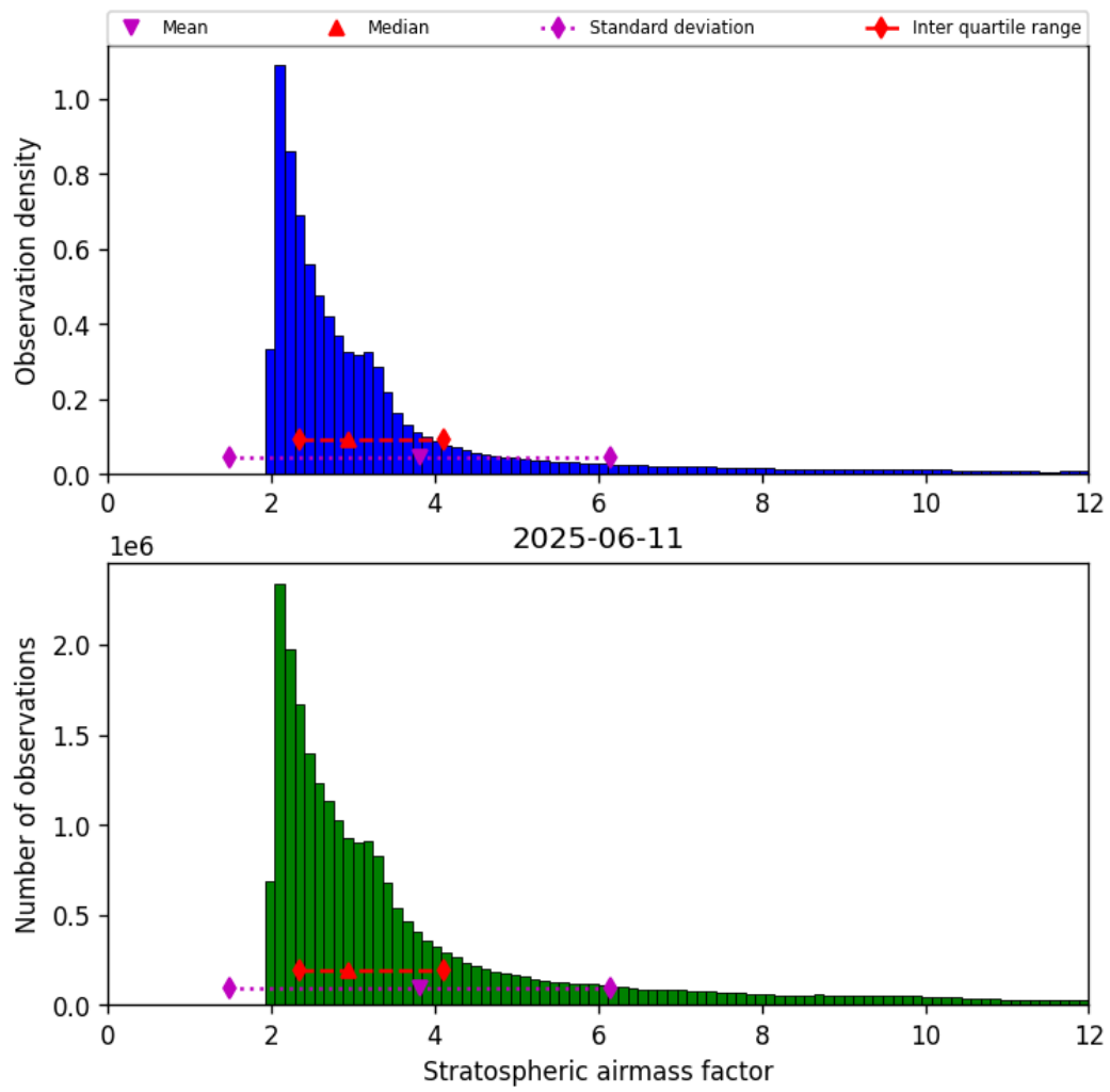
Figure 42: Histogram of “Stratospheric airmass factor” for 2025-06-11 to 2025-06-12
