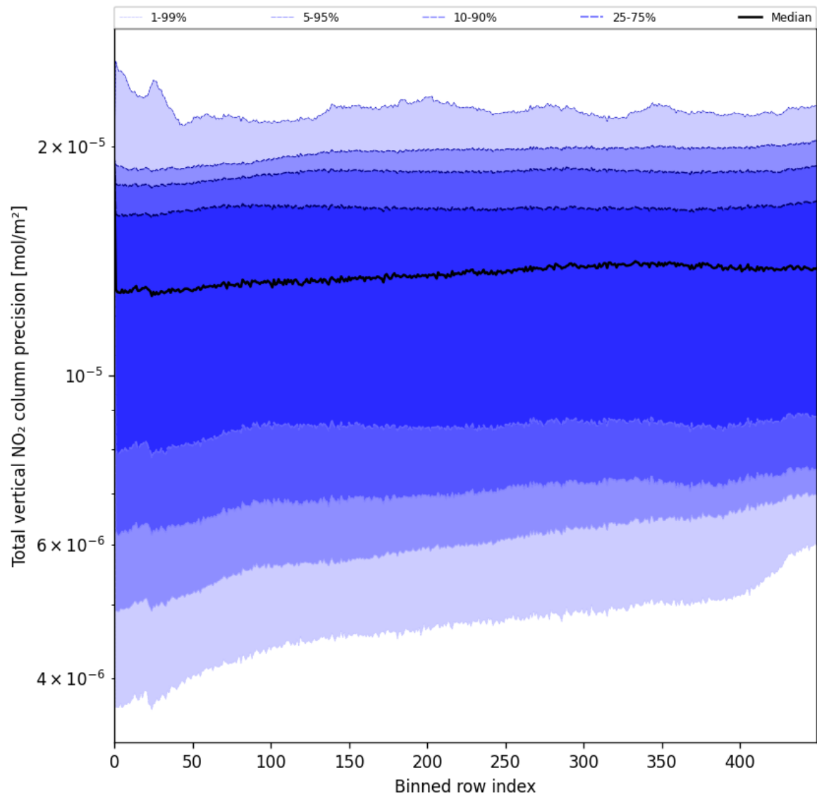
Figure 54: Along track statistics of "Total vertical NO 2 column precision" for 2025-06-11 to 2025-06-12
