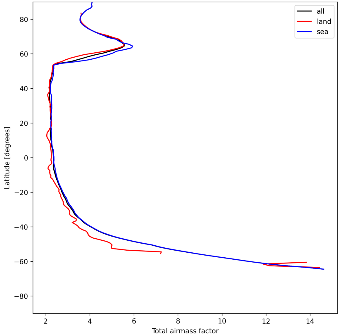
Figure 13: Zonal average of “Total airmass factor” for 2025-06-11 to 2025-06-12.
