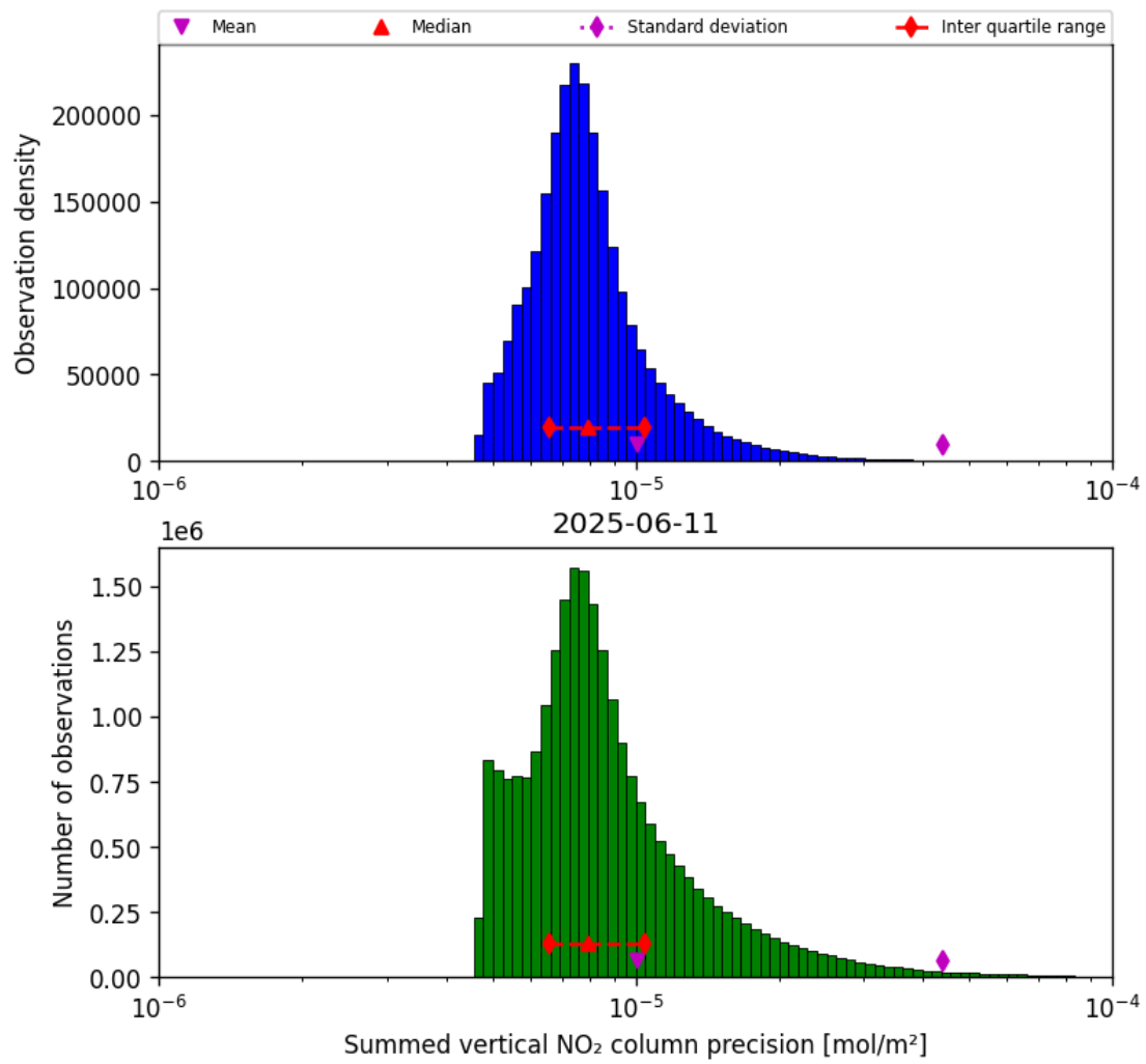
Figure 39: Histogram of “Summed vertical NO 2 column precision” for 2025-06-11 to 2025-06-12
