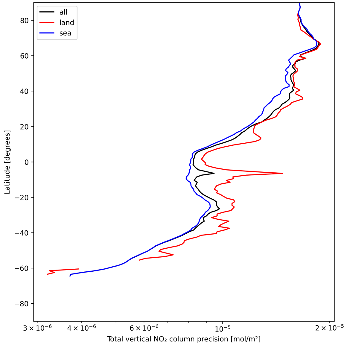
Figure 20: Zonal average of “Total vertical NO 2 column precision” for 2025-06-11 to 2025-06-12.
