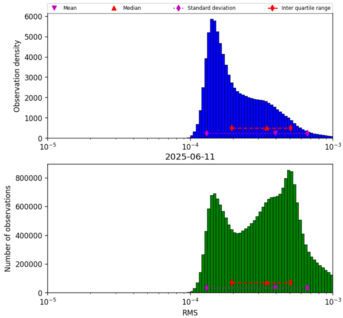
Figure 41: Histogram of “RMS” for 2025-06-11 to 2025-06-12
