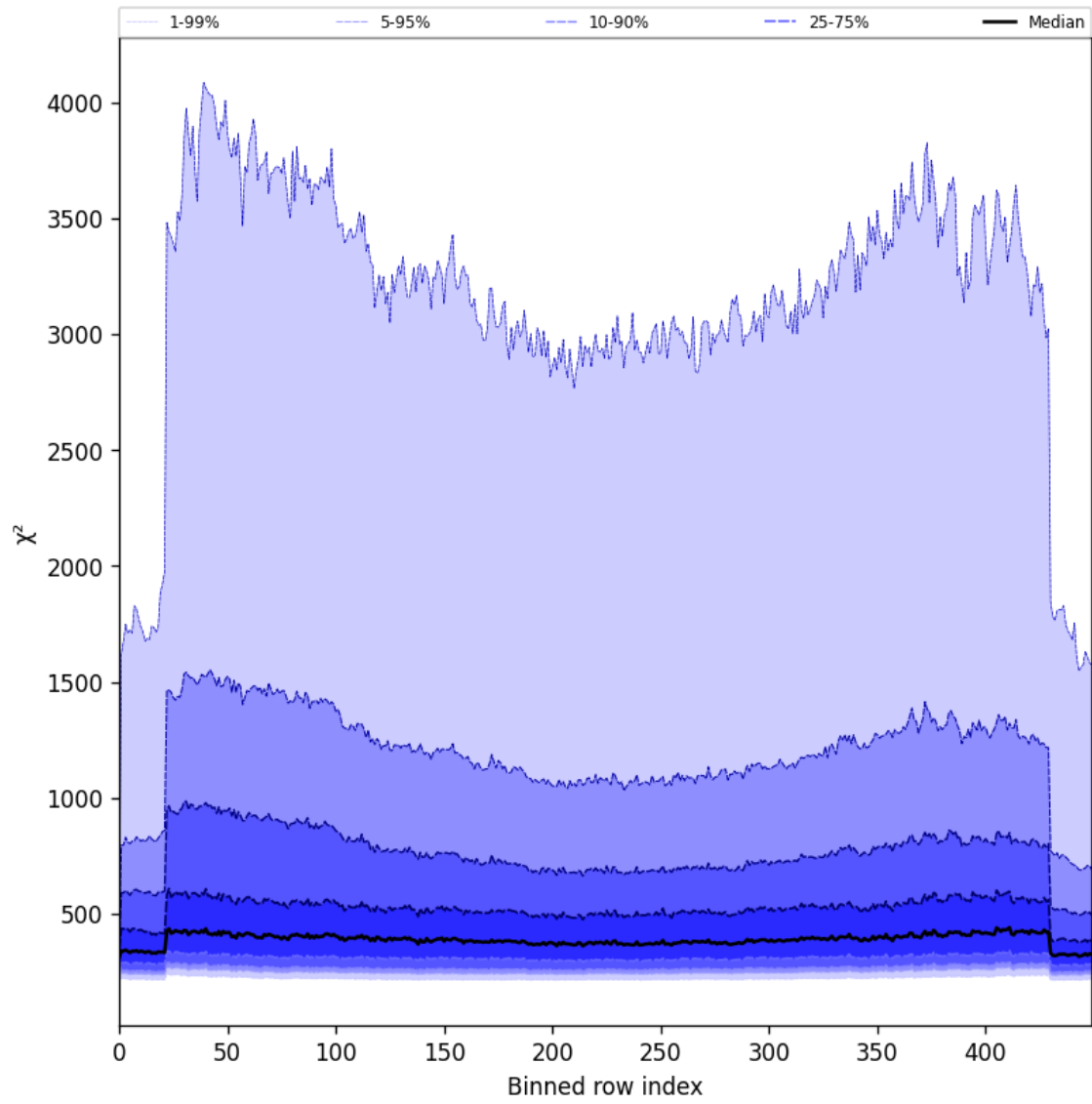
Figure 57: Along track statistics of “ \chi^2 ” for 2025-06-11 to 2025-06-12
