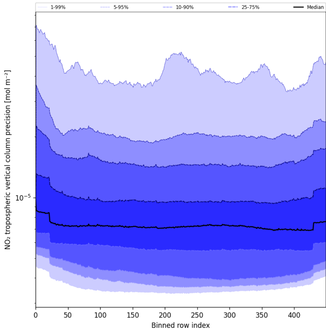
Figure 45: Along track statistics of “NO 2 tropospheric vertical column precision” for 2025-06-11 to 2025-06-12
