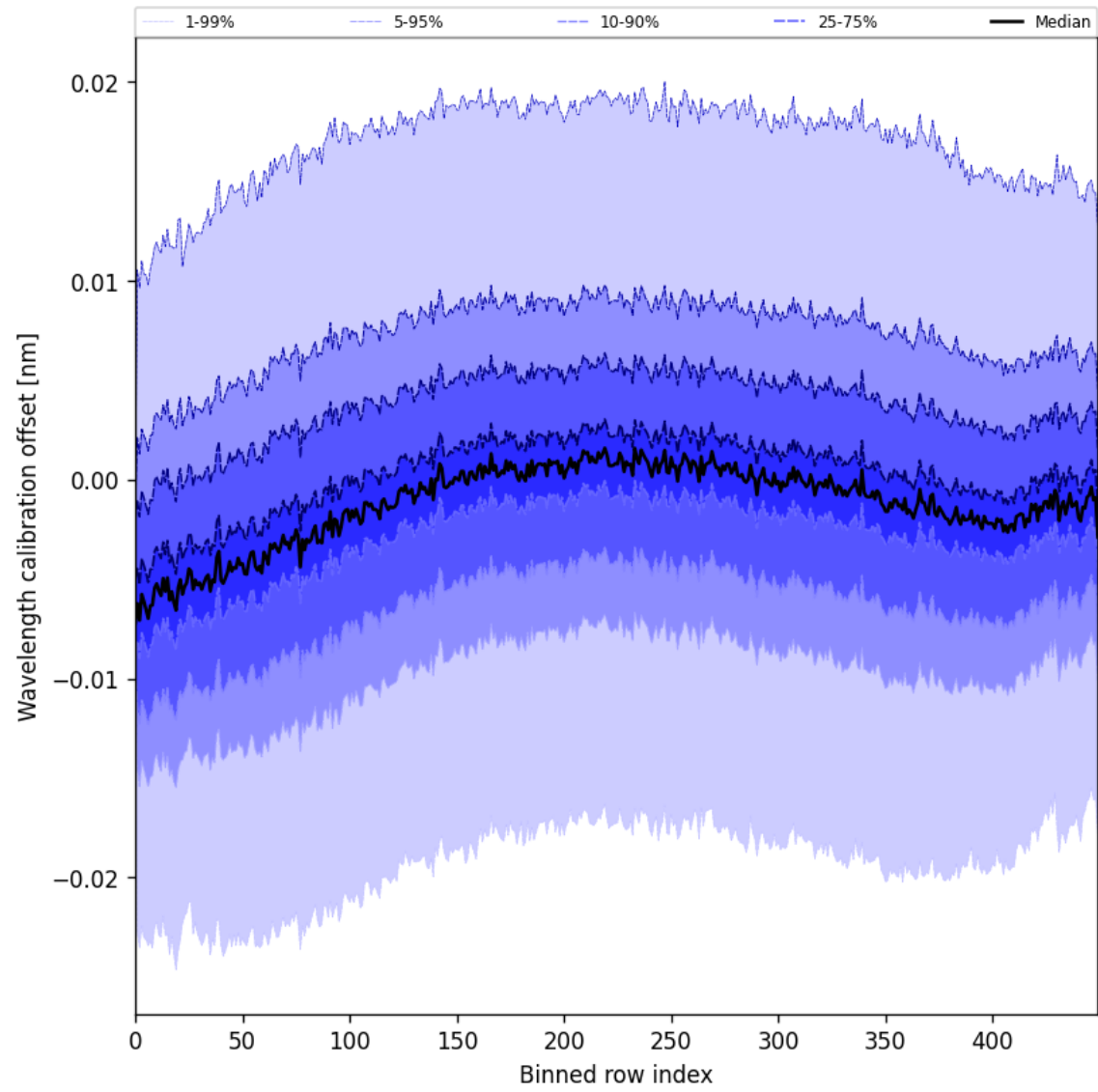
Figure 50: Along track statistics of “Wavelength calibration offset” for 2025-06-11 to 2025-06-12
