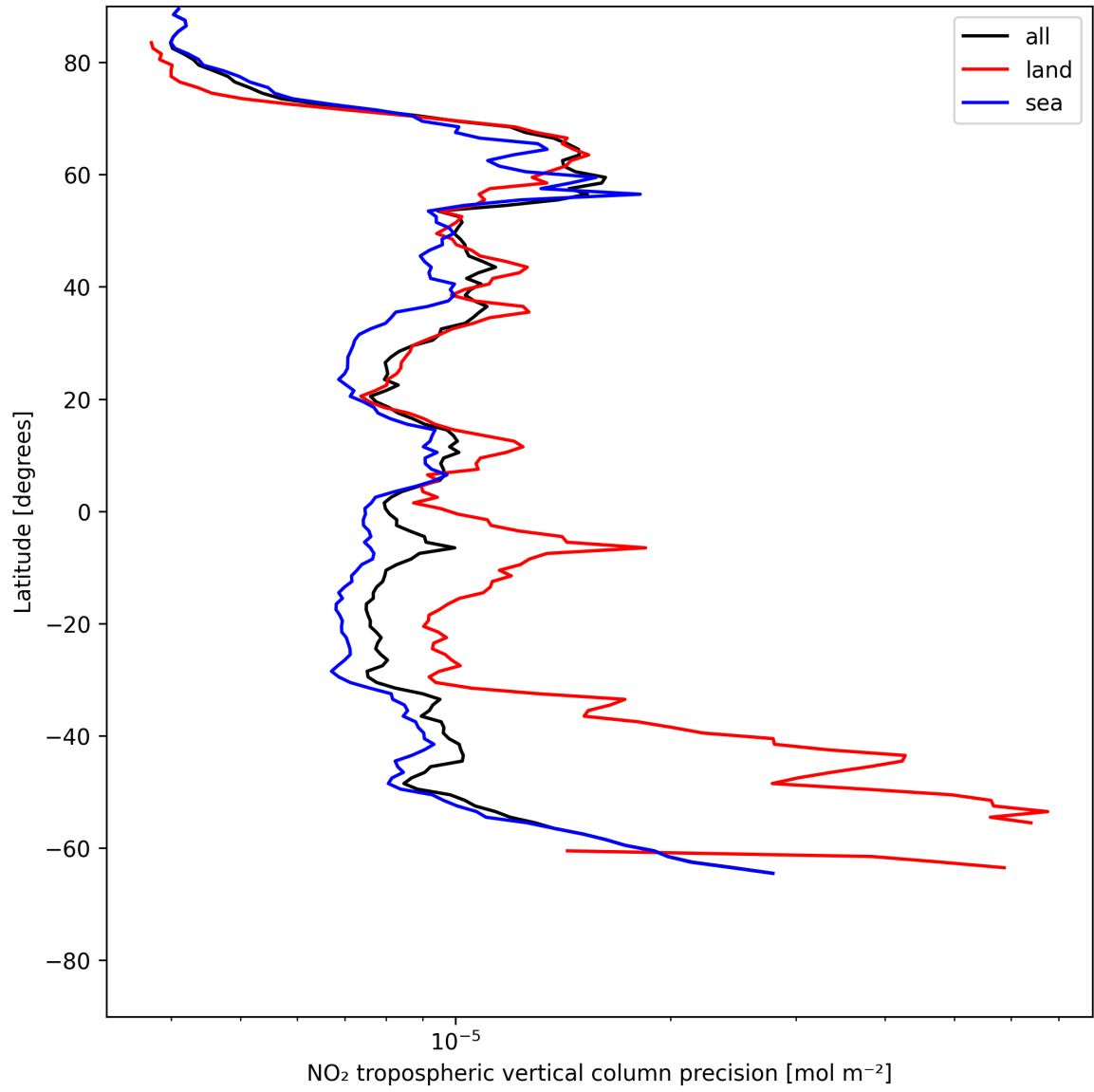
Figure 11: Zonal average of “NO 2 tropospheric vertical column precision” for 2025-06-11 to 2025-06-12.
