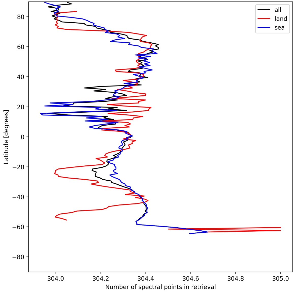
Figure 14: Zonal average of “Number of spectral points in retrieval” for 2025-06-11 to 2025-06-12.
