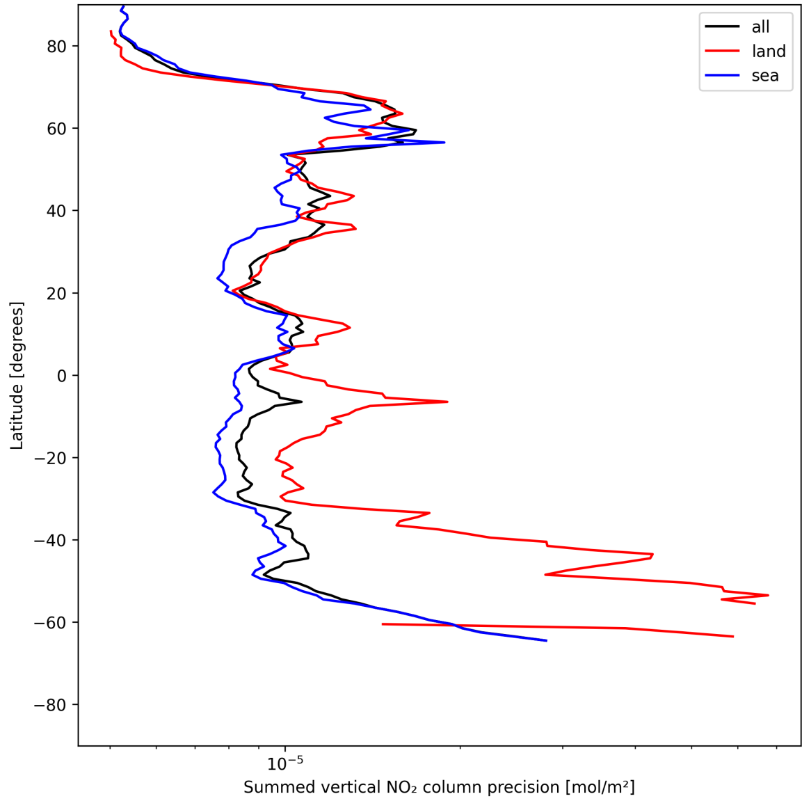
Figure 22: Zonal average of “Summed vertical NO 2 column precision” for 2025-06-11 to 2025-06-12.
