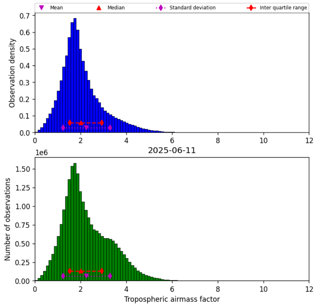
Figure 29: Histogram of “Tropospheric airmass factor” for 2025-06-11 to 2025-06-12
