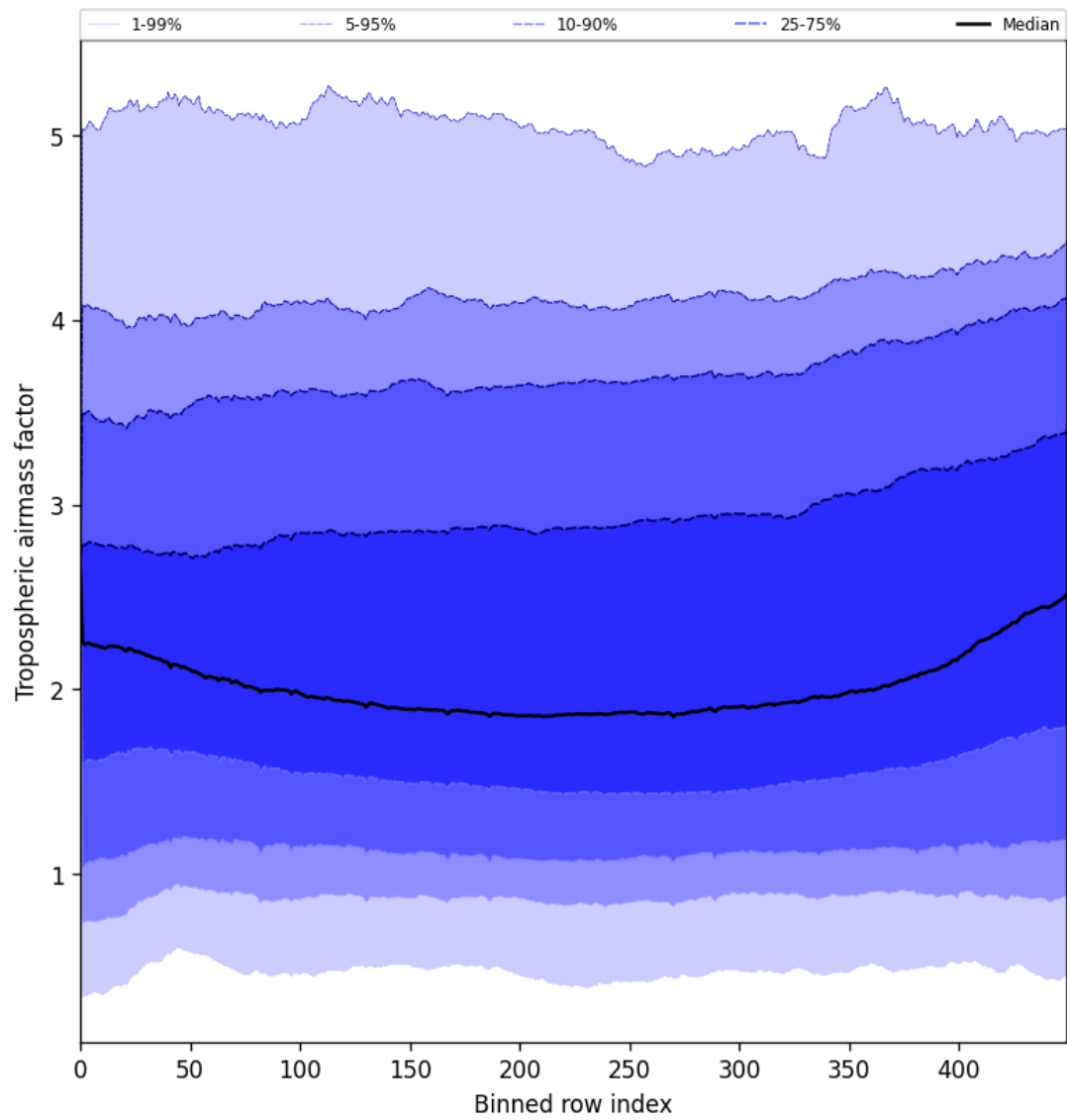
Figure 46: Along track statistics of “Tropospheric airmass factor” for 2025-06-11 to 2025-06-12
