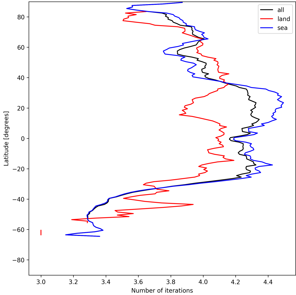
Figure 15: Zonal average of “Number of iterations” for 2025-06-11 to 2025-06-12.
