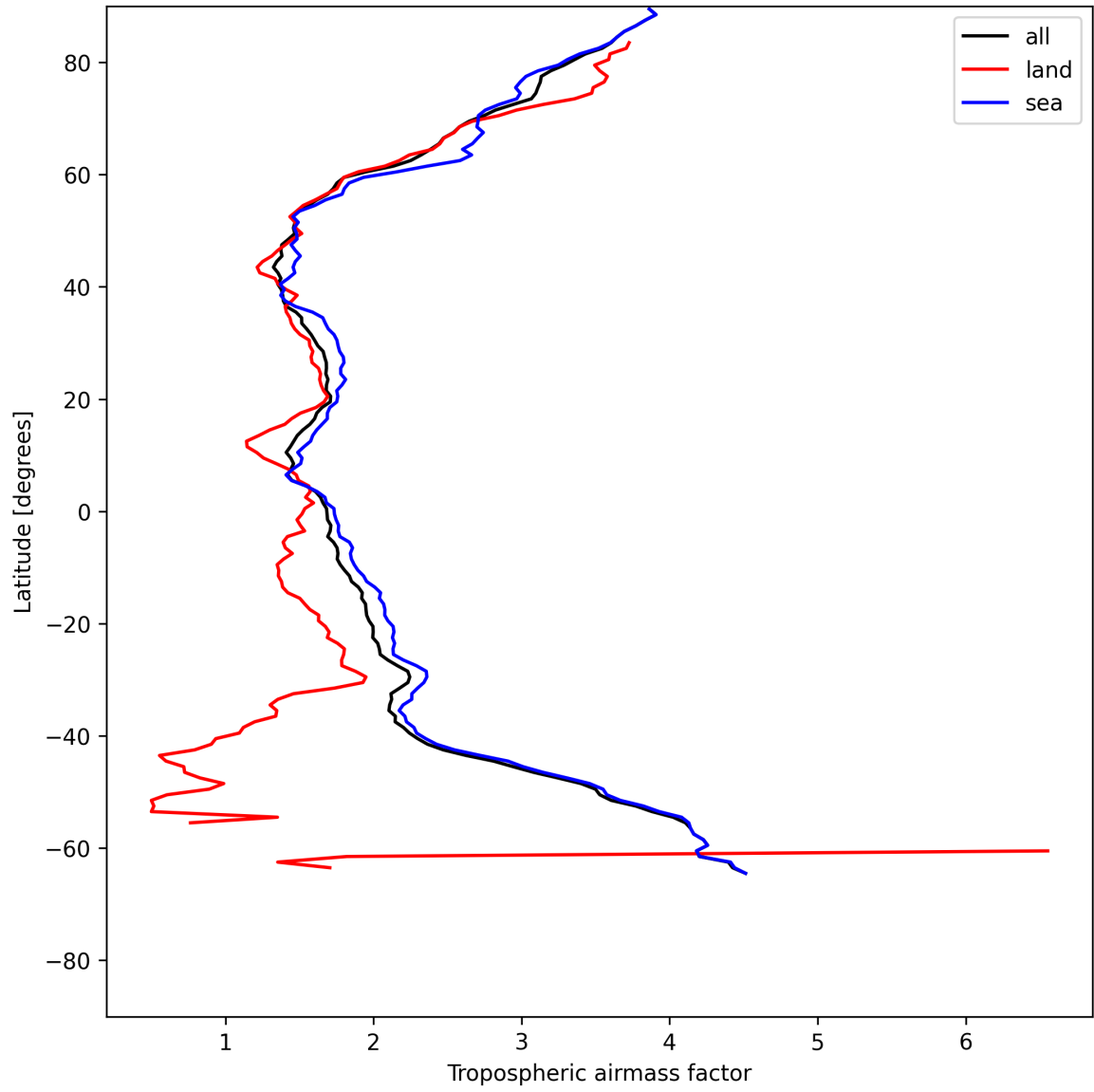
Figure 12: Zonal average of “Tropospheric airmass factor” for 2025-06-11 to 2025-06-12.
