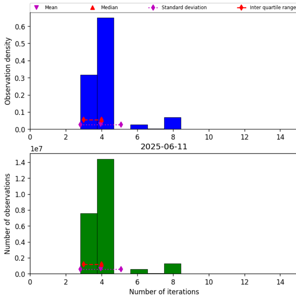
Figure 32: Histogram of “Number of iterations” for 2025-06-11 to 2025-06-12
