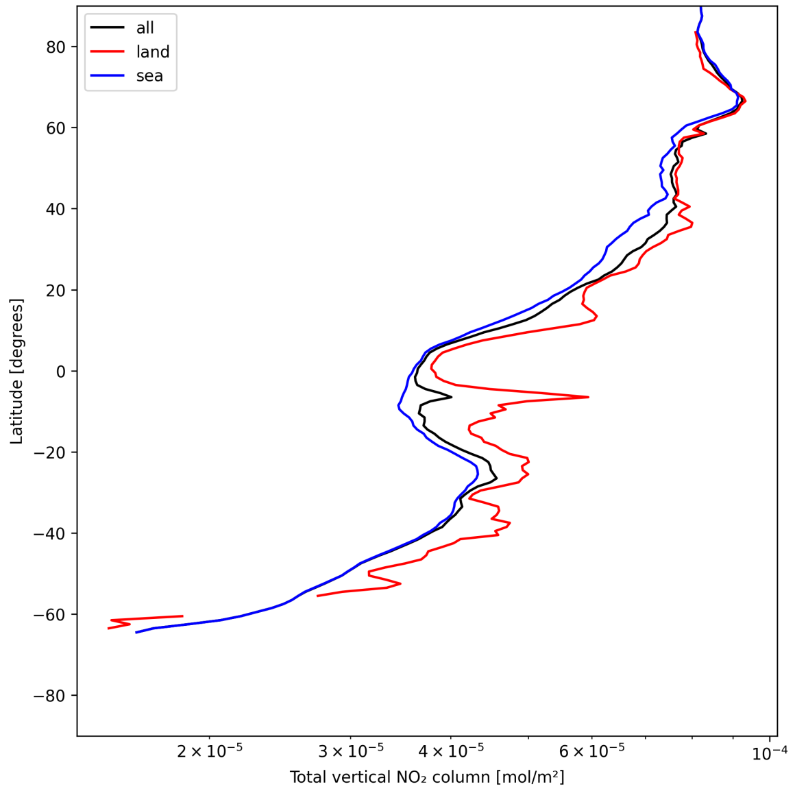
Figure 19: Zonal average of “Total vertical NO 2 column” for 2025-06-11 to 2025-06-12.
