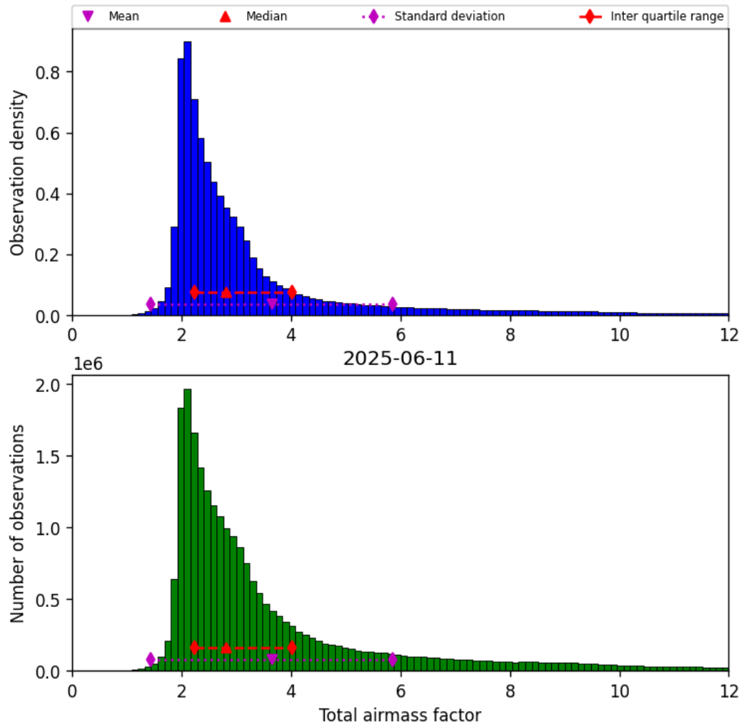
Figure 30: Histogram of “Total airmass factor” for 2025-06-11 to 2025-06-12
