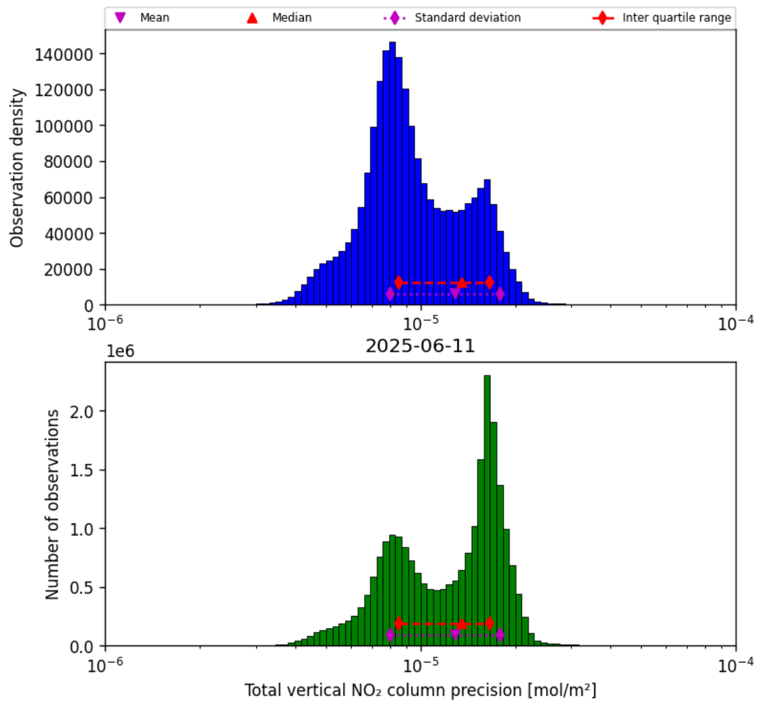
Figure 37: Histogram of “Total vertical NO 2 column precision” for 2025-06-11 to 2025-06-12
