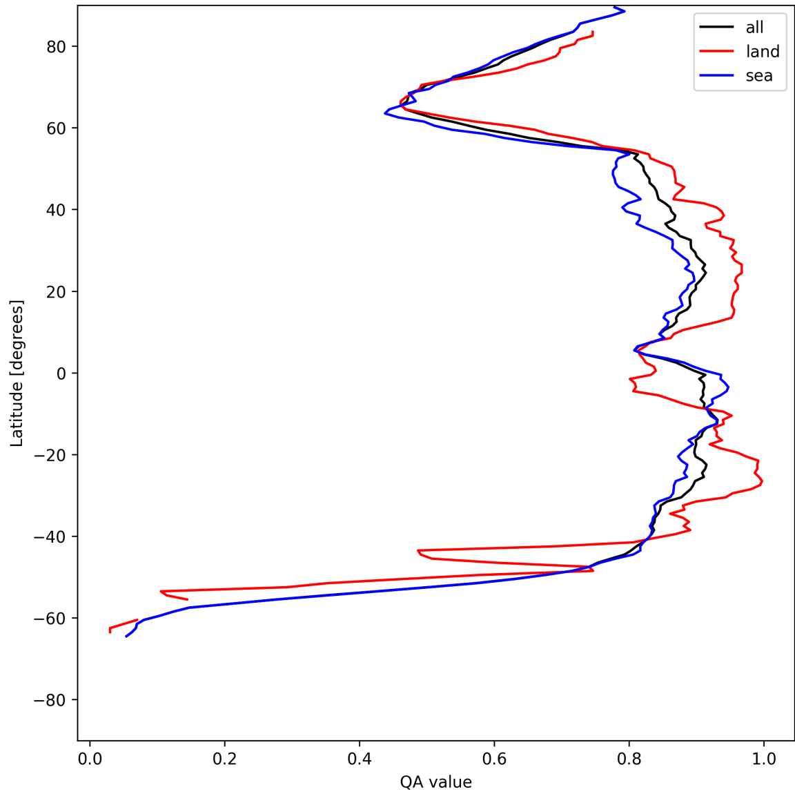
Figure 9: Zonal average of “QA value” for 2025-06-11 to 2025-06-12.
