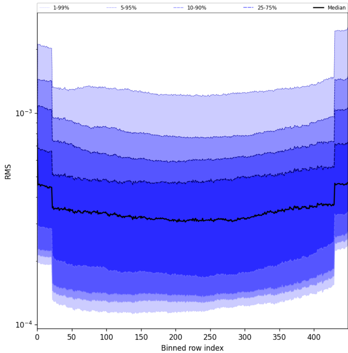
Figure 58: Along track statistics of “RMS” for 2025-06-11 to 2025-06-12
