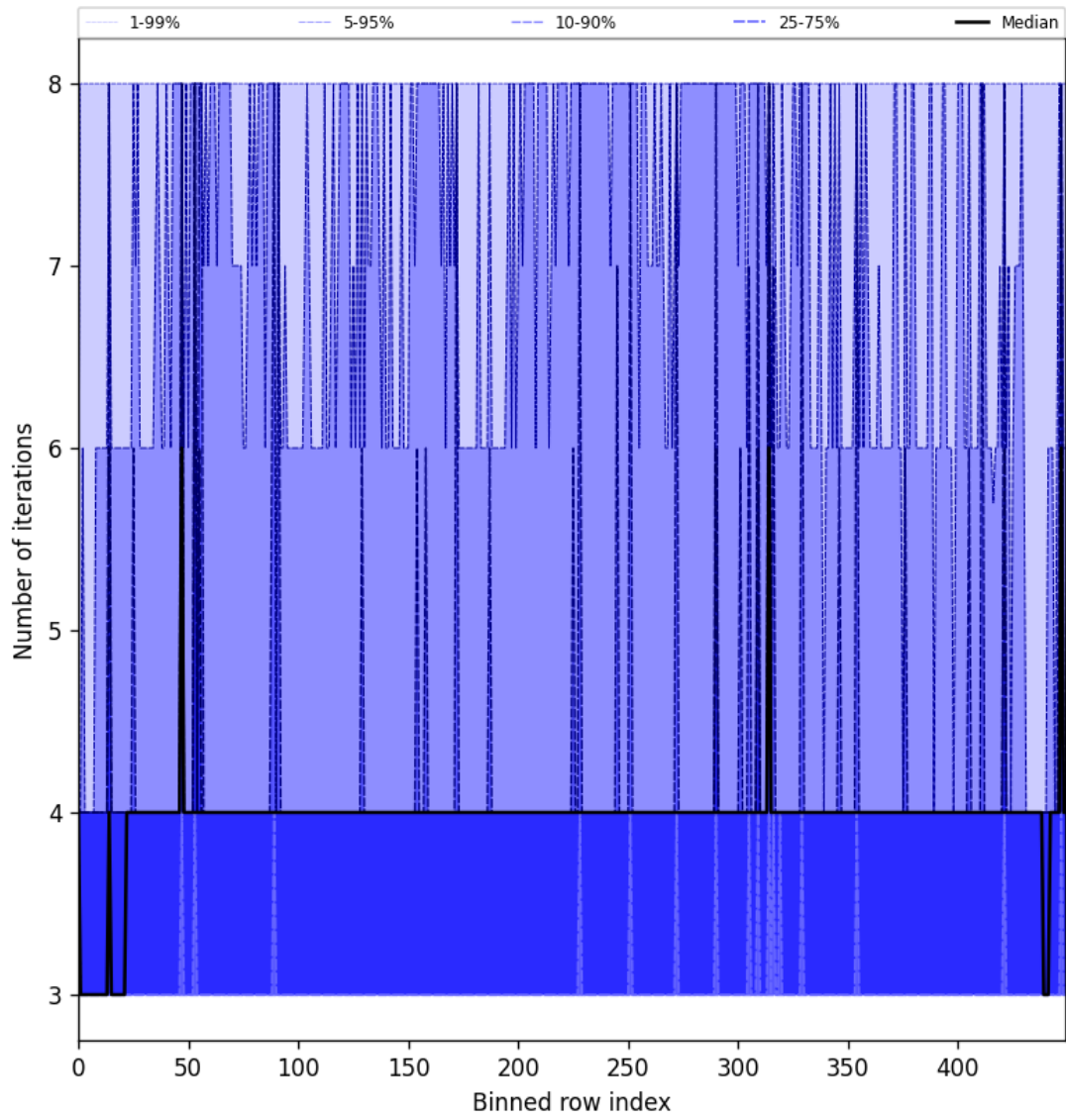
Figure 49: Along track statistics of “Number of iterations” for 2025-06-11 to 2025-06-12
