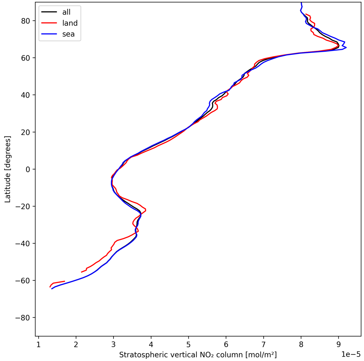
Figure 17: Zonal average of “Stratospheric vertical NO 2 column” for 2025-06-11 to 2025-06-12.
