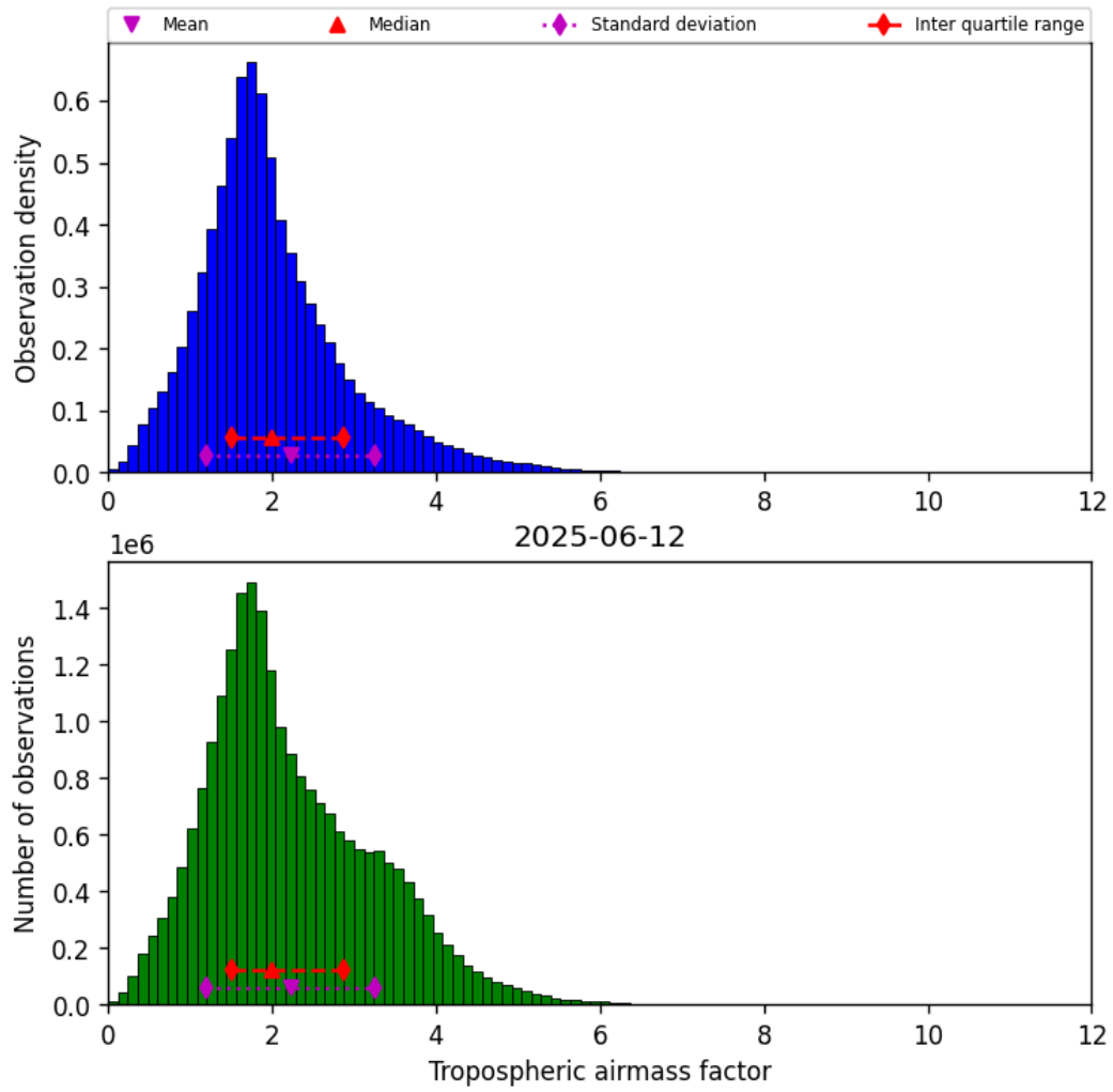
Figure 29: Histogram of “Tropospheric airmass factor” for 2025-06-12 to 2025-06-13
