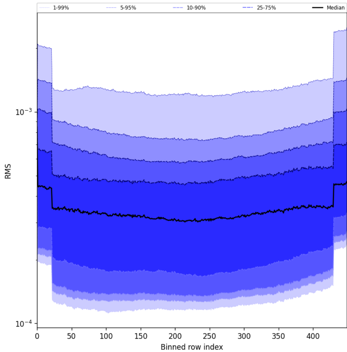
Figure 58: Along track statistics of “RMS” for 2025-06-12 to 2025-06-13
