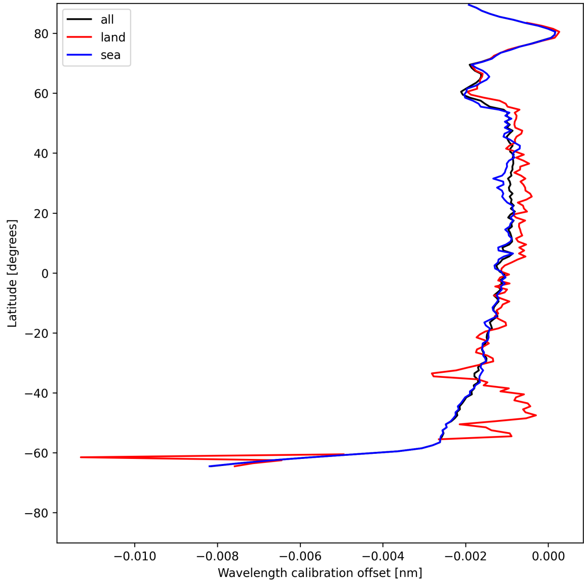
Figure 16: Zonal average of “Wavelength calibration offset” for 2025-06-12 to 2025-06-13.
