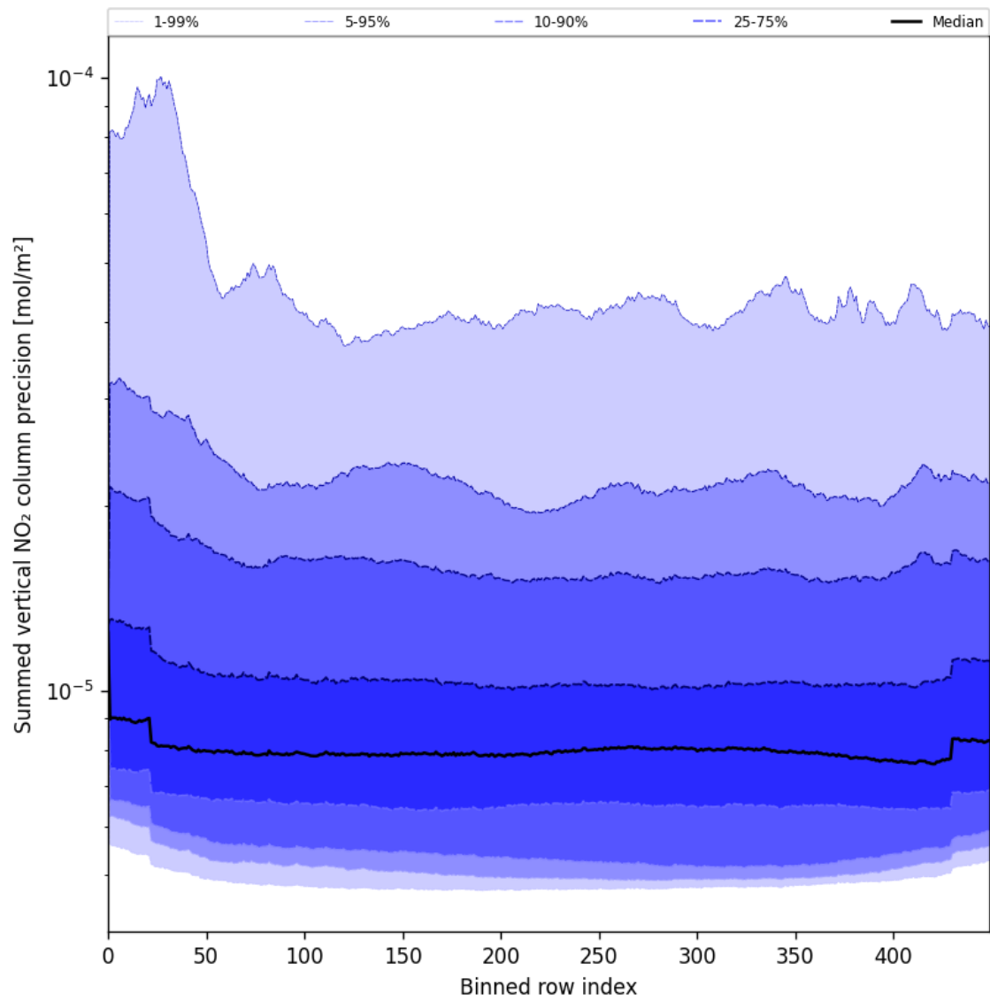
Figure 56: Along track statistics of “Summed vertical NO 2 column precision” for 2025-06-12 to 2025-06-13
