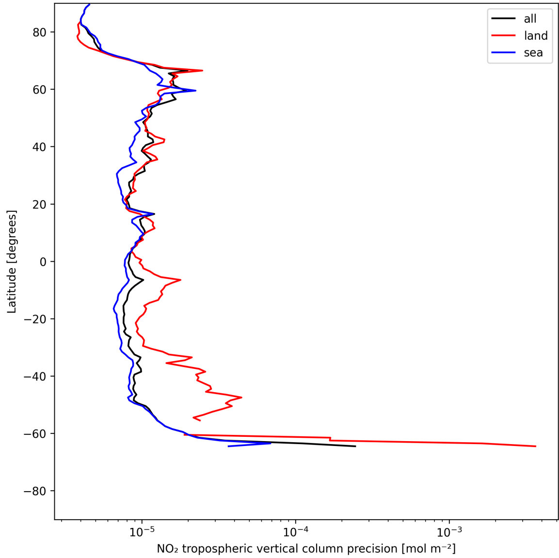
Figure 11: Zonal average of “NO 2 tropospheric vertical column precision” for 2025-06-12 to 2025-06-13.
