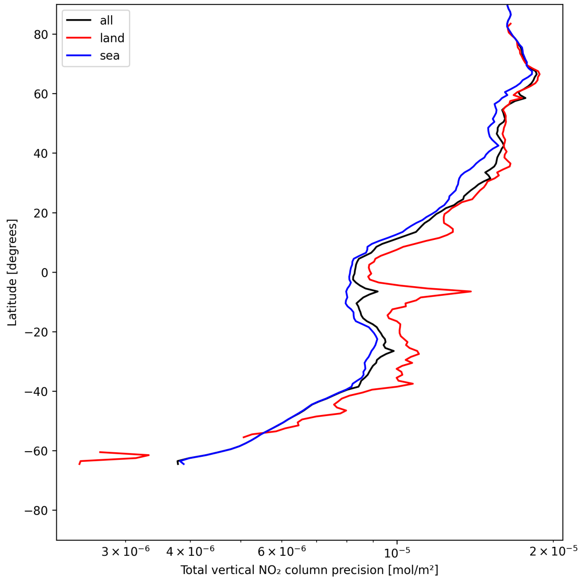
Figure 20: Zonal average of “Total vertical NO 2 column precision” for 2025-06-12 to 2025-06-13.
