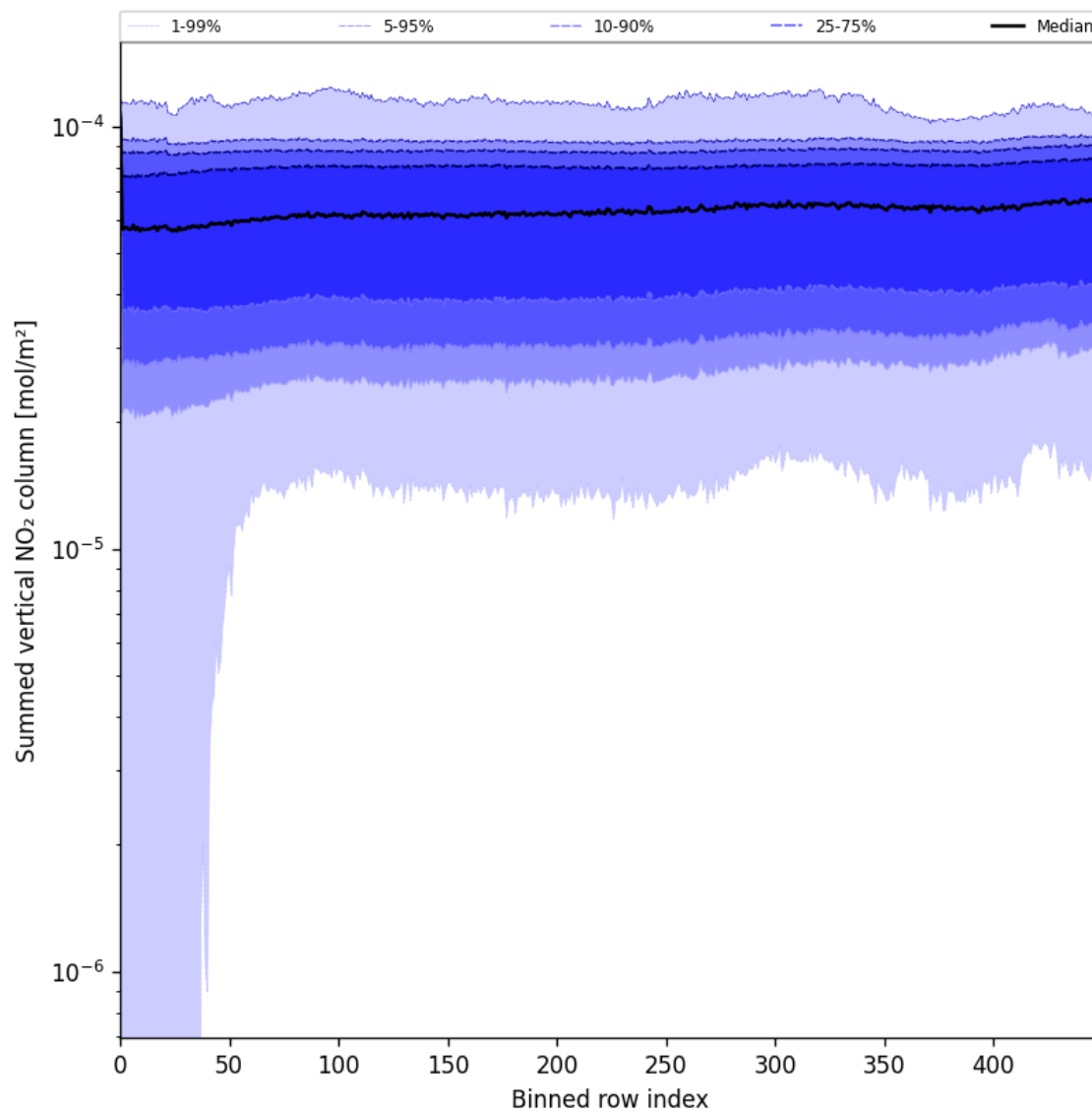
Figure 55: Along track statistics of “Summed vertical NO 2 column” for 2025-06-12 to 2025-06-13
