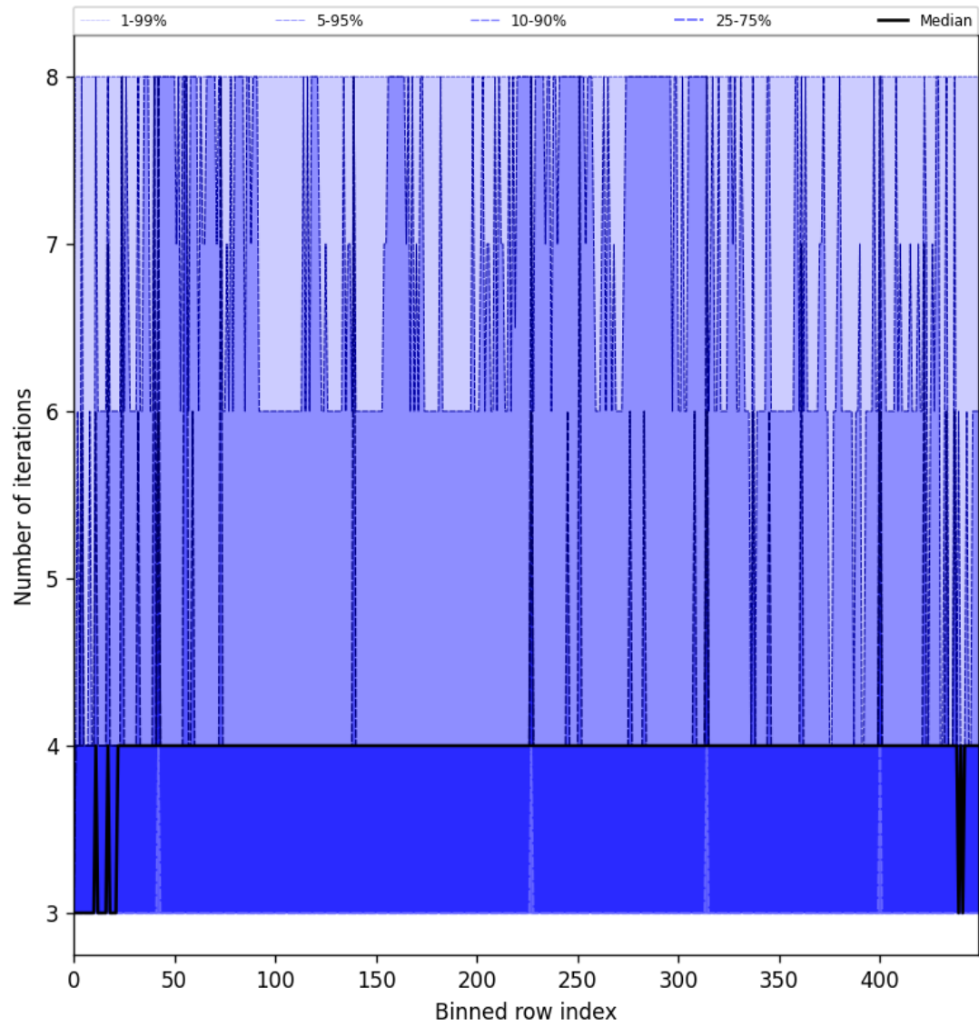
Figure 49: Along track statistics of “Number of iterations” for 2025-06-12 to 2025-06-13
