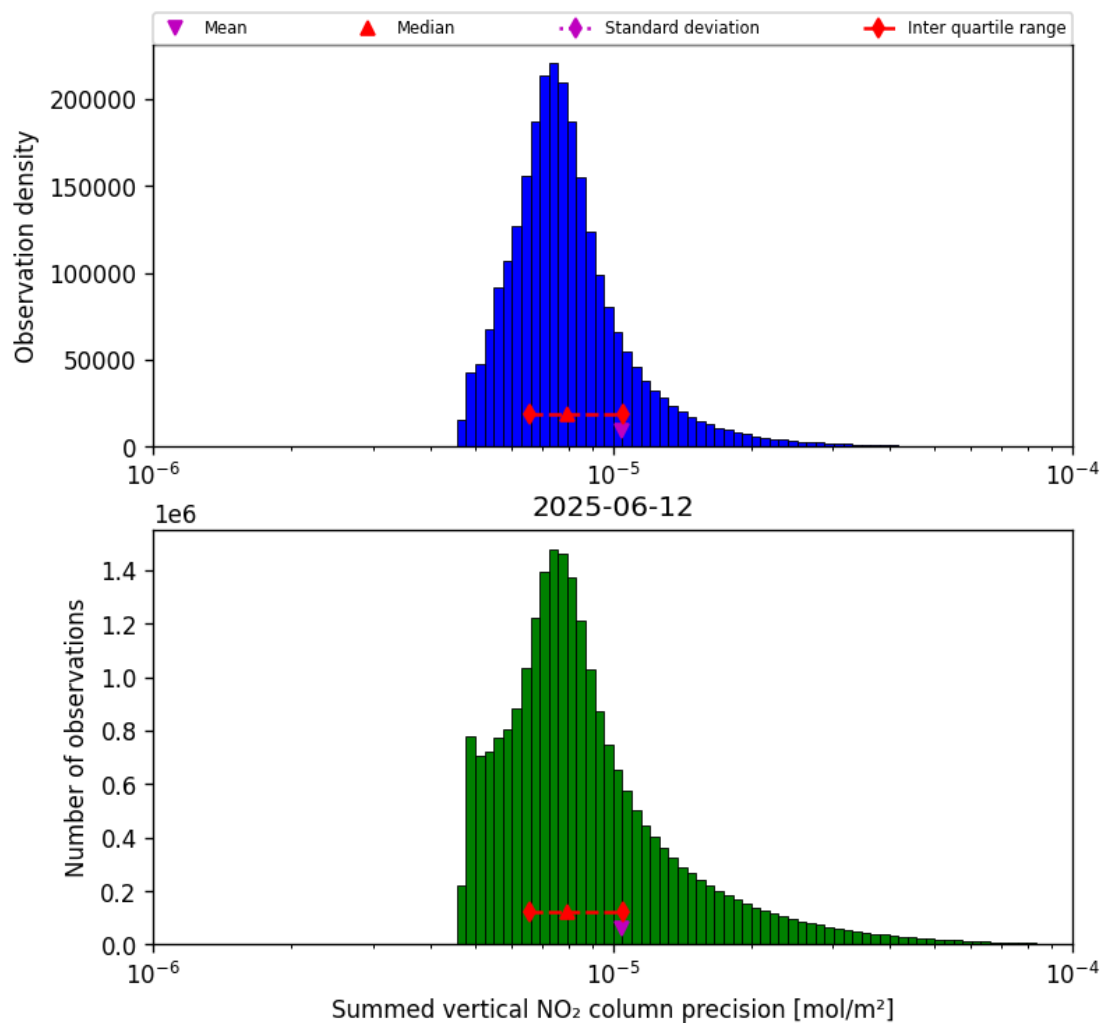
Figure 39: Histogram of "Summed vertical NO 2 column precision" for 2025-06-12 to 2025-06-13
