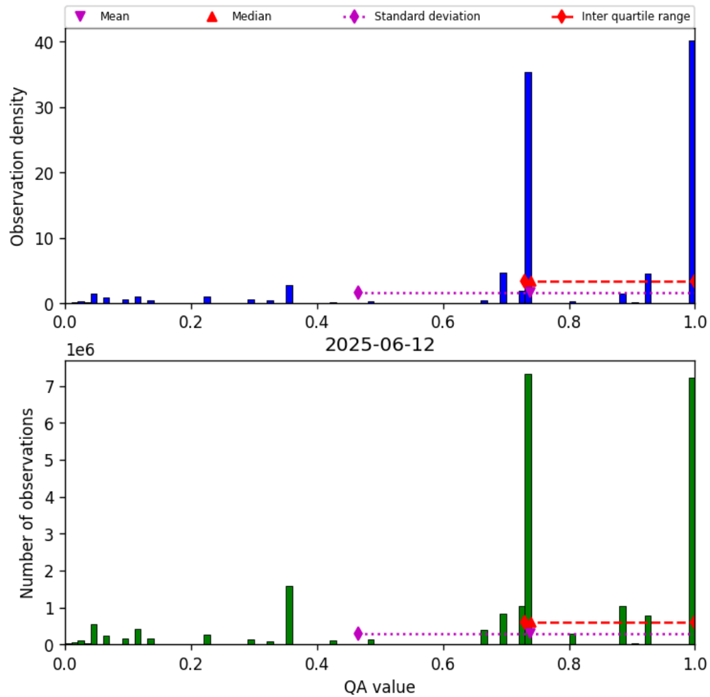
Figure 26: Histogram of “QA value” for 2025-06-12 to 2025-06-13
