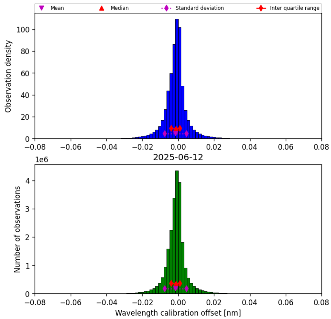
Figure 33: Histogram of “Wavelength calibration offset” for 2025-06-12 to 2025-06-13
