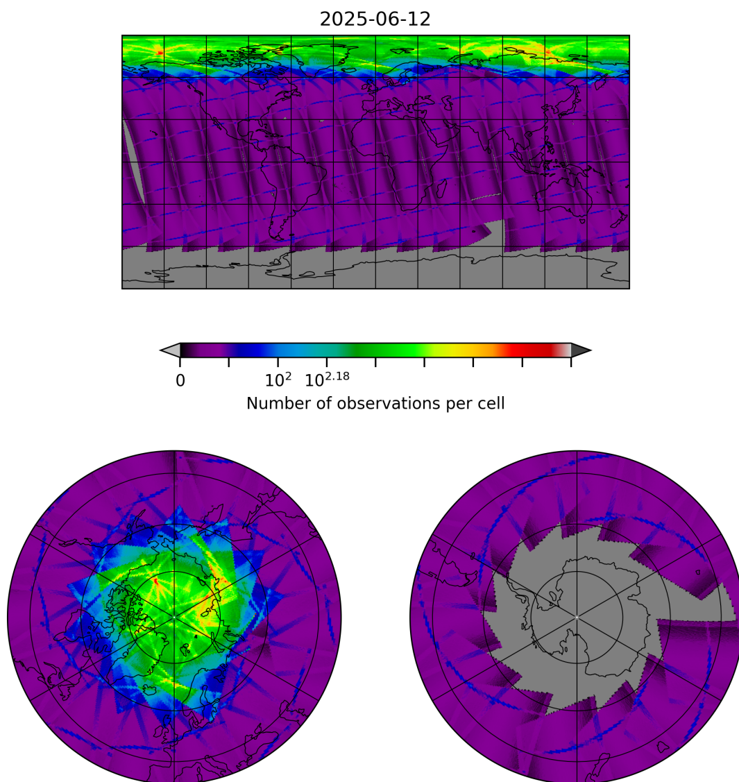
Figure 8: Map of the number of observations for 2025-06-12 to 2025-06-13
