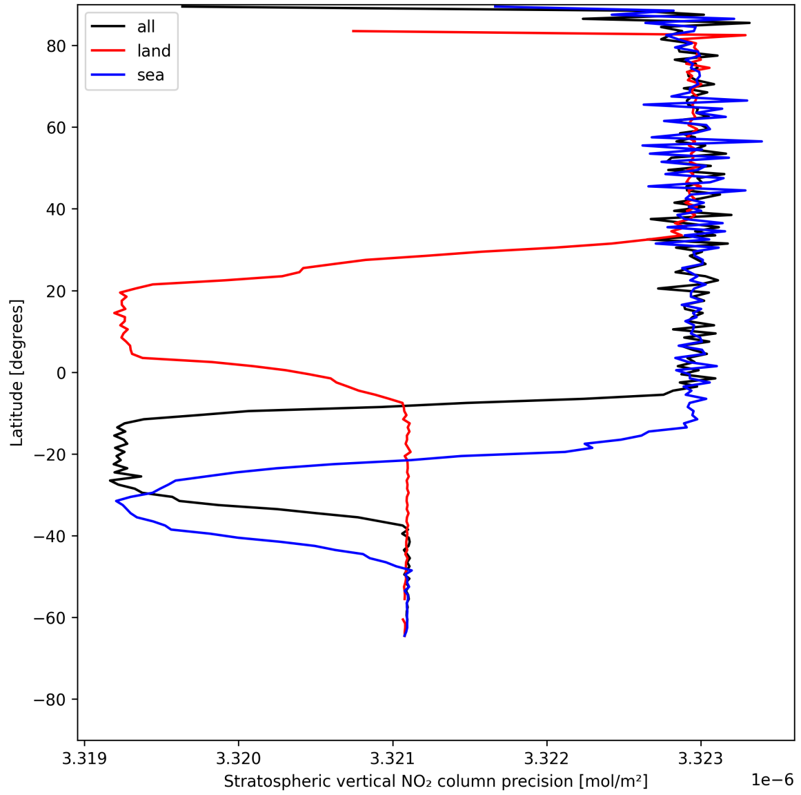
Figure 18: Zonal average of “Stratospheric vertical NO 2 column precision” for 2025-06-12 to 2025-06-13.
