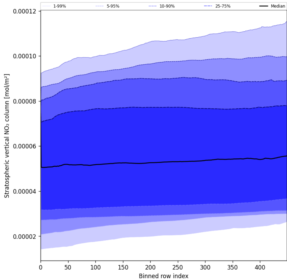
Figure 51: Along track statistics of “Stratospheric vertical NO 2 column” for 2025-06-12 to 2025-06-13
