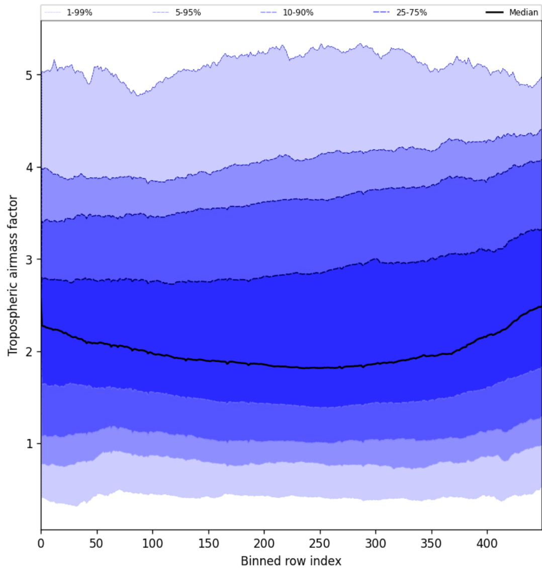
Figure 46: Along track statistics of “Tropospheric air mass factor” for 2025-06-12 to 2025-06-13
