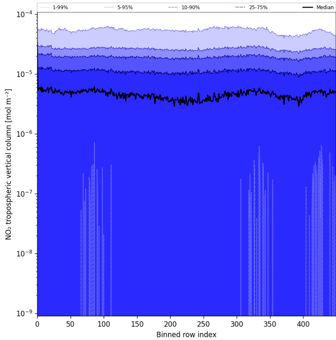
Figure 44: Along track statistics of "NO 2 tropospheric vertical column" for 2025-06-12 to 2025-06-13
