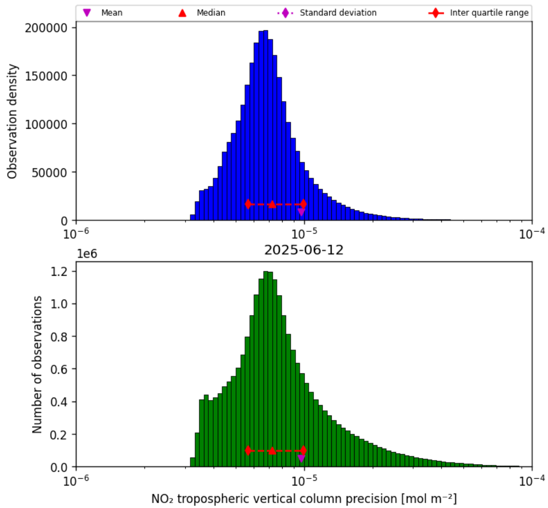
Figure 28: Histogram of “NO 2 tropospheric vertical column precision” for 2025-06-12 to 2025-06-13
