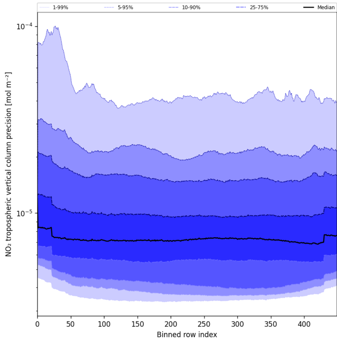
Figure 45: Along track statistics of “NO 2 tropospheric vertical column precision” for 2025-06-12 to 2025-06-13
