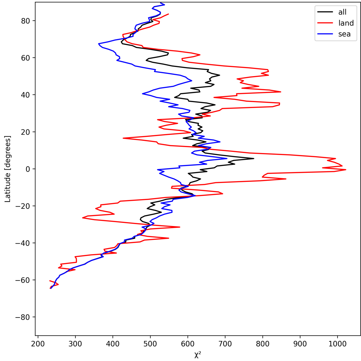
Figure 23: Zonal average of “ \chi^2 ” for 2025-06-12 to 2025-06-13.
