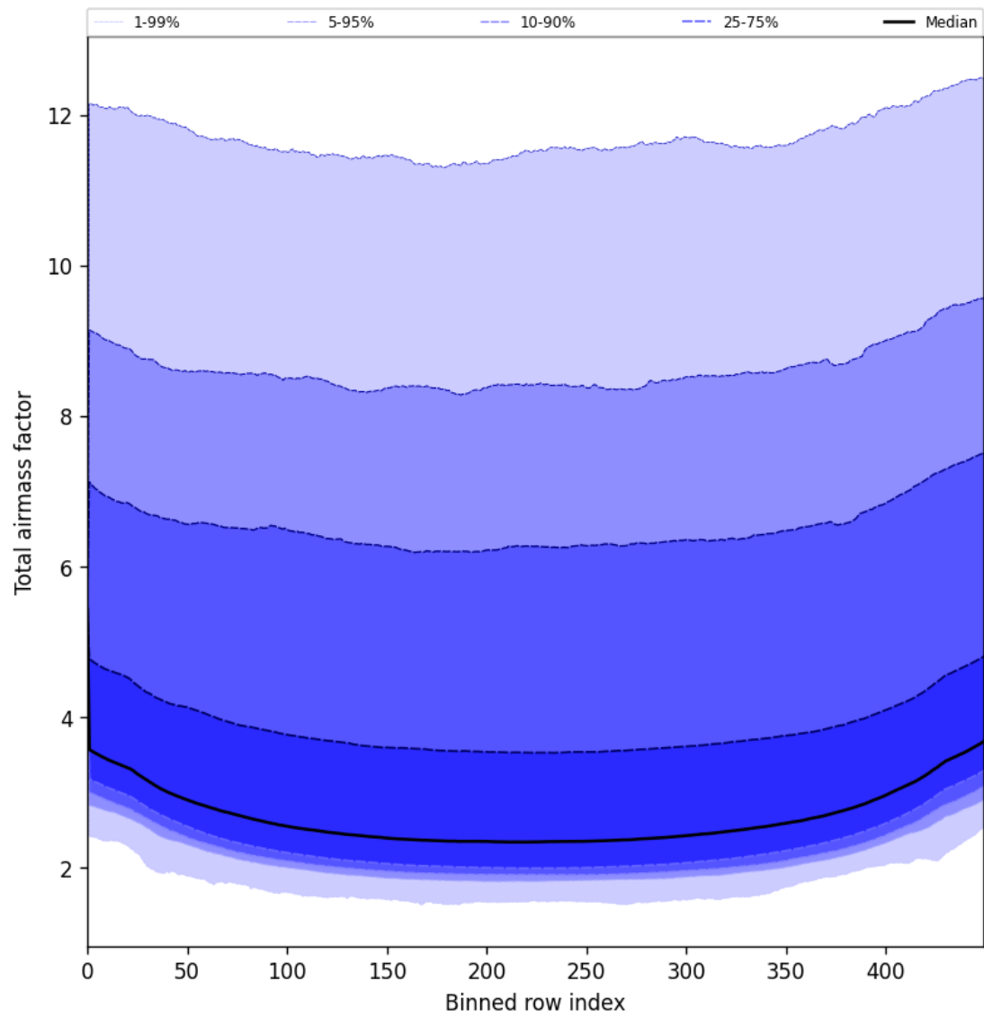
Figure 47: Along track statistics of “Total airmass factor” for 2025-06-12 to 2025-06-13
