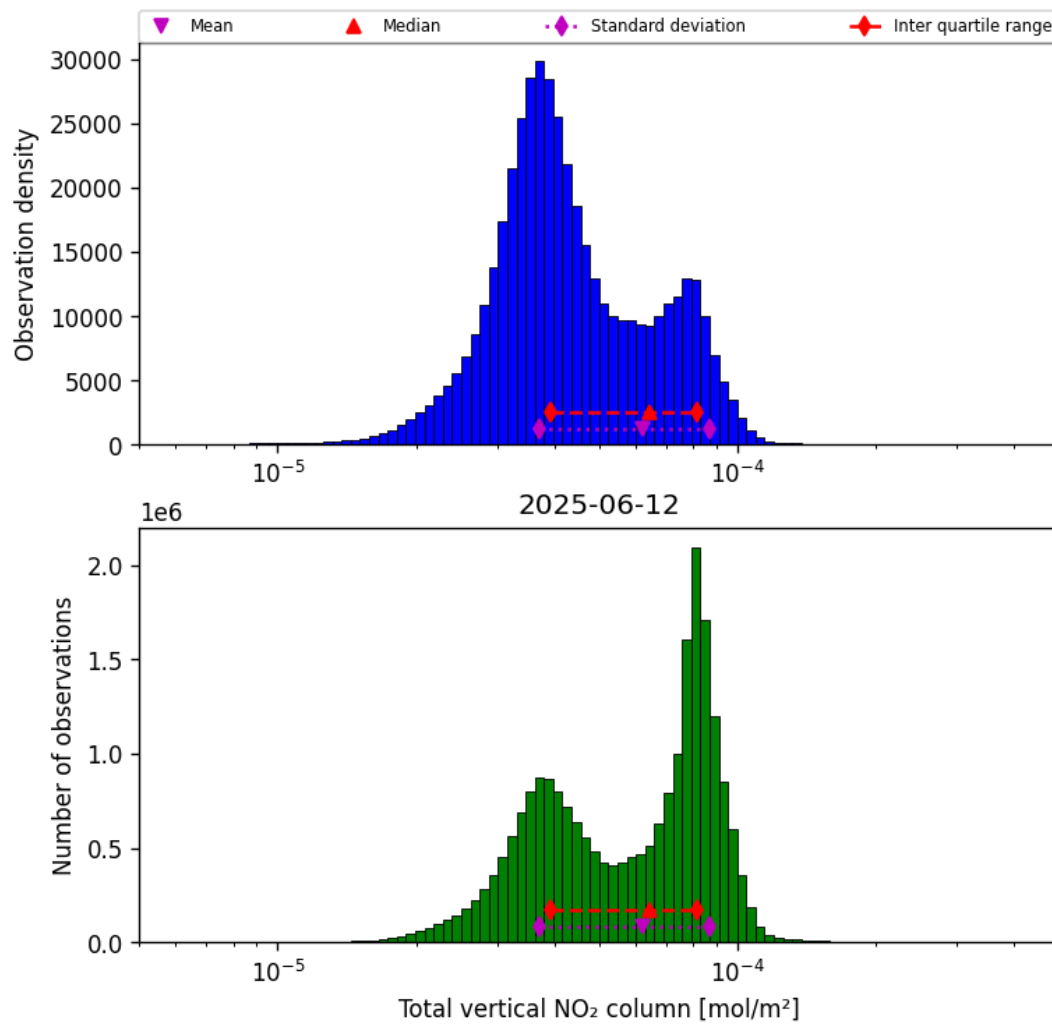
Figure 36: Histogram of “Total vertical NO 2 column” for 2025-06-12 to 2025-06-13
