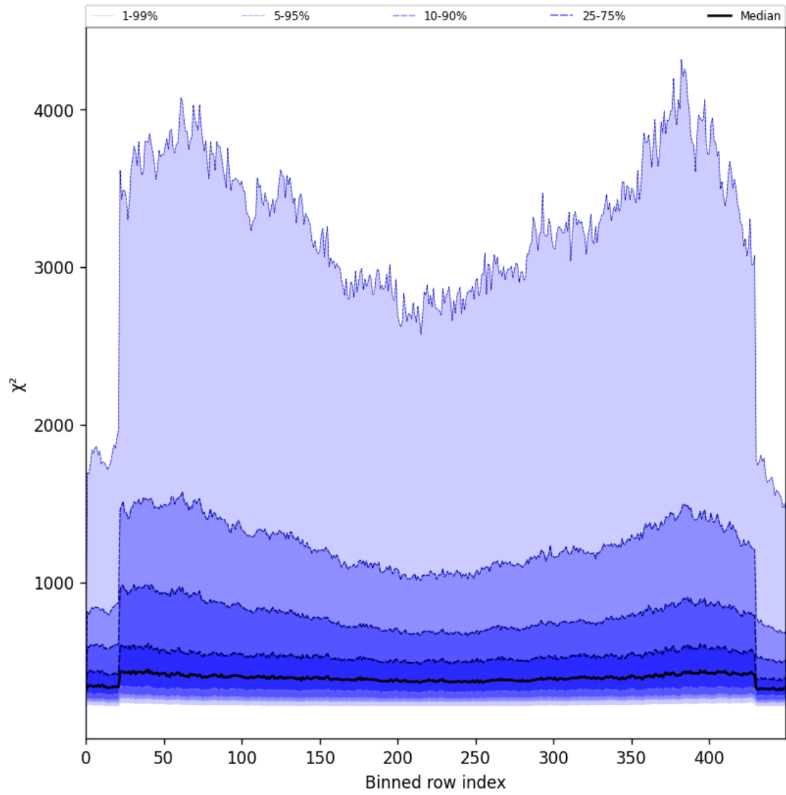
Figure 57: Along track statistics of “ \chi^2 ” for 2025-06-12 to 2025-06-13
