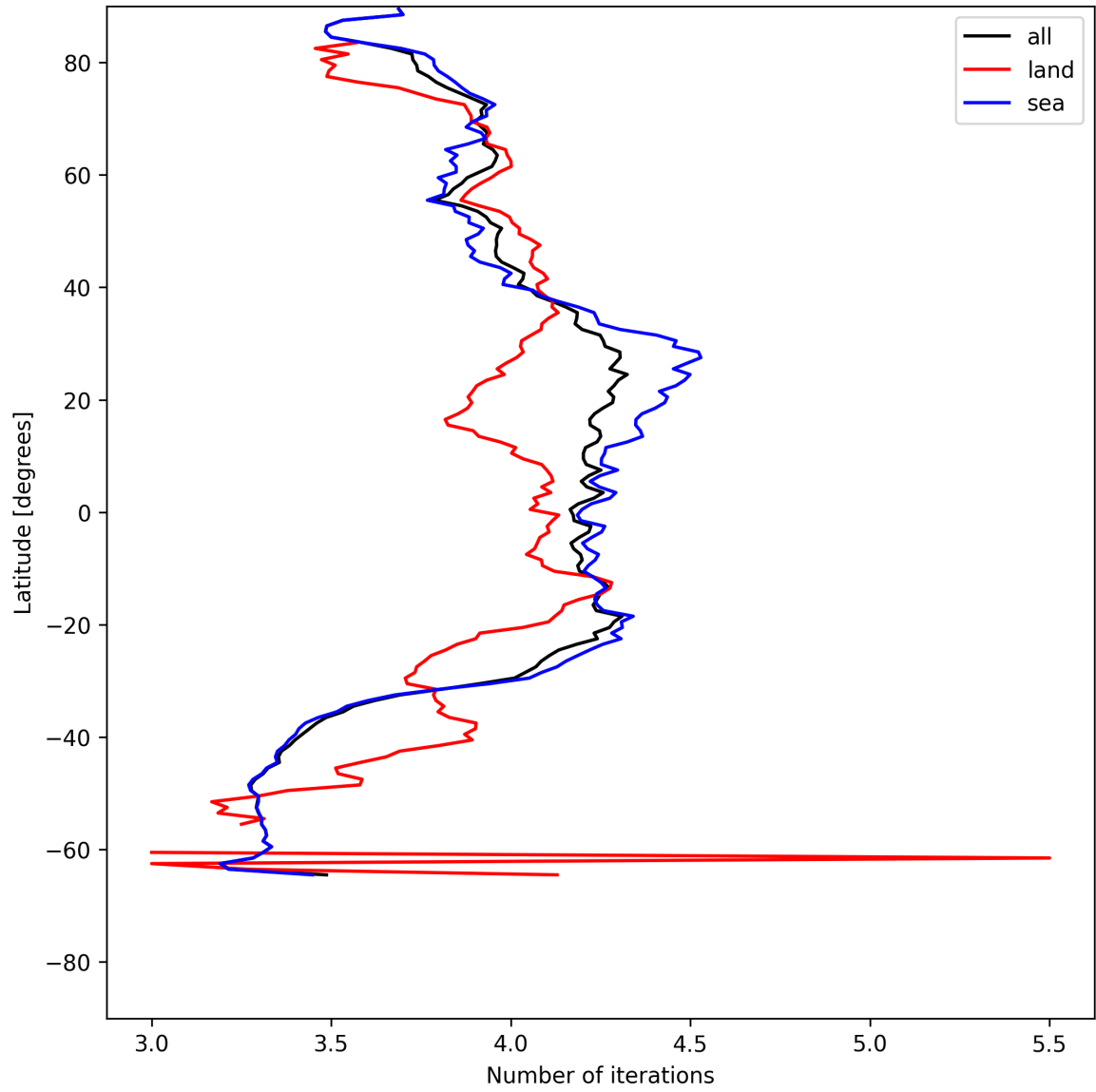
Figure 15: Zonal average of “Number of iterations” for 2025-06-12 to 2025-06-13.
