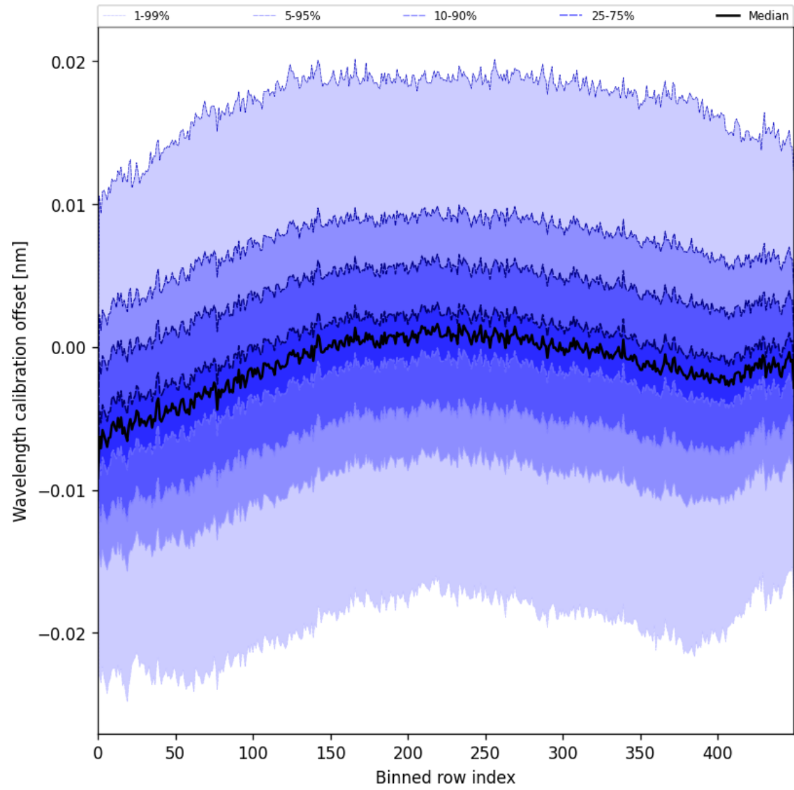
Figure 50: Along track statistics of “Wavelength calibration offset” for 2025-06-12 to 2025-06-13
