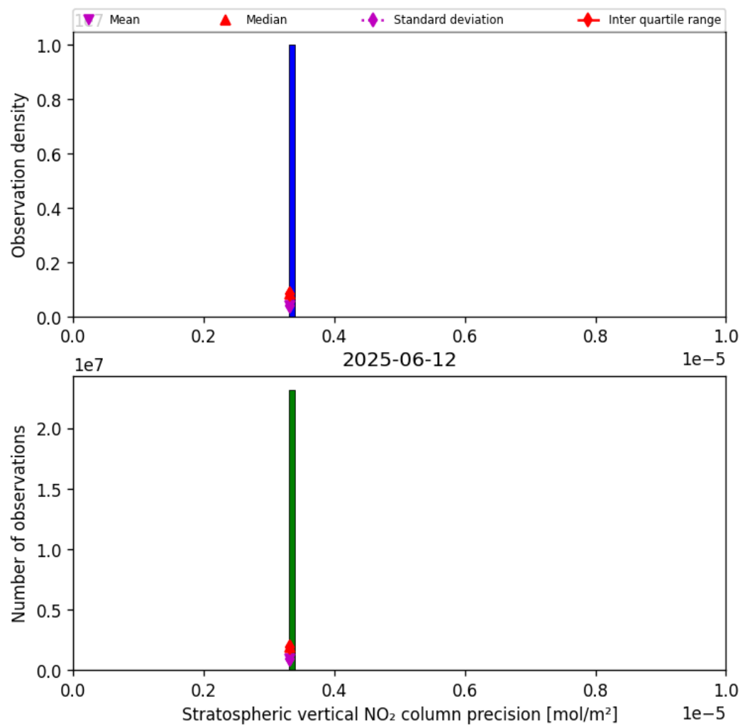
Figure 35: Histogram of “Stratospheric vertical NO 2 column precision” for 2025-06-12 to 2025-06-13
