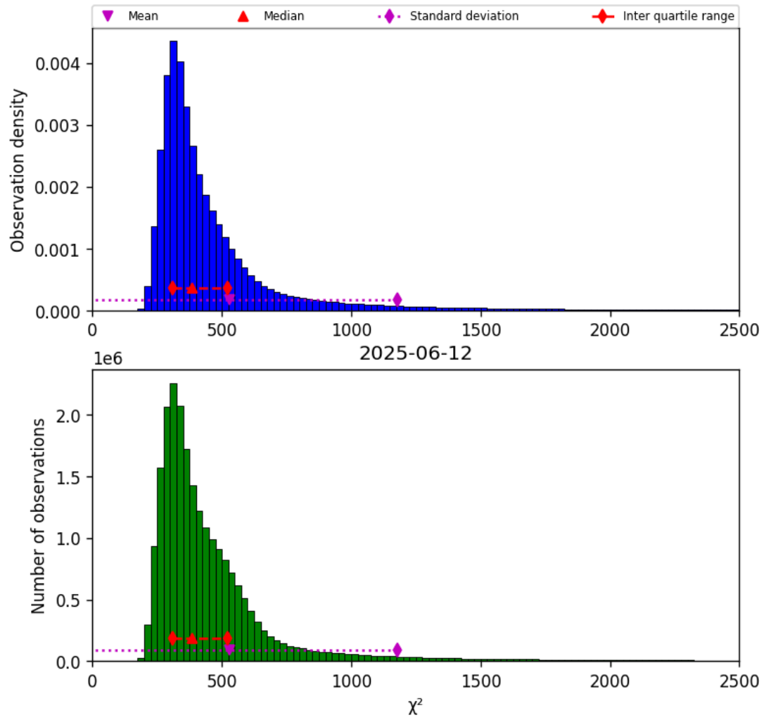
Figure 40: Histogram of “ \chi^2 ” for 2025-06-12 to 2025-06-13
