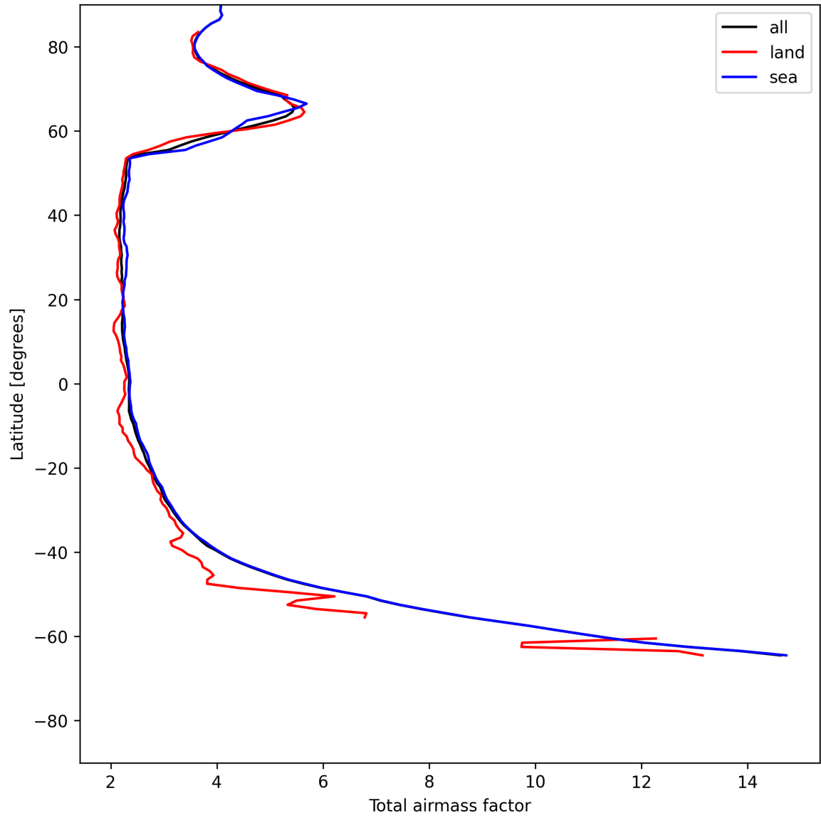
Figure 13: Zonal average of “Total airmass factor” for 2025-06-12 to 2025-06-13.
