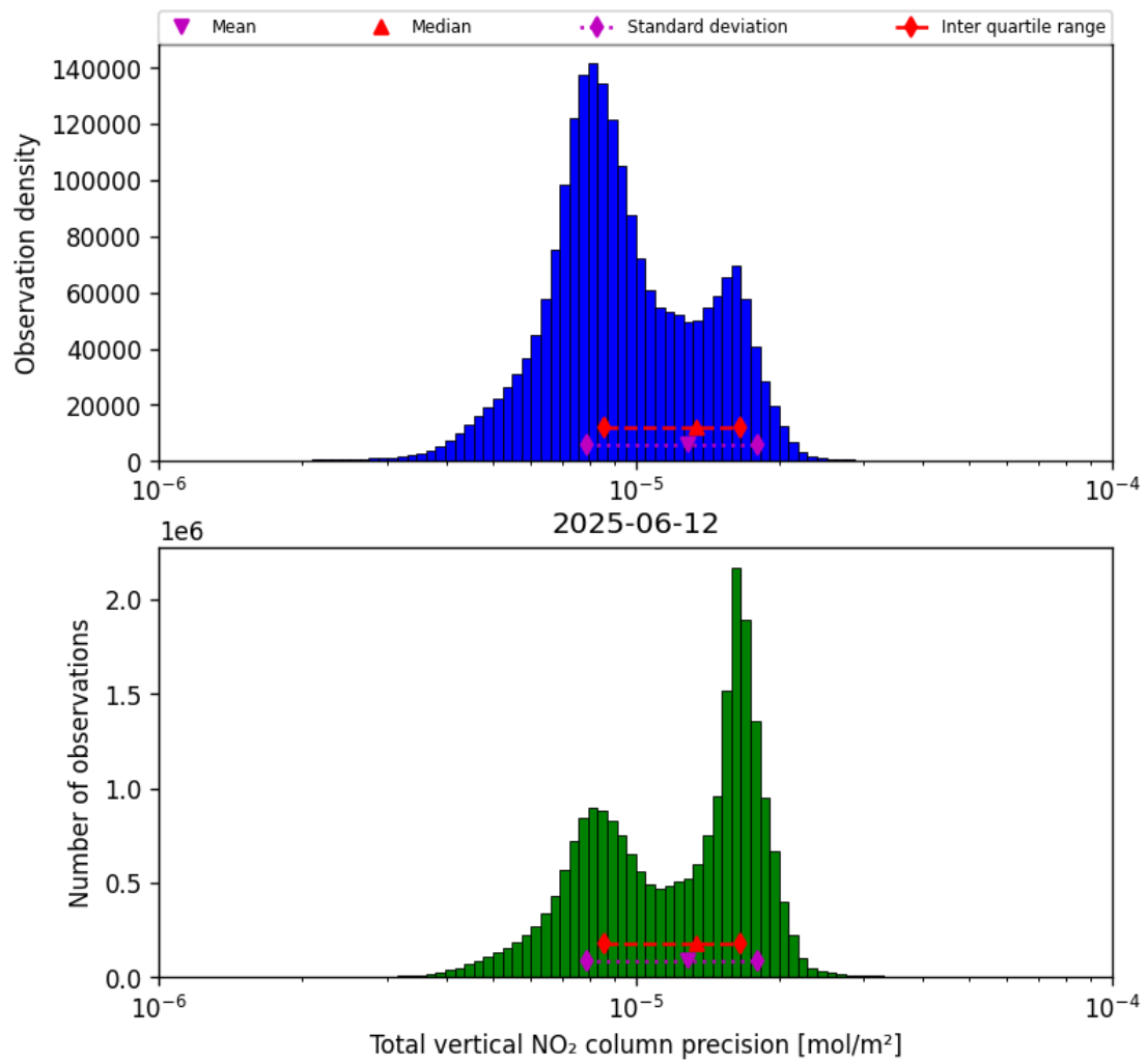
Figure 37: Histogram of “Total vertical NO 2 column precision” for 2025-06-12 to 2025-06-13
