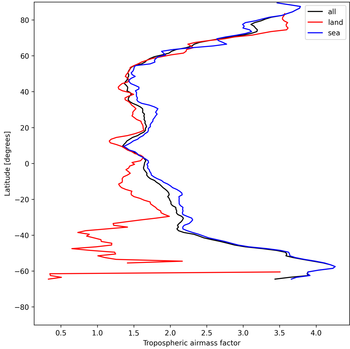
Figure 12: Zonal average of “Tropospheric airmass factor” for 2025-06-12 to 2025-06-13.
