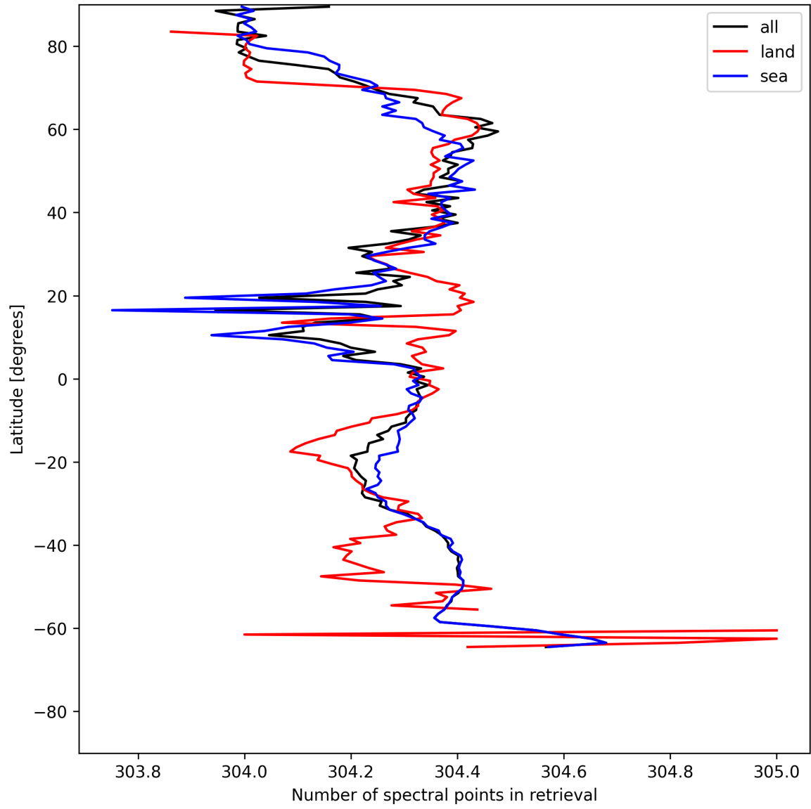
Figure 14: Zonal average of “Number of spectral points in retrieval” for 2025-06-12 to 2025-06-13.
