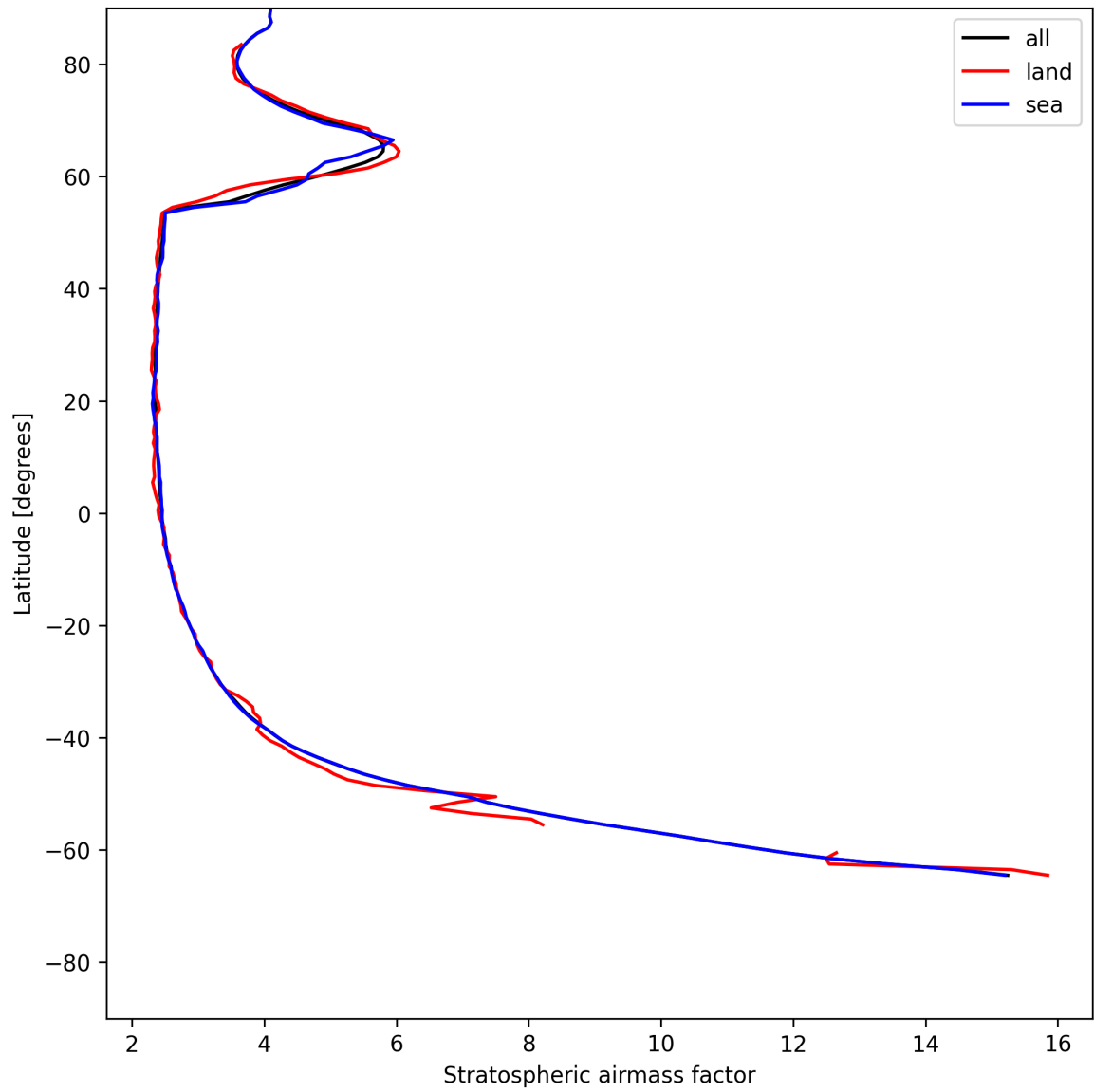
Figure 25: Zonal average of “Stratospheric air mass factor” for 2025-06-12 to 2025-06-13.
