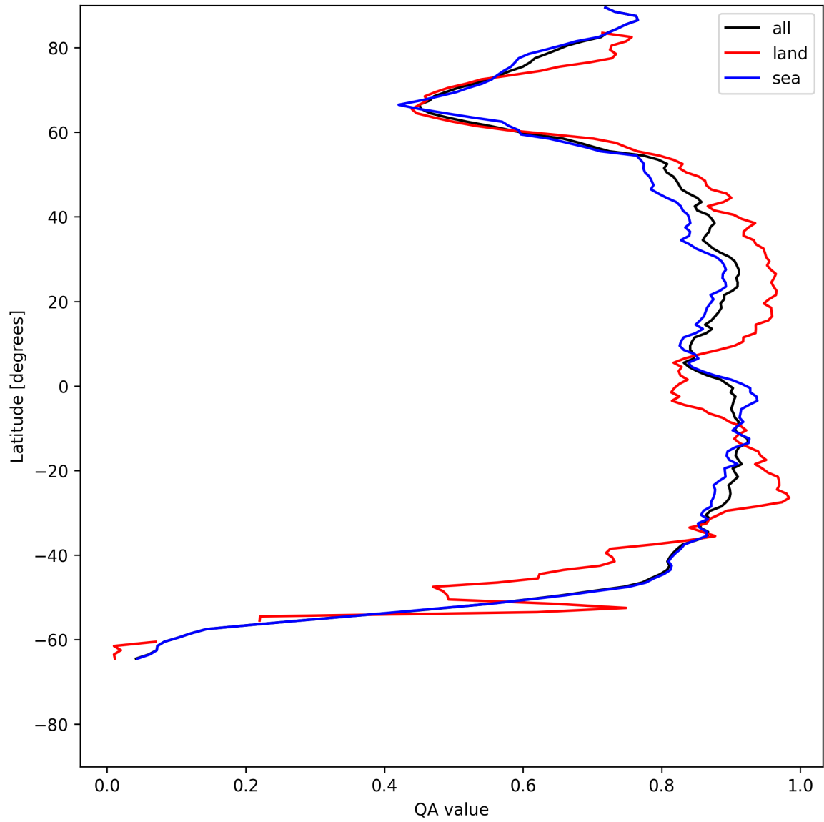
Figure 9: Zonal average of “QA value” for 2025-06-12 to 2025-06-13.
