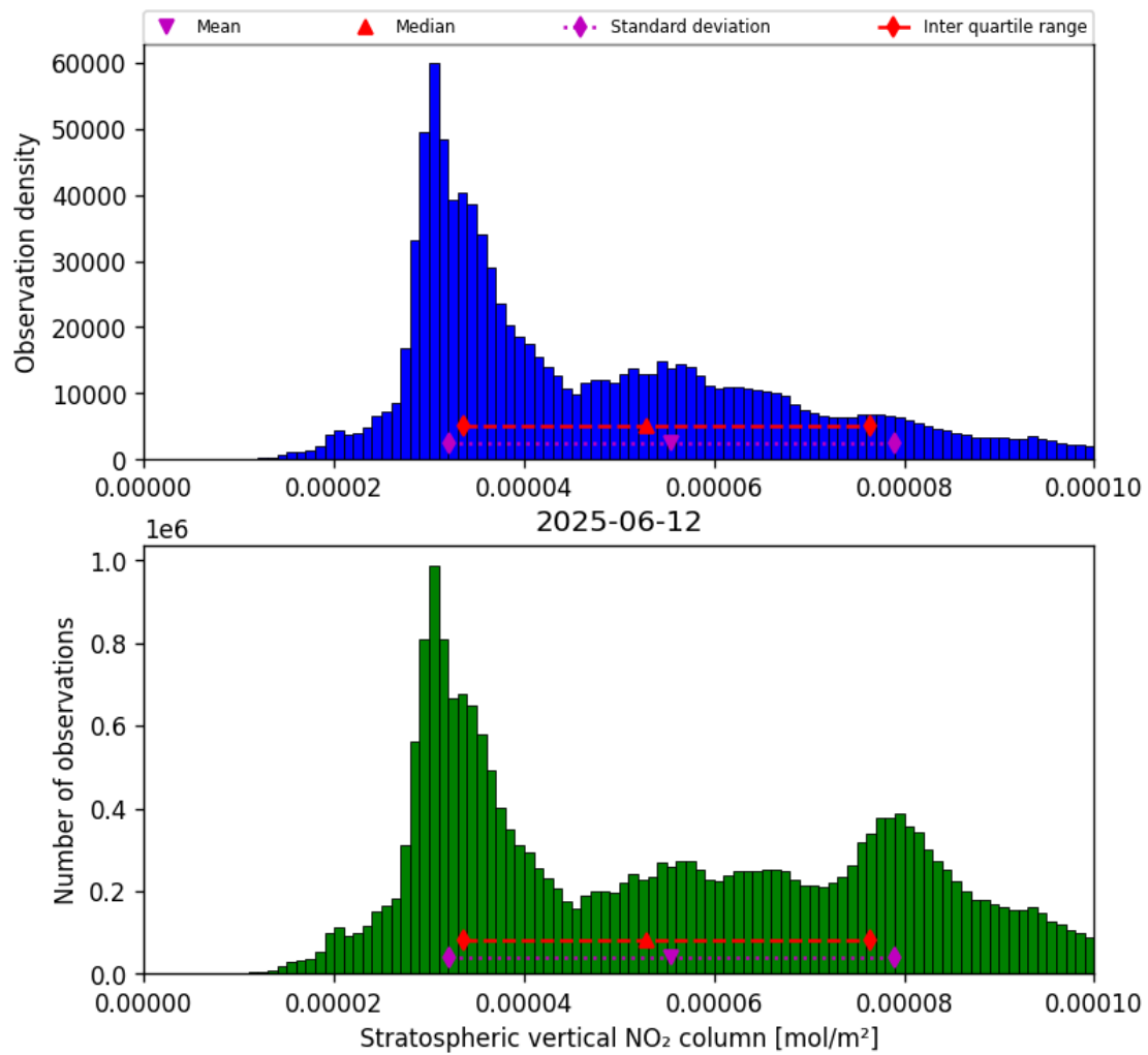
Figure 34: Histogram of “Stratospheric vertical NO 2 column” for 2025-06-12 to 2025-06-13
