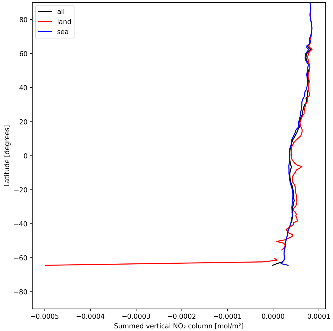
Figure 21: Zonal average of “Summed vertical NO 2 column” for 2025-06-12 to 2025-06-13.
