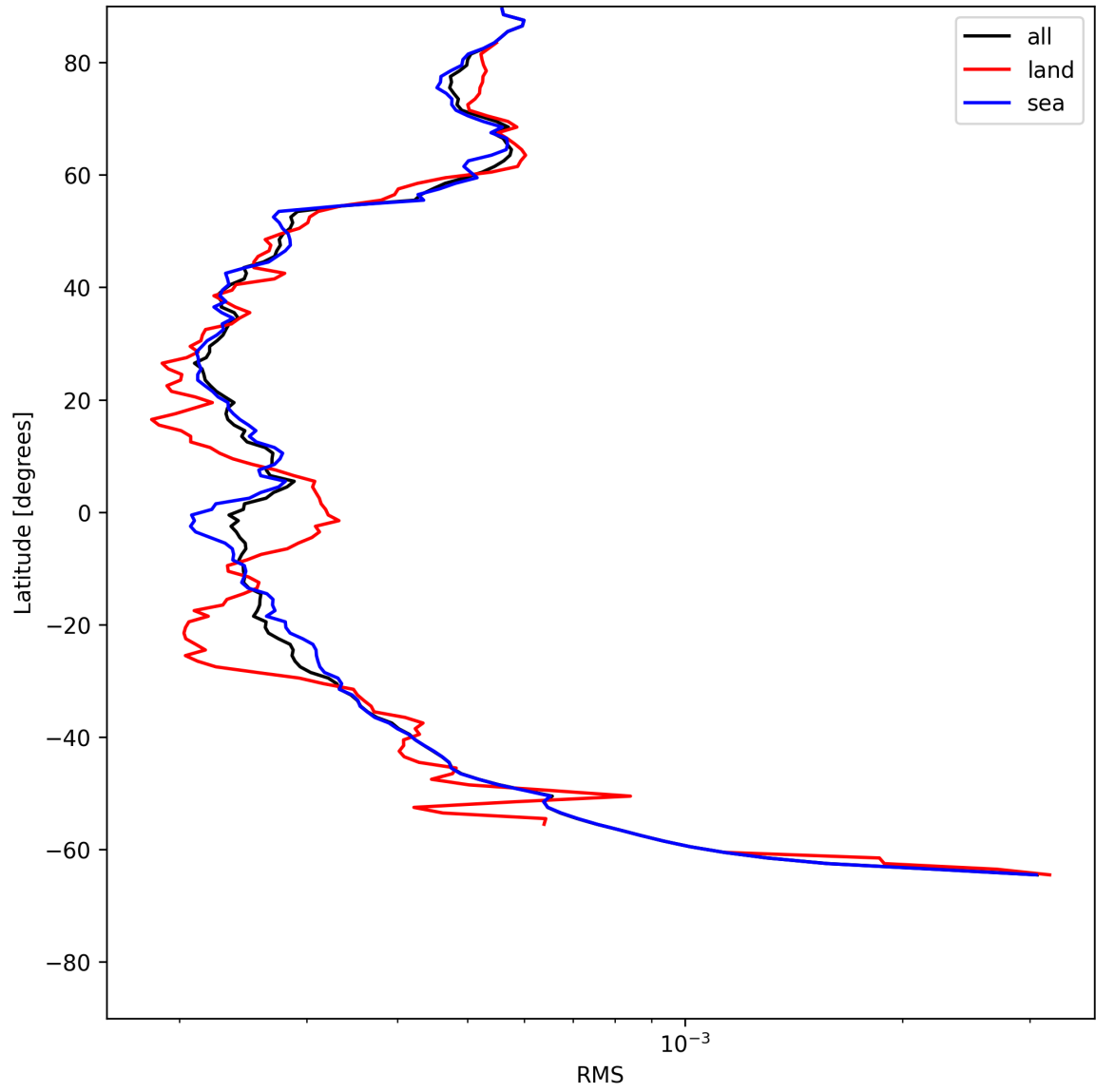
Figure 24: Zonal average of “RMS” for 2025-06-12 to 2025-06-13.
