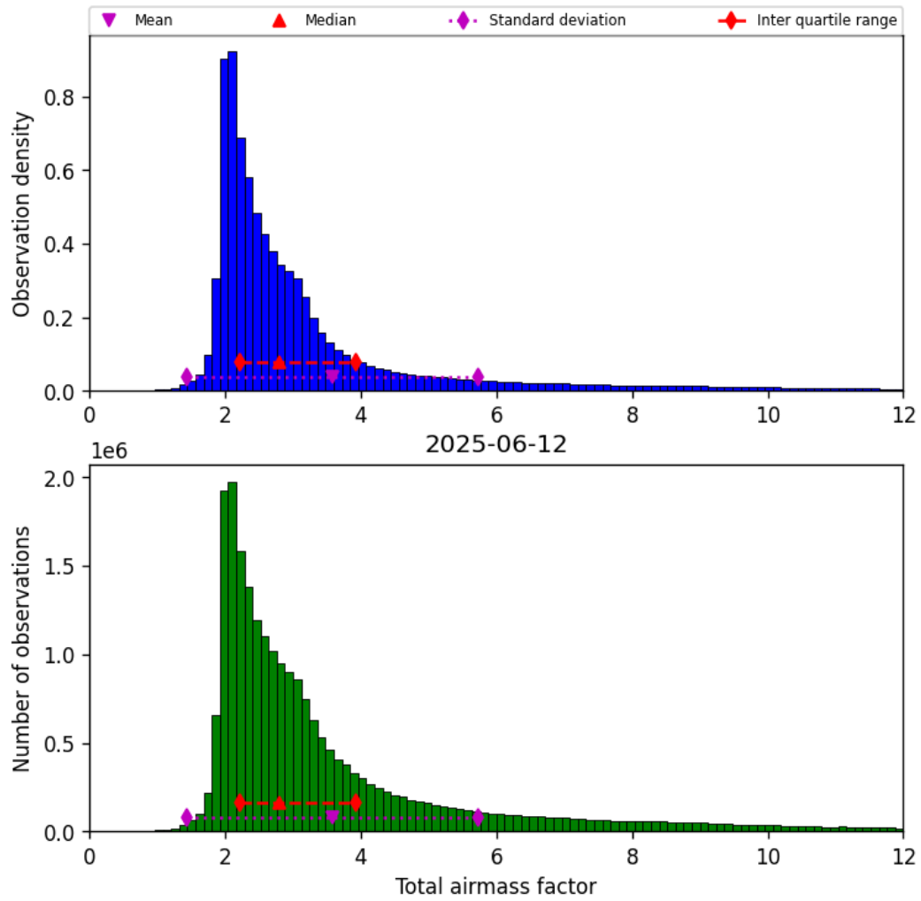
Figure 30: Histogram of “Total airmass factor” for 2025-06-12 to 2025-06-13
