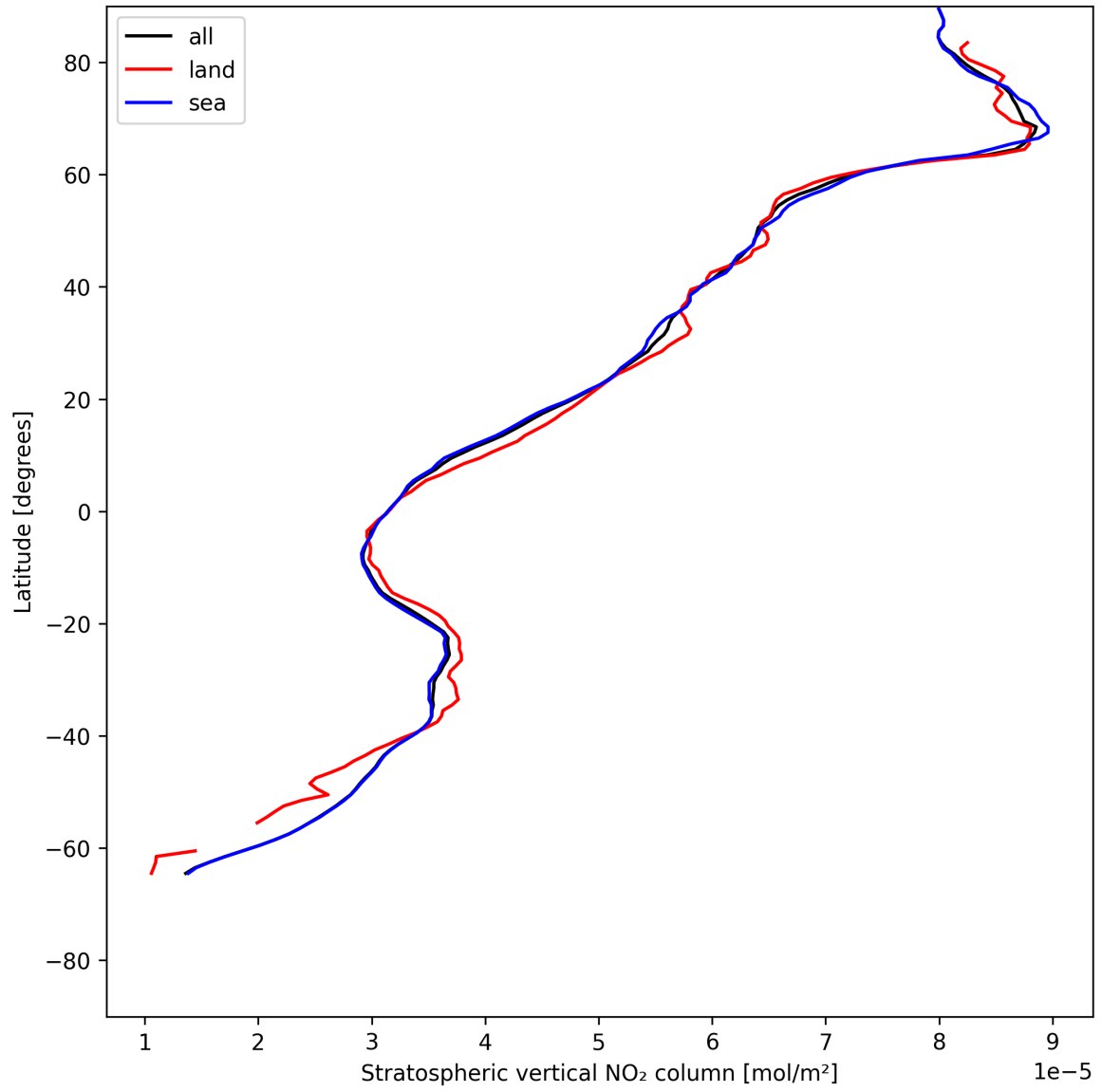
Figure 17: Zonal average of “Stratospheric vertical NO 2 column” for 2025-06-12 to 2025-06-13.
