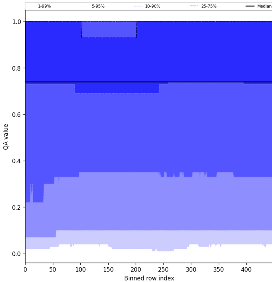
Figure 43: Along track statistics of “QA value” for 2025-06-12 to 2025-06-13
