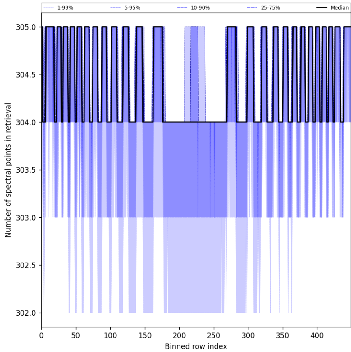
Figure 48: Along track statistics of “Number of spectral points in retrieval” for 2025-06-12 to 2025-06-13
