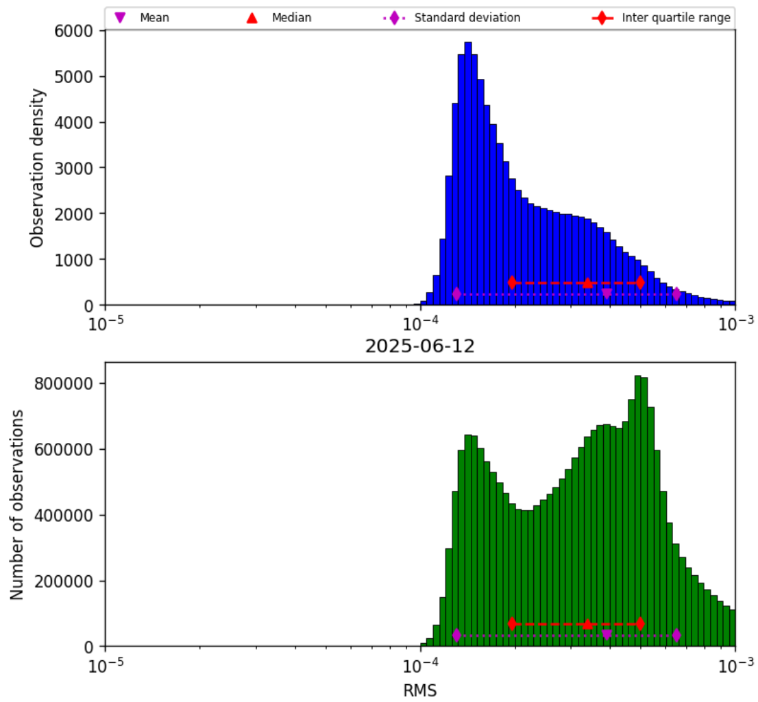
Figure 41: Histogram of “RMS” for 2025-06-12 to 2025-06-13
