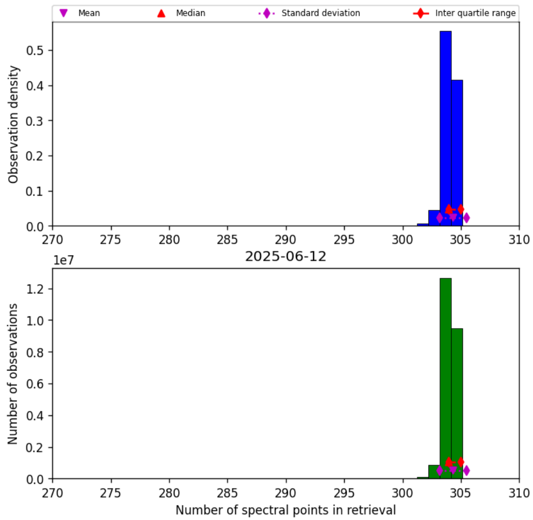
Figure 31: Histogram of “Number of spectral points in retrieval” for 2025-06-12 to 2025-06-13
