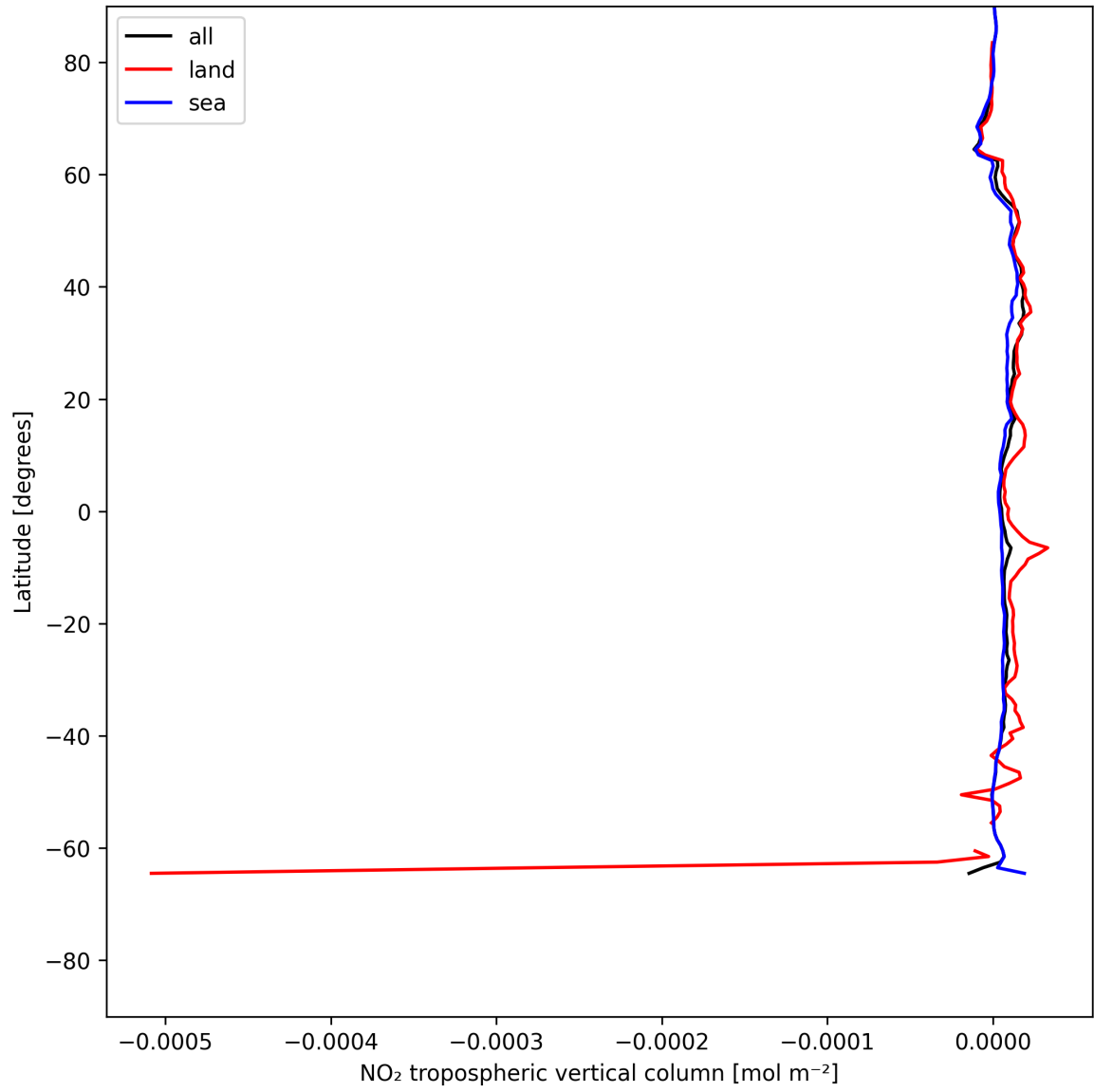
Figure 10: Zonal average of “NO 2 tropospheric vertical column” for 2025-06-12 to 2025-06-13.
