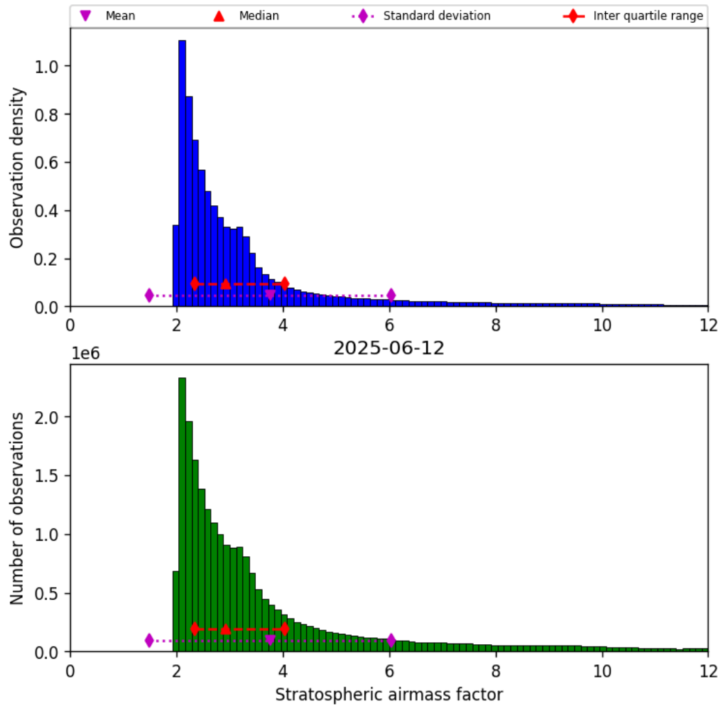
Figure 42: Histogram of “Stratospheric airmass factor” for 2025-06-12 to 2025-06-13
