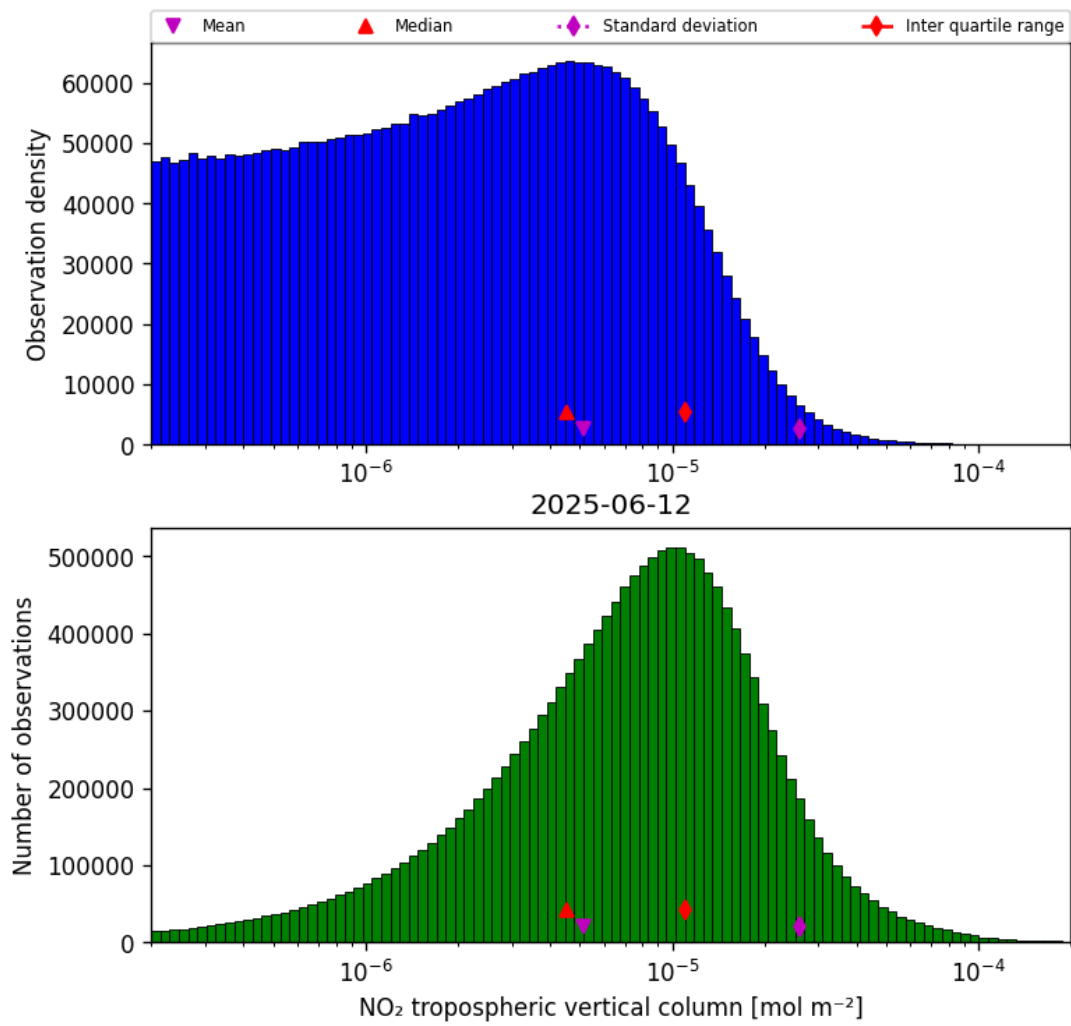
Figure 27: Histogram of “NO 2 tropospheric vertical column” for 2025-06-12 to 2025-06-13
