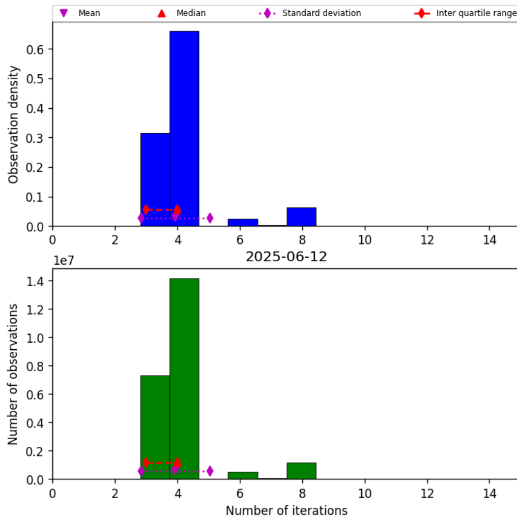
Figure 32: Histogram of “Number of iterations” for 2025-06-12 to 2025-06-13
