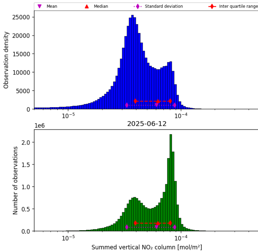
Figure 38: Histogram of "Summed vertical NO 2 column" for 2025-06-12 to 2025-06-13
