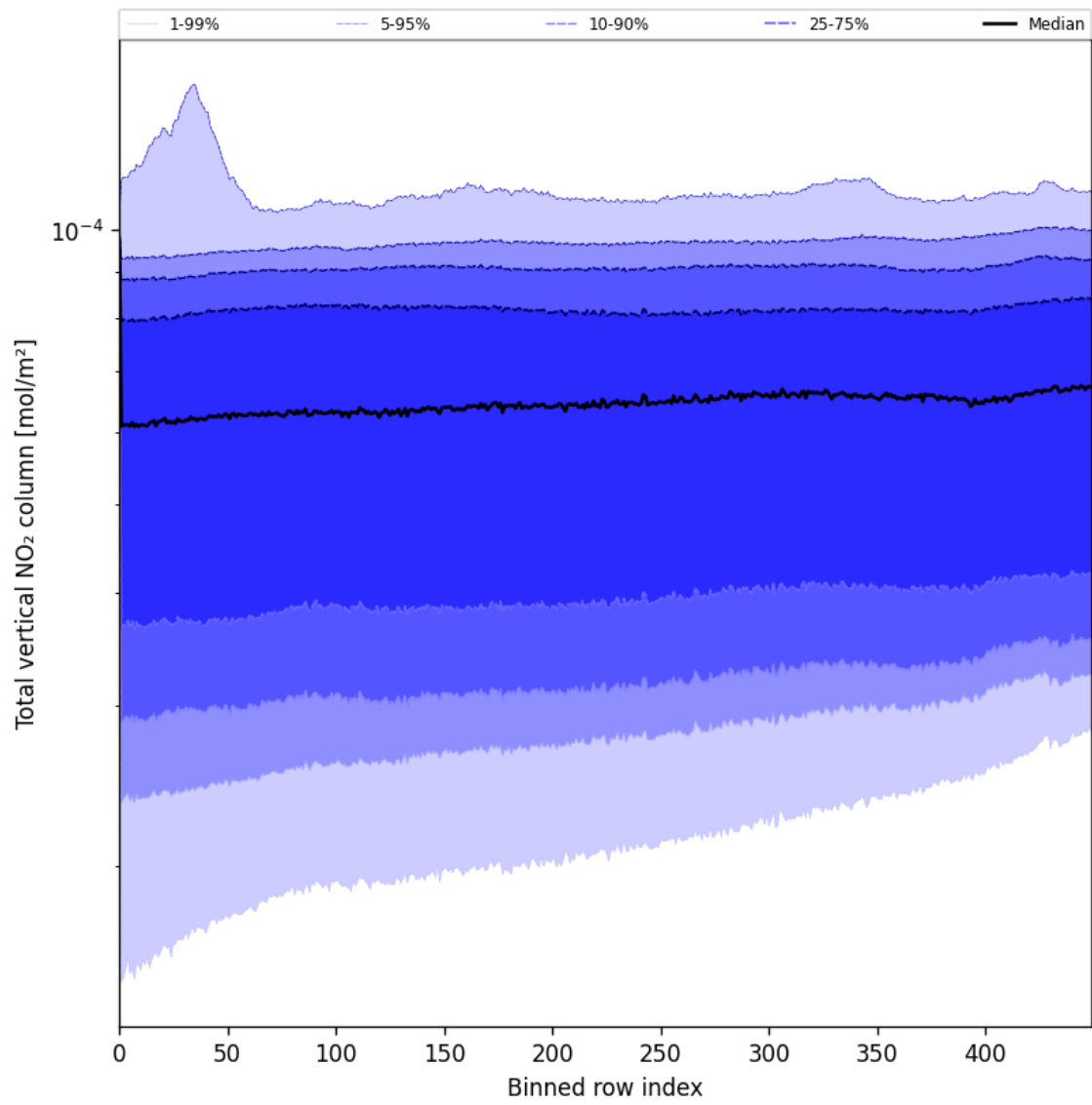
Figure 53: Along track statistics of “Total vertical NO 2 column” for 2025-06-12 to 2025-06-13
