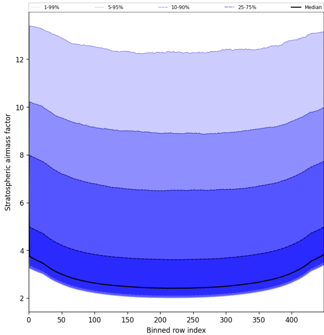
Figure 59: Along track statistics of “Stratospheric airmass factor” for 2025-06-12 to 2025-06-13
