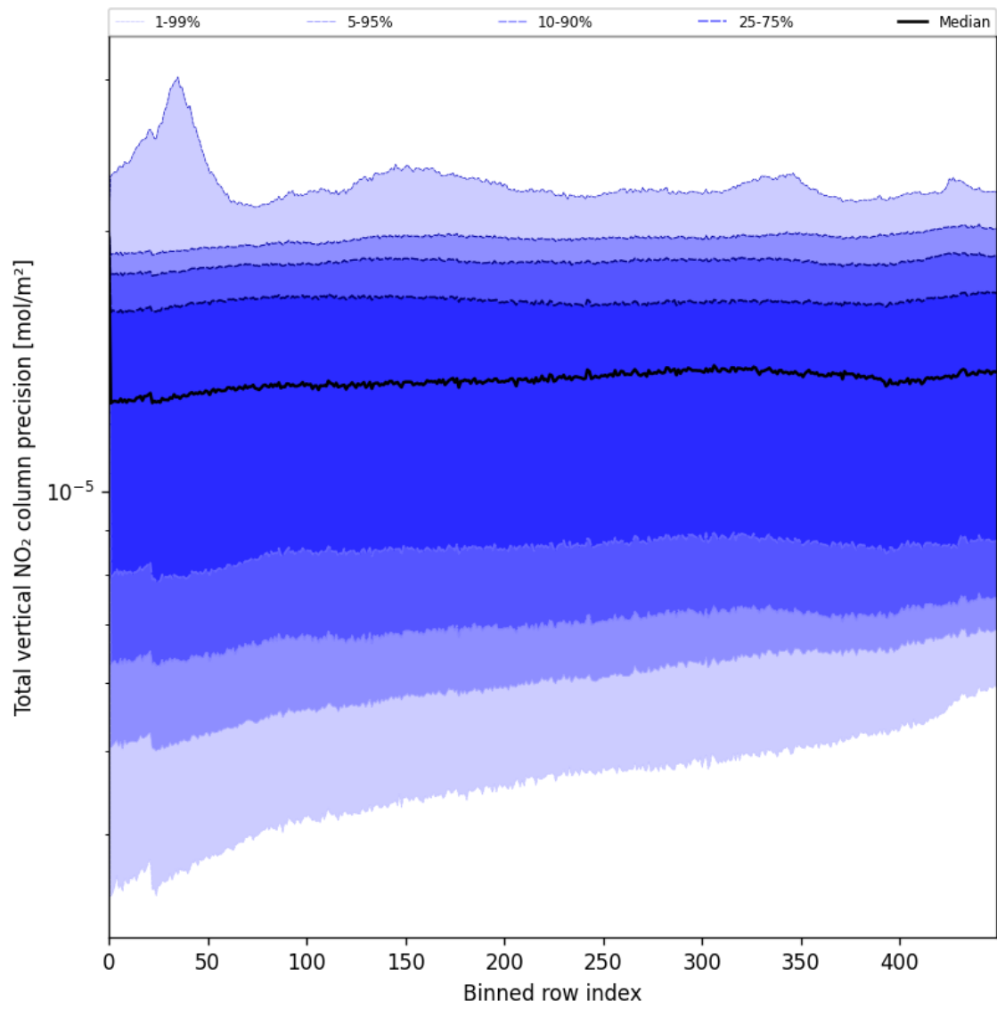
Figure 54: Along track statistics of “Total vertical NO 2 column precision” for 2025-06-12 to 2025-06-13
