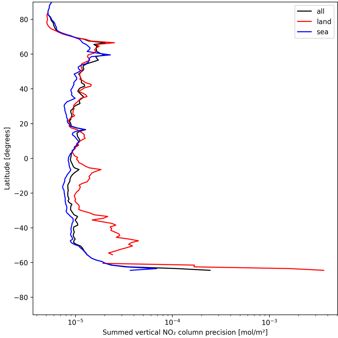
Figure 22: Zonal average of “Summed vertical NO 2 column precision” for 2025-06-12 to 2025-06-13.
