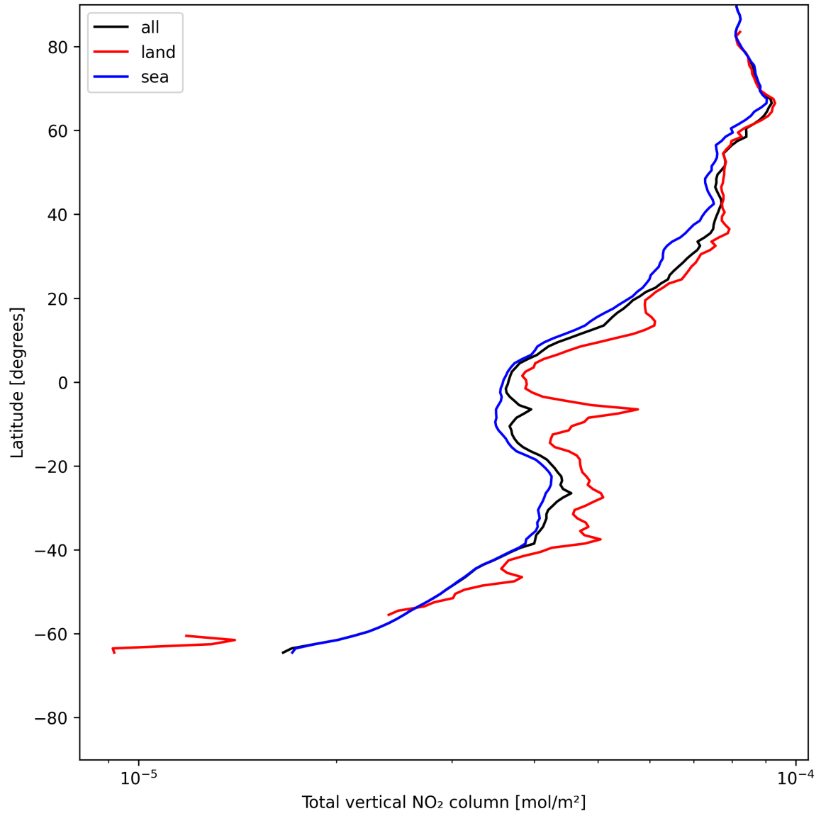
Figure 19: Zonal average of “Total vertical NO 2 column” for 2025-06-12 to 2025-06-13.
