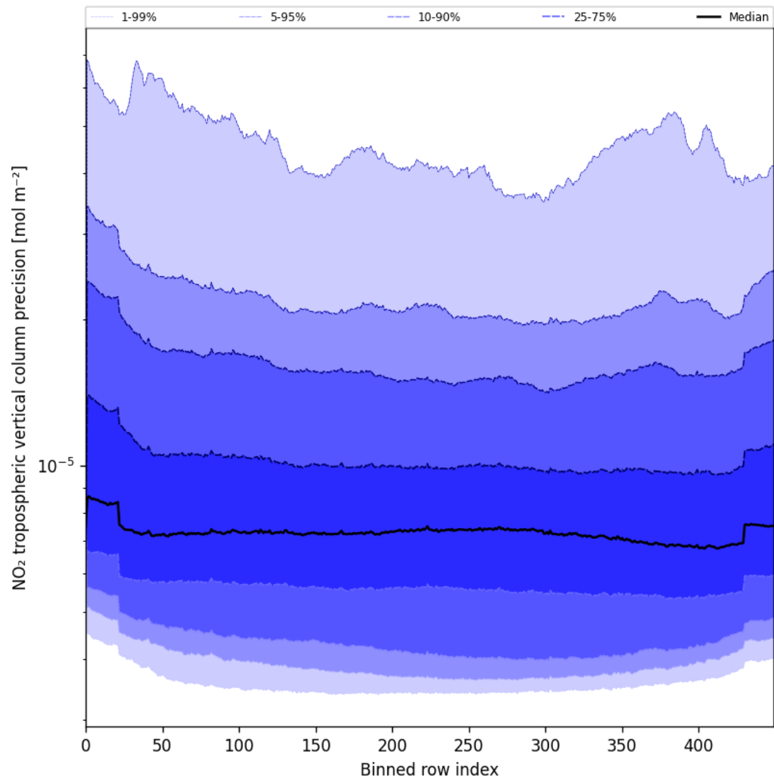
Figure 45: Along track statistics of “NO 2 tropospheric vertical column precision” for 2025-06-13 to 2025-06-14
