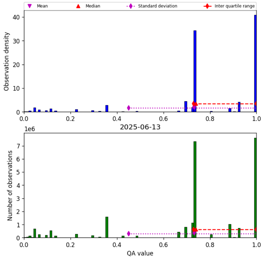
Figure 26: Histogram of “QA value” for 2025-06-13 to 2025-06-14
