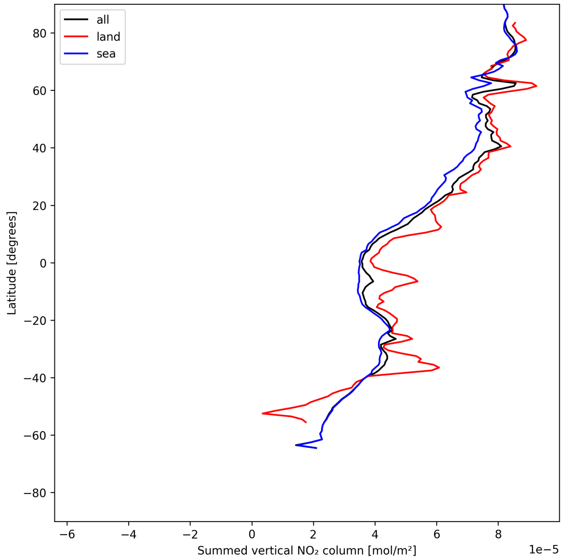
Figure 21: Zonal average of “Summed vertical NO 2 column” for 2025-06-13 to 2025-06-14.
