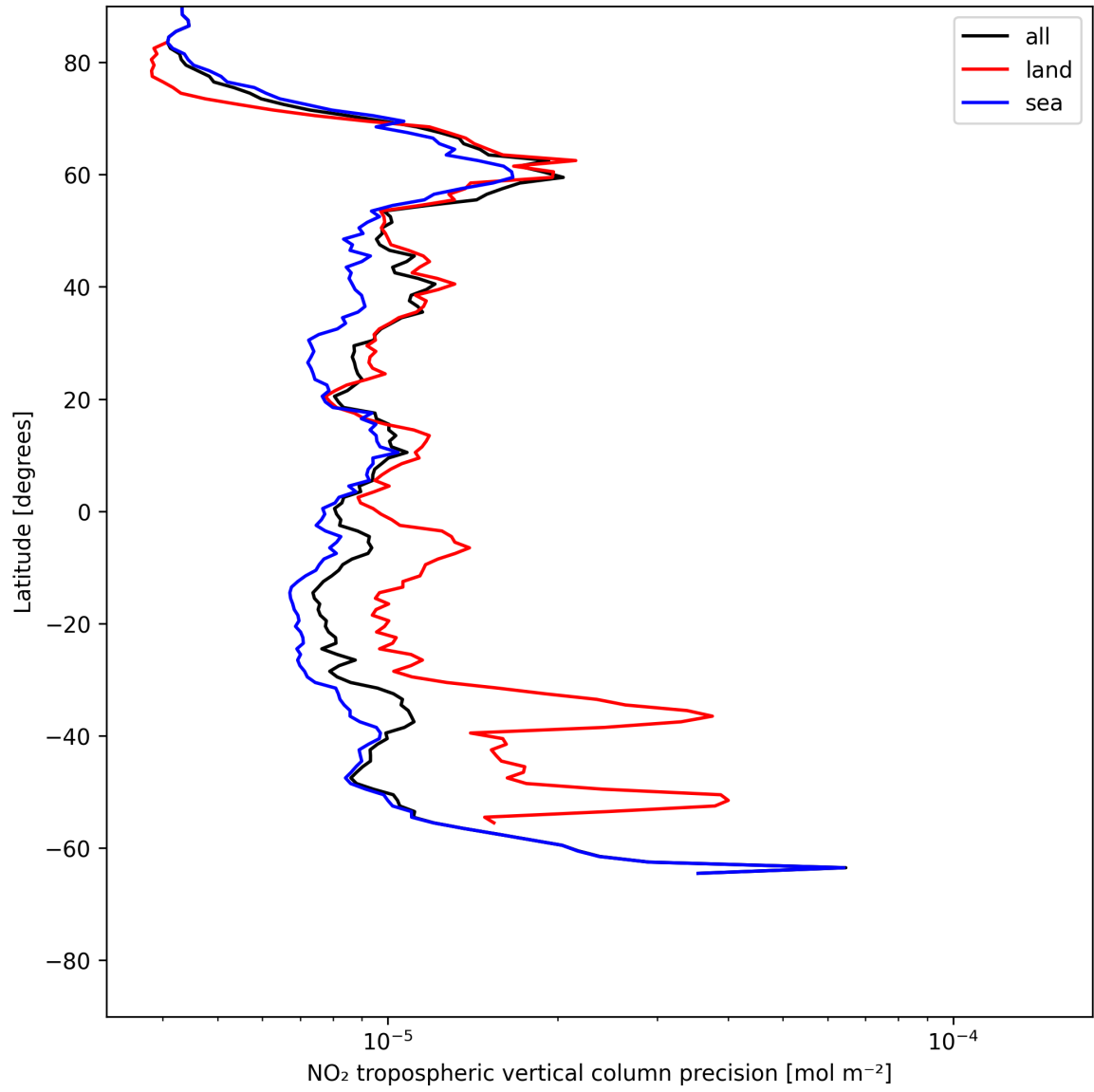
Figure 11: Zonal average of “NO 2 tropospheric vertical column precision” for 2025-06-13 to 2025-06-14.
