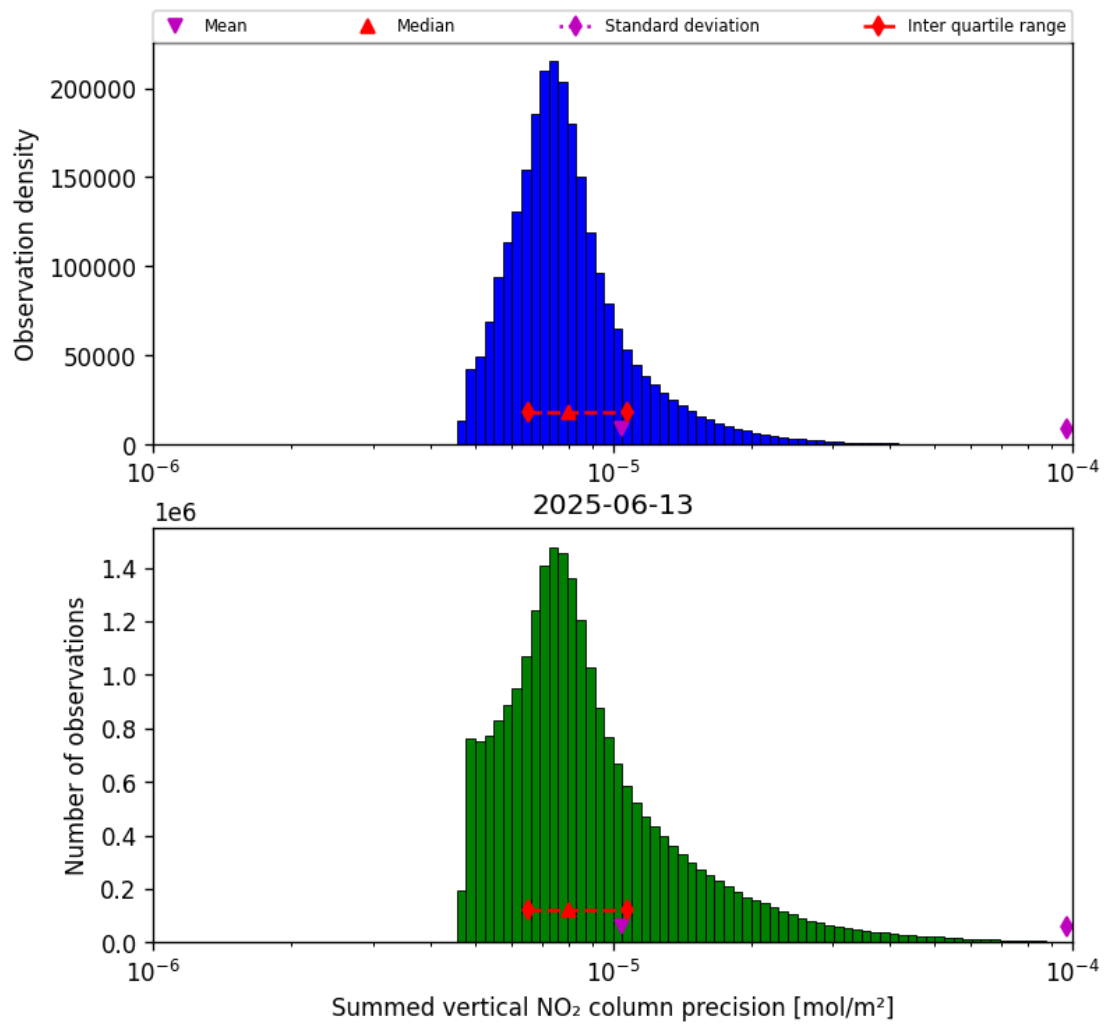
Figure 39: Histogram of “Summed vertical NO 2 column precision” for 2025-06-13 to 2025-06-14
