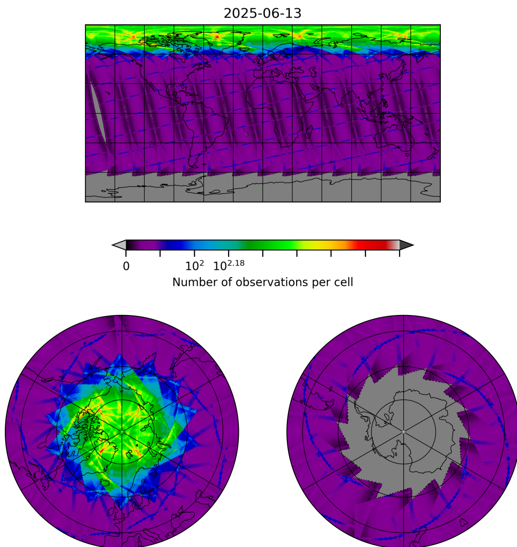
Figure 8: Map of the number of observations for 2025-06-13 to 2025-06-14
