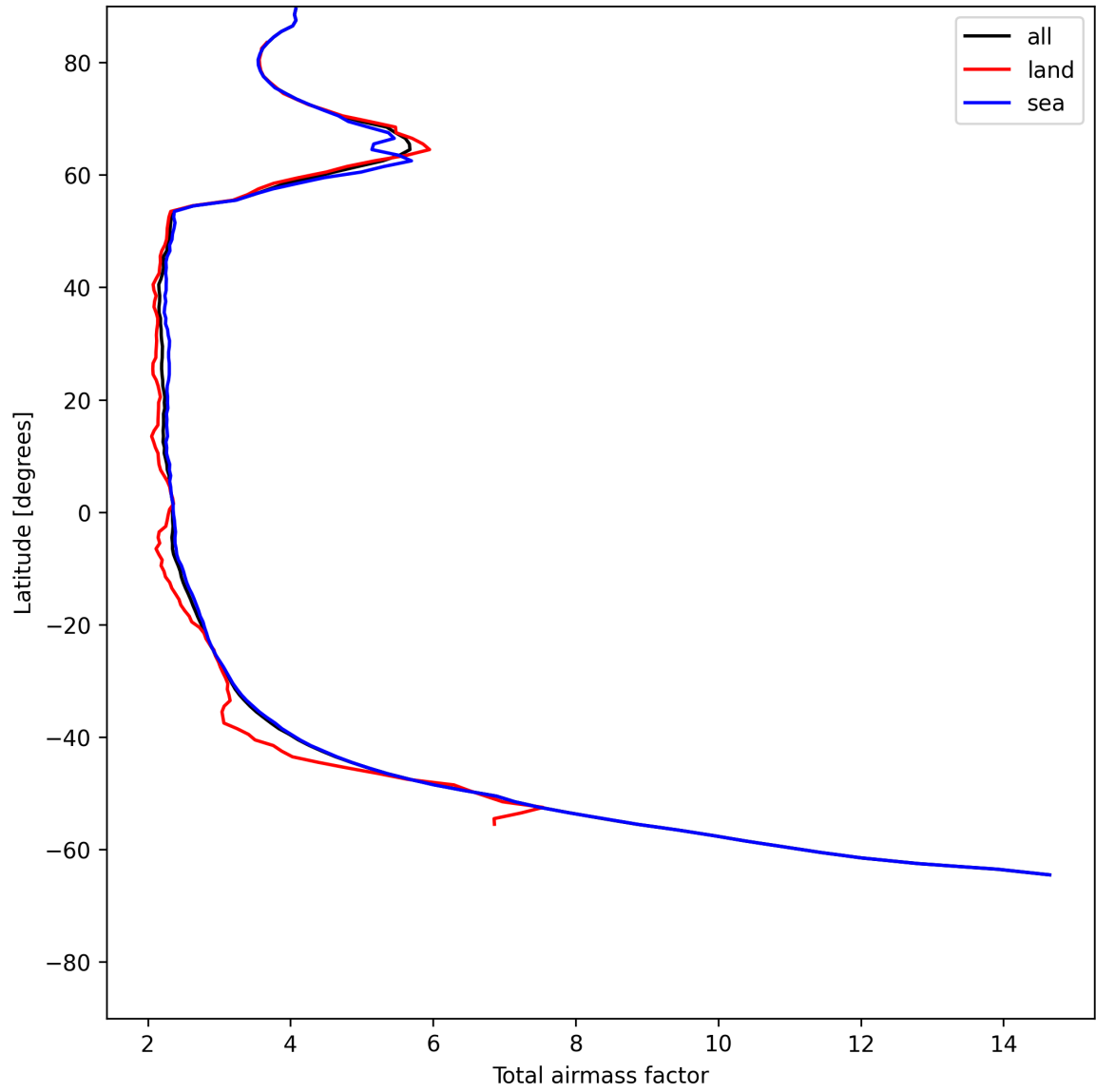
Figure 13: Zonal average of “Total airmass factor” for 2025-06-13 to 2025-06-14.
