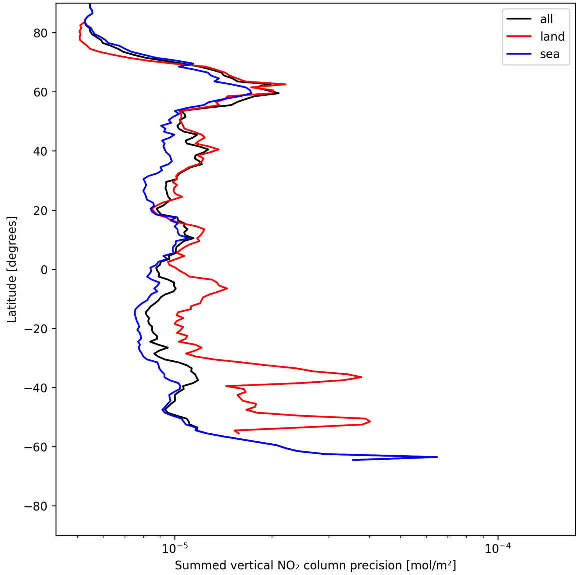
Figure 22: Zonal average of “Summed vertical NO 2 column precision” for 2025-06-13 to 2025-06-14.
