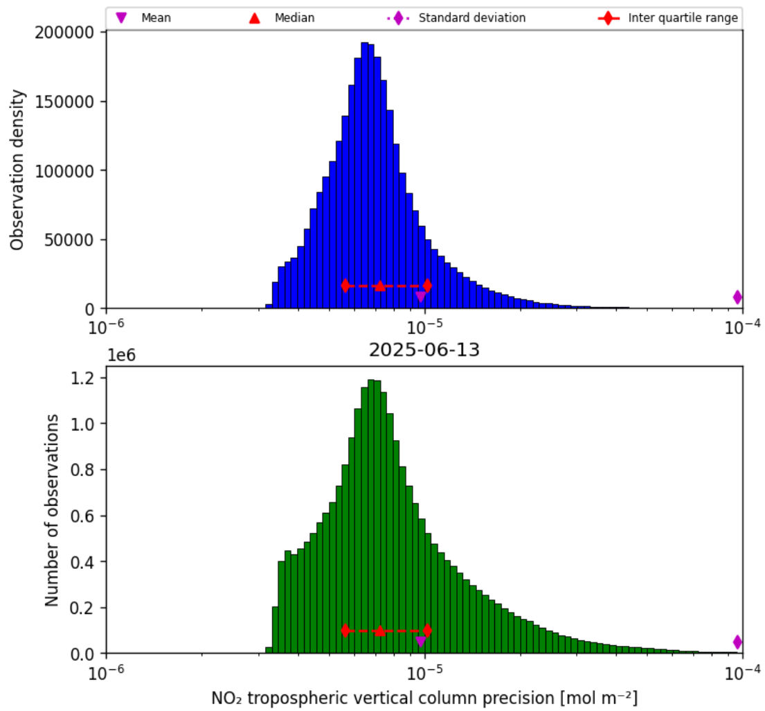
Figure 28: Histogram of “NO 2 tropospheric vertical column precision” for 2025-06-13 to 2025-06-14
