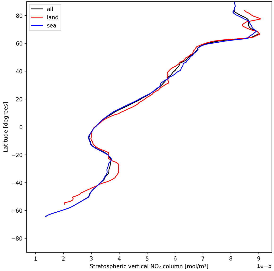
Figure 17: Zonal average of “Stratospheric vertical NO 2 column” for 2025-06-13 to 2025-06-14.
