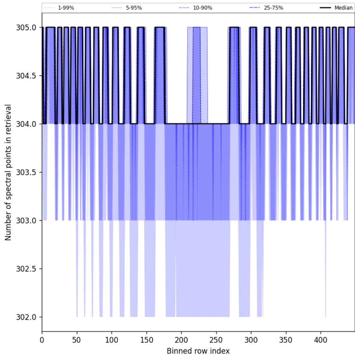
Figure 48: Along track statistics of “Number of spectral points in retrieval” for 2025-06-13 to 2025-06-14
