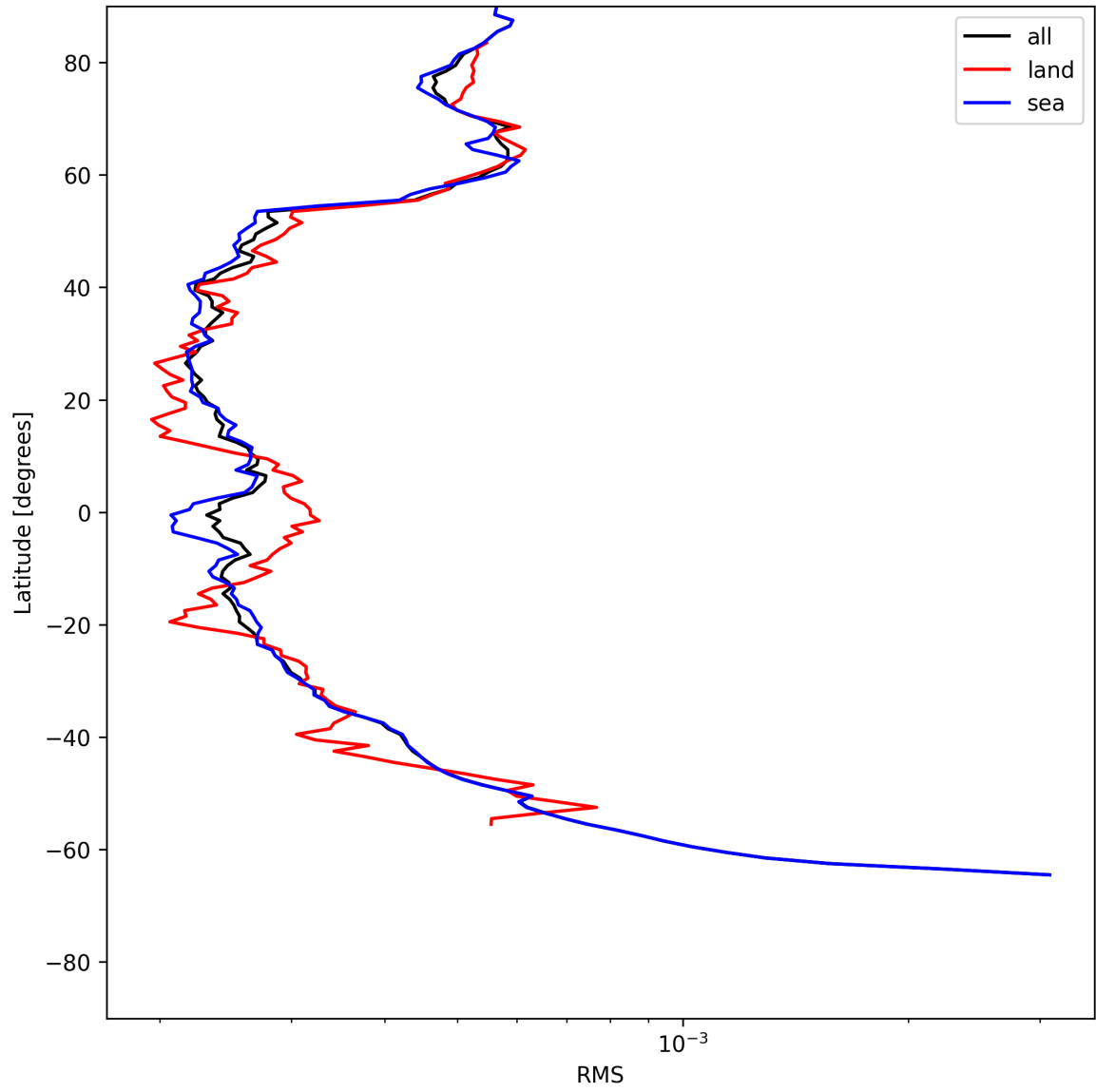
Figure 24: Zonal average of “RMS” for 2025-06-13 to 2025-06-14.
