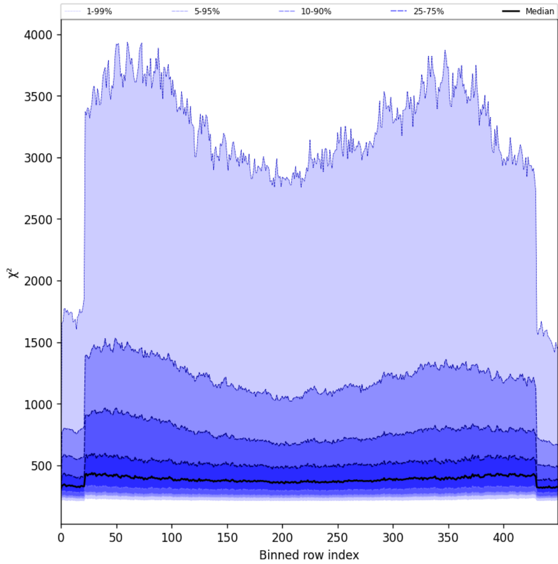
Figure 57: Along track statistics of “ \chi^2 ” for 2025-06-13 to 2025-06-14
