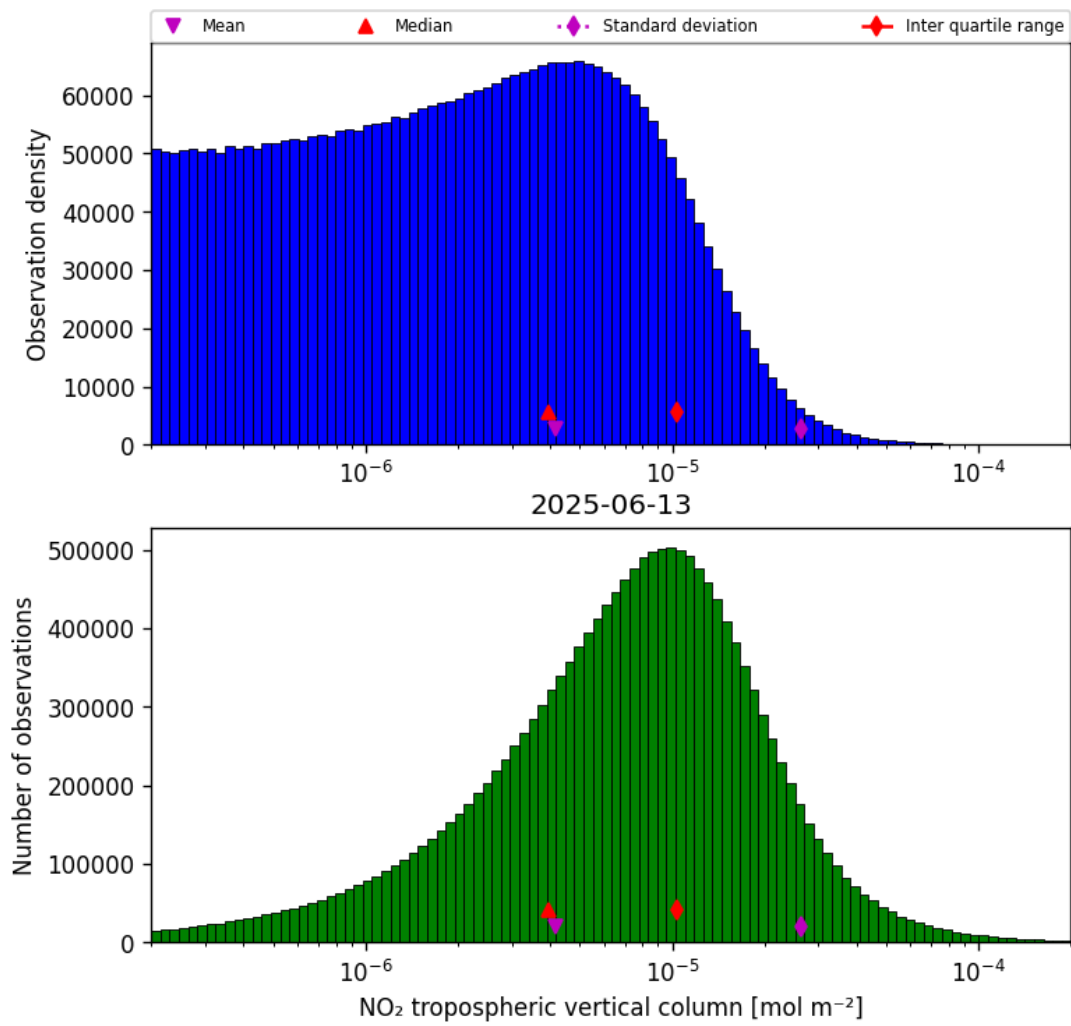
Figure 27: Histogram of “NO 2 tropospheric vertical column” for 2025-06-13 to 2025-06-14
