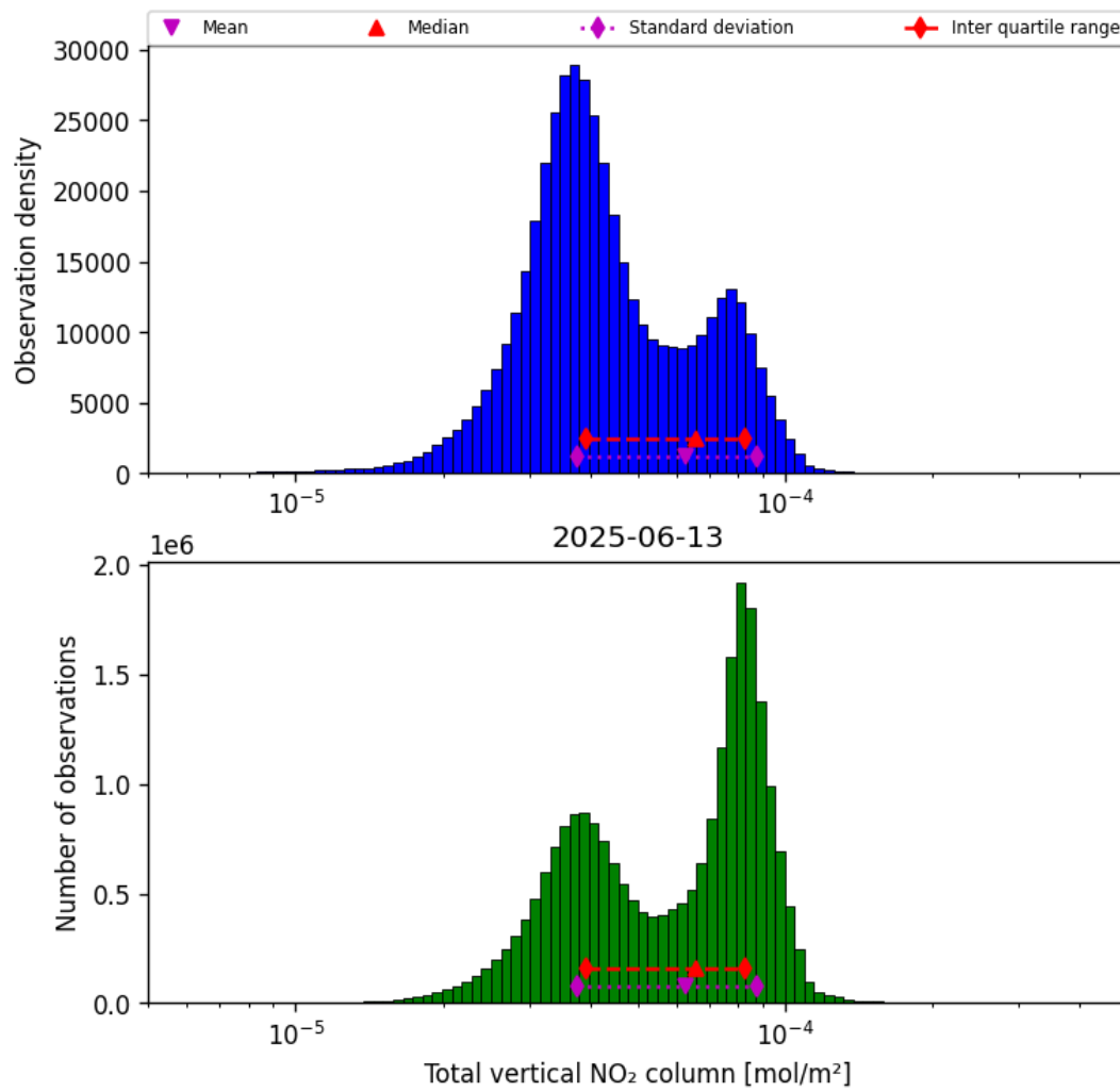
Figure 36: Histogram of “Total vertical NO 2 column” for 2025-06-13 to 2025-06-14
