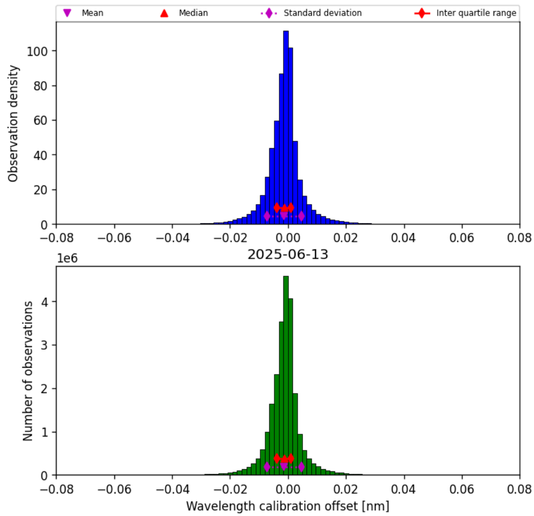
Figure 33: Histogram of “Wavelength calibration offset” for 2025-06-13 to 2025-06-14
