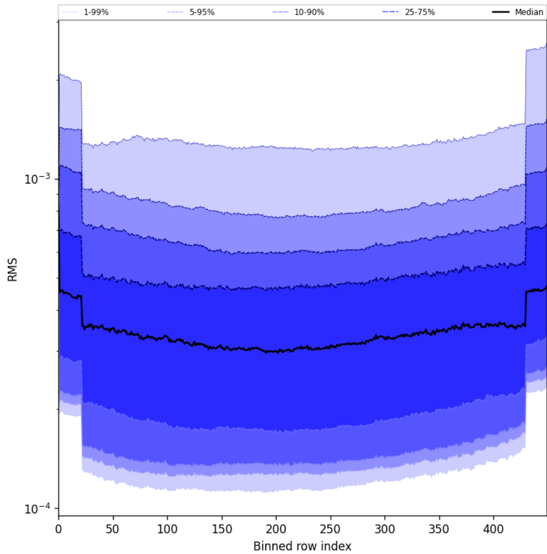
Figure 58: Along track statistics of “RMS” for 2025-06-13 to 2025-06-14
