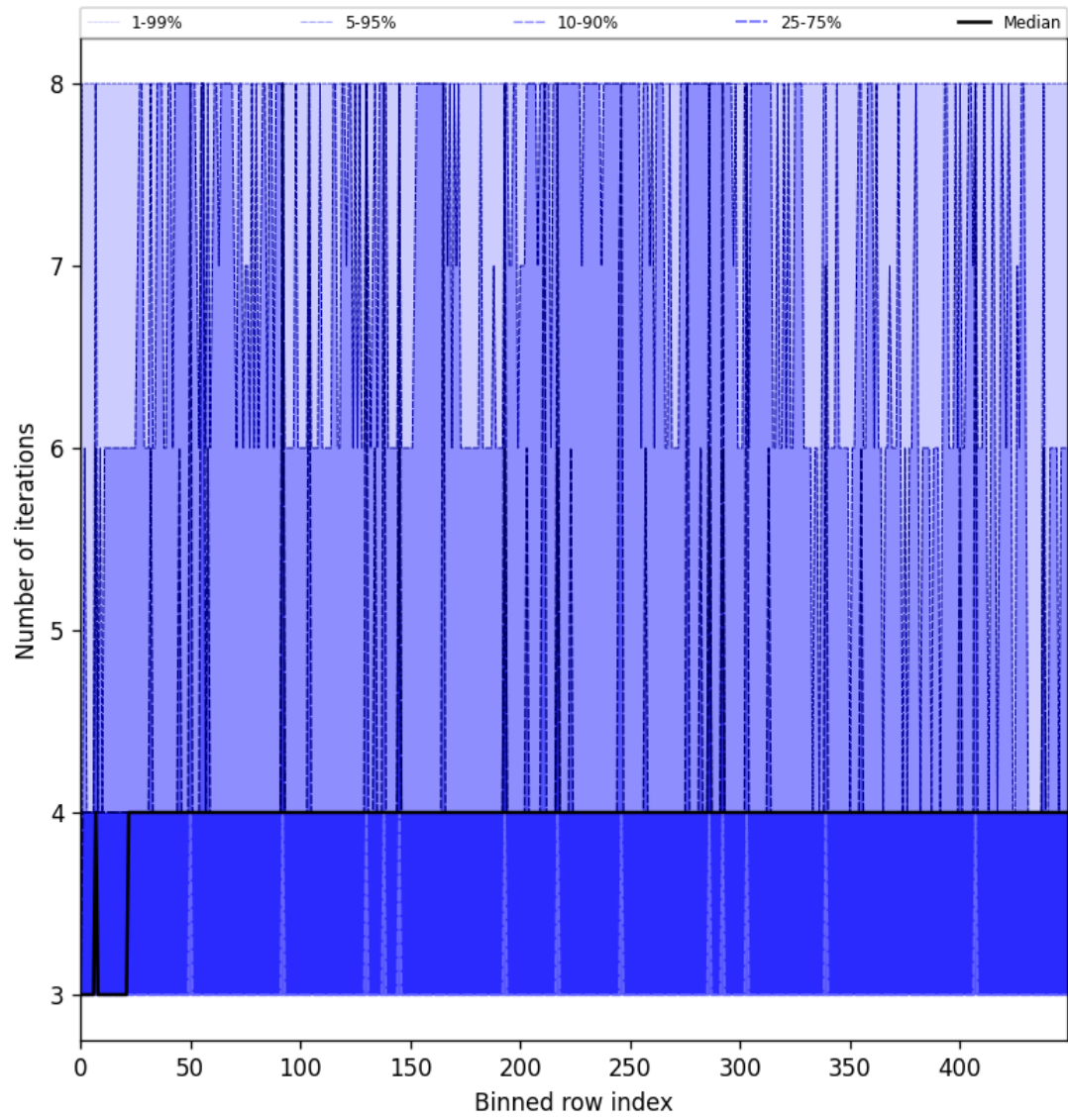
Figure 49: Along track statistics of “Number of iterations” for 2025-06-13 to 2025-06-14
