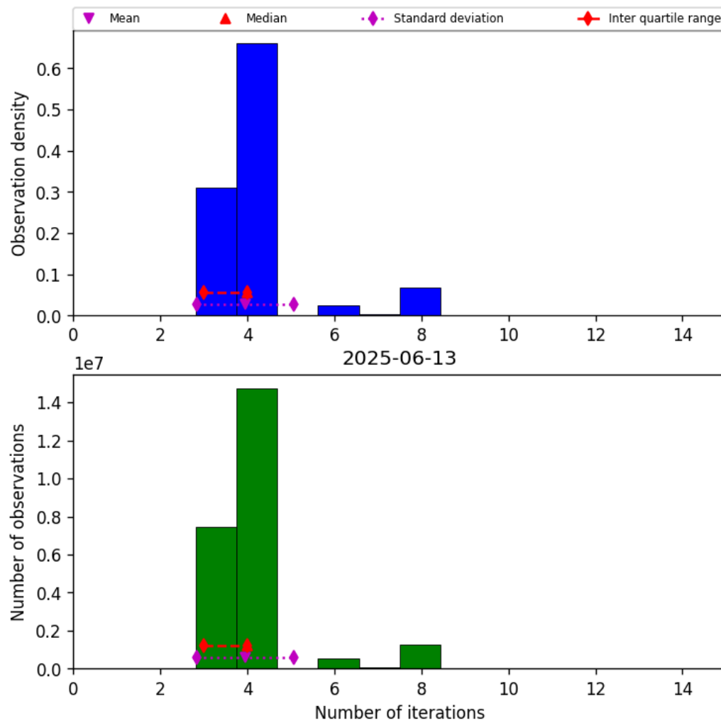
Figure 32: Histogram of “Number of iterations” for 2025-06-13 to 2025-06-14
