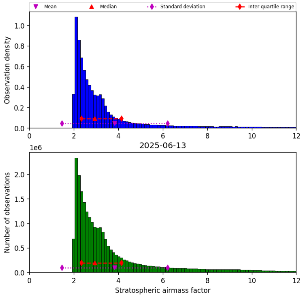
Figure 42: Histogram of “Stratospheric airmass factor” for 2025-06-13 to 2025-06-14
