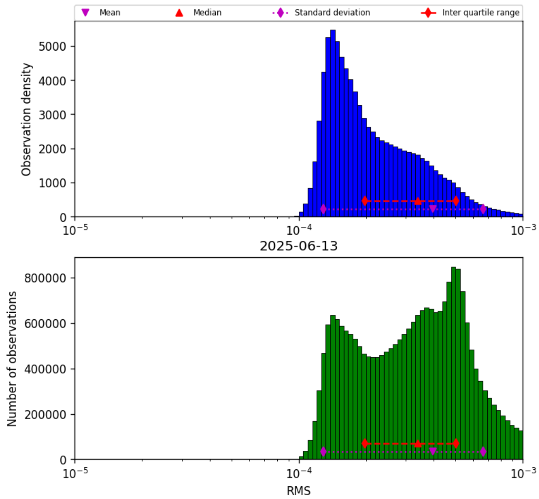
Figure 41: Histogram of “RMS” for 2025-06-13 to 2025-06-14
