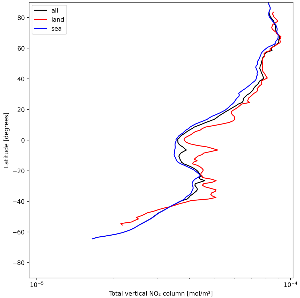
Figure 19: Zonal average of “Total vertical NO 2 column” for 2025-06-13 to 2025-06-14.
