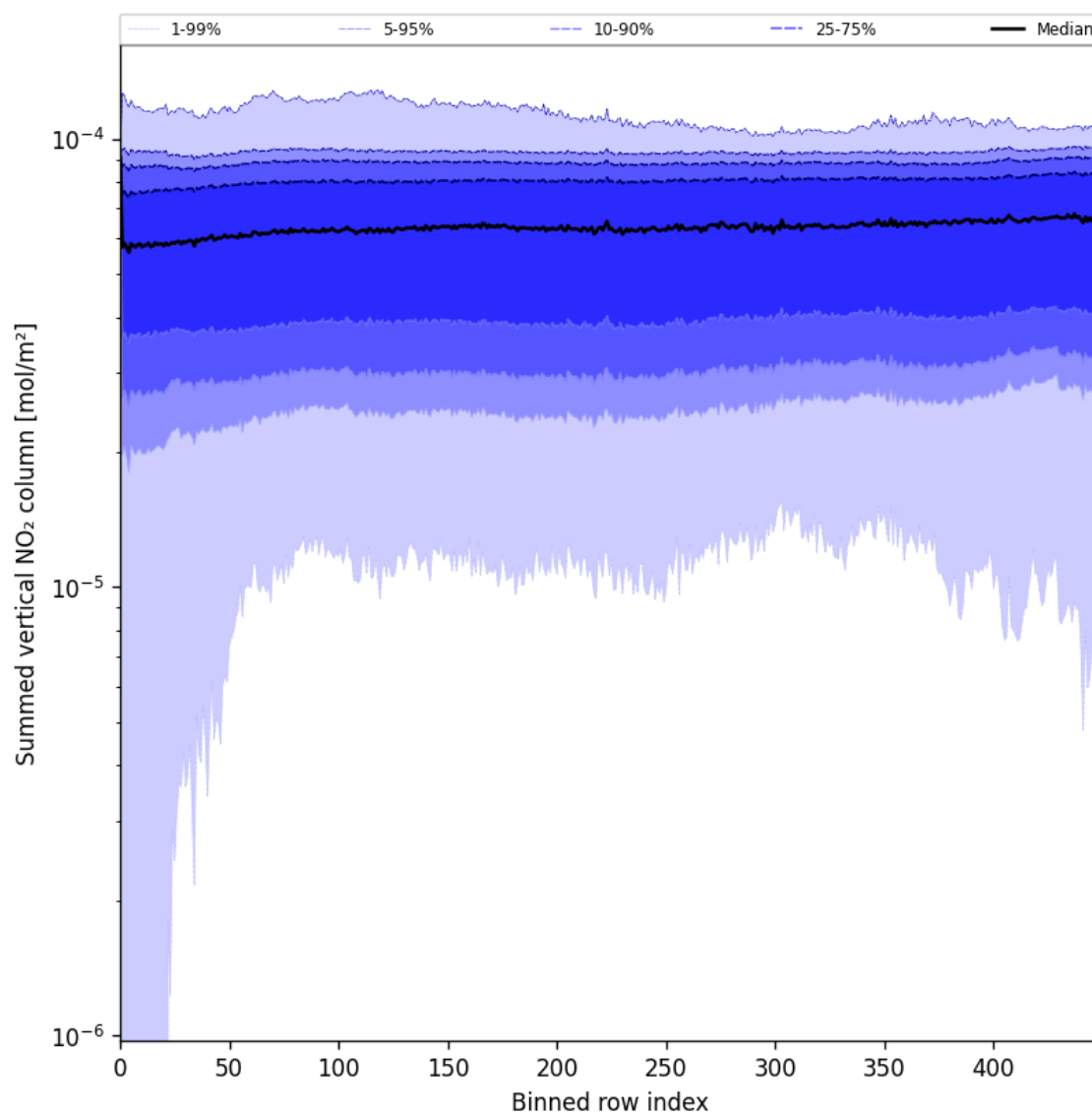
Figure 55: Along track statistics of “Summed vertical NO 2 column” for 2025-06-13 to 2025-06-14
