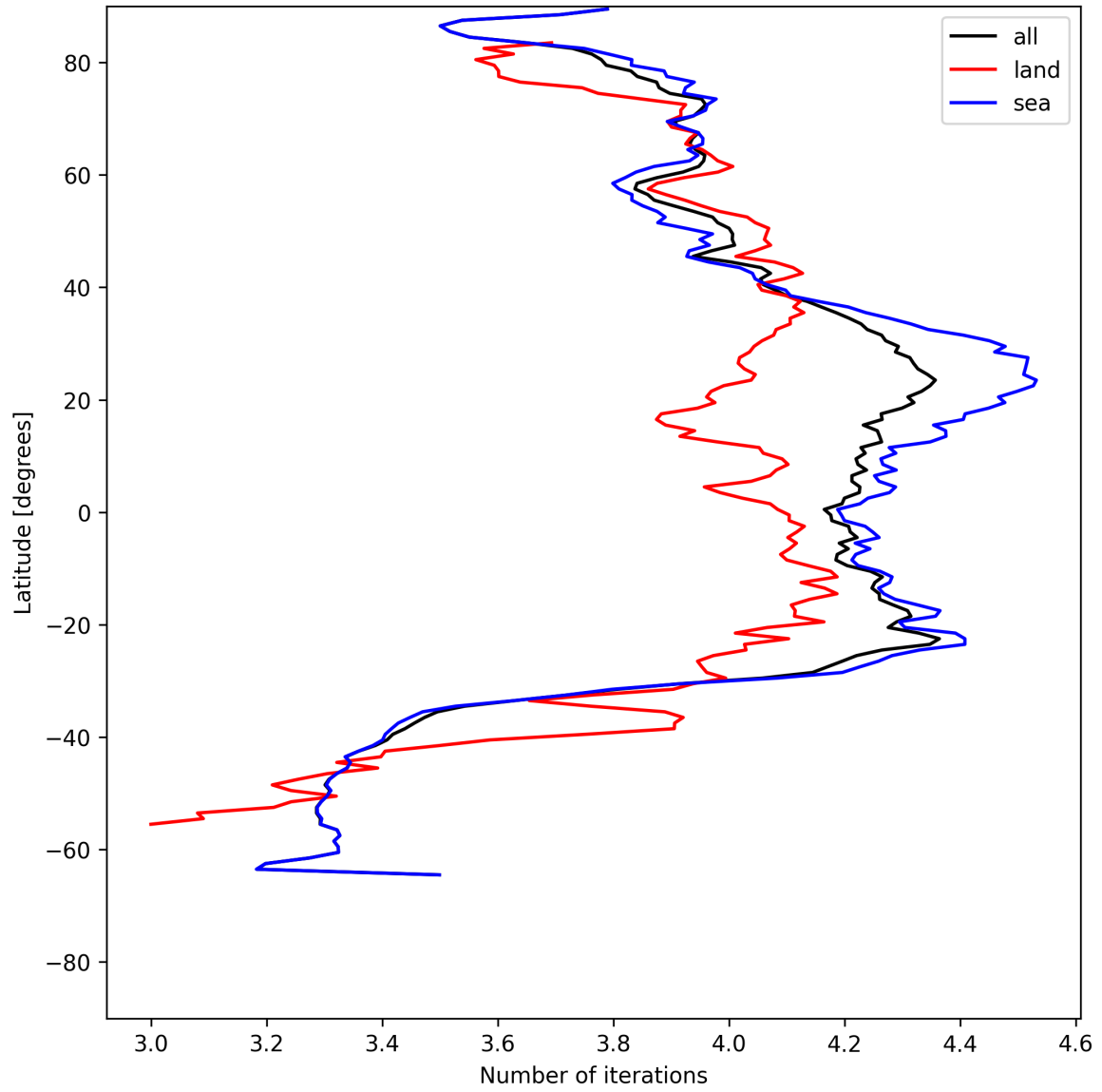
Figure 15: Zonal average of “Number of iterations” for 2025-06-13 to 2025-06-14.
