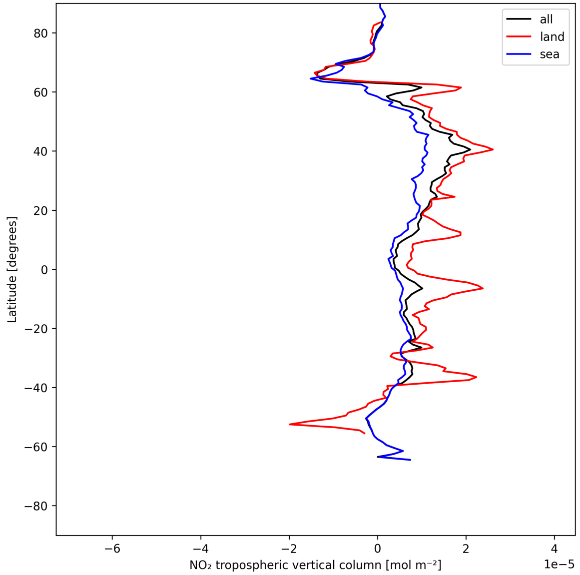
Figure 10: Zonal average of “NO 2 tropospheric vertical column” for 2025-06-13 to 2025-06-14.
