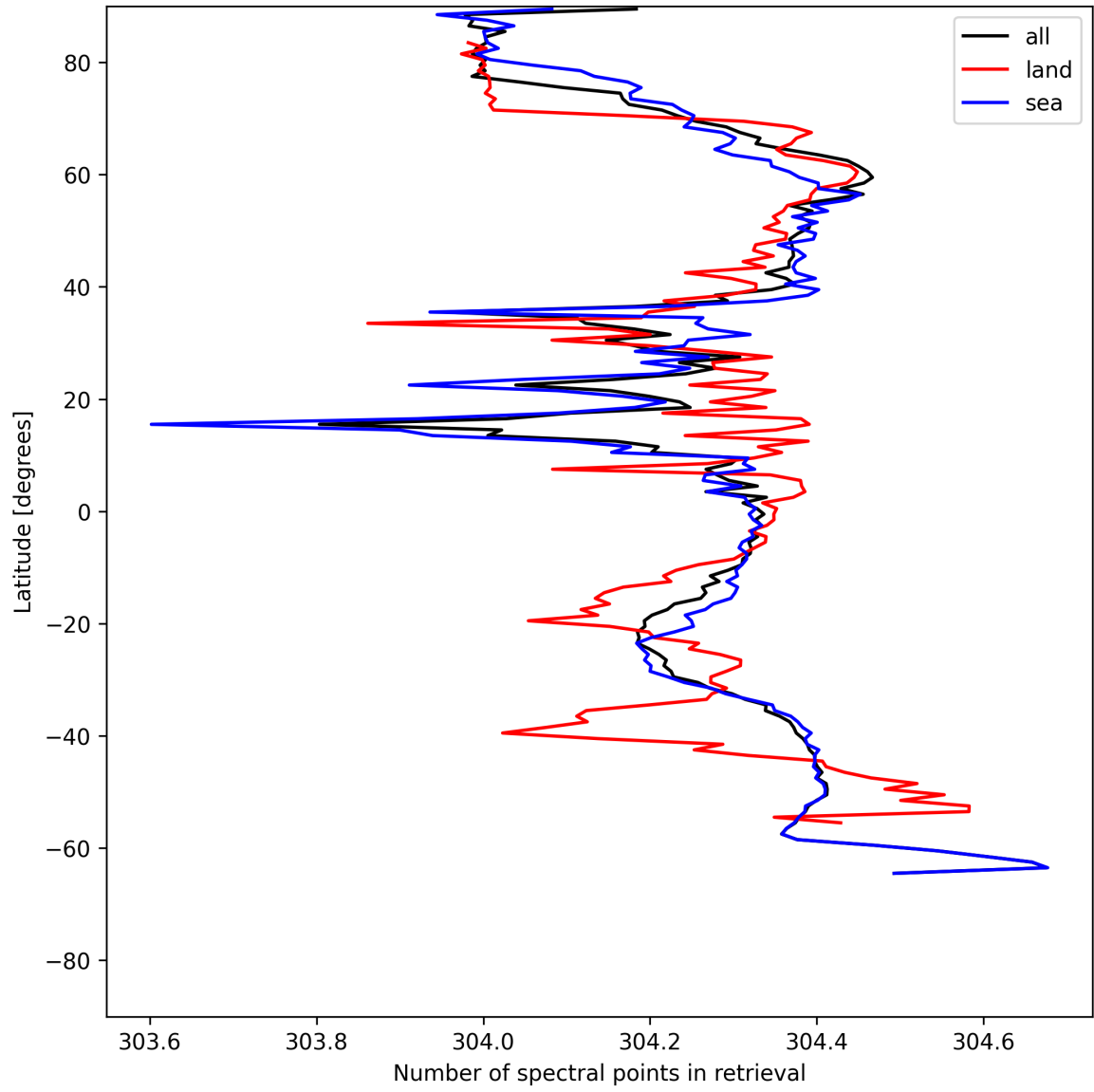
Figure 14: Zonal average of “Number of spectral points in retrieval” for 2025-06-13 to 2025-06-14.
