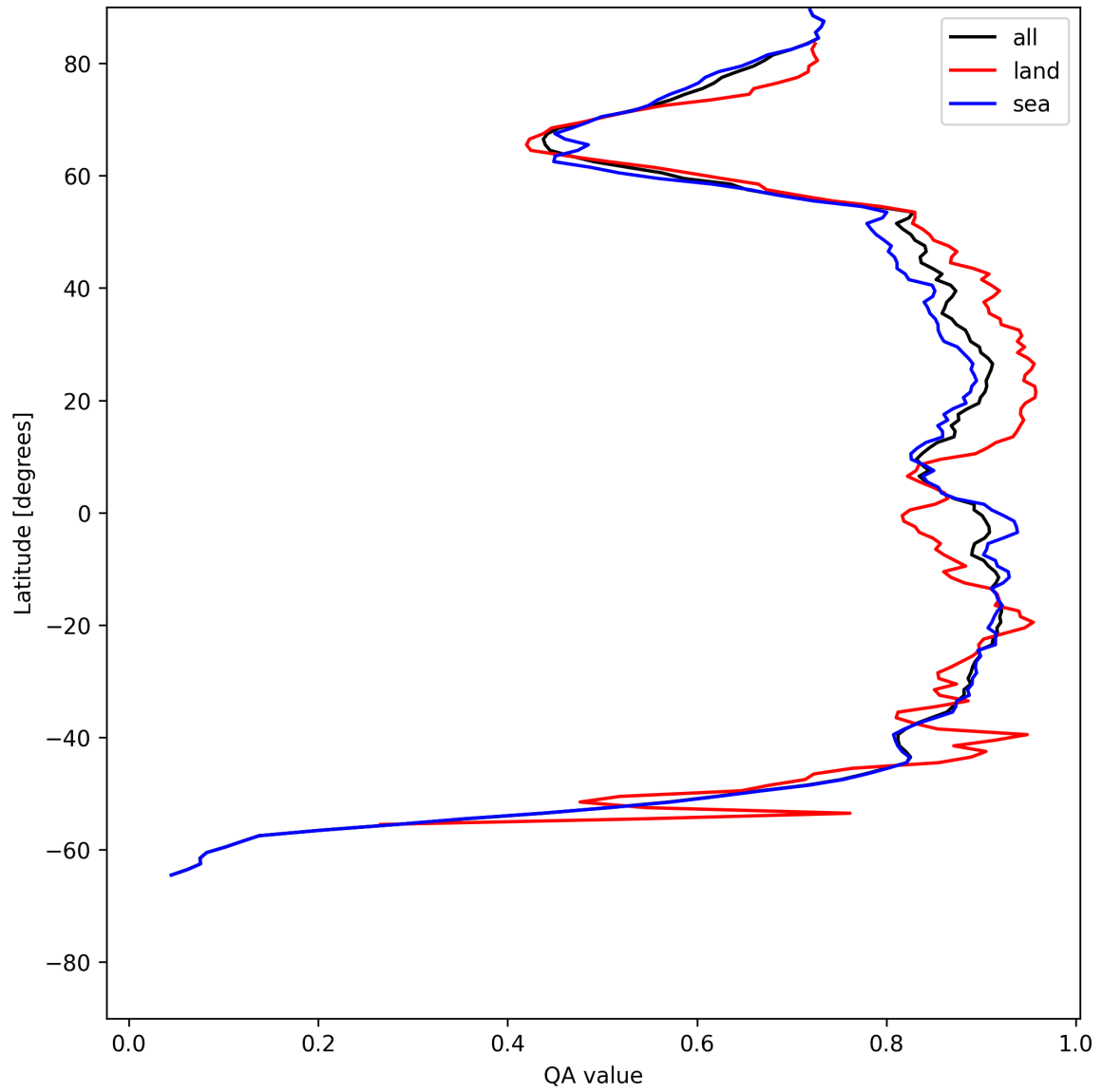
Figure 9: Zonal average of “QA value” for 2025-06-13 to 2025-06-14.
