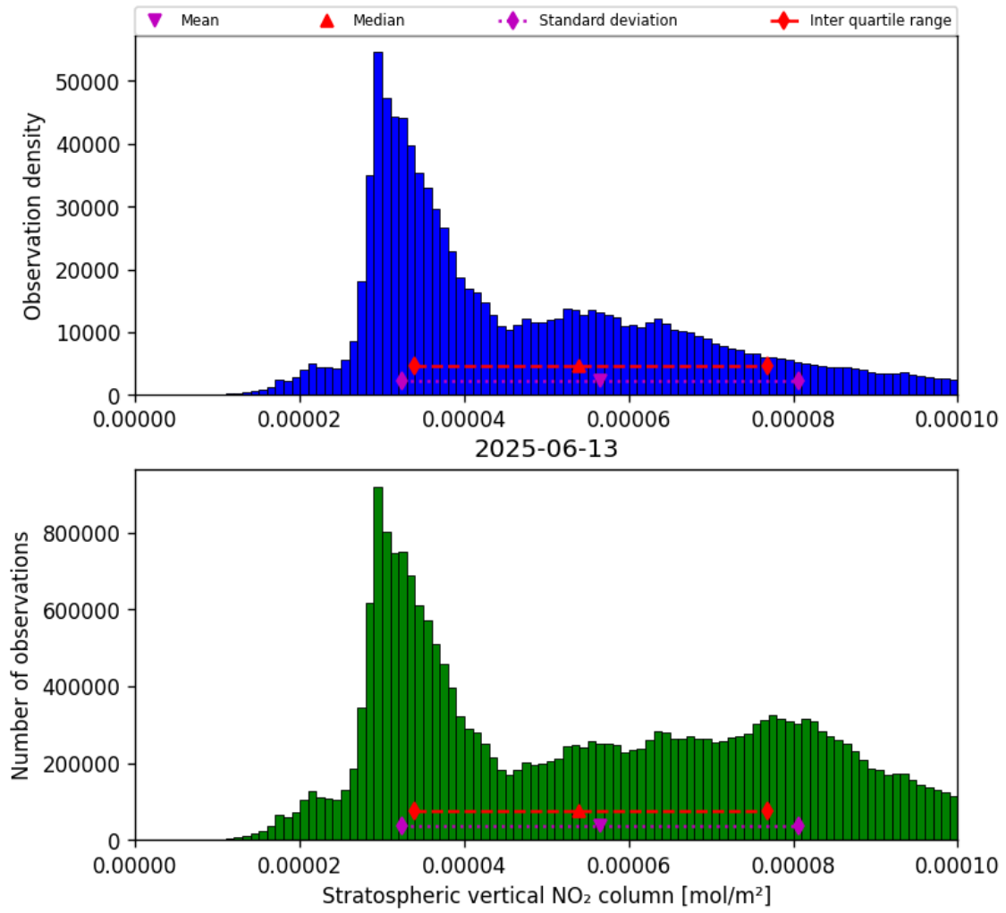
Figure 34: Histogram of “Stratospheric vertical NO 2 column” for 2025-06-13 to 2025-06-14
