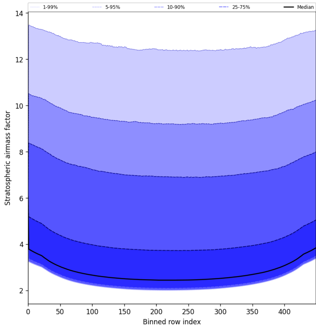
Figure 59: Along track statistics of “Stratospheric airmass factor” for 2025-06-13 to 2025-06-14
