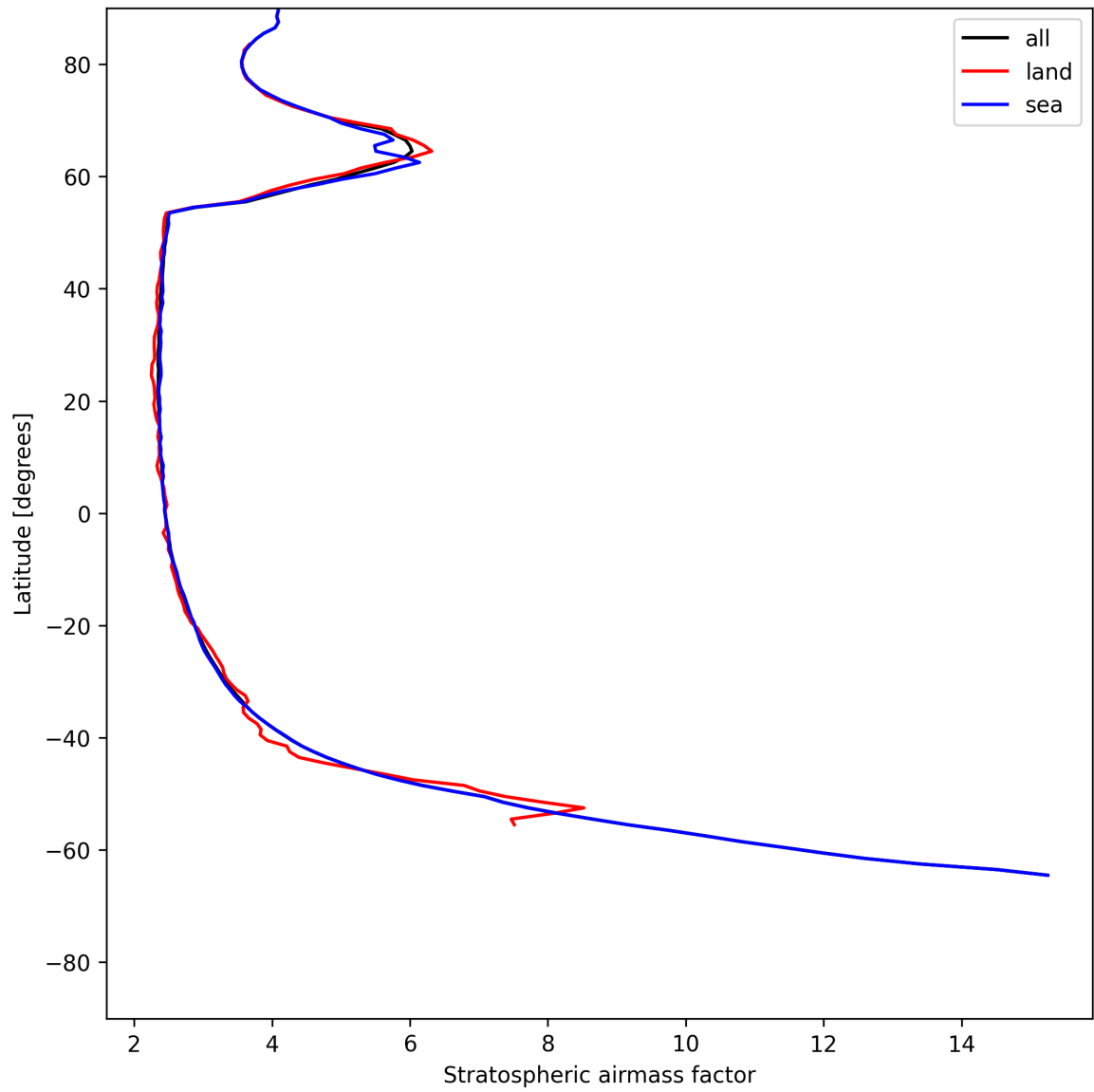
Figure 25: Zonal average of “Stratospheric airmass factor” for 2025-06-13 to 2025-06-14.
