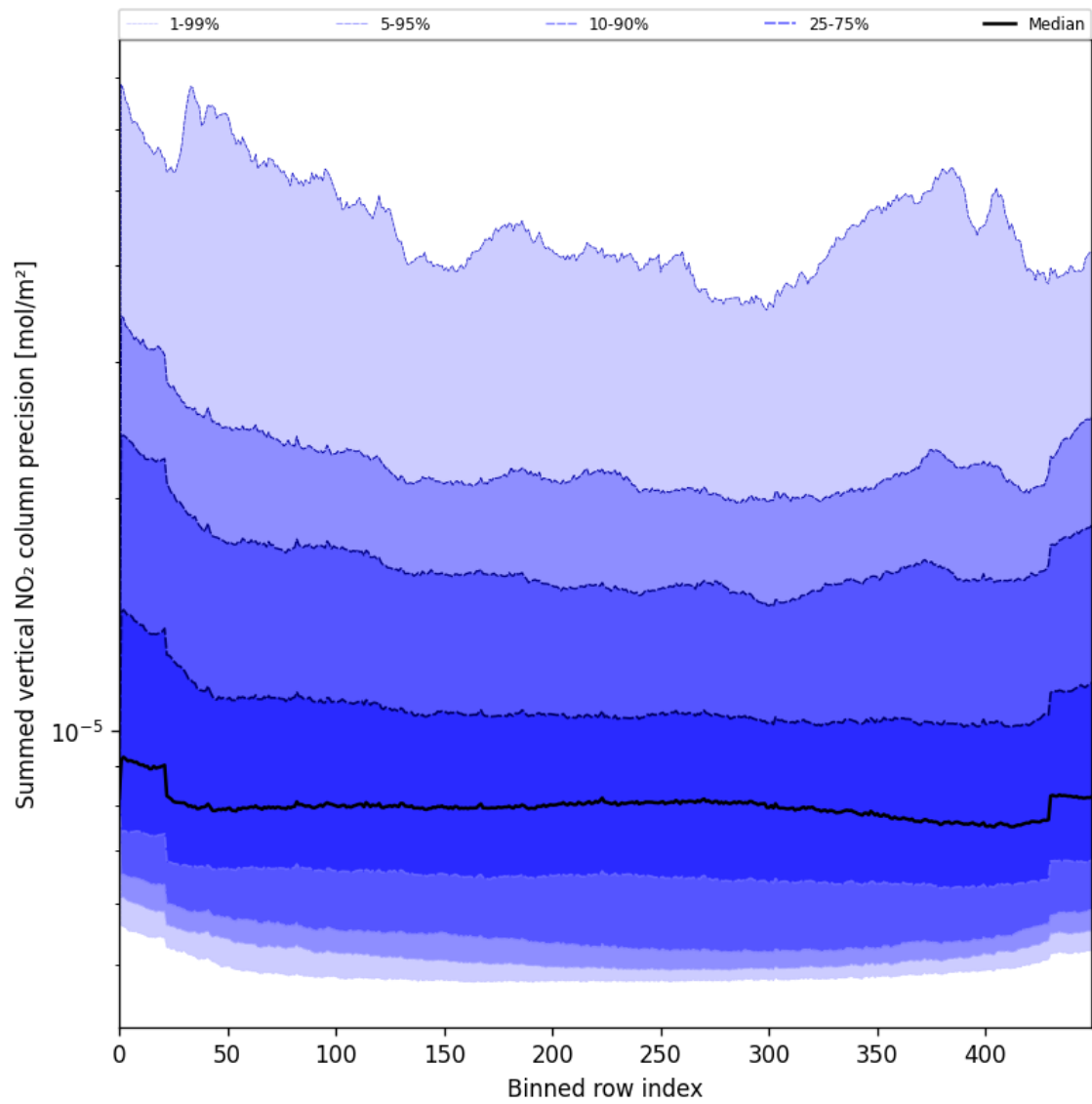
Figure 56: Along track statistics of “Summed vertical NO 2 column precision” for 2025-06-13 to 2025-06-14
