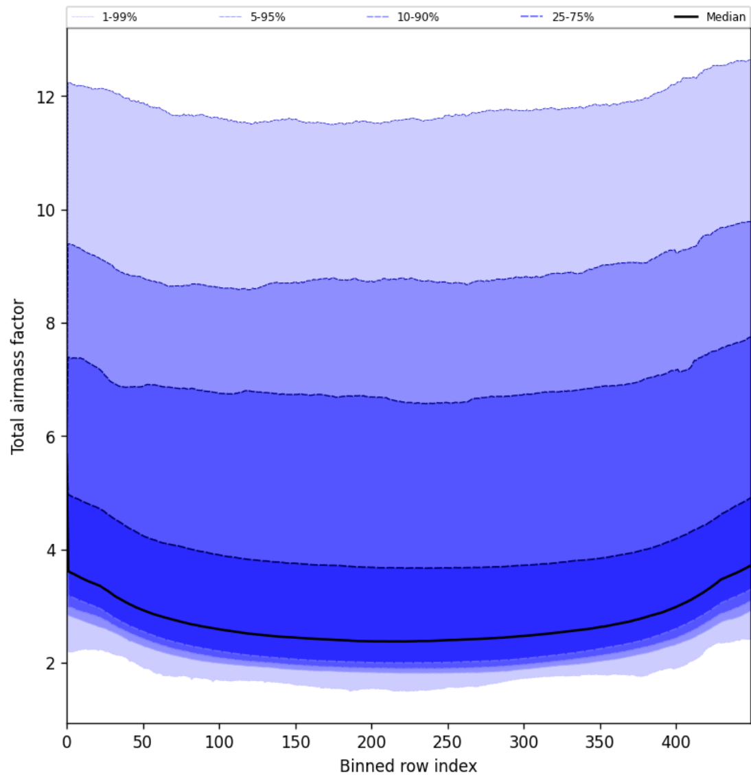
Figure 47: Along track statistics of “Total airmass factor” for 2025-06-13 to 2025-06-14
