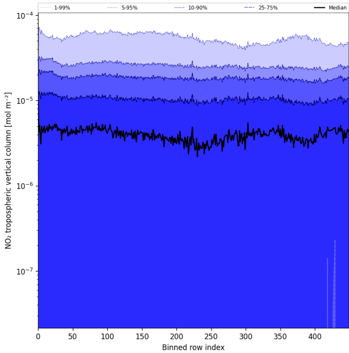
Figure 44: Along track statistics of “NO 2 tropospheric vertical column” for 2025-06-13 to 2025-06-14
