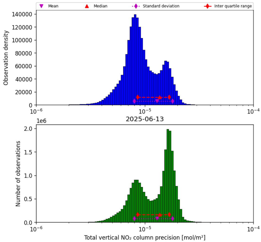
Figure 37: Histogram of “Total vertical NO 2 column precision” for 2025-06-13 to 2025-06-14
