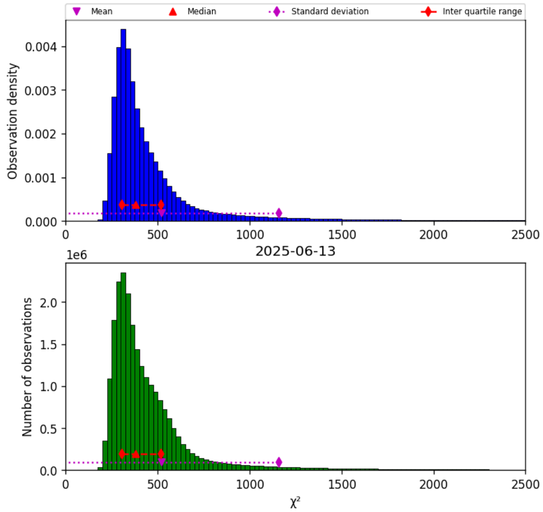
Figure 40: Histogram of “ \chi^2 ” for 2025-06-13 to 2025-06-14
