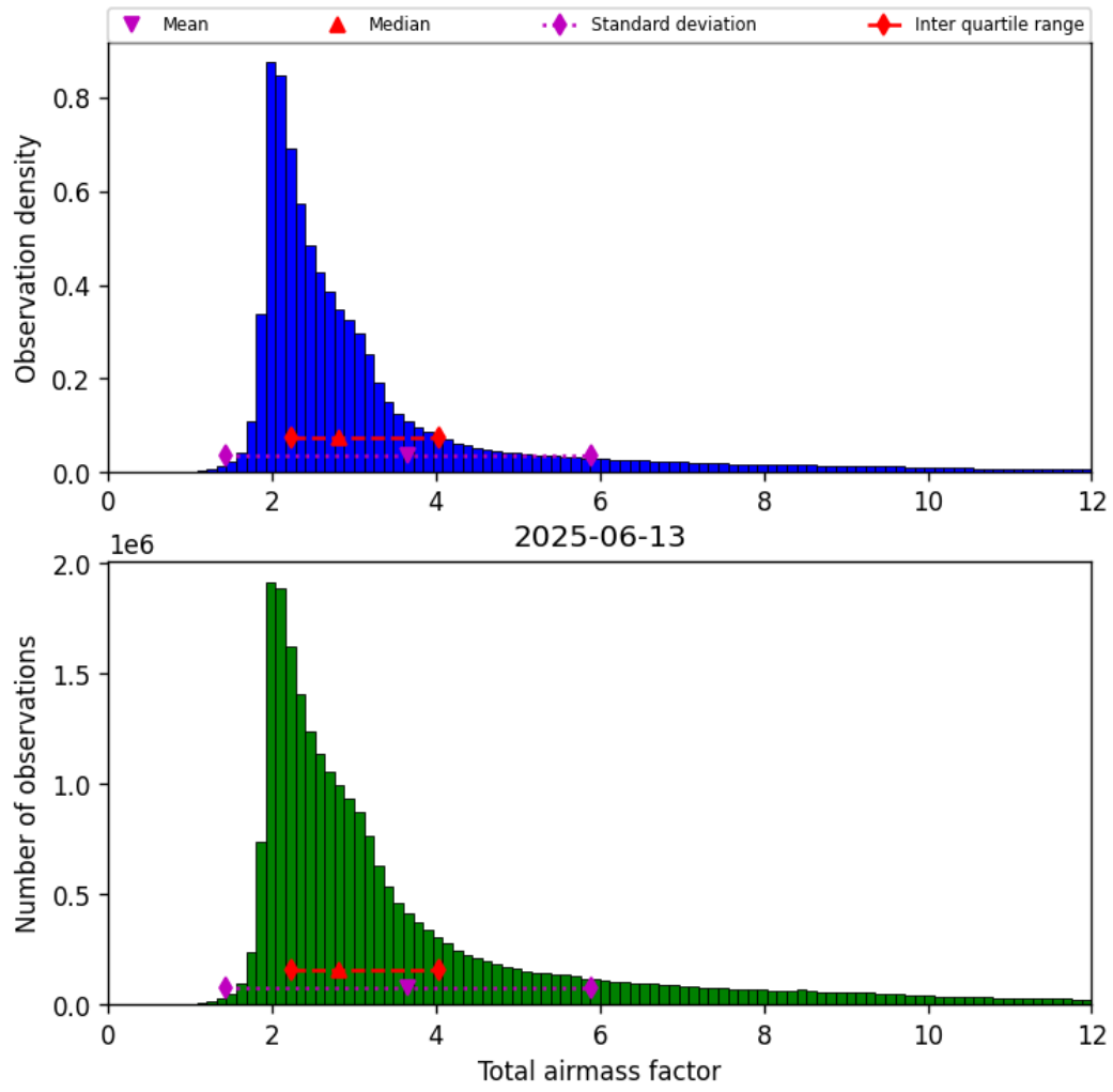
Figure 30: Histogram of “Total airmass factor” for 2025-06-13 to 2025-06-14
