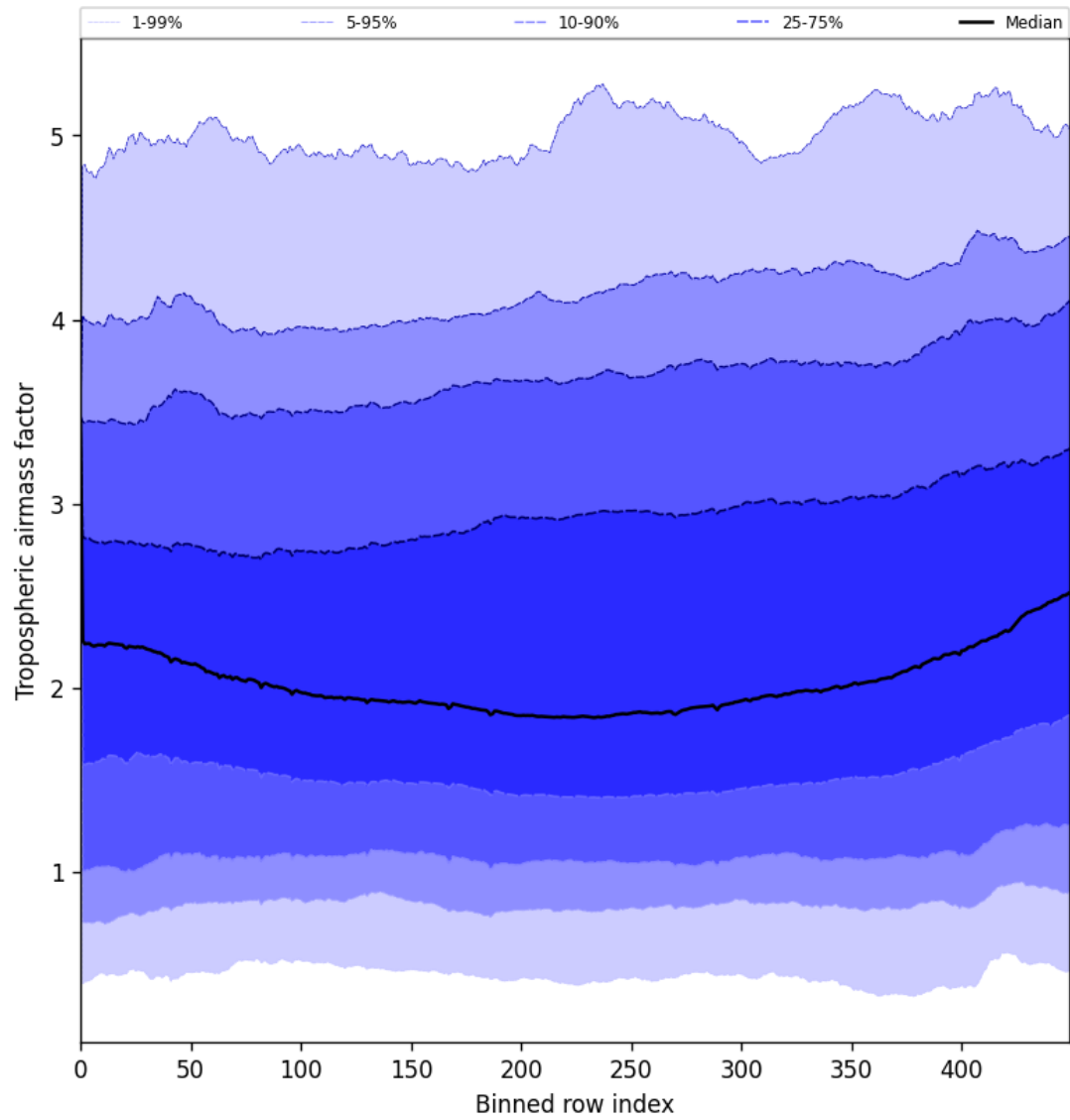
Figure 46: Along track statistics of “Tropospheric airmass factor” for 2025-06-13 to 2025-06-14
