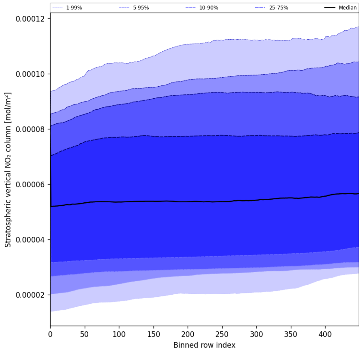
Figure 51: Along track statistics of “Stratospheric vertical NO 2 column” for 2025-06-13 to 2025-06-14
