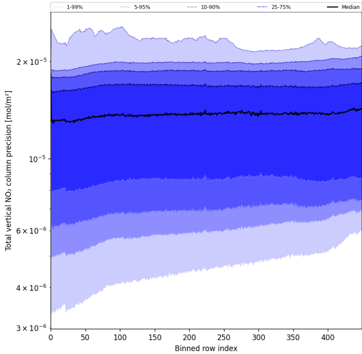
Figure 54: Along track statistics of “Total vertical NO 2 column precision” for 2025-06-13 to 2025-06-14
