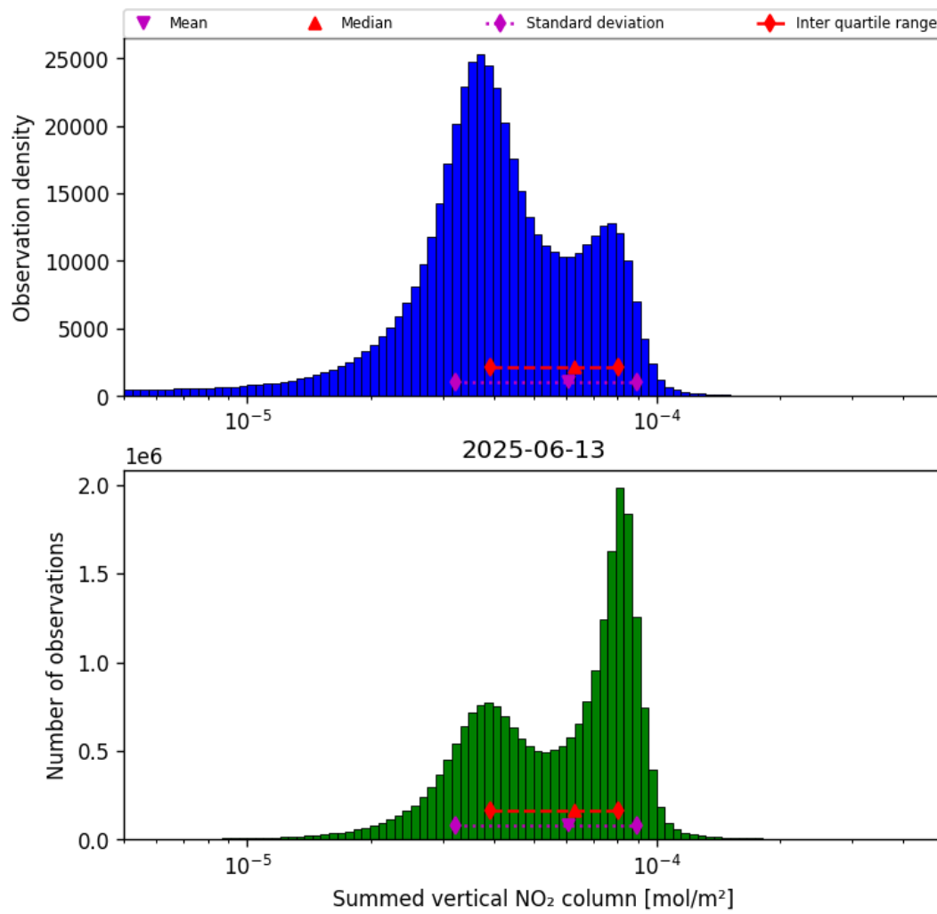
Figure 38: Histogram of "Summed vertical NO 2 column" for 2025-06-13 to 2025-06-14
