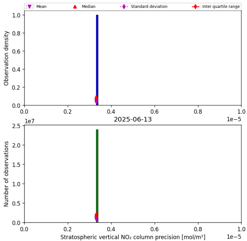
Figure 35: Histogram of “Stratospheric vertical NO 2 column precision” for 2025-06-13 to 2025-06-14
