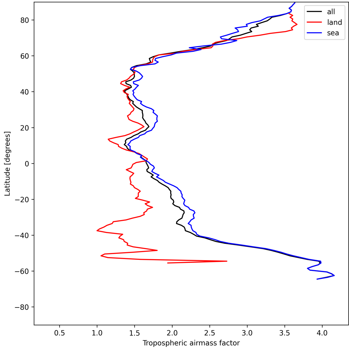
Figure 12: Zonal average of “Tropospheric airmass factor” for 2025-06-13 to 2025-06-14.
