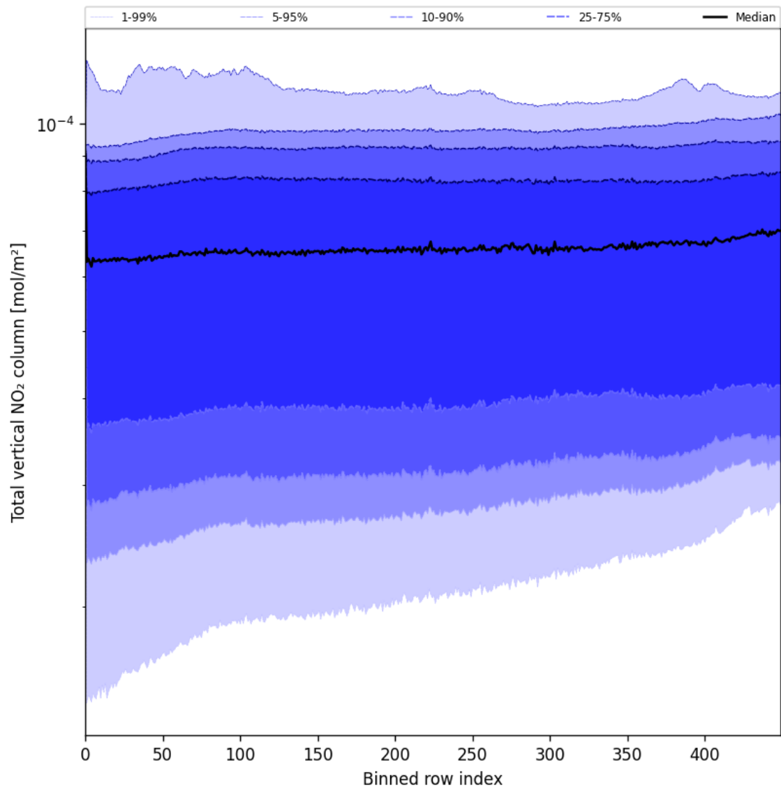
Figure 53: Along track statistics of “Total vertical NO 2 column” for 2025-06-13 to 2025-06-14
