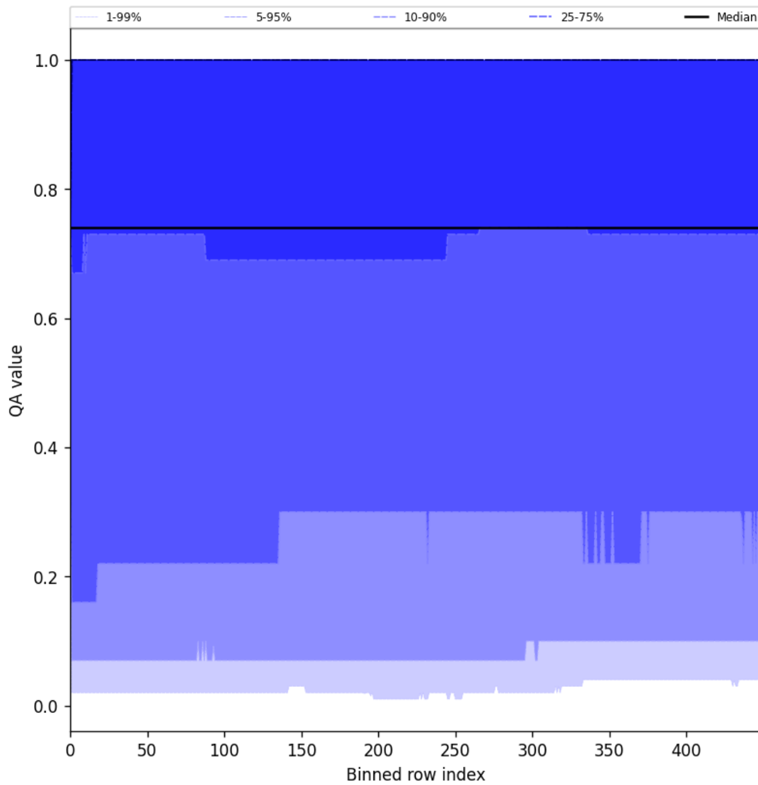
Figure 43: Along track statistics of "QA value" for 2025-06-13 to 2025-06-14
