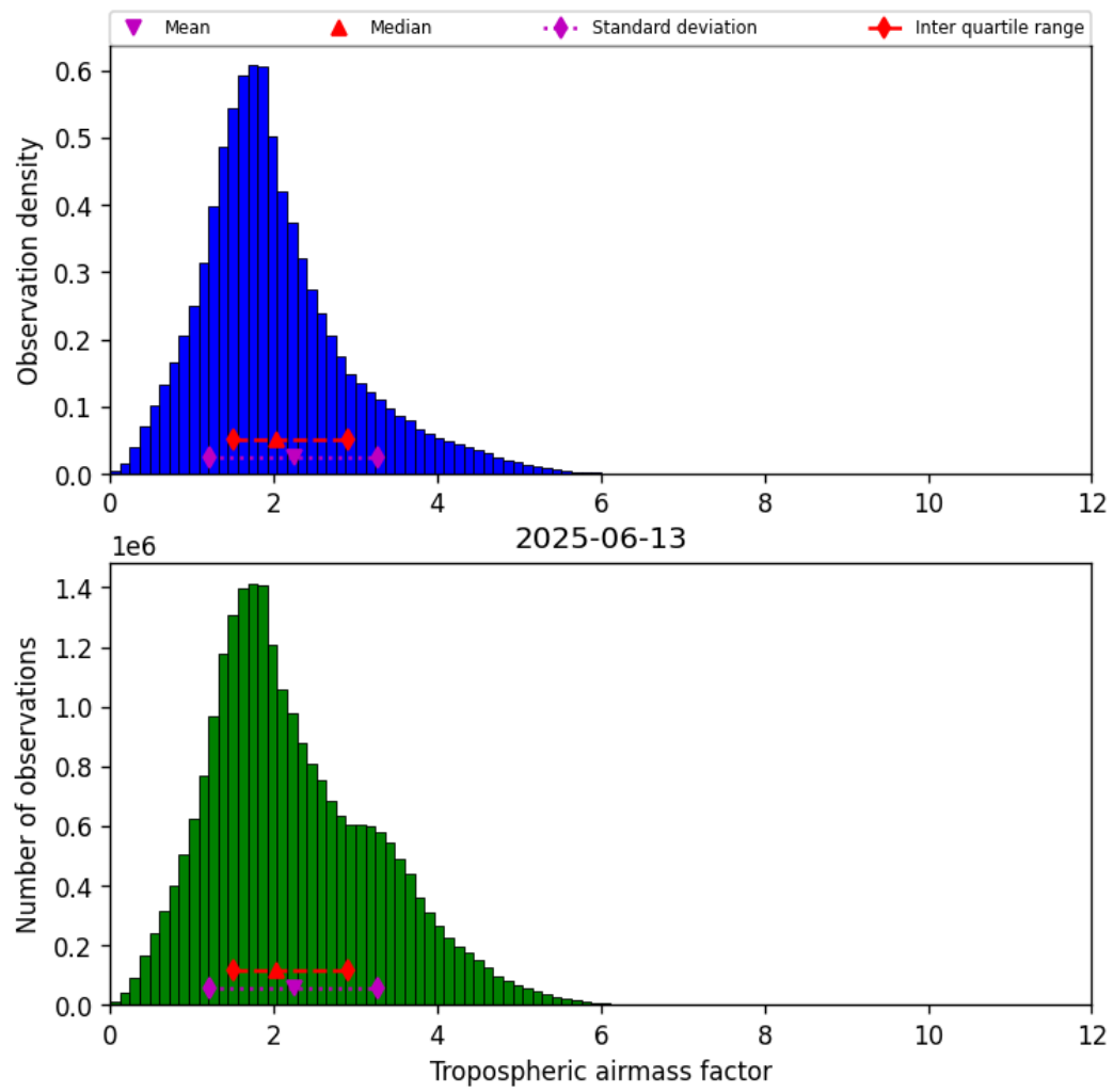
Figure 29: Histogram of “Tropospheric airmass factor” for 2025-06-13 to 2025-06-14
