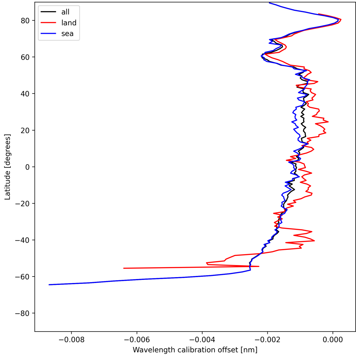
Figure 16: Zonal average of “Wavelength calibration offset” for 2025-06-13 to 2025-06-14.
