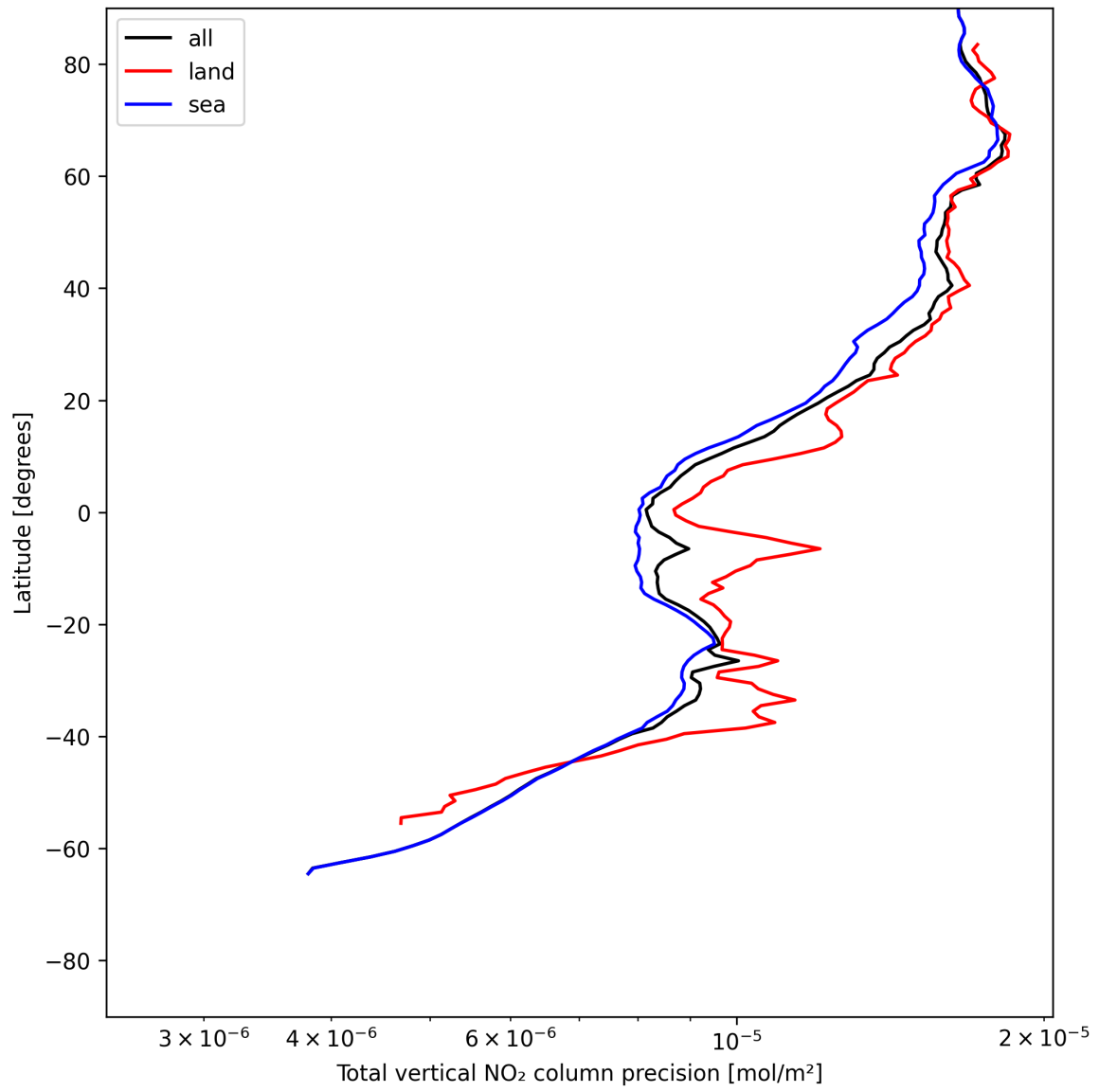
Figure 20: Zonal average of “Total vertical NO 2 column precision” for 2025-06-13 to 2025-06-14.
