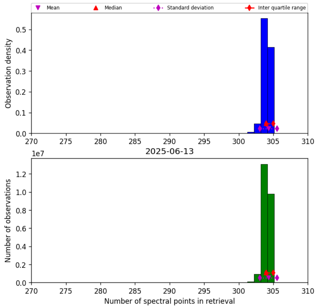
Figure 31: Histogram of “Number of spectral points in retrieval” for 2025-06-13 to 2025-06-14
