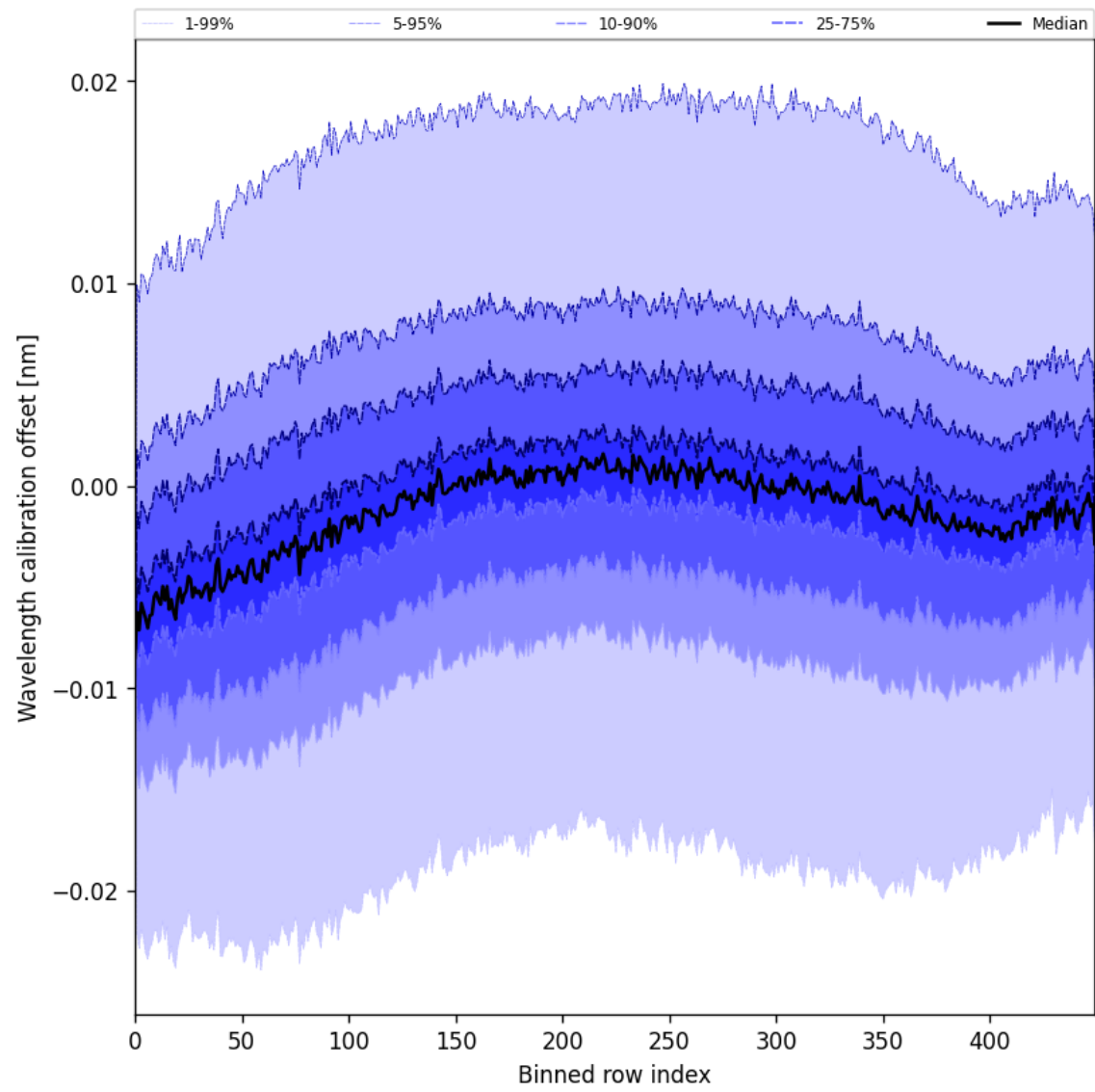
Figure 50: Along track statistics of “Wavelength calibration offset” for 2025-06-13 to 2025-06-14
