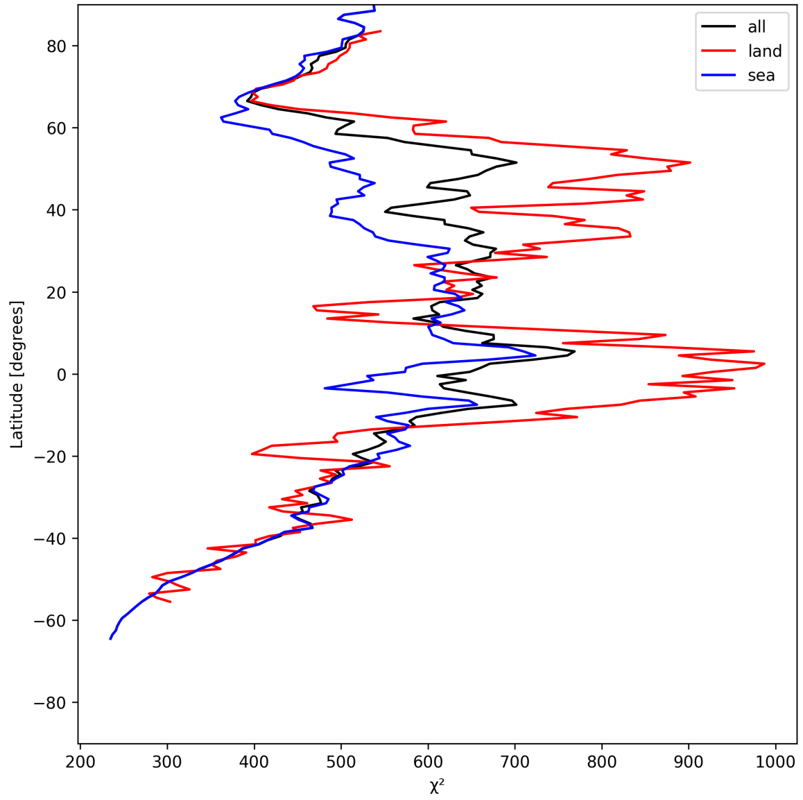
Figure 23: Zonal average of “ \chi^2 ” for 2025-06-13 to 2025-06-14.
