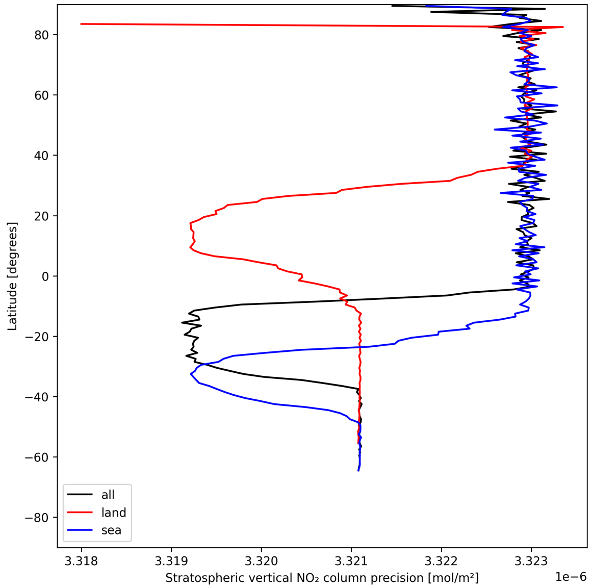
Figure 18: Zonal average of “Stratospheric vertical NO 2 column precision” for 2025-06-13 to 2025-06-14.
