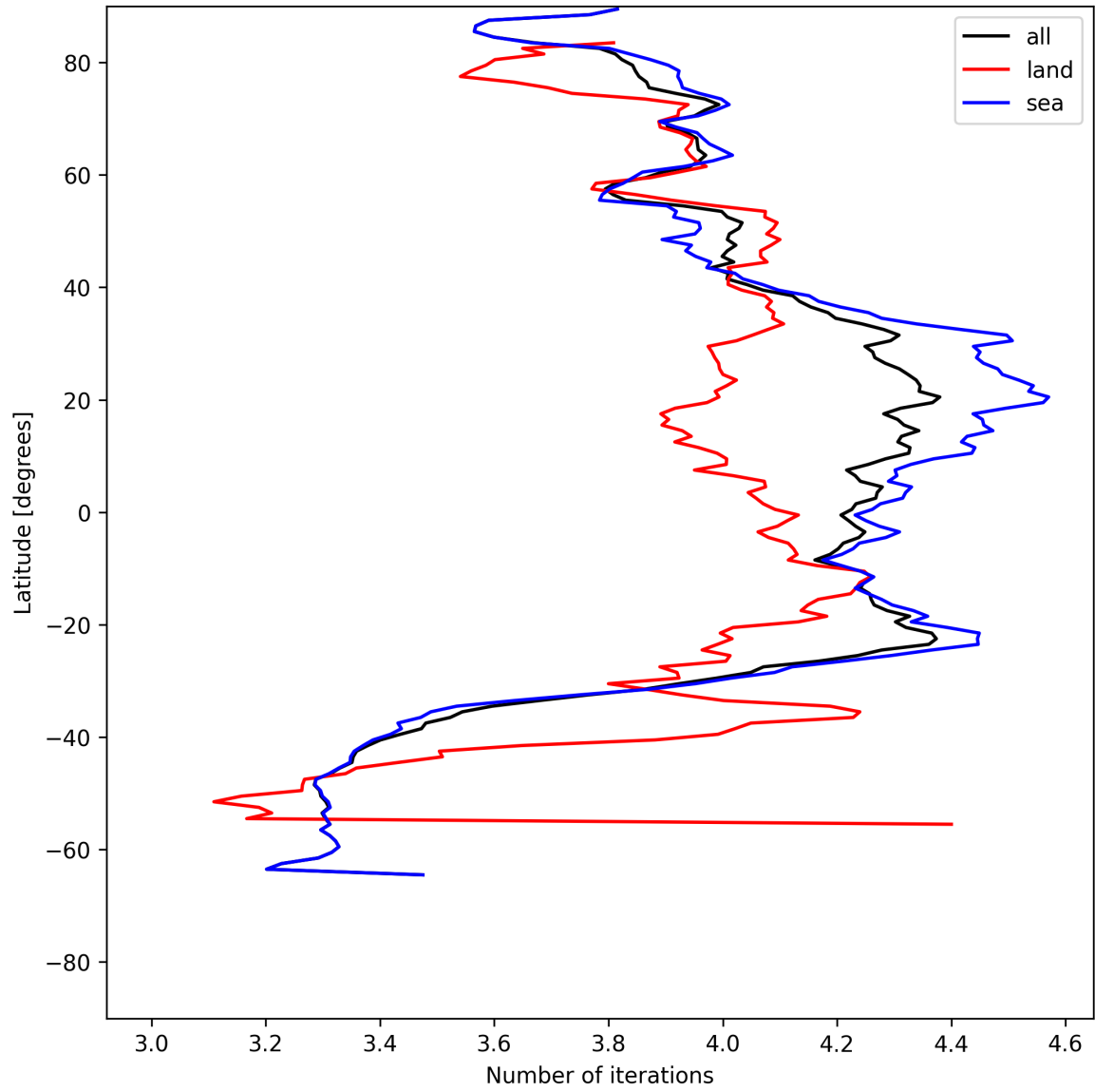
Figure 15: Zonal average of “Number of iterations” for 2025-06-14 to 2025-06-14.
