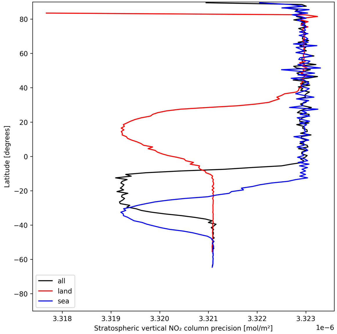
Figure 18: Zonal average of “Stratospheric vertical NO 2 column precision” for 2025-06-14 to 2025-06-14.
