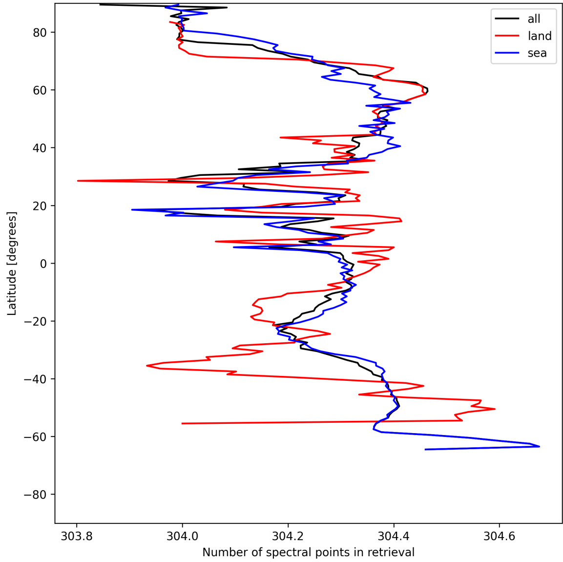
Figure 14: Zonal average of “Number of spectral points in retrieval” for 2025-06-14 to 2025-06-14.
