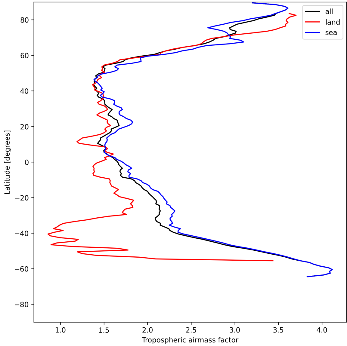
Figure 12: Zonal average of “Tropospheric airmass factor” for 2025-06-14 to 2025-06-14.
