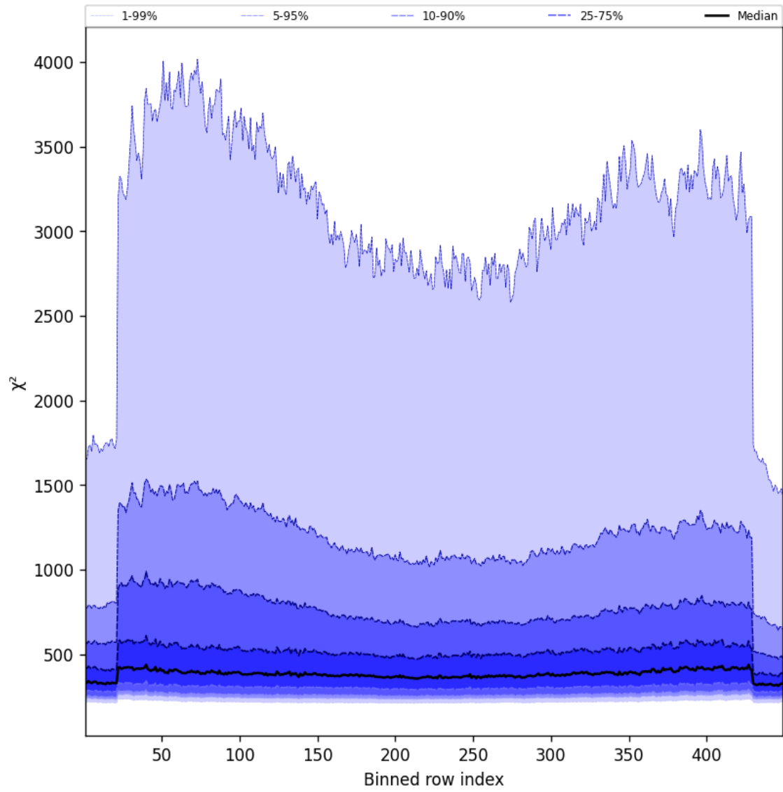
Figure 57: Along track statistics of “ \chi^2 ” for 2025-06-14 to 2025-06-14
