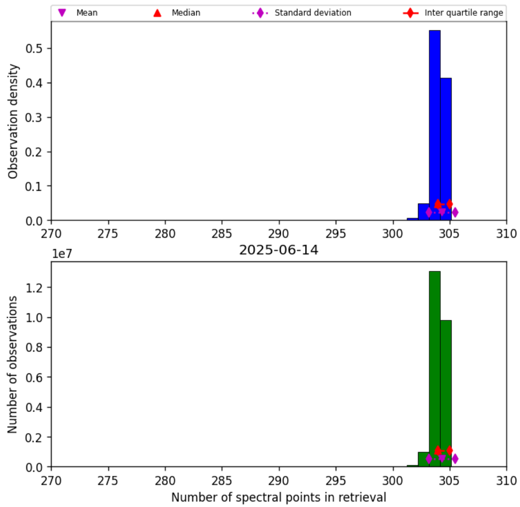
Figure 31: Histogram of “Number of spectral points in retrieval” for 2025-06-14 to 2025-06-14
