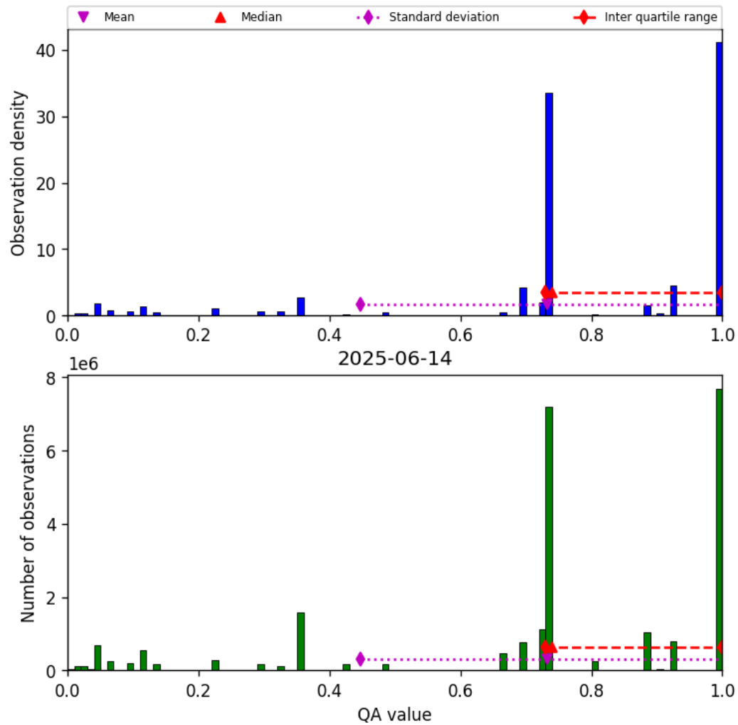
Figure 26: Histogram of “QA value” for 2025-06-14 to 2025-06-14
