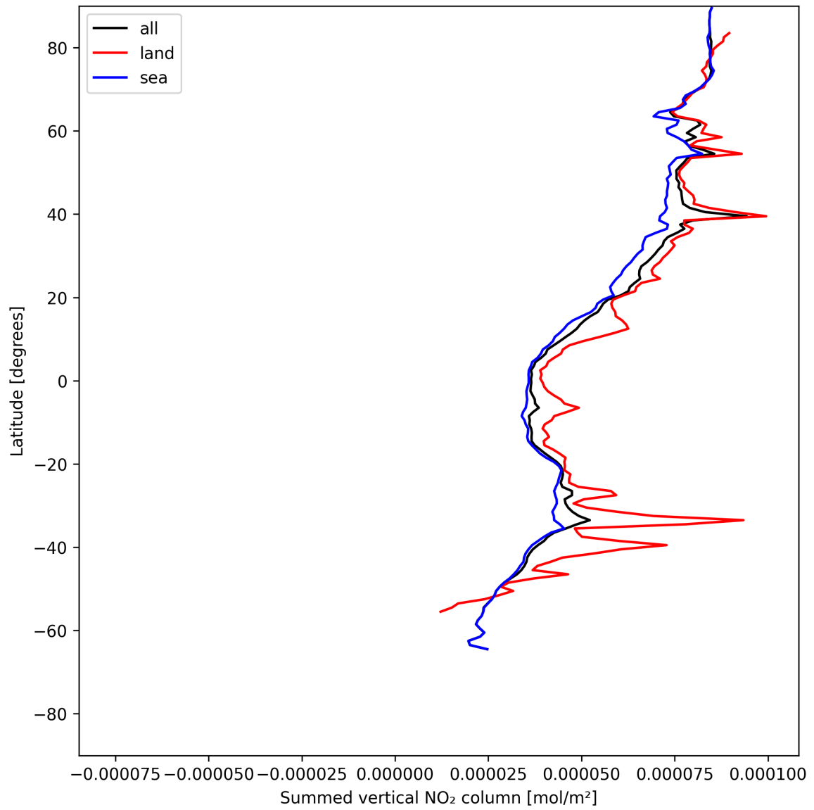
Figure 21: Zonal average of “Summed vertical NO 2 column” for 2025-06-14 to 2025-06-14.
