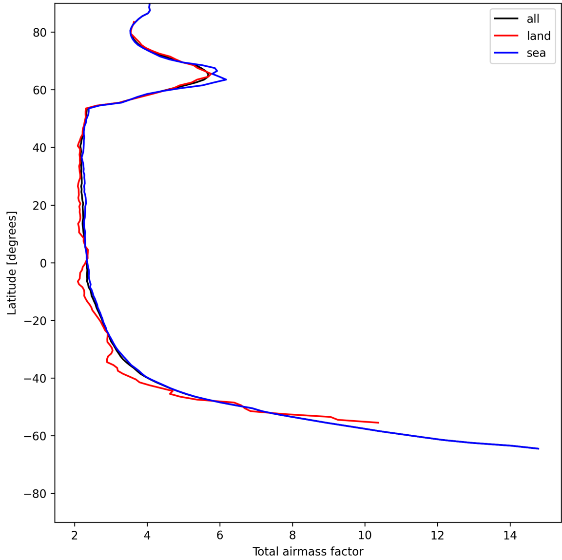
Figure 13: Zonal average of “Total airmass factor” for 2025-06-14 to 2025-06-14.
