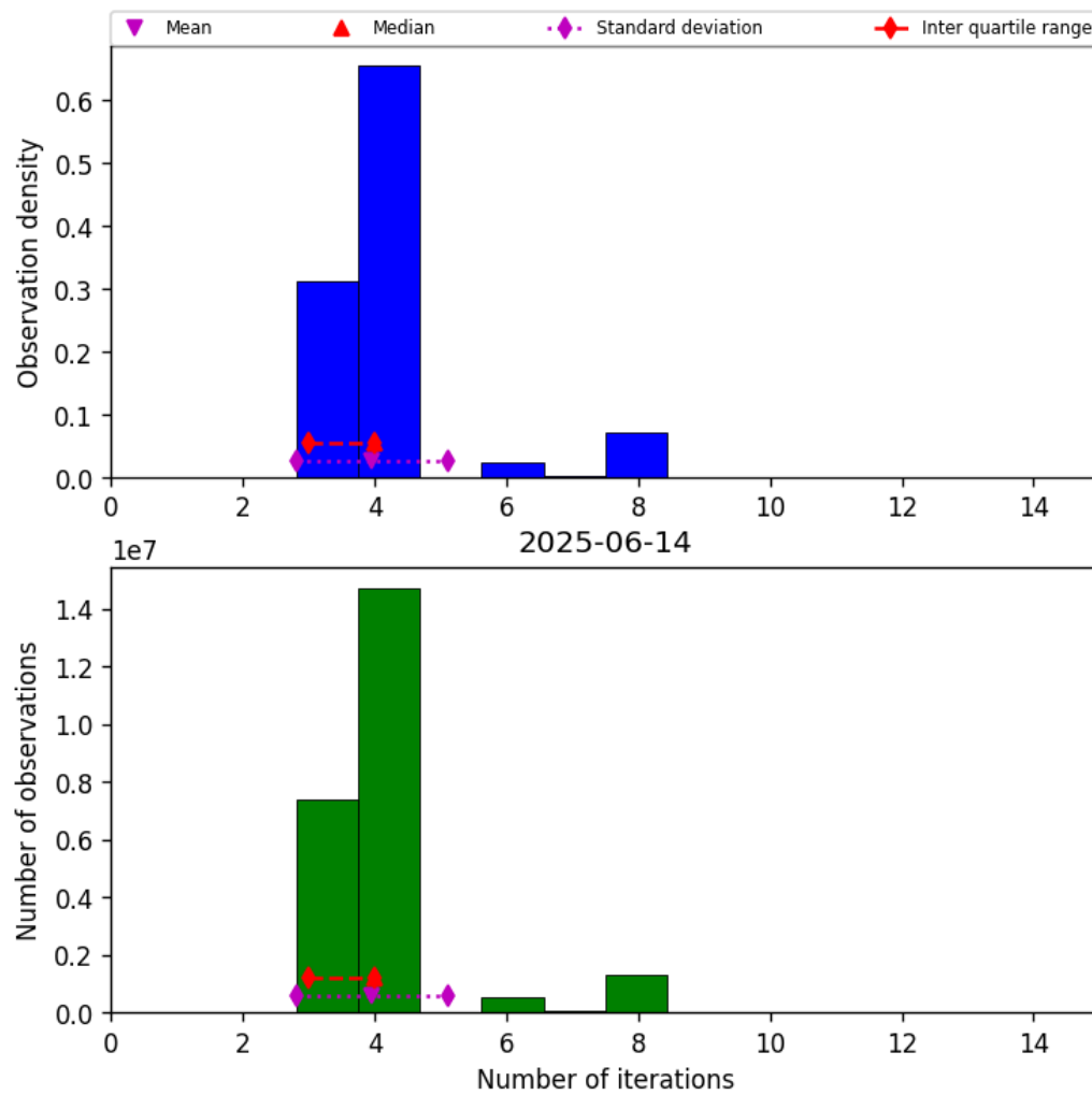
Figure 32: Histogram of “Number of iterations” for 2025-06-14 to 2025-06-14
