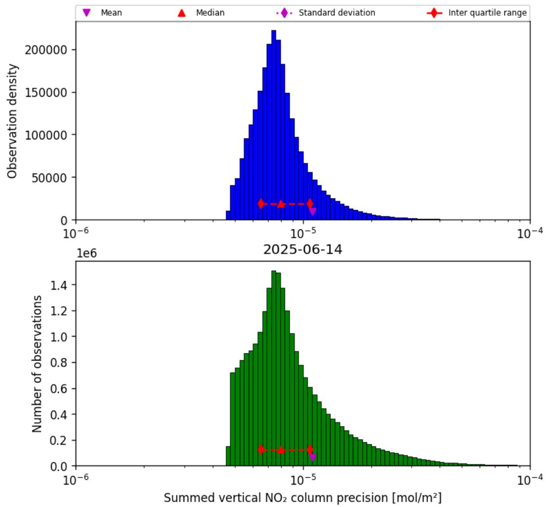
Figure 39: Histogram of "Summed vertical NO 2 column precision" for 2025-06-14 to 2025-06-14
