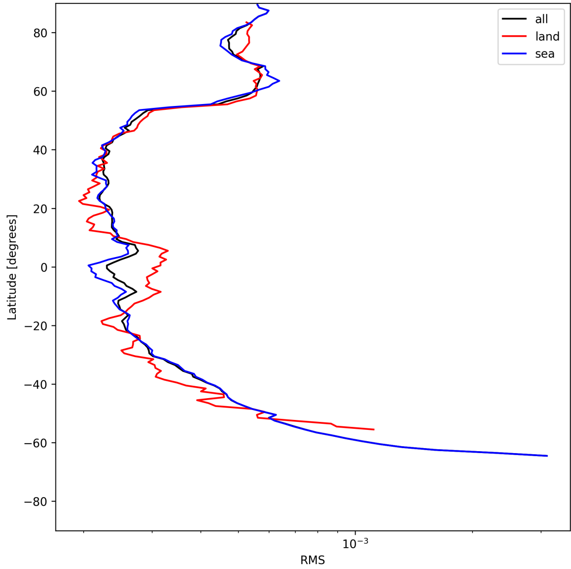
Figure 24: Zonal average of “RMS” for 2025-06-14 to 2025-06-14.
