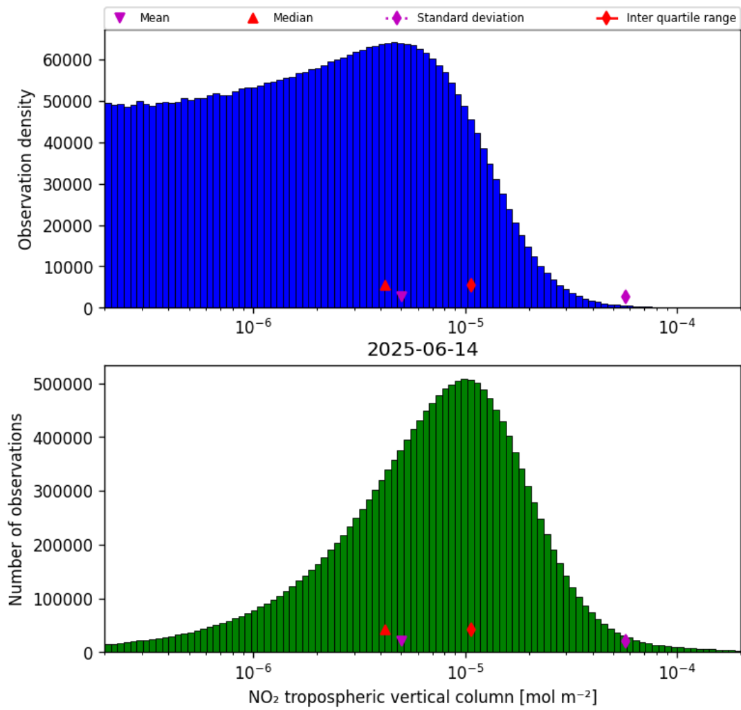
Figure 27: Histogram of “NO 2 tropospheric vertical column” for 2025-06-14 to 2025-06-14
