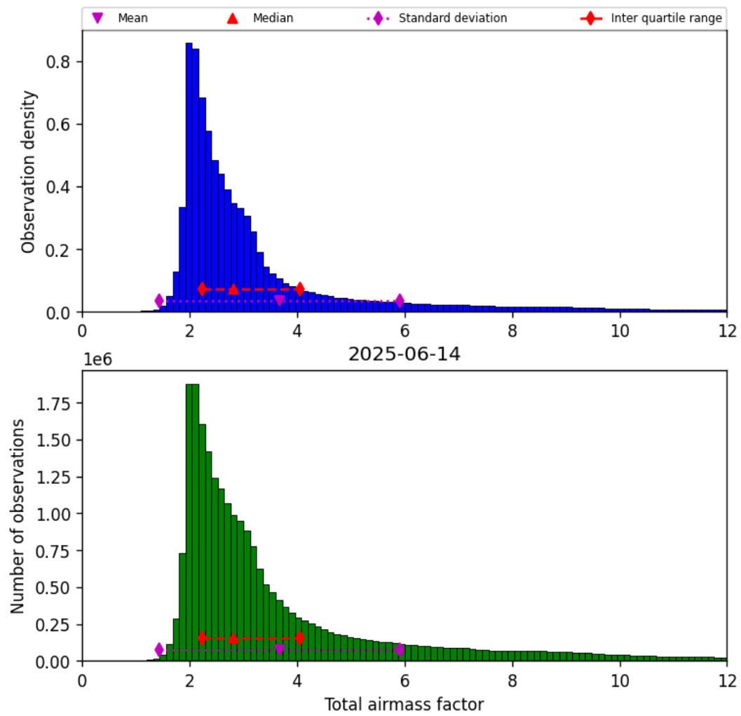
Figure 30: Histogram of “Total airmass factor” for 2025-06-14 to 2025-06-14
