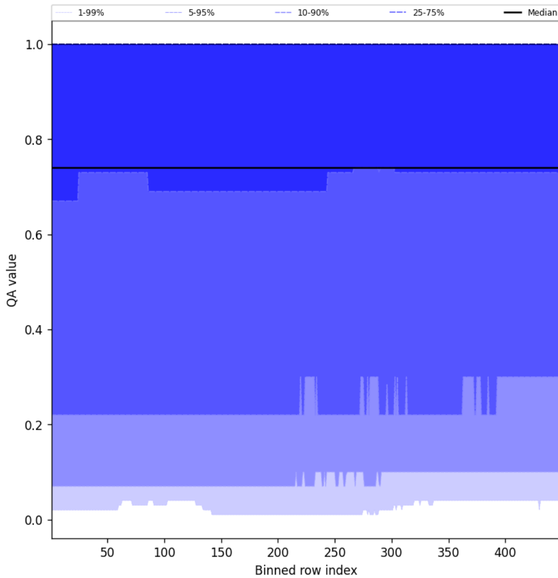
Figure 43: Along track statistics of “QA value” for 2025-06-14 to 2025-06-14
