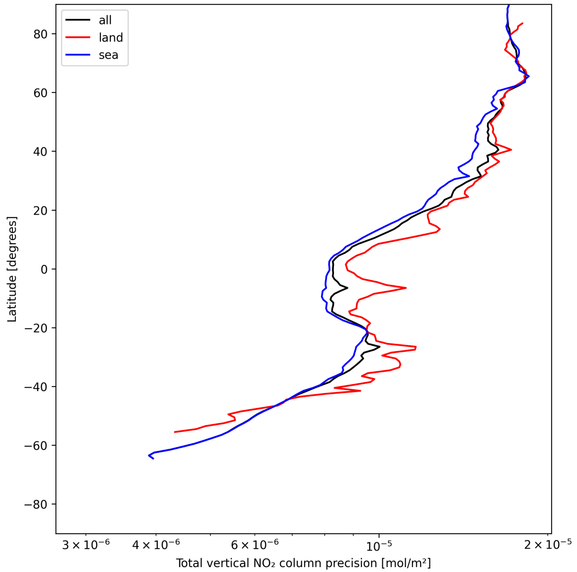
Figure 20: Zonal average of “Total vertical NO 2 column precision” for 2025-06-14 to 2025-06-14.
