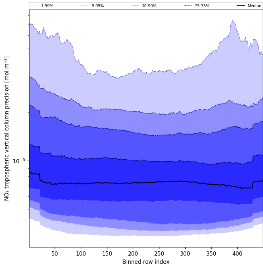
Figure 45: Along track statistics of “NO 2 tropospheric vertical column precision” for 2025-06-14 to 2025-06-14
