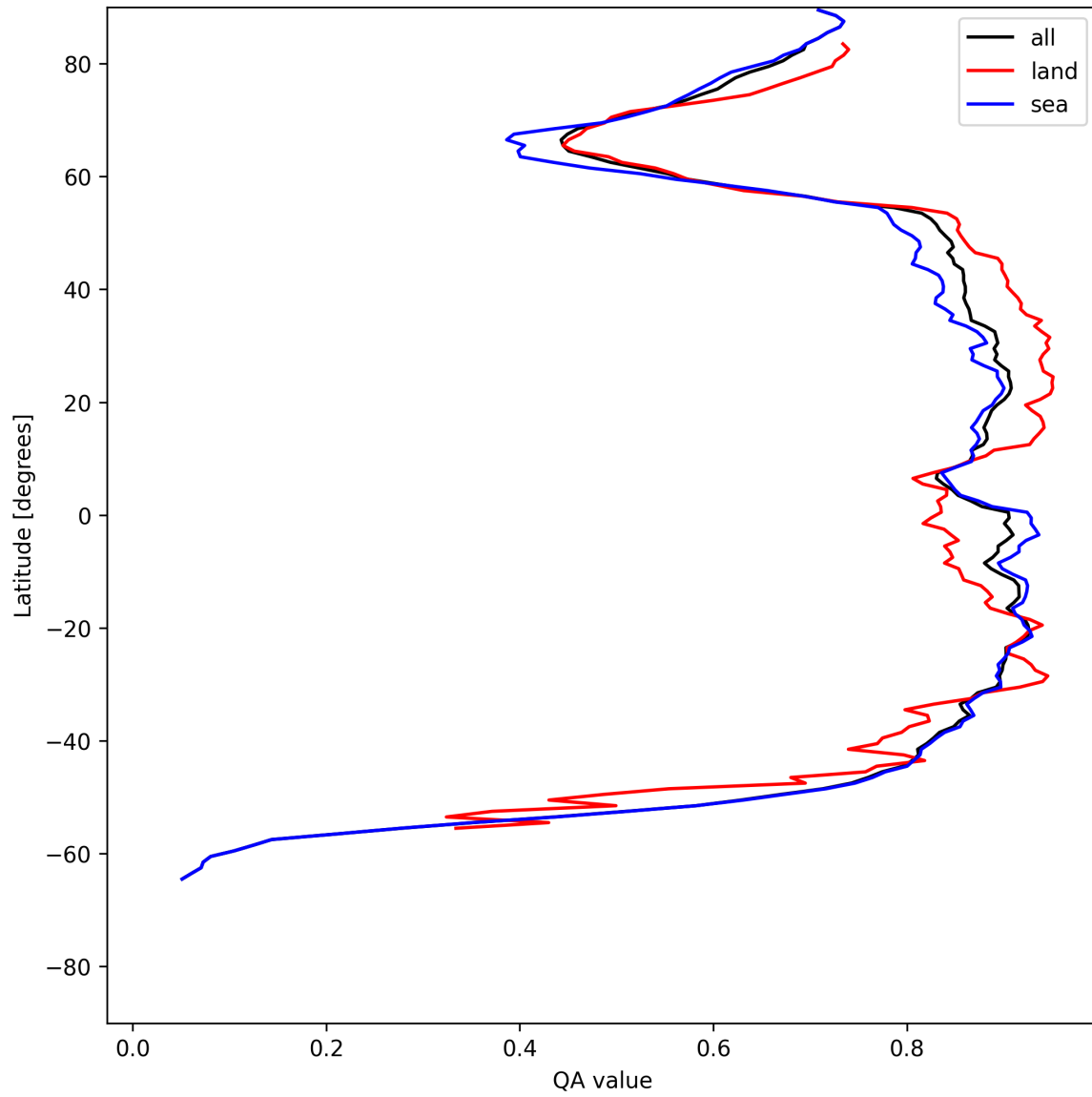
Figure 9: Zonal average of “QA value” for 2025-06-14 to 2025-06-14.
