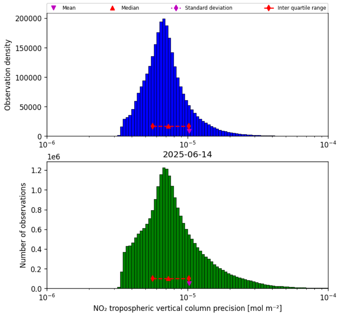
Figure 28: Histogram of "NO 2 tropospheric vertical column precision" for 2025-06-14 to 2025-06-14
