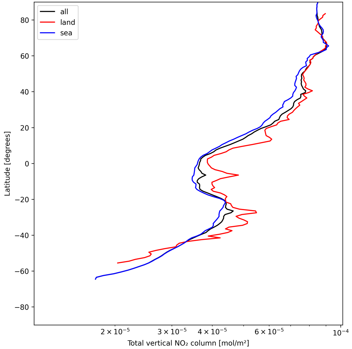
Figure 19: Zonal average of “Total vertical NO 2 column” for 2025-06-14 to 2025-06-14.
