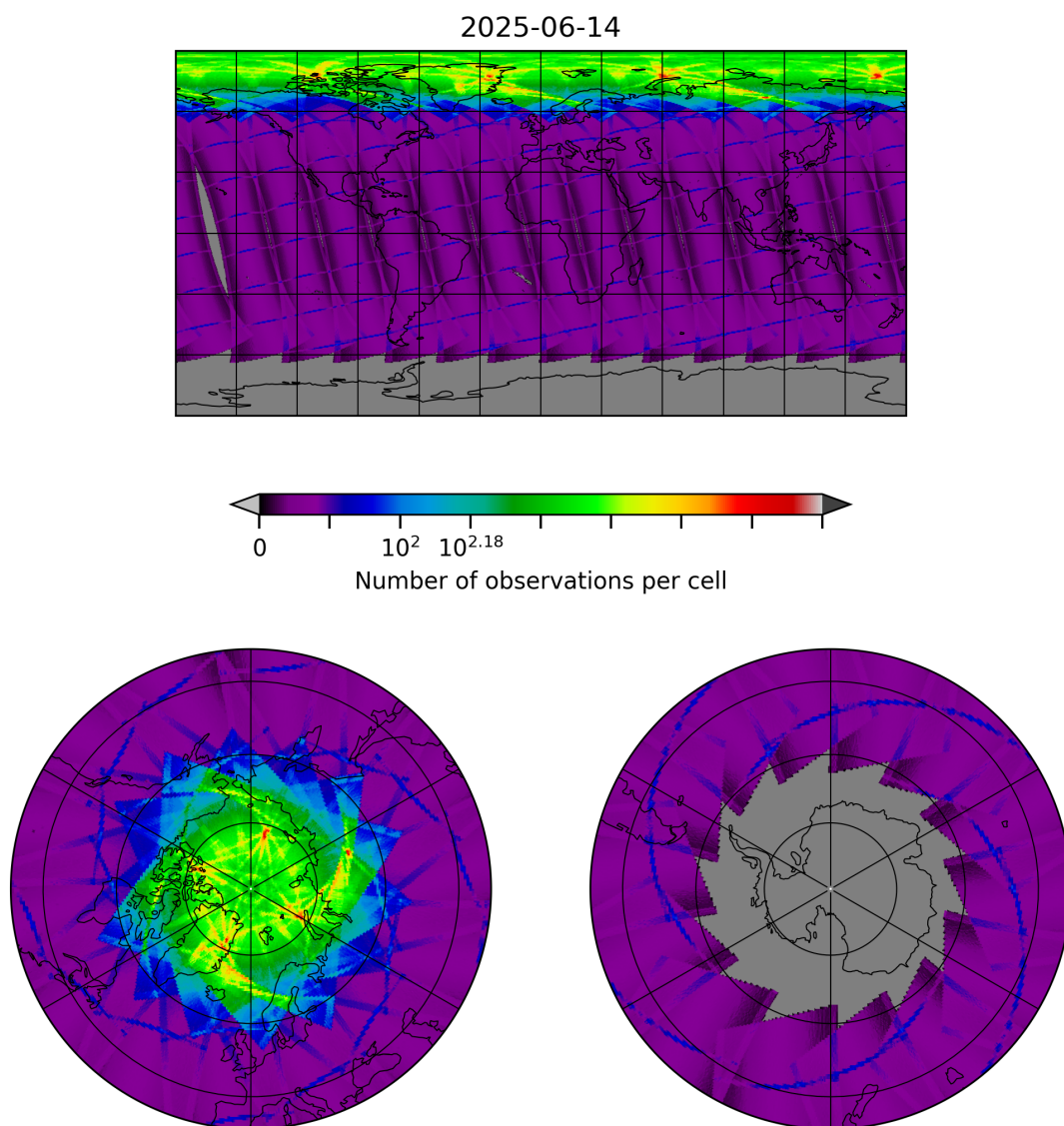
Figure 8: Map of the number of observations for 2025-06-14 to 2025-06-14
