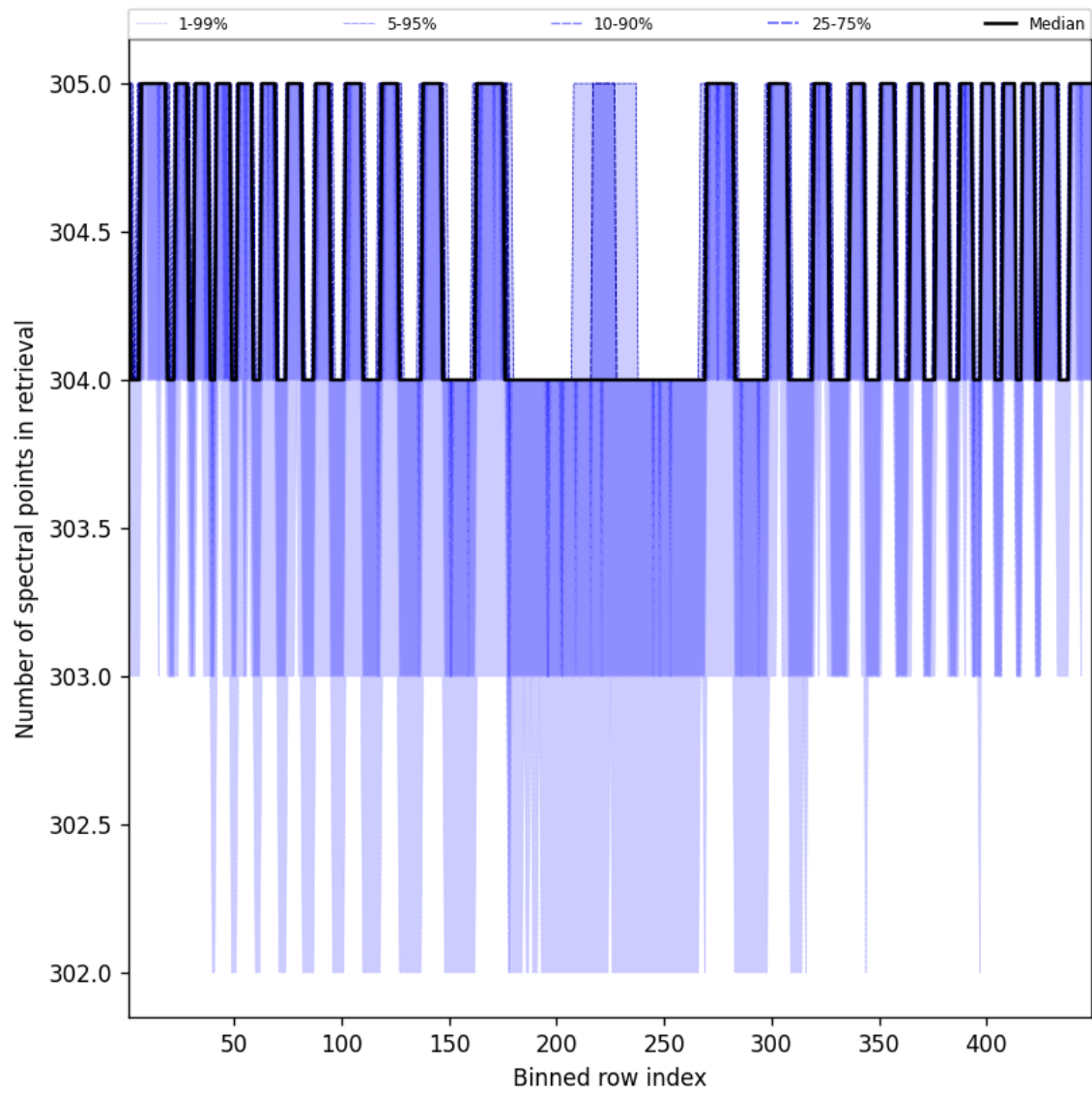
Figure 48: Along track statistics of “Number of spectral points in retrieval” for 2025-06-14 to 2025-06-14
