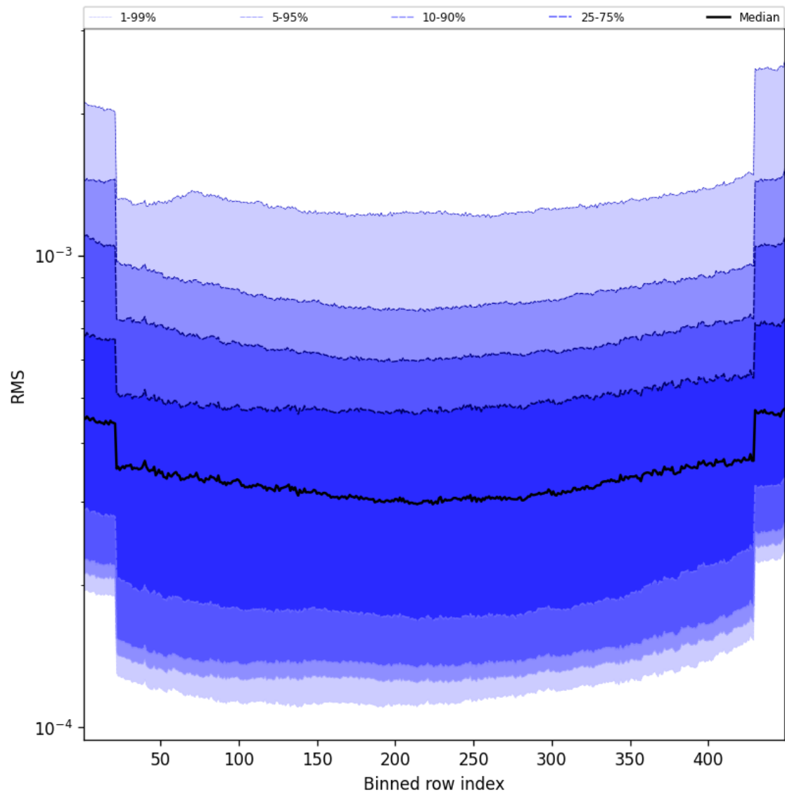
Figure 58: Along track statistics of “RMS” for 2025-06-14 to 2025-06-14
