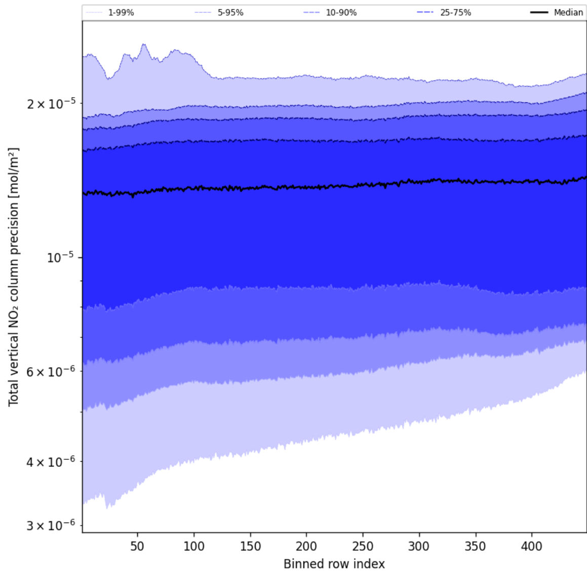
Figure 54: Along track statistics of "Total vertical NO 2 column precision" for 2025-06-14 to 2025-06-14
