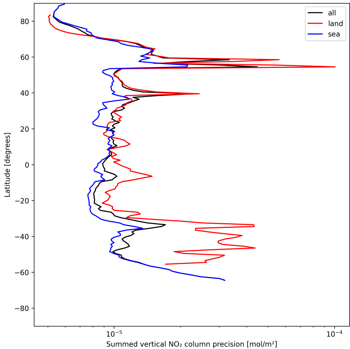
Figure 22: Zonal average of “Summed vertical NO 2 column precision” for 2025-06-14 to 2025-06-14.
