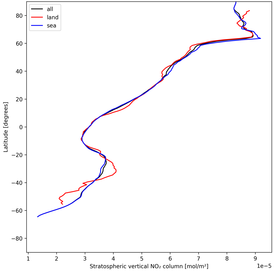
Figure 17: Zonal average of “Stratospheric vertical NO 2 column” for 2025-06-14 to 2025-06-14.
