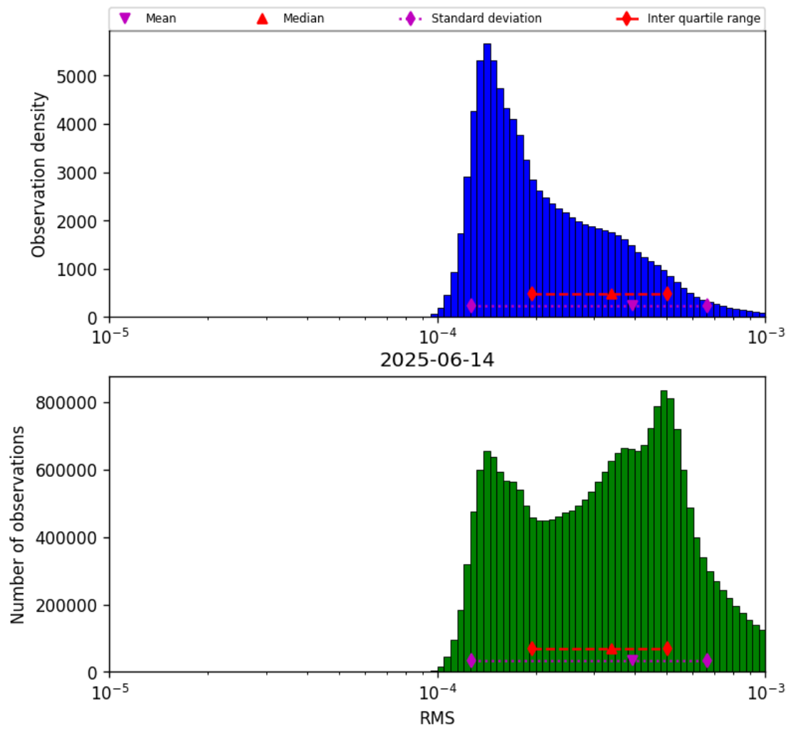
Figure 41: Histogram of “RMS” for 2025-06-14 to 2025-06-14
