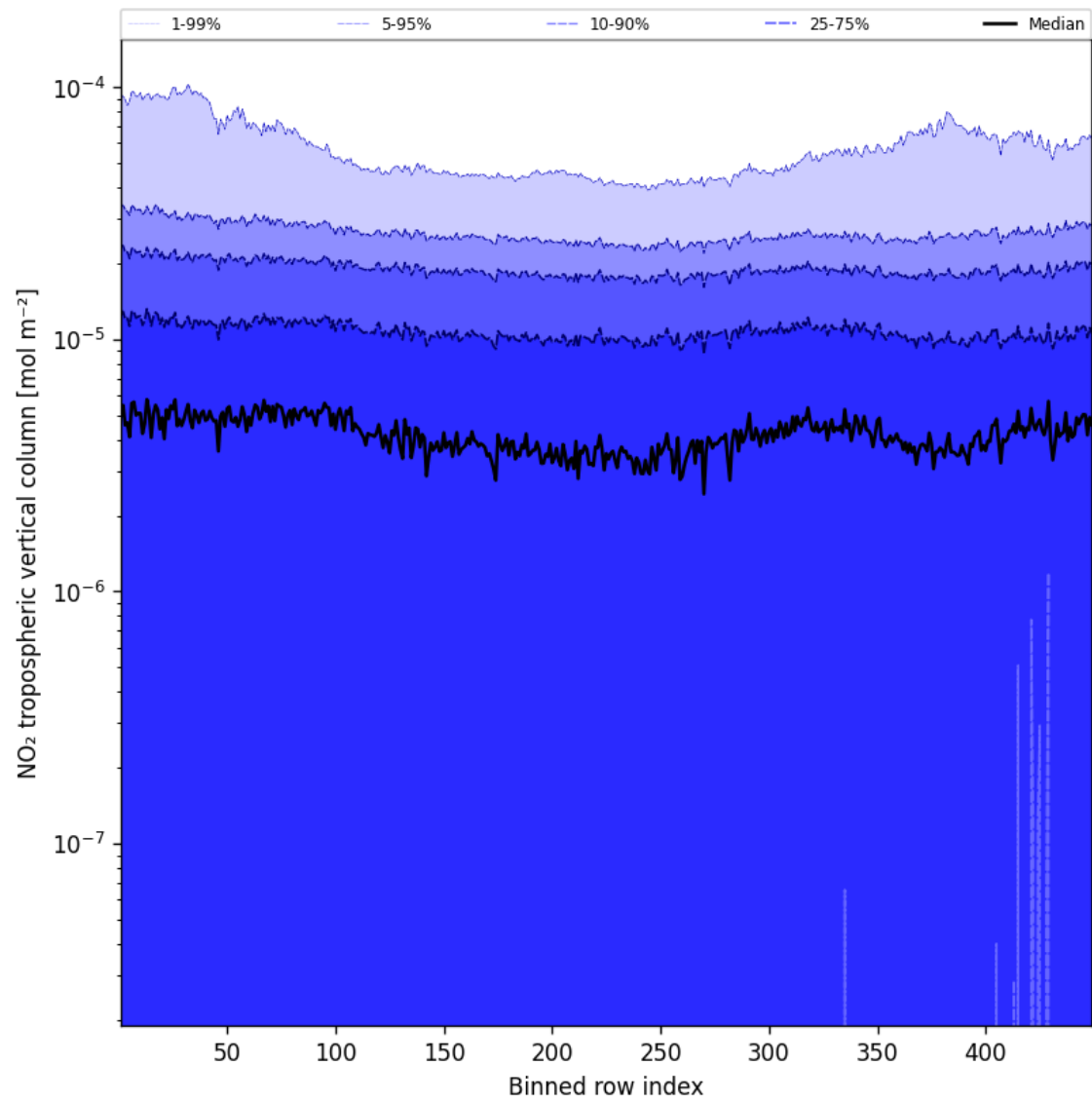
Figure 44: Along track statistics of “NO 2 tropospheric vertical column” for 2025-06-14 to 2025-06-14
