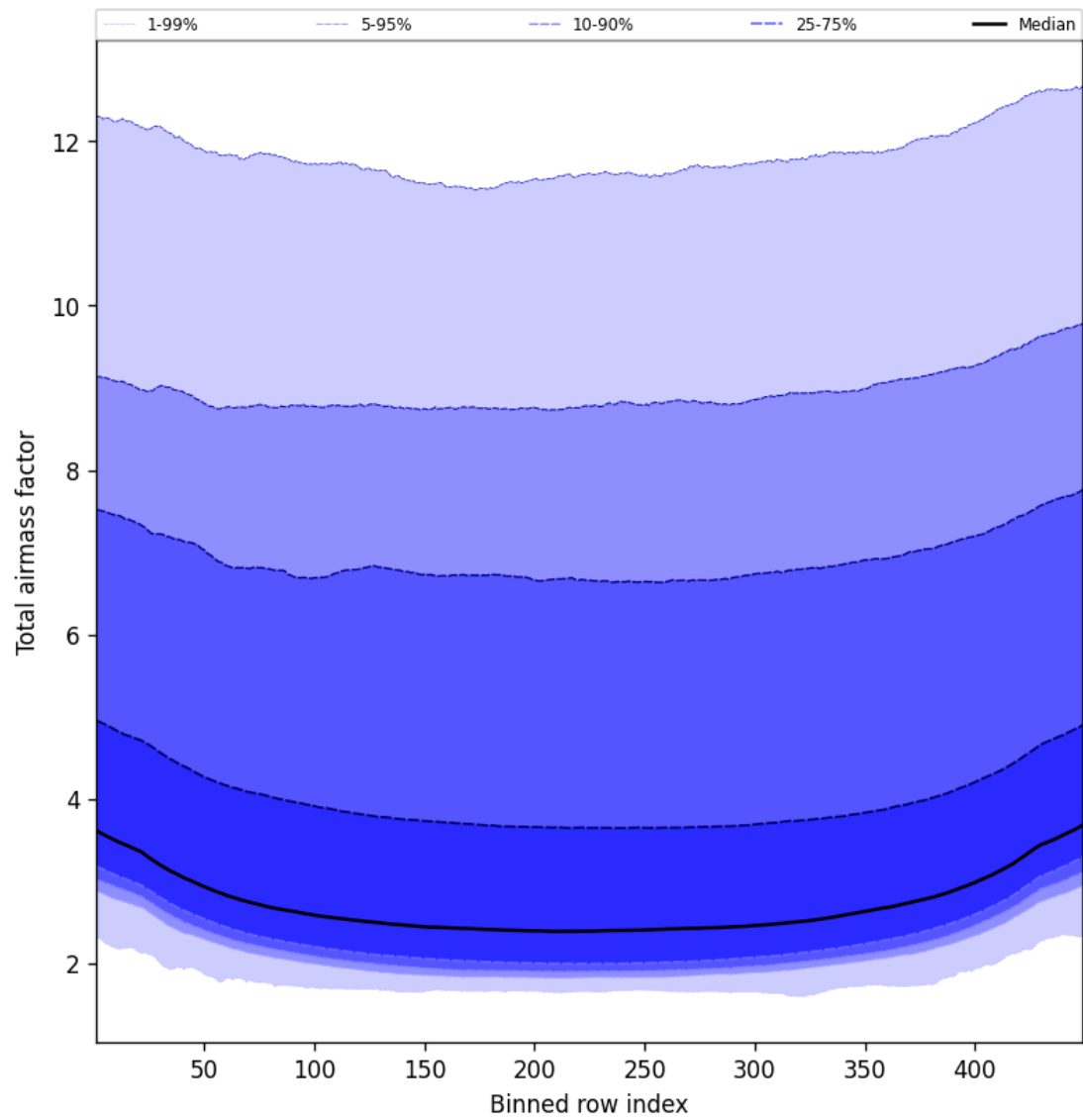
Figure 47: Along track statistics of “Total airmass factor” for 2025-06-14 to 2025-06-14
