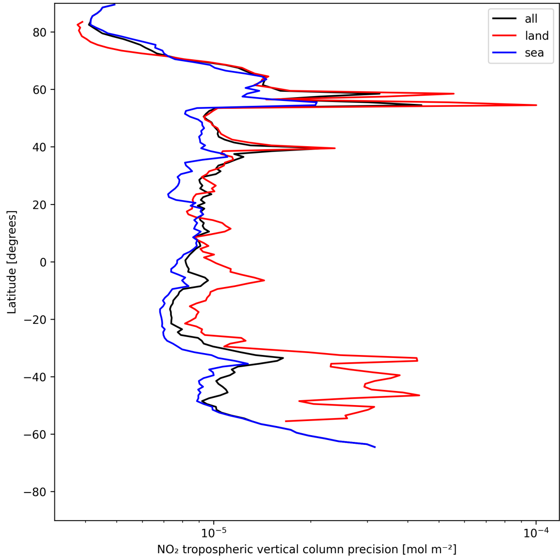
Figure 11: Zonal average of “NO 2 tropospheric vertical column precision” for 2025-06-14 to 2025-06-14.
