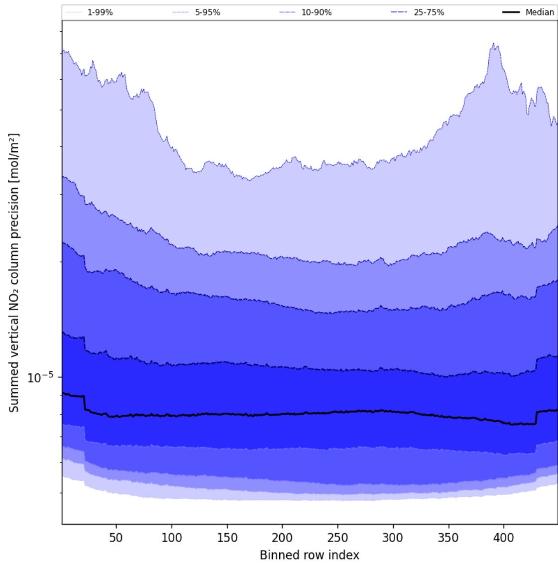
Figure 56: Along track statistics of “Summed vertical NO 2 column precision” for 2025-06-14 to 2025-06-14
