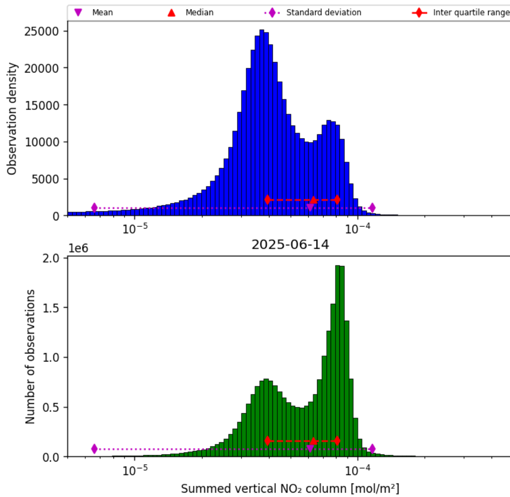
Figure 38: Histogram of "Summed vertical NO 2 column" for 2025-06-14 to 2025-06-14
