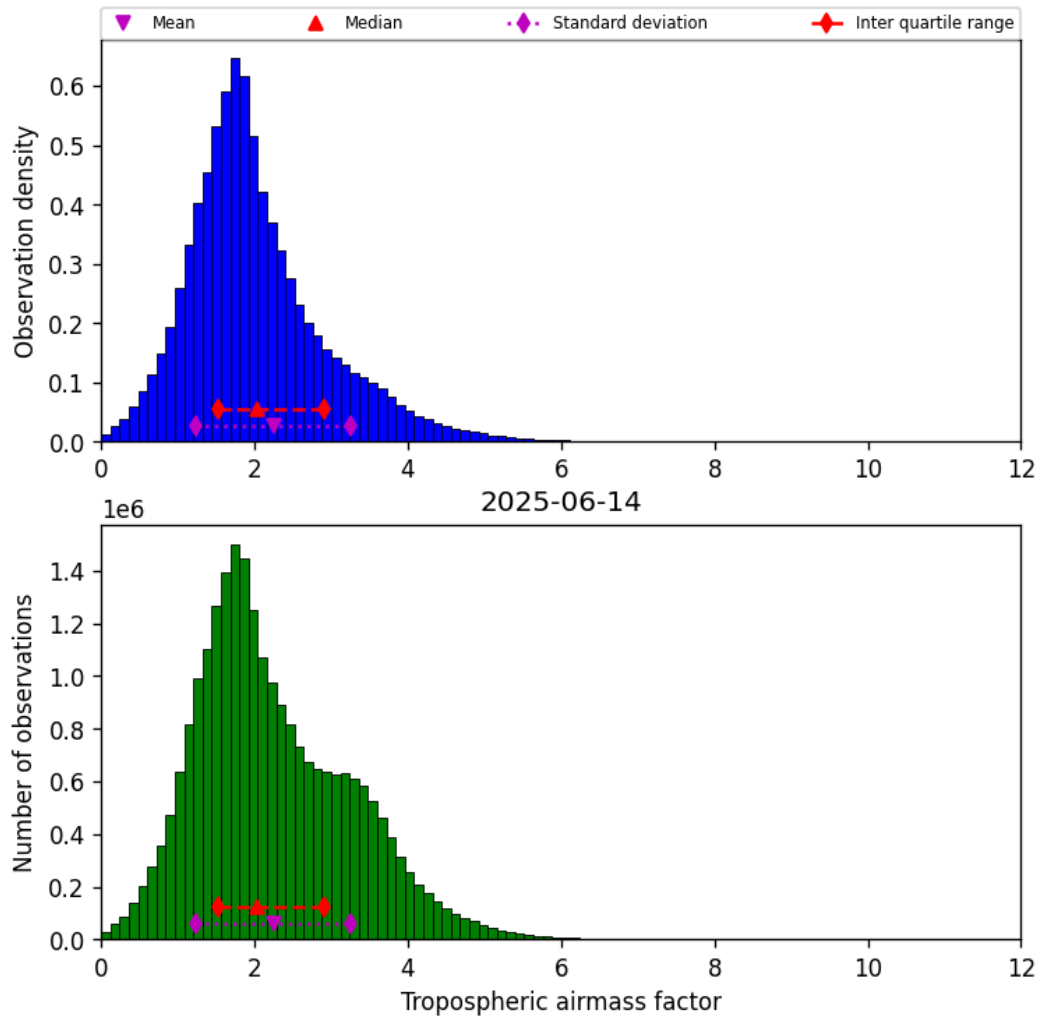
Figure 29: Histogram of “Tropospheric airmass factor” for 2025-06-14 to 2025-06-14
