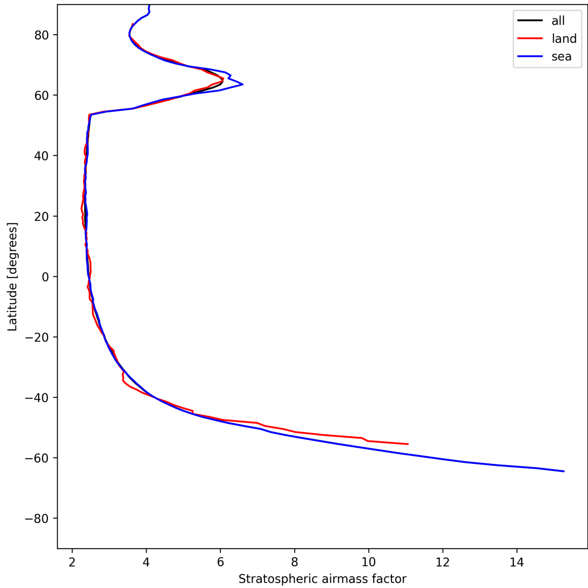
Figure 25: Zonal average of “Stratospheric air mass factor” for 2025-06-14 to 2025-06-14.
