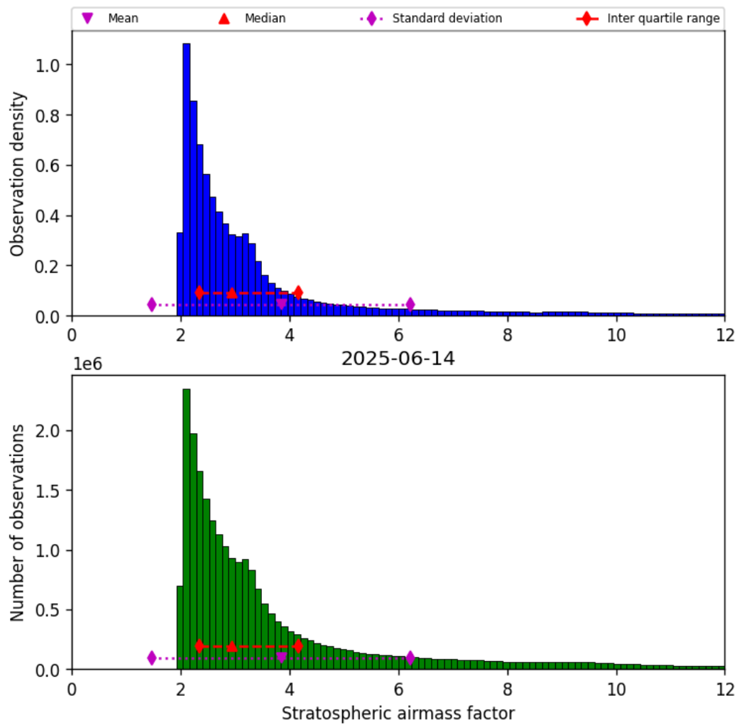
Figure 42: Histogram of “Stratospheric airmass factor” for 2025-06-14 to 2025-06-14
