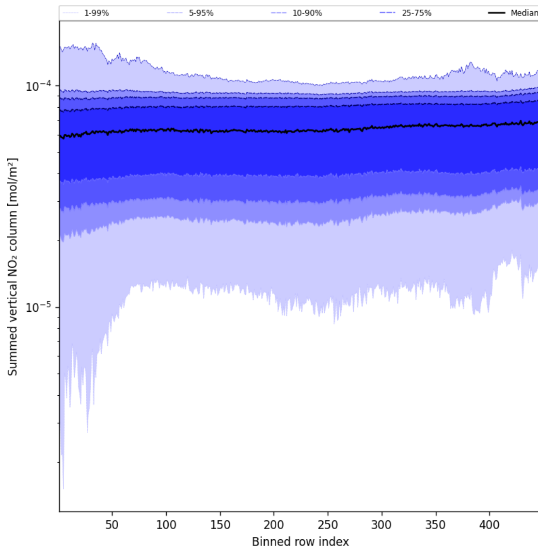
Figure 55: Along track statistics of “Summed vertical NO 2 column” for 2025-06-14 to 2025-06-14
