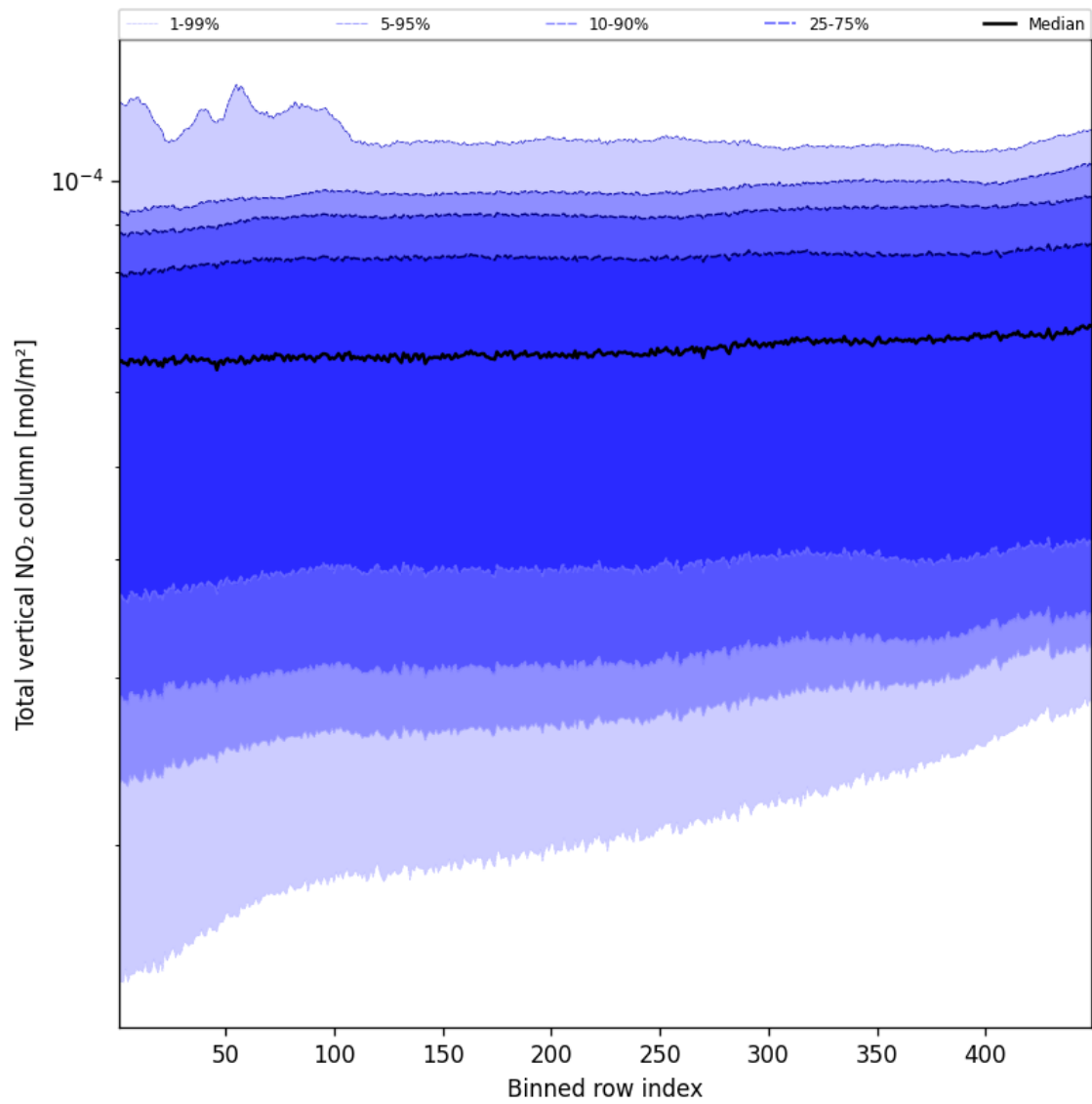
Figure 53: Along track statistics of “Total vertical NO 2 column” for 2025-06-14 to 2025-06-14
