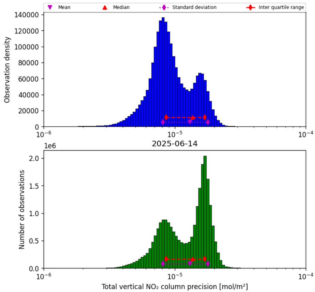
Figure 37: Histogram of "Total vertical NO 2 column precision" for 2025-06-14 to 2025-06-14
