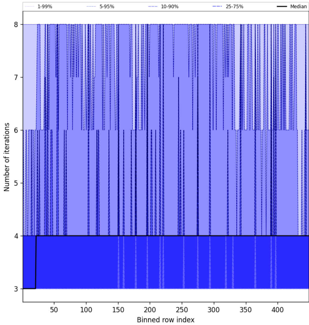
Figure 49: Along track statistics of “Number of iterations” for 2025-06-14 to 2025-06-14
