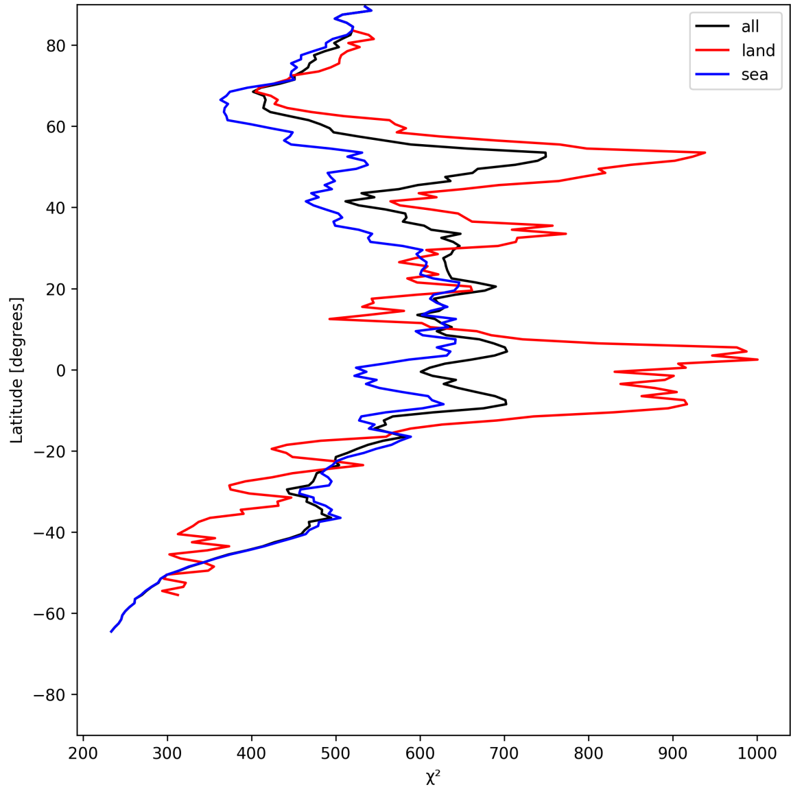
Figure 23: Zonal average of “ \chi^2 ” for 2025-06-14 to 2025-06-14.
