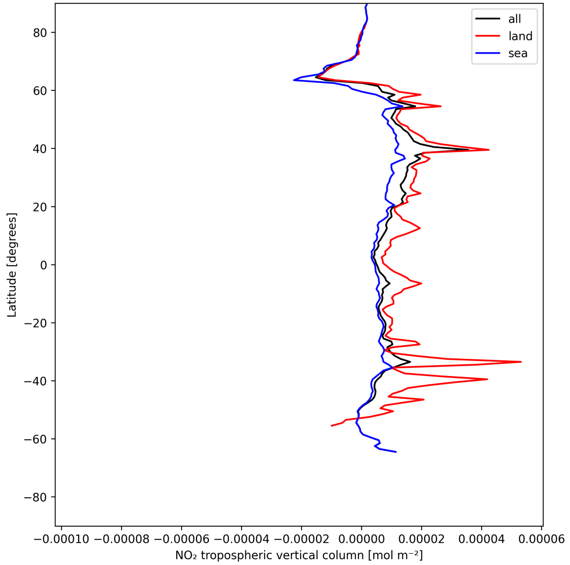
Figure 10: Zonal average of “NO 2 tropospheric vertical column” for 2025-06-14 to 2025-06-14.
