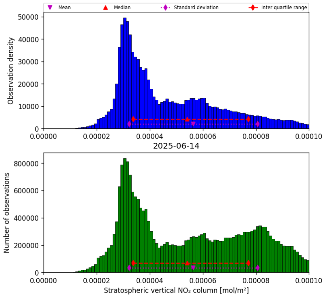
Figure 34: Histogram of “Stratospheric vertical NO 2 column” for 2025-06-14 to 2025-06-14
