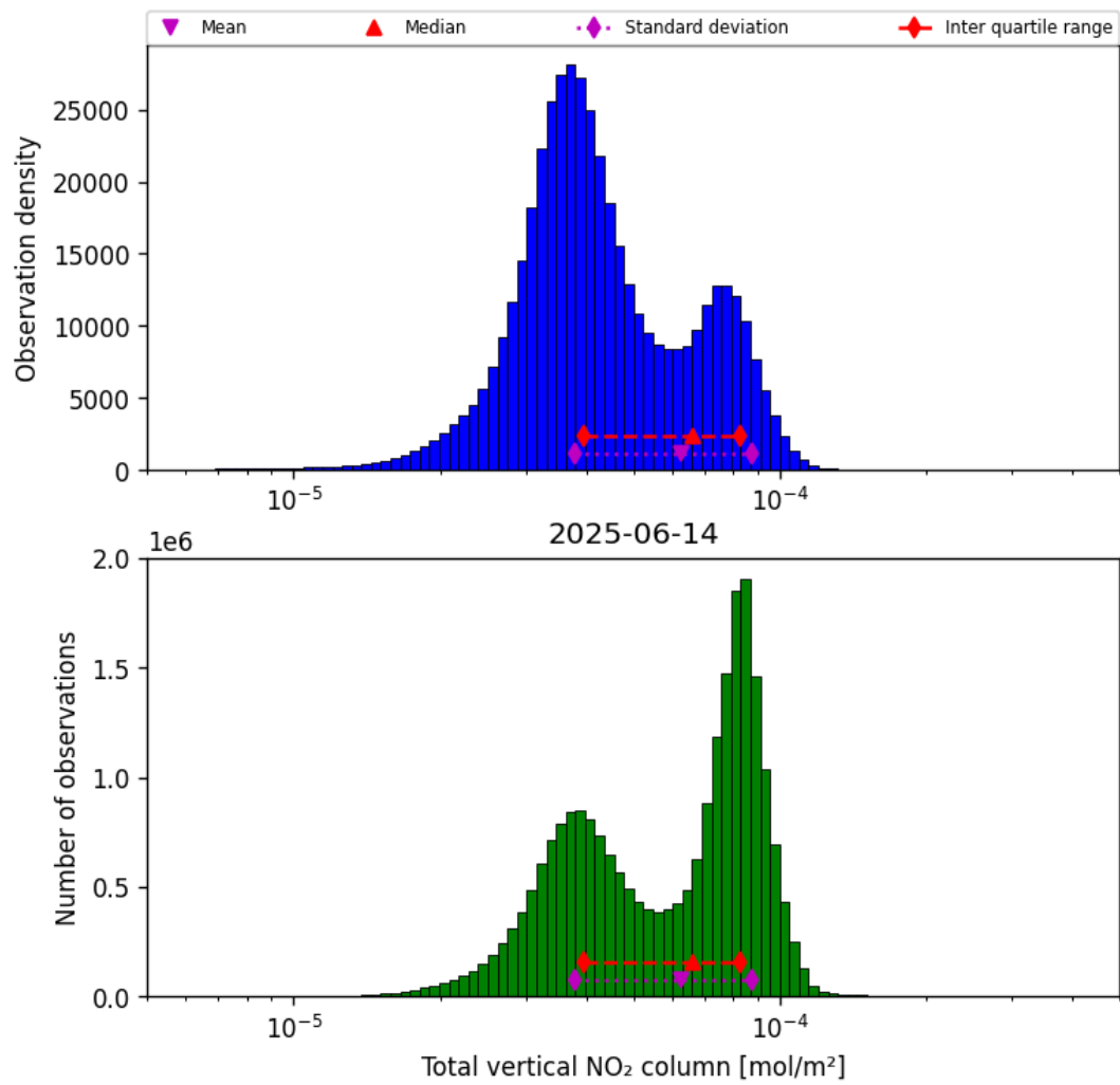
Figure 36: Histogram of “Total vertical NO 2 column” for 2025-06-14 to 2025-06-14
