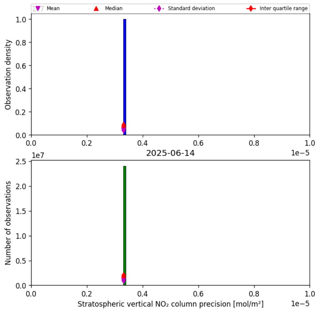
Figure 35: Histogram of “Stratospheric vertical NO 2 column precision” for 2025-06-14 to 2025-06-14
