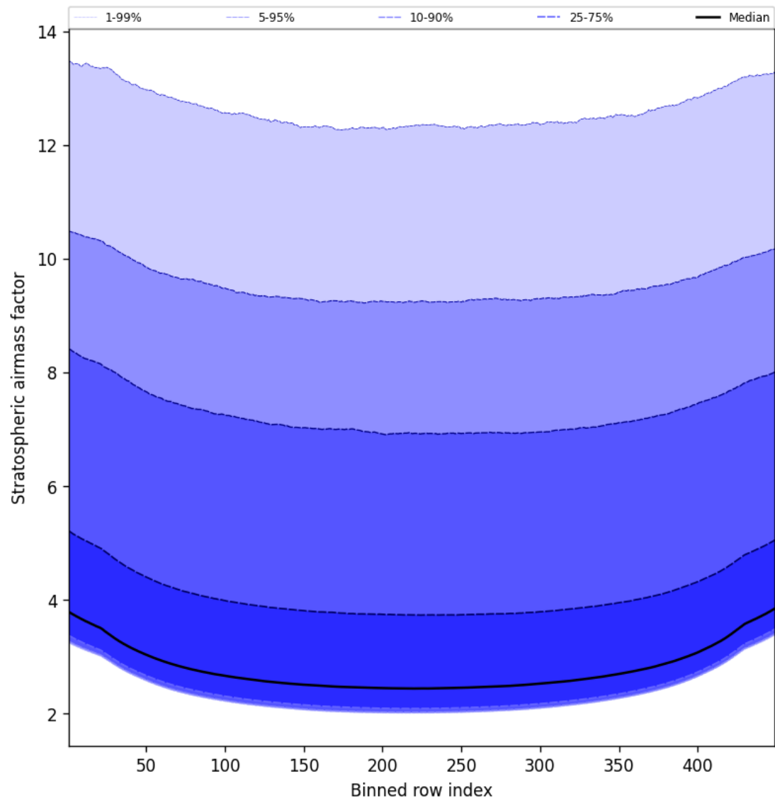
Figure 59: Along track statistics of “Stratospheric airmass factor” for 2025-06-14 to 2025-06-14
