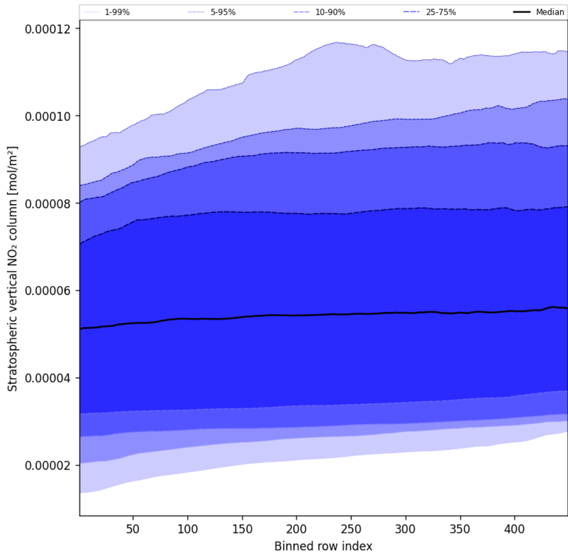
Figure 51: Along track statistics of “Stratospheric vertical NO 2 column” for 2025-06-14 to 2025-06-14
