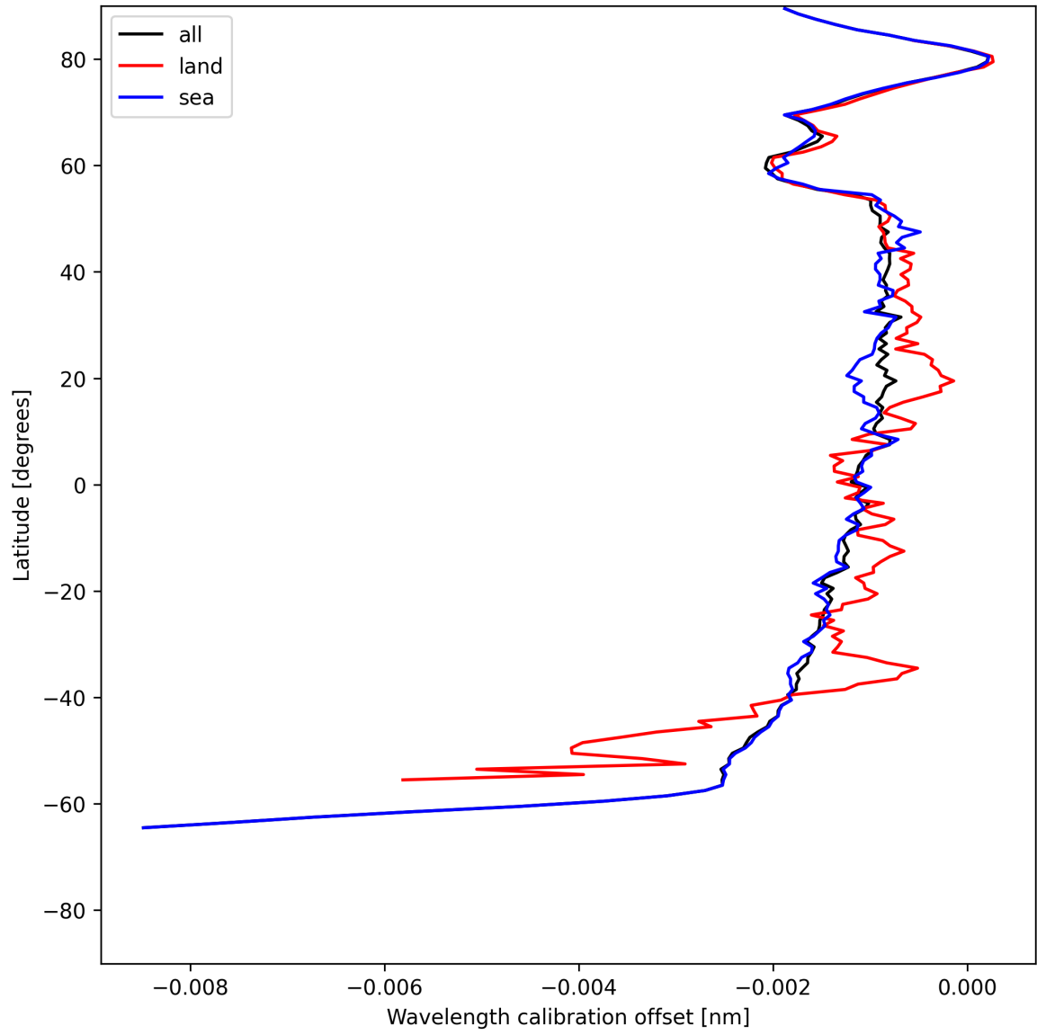
Figure 16: Zonal average of “Wavelength calibration offset” for 2025-06-14 to 2025-06-14.
