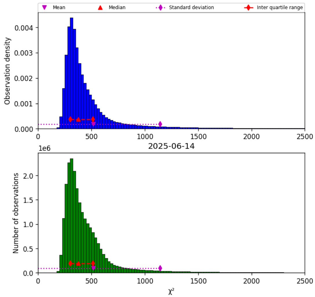
Figure 40: Histogram of “ \chi^2 ” for 2025-06-14 to 2025-06-14
