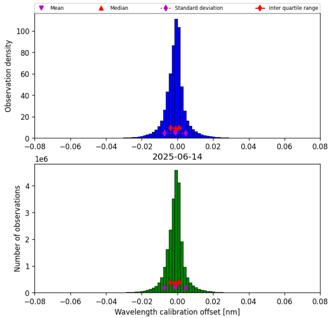
Figure 33: Histogram of “Wavelength calibration offset” for 2025-06-14 to 2025-06-14
