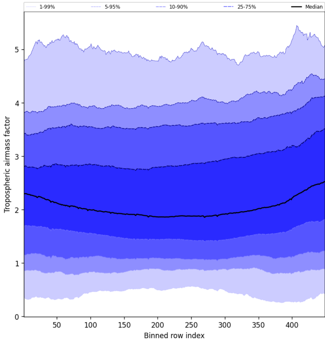
Figure 46: Along track statistics of “Tropospheric airmass factor” for 2025-06-14 to 2025-06-14
