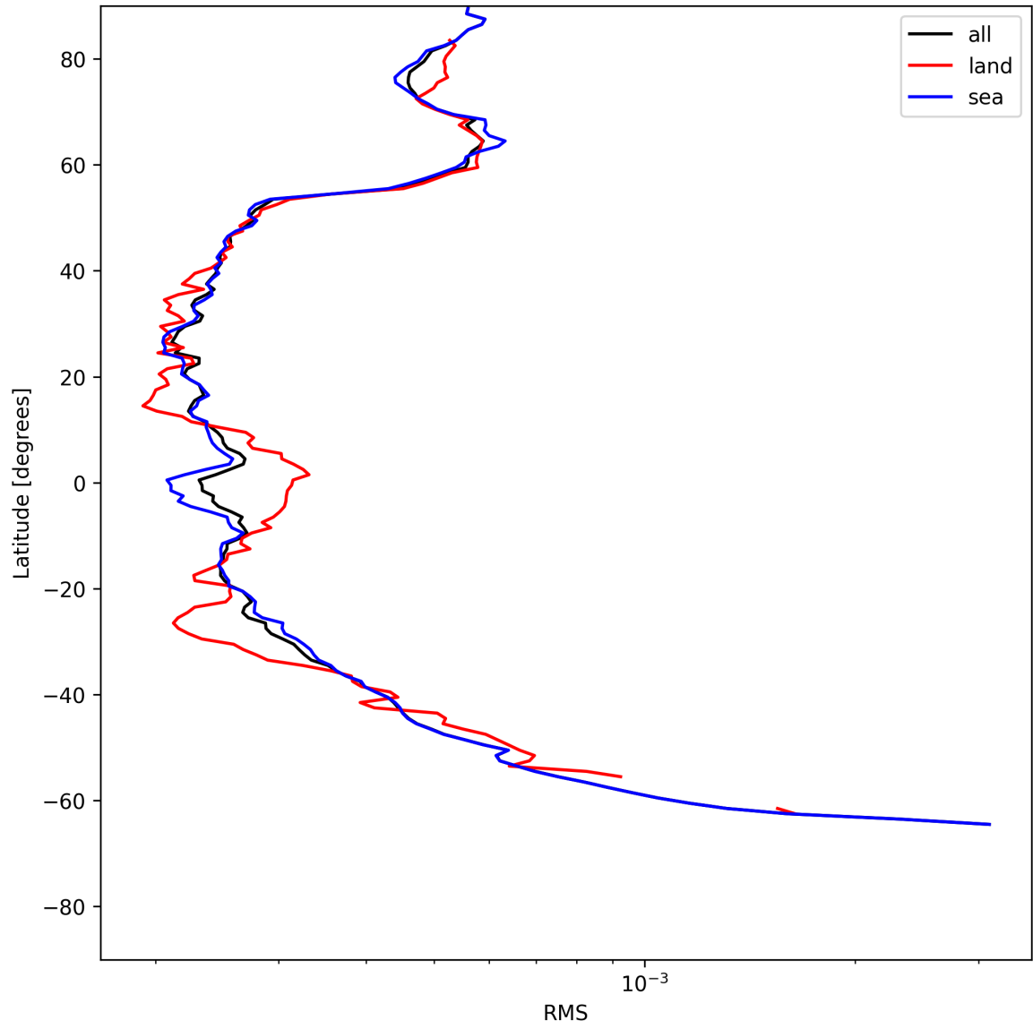
Figure 24: Zonal average of “RMS” for 2025-06-15 to 2025-06-16.
