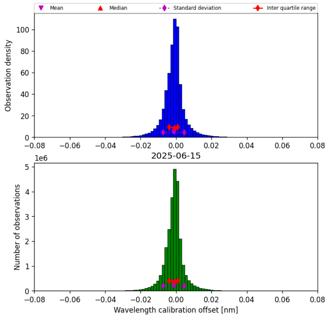
Figure 33: Histogram of “Wavelength calibration offset” for 2025-06-15 to 2025-06-16
