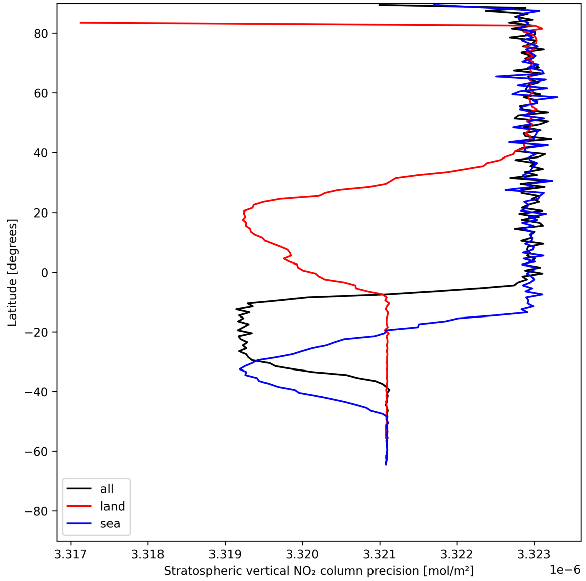
Figure 18: Zonal average of “Stratospheric vertical NO 2 column precision” for 2025-06-15 to 2025-06-16.
