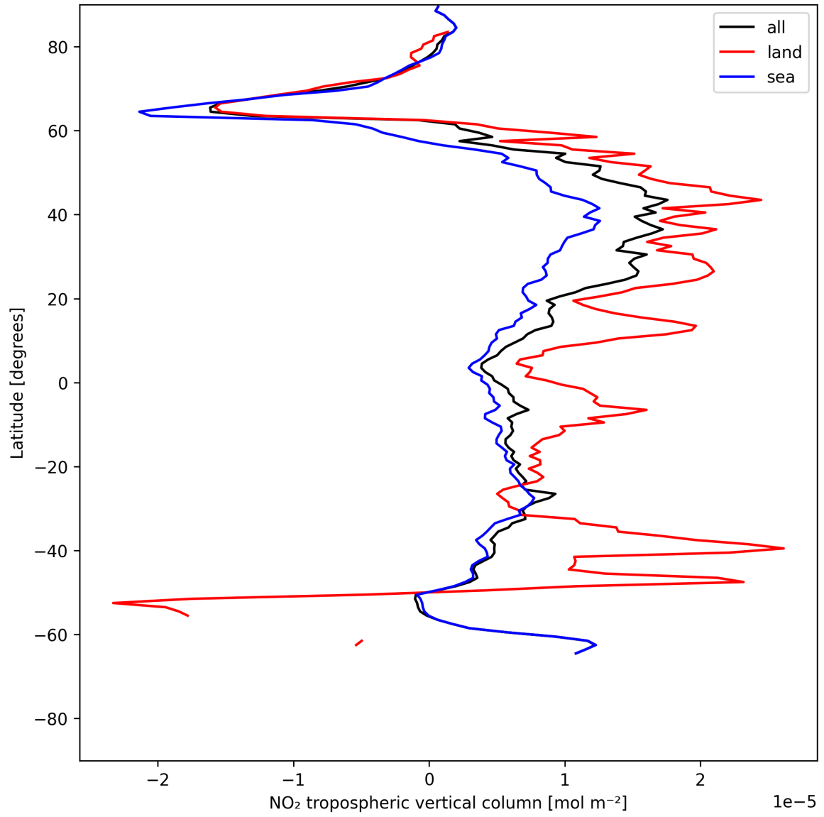
Figure 10: Zonal average of “NO 2 tropospheric vertical column” for 2025-06-15 to 2025-06-16.
