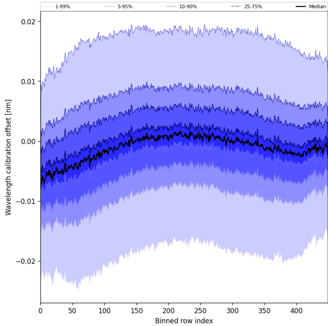
Figure 50: Along track statistics of “Wavelength calibration offset” for 2025-06-15 to 2025-06-16
