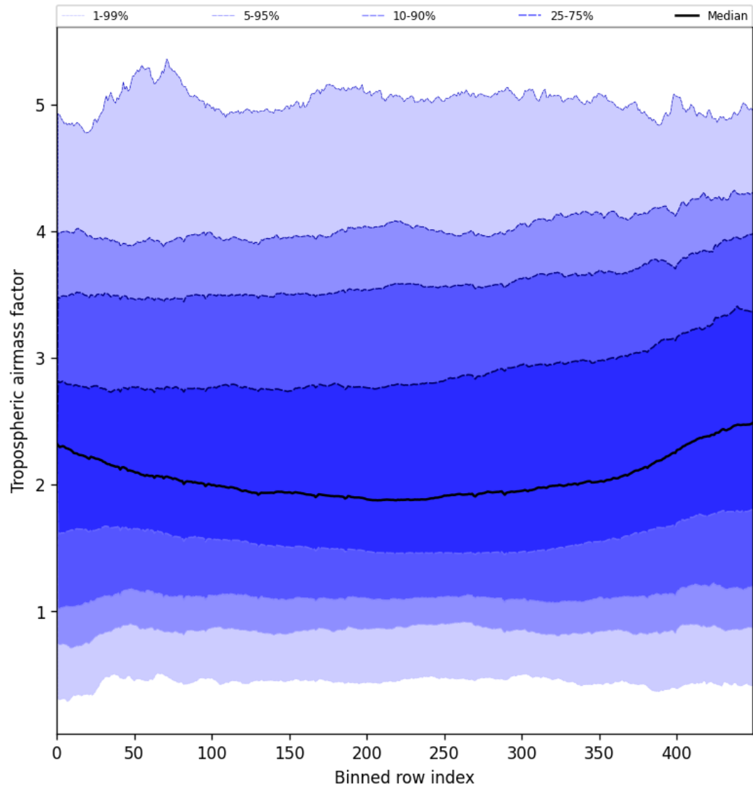
Figure 46: Along track statistics of “Tropospheric airmass factor” for 2025-06-15 to 2025-06-16
