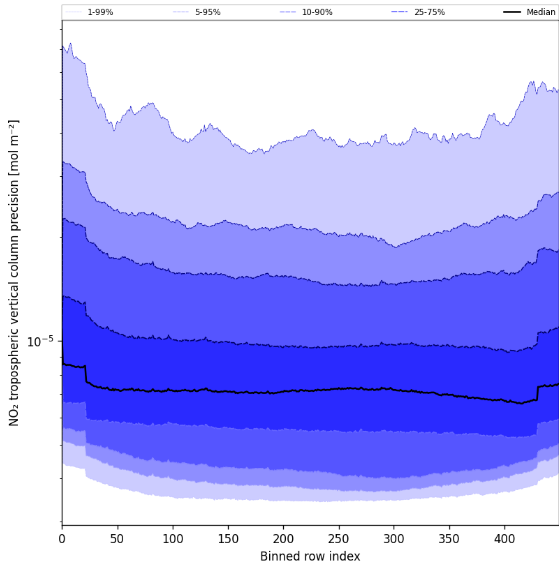
Figure 45: Along track statistics of “NO 2 tropospheric vertical column precision” for 2025-06-15 to 2025-06-16
