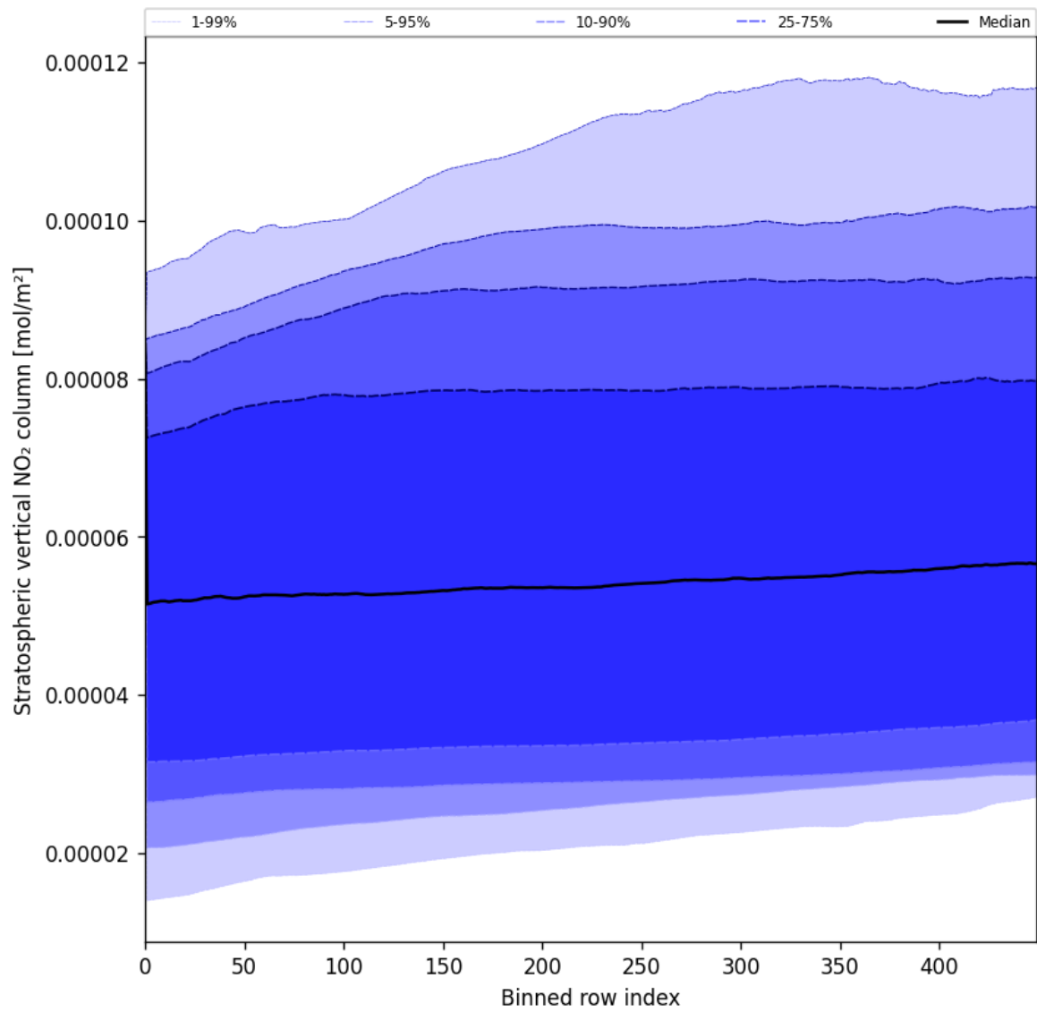
Figure 51: Along track statistics of “Stratospheric vertical NO 2 column” for 2025-06-15 to 2025-06-16
