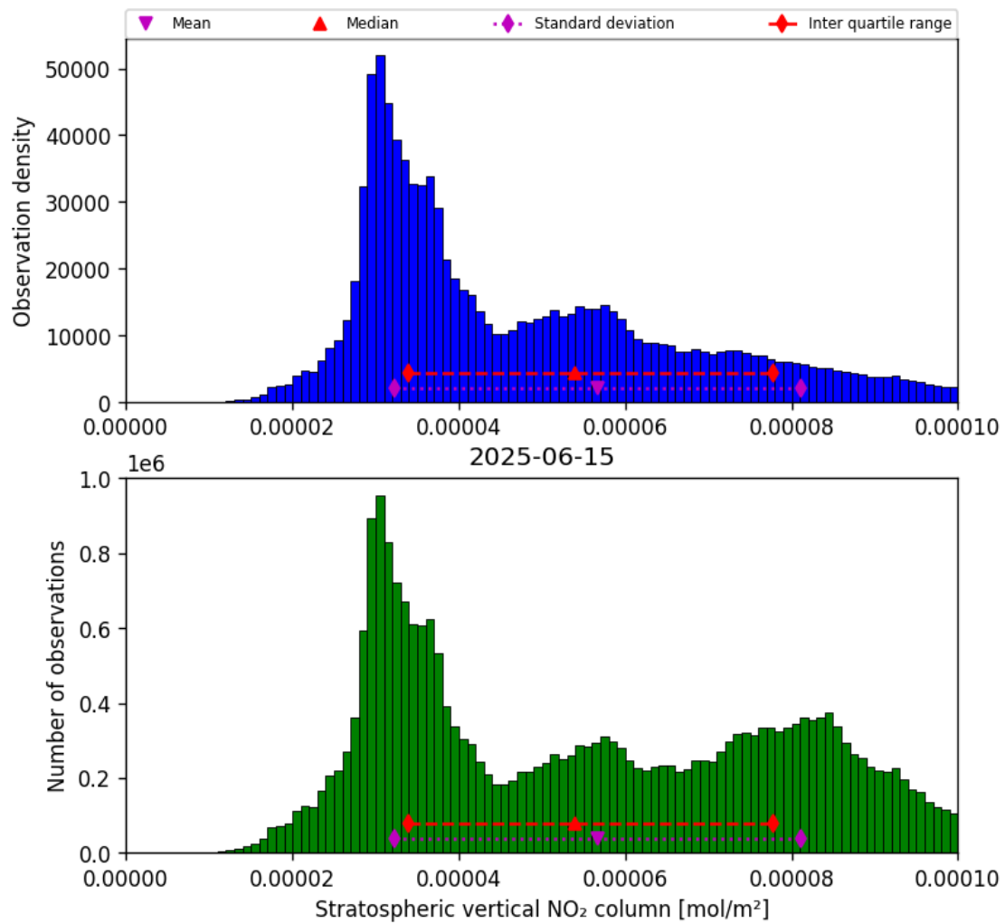
Figure 34: Histogram of “Stratospheric vertical NO 2 column” for 2025-06-15 to 2025-06-16
