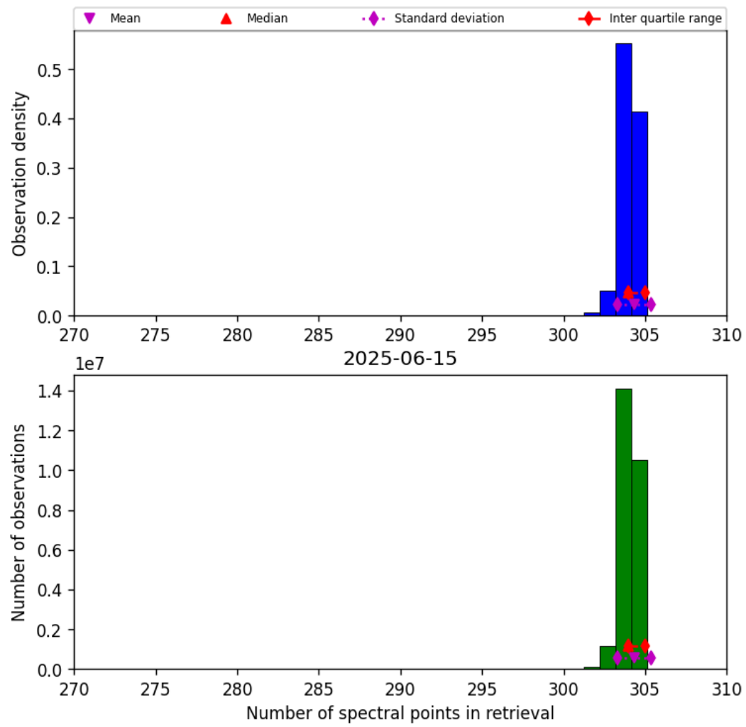
Figure 31: Histogram of “Number of spectral points in retrieval” for 2025-06-15 to 2025-06-16
