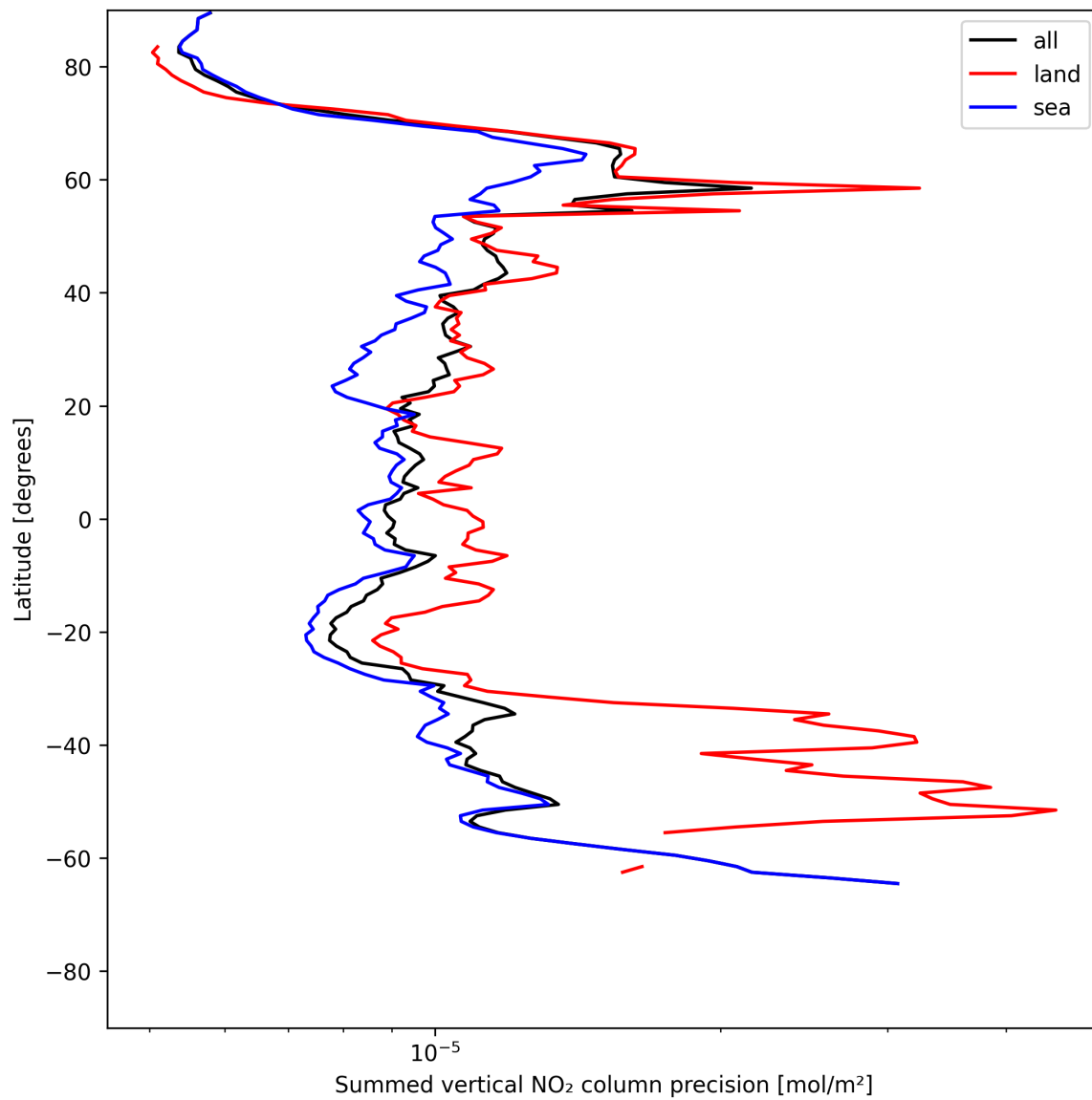
Figure 22: Zonal average of “Summed vertical NO 2 column precision” for 2025-06-15 to 2025-06-16.
