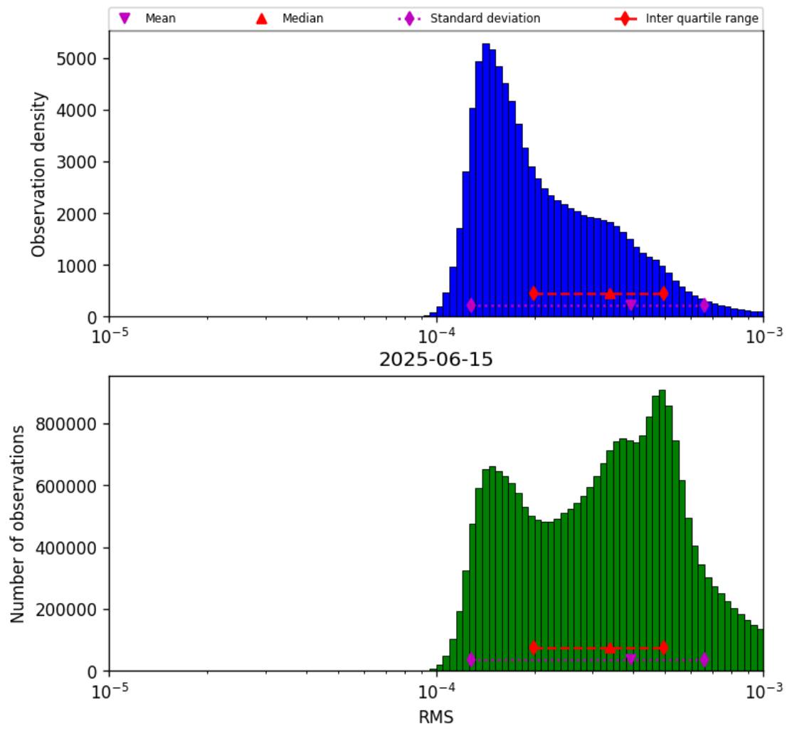
Figure 41: Histogram of “RMS” for 2025-06-15 to 2025-06-16
