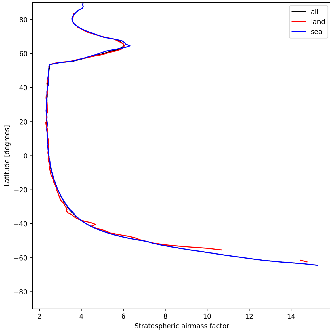
Figure 25: Zonal average of “Stratospheric air mass factor” for 2025-06-15 to 2025-06-16.
