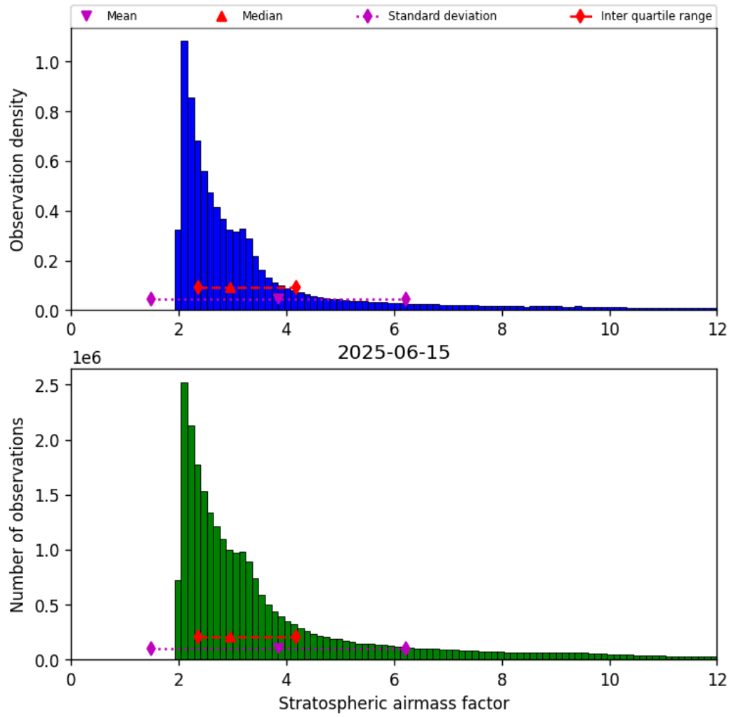
Figure 42: Histogram of “Stratospheric airmass factor” for 2025-06-15 to 2025-06-16
