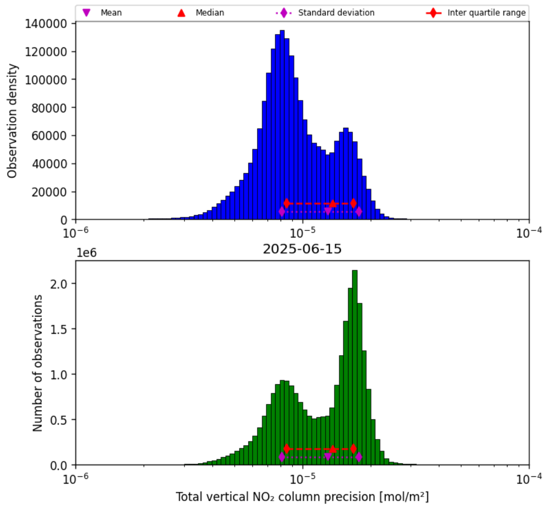
Figure 37: Histogram of “Total vertical NO 2 column precision” for 2025-06-15 to 2025-06-16
