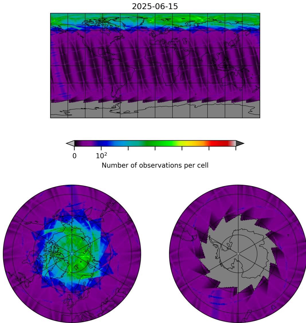
Figure 8: Map of the number of observations for 2025-06-15 to 2025-06-16
