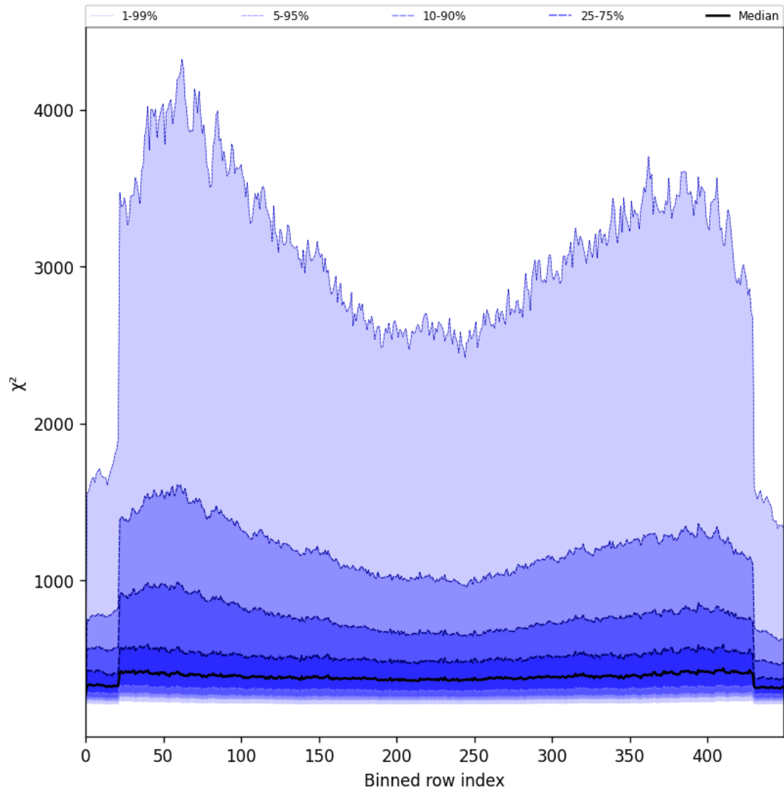
Figure 57: Along track statistics of “ \chi^2 ” for 2025-06-15 to 2025-06-16
