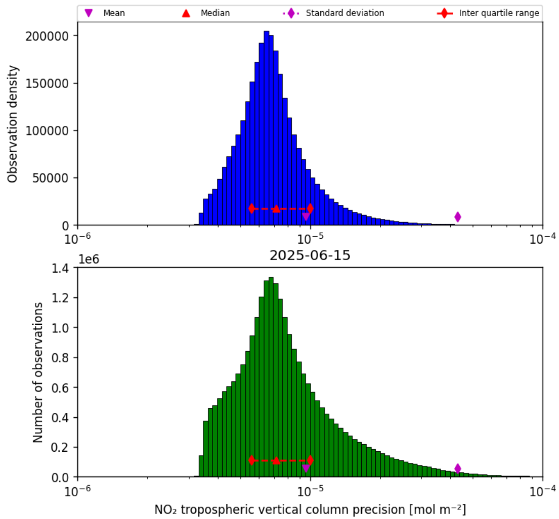
Figure 28: Histogram of “NO 2 tropospheric vertical column precision” for 2025-06-15 to 2025-06-16
