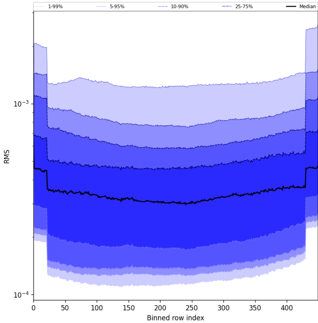
Figure 58: Along track statistics of “RMS” for 2025-06-15 to 2025-06-16
