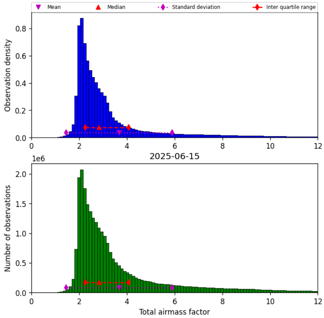
Figure 30: Histogram of “Total airmass factor” for 2025-06-15 to 2025-06-16
