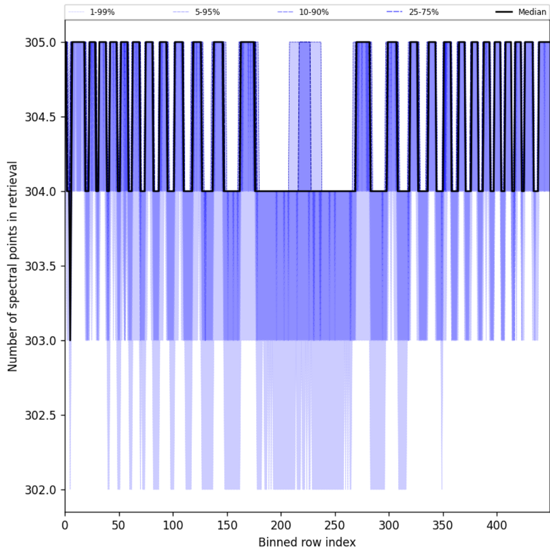
Figure 48: Along track statistics of “Number of spectral points in retrieval” for 2025-06-15 to 2025-06-16
