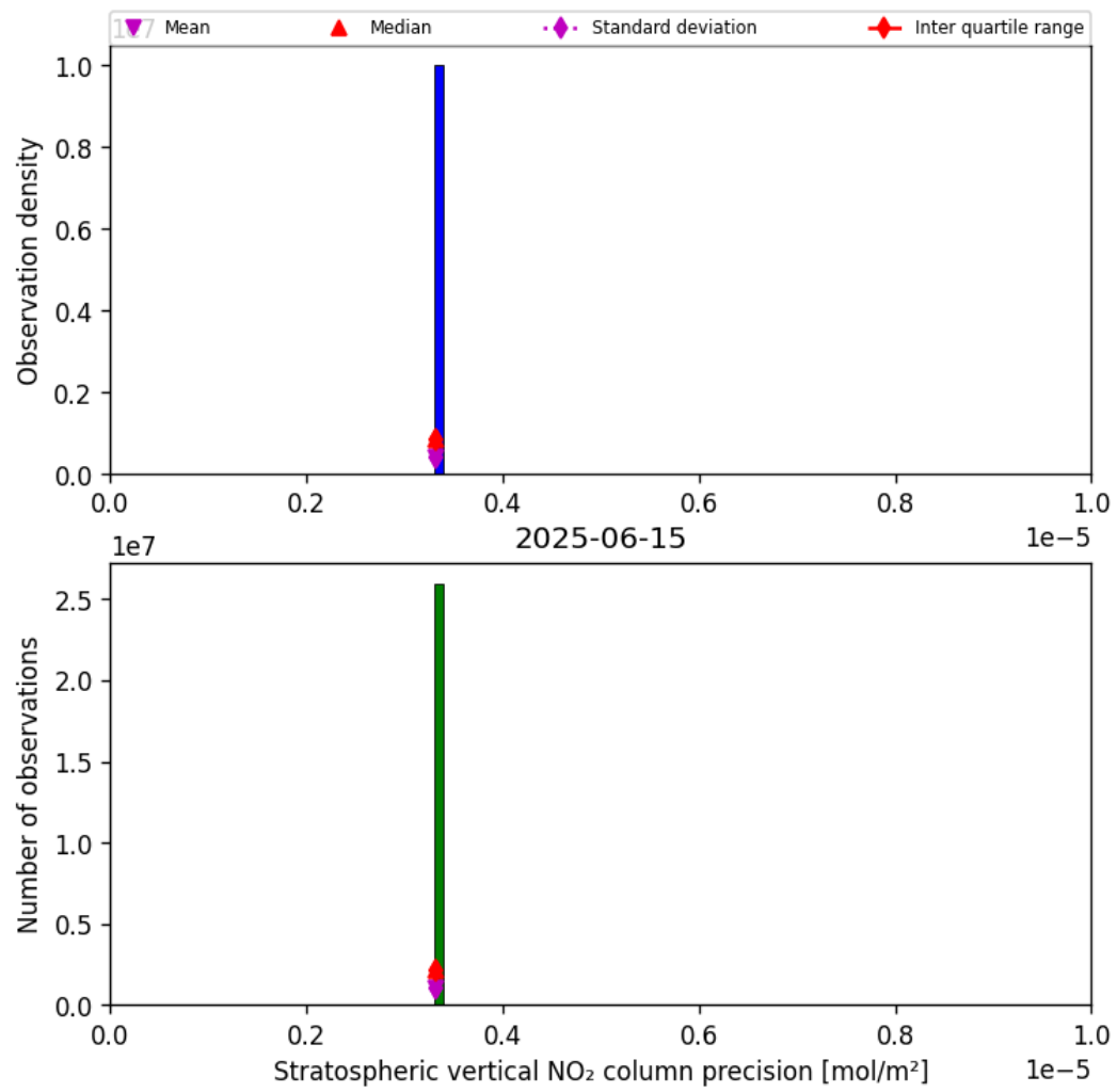
Figure 35: Histogram of “Stratospheric vertical NO 2 column precision” for 2025-06-15 to 2025-06-16
