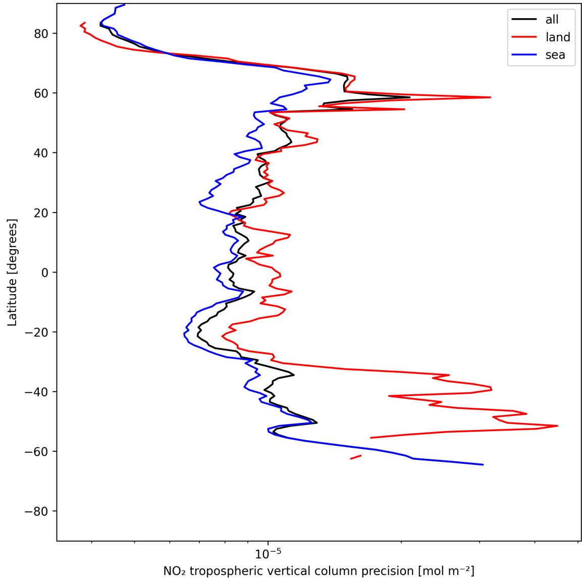
Figure 11: Zonal average of “NO 2 tropospheric vertical column precision” for 2025-06-15 to 2025-06-16.
