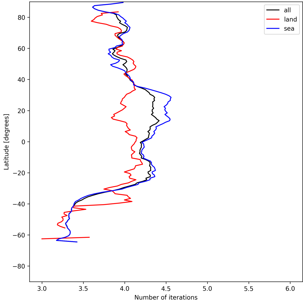
Figure 15: Zonal average of “Number of iterations” for 2025-06-15 to 2025-06-16.
