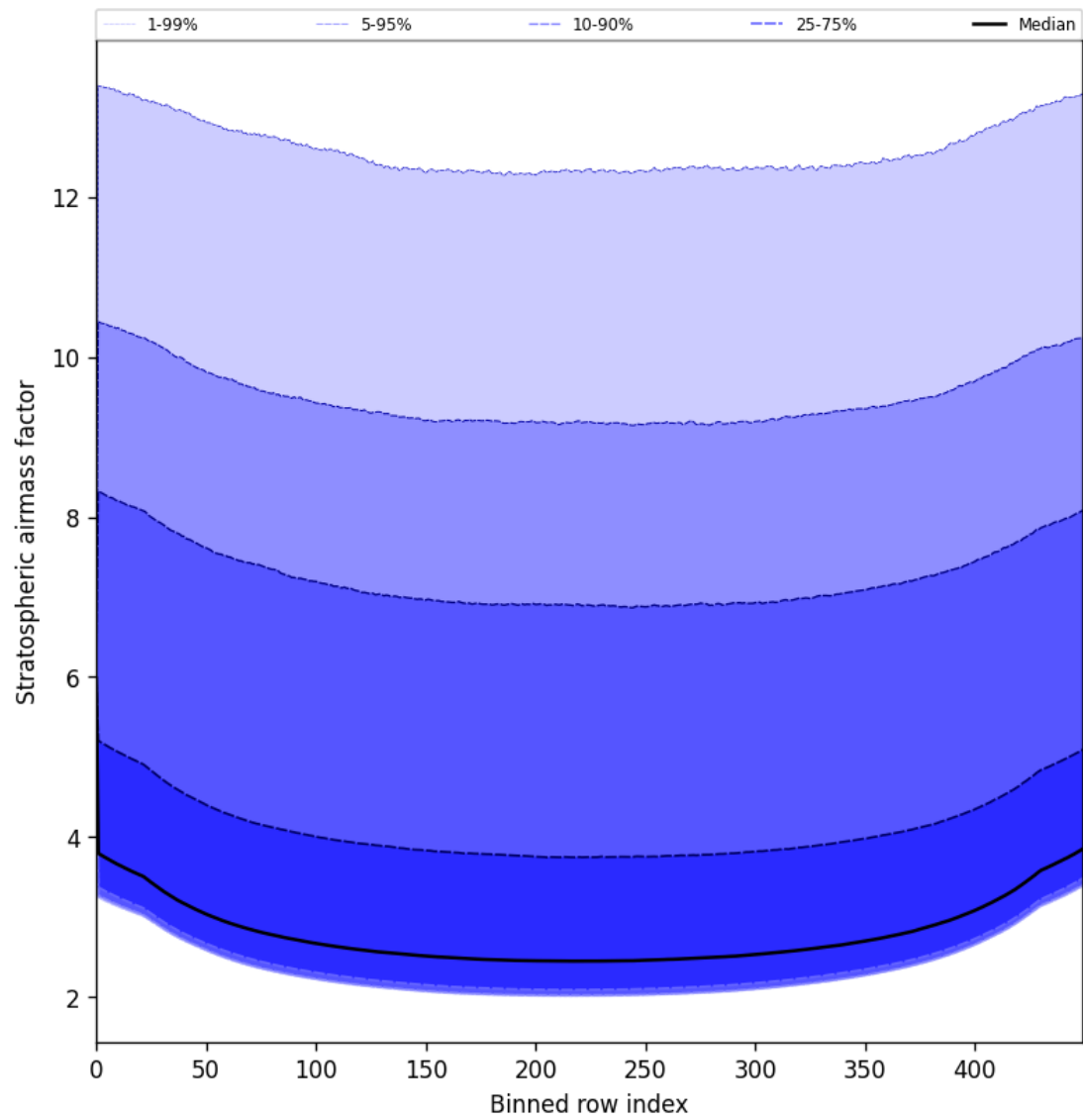
Figure 59: Along track statistics of “Stratospheric airmass factor” for 2025-06-15 to 2025-06-16
