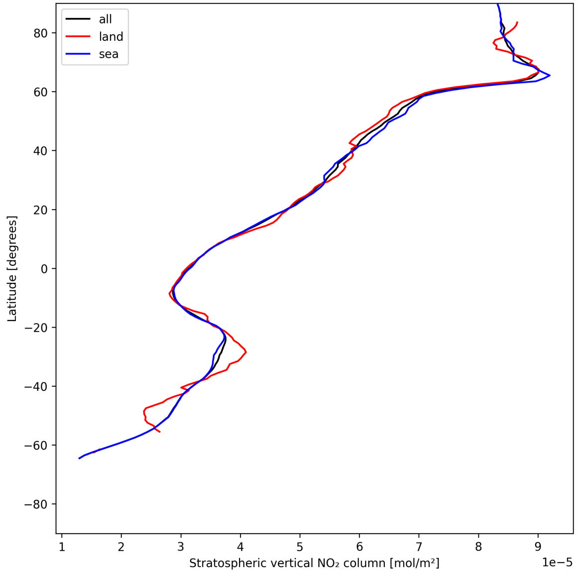
Figure 17: Zonal average of “Stratospheric vertical NO 2 column” for 2025-06-15 to 2025-06-16.
