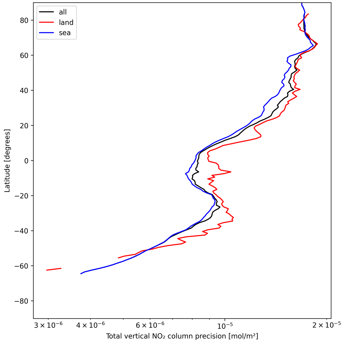
Figure 20: Zonal average of “Total vertical NO 2 column precision” for 2025-06-15 to 2025-06-16.
