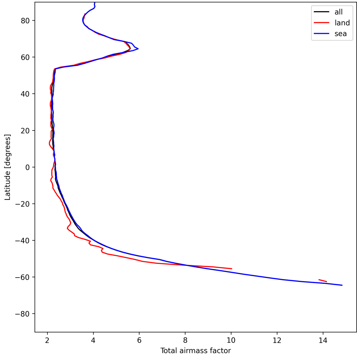
Figure 13: Zonal average of “Total airmass factor” for 2025-06-15 to 2025-06-16.
