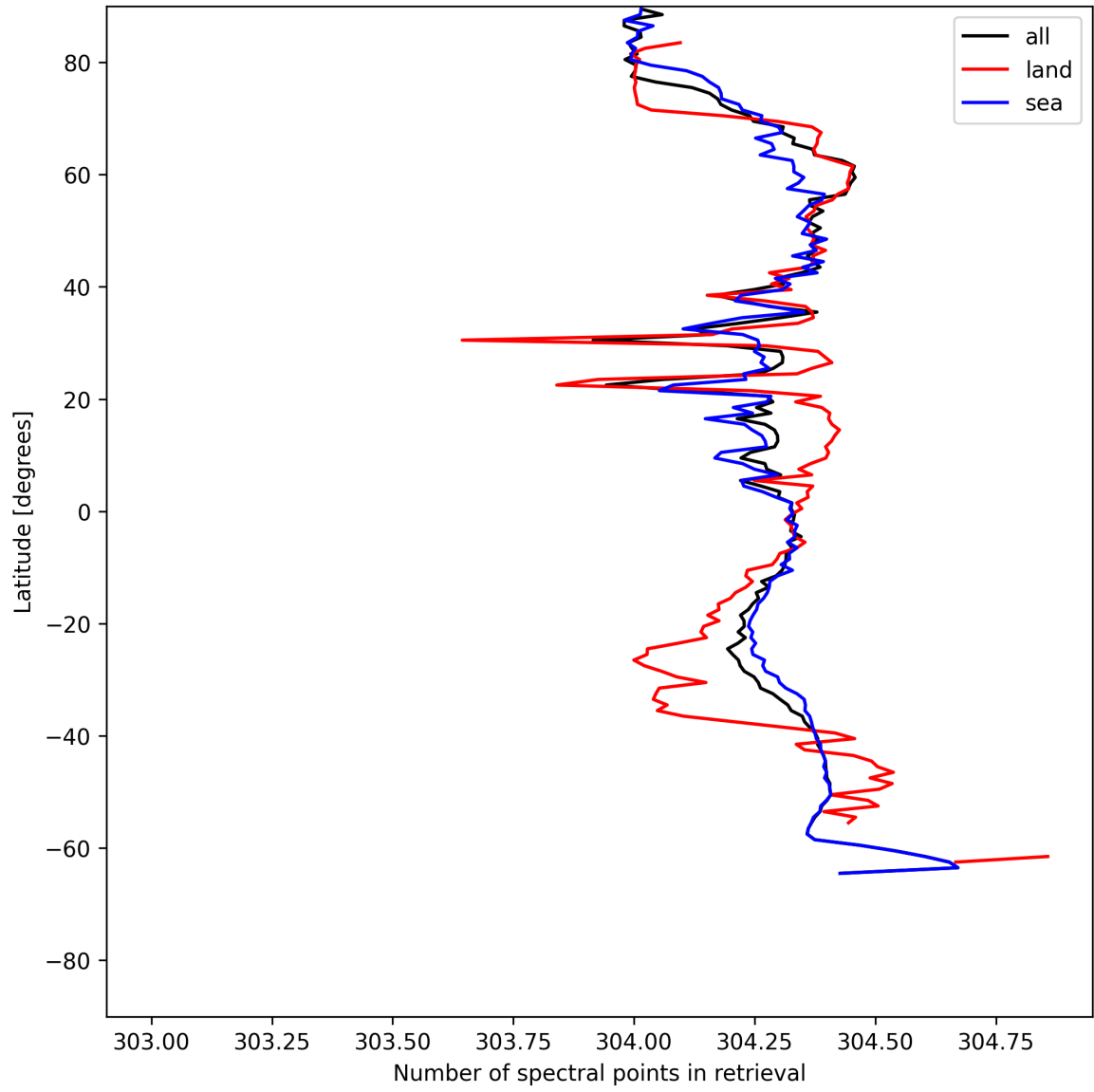
Figure 14: Zonal average of “Number of spectral points in retrieval” for 2025-06-15 to 2025-06-16.
