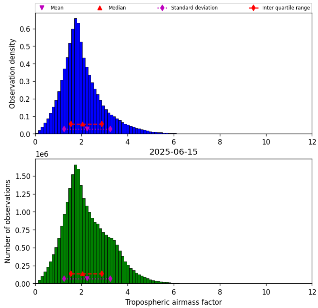
Figure 29: Histogram of “Tropospheric airmass factor” for 2025-06-15 to 2025-06-16
