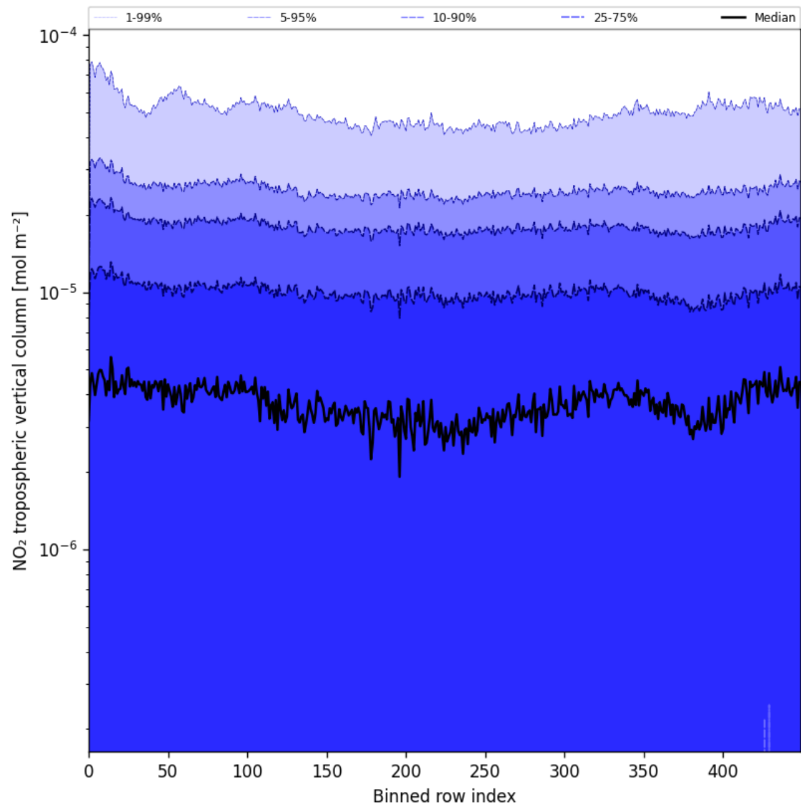
Figure 44: Along track statistics of “NO 2 tropospheric vertical column” for 2025-06-15 to 2025-06-16
