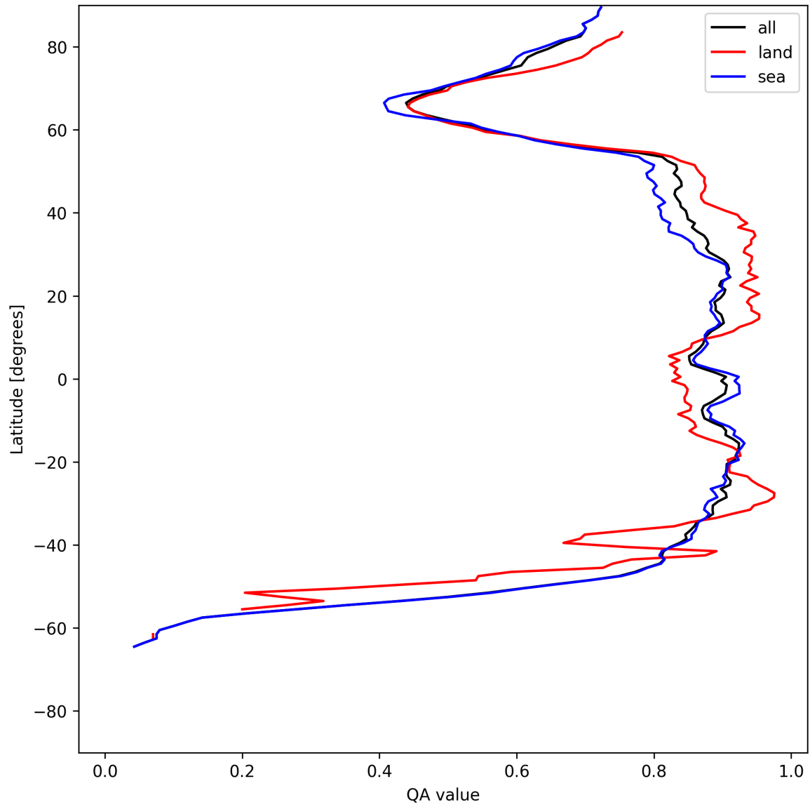
Figure 9: Zonal average of “QA value” for 2025-06-15 to 2025-06-16.
