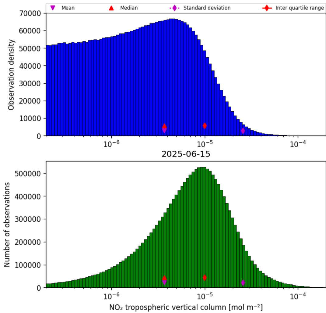
Figure 27: Histogram of “NO 2 tropospheric vertical column” for 2025-06-15 to 2025-06-16
