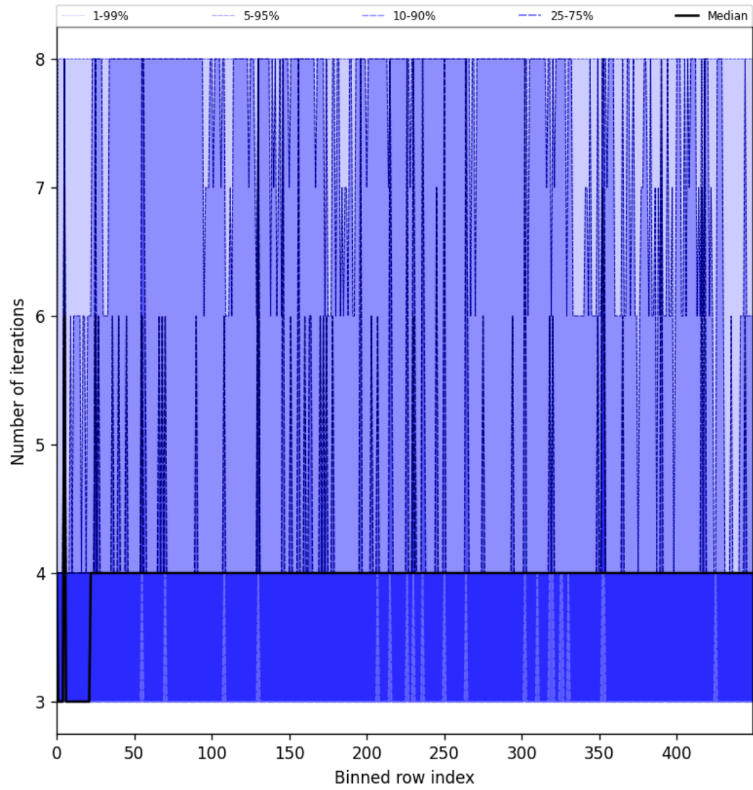
Figure 49: Along track statistics of “Number of iterations” for 2025-06-15 to 2025-06-16
