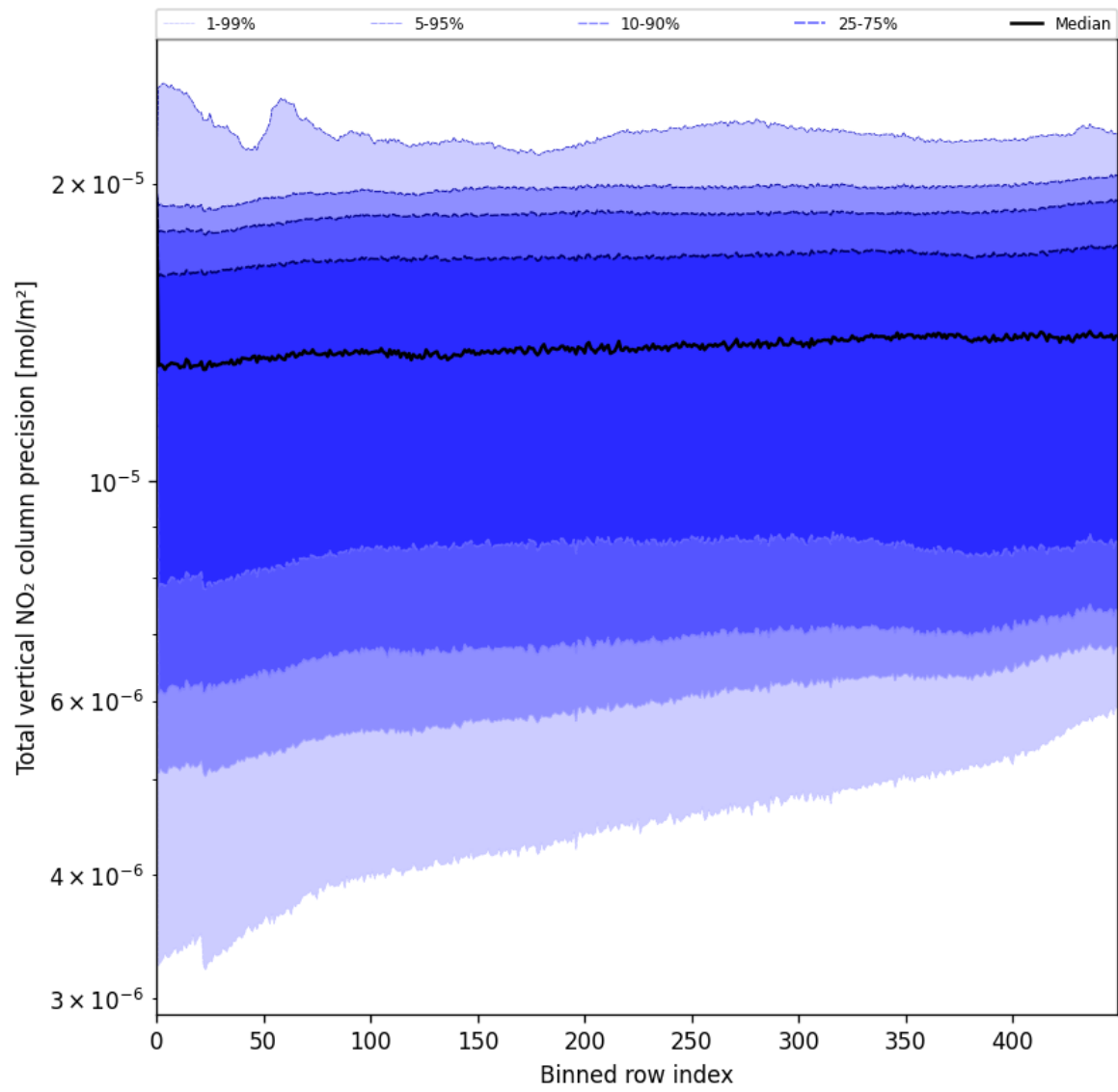
Figure 54: Along track statistics of “Total vertical NO 2 column precision” for 2025-06-15 to 2025-06-16
