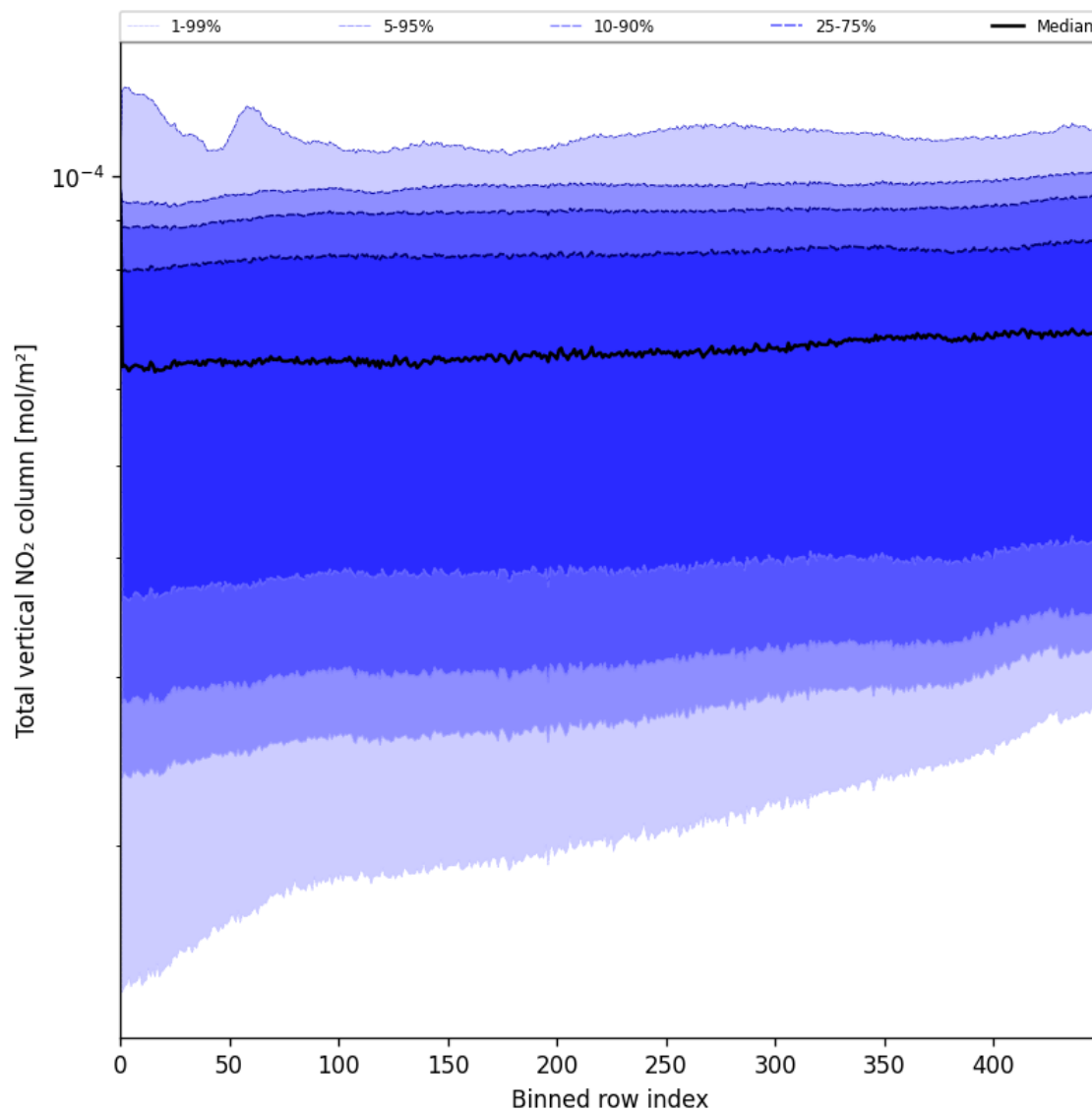
Figure 53: Along track statistics of “Total vertical NO 2 column” for 2025-06-15 to 2025-06-16
