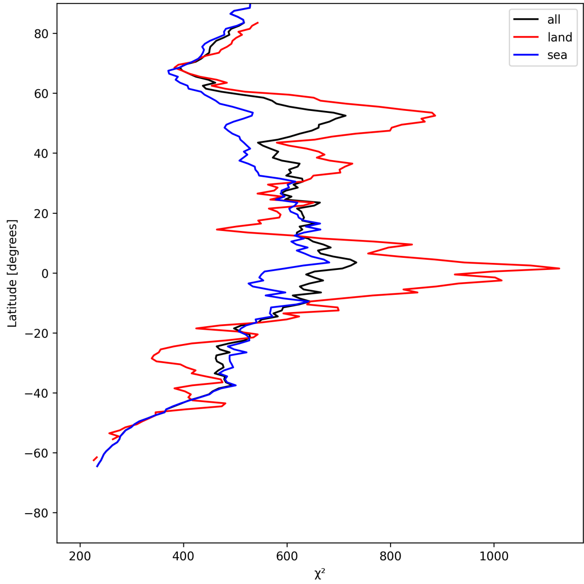
Figure 23: Zonal average of “ \chi^2 ” for 2025-06-15 to 2025-06-16.
