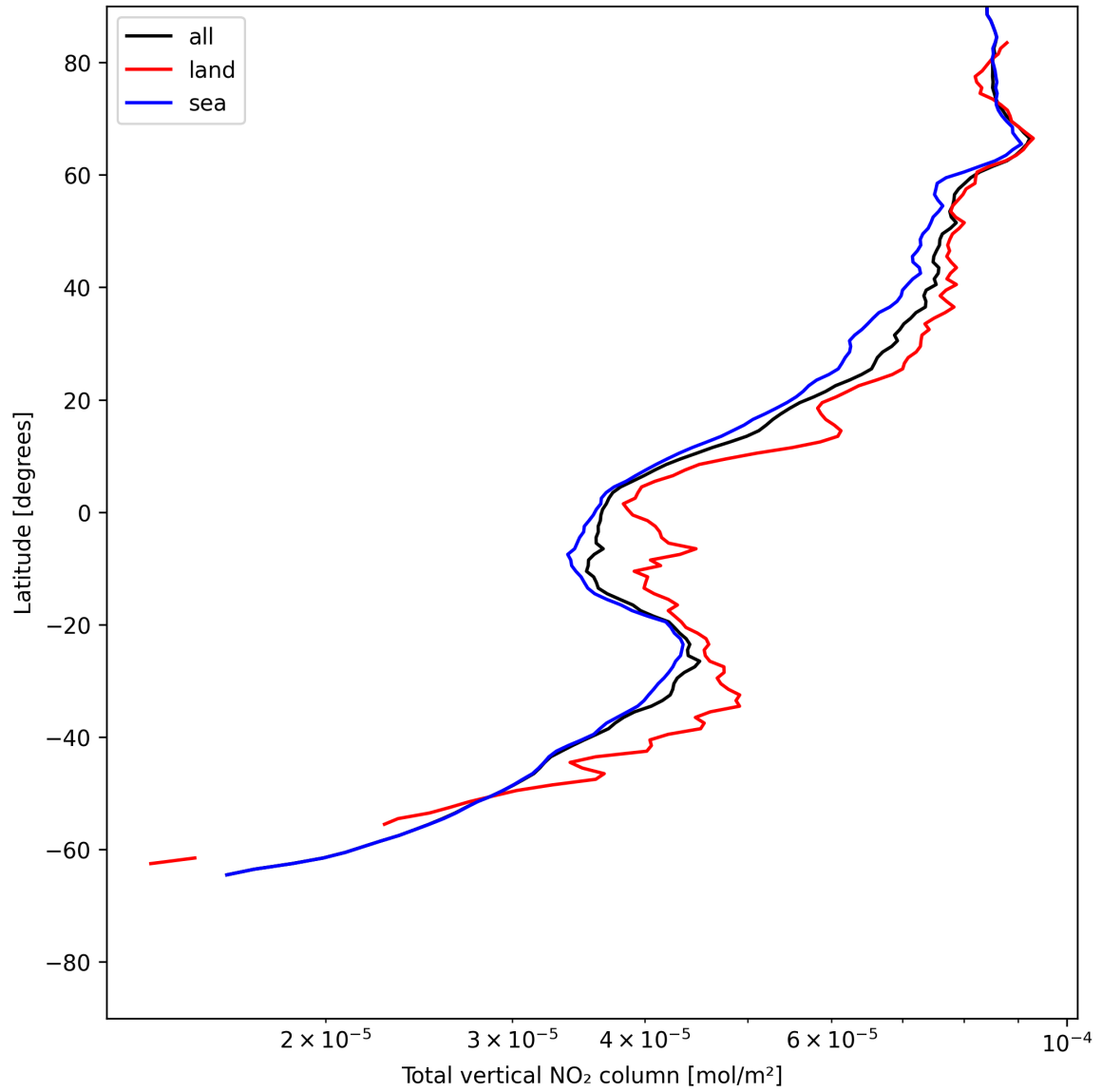
Figure 19: Zonal average of “Total vertical NO 2 column” for 2025-06-15 to 2025-06-16.
