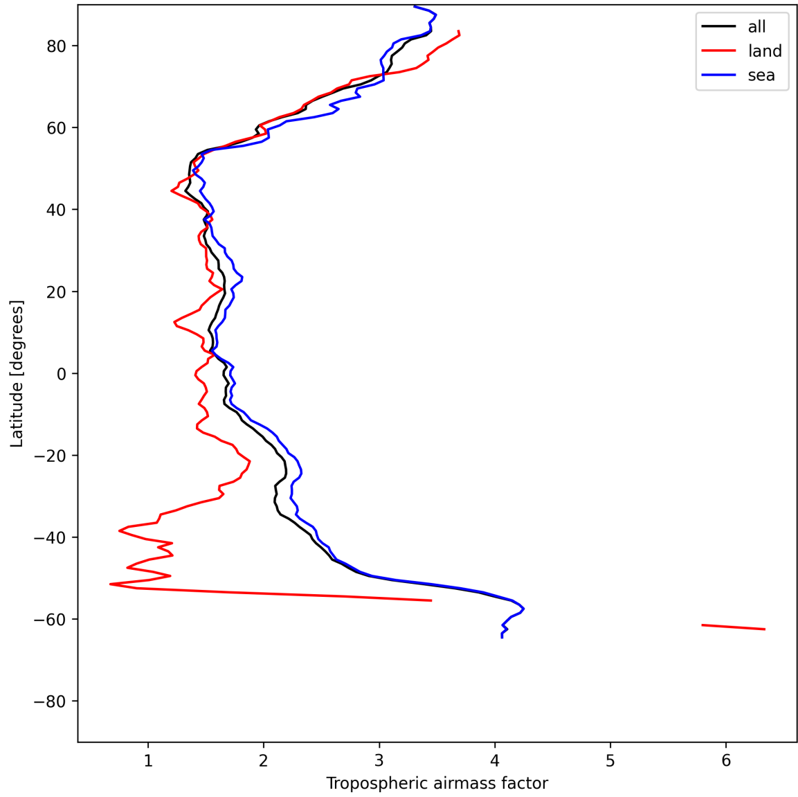
Figure 12: Zonal average of “Tropospheric airmass factor” for 2025-06-15 to 2025-06-16.
