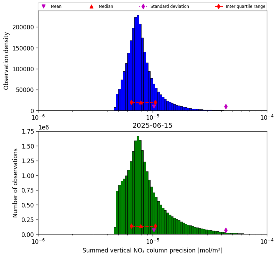
Figure 39: Histogram of “Summed vertical NO 2 column precision” for 2025-06-15 to 2025-06-16
