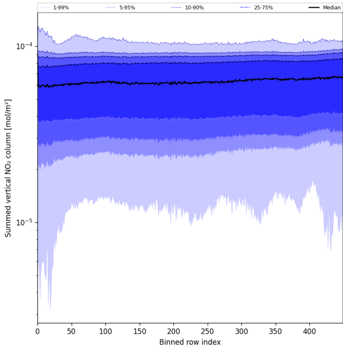
Figure 55: Along track statistics of “Summed vertical NO 2 column” for 2025-06-15 to 2025-06-16
