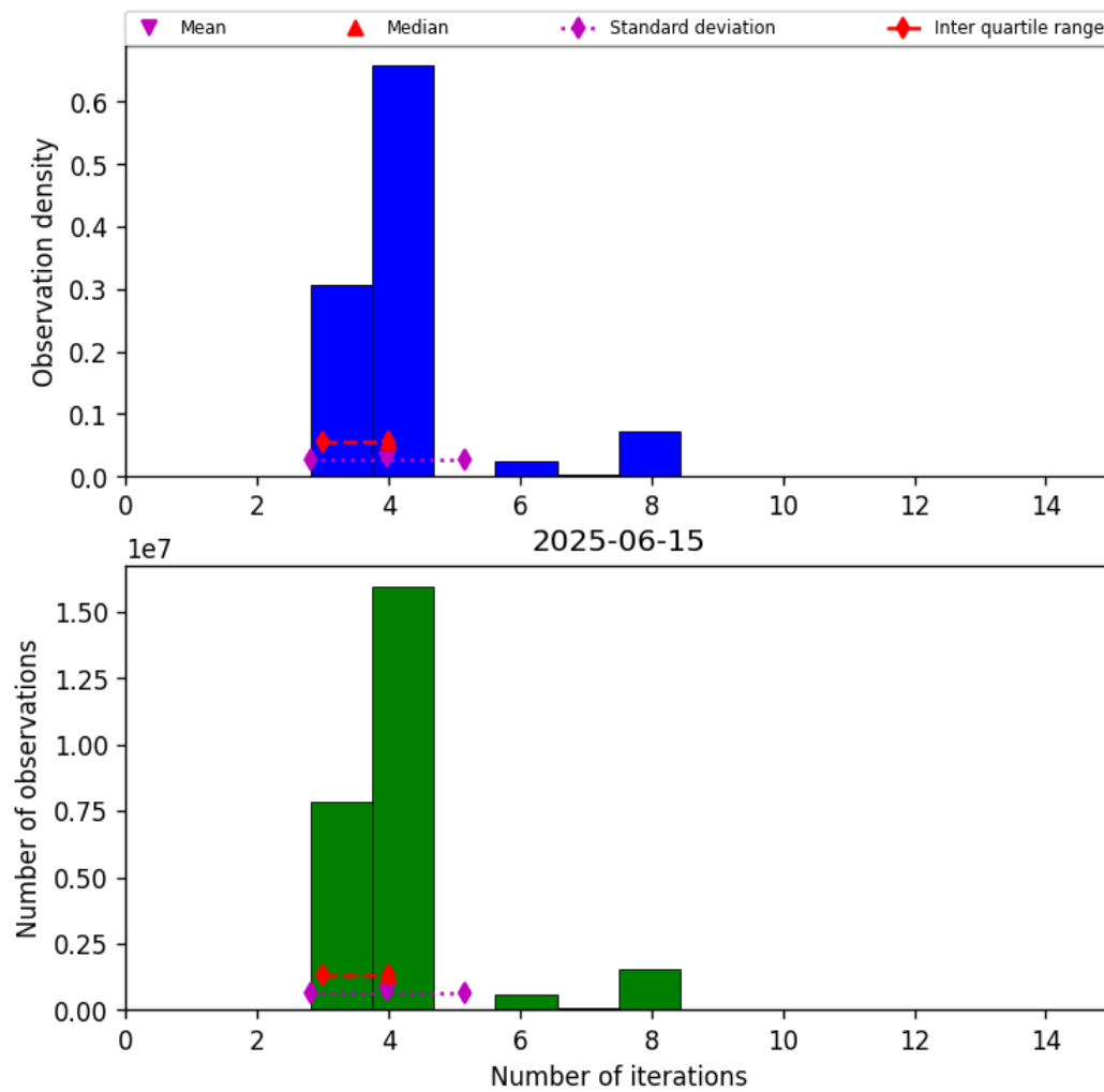
Figure 32: Histogram of “Number of iterations” for 2025-06-15 to 2025-06-16
