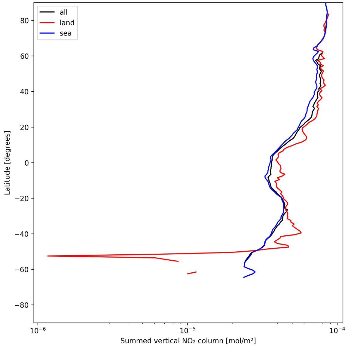
Figure 21: Zonal average of “Summed vertical NO 2 column” for 2025-06-15 to 2025-06-16.
