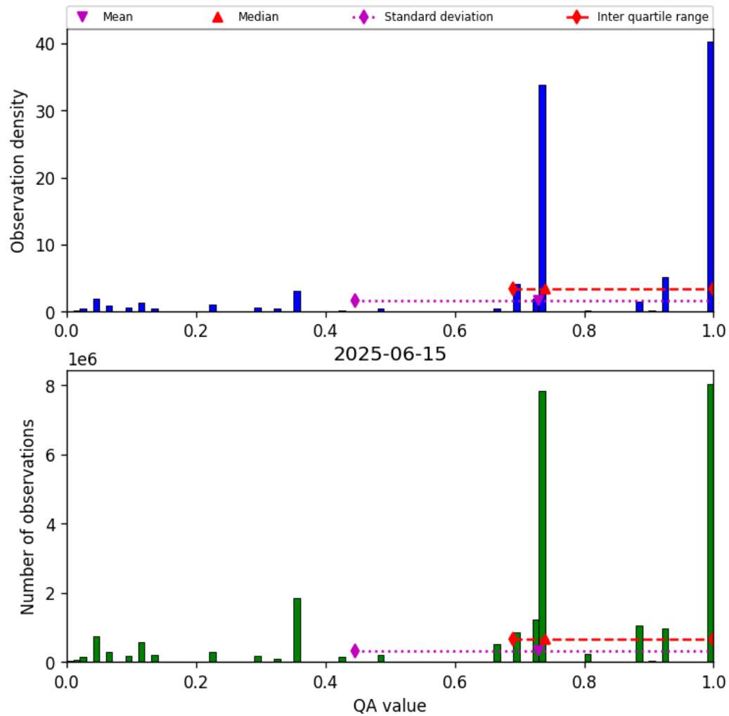
Figure 26: Histogram of “QA value” for 2025-06-15 to 2025-06-16
