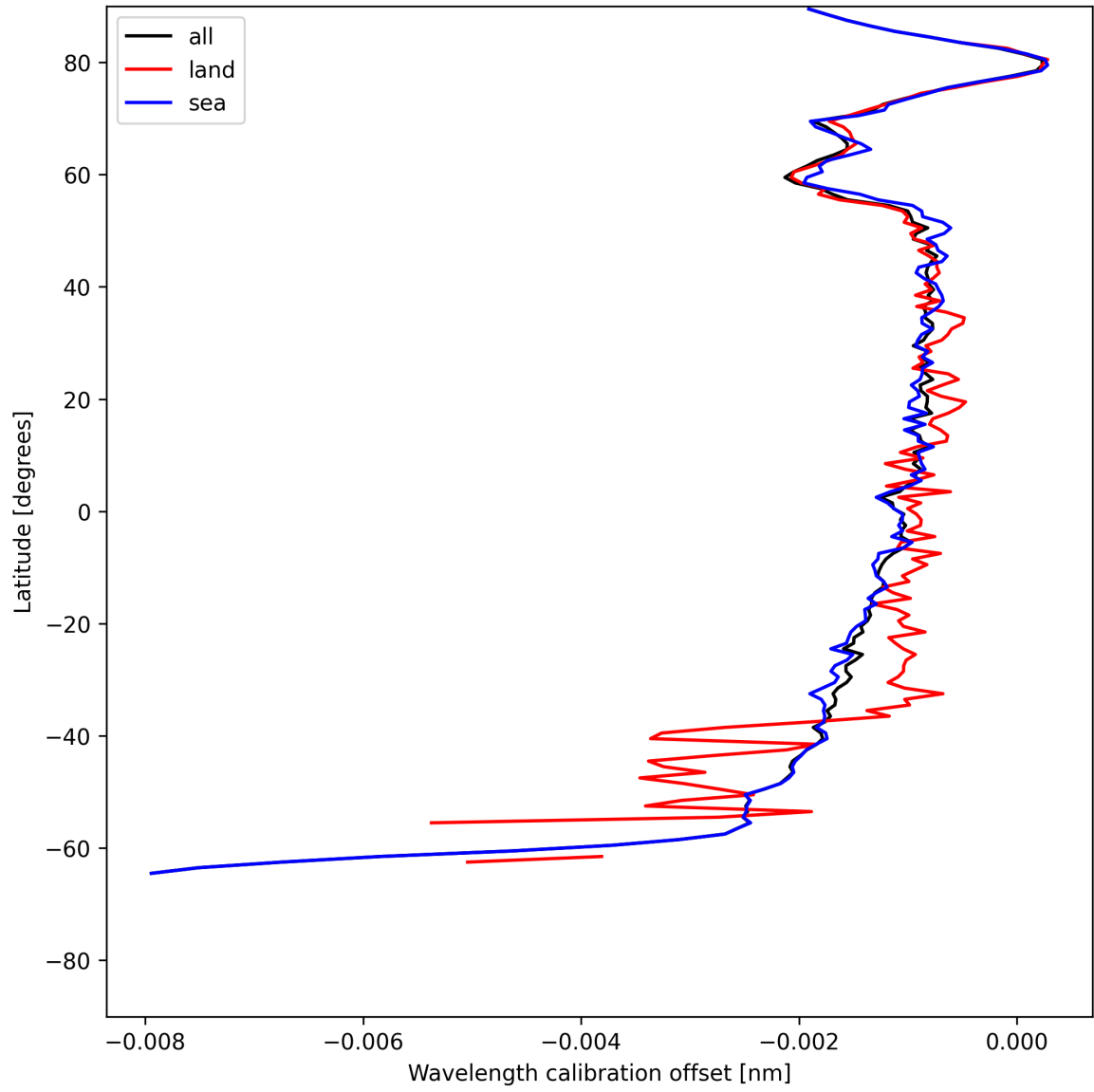
Figure 16: Zonal average of “Wavelength calibration offset” for 2025-06-15 to 2025-06-16.
