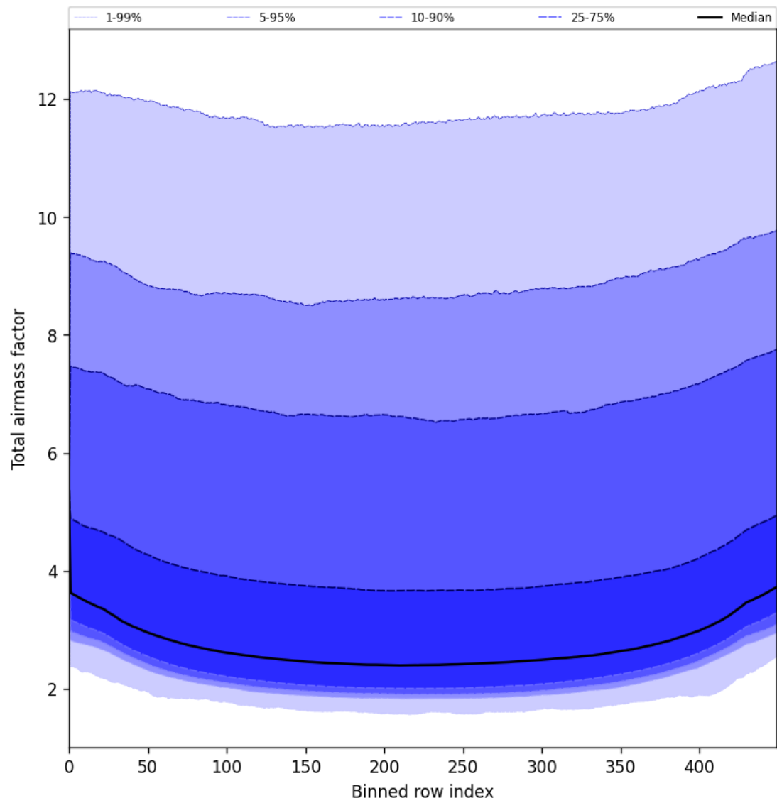
Figure 47: Along track statistics of “Total airmass factor” for 2025-06-15 to 2025-06-16
