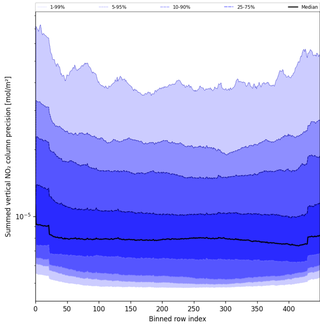
Figure 56: Along track statistics of “Summed vertical NO 2 column precision” for 2025-06-15 to 2025-06-16
