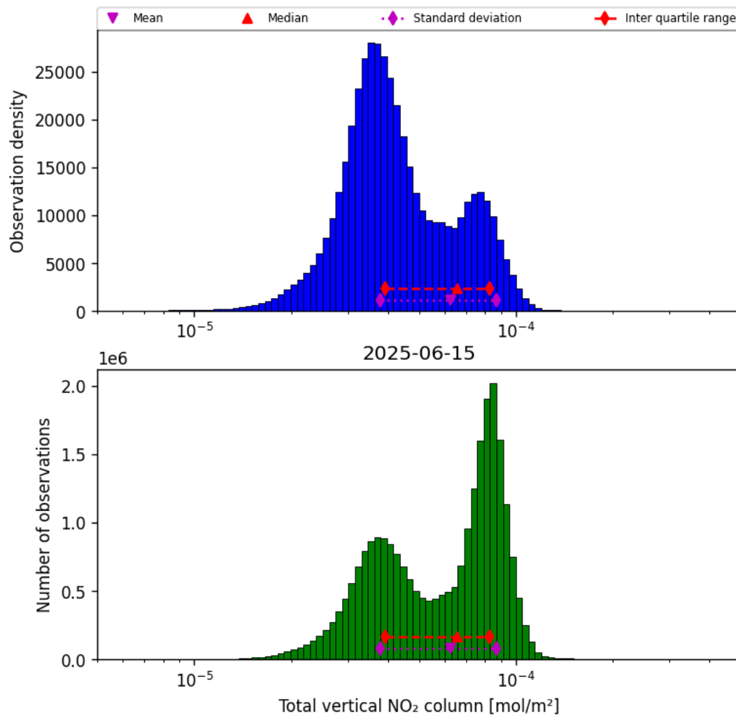
Figure 36: Histogram of “Total vertical NO 2 column” for 2025-06-15 to 2025-06-16
