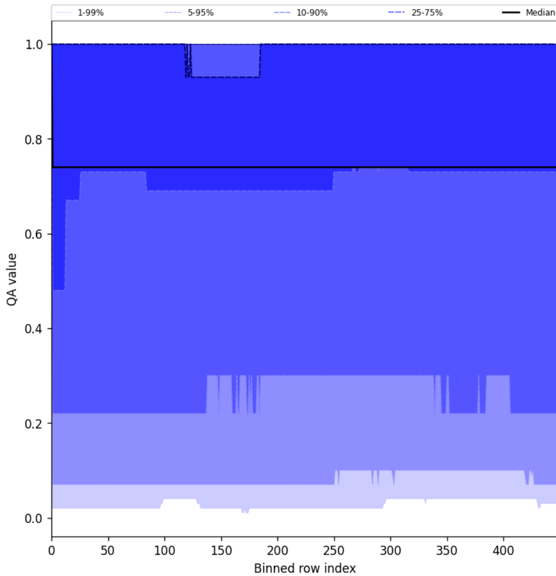
Figure 43: Along track statistics of “QA value” for 2025-06-15 to 2025-06-16
