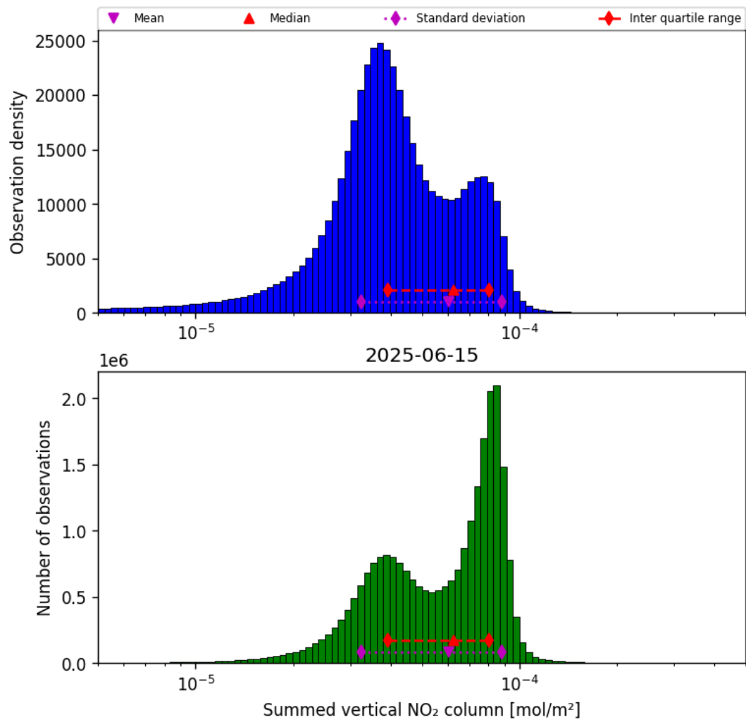
Figure 38: Histogram of “Summed vertical NO 2 column” for 2025-06-15 to 2025-06-16
