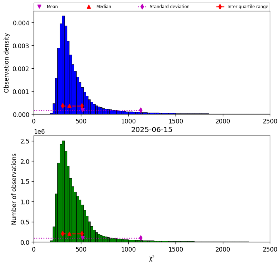
Figure 40: Histogram of “ \chi^2 ” for 2025-06-15 to 2025-06-16
