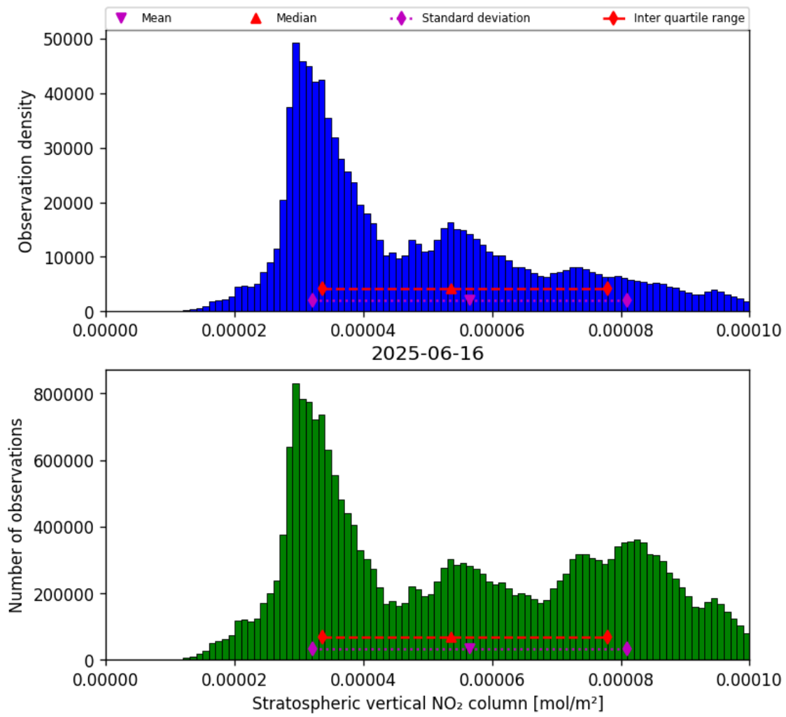
Figure 34: Histogram of “Stratospheric vertical NO 2 column” for 2025-06-16 to 2025-06-17
