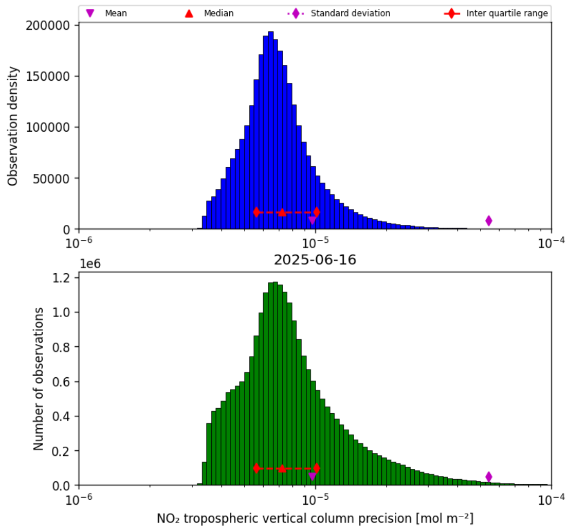
Figure 28: Histogram of “NO 2 tropospheric vertical column precision” for 2025-06-16 to 2025-06-17
