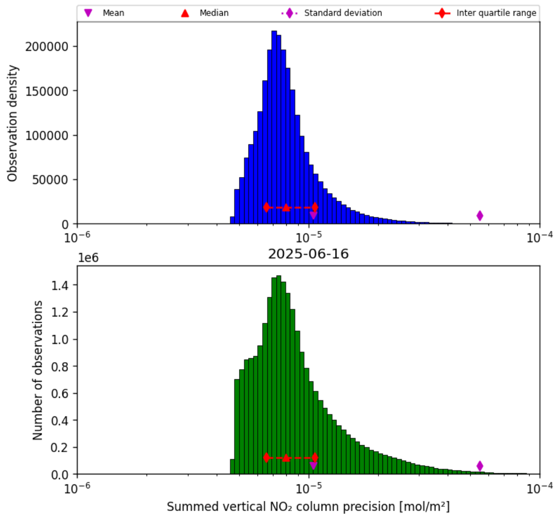
Figure 39: Histogram of “Summed vertical NO 2 column precision” for 2025-06-16 to 2025-06-17
