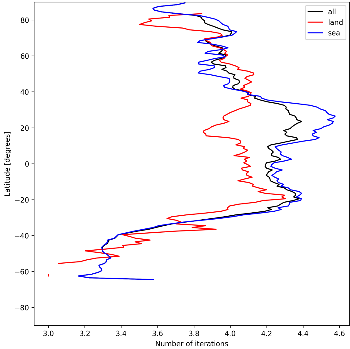
Figure 15: Zonal average of “Number of iterations” for 2025-06-16 to 2025-06-17.
