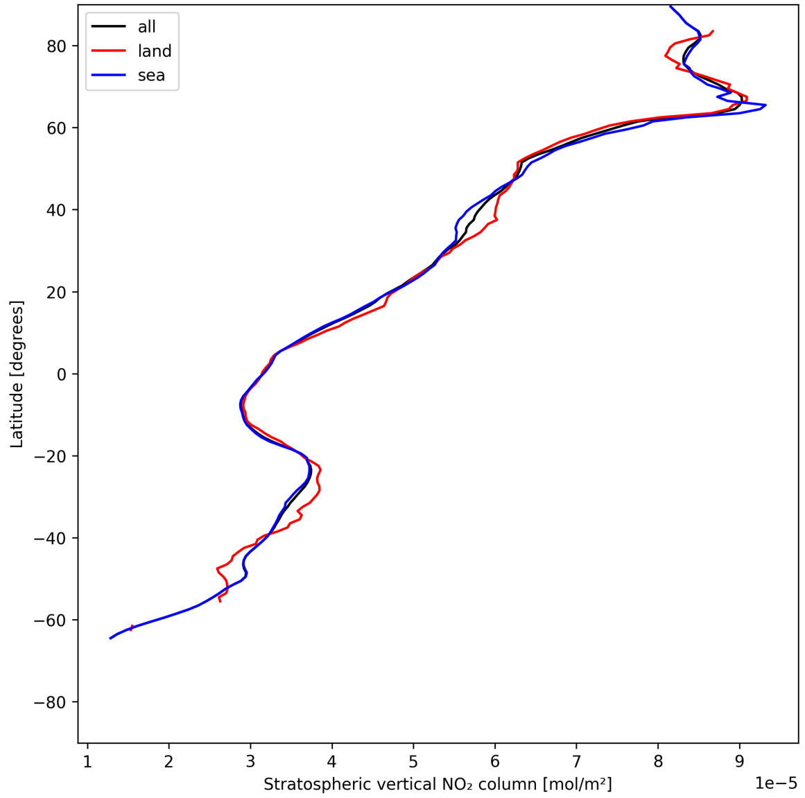
Figure 17: Zonal average of “Stratospheric vertical NO 2 column” for 2025-06-16 to 2025-06-17.
