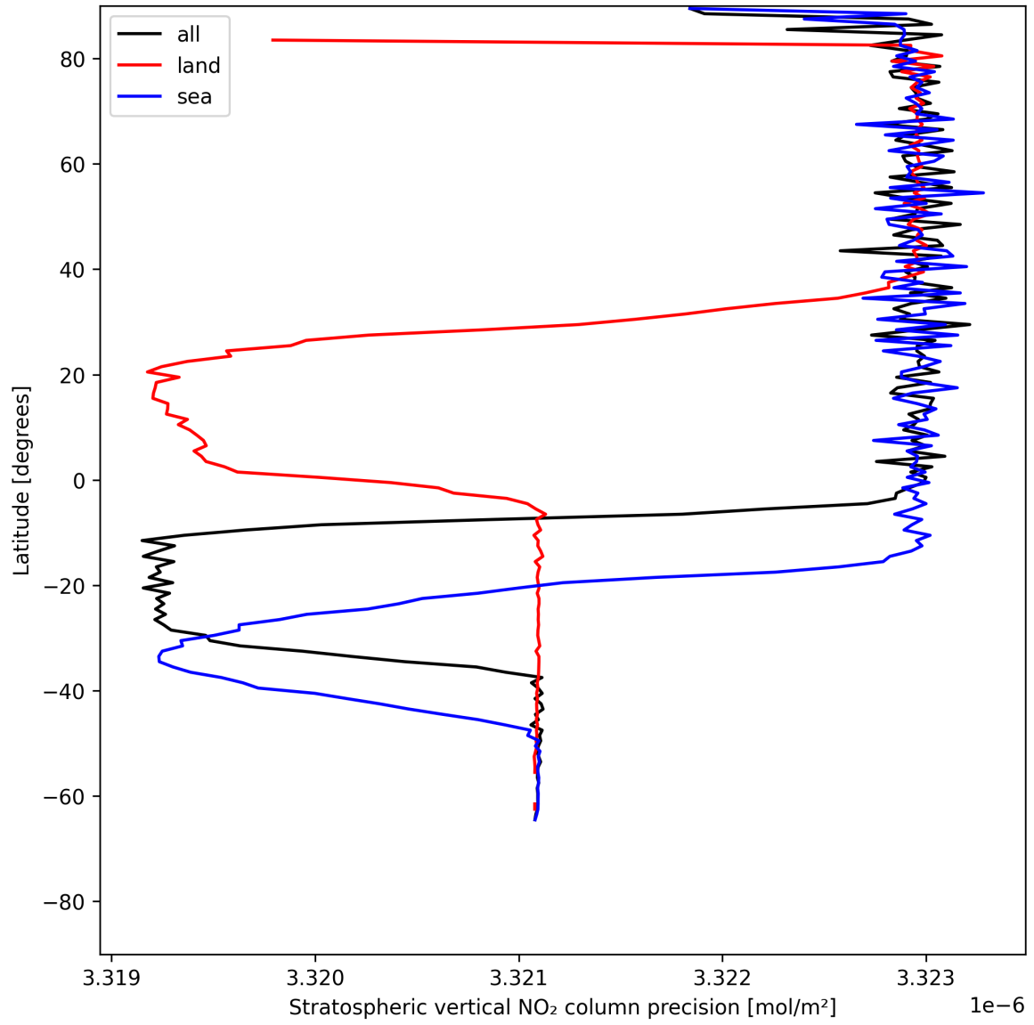
Figure 18: Zonal average of “Stratospheric vertical NO 2 column precision” for 2025-06-16 to 2025-06-17.
