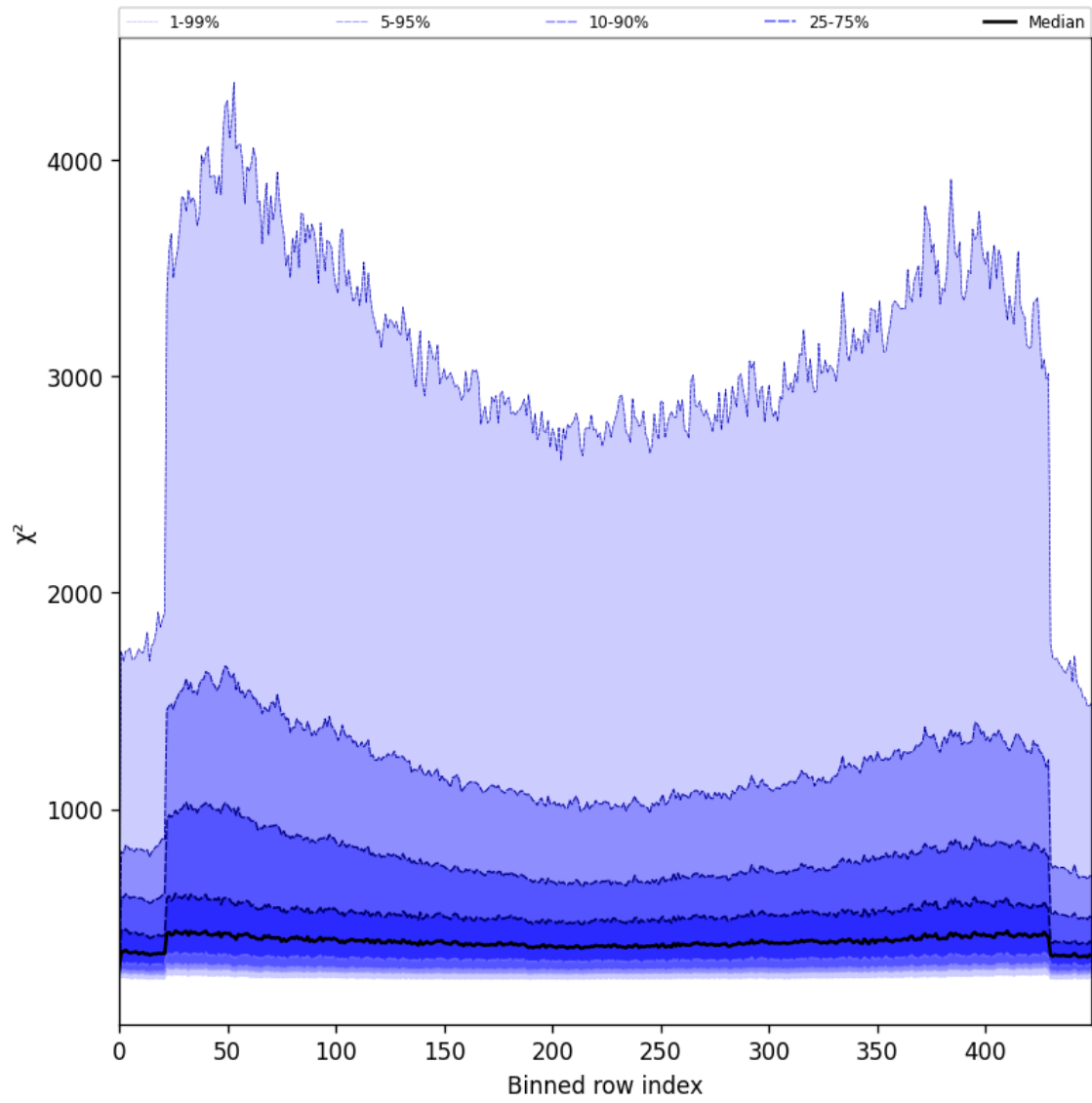
Figure 57: Along track statistics of “ \chi^2 ” for 2025-06-16 to 2025-06-17
