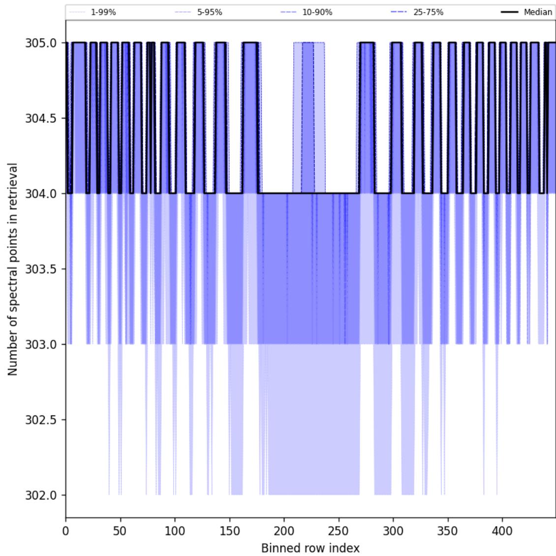
Figure 48: Along track statistics of “Number of spectral points in retrieval” for 2025-06-16 to 2025-06-17
