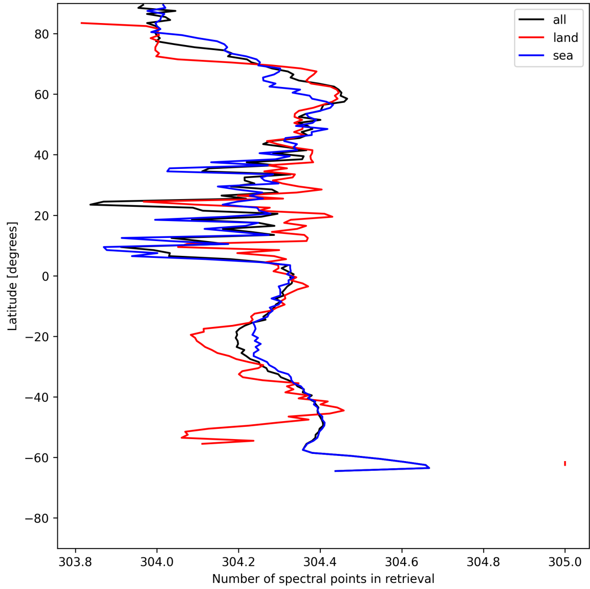
Figure 14: Zonal average of “Number of spectral points in retrieval” for 2025-06-16 to 2025-06-17.
