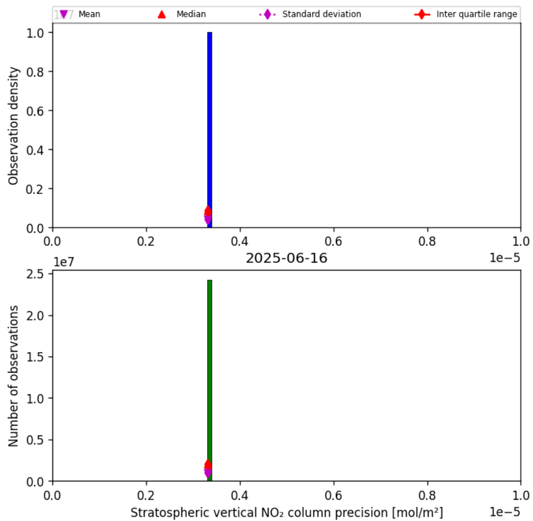
Figure 35: Histogram of “Stratospheric vertical NO 2 column precision” for 2025-06-16 to 2025-06-17
