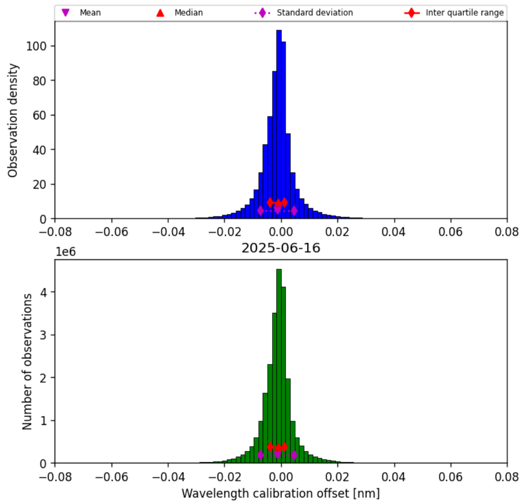
Figure 33: Histogram of “Wavelength calibration offset” for 2025-06-16 to 2025-06-17
