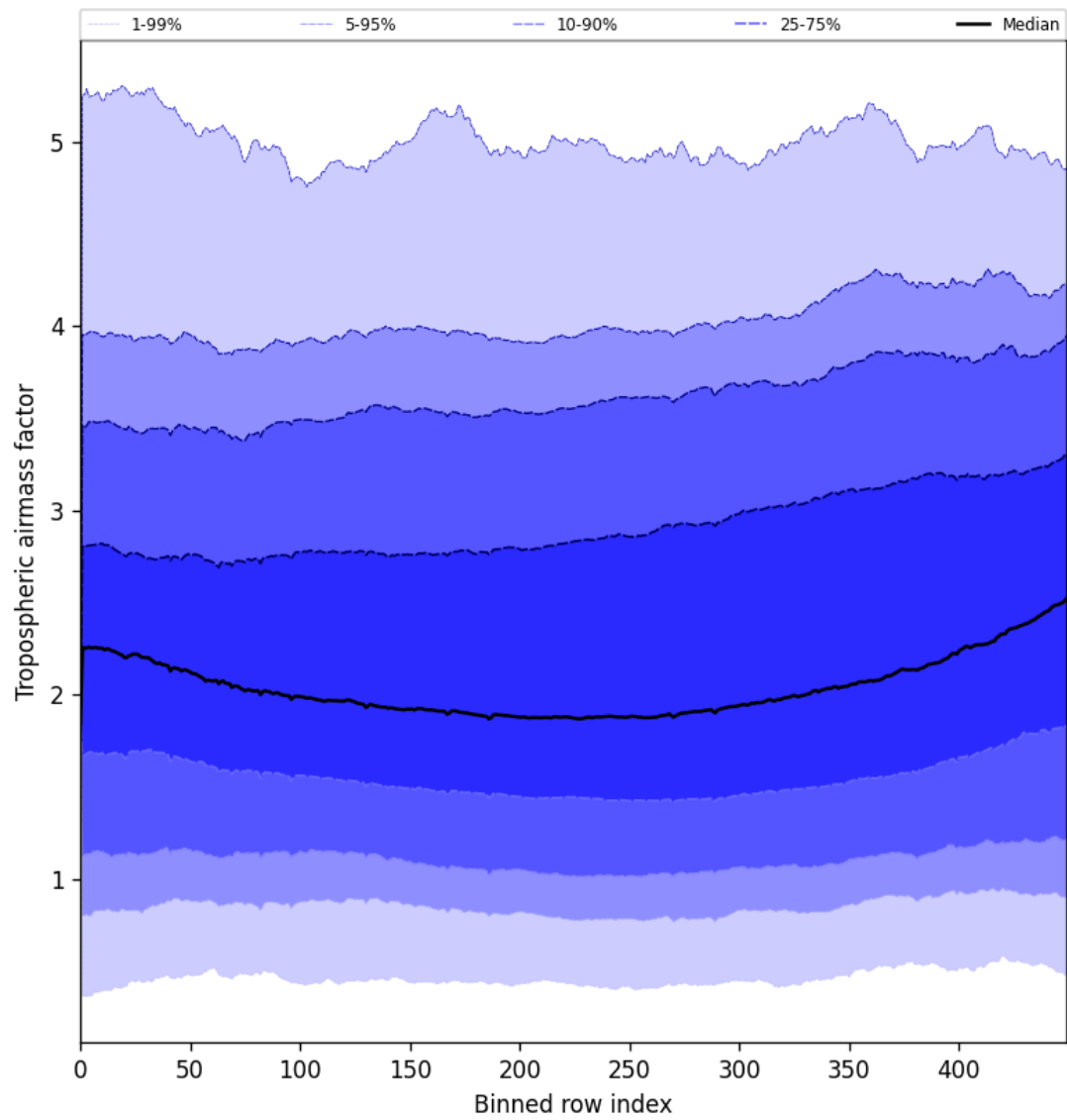
Figure 46: Along track statistics of “Tropospheric airmass factor” for 2025-06-16 to 2025-06-17
