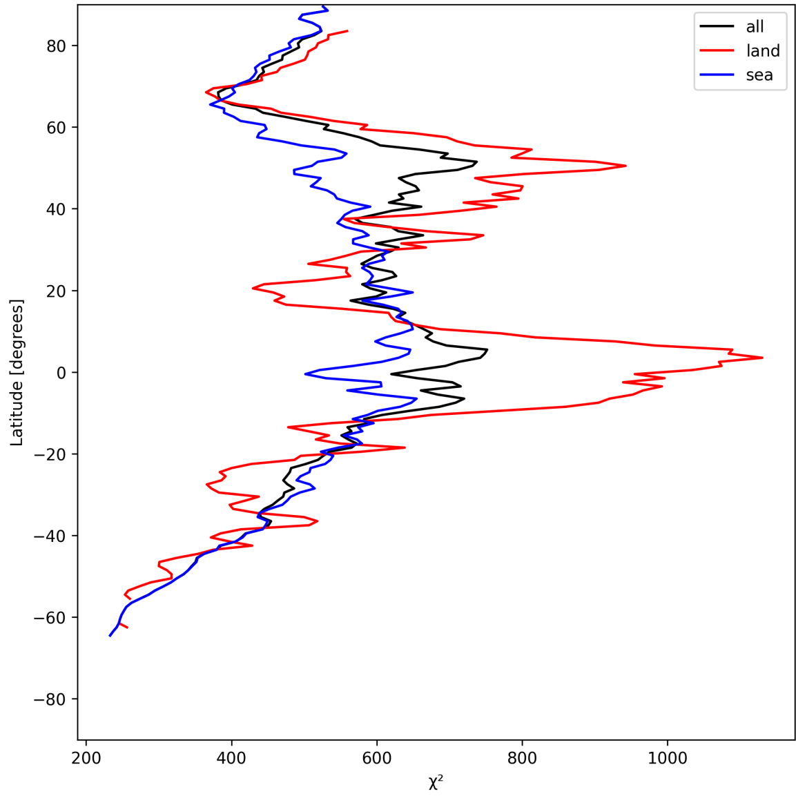
Figure 23: Zonal average of “ \chi^2 ” for 2025-06-16 to 2025-06-17.
