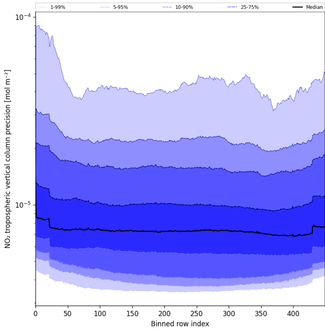
Figure 45: Along track statistics of “NO 2 tropospheric vertical column precision” for 2025-06-16 to 2025-06-17
