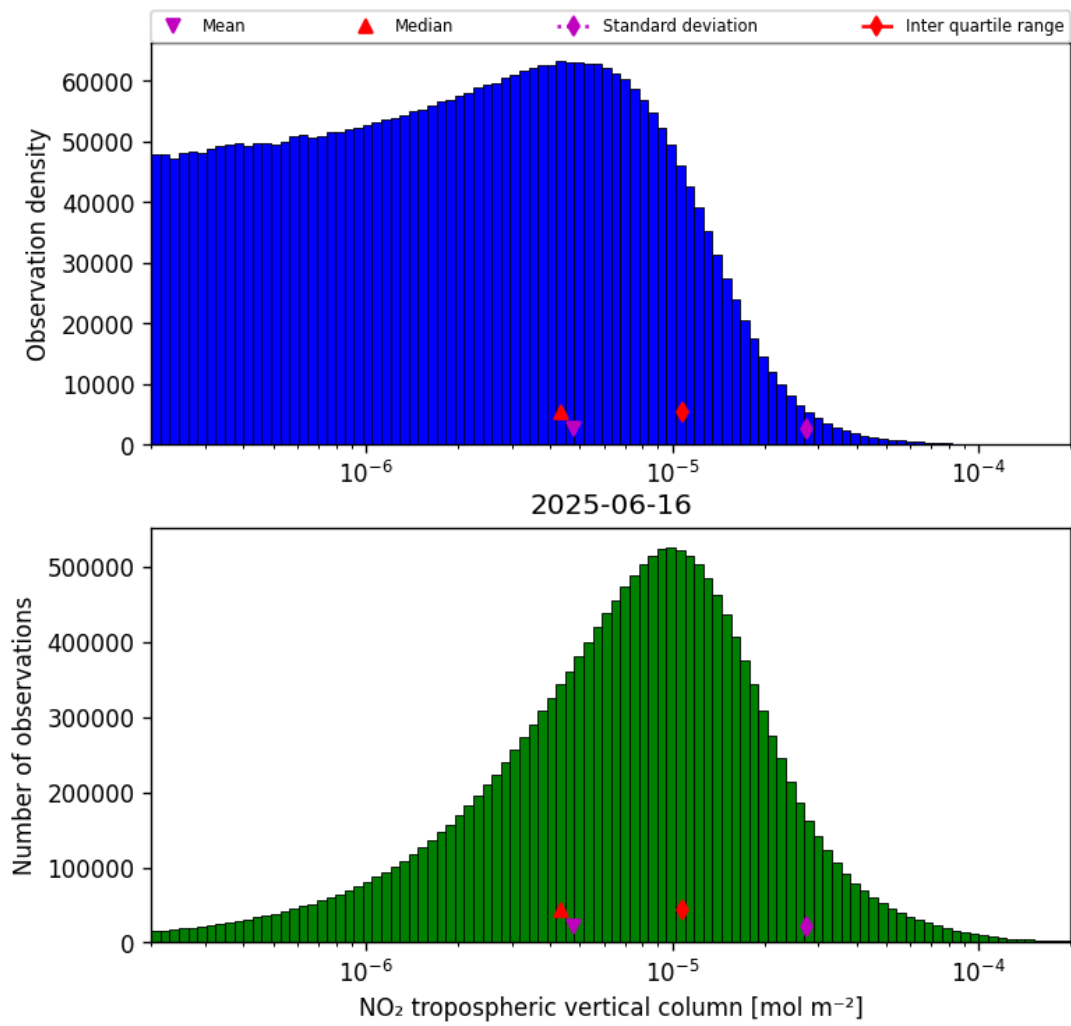
Figure 27: Histogram of “NO 2 tropospheric vertical column” for 2025-06-16 to 2025-06-17
