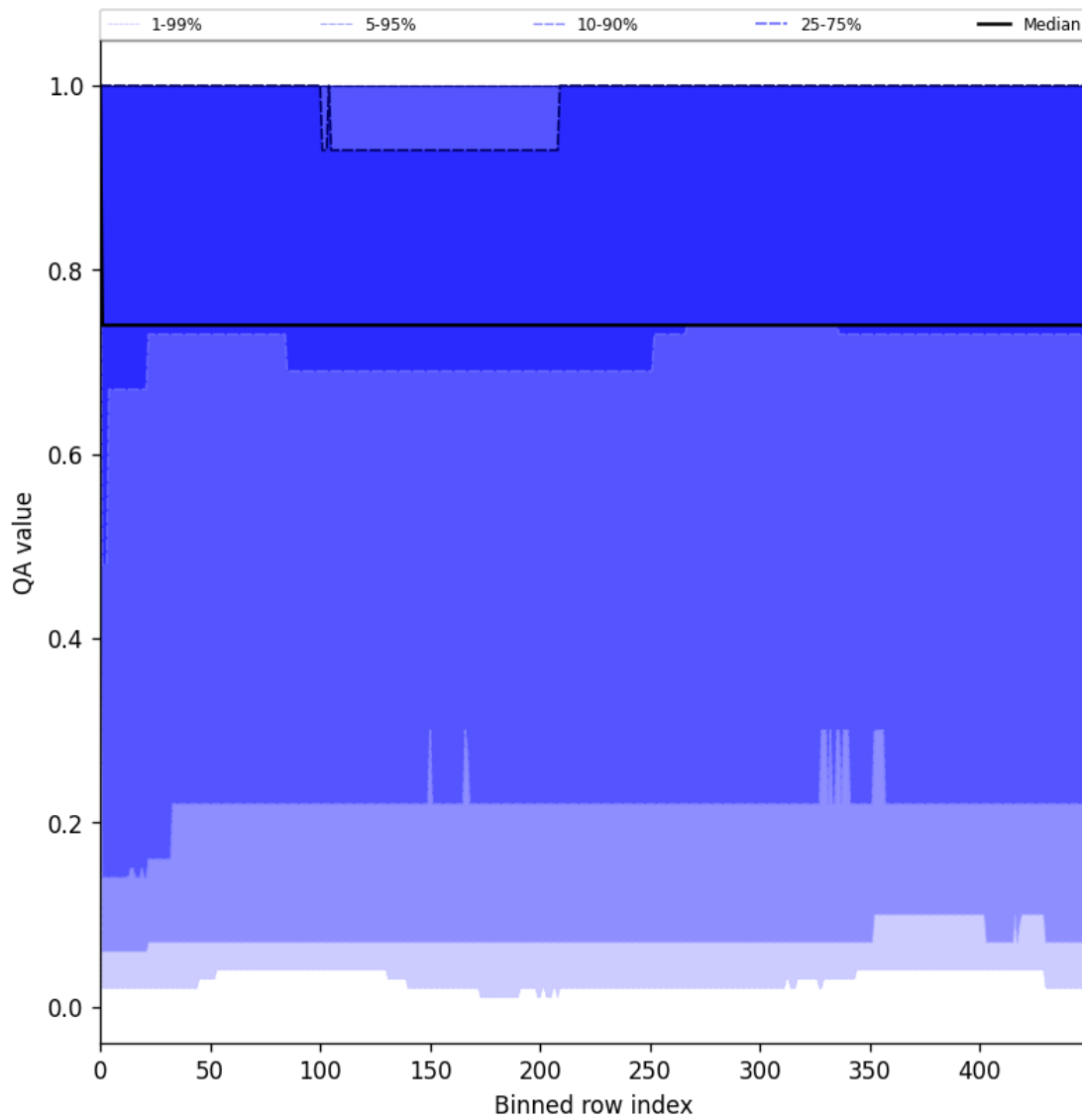
Figure 43: Along track statistics of “QA value” for 2025-06-16 to 2025-06-17
