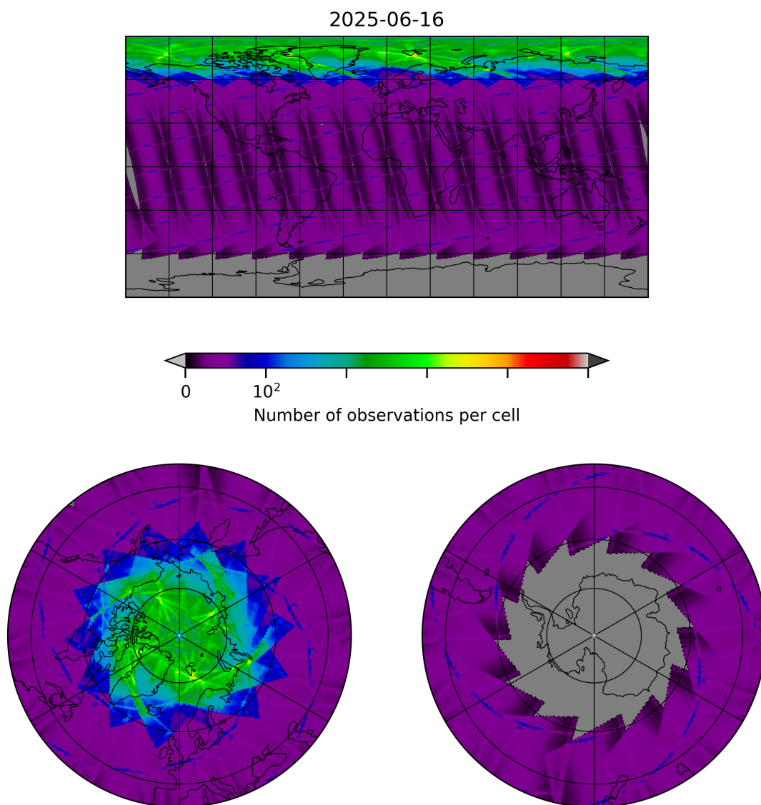
Figure 8: Map of the number of observations for 2025-06-16 to 2025-06-17
