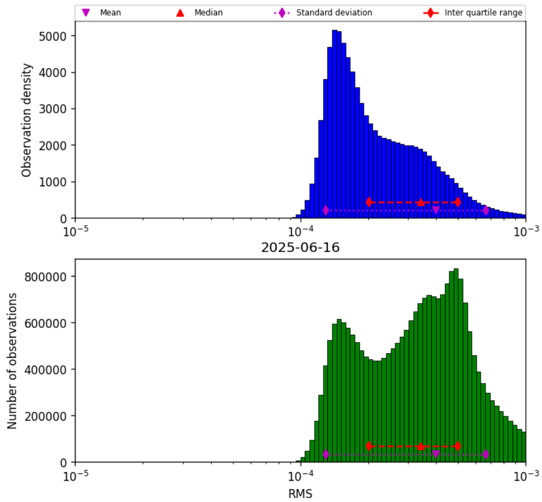
Figure 41: Histogram of “RMS” for 2025-06-16 to 2025-06-17
