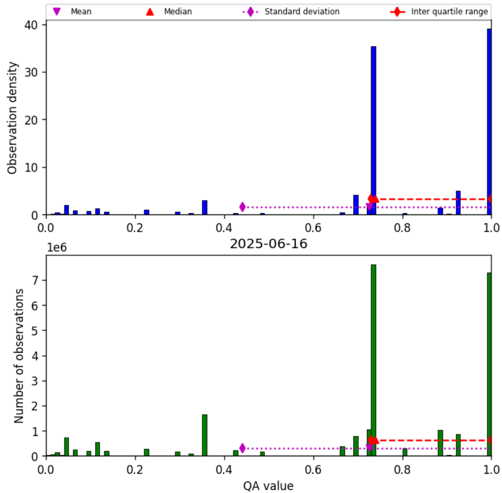
Figure 26: Histogram of “QA value” for 2025-06-16 to 2025-06-17
