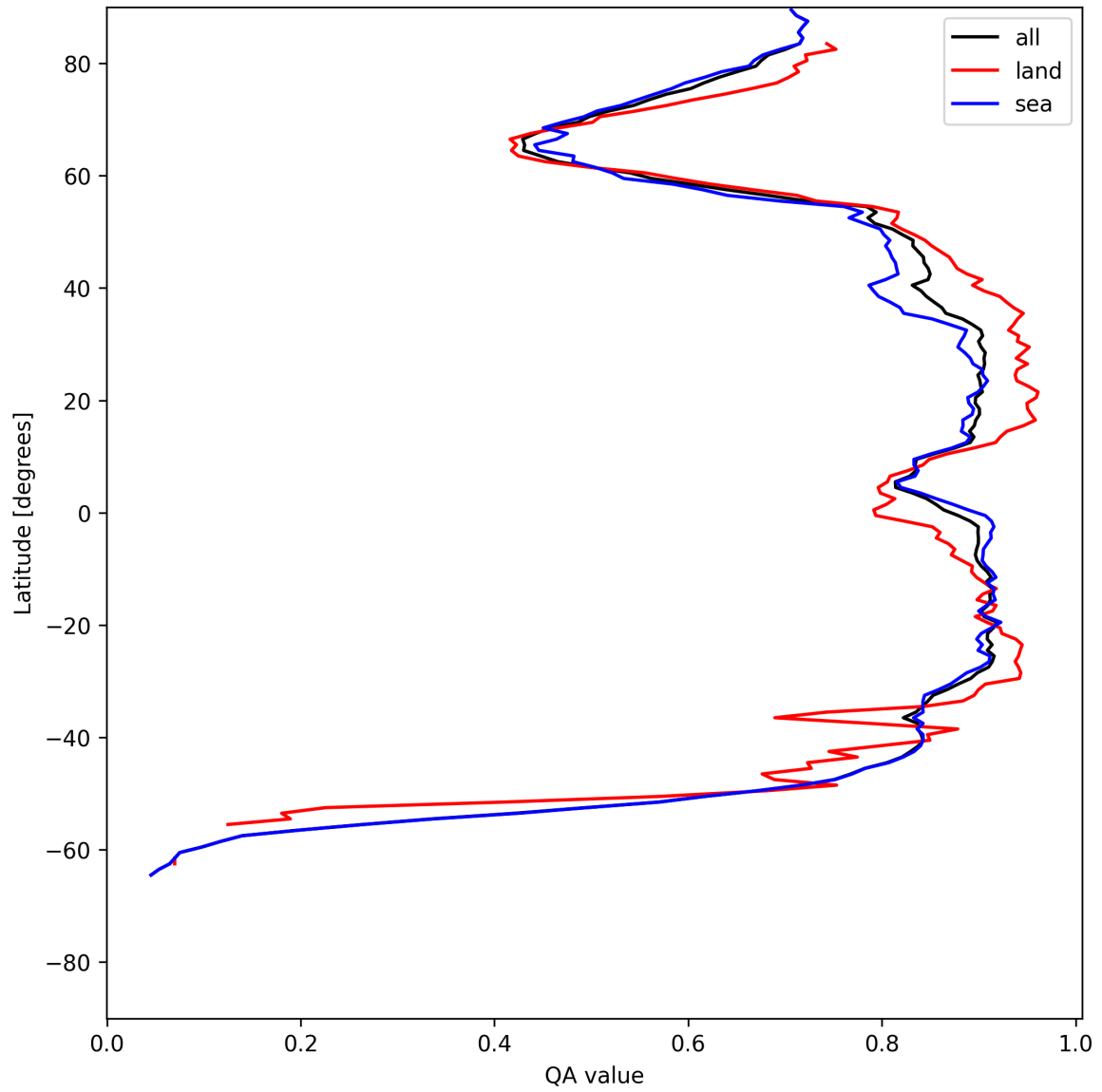
Figure 9: Zonal average of “QA value” for 2025-06-16 to 2025-06-17.
