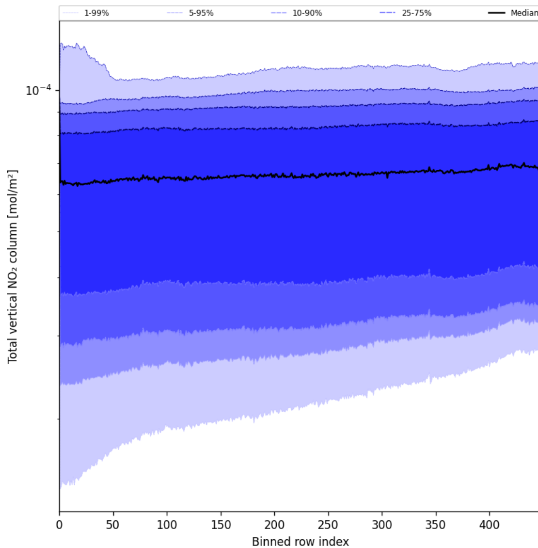
Figure 53: Along track statistics of “Total vertical NO 2 column” for 2025-06-16 to 2025-06-17
