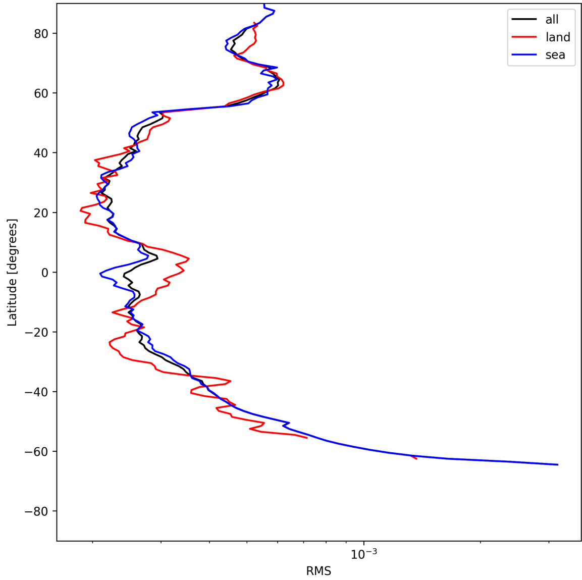
Figure 24: Zonal average of “RMS” for 2025-06-16 to 2025-06-17.
