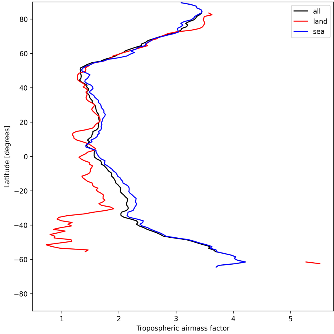
Figure 12: Zonal average of “Tropospheric air mass factor” for 2025-06-16 to 2025-06-17.
