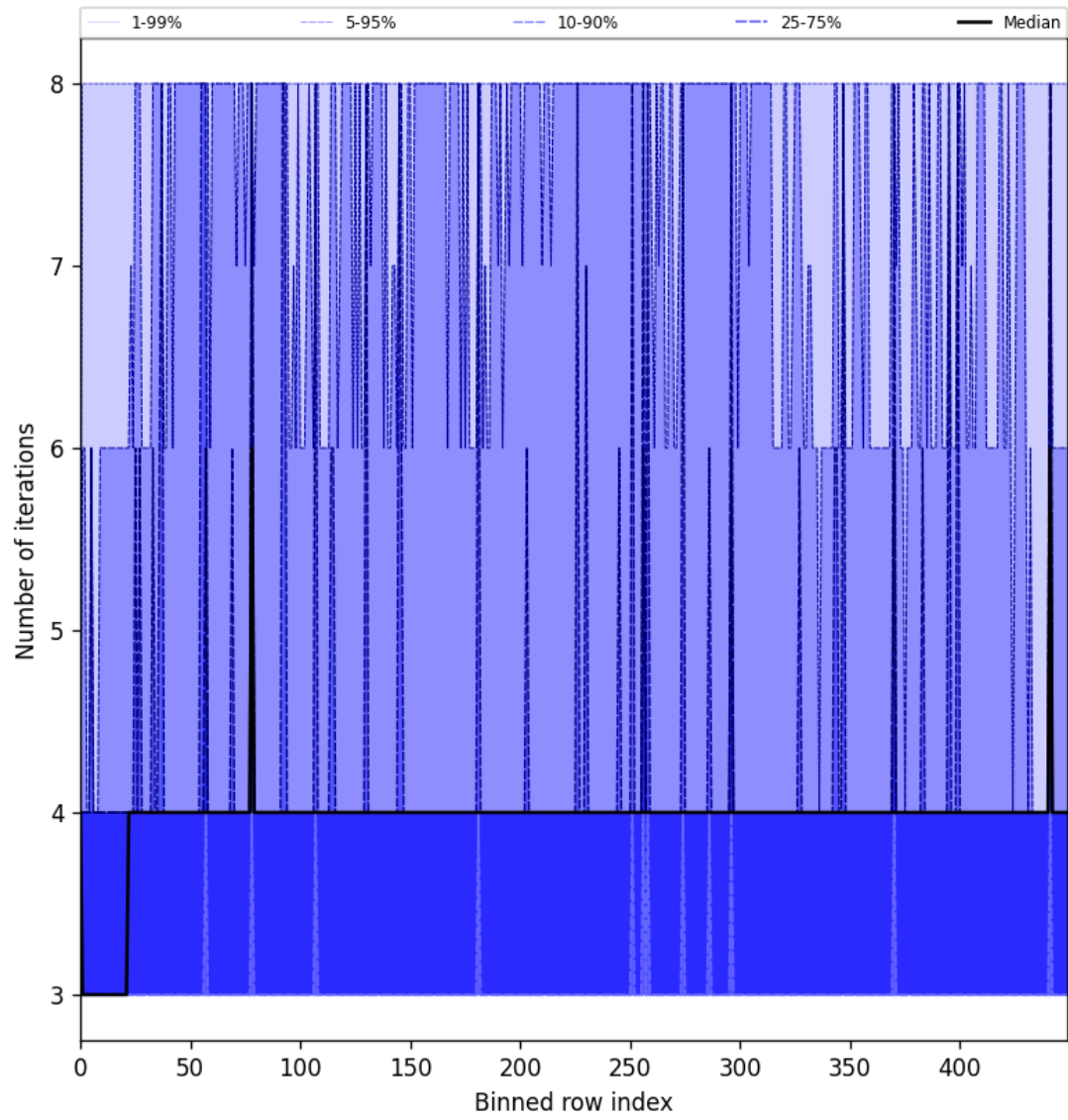
Figure 49: Along track statistics of “Number of iterations” for 2025-06-16 to 2025-06-17
