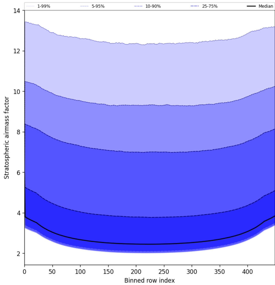
Figure 59: Along track statistics of “Stratospheric airmass factor” for 2025-06-16 to 2025-06-17
