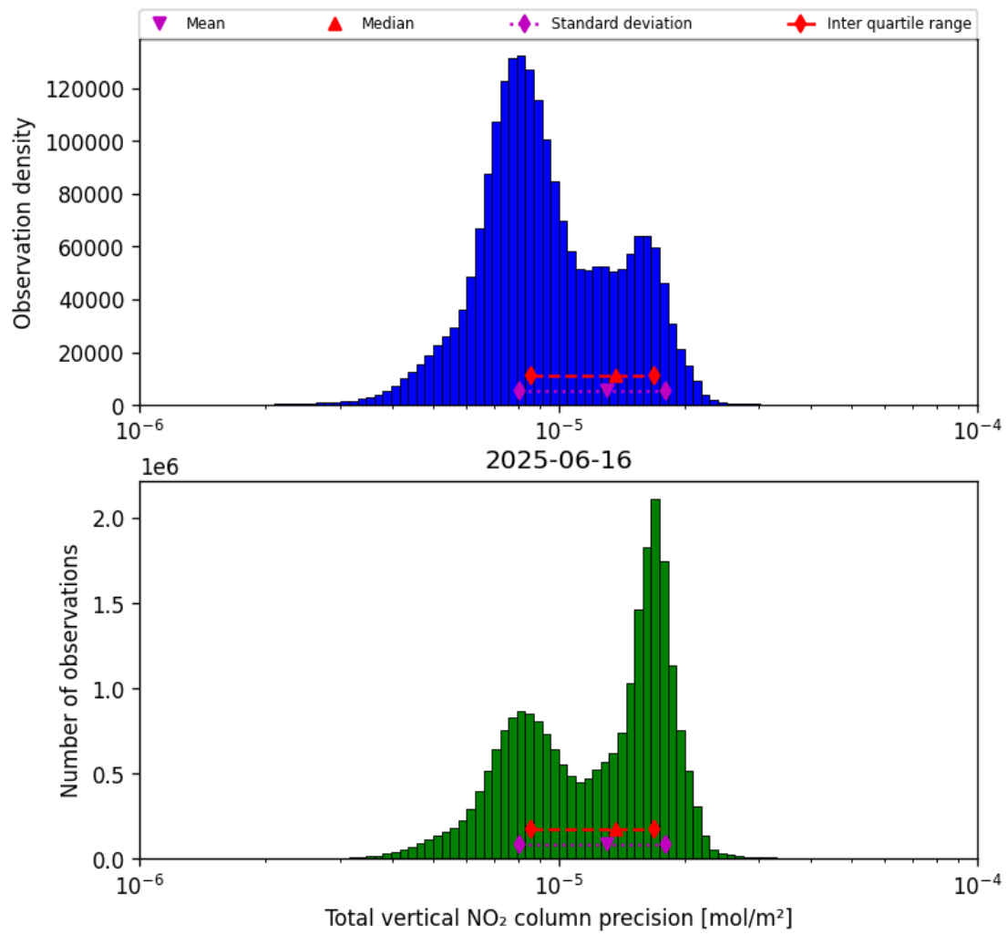
Figure 37: Histogram of “Total vertical NO 2 column precision” for 2025-06-16 to 2025-06-17
