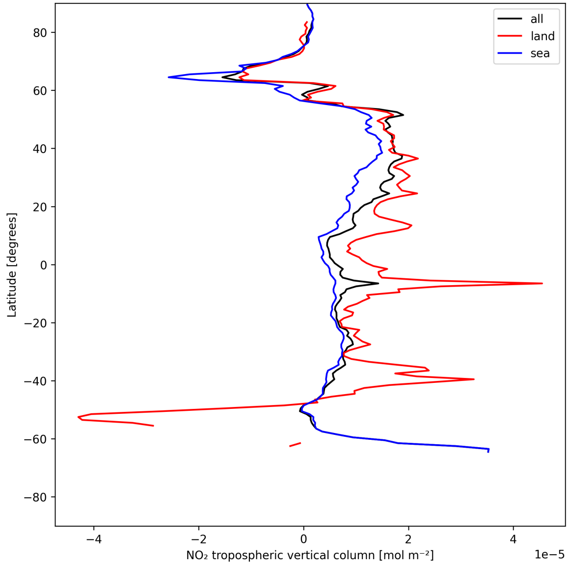
Figure 10: Zonal average of “NO 2 tropospheric vertical column” for 2025-06-16 to 2025-06-17.
