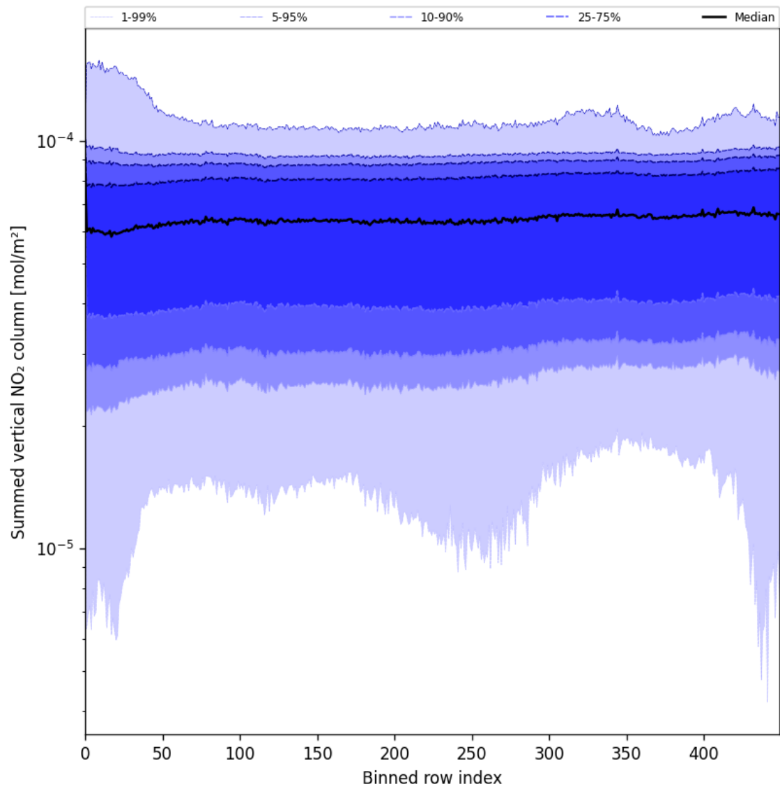
Figure 55: Along track statistics of “Summed vertical NO 2 column” for 2025-06-16 to 2025-06-17
