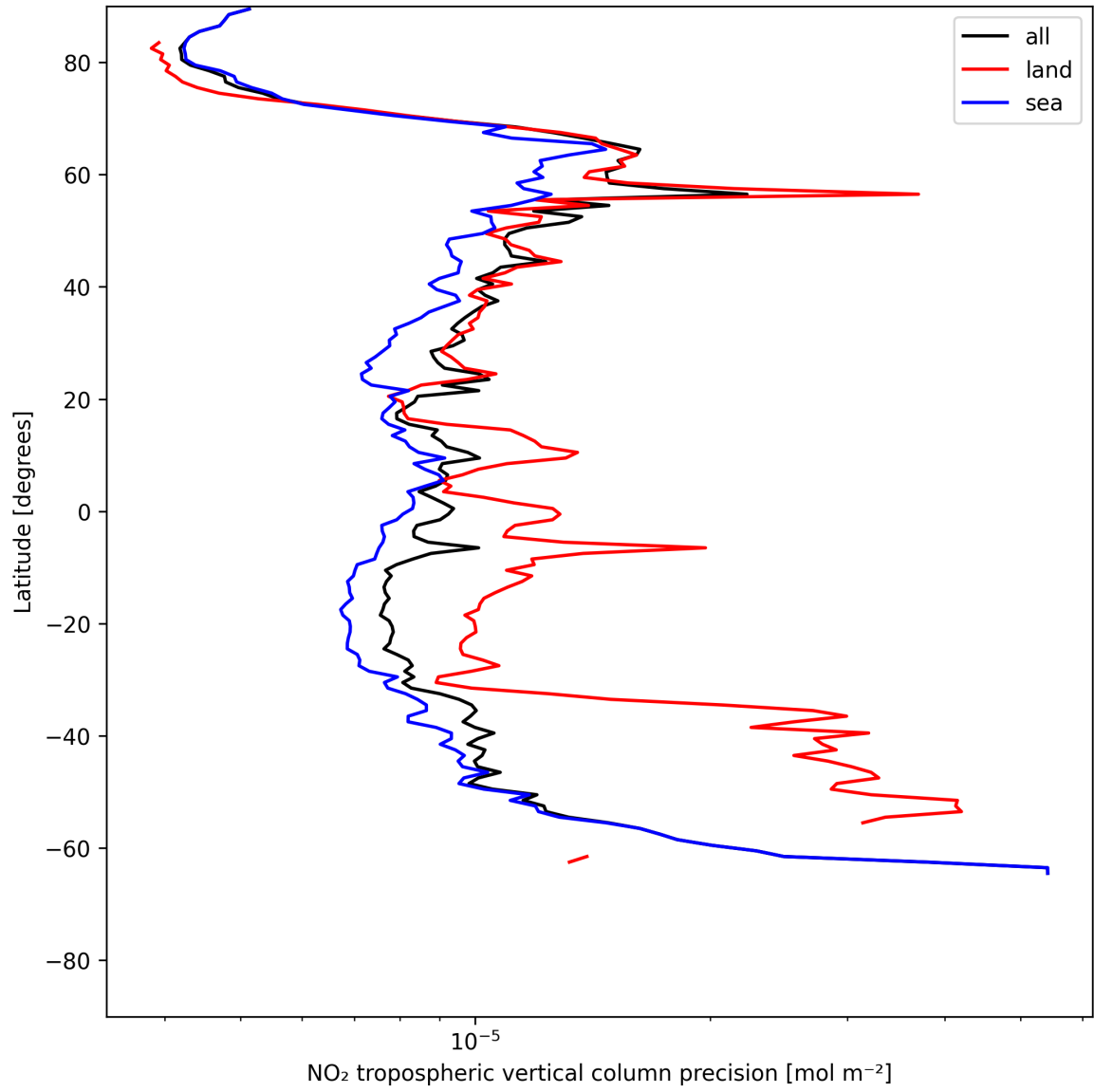
Figure 11: Zonal average of “NO 2 tropospheric vertical column precision” for 2025-06-16 to 2025-06-17.
