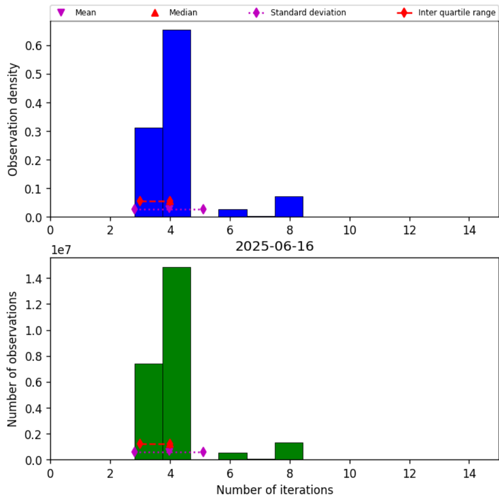
Figure 32: Histogram of “Number of iterations” for 2025-06-16 to 2025-06-17
