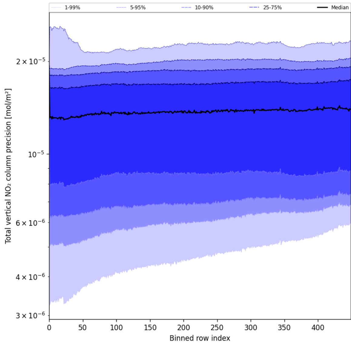
Figure 54: Along track statistics of “Total vertical NO 2 column precision” for 2025-06-16 to 2025-06-17
