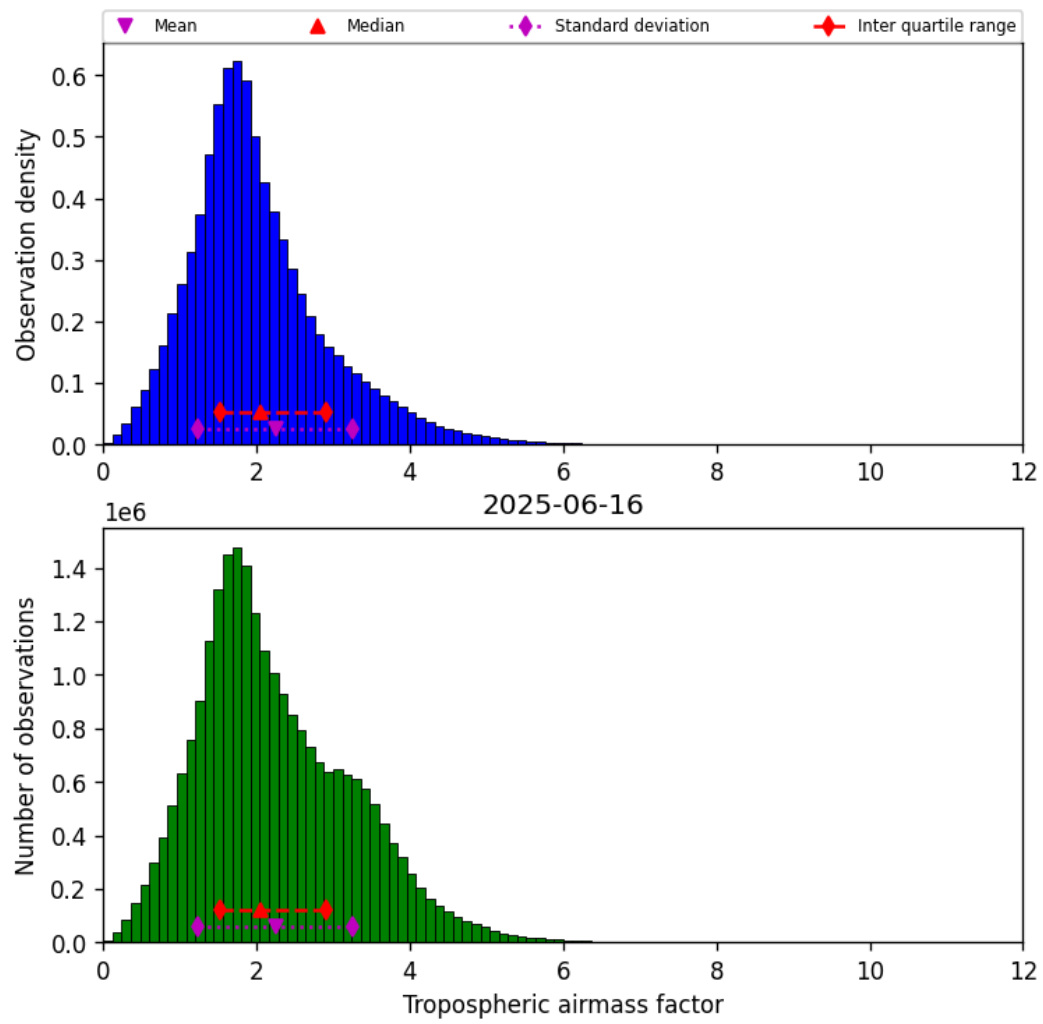
Figure 29: Histogram of “Tropospheric airmass factor” for 2025-06-16 to 2025-06-17
