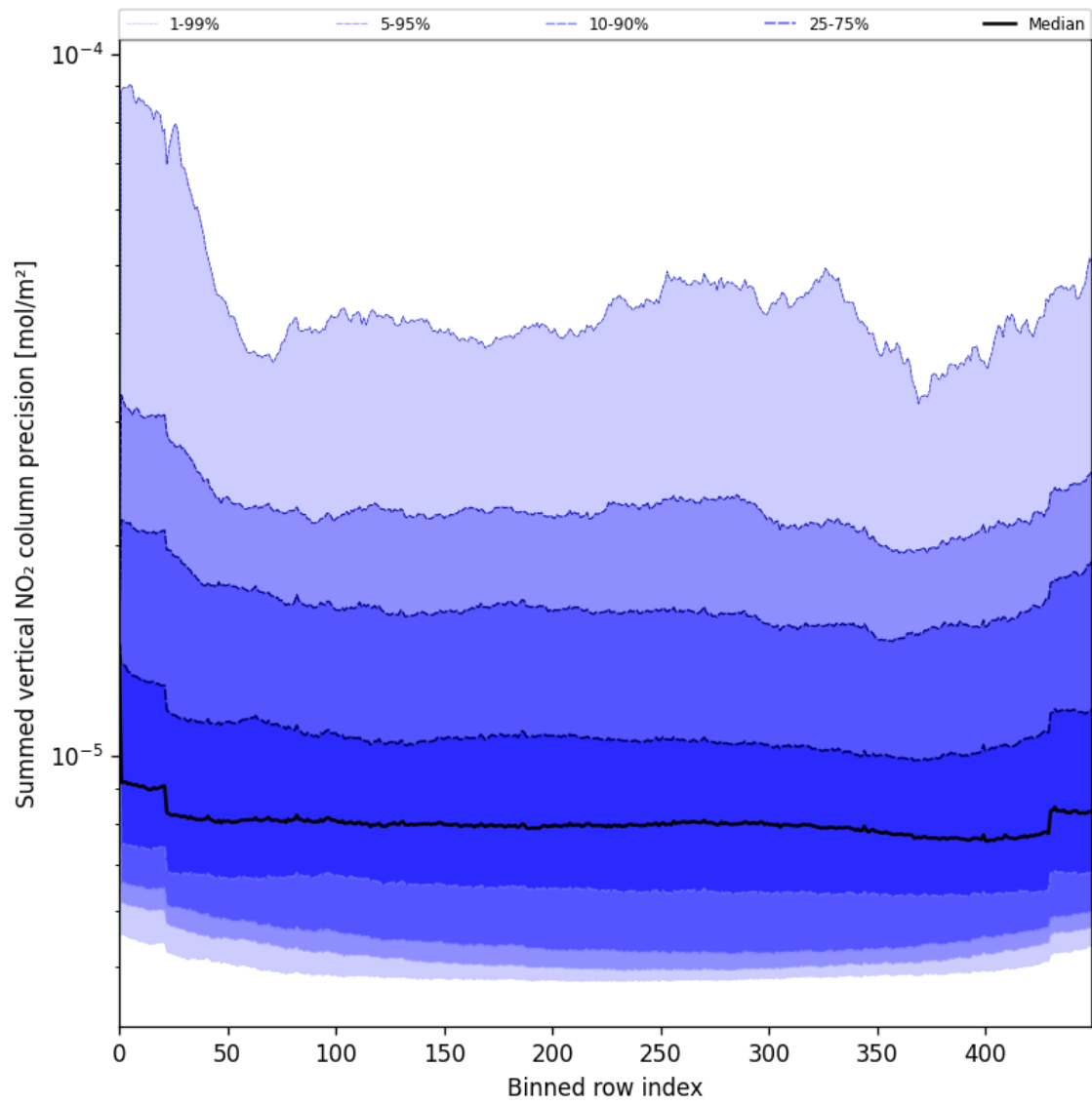
Figure 56: Along track statistics of “Summed vertical NO 2 column precision” for 2025-06-16 to 2025-06-17
