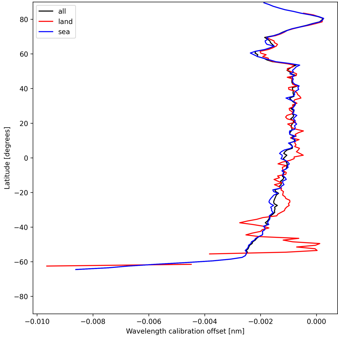
Figure 16: Zonal average of “Wavelength calibration offset” for 2025-06-16 to 2025-06-17.
