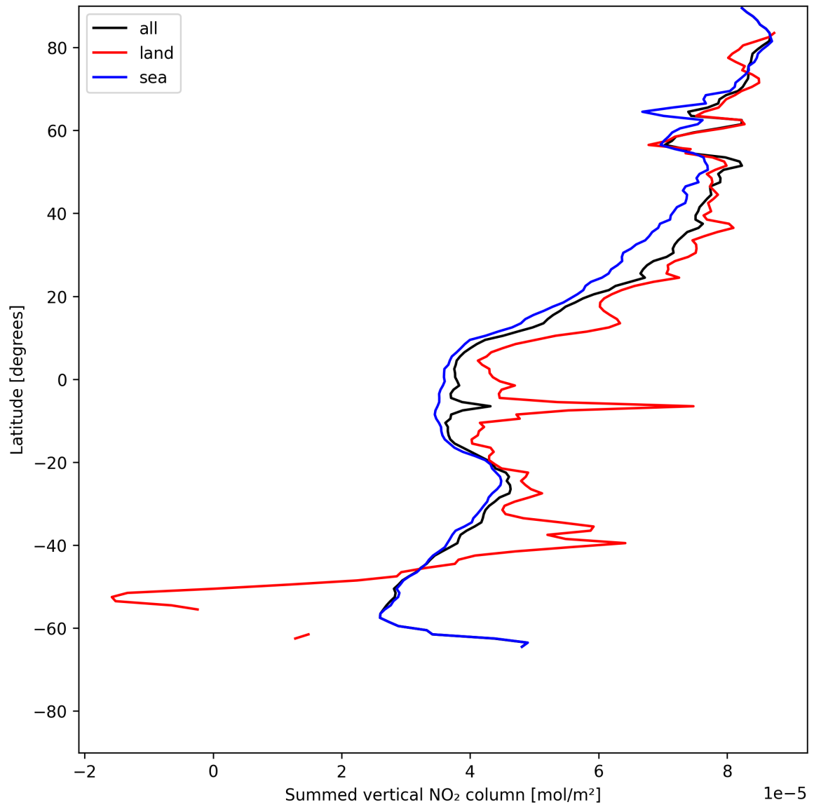
Figure 21: Zonal average of “Summed vertical NO 2 column” for 2025-06-16 to 2025-06-17.
