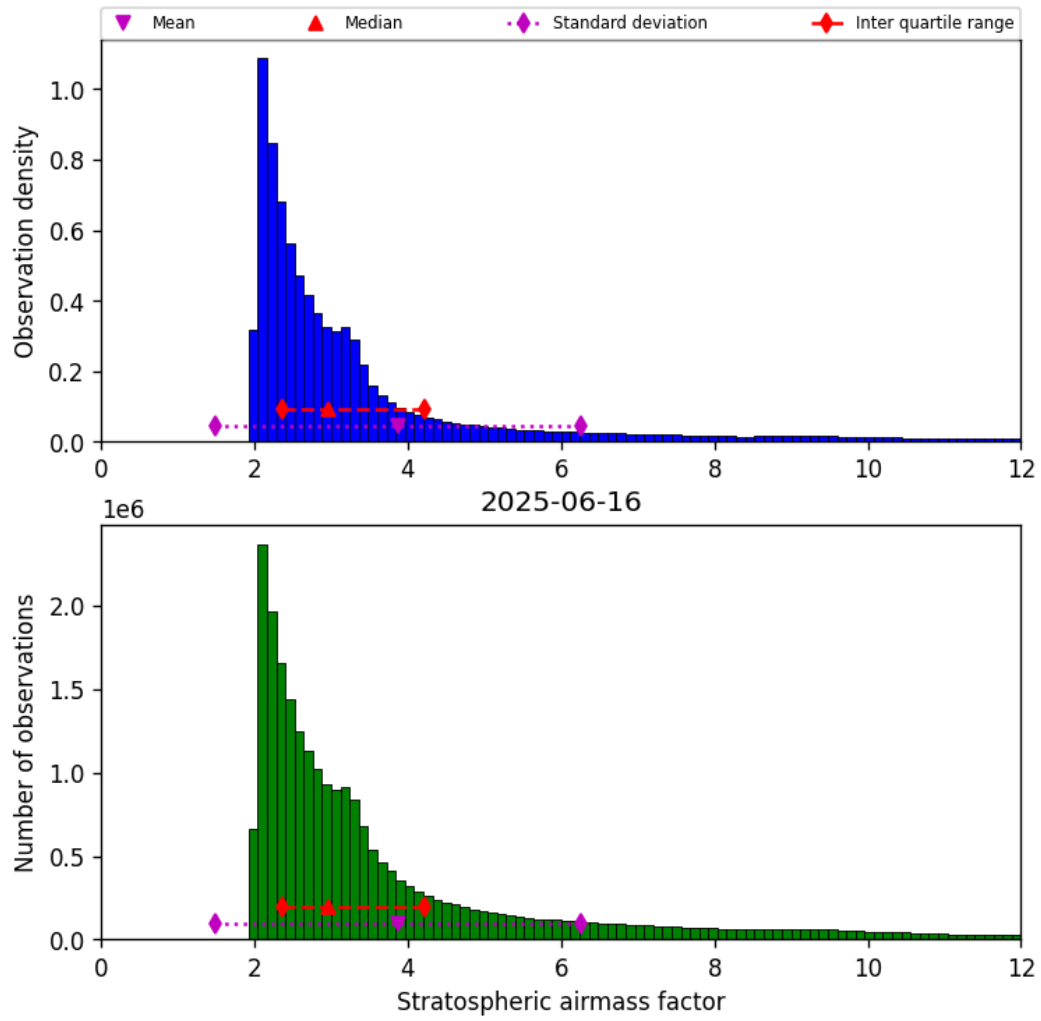
Figure 42: Histogram of “Stratospheric airmass factor” for 2025-06-16 to 2025-06-17
