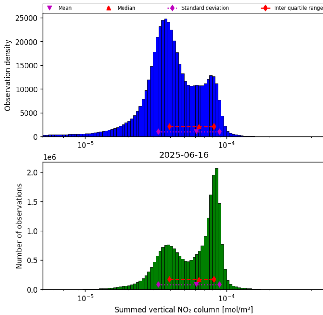
Figure 38: Histogram of “Summed vertical NO 2 column” for 2025-06-16 to 2025-06-17
