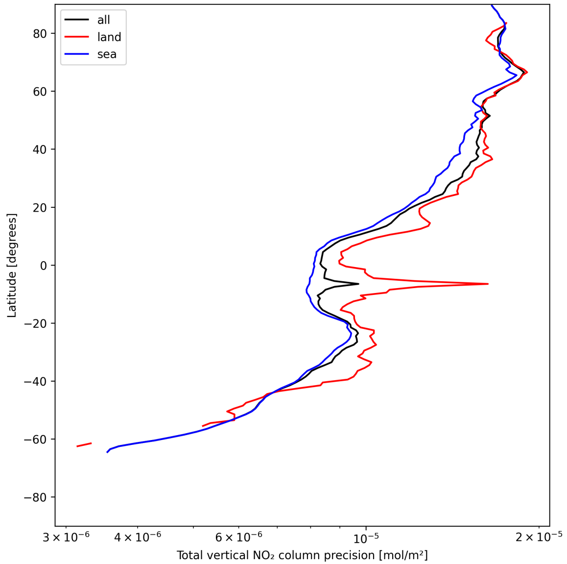
Figure 20: Zonal average of “Total vertical NO 2 column precision” for 2025-06-16 to 2025-06-17.
