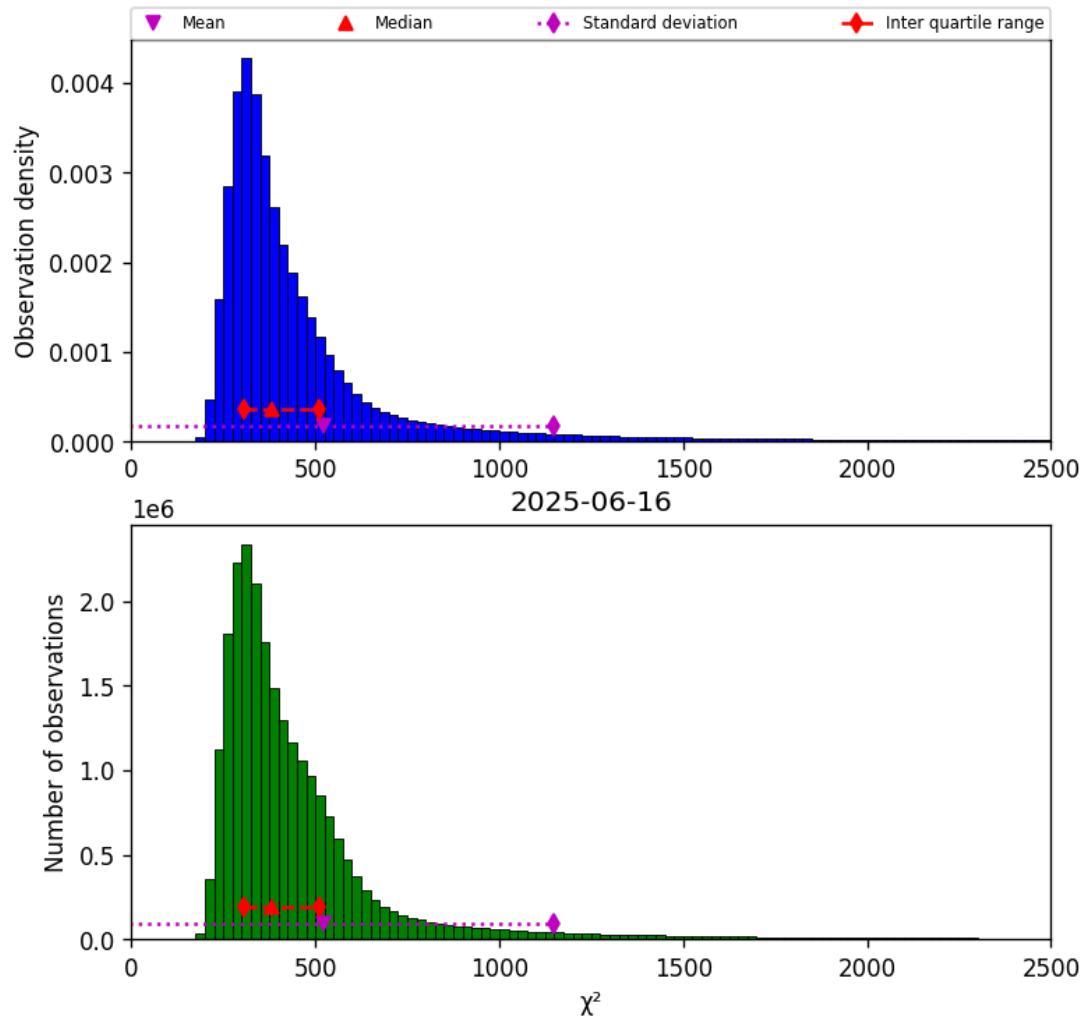
Figure 40: Histogram of “ \chi^2 ” for 2025-06-16 to 2025-06-17
