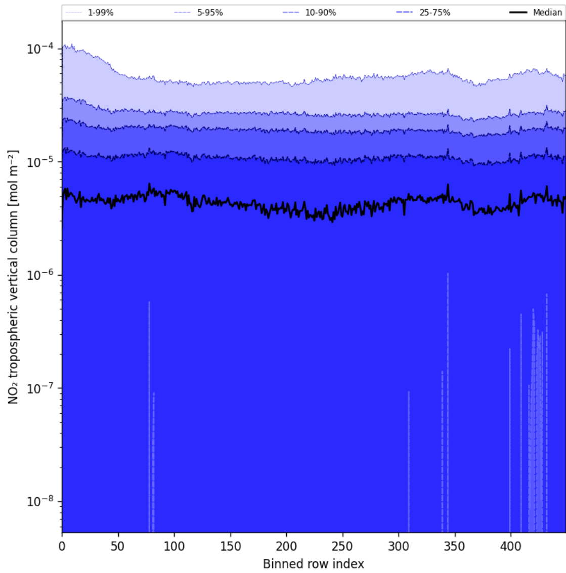
Figure 44: Along track statistics of “NO 2 tropospheric vertical column” for 2025-06-16 to 2025-06-17
