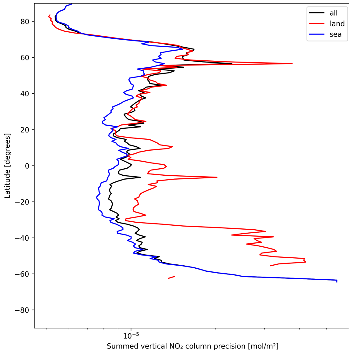
Figure 22: Zonal average of “Summed vertical NO 2 column precision” for 2025-06-16 to 2025-06-17.
