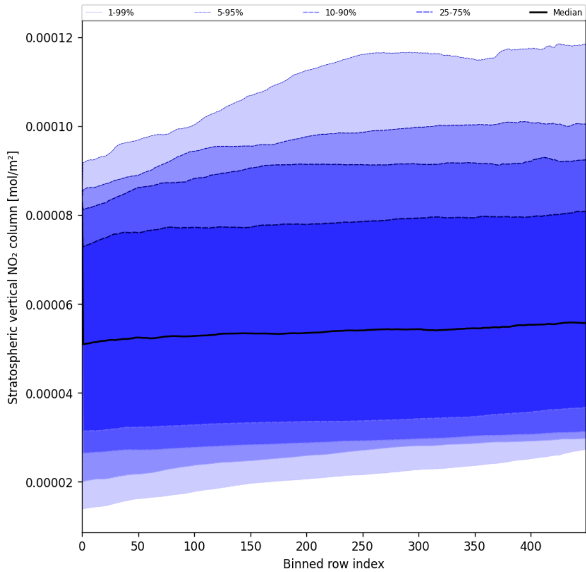
Figure 51: Along track statistics of “Stratospheric vertical NO 2 column” for 2025-06-16 to 2025-06-17
