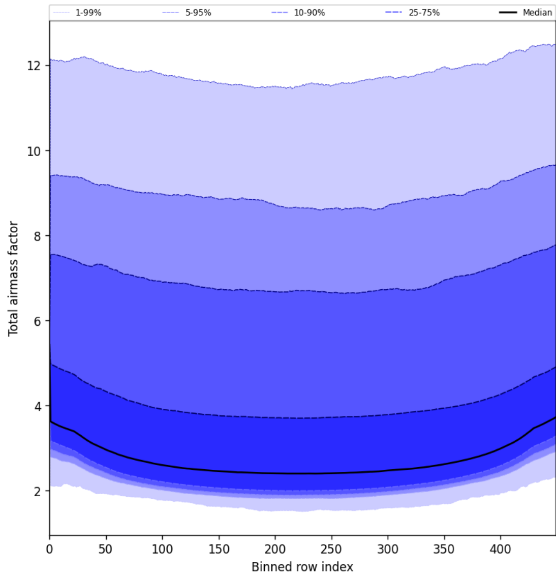
Figure 47: Along track statistics of “Total airmass factor” for 2025-06-16 to 2025-06-17
