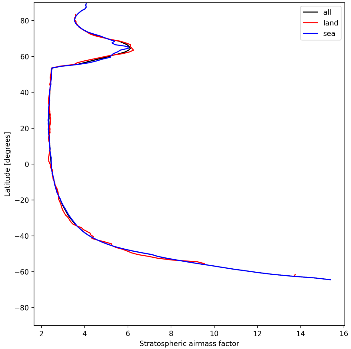
Figure 25: Zonal average of “Stratospheric airmass factor” for 2025-06-16 to 2025-06-17.
