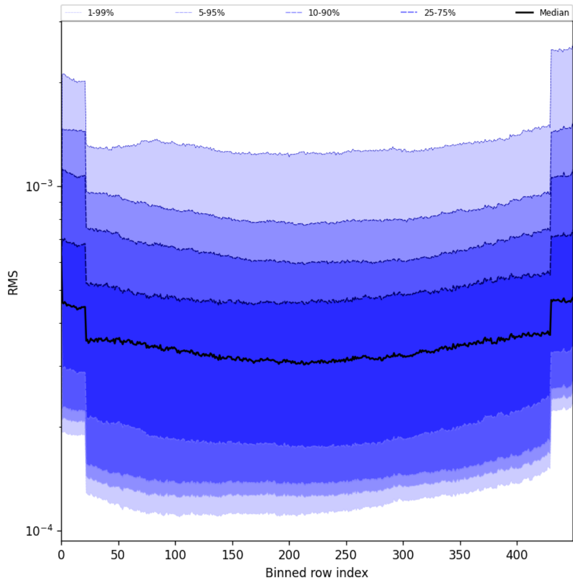
Figure 58: Along track statistics of “RMS” for 2025-06-16 to 2025-06-17
