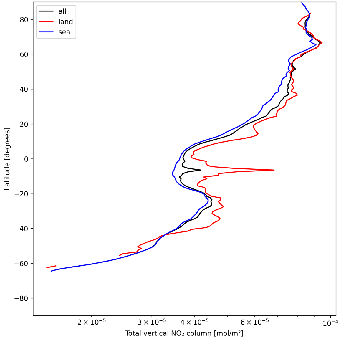
Figure 19: Zonal average of “Total vertical NO 2 column” for 2025-06-16 to 2025-06-17.
