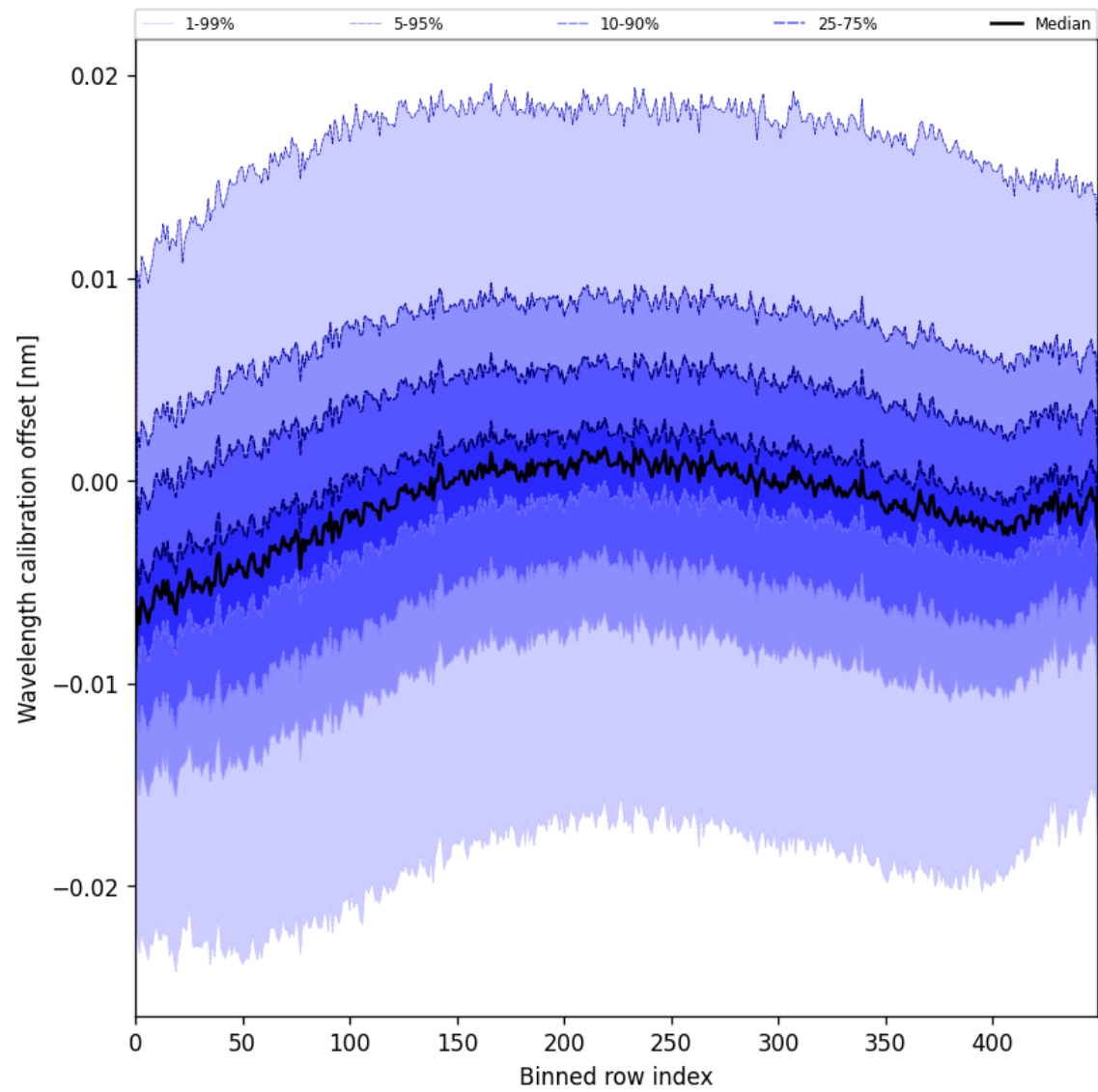
Figure 50: Along track statistics of “Wavelength calibration offset” for 2025-06-16 to 2025-06-17
