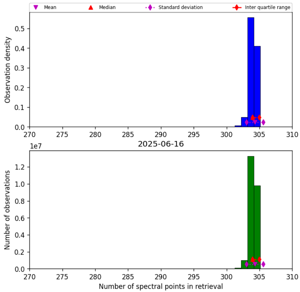
Figure 31: Histogram of “Number of spectral points in retrieval” for 2025-06-16 to 2025-06-17
