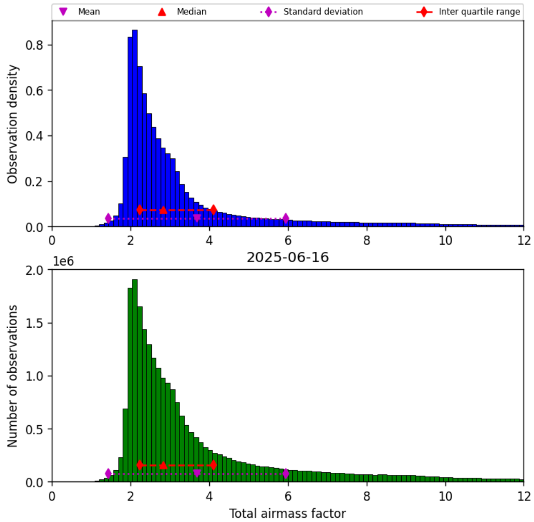
Figure 30: Histogram of “Total airmass factor” for 2025-06-16 to 2025-06-17
