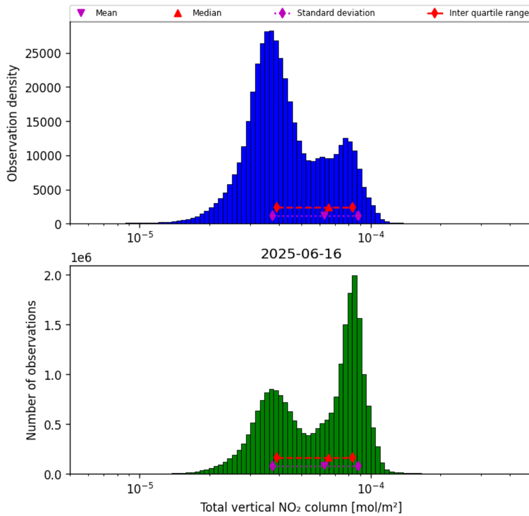
Figure 36: Histogram of “Total vertical NO 2 column” for 2025-06-16 to 2025-06-17
