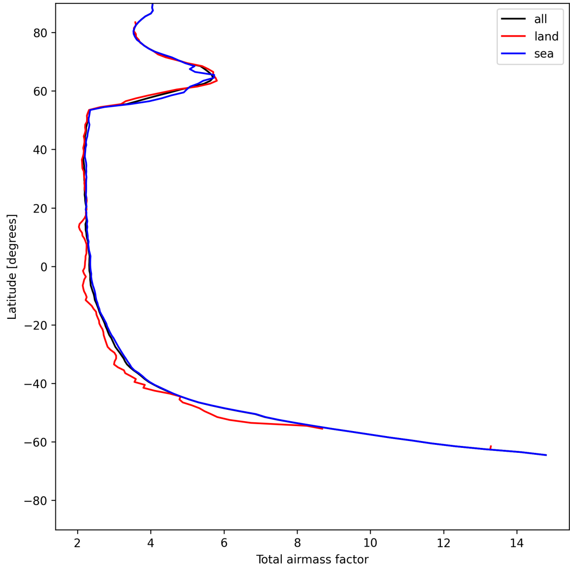
Figure 13: Zonal average of “Total airmass factor” for 2025-06-16 to 2025-06-17.
