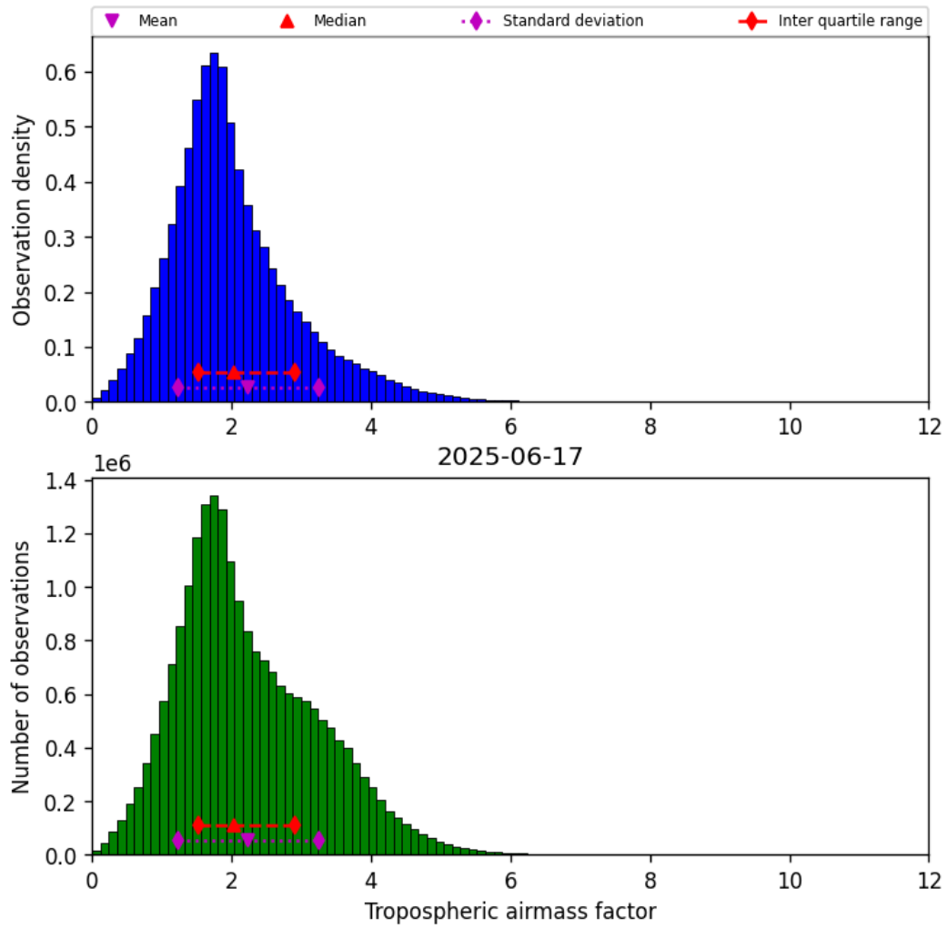
Figure 29: Histogram of “Tropospheric airmass factor” for 2025-06-17 to 2025-06-17
