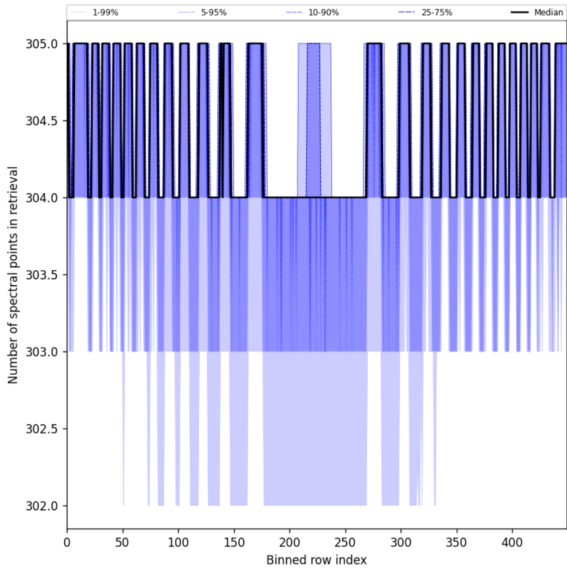
Figure 48: Along track statistics of “Number of spectral points in retrieval” for 2025-06-17 to 2025-06-17
