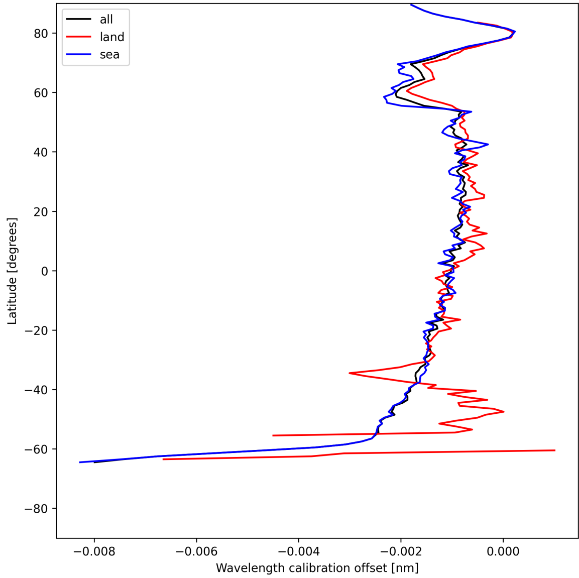
Figure 16: Zonal average of “Wavelength calibration offset” for 2025-06-17 to 2025-06-17.
