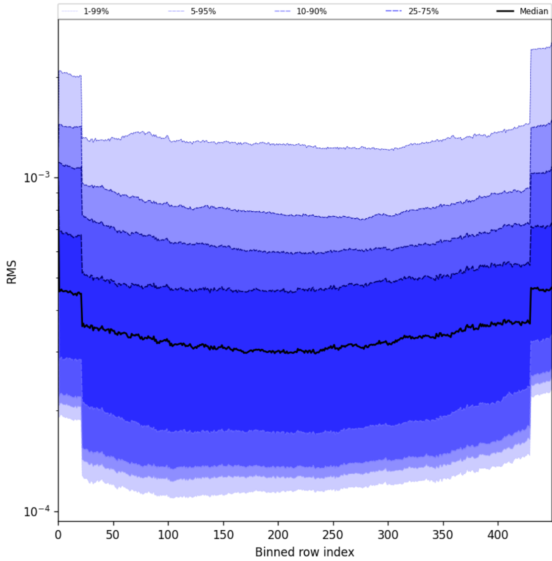
Figure 58: Along track statistics of “RMS” for 2025-06-17 to 2025-06-17
