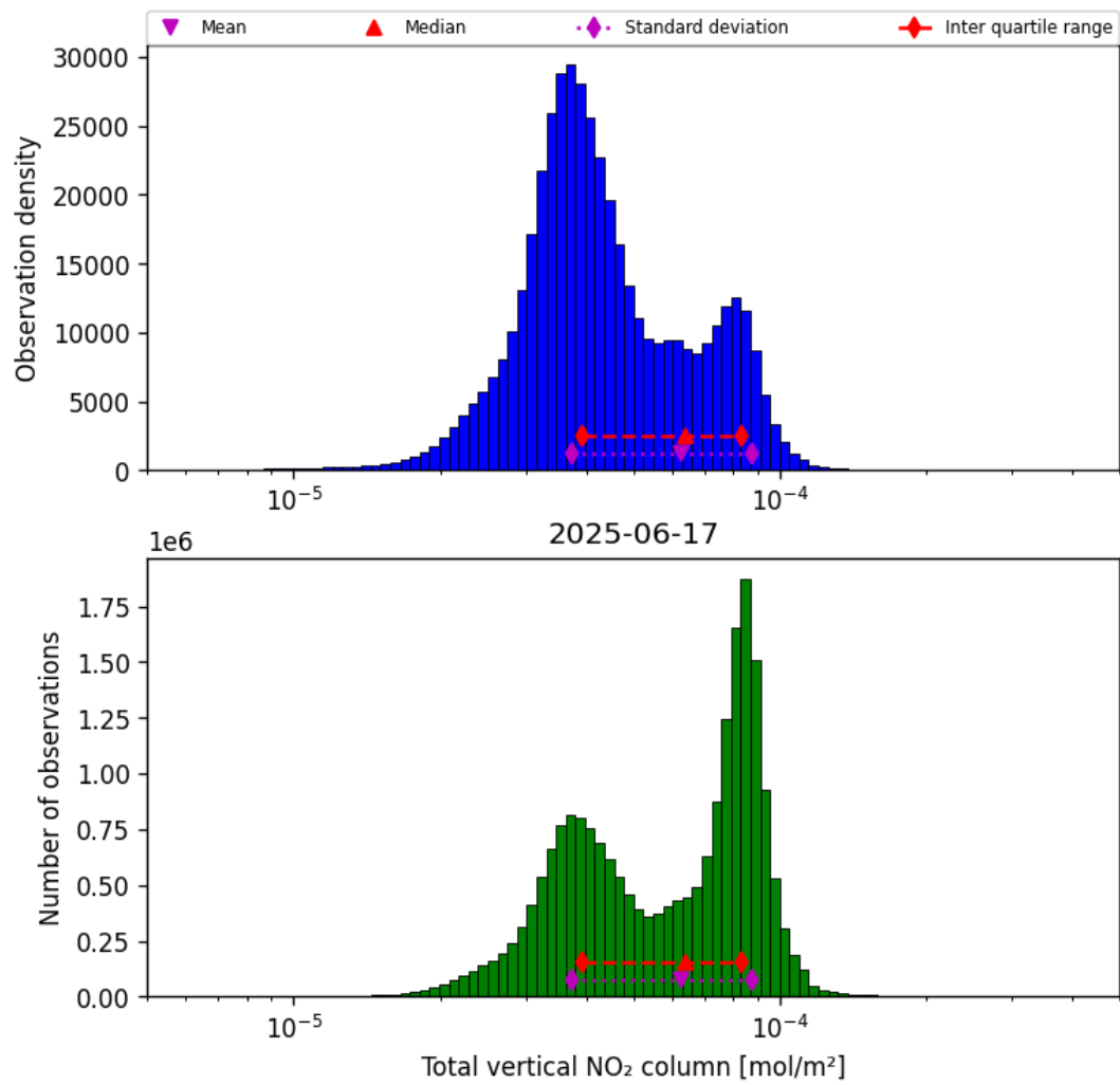
Figure 36: Histogram of “Total vertical NO 2 column” for 2025-06-17 to 2025-06-17
