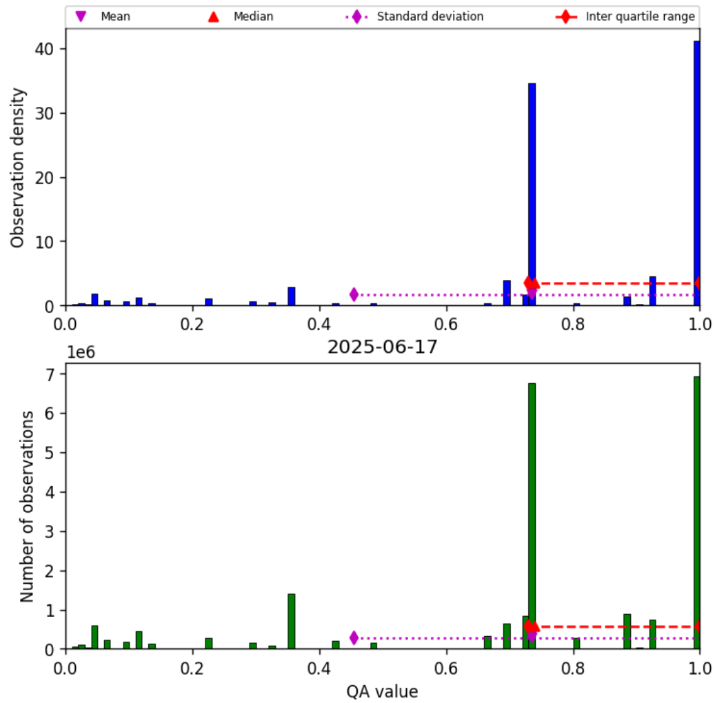
Figure 26: Histogram of “QA value” for 2025-06-17 to 2025-06-17
