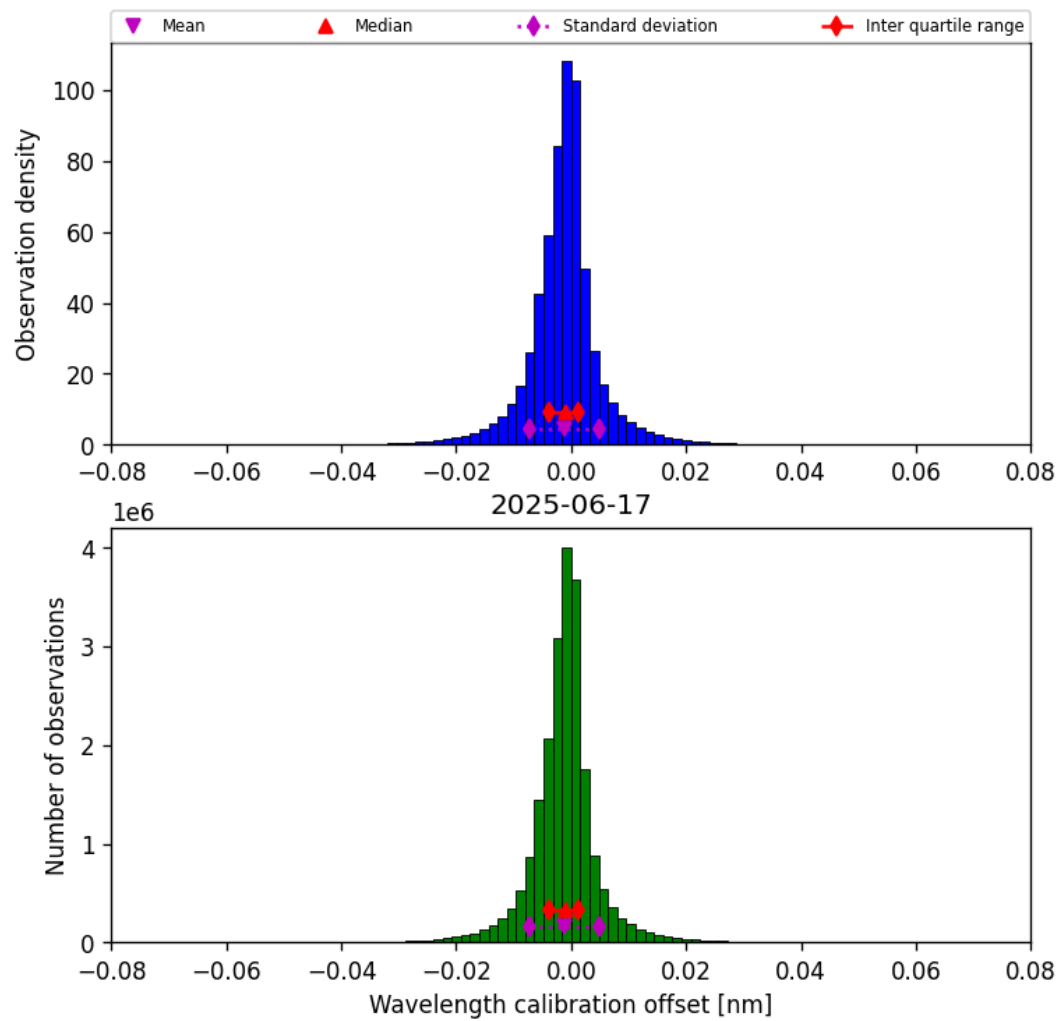
Figure 33: Histogram of “Wavelength calibration offset” for 2025-06-17 to 2025-06-17
