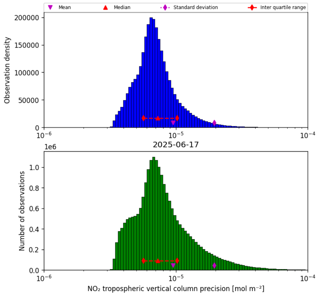
Figure 28: Histogram of "NO 2 tropospheric vertical column precision" for 2025-06-17 to 2025-06-17
