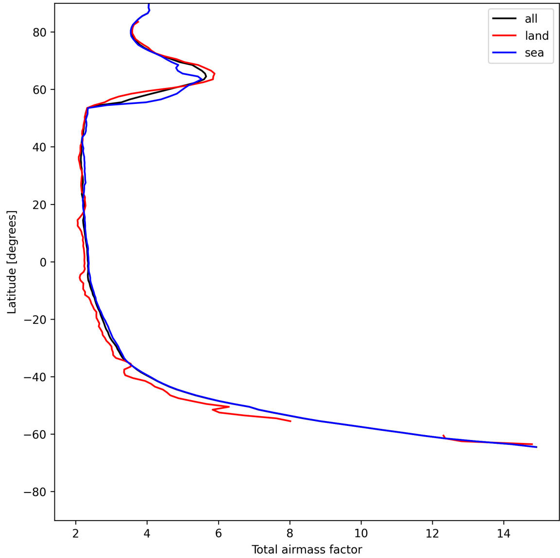
Figure 13: Zonal average of “Total airmass factor” for 2025-06-17 to 2025-06-17.
