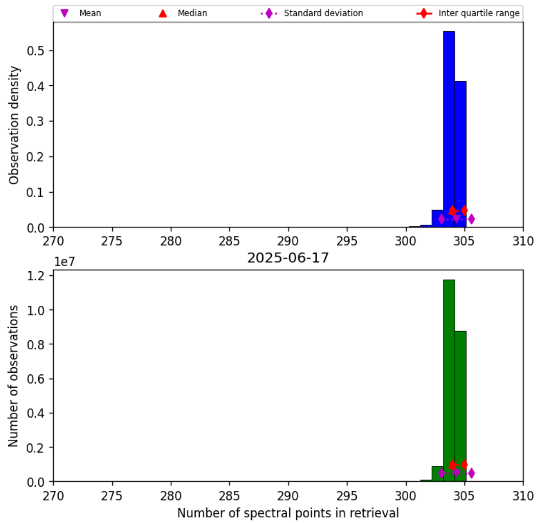
Figure 31: Histogram of “Number of spectral points in retrieval” for 2025-06-17 to 2025-06-17
