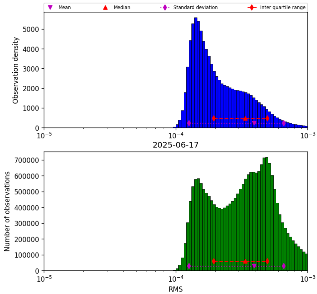
Figure 41: Histogram of “RMS” for 2025-06-17 to 2025-06-17
