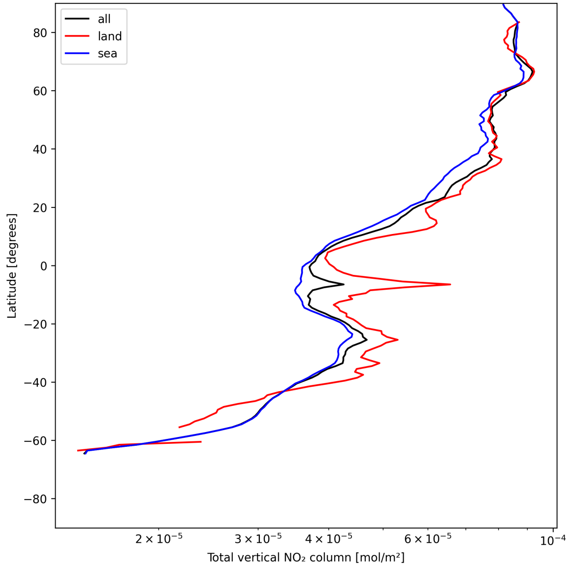
Figure 19: Zonal average of “Total vertical NO 2 column” for 2025-06-17 to 2025-06-17.
