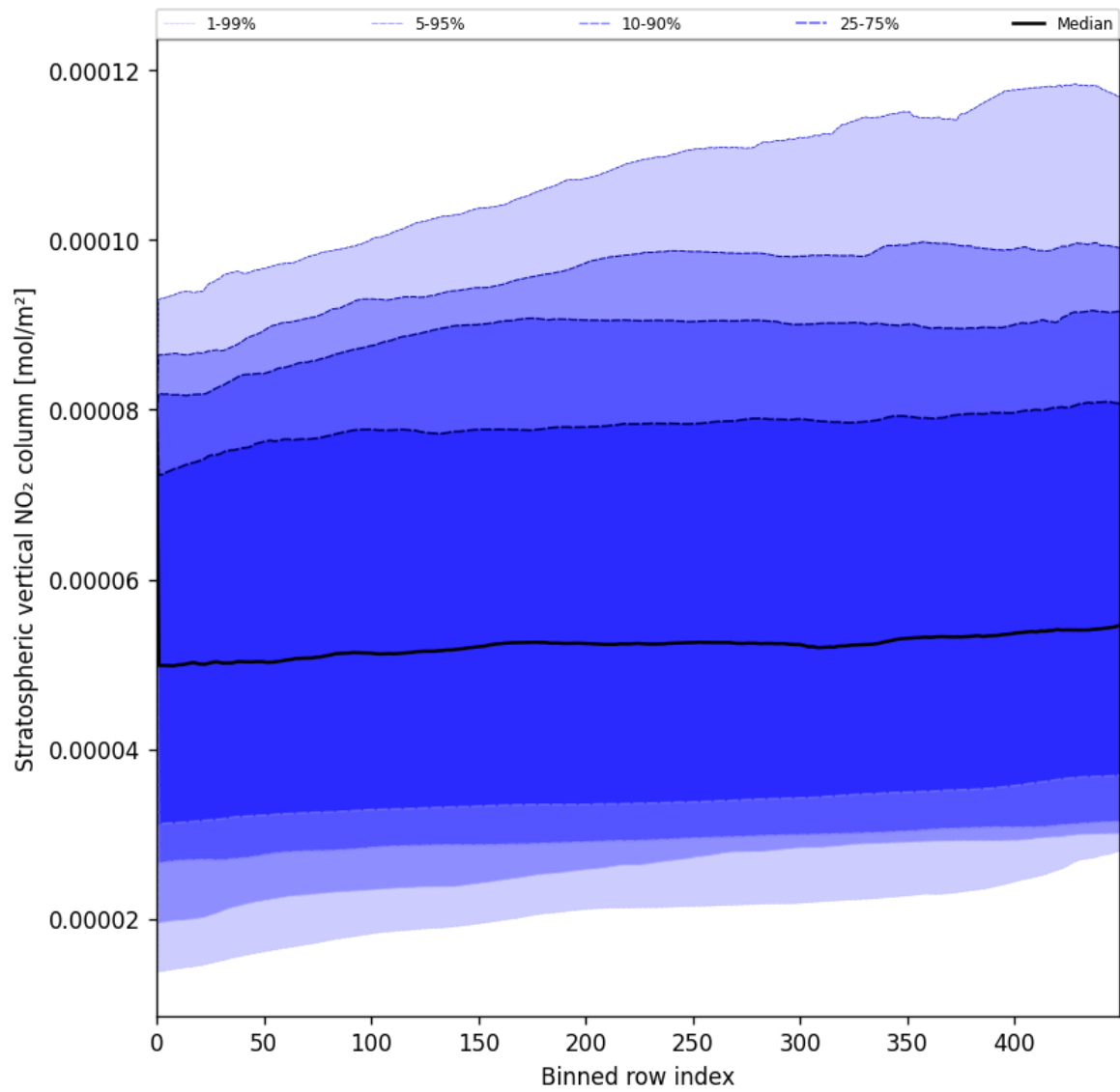
Figure 51: Along track statistics of “Stratospheric vertical NO 2 column” for 2025-06-17 to 2025-06-17
