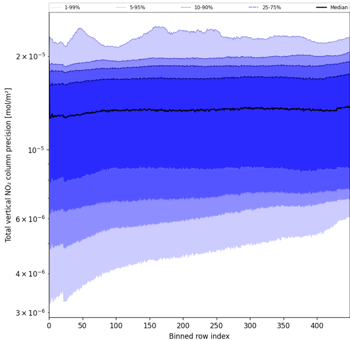
Figure 54: Along track statistics of “Total vertical NO 2 column precision” for 2025-06-17 to 2025-06-17
