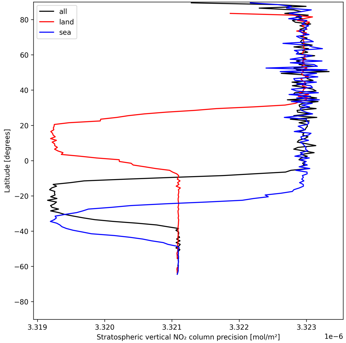
Figure 18: Zonal average of “Stratospheric vertical NO 2 column precision” for 2025-06-17 to 2025-06-17.
