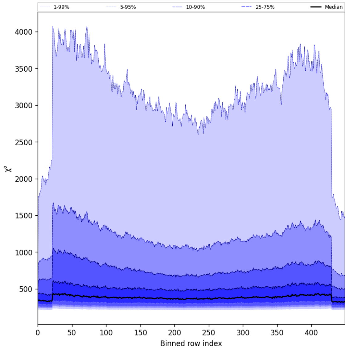
Figure 57: Along track statistics of “ \chi^2 ” for 2025-06-17 to 2025-06-17
