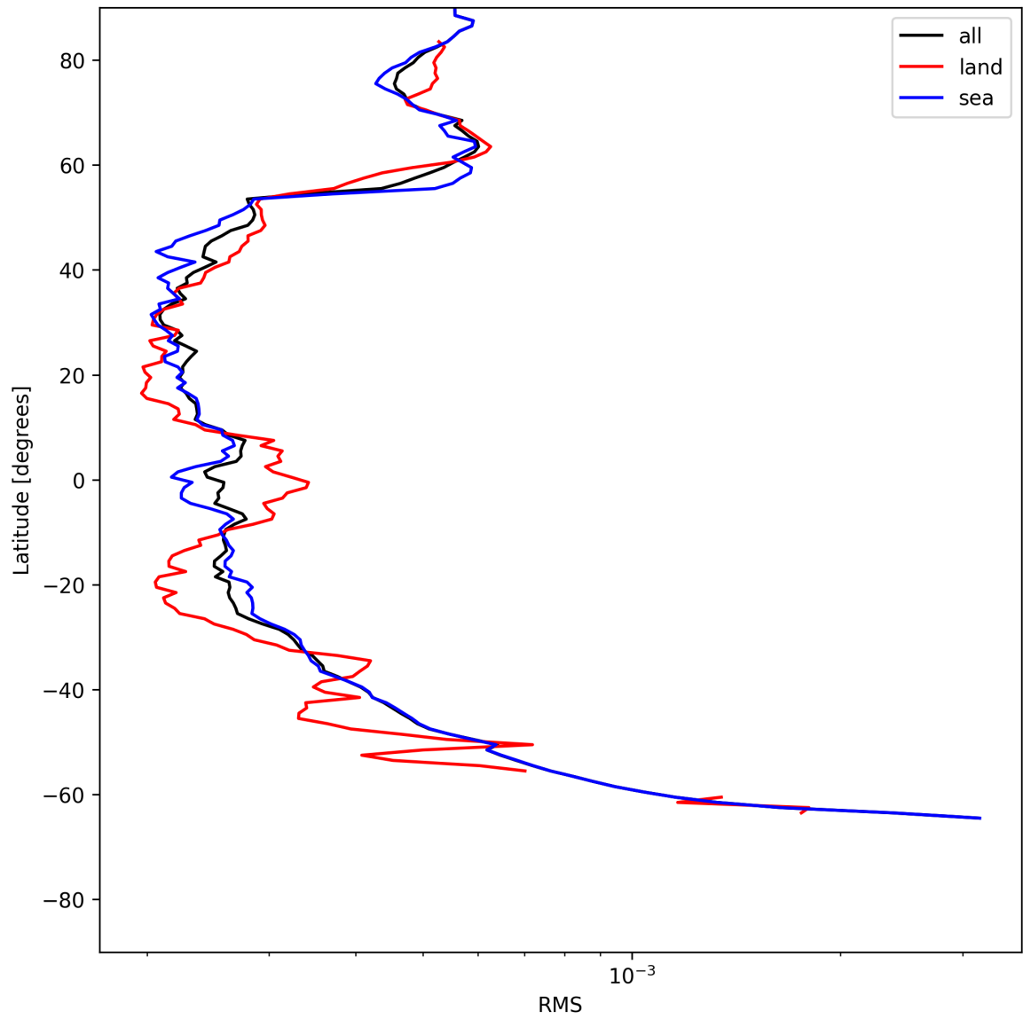
Figure 24: Zonal average of “RMS” for 2025-06-17 to 2025-06-17.
