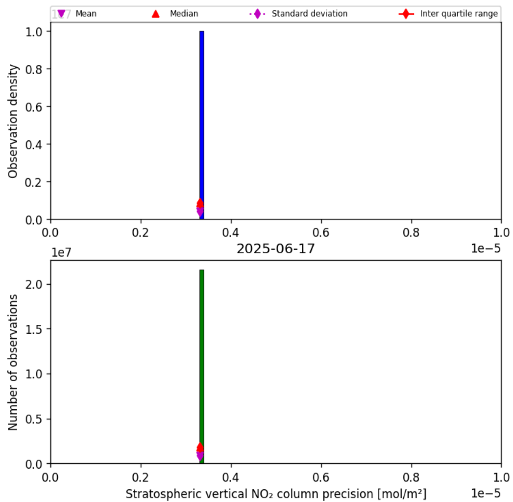
Figure 35: Histogram of “Stratospheric vertical NO 2 column precision” for 2025-06-17 to 2025-06-17
