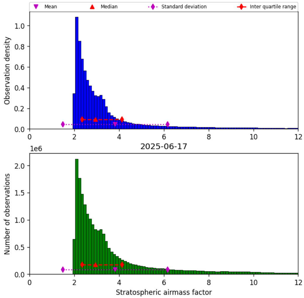
Figure 42: Histogram of “Stratospheric airmass factor” for 2025-06-17 to 2025-06-17
