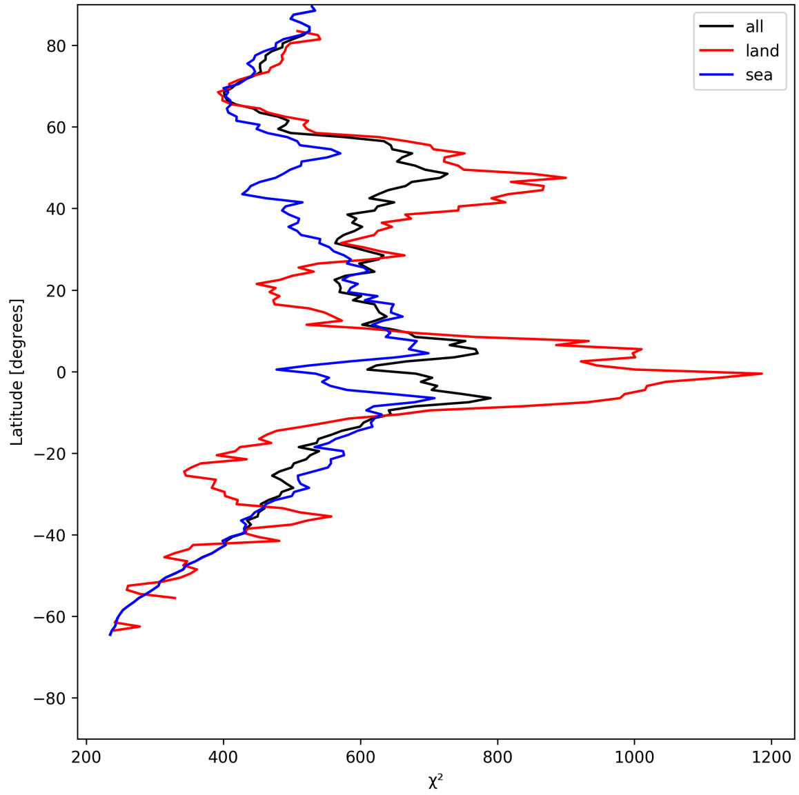
Figure 23: Zonal average of “ \chi^2 ” for 2025-06-17 to 2025-06-17.
