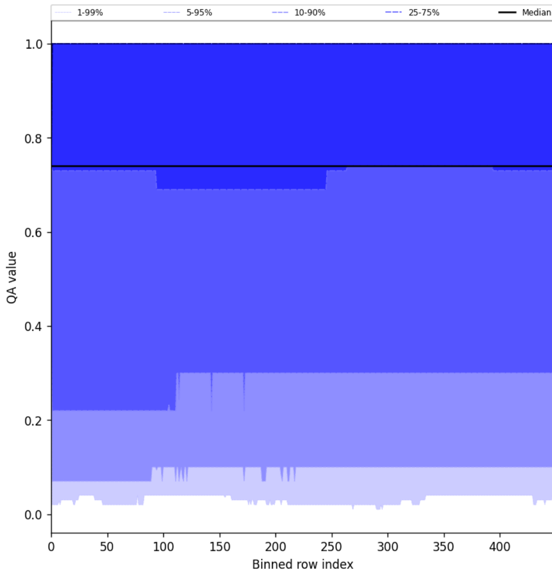
Figure 43: Along track statistics of “QA value” for 2025-06-17 to 2025-06-17
