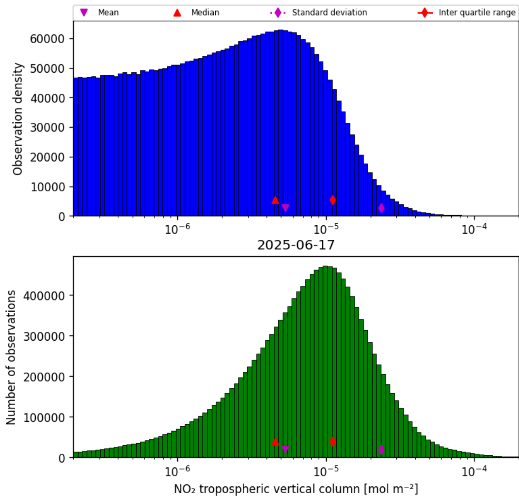
Figure 27: Histogram of “NO 2 tropospheric vertical column” for 2025-06-17 to 2025-06-17
