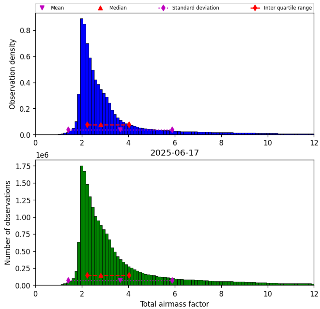
Figure 30: Histogram of “Total airmass factor” for 2025-06-17 to 2025-06-17
