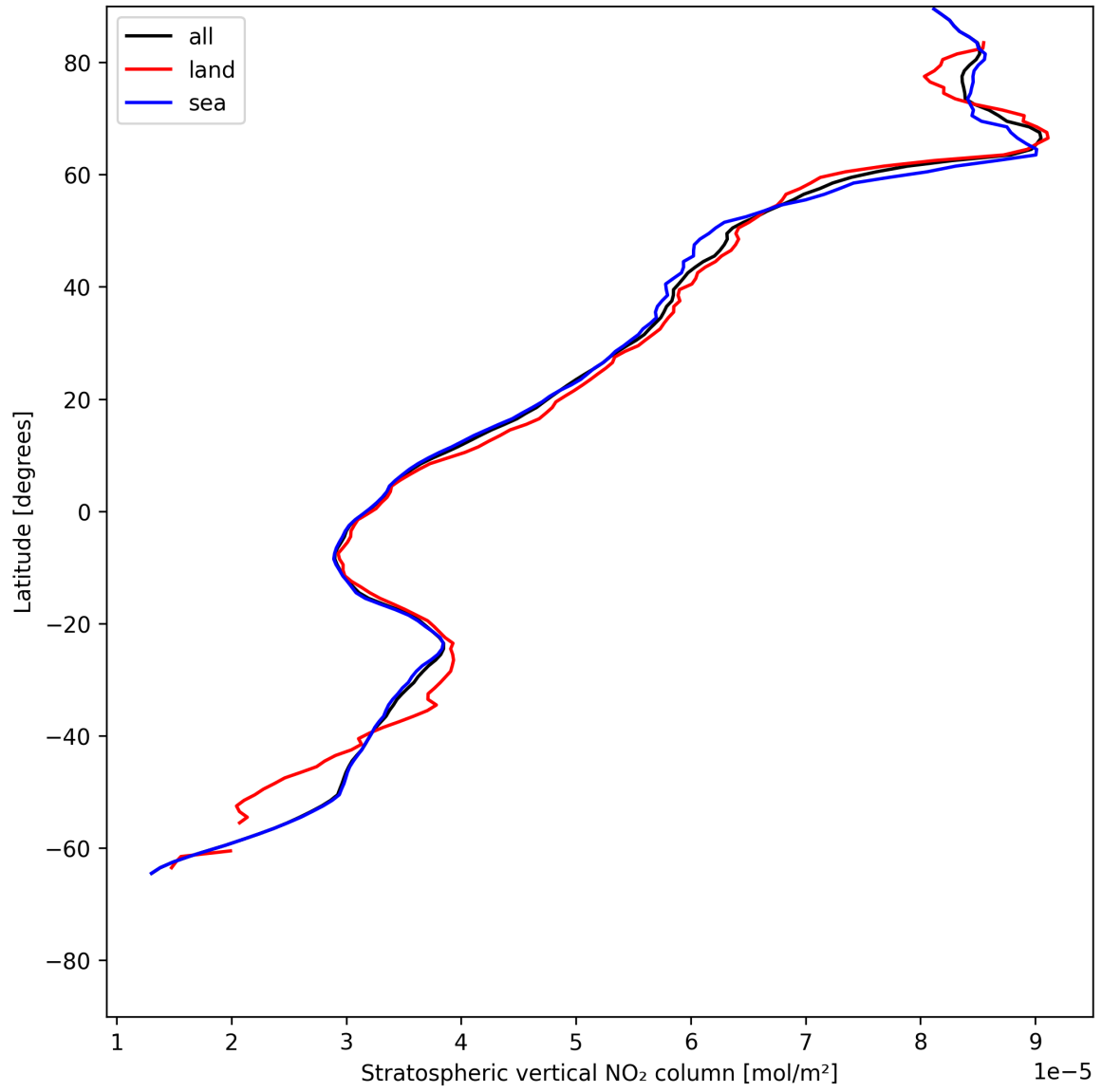
Figure 17: Zonal average of “Stratospheric vertical NO 2 column” for 2025-06-17 to 2025-06-17.
