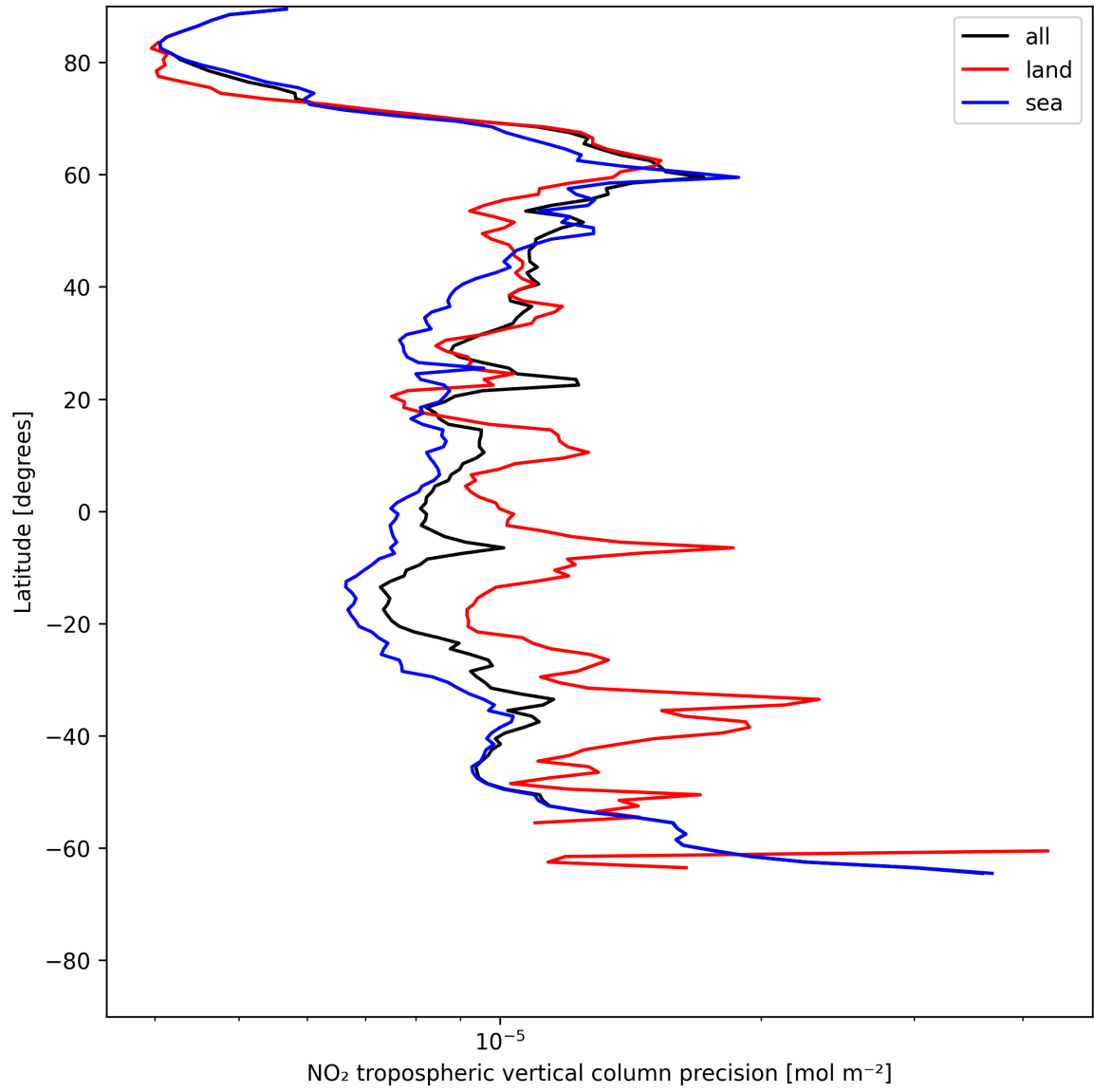
Figure 11: Zonal average of “NO 2 tropospheric vertical column precision” for 2025-06-17 to 2025-06-17.
