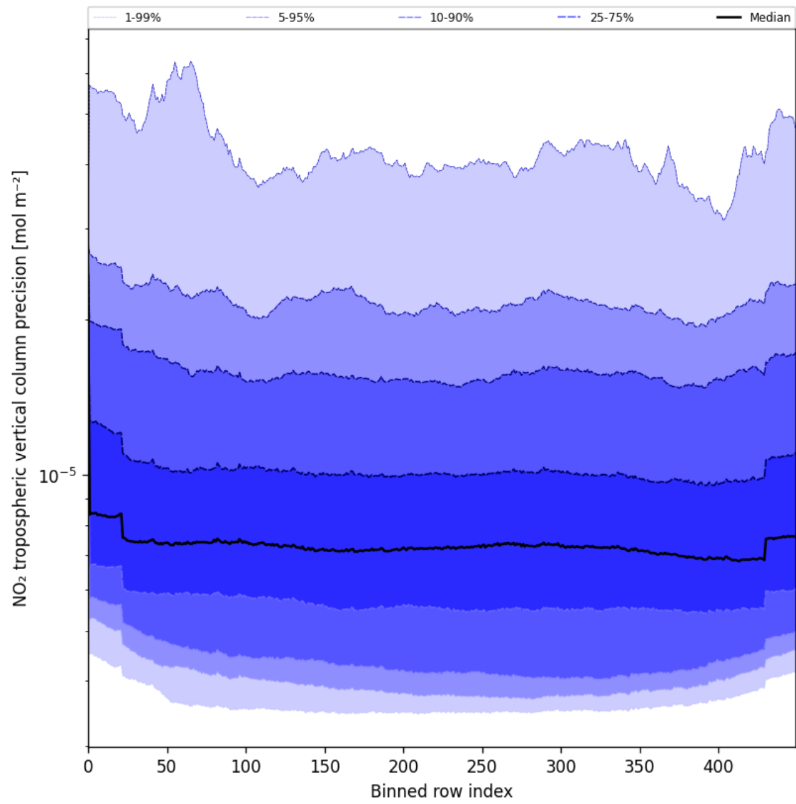
Figure 45: Along track statistics of “NO 2 tropospheric vertical column precision” for 2025-06-17 to 2025-06-17
