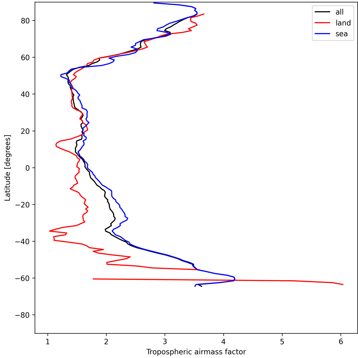
Figure 12: Zonal average of “Tropospheric airmass factor” for 2025-06-17 to 2025-06-17.
