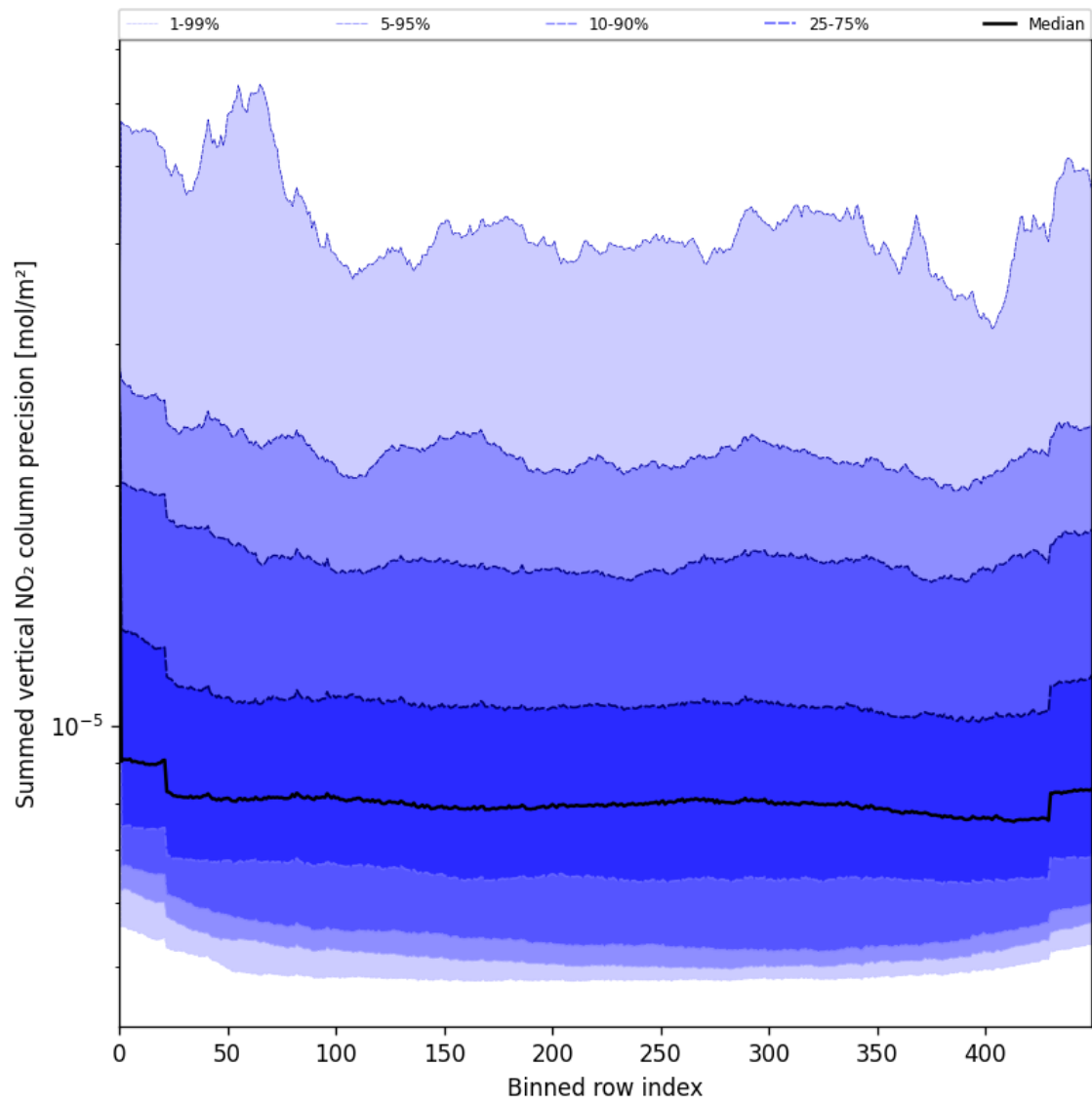
Figure 56: Along track statistics of “Summed vertical NO 2 column precision” for 2025-06-17 to 2025-06-17
