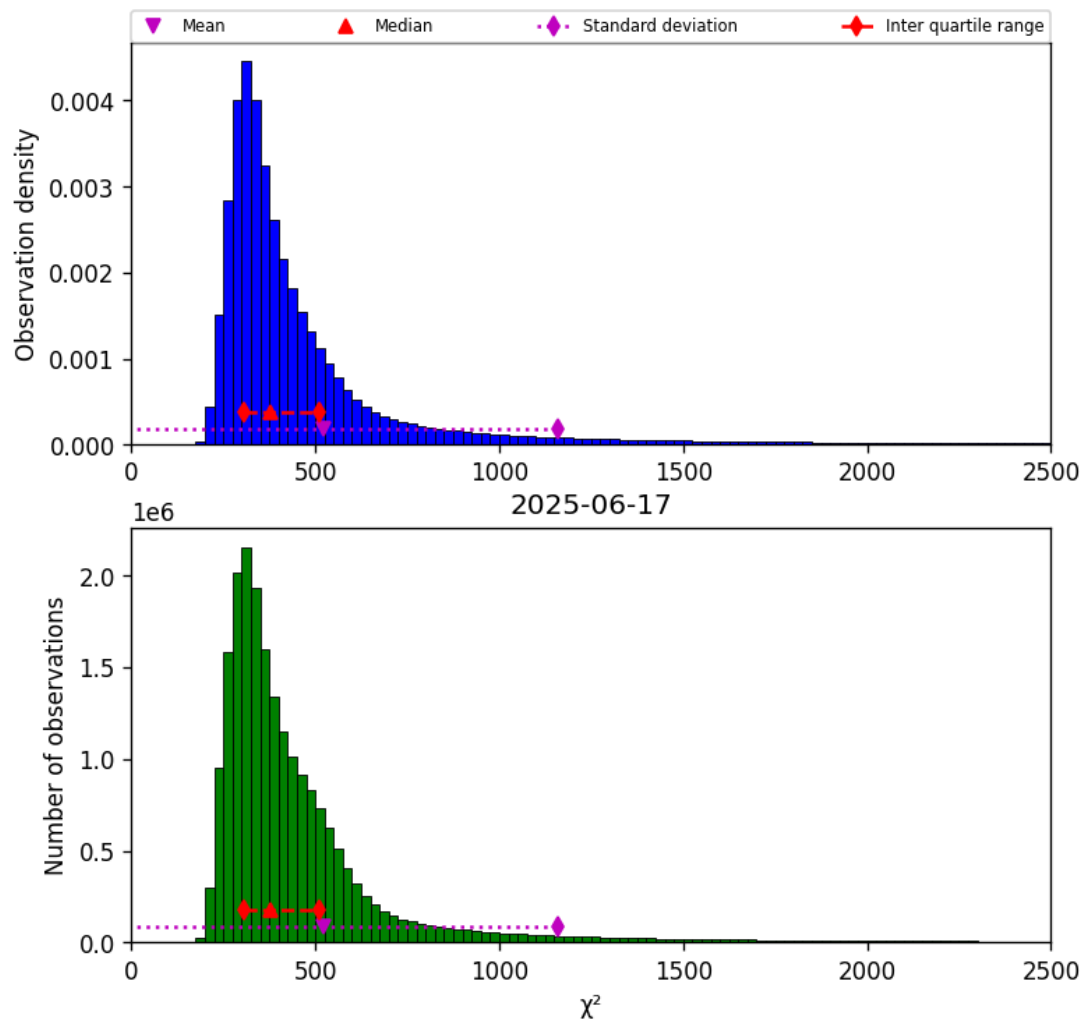
Figure 40: Histogram of “ \chi^2 ” for 2025-06-17 to 2025-06-17
