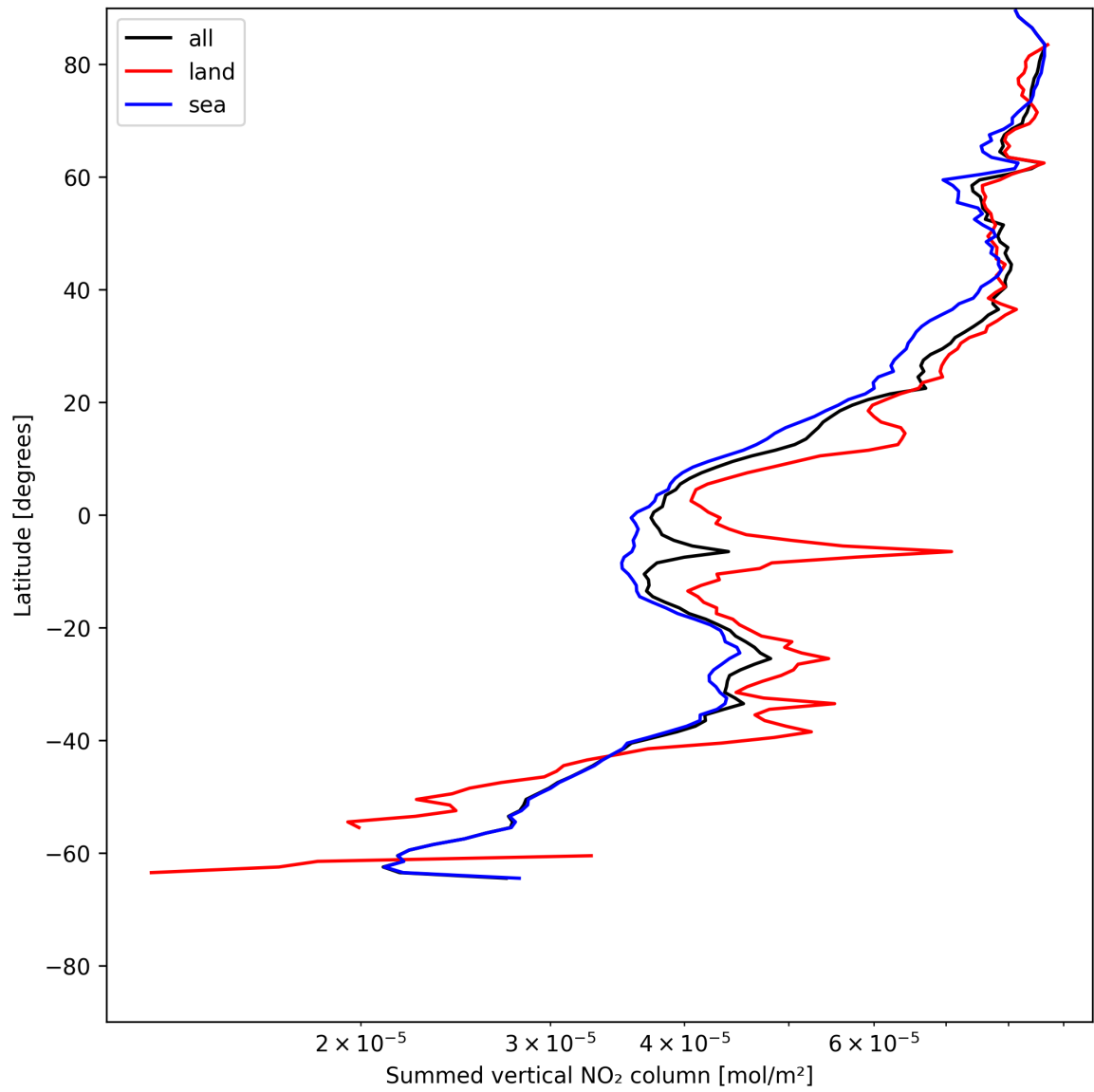
Figure 21: Zonal average of “Summed vertical NO 2 column” for 2025-06-17 to 2025-06-17.
