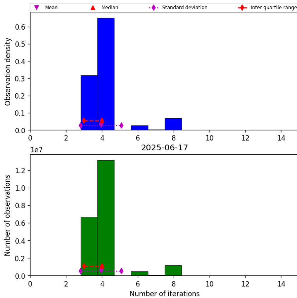
Figure 32: Histogram of “Number of iterations” for 2025-06-17 to 2025-06-17
