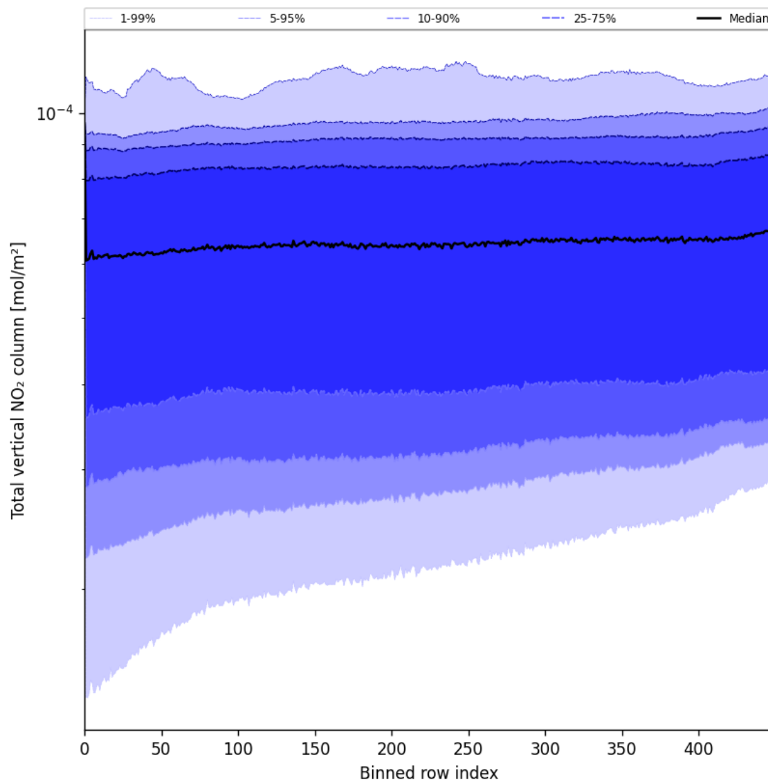
Figure 53: Along track statistics of “Total vertical NO 2 column” for 2025-06-17 to 2025-06-17
