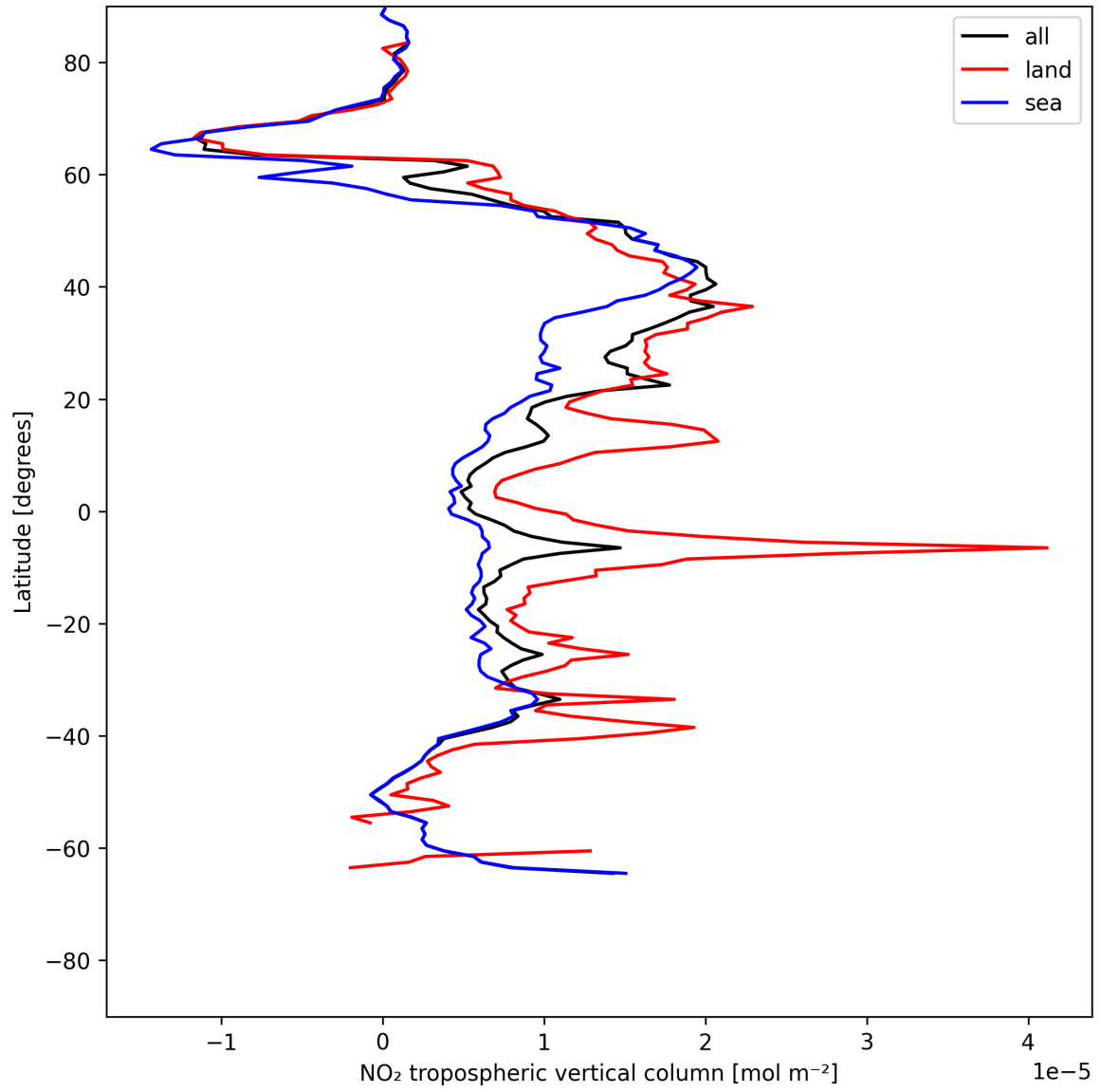
Figure 10: Zonal average of “NO 2 tropospheric vertical column” for 2025-06-17 to 2025-06-17.
