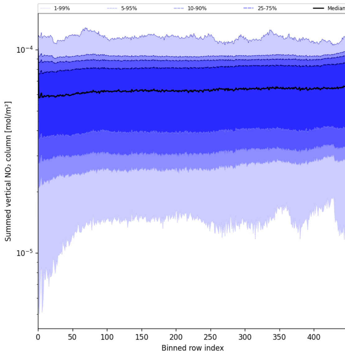
Figure 55: Along track statistics of “Summed vertical NO 2 column” for 2025-06-17 to 2025-06-17
