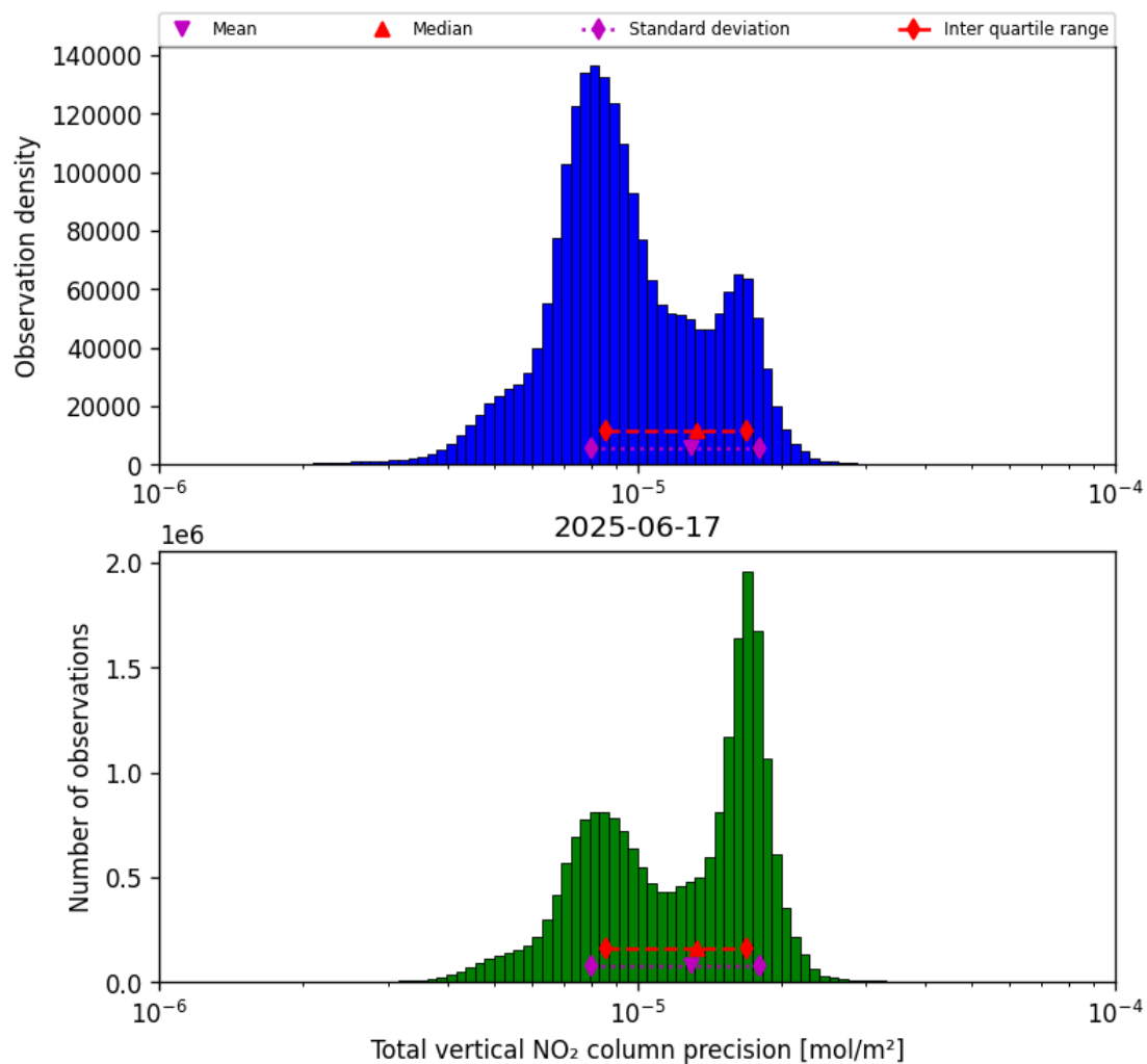
Figure 37: Histogram of “Total vertical NO 2 column precision” for 2025-06-17 to 2025-06-17
