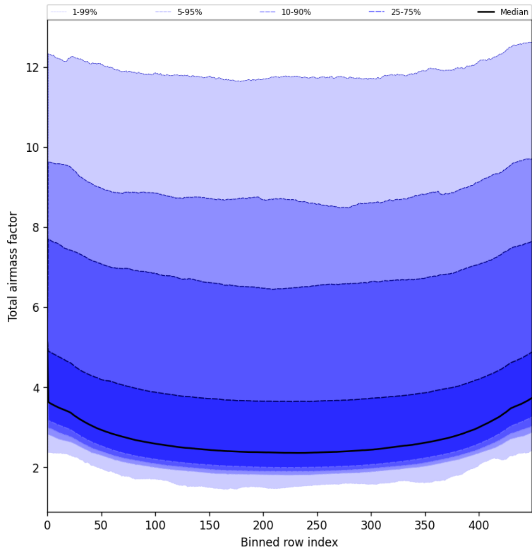
Figure 47: Along track statistics of “Total airmass factor” for 2025-06-17 to 2025-06-17
