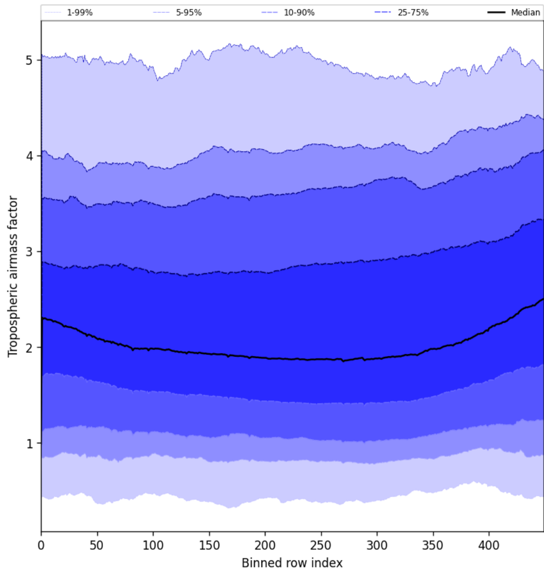
Figure 46: Along track statistics of “Tropospheric airmass factor” for 2025-06-17 to 2025-06-17
