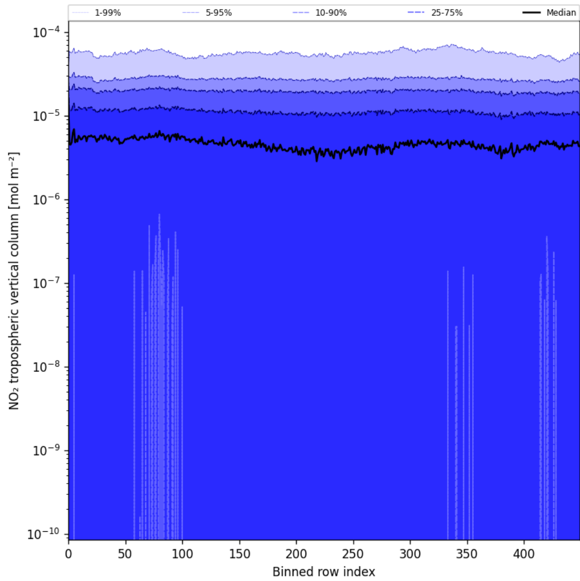
Figure 44: Along track statistics of "NO 2 tropospheric vertical column" for 2025-06-17 to 2025-06-17
