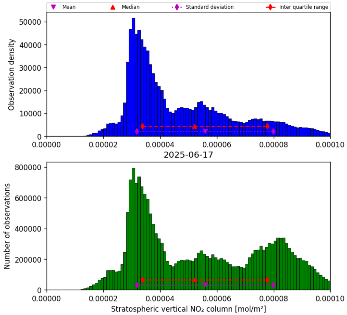
Figure 34: Histogram of “Stratospheric vertical NO 2 column” for 2025-06-17 to 2025-06-17
