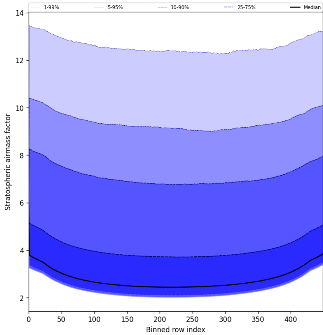
Figure 59: Along track statistics of “Stratospheric airmass factor” for 2025-06-17 to 2025-06-17
