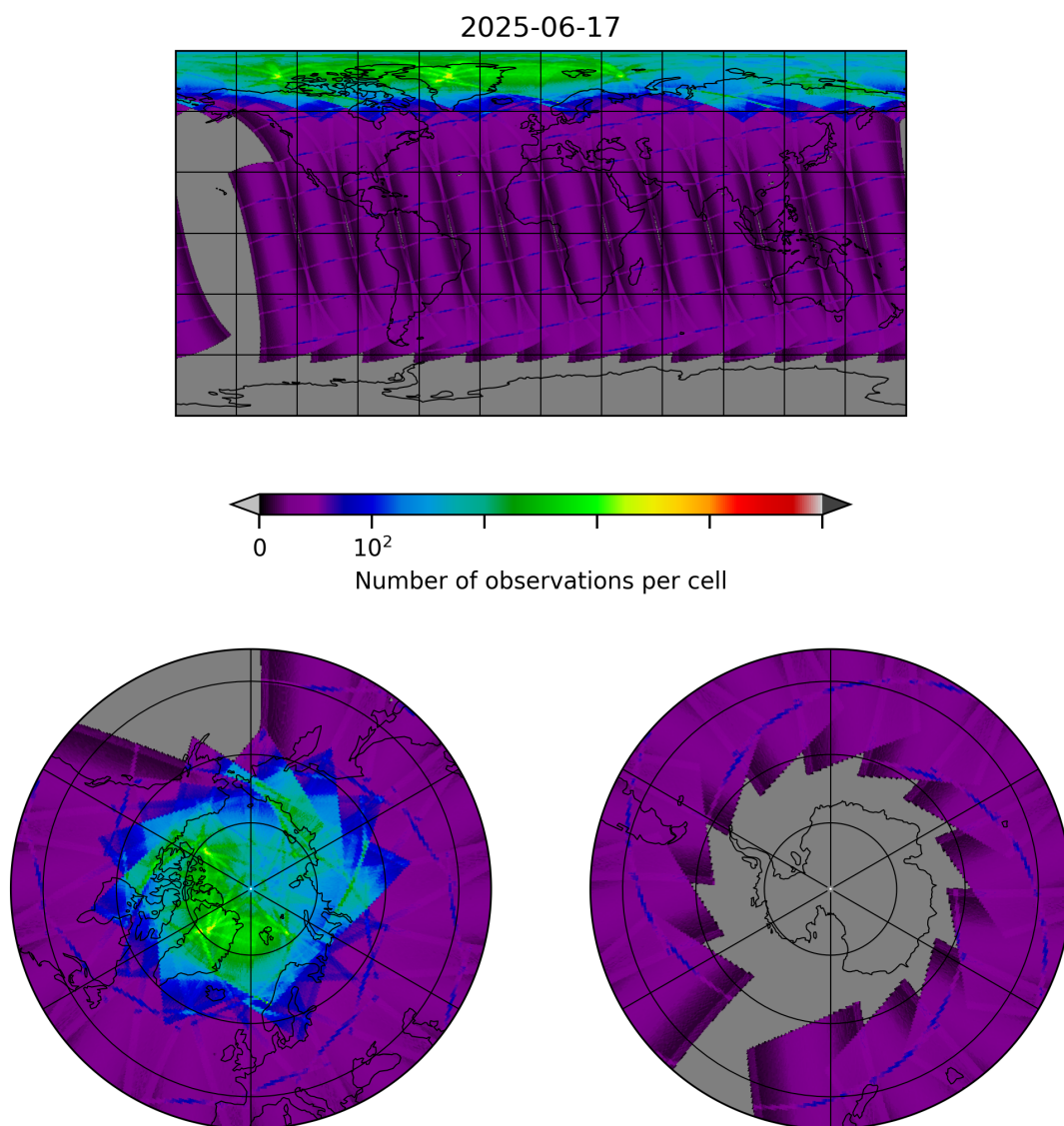
Figure 8: Map of the number of observations for 2025-06-17 to 2025-06-17
