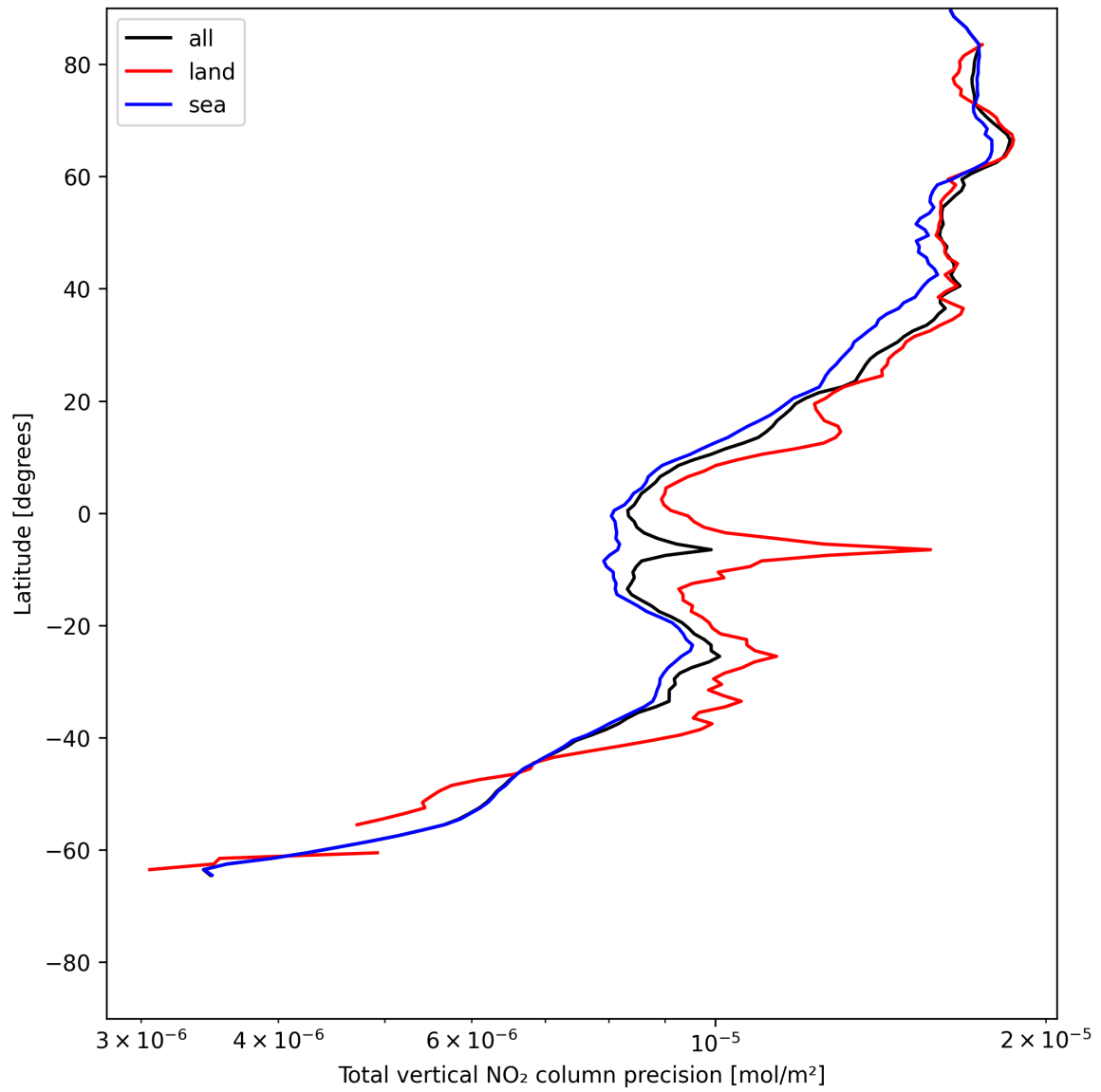
Figure 20: Zonal average of “Total vertical NO 2 column precision” for 2025-06-17 to 2025-06-17.
