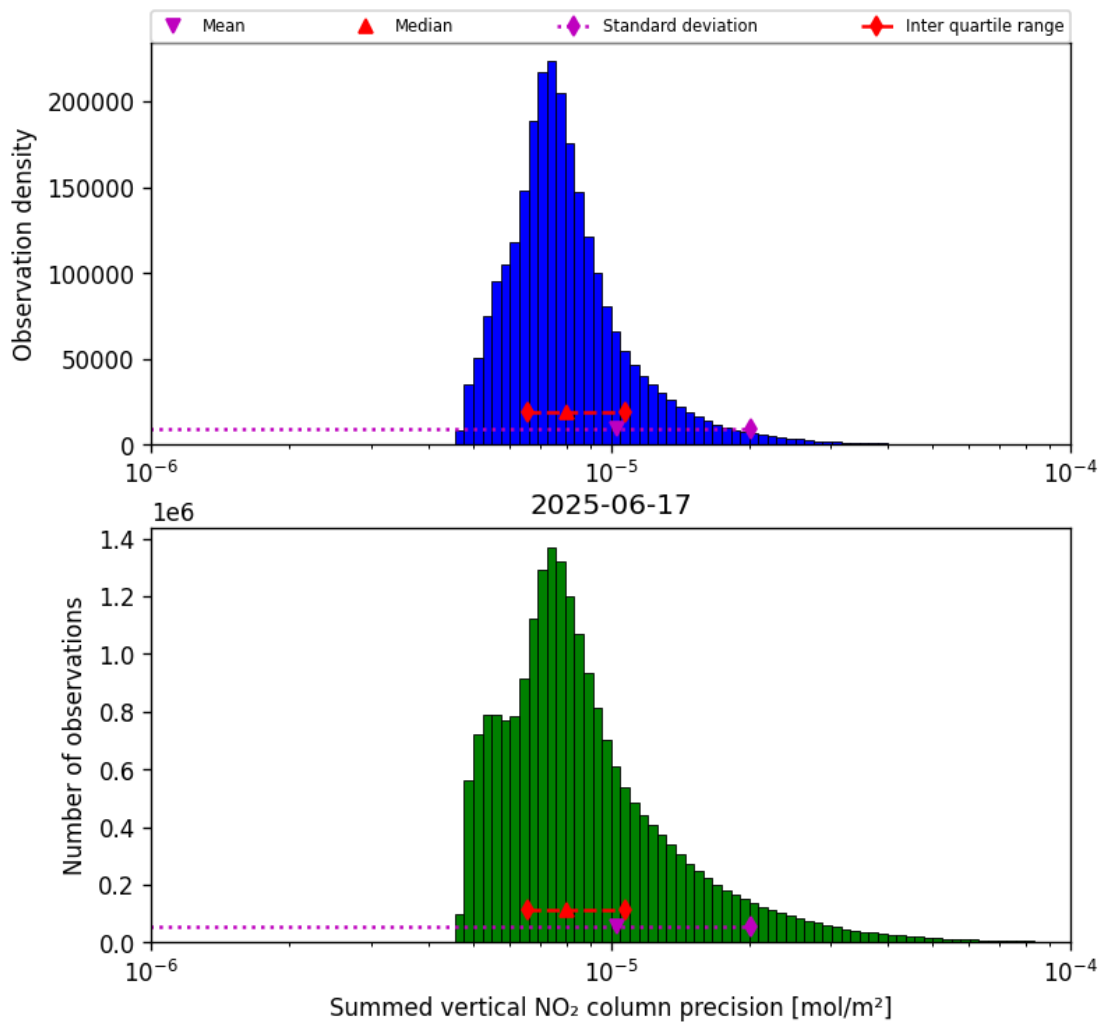
Figure 39: Histogram of "Summed vertical NO 2 column precision" for 2025-06-17 to 2025-06-17
