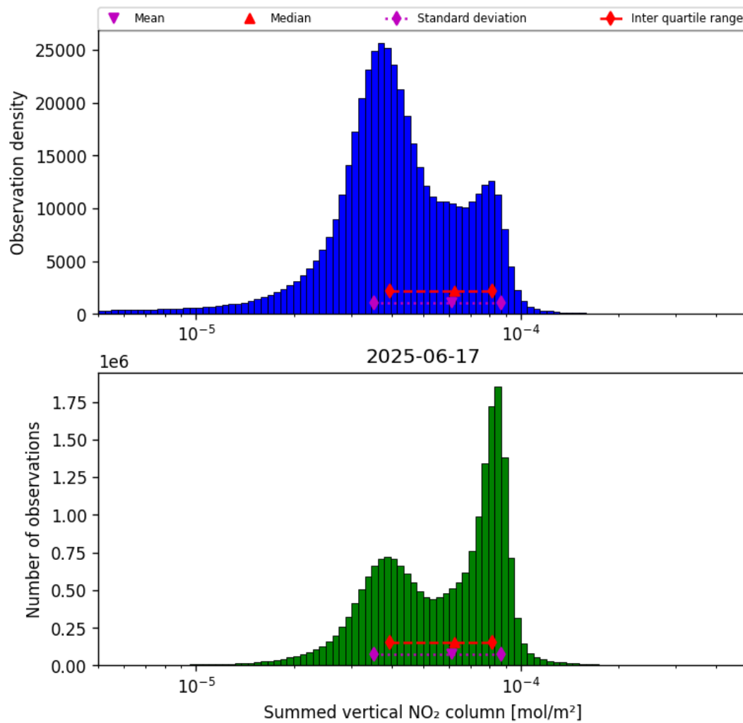
Figure 38: Histogram of “Summed vertical NO 2 column” for 2025-06-17 to 2025-06-17
