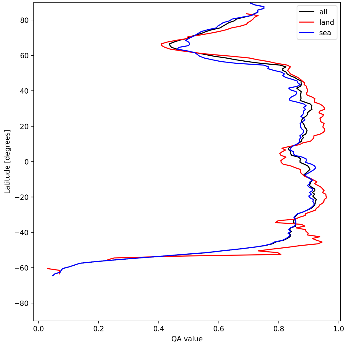
Figure 9: Zonal average of “QA value” for 2025-06-17 to 2025-06-17.
