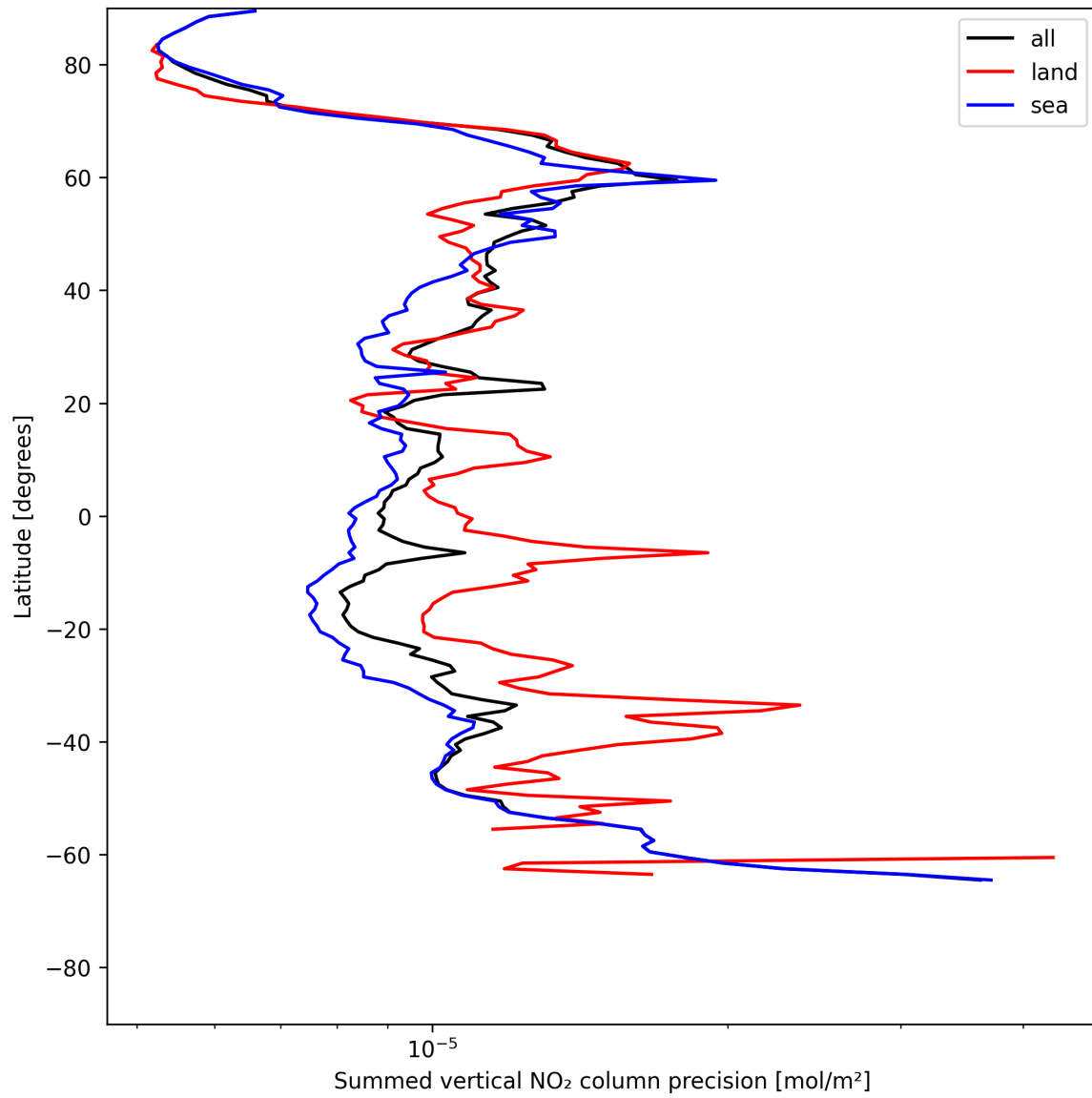
Figure 22: Zonal average of “Summed vertical NO 2 column precision” for 2025-06-17 to 2025-06-17.
