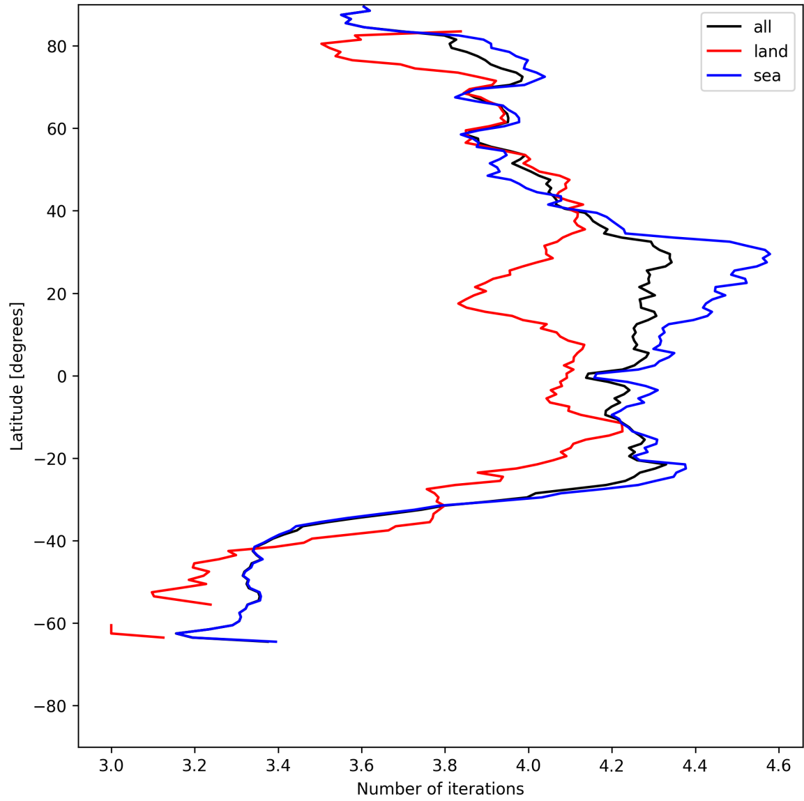
Figure 15: Zonal average of “Number of iterations” for 2025-06-17 to 2025-06-17.
