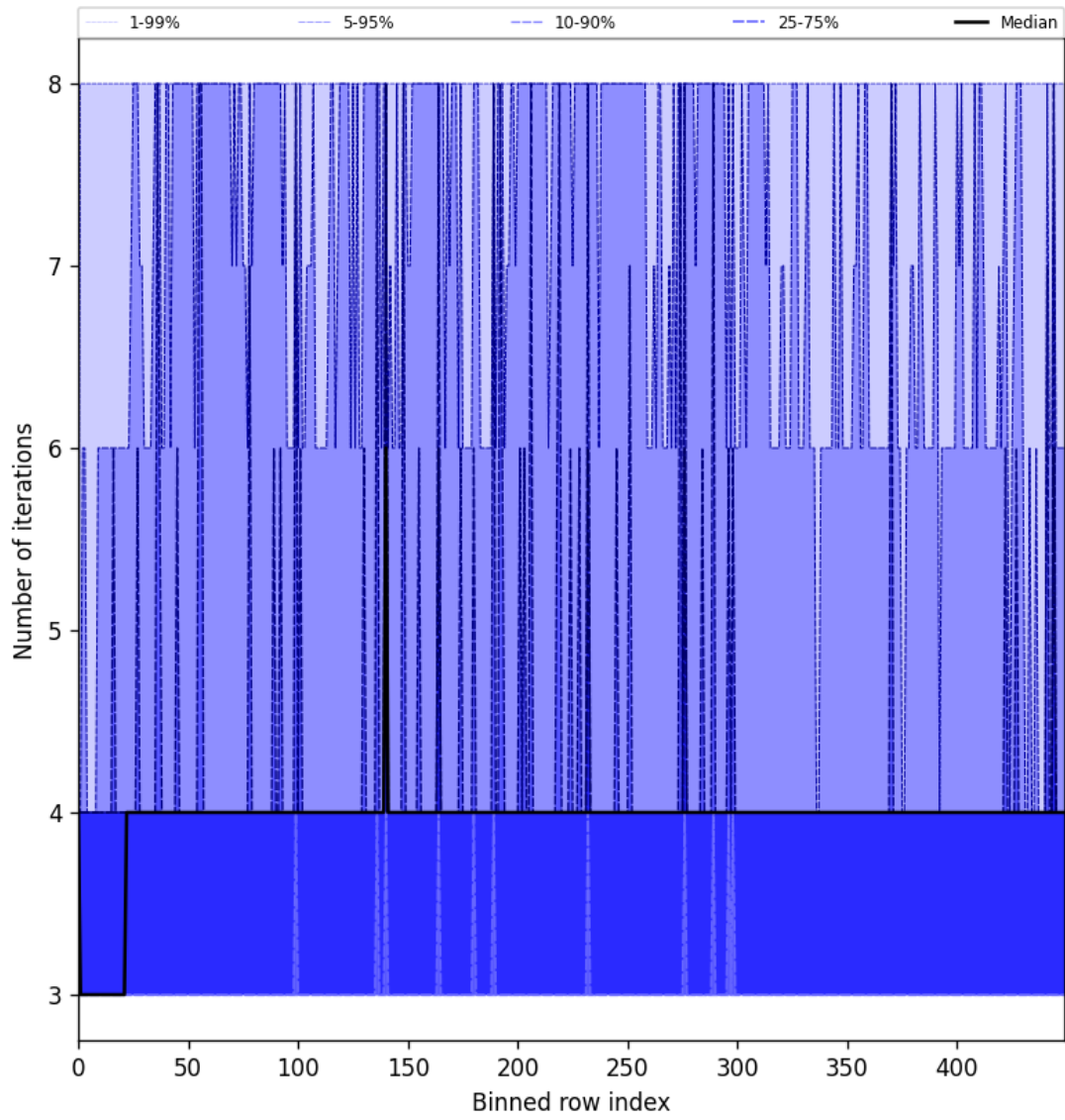
Figure 49: Along track statistics of “Number of iterations” for 2025-06-17 to 2025-06-17
