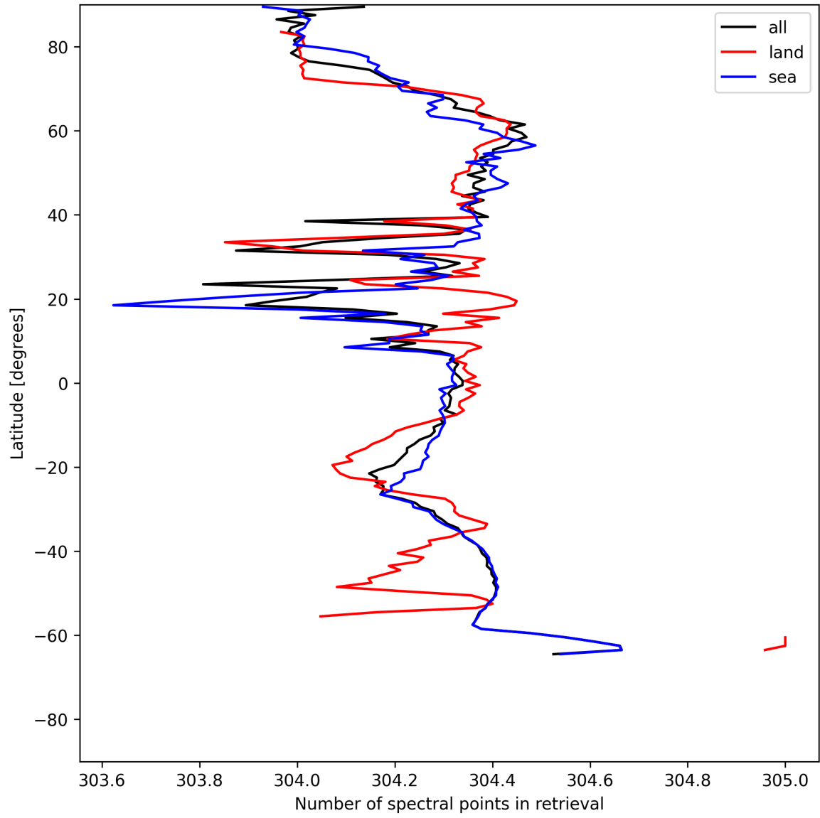
Figure 14: Zonal average of “Number of spectral points in retrieval” for 2025-06-17 to 2025-06-17.
