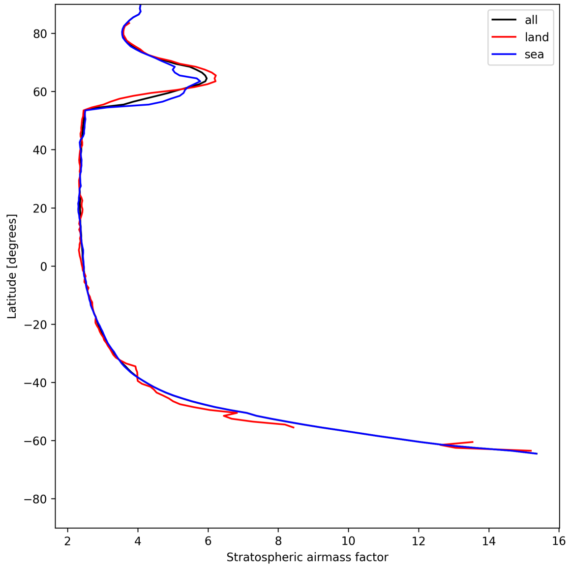
Figure 25: Zonal average of “Stratospheric airmass factor” for 2025-06-17 to 2025-06-17.
