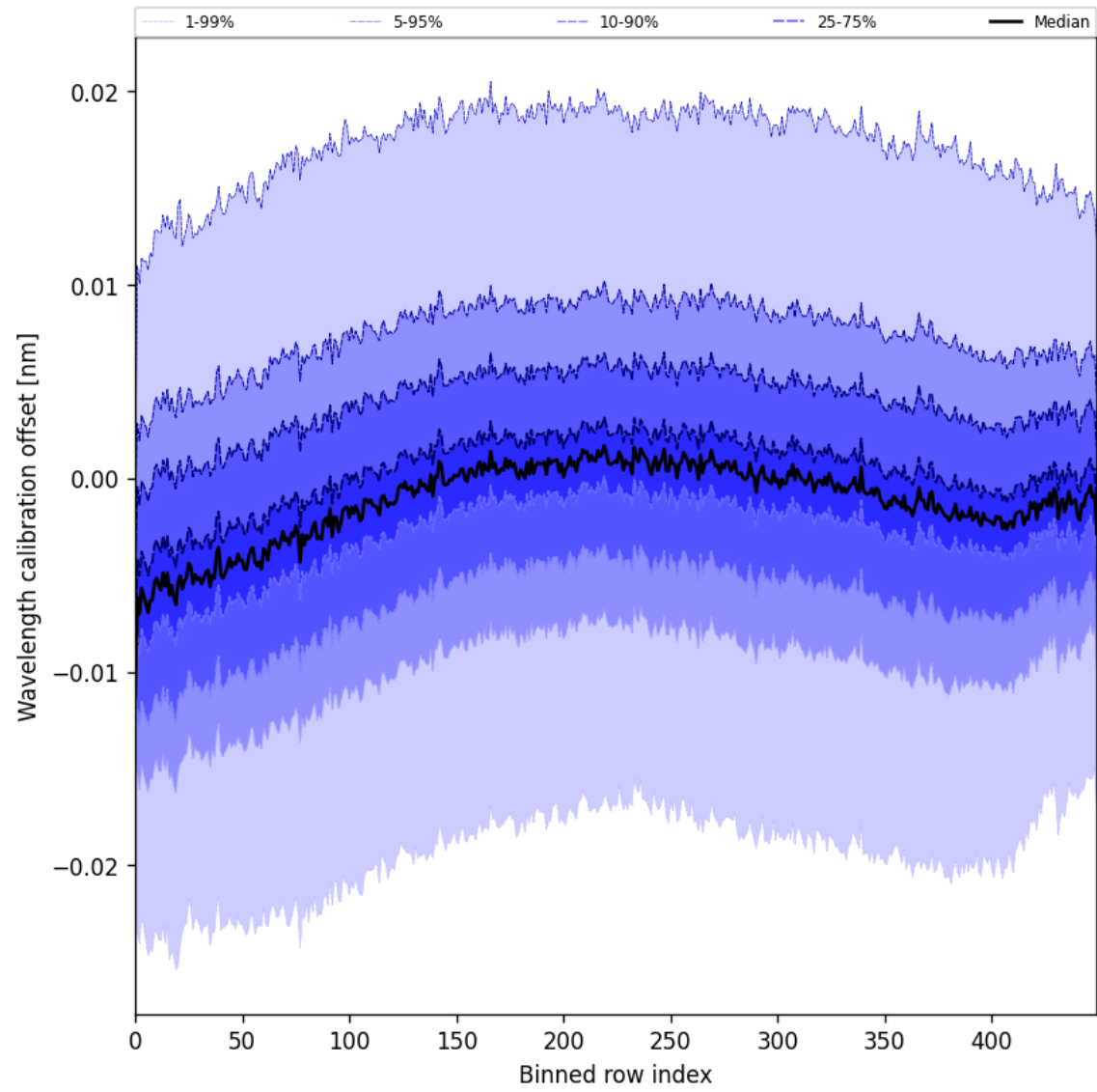
Figure 50: Along track statistics of “Wavelength calibration offset” for 2025-06-17 to 2025-06-17
