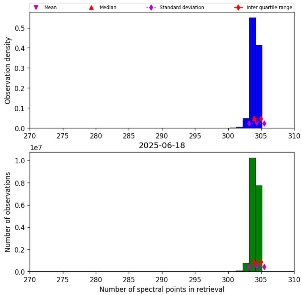
Figure 31: Histogram of “Number of spectral points in retrieval” for 2025-06-18 to 2025-06-19
