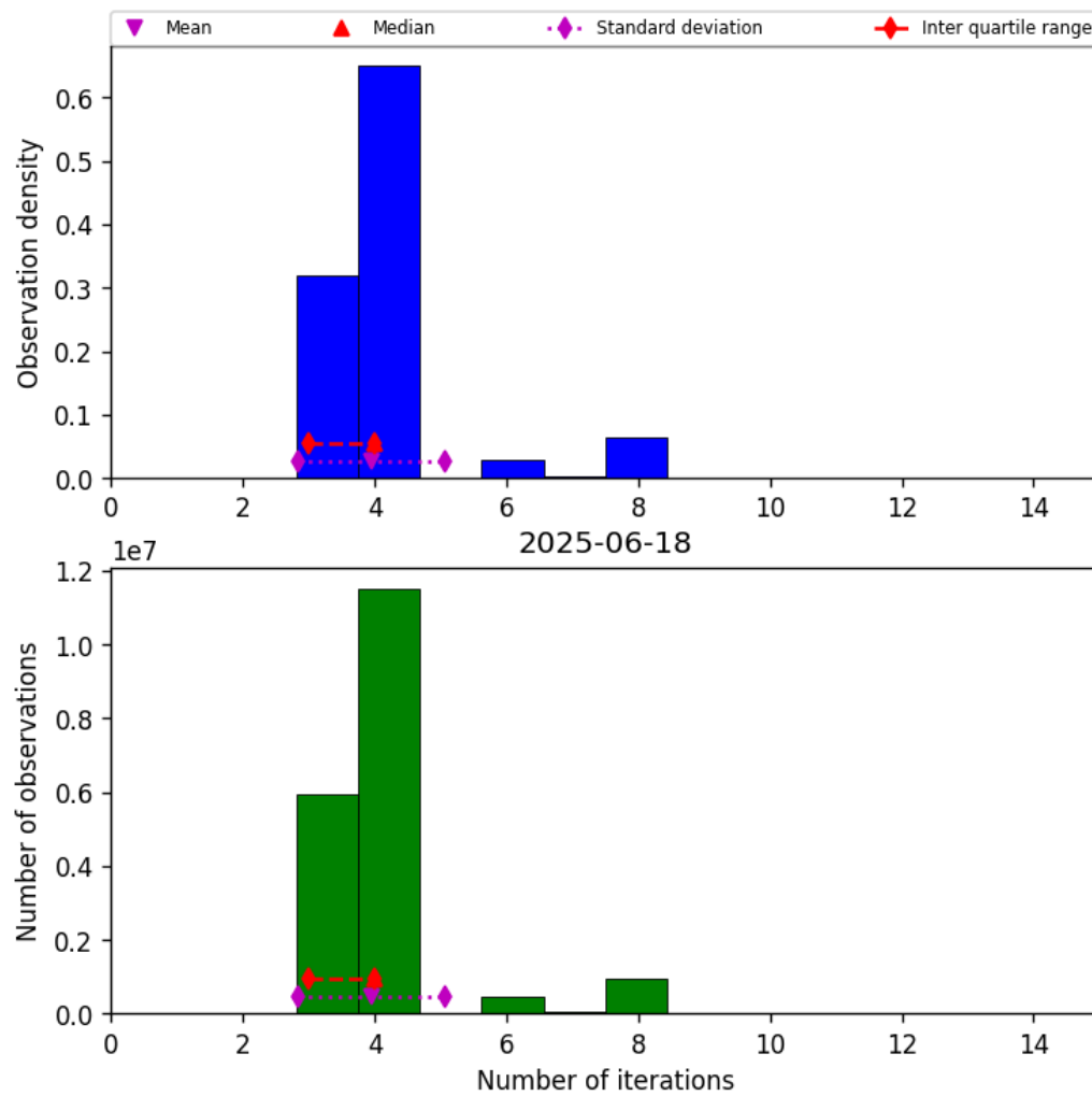
Figure 32: Histogram of “Number of iterations” for 2025-06-18 to 2025-06-19
