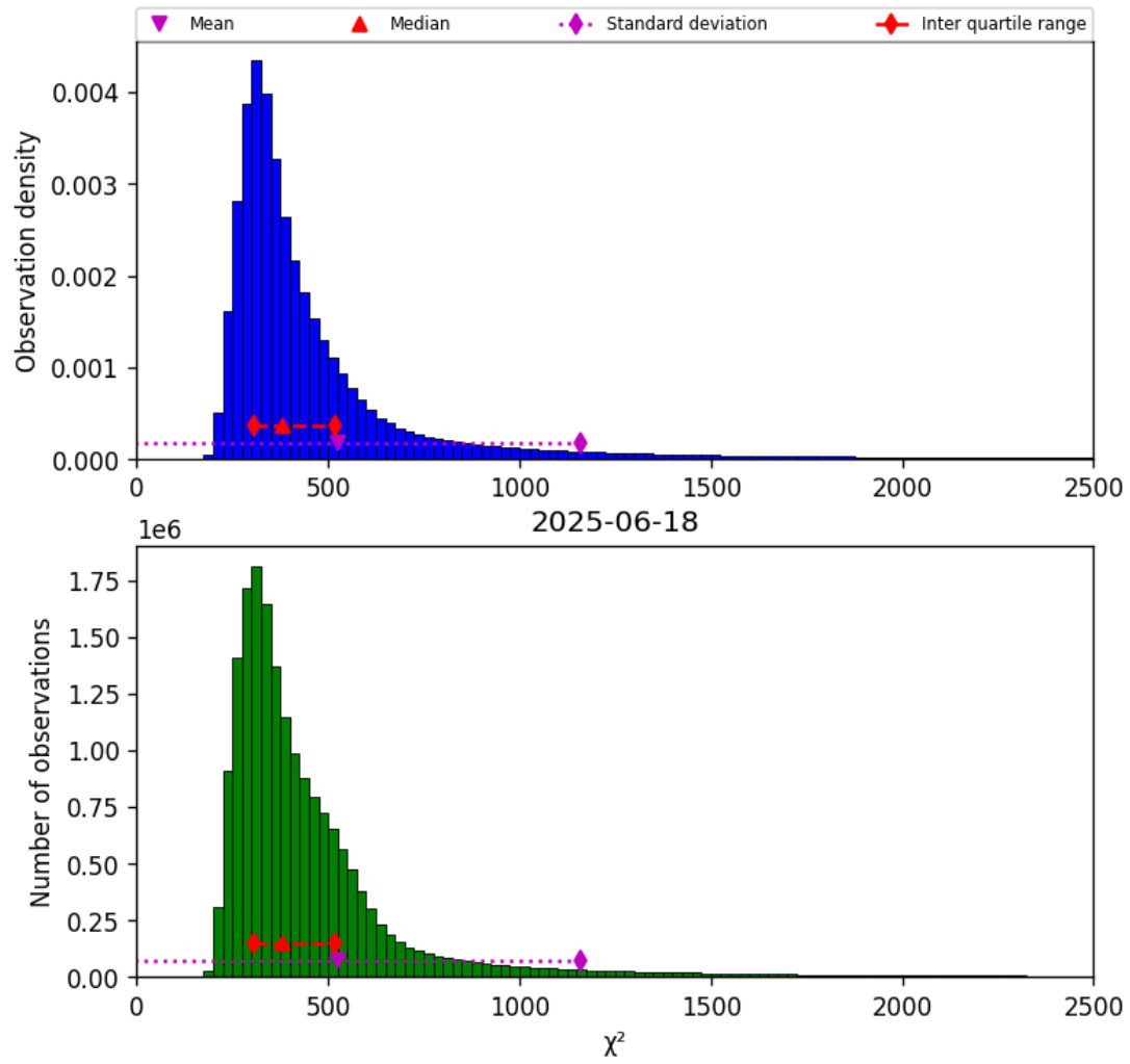
Figure 40: Histogram of “ \chi^2 ” for 2025-06-18 to 2025-06-19
