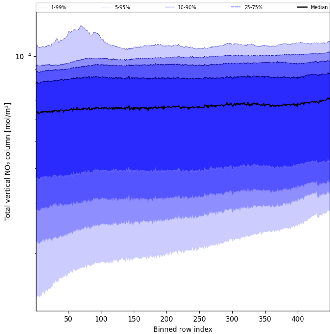
Figure 53: Along track statistics of “Total vertical NO 2 column” for 2025-06-18 to 2025-06-19
