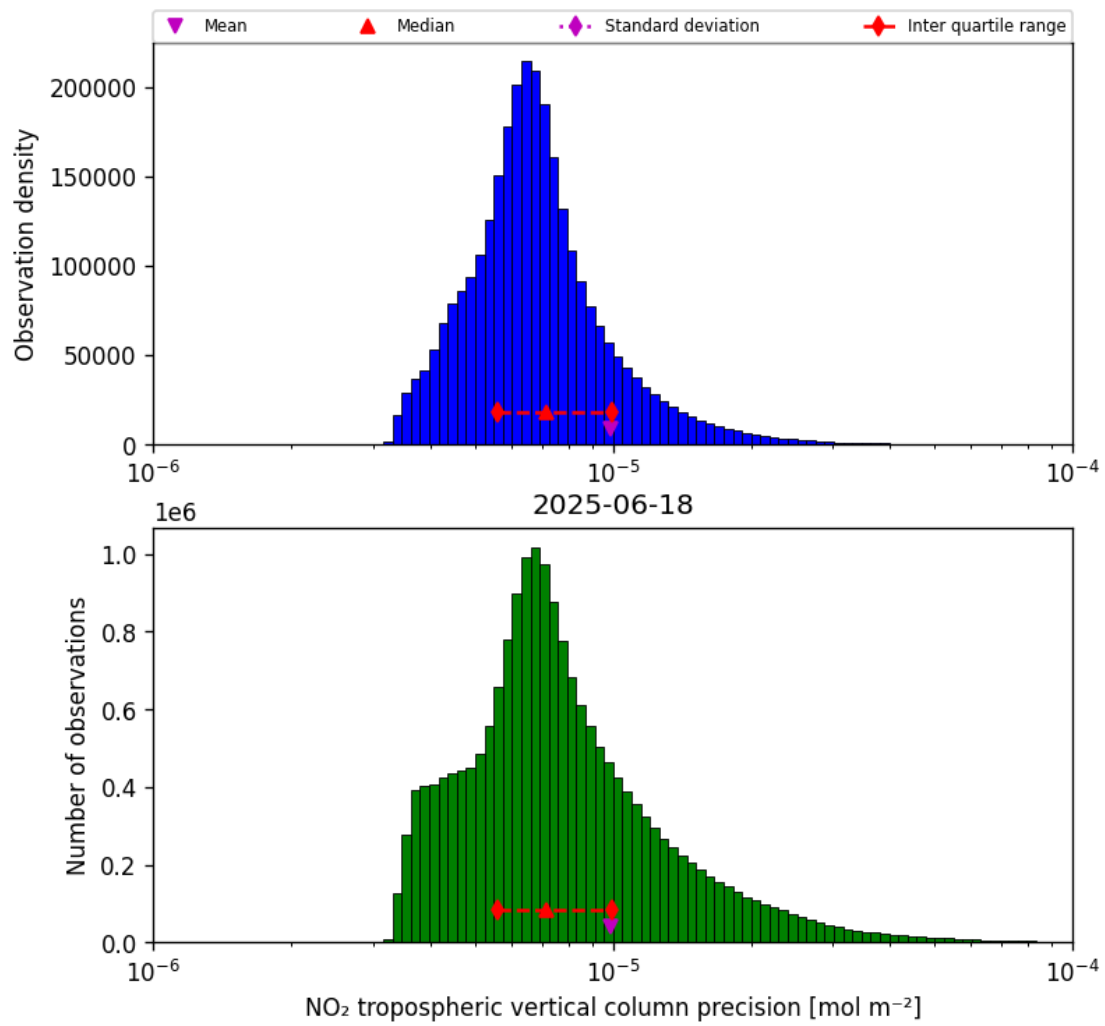
Figure 28: Histogram of “NO 2 tropospheric vertical column precision” for 2025-06-18 to 2025-06-19
