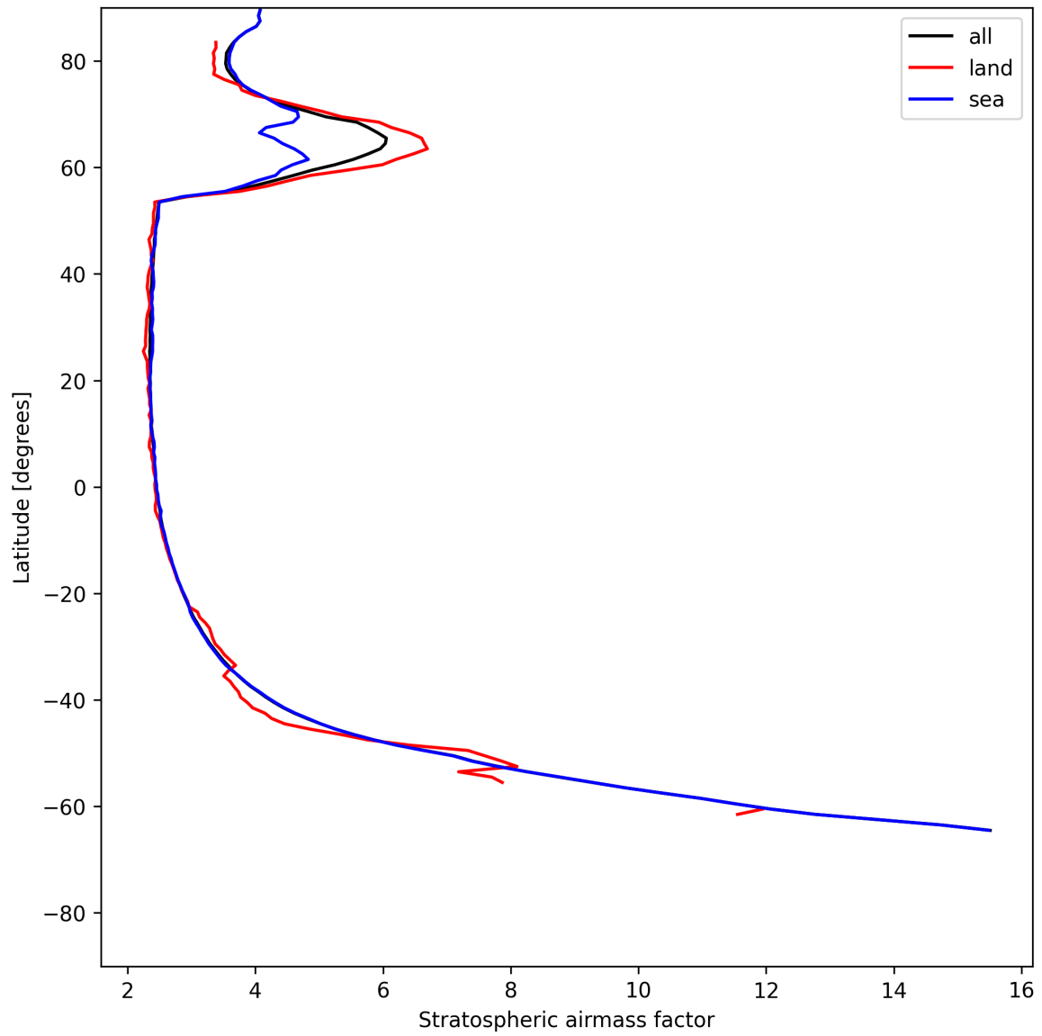
Figure 25: Zonal average of “Stratospheric airmass factor” for 2025-06-18 to 2025-06-19.
