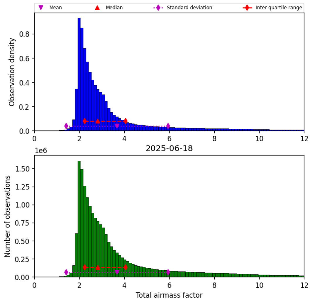
Figure 30: Histogram of “Total airmass factor” for 2025-06-18 to 2025-06-19
