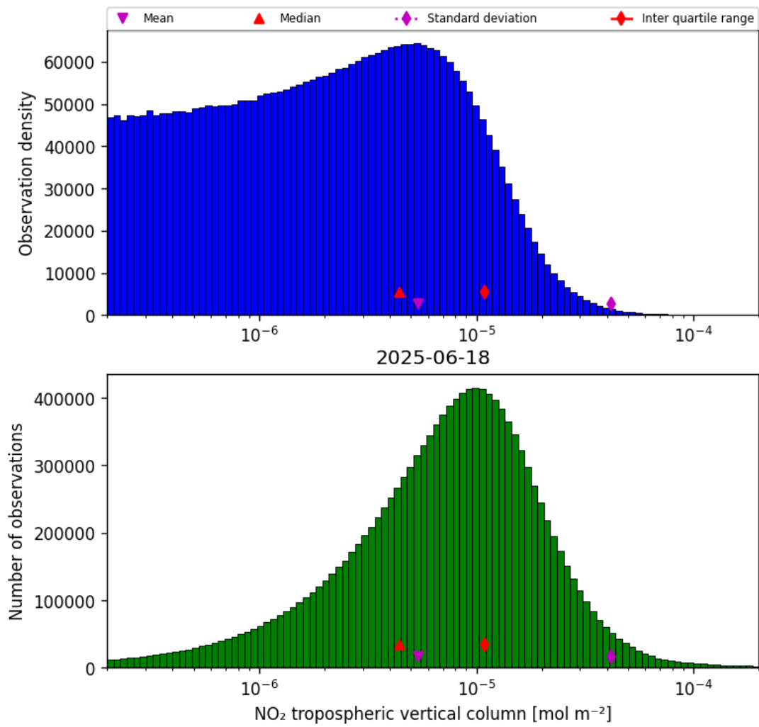
Figure 27: Histogram of “NO 2 tropospheric vertical column” for 2025-06-18 to 2025-06-19
