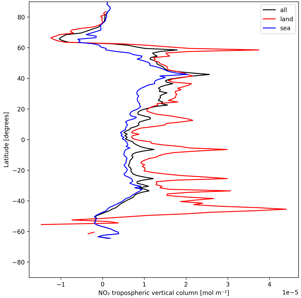
Figure 10: Zonal average of “NO 2 tropospheric vertical column” for 2025-06-18 to 2025-06-19.
