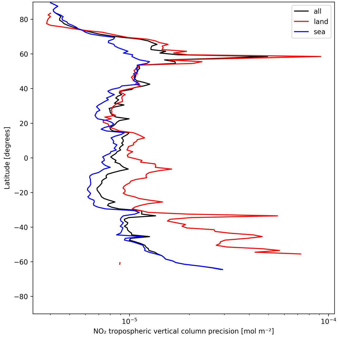
Figure 11: Zonal average of “NO 2 tropospheric vertical column precision” for 2025-06-18 to 2025-06-19.
