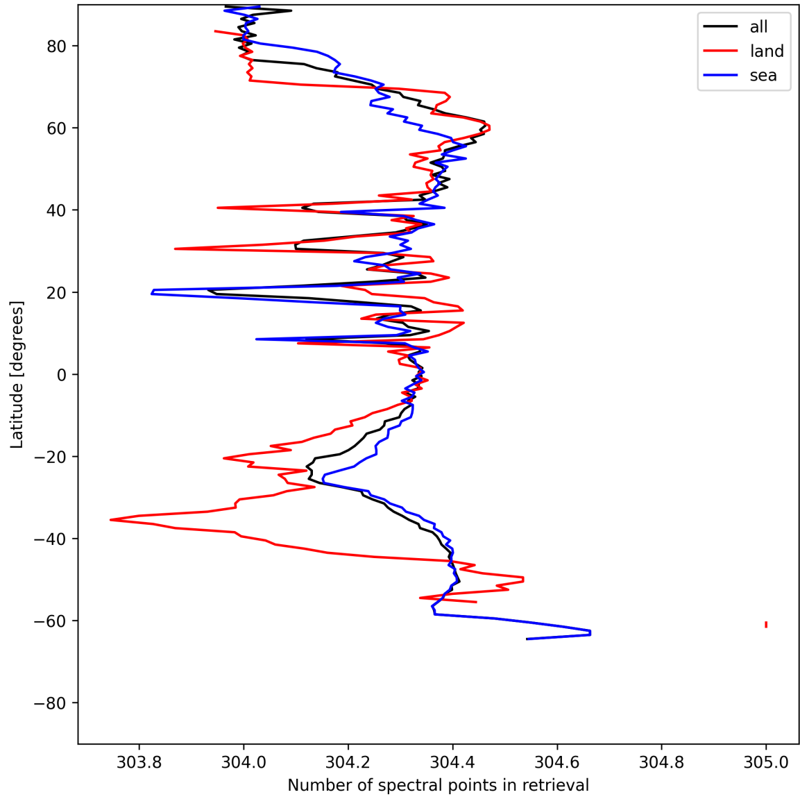
Figure 14: Zonal average of “Number of spectral points in retrieval” for 2025-06-18 to 2025-06-19.
