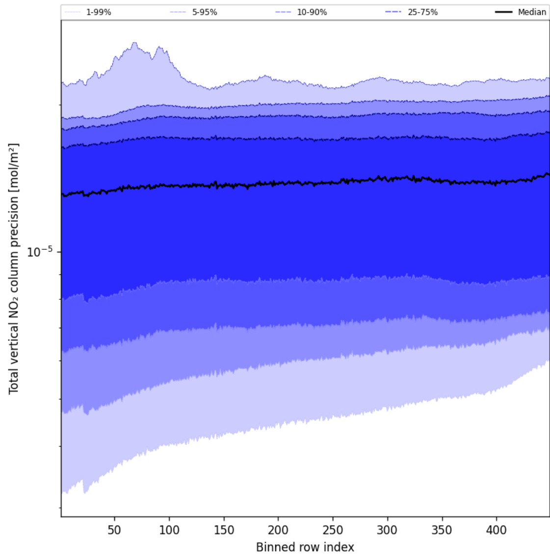
Figure 54: Along track statistics of “Total vertical NO 2 column precision” for 2025-06-18 to 2025-06-19
