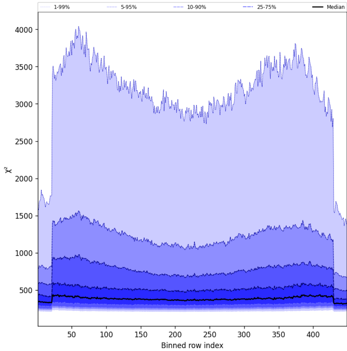
Figure 57: Along track statistics of “ \chi^2 ” for 2025-06-18 to 2025-06-19
