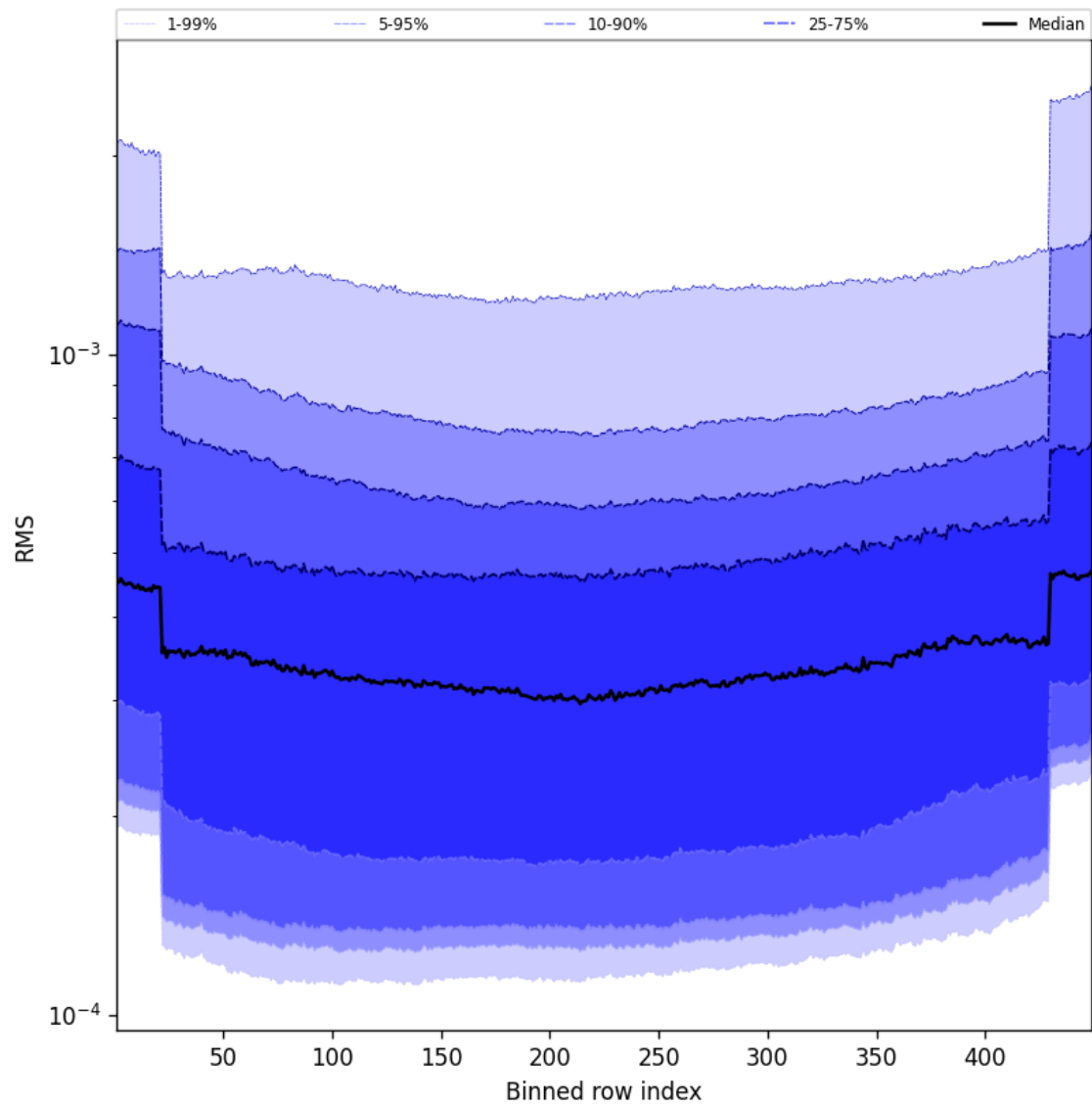
Figure 58: Along track statistics of “RMS” for 2025-06-18 to 2025-06-19
