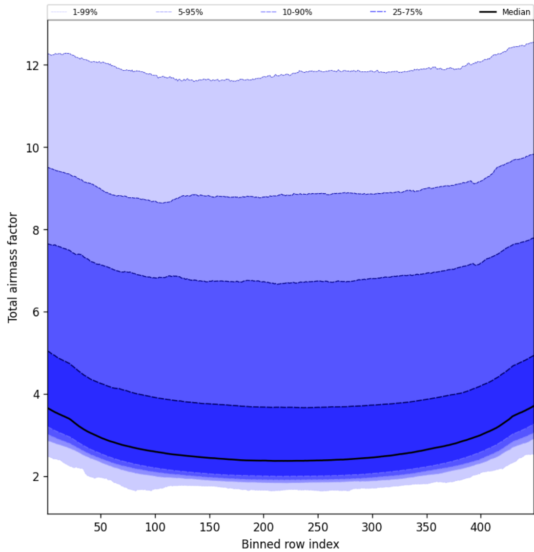
Figure 47: Along track statistics of “Total airmass factor” for 2025-06-18 to 2025-06-19
