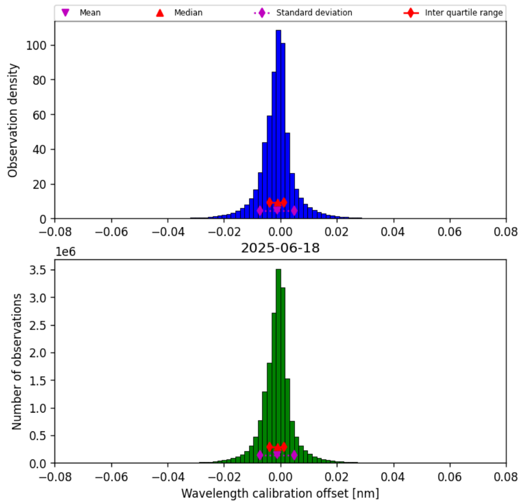
Figure 33: Histogram of “Wavelength calibration offset” for 2025-06-18 to 2025-06-19
