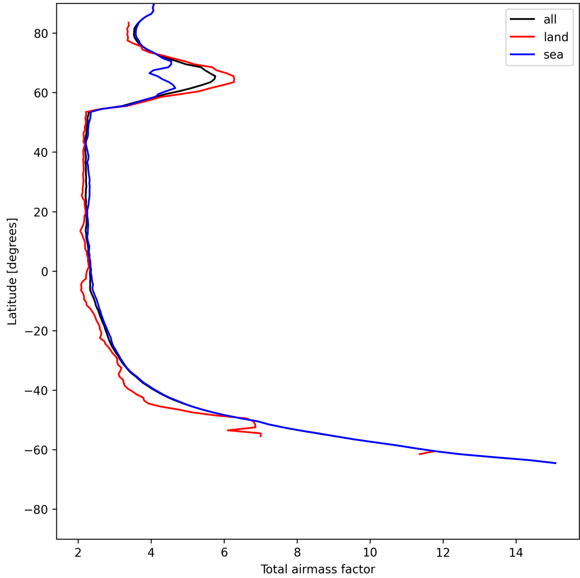
Figure 13: Zonal average of “Total airmass factor” for 2025-06-18 to 2025-06-19.
