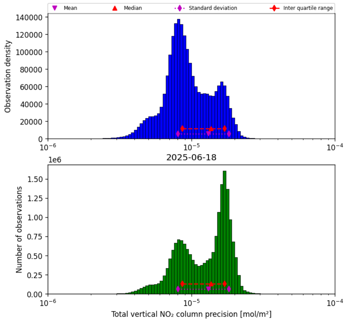
Figure 37: Histogram of “Total vertical NO 2 column precision” for 2025-06-18 to 2025-06-19
