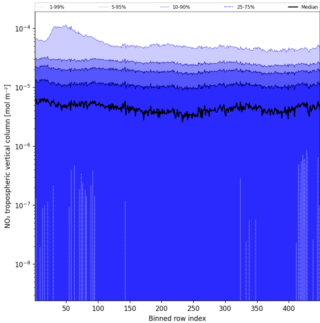
Figure 44: Along track statistics of “NO 2 tropospheric vertical column” for 2025-06-18 to 2025-06-19
