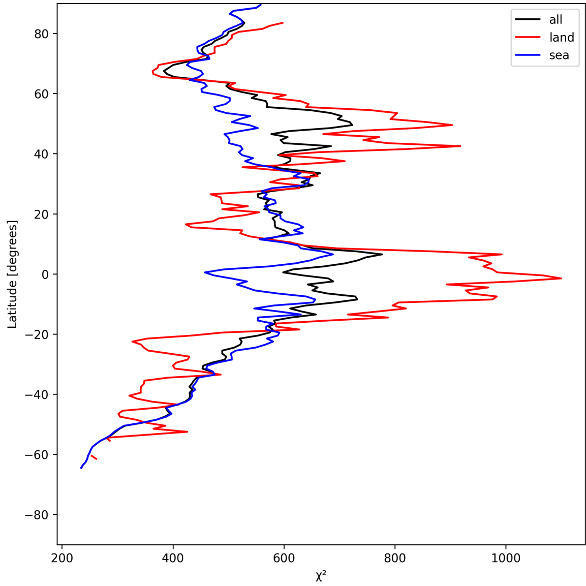
Figure 23: Zonal average of “ \chi^2 ” for 2025-06-18 to 2025-06-19.
