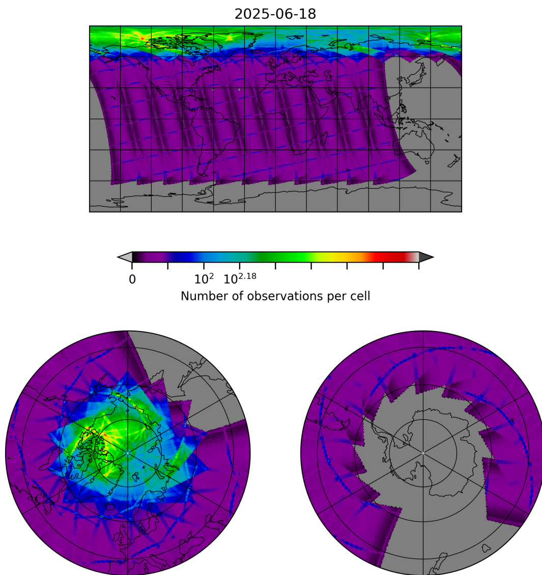
Figure 8: Map of the number of observations for 2025-06-18 to 2025-06-19
