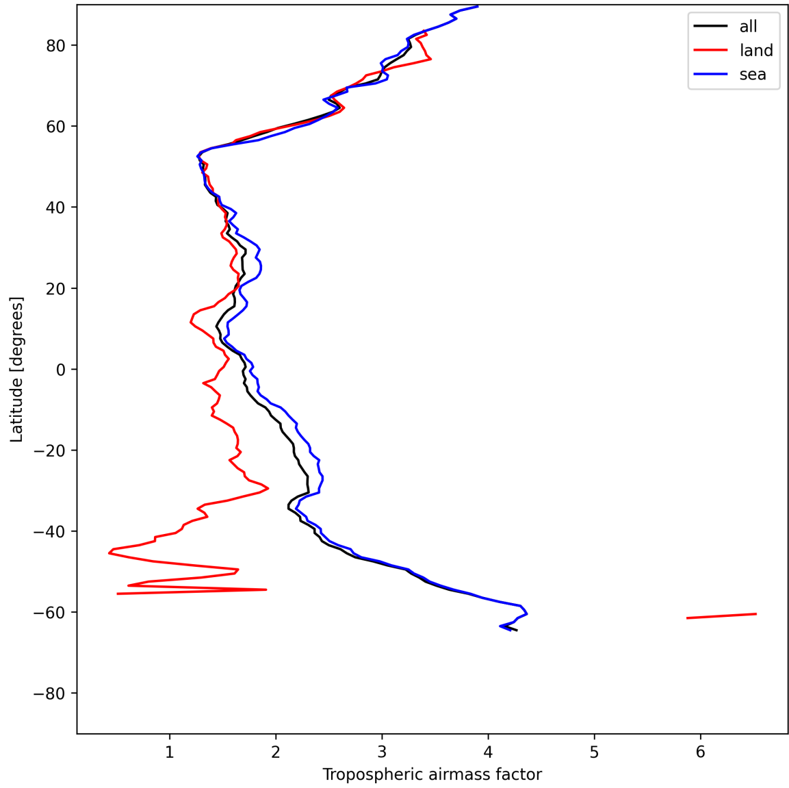
Figure 12: Zonal average of “Tropospheric airmass factor” for 2025-06-18 to 2025-06-19.
