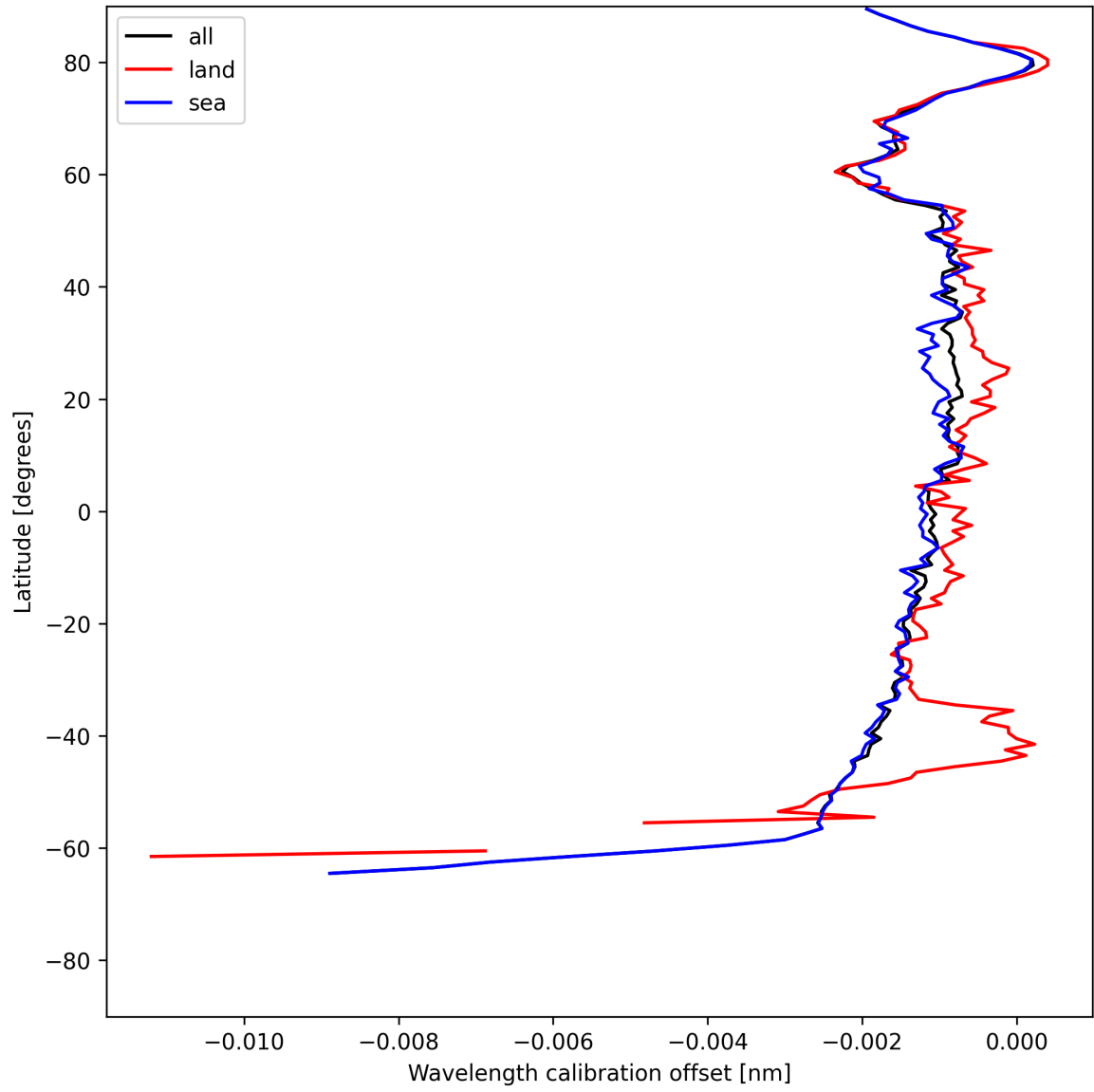
Figure 16: Zonal average of “Wavelength calibration offset” for 2025-06-18 to 2025-06-19.
