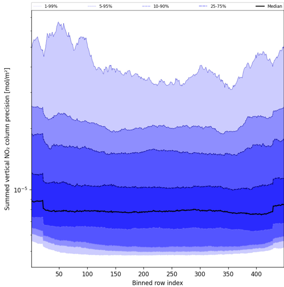
Figure 56: Along track statistics of “Summed vertical NO 2 column precision” for 2025-06-18 to 2025-06-19
