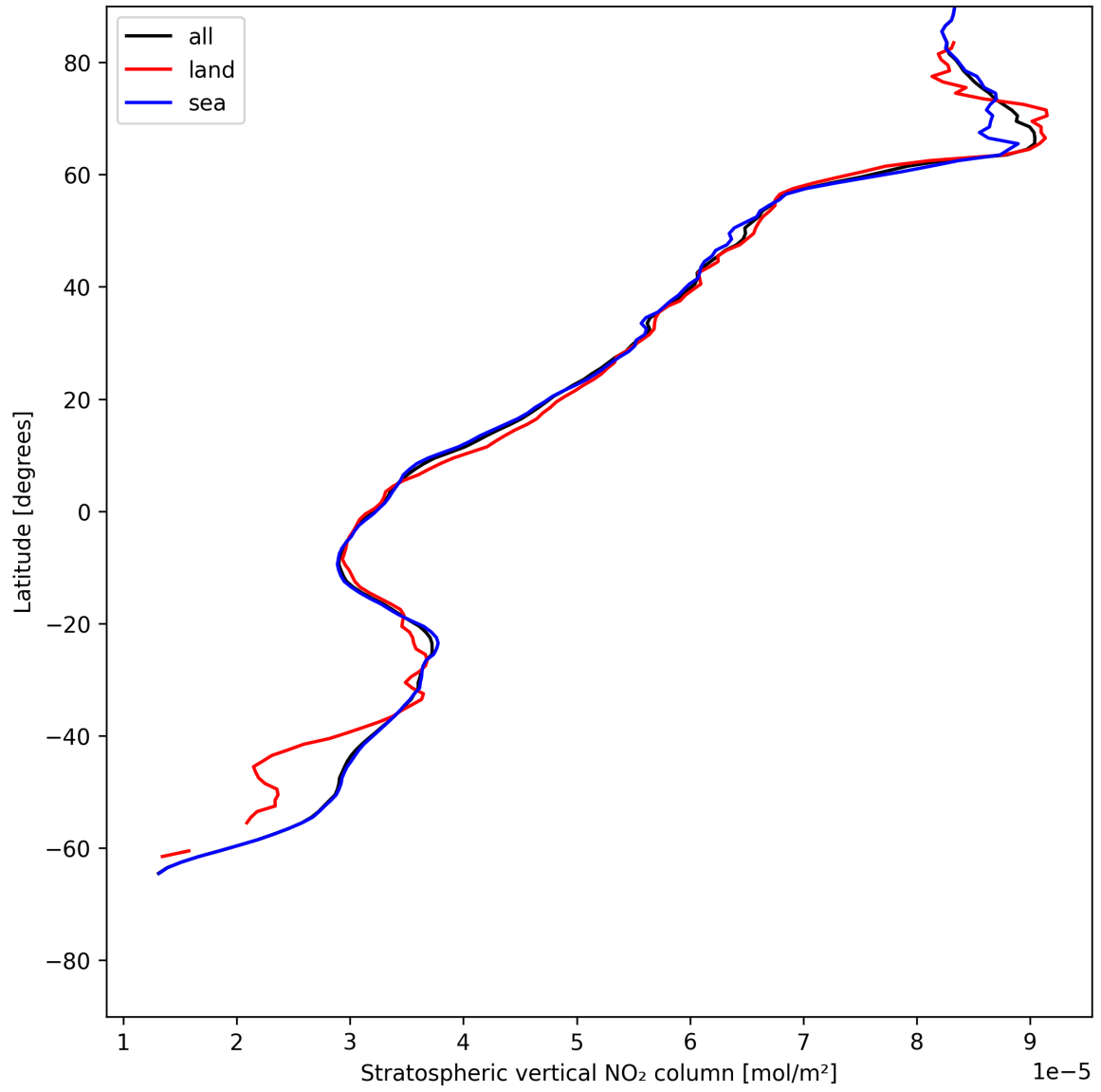
Figure 17: Zonal average of “Stratospheric vertical NO 2 column” for 2025-06-18 to 2025-06-19.
