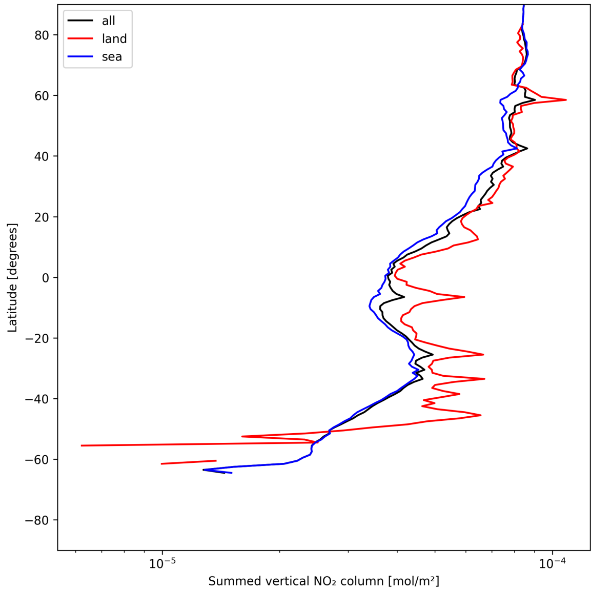
Figure 21: Zonal average of “Summed vertical NO 2 column” for 2025-06-18 to 2025-06-19.
