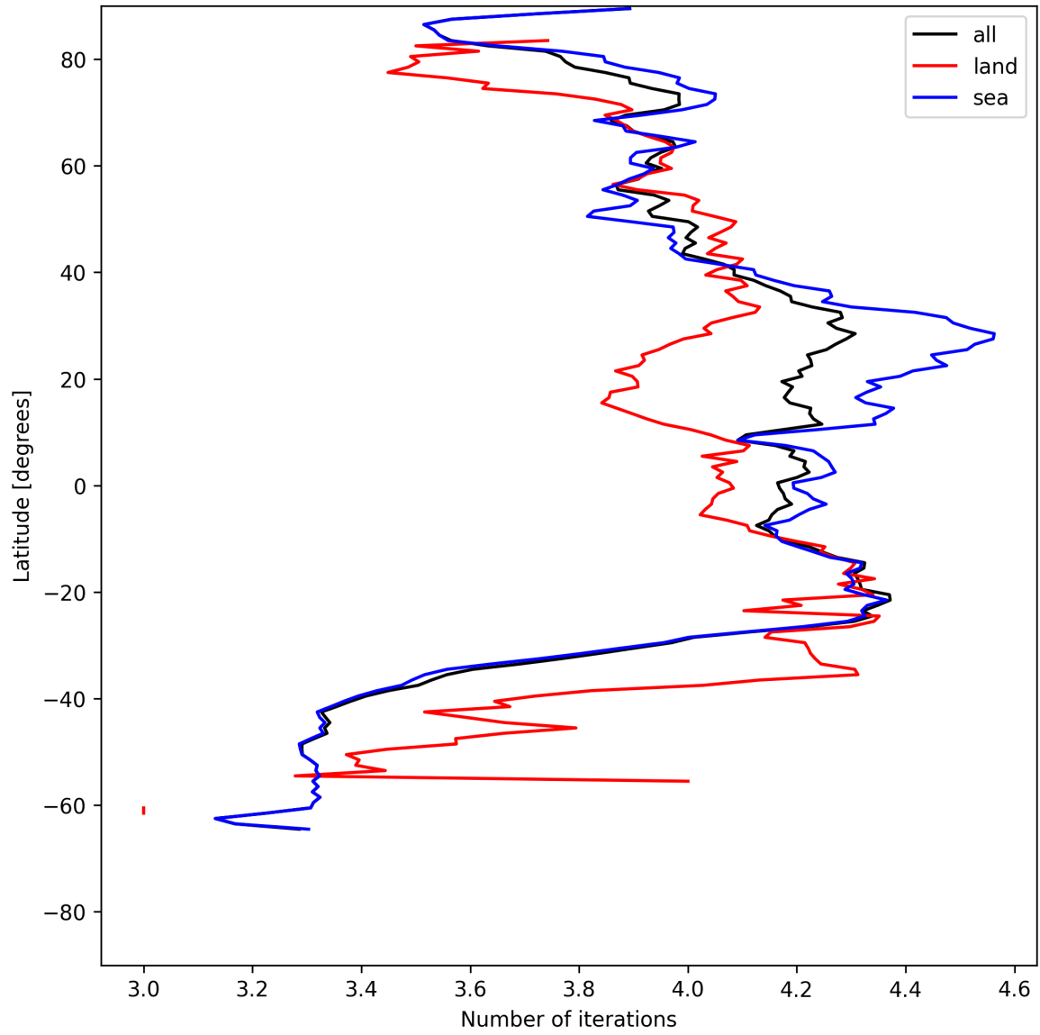
Figure 15: Zonal average of “Number of iterations” for 2025-06-18 to 2025-06-19.
