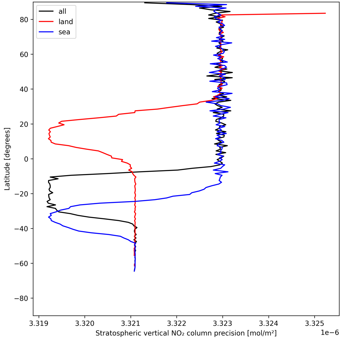
Figure 18: Zonal average of “Stratospheric vertical NO 2 column precision” for 2025-06-18 to 2025-06-19.
