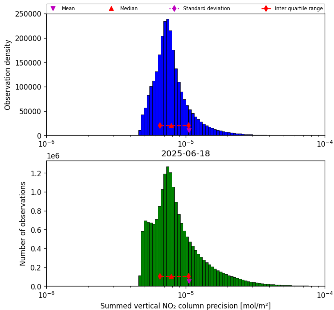
Figure 39: Histogram of "Summed vertical NO 2 column precision" for 2025-06-18 to 2025-06-19
