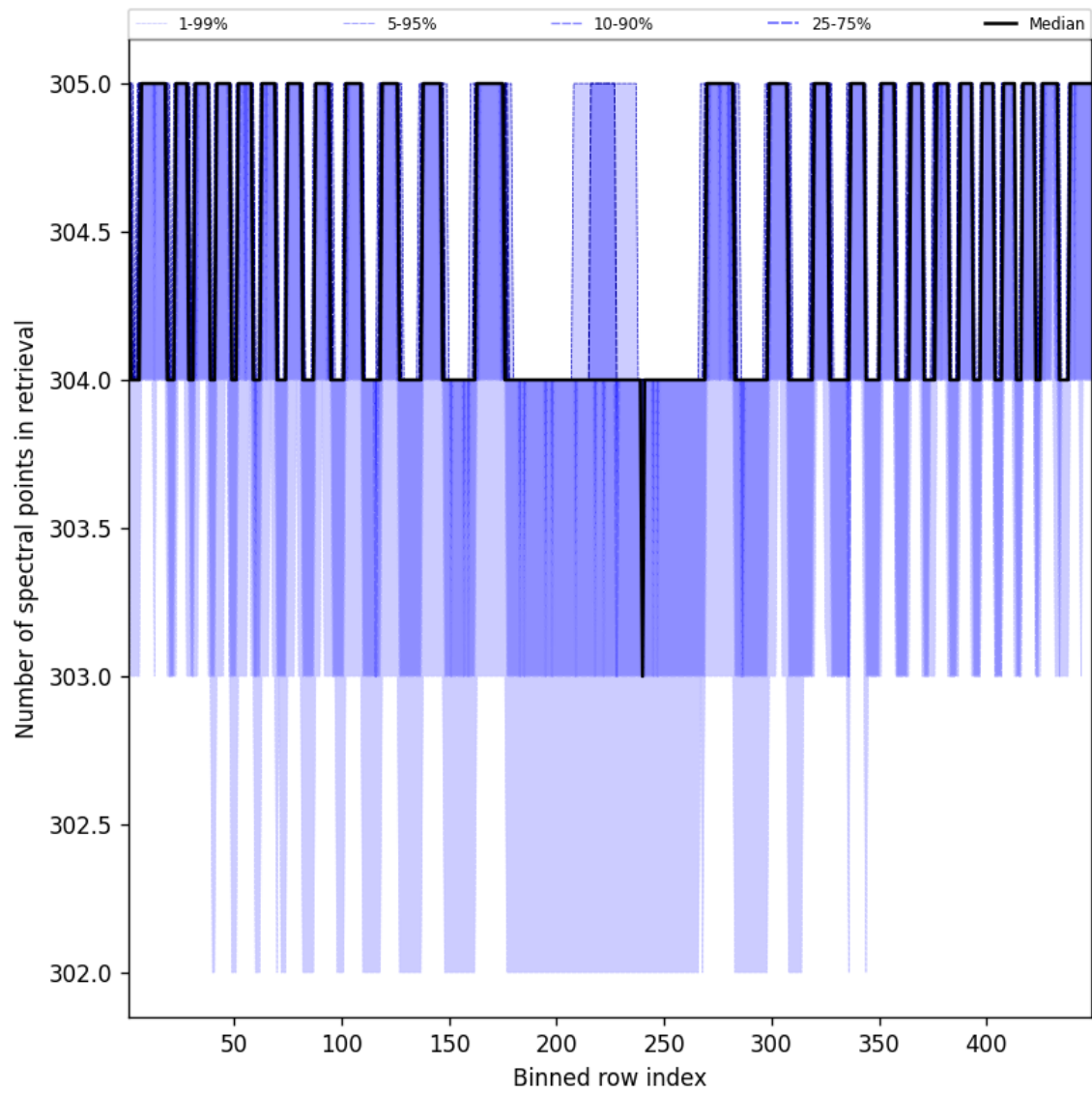
Figure 48: Along track statistics of “Number of spectral points in retrieval” for 2025-06-18 to 2025-06-19
