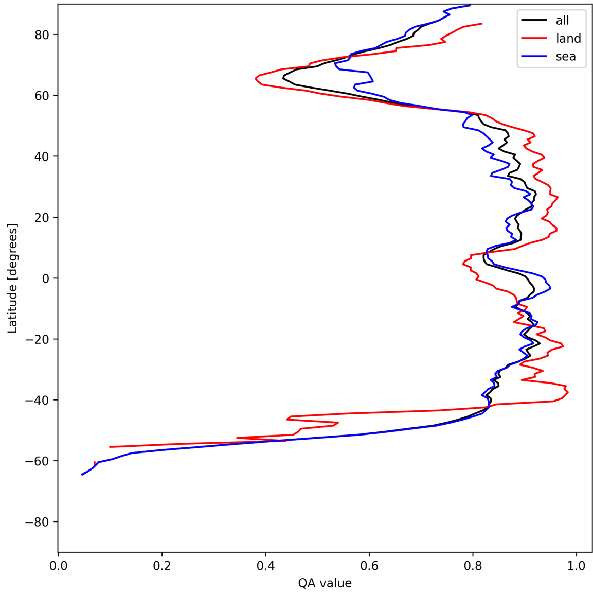
Figure 9: Zonal average of “QA value” for 2025-06-18 to 2025-06-19.
