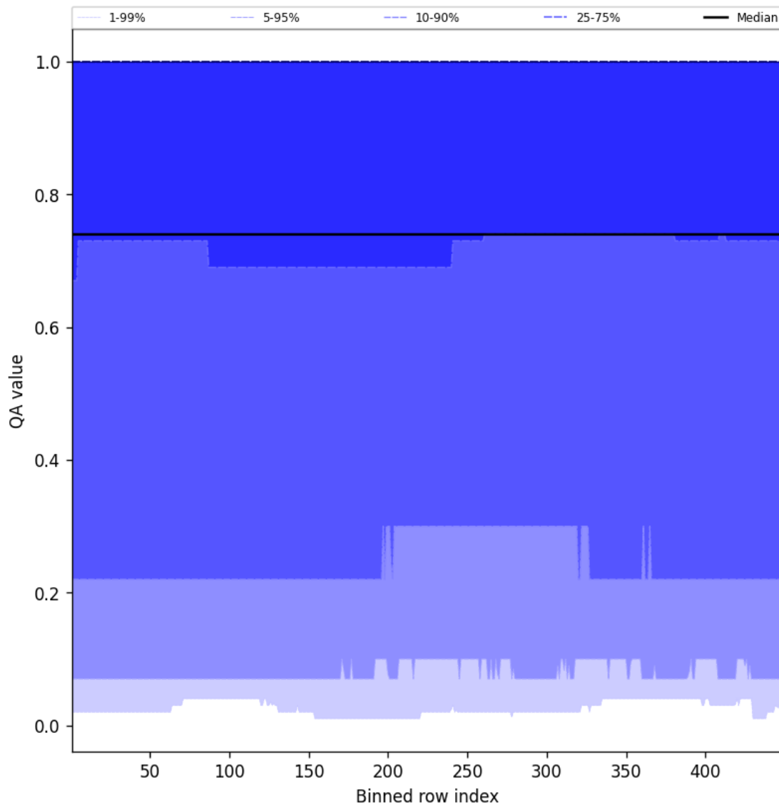
Figure 43: Along track statistics of “QA value” for 2025-06-18 to 2025-06-19
