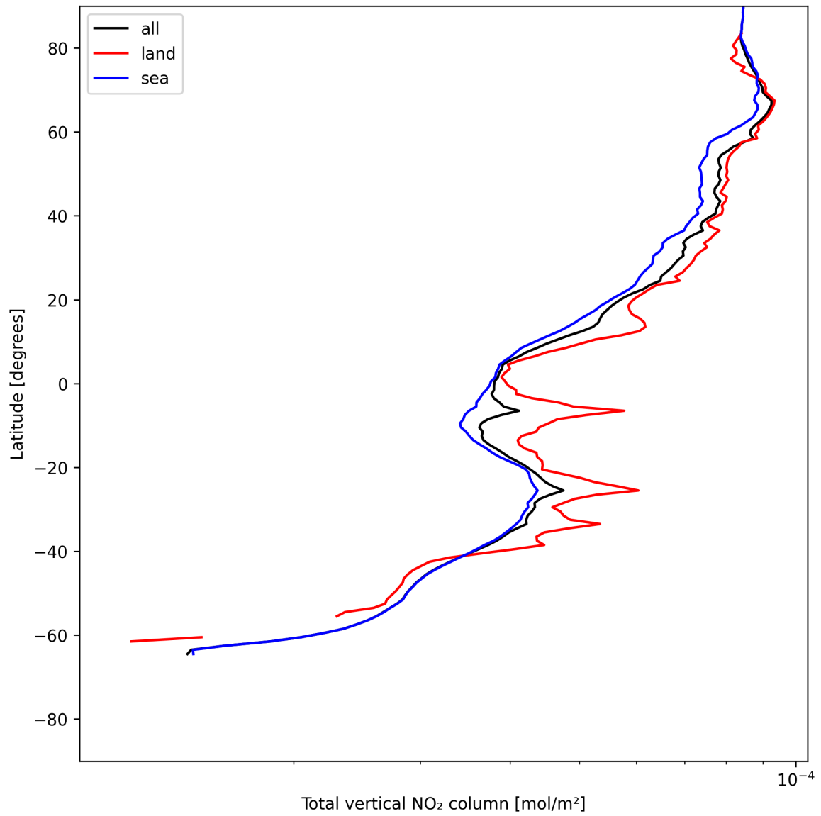
Figure 19: Zonal average of “Total vertical NO 2 column” for 2025-06-18 to 2025-06-19.
