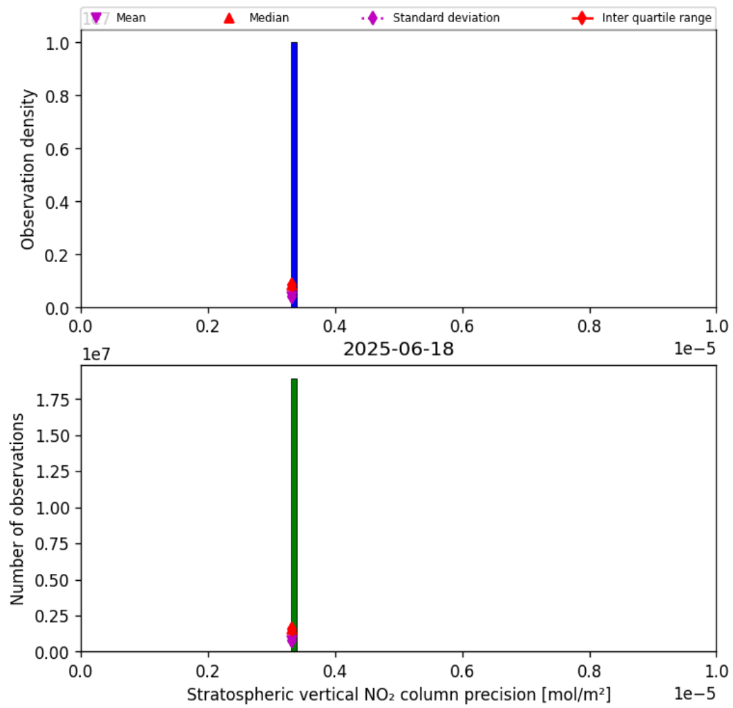
Figure 35: Histogram of “Stratospheric vertical NO 2 column precision” for 2025-06-18 to 2025-06-19
