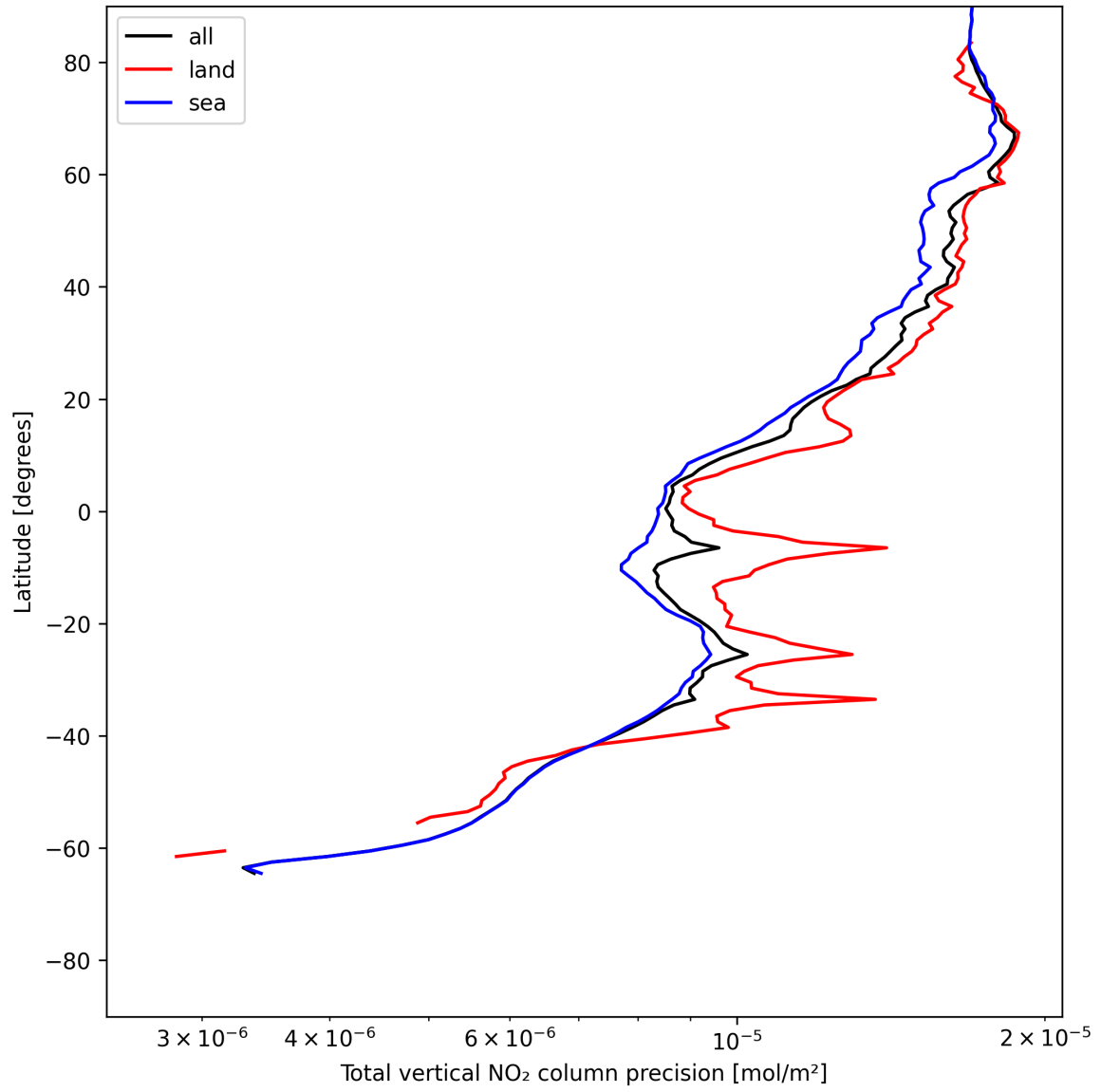
Figure 20: Zonal average of "Total vertical NO 2 column precision" for 2025-06-18 to 2025-06-19.
