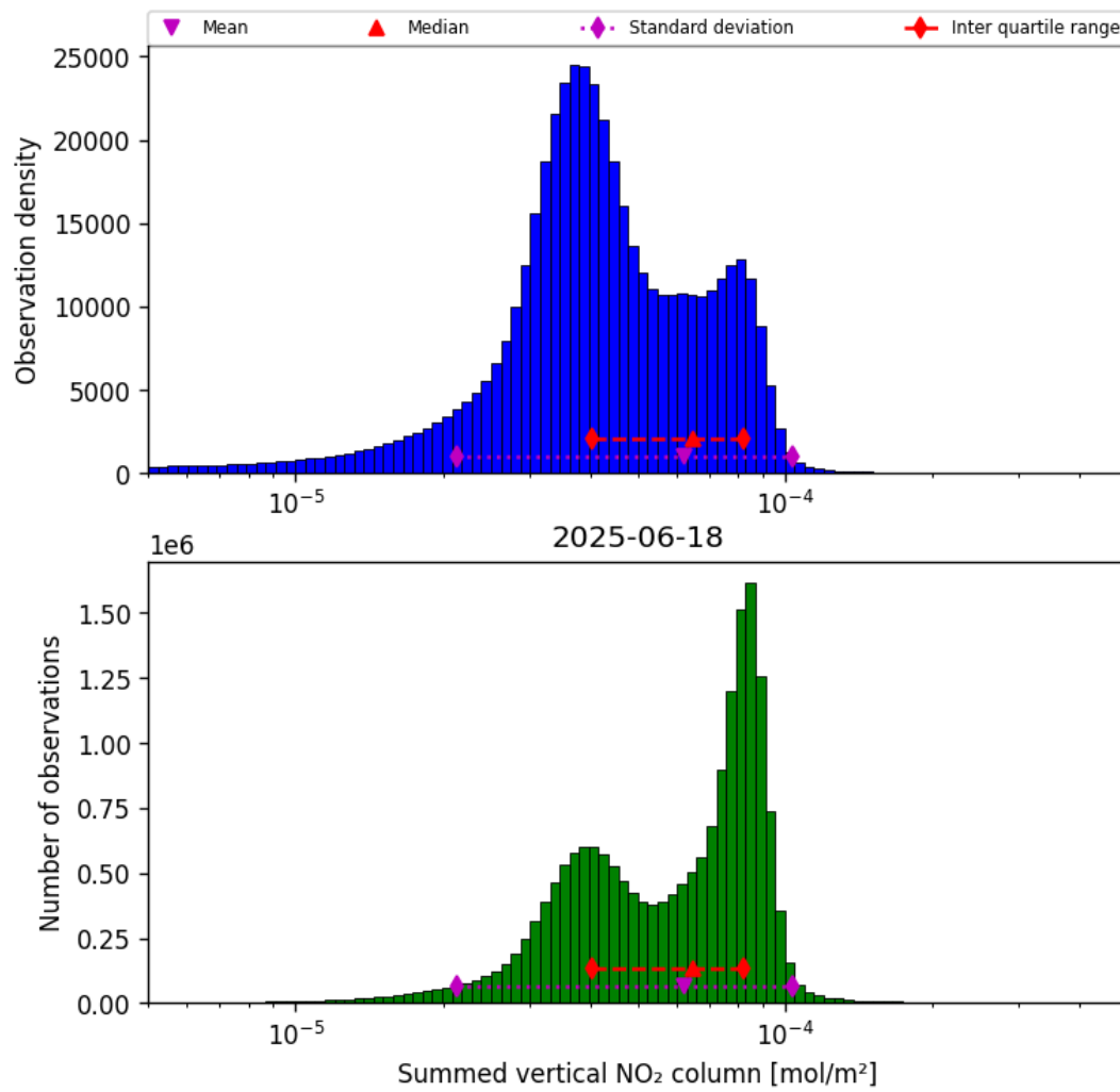
Figure 38: Histogram of “Summed vertical NO 2 column” for 2025-06-18 to 2025-06-19
