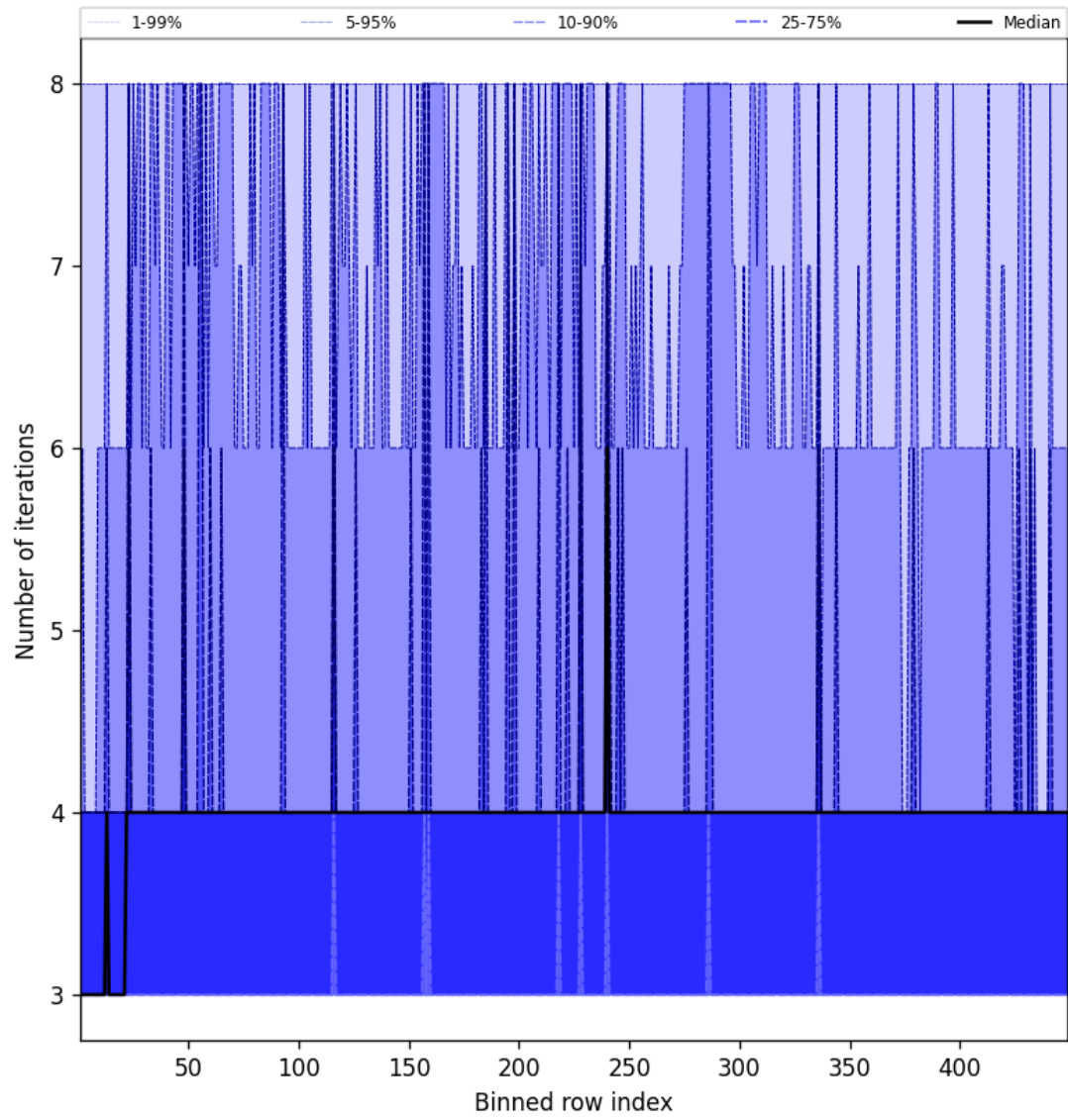
Figure 49: Along track statistics of “Number of iterations” for 2025-06-18 to 2025-06-19
