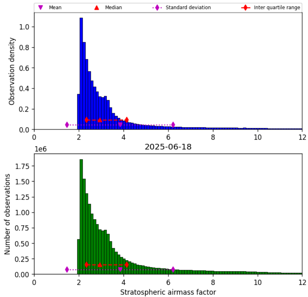
Figure 42: Histogram of “Stratospheric airmass factor” for 2025-06-18 to 2025-06-19
