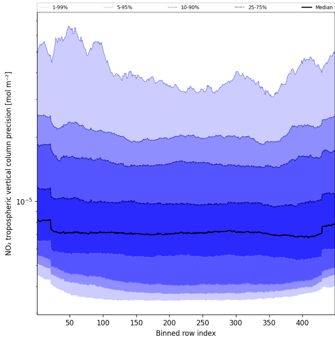
Figure 45: Along track statistics of “NO 2 tropospheric vertical column precision” for 2025-06-18 to 2025-06-19
