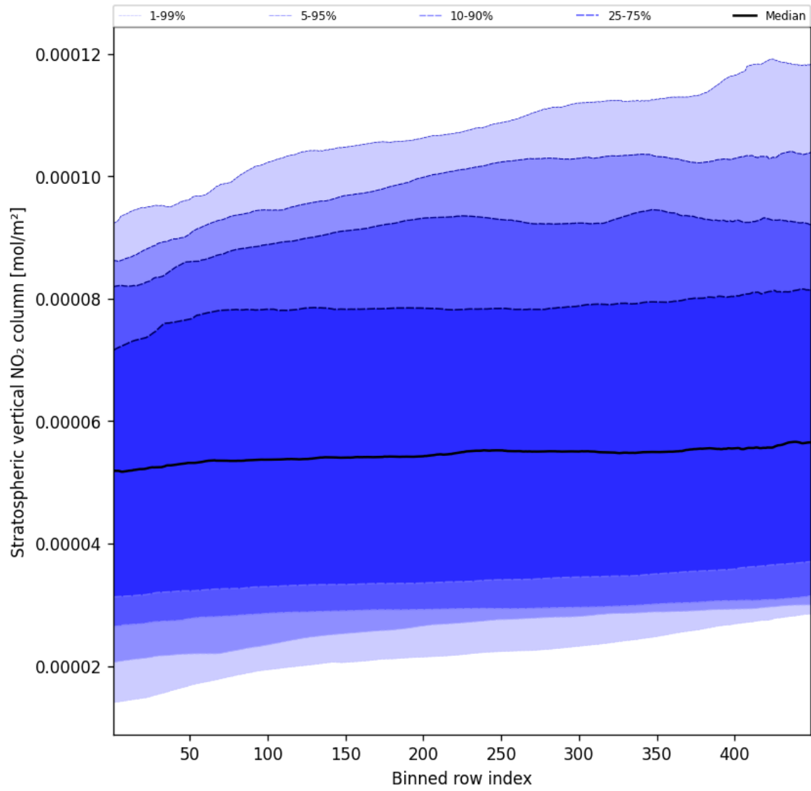
Figure 51: Along track statistics of “Stratospheric vertical NO 2 column” for 2025-06-18 to 2025-06-19
