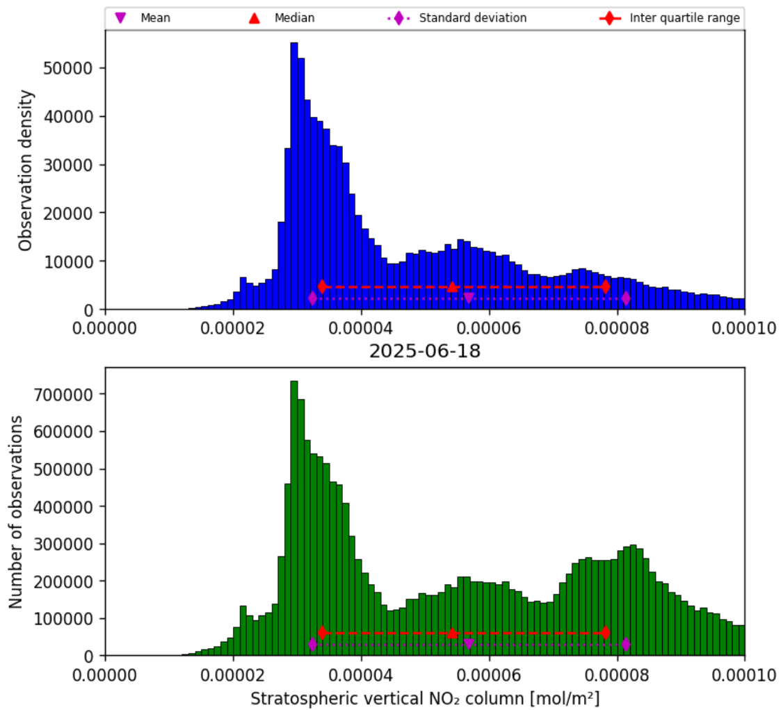
Figure 34: Histogram of “Stratospheric vertical NO 2 column” for 2025-06-18 to 2025-06-19
