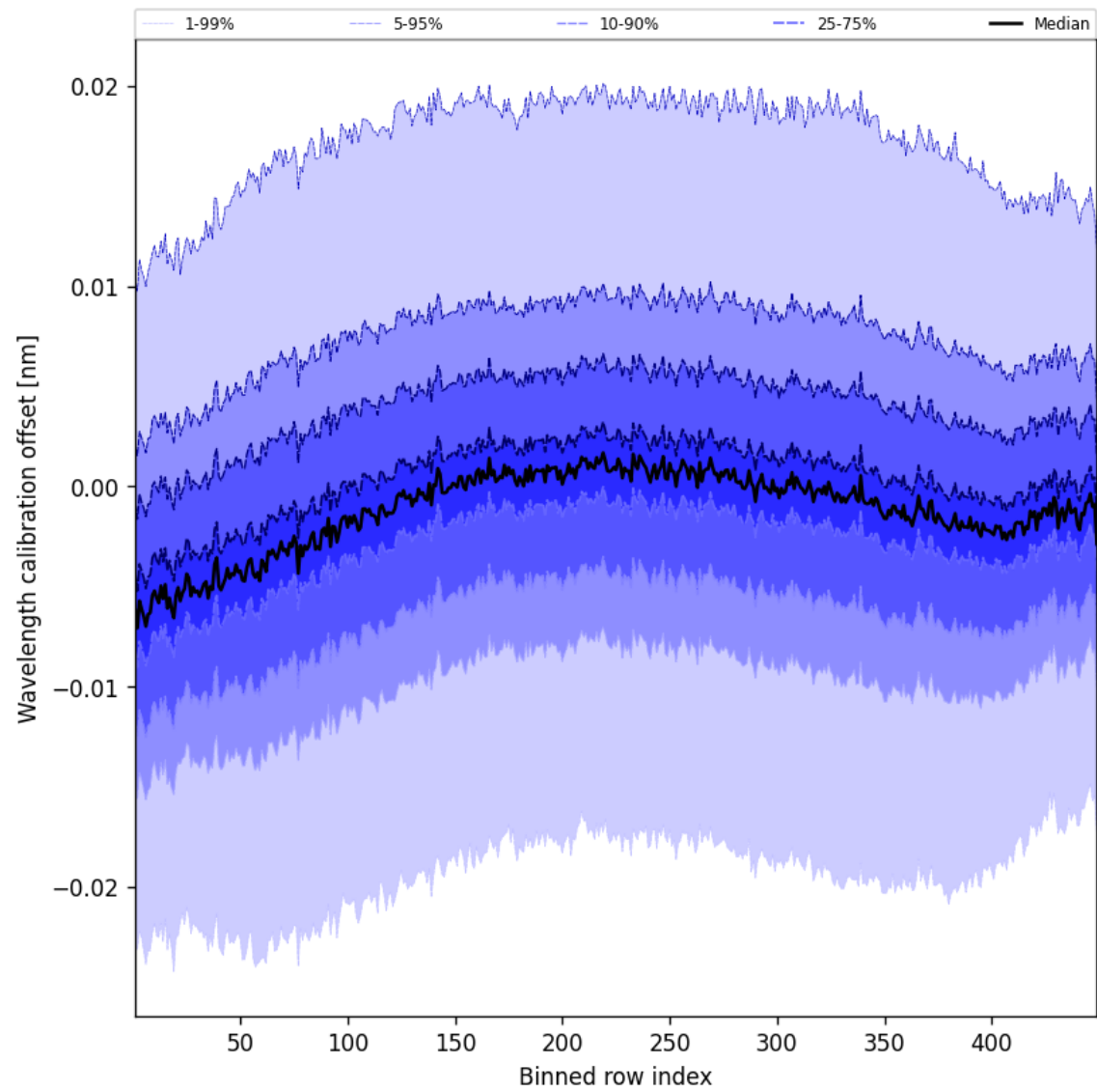
Figure 50: Along track statistics of “Wavelength calibration offset” for 2025-06-18 to 2025-06-19
