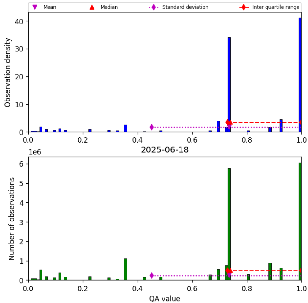
Figure 26: Histogram of “QA value” for 2025-06-18 to 2025-06-19
