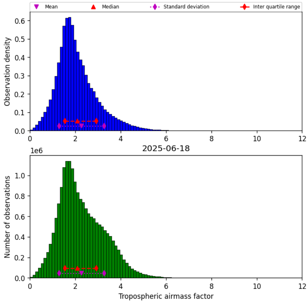
Figure 29: Histogram of “Tropospheric airmass factor” for 2025-06-18 to 2025-06-19
