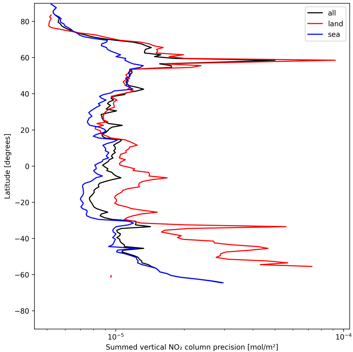
Figure 22: Zonal average of “Summed vertical NO 2 column precision” for 2025-06-18 to 2025-06-19.
