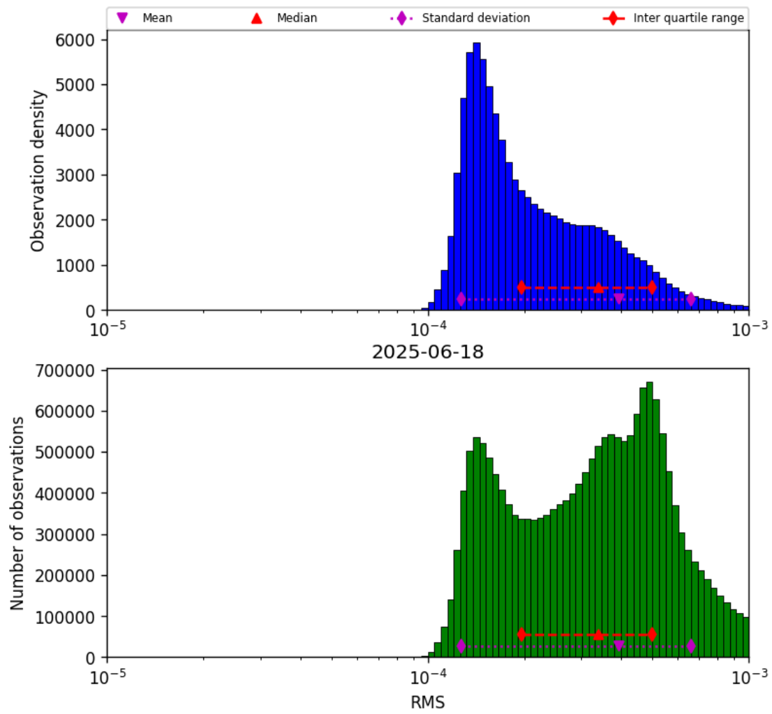
Figure 41: Histogram of “RMS” for 2025-06-18 to 2025-06-19
