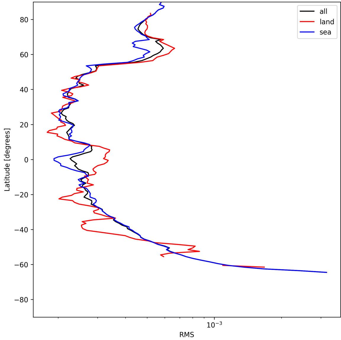
Figure 24: Zonal average of “RMS” for 2025-06-18 to 2025-06-19.
