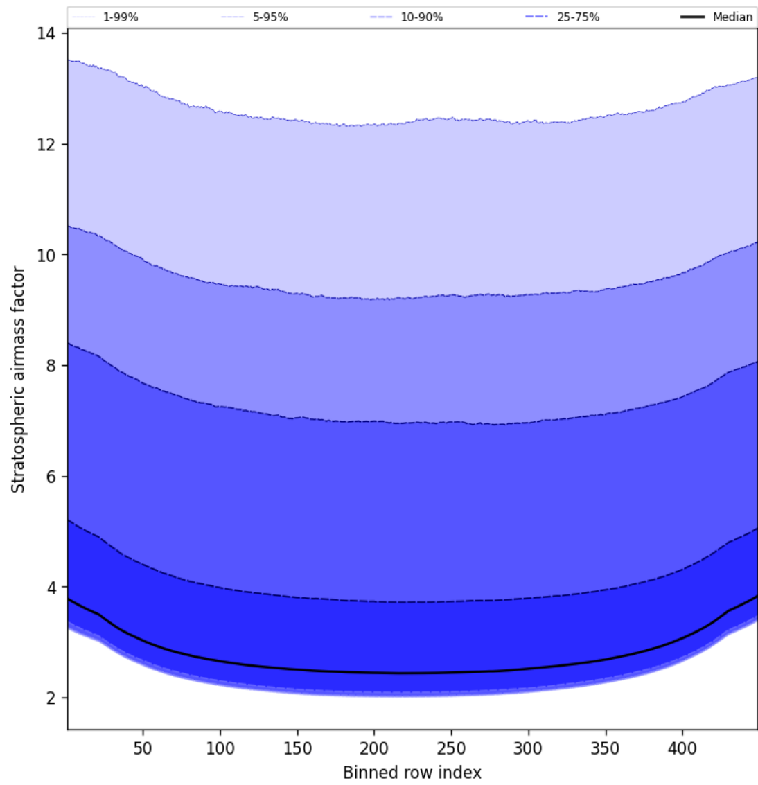
Figure 59: Along track statistics of “Stratospheric airmass factor” for 2025-06-18 to 2025-06-19
