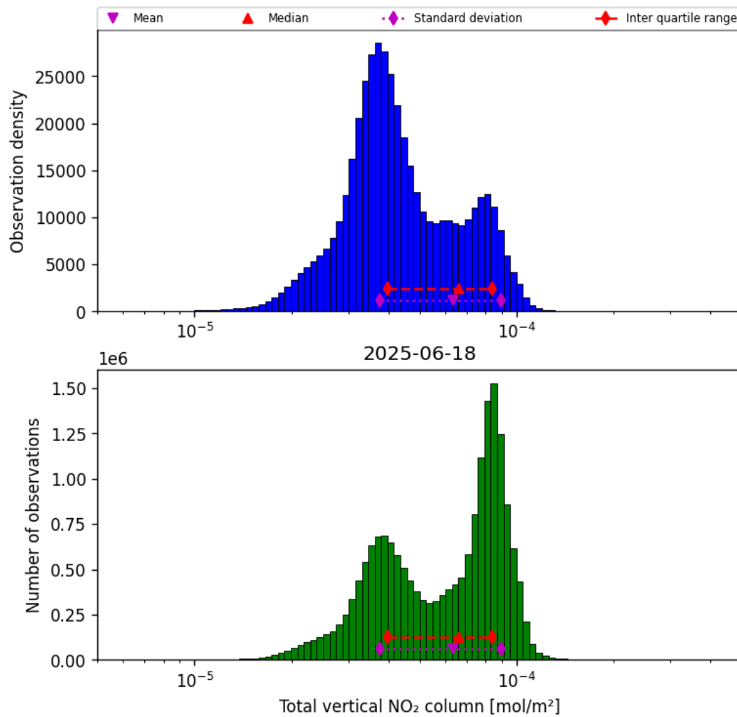
Figure 36: Histogram of “Total vertical NO 2 column” for 2025-06-18 to 2025-06-19
