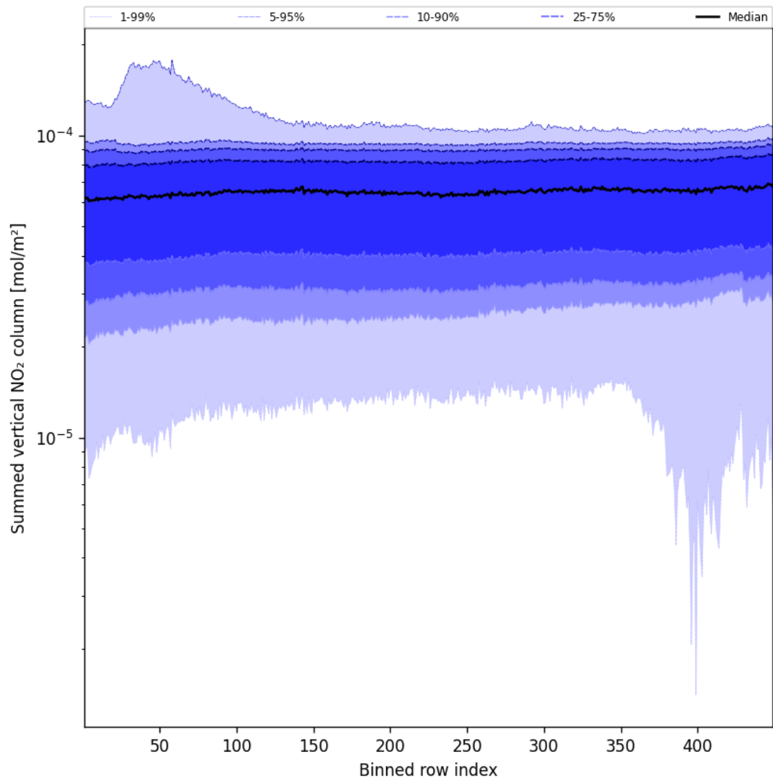
Figure 55: Along track statistics of “Summed vertical NO 2 column” for 2025-06-18 to 2025-06-19
