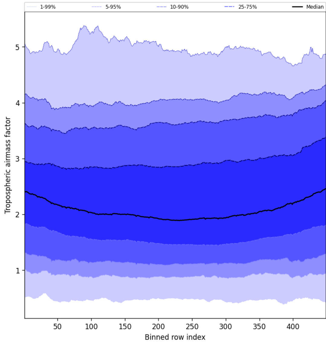
Figure 46: Along track statistics of “Tropospheric airmass factor” for 2025-06-18 to 2025-06-19
