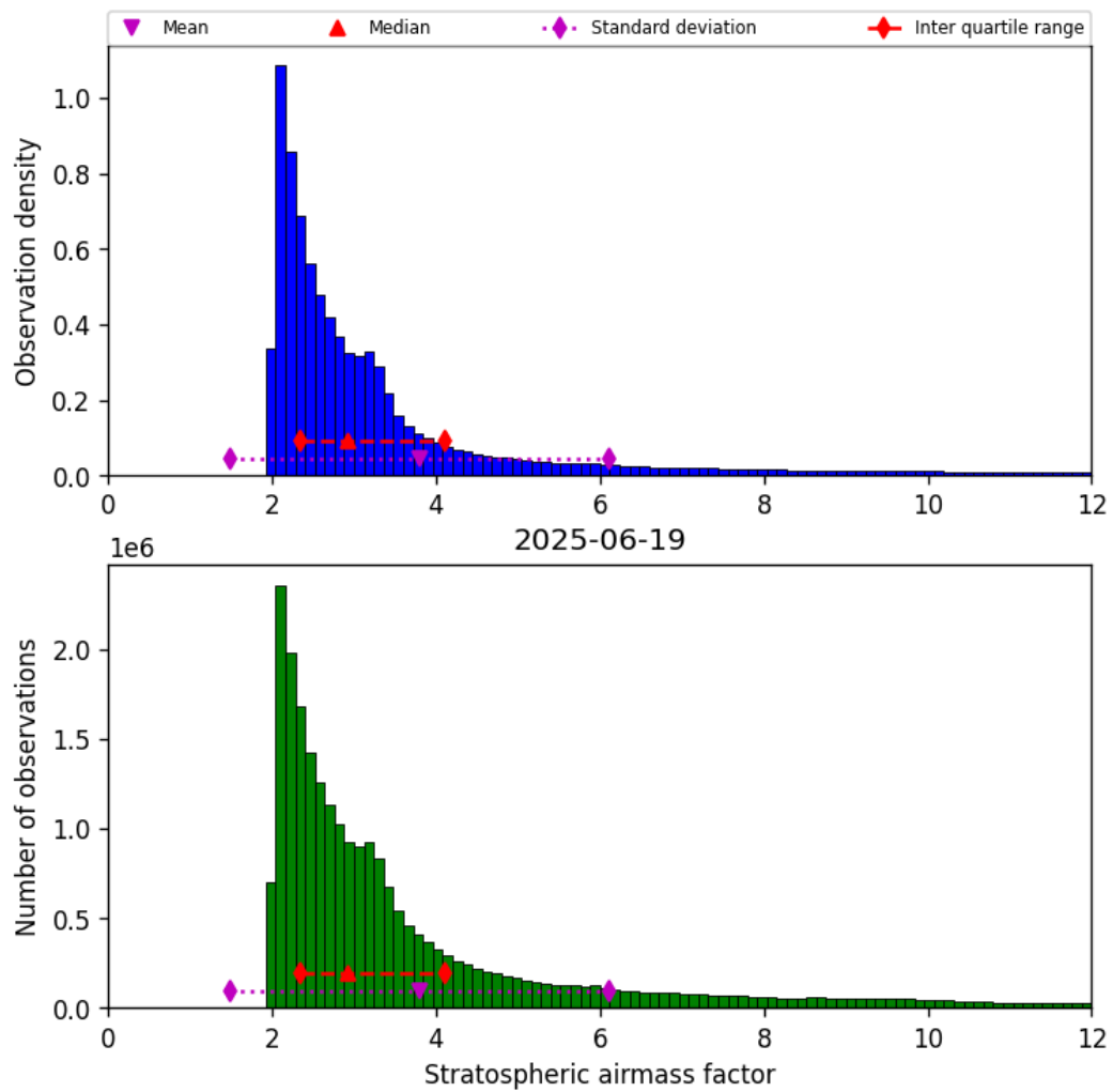
Figure 42: Histogram of “Stratospheric airmass factor” for 2025-06-19 to 2025-06-20
