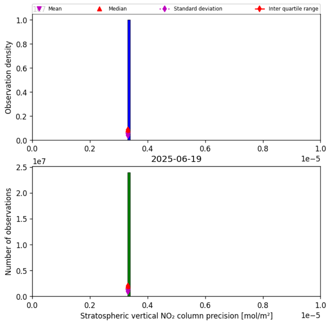
Figure 35: Histogram of “Stratospheric vertical NO 2 column precision” for 2025-06-19 to 2025-06-20
