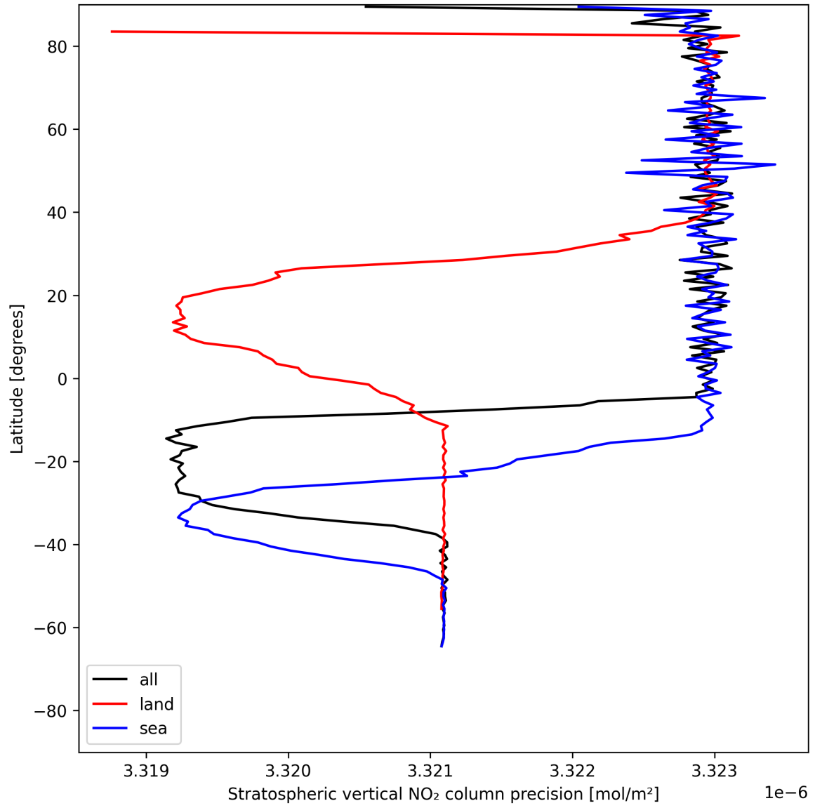
Figure 18: Zonal average of “Stratospheric vertical NO 2 column precision” for 2025-06-19 to 2025-06-20.
