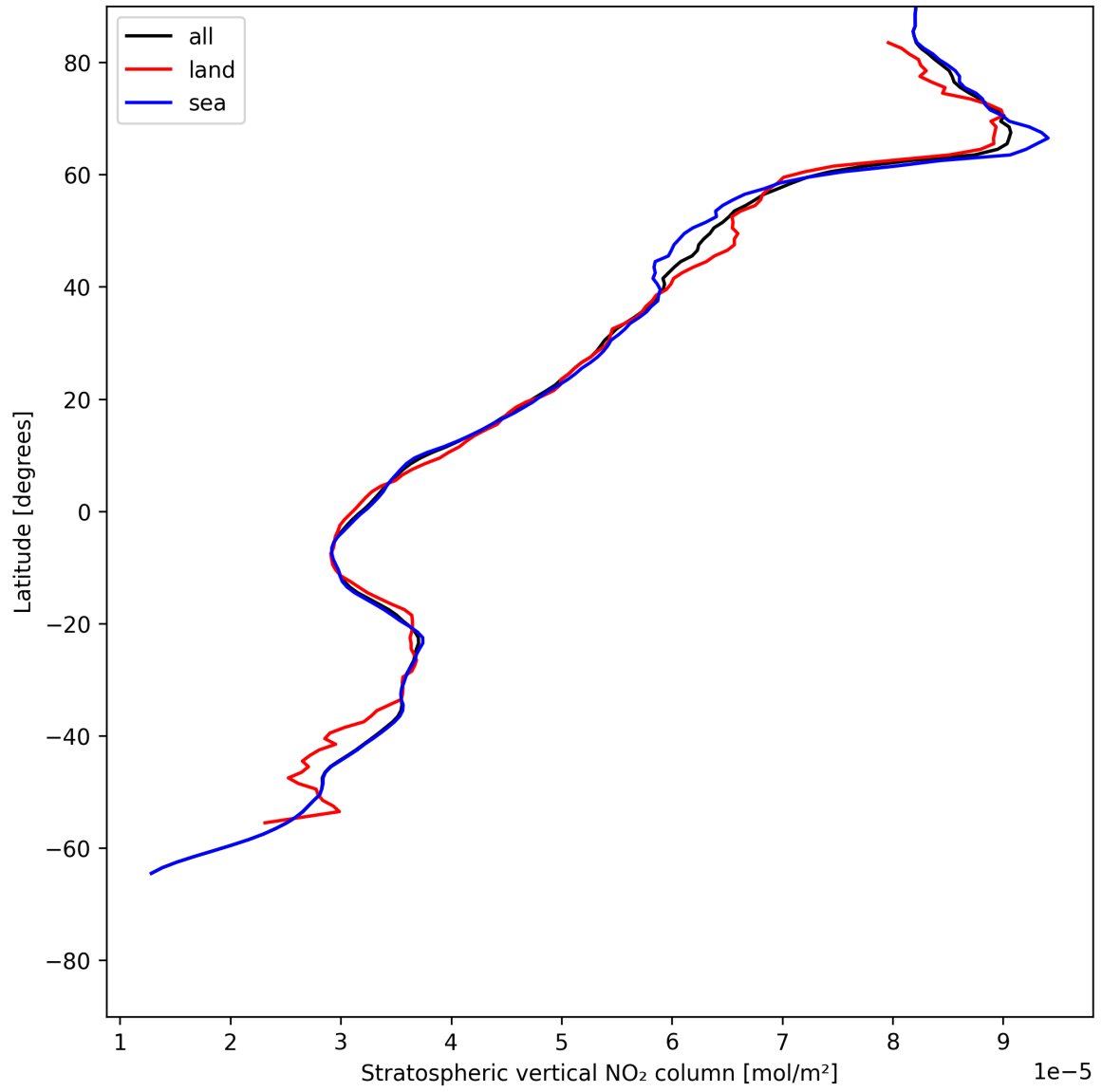
Figure 17: Zonal average of “Stratospheric vertical NO 2 column” for 2025-06-19 to 2025-06-20.
