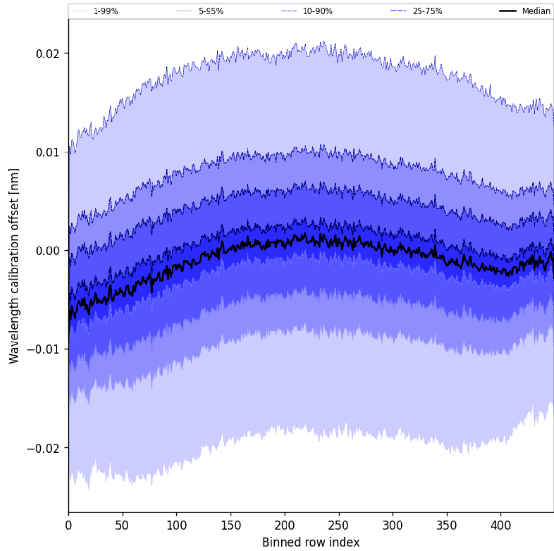
Figure 50: Along track statistics of “Wavelength calibration offset” for 2025-06-19 to 2025-06-20
