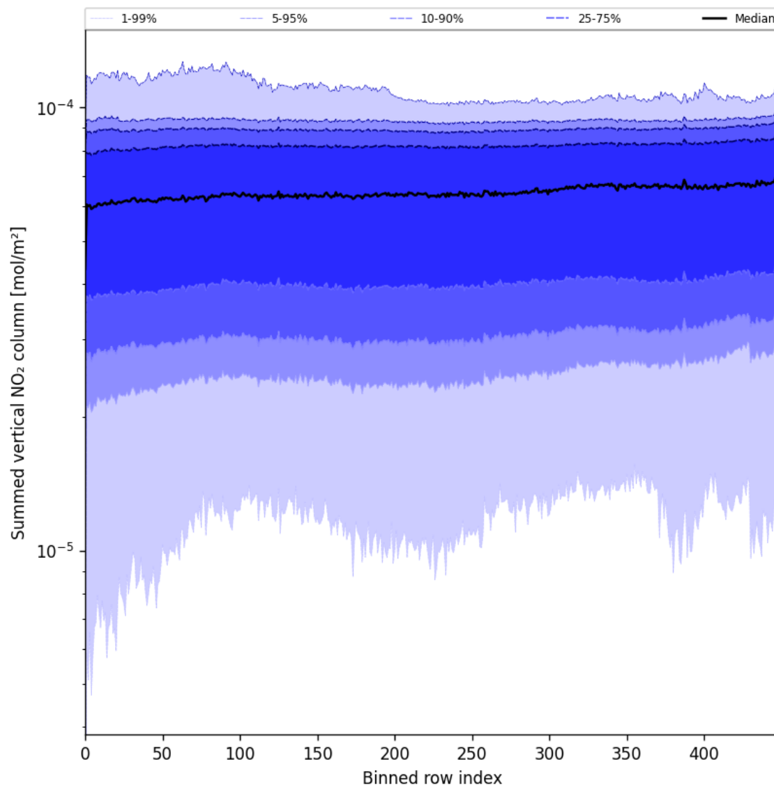
Figure 55: Along track statistics of “Summed vertical NO 2 column” for 2025-06-19 to 2025-06-20
