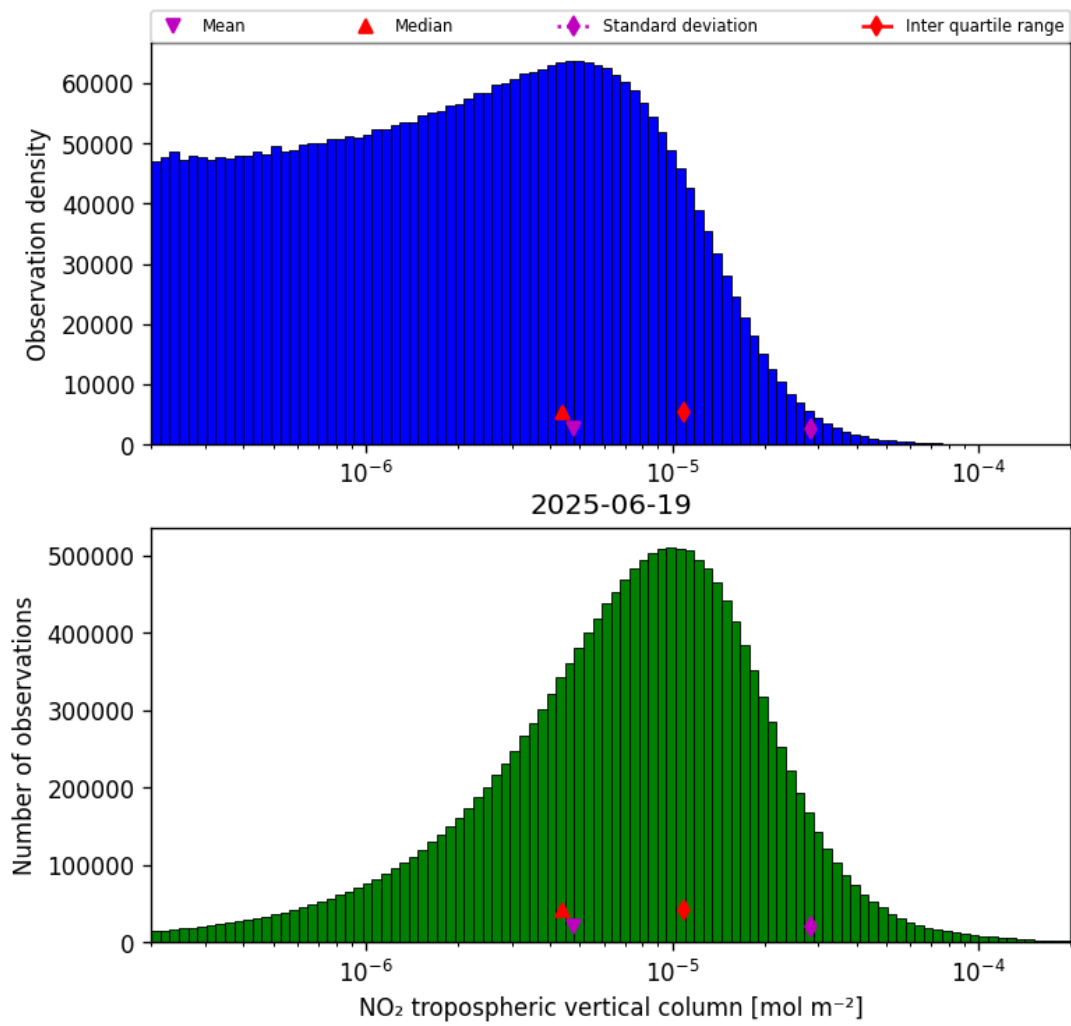
Figure 27: Histogram of “NO 2 tropospheric vertical column” for 2025-06-19 to 2025-06-20
