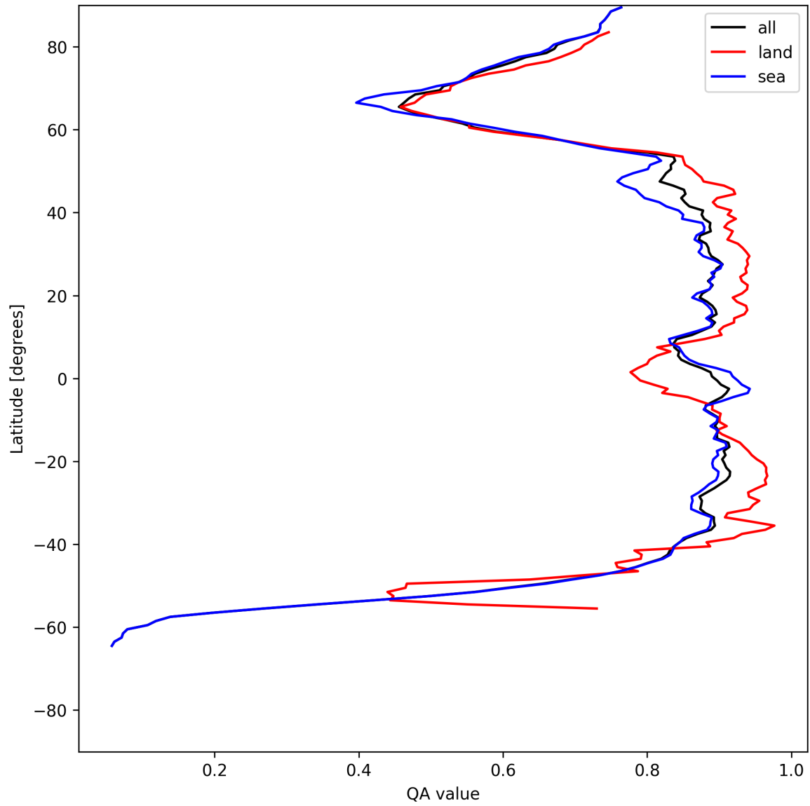
Figure 9: Zonal average of “QA value” for 2025-06-19 to 2025-06-20.
