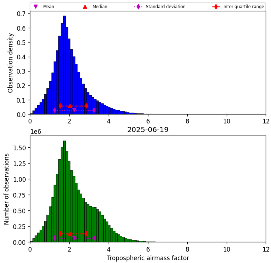
Figure 29: Histogram of “Tropospheric airmass factor” for 2025-06-19 to 2025-06-20
