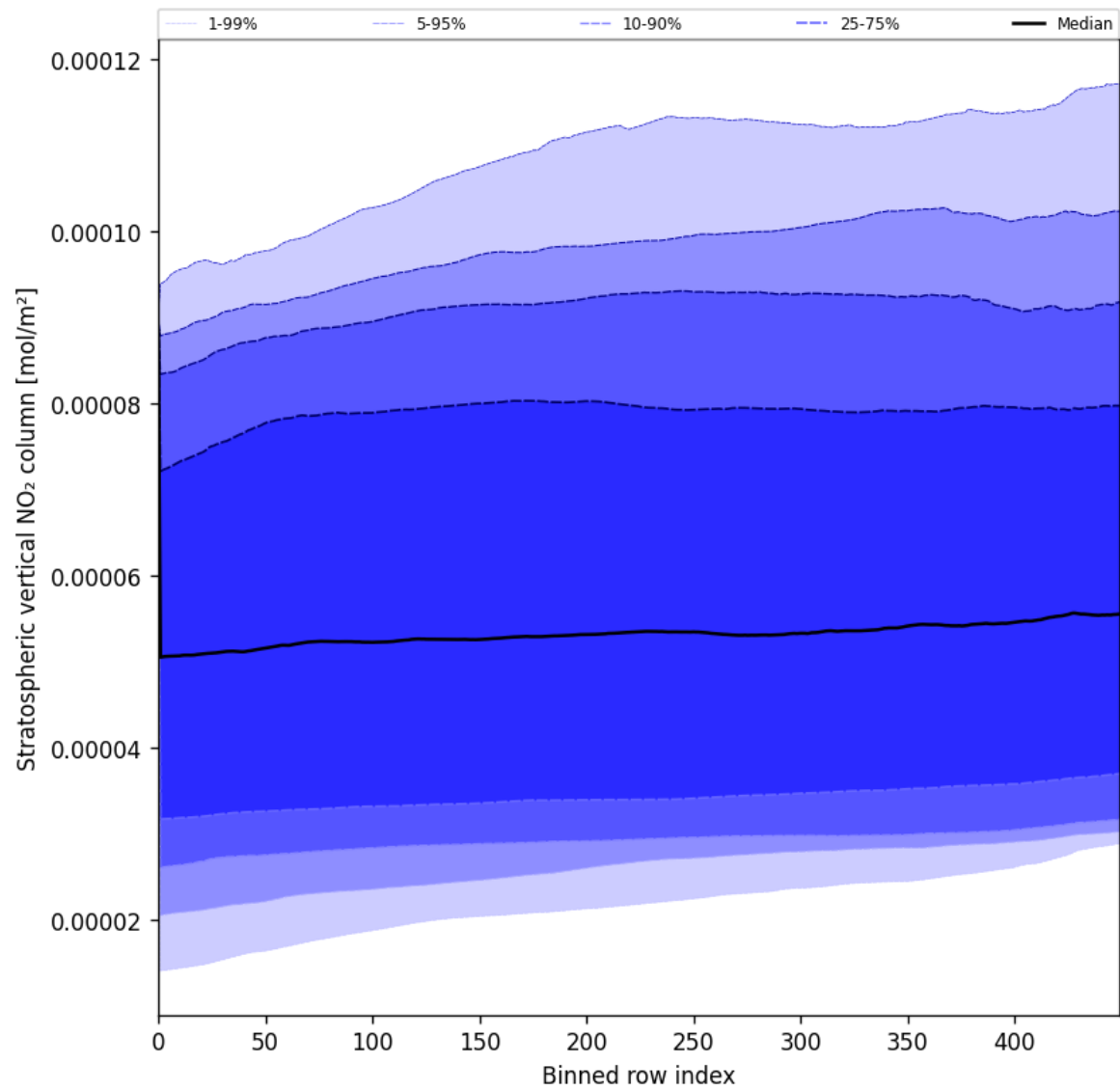
Figure 51: Along track statistics of “Stratospheric vertical NO 2 column” for 2025-06-19 to 2025-06-20
