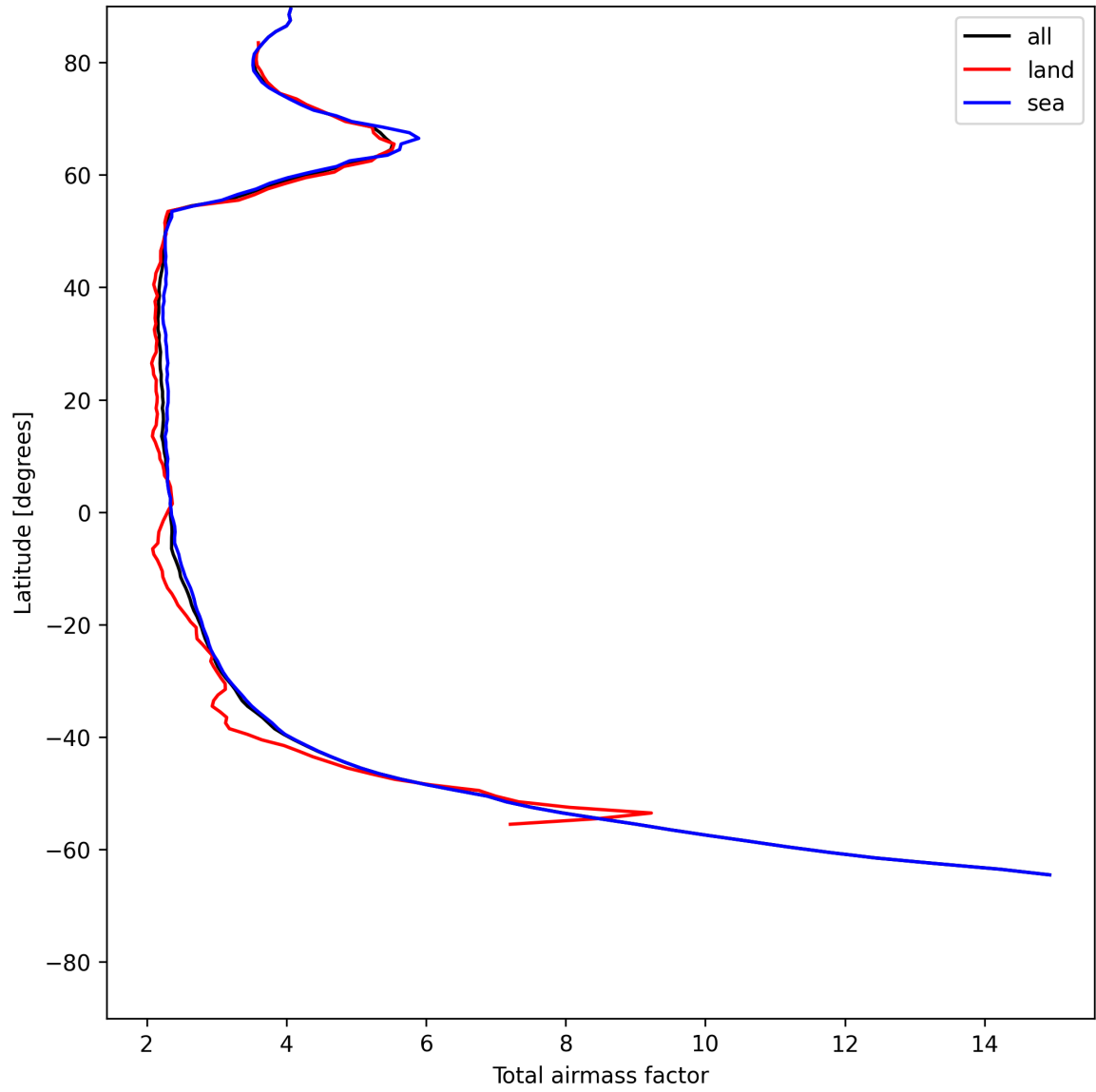
Figure 13: Zonal average of “Total airmass factor” for 2025-06-19 to 2025-06-20.
