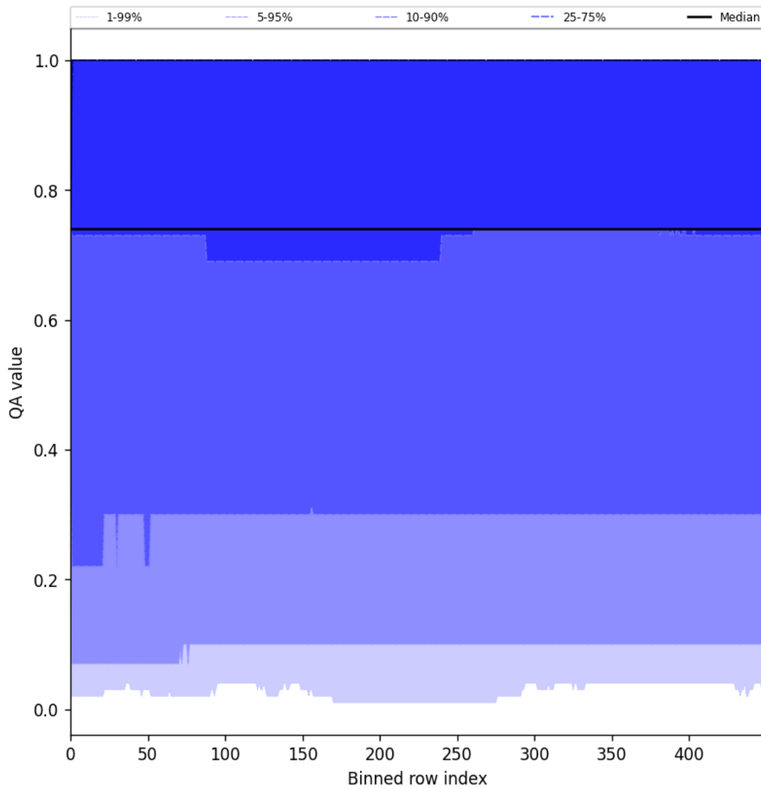
Figure 43: Along track statistics of “QA value” for 2025-06-19 to 2025-06-20
