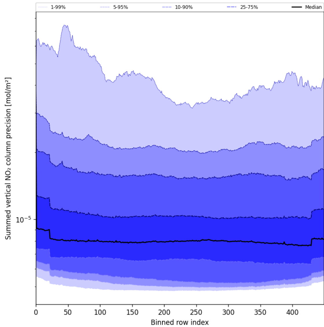
Figure 56: Along track statistics of “Summed vertical NO 2 column precision” for 2025-06-19 to 2025-06-20
