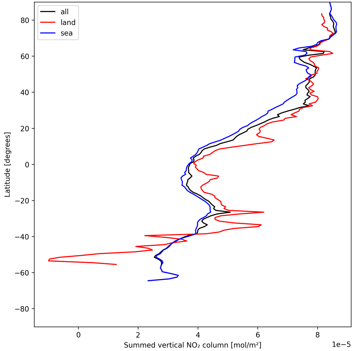
Figure 21: Zonal average of “Summed vertical NO 2 column” for 2025-06-19 to 2025-06-20.
