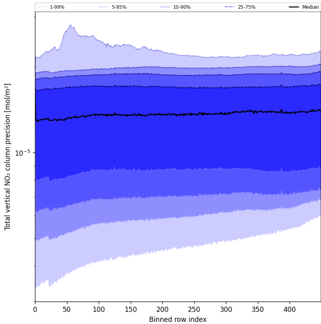
Figure 54: Along track statistics of “Total vertical NO 2 column precision” for 2025-06-19 to 2025-06-20
