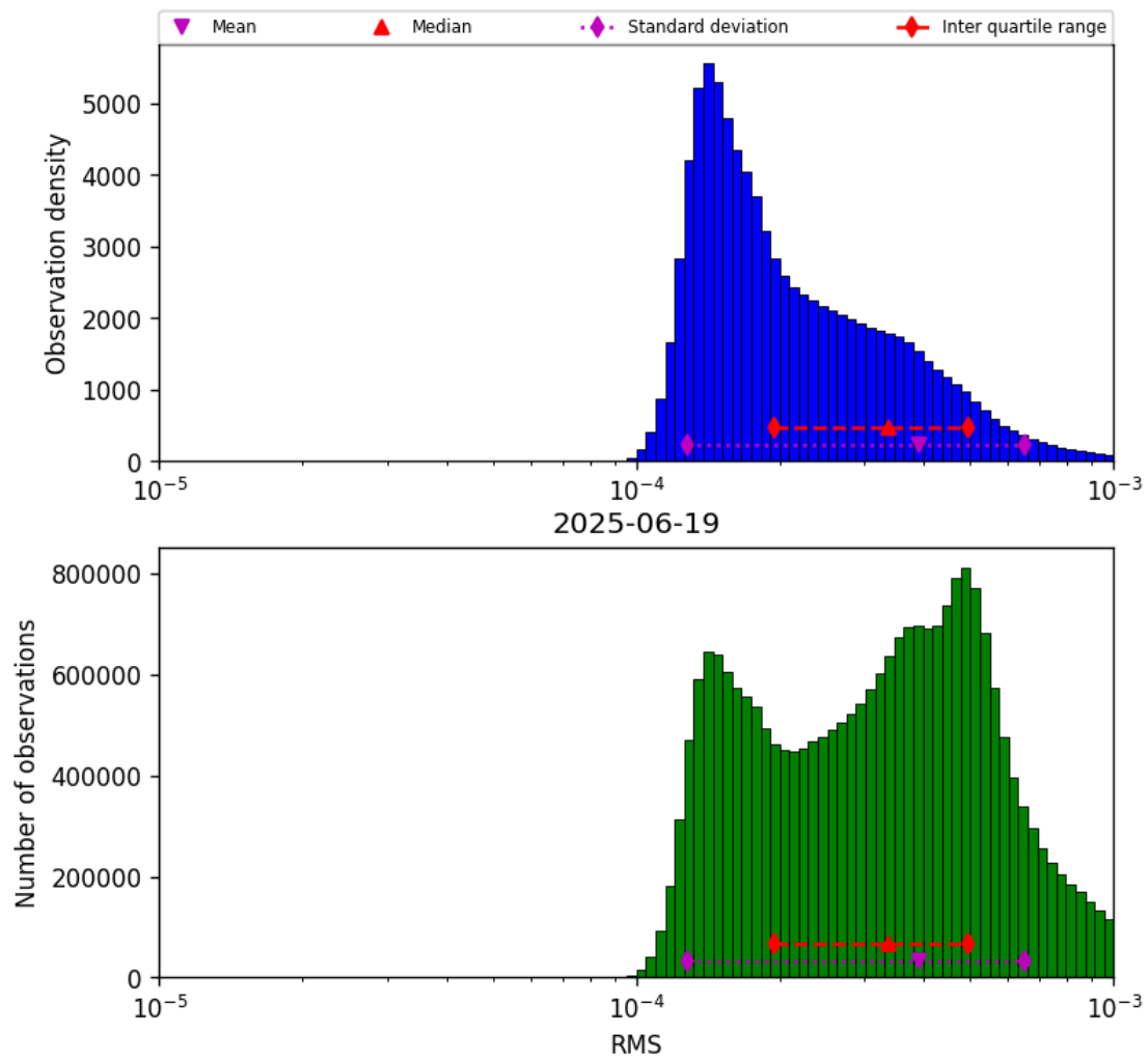
Figure 41: Histogram of “RMS” for 2025-06-19 to 2025-06-20
