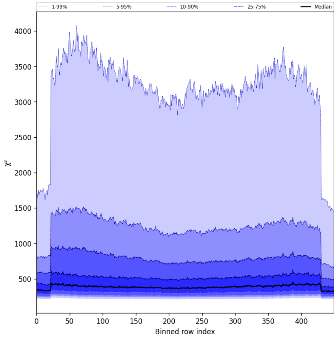
Figure 57: Along track statistics of " \chi^2 " for 2025-06-19 to 2025-06-20
