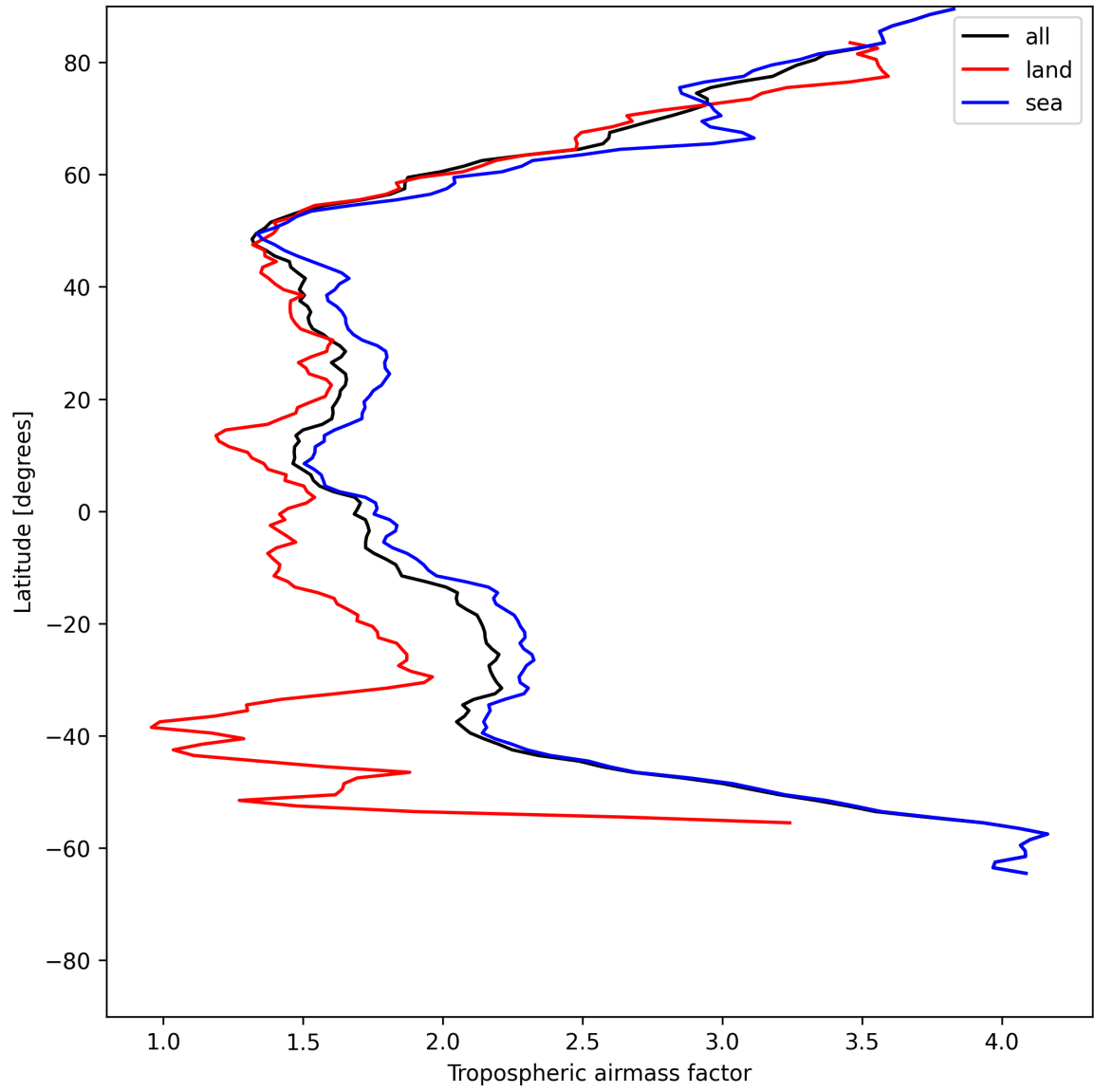
Figure 12: Zonal average of “Tropospheric airmass factor” for 2025-06-19 to 2025-06-20.
