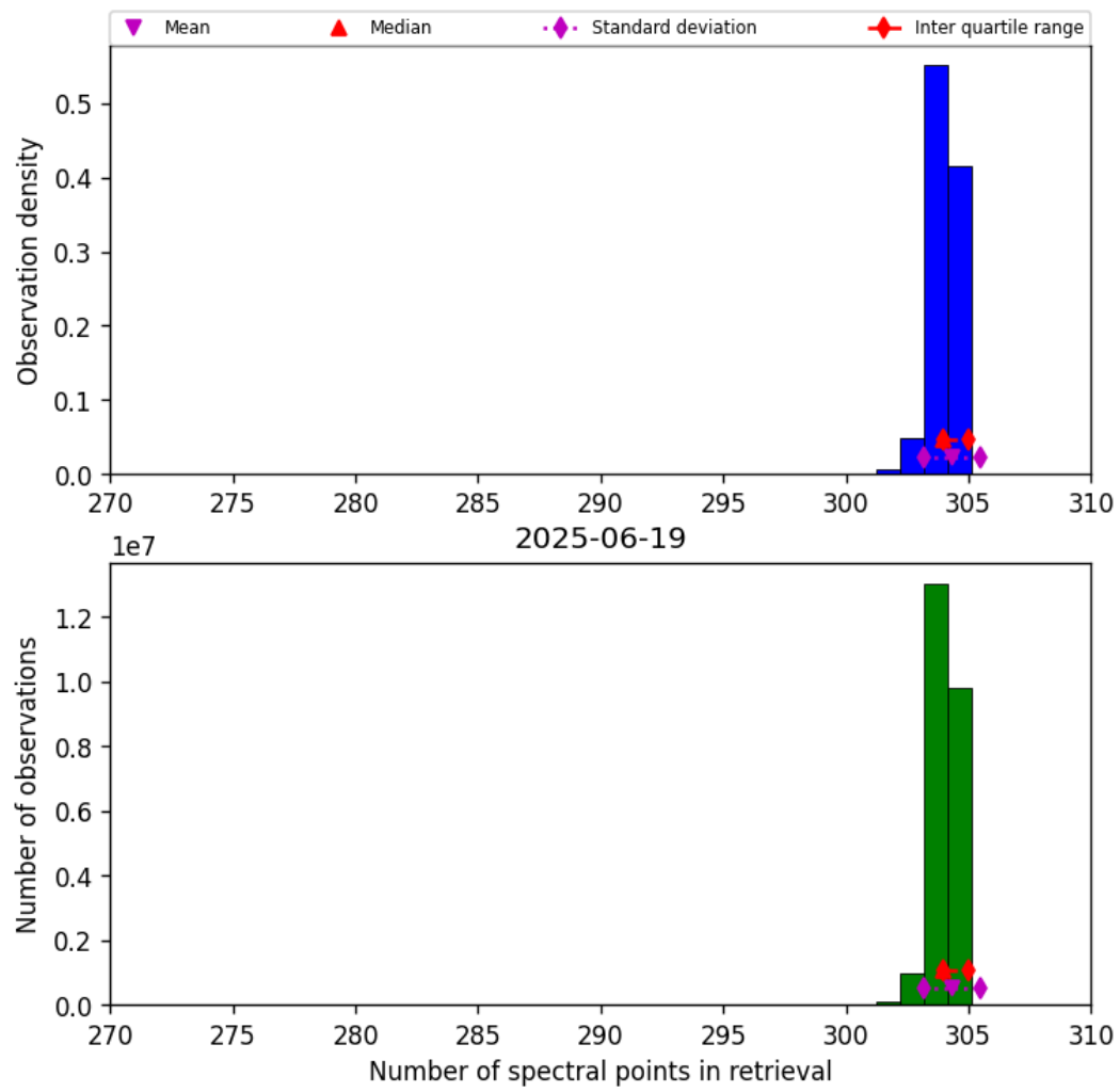
Figure 31: Histogram of “Number of spectral points in retrieval” for 2025-06-19 to 2025-06-20
