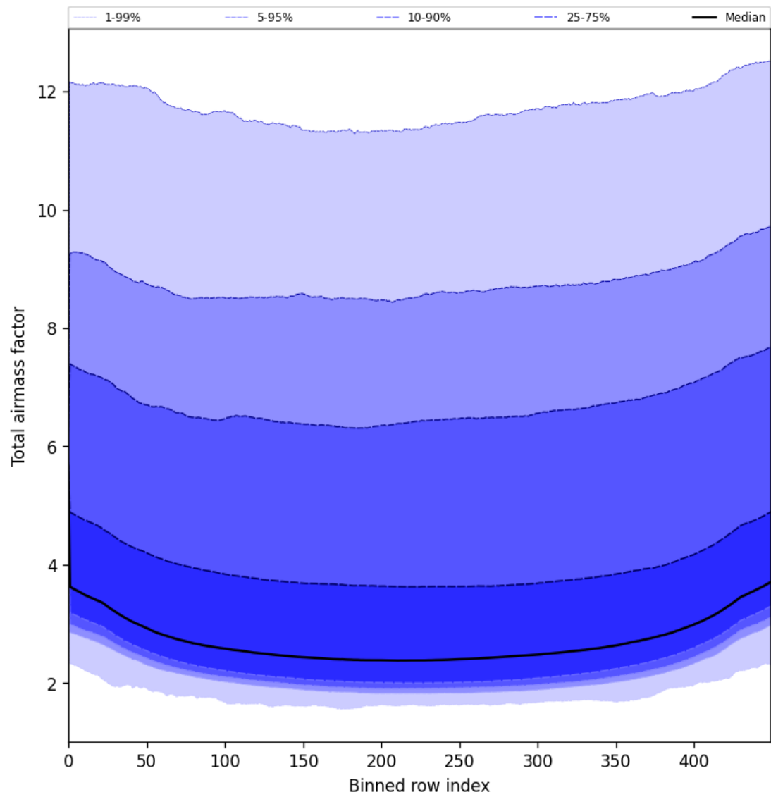
Figure 47: Along track statistics of “Total airmass factor” for 2025-06-19 to 2025-06-20
