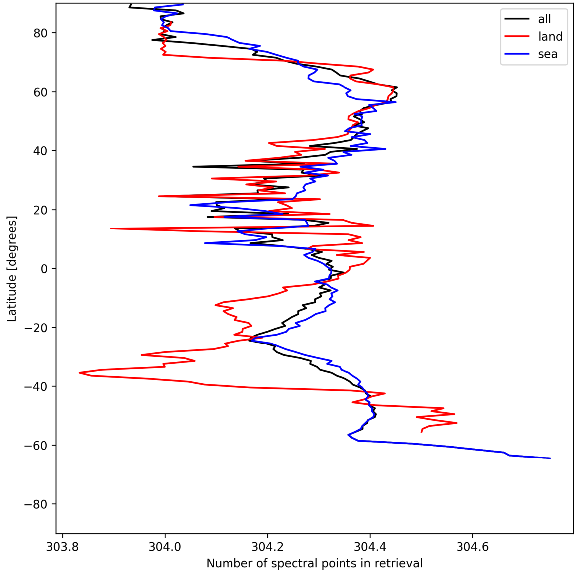
Figure 14: Zonal average of “Number of spectral points in retrieval” for 2025-06-19 to 2025-06-20.
