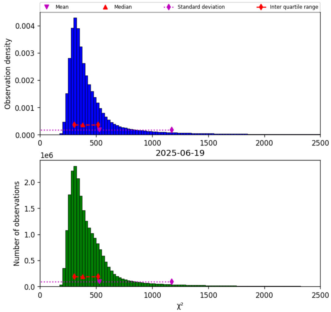
Figure 40: Histogram of “ \chi^2 ” for 2025-06-19 to 2025-06-20
