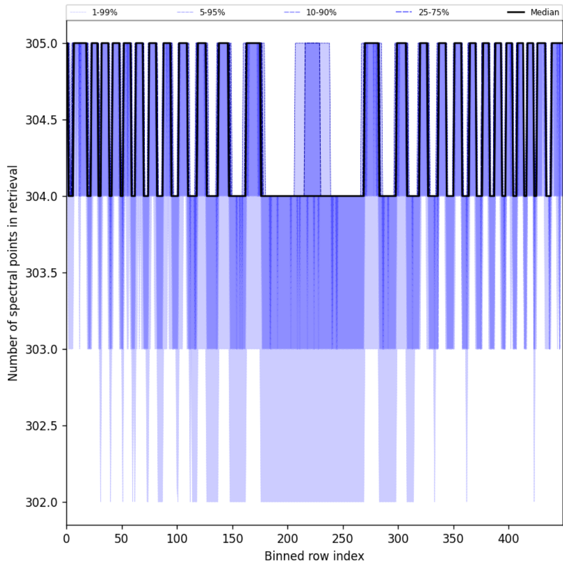
Figure 48: Along track statistics of “Number of spectral points in retrieval” for 2025-06-19 to 2025-06-20
