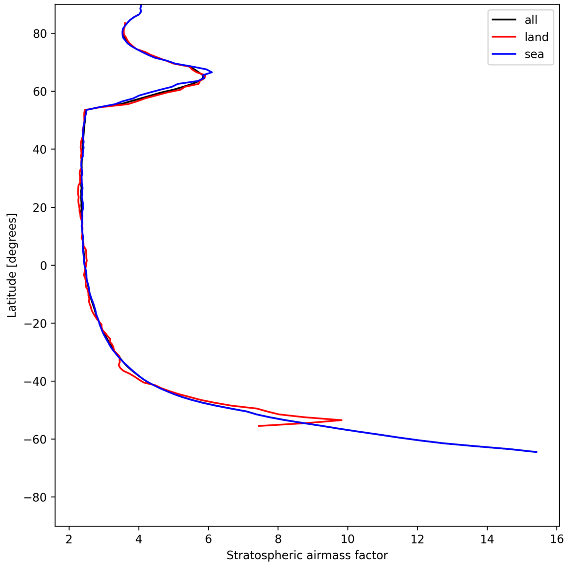
Figure 25: Zonal average of “Stratospheric airmass factor” for 2025-06-19 to 2025-06-20.
