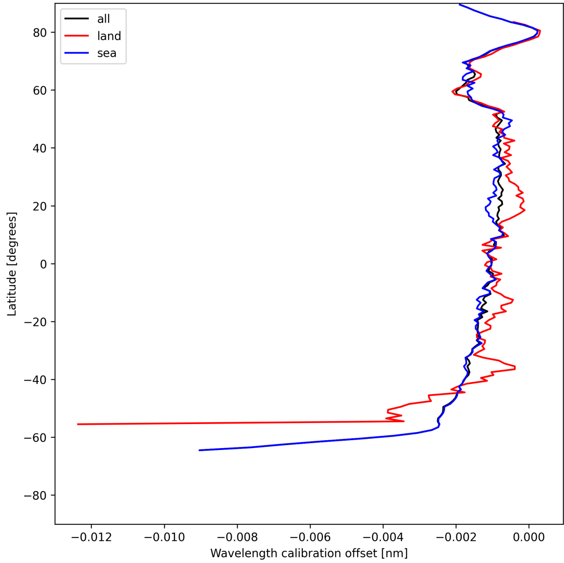
Figure 16: Zonal average of “Wavelength calibration offset” for 2025-06-19 to 2025-06-20.
