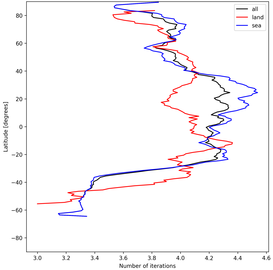
Figure 15: Zonal average of “Number of iterations” for 2025-06-19 to 2025-06-20.
