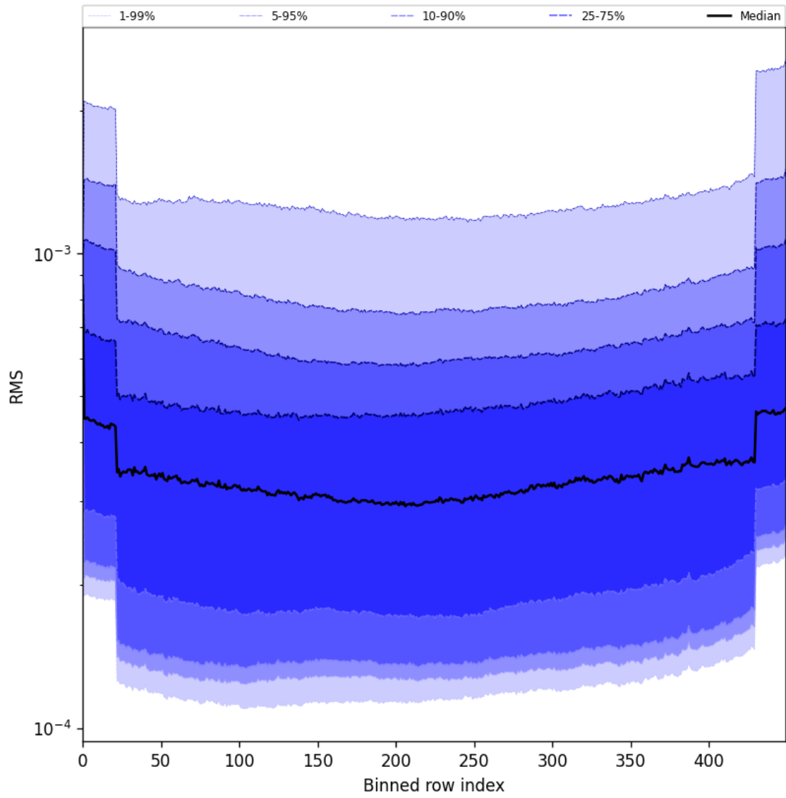
Figure 58: Along track statistics of “RMS” for 2025-06-19 to 2025-06-20
