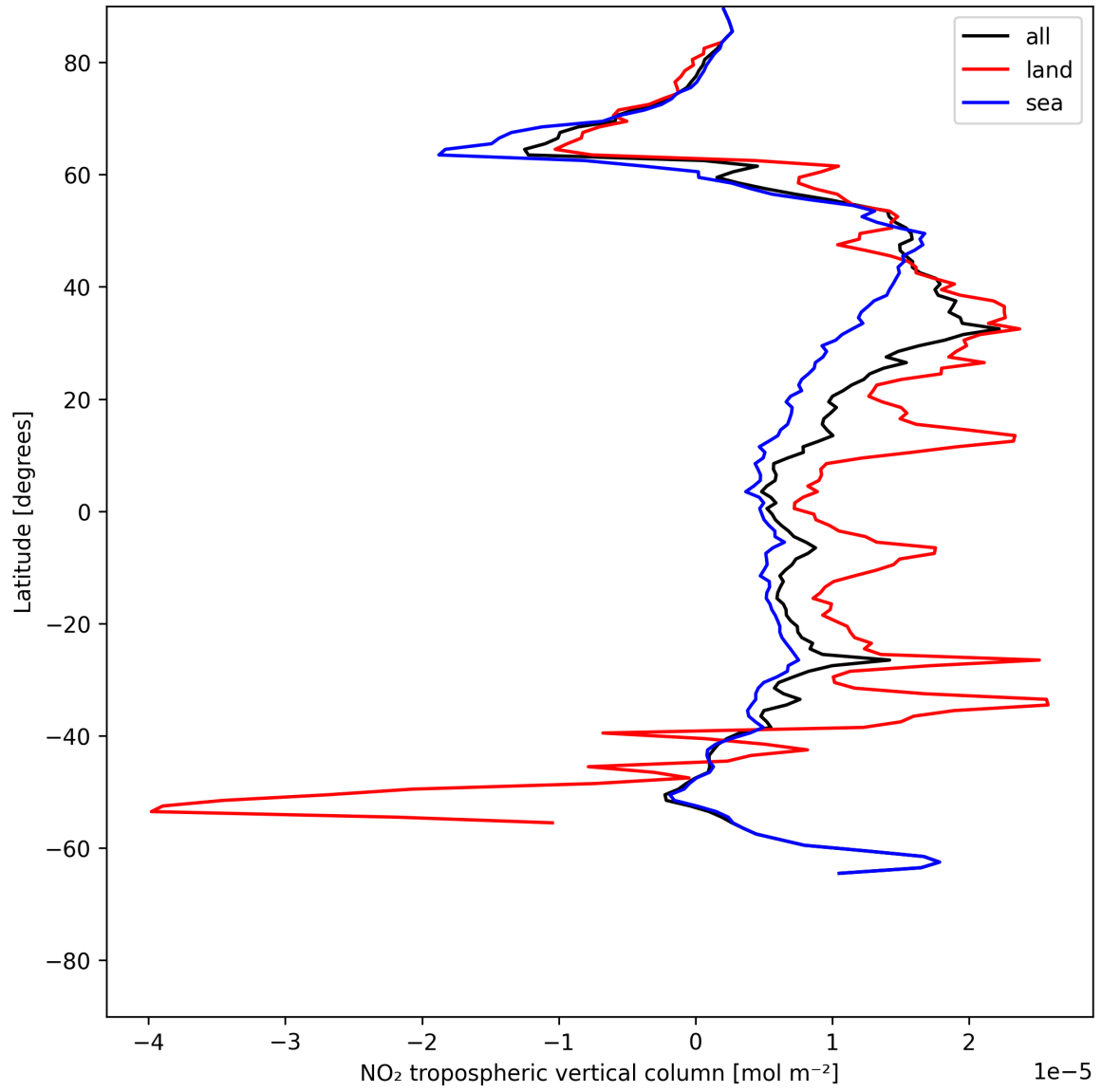
Figure 10: Zonal average of “NO 2 tropospheric vertical column” for 2025-06-19 to 2025-06-20.
