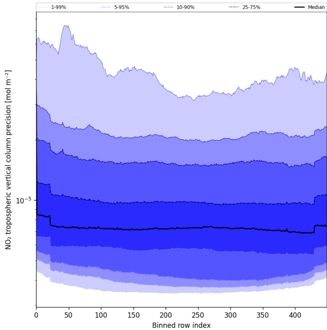
Figure 45: Along track statistics of “NO 2 tropospheric vertical column precision” for 2025-06-19 to 2025-06-20
