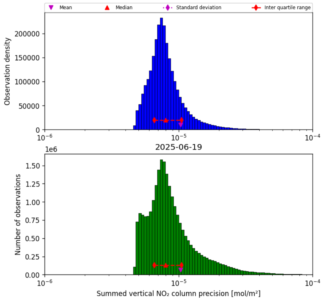
Figure 39: Histogram of “Summed vertical NO 2 column precision” for 2025-06-19 to 2025-06-20
