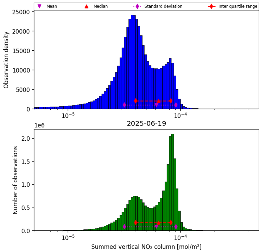
Figure 38: Histogram of “Summed vertical NO 2 column” for 2025-06-19 to 2025-06-20
