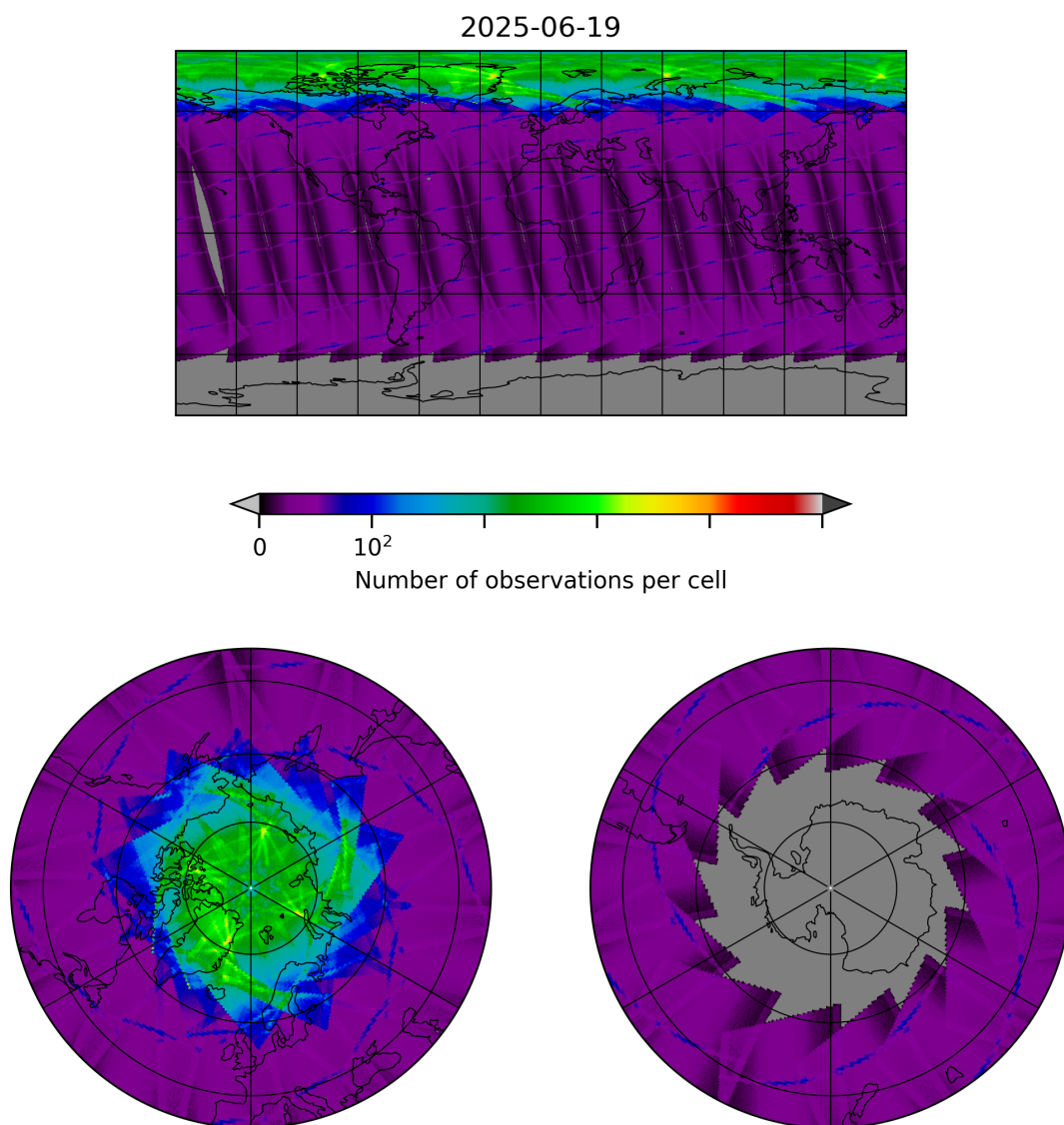
Figure 8: Map of the number of observations for 2025-06-19 to 2025-06-20
