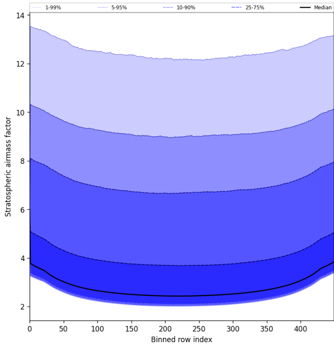
Figure 59: Along track statistics of “Stratospheric airmass factor” for 2025-06-19 to 2025-06-20
