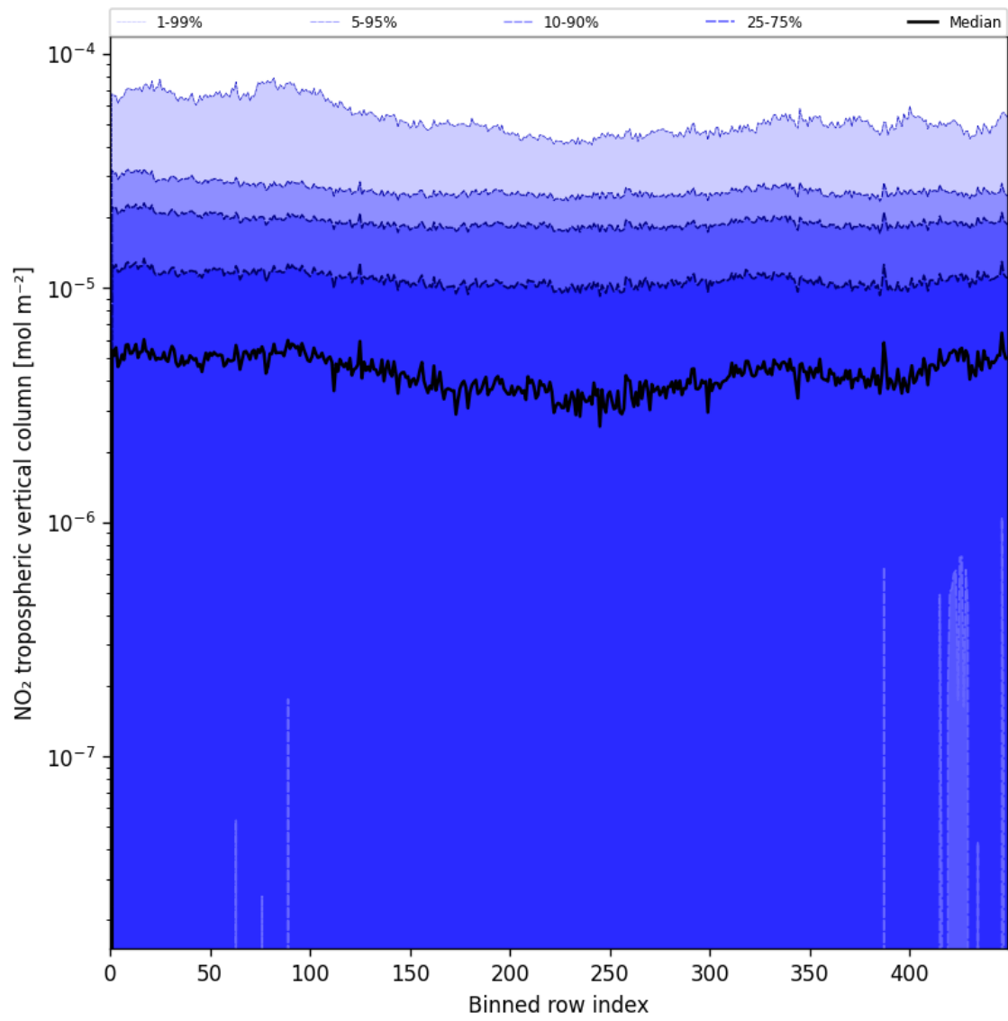
Figure 44: Along track statistics of “NO 2 tropospheric vertical column” for 2025-06-19 to 2025-06-20
