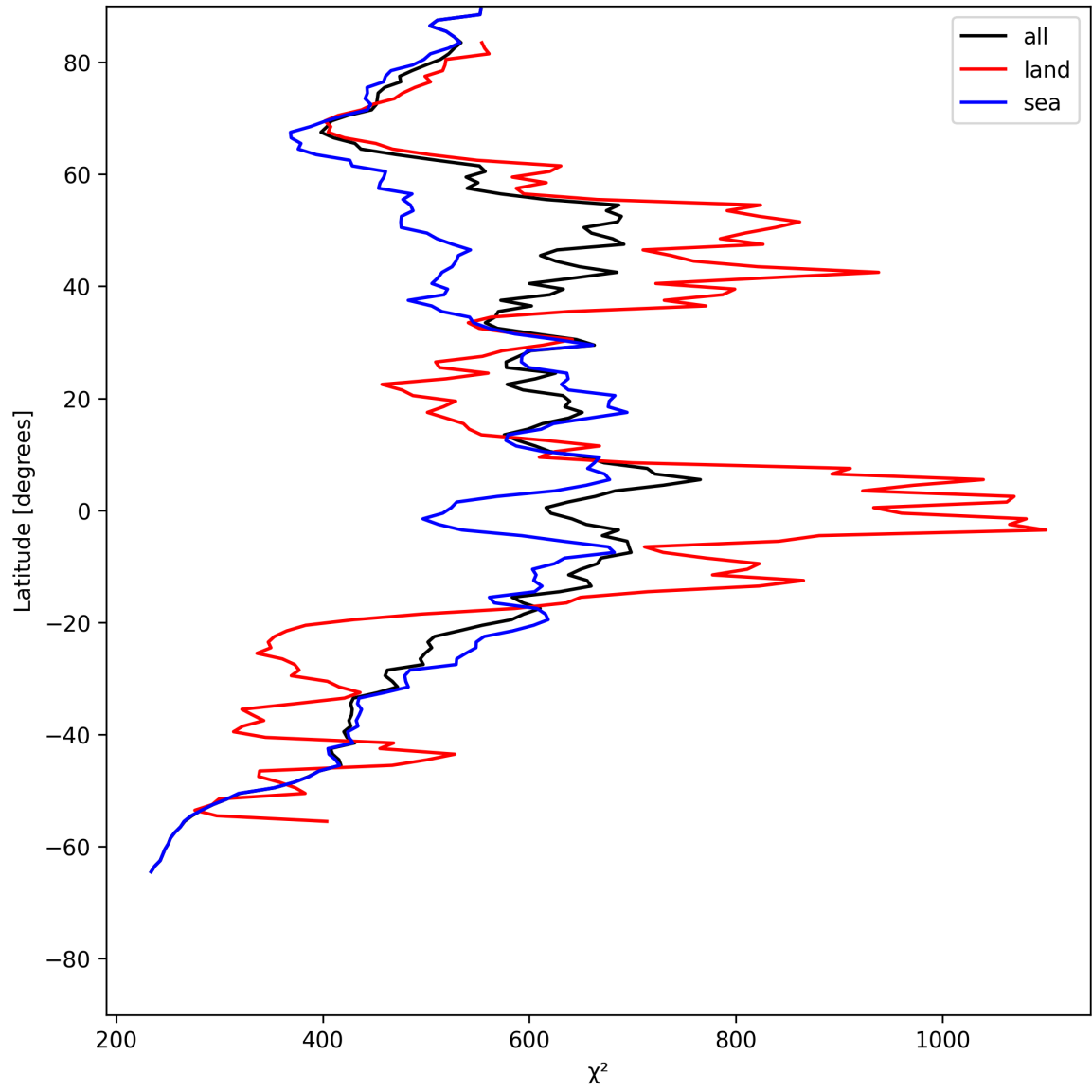
Figure 23: Zonal average of “ \chi^2 ” for 2025-06-19 to 2025-06-20.
