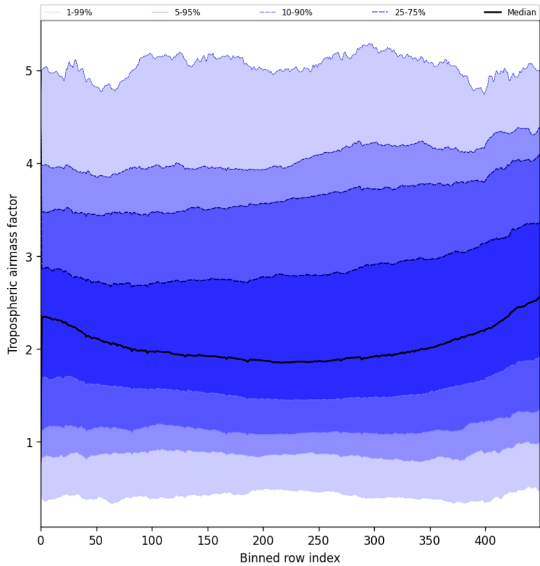
Figure 46: Along track statistics of “Tropospheric air mass factor” for 2025-06-19 to 2025-06-20
