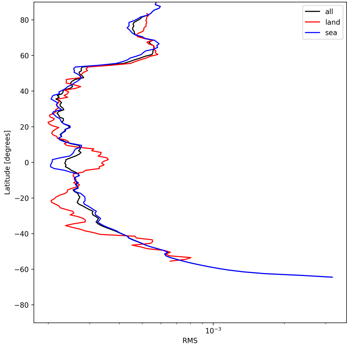
Figure 24: Zonal average of “RMS” for 2025-06-19 to 2025-06-20.
