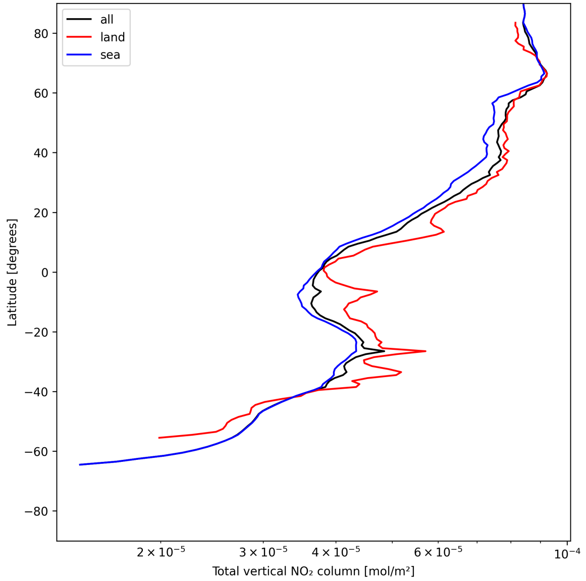
Figure 19: Zonal average of “Total vertical NO 2 column” for 2025-06-19 to 2025-06-20.
