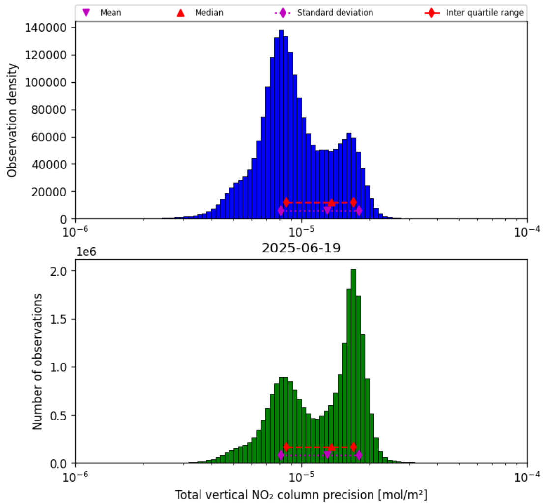
Figure 37: Histogram of “Total vertical NO 2 column precision” for 2025-06-19 to 2025-06-20
