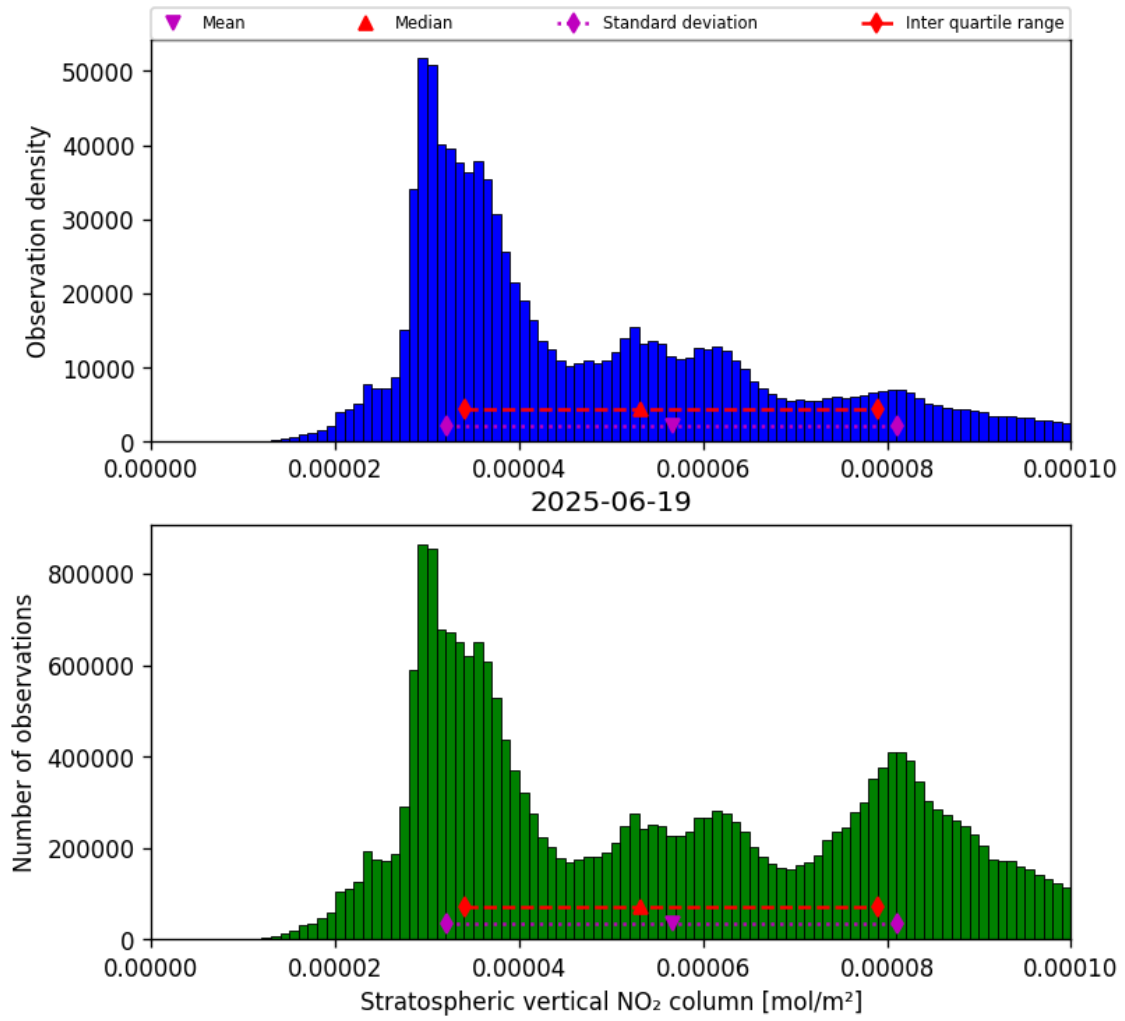
Figure 34: Histogram of “Stratospheric vertical NO 2 column” for 2025-06-19 to 2025-06-20
