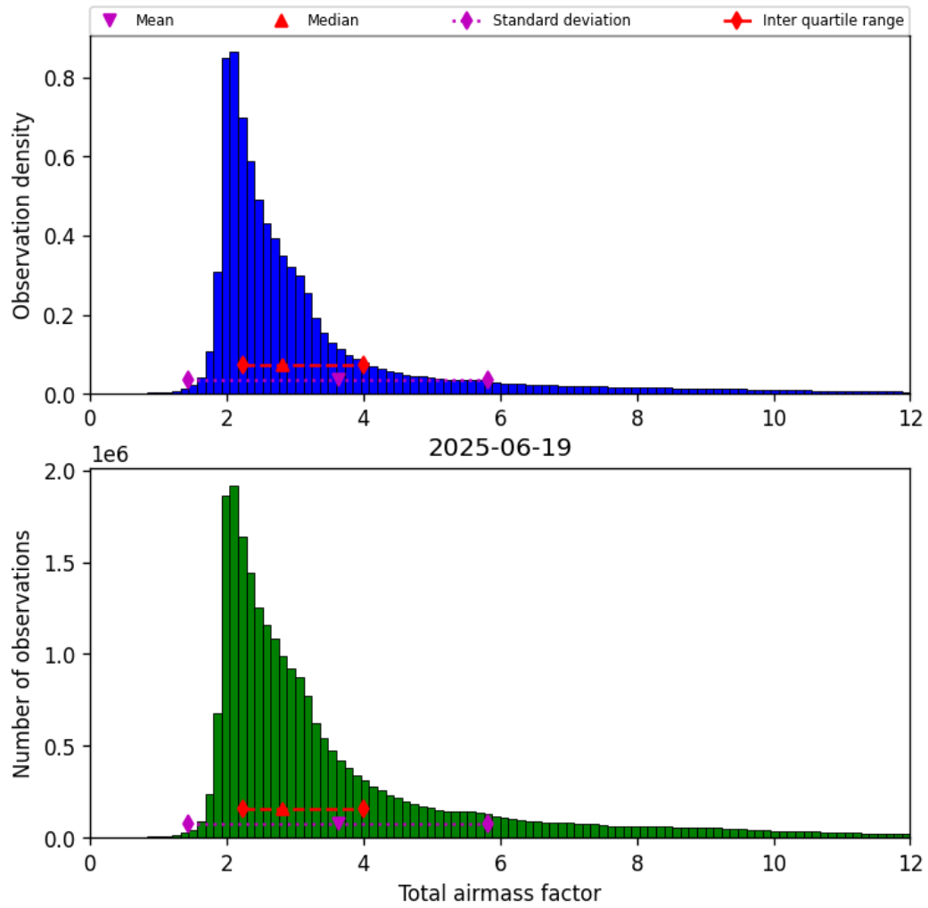
Figure 30: Histogram of “Total airmass factor” for 2025-06-19 to 2025-06-20
