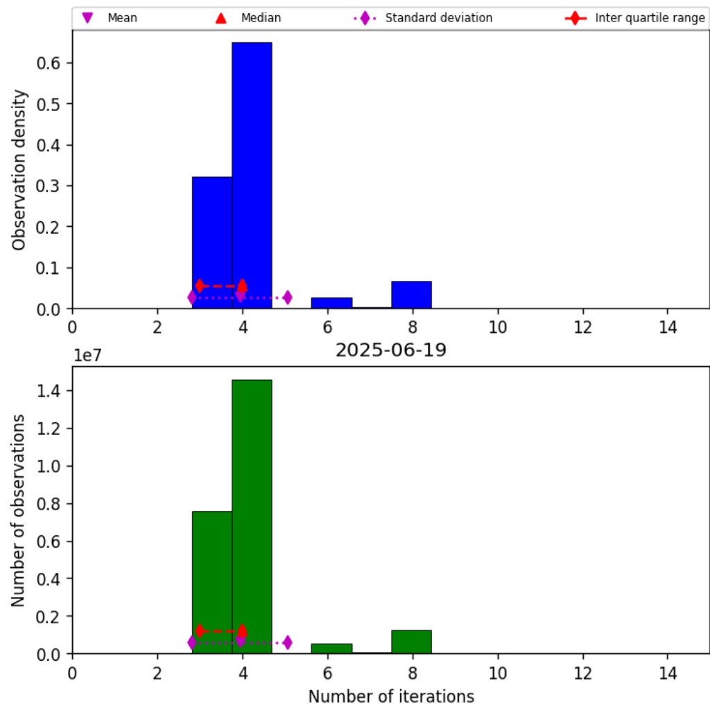
Figure 32: Histogram of “Number of iterations” for 2025-06-19 to 2025-06-20
