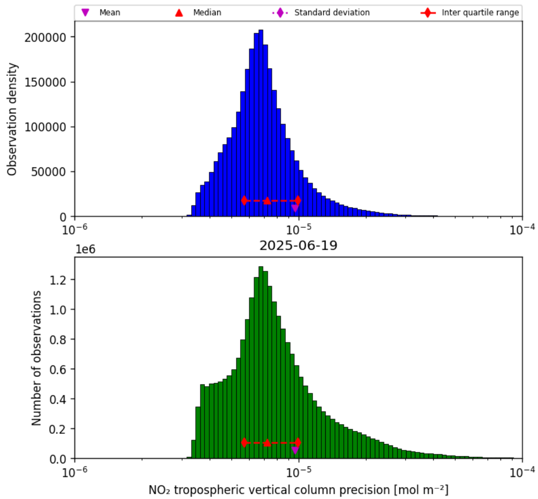
Figure 28: Histogram of “NO 2 tropospheric vertical column precision” for 2025-06-19 to 2025-06-20
