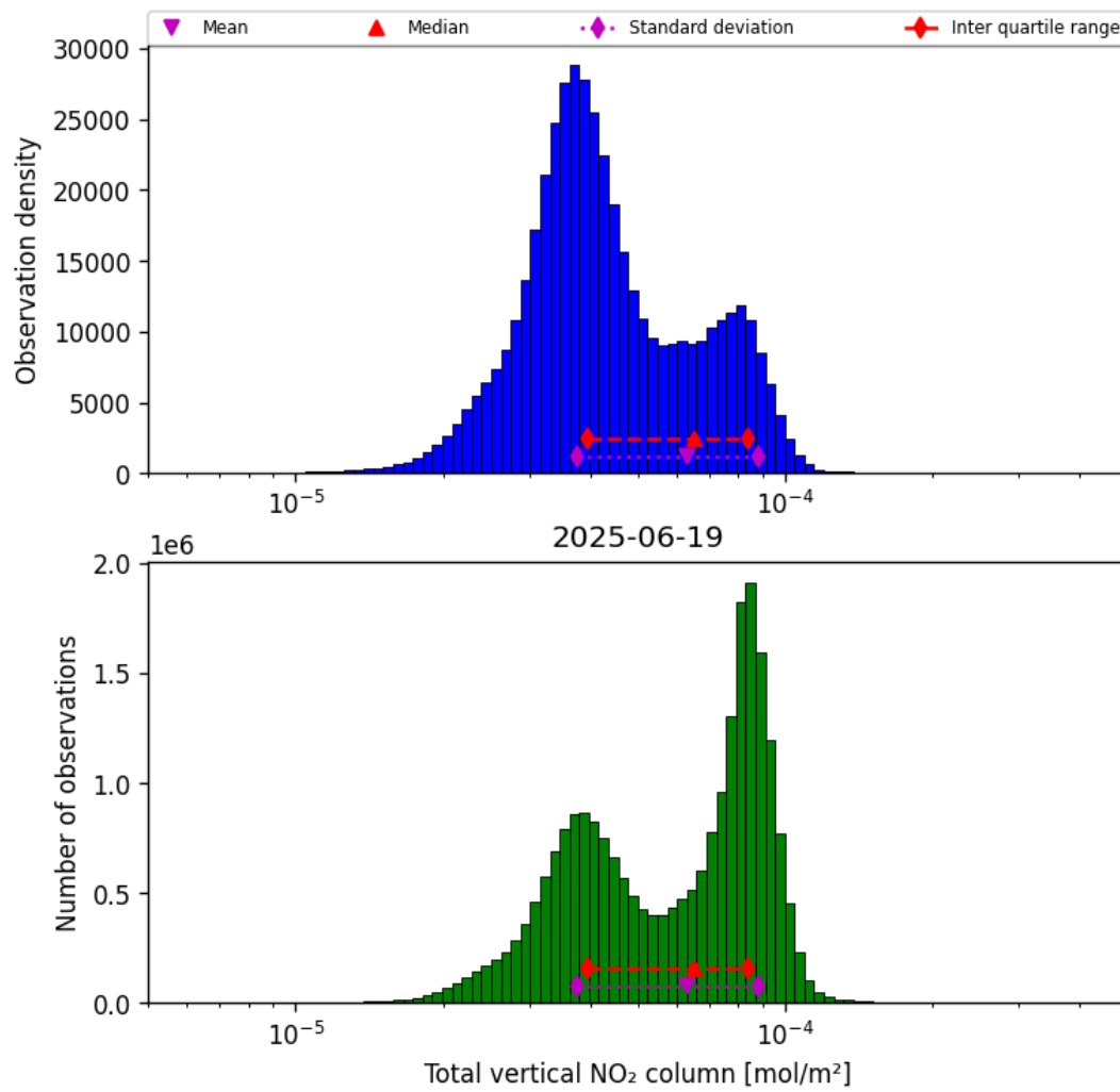
Figure 36: Histogram of “Total vertical NO 2 column” for 2025-06-19 to 2025-06-20
