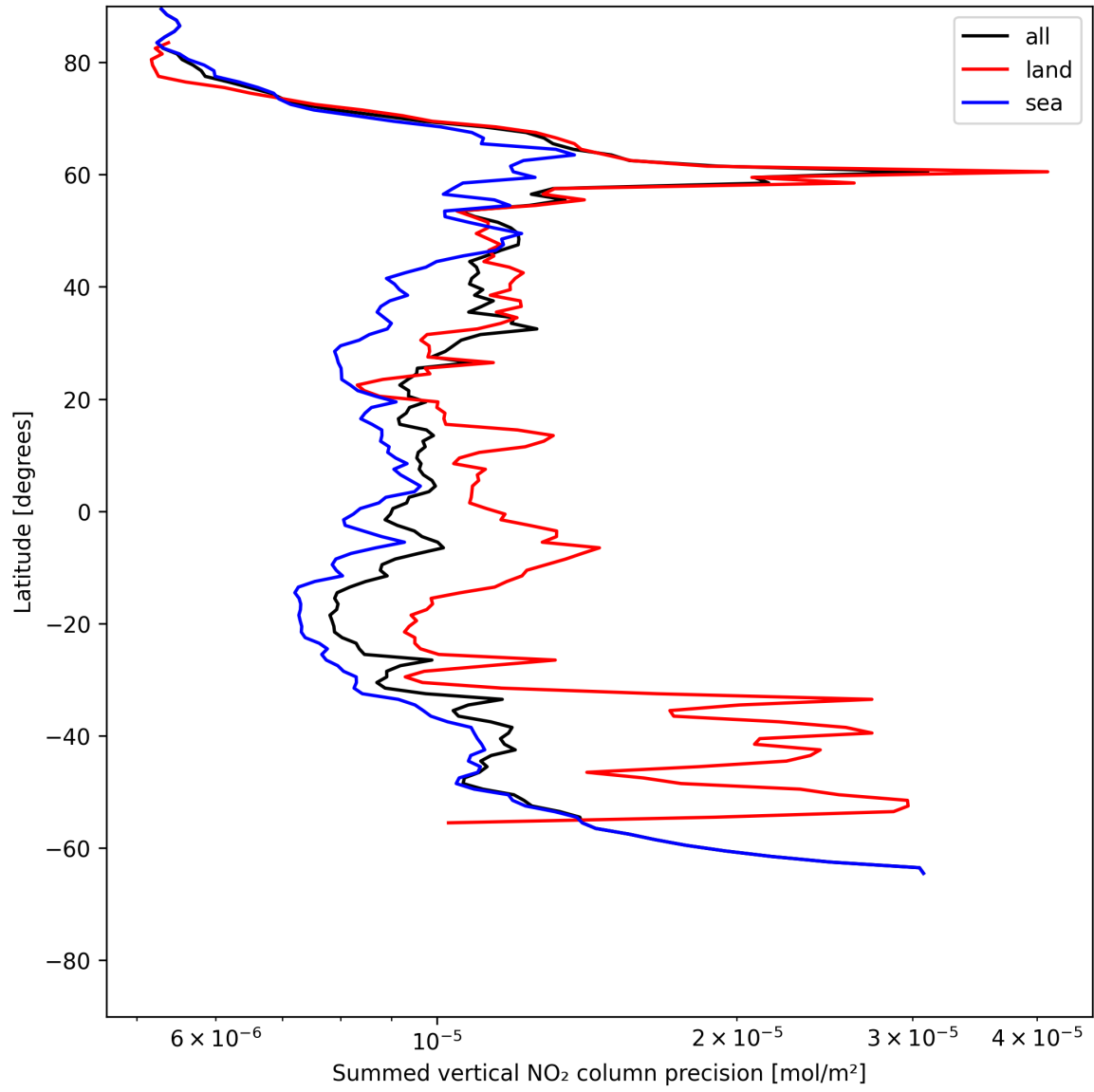
Figure 22: Zonal average of “Summed vertical NO 2 column precision” for 2025-06-19 to 2025-06-20.
