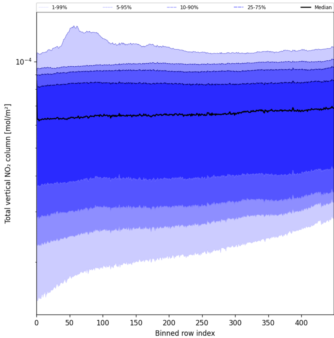
Figure 53: Along track statistics of “Total vertical NO 2 column” for 2025-06-19 to 2025-06-20
