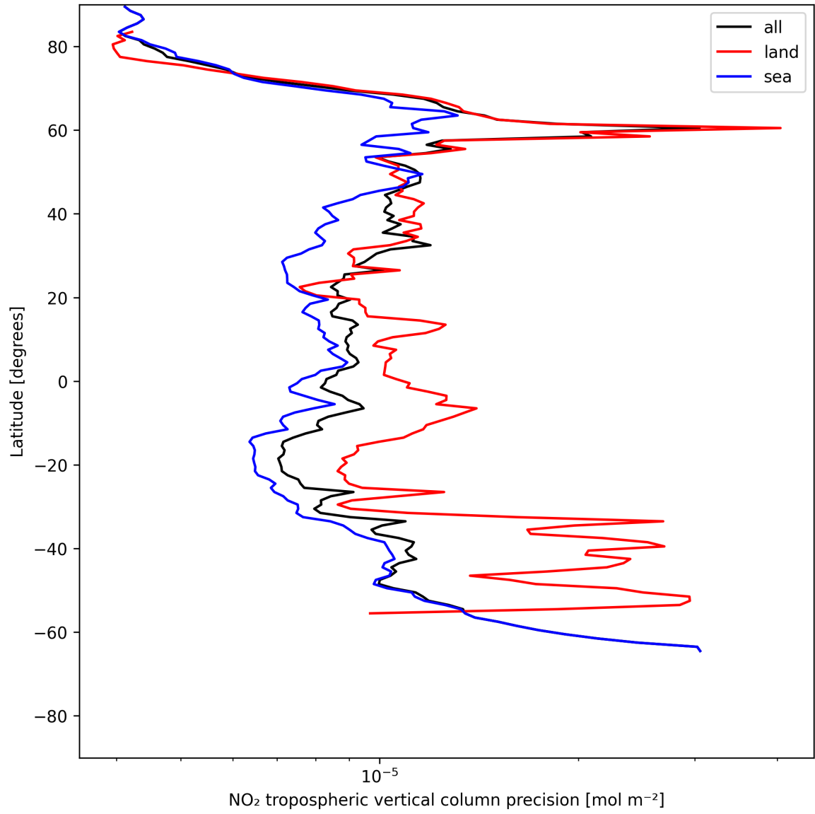
Figure 11: Zonal average of “NO 2 tropospheric vertical column precision” for 2025-06-19 to 2025-06-20.
