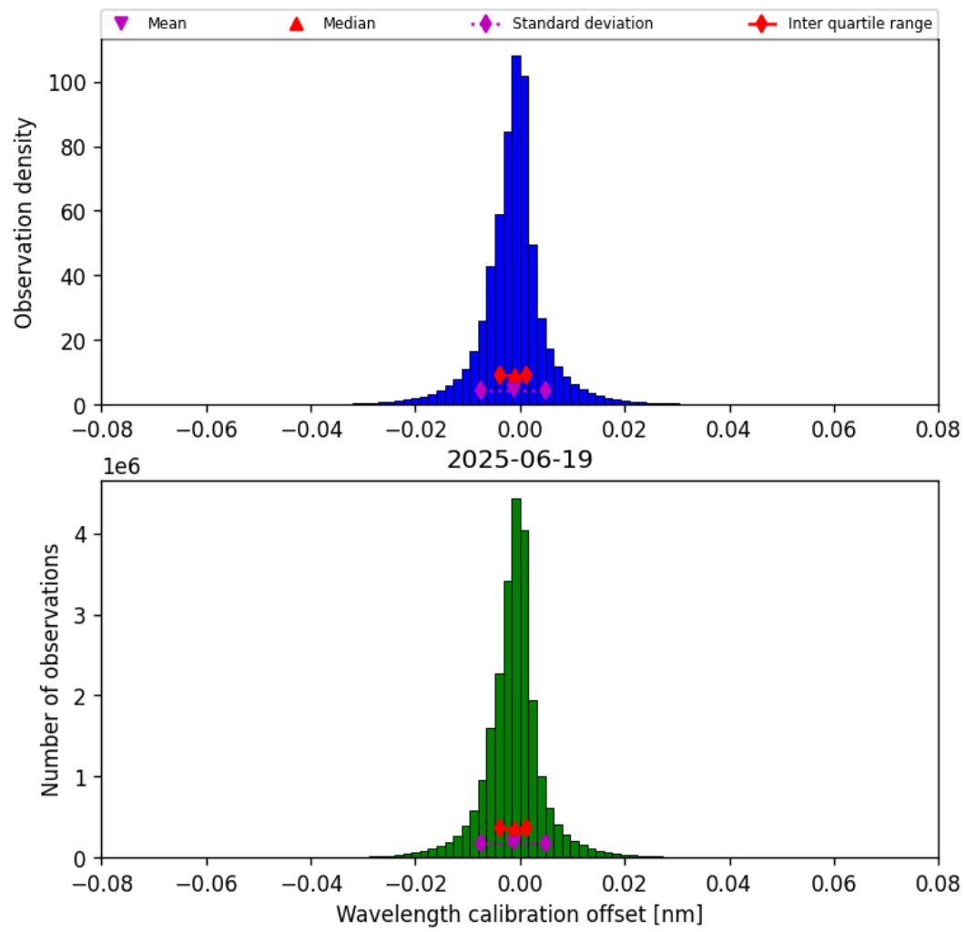
Figure 33: Histogram of “Wavelength calibration offset” for 2025-06-19 to 2025-06-20
