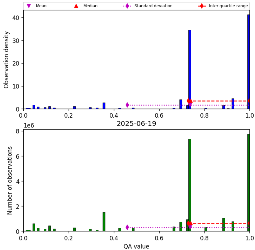
Figure 26: Histogram of “QA value” for 2025-06-19 to 2025-06-20
