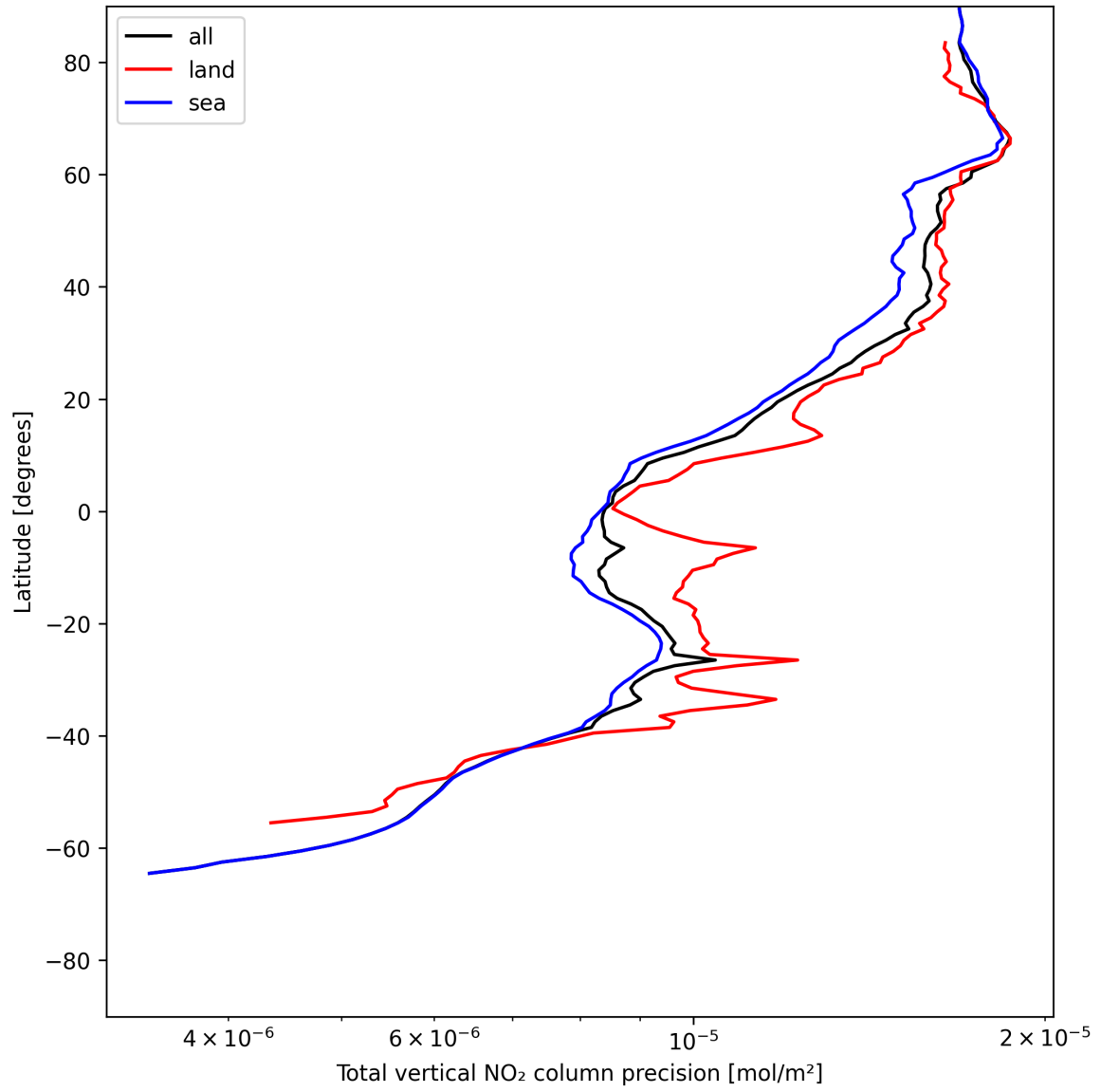
Figure 20: Zonal average of “Total vertical NO 2 column precision” for 2025-06-19 to 2025-06-20.
