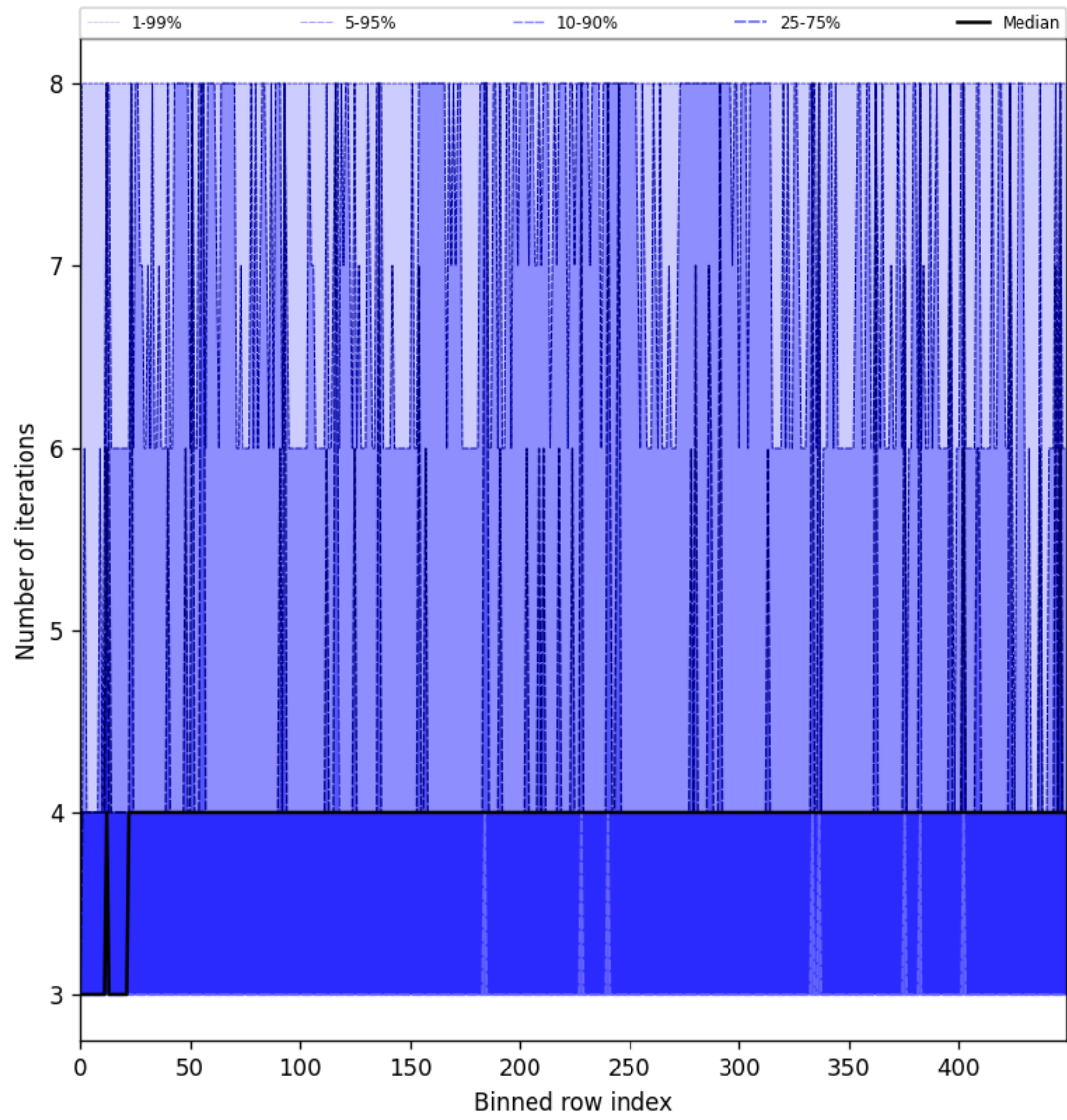
Figure 49: Along track statistics of “Number of iterations” for 2025-06-19 to 2025-06-20
