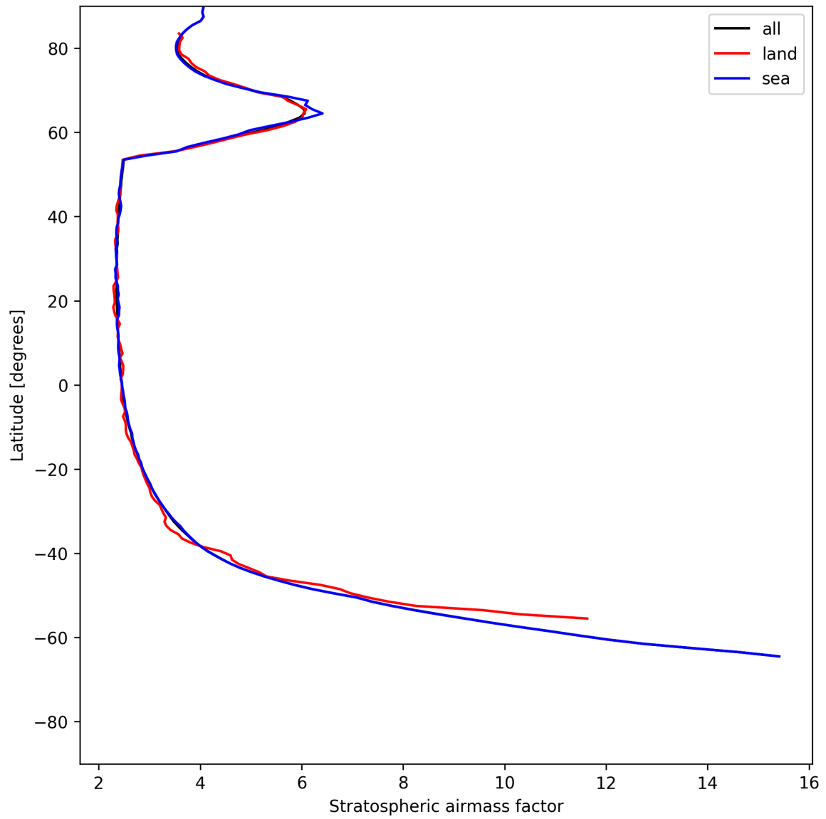
Figure 25: Zonal average of “Stratospheric airmass factor” for 2025-06-20 to 2025-06-20.
