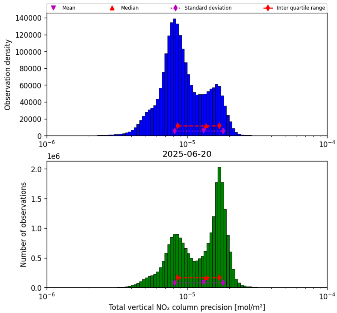
Figure 37: Histogram of "Total vertical NO 2 column precision" for 2025-06-20 to 2025-06-20
