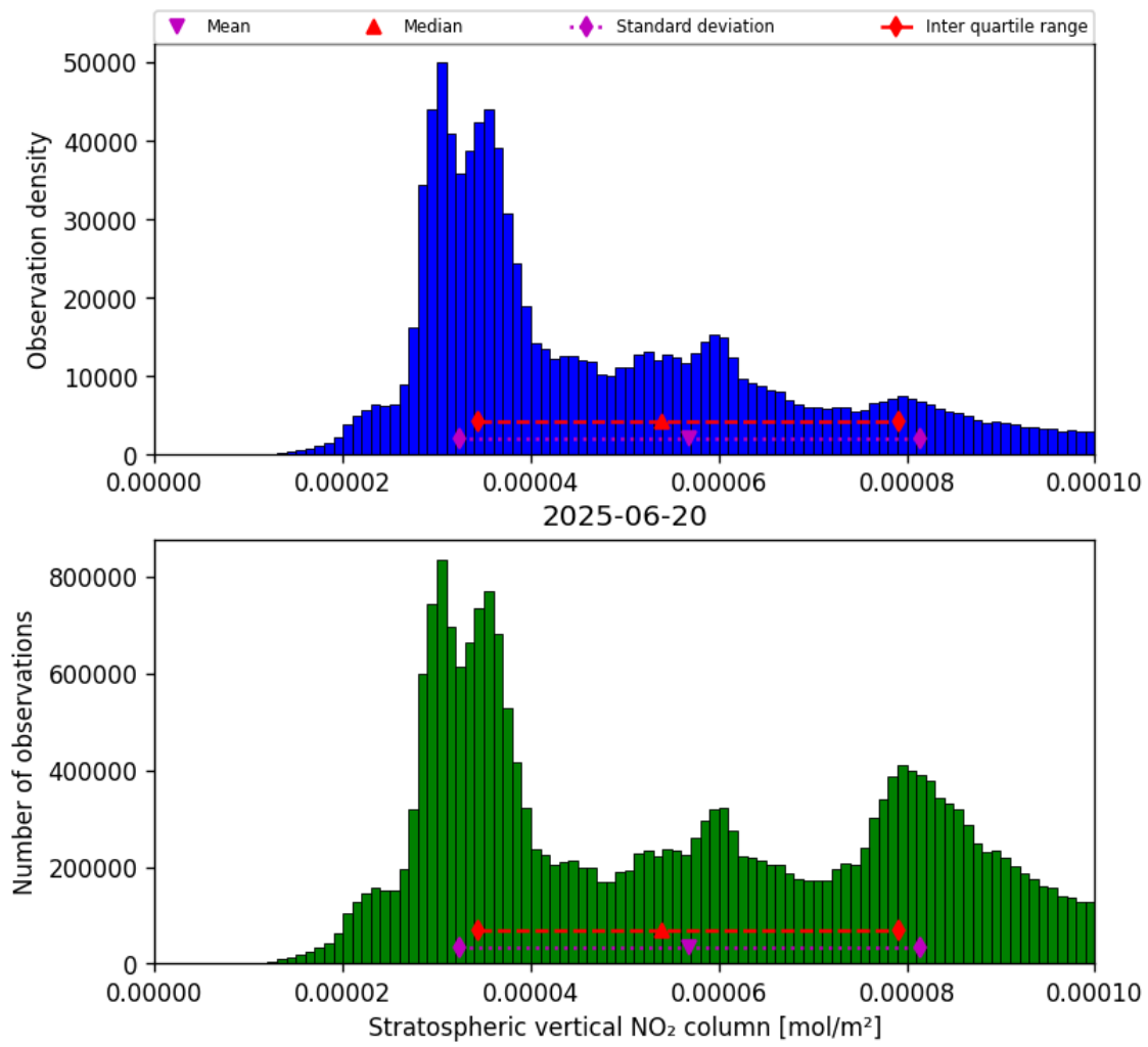
Figure 34: Histogram of “Stratospheric vertical NO 2 column” for 2025-06-20 to 2025-06-20
