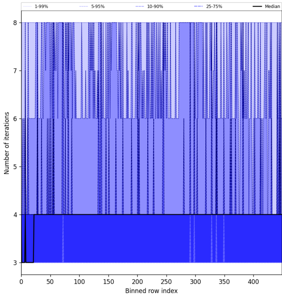
Figure 49: Along track statistics of “Number of iterations” for 2025-06-20 to 2025-06-20
