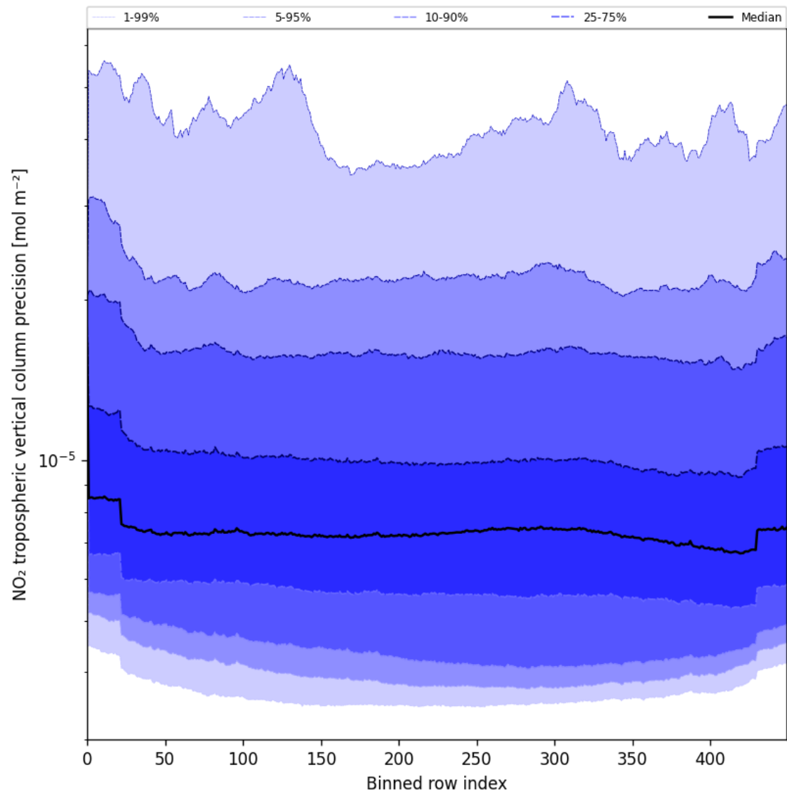
Figure 45: Along track statistics of “NO 2 tropospheric vertical column precision” for 2025-06-20 to 2025-06-20
