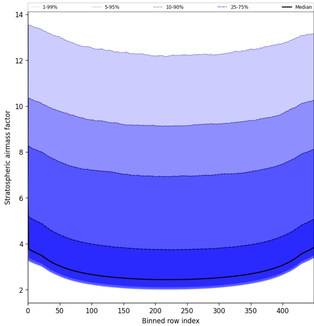
Figure 59: Along track statistics of “Stratospheric airmass factor” for 2025-06-20 to 2025-06-20
