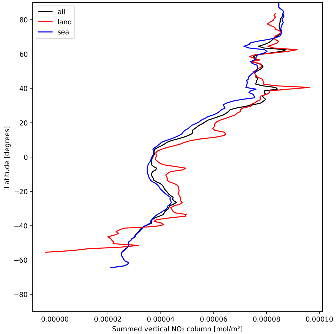
Figure 21: Zonal average of “Summed vertical NO 2 column” for 2025-06-20 to 2025-06-20.
