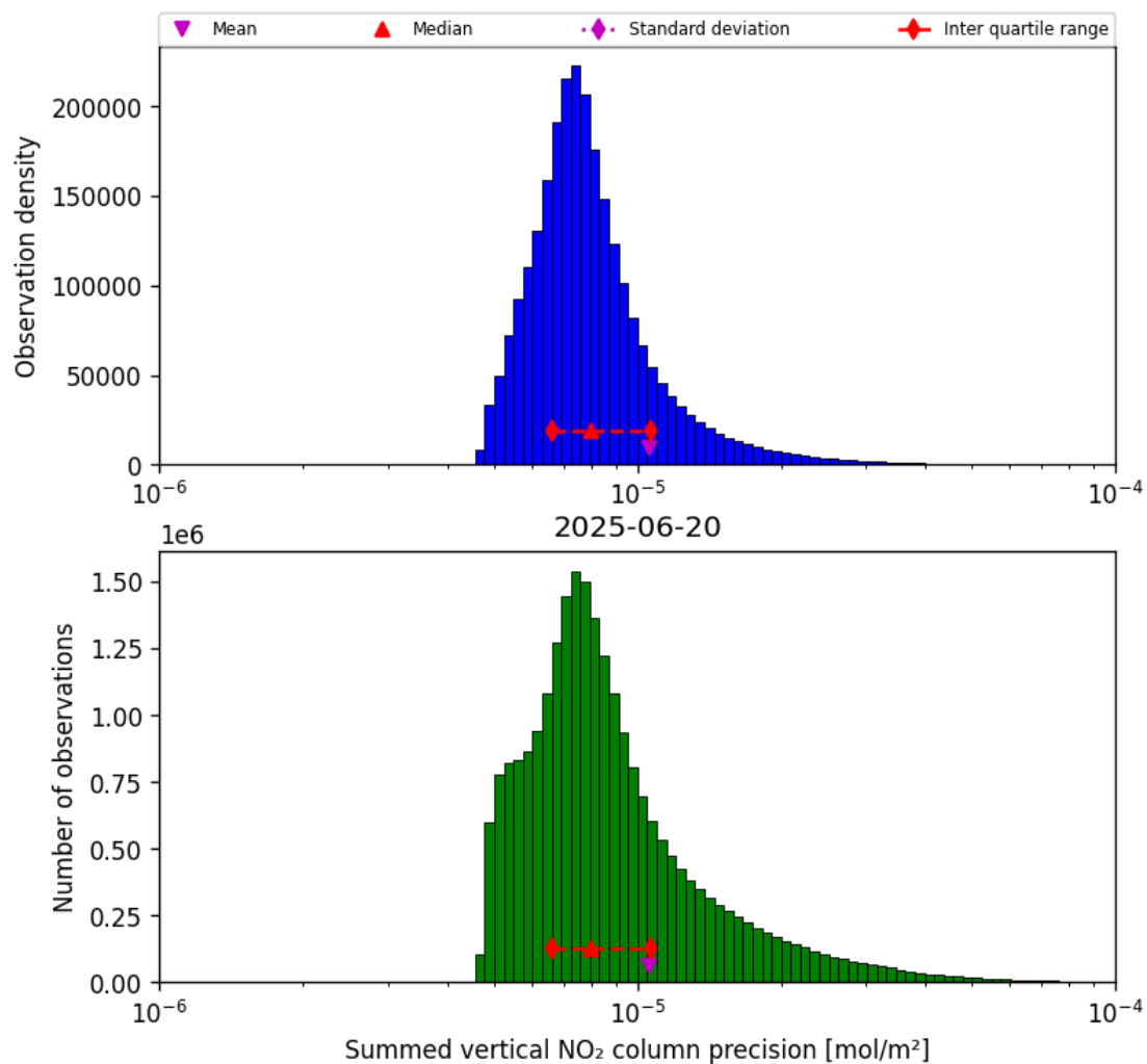
Figure 39: Histogram of "Summed vertical NO 2 column precision" for 2025-06-20 to 2025-06-20
