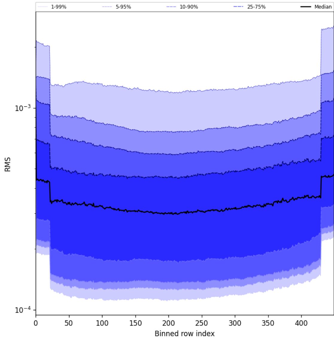
Figure 58: Along track statistics of “RMS” for 2025-06-20 to 2025-06-20
