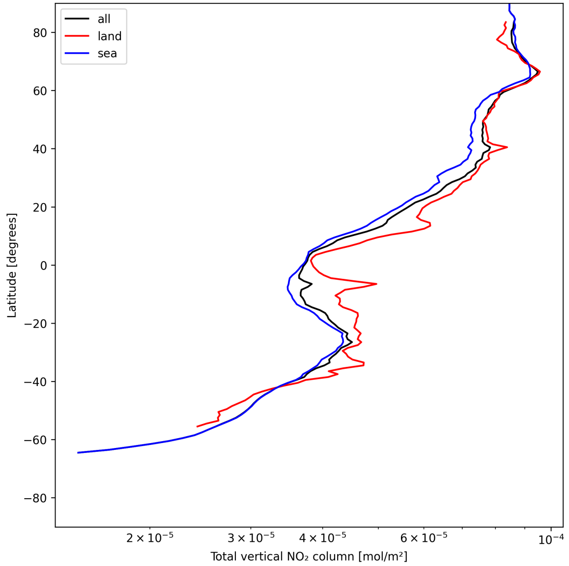
Figure 19: Zonal average of “Total vertical NO 2 column” for 2025-06-20 to 2025-06-20.
