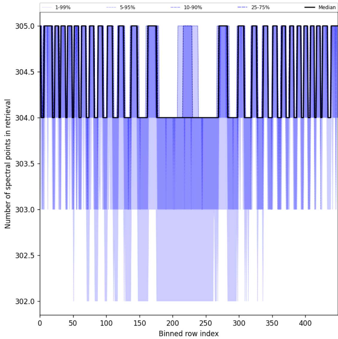
Figure 48: Along track statistics of “Number of spectral points in retrieval” for 2025-06-20 to 2025-06-20
