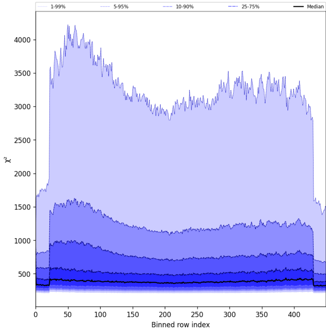
Figure 57: Along track statistics of “ \chi^2 ” for 2025-06-20 to 2025-06-20
