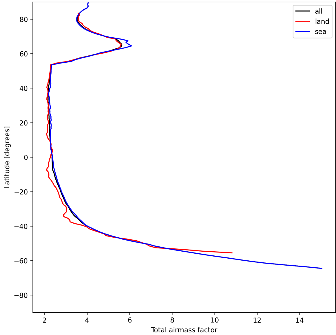
Figure 13: Zonal average of “Total airmass factor” for 2025-06-20 to 2025-06-20.
