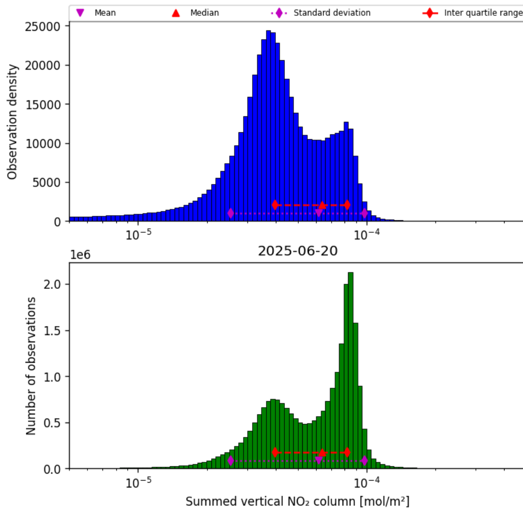
Figure 38: Histogram of “Summed vertical NO 2 column” for 2025-06-20 to 2025-06-20
