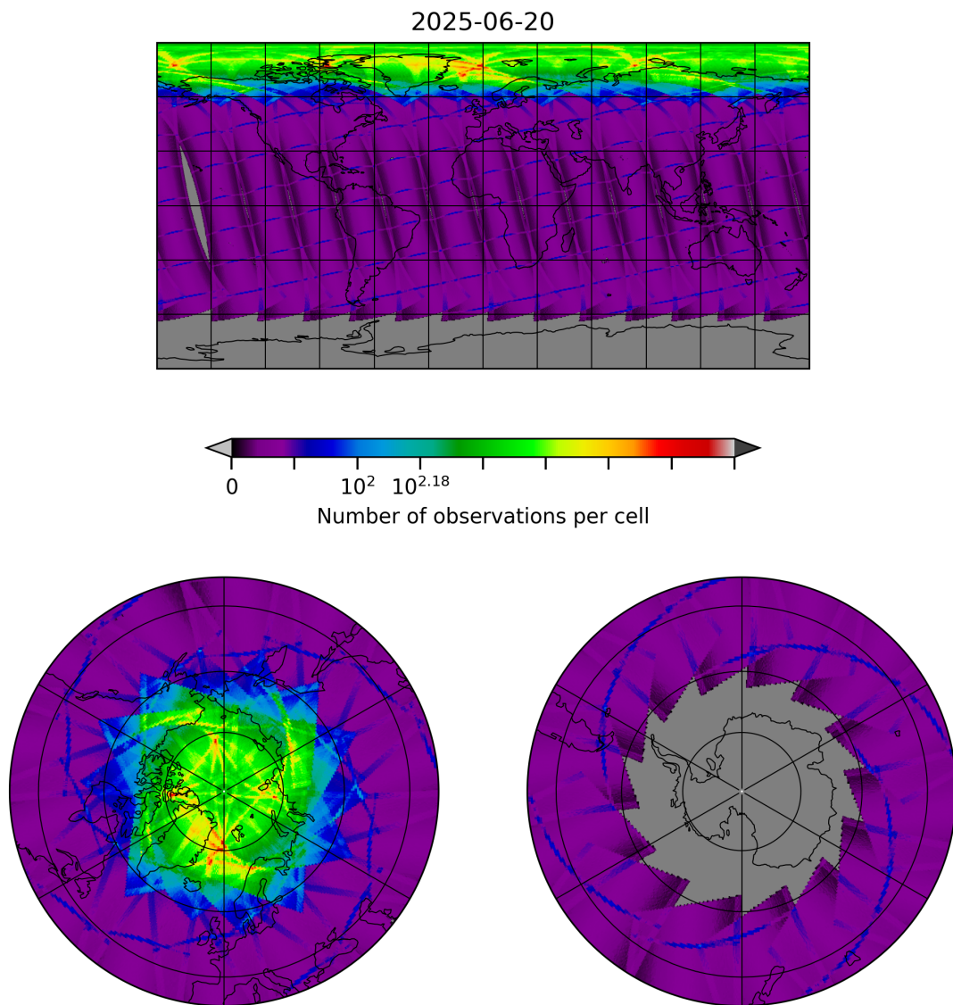
Figure 8: Map of the number of observations for 2025-06-20 to 2025-06-20
