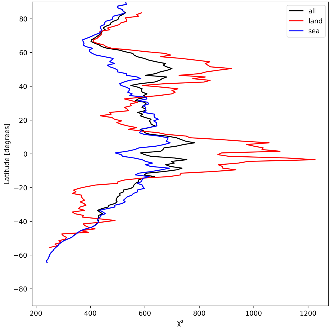
Figure 23: Zonal average of “ \chi^2 ” for 2025-06-20 to 2025-06-20.
