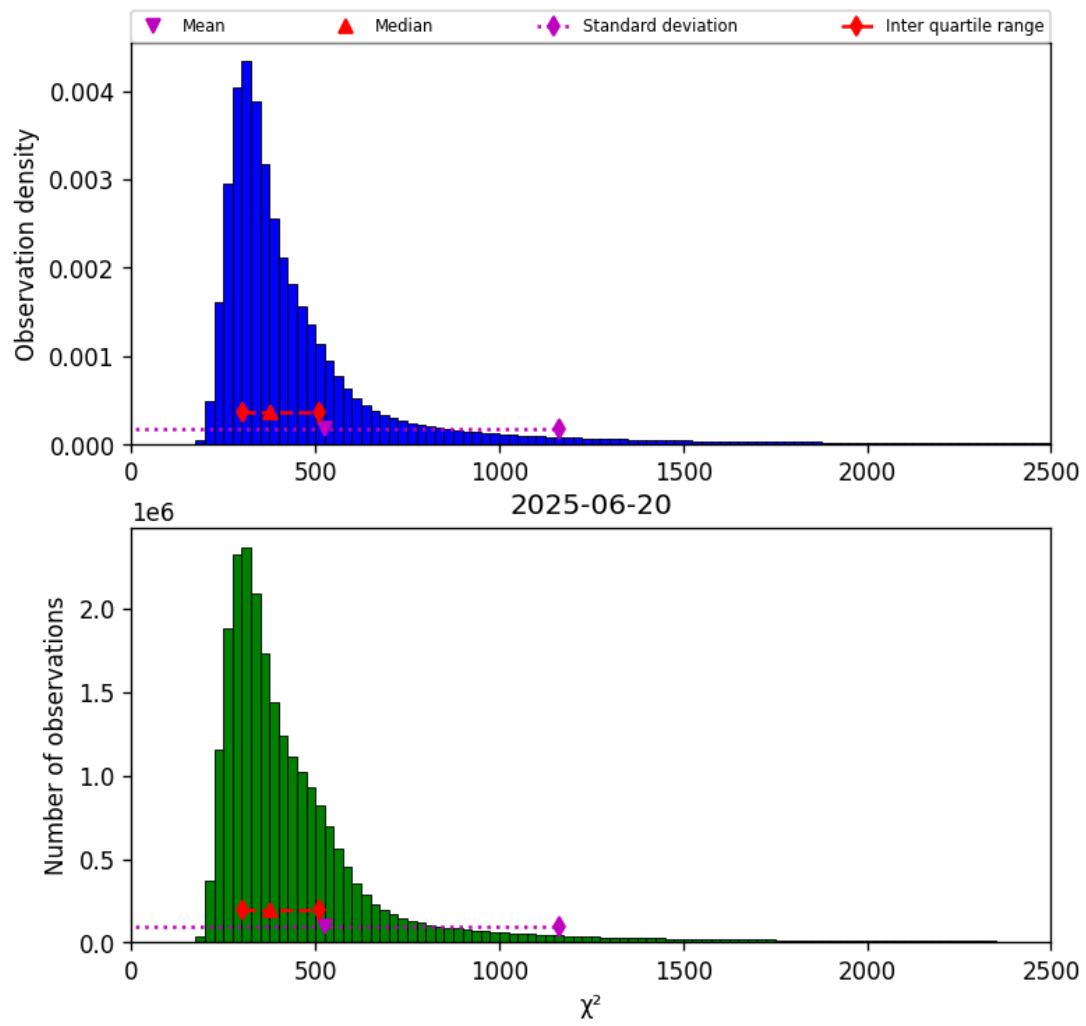
Figure 40: Histogram of “ \chi^2 ” for 2025-06-20 to 2025-06-20
