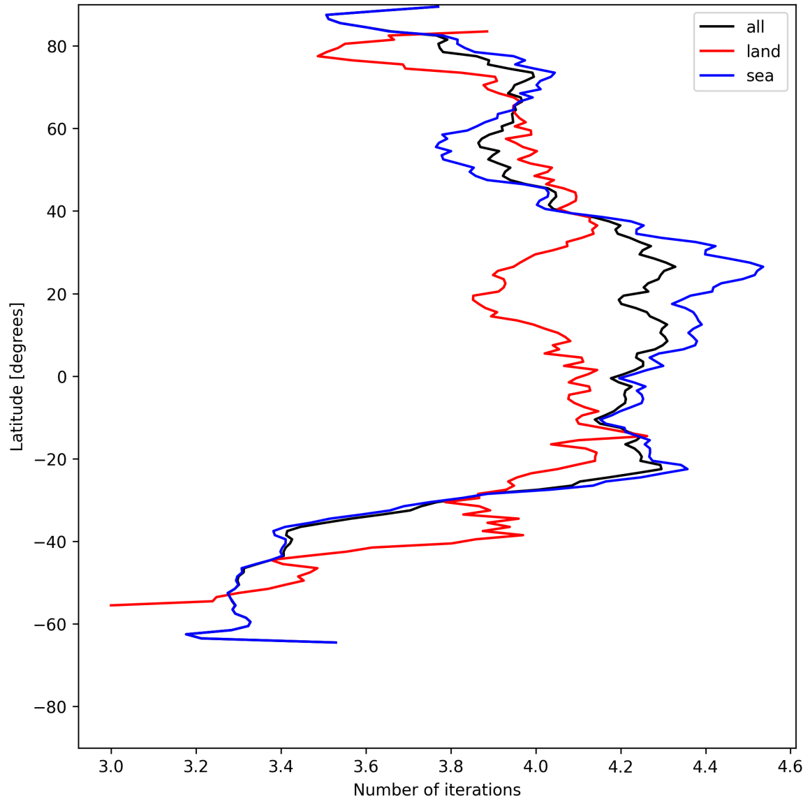
Figure 15: Zonal average of “Number of iterations” for 2025-06-20 to 2025-06-20.
