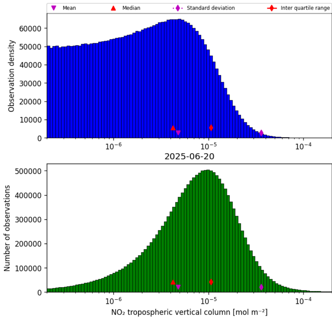
Figure 27: Histogram of “NO 2 tropospheric vertical column” for 2025-06-20 to 2025-06-20
