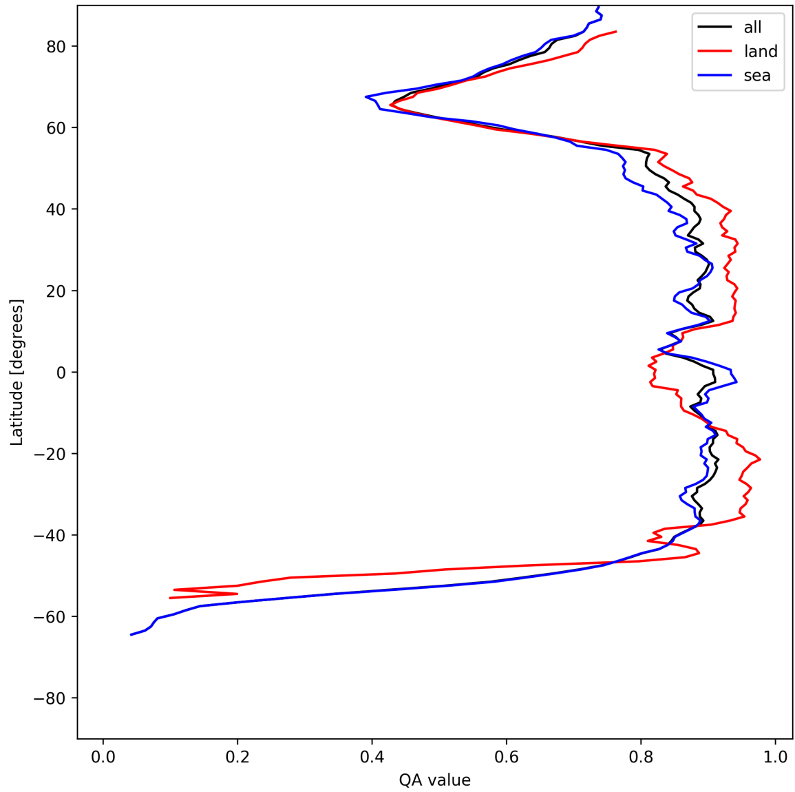
Figure 9: Zonal average of “QA value” for 2025-06-20 to 2025-06-20.
