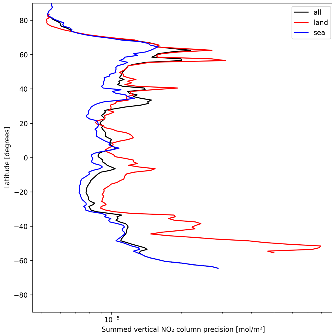
Figure 22: Zonal average of “Summed vertical NO 2 column precision” for 2025-06-20 to 2025-06-20.
