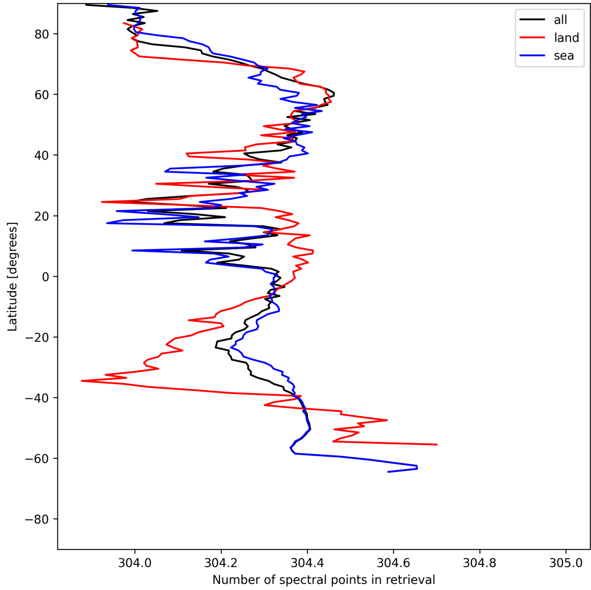
Figure 14: Zonal average of “Number of spectral points in retrieval” for 2025-06-20 to 2025-06-20.
