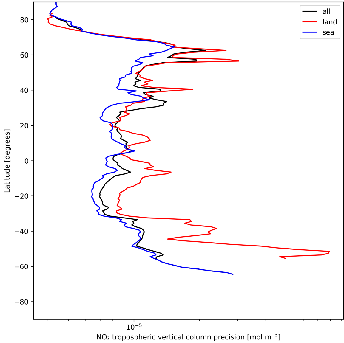
Figure 11: Zonal average of “NO 2 tropospheric vertical column precision” for 2025-06-20 to 2025-06-20.
