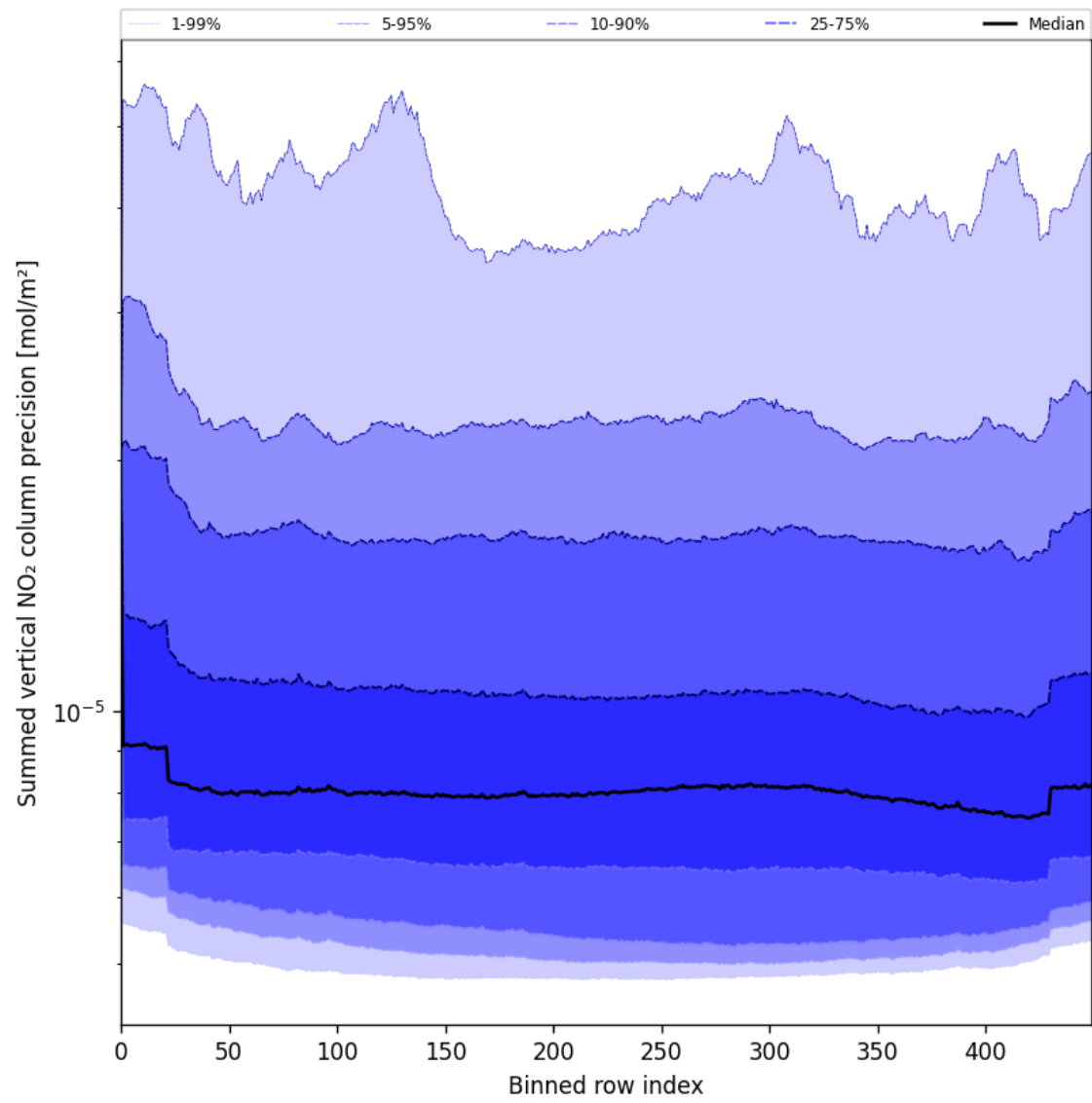
Figure 56: Along track statistics of “Summed vertical NO 2 column precision” for 2025-06-20 to 2025-06-20
