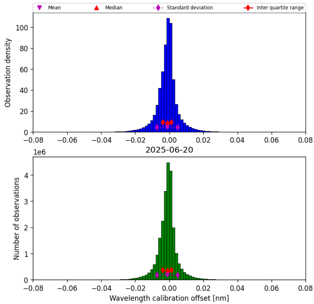
Figure 33: Histogram of “Wavelength calibration offset” for 2025-06-20 to 2025-06-20
