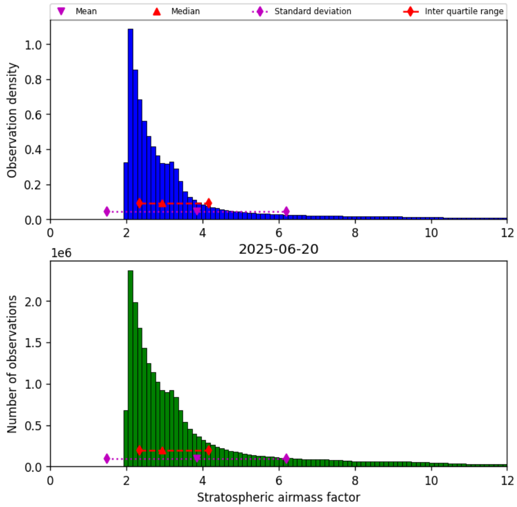
Figure 42: Histogram of “Stratospheric airmass factor” for 2025-06-20 to 2025-06-20
