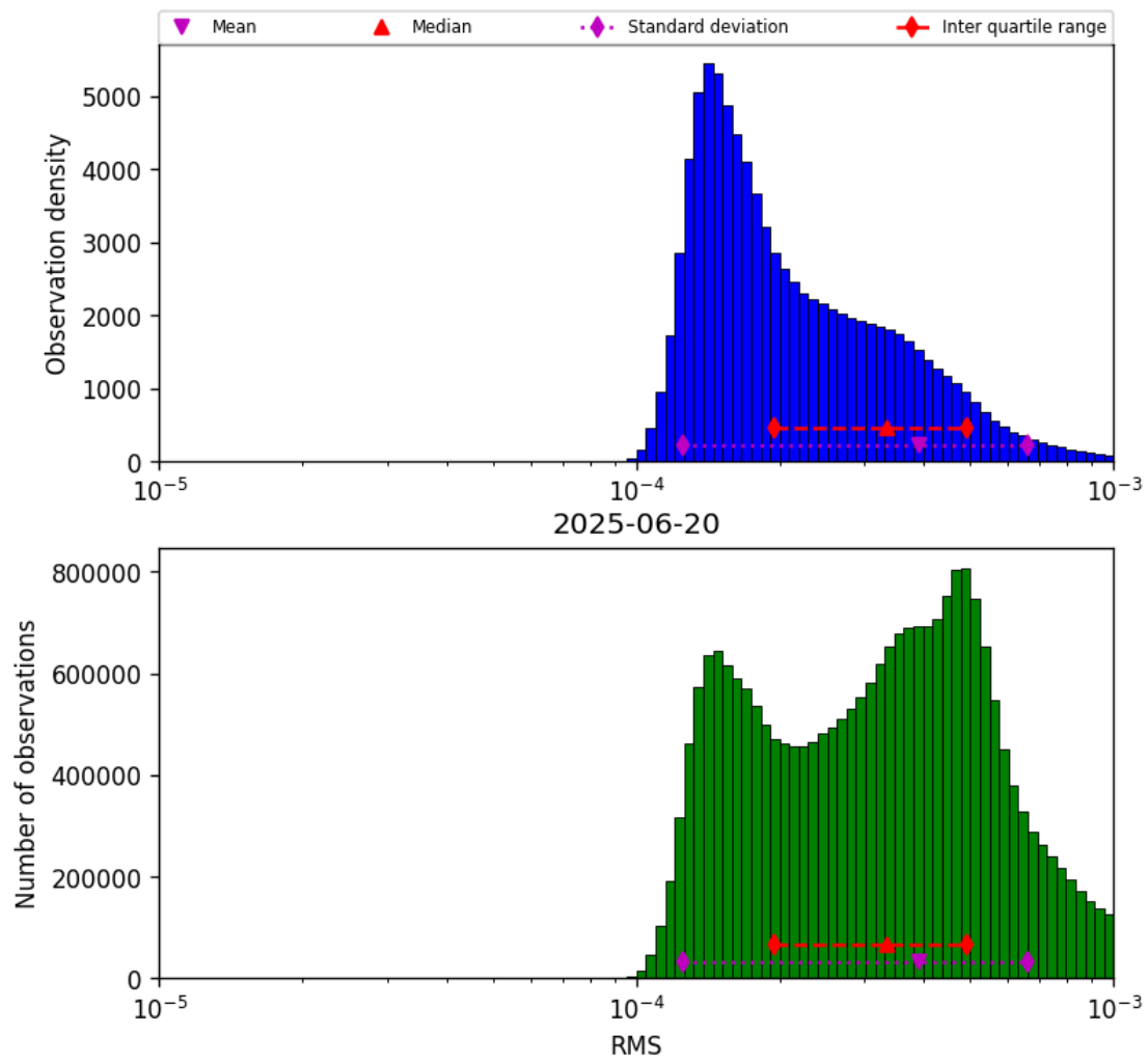
Figure 41: Histogram of “RMS” for 2025-06-20 to 2025-06-20
