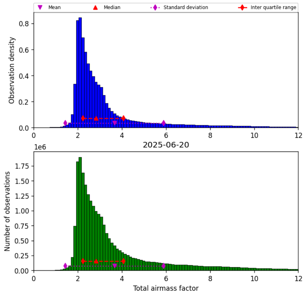
Figure 30: Histogram of “Total airmass factor” for 2025-06-20 to 2025-06-20
