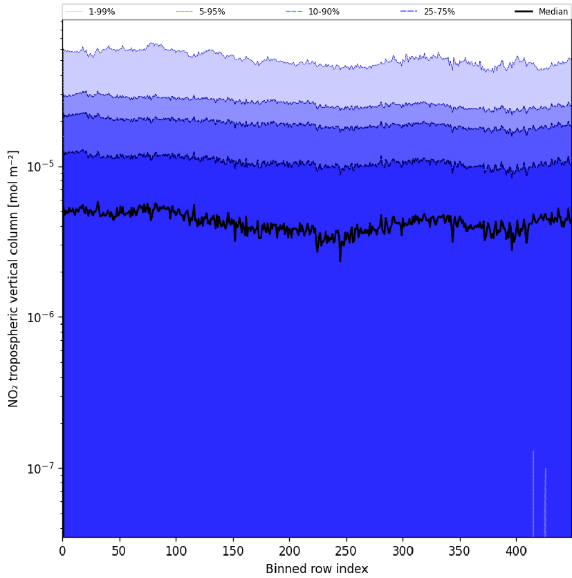
Figure 44: Along track statistics of “NO 2 tropospheric vertical column” for 2025-06-20 to 2025-06-20
