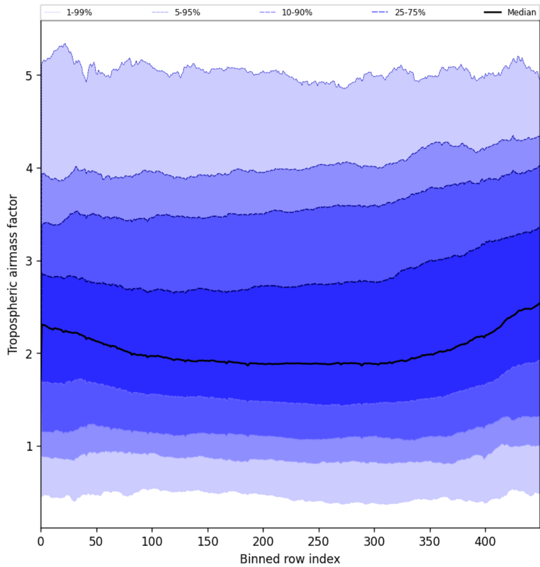
Figure 46: Along track statistics of “Tropospheric airmass factor” for 2025-06-20 to 2025-06-20
