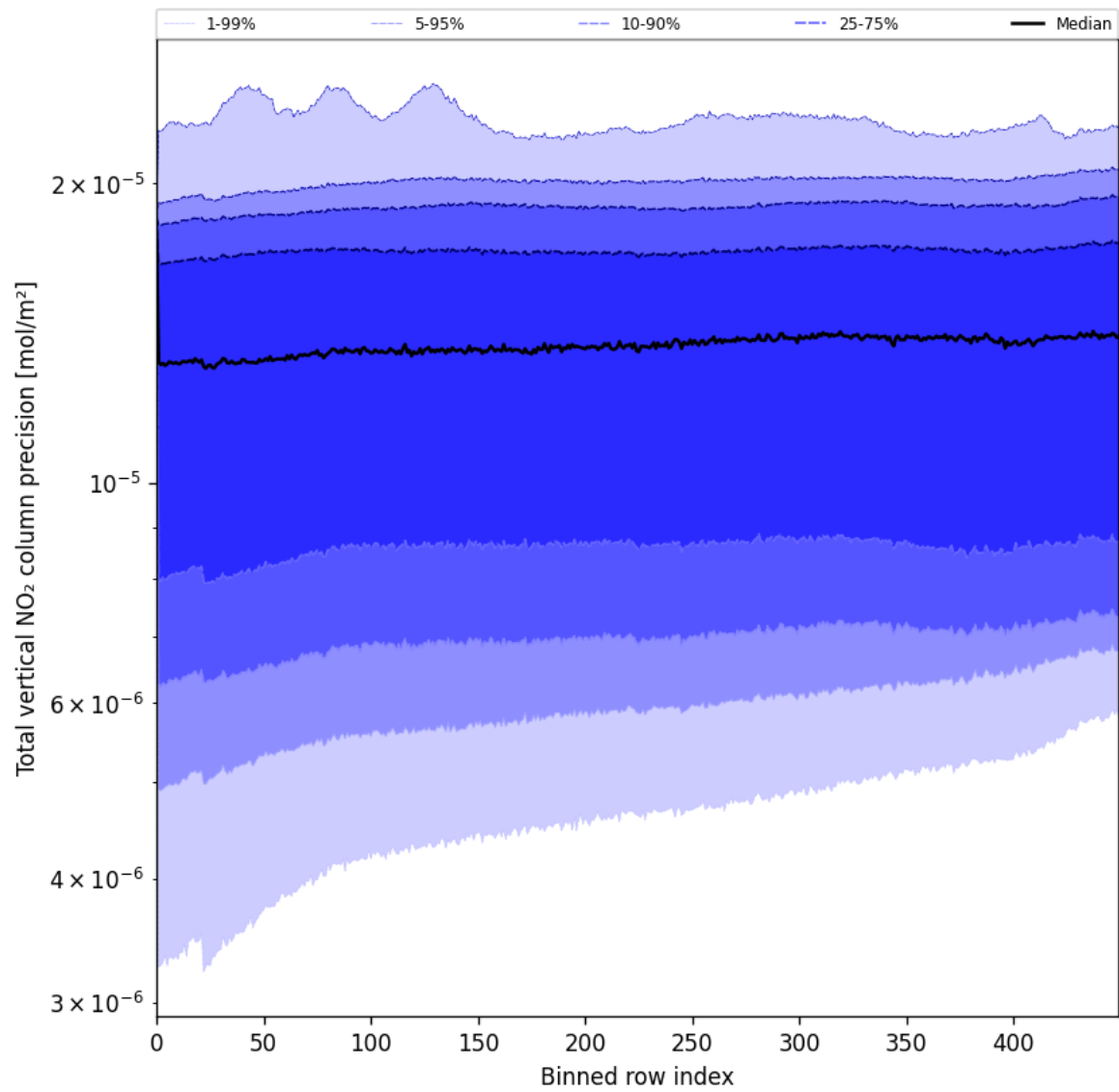
Figure 54: Along track statistics of “Total vertical NO 2 column precision” for 2025-06-20 to 2025-06-20
