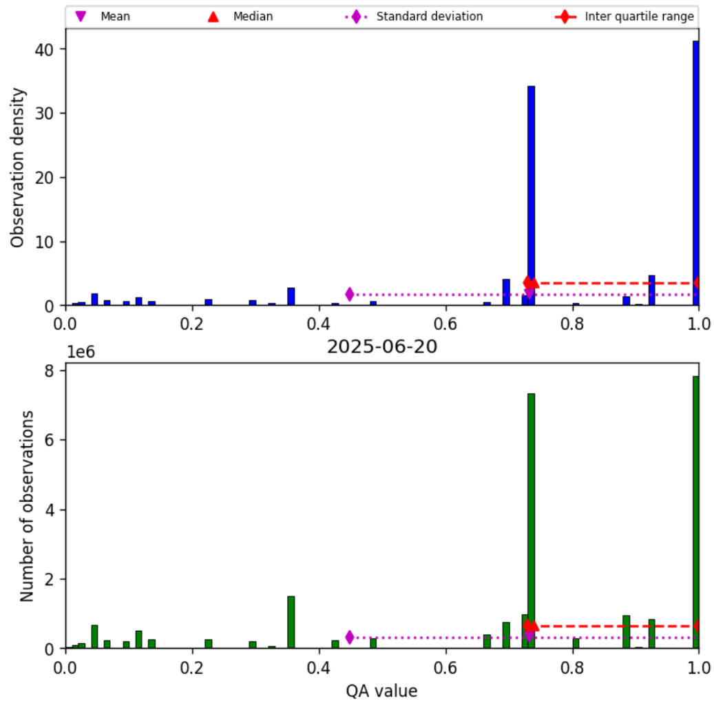
Figure 26: Histogram of “QA value” for 2025-06-20 to 2025-06-20
