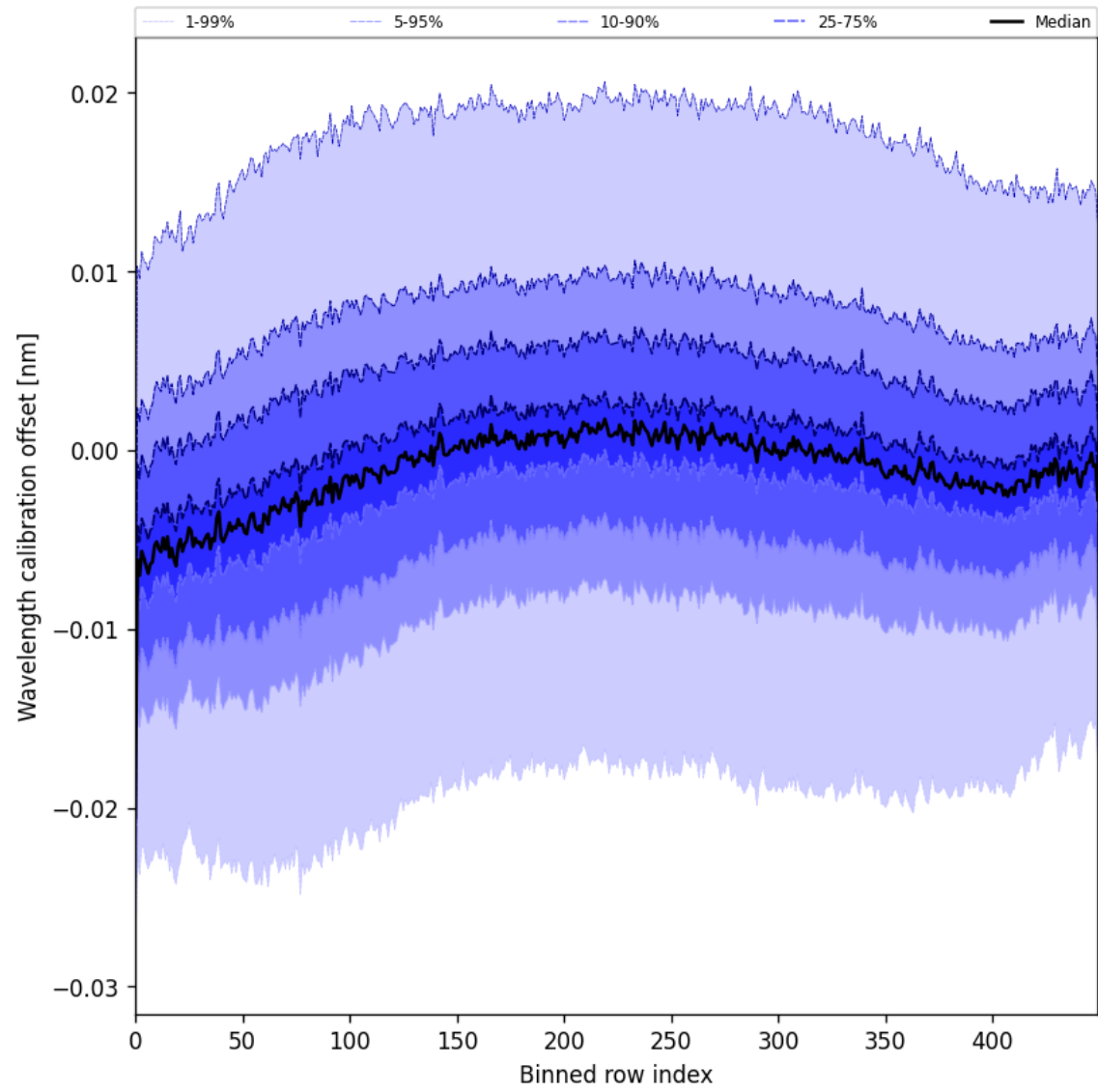
Figure 50: Along track statistics of “Wavelength calibration offset” for 2025-06-20 to 2025-06-20
