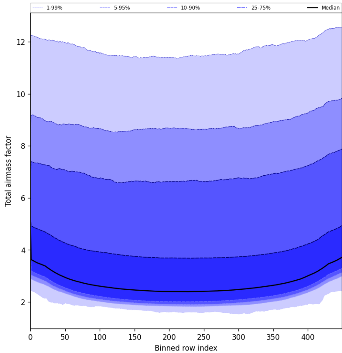
Figure 47: Along track statistics of “Total airmass factor” for 2025-06-20 to 2025-06-20
