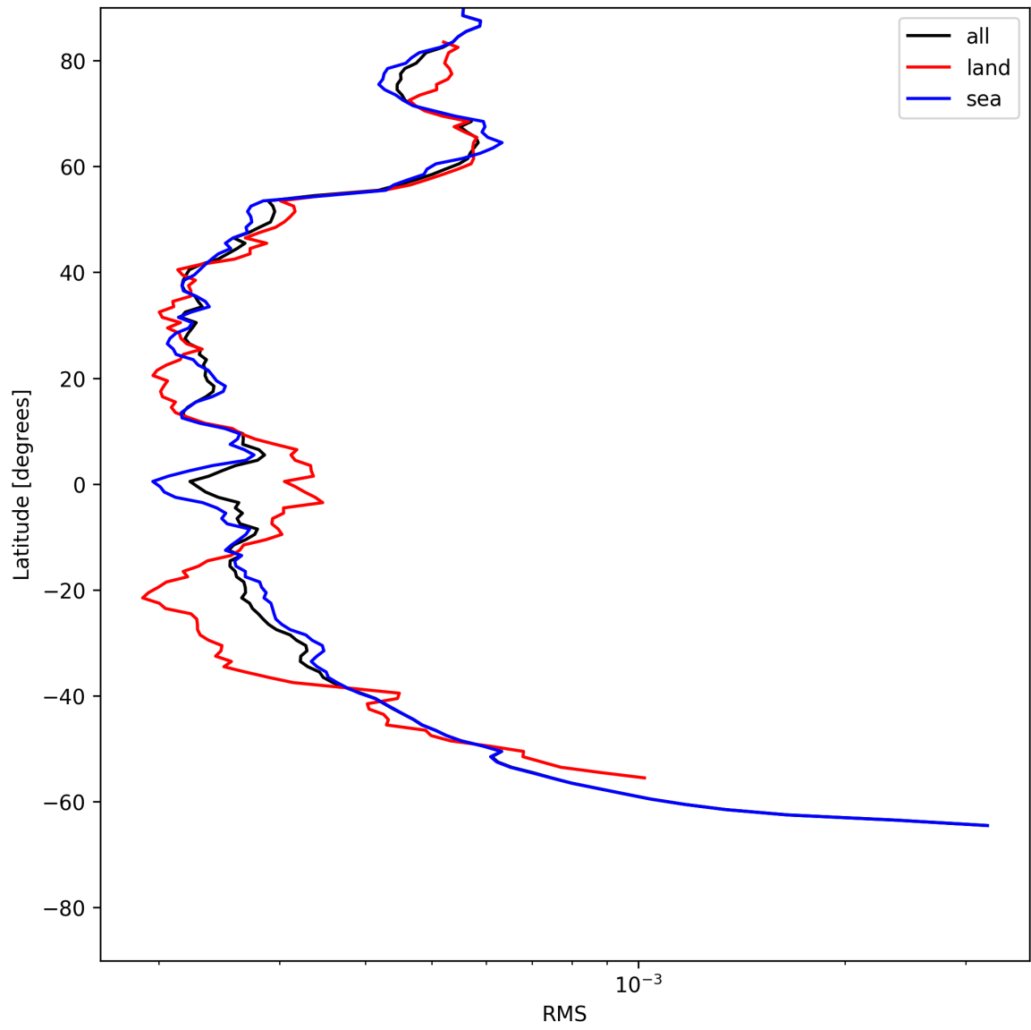
Figure 24: Zonal average of “RMS” for 2025-06-20 to 2025-06-20.
