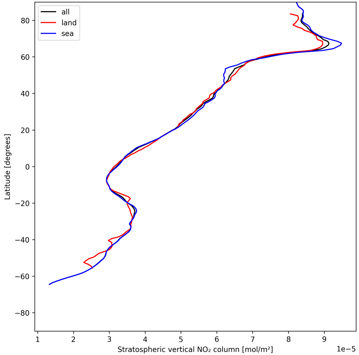
Figure 17: Zonal average of “Stratospheric vertical NO 2 column” for 2025-06-20 to 2025-06-20.
