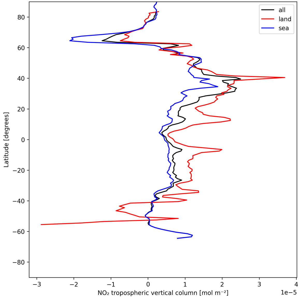
Figure 10: Zonal average of “NO 2 tropospheric vertical column” for 2025-06-20 to 2025-06-20.
