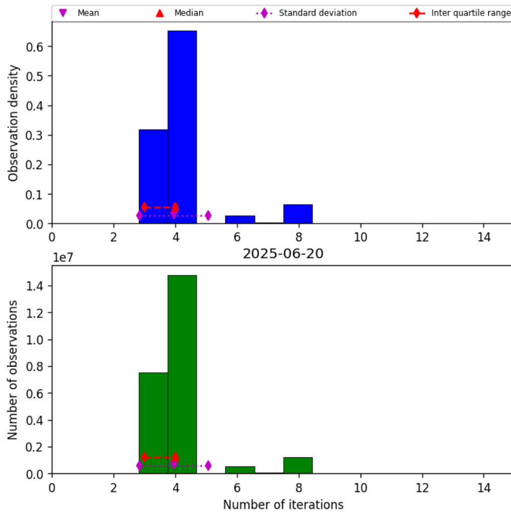
Figure 32: Histogram of “Number of iterations” for 2025-06-20 to 2025-06-20
