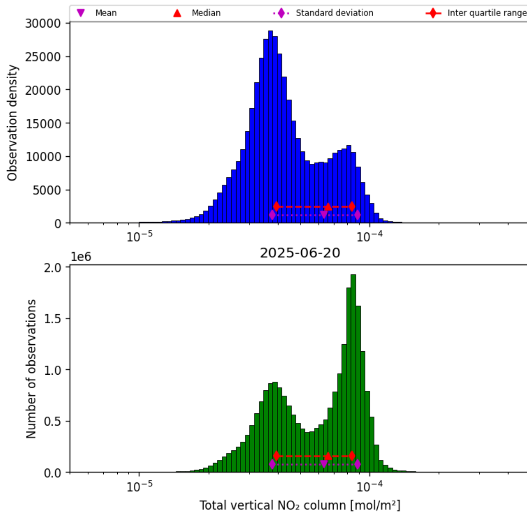
Figure 36: Histogram of "Total vertical NO 2 column" for 2025-06-20 to 2025-06-20
