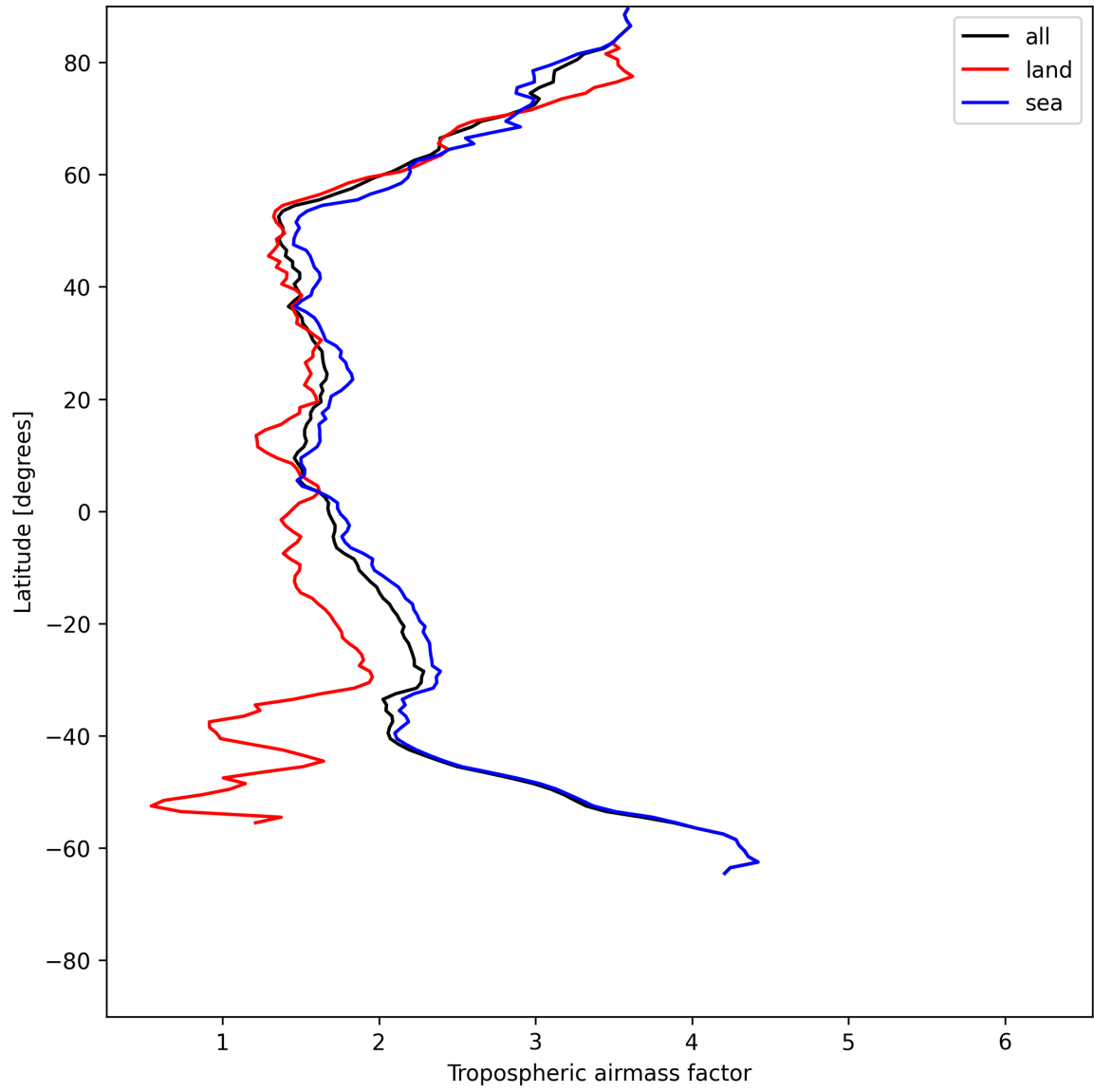
Figure 12: Zonal average of “Tropospheric airmass factor” for 2025-06-20 to 2025-06-20.
