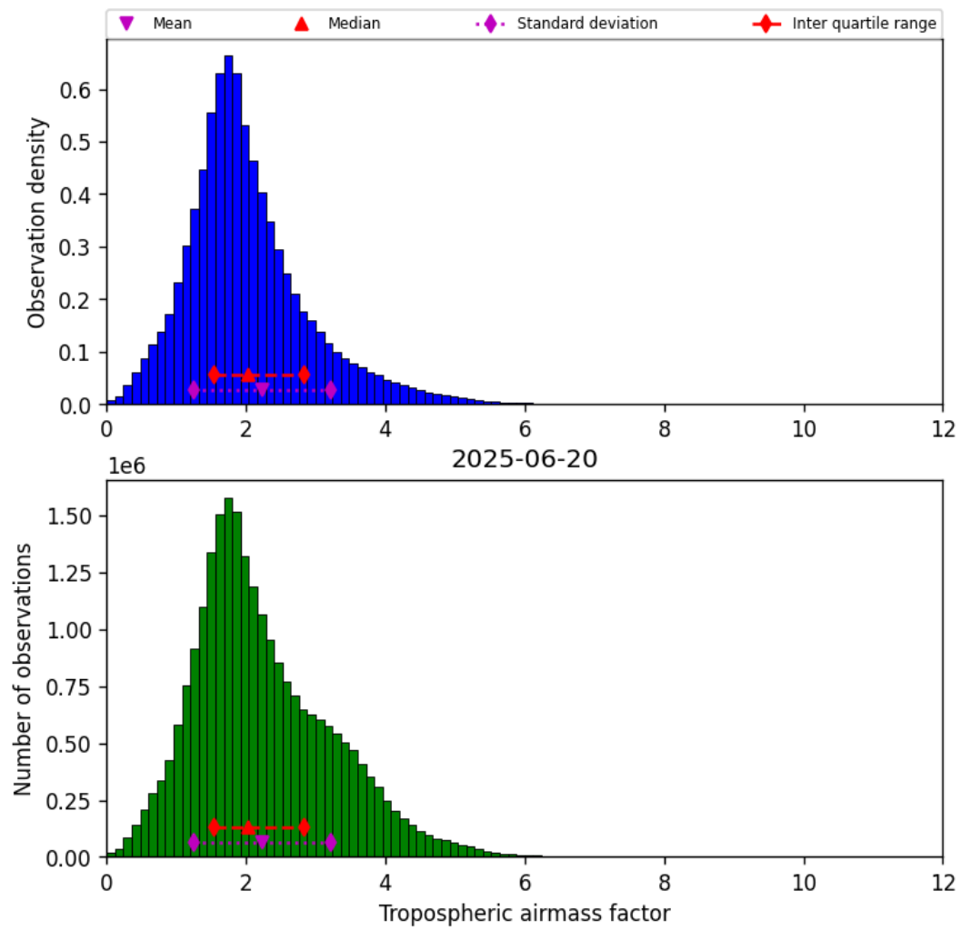
Figure 29: Histogram of “Tropospheric airmass factor” for 2025-06-20 to 2025-06-20
