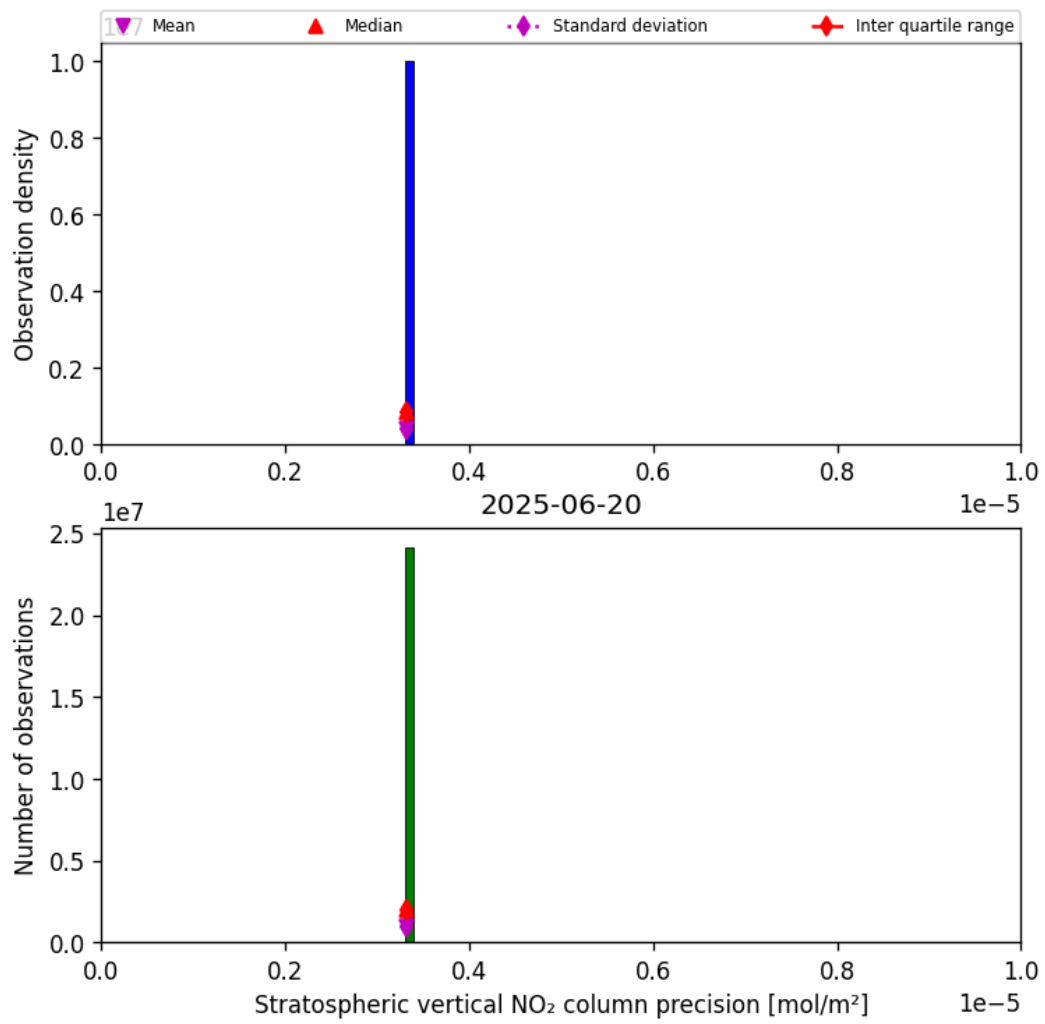
Figure 35: Histogram of “Stratospheric vertical NO 2 column precision” for 2025-06-20 to 2025-06-20
