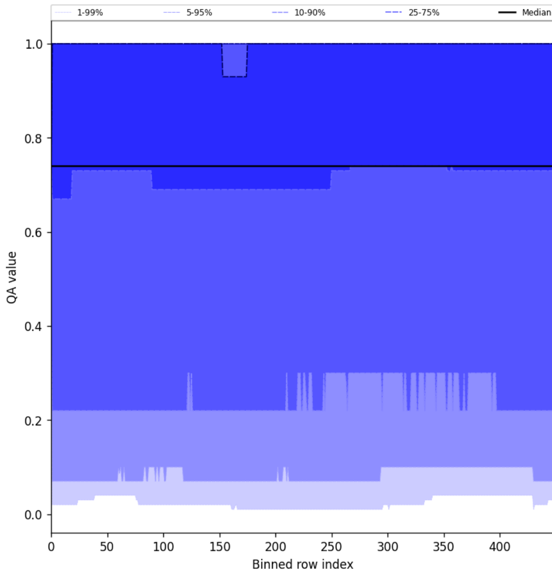
Figure 43: Along track statistics of "QA value" for 2025-06-20 to 2025-06-20
