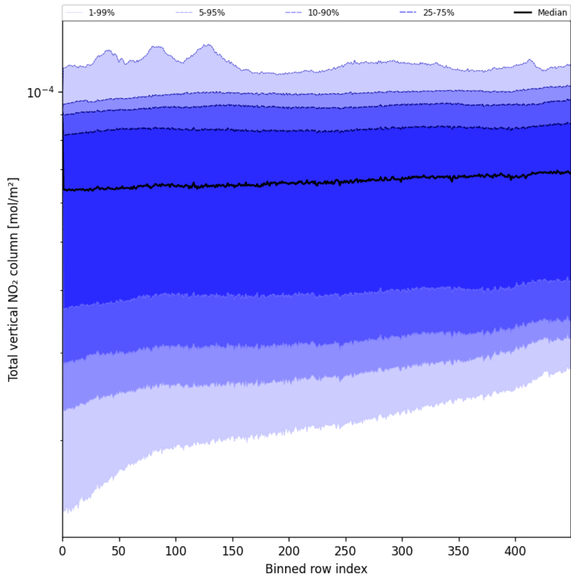
Figure 53: Along track statistics of “Total vertical NO 2 column” for 2025-06-20 to 2025-06-20
