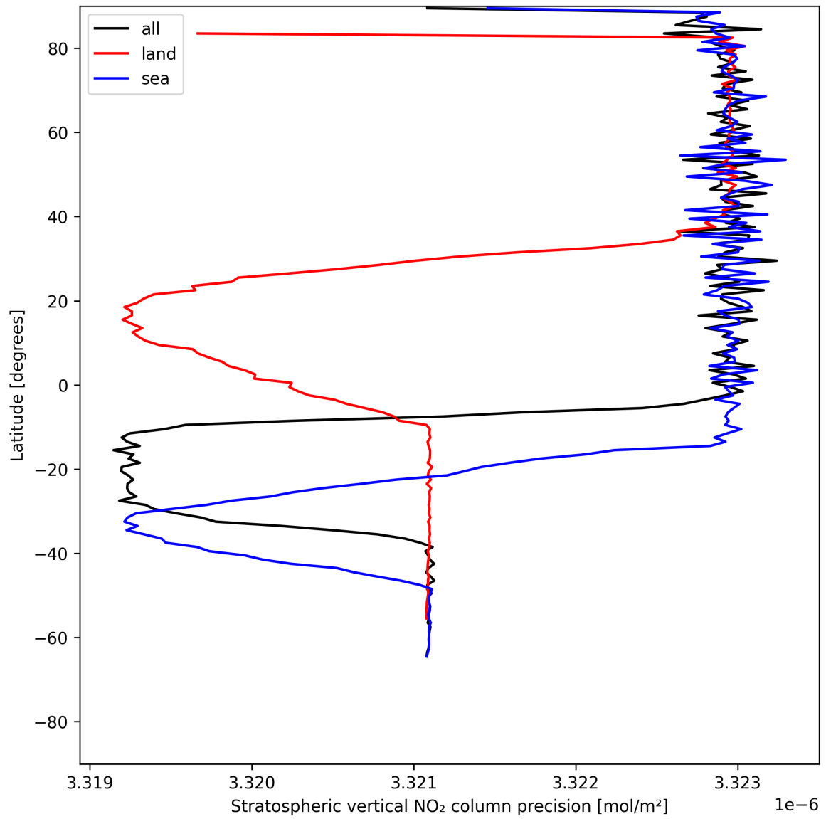
Figure 18: Zonal average of “Stratospheric vertical NO 2 column precision” for 2025-06-20 to 2025-06-20.
