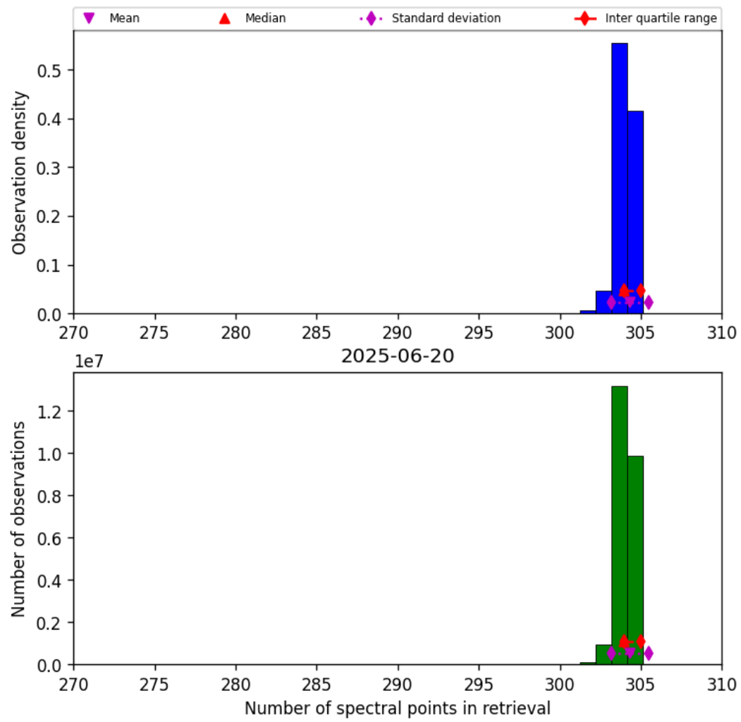
Figure 31: Histogram of “Number of spectral points in retrieval” for 2025-06-20 to 2025-06-20
