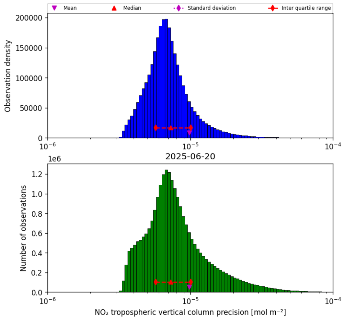
Figure 28: Histogram of “NO 2 tropospheric vertical column precision” for 2025-06-20 to 2025-06-20
