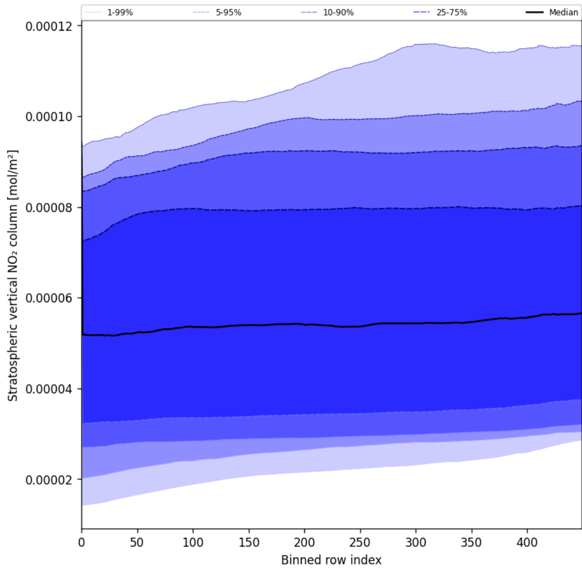
Figure 51: Along track statistics of “Stratospheric vertical NO 2 column” for 2025-06-20 to 2025-06-20
