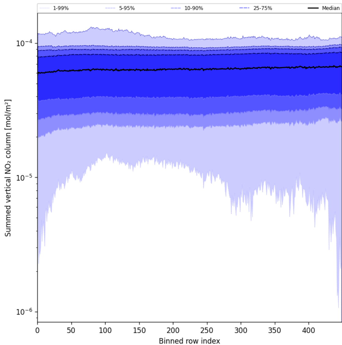
Figure 55: Along track statistics of “Summed vertical NO 2 column” for 2025-06-20 to 2025-06-20
