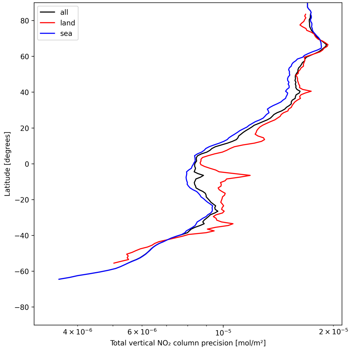
Figure 20: Zonal average of “Total vertical NO 2 column precision” for 2025-06-20 to 2025-06-20.
