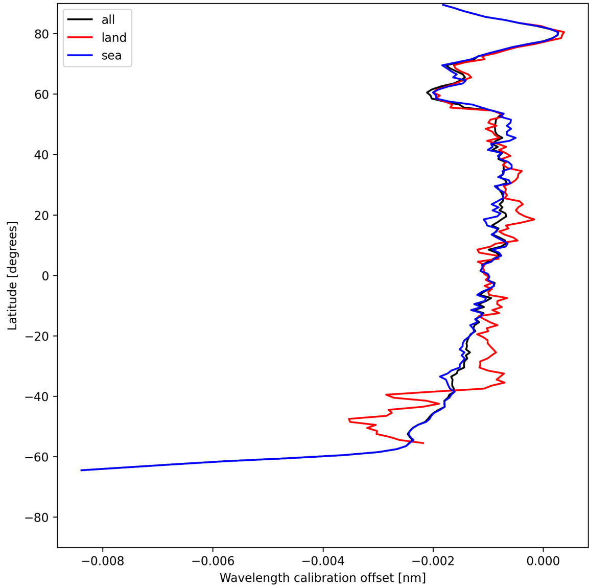
Figure 16: Zonal average of “Wavelength calibration offset” for 2025-06-20 to 2025-06-20.
