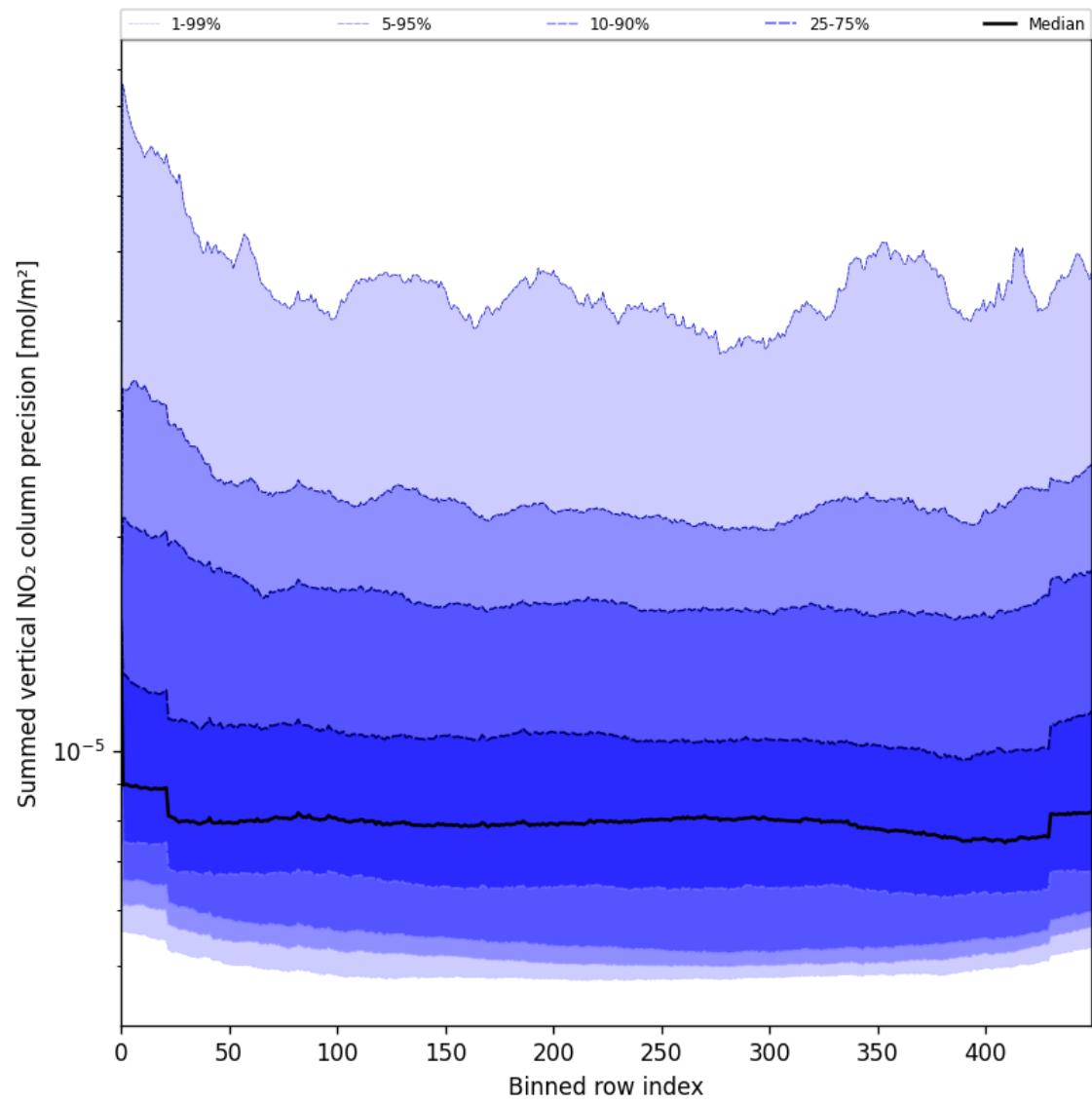
Figure 56: Along track statistics of “Summed vertical NO 2 column precision” for 2025-06-21 to 2025-06-22
