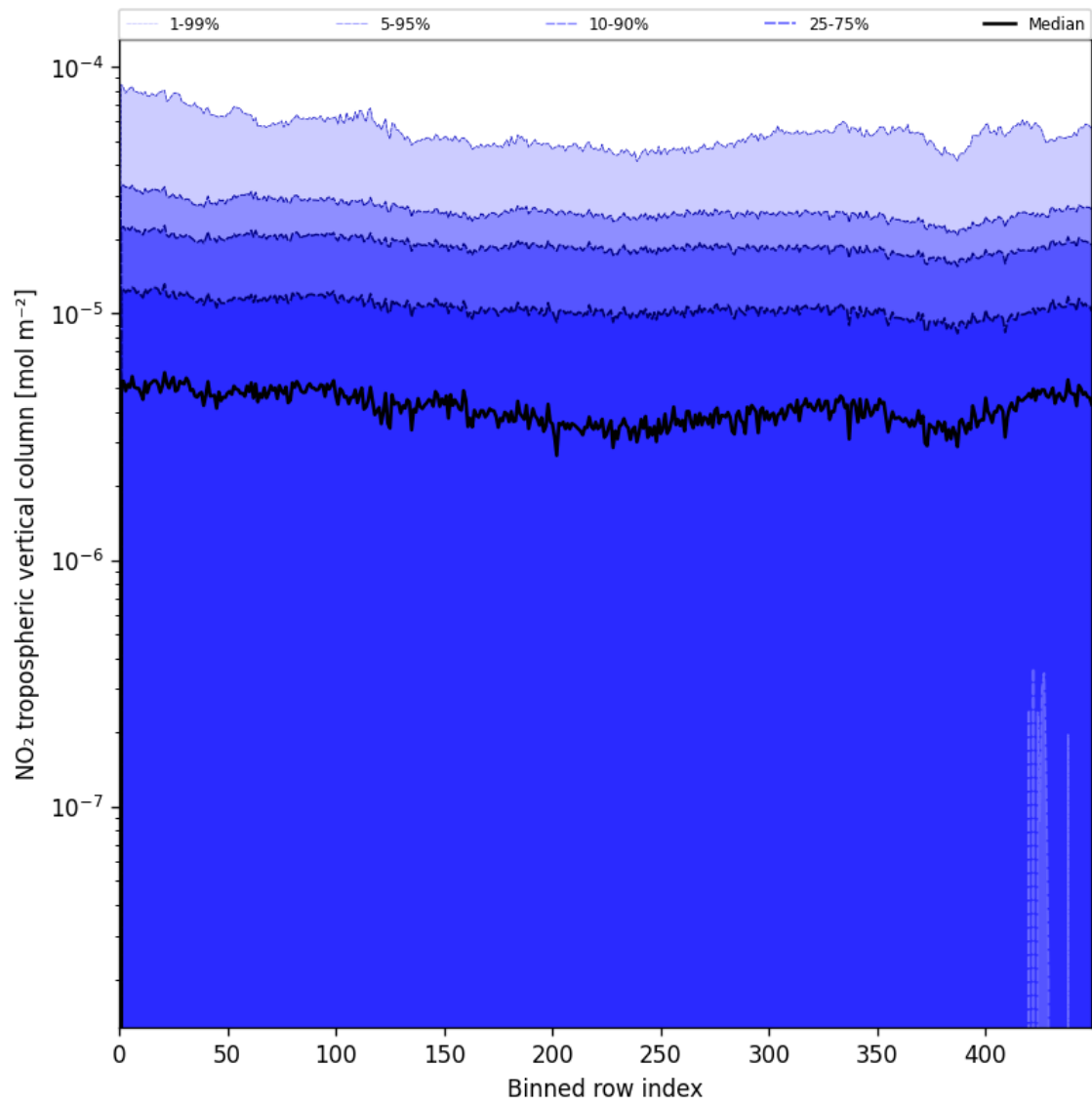
Figure 44: Along track statistics of “NO 2 tropospheric vertical column” for 2025-06-21 to 2025-06-22
