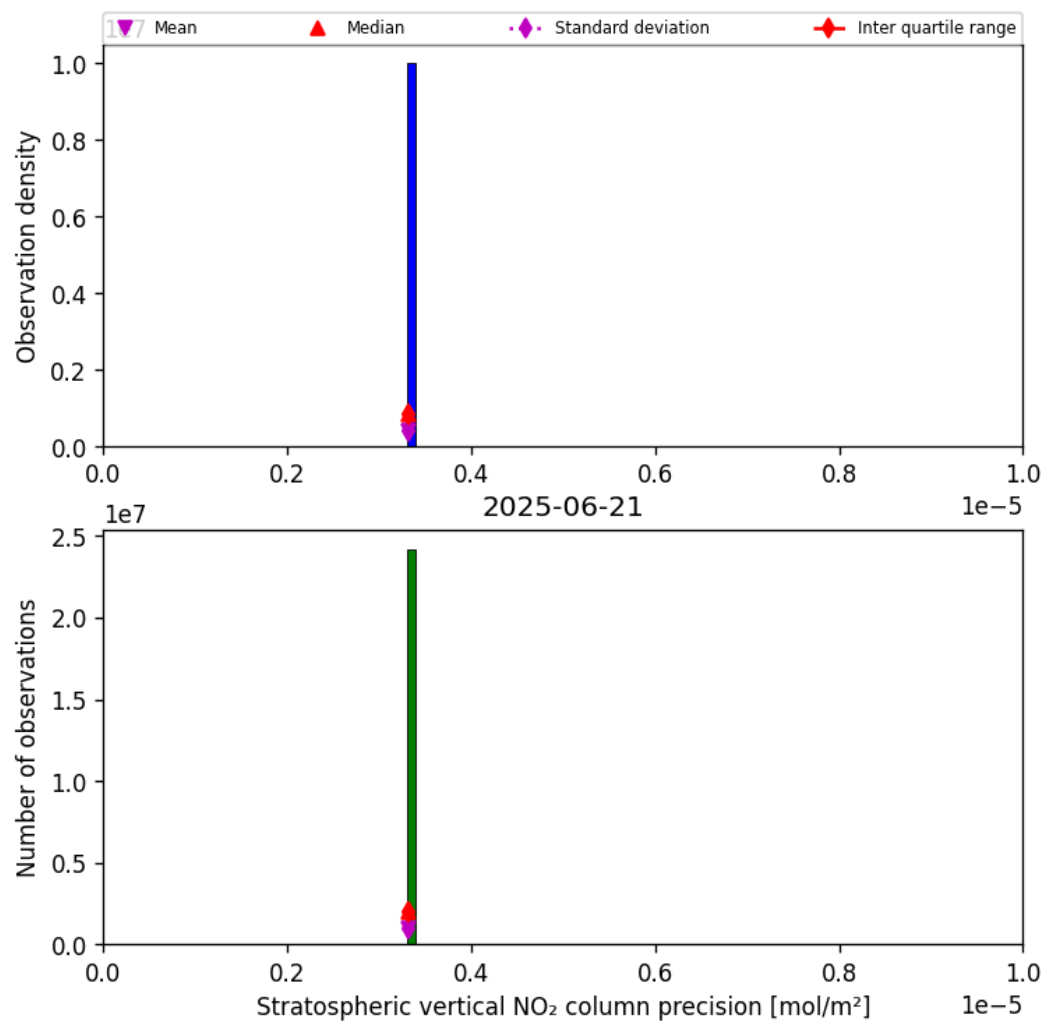
Figure 35: Histogram of “Stratospheric vertical NO 2 column precision” for 2025-06-21 to 2025-06-22
