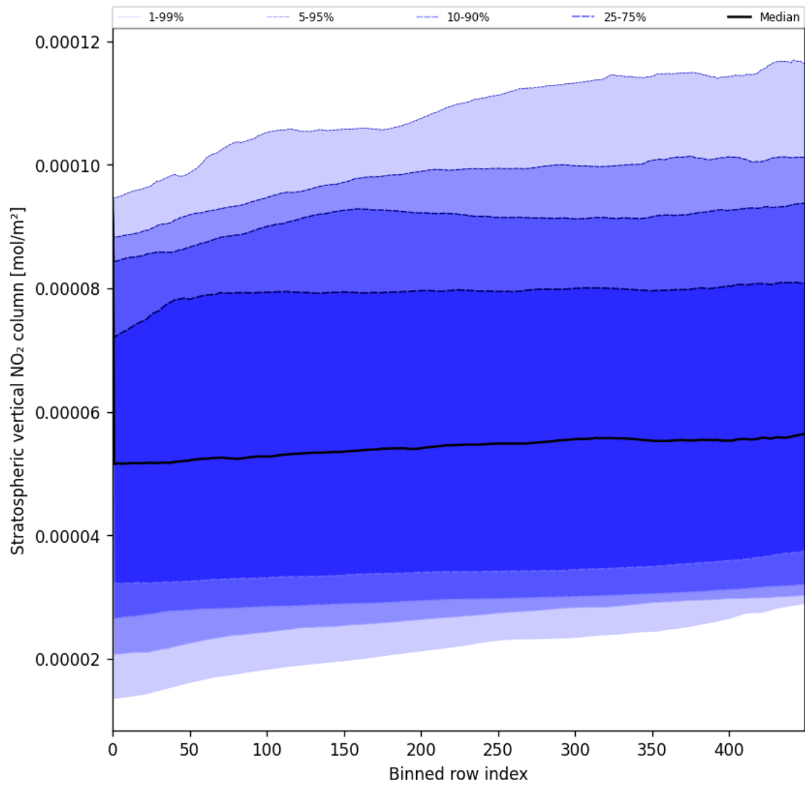
Figure 51: Along track statistics of “Stratospheric vertical NO 2 column” for 2025-06-21 to 2025-06-22
