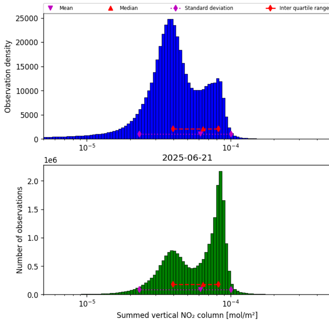
Figure 38: Histogram of “Summed vertical NO 2 column” for 2025-06-21 to 2025-06-22
