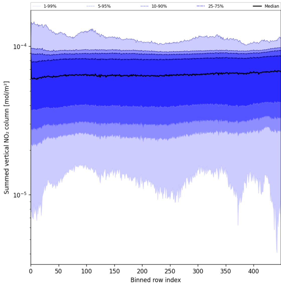
Figure 55: Along track statistics of “Summed vertical NO 2 column” for 2025-06-21 to 2025-06-22
