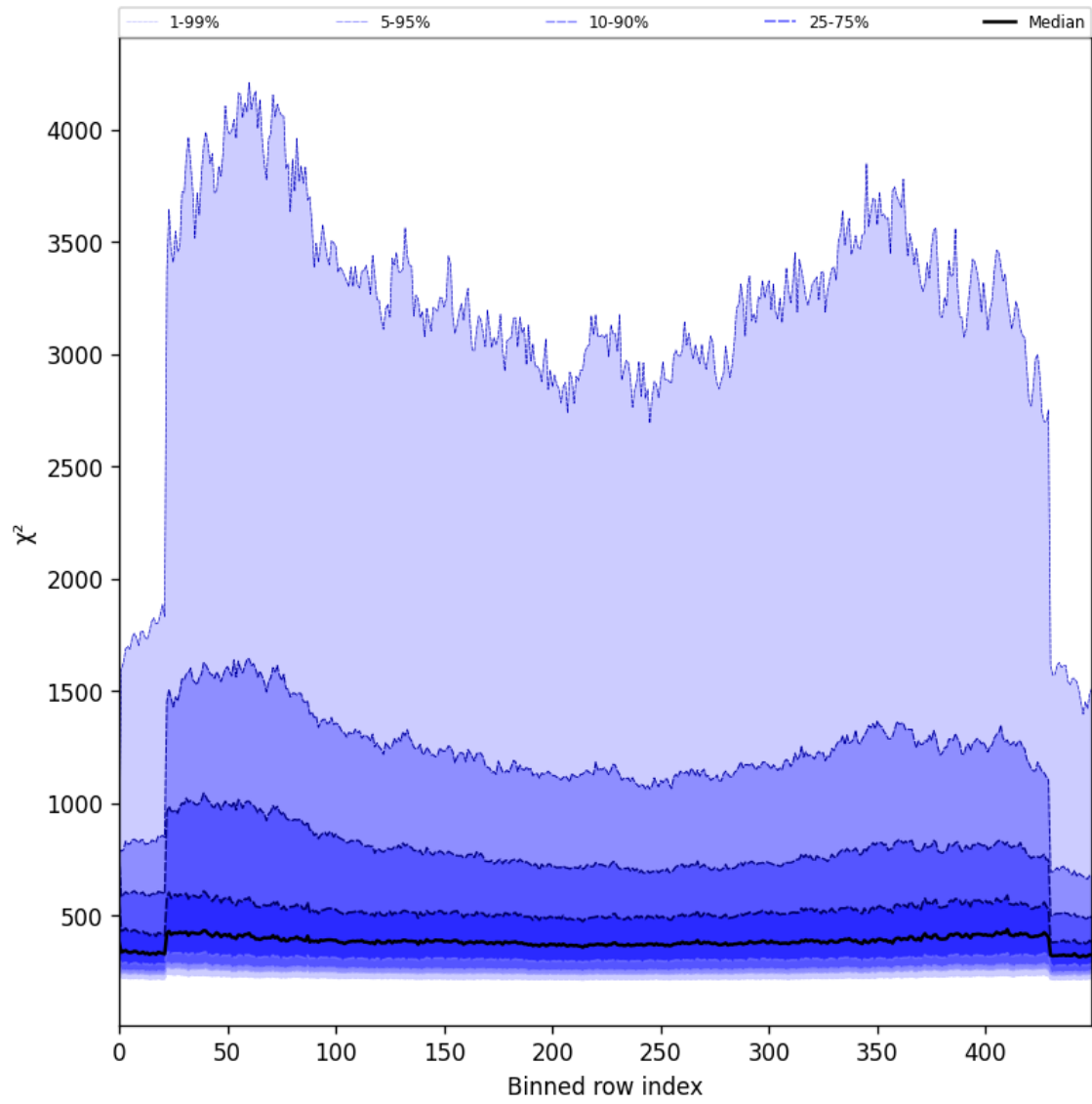
Figure 57: Along track statistics of “ \chi^2 ” for 2025-06-21 to 2025-06-22
