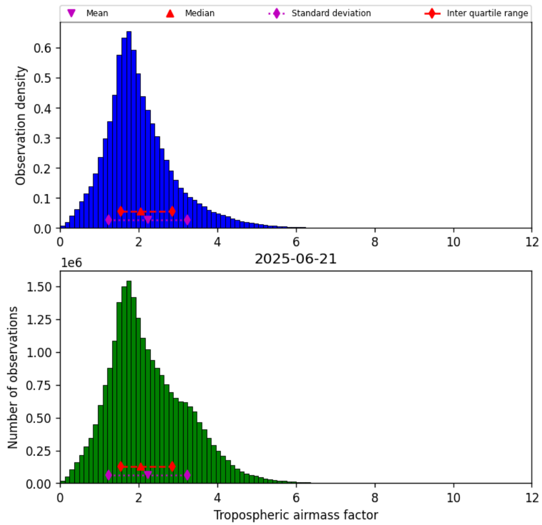
Figure 29: Histogram of “Tropospheric airmass factor” for 2025-06-21 to 2025-06-22
