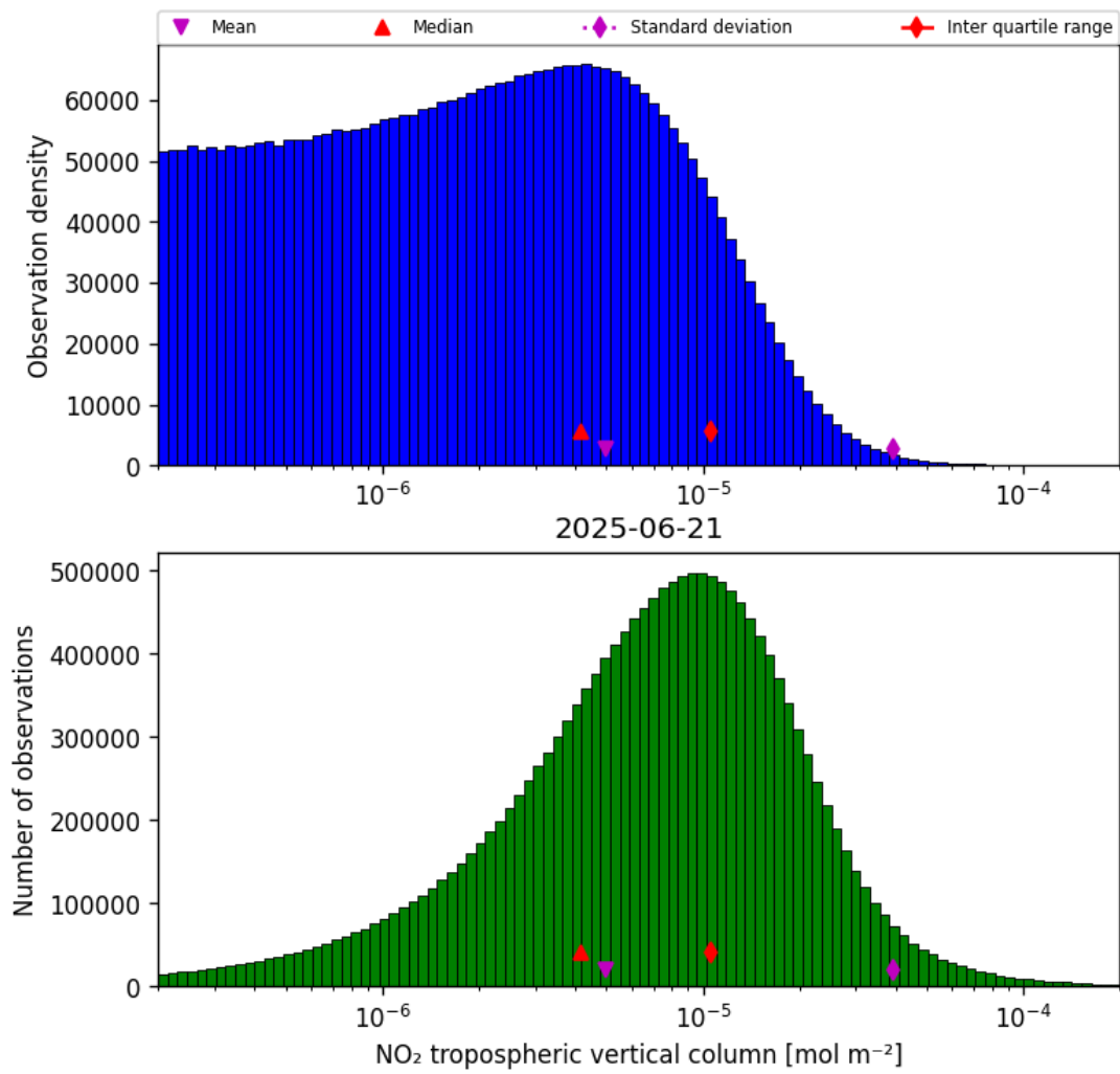
Figure 27: Histogram of “NO 2 tropospheric vertical column” for 2025-06-21 to 2025-06-22
