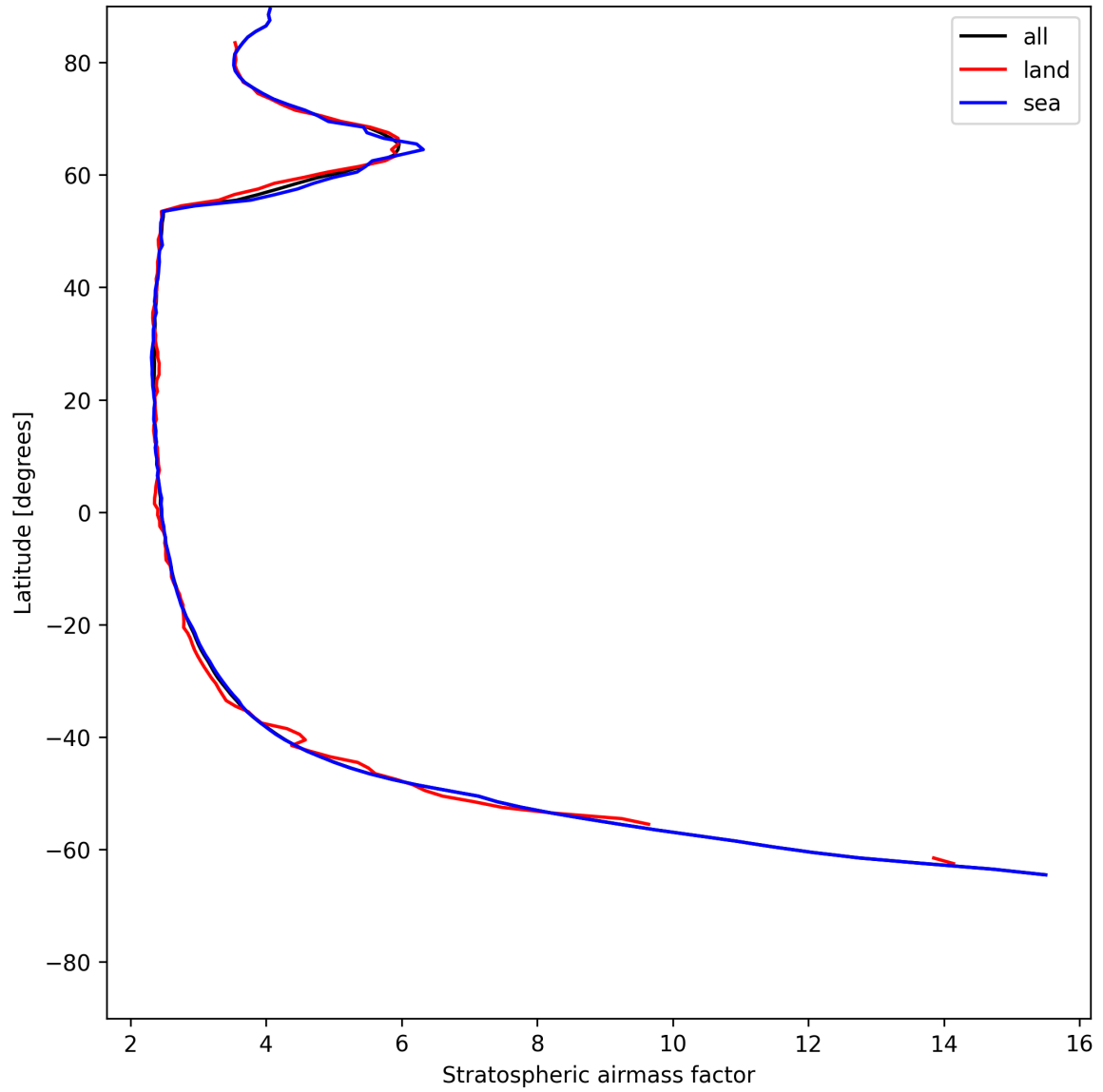
Figure 25: Zonal average of “Stratospheric airmass factor” for 2025-06-21 to 2025-06-22.
