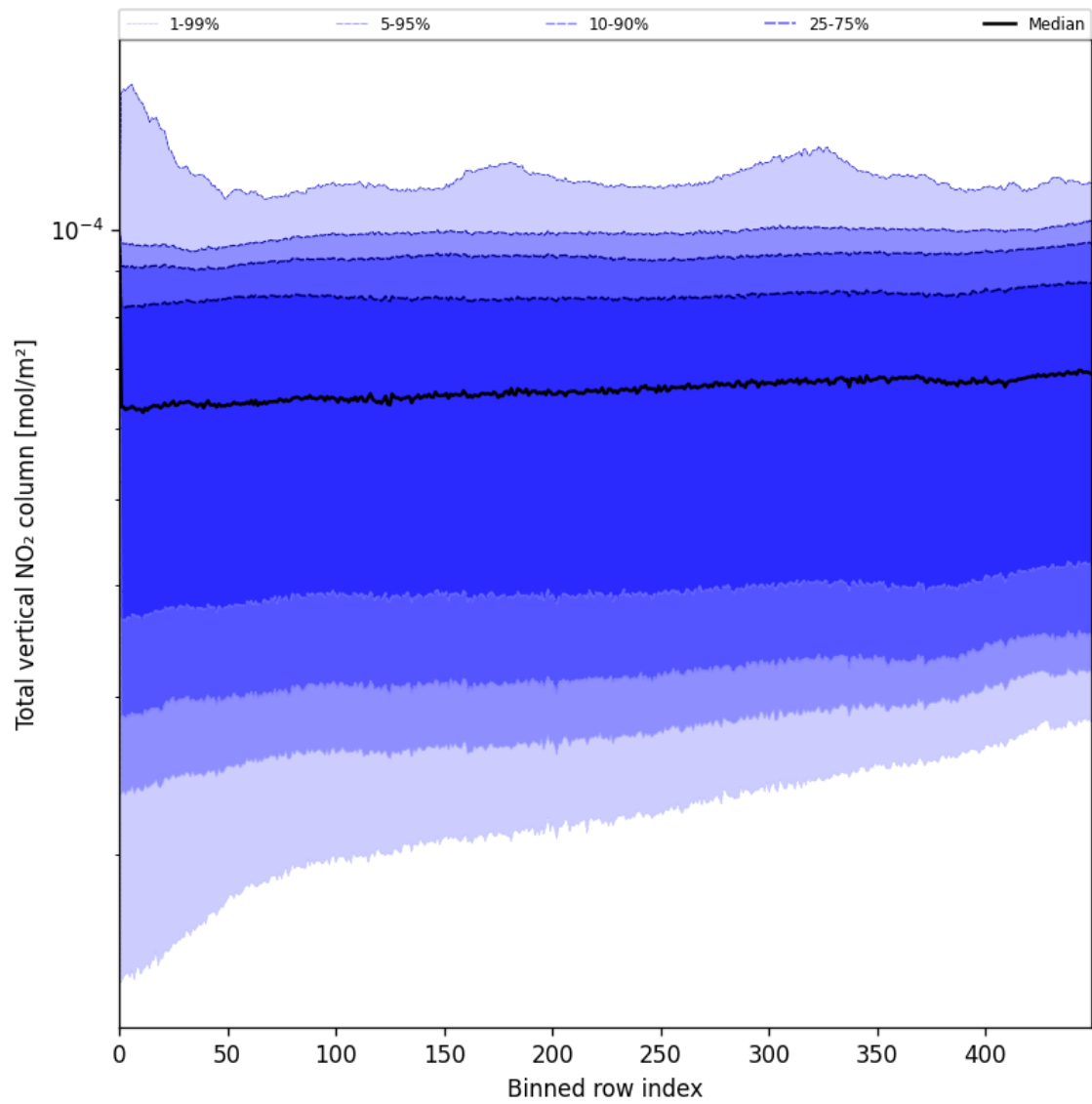
Figure 53: Along track statistics of “Total vertical NO 2 column” for 2025-06-21 to 2025-06-22
