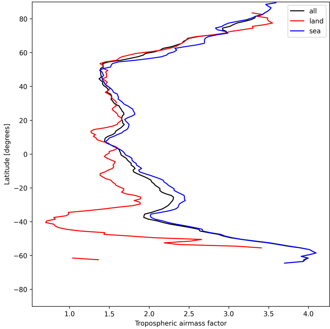
Figure 12: Zonal average of “Tropospheric airmass factor” for 2025-06-21 to 2025-06-22.
