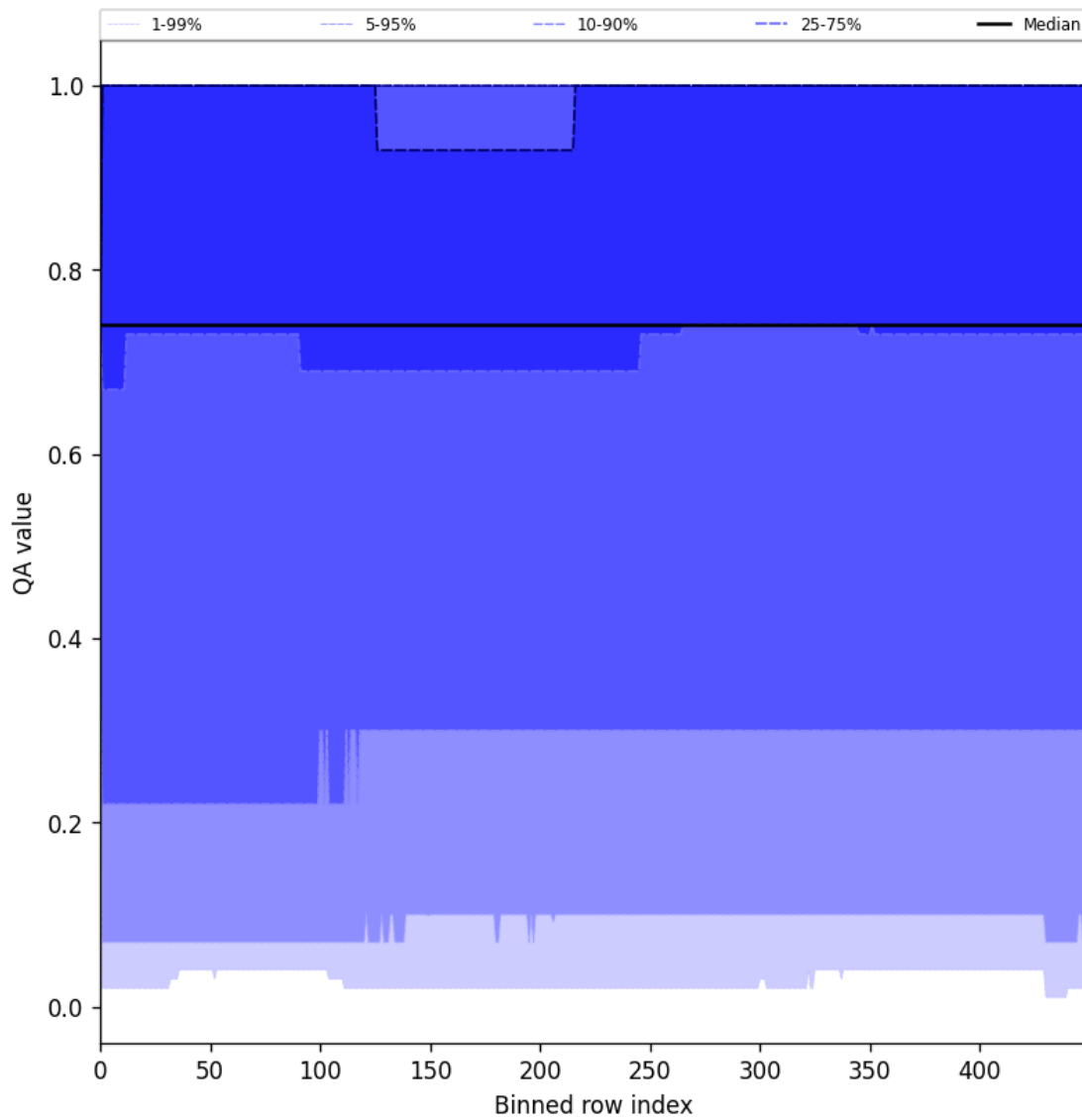
Figure 43: Along track statistics of “QA value” for 2025-06-21 to 2025-06-22
