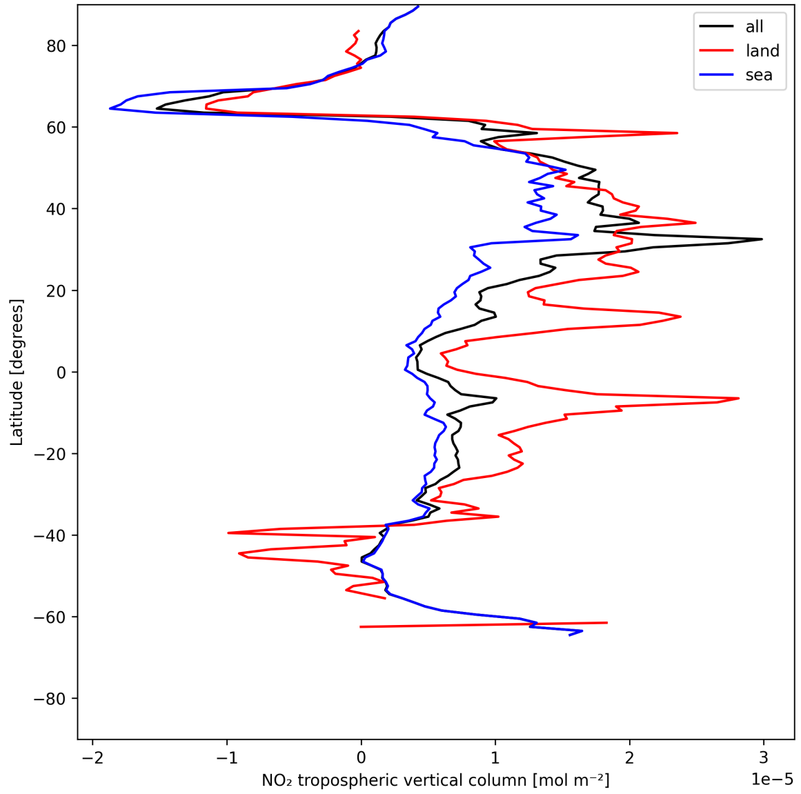
Figure 10: Zonal average of “NO 2 tropospheric vertical column” for 2025-06-21 to 2025-06-22.
