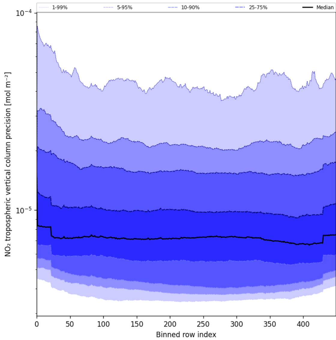
Figure 45: Along track statistics of “NO 2 tropospheric vertical column precision” for 2025-06-21 to 2025-06-22
