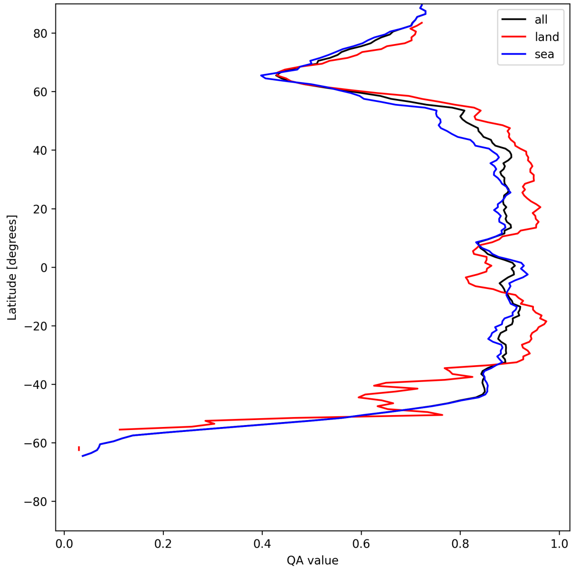
Figure 9: Zonal average of “QA value” for 2025-06-21 to 2025-06-22.
