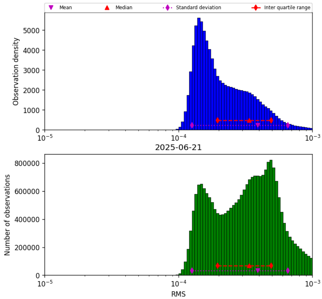
Figure 41: Histogram of “RMS” for 2025-06-21 to 2025-06-22
