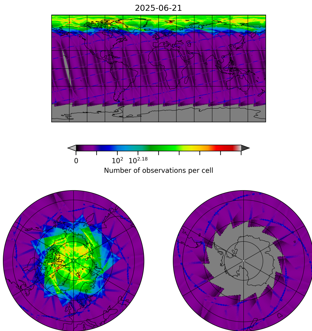
Figure 8: Map of the number of observations for 2025-06-21 to 2025-06-22
