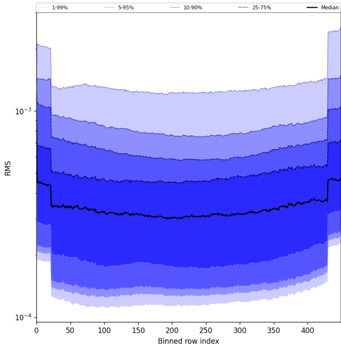
Figure 58: Along track statistics of “RMS” for 2025-06-21 to 2025-06-22
