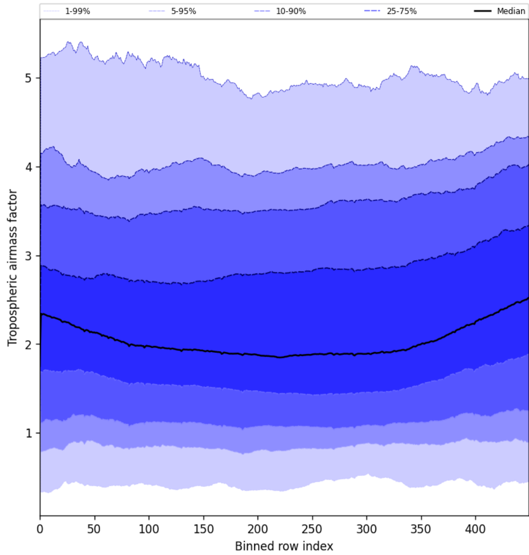
Figure 46: Along track statistics of “Tropospheric airmass factor” for 2025-06-21 to 2025-06-22
