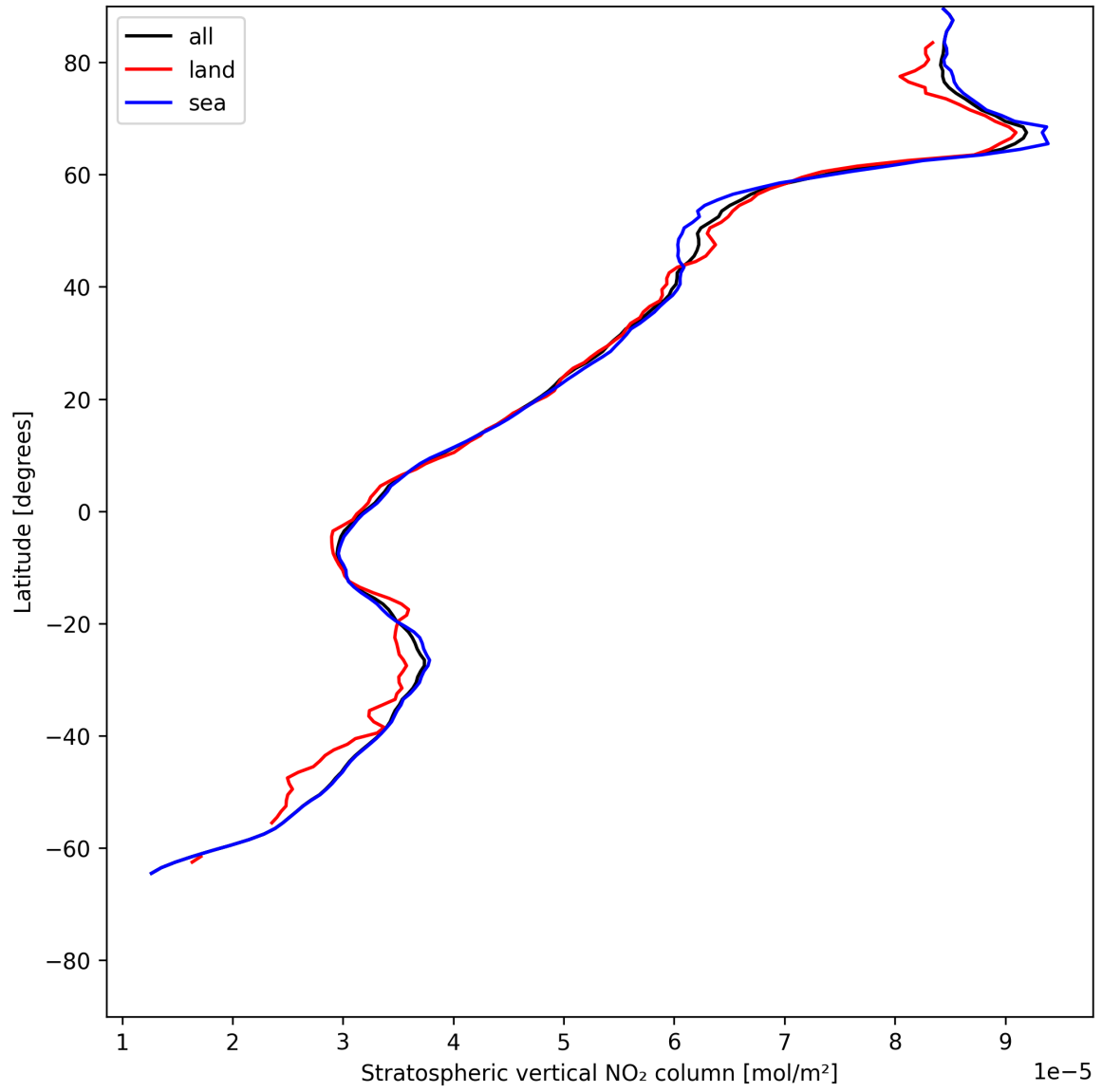
Figure 17: Zonal average of “Stratospheric vertical NO 2 column” for 2025-06-21 to 2025-06-22.
