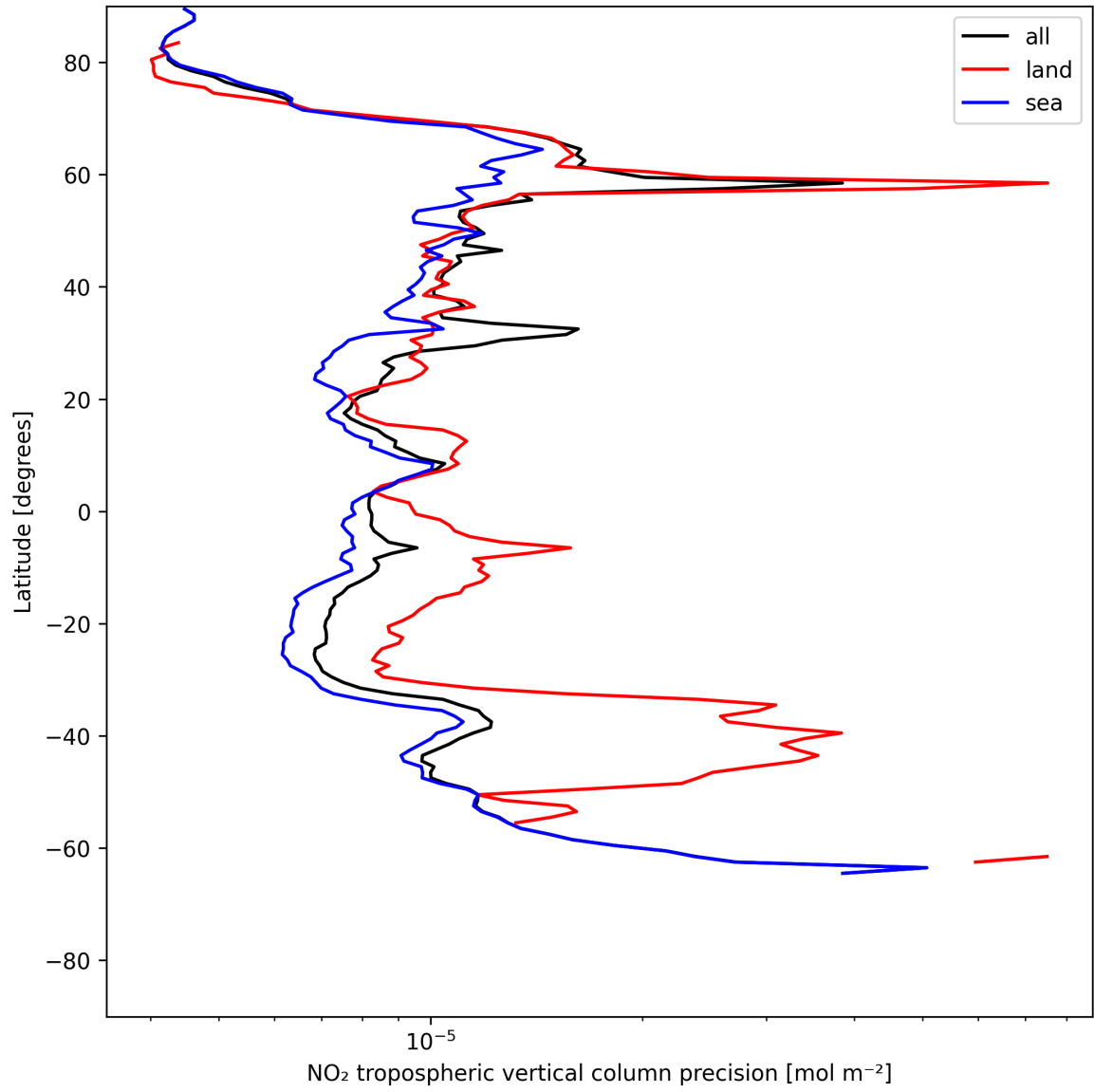
Figure 11: Zonal average of “NO 2 tropospheric vertical column precision” for 2025-06-21 to 2025-06-22.
