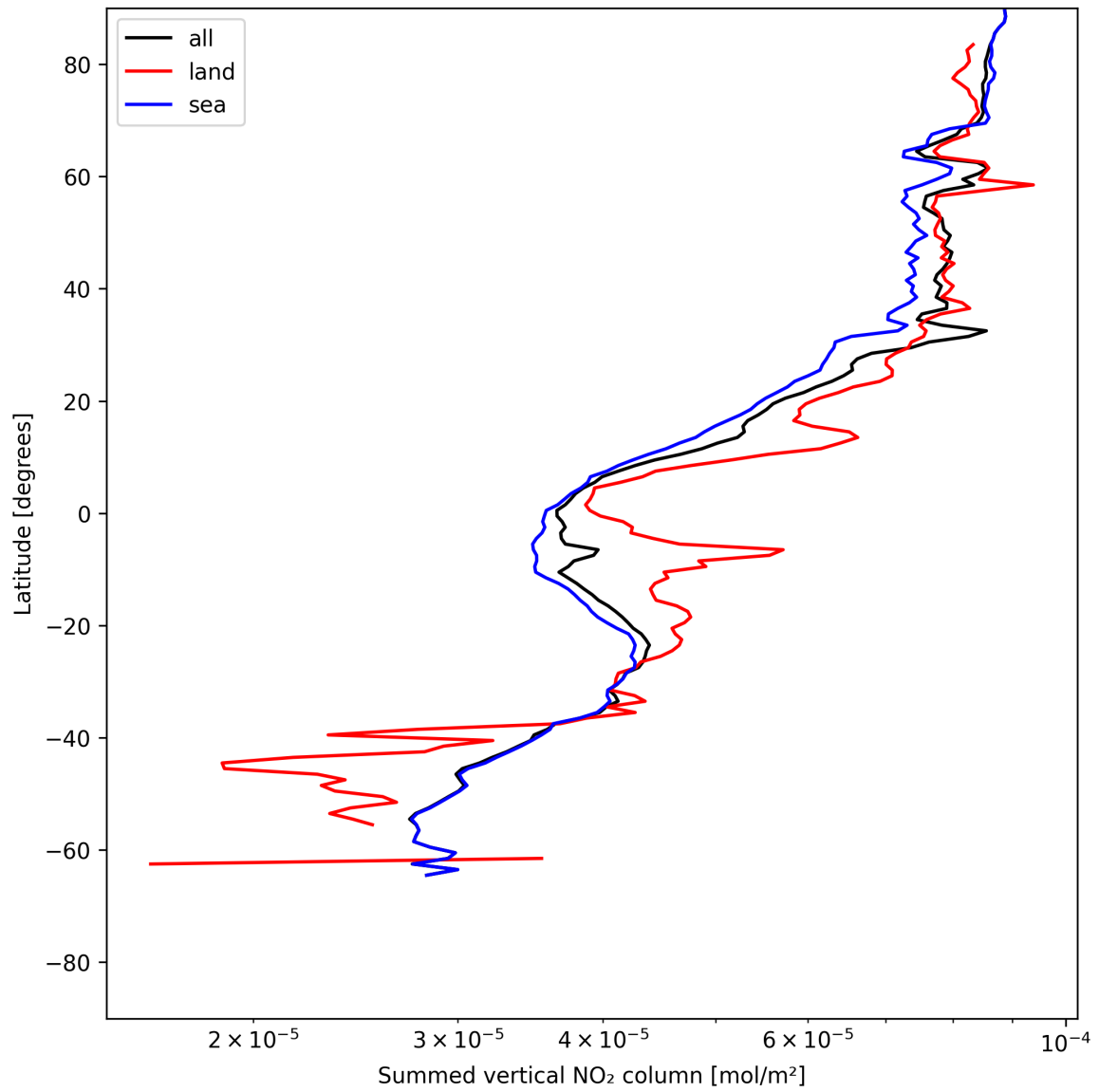
Figure 21: Zonal average of “Summed vertical NO 2 column” for 2025-06-21 to 2025-06-22.
