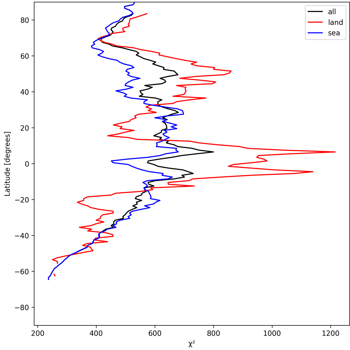
Figure 23: Zonal average of “ \chi^2 ” for 2025-06-21 to 2025-06-22.
