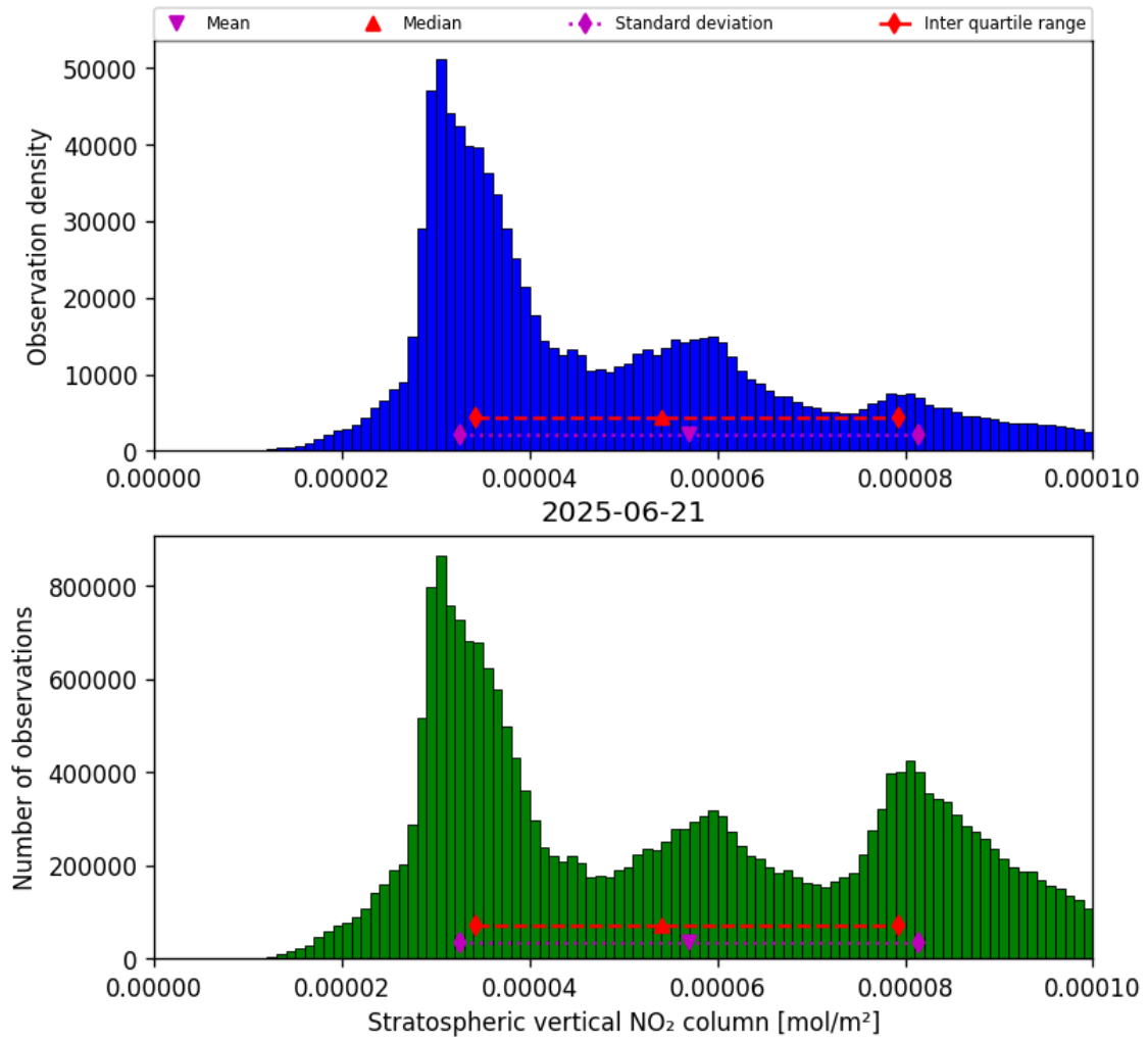
Figure 34: Histogram of “Stratospheric vertical NO 2 column” for 2025-06-21 to 2025-06-22
