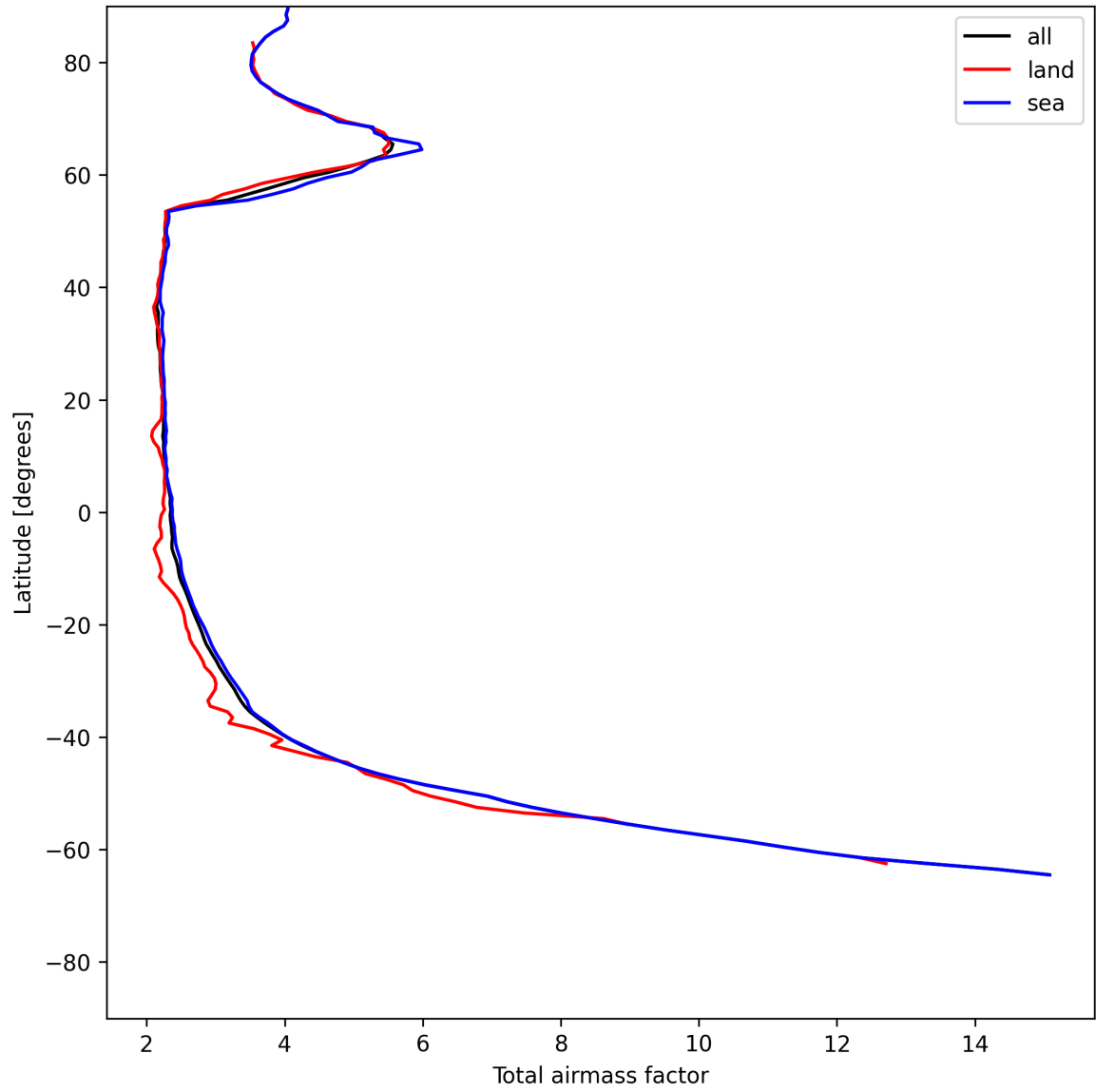
Figure 13: Zonal average of “Total airmass factor” for 2025-06-21 to 2025-06-22.
