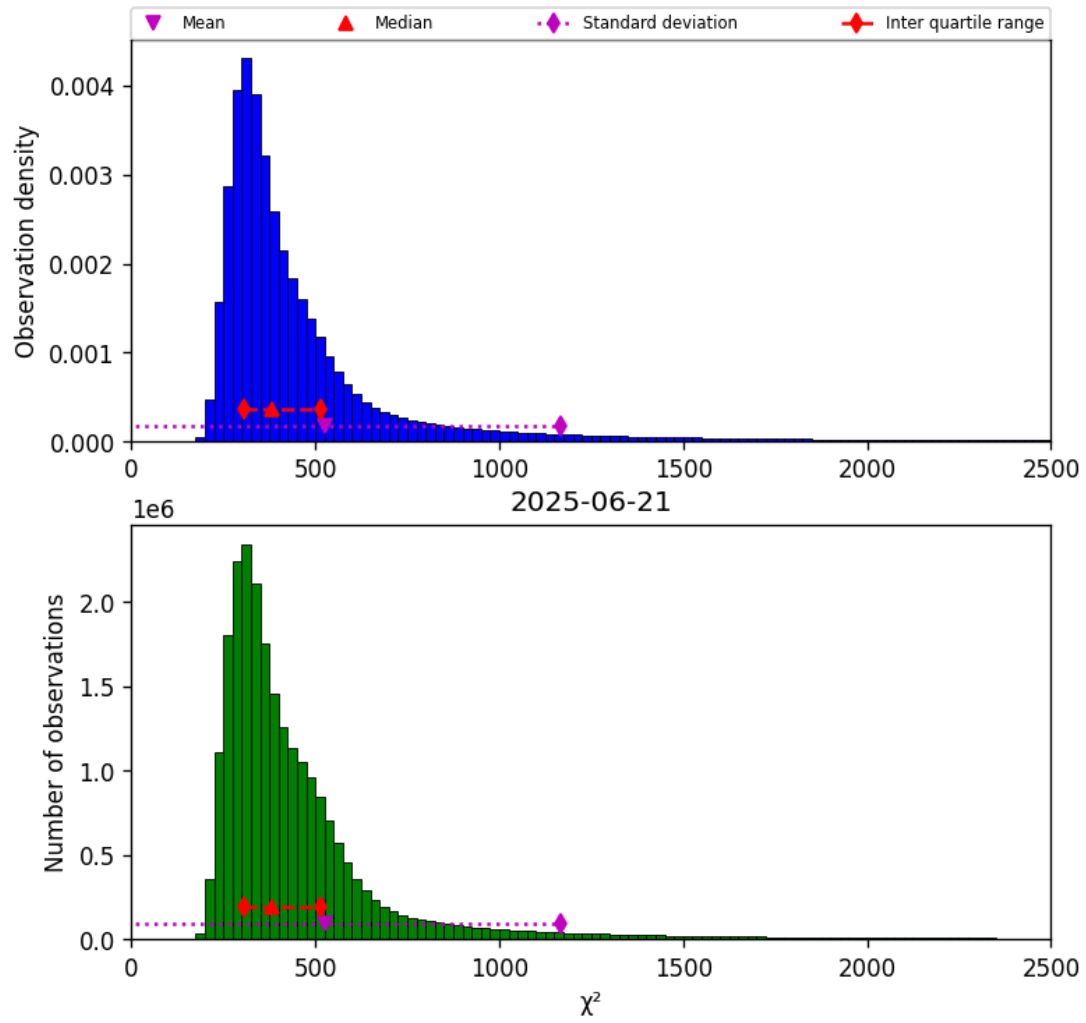
Figure 40: Histogram of “ \chi^2 ” for 2025-06-21 to 2025-06-22
