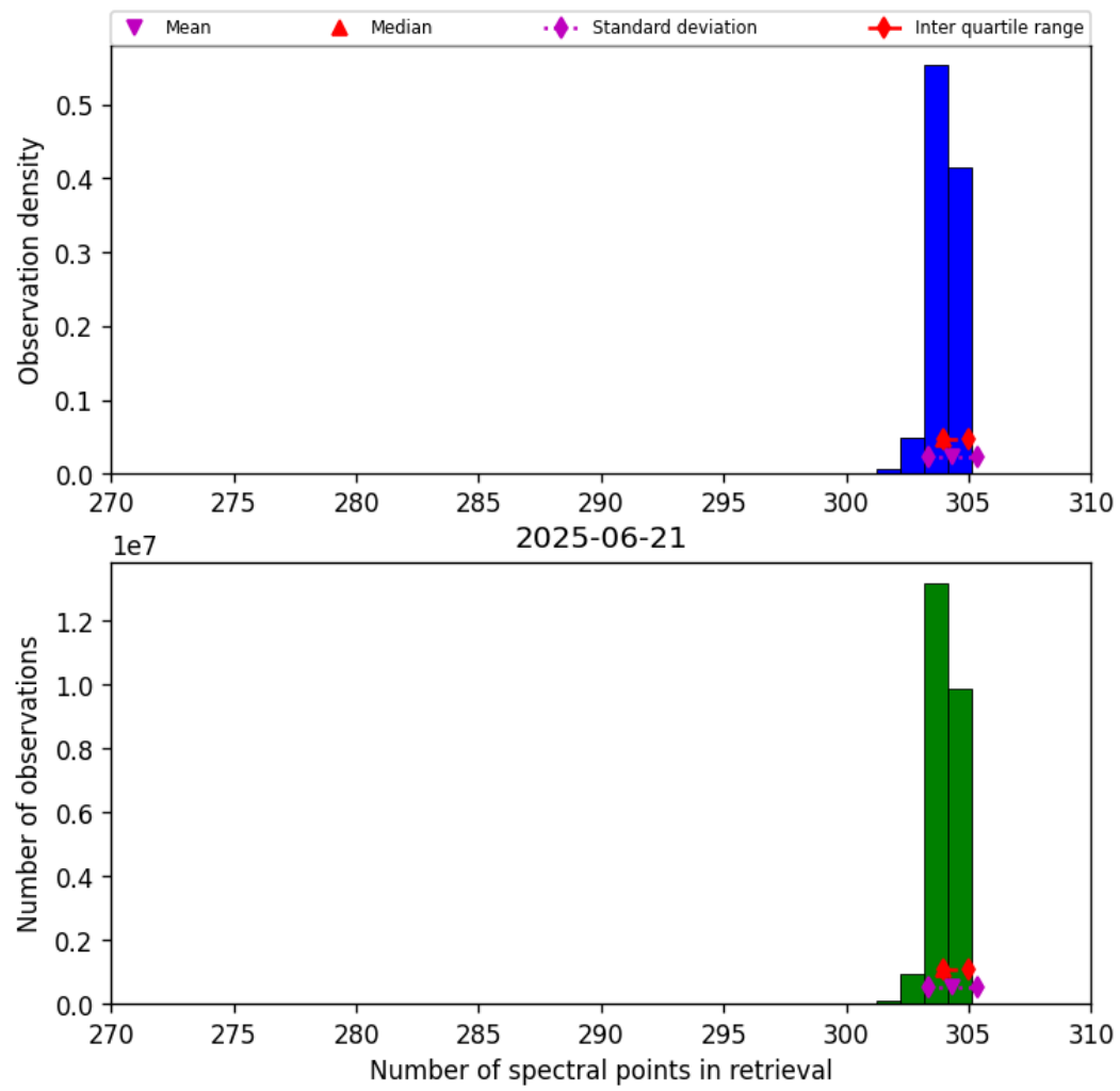
Figure 31: Histogram of “Number of spectral points in retrieval” for 2025-06-21 to 2025-06-22
