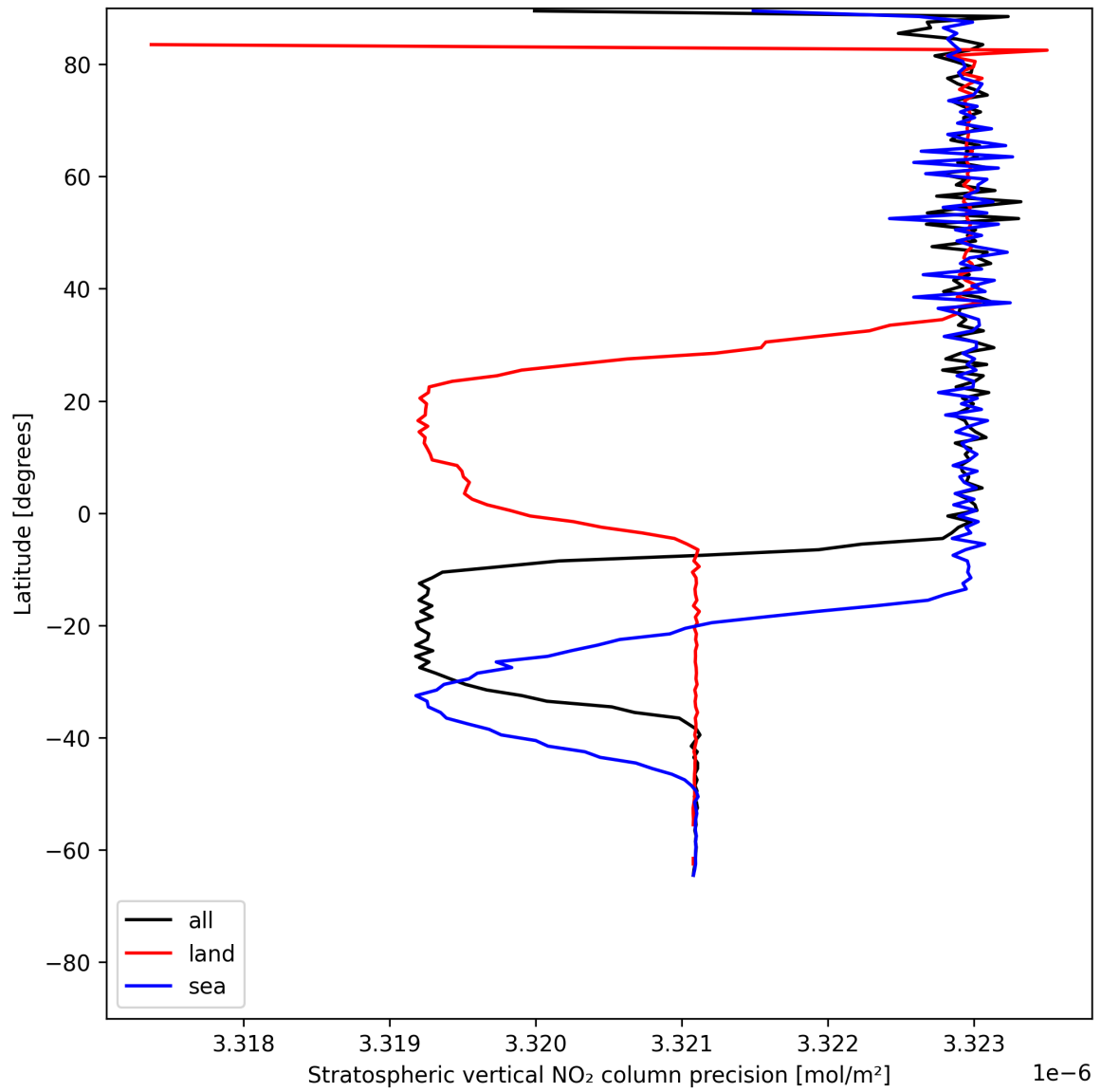
Figure 18: Zonal average of “Stratospheric vertical NO 2 column precision” for 2025-06-21 to 2025-06-22.
