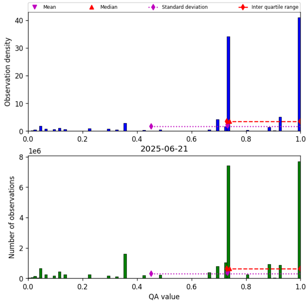
Figure 26: Histogram of “QA value” for 2025-06-21 to 2025-06-22
