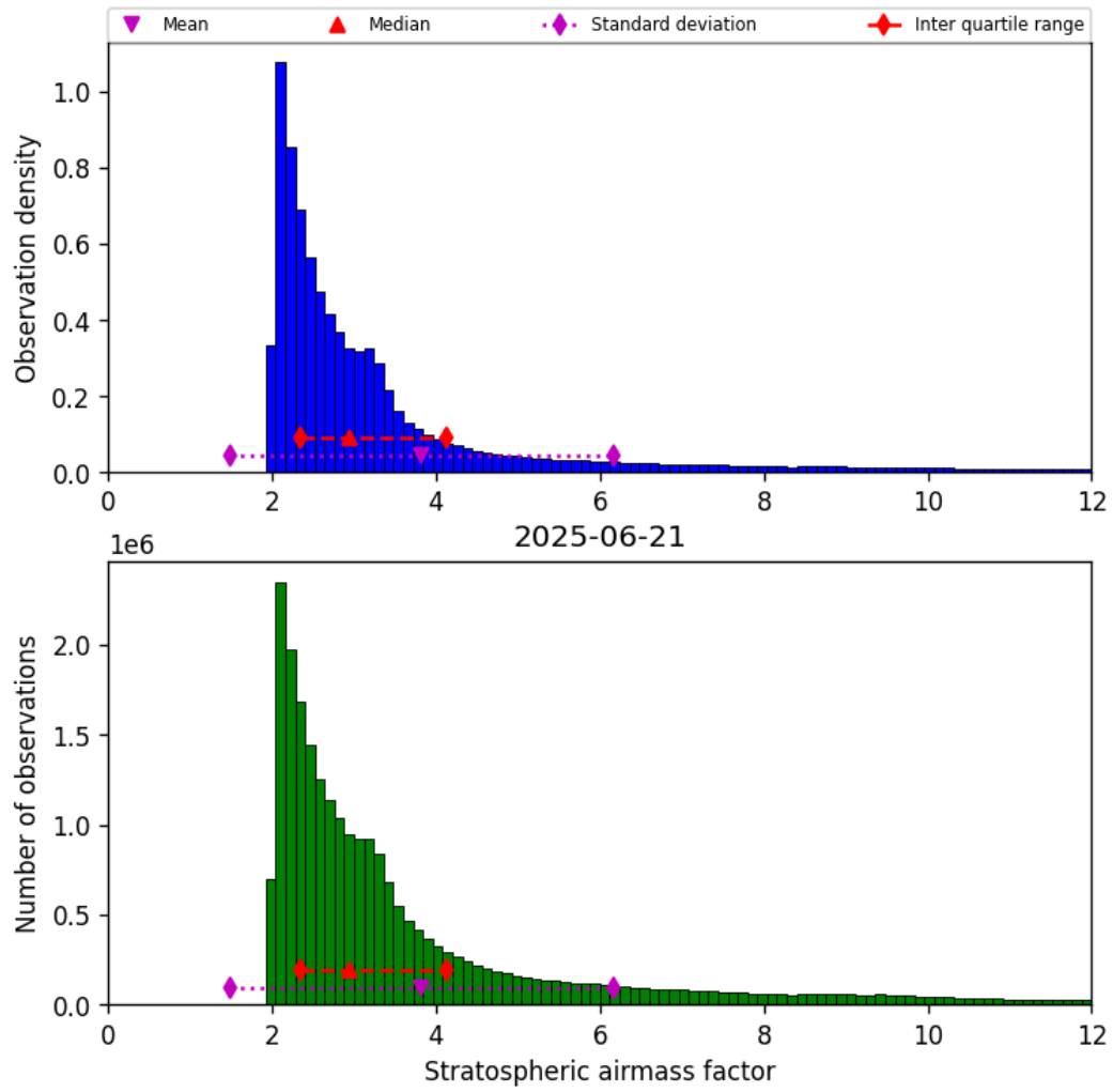
Figure 42: Histogram of “Stratospheric airmass factor” for 2025-06-21 to 2025-06-22
