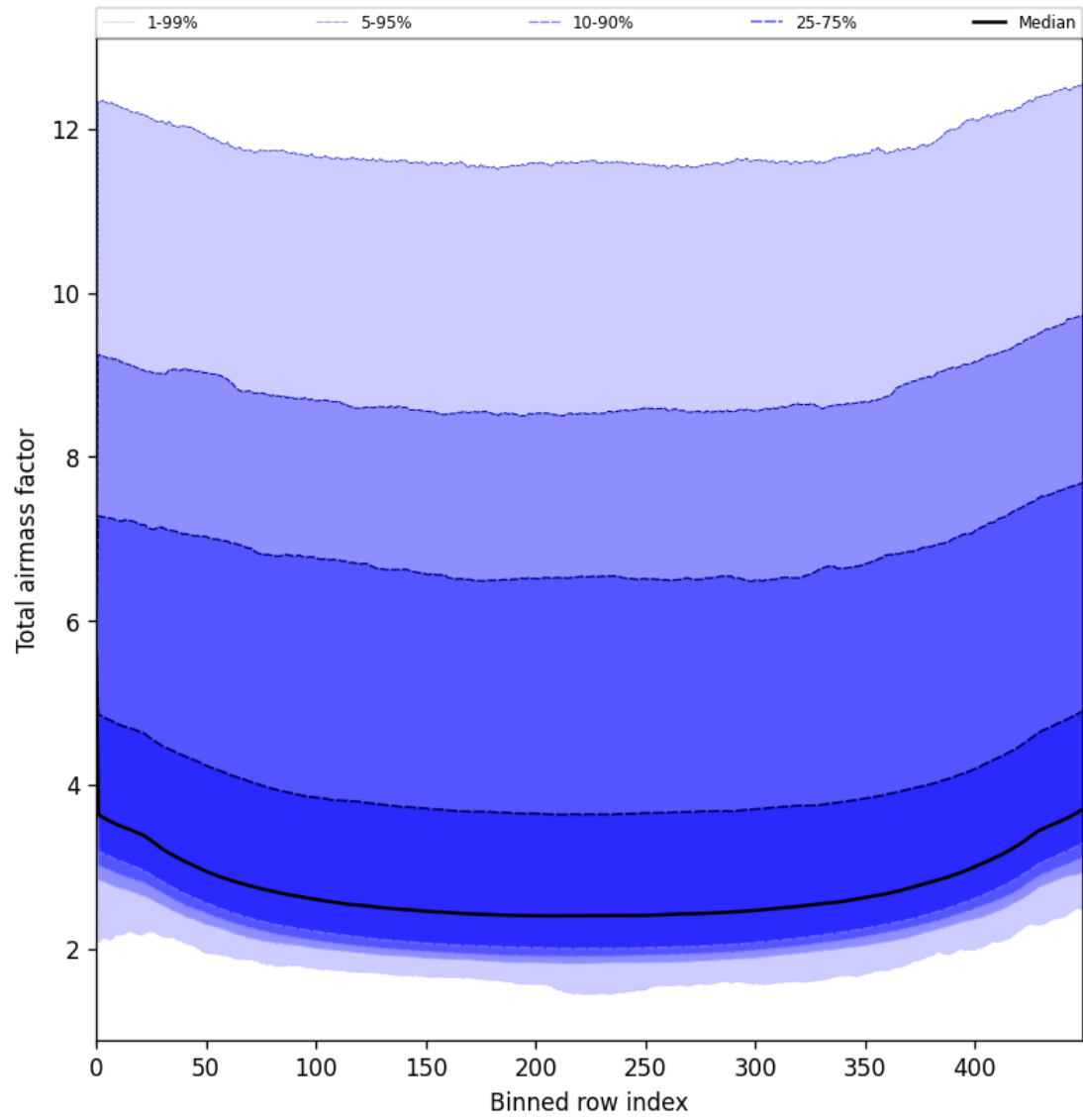
Figure 47: Along track statistics of “Total airmass factor” for 2025-06-21 to 2025-06-22
