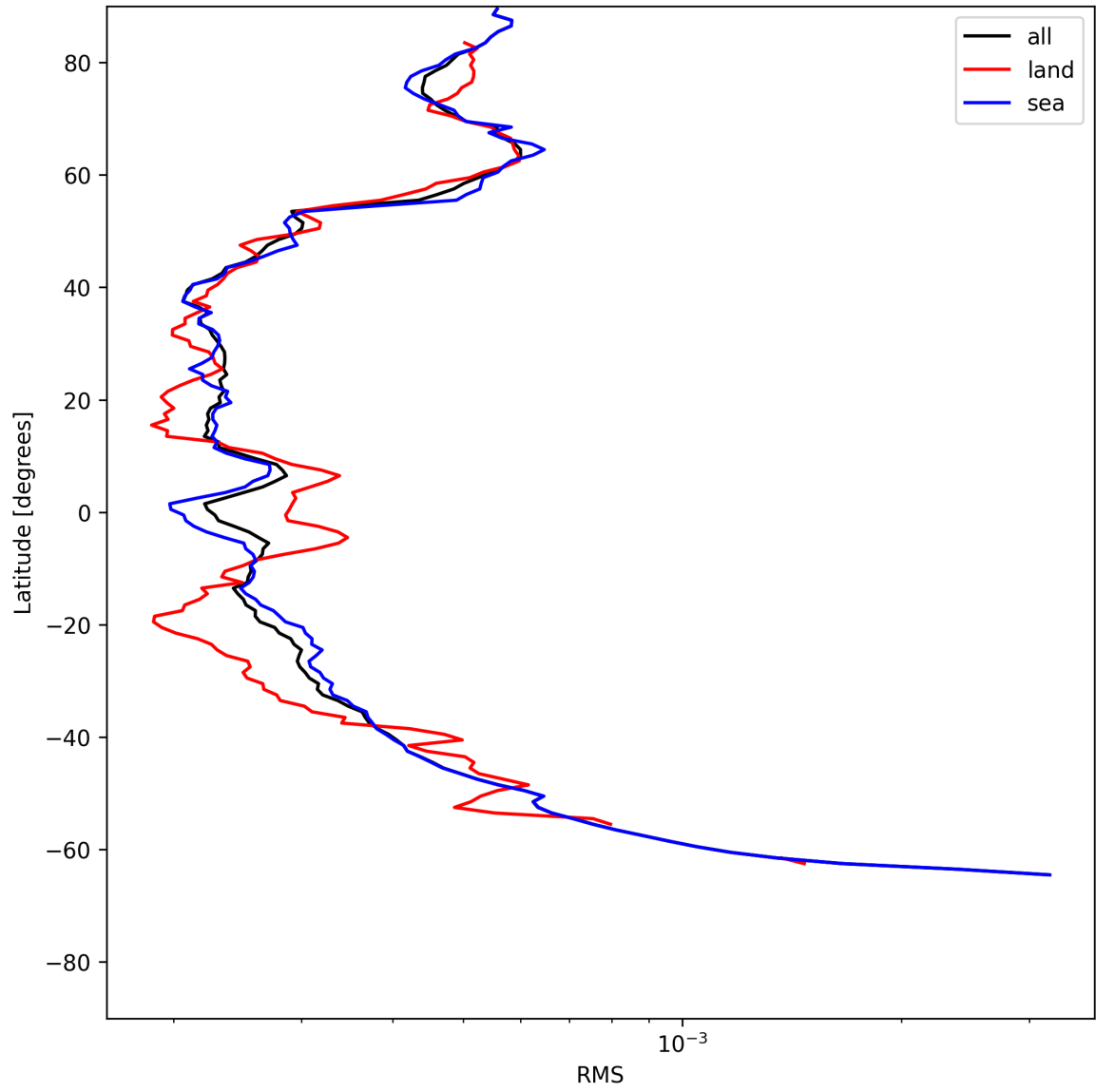
Figure 24: Zonal average of “RMS” for 2025-06-21 to 2025-06-22.
