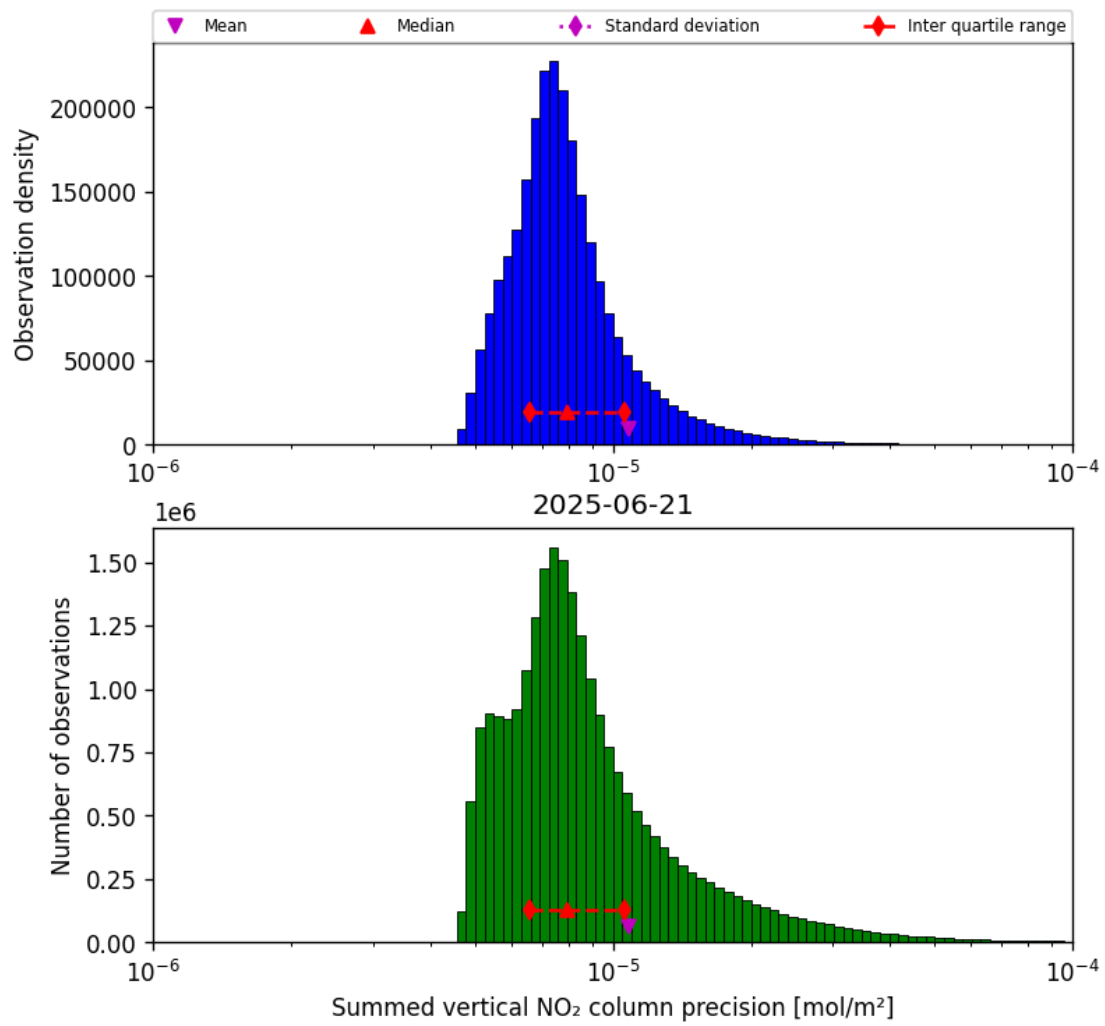
Figure 39: Histogram of "Summed vertical NO 2 column precision" for 2025-06-21 to 2025-06-22
