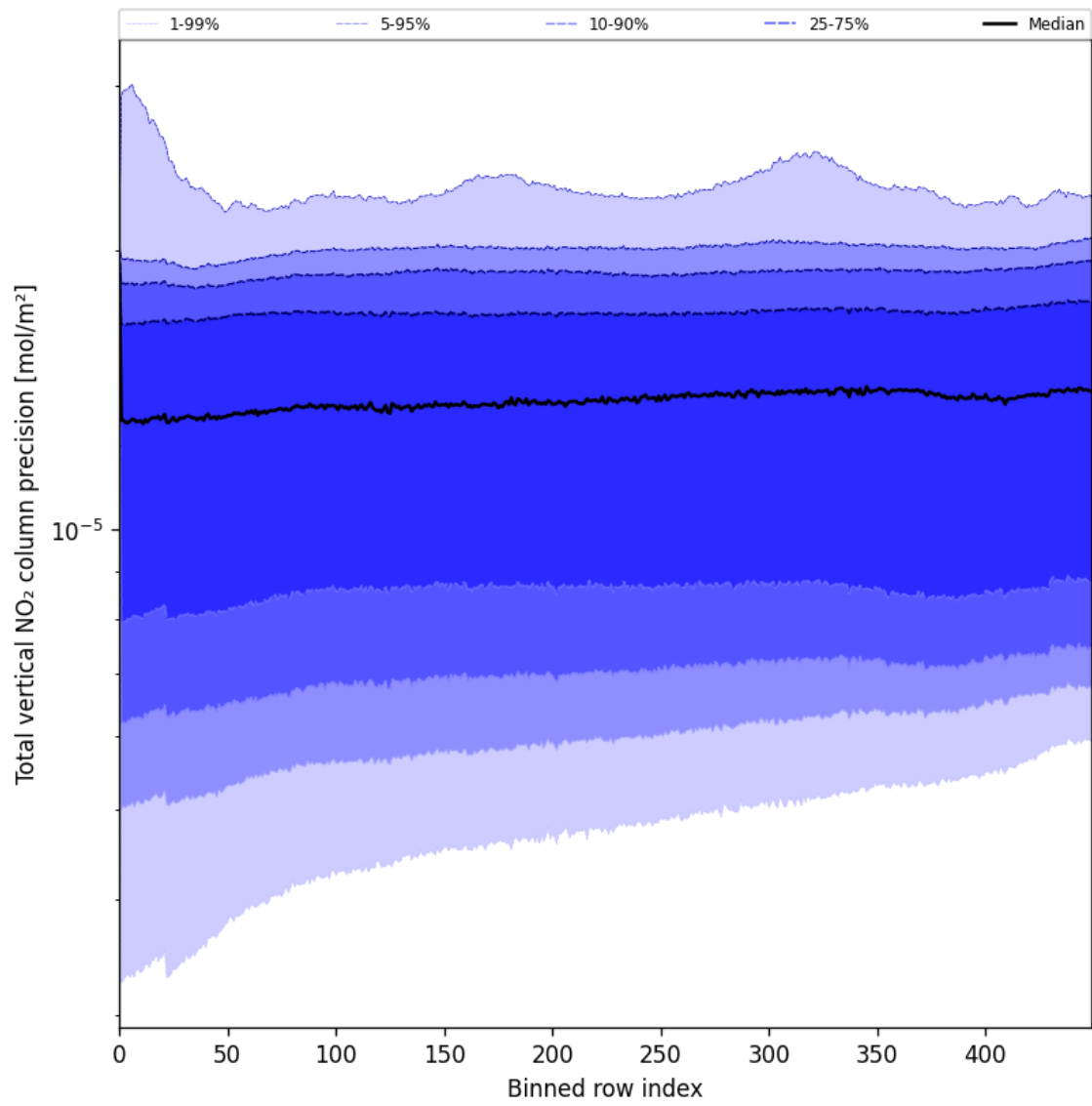
Figure 54: Along track statistics of “Total vertical NO 2 column precision” for 2025-06-21 to 2025-06-22
