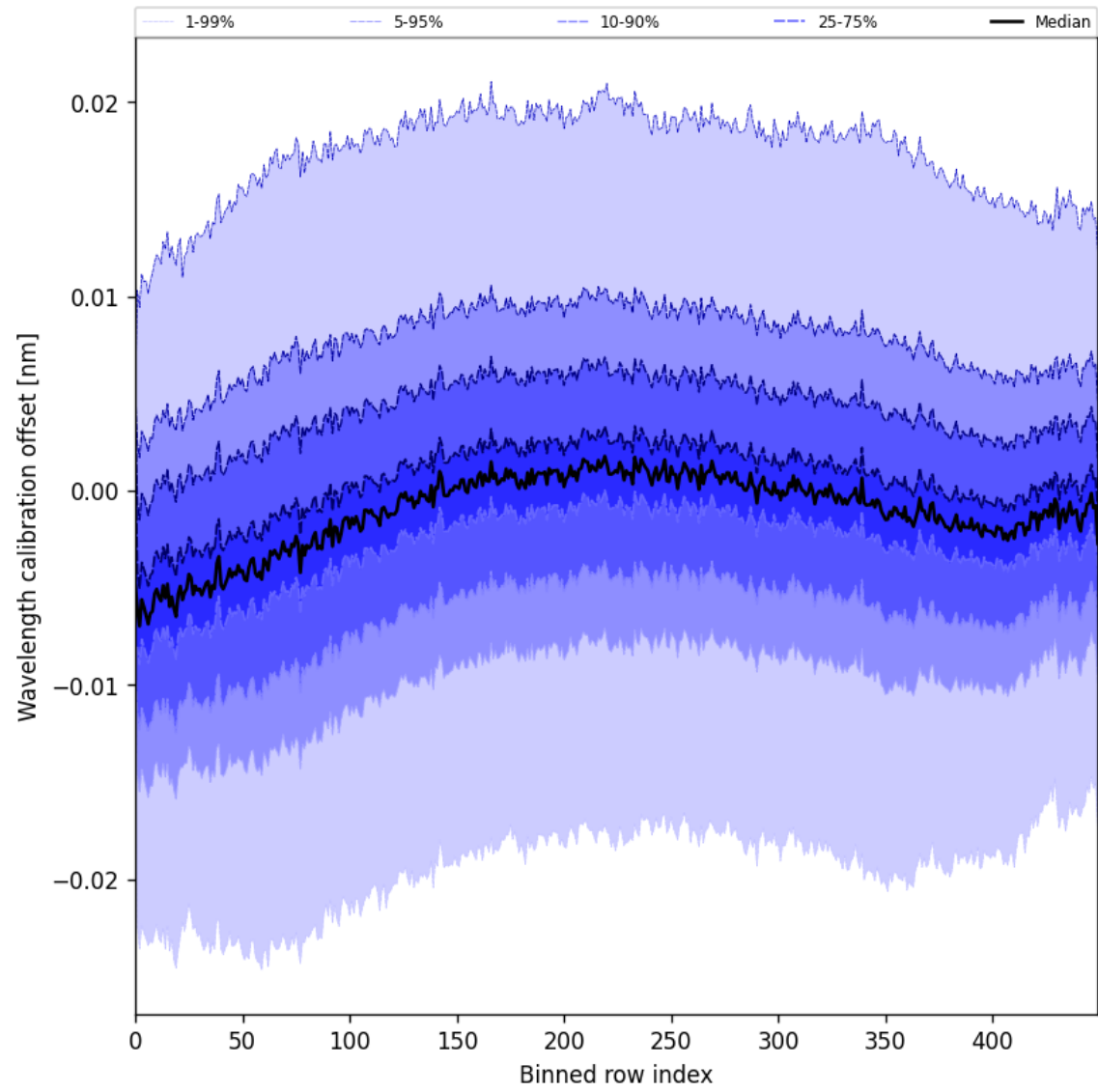
Figure 50: Along track statistics of “Wavelength calibration offset” for 2025-06-21 to 2025-06-22
