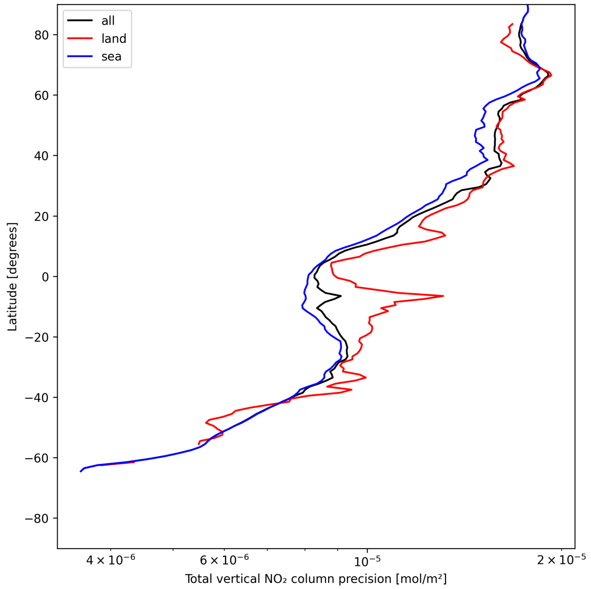
Figure 20: Zonal average of “Total vertical NO 2 column precision” for 2025-06-21 to 2025-06-22.
