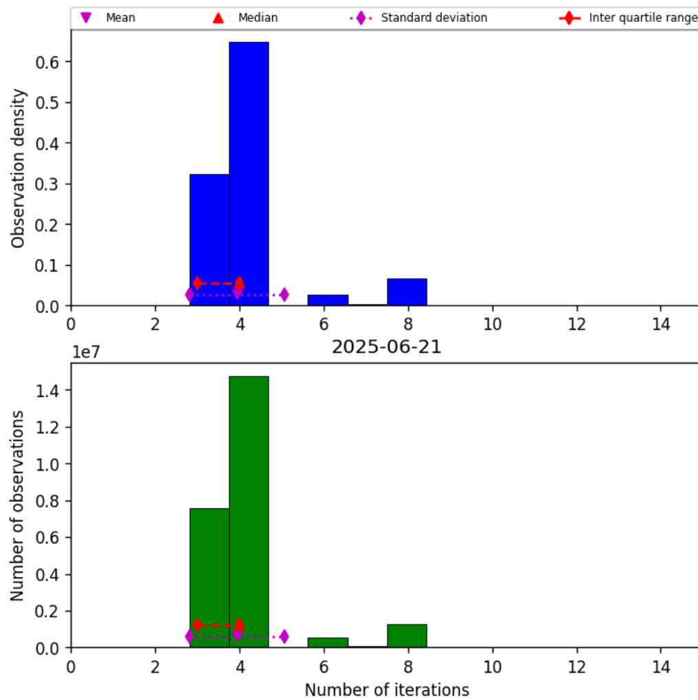
Figure 32: Histogram of “Number of iterations” for 2025-06-21 to 2025-06-22
