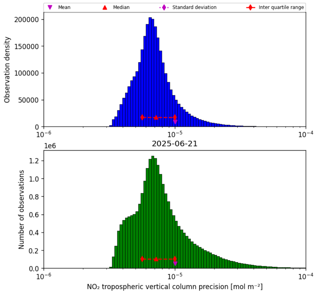
Figure 28: Histogram of “NO 2 tropospheric vertical column precision” for 2025-06-21 to 2025-06-22
