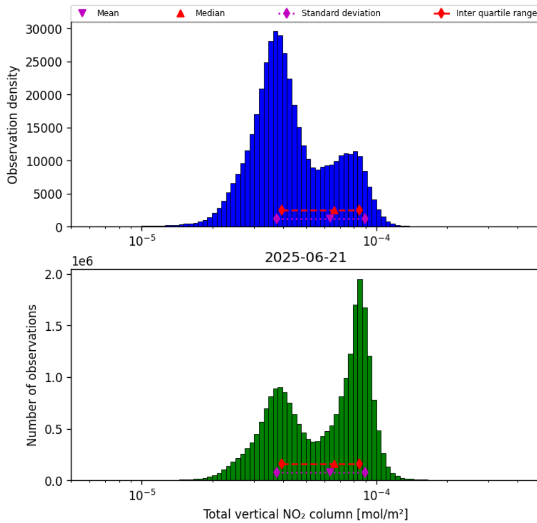
Figure 36: Histogram of “Total vertical NO 2 column” for 2025-06-21 to 2025-06-22
