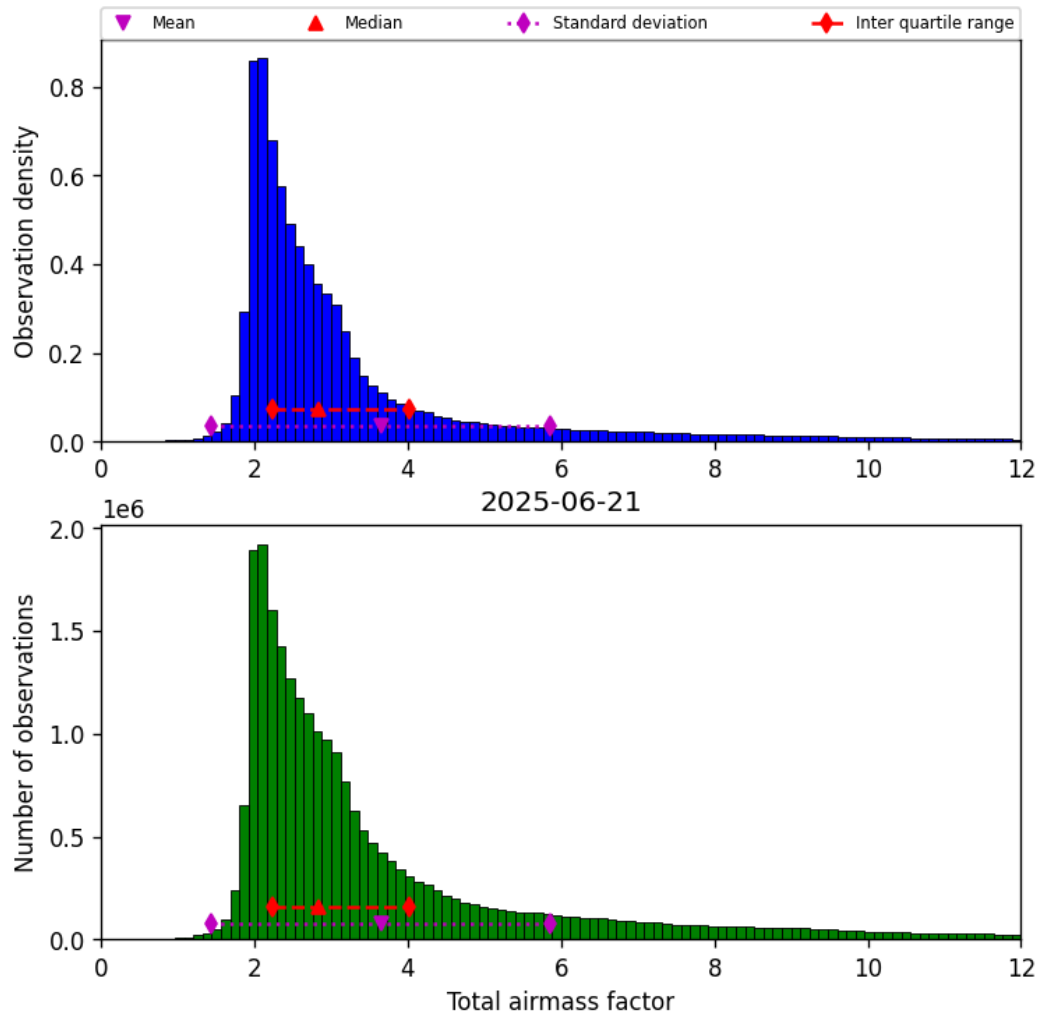
Figure 30: Histogram of “Total airmass factor” for 2025-06-21 to 2025-06-22
