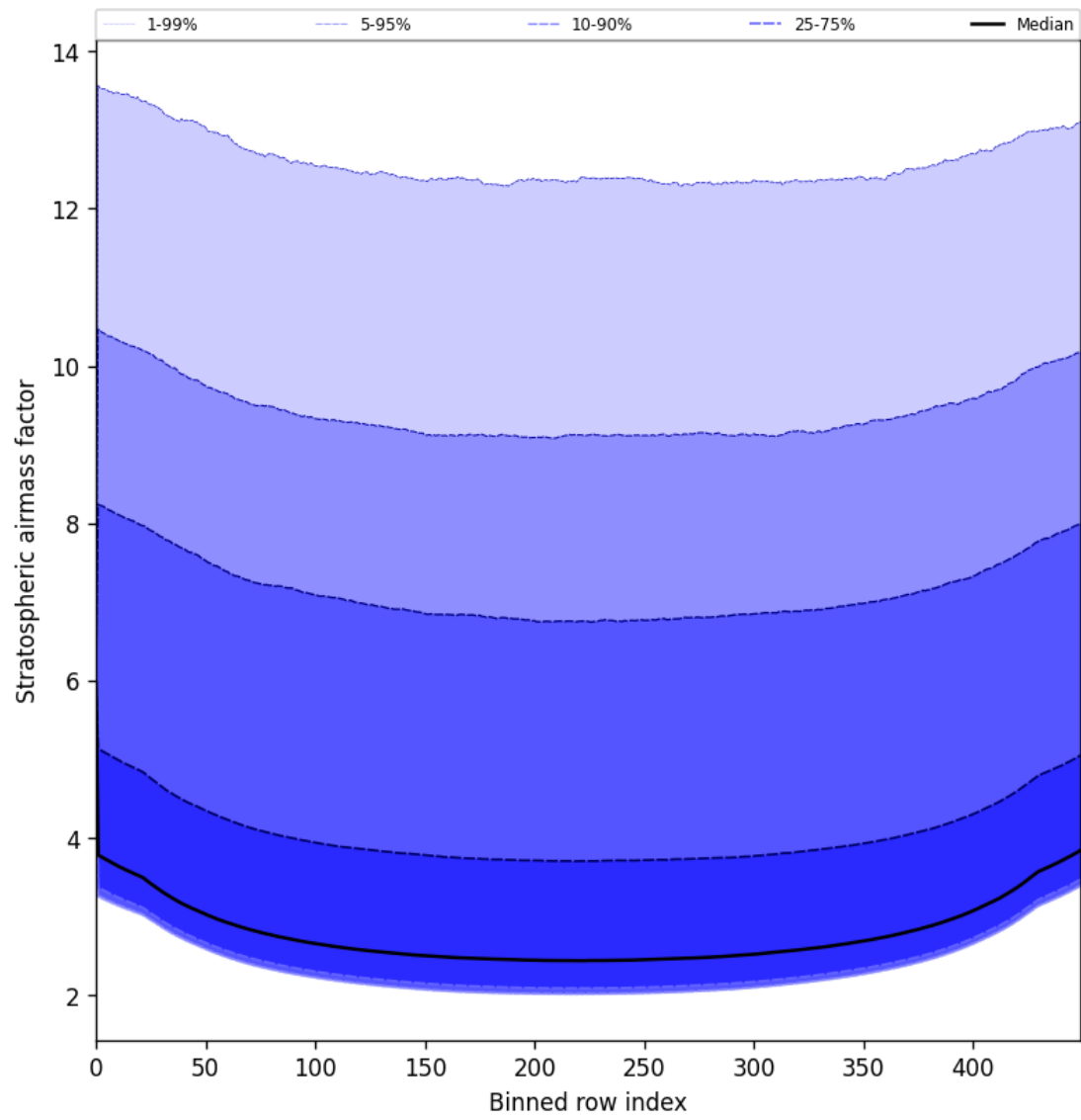
Figure 59: Along track statistics of “Stratospheric airmass factor” for 2025-06-21 to 2025-06-22
