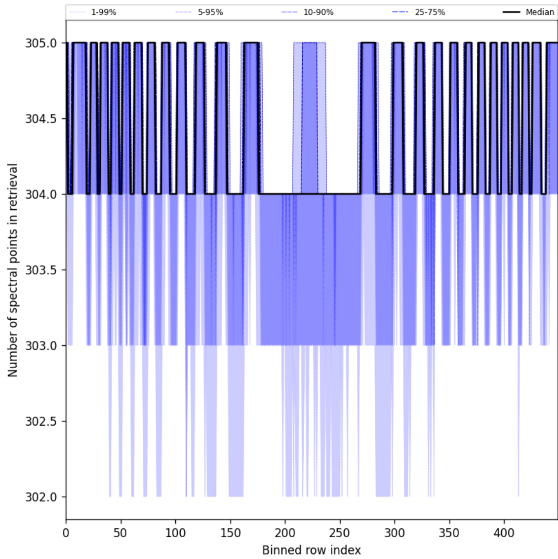
Figure 48: Along track statistics of “Number of spectral points in retrieval” for 2025-06-21 to 2025-06-22
