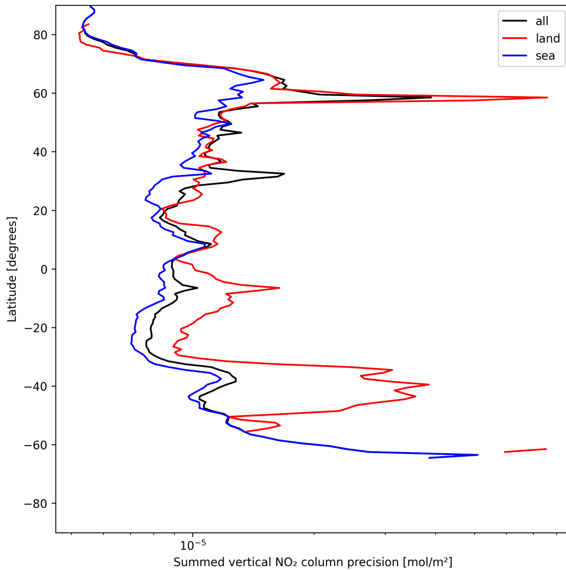
Figure 22: Zonal average of “Summed vertical NO 2 column precision” for 2025-06-21 to 2025-06-22.
