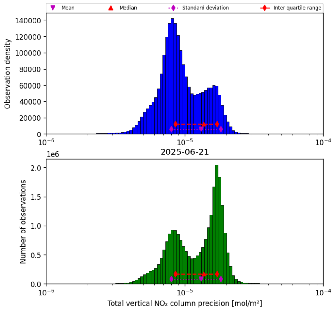
Figure 37: Histogram of “Total vertical NO 2 column precision” for 2025-06-21 to 2025-06-22
