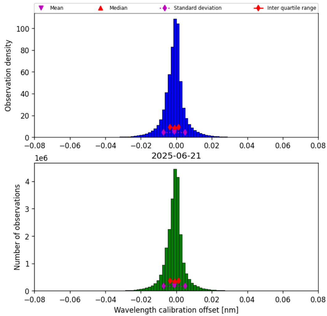
Figure 33: Histogram of “Wavelength calibration offset” for 2025-06-21 to 2025-06-22
