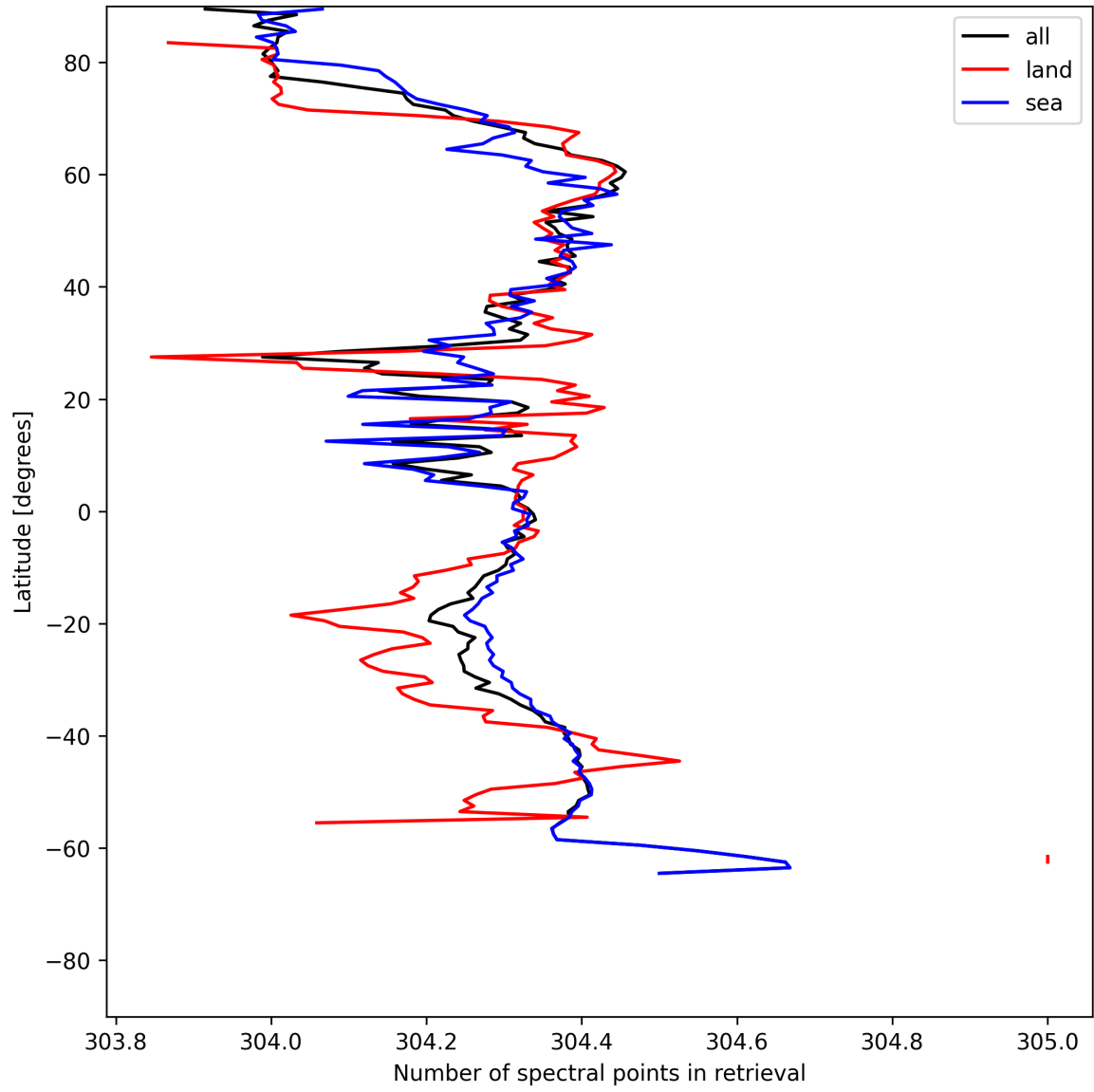
Figure 14: Zonal average of “Number of spectral points in retrieval” for 2025-06-21 to 2025-06-22.
