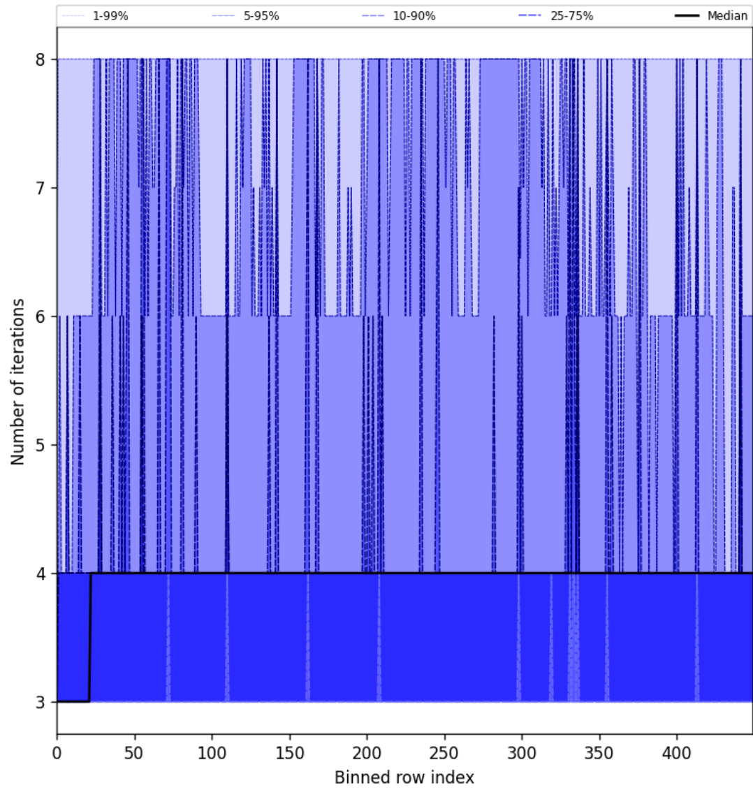
Figure 49: Along track statistics of “Number of iterations” for 2025-06-21 to 2025-06-22
