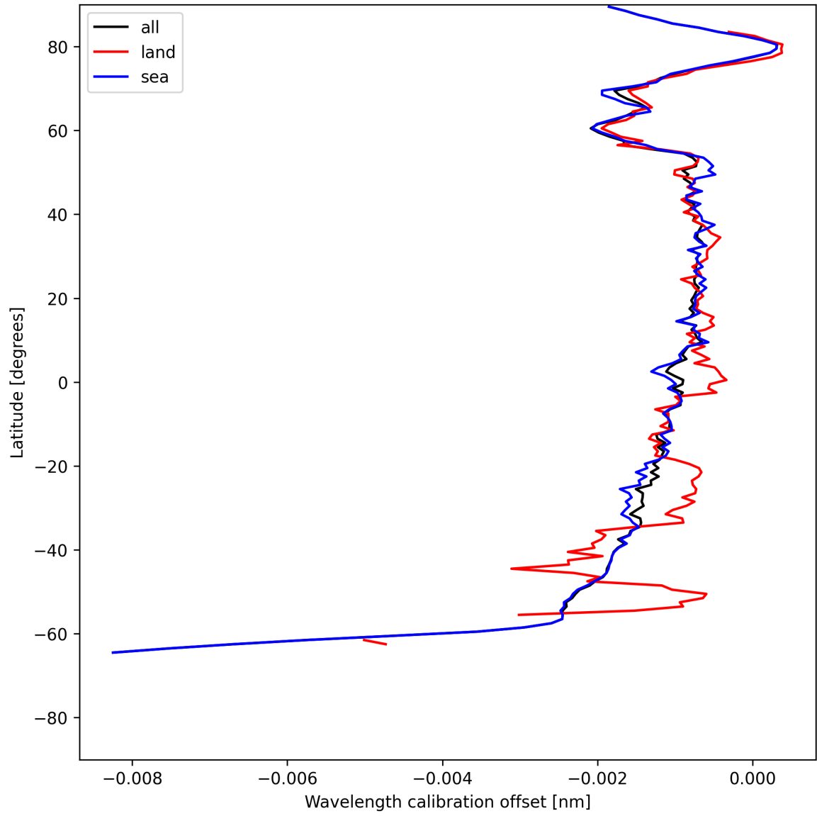
Figure 16: Zonal average of “Wavelength calibration offset” for 2025-06-21 to 2025-06-22.
