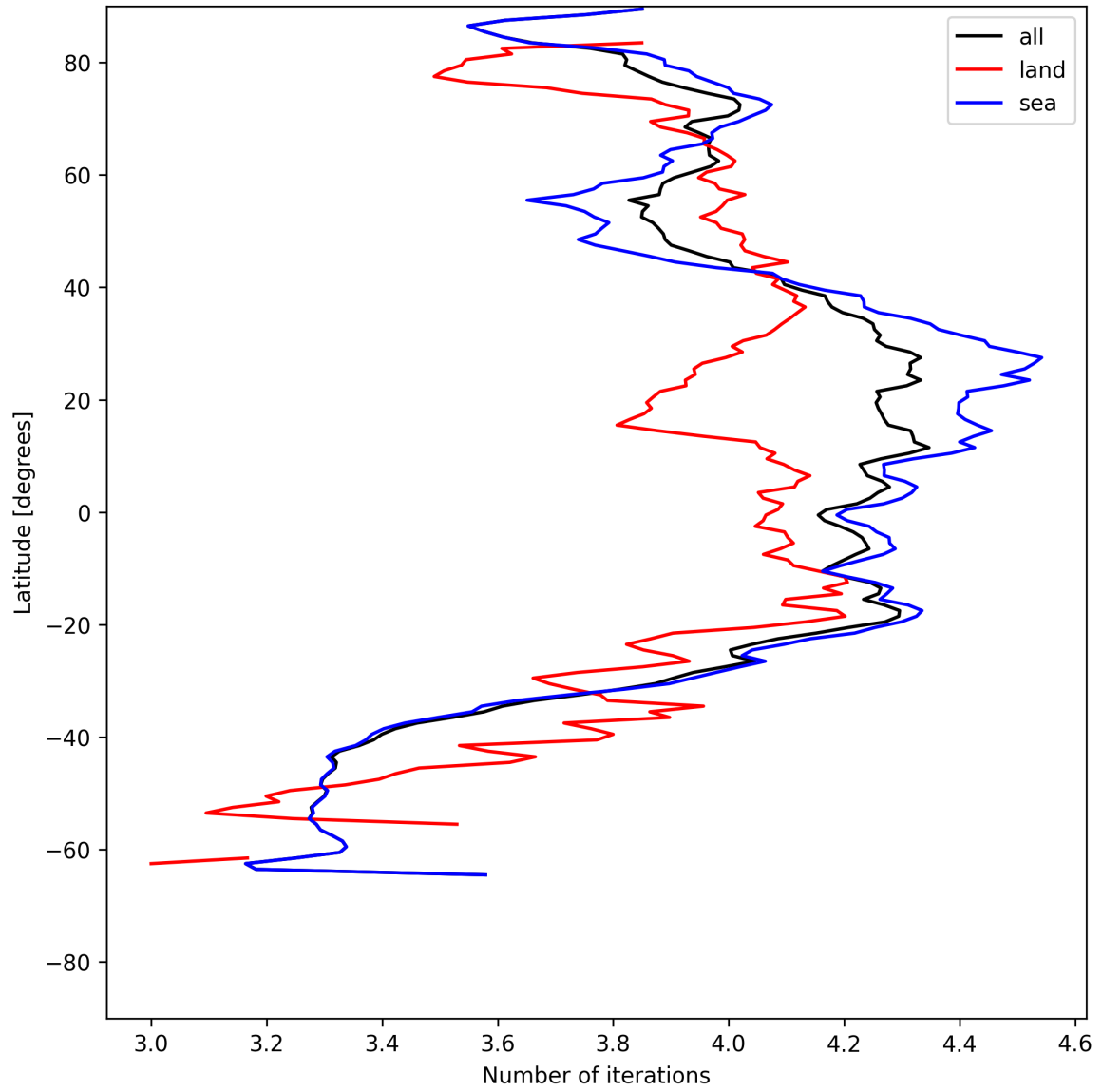
Figure 15: Zonal average of “Number of iterations” for 2025-06-21 to 2025-06-22.
