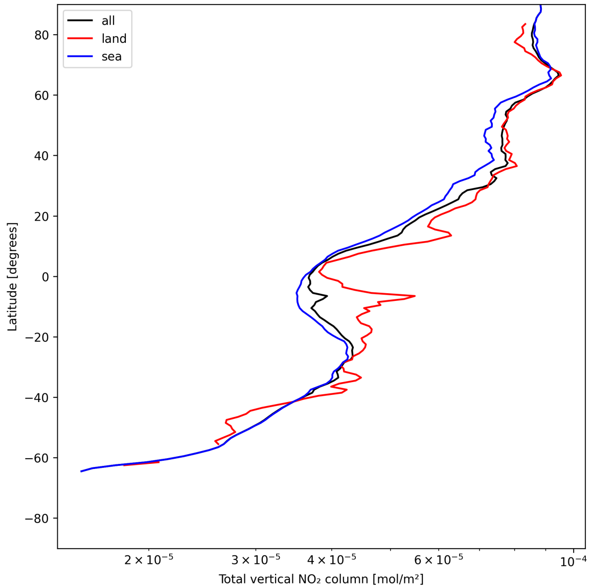
Figure 19: Zonal average of “Total vertical NO 2 column” for 2025-06-21 to 2025-06-22.
