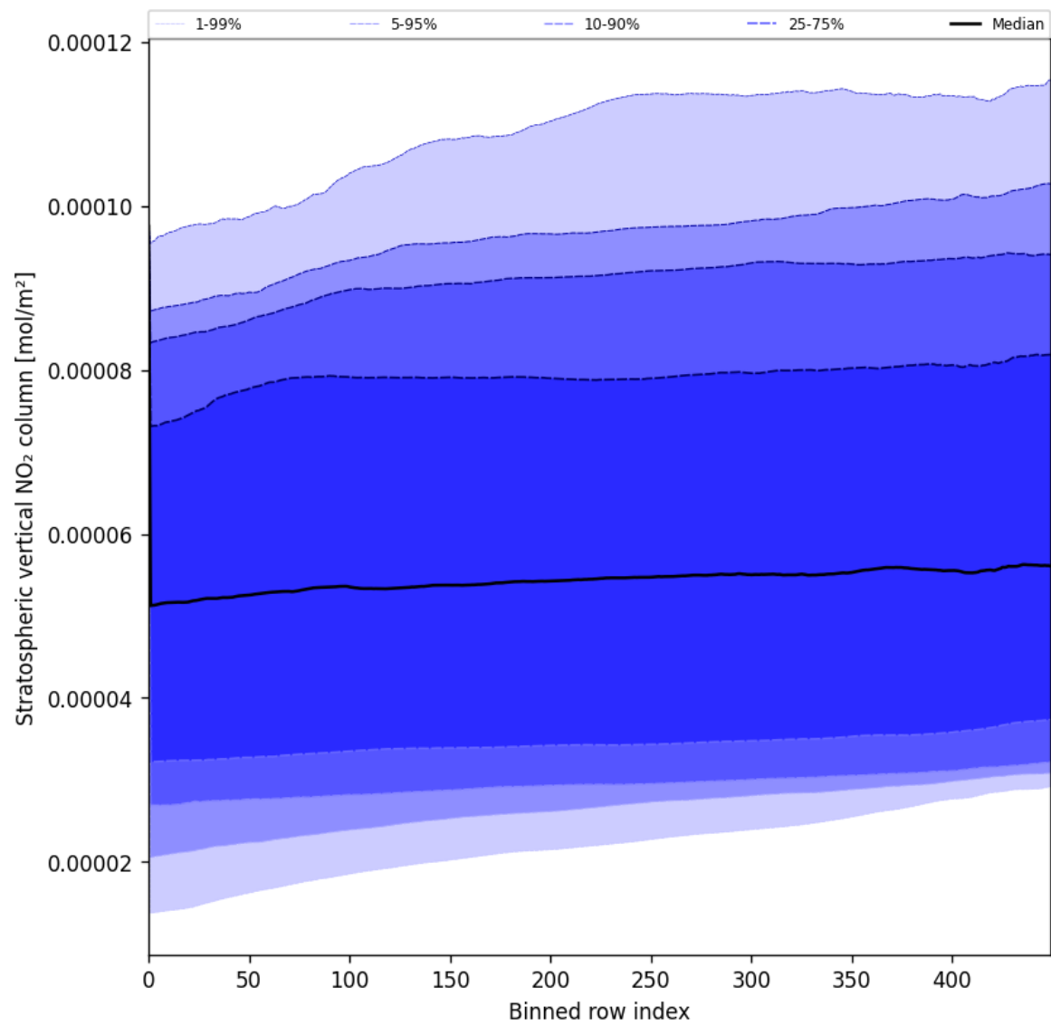
Figure 51: Along track statistics of “Stratospheric vertical NO 2 column” for 2025-06-22 to 2025-06-23
