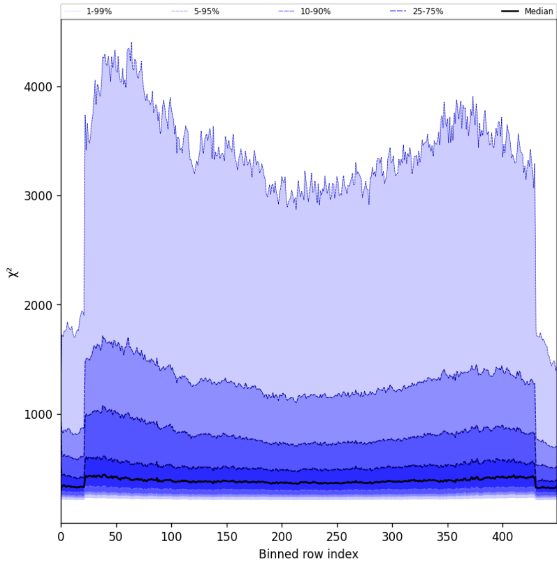
Figure 57: Along track statistics of “ \chi^2 ” for 2025-06-22 to 2025-06-23
