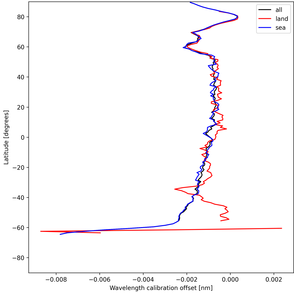
Figure 16: Zonal average of “Wavelength calibration offset” for 2025-06-22 to 2025-06-23.
