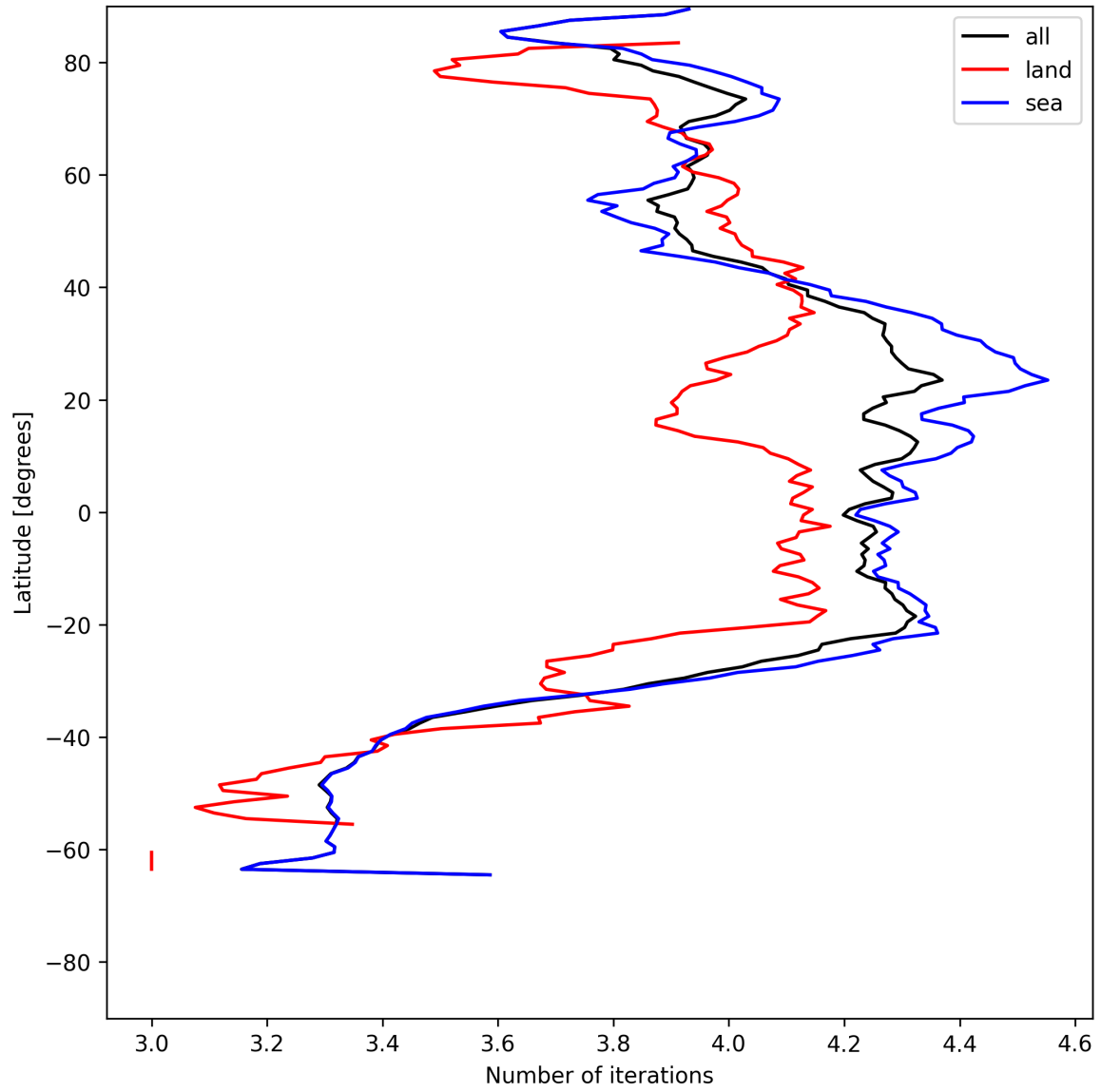
Figure 15: Zonal average of “Number of iterations” for 2025-06-22 to 2025-06-23.
