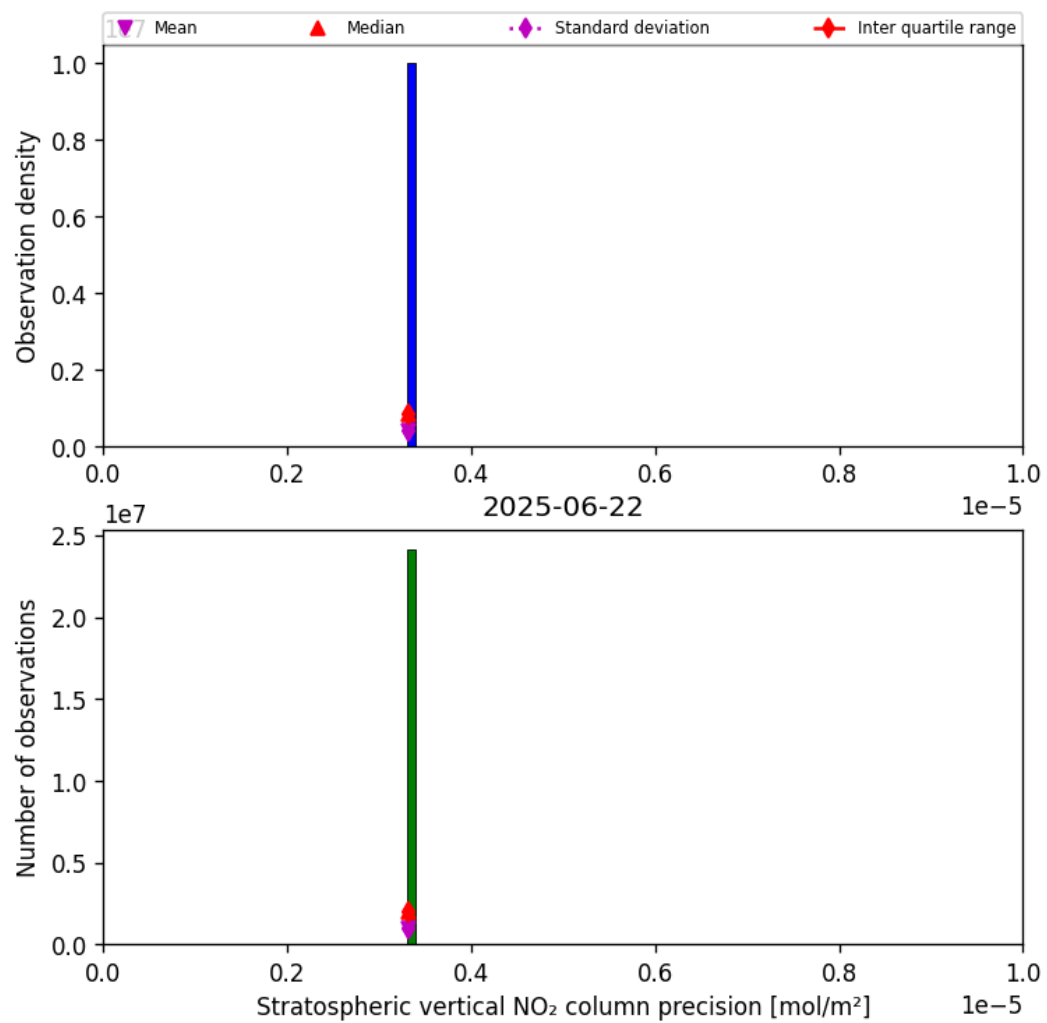
Figure 35: Histogram of “Stratospheric vertical NO 2 column precision” for 2025-06-22 to 2025-06-23
