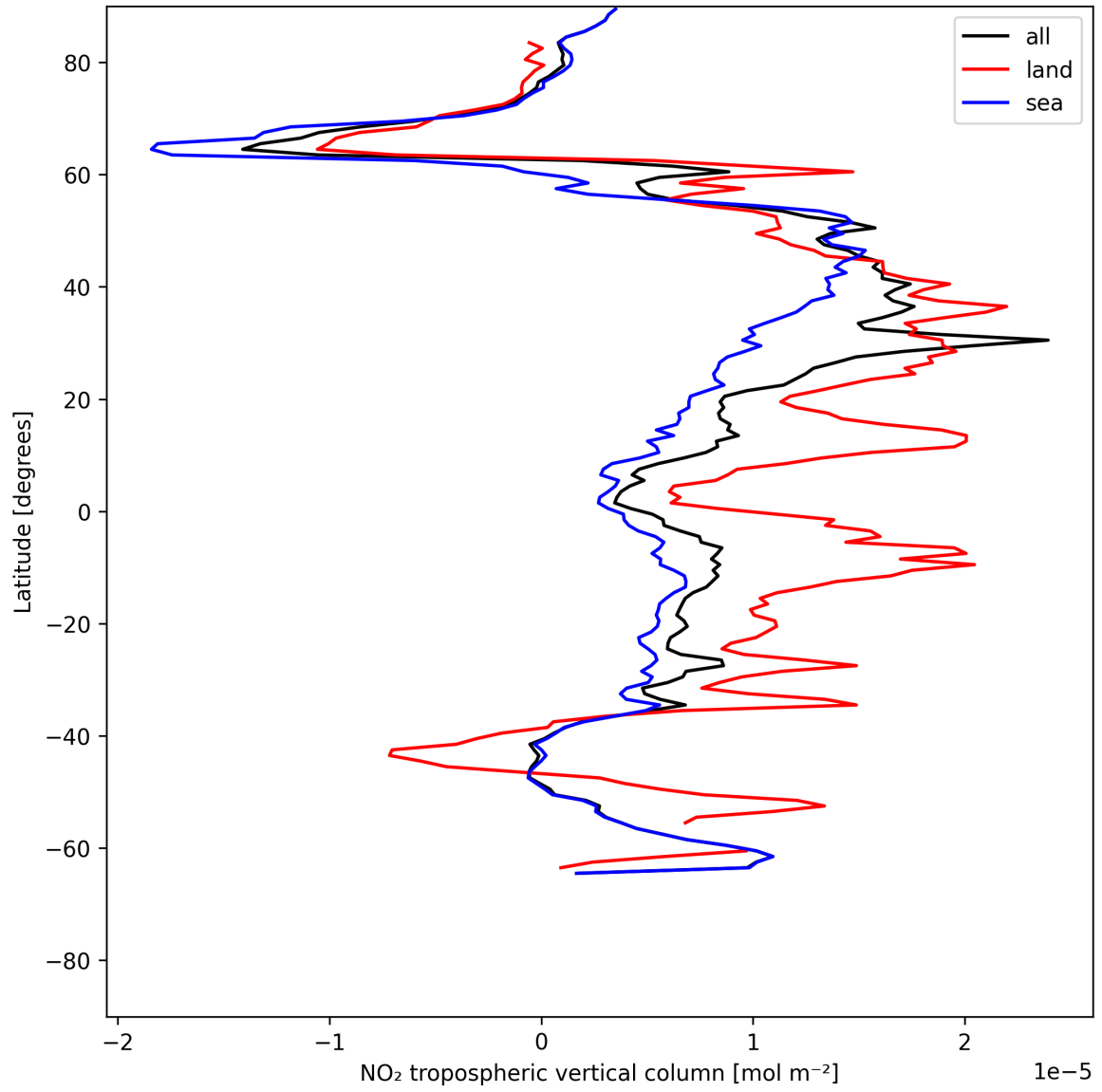
Figure 10: Zonal average of “NO 2 tropospheric vertical column” for 2025-06-22 to 2025-06-23.
