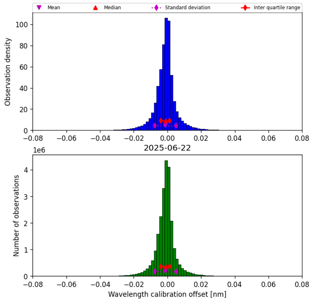
Figure 33: Histogram of “Wavelength calibration offset” for 2025-06-22 to 2025-06-23
