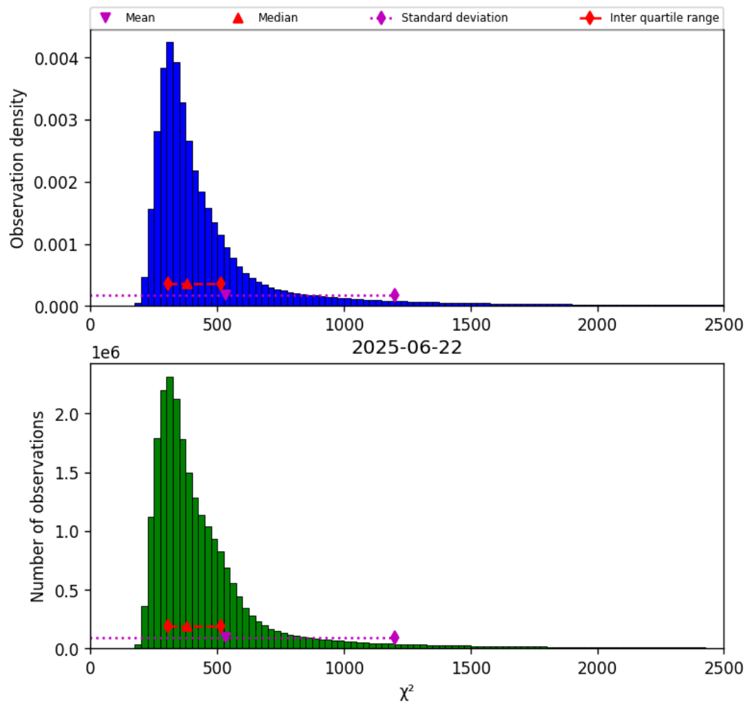
Figure 40: Histogram of “ \chi^2 ” for 2025-06-22 to 2025-06-23
