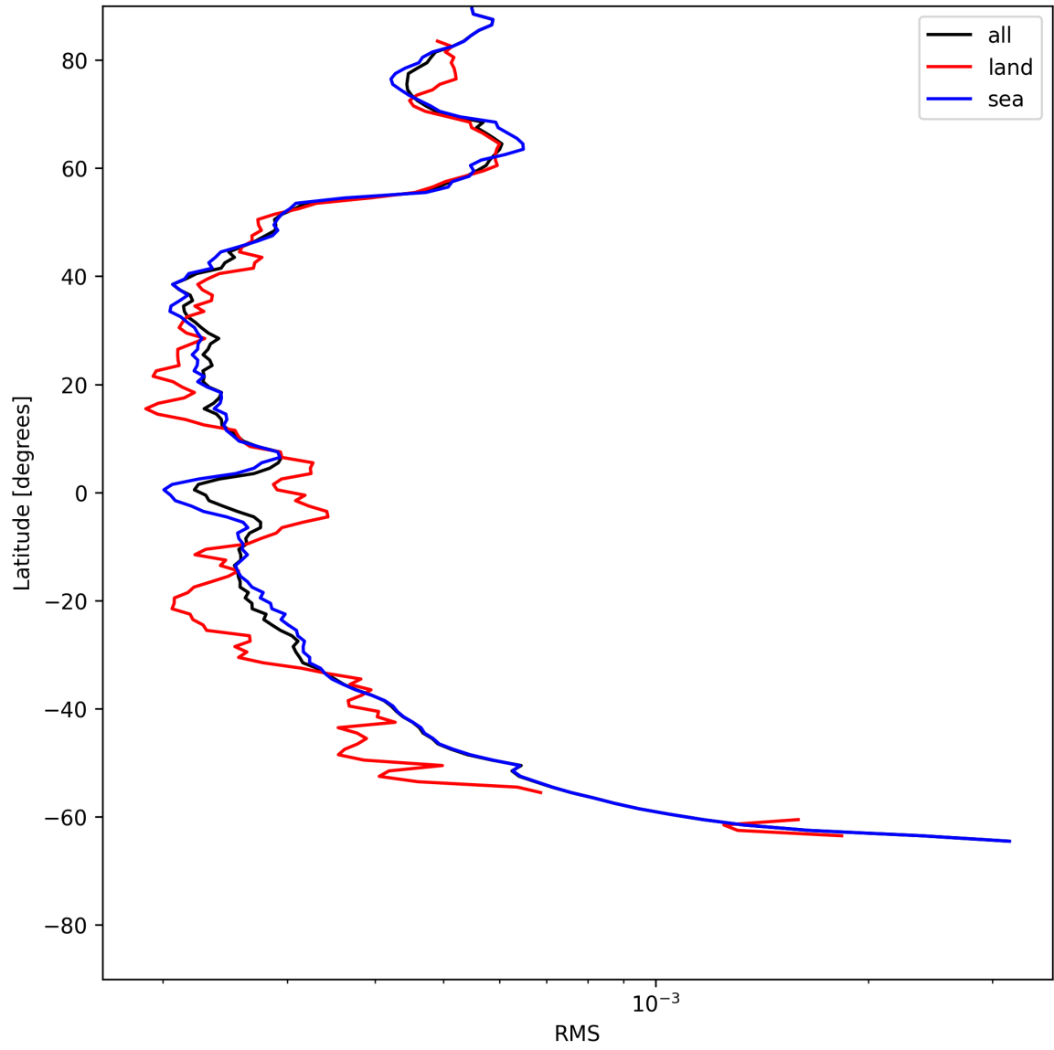
Figure 24: Zonal average of “RMS” for 2025-06-22 to 2025-06-23.
