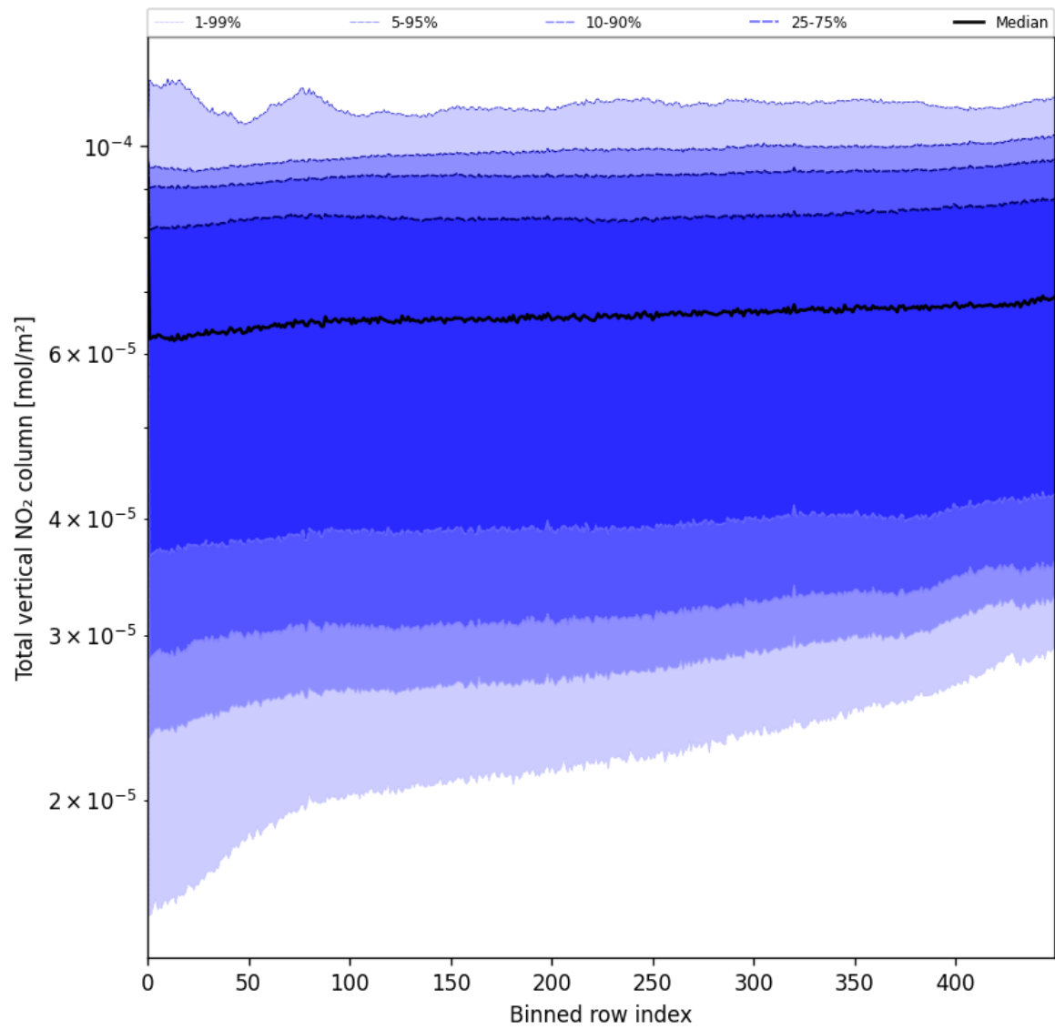
Figure 53: Along track statistics of “Total vertical NO 2 column” for 2025-06-22 to 2025-06-23
