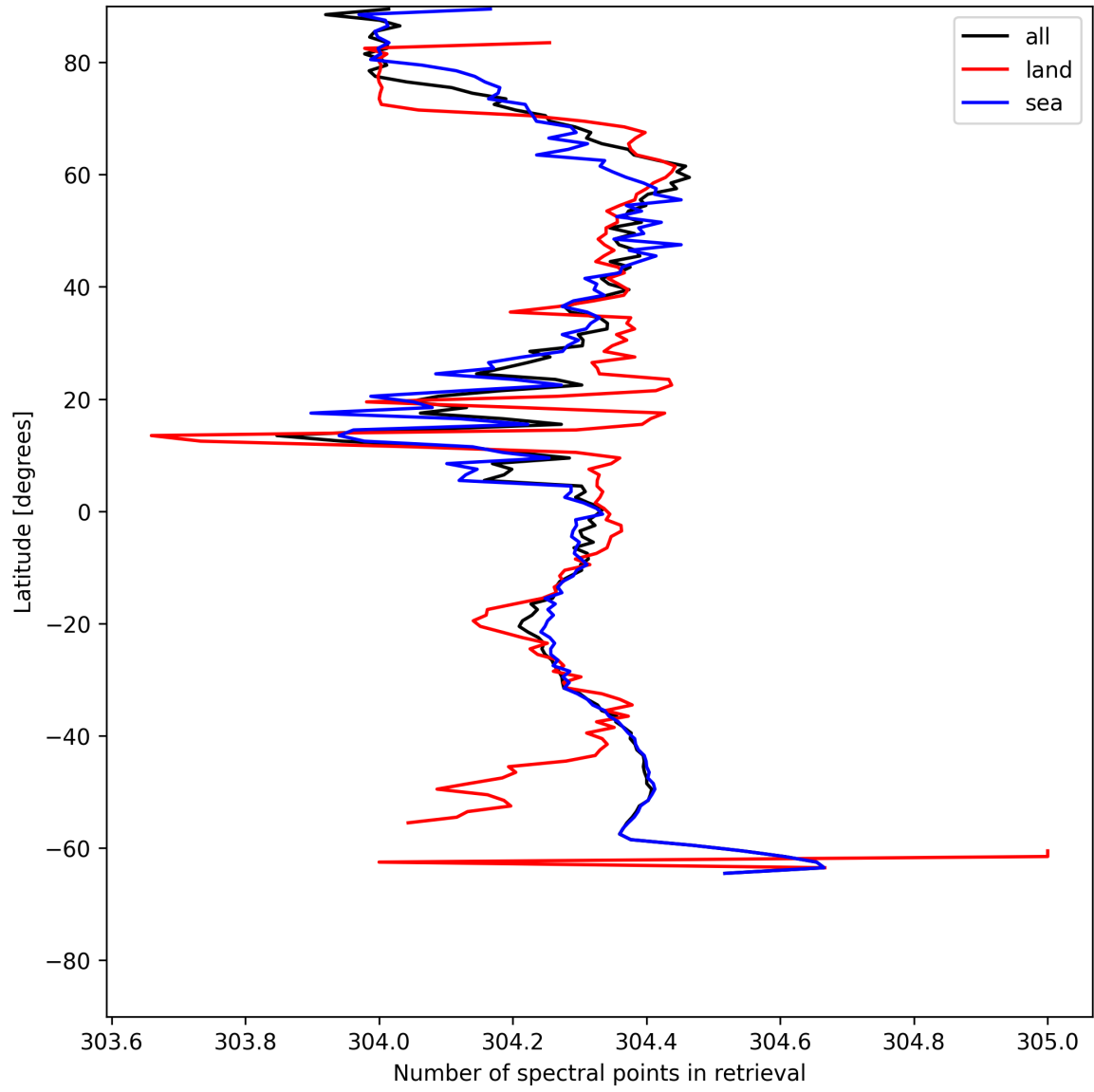
Figure 14: Zonal average of “Number of spectral points in retrieval” for 2025-06-22 to 2025-06-23.
