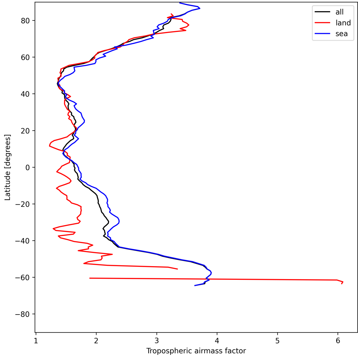
Figure 12: Zonal average of “Tropospheric airmass factor” for 2025-06-22 to 2025-06-23.
