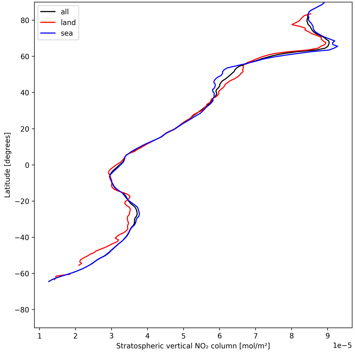
Figure 17: Zonal average of “Stratospheric vertical NO 2 column” for 2025-06-22 to 2025-06-23.
