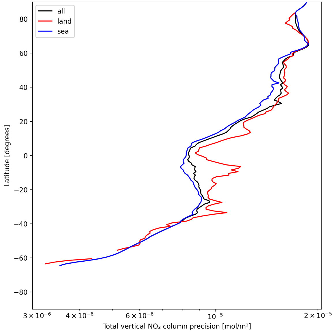
Figure 20: Zonal average of “Total vertical NO 2 column precision” for 2025-06-22 to 2025-06-23.
