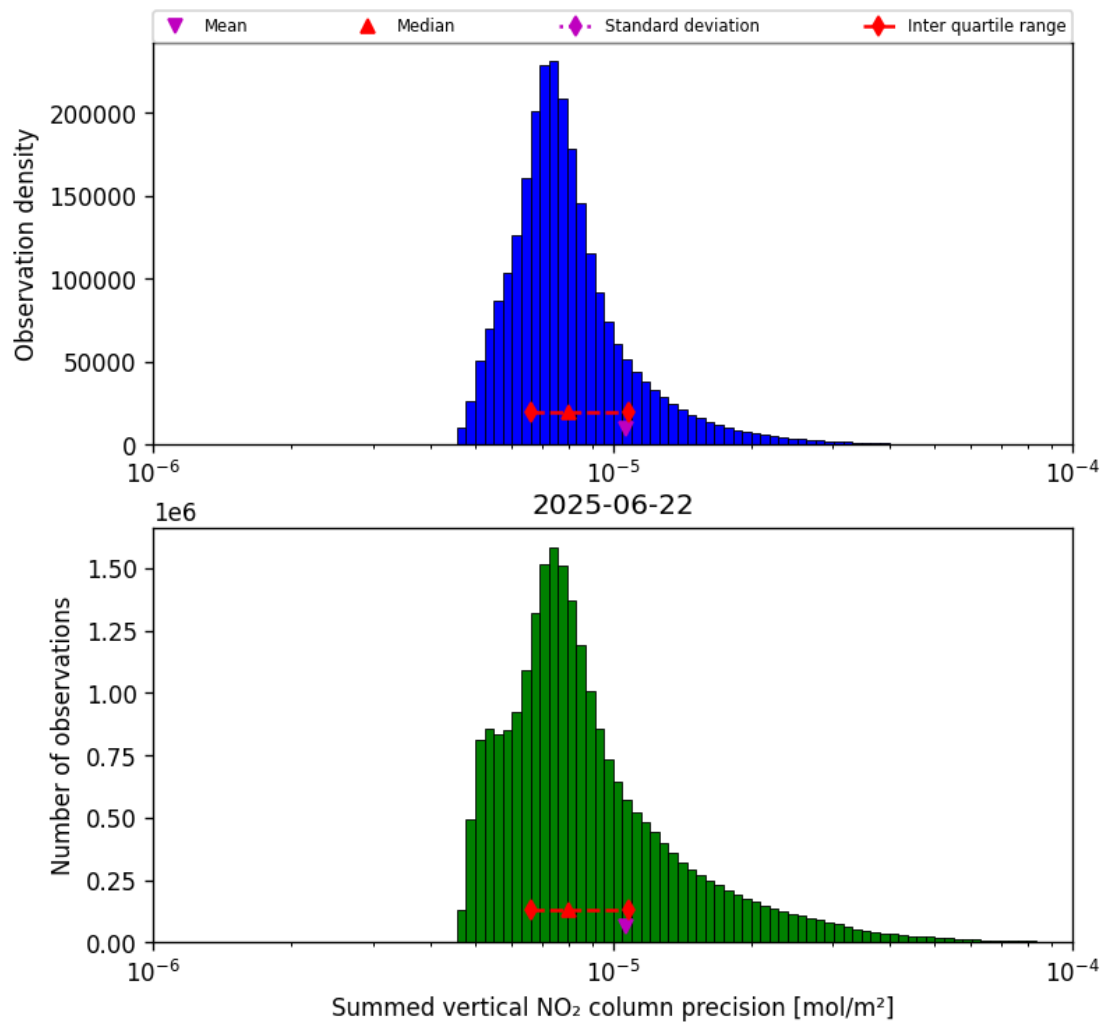
Figure 39: Histogram of “Summed vertical NO 2 column precision” for 2025-06-22 to 2025-06-23
