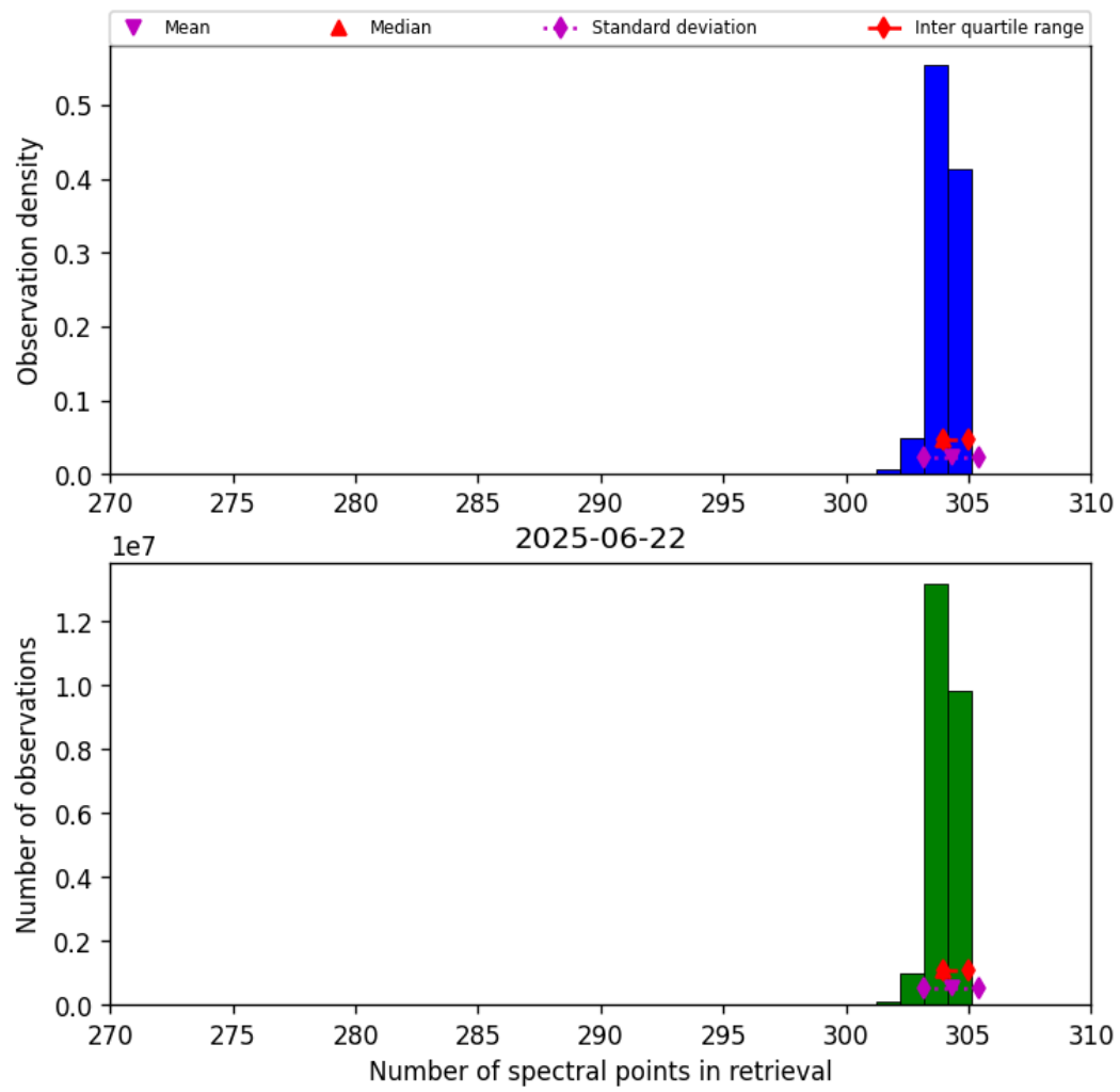
Figure 31: Histogram of “Number of spectral points in retrieval” for 2025-06-22 to 2025-06-23
