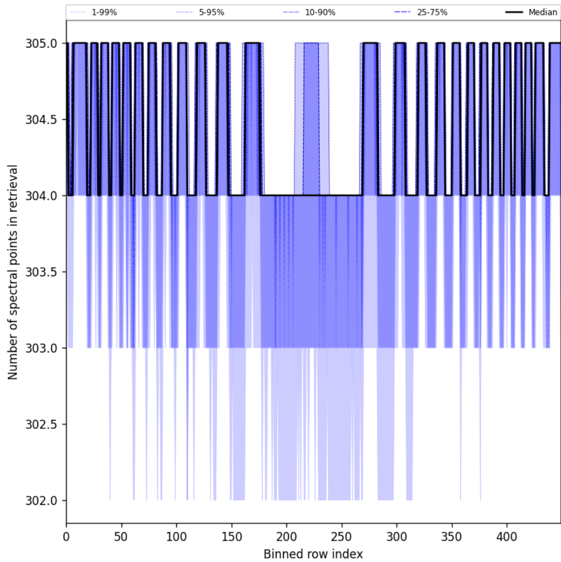
Figure 48: Along track statistics of “Number of spectral points in retrieval” for 2025-06-22 to 2025-06-23
