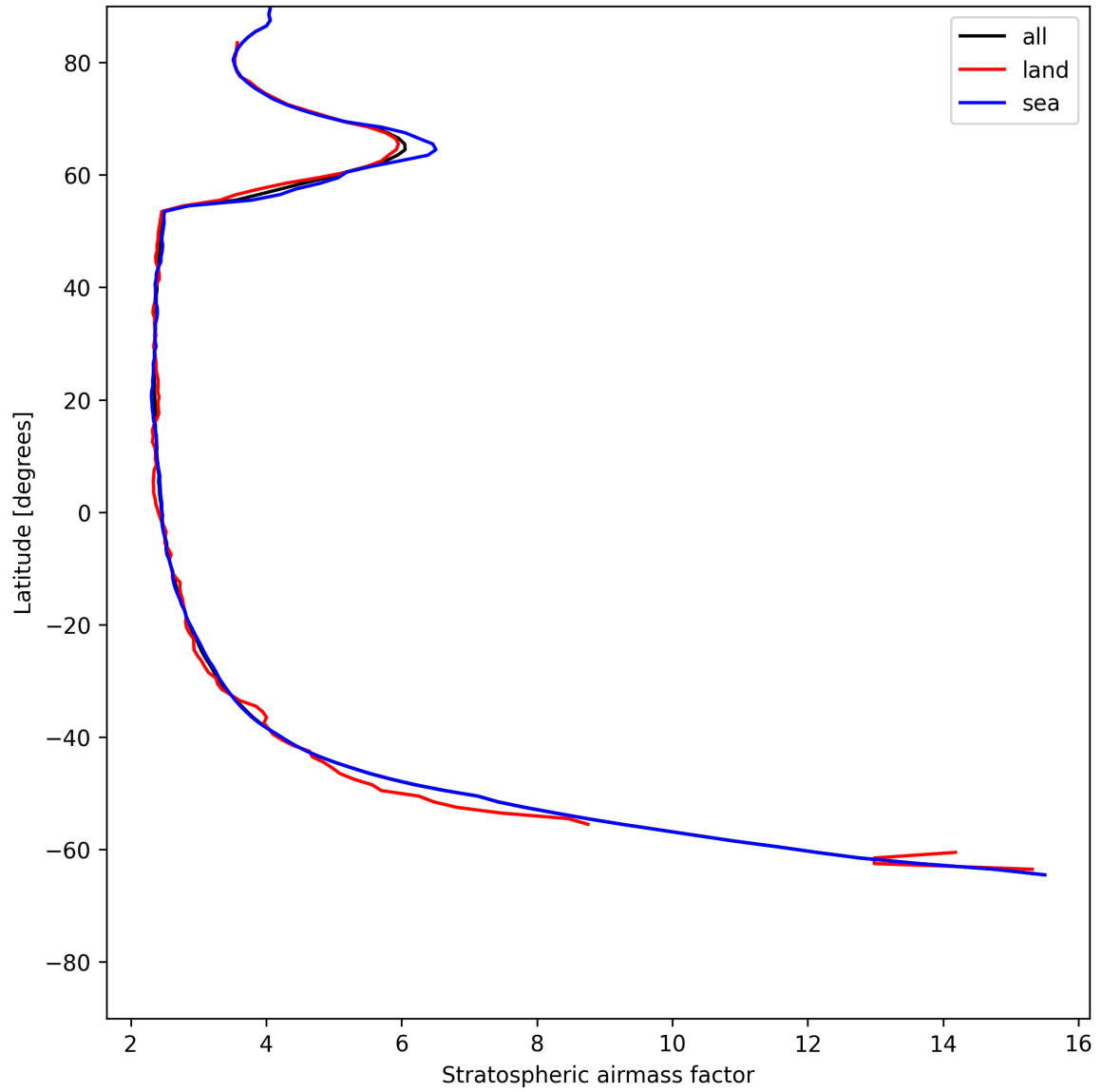
Figure 25: Zonal average of “Stratospheric airmass factor” for 2025-06-22 to 2025-06-23.
