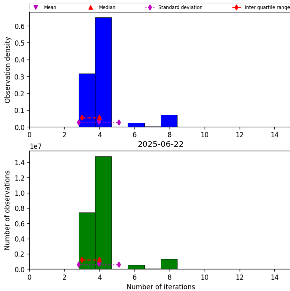
Figure 32: Histogram of “Number of iterations” for 2025-06-22 to 2025-06-23
