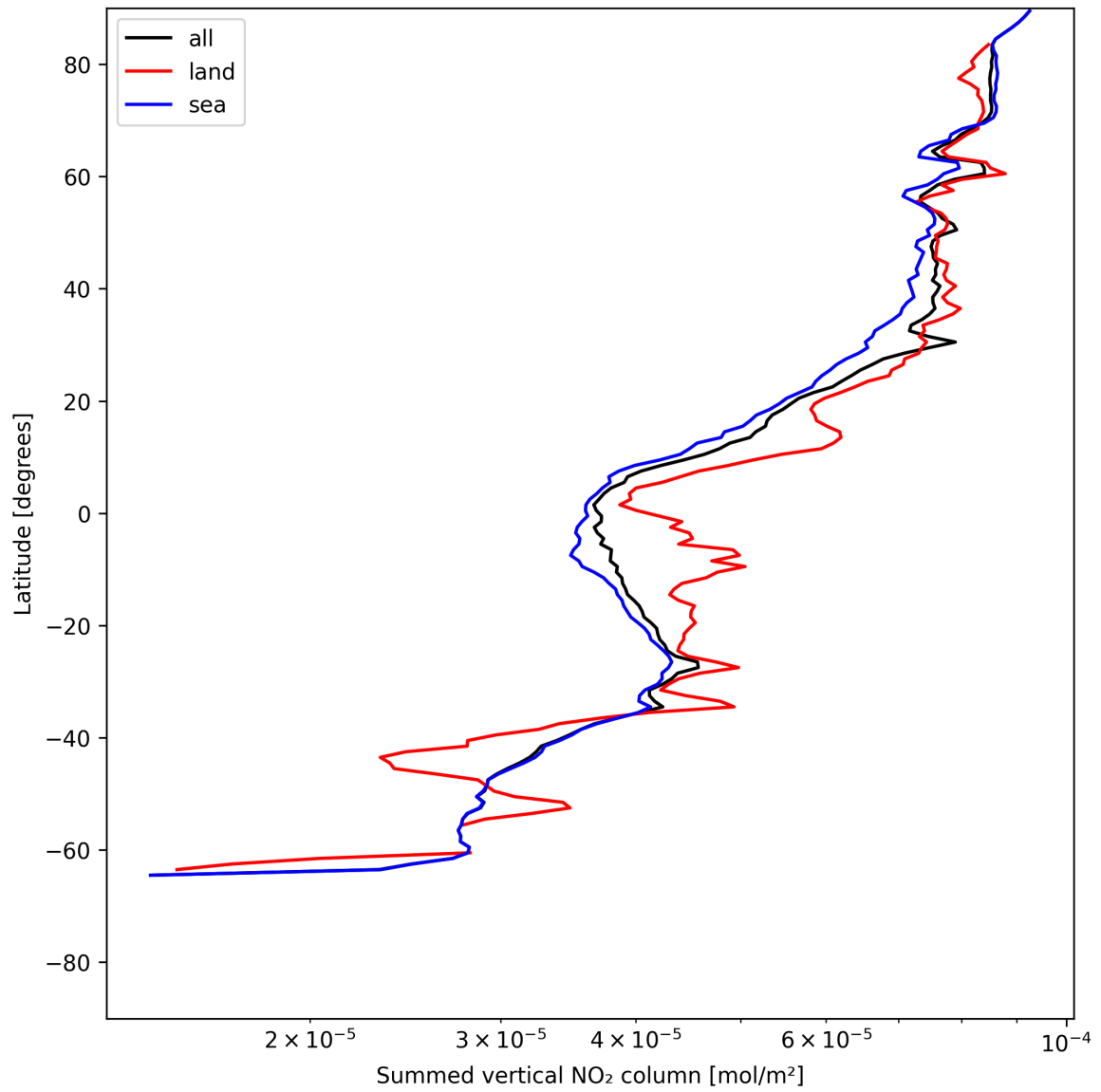
Figure 21: Zonal average of “Summed vertical NO 2 column” for 2025-06-22 to 2025-06-23.
