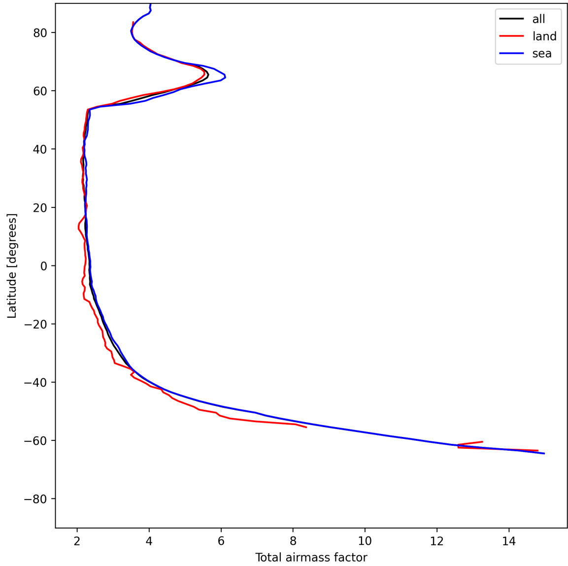
Figure 13: Zonal average of “Total airmass factor” for 2025-06-22 to 2025-06-23.
