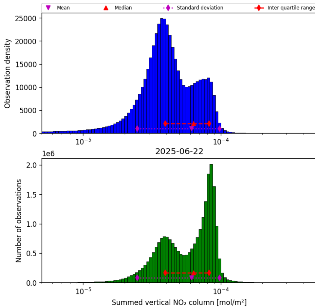
Figure 38: Histogram of “Summed vertical NO 2 column” for 2025-06-22 to 2025-06-23
