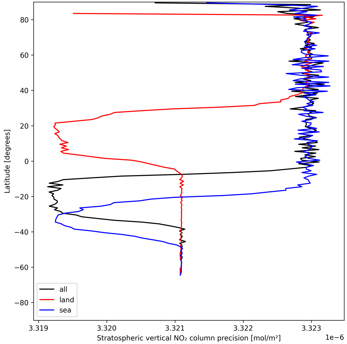
Figure 18: Zonal average of “Stratospheric vertical NO 2 column precision” for 2025-06-22 to 2025-06-23.
