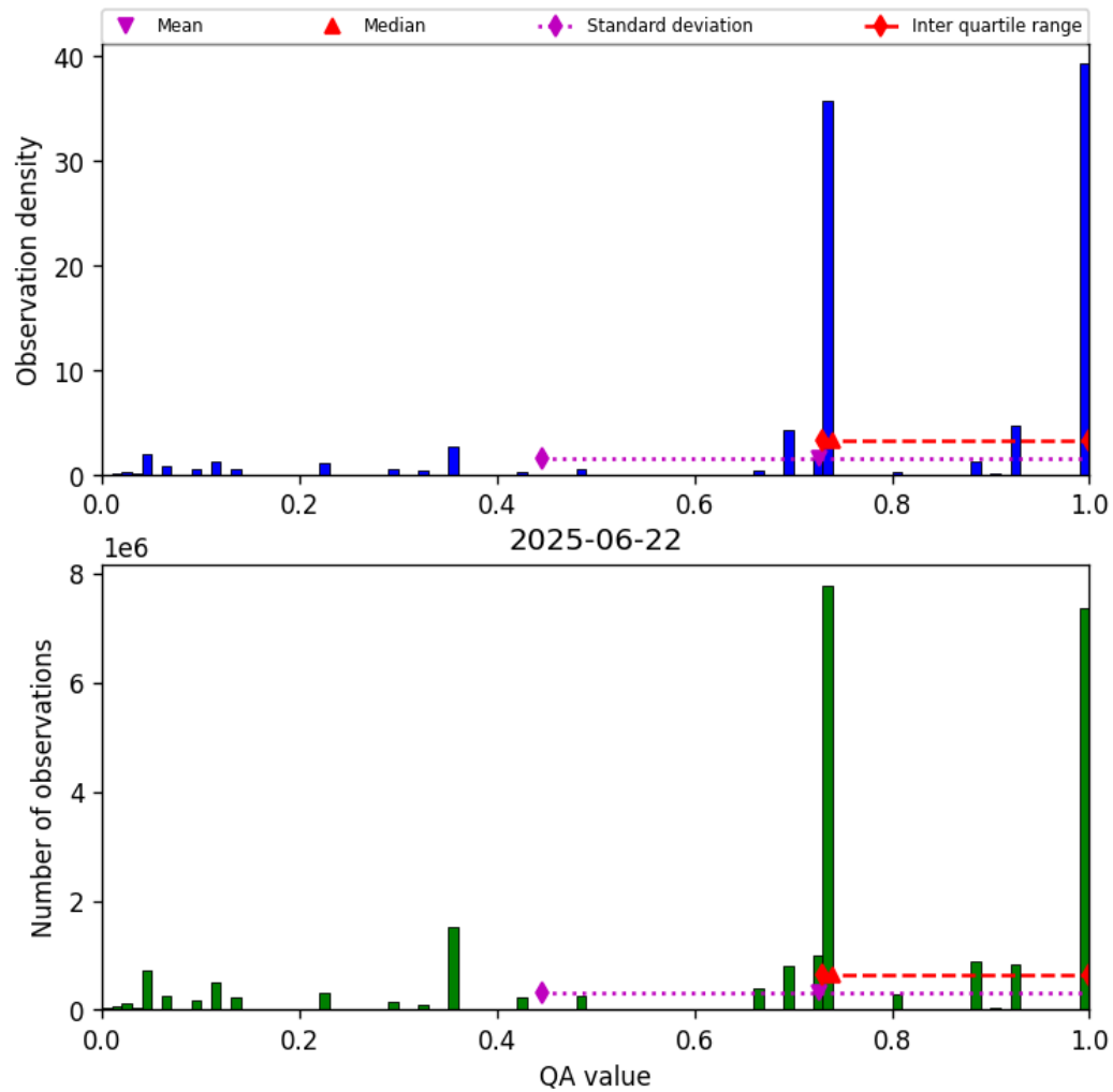
Figure 26: Histogram of “QA value” for 2025-06-22 to 2025-06-23
