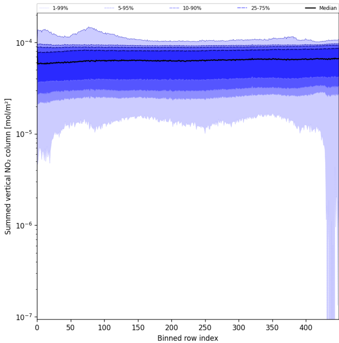
Figure 55: Along track statistics of “Summed vertical NO 2 column” for 2025-06-22 to 2025-06-23
