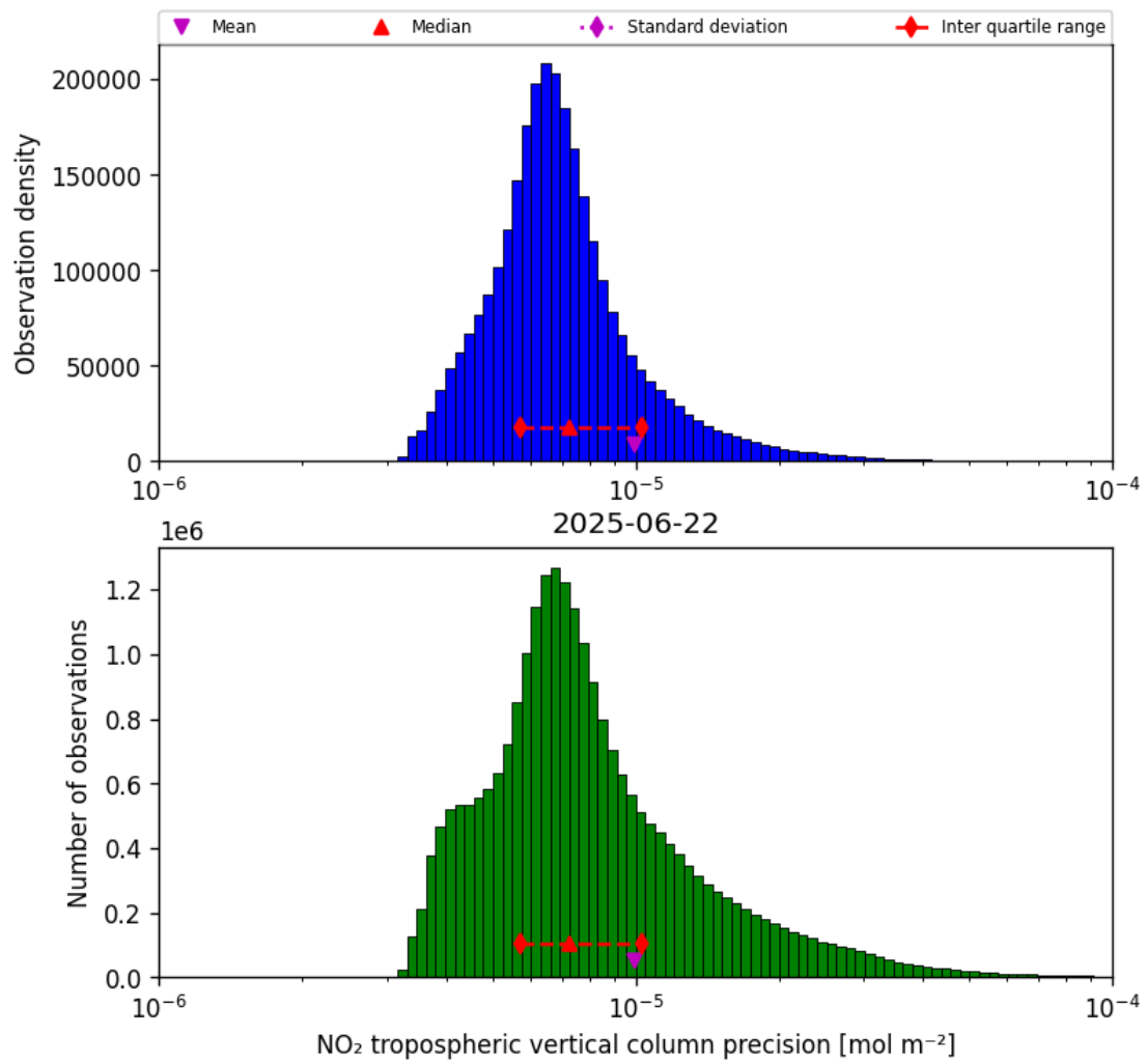
Figure 28: Histogram of “NO 2 tropospheric vertical column precision” for 2025-06-22 to 2025-06-23
