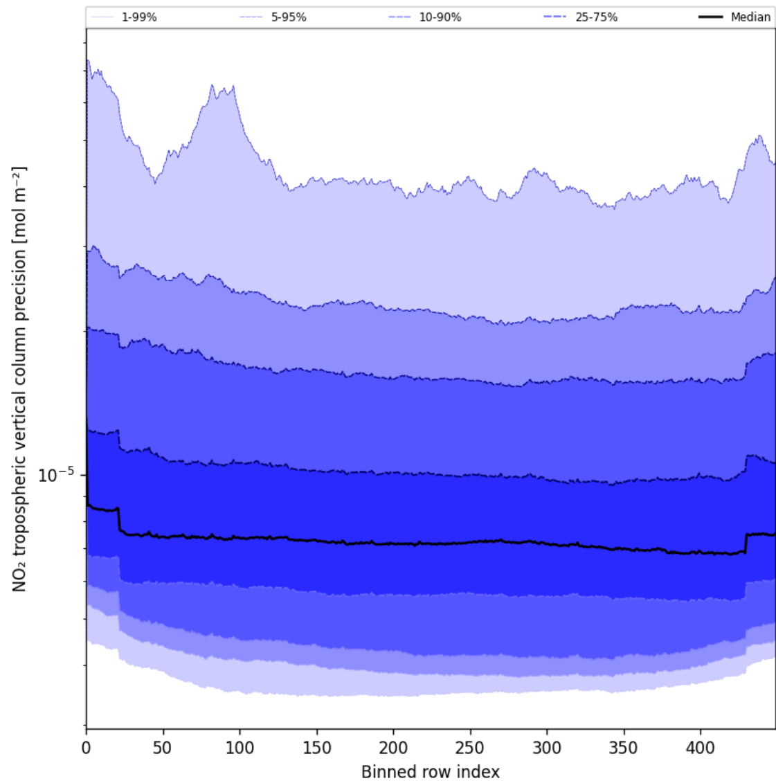
Figure 45: Along track statistics of “NO 2 tropospheric vertical column precision” for 2025-06-22 to 2025-06-23
