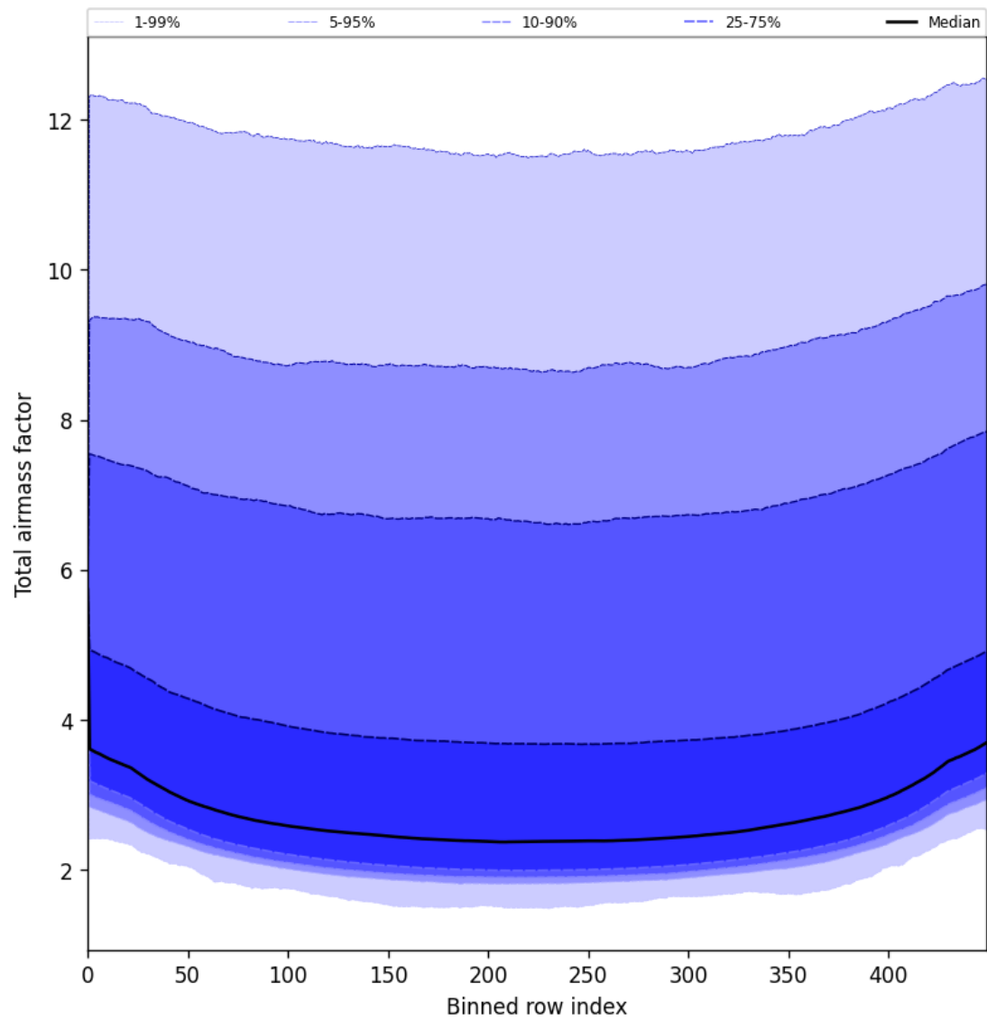
Figure 47: Along track statistics of “Total airmass factor” for 2025-06-22 to 2025-06-23
