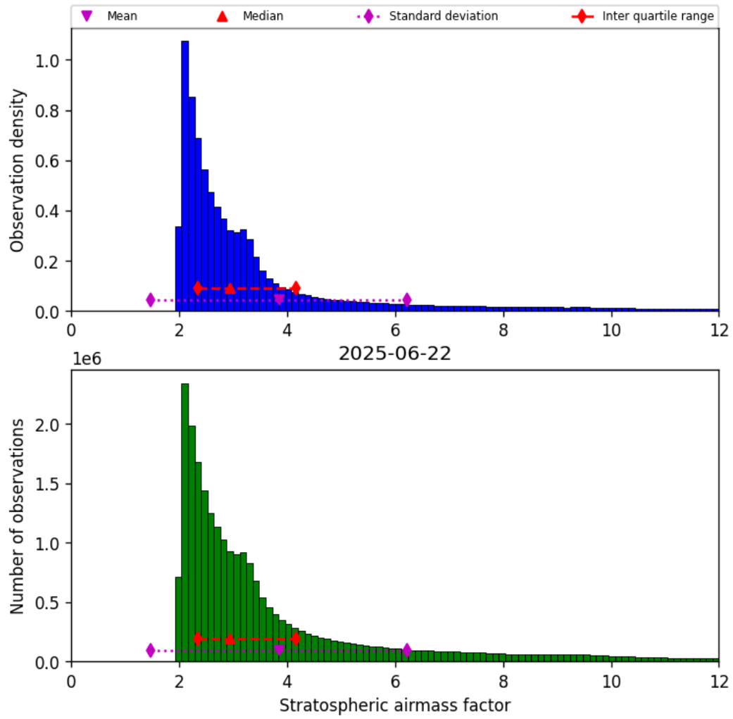
Figure 42: Histogram of “Stratospheric airmass factor” for 2025-06-22 to 2025-06-23
