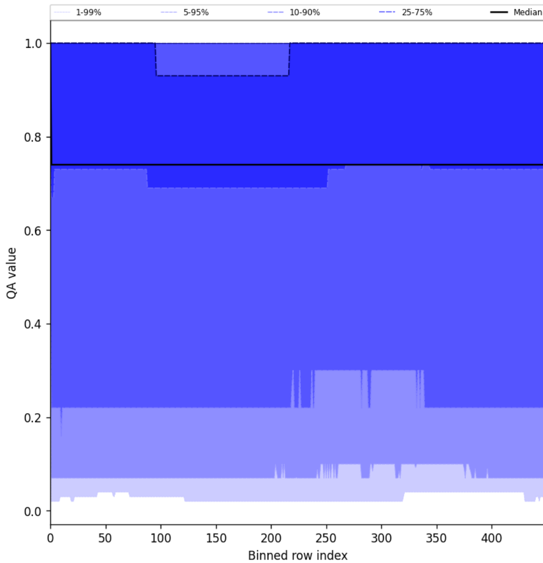
Figure 43: Along track statistics of “QA value” for 2025-06-22 to 2025-06-23
