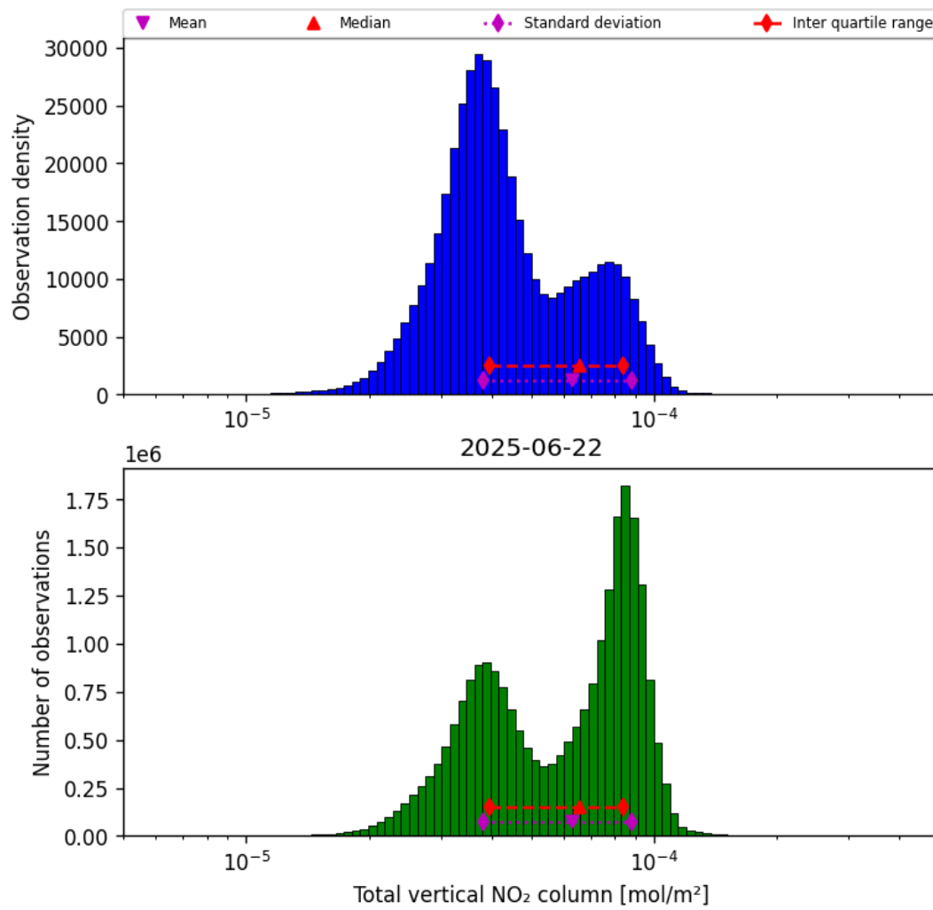
Figure 36: Histogram of “Total vertical NO 2 column” for 2025-06-22 to 2025-06-23
