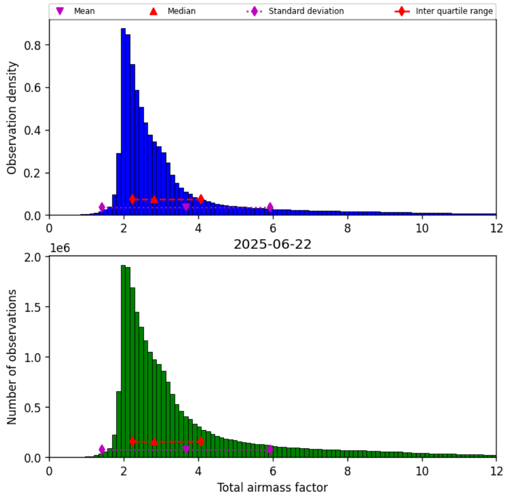
Figure 30: Histogram of “Total airmass factor” for 2025-06-22 to 2025-06-23
