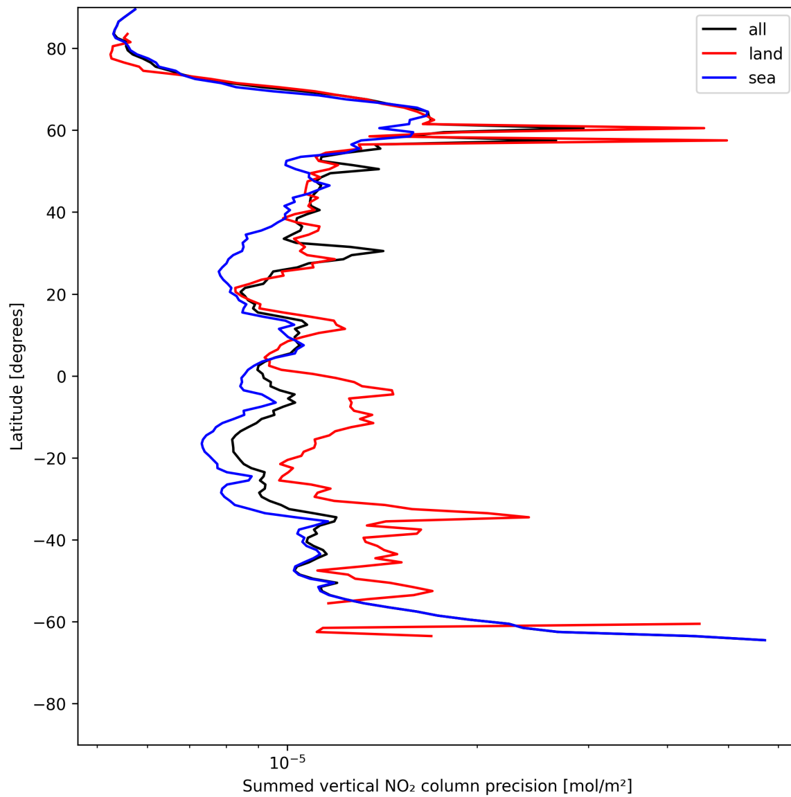
Figure 22: Zonal average of “Summed vertical NO 2 column precision” for 2025-06-22 to 2025-06-23.
