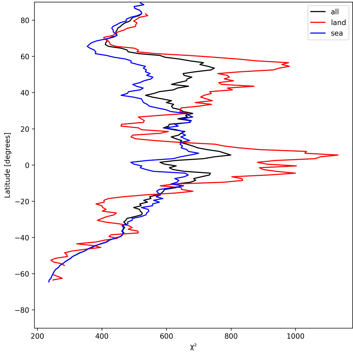
Figure 23: Zonal average of “ \chi^2 ” for 2025-06-22 to 2025-06-23.
