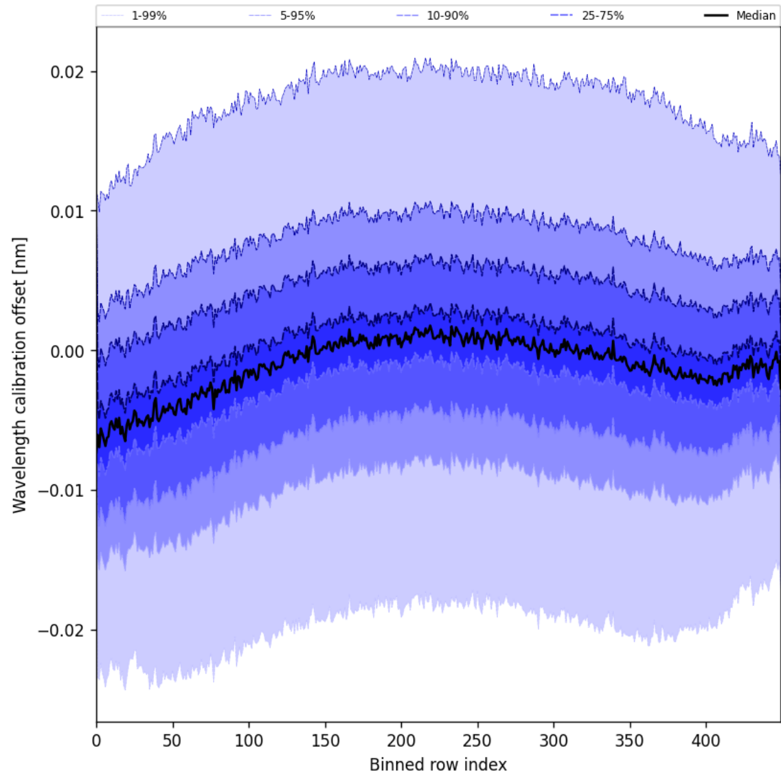
Figure 50: Along track statistics of “Wavelength calibration offset” for 2025-06-22 to 2025-06-23
