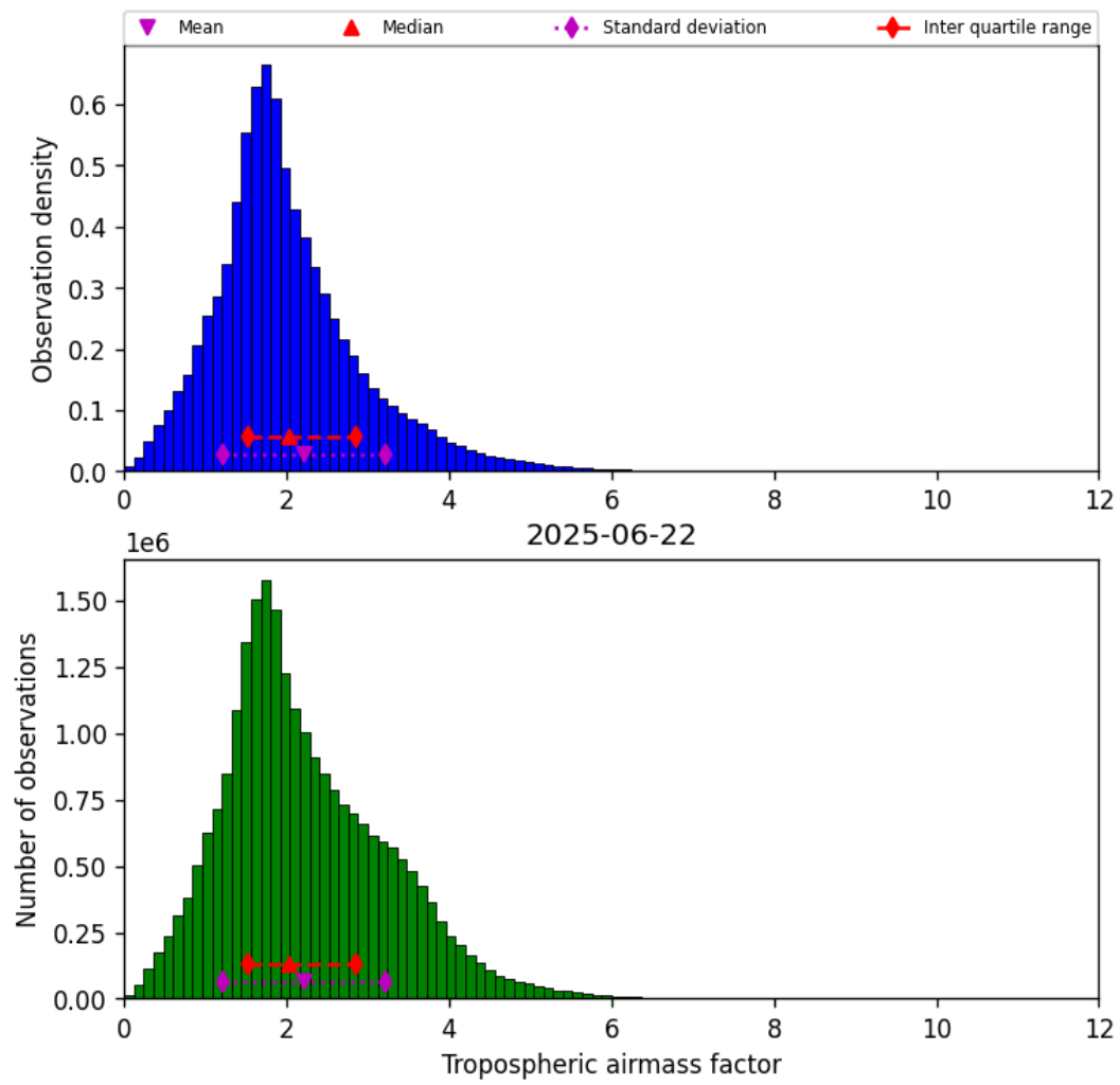
Figure 29: Histogram of “Tropospheric airmass factor” for 2025-06-22 to 2025-06-23
