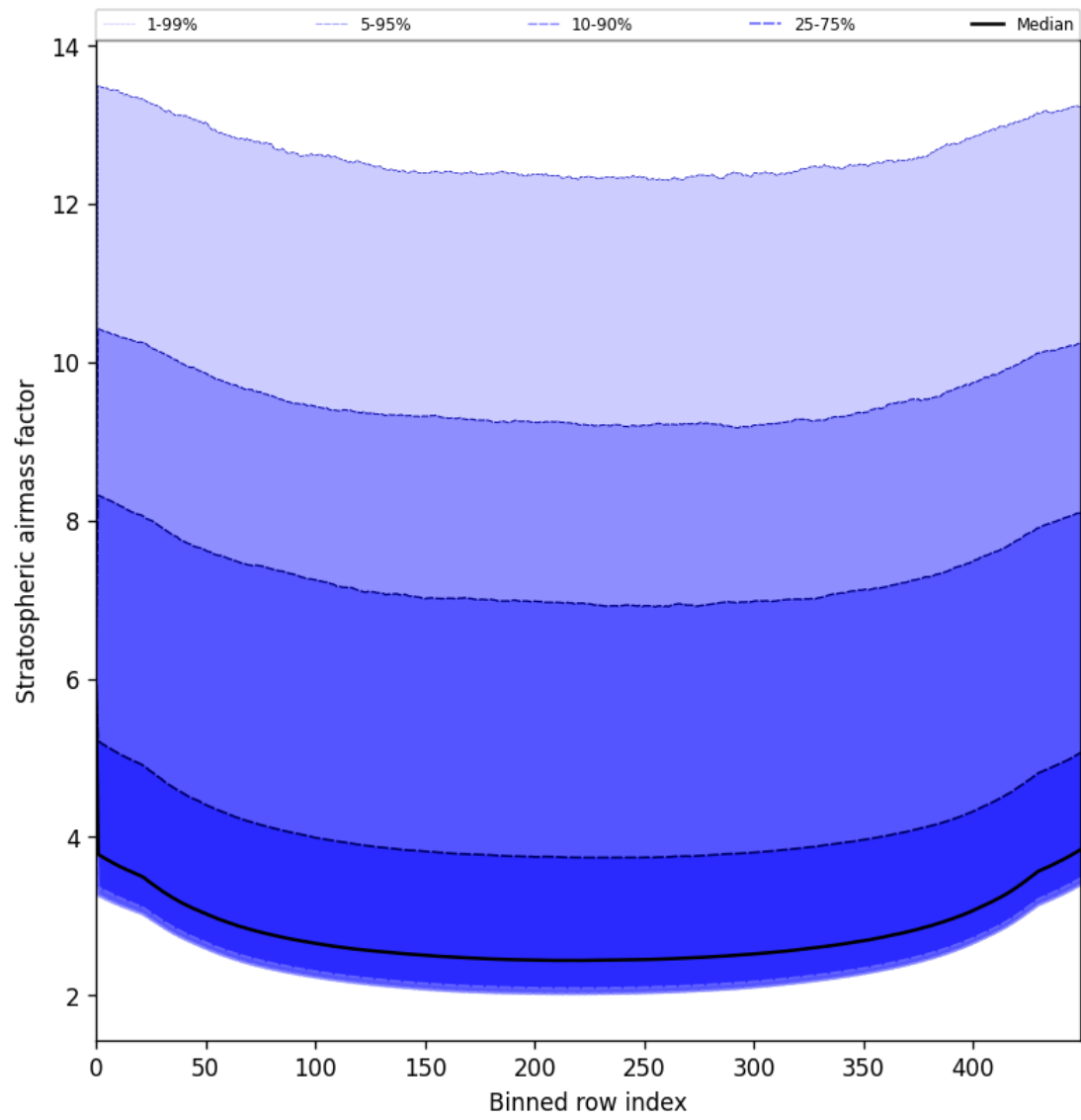
Figure 59: Along track statistics of “Stratospheric airmass factor” for 2025-06-22 to 2025-06-23
