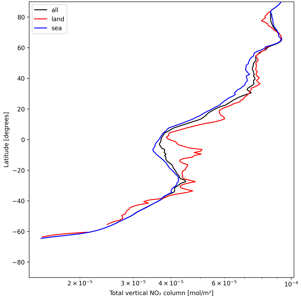
Figure 19: Zonal average of “Total vertical NO 2 column” for 2025-06-22 to 2025-06-23.
