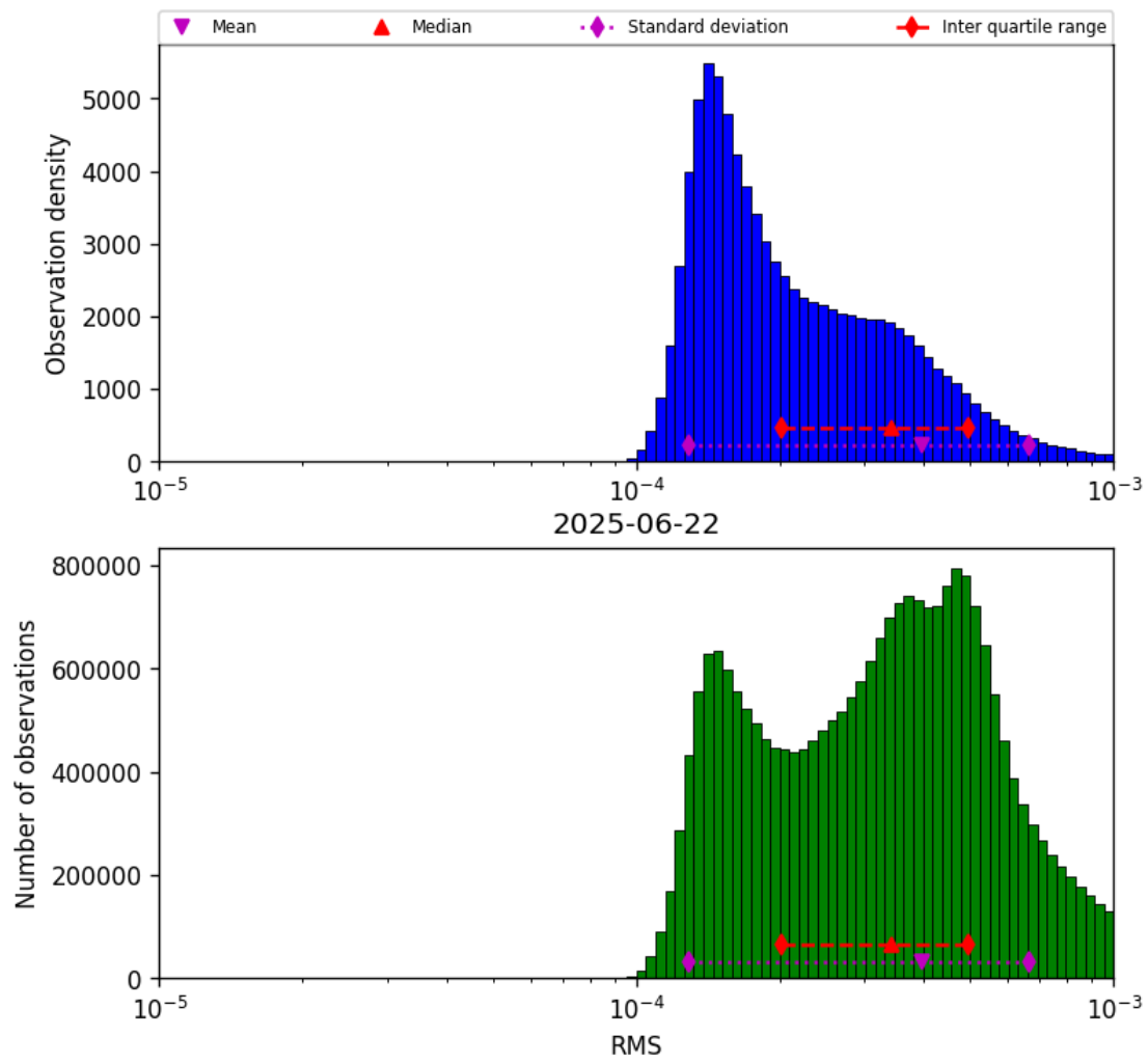
Figure 41: Histogram of “RMS” for 2025-06-22 to 2025-06-23
