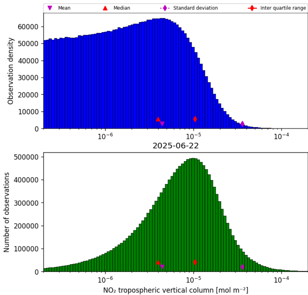
Figure 27: Histogram of “NO 2 tropospheric vertical column” for 2025-06-22 to 2025-06-23
