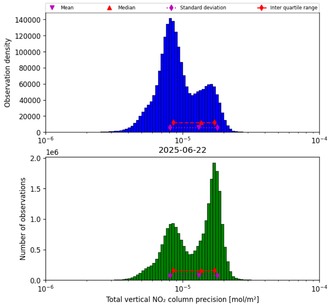
Figure 37: Histogram of “Total vertical NO 2 column precision” for 2025-06-22 to 2025-06-23
