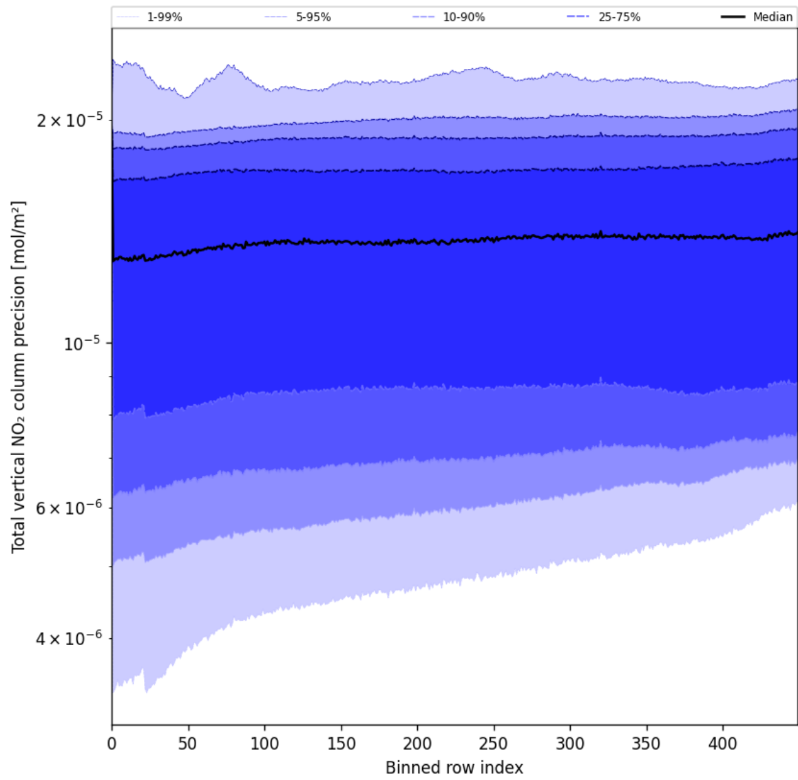
Figure 54: Along track statistics of “Total vertical NO 2 column precision” for 2025-06-22 to 2025-06-23
