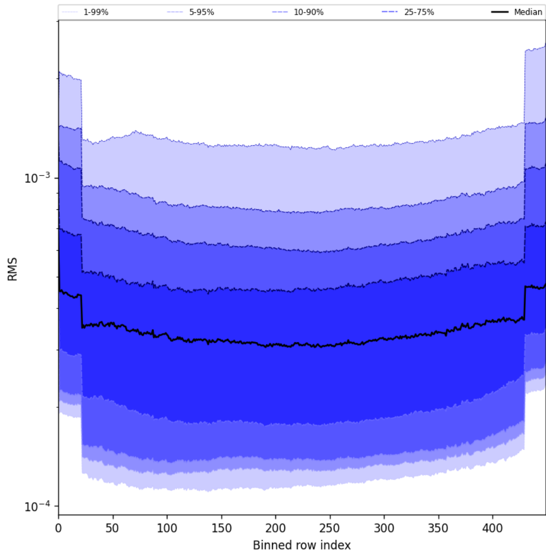
Figure 58: Along track statistics of “RMS” for 2025-06-22 to 2025-06-23
