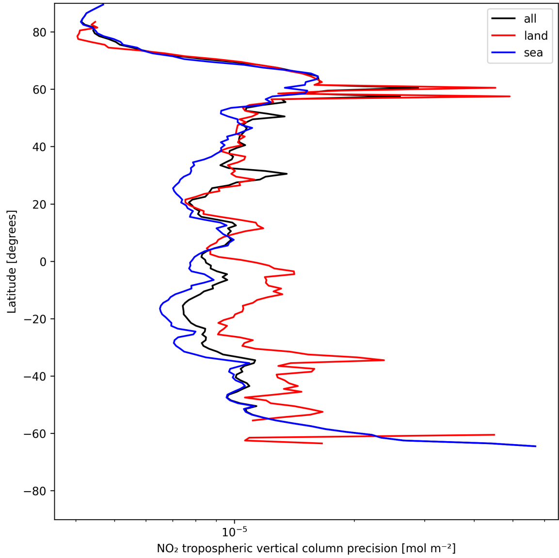
Figure 11: Zonal average of “NO 2 tropospheric vertical column precision” for 2025-06-22 to 2025-06-23.
