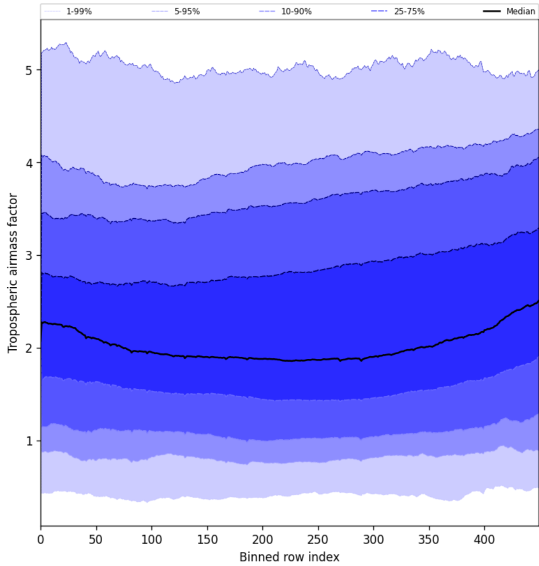
Figure 46: Along track statistics of “Tropospheric airmass factor” for 2025-06-22 to 2025-06-23
