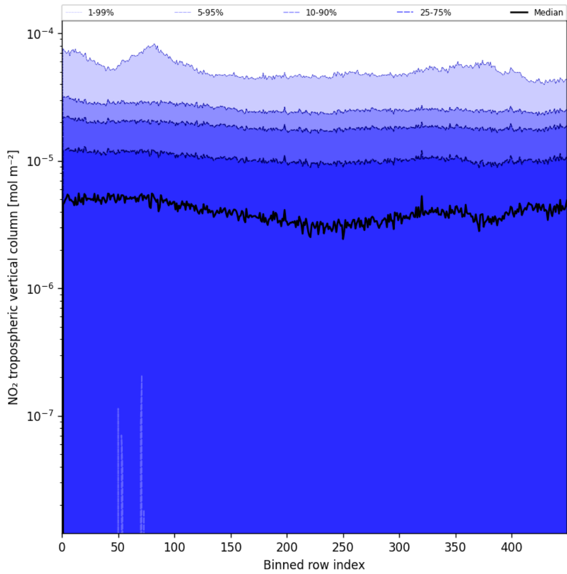
Figure 44: Along track statistics of “NO 2 tropospheric vertical column” for 2025-06-22 to 2025-06-23
