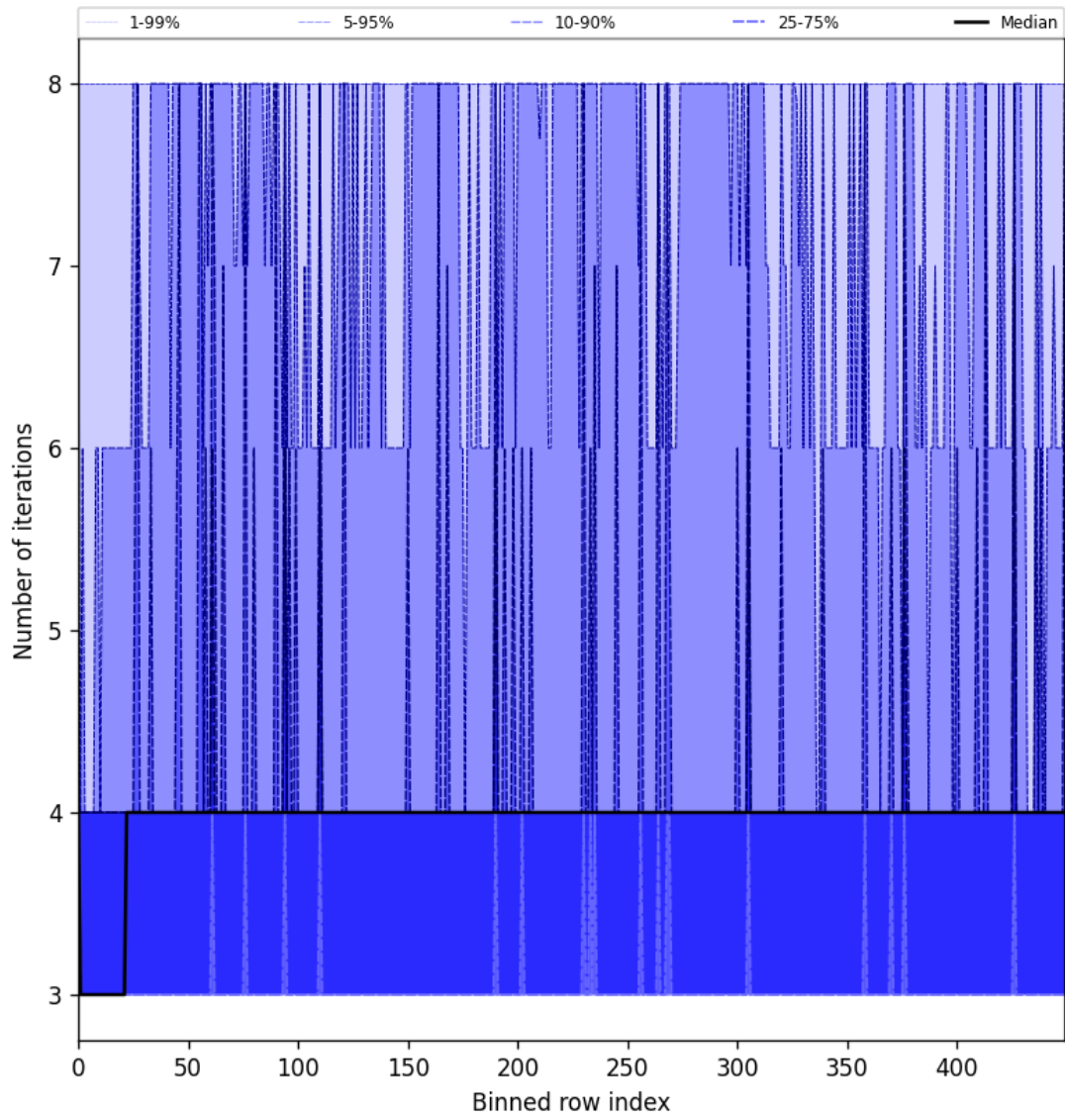
Figure 49: Along track statistics of “Number of iterations” for 2025-06-22 to 2025-06-23
