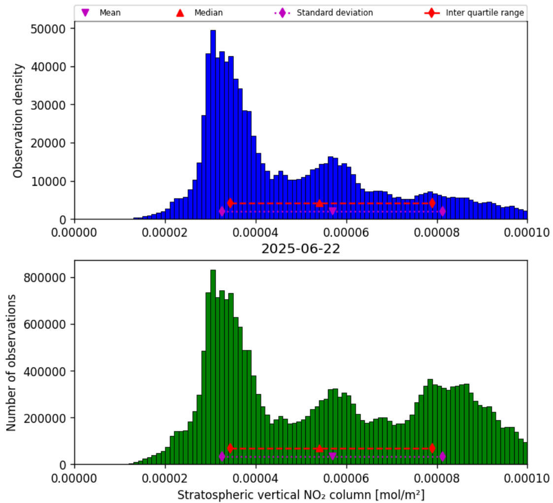
Figure 34: Histogram of “Stratospheric vertical NO 2 column” for 2025-06-22 to 2025-06-23
