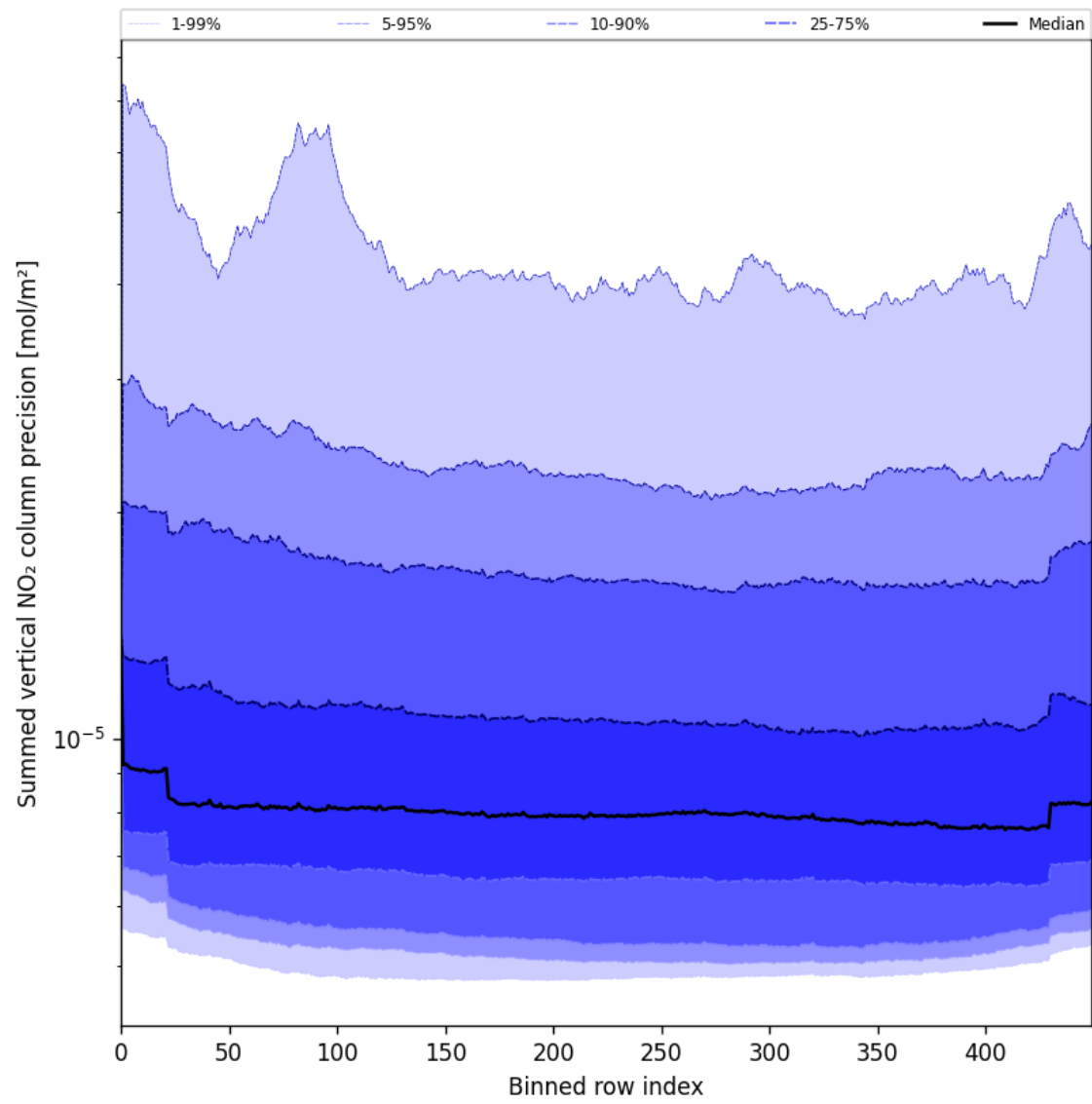
Figure 56: Along track statistics of “Summed vertical NO 2 column precision” for 2025-06-22 to 2025-06-23
