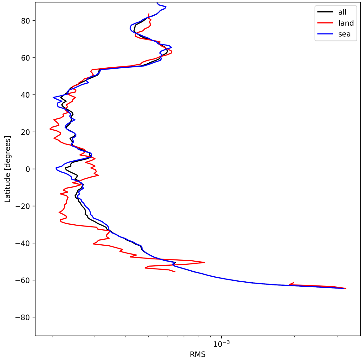
Figure 24: Zonal average of “RMS” for 2025-06-23 to 2025-06-24.
