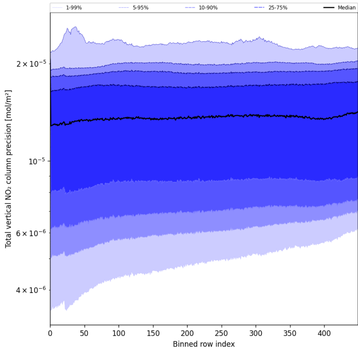
Figure 54: Along track statistics of “Total vertical NO 2 column precision” for 2025-06-23 to 2025-06-24
