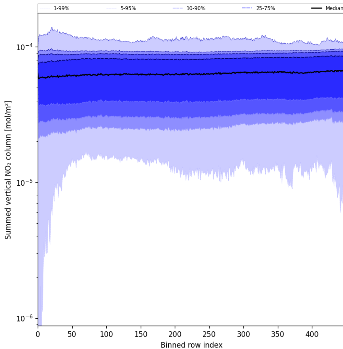
Figure 55: Along track statistics of “Summed vertical NO 2 column” for 2025-06-23 to 2025-06-24
