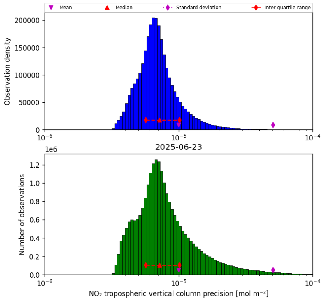
Figure 28: Histogram of “NO 2 tropospheric vertical column precision” for 2025-06-23 to 2025-06-24
