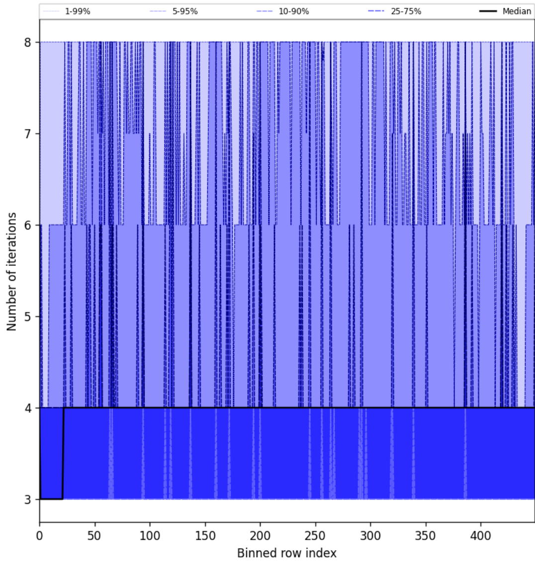
Figure 49: Along track statistics of “Number of iterations” for 2025-06-23 to 2025-06-24
