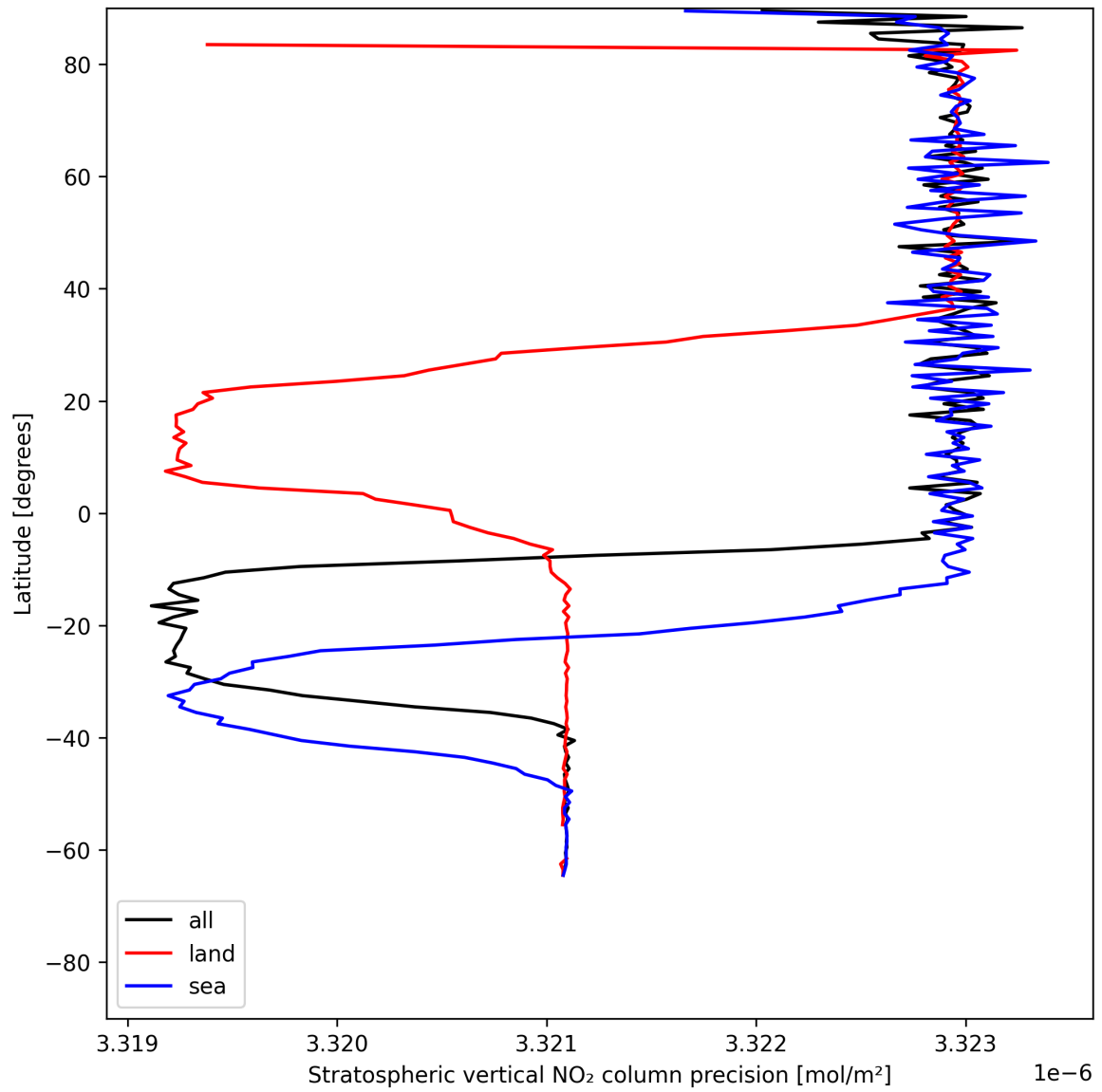
Figure 18: Zonal average of “Stratospheric vertical NO 2 column precision” for 2025-06-23 to 2025-06-24.
