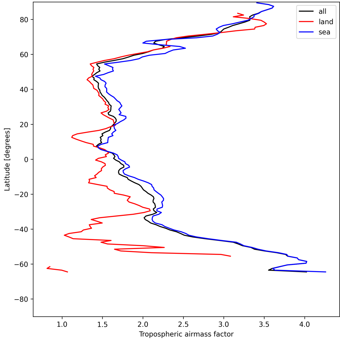
Figure 12: Zonal average of “Tropospheric air mass factor” for 2025-06-23 to 2025-06-24.
