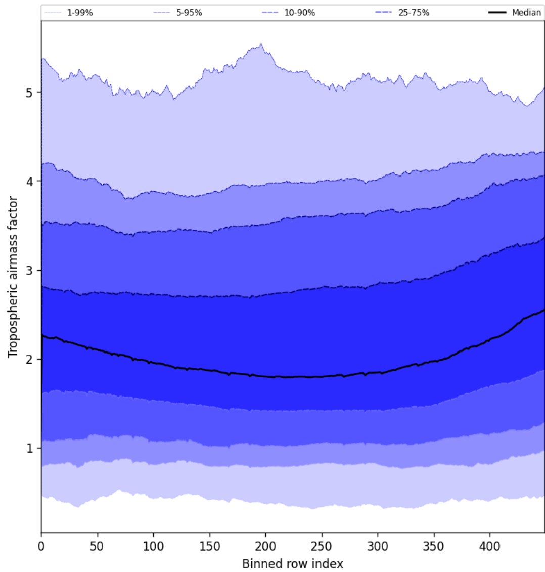
Figure 46: Along track statistics of “Tropospheric airmass factor” for 2025-06-23 to 2025-06-24
