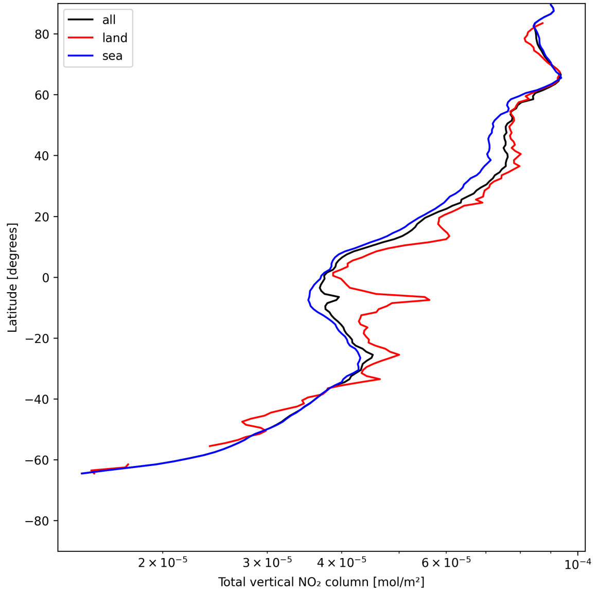
Figure 19: Zonal average of “Total vertical NO 2 column” for 2025-06-23 to 2025-06-24.
