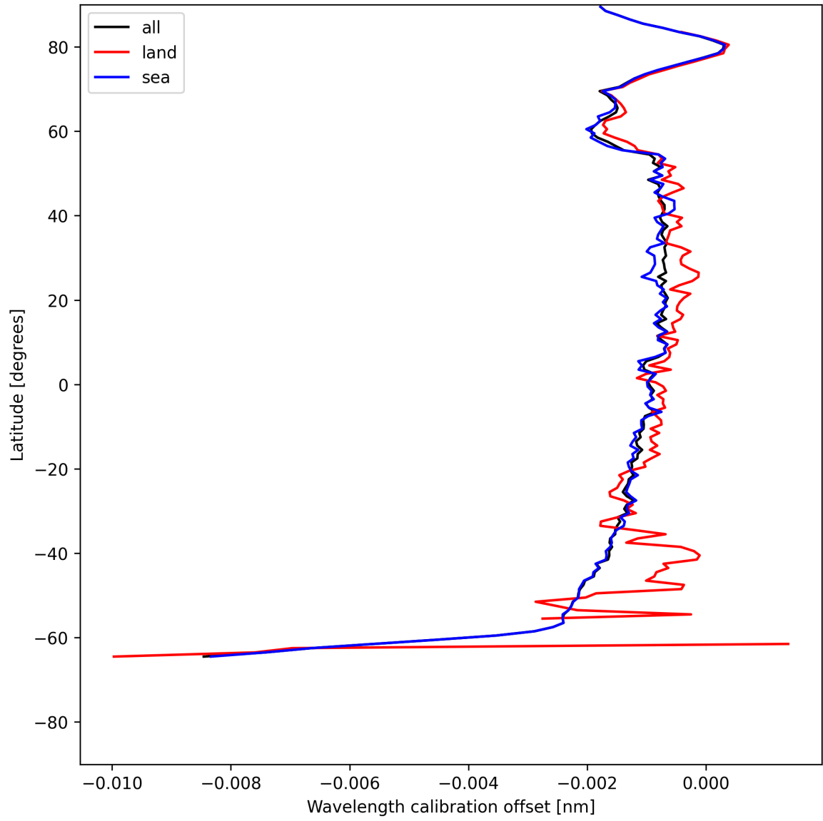
Figure 16: Zonal average of “Wavelength calibration offset” for 2025-06-23 to 2025-06-24.
