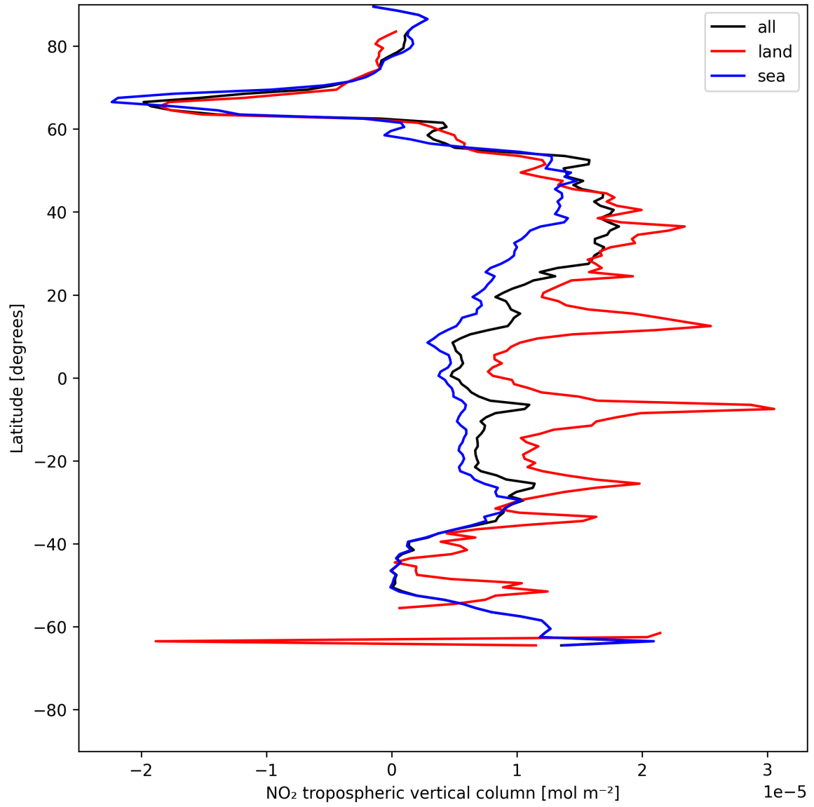
Figure 10: Zonal average of “NO 2 tropospheric vertical column” for 2025-06-23 to 2025-06-24.
