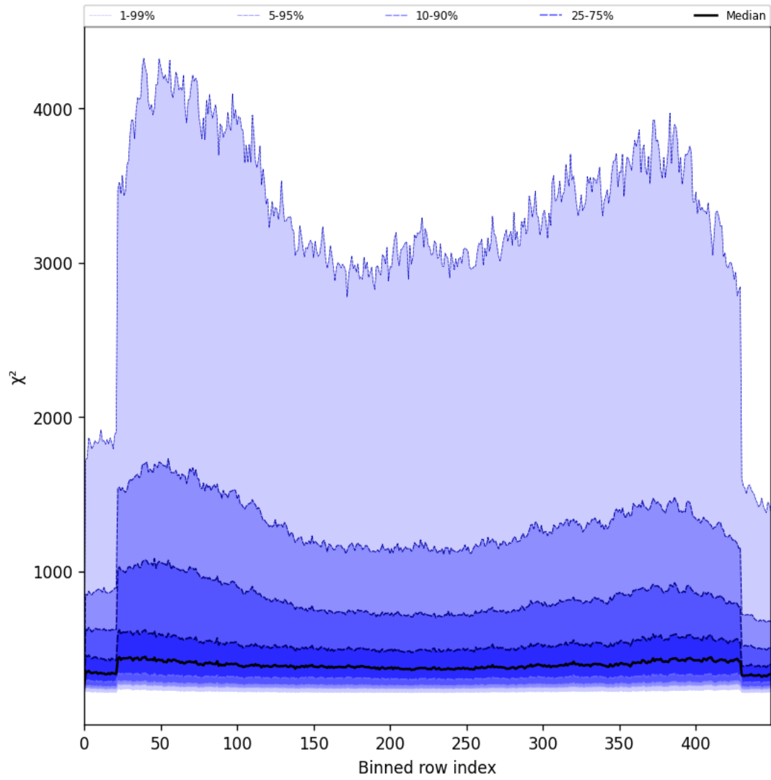
Figure 57: Along track statistics of “ \chi^2 ” for 2025-06-23 to 2025-06-24
