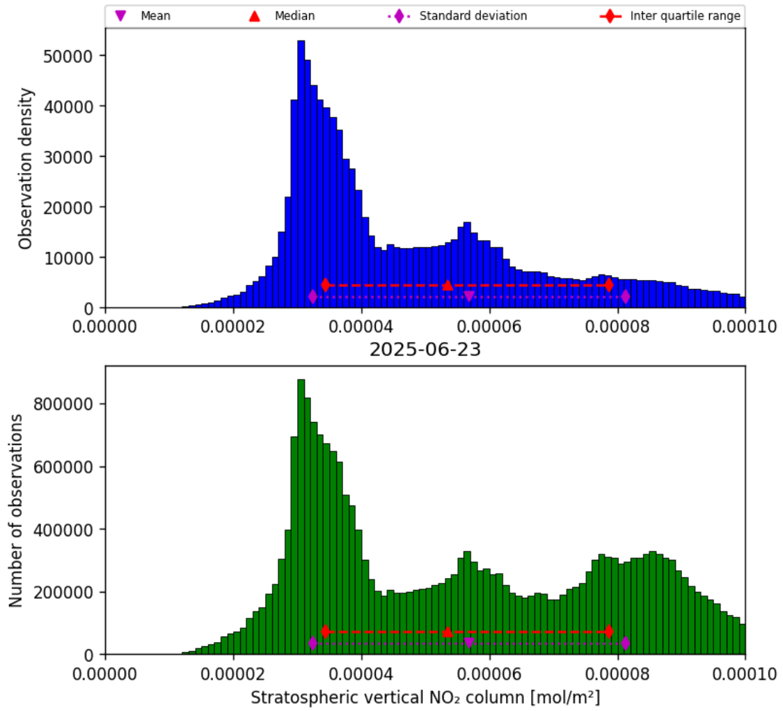
Figure 34: Histogram of “Stratospheric vertical NO 2 column” for 2025-06-23 to 2025-06-24
