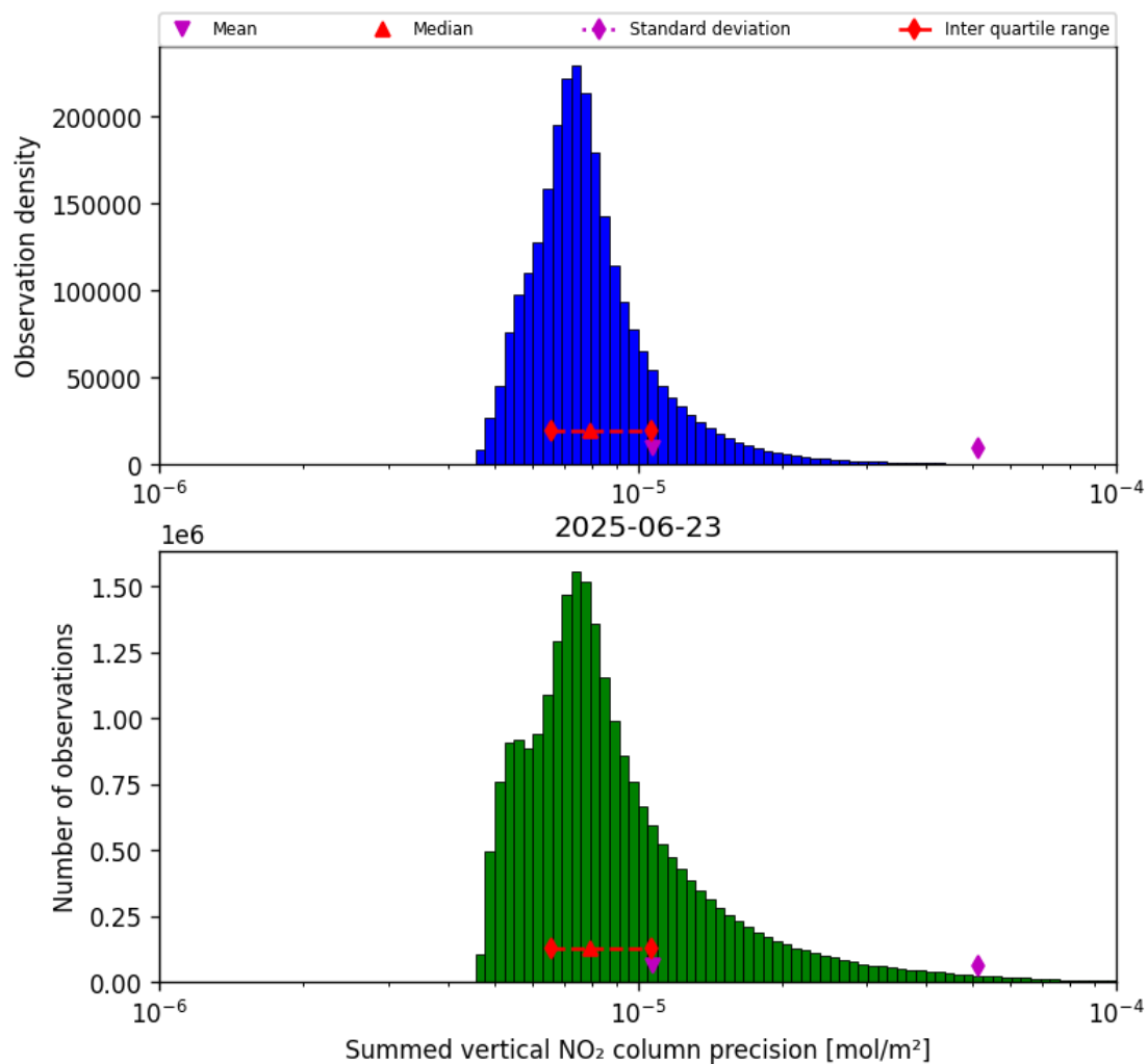
Figure 39: Histogram of “Summed vertical NO 2 column precision” for 2025-06-23 to 2025-06-24
