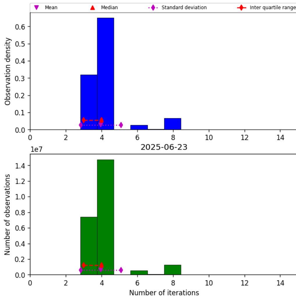
Figure 32: Histogram of “Number of iterations” for 2025-06-23 to 2025-06-24
