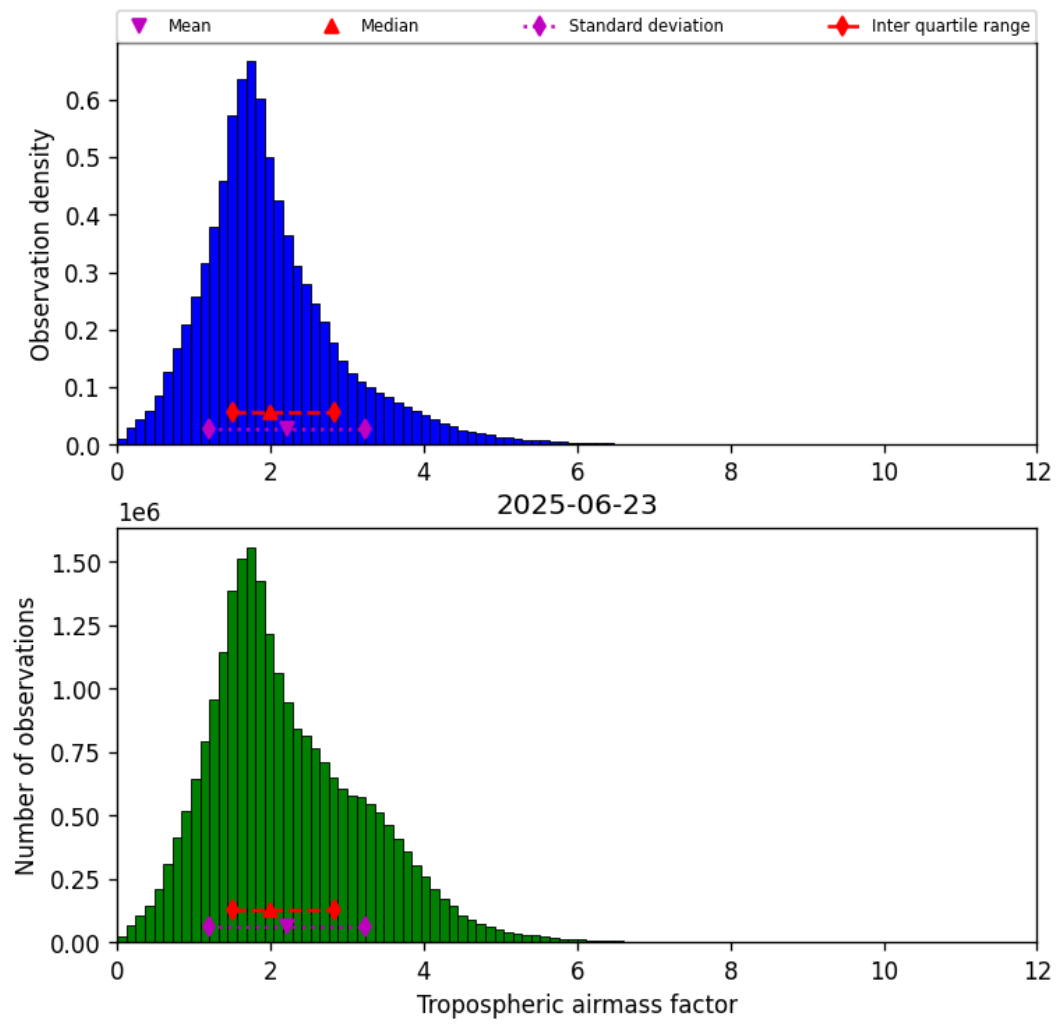
Figure 29: Histogram of “Tropospheric airmass factor” for 2025-06-23 to 2025-06-24
