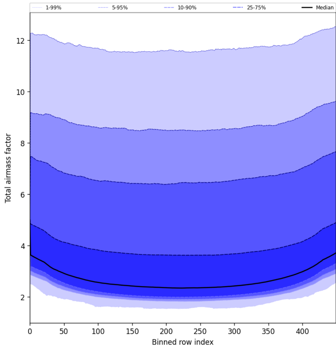
Figure 47: Along track statistics of “Total airmass factor” for 2025-06-23 to 2025-06-24
