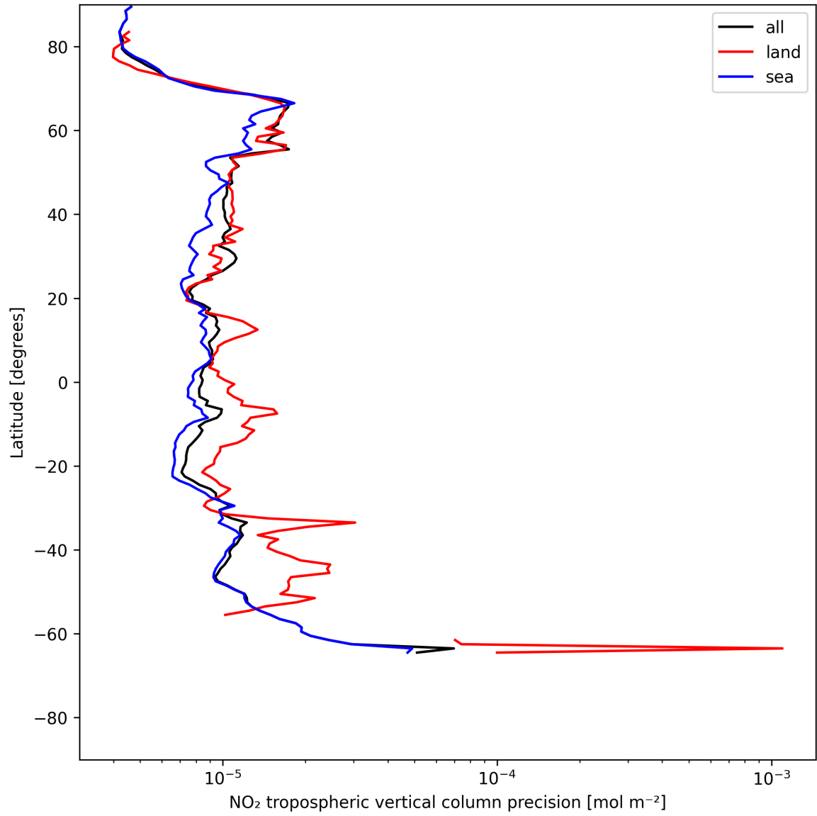
Figure 11: Zonal average of “NO 2 tropospheric vertical column precision” for 2025-06-23 to 2025-06-24.
