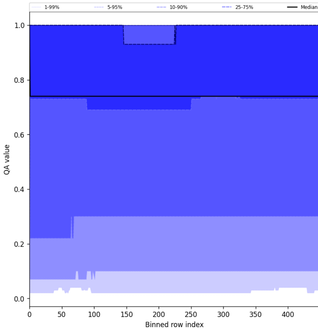
Figure 43: Along track statistics of “QA value” for 2025-06-23 to 2025-06-24
