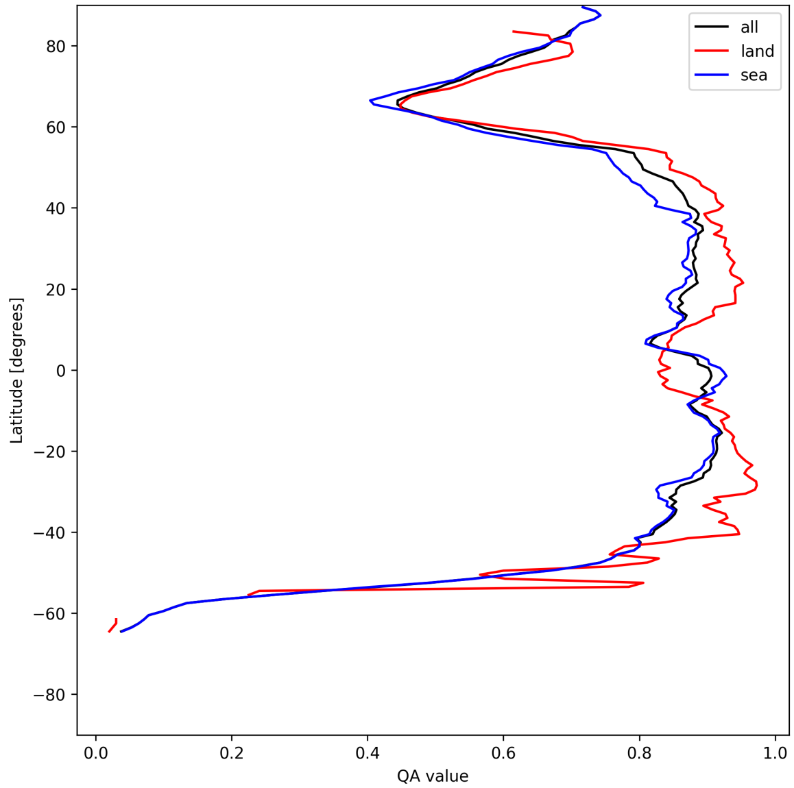
Figure 9: Zonal average of “QA value” for 2025-06-23 to 2025-06-24.
