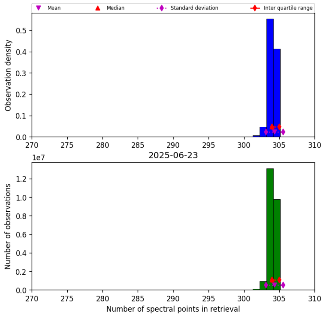
Figure 31: Histogram of “Number of spectral points in retrieval” for 2025-06-23 to 2025-06-24
