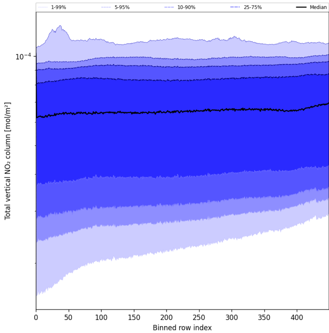
Figure 53: Along track statistics of “Total vertical NO 2 column” for 2025-06-23 to 2025-06-24
