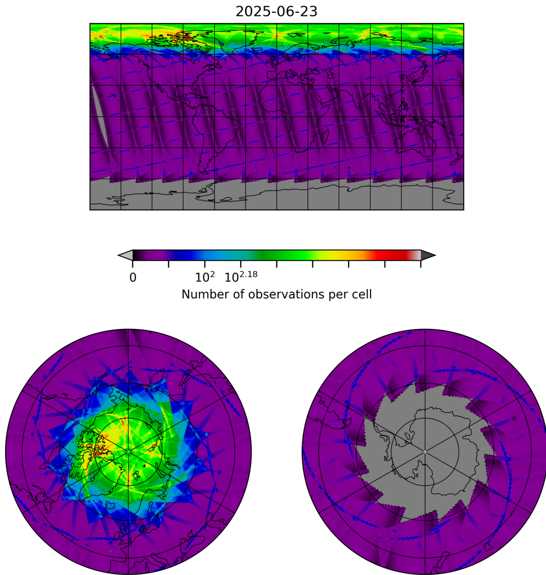
Figure 8: Map of the number of observations for 2025-06-23 to 2025-06-24
