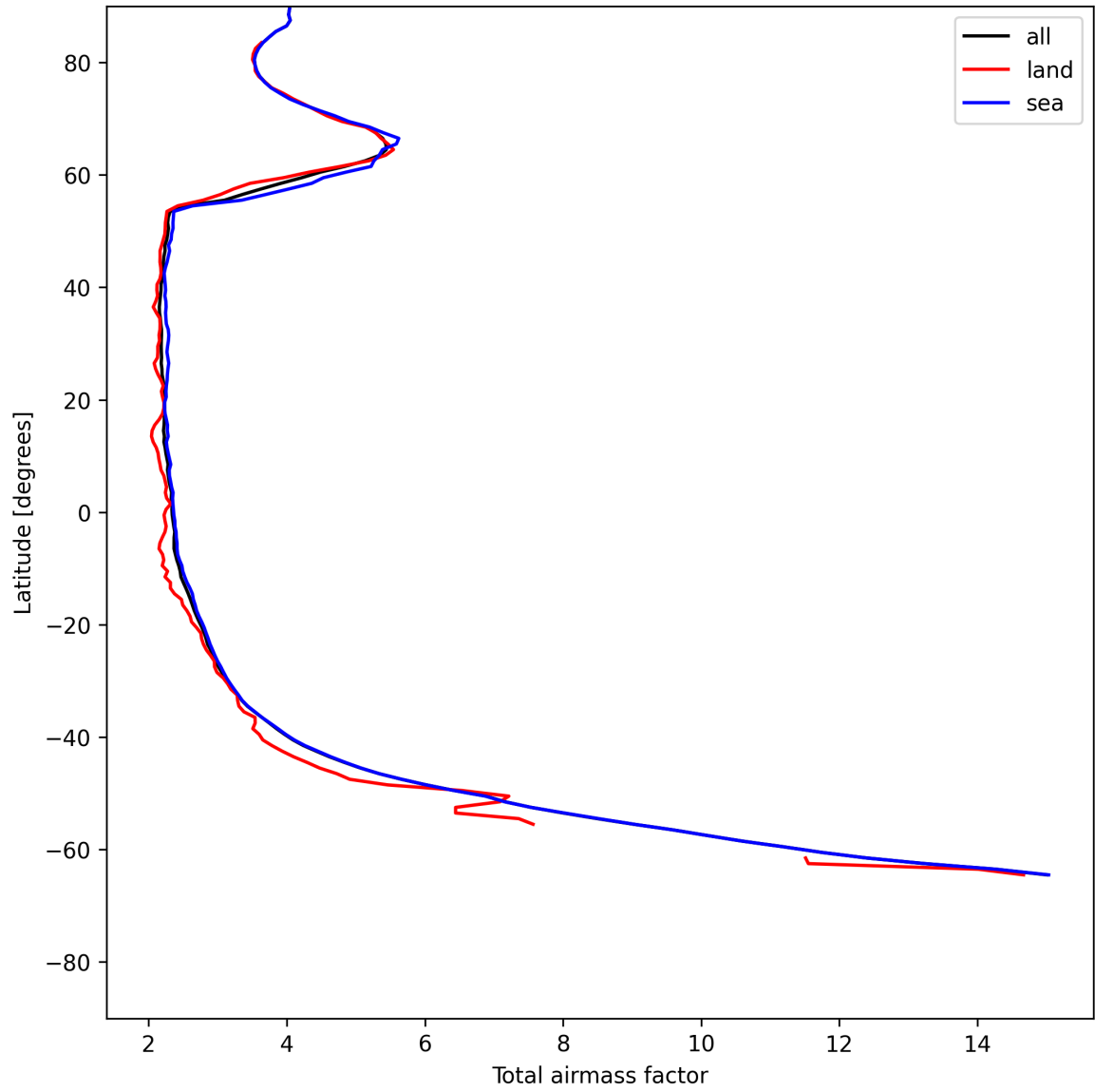
Figure 13: Zonal average of “Total airmass factor” for 2025-06-23 to 2025-06-24.
