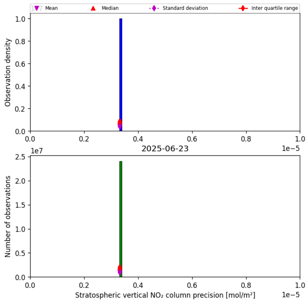
Figure 35: Histogram of “Stratospheric vertical NO 2 column precision” for 2025-06-23 to 2025-06-24
