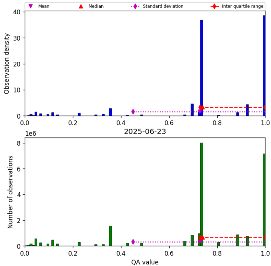
Figure 26: Histogram of “QA value” for 2025-06-23 to 2025-06-24
