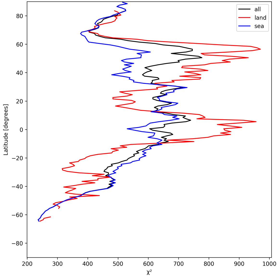
Figure 23: Zonal average of “ \chi^2 ” for 2025-06-23 to 2025-06-24.
