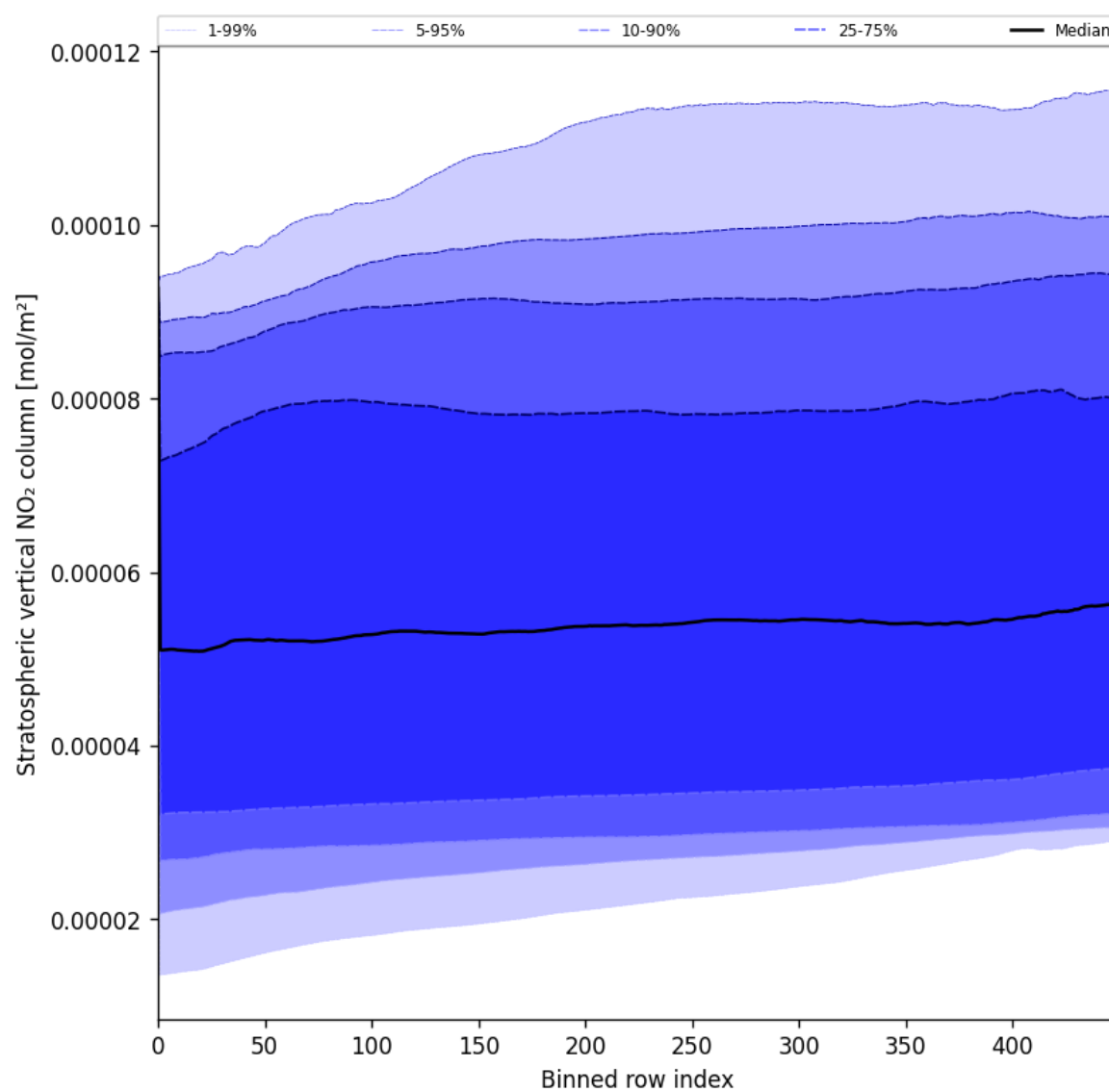
Figure 51: Along track statistics of “Stratospheric vertical NO 2 column” for 2025-06-23 to 2025-06-24
