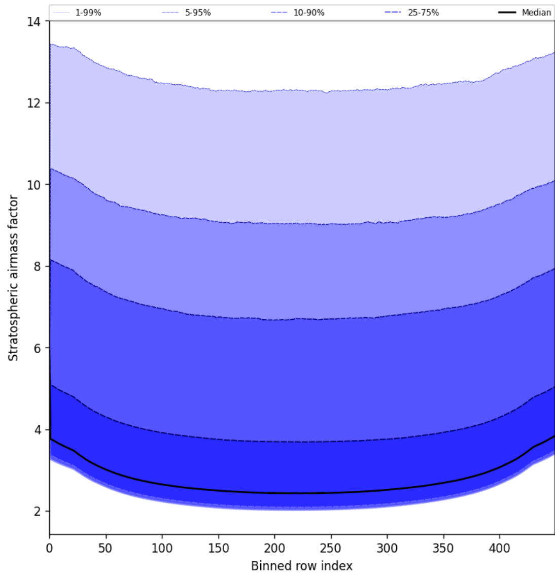
Figure 59: Along track statistics of “Stratospheric airmass factor” for 2025-06-23 to 2025-06-24
