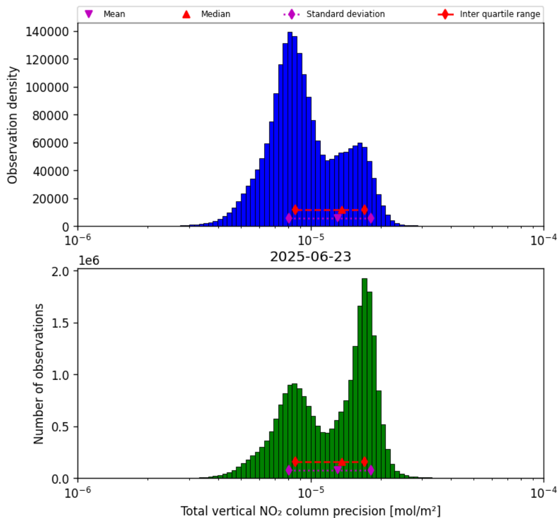
Figure 37: Histogram of “Total vertical NO 2 column precision” for 2025-06-23 to 2025-06-24
