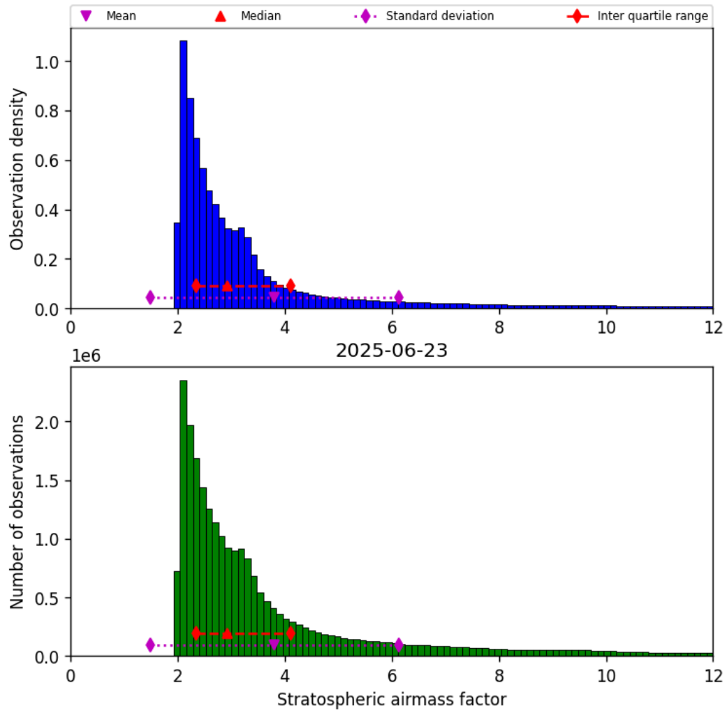
Figure 42: Histogram of “Stratospheric airmass factor” for 2025-06-23 to 2025-06-24
