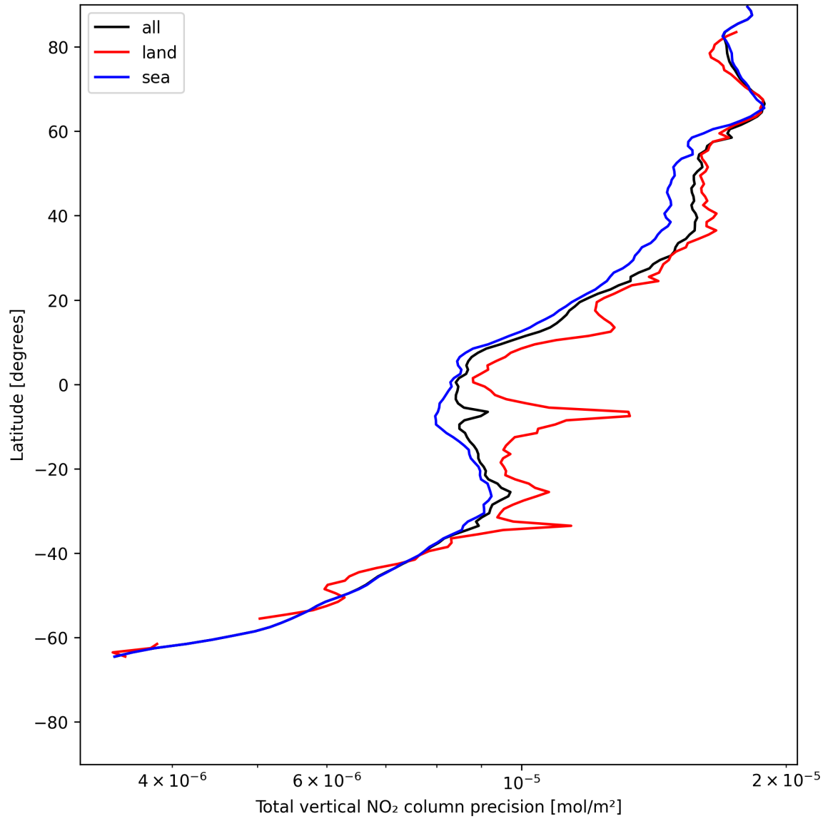
Figure 20: Zonal average of “Total vertical NO 2 column precision” for 2025-06-23 to 2025-06-24.
