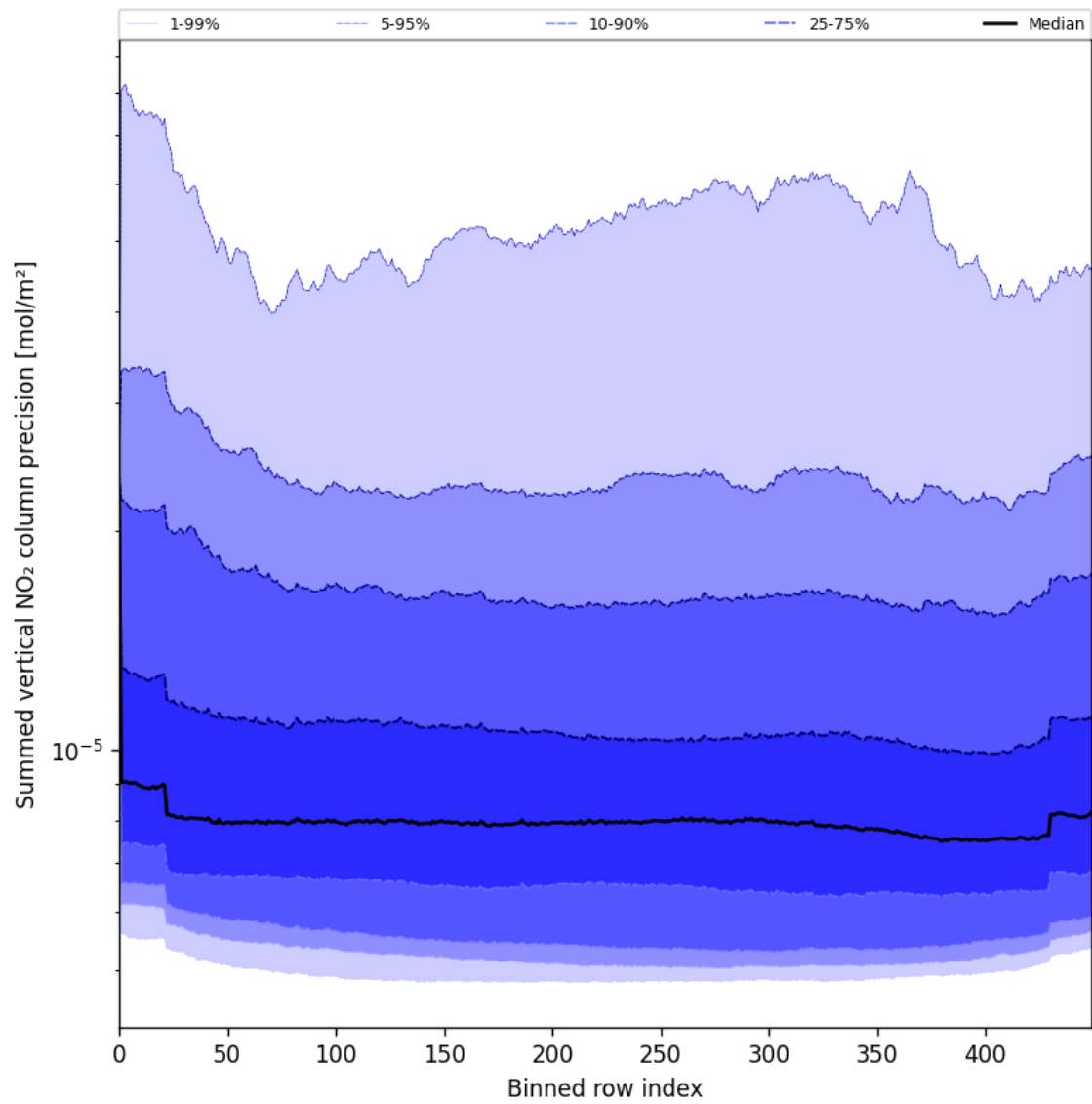
Figure 56: Along track statistics of “Summed vertical NO 2 column precision” for 2025-06-23 to 2025-06-24
