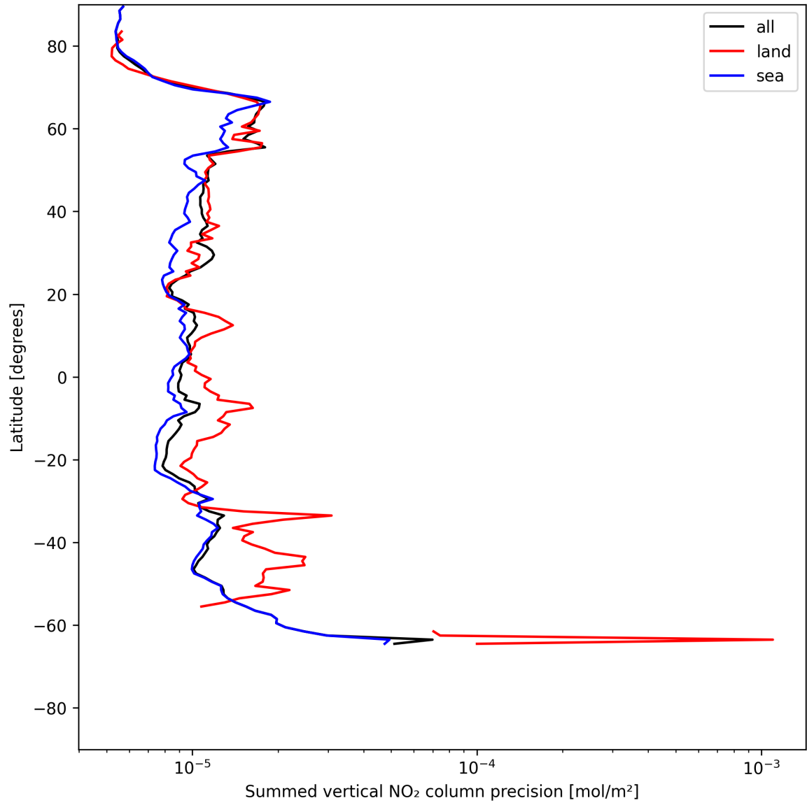
Figure 22: Zonal average of “Summed vertical NO 2 column precision” for 2025-06-23 to 2025-06-24.
