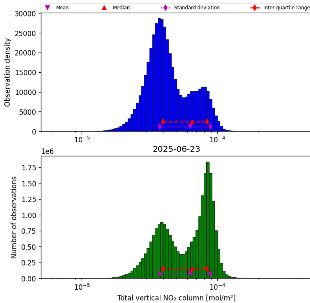
Figure 36: Histogram of “Total vertical NO 2 column” for 2025-06-23 to 2025-06-24
