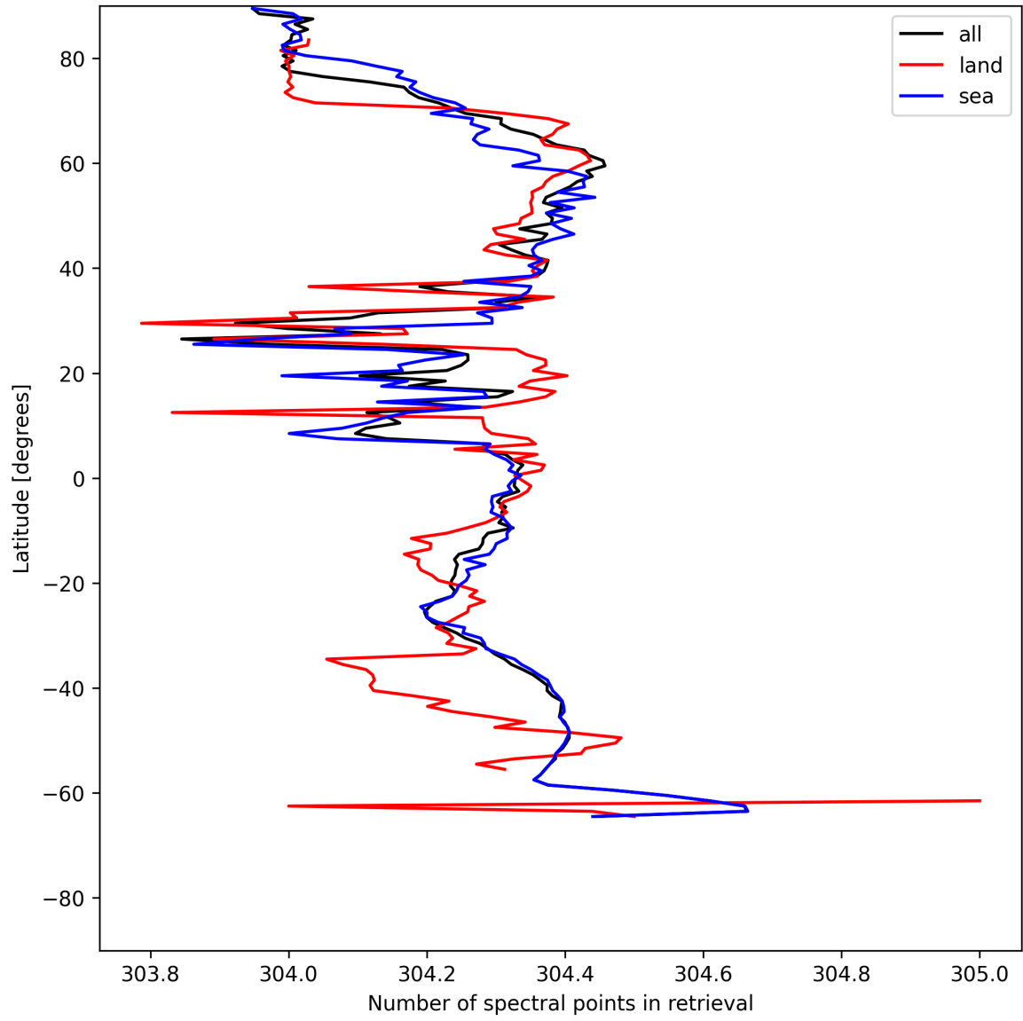
Figure 14: Zonal average of “Number of spectral points in retrieval” for 2025-06-23 to 2025-06-24.
