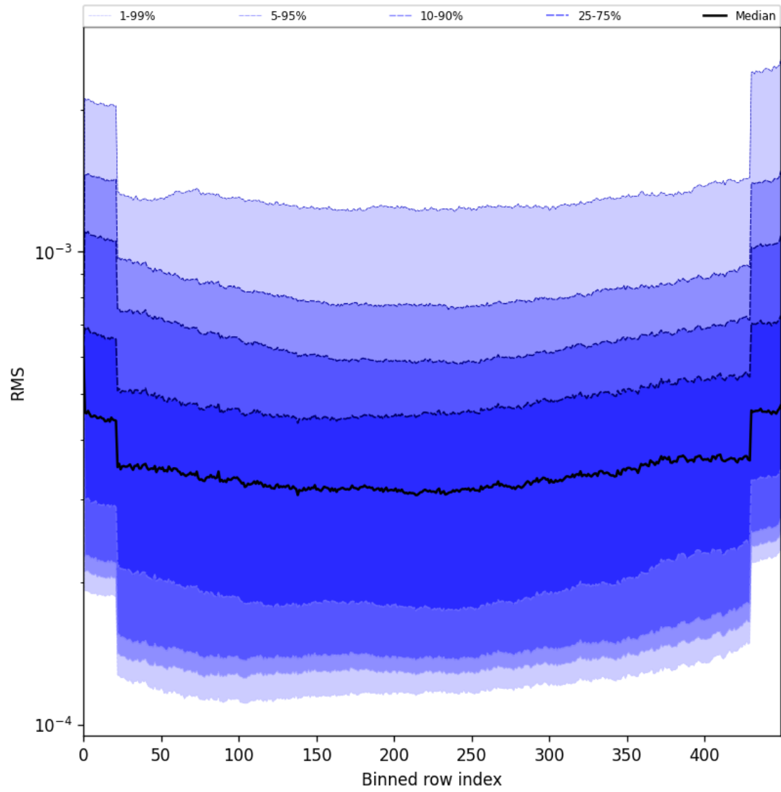
Figure 58: Along track statistics of “RMS” for 2025-06-23 to 2025-06-24
