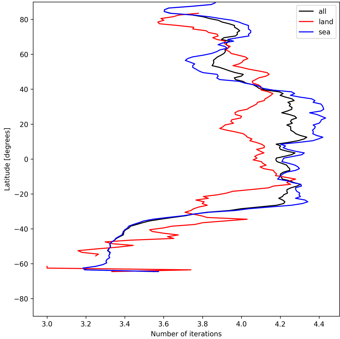
Figure 15: Zonal average of “Number of iterations” for 2025-06-23 to 2025-06-24.
