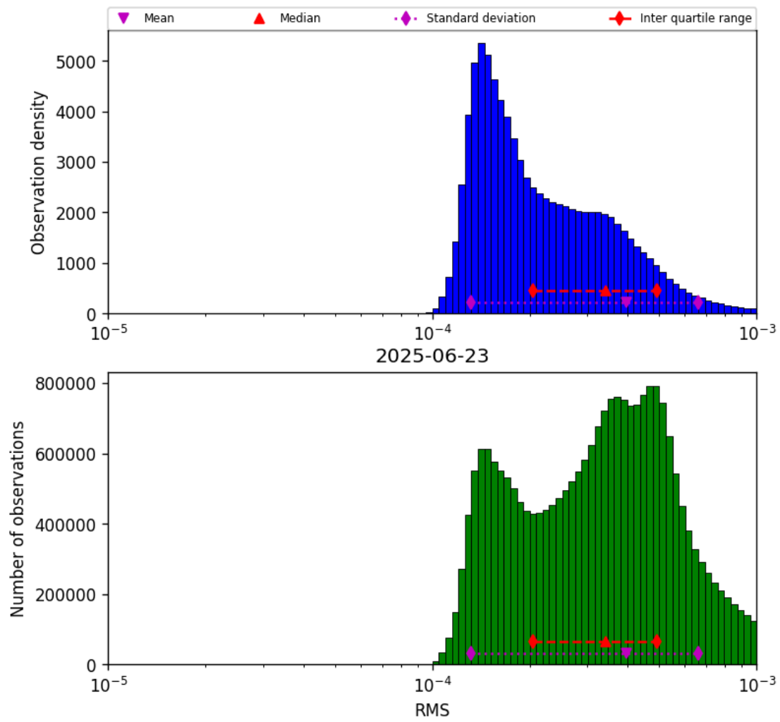
Figure 41: Histogram of “RMS” for 2025-06-23 to 2025-06-24
