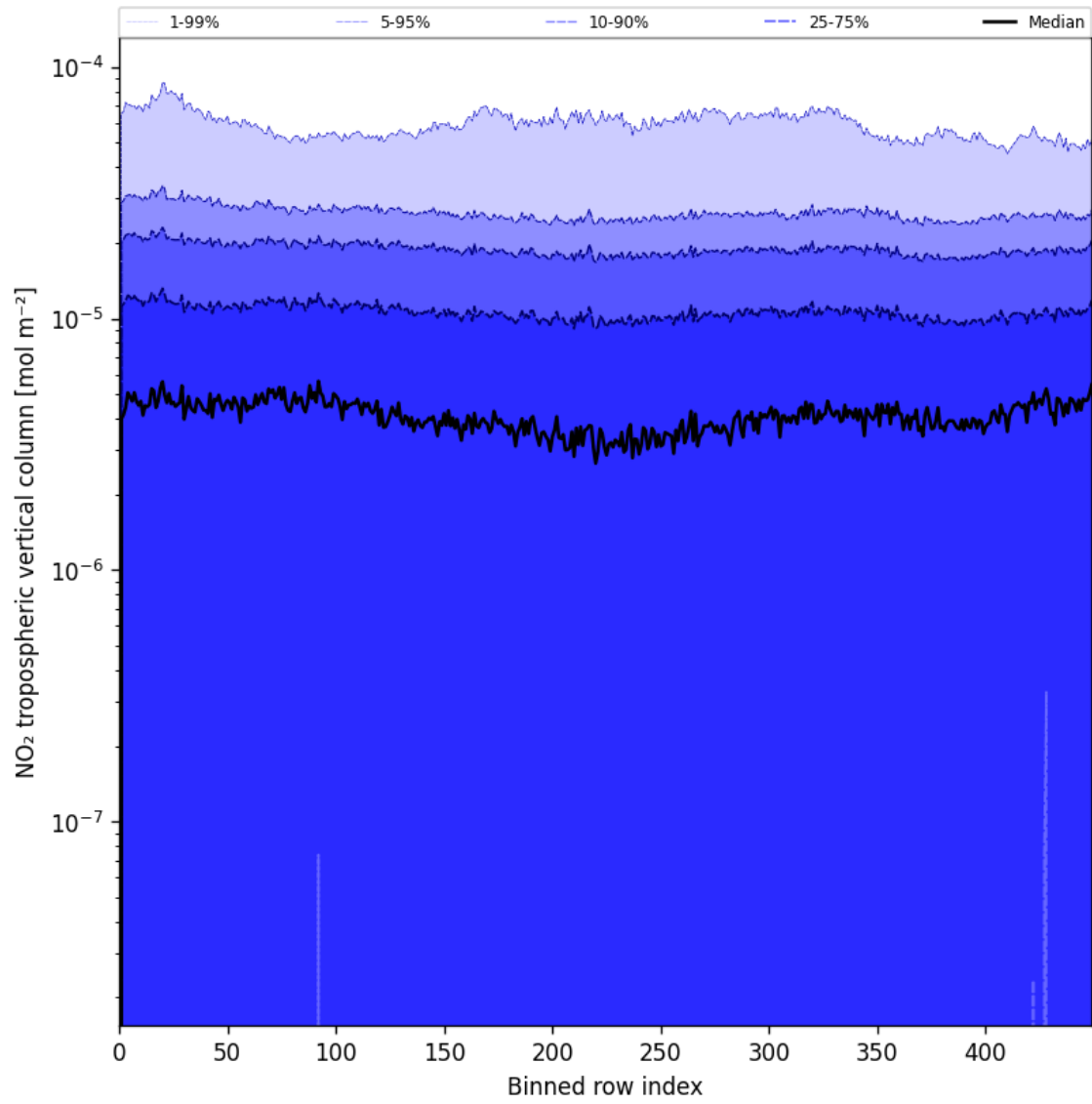
Figure 44: Along track statistics of “NO 2 tropospheric vertical column” for 2025-06-23 to 2025-06-24
