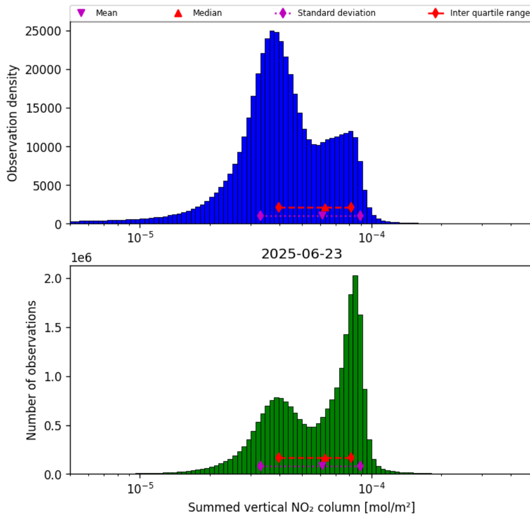
Figure 38: Histogram of “Summed vertical NO 2 column” for 2025-06-23 to 2025-06-24
