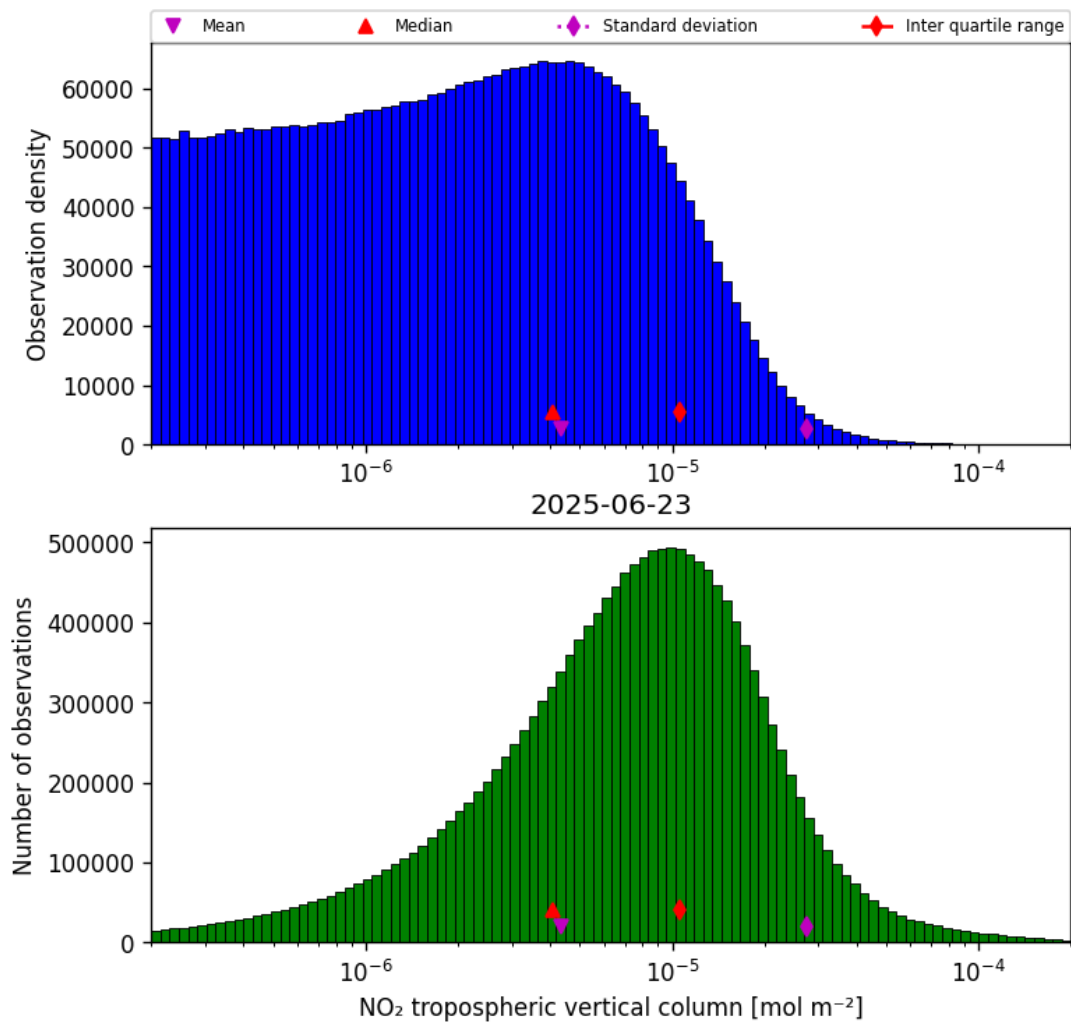
Figure 27: Histogram of “NO 2 tropospheric vertical column” for 2025-06-23 to 2025-06-24
