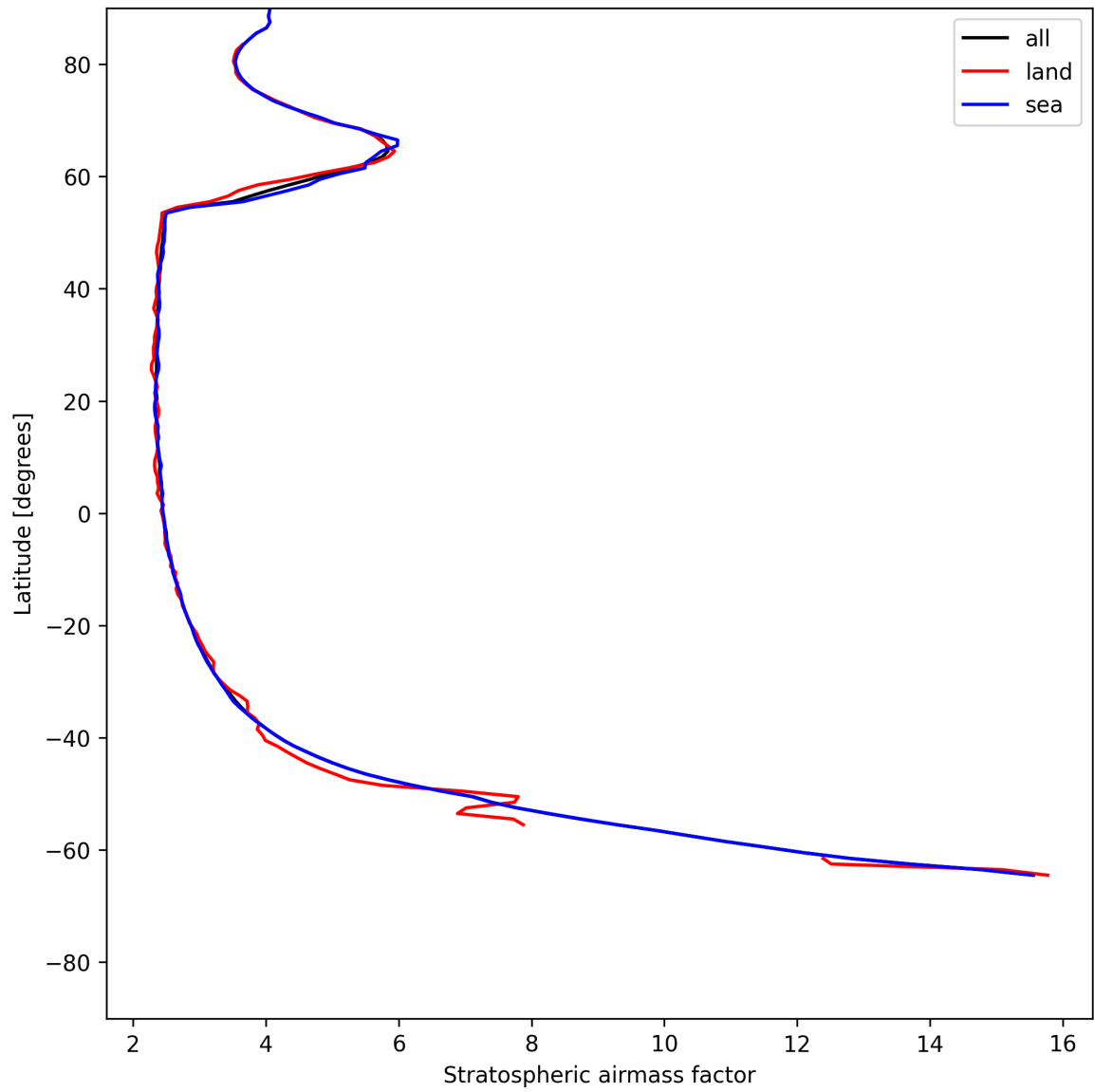
Figure 25: Zonal average of “Stratospheric air mass factor” for 2025-06-23 to 2025-06-24.
