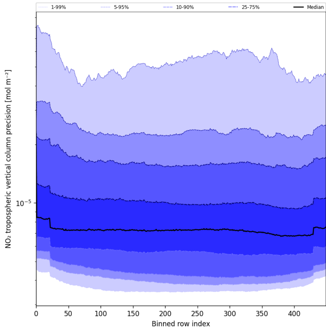
Figure 45: Along track statistics of “NO 2 tropospheric vertical column precision” for 2025-06-23 to 2025-06-24
