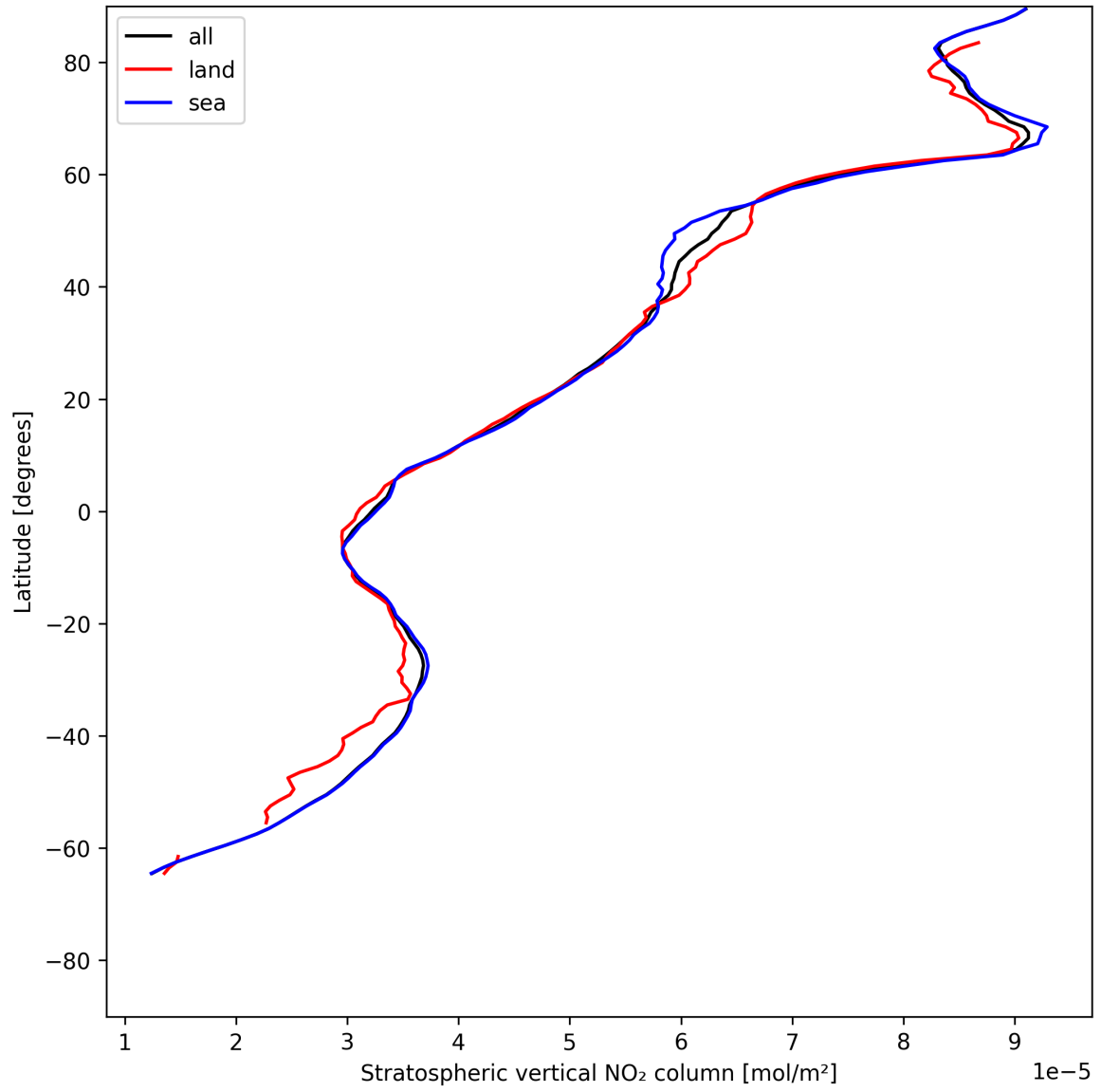
Figure 17: Zonal average of “Stratospheric vertical NO 2 column” for 2025-06-23 to 2025-06-24.
