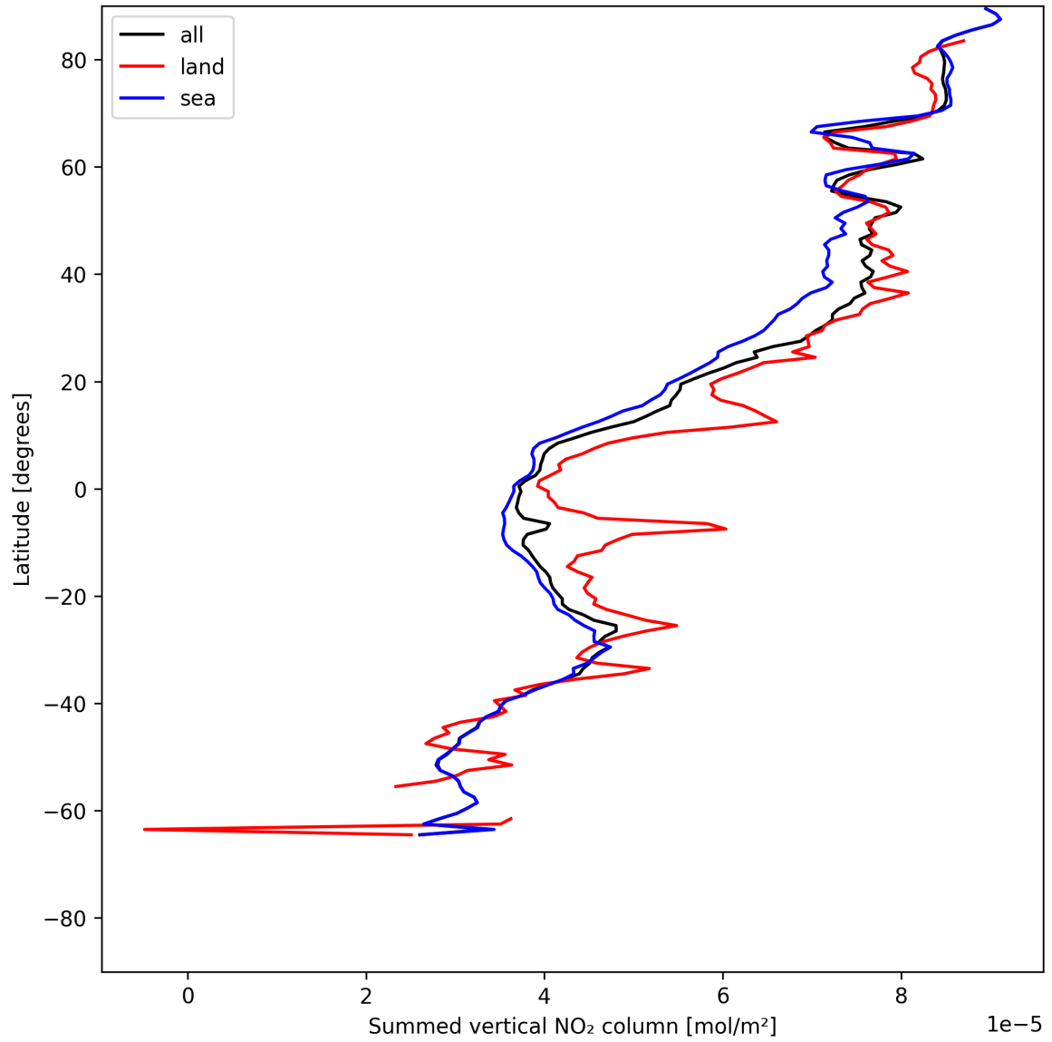
Figure 21: Zonal average of “Summed vertical NO 2 column” for 2025-06-23 to 2025-06-24.
