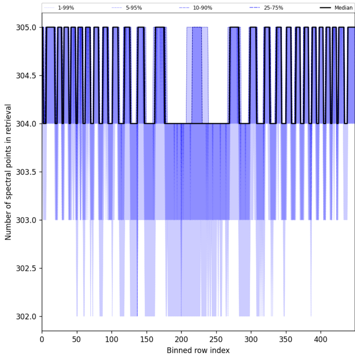
Figure 48: Along track statistics of “Number of spectral points in retrieval” for 2025-06-23 to 2025-06-24
