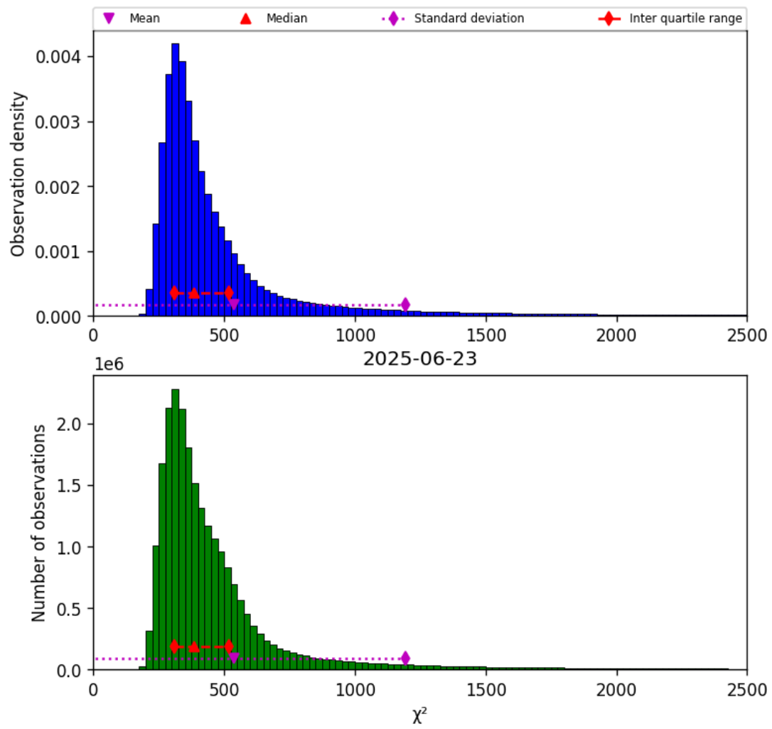
Figure 40: Histogram of “ \chi^2 ” for 2025-06-23 to 2025-06-24
