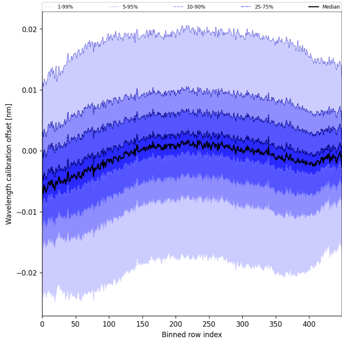
Figure 50: Along track statistics of “Wavelength calibration offset” for 2025-06-23 to 2025-06-24
