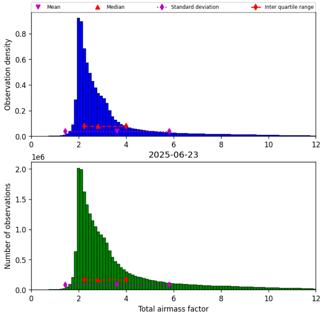
Figure 30: Histogram of “Total airmass factor” for 2025-06-23 to 2025-06-24
