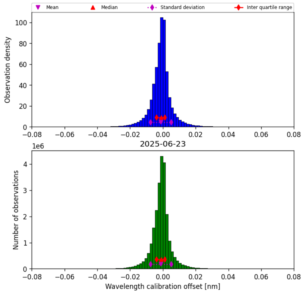
Figure 33: Histogram of “Wavelength calibration offset” for 2025-06-23 to 2025-06-24
