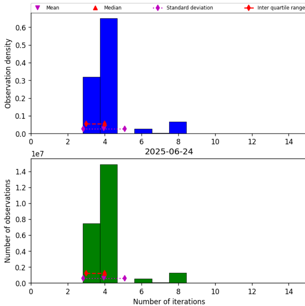
Figure 32: Histogram of “Number of iterations” for 2025-06-24 to 2025-06-25
