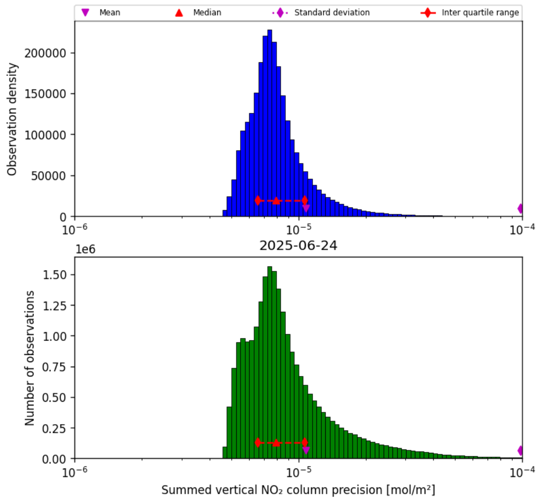
Figure 39: Histogram of “Summed vertical NO 2 column precision” for 2025-06-24 to 2025-06-25
