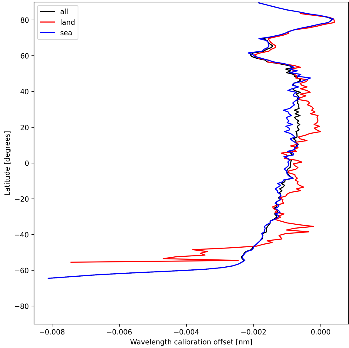
Figure 16: Zonal average of “Wavelength calibration offset” for 2025-06-24 to 2025-06-25.
