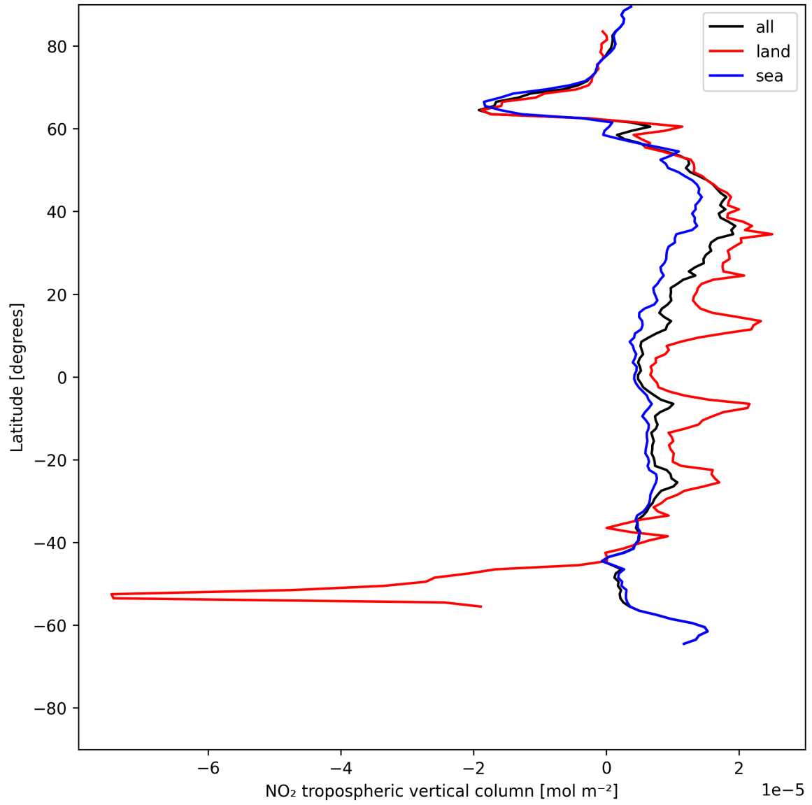
Figure 10: Zonal average of “NO 2 tropospheric vertical column” for 2025-06-24 to 2025-06-25.
