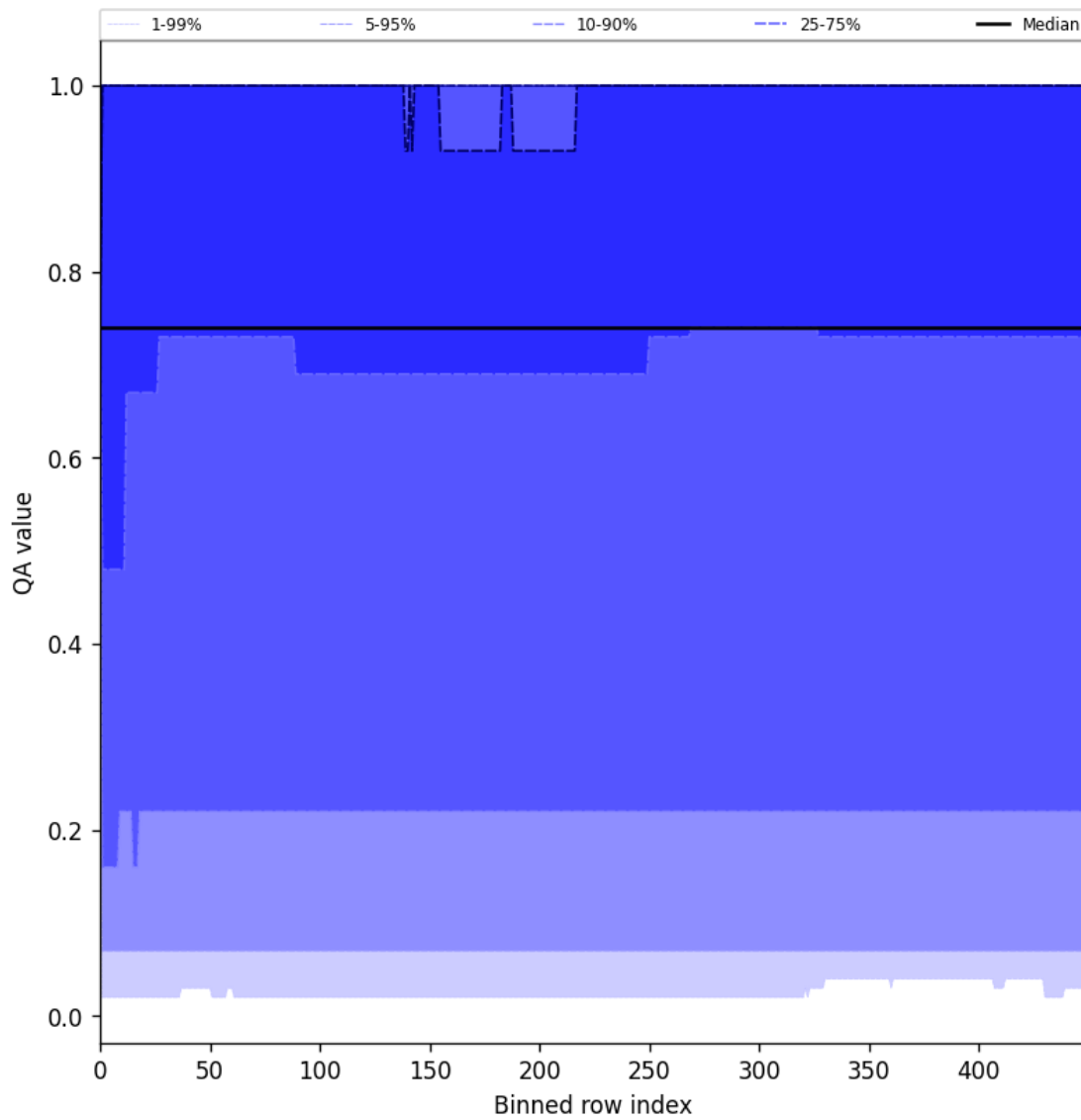
Figure 43: Along track statistics of “QA value” for 2025-06-24 to 2025-06-25
