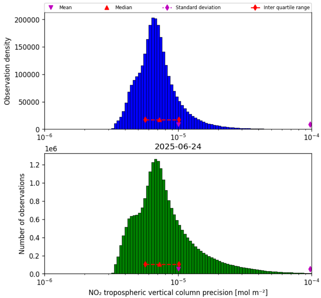
Figure 28: Histogram of “NO 2 tropospheric vertical column precision” for 2025-06-24 to 2025-06-25
