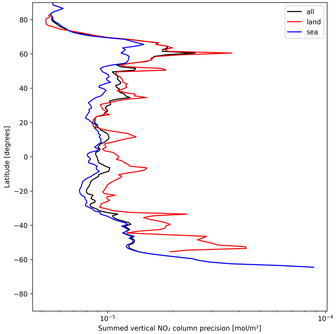
Figure 22: Zonal average of “Summed vertical NO 2 column precision” for 2025-06-24 to 2025-06-25.
