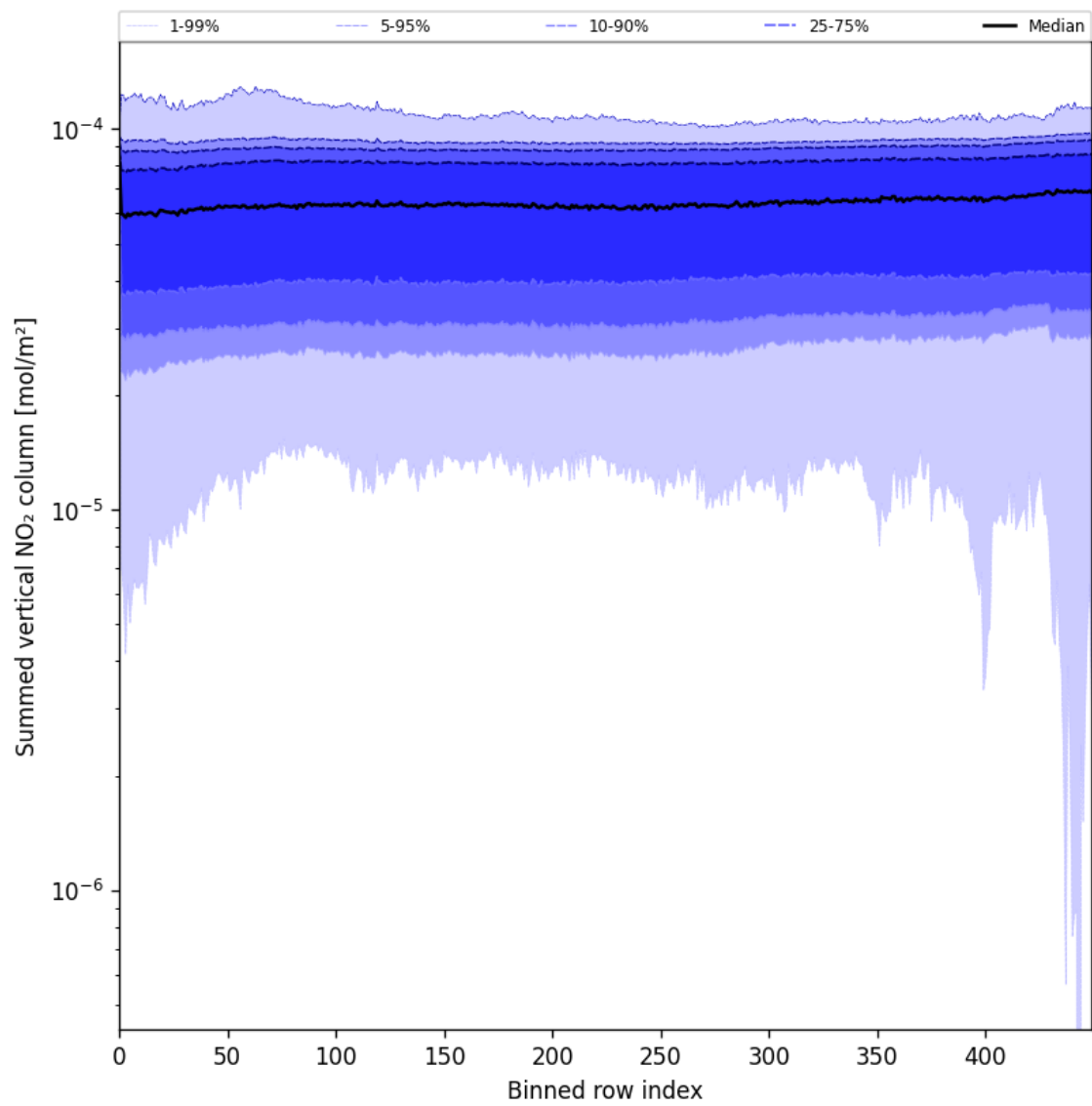
Figure 55: Along track statistics of “Summed vertical NO 2 column” for 2025-06-24 to 2025-06-25
