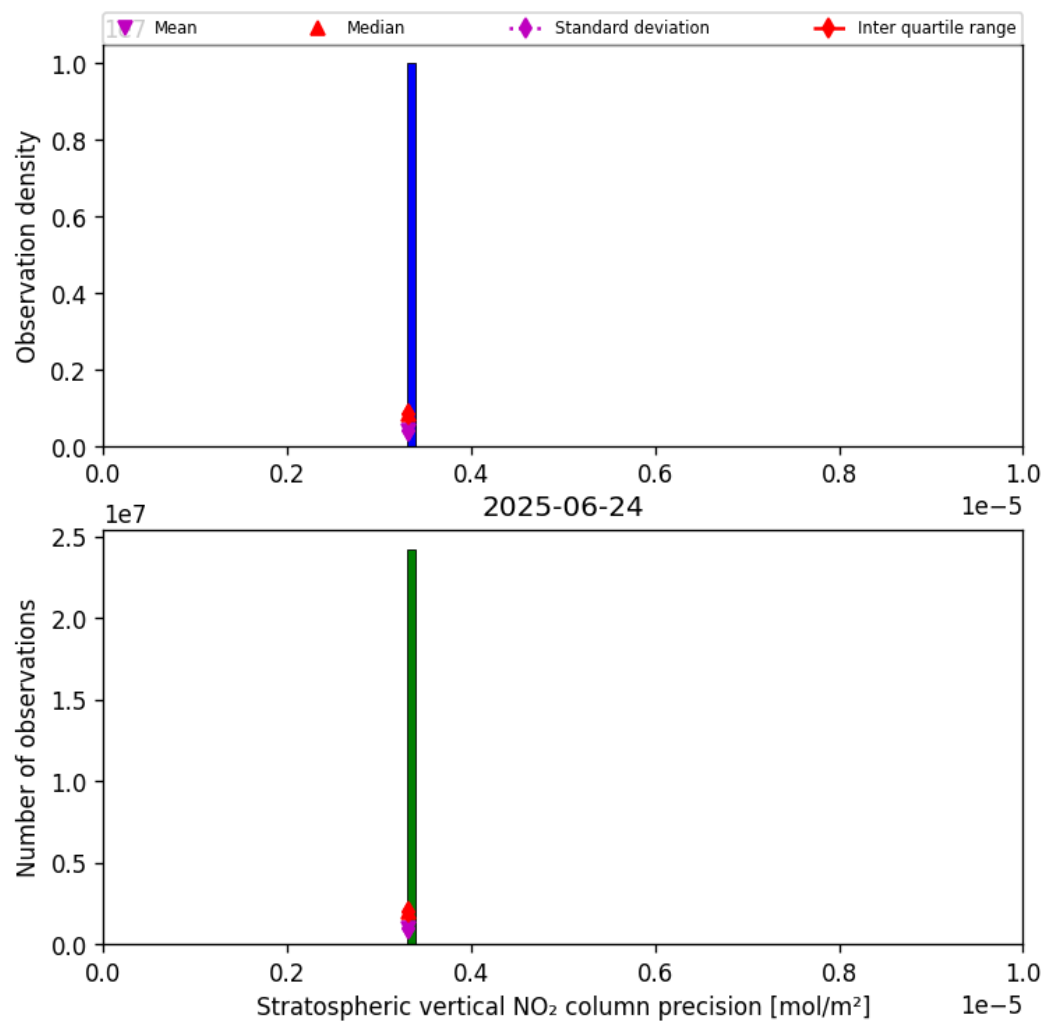
Figure 35: Histogram of “Stratospheric vertical NO 2 column precision” for 2025-06-24 to 2025-06-25
