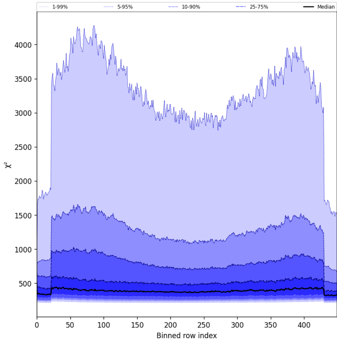
Figure 57: Along track statistics of “ \chi^2 ” for 2025-06-24 to 2025-06-25
