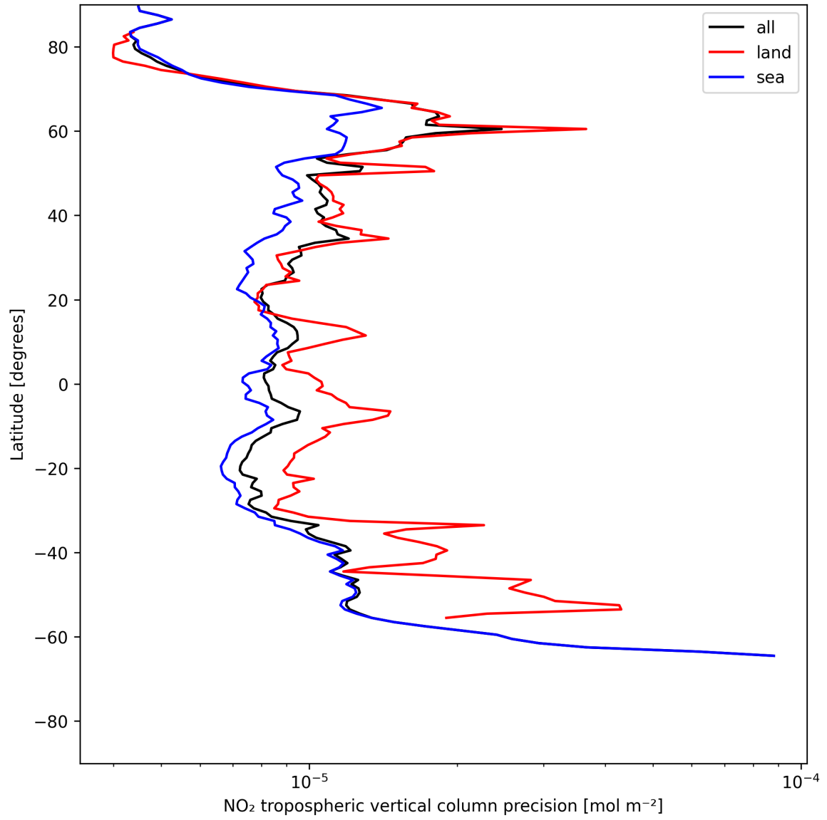
Figure 11: Zonal average of “NO 2 tropospheric vertical column precision” for 2025-06-24 to 2025-06-25.
