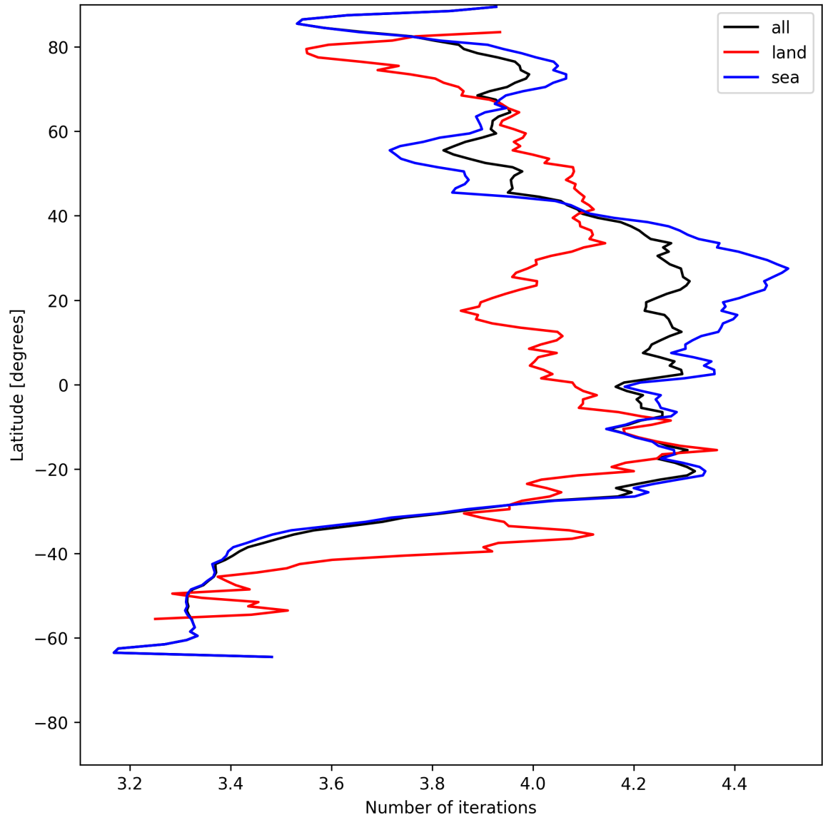
Figure 15: Zonal average of “Number of iterations” for 2025-06-24 to 2025-06-25.
