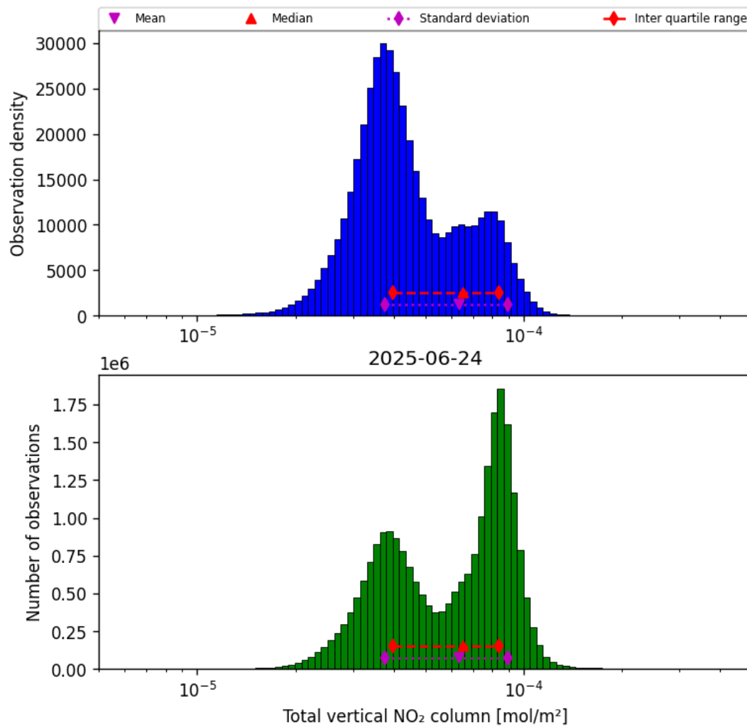
Figure 36: Histogram of “Total vertical NO 2 column” for 2025-06-24 to 2025-06-25
