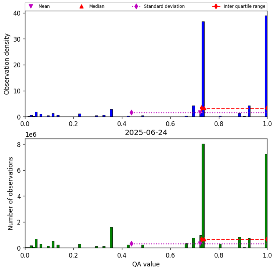
Figure 26: Histogram of “QA value” for 2025-06-24 to 2025-06-25
