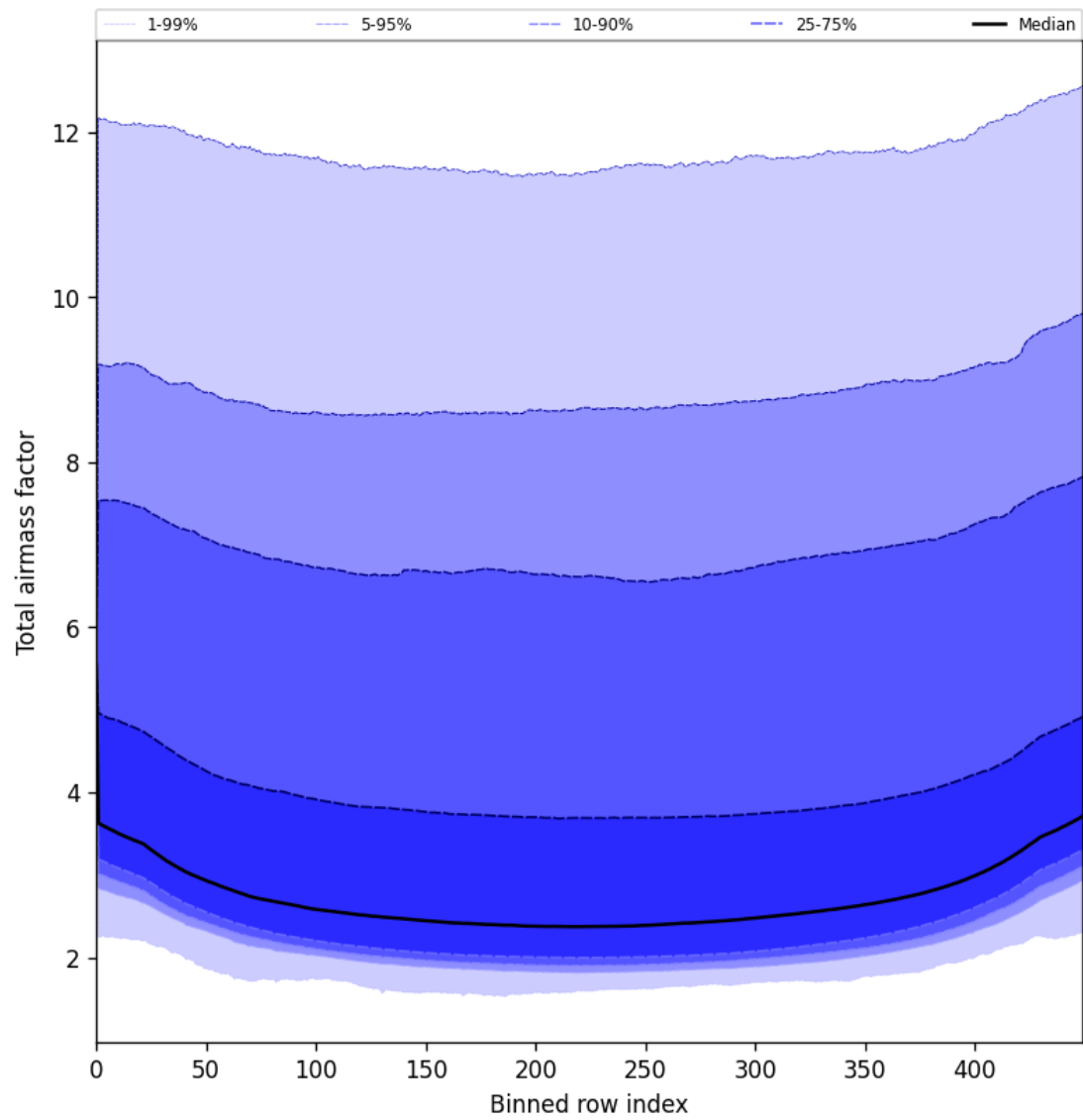
Figure 47: Along track statistics of “Total airmass factor” for 2025-06-24 to 2025-06-25
