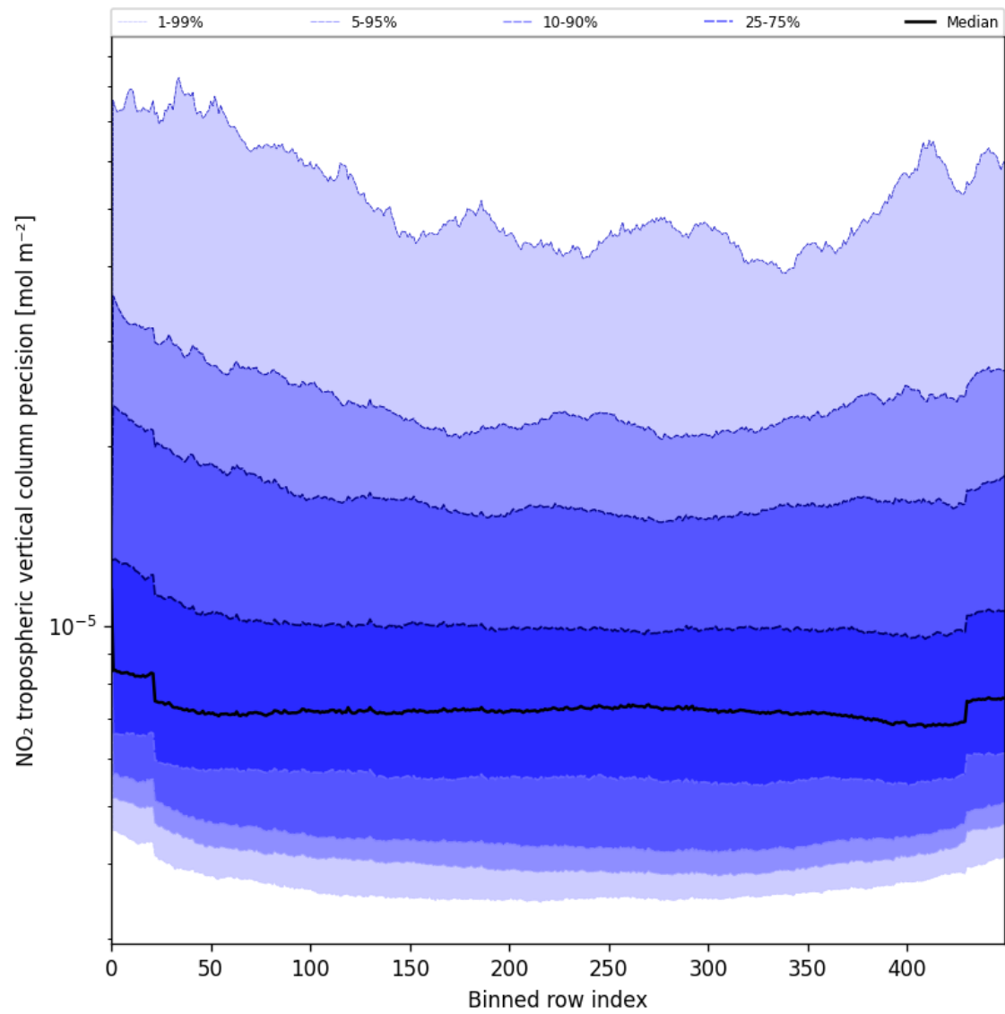
Figure 45: Along track statistics of “NO 2 tropospheric vertical column precision” for 2025-06-24 to 2025-06-25
