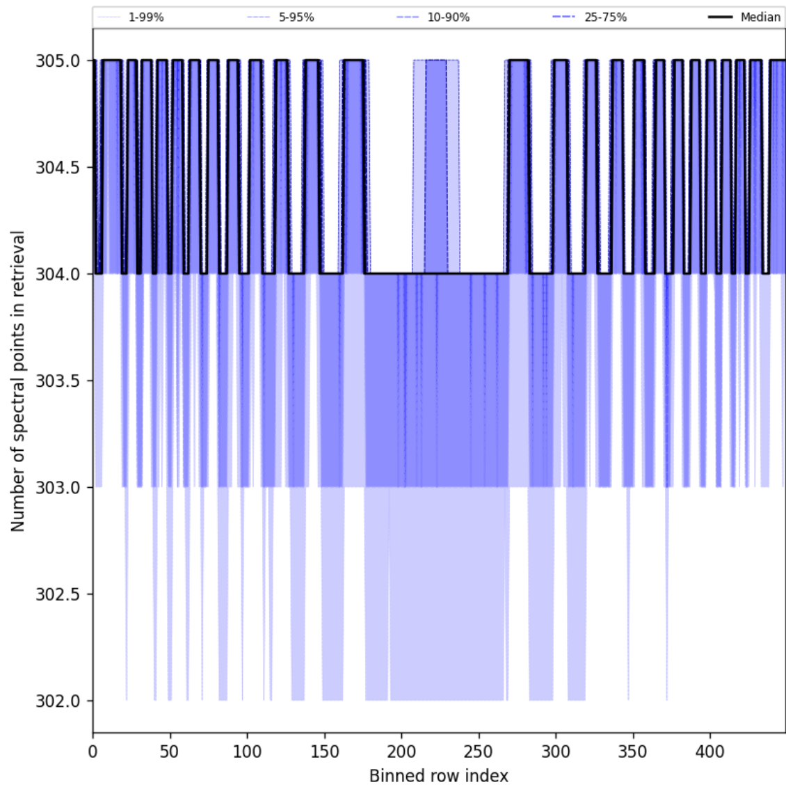
Figure 48: Along track statistics of “Number of spectral points in retrieval” for 2025-06-24 to 2025-06-25
