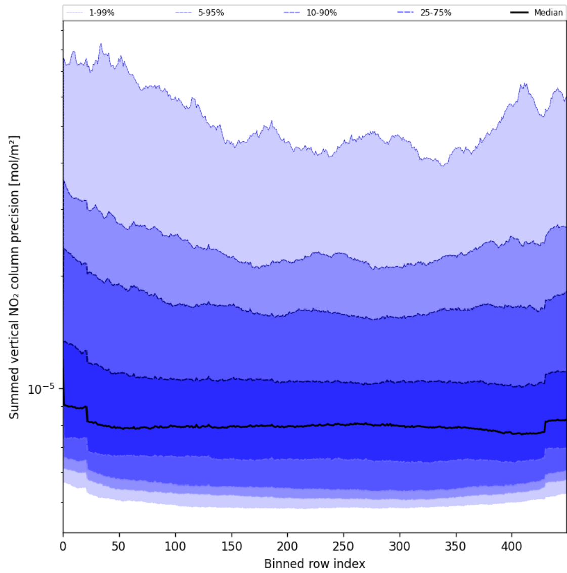
Figure 56: Along track statistics of “Summed vertical NO 2 column precision” for 2025-06-24 to 2025-06-25
