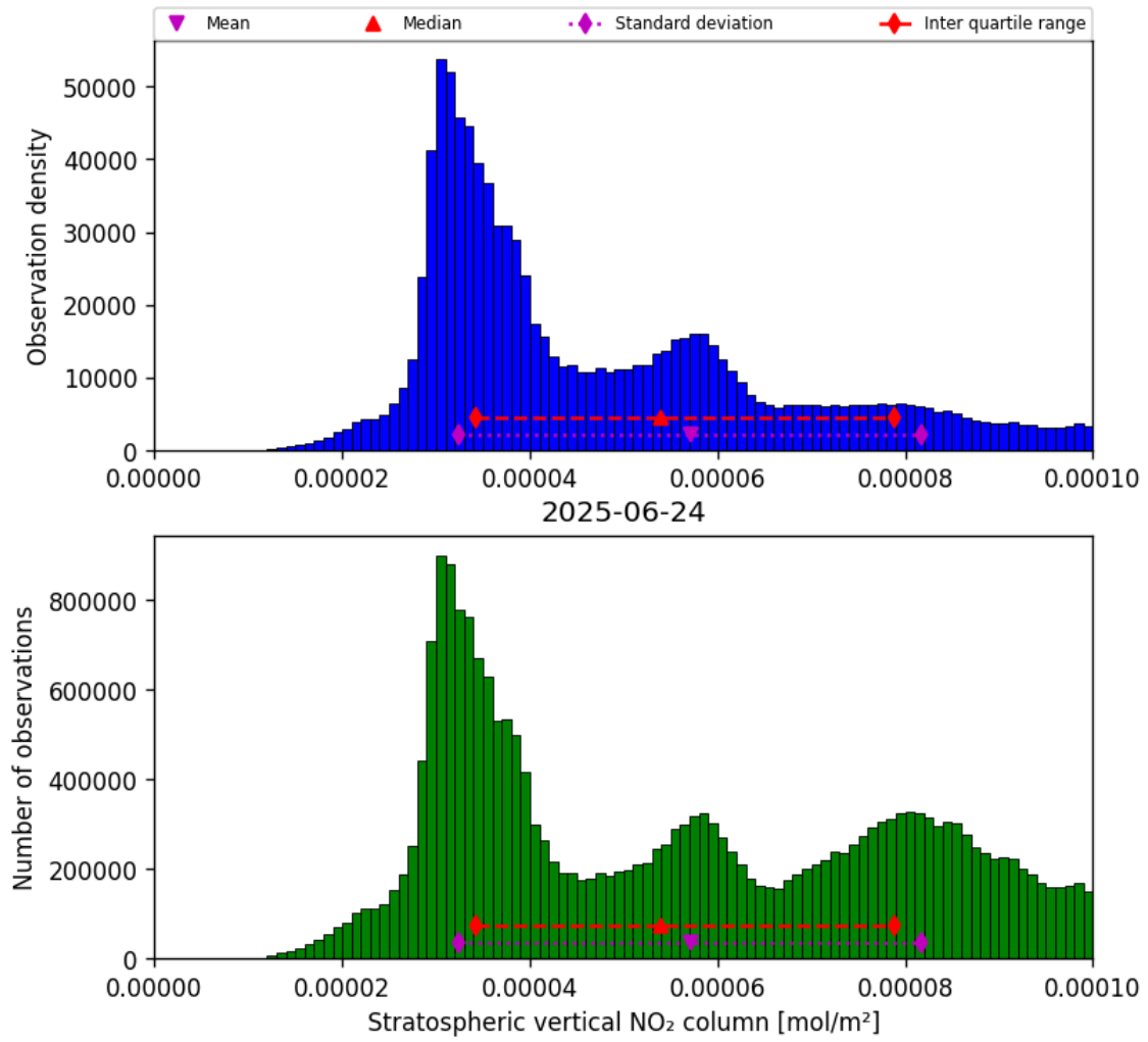
Figure 34: Histogram of “Stratospheric vertical NO 2 column” for 2025-06-24 to 2025-06-25
