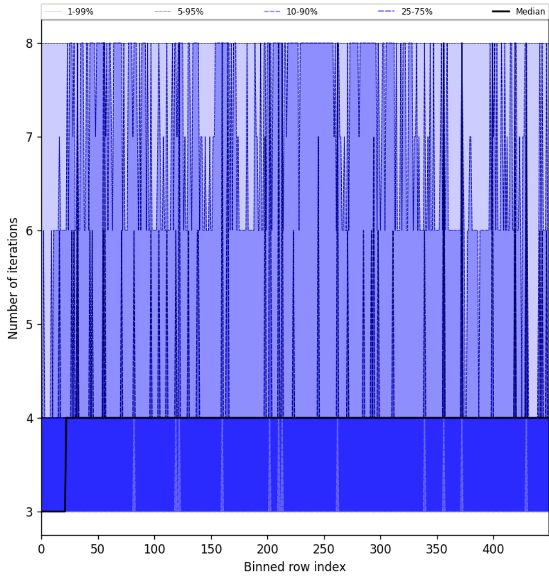
Figure 49: Along track statistics of “Number of iterations” for 2025-06-24 to 2025-06-25
