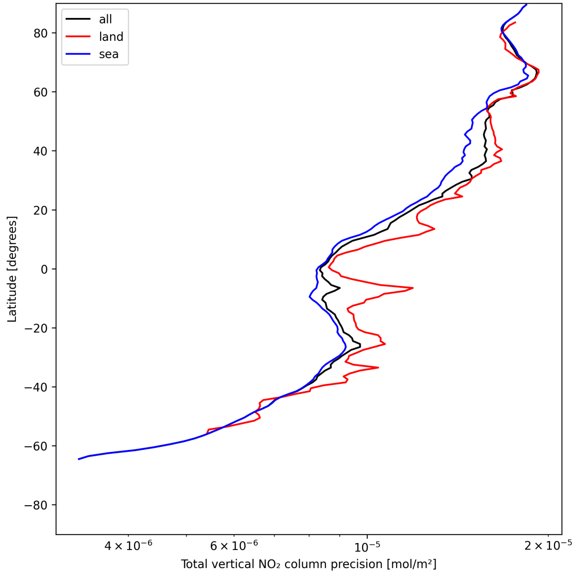
Figure 20: Zonal average of “Total vertical NO 2 column precision” for 2025-06-24 to 2025-06-25.
