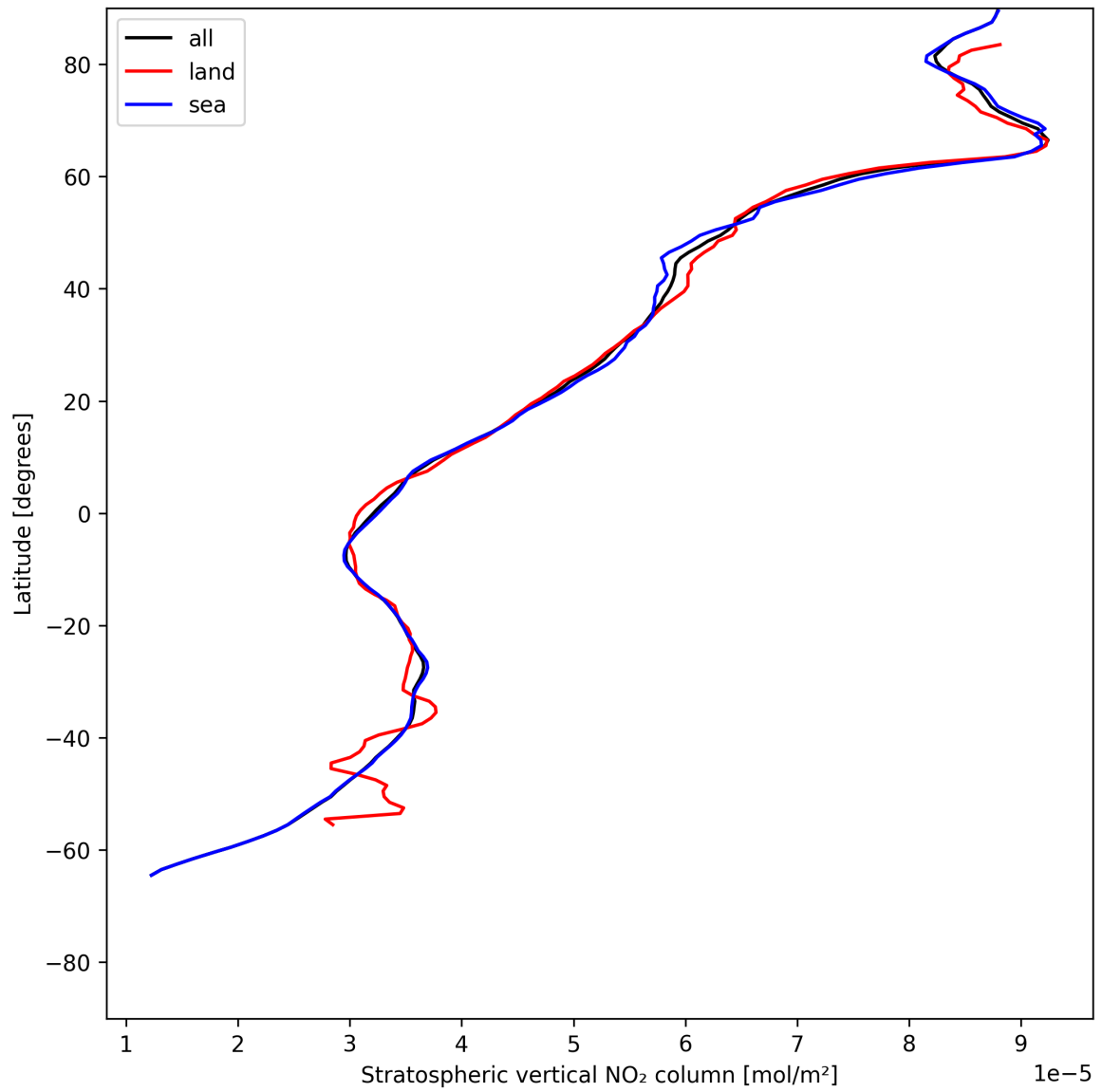
Figure 17: Zonal average of “Stratospheric vertical NO 2 column” for 2025-06-24 to 2025-06-25.
