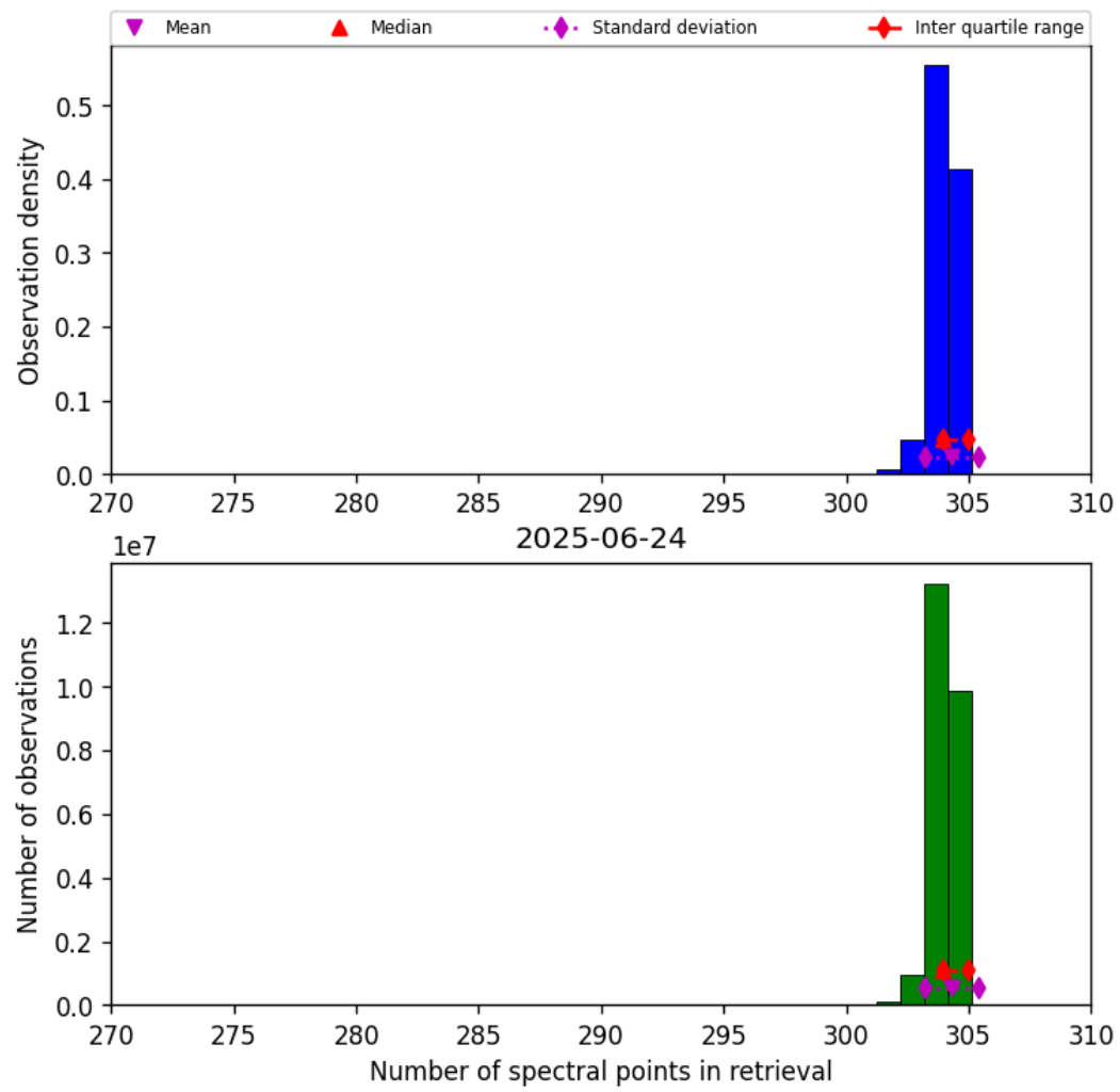
Figure 31: Histogram of “Number of spectral points in retrieval” for 2025-06-24 to 2025-06-25
