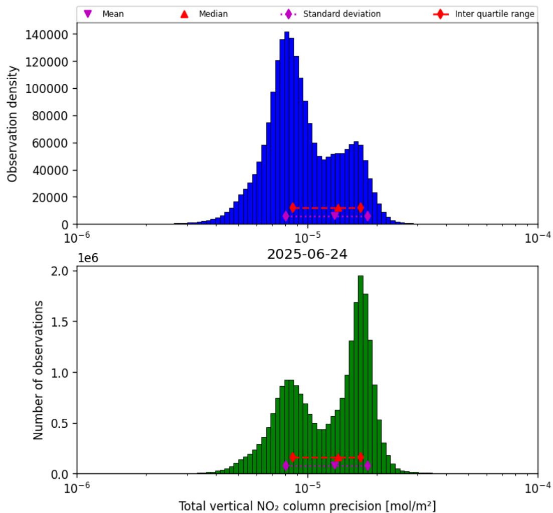
Figure 37: Histogram of “Total vertical NO 2 column precision” for 2025-06-24 to 2025-06-25
