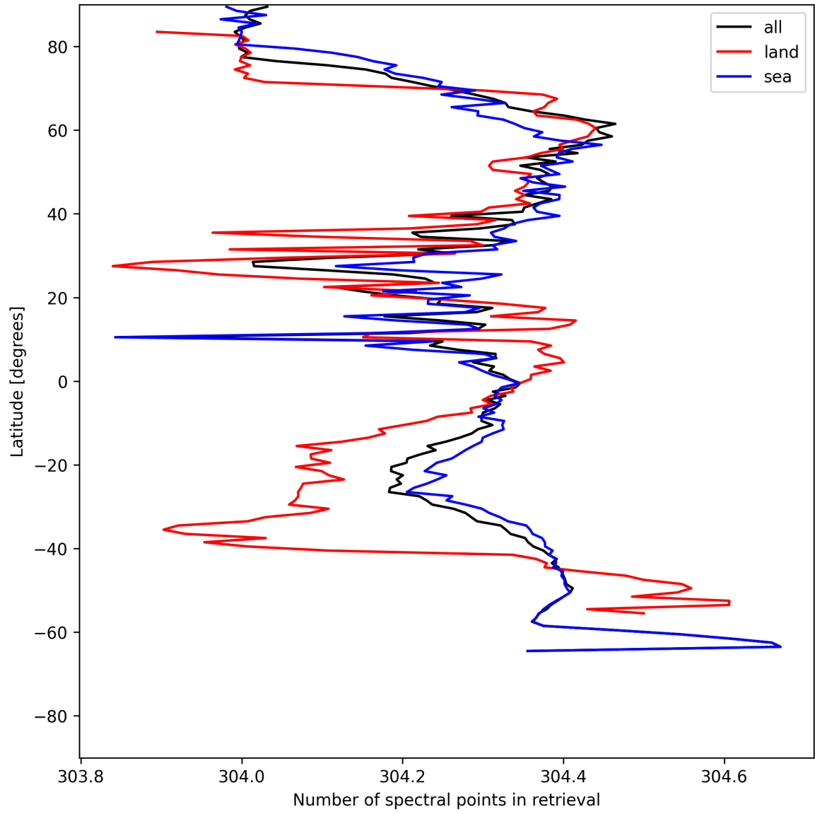
Figure 14: Zonal average of “Number of spectral points in retrieval” for 2025-06-24 to 2025-06-25.
