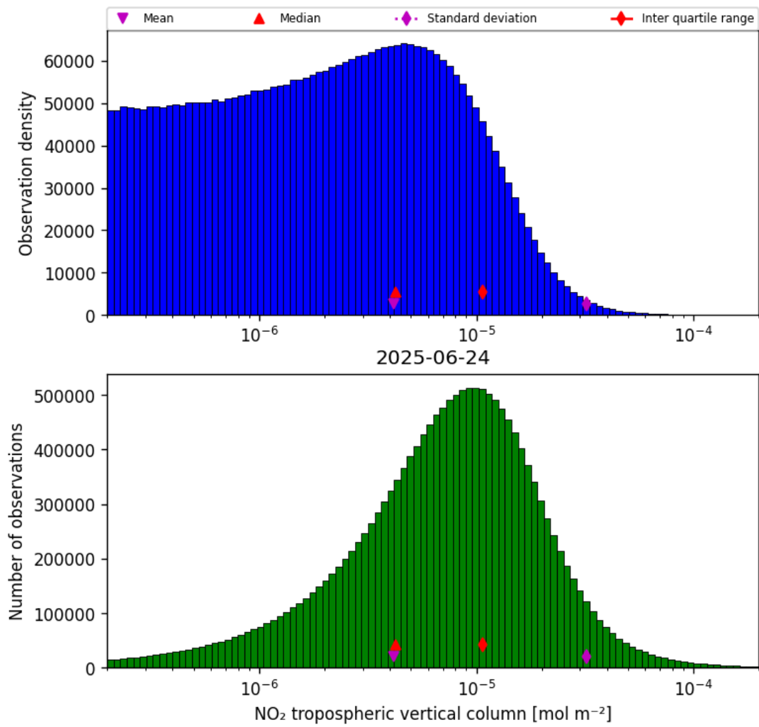
Figure 27: Histogram of “NO 2 tropospheric vertical column” for 2025-06-24 to 2025-06-25
