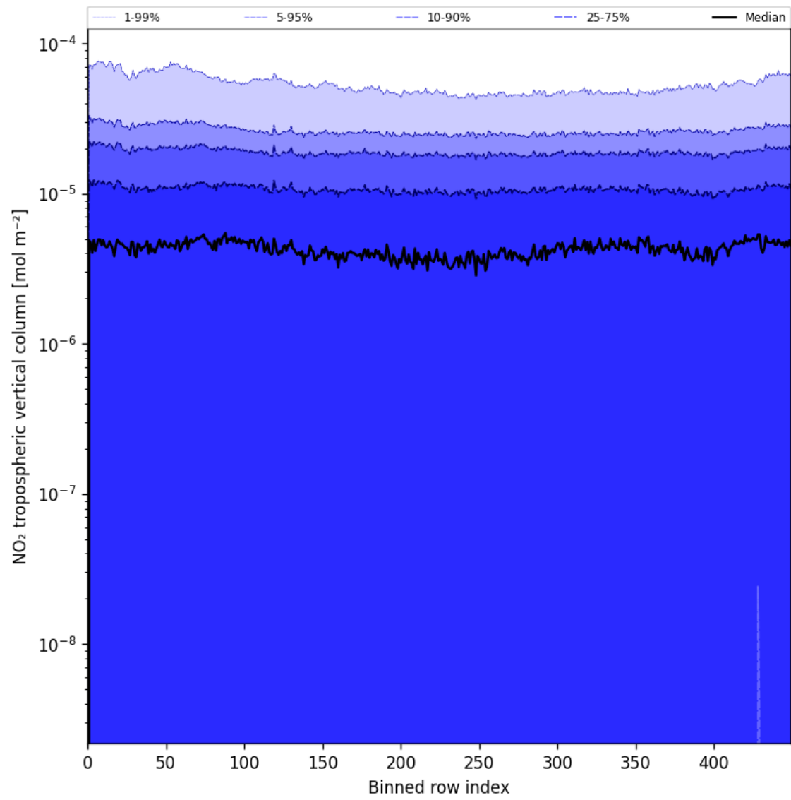
Figure 44: Along track statistics of “NO 2 tropospheric vertical column” for 2025-06-24 to 2025-06-25
