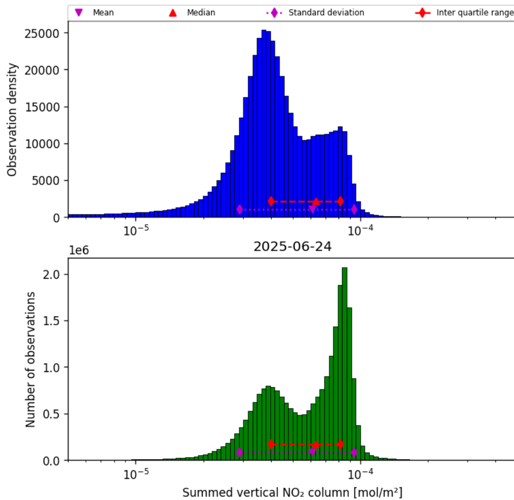
Figure 38: Histogram of “Summed vertical NO 2 column” for 2025-06-24 to 2025-06-25
