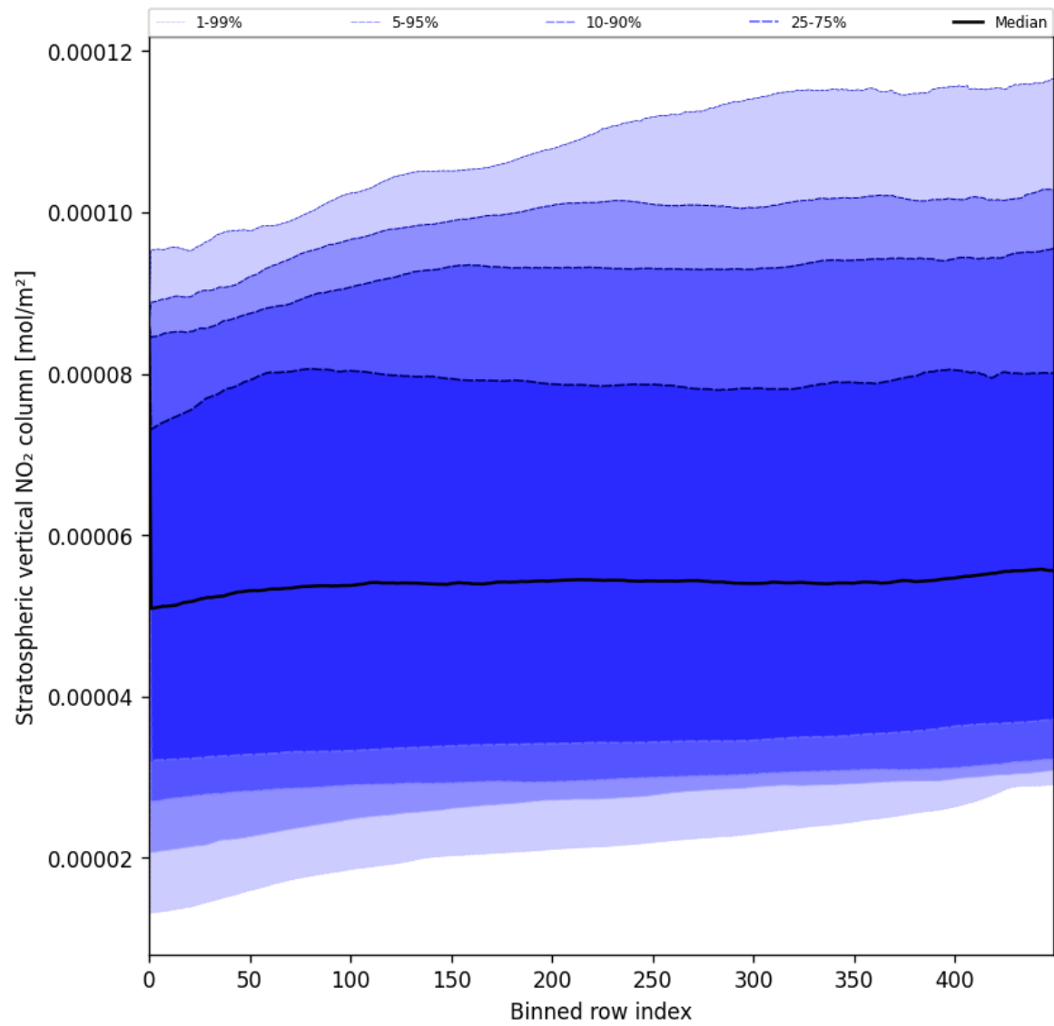
Figure 51: Along track statistics of “Stratospheric vertical NO 2 column” for 2025-06-24 to 2025-06-25
