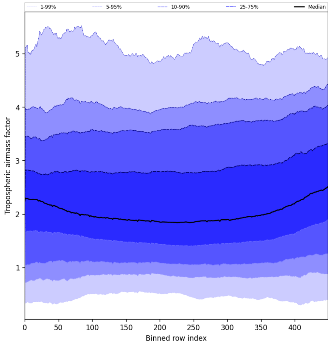
Figure 46: Along track statistics of “Tropospheric airmass factor” for 2025-06-24 to 2025-06-25
