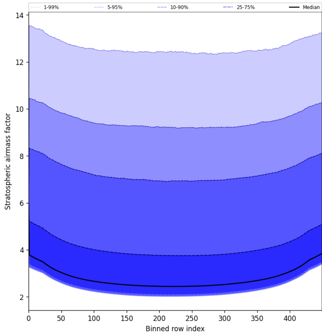
Figure 59: Along track statistics of “Stratospheric airmass factor” for 2025-06-24 to 2025-06-25
