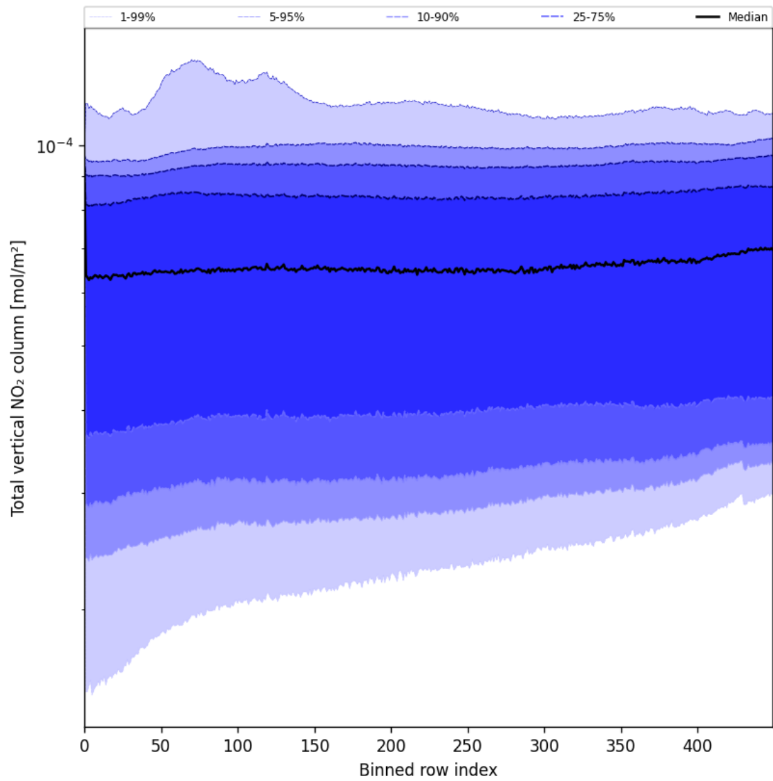
Figure 53: Along track statistics of “Total vertical NO 2 column” for 2025-06-24 to 2025-06-25
