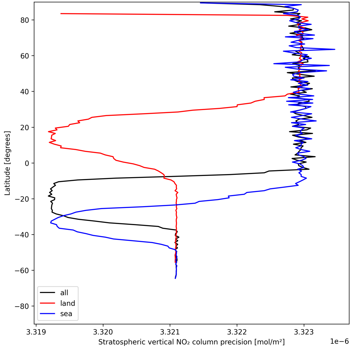
Figure 18: Zonal average of “Stratospheric vertical NO 2 column precision” for 2025-06-24 to 2025-06-25.
