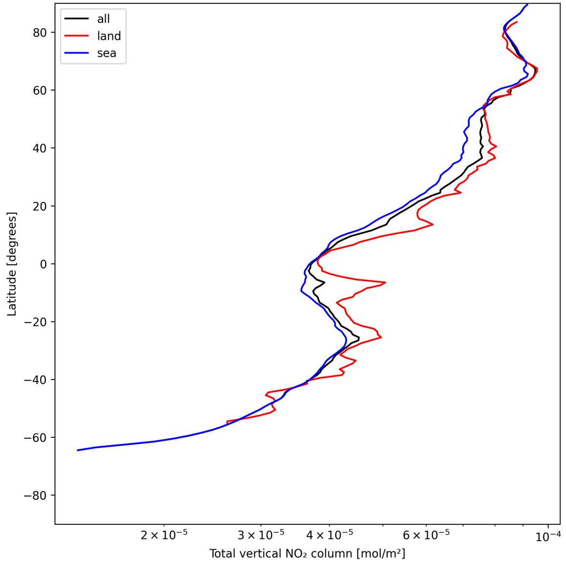
Figure 19: Zonal average of “Total vertical NO 2 column” for 2025-06-24 to 2025-06-25.
