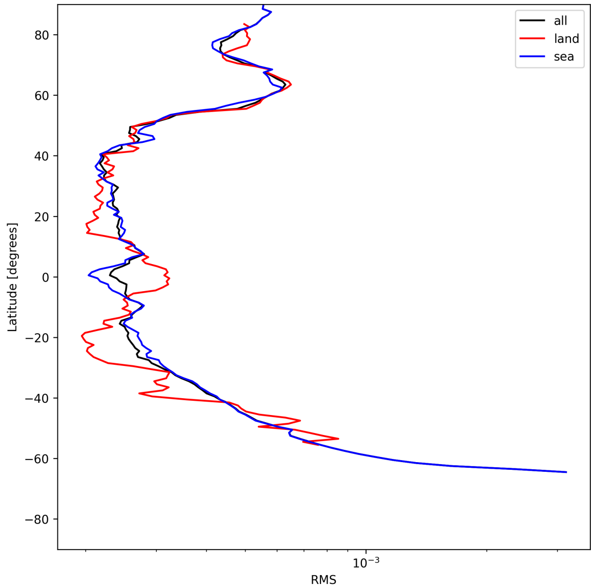
Figure 24: Zonal average of “RMS” for 2025-06-24 to 2025-06-25.
