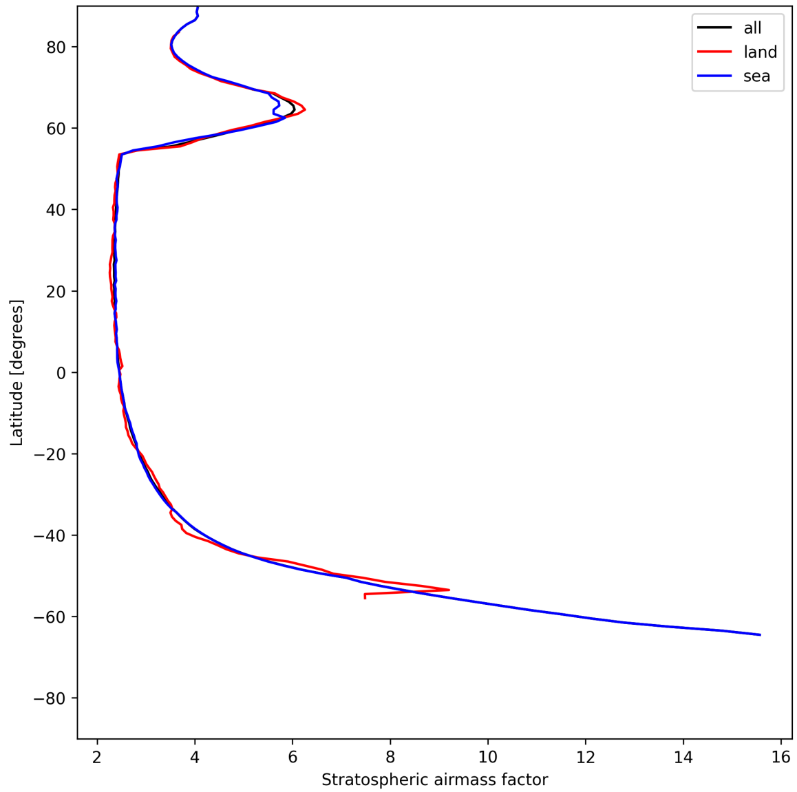
Figure 25: Zonal average of “Stratospheric air mass factor” for 2025-06-24 to 2025-06-25.
