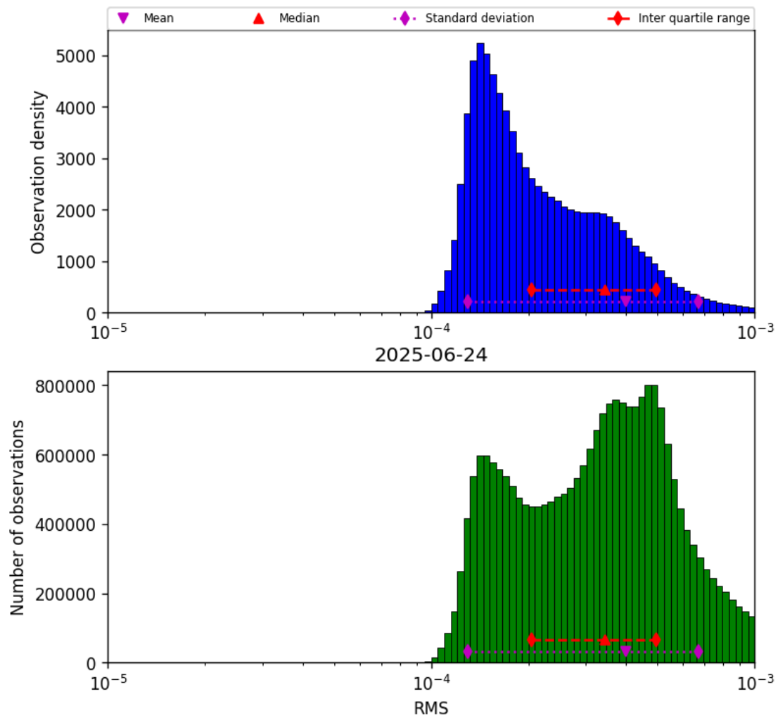
Figure 41: Histogram of “RMS” for 2025-06-24 to 2025-06-25
