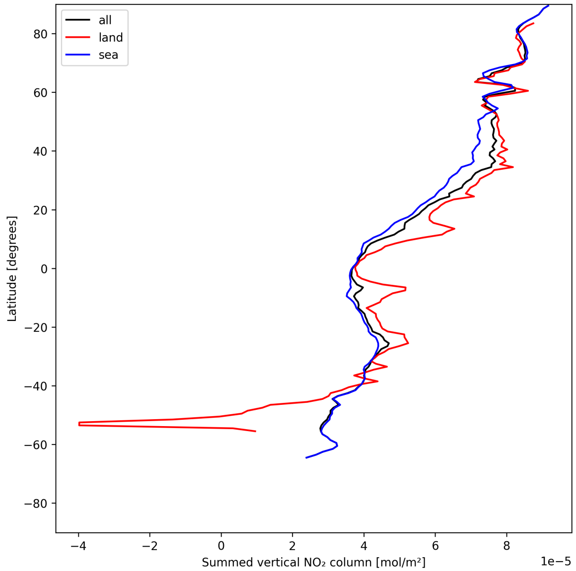
Figure 21: Zonal average of “Summed vertical NO 2 column” for 2025-06-24 to 2025-06-25.
