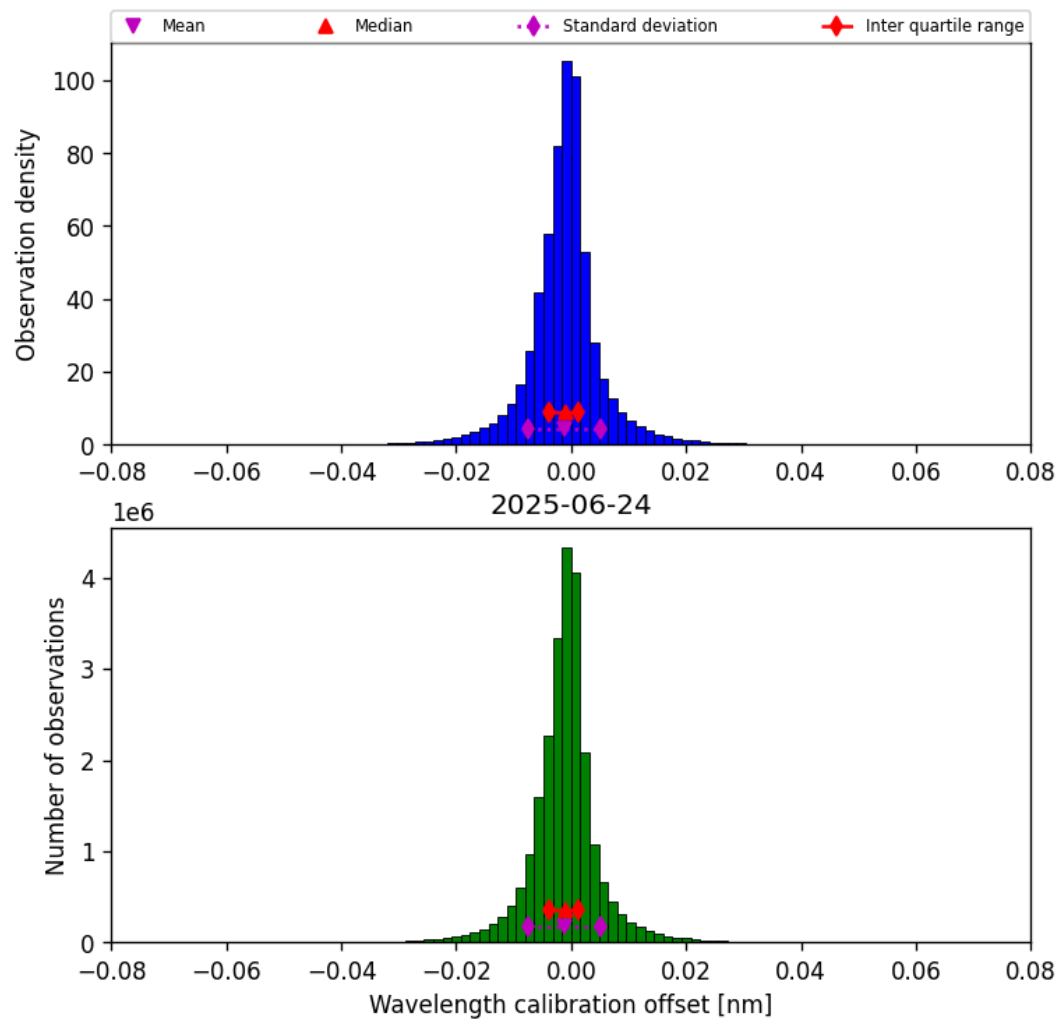
Figure 33: Histogram of “Wavelength calibration offset” for 2025-06-24 to 2025-06-25
