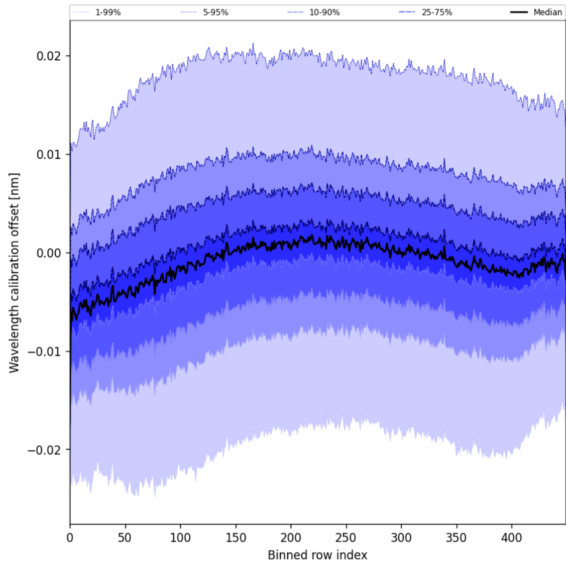
Figure 50: Along track statistics of “Wavelength calibration offset” for 2025-06-24 to 2025-06-25
