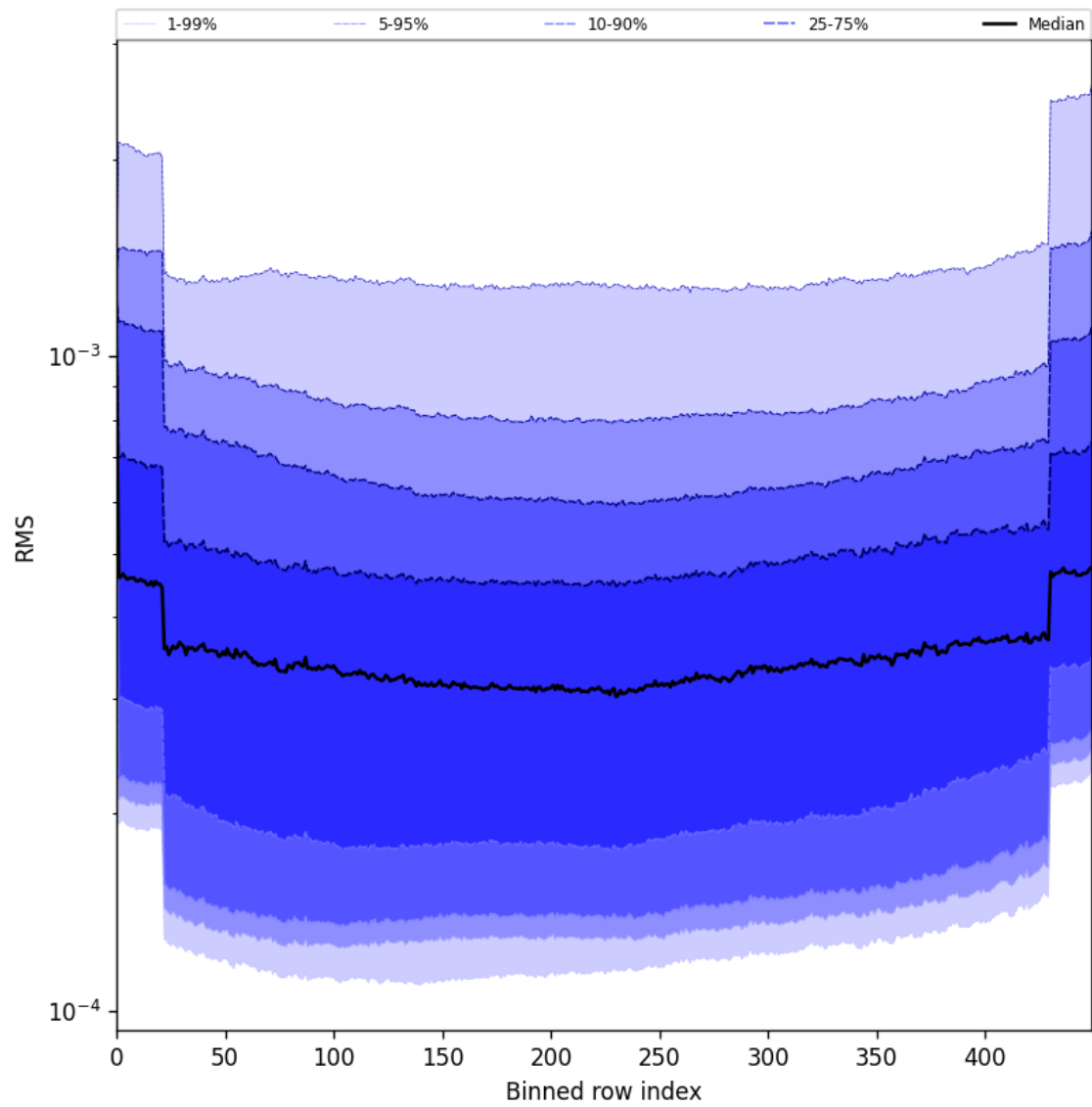
Figure 58: Along track statistics of “RMS” for 2025-06-24 to 2025-06-25
