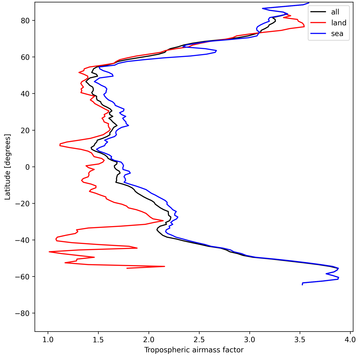
Figure 12: Zonal average of “Tropospheric airmass factor” for 2025-06-24 to 2025-06-25.
