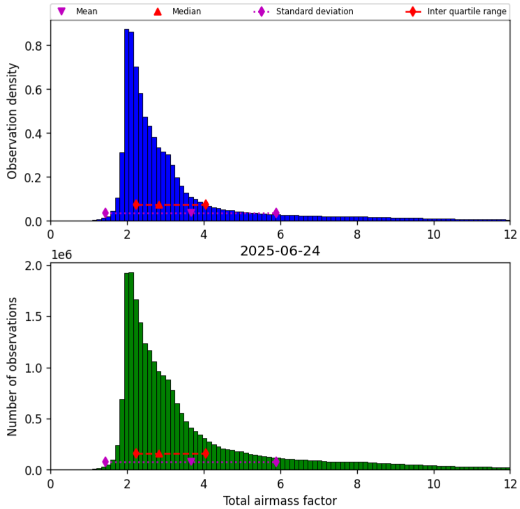
Figure 30: Histogram of “Total airmass factor” for 2025-06-24 to 2025-06-25
