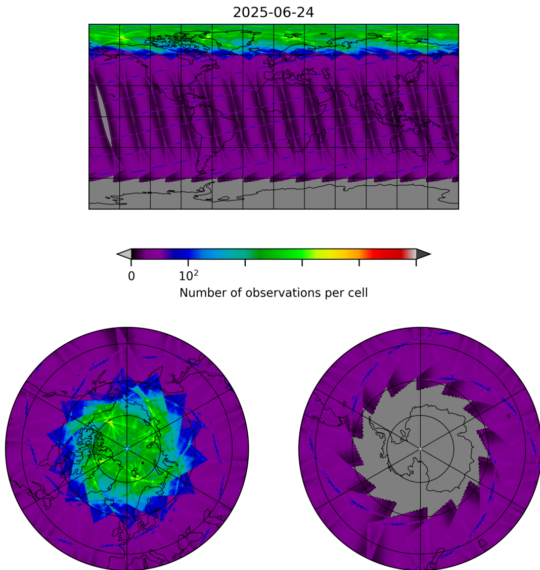
Figure 8: Map of the number of observations for 2025-06-24 to 2025-06-25
