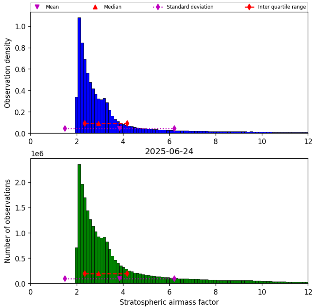
Figure 42: Histogram of “Stratospheric airmass factor” for 2025-06-24 to 2025-06-25
