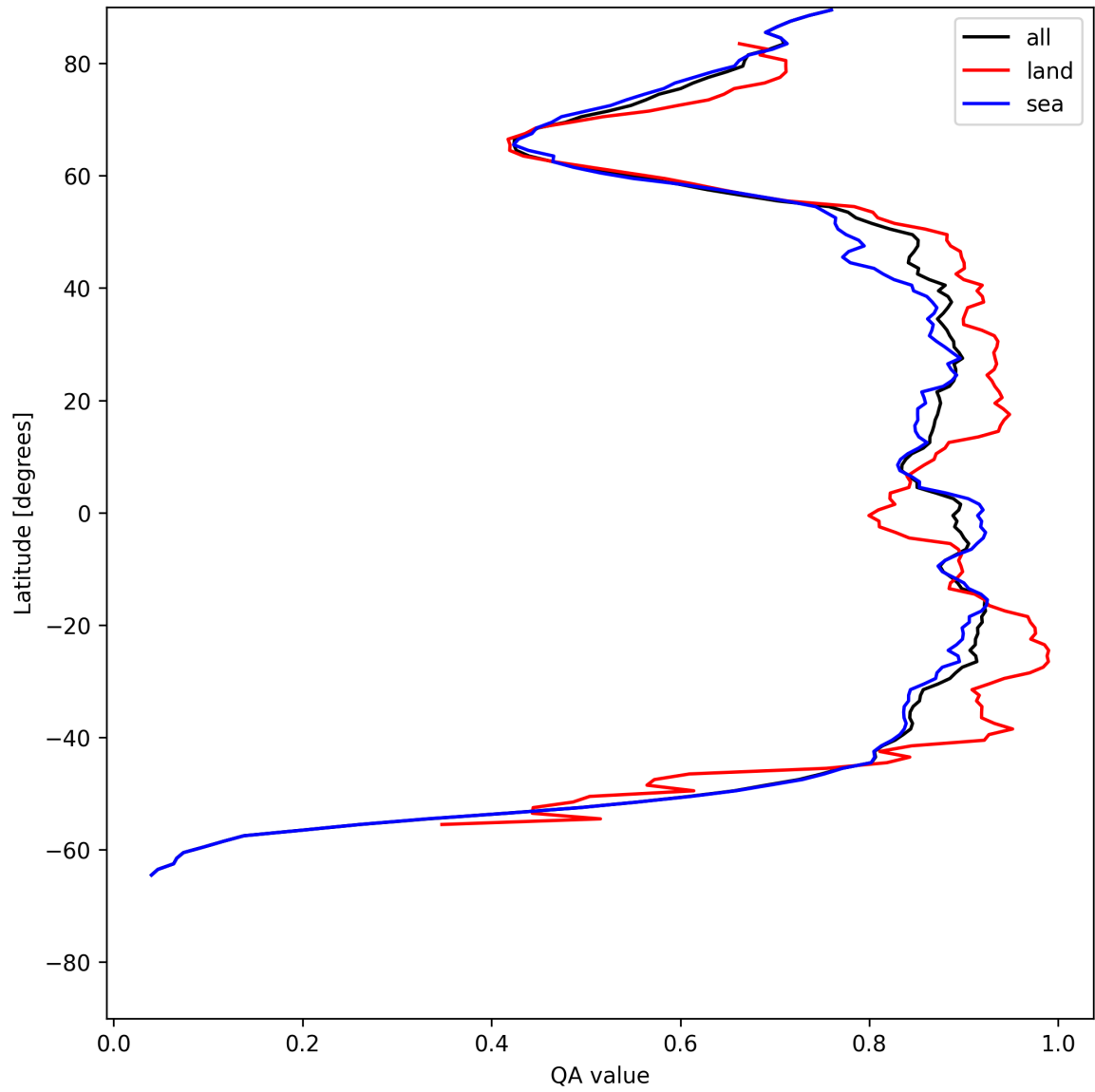
Figure 9: Zonal average of “QA value” for 2025-06-24 to 2025-06-25.
