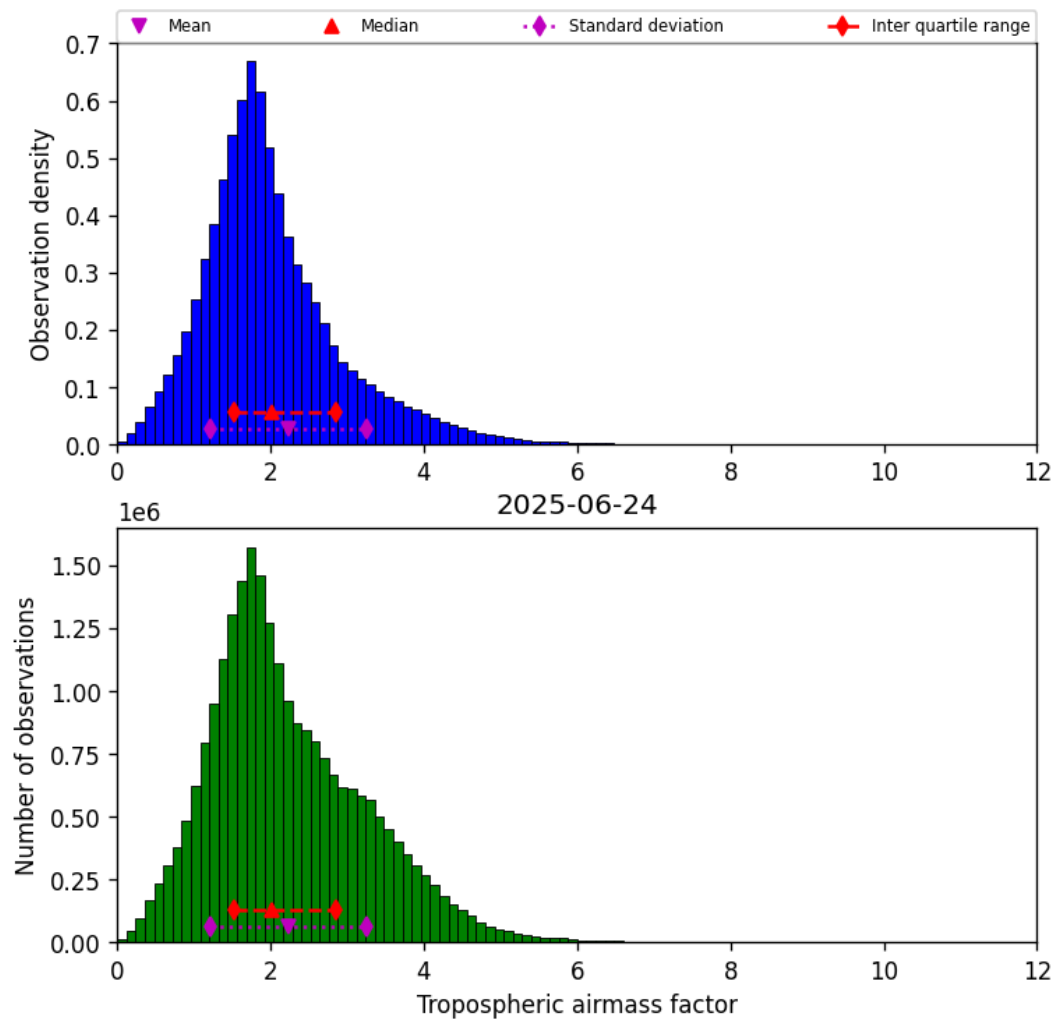
Figure 29: Histogram of “Tropospheric airmass factor” for 2025-06-24 to 2025-06-25
