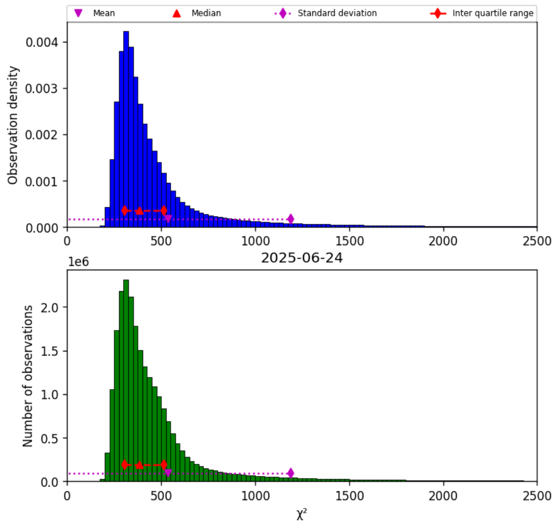
Figure 40: Histogram of “ \chi^2 ” for 2025-06-24 to 2025-06-25
