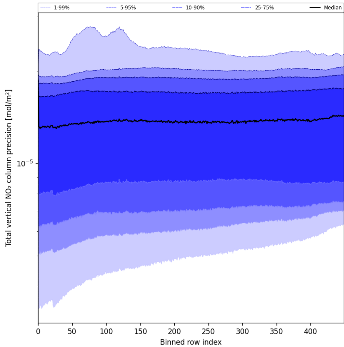
Figure 54: Along track statistics of “Total vertical NO 2 column precision” for 2025-06-24 to 2025-06-25
