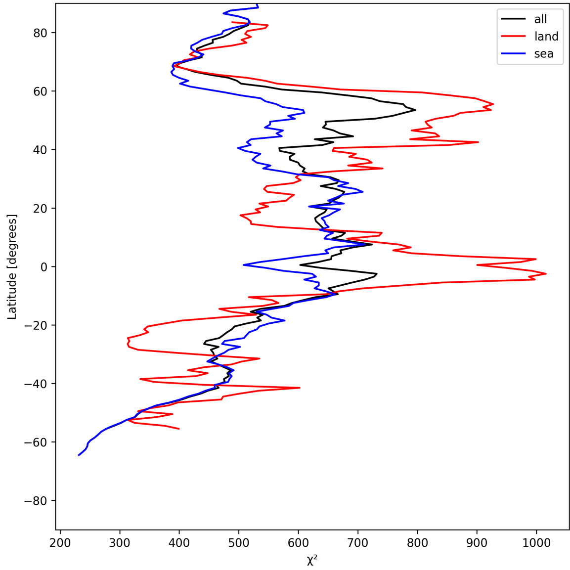
Figure 23: Zonal average of “ \chi^2 ” for 2025-06-24 to 2025-06-25.
