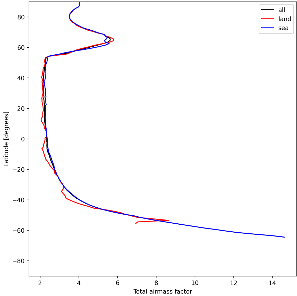
Figure 13: Zonal average of “Total airmass factor” for 2025-06-24 to 2025-06-25.
