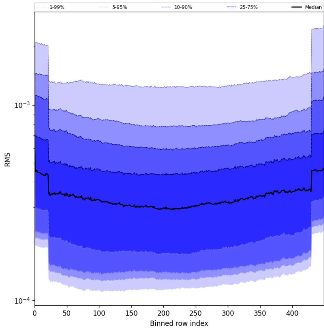
Figure 58: Along track statistics of “RMS” for 2025-06-26 to 2025-06-27
