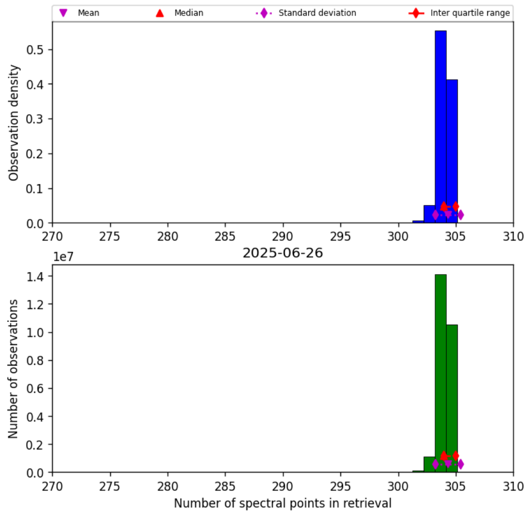
Figure 31: Histogram of “Number of spectral points in retrieval” for 2025-06-26 to 2025-06-27
