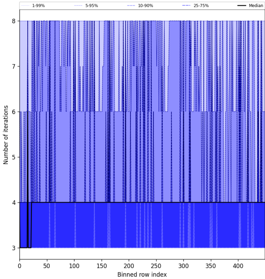
Figure 49: Along track statistics of “Number of iterations” for 2025-06-26 to 2025-06-27
