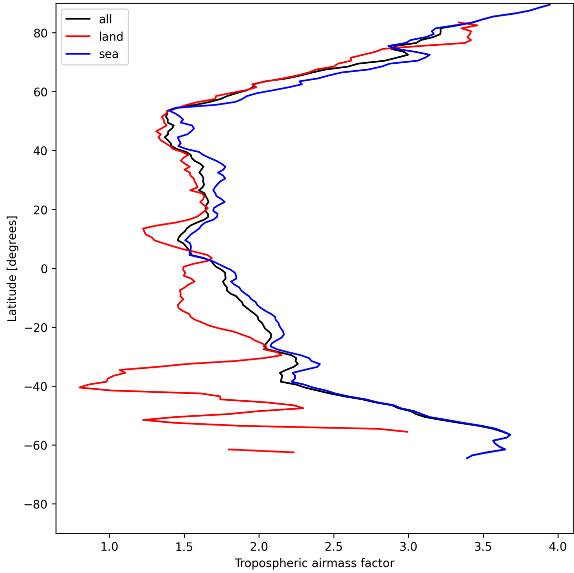
Figure 12: Zonal average of “Tropospheric airmass factor” for 2025-06-26 to 2025-06-27.
