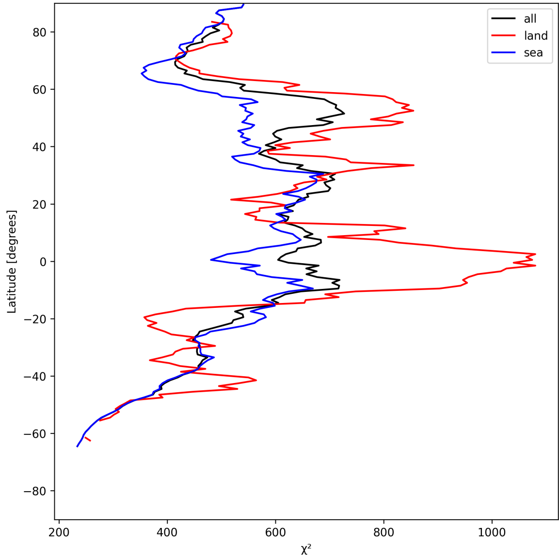
Figure 23: Zonal average of “ \chi^2 ” for 2025-06-26 to 2025-06-27.
