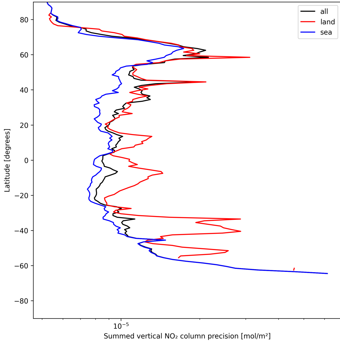
Figure 22: Zonal average of “Summed vertical NO 2 column precision” for 2025-06-26 to 2025-06-27.
