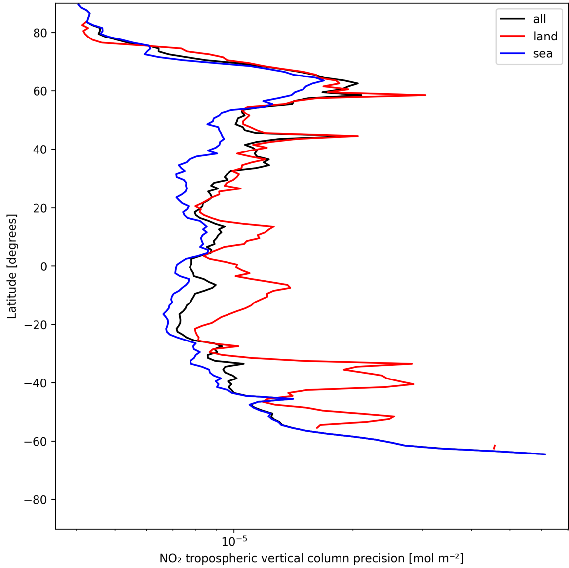
Figure 11: Zonal average of “NO 2 tropospheric vertical column precision” for 2025-06-26 to 2025-06-27.
