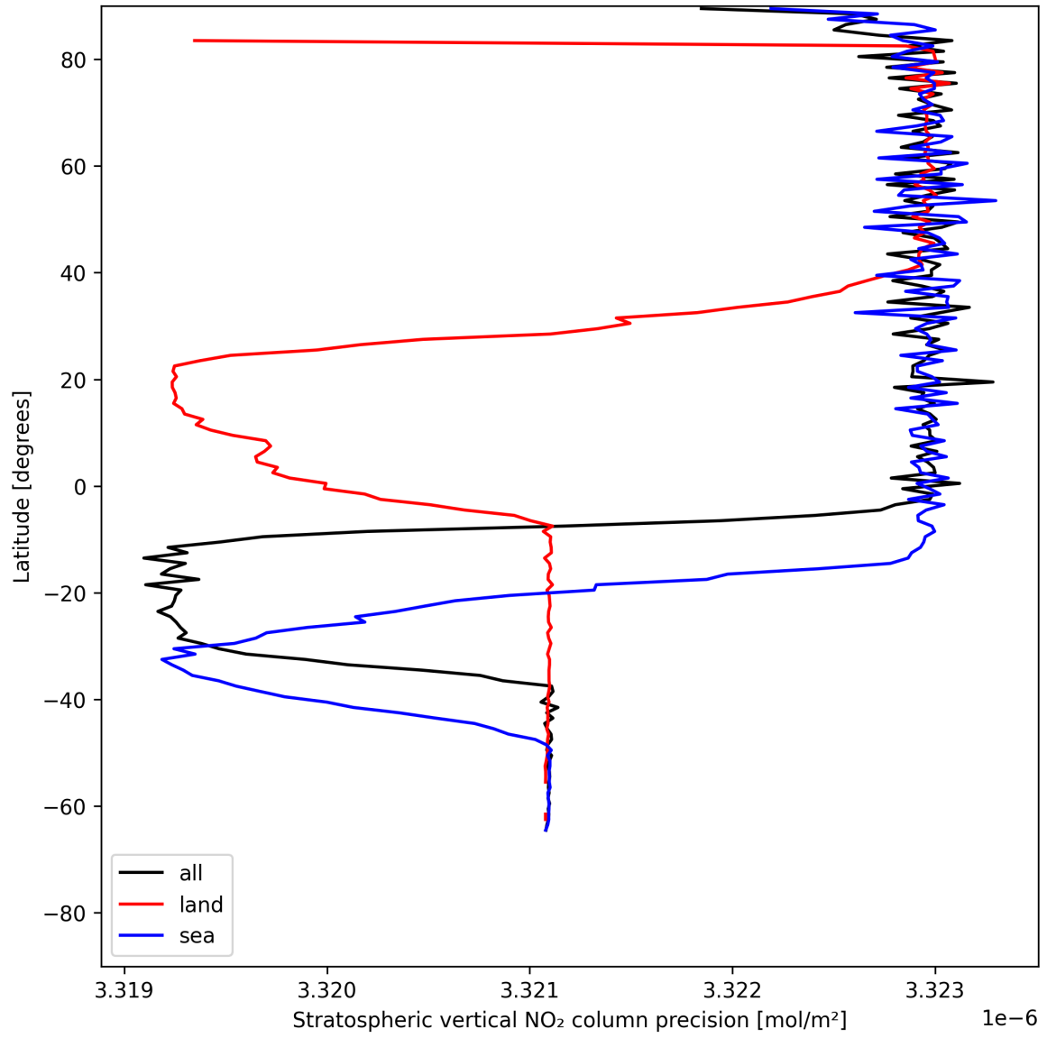
Figure 18: Zonal average of “Stratospheric vertical NO 2 column precision” for 2025-06-26 to 2025-06-27.
