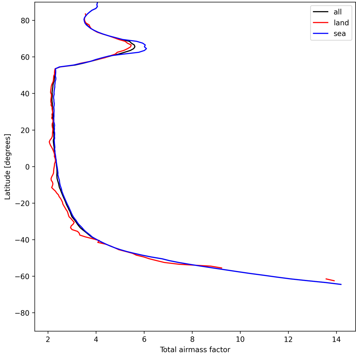
Figure 13: Zonal average of “Total airmass factor” for 2025-06-26 to 2025-06-27.
