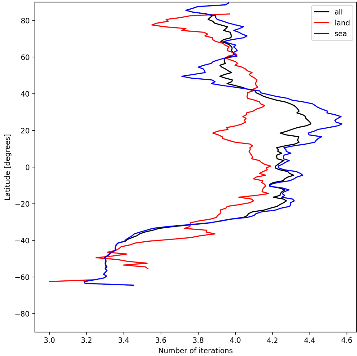
Figure 15: Zonal average of “Number of iterations” for 2025-06-26 to 2025-06-27.
