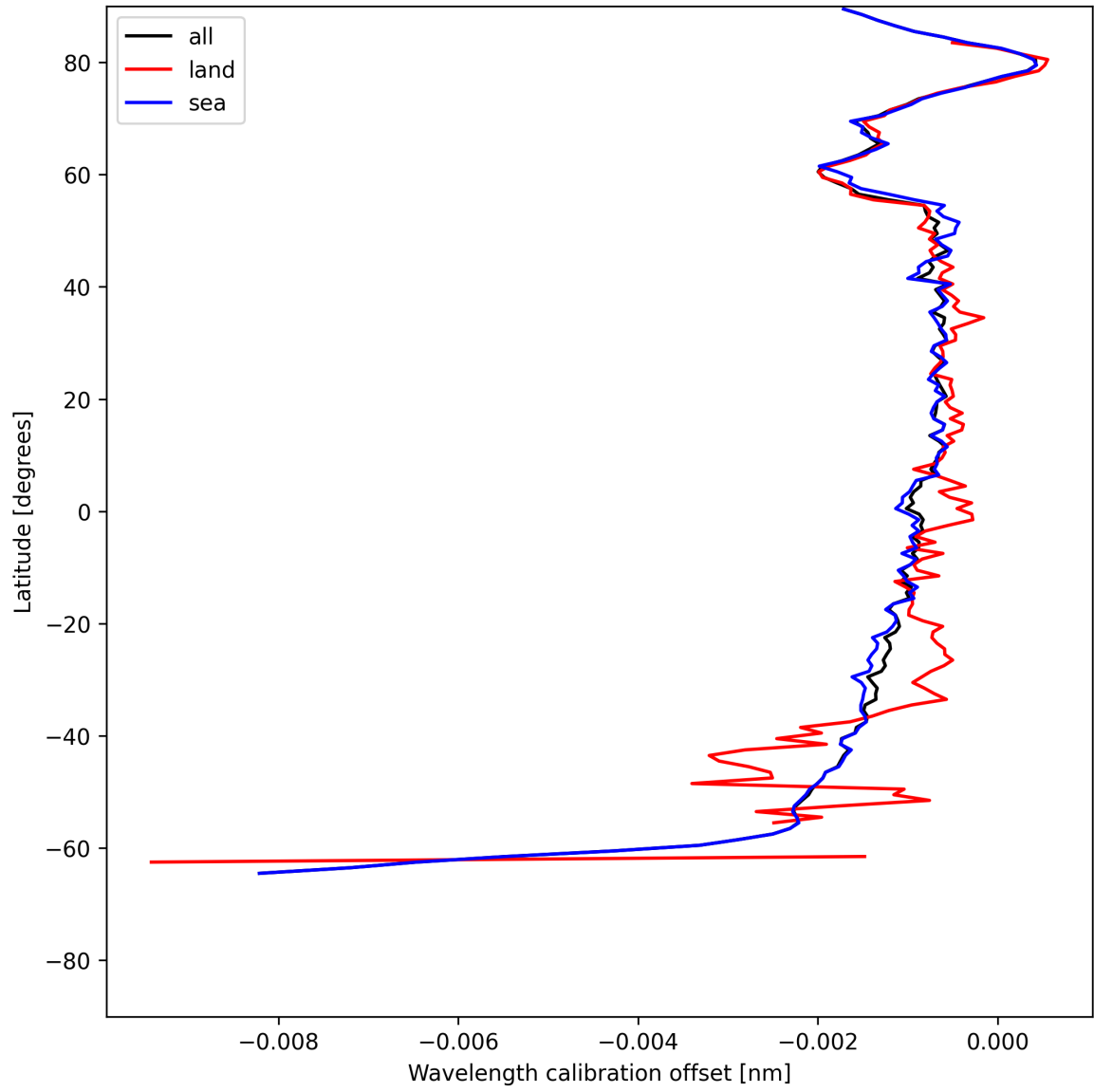
Figure 16: Zonal average of “Wavelength calibration offset” for 2025-06-26 to 2025-06-27.
