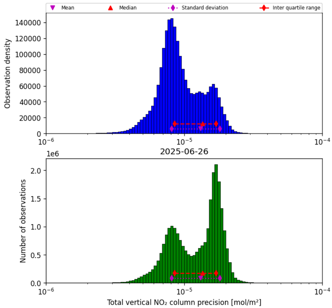
Figure 37: Histogram of “Total vertical NO 2 column precision” for 2025-06-26 to 2025-06-27
