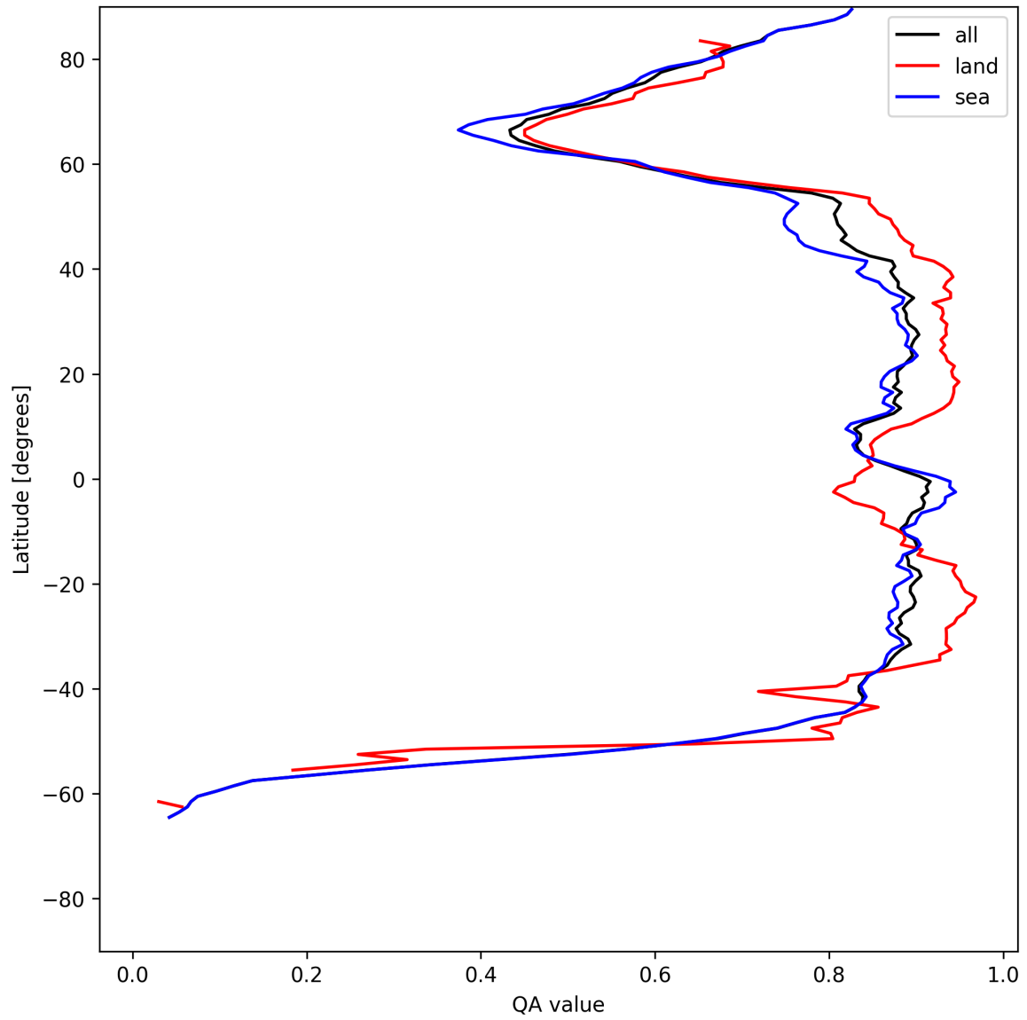
Figure 9: Zonal average of “QA value” for 2025-06-26 to 2025-06-27.
