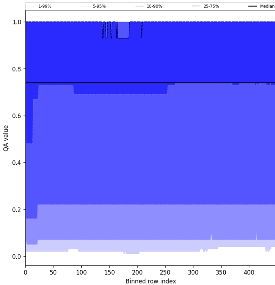
Figure 43: Along track statistics of “QA value” for 2025-06-26 to 2025-06-27
