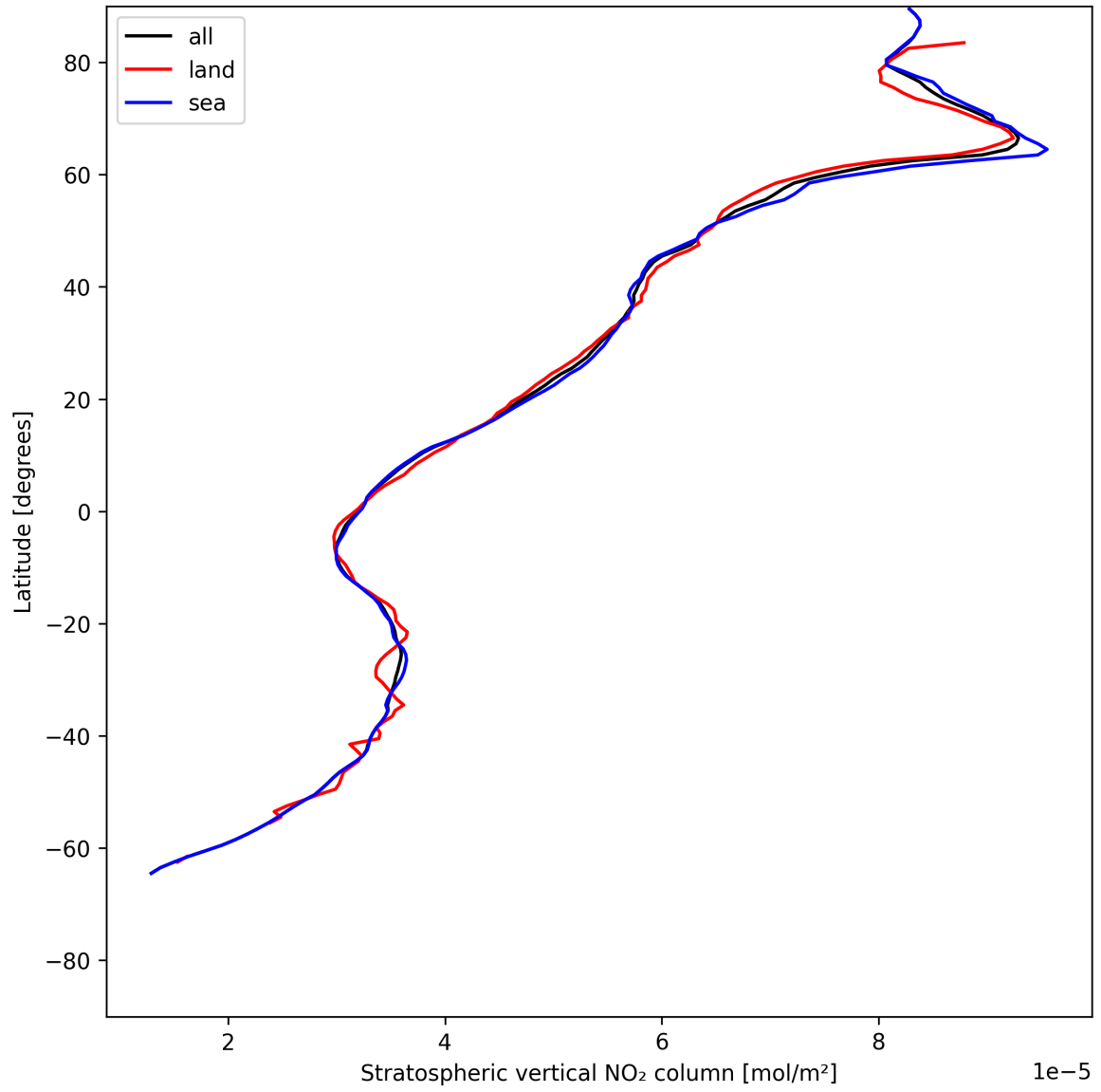
Figure 17: Zonal average of “Stratospheric vertical NO 2 column” for 2025-06-26 to 2025-06-27.
