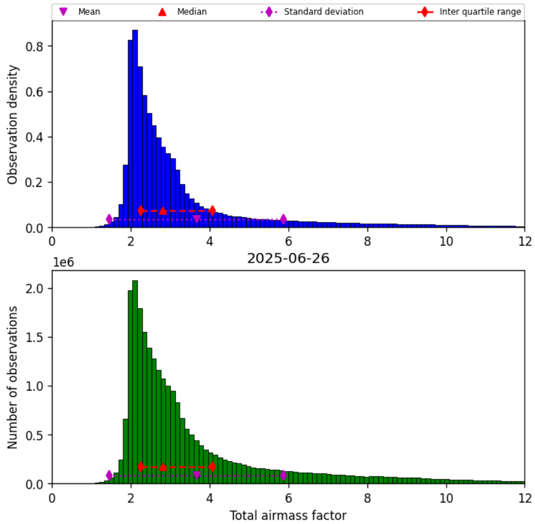
Figure 30: Histogram of “Total airmass factor” for 2025-06-26 to 2025-06-27
