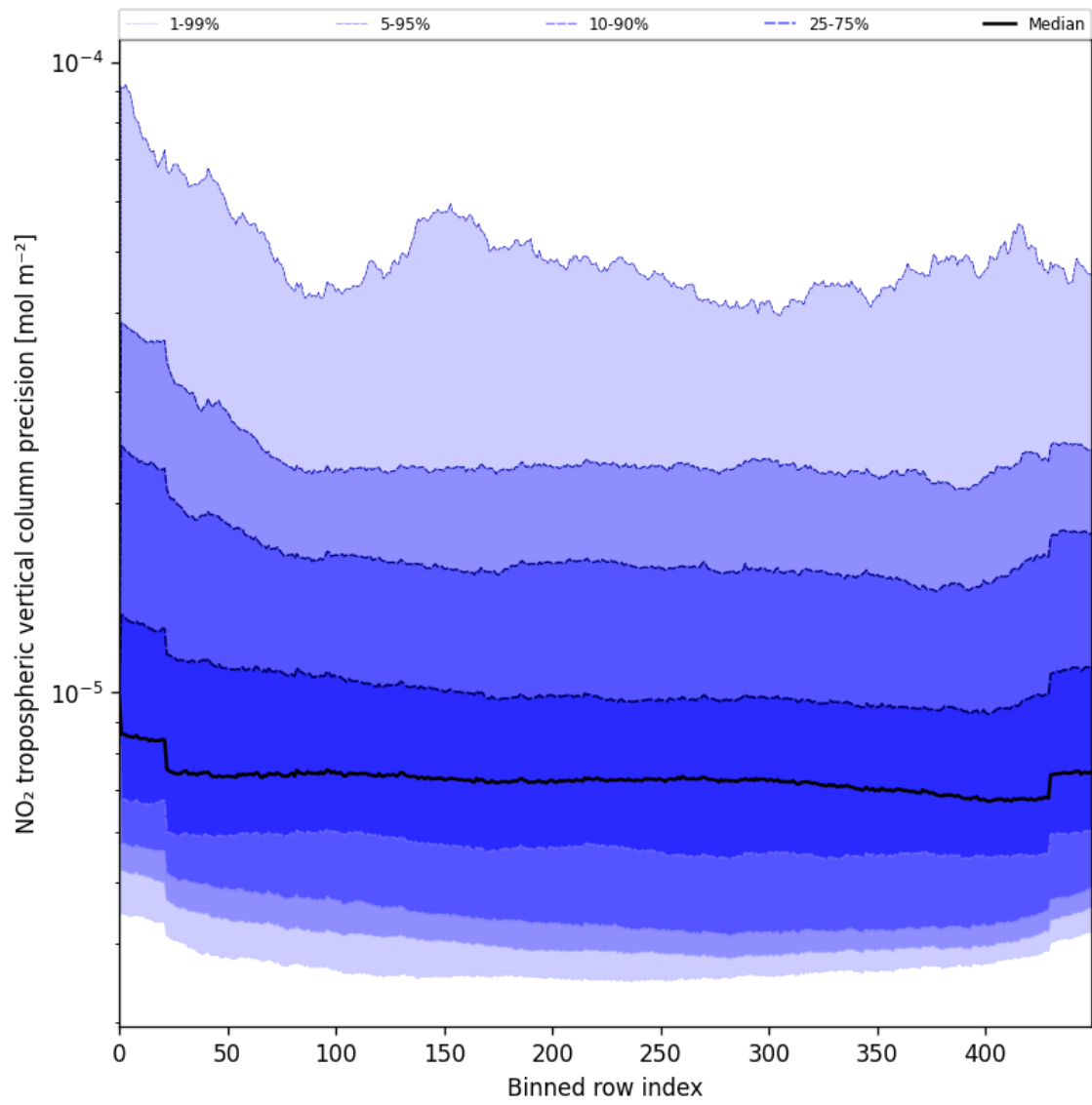
Figure 45: Along track statistics of “NO 2 tropospheric vertical column precision” for 2025-06-26 to 2025-06-27
