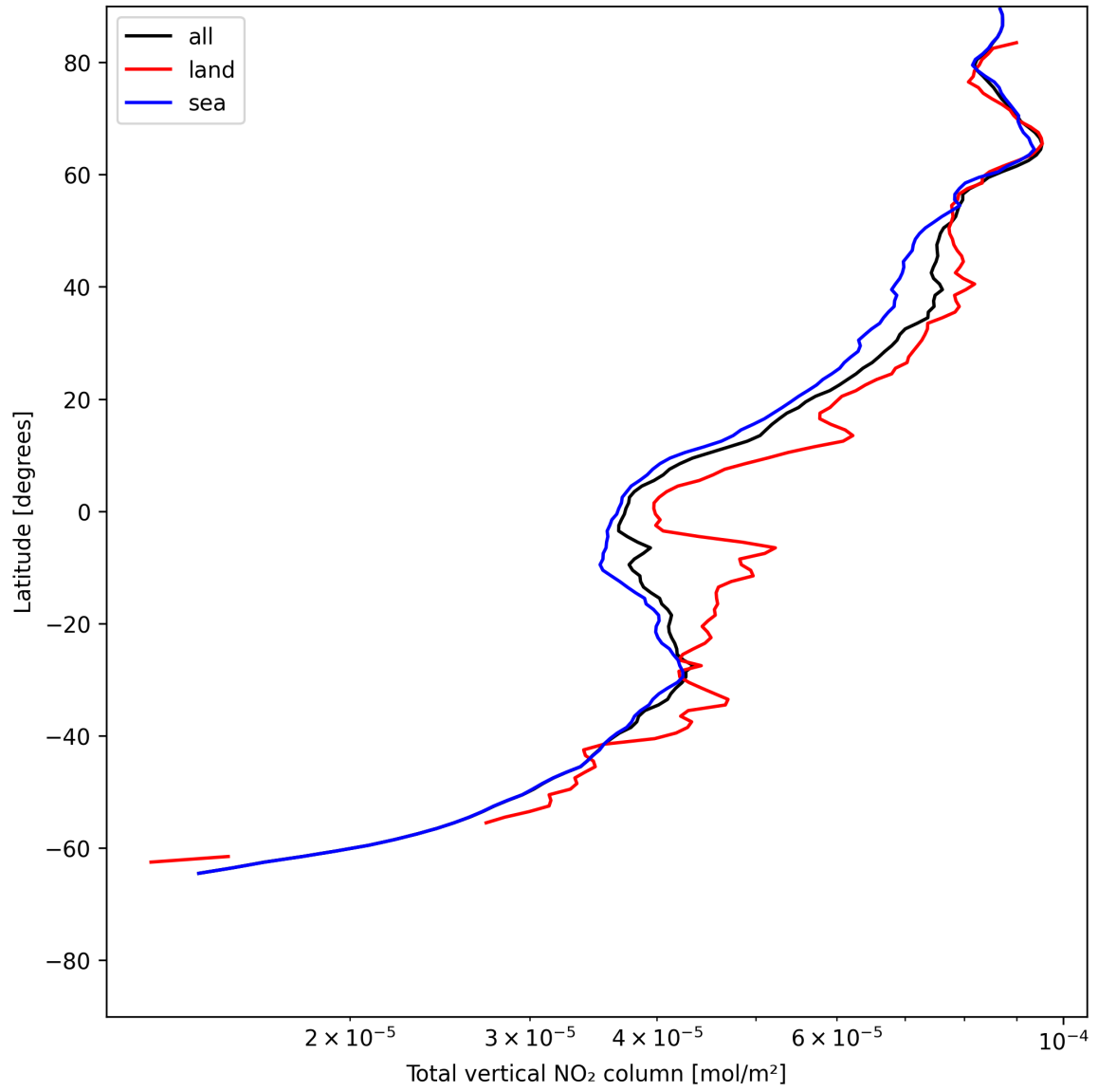
Figure 19: Zonal average of “Total vertical NO 2 column” for 2025-06-26 to 2025-06-27.
