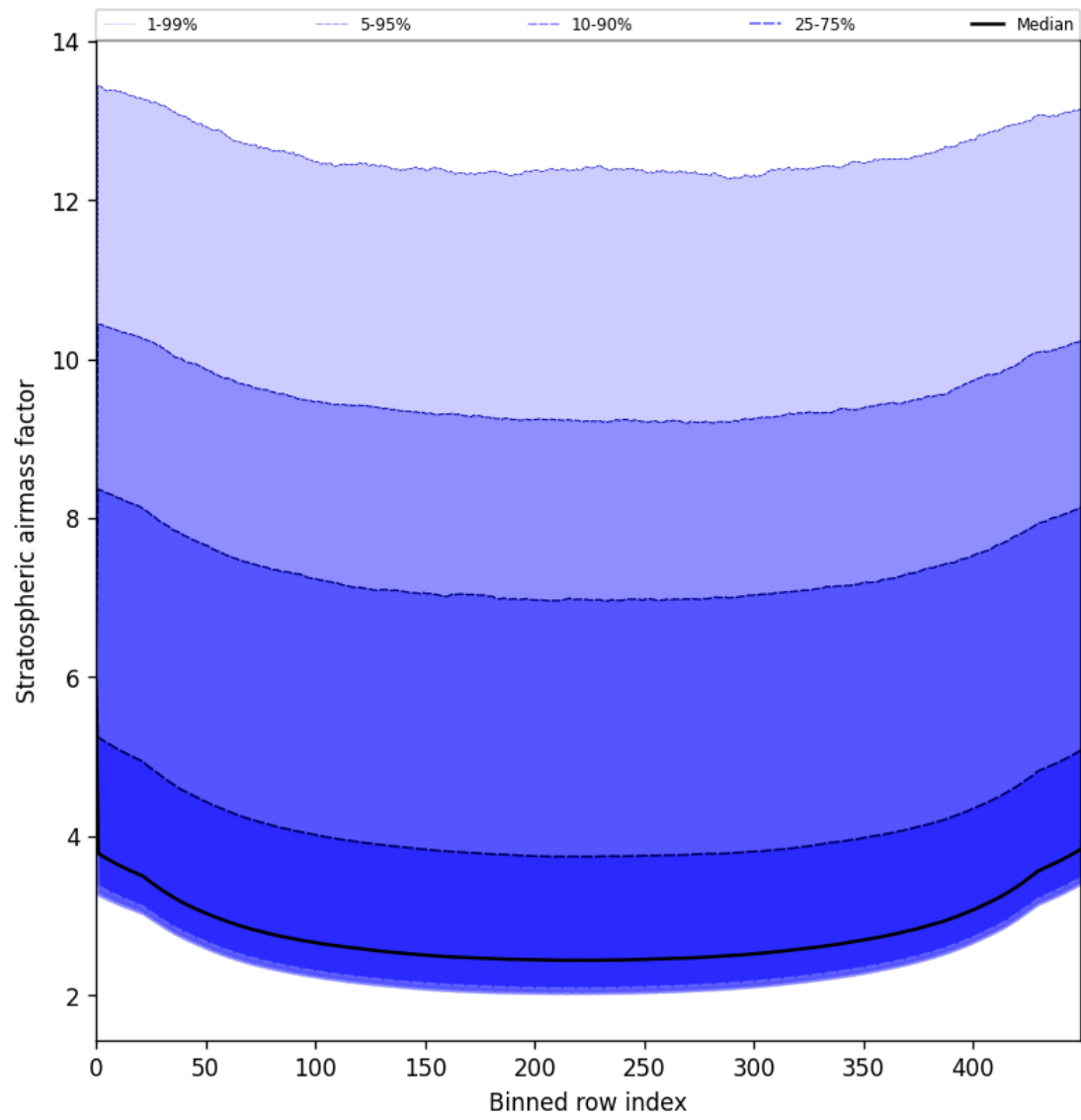
Figure 59: Along track statistics of “Stratospheric airmass factor” for 2025-06-26 to 2025-06-27
