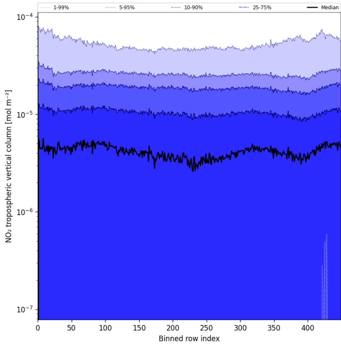
Figure 44: Along track statistics of “NO 2 tropospheric vertical column” for 2025-06-26 to 2025-06-27
