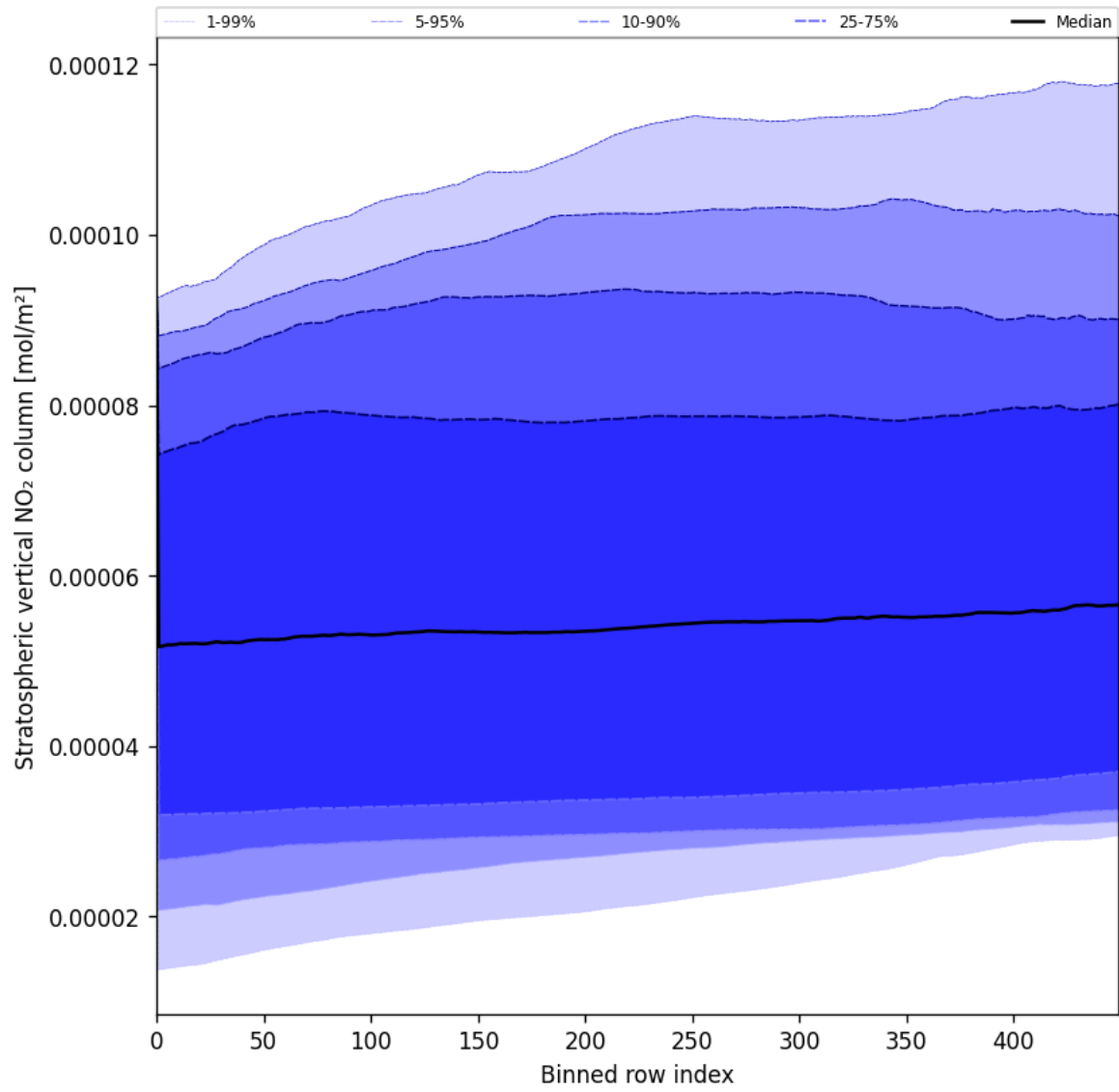
Figure 51: Along track statistics of “Stratospheric vertical NO 2 column” for 2025-06-26 to 2025-06-27
