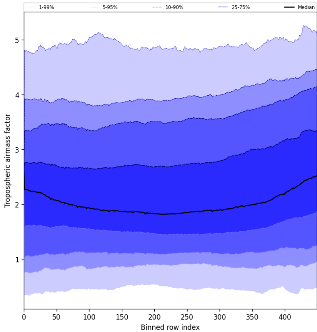
Figure 46: Along track statistics of “Tropospheric airmass factor” for 2025-06-26 to 2025-06-27
