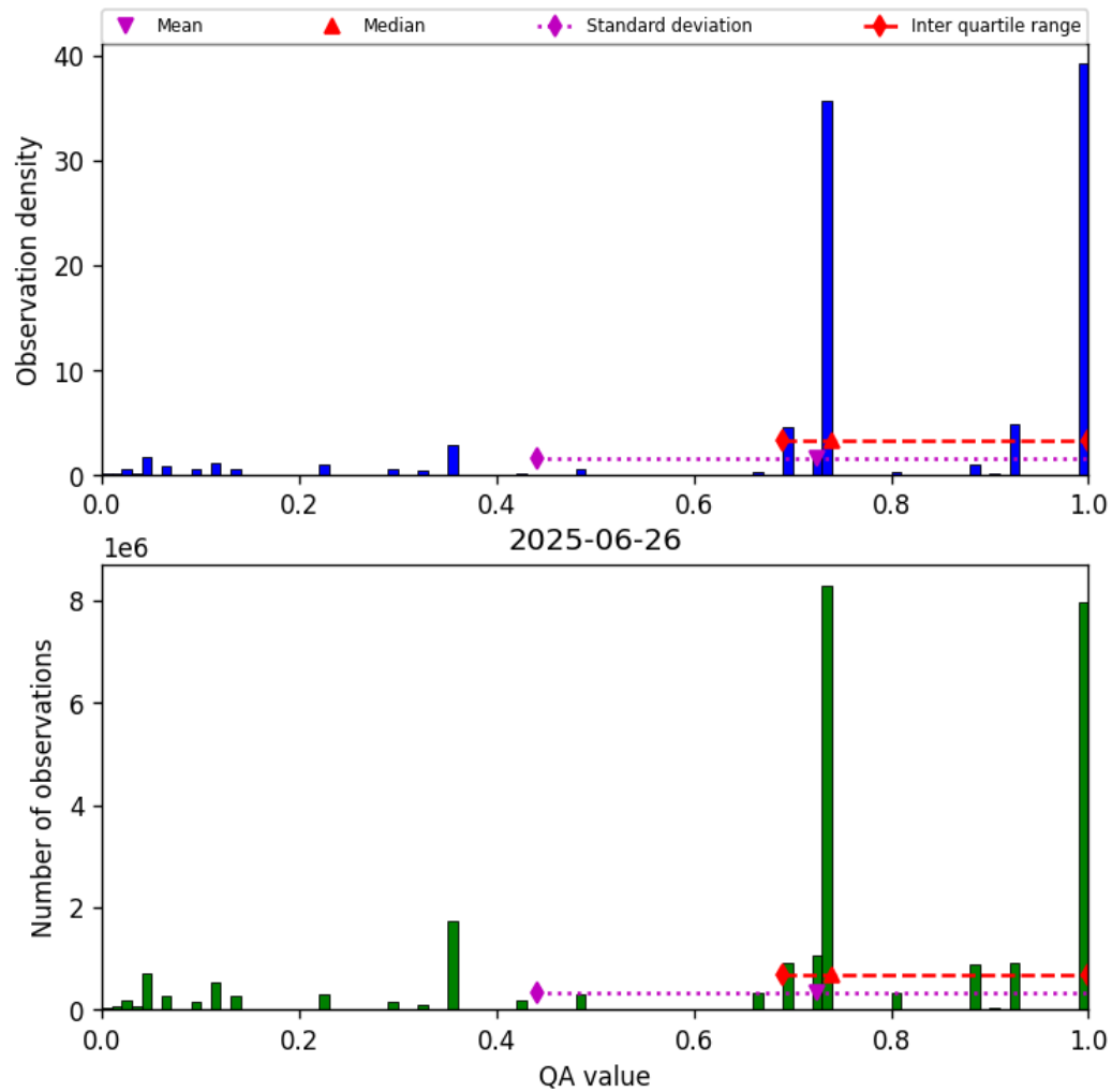
Figure 26: Histogram of “QA value” for 2025-06-26 to 2025-06-27
