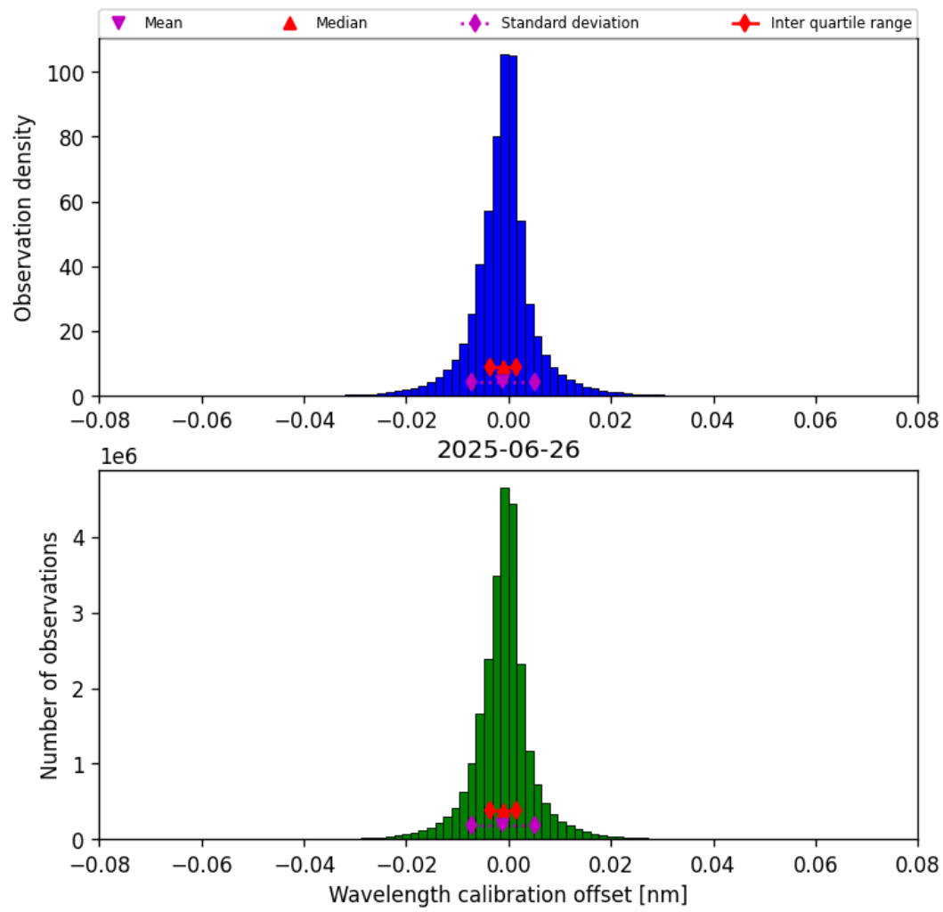
Figure 33: Histogram of “Wavelength calibration offset” for 2025-06-26 to 2025-06-27
