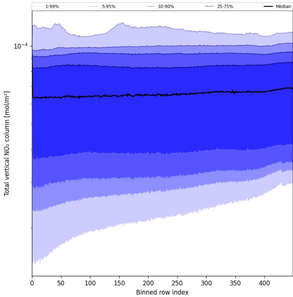
Figure 53: Along track statistics of “Total vertical NO 2 column” for 2025-06-26 to 2025-06-27
