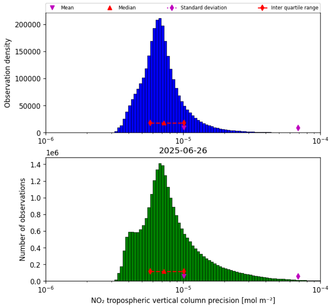
Figure 28: Histogram of “NO 2 tropospheric vertical column precision” for 2025-06-26 to 2025-06-27
