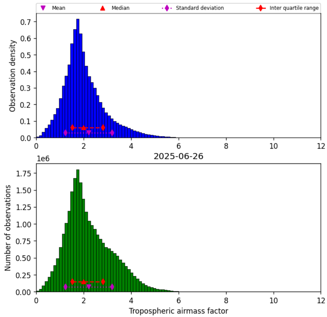
Figure 29: Histogram of “Tropospheric airmass factor” for 2025-06-26 to 2025-06-27
