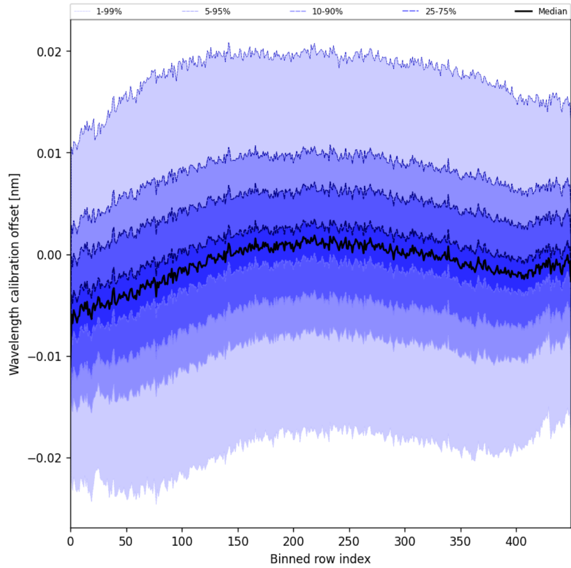
Figure 50: Along track statistics of “Wavelength calibration offset” for 2025-06-26 to 2025-06-27
