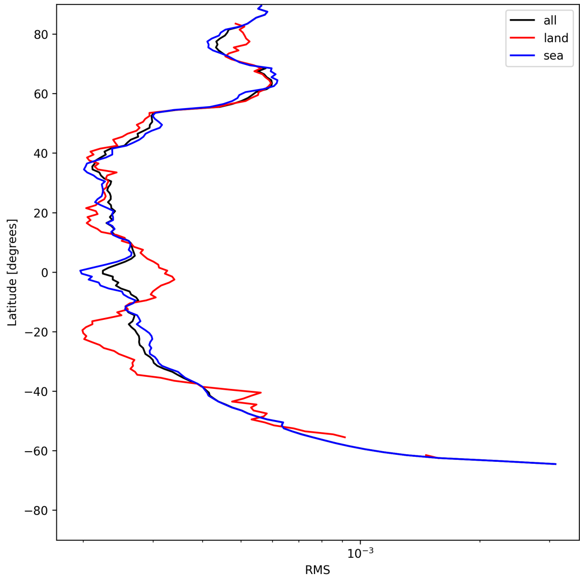
Figure 24: Zonal average of “RMS” for 2025-06-26 to 2025-06-27.
