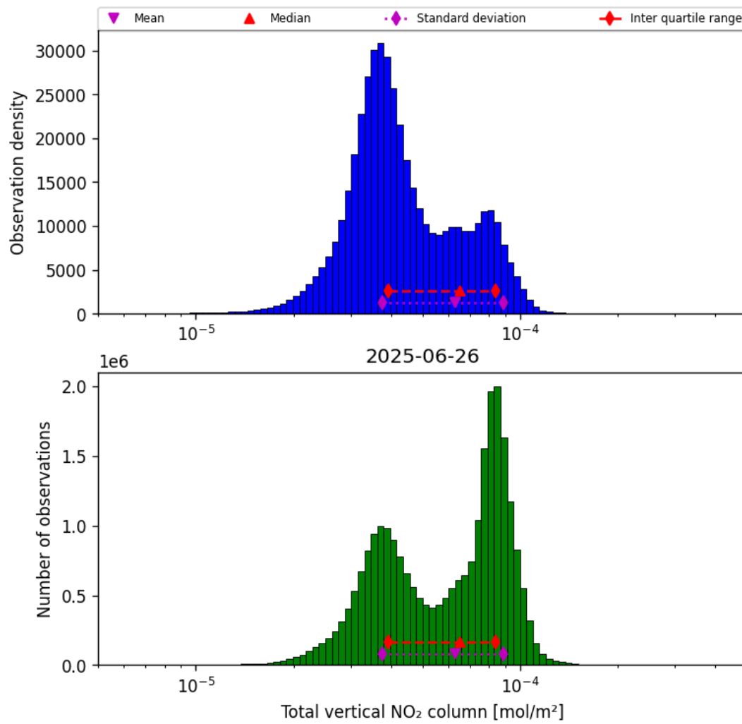
Figure 36: Histogram of “Total vertical NO 2 column” for 2025-06-26 to 2025-06-27
