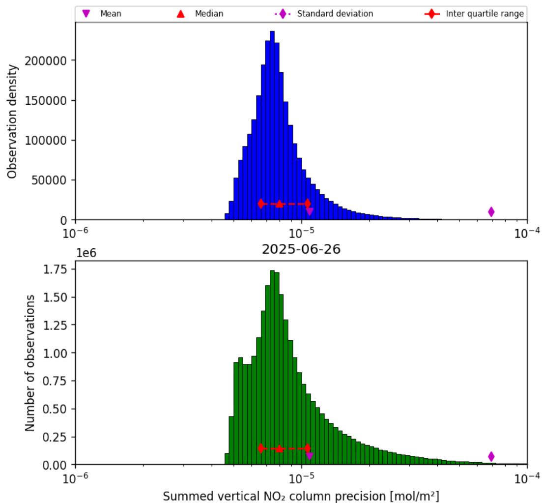
Figure 39: Histogram of “Summed vertical NO 2 column precision” for 2025-06-26 to 2025-06-27
