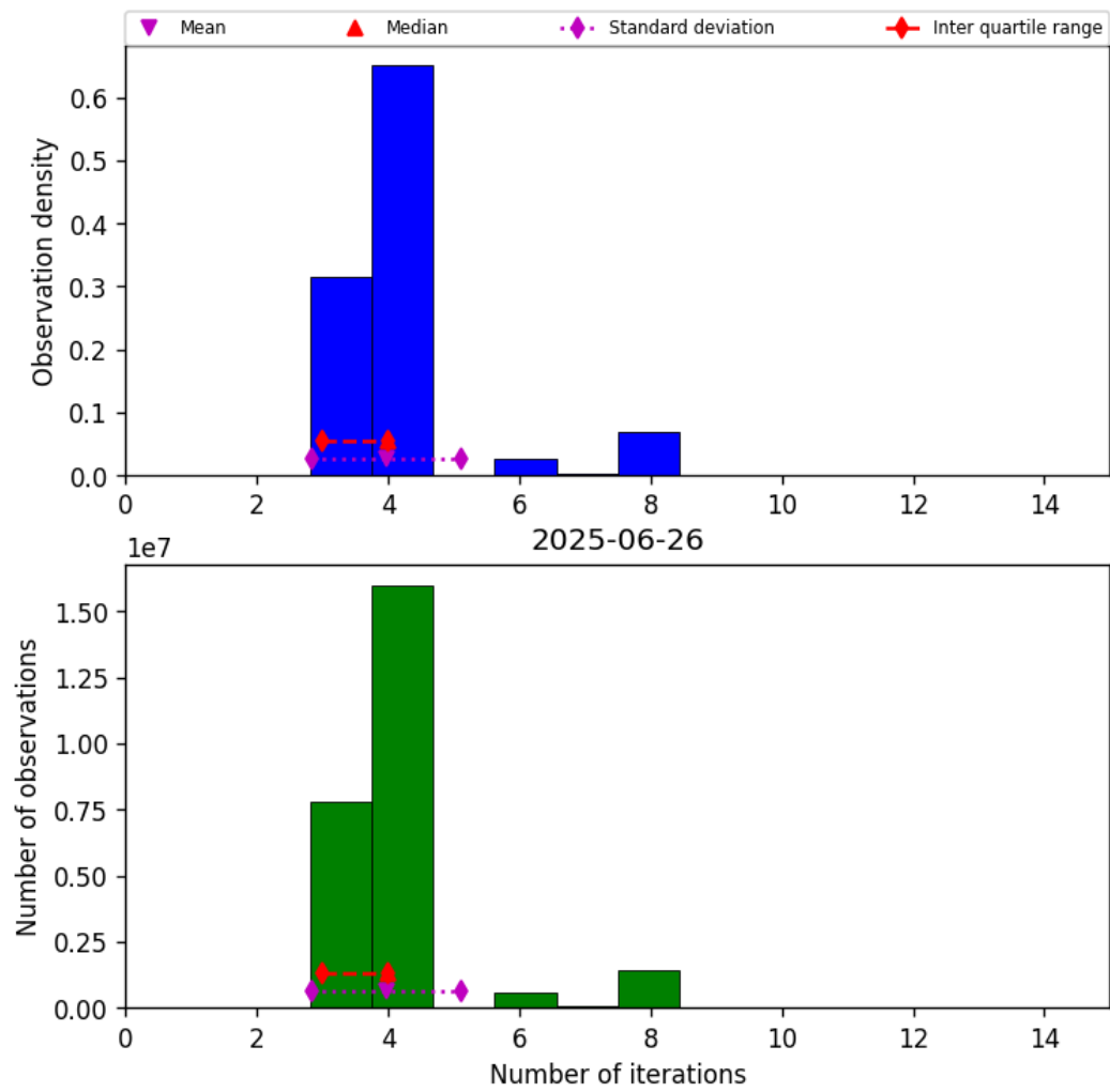
Figure 32: Histogram of “Number of iterations” for 2025-06-26 to 2025-06-27
