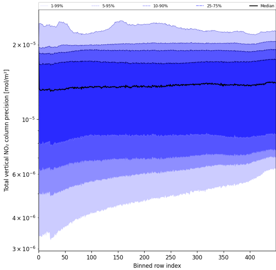
Figure 54: Along track statistics of "Total vertical NO 2 column precision" for 2025-06-26 to 2025-06-27
