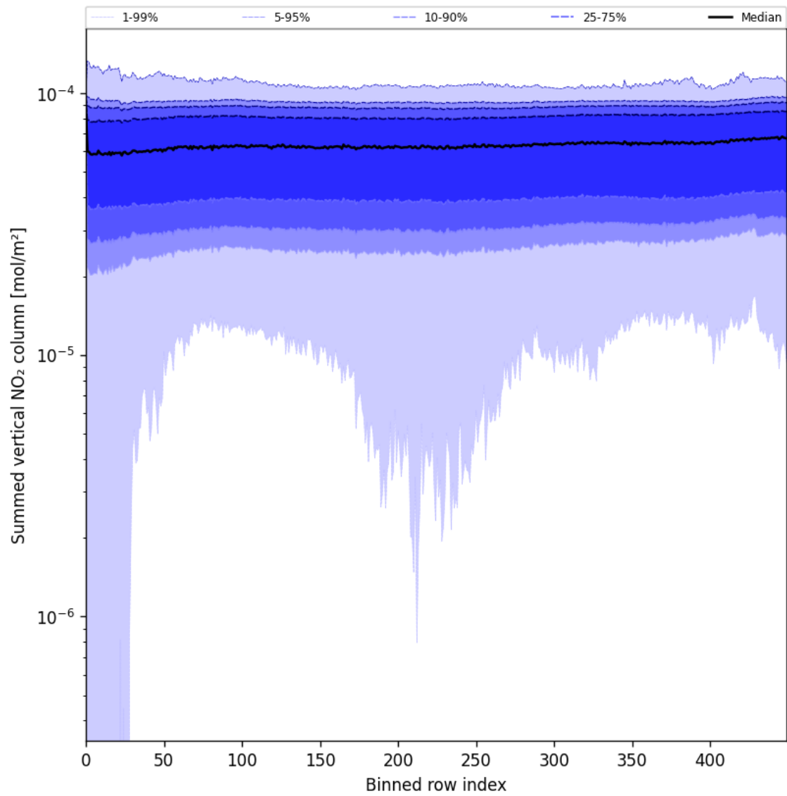
Figure 55: Along track statistics of “Summed vertical NO 2 column” for 2025-06-26 to 2025-06-27
