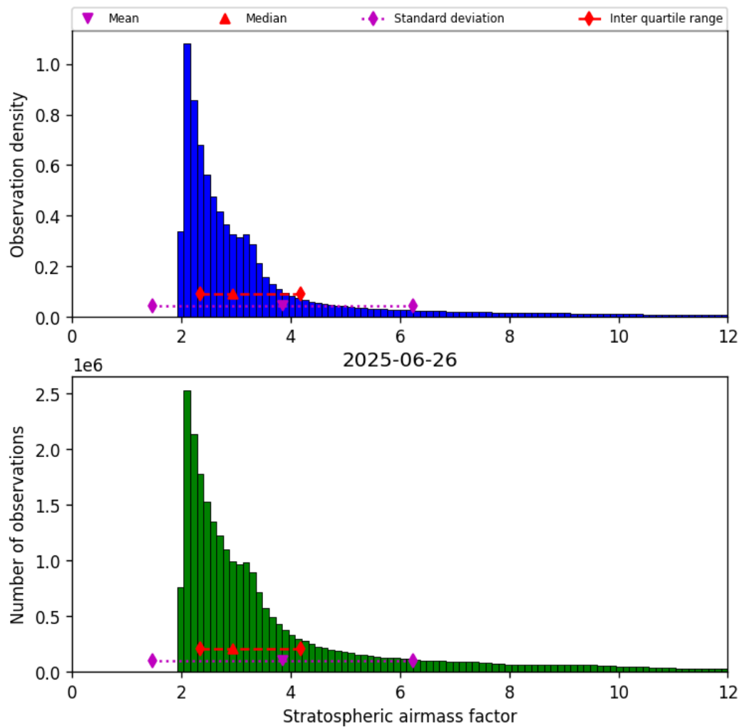
Figure 42: Histogram of “Stratospheric airmass factor” for 2025-06-26 to 2025-06-27
