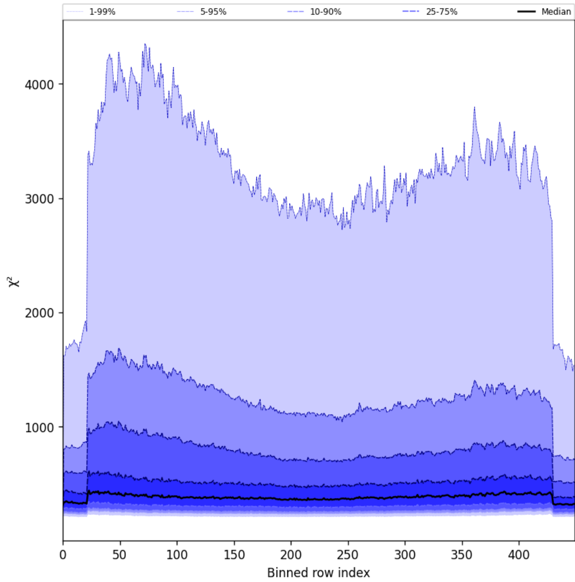
Figure 57: Along track statistics of “ \chi^2 ” for 2025-06-26 to 2025-06-27
