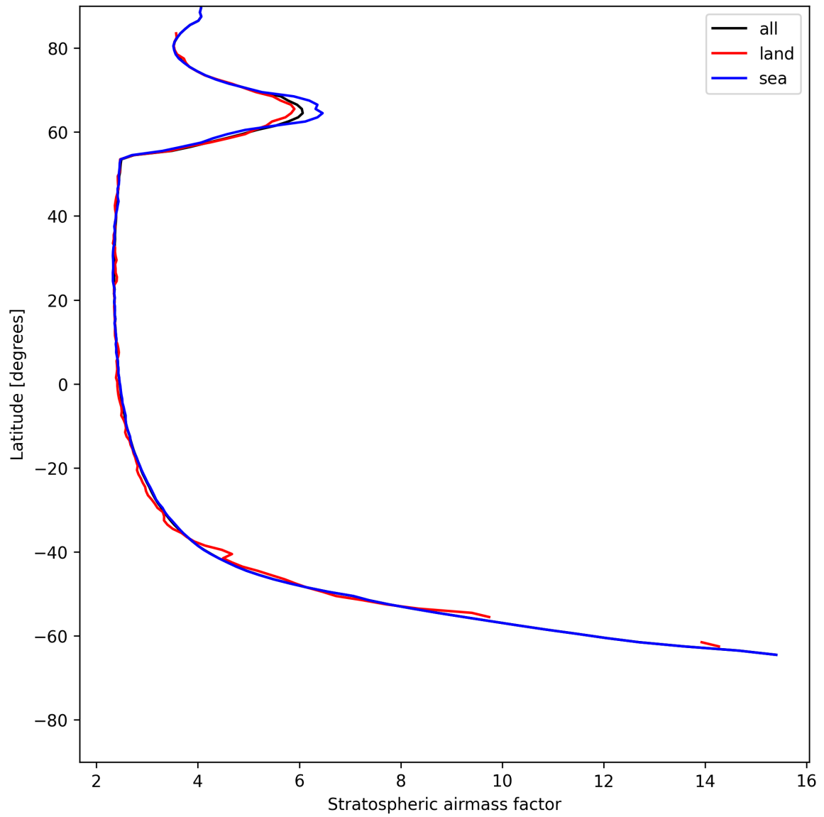
Figure 25: Zonal average of “Stratospheric airmass factor” for 2025-06-26 to 2025-06-27.
