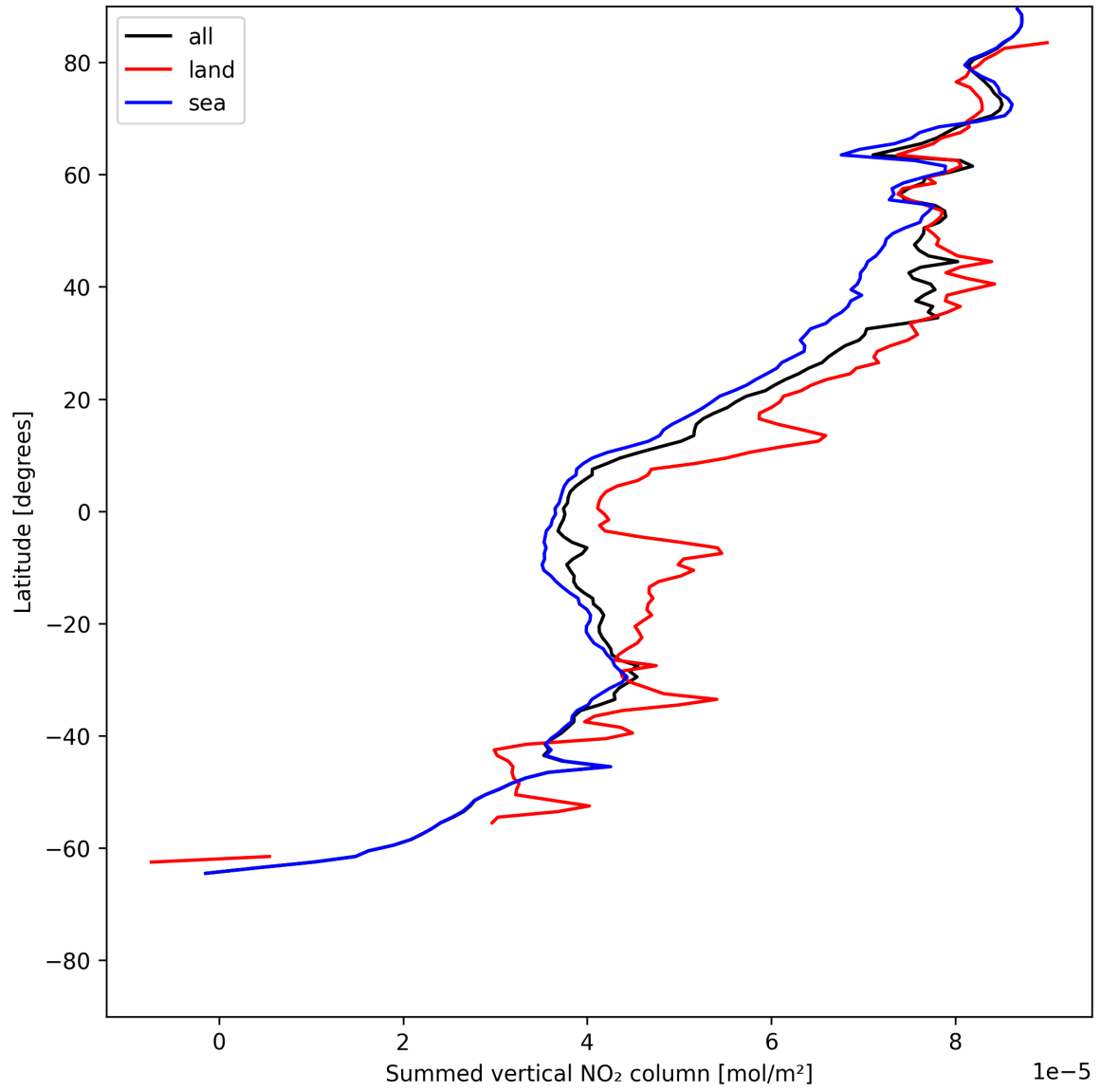
Figure 21: Zonal average of “Summed vertical NO 2 column” for 2025-06-26 to 2025-06-27.
