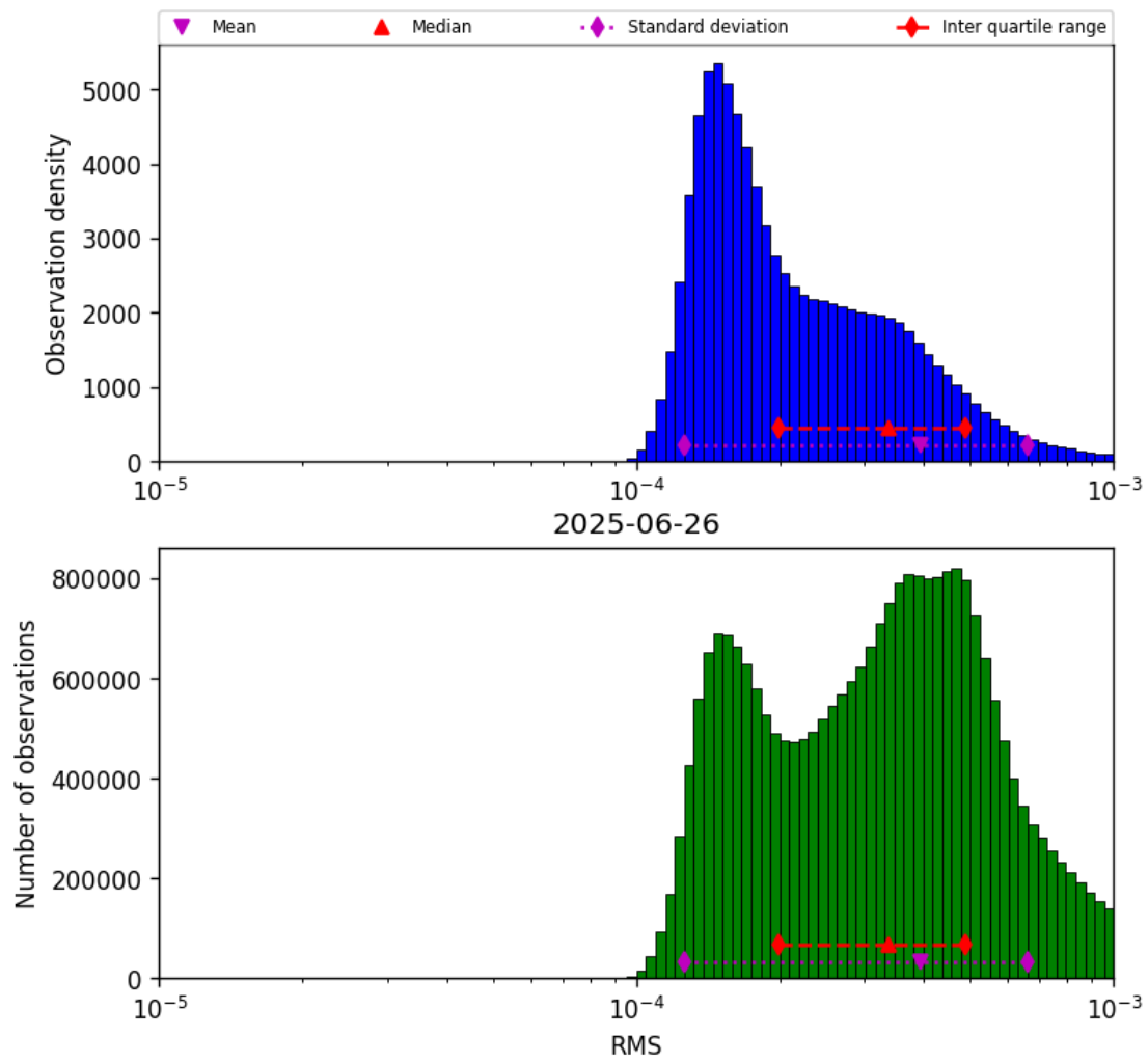
Figure 41: Histogram of “RMS” for 2025-06-26 to 2025-06-27
