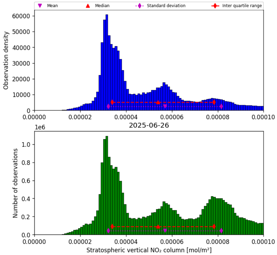
Figure 34: Histogram of “Stratospheric vertical NO 2 column” for 2025-06-26 to 2025-06-27
