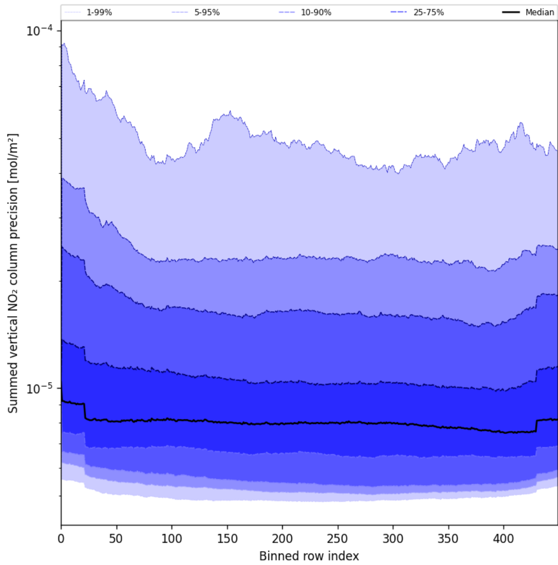
Figure 56: Along track statistics of “Summed vertical NO 2 column precision” for 2025-06-26 to 2025-06-27
