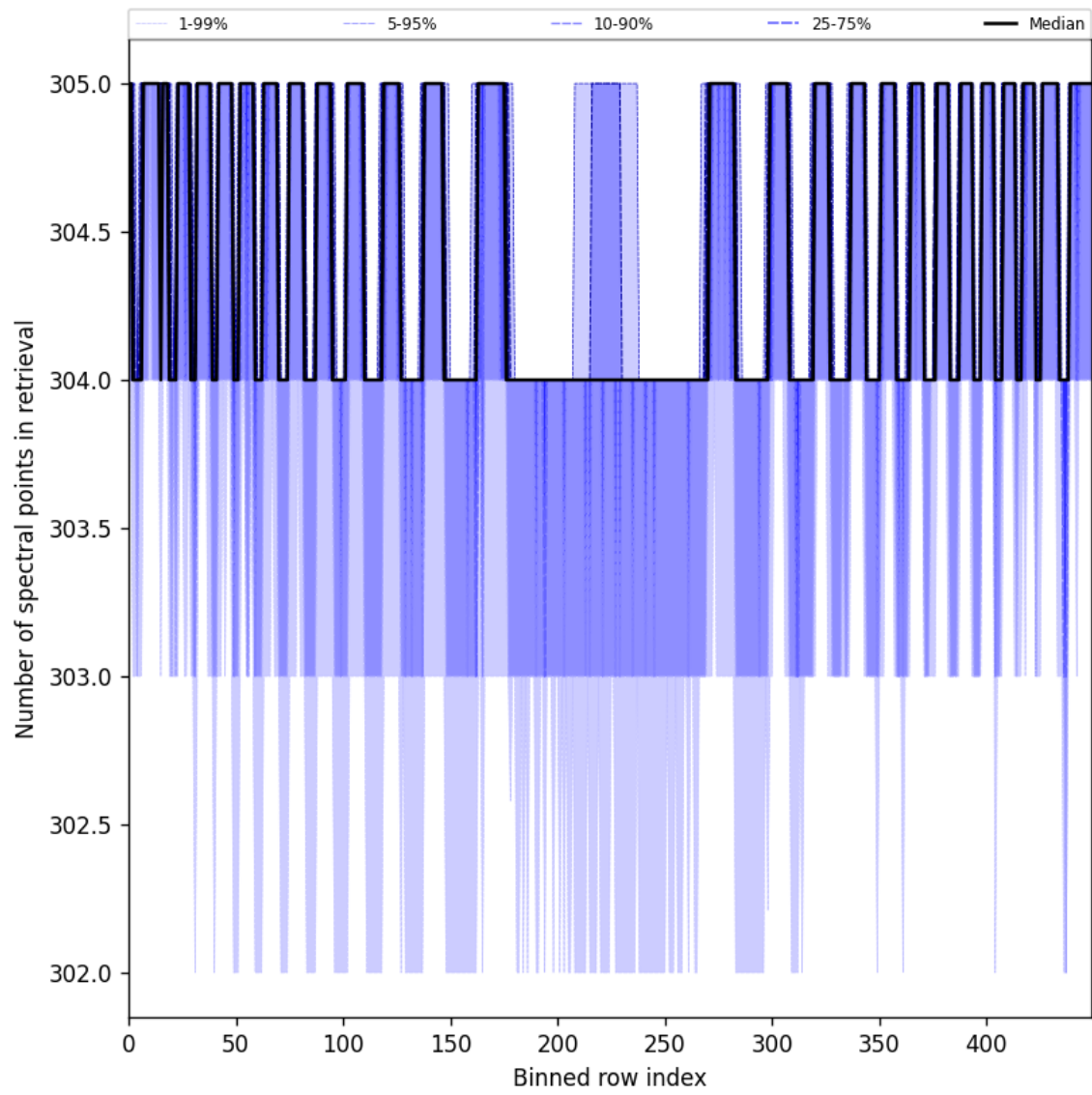
Figure 48: Along track statistics of “Number of spectral points in retrieval” for 2025-06-26 to 2025-06-27
