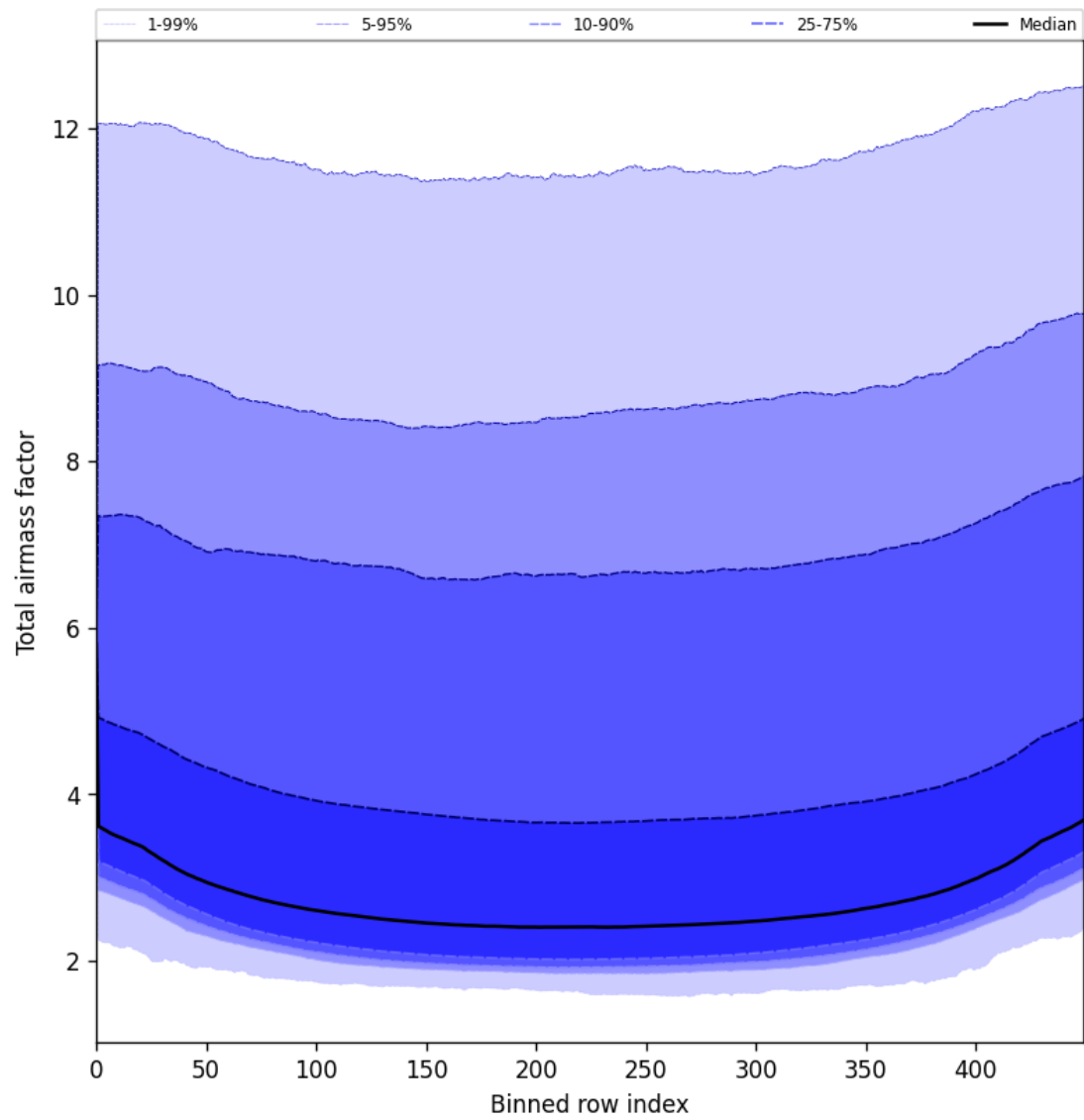
Figure 47: Along track statistics of “Total airmass factor” for 2025-06-26 to 2025-06-27
