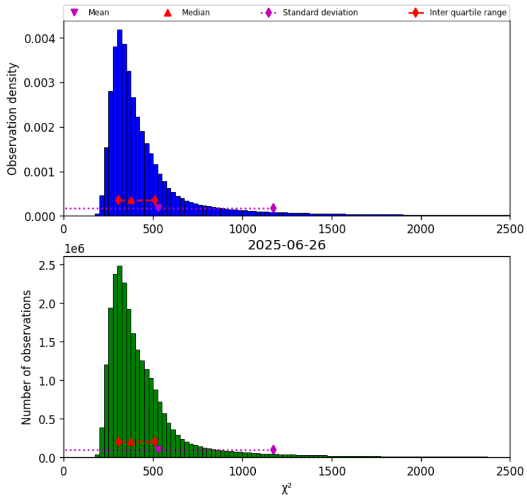
Figure 40: Histogram of " \chi^2 " for 2025-06-26 to 2025-06-27
