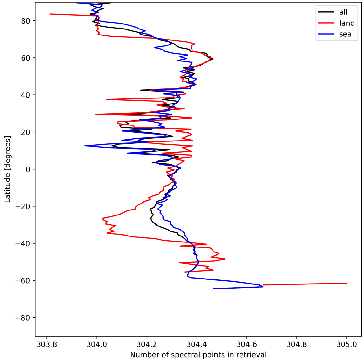
Figure 14: Zonal average of “Number of spectral points in retrieval” for 2025-06-26 to 2025-06-27.
