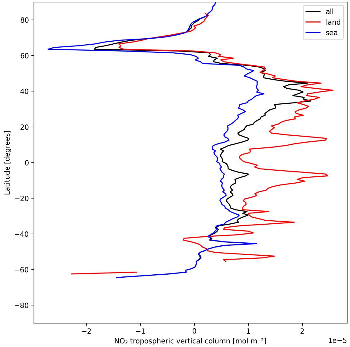
Figure 10: Zonal average of “NO 2 tropospheric vertical column” for 2025-06-26 to 2025-06-27.
