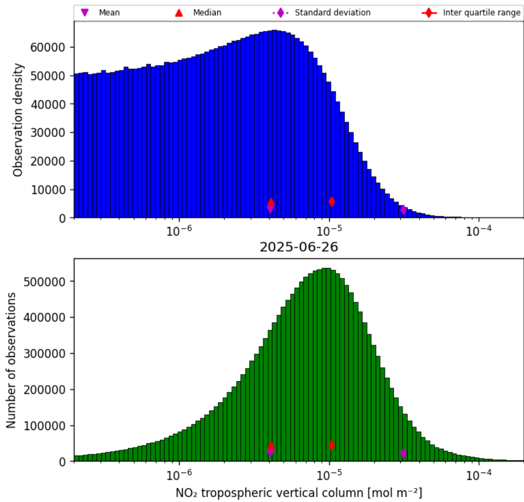
Figure 27: Histogram of “NO 2 tropospheric vertical column” for 2025-06-26 to 2025-06-27
