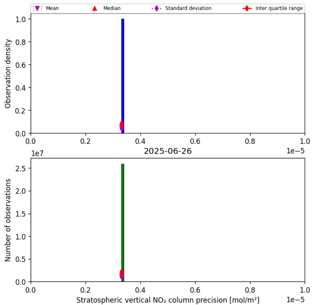
Figure 35: Histogram of “Stratospheric vertical NO 2 column precision” for 2025-06-26 to 2025-06-27
