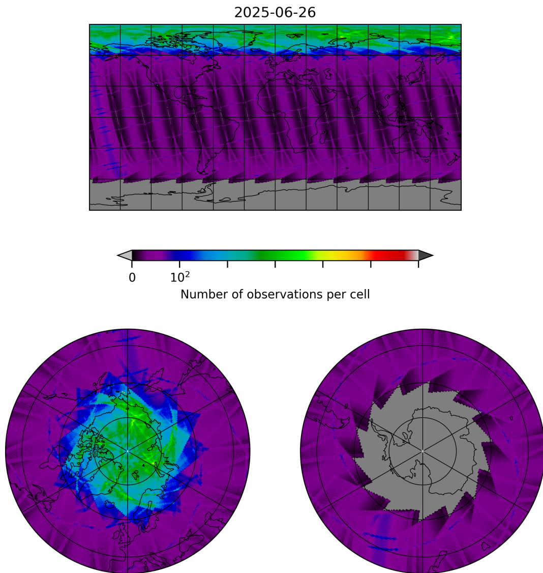
Figure 8: Map of the number of observations for 2025-06-26 to 2025-06-27
