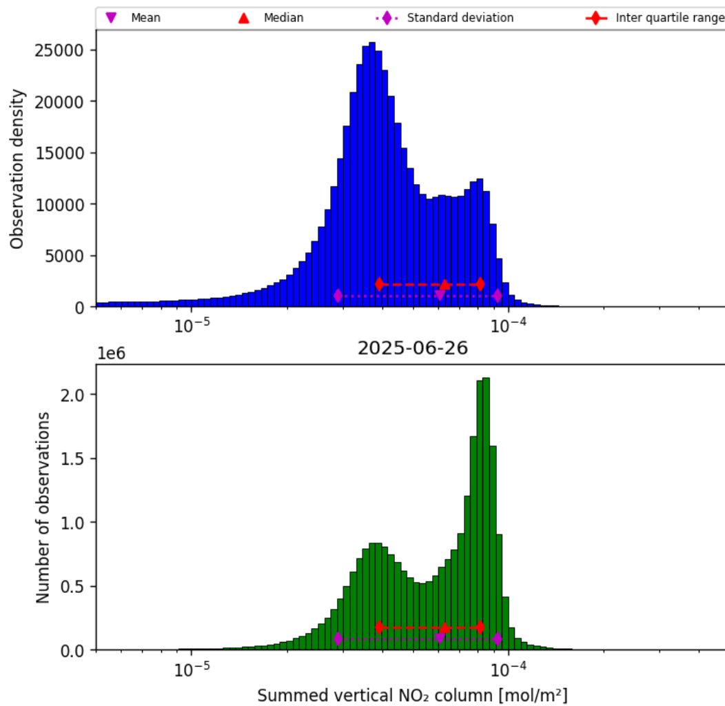
Figure 38: Histogram of “Summed vertical NO 2 column” for 2025-06-26 to 2025-06-27
