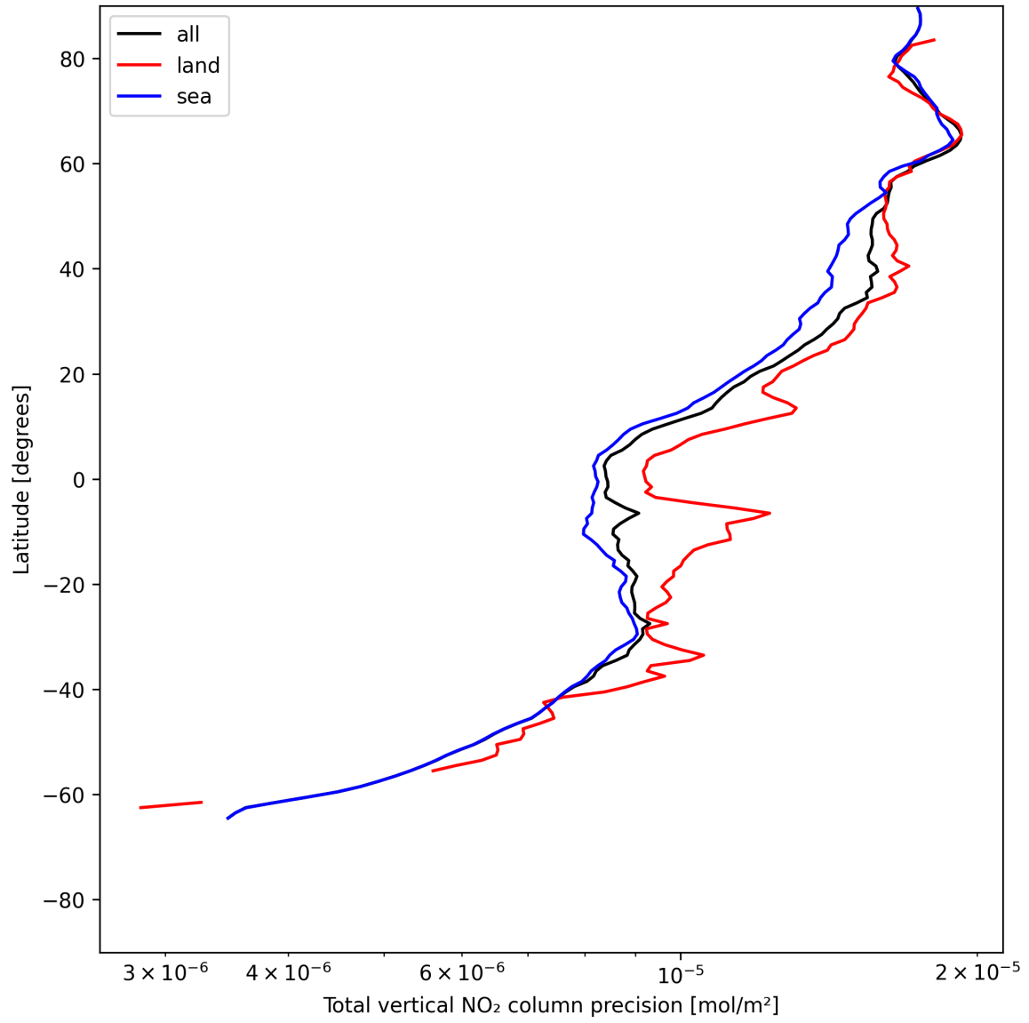
Figure 20: Zonal average of “Total vertical NO 2 column precision” for 2025-06-26 to 2025-06-27.
