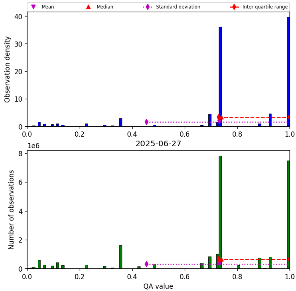
Figure 26: Histogram of “QA value” for 2025-06-27 to 2025-06-28
