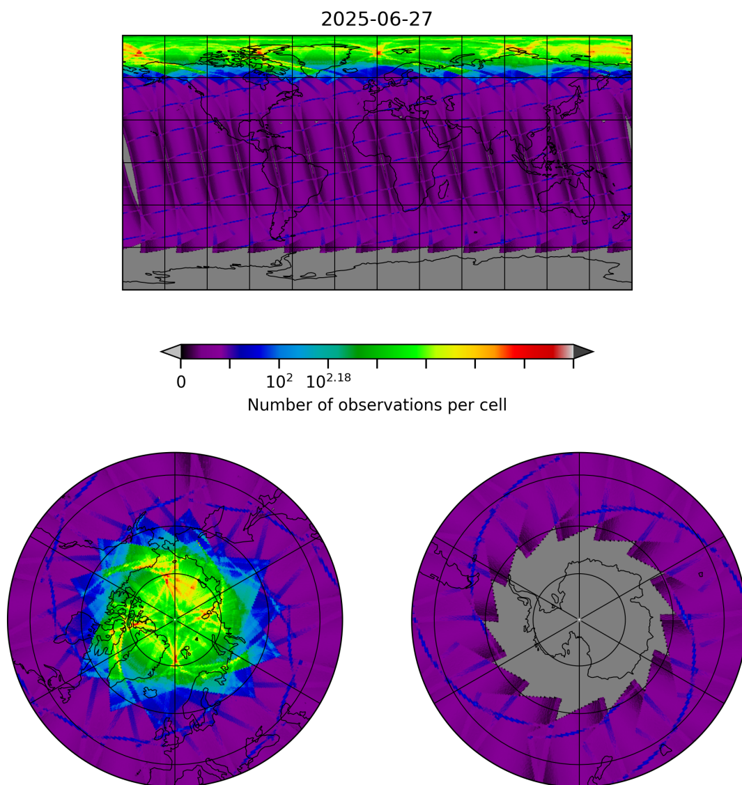
Figure 8: Map of the number of observations for 2025-06-27 to 2025-06-28
