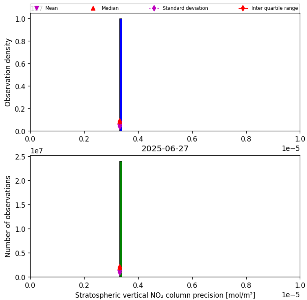
Figure 35: Histogram of “Stratospheric vertical NO 2 column precision” for 2025-06-27 to 2025-06-28
