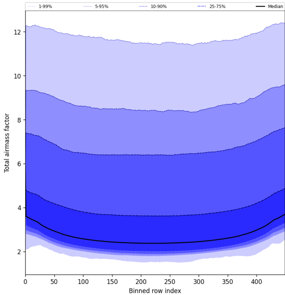
Figure 47: Along track statistics of “Total airmass factor” for 2025-06-27 to 2025-06-28
