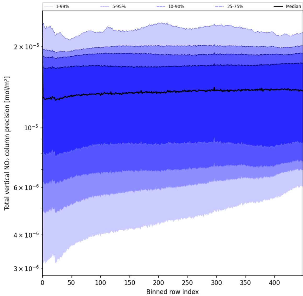
Figure 54: Along track statistics of “Total vertical NO 2 column precision” for 2025-06-27 to 2025-06-28
