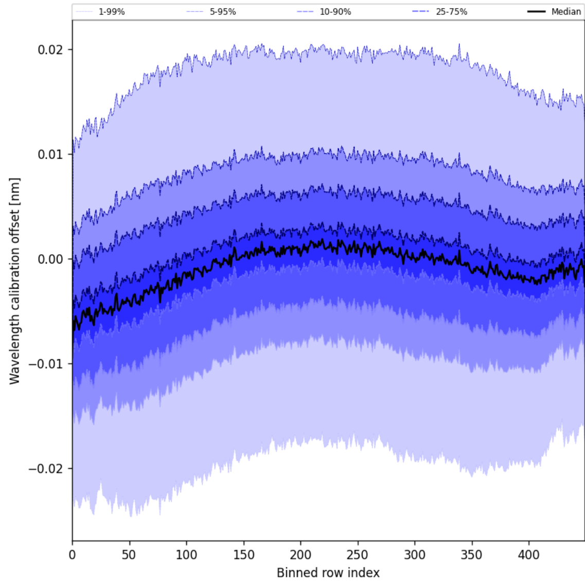
Figure 50: Along track statistics of “Wavelength calibration offset” for 2025-06-27 to 2025-06-28
