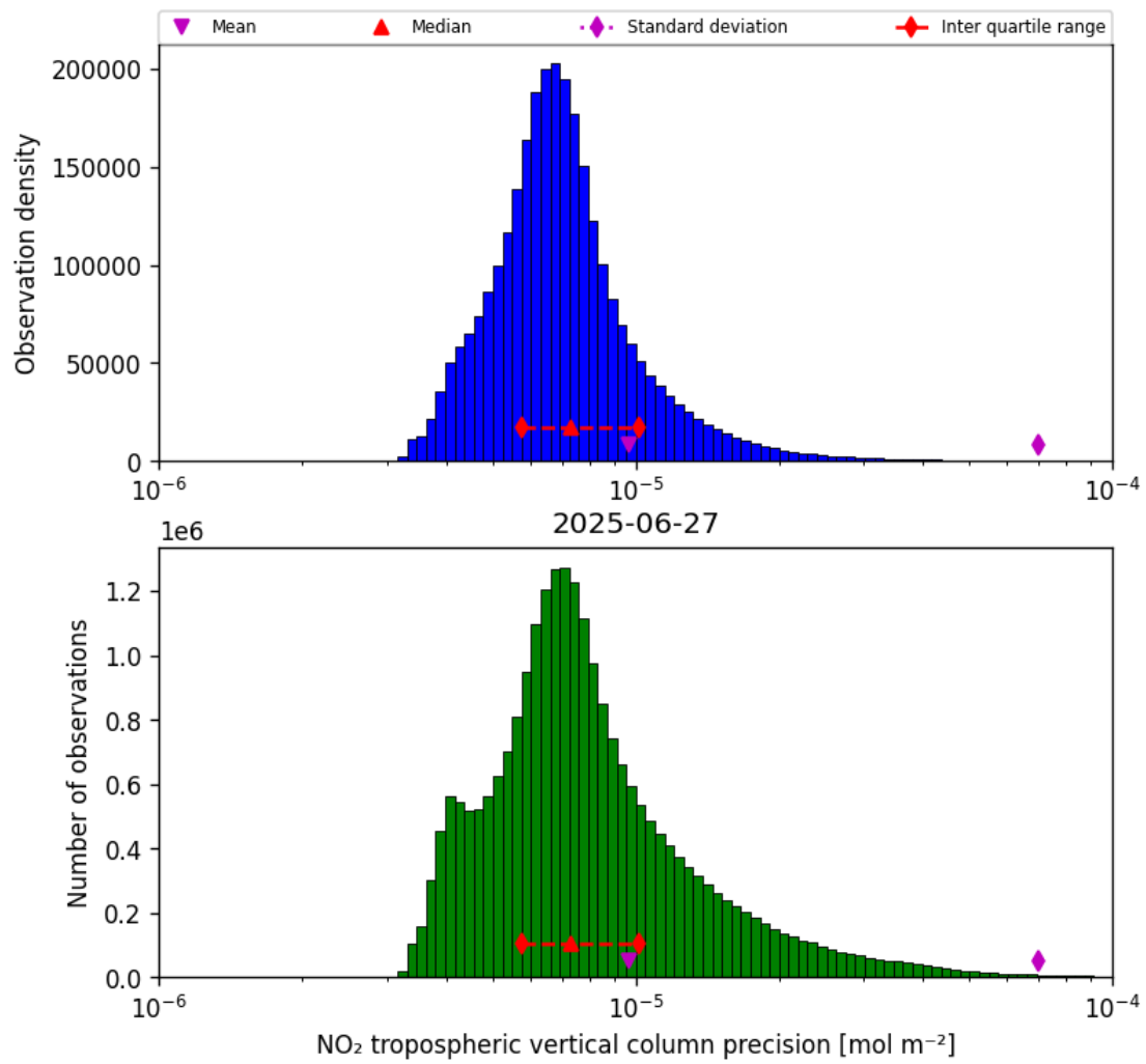
Figure 28: Histogram of “NO 2 tropospheric vertical column precision” for 2025-06-27 to 2025-06-28
