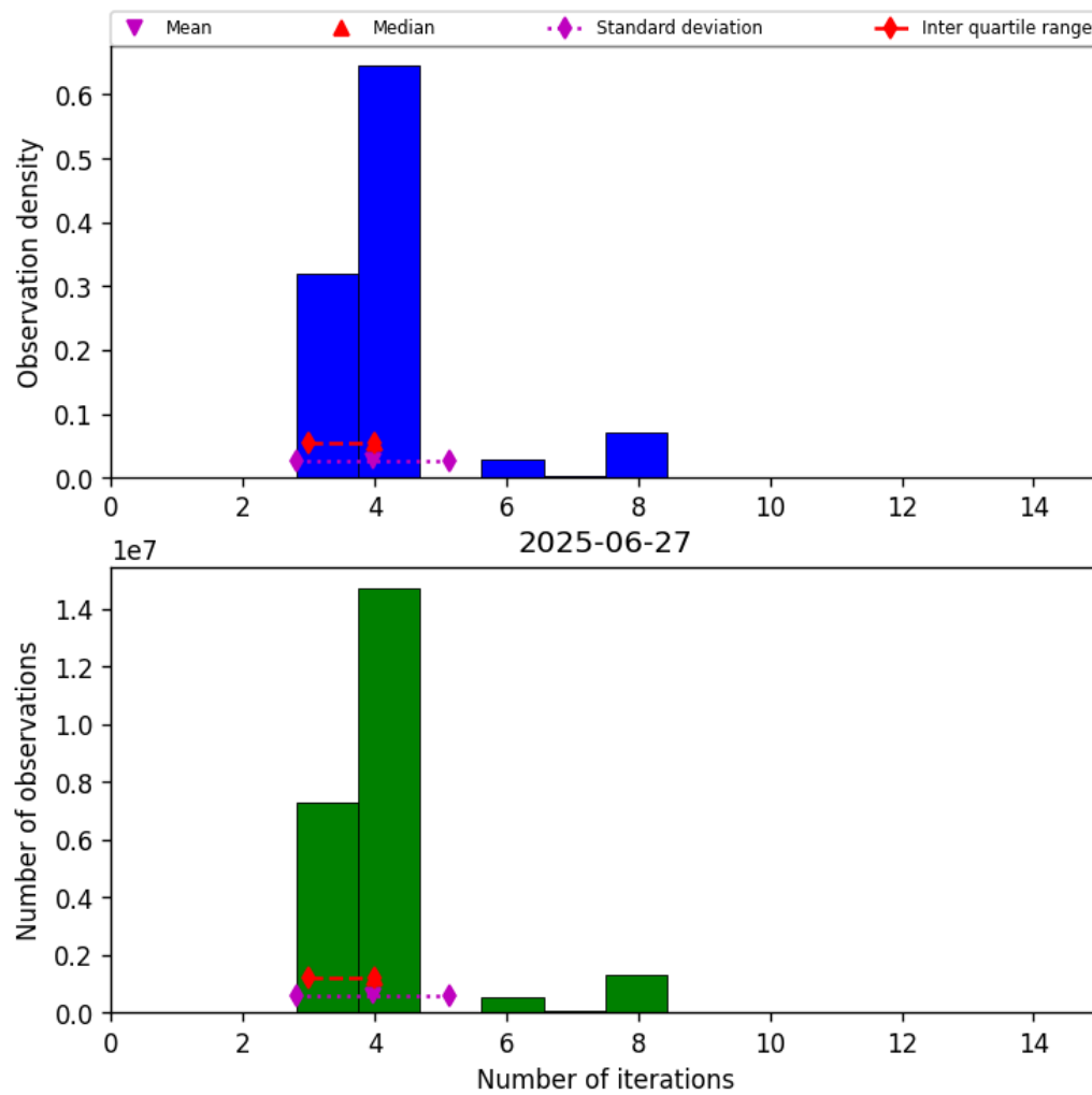
Figure 32: Histogram of “Number of iterations” for 2025-06-27 to 2025-06-28
