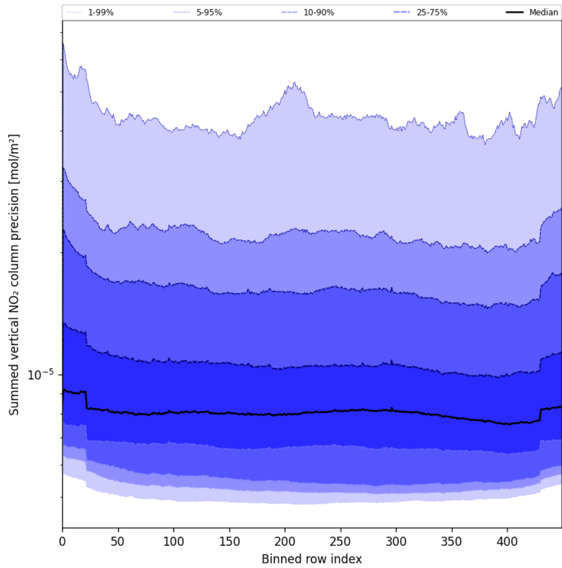
Figure 56: Along track statistics of “Summed vertical NO 2 column precision” for 2025-06-27 to 2025-06-28
