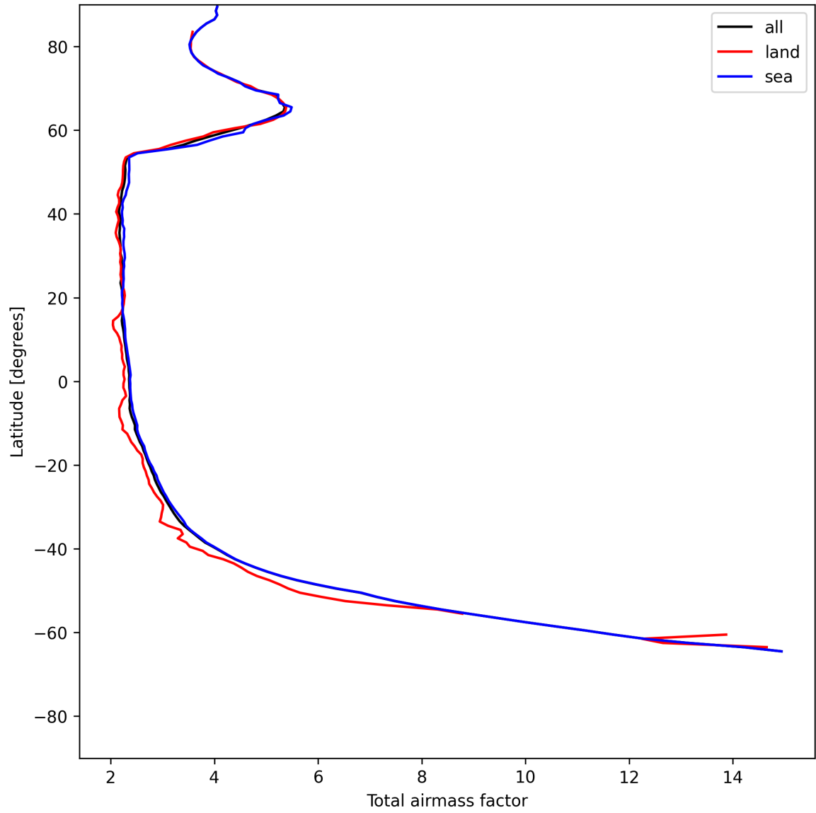
Figure 13: Zonal average of “Total airmass factor” for 2025-06-27 to 2025-06-28.
