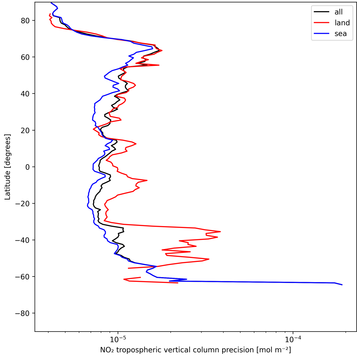
Figure 11: Zonal average of “NO 2 tropospheric vertical column precision” for 2025-06-27 to 2025-06-28.
