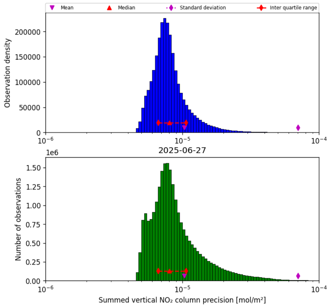
Figure 39: Histogram of “Summed vertical NO 2 column precision” for 2025-06-27 to 2025-06-28
