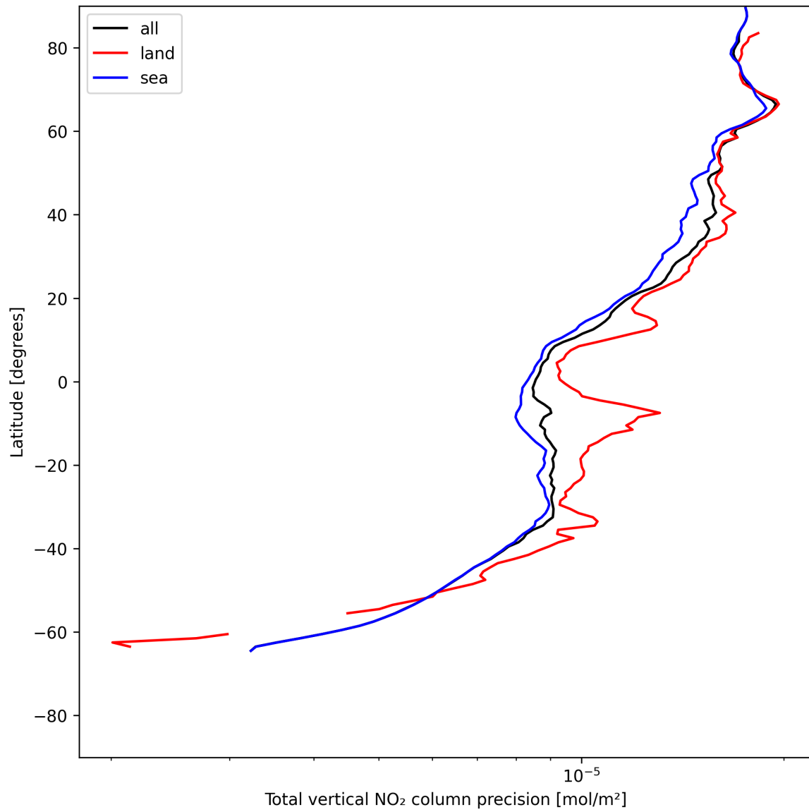
Figure 20: Zonal average of “Total vertical NO 2 column precision” for 2025-06-27 to 2025-06-28.
