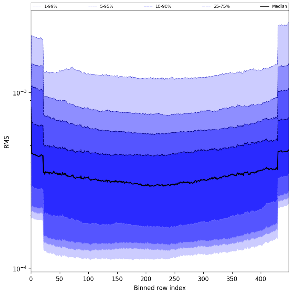
Figure 58: Along track statistics of “RMS” for 2025-06-27 to 2025-06-28
