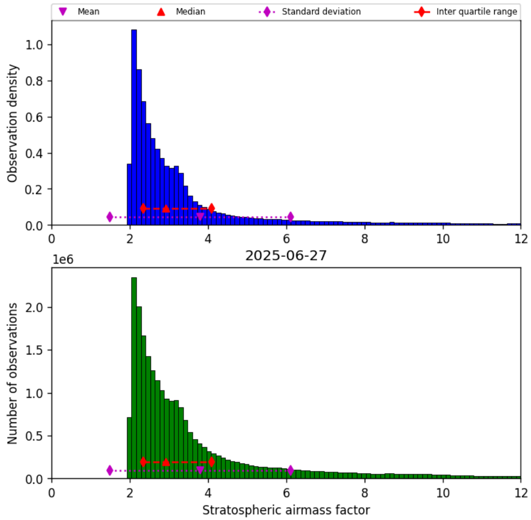
Figure 42: Histogram of “Stratospheric airmass factor” for 2025-06-27 to 2025-06-28
