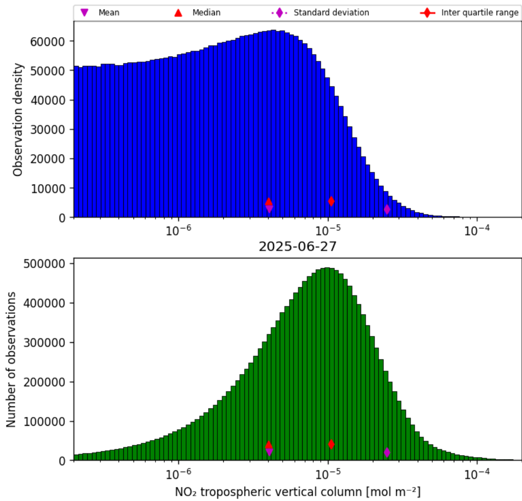
Figure 27: Histogram of “NO 2 tropospheric vertical column” for 2025-06-27 to 2025-06-28
