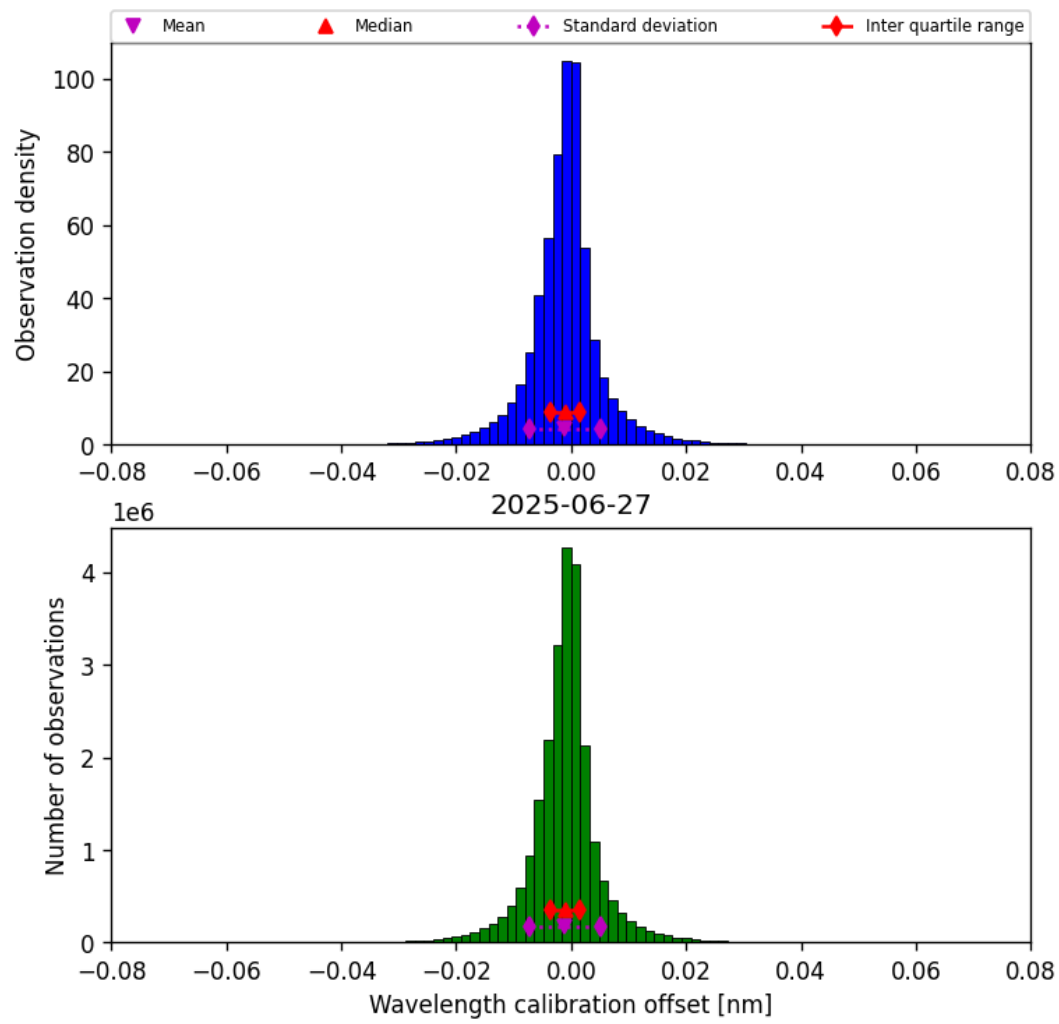
Figure 33: Histogram of “Wavelength calibration offset” for 2025-06-27 to 2025-06-28
