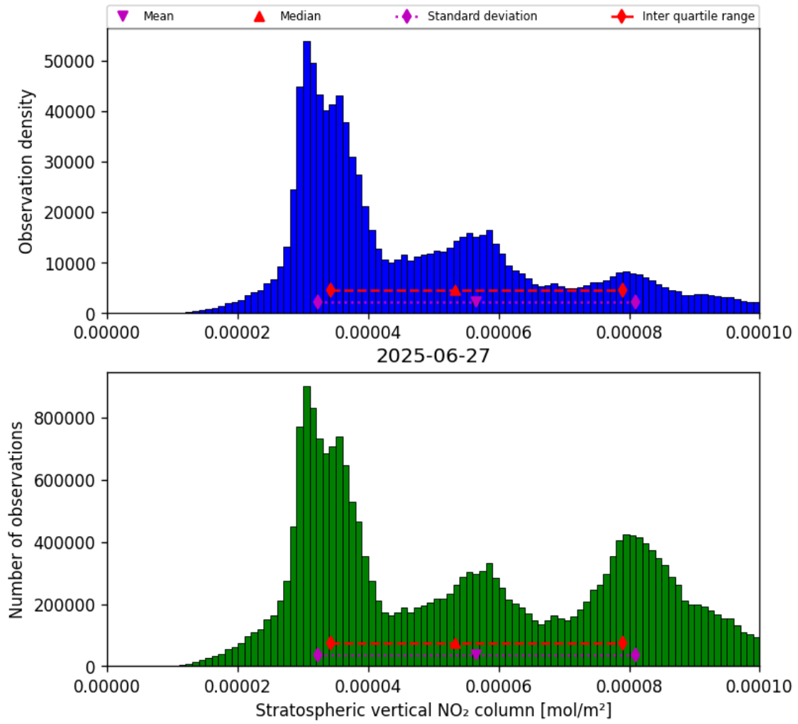
Figure 34: Histogram of “Stratospheric vertical NO 2 column” for 2025-06-27 to 2025-06-28
