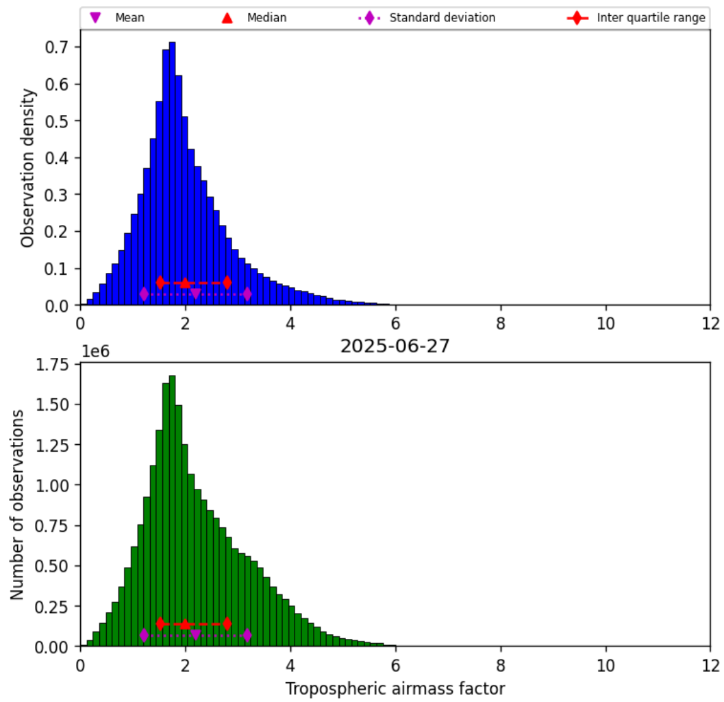
Figure 29: Histogram of “Tropospheric airmass factor” for 2025-06-27 to 2025-06-28
