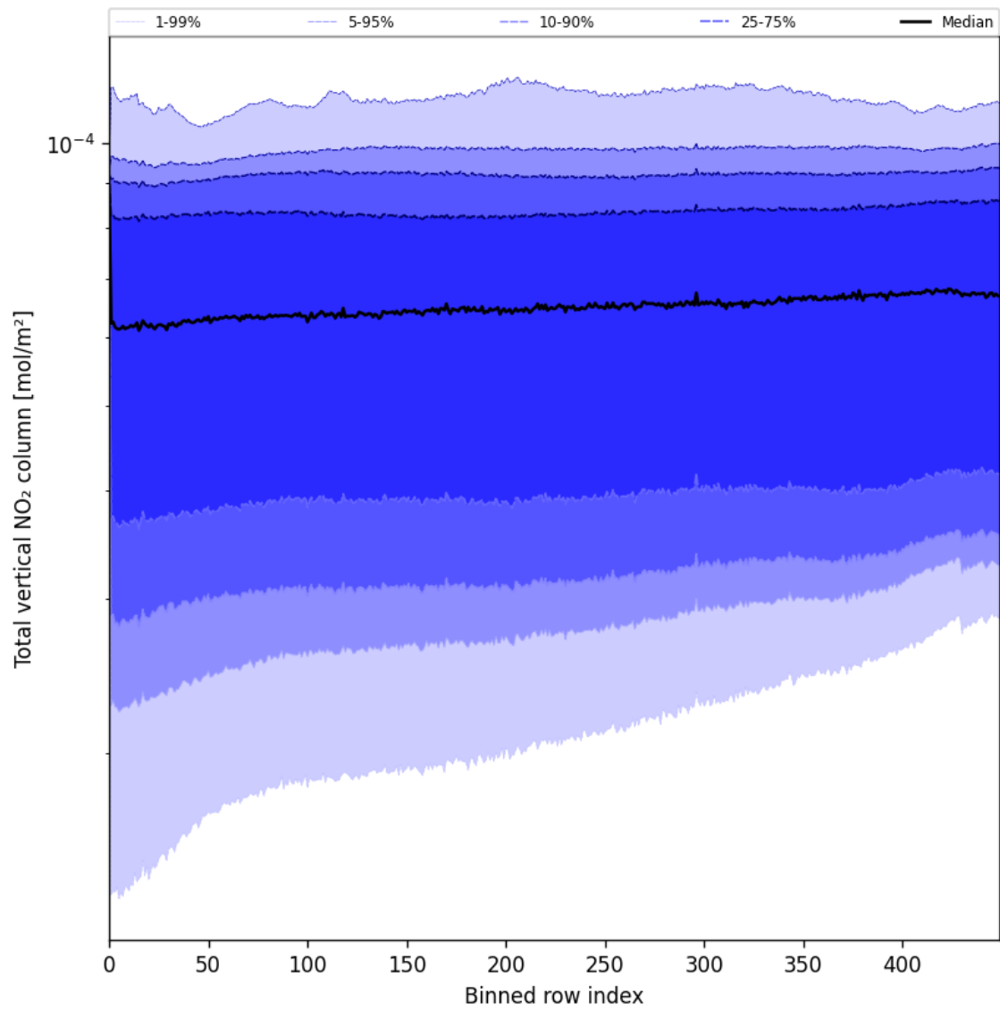
Figure 53: Along track statistics of “Total vertical NO 2 column” for 2025-06-27 to 2025-06-28
