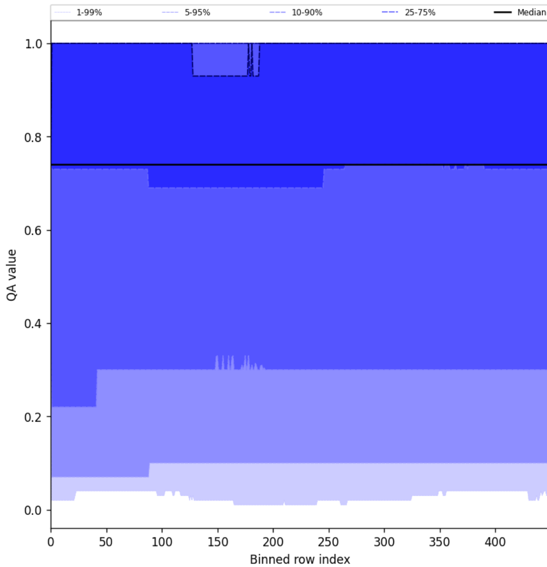
Figure 43: Along track statistics of “QA value” for 2025-06-27 to 2025-06-28
