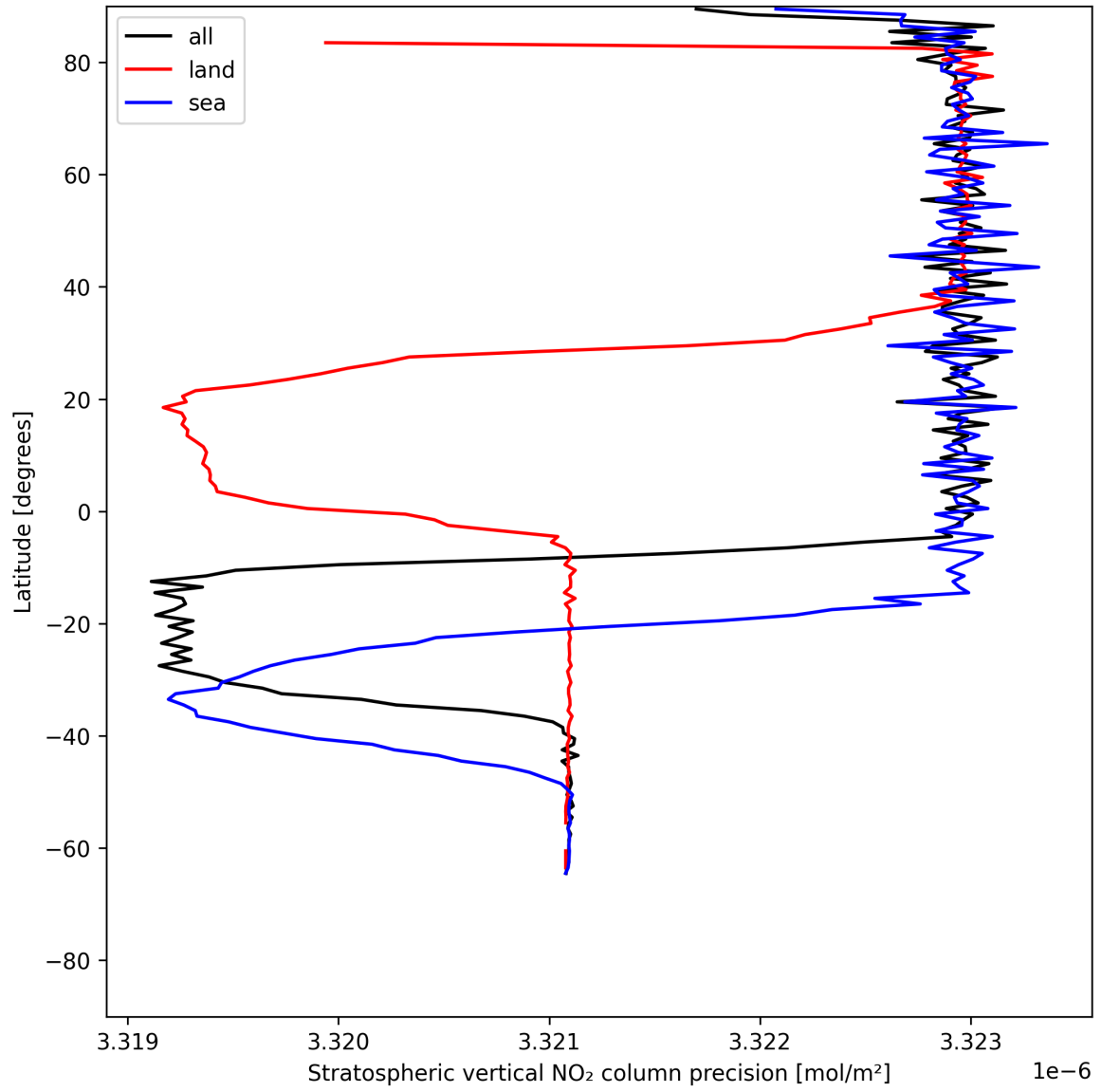
Figure 18: Zonal average of “Stratospheric vertical NO 2 column precision” for 2025-06-27 to 2025-06-28.
