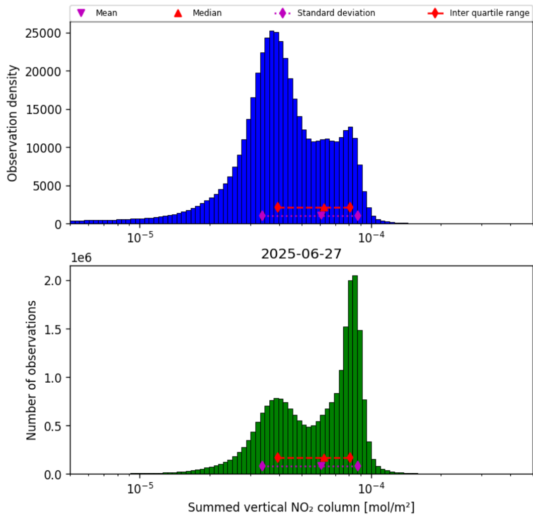
Figure 38: Histogram of “Summed vertical NO 2 column” for 2025-06-27 to 2025-06-28
