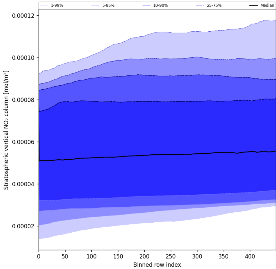
Figure 51: Along track statistics of “Stratospheric vertical NO 2 column” for 2025-06-27 to 2025-06-28
