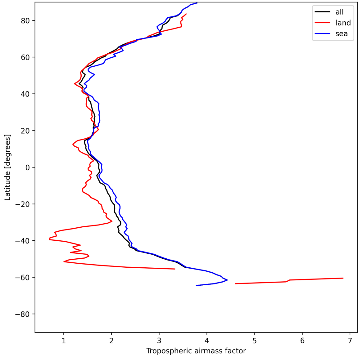
Figure 12: Zonal average of “Tropospheric airmass factor” for 2025-06-27 to 2025-06-28.
