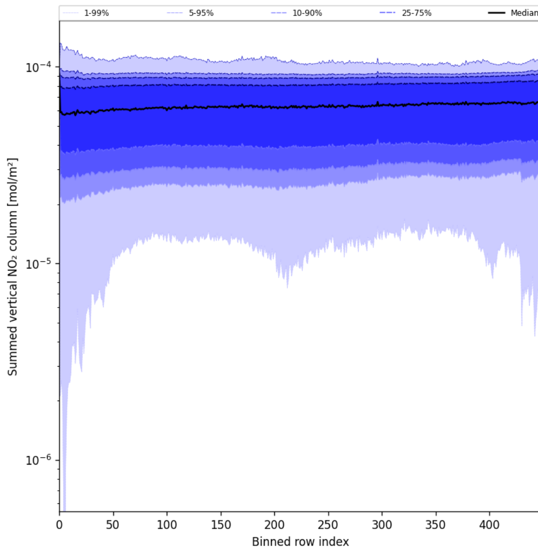
Figure 55: Along track statistics of “Summed vertical NO 2 column” for 2025-06-27 to 2025-06-28
