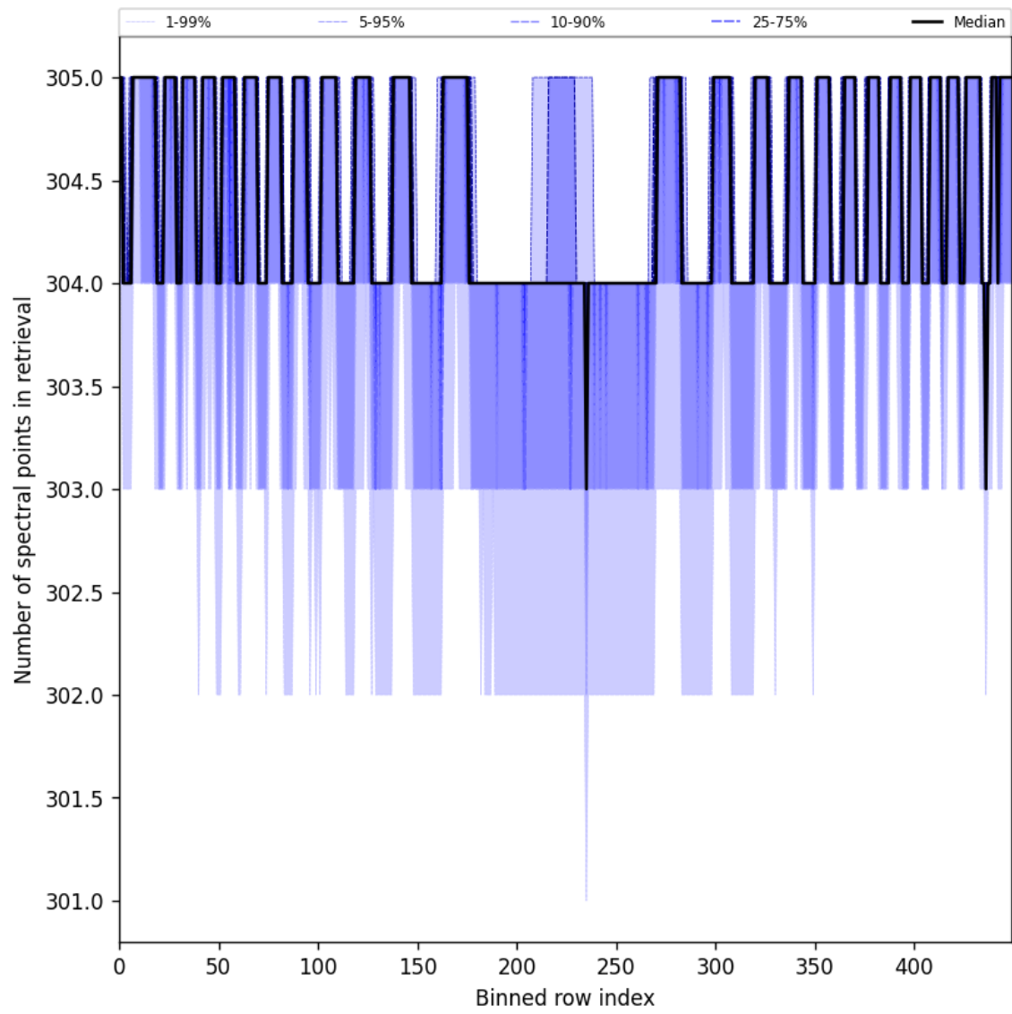
Figure 48: Along track statistics of “Number of spectral points in retrieval” for 2025-06-27 to 2025-06-28
