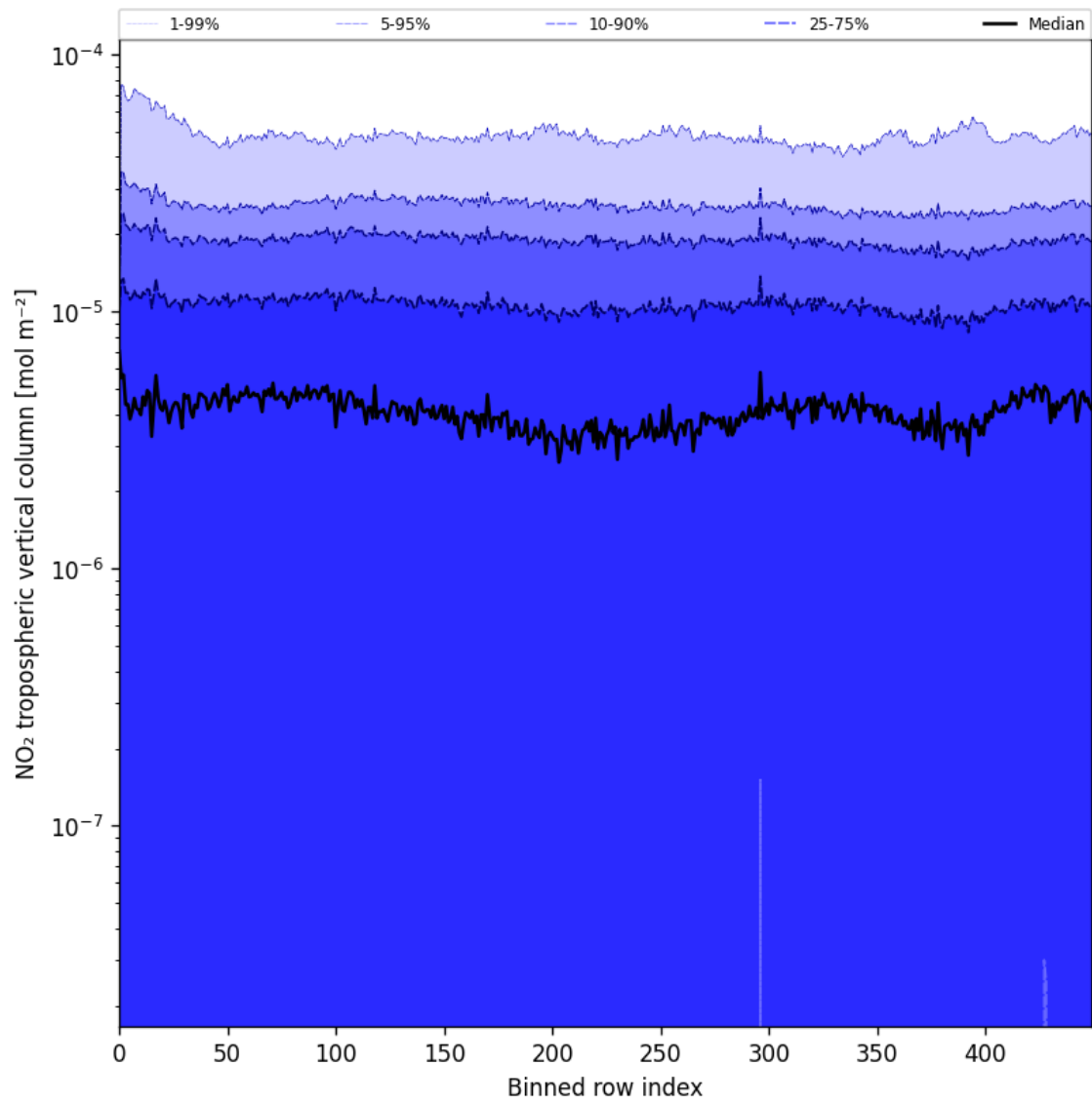
Figure 44: Along track statistics of "NO 2 tropospheric vertical column" for 2025-06-27 to 2025-06-28
