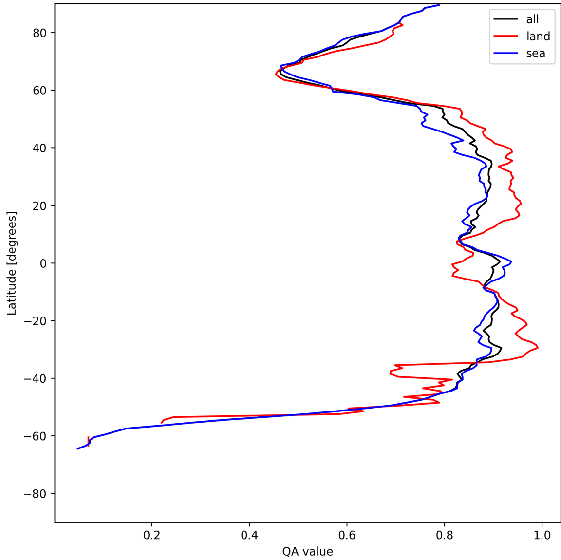
Figure 9: Zonal average of “QA value” for 2025-06-27 to 2025-06-28.
