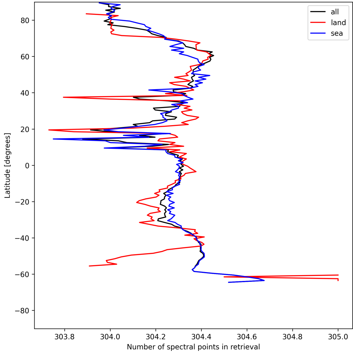
Figure 14: Zonal average of “Number of spectral points in retrieval” for 2025-06-27 to 2025-06-28.
