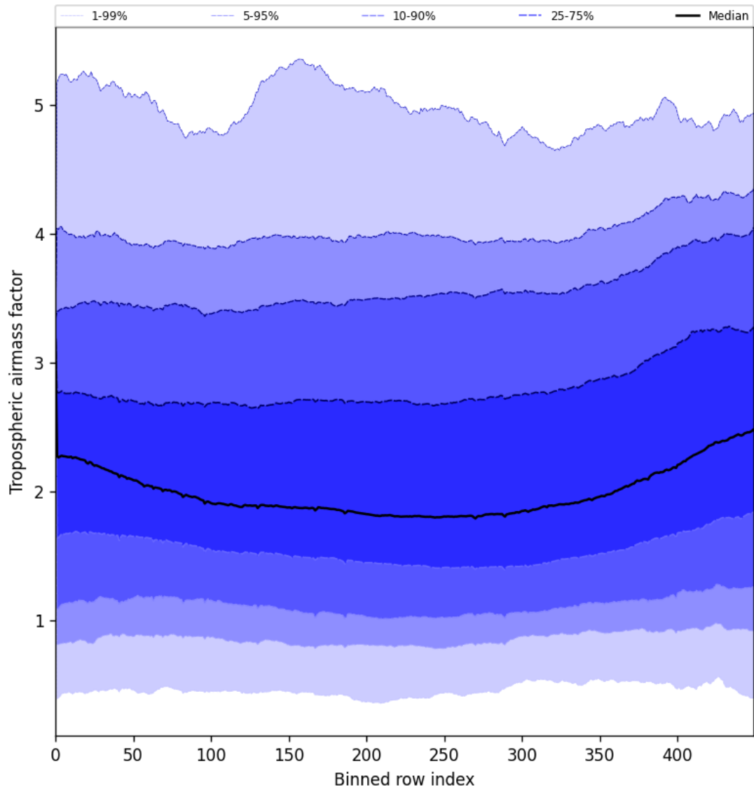
Figure 46: Along track statistics of “Tropospheric airmass factor” for 2025-06-27 to 2025-06-28
