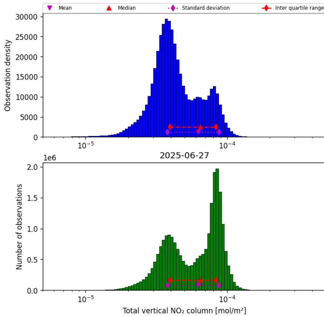
Figure 36: Histogram of “Total vertical NO 2 column” for 2025-06-27 to 2025-06-28
