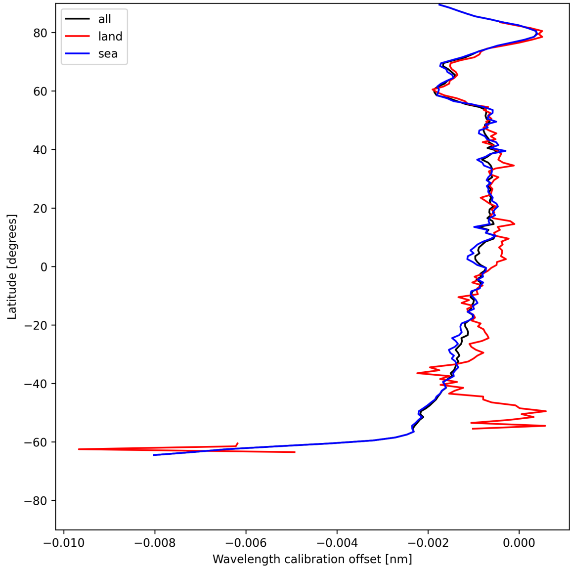
Figure 16: Zonal average of “Wavelength calibration offset” for 2025-06-27 to 2025-06-28.
