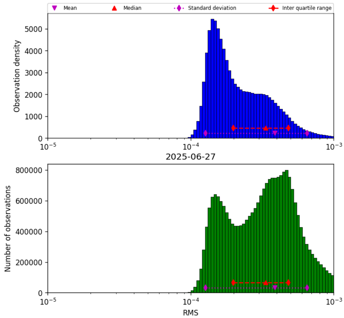
Figure 41: Histogram of “RMS” for 2025-06-27 to 2025-06-28
