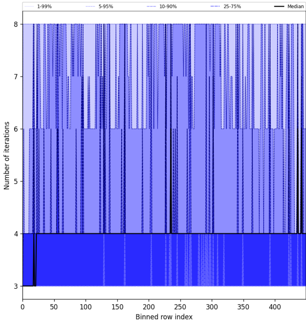
Figure 49: Along track statistics of “Number of iterations” for 2025-06-27 to 2025-06-28
