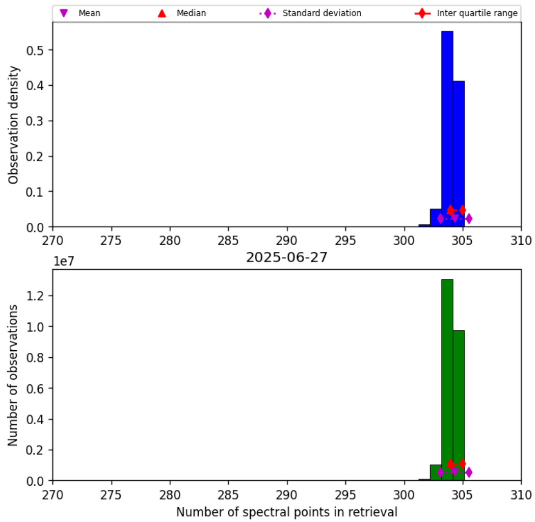
Figure 31: Histogram of “Number of spectral points in retrieval” for 2025-06-27 to 2025-06-28
