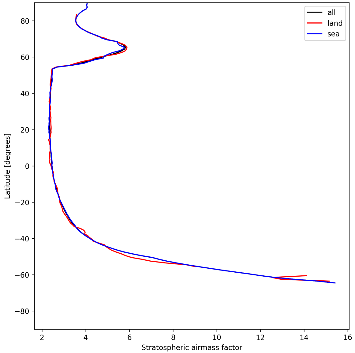
Figure 25: Zonal average of “Stratospheric airmass factor” for 2025-06-27 to 2025-06-28.
