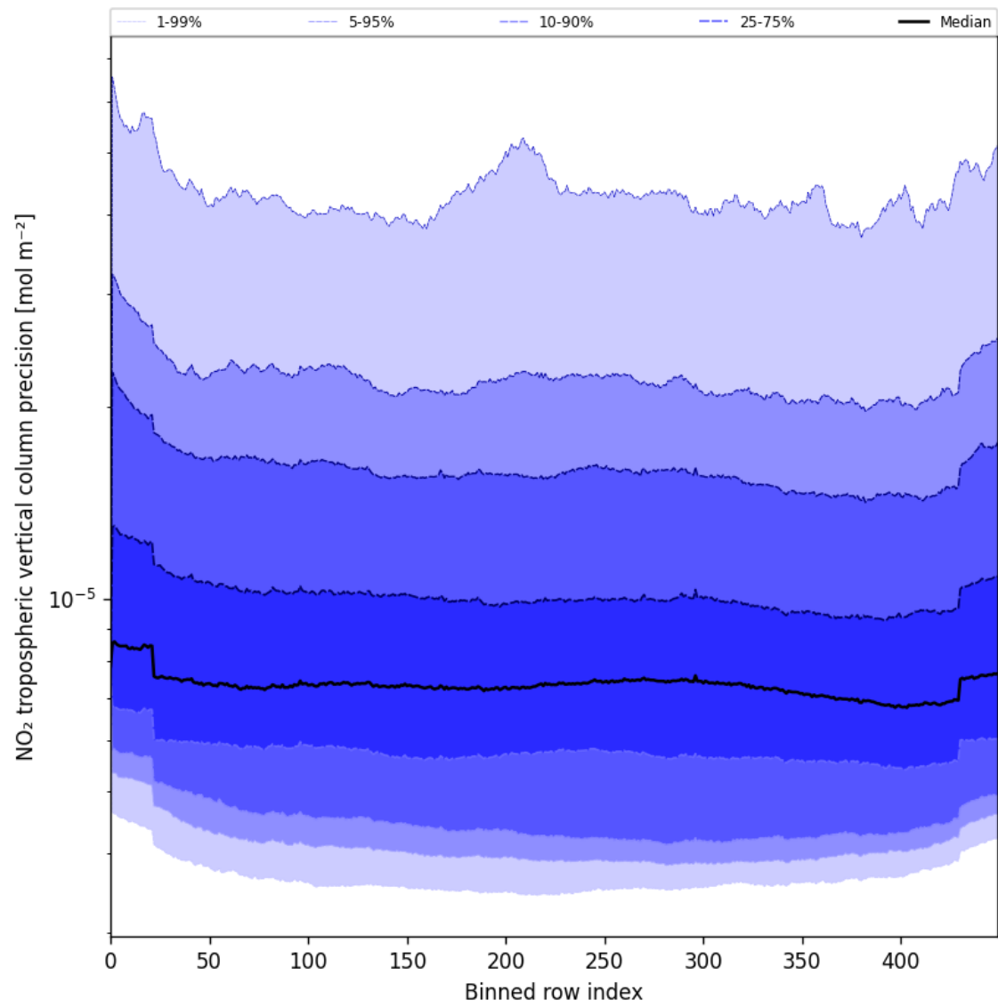
Figure 45: Along track statistics of “NO 2 tropospheric vertical column precision” for 2025-06-27 to 2025-06-28
