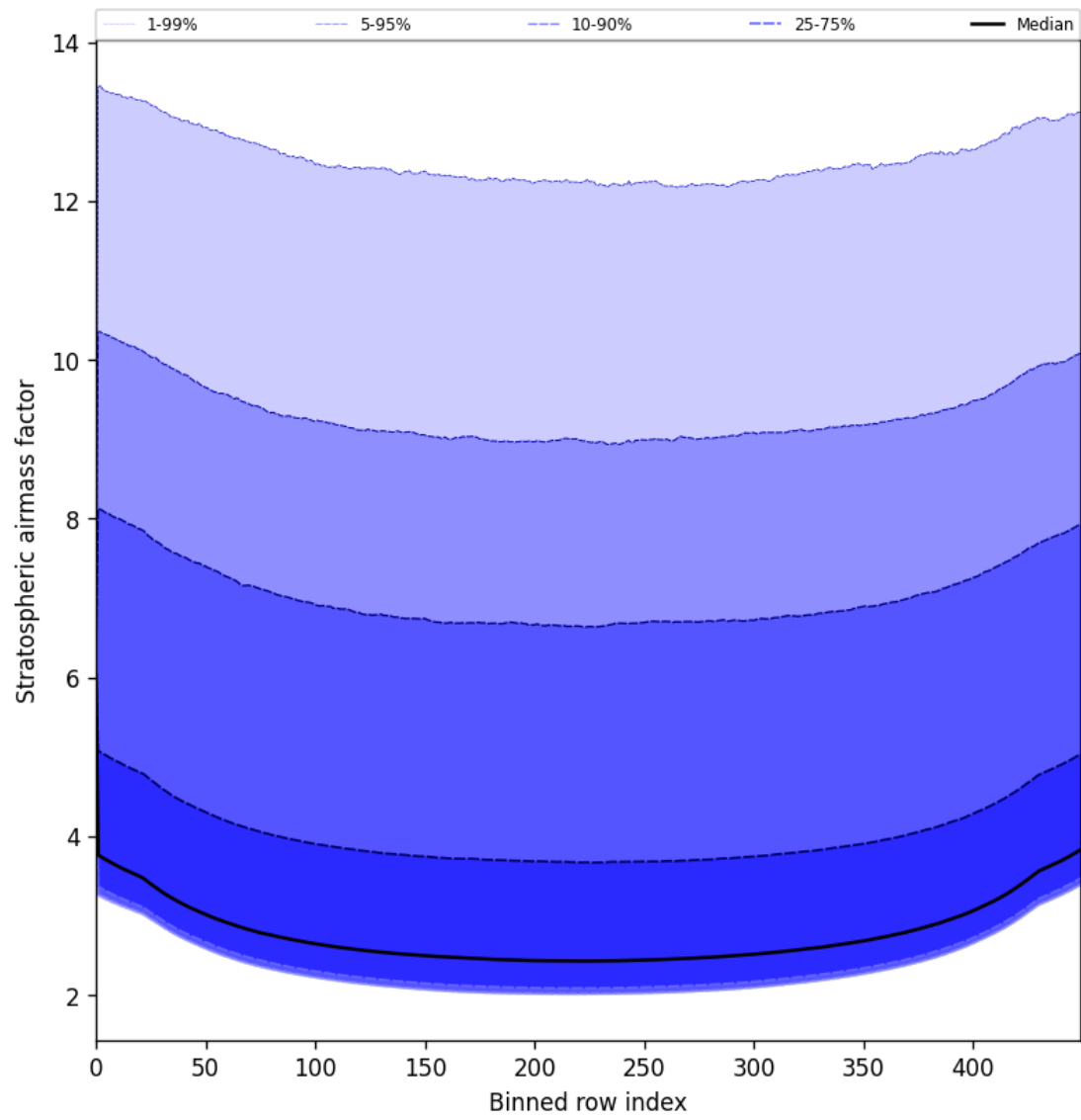
Figure 59: Along track statistics of “Stratospheric airmass factor” for 2025-06-27 to 2025-06-28
