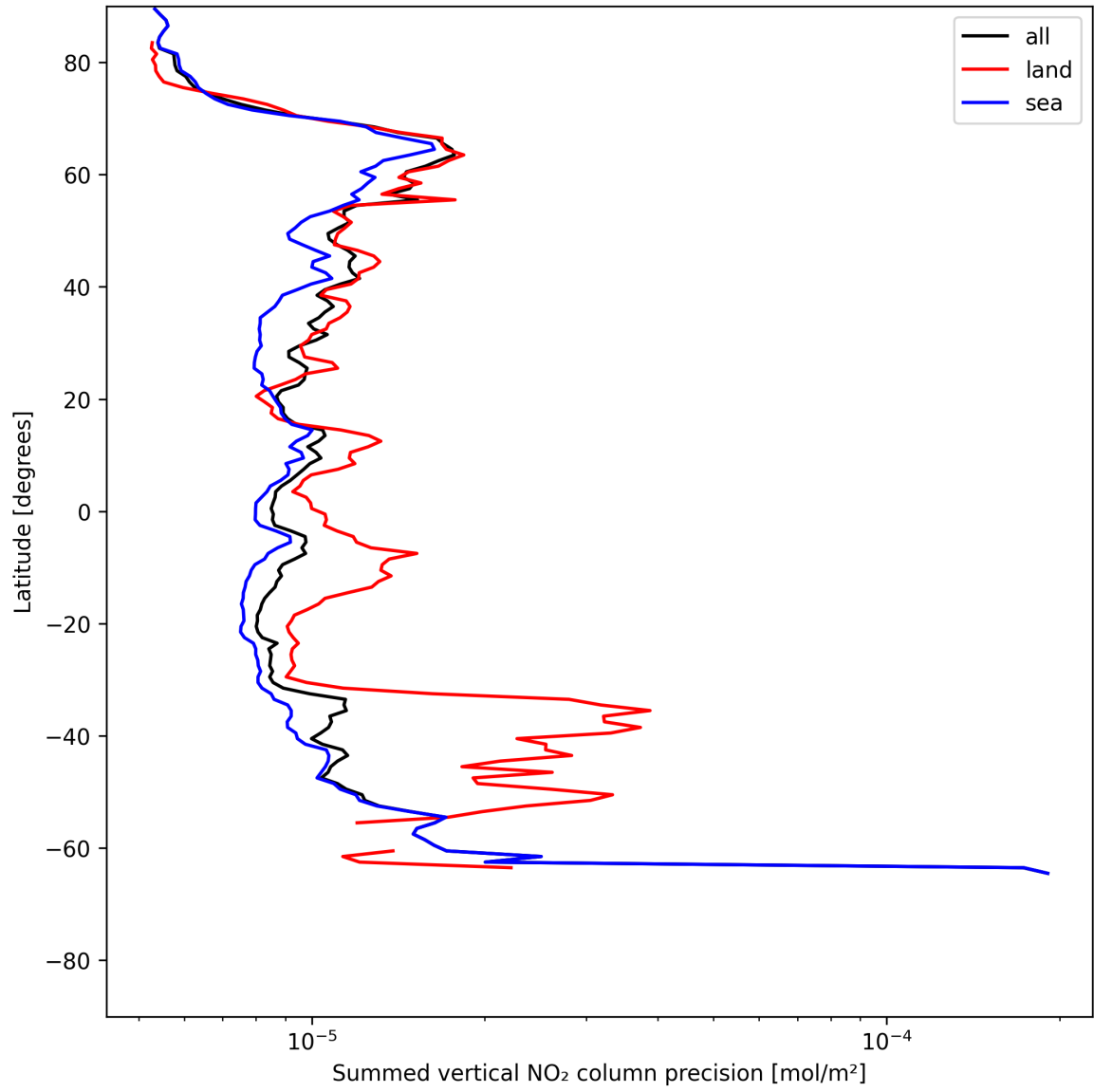
Figure 22: Zonal average of “Summed vertical NO 2 column precision” for 2025-06-27 to 2025-06-28.
