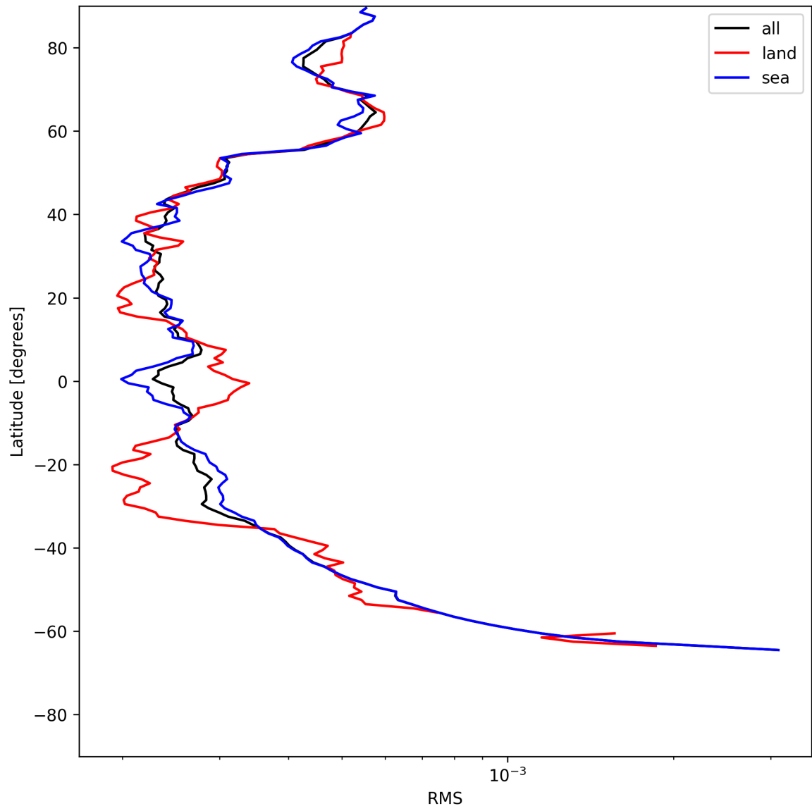
Figure 24: Zonal average of “RMS” for 2025-06-27 to 2025-06-28.
