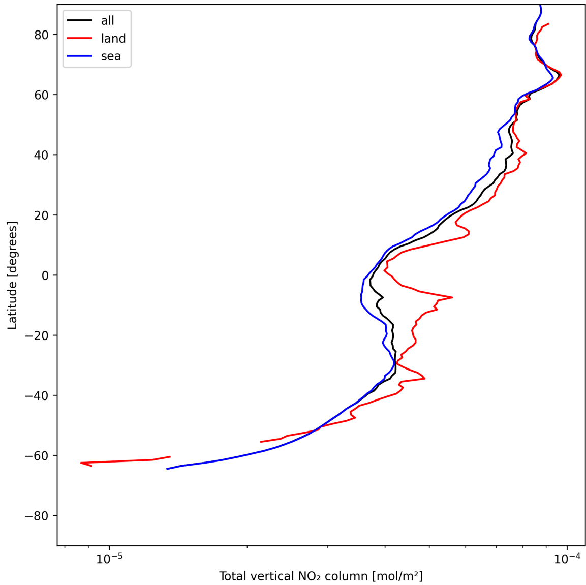
Figure 19: Zonal average of “Total vertical NO 2 column” for 2025-06-27 to 2025-06-28.
