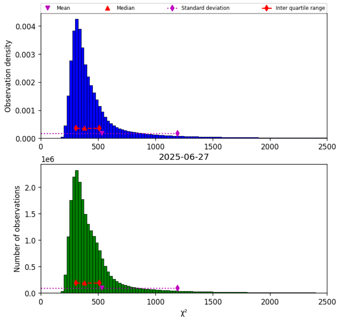
Figure 40: Histogram of “ \chi^2 ” for 2025-06-27 to 2025-06-28
