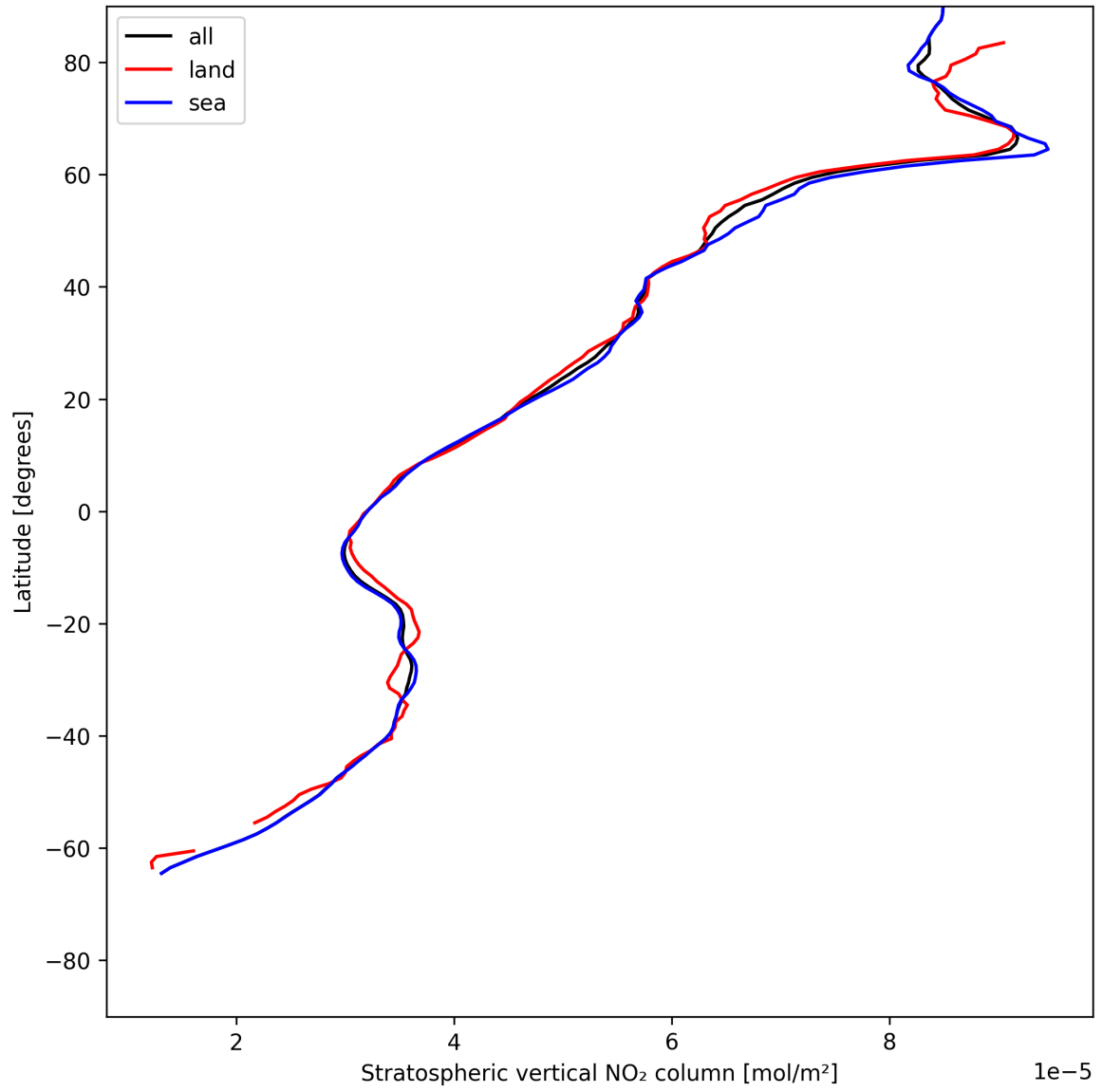
Figure 17: Zonal average of “Stratospheric vertical NO 2 column” for 2025-06-27 to 2025-06-28.
