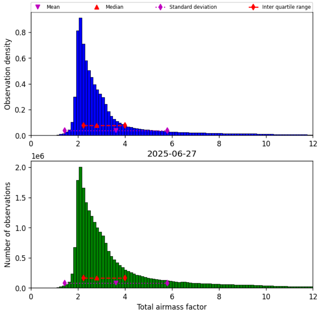
Figure 30: Histogram of “Total airmass factor” for 2025-06-27 to 2025-06-28
