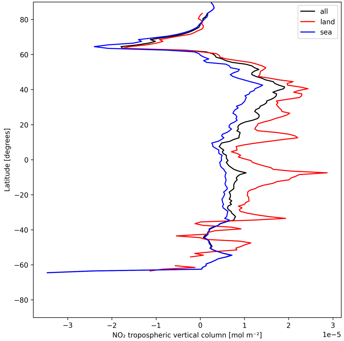
Figure 10: Zonal average of “NO 2 tropospheric vertical column” for 2025-06-27 to 2025-06-28.
