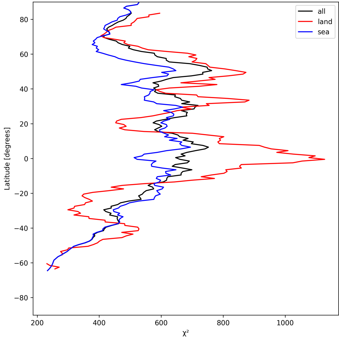
Figure 23: Zonal average of “ \chi^2 ” for 2025-06-27 to 2025-06-28.
