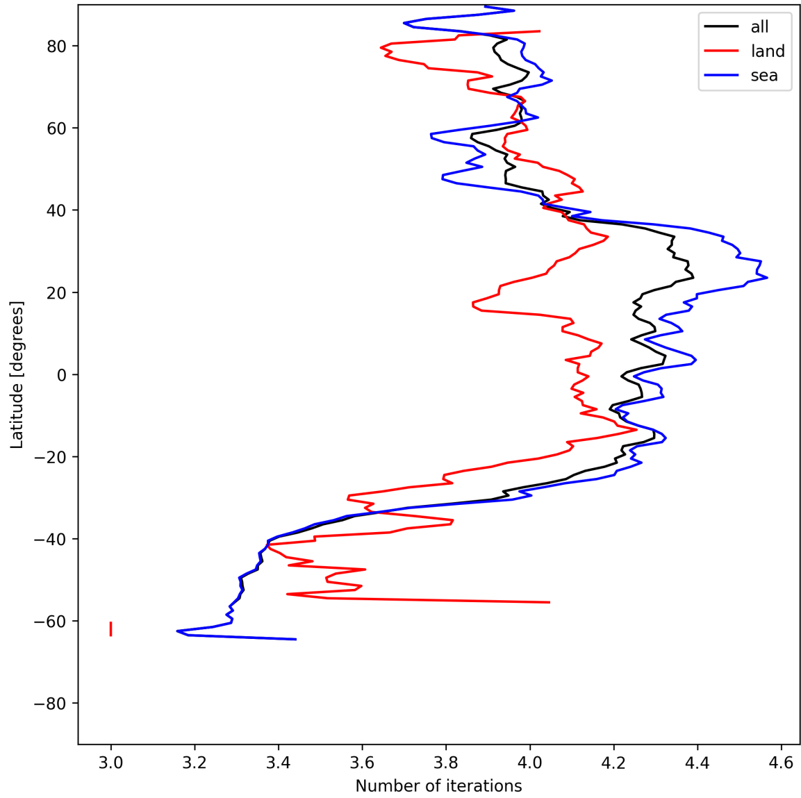
Figure 15: Zonal average of “Number of iterations” for 2025-06-27 to 2025-06-28.
