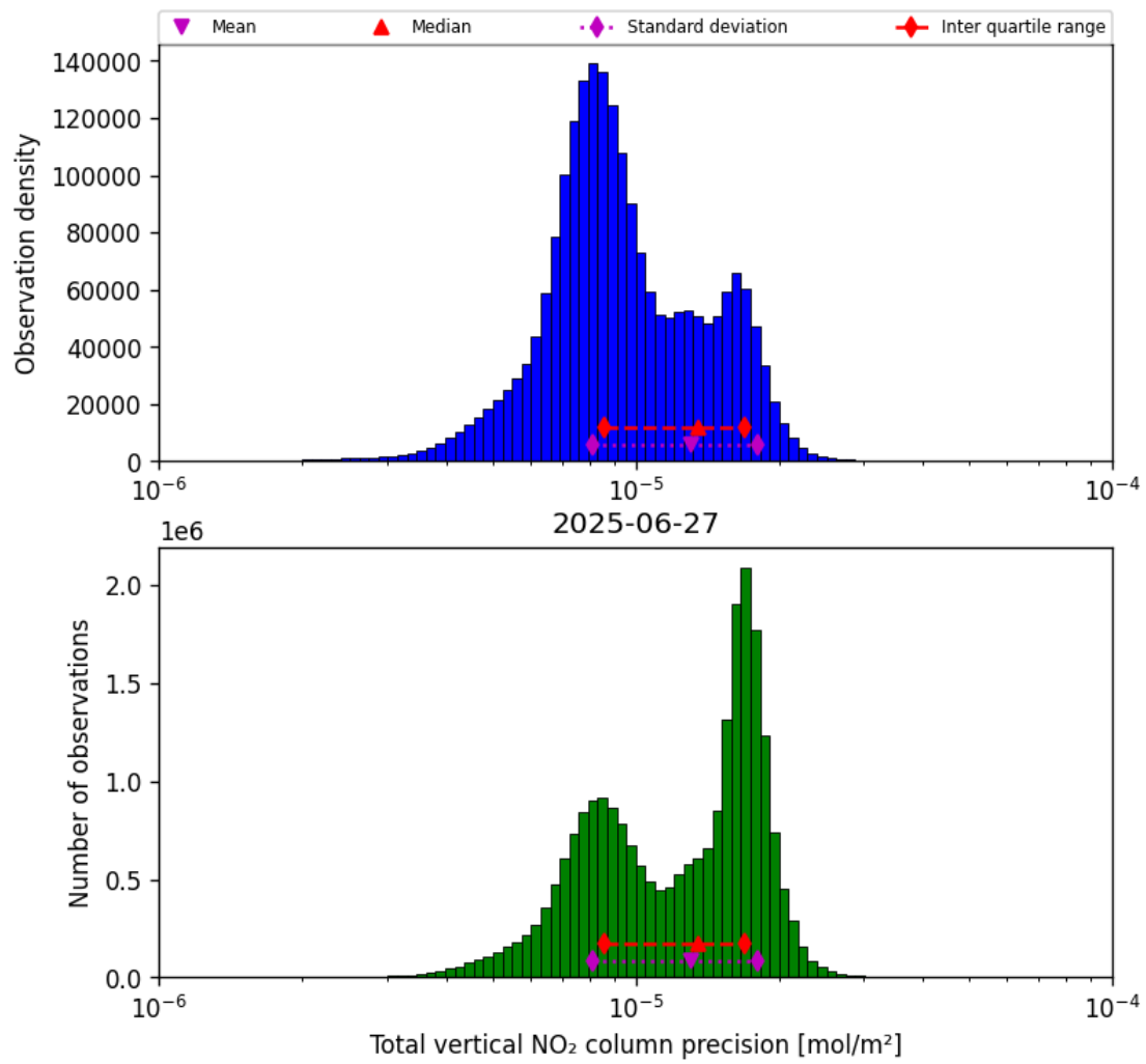
Figure 37: Histogram of “Total vertical NO 2 column precision” for 2025-06-27 to 2025-06-28
