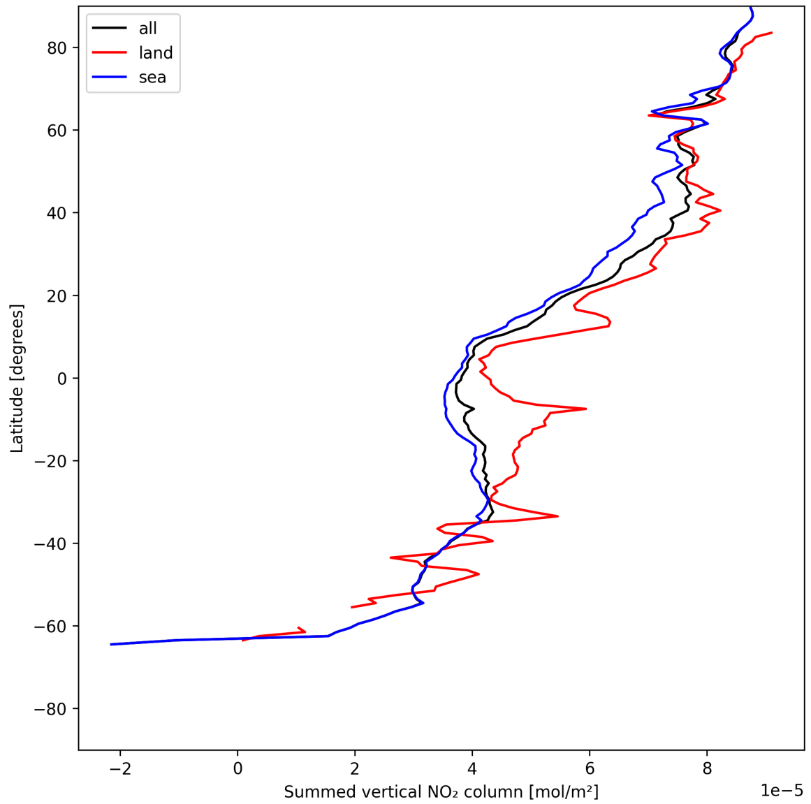
Figure 21: Zonal average of “Summed vertical NO 2 column” for 2025-06-27 to 2025-06-28.
