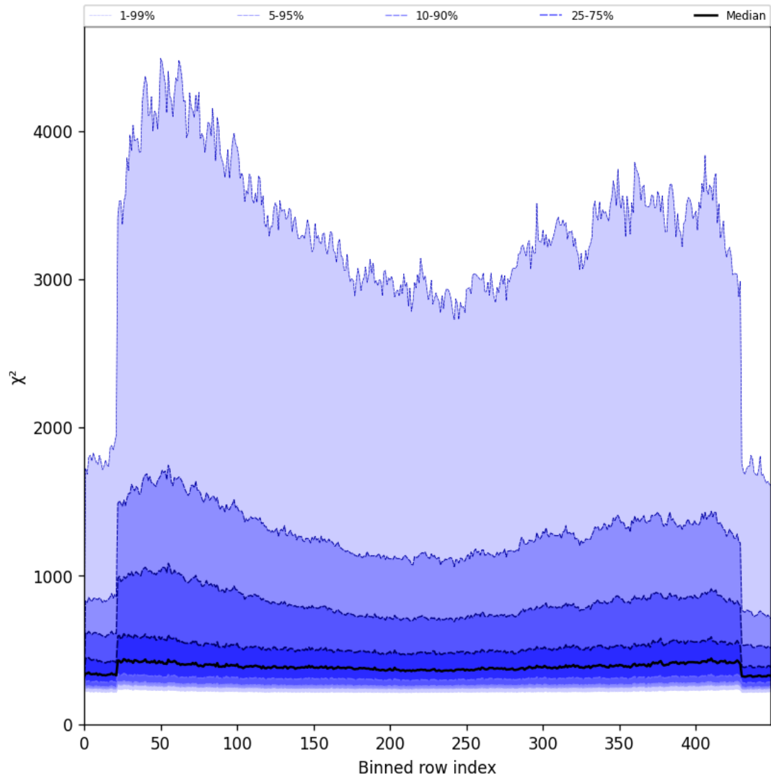
Figure 57: Along track statistics of “ \chi^2 ” for 2025-06-27 to 2025-06-28
