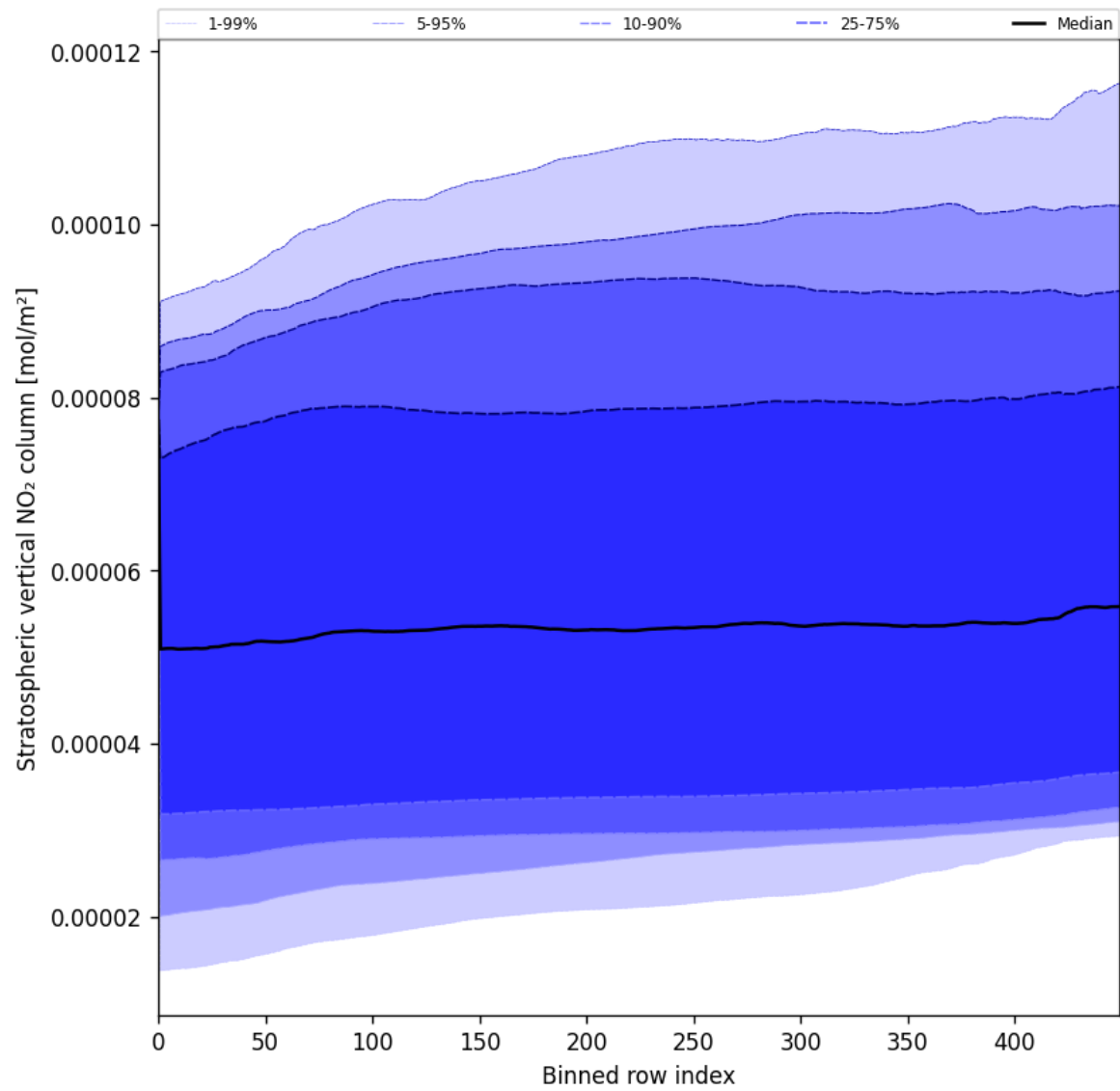
Figure 51: Along track statistics of “Stratospheric vertical NO 2 column” for 2025-06-28 to 2025-06-29
