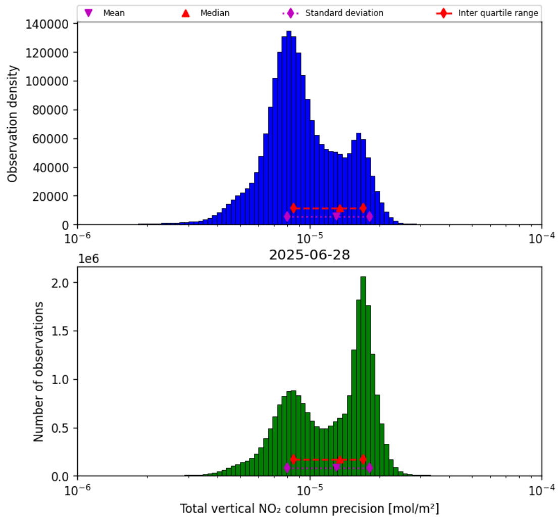
Figure 37: Histogram of “Total vertical NO 2 column precision” for 2025-06-28 to 2025-06-29
