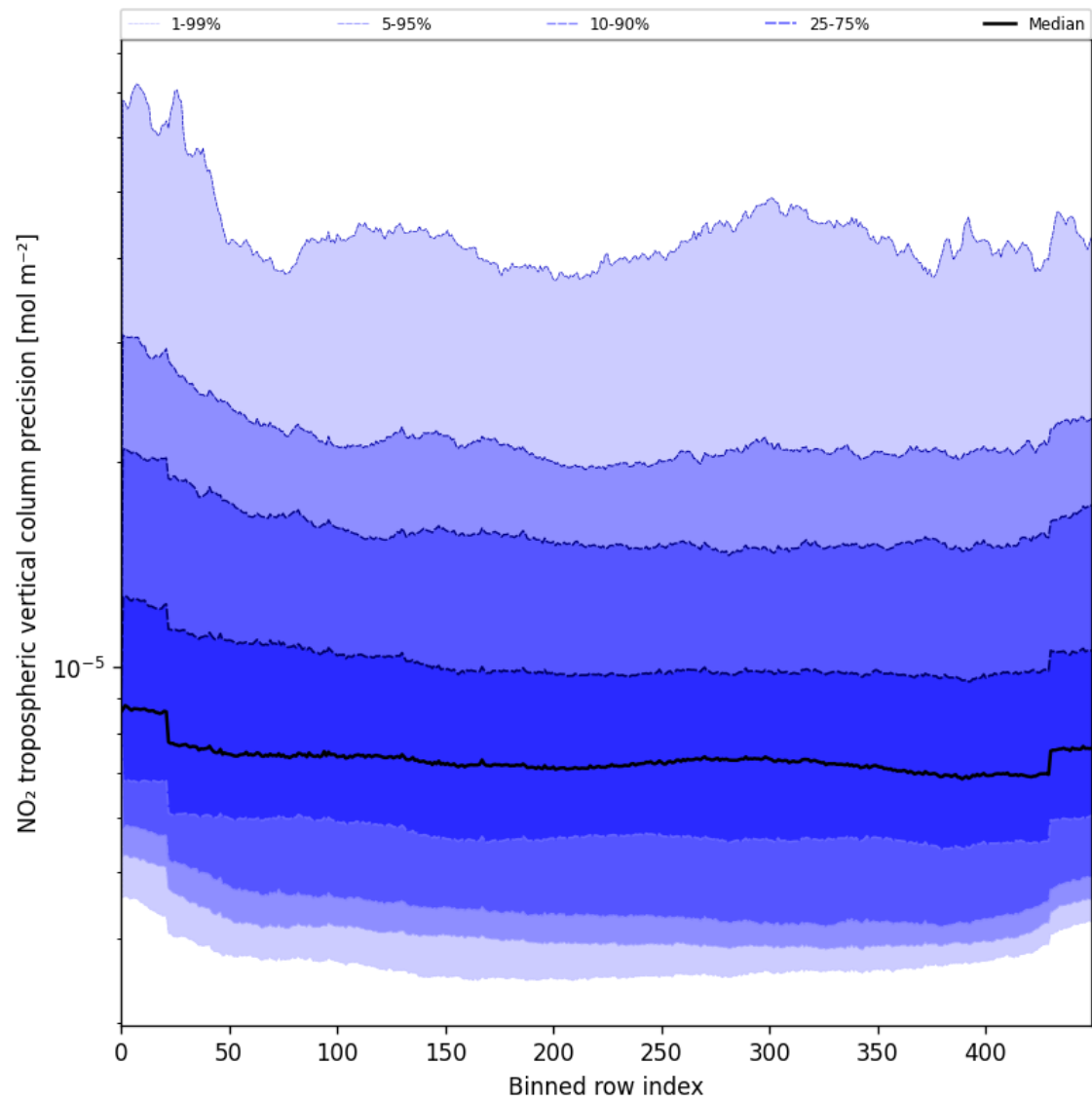
Figure 45: Along track statistics of “NO 2 tropospheric vertical column precision” for 2025-06-28 to 2025-06-29
