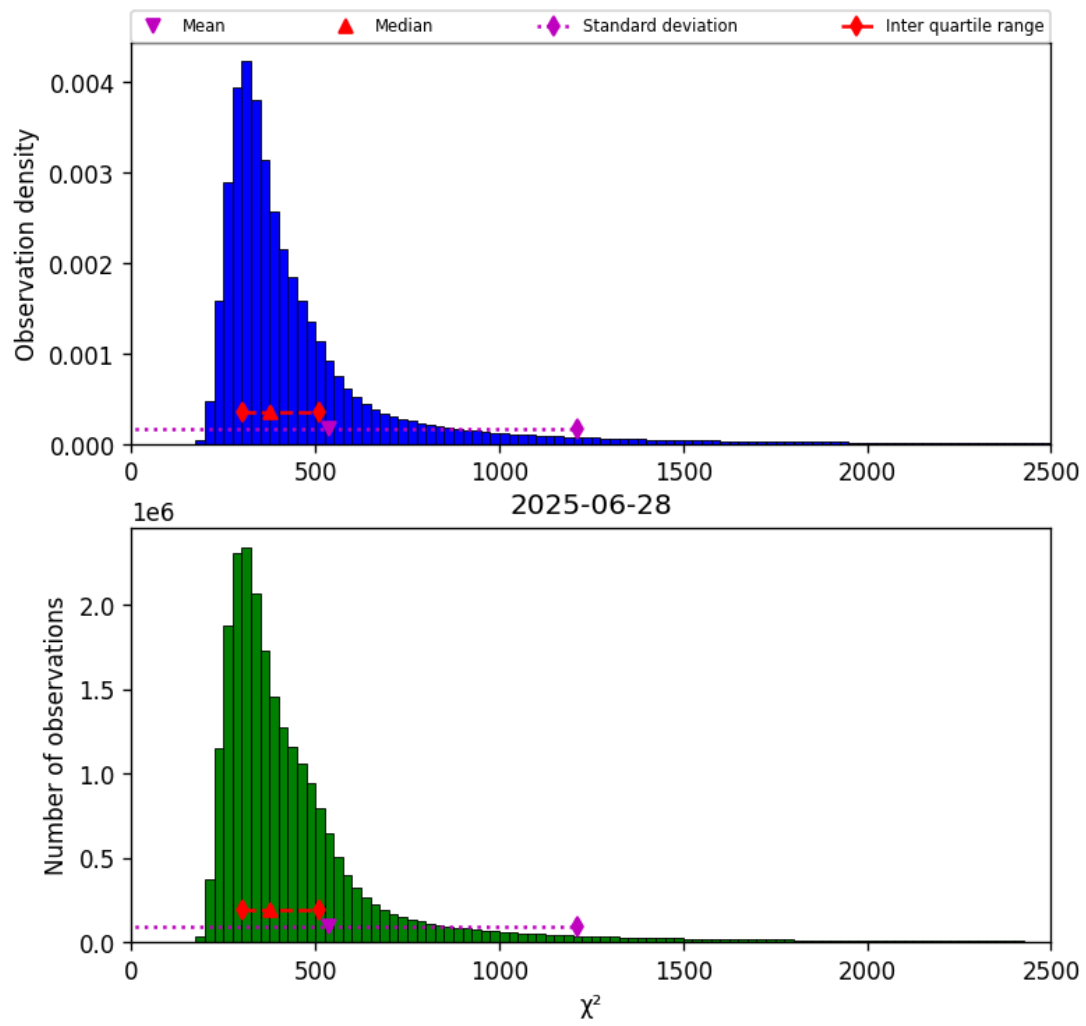
Figure 40: Histogram of “ \chi^2 ” for 2025-06-28 to 2025-06-29
