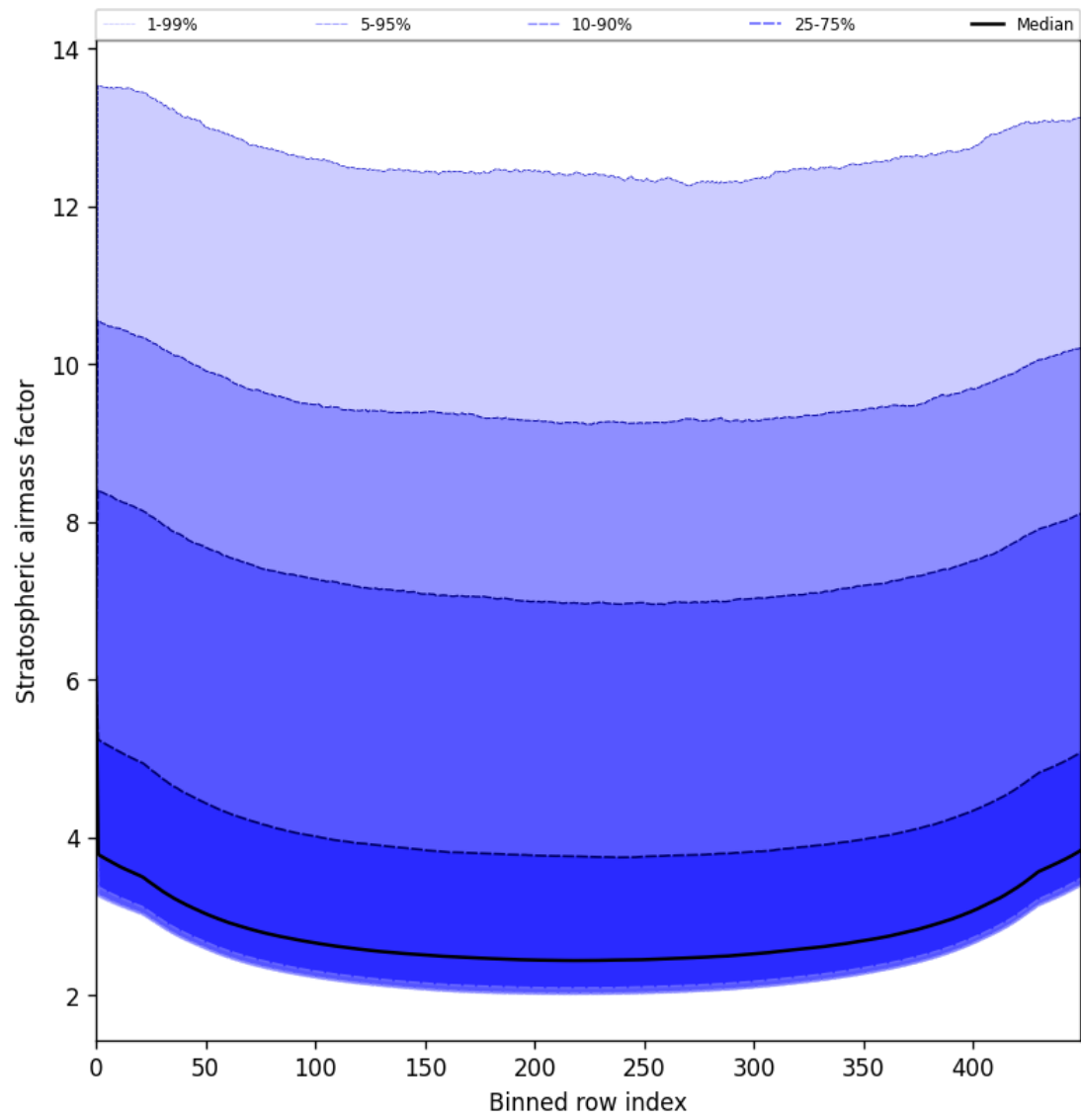
Figure 59: Along track statistics of “Stratospheric airmass factor” for 2025-06-28 to 2025-06-29
