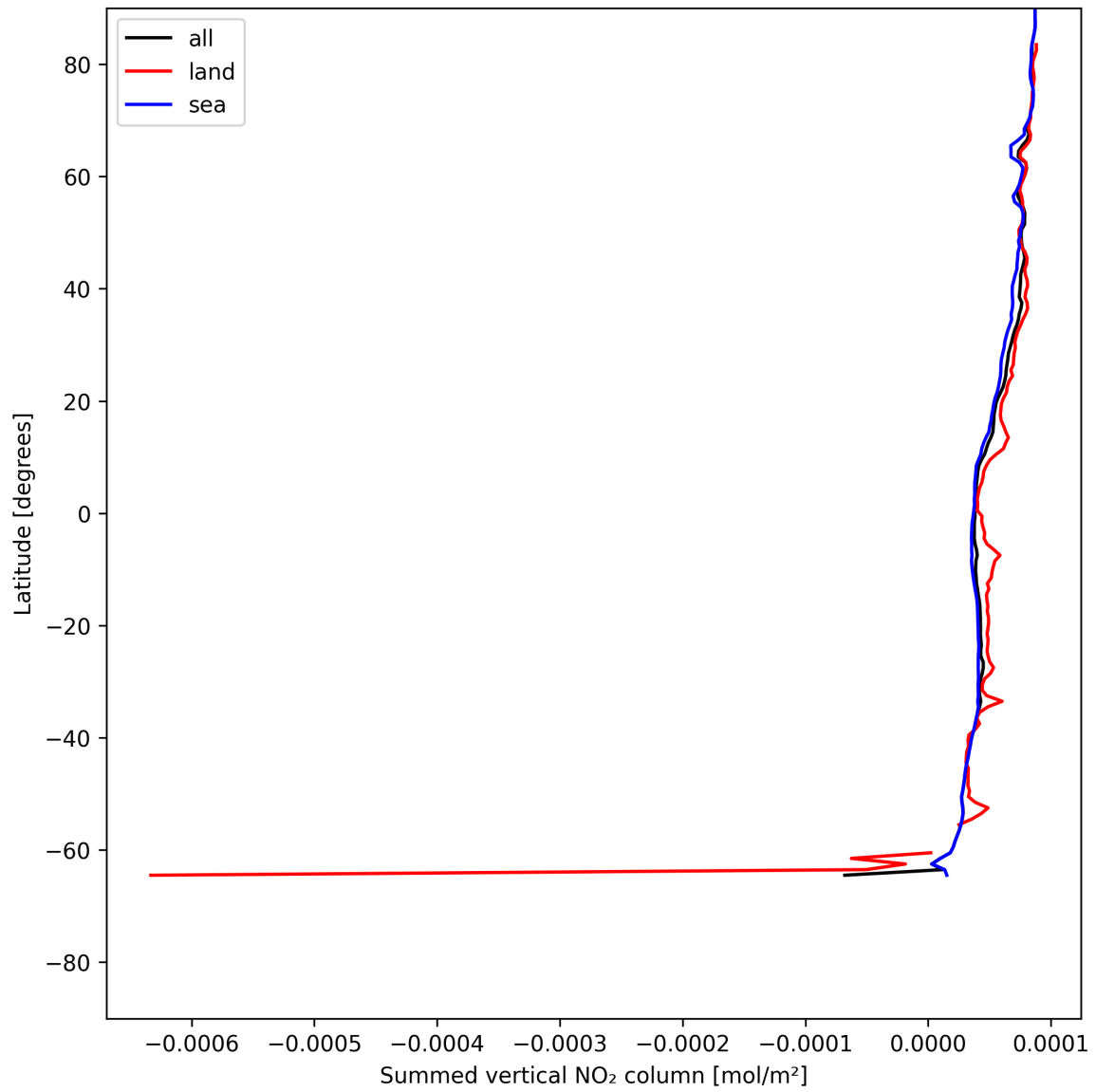
Figure 21: Zonal average of “Summed vertical NO 2 column” for 2025-06-28 to 2025-06-29.
