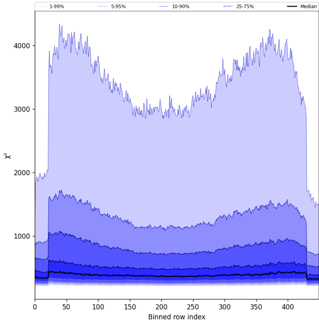
Figure 57: Along track statistics of “ \chi^2 ” for 2025-06-28 to 2025-06-29
