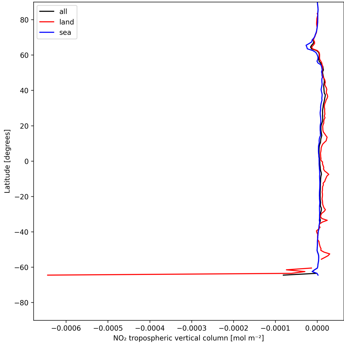
Figure 10: Zonal average of “NO 2 tropospheric vertical column” for 2025-06-28 to 2025-06-29.
