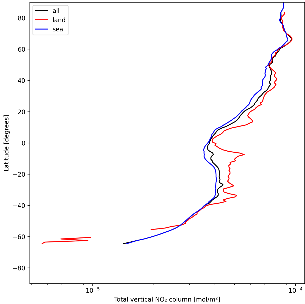
Figure 19: Zonal average of “Total vertical NO 2 column” for 2025-06-28 to 2025-06-29.
