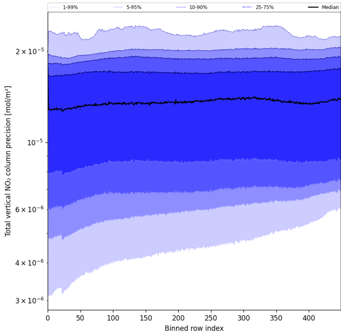
Figure 54: Along track statistics of "Total vertical NO 2 column precision" for 2025-06-28 to 2025-06-29
