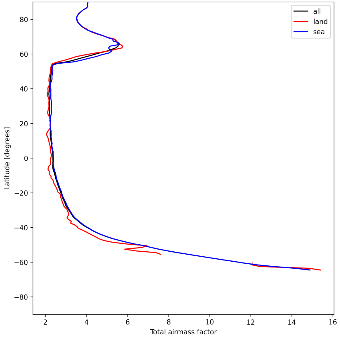
Figure 13: Zonal average of “Total airmass factor” for 2025-06-28 to 2025-06-29.
