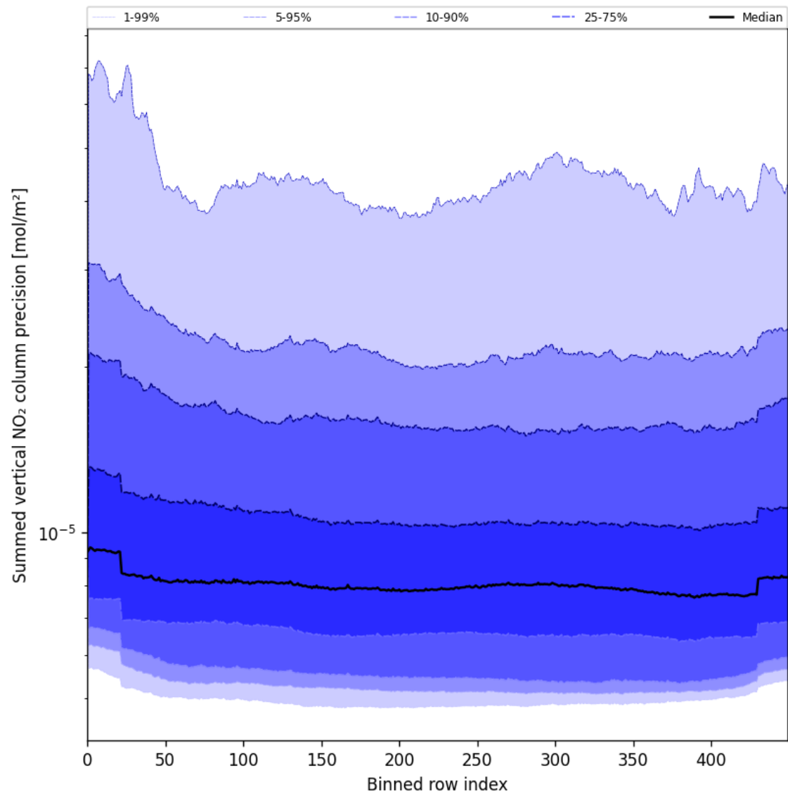
Figure 56: Along track statistics of “Summed vertical NO 2 column precision” for 2025-06-28 to 2025-06-29
