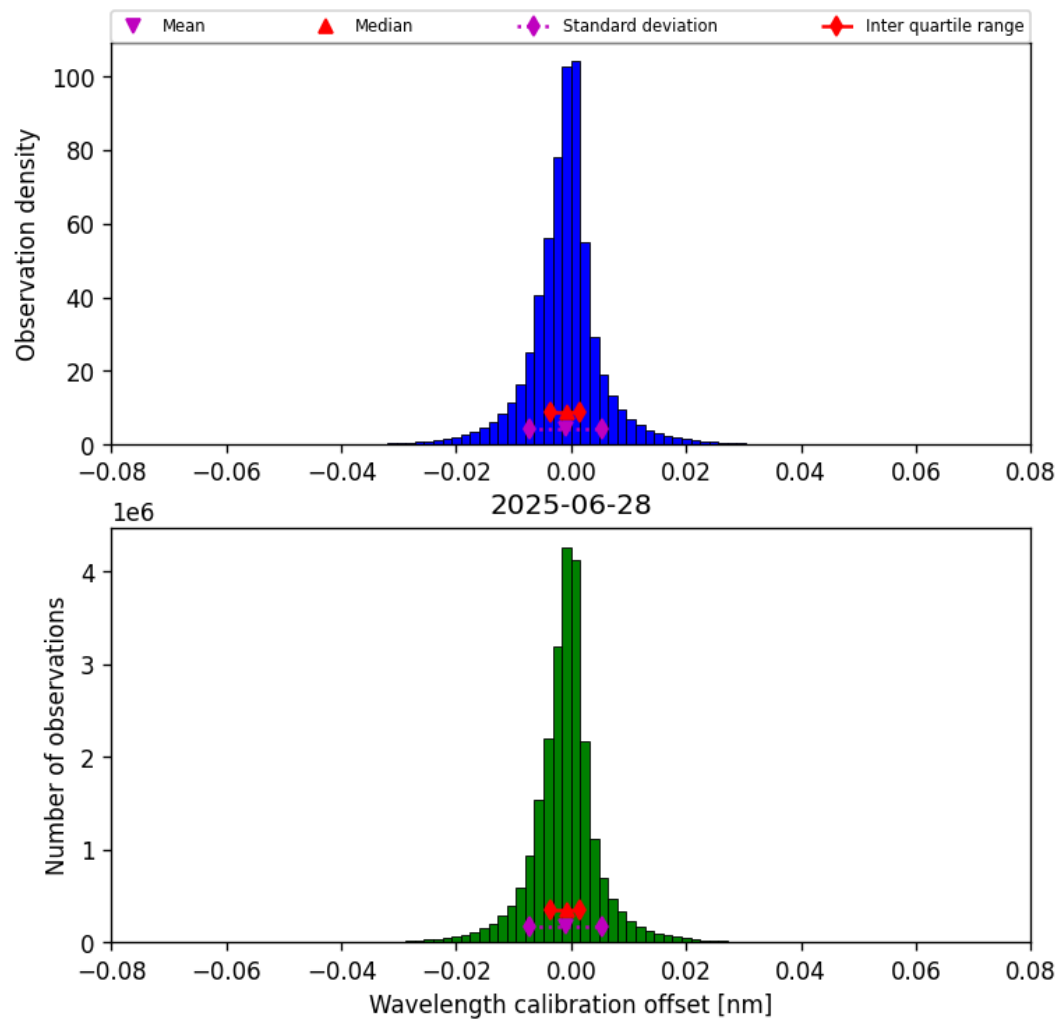
Figure 33: Histogram of “Wavelength calibration offset” for 2025-06-28 to 2025-06-29
