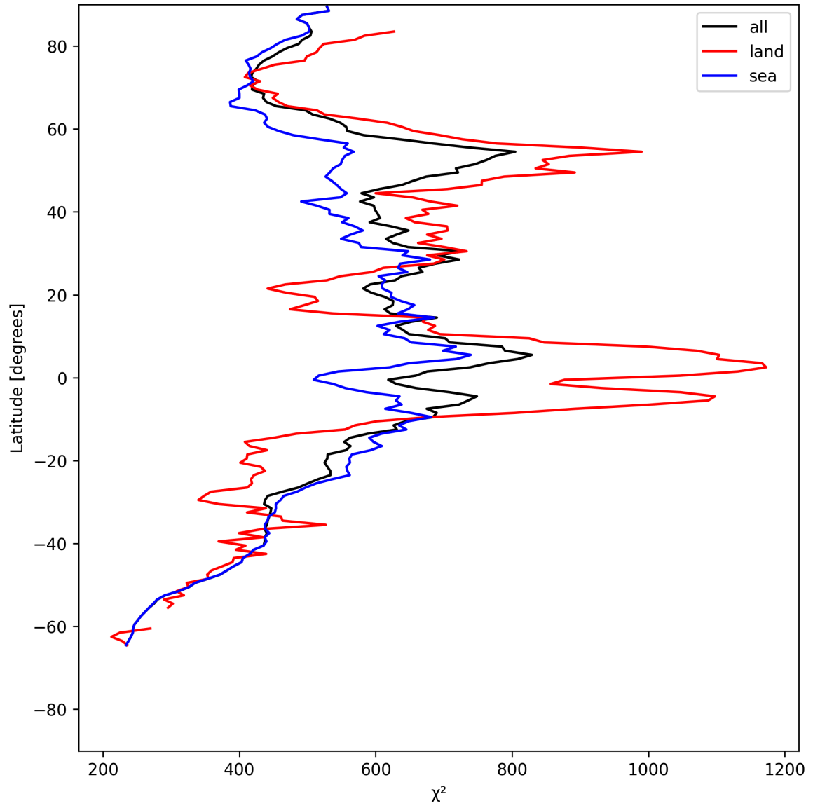
Figure 23: Zonal average of “ \chi^2 ” for 2025-06-28 to 2025-06-29.
