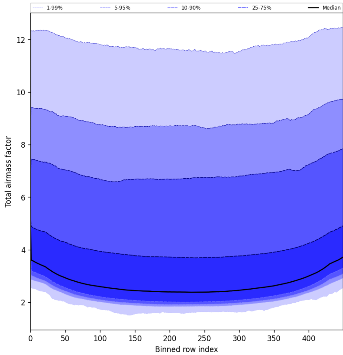
Figure 47: Along track statistics of “Total airmass factor” for 2025-06-28 to 2025-06-29
