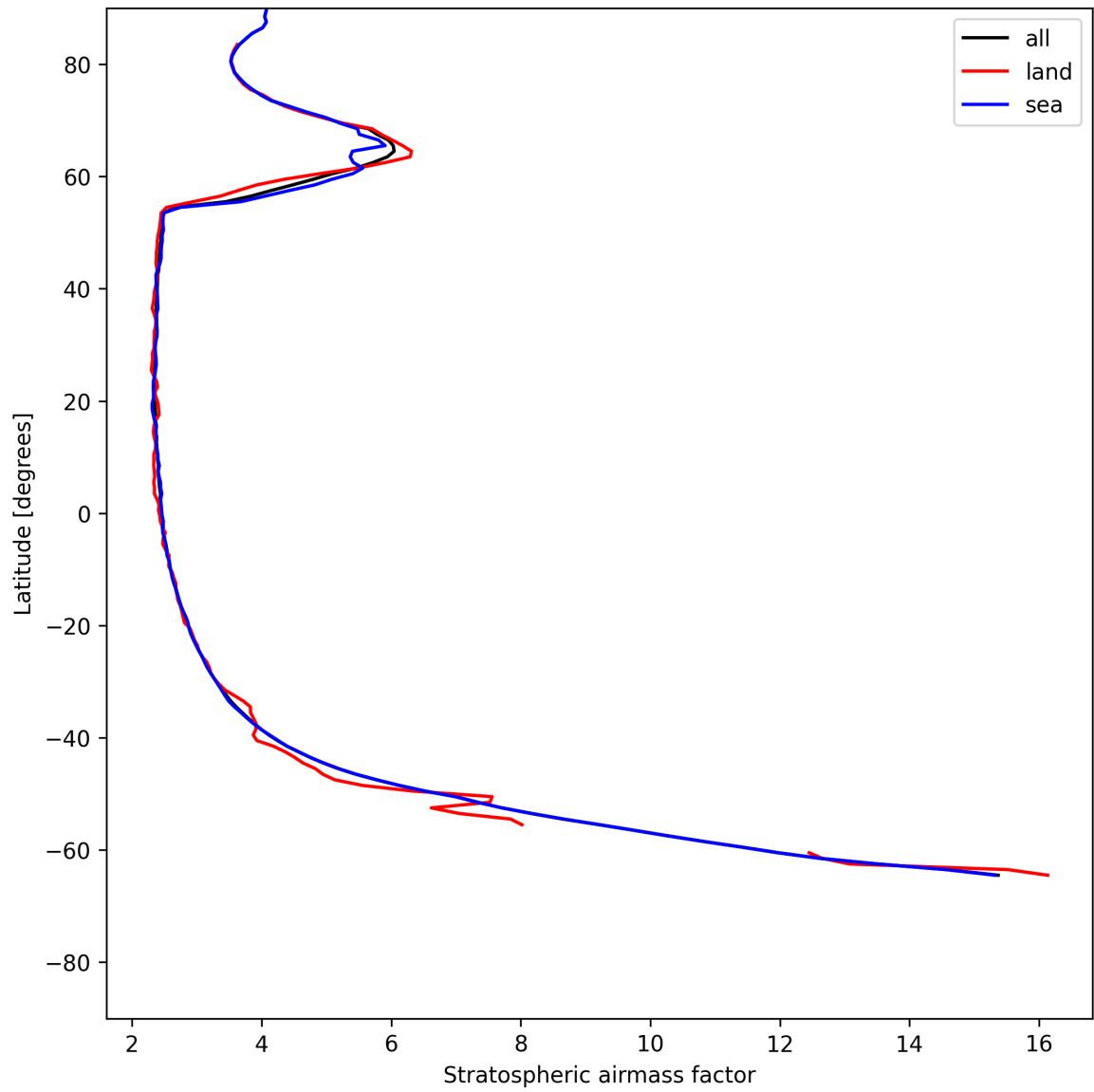
Figure 25: Zonal average of “Stratospheric air mass factor” for 2025-06-28 to 2025-06-29.
