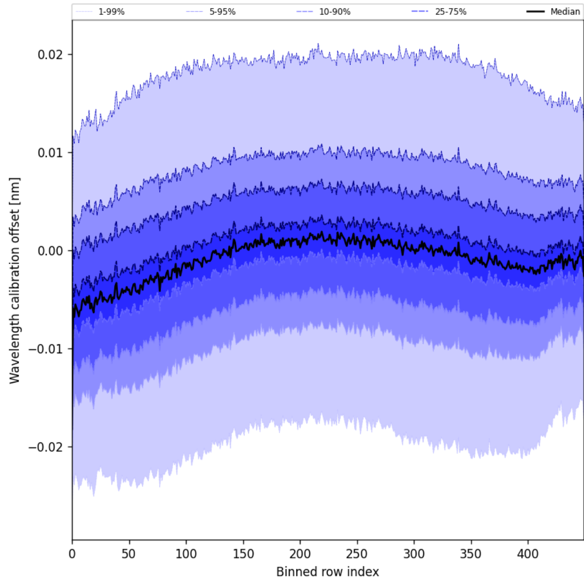
Figure 50: Along track statistics of “Wavelength calibration offset” for 2025-06-28 to 2025-06-29
