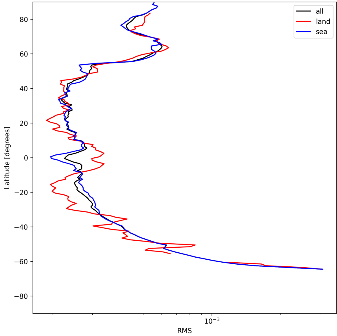
Figure 24: Zonal average of “RMS” for 2025-06-28 to 2025-06-29.
