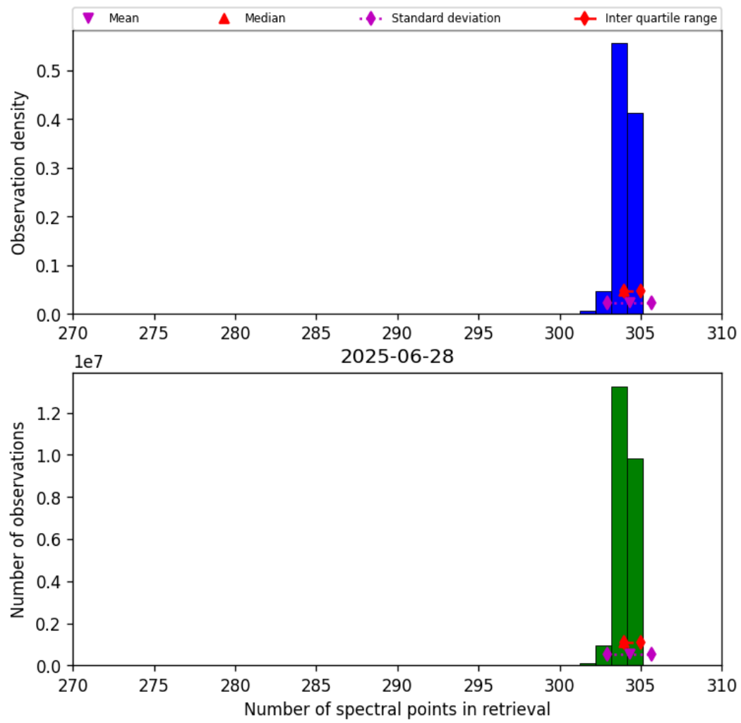
Figure 31: Histogram of “Number of spectral points in retrieval” for 2025-06-28 to 2025-06-29
