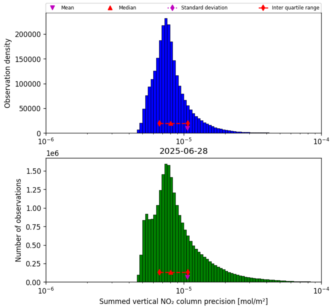
Figure 39: Histogram of “Summed vertical NO 2 column precision” for 2025-06-28 to 2025-06-29
