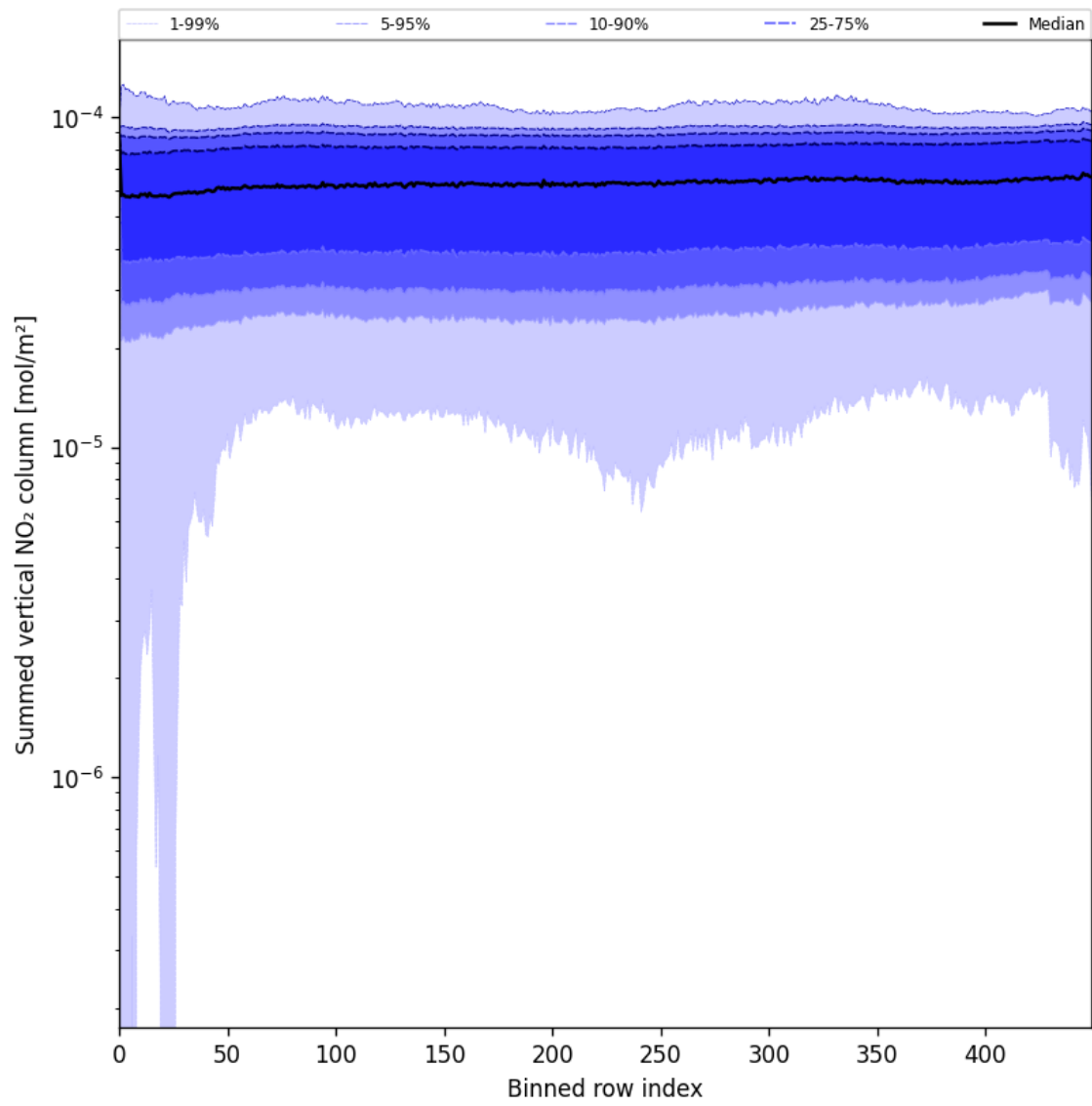
Figure 55: Along track statistics of “Summed vertical NO 2 column” for 2025-06-28 to 2025-06-29
