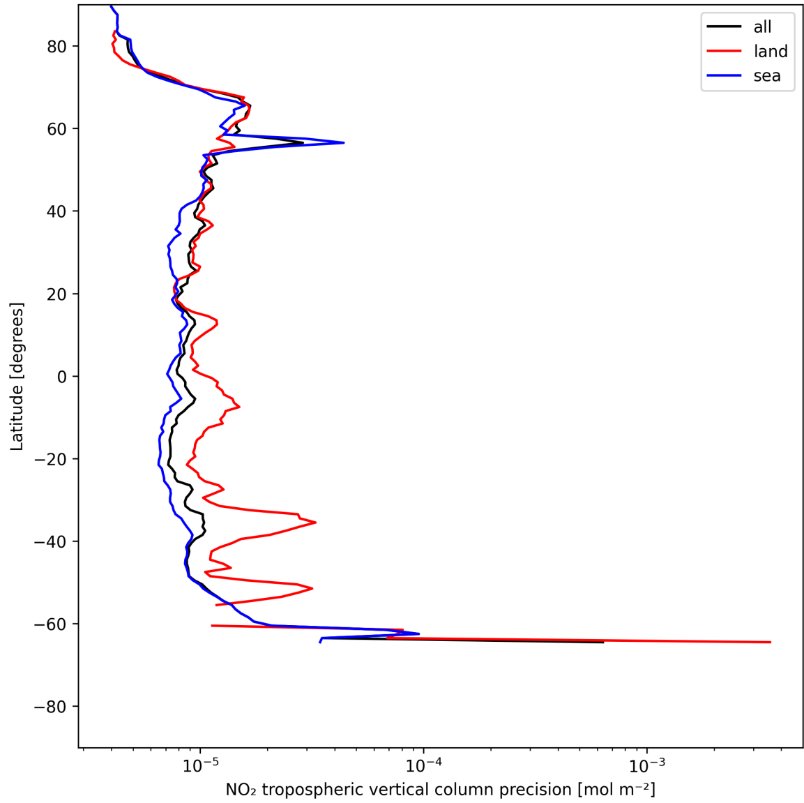
Figure 11: Zonal average of “NO 2 tropospheric vertical column precision” for 2025-06-28 to 2025-06-29.
