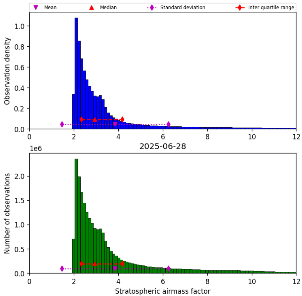
Figure 42: Histogram of “Stratospheric airmass factor” for 2025-06-28 to 2025-06-29
