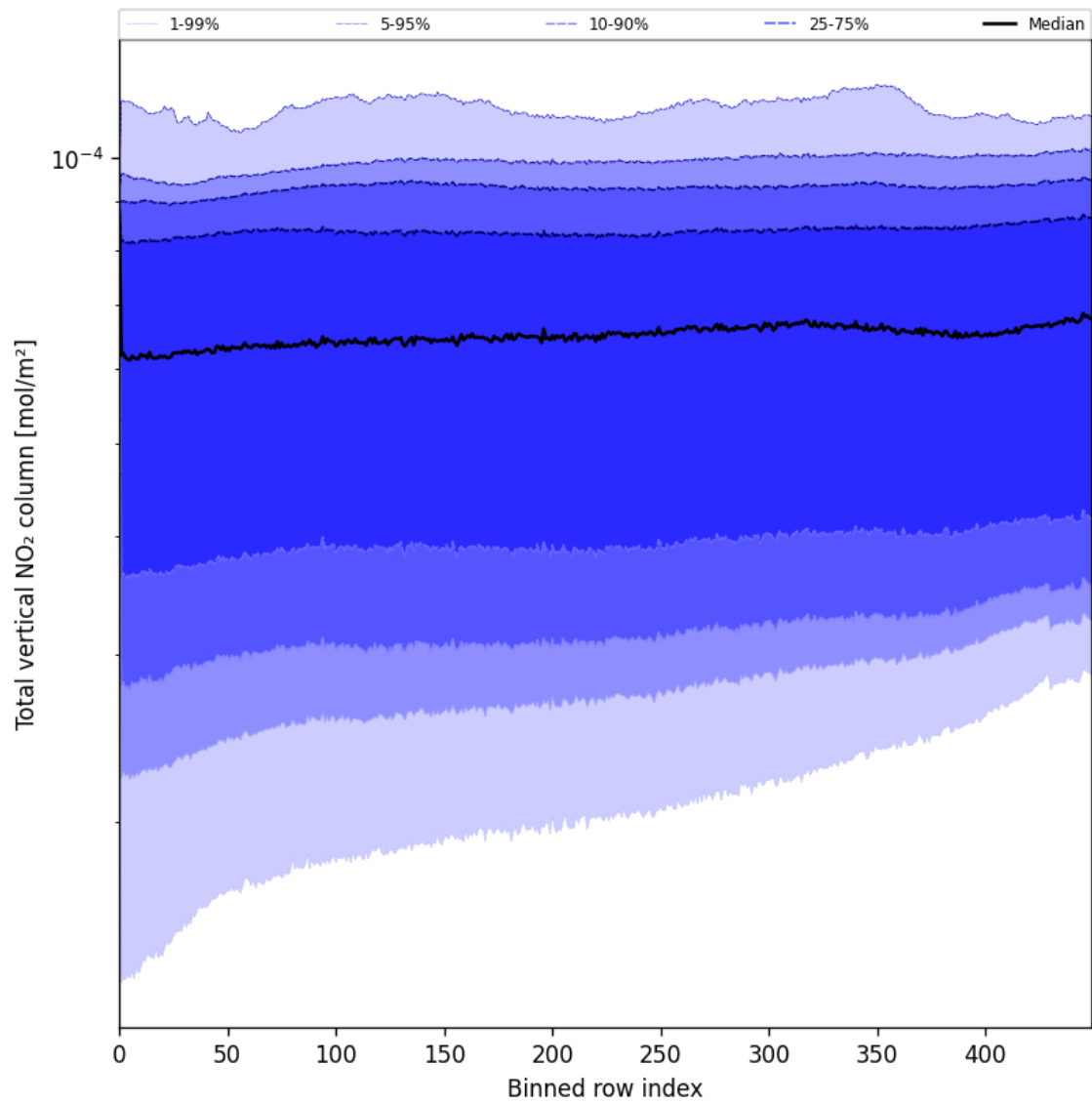
Figure 53: Along track statistics of “Total vertical NO 2 column” for 2025-06-28 to 2025-06-29
