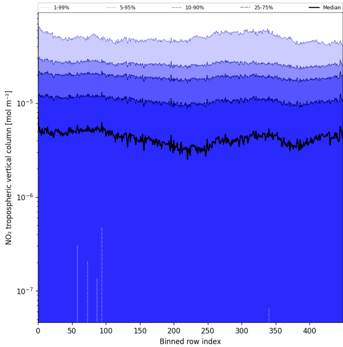
Figure 44: Along track statistics of “NO 2 tropospheric vertical column” for 2025-06-28 to 2025-06-29
