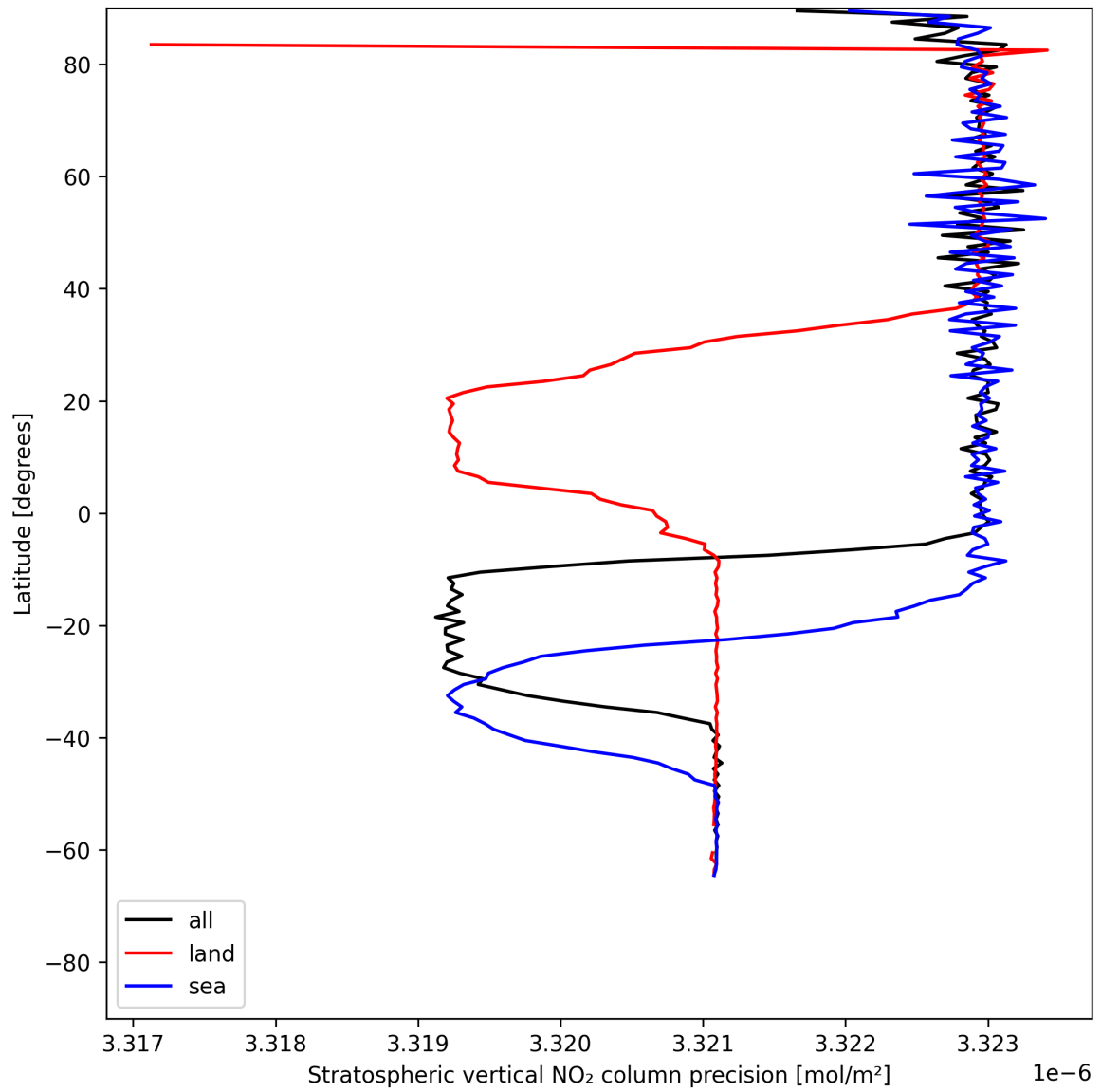
Figure 18: Zonal average of “Stratospheric vertical NO 2 column precision” for 2025-06-28 to 2025-06-29.
