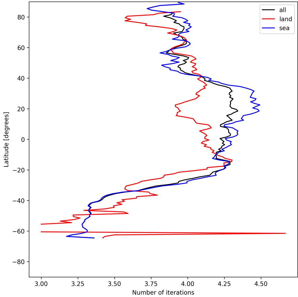
Figure 15: Zonal average of “Number of iterations” for 2025-06-28 to 2025-06-29.
