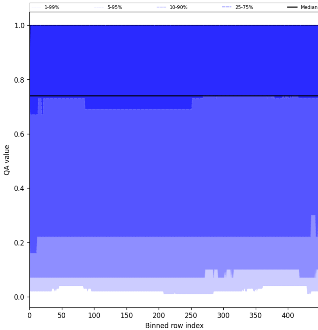
Figure 43: Along track statistics of "QA value" for 2025-06-28 to 2025-06-29
