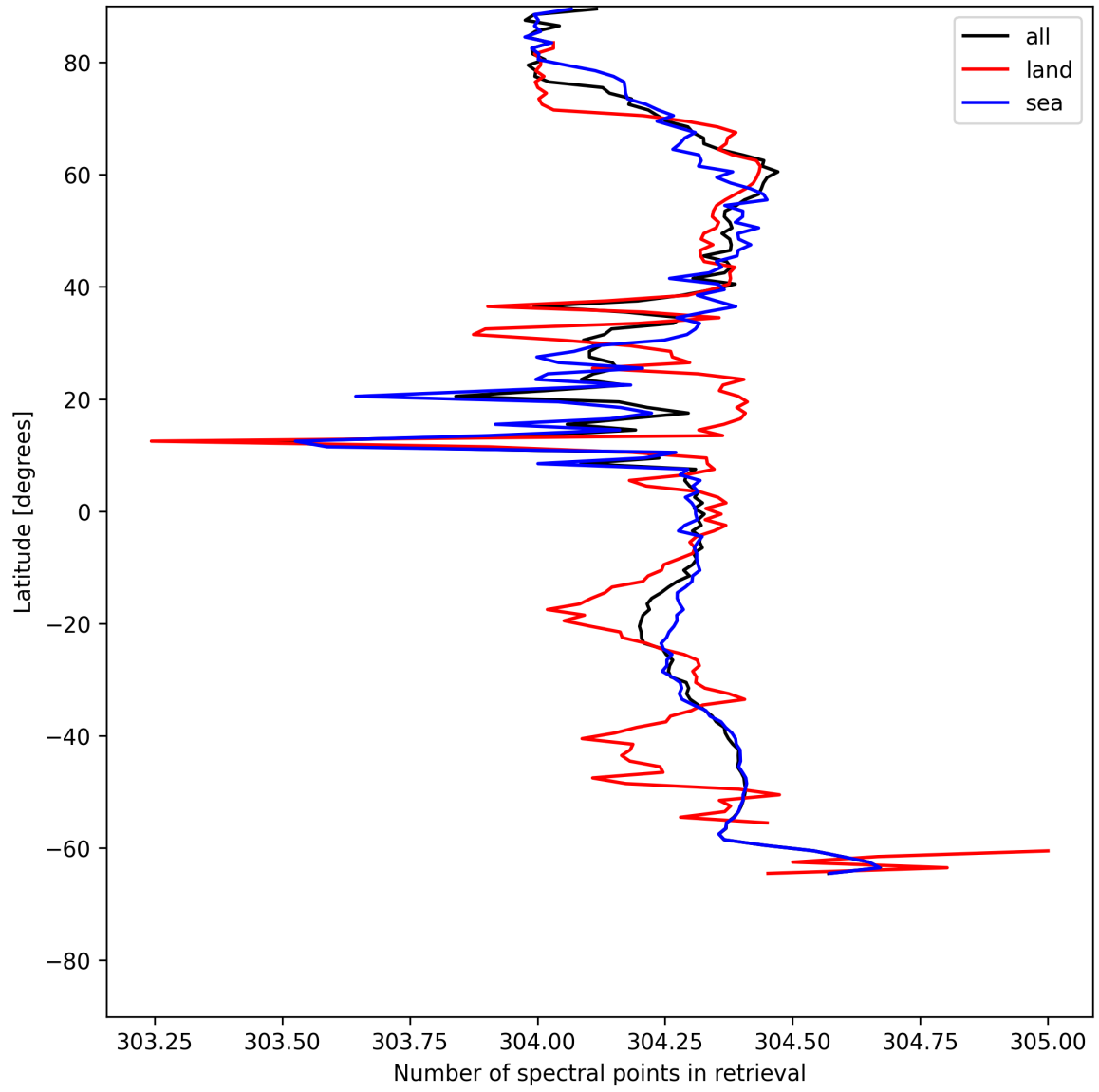
Figure 14: Zonal average of “Number of spectral points in retrieval” for 2025-06-28 to 2025-06-29.
