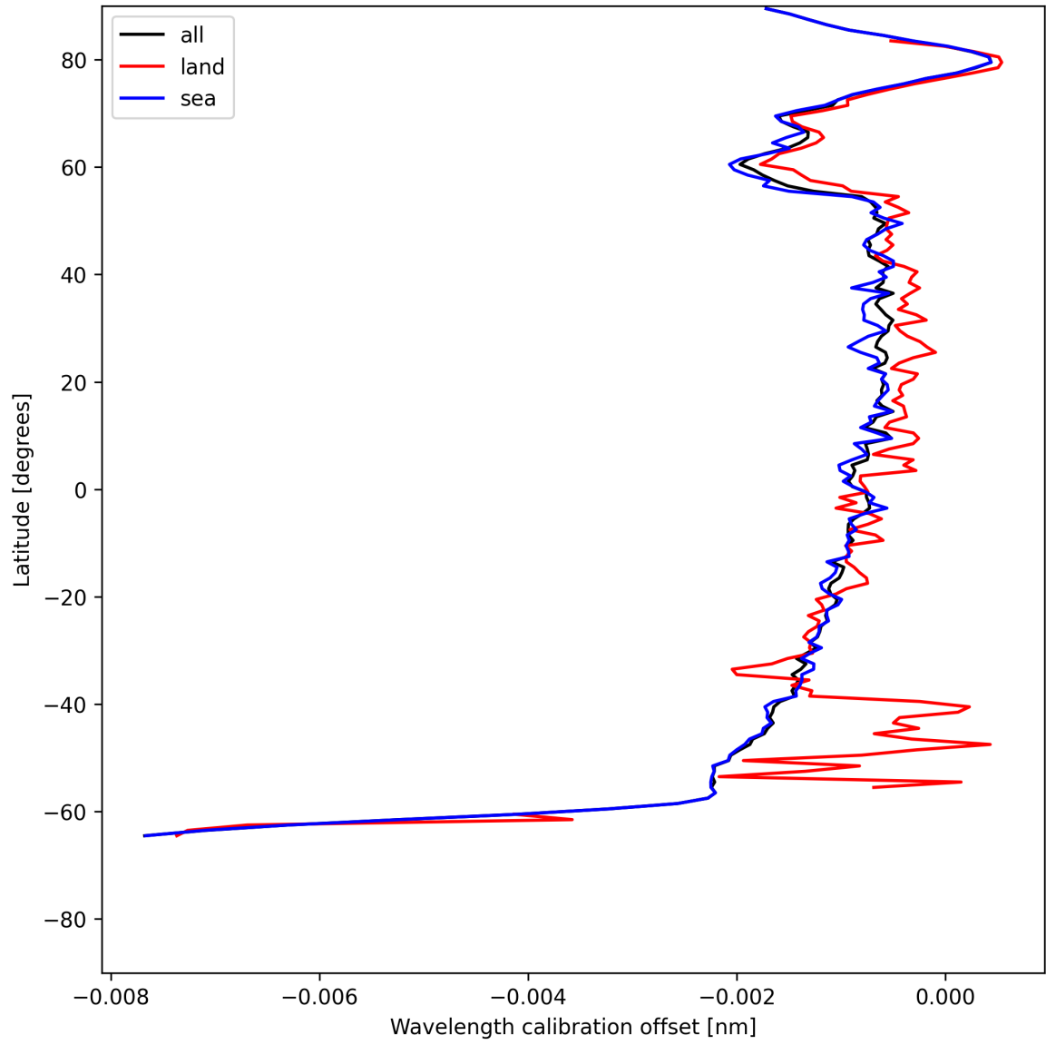
Figure 16: Zonal average of “Wavelength calibration offset” for 2025-06-28 to 2025-06-29.
