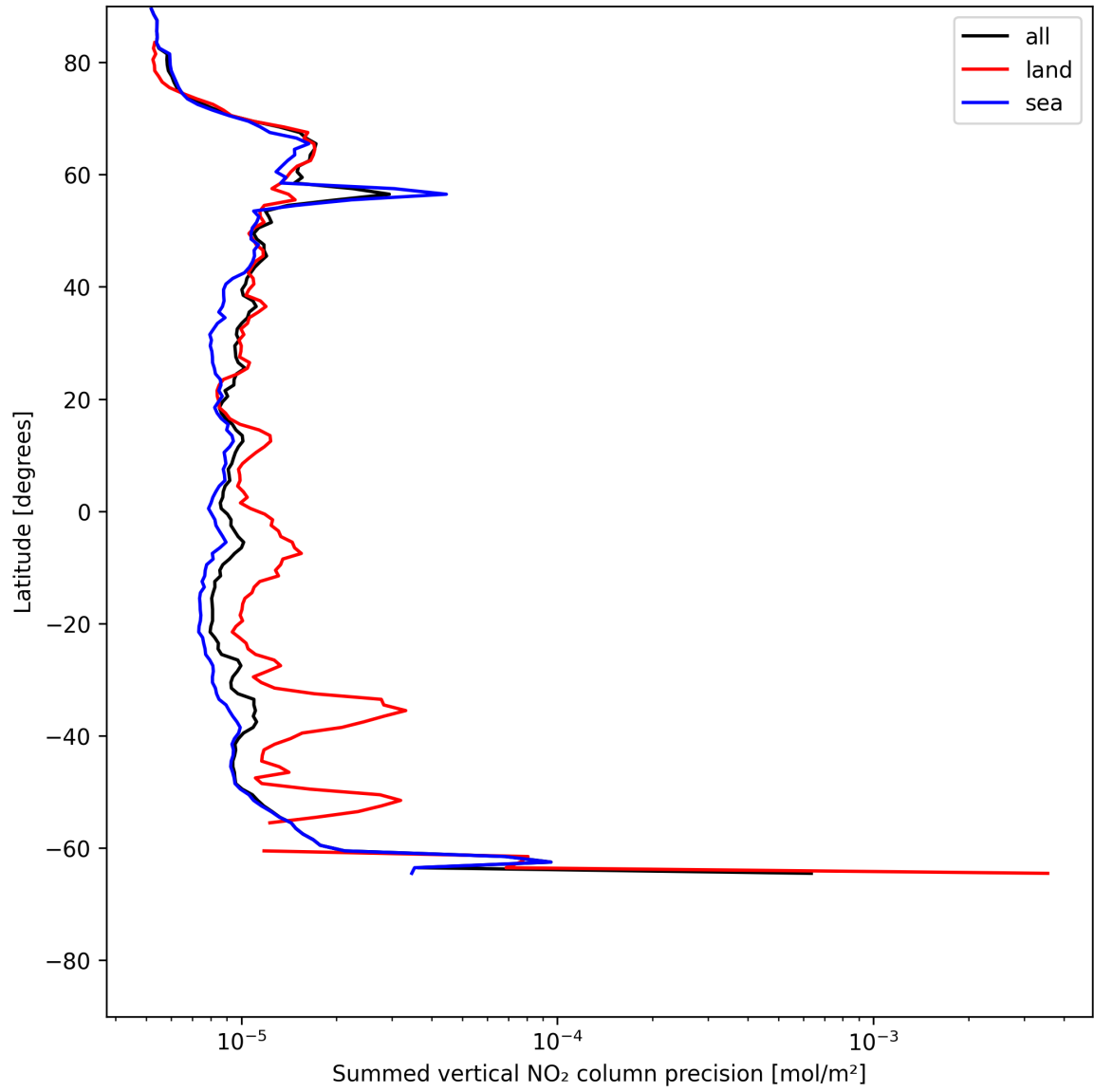
Figure 22: Zonal average of “Summed vertical NO 2 column precision” for 2025-06-28 to 2025-06-29.
