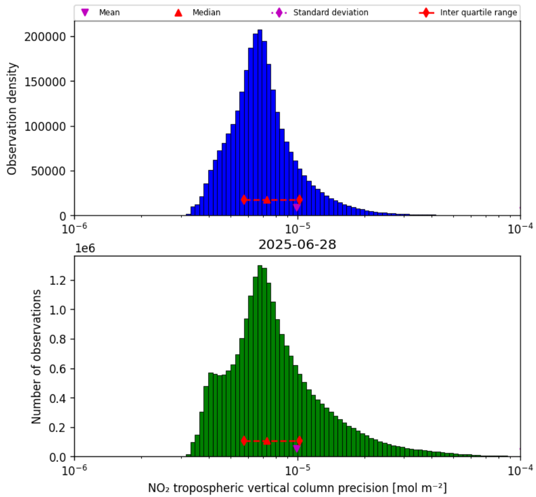
Figure 28: Histogram of “NO 2 tropospheric vertical column precision” for 2025-06-28 to 2025-06-29
