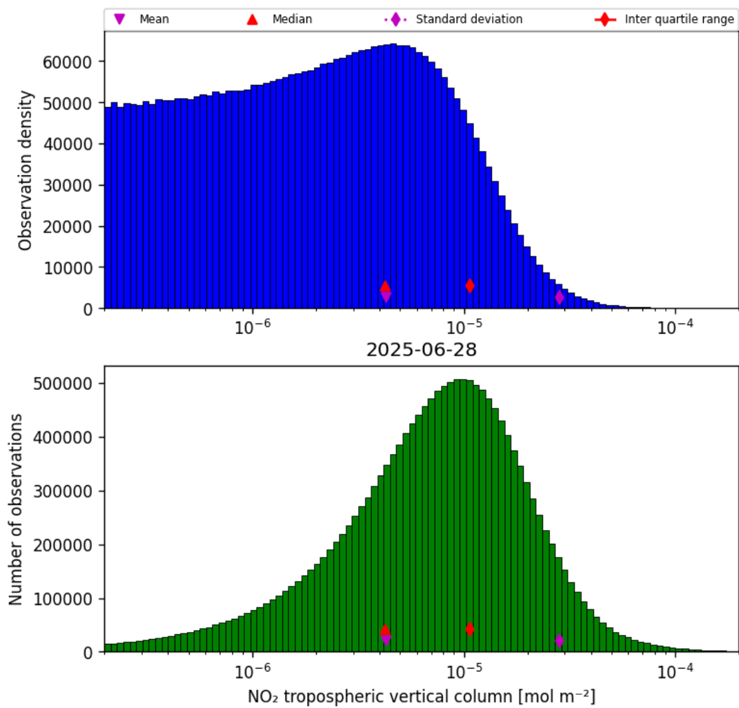
Figure 27: Histogram of “NO 2 tropospheric vertical column” for 2025-06-28 to 2025-06-29
