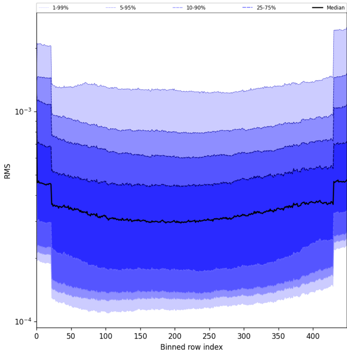
Figure 58: Along track statistics of “RMS” for 2025-06-28 to 2025-06-29
