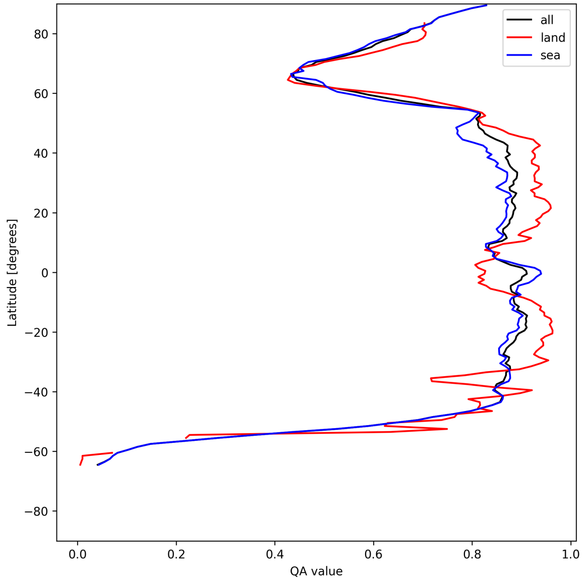
Figure 9: Zonal average of “QA value” for 2025-06-28 to 2025-06-29.
