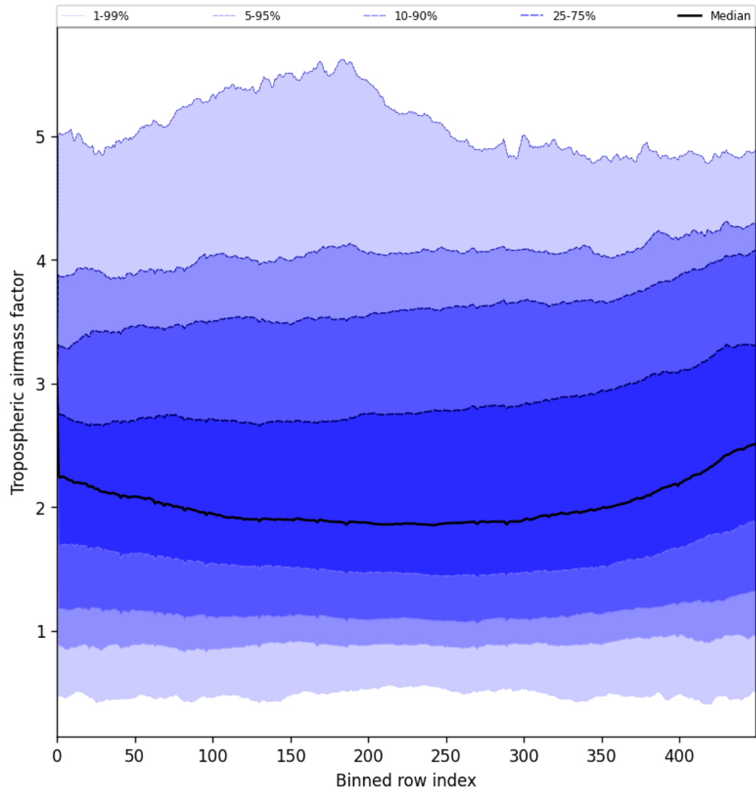
Figure 46: Along track statistics of “Tropospheric airmass factor” for 2025-06-28 to 2025-06-29
