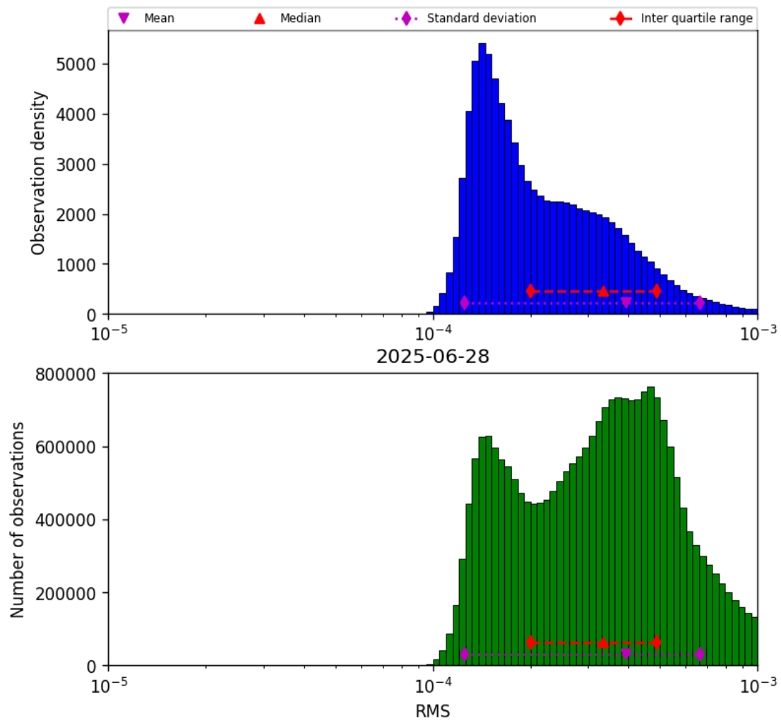
Figure 41: Histogram of “RMS” for 2025-06-28 to 2025-06-29
