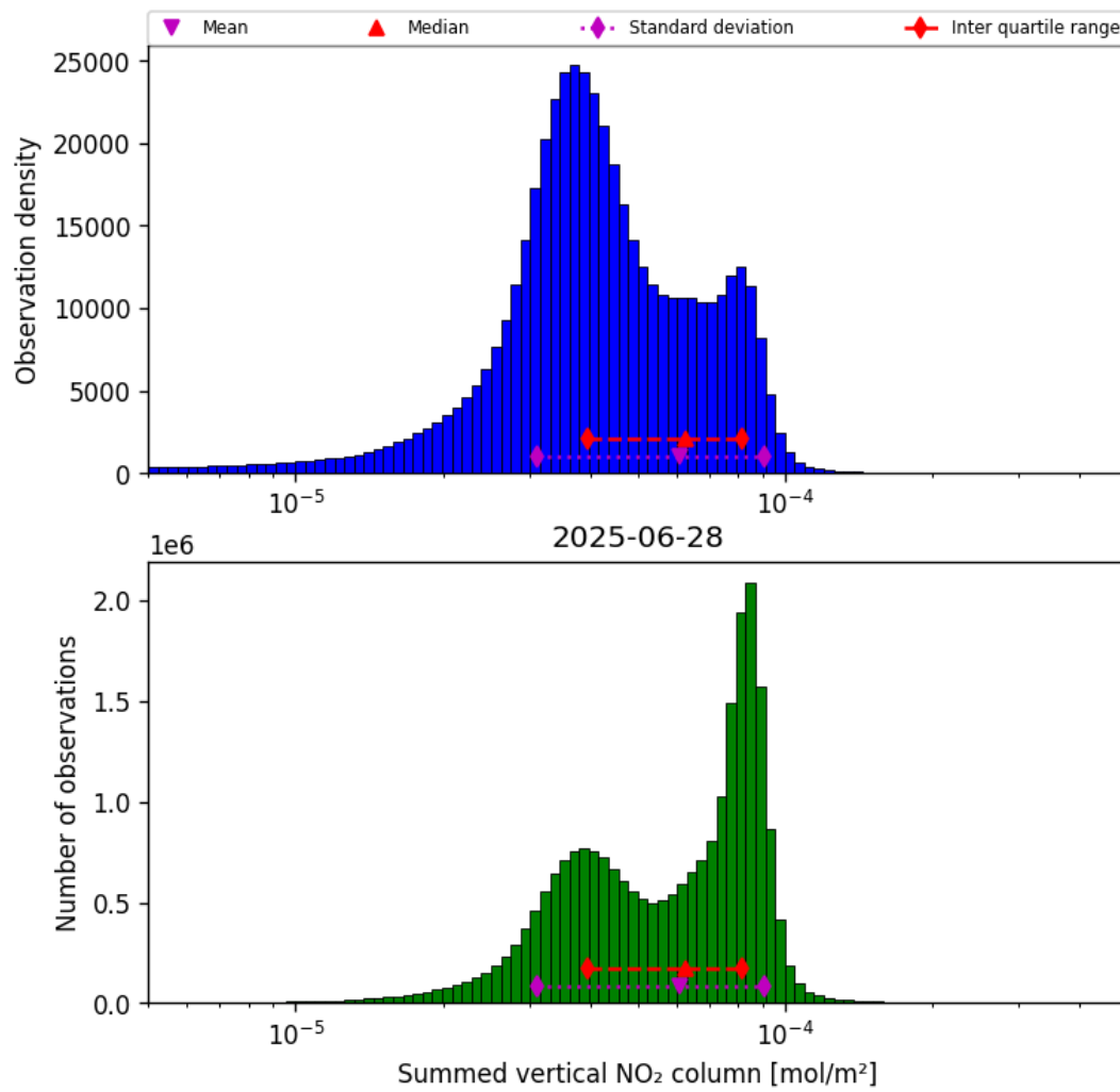
Figure 38: Histogram of “Summed vertical NO 2 column” for 2025-06-28 to 2025-06-29
