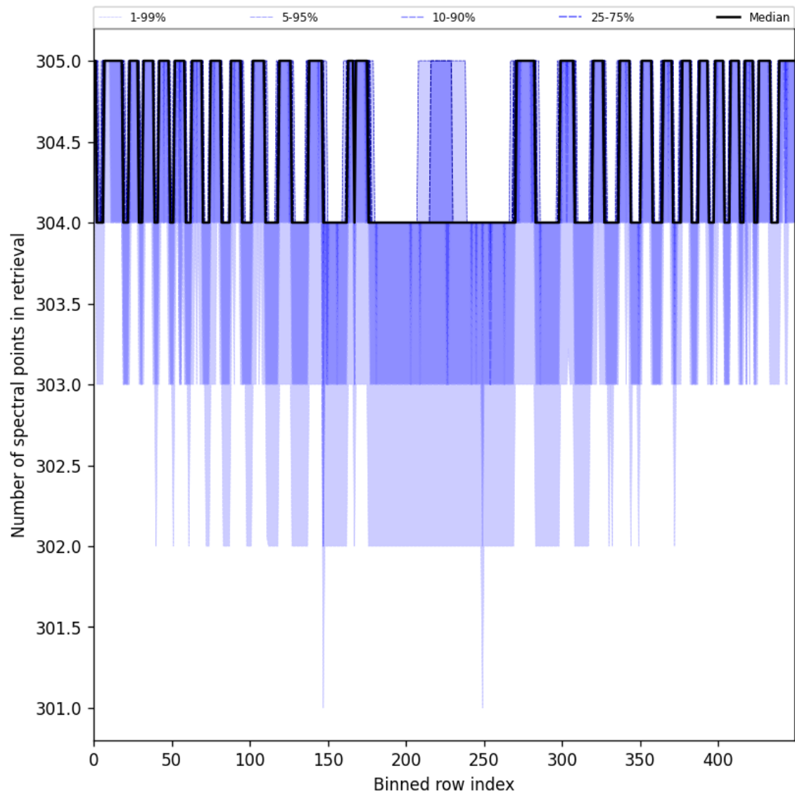
Figure 48: Along track statistics of “Number of spectral points in retrieval” for 2025-06-28 to 2025-06-29
