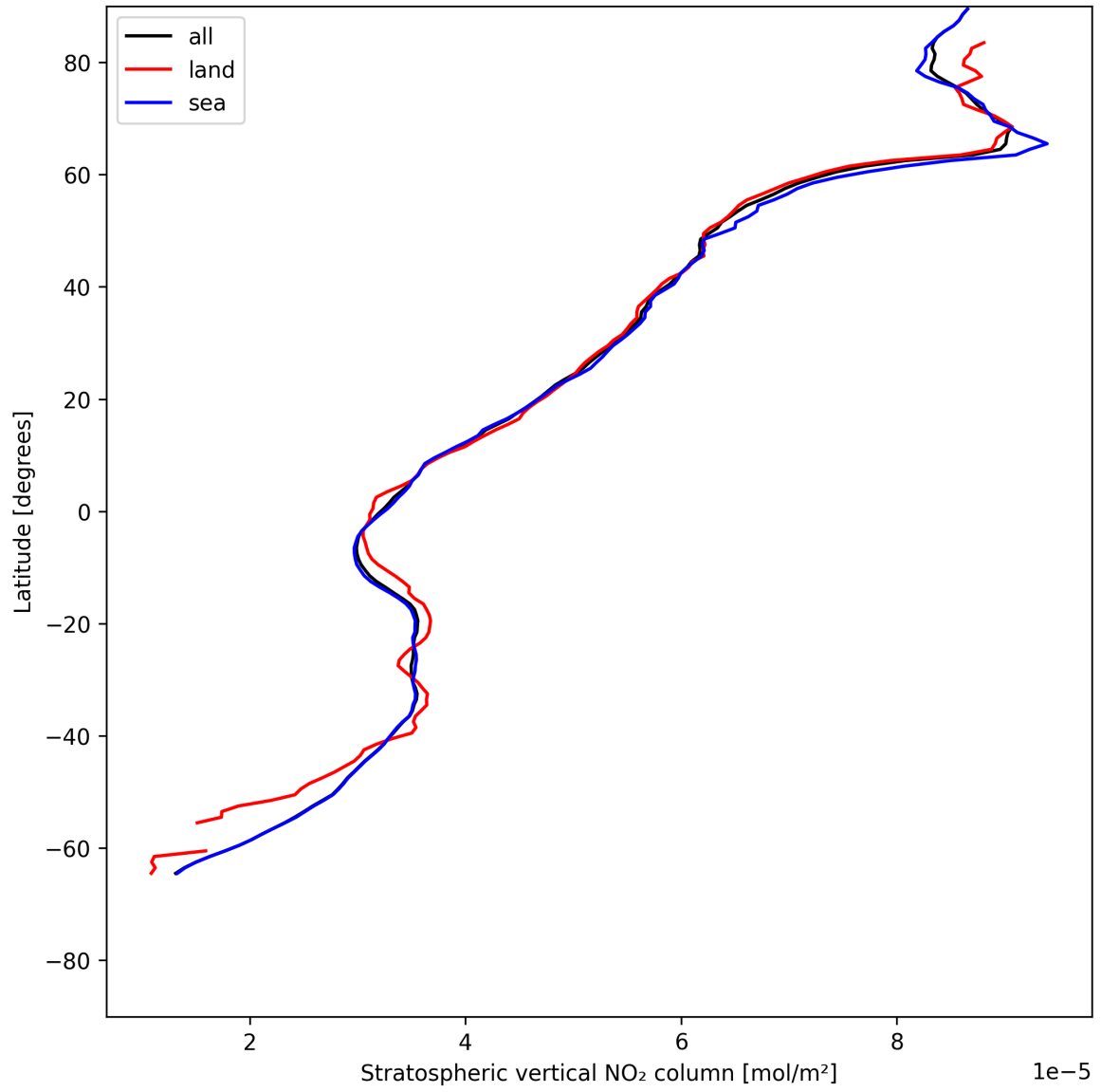
Figure 17: Zonal average of “Stratospheric vertical NO 2 column” for 2025-06-28 to 2025-06-29.
