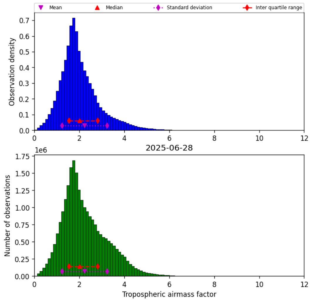
Figure 29: Histogram of “Tropospheric airmass factor” for 2025-06-28 to 2025-06-29
