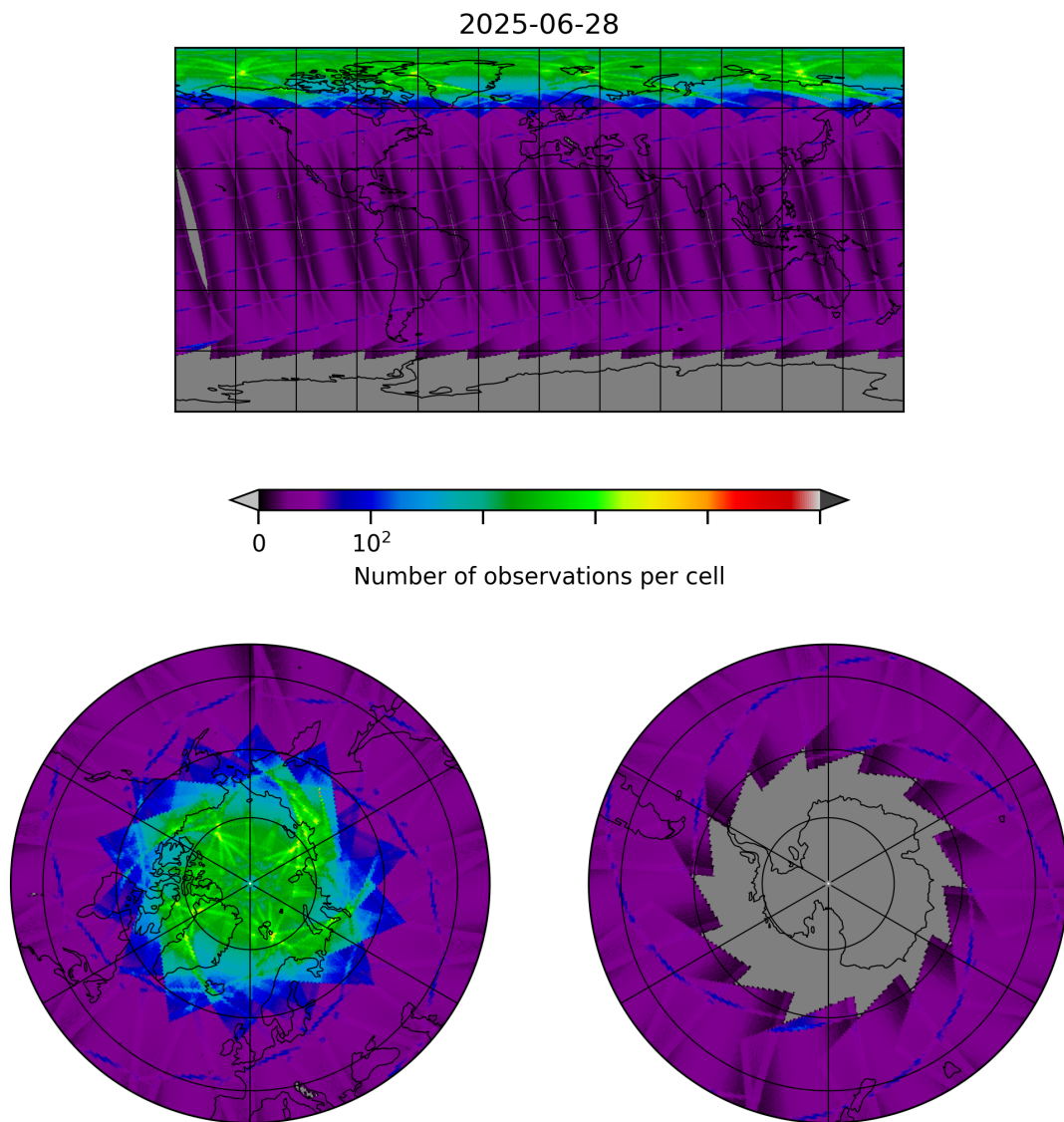
Figure 8: Map of the number of observations for 2025-06-28 to 2025-06-29
