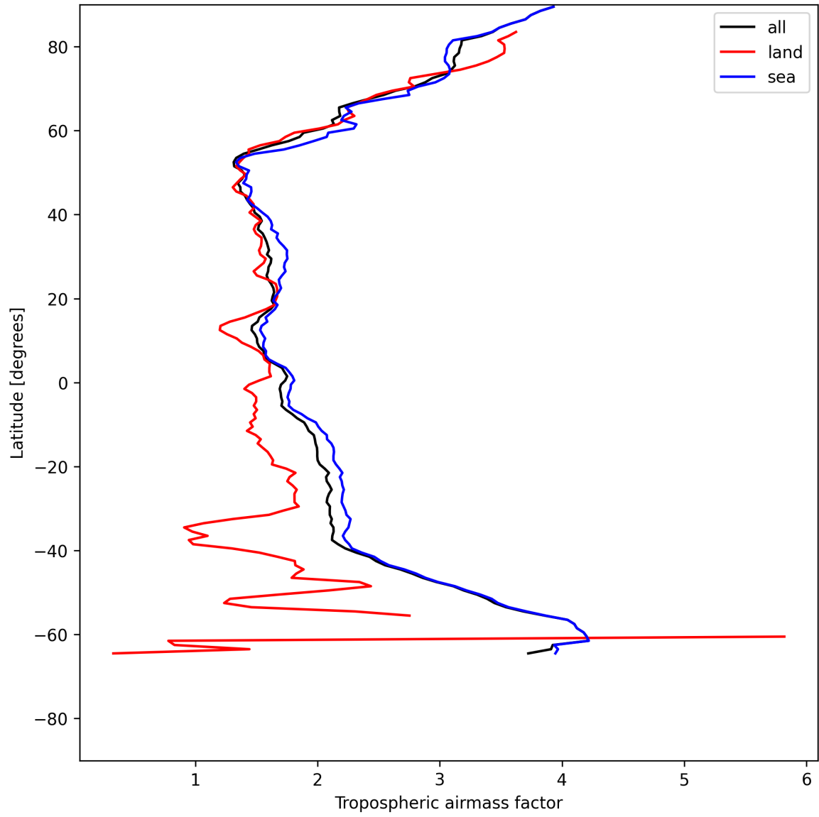
Figure 12: Zonal average of “Tropospheric airmass factor” for 2025-06-28 to 2025-06-29.
