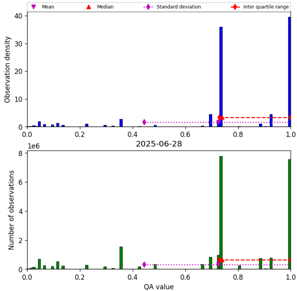
Figure 26: Histogram of “QA value” for 2025-06-28 to 2025-06-29
