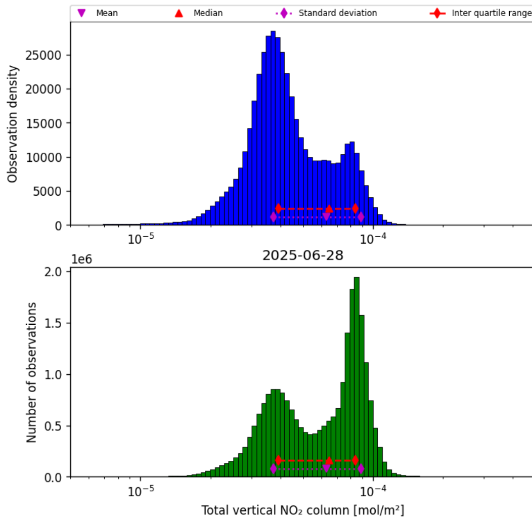
Figure 36: Histogram of "Total vertical NO 2 column" for 2025-06-28 to 2025-06-29
