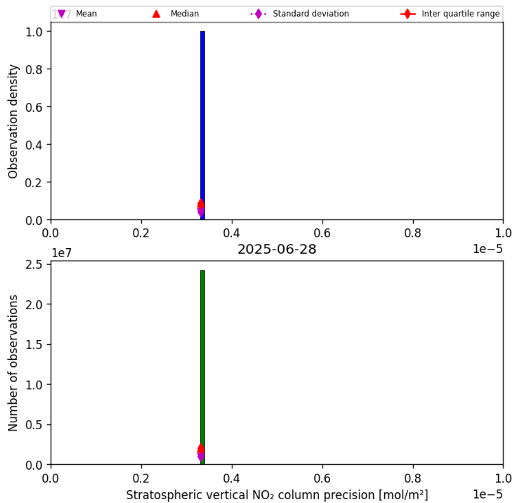
Figure 35: Histogram of “Stratospheric vertical NO 2 column precision” for 2025-06-28 to 2025-06-29
