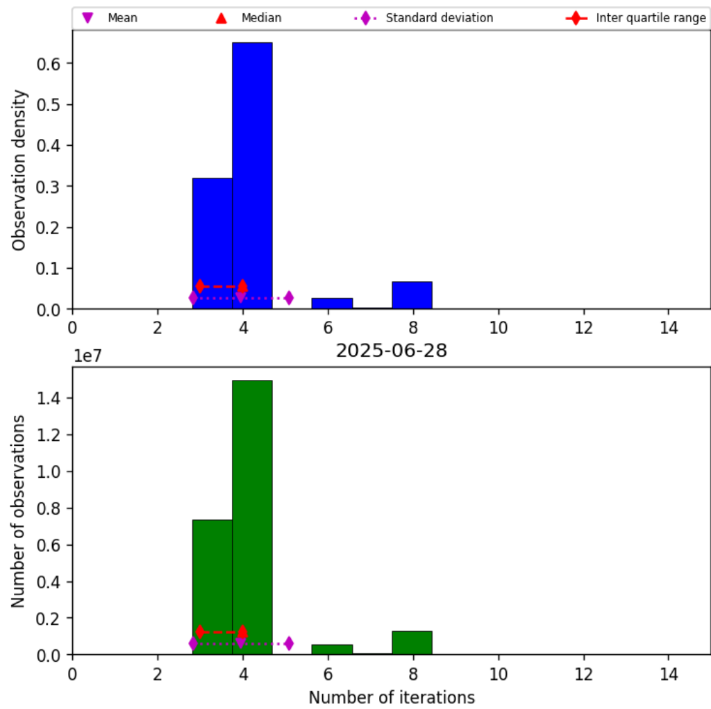
Figure 32: Histogram of “Number of iterations” for 2025-06-28 to 2025-06-29
