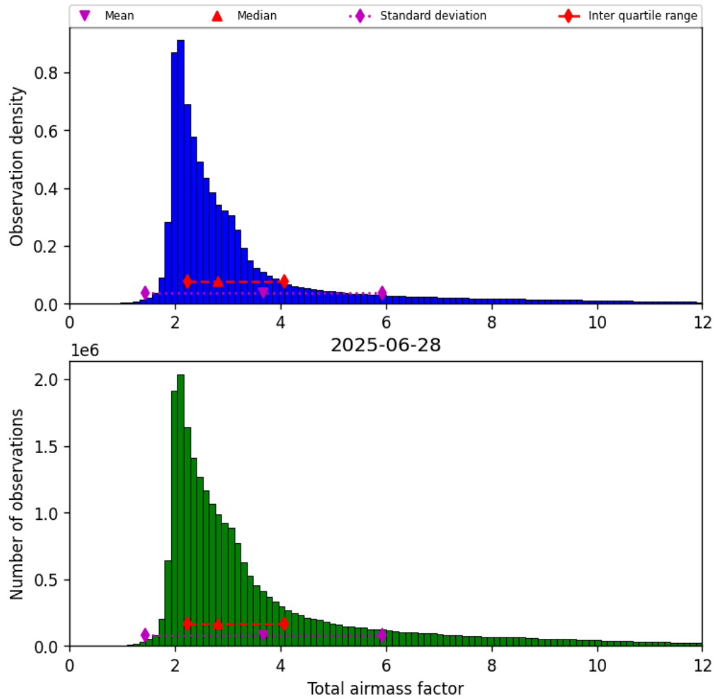
Figure 30: Histogram of “Total airmass factor” for 2025-06-28 to 2025-06-29
