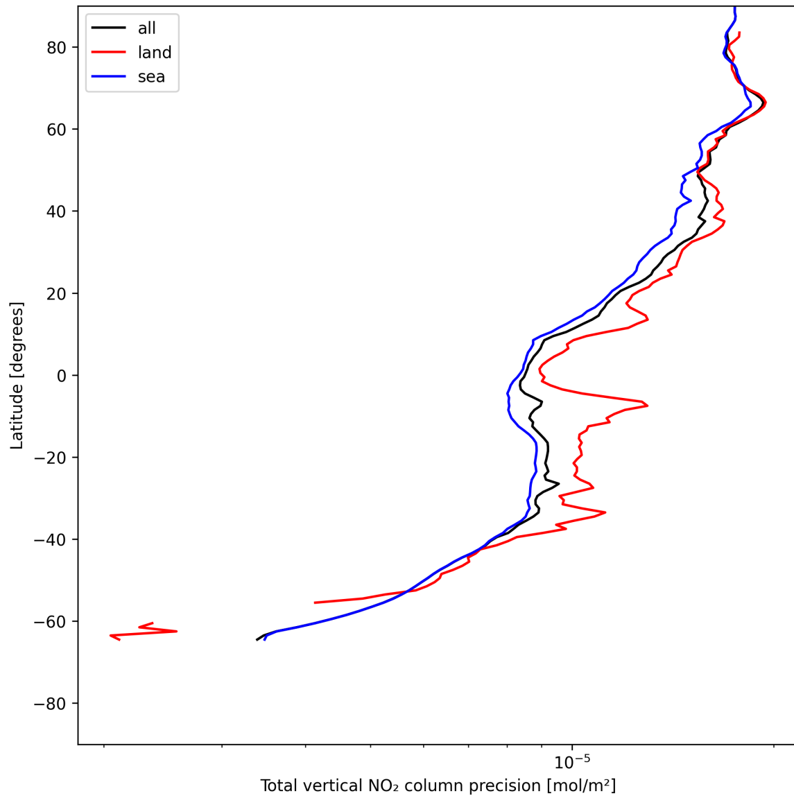
Figure 20: Zonal average of “Total vertical NO 2 column precision” for 2025-06-28 to 2025-06-29.
