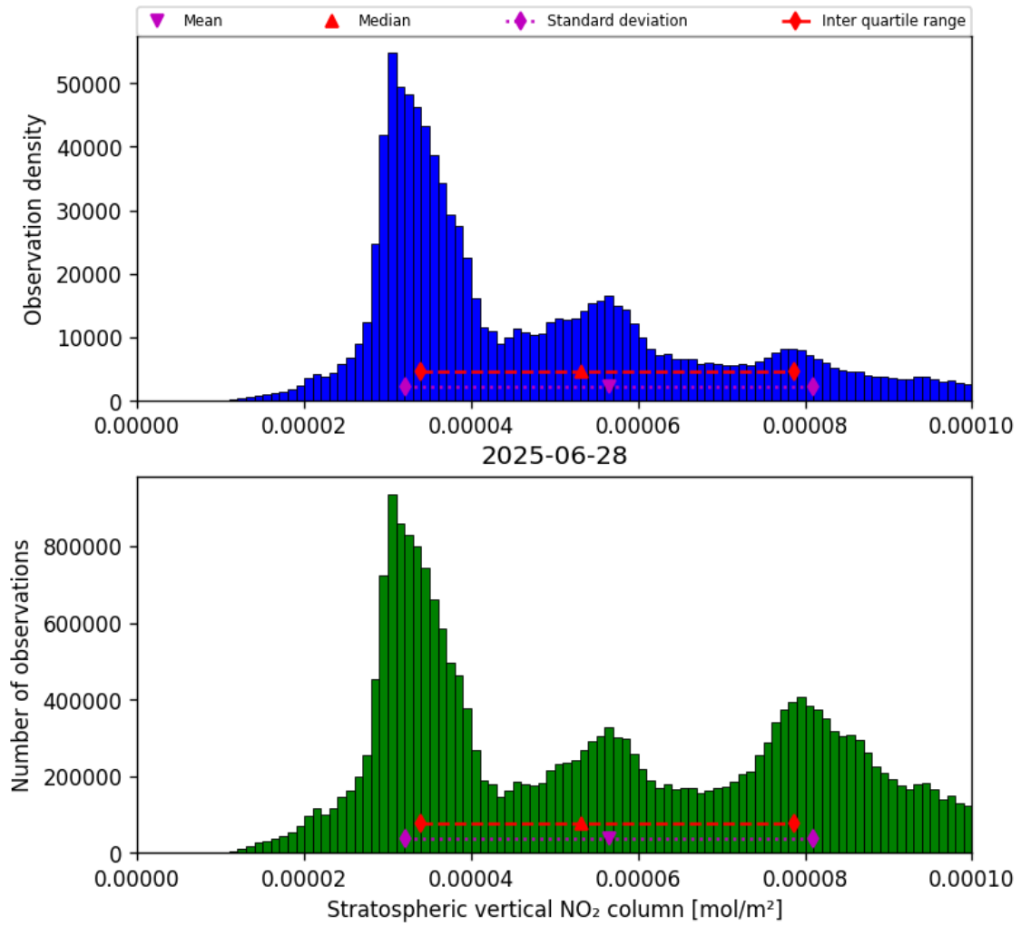
Figure 34: Histogram of “Stratospheric vertical NO 2 column” for 2025-06-28 to 2025-06-29
