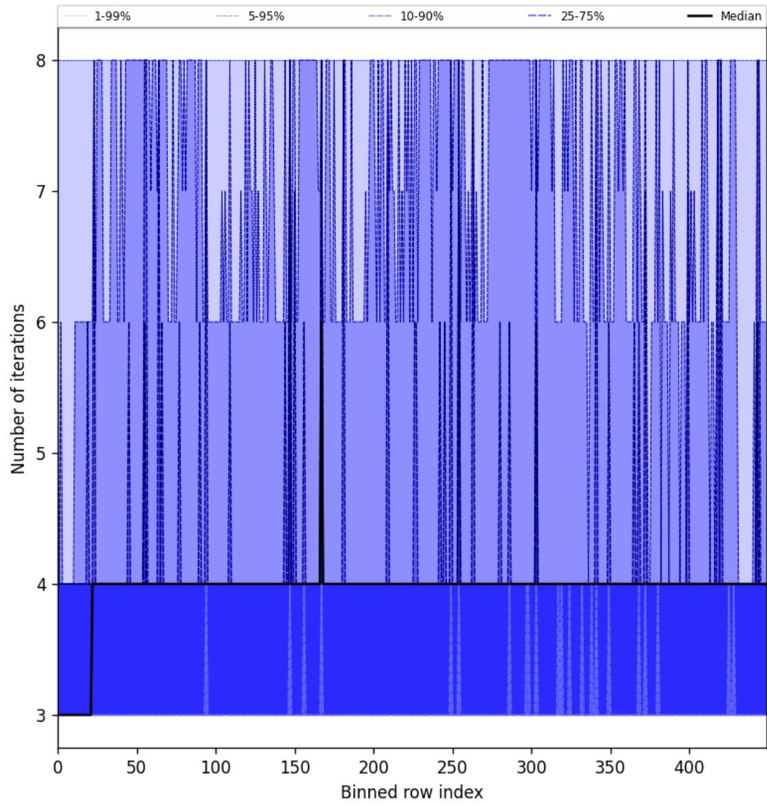
Figure 49: Along track statistics of “Number of iterations” for 2025-06-28 to 2025-06-29
