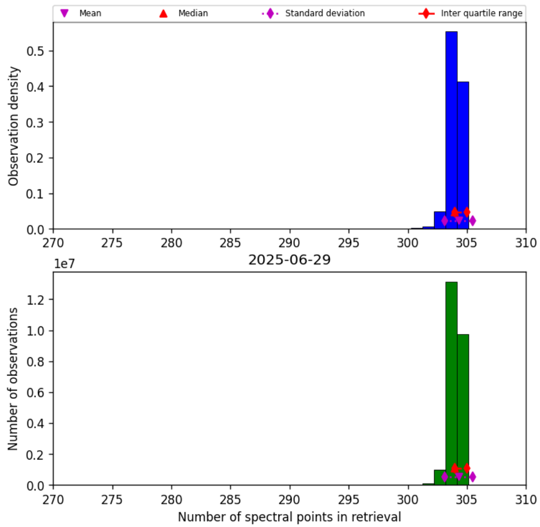
Figure 31: Histogram of “Number of spectral points in retrieval” for 2025-06-29 to 2025-06-30
