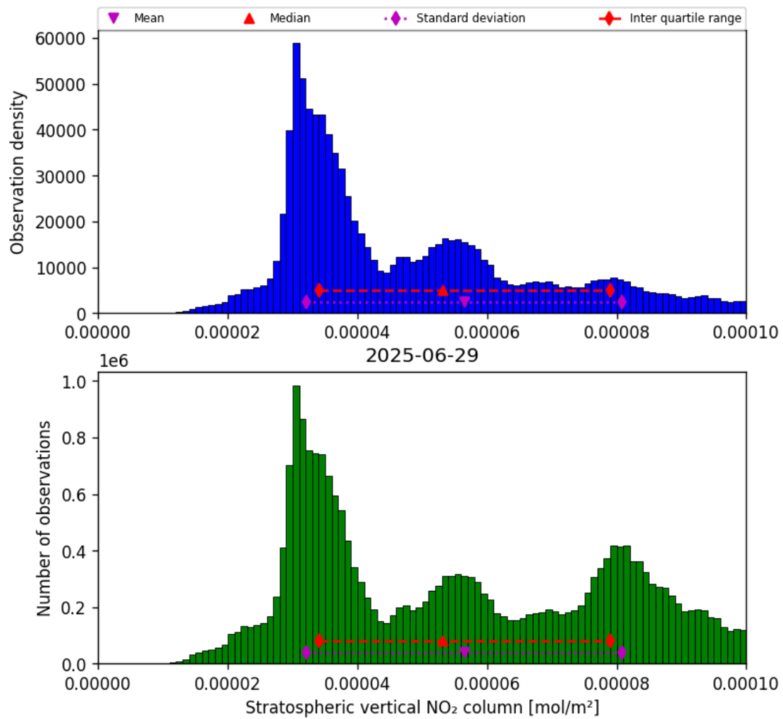
Figure 34: Histogram of “Stratospheric vertical NO 2 column” for 2025-06-29 to 2025-06-30
