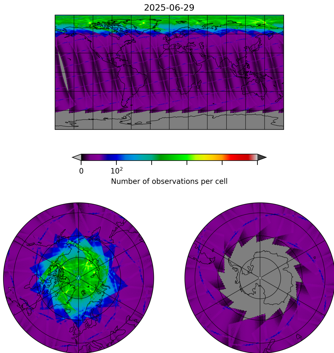
Figure 8: Map of the number of observations for 2025-06-29 to 2025-06-30
