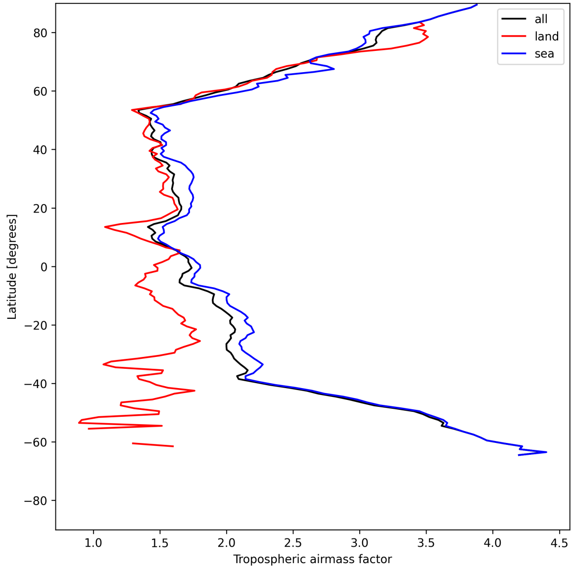
Figure 12: Zonal average of “Tropospheric airmass factor” for 2025-06-29 to 2025-06-30.
