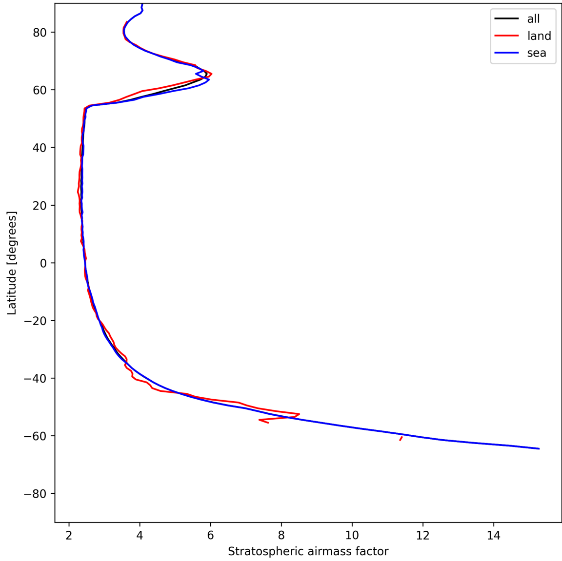
Figure 25: Zonal average of “Stratospheric air mass factor” for 2025-06-29 to 2025-06-30.
