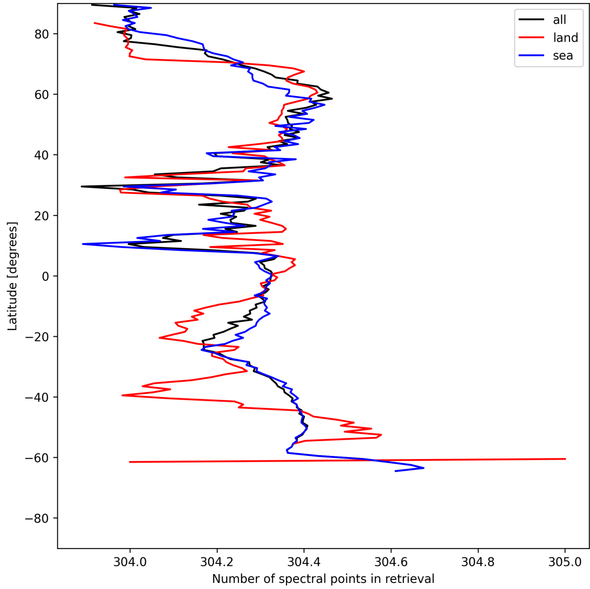
Figure 14: Zonal average of “Number of spectral points in retrieval” for 2025-06-29 to 2025-06-30.
