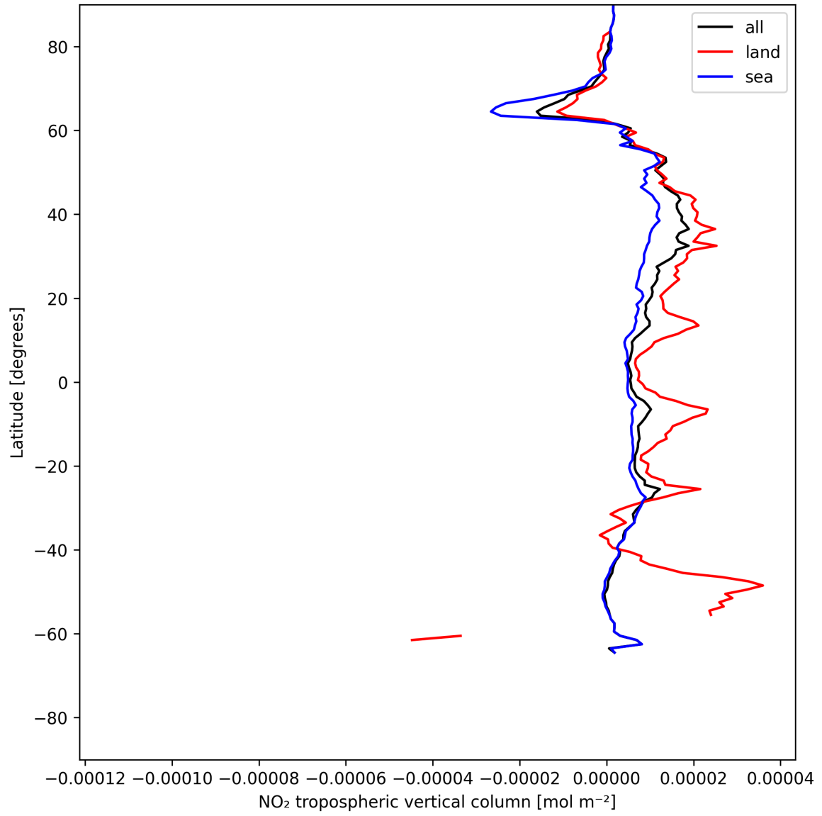
Figure 10: Zonal average of “NO 2 tropospheric vertical column” for 2025-06-29 to 2025-06-30.
