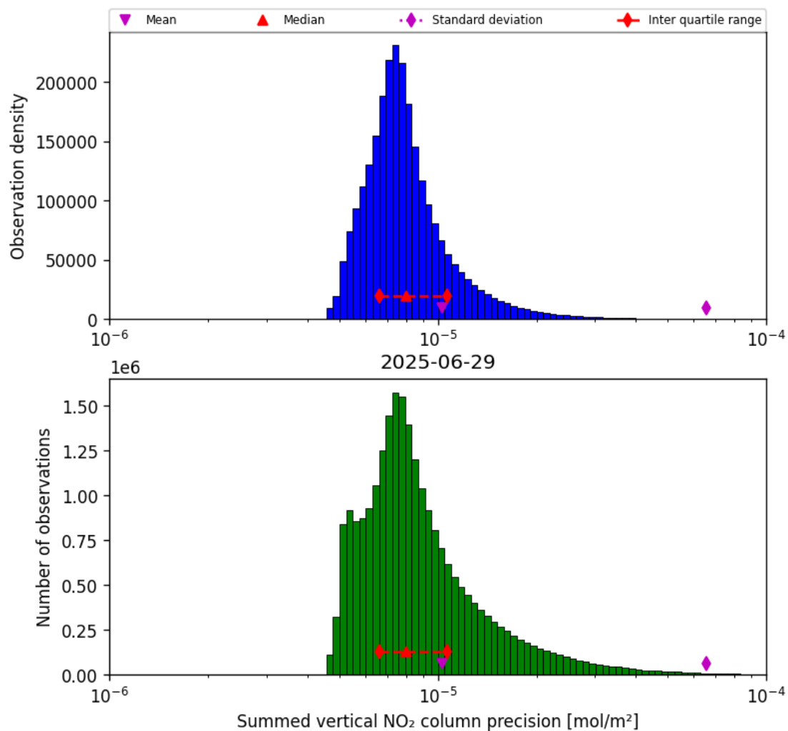
Figure 39: Histogram of “Summed vertical NO 2 column precision” for 2025-06-29 to 2025-06-30
