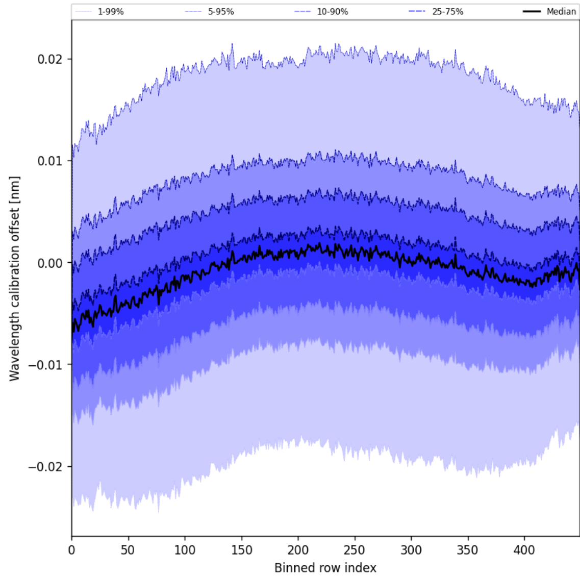
Figure 50: Along track statistics of “Wavelength calibration offset” for 2025-06-29 to 2025-06-30
