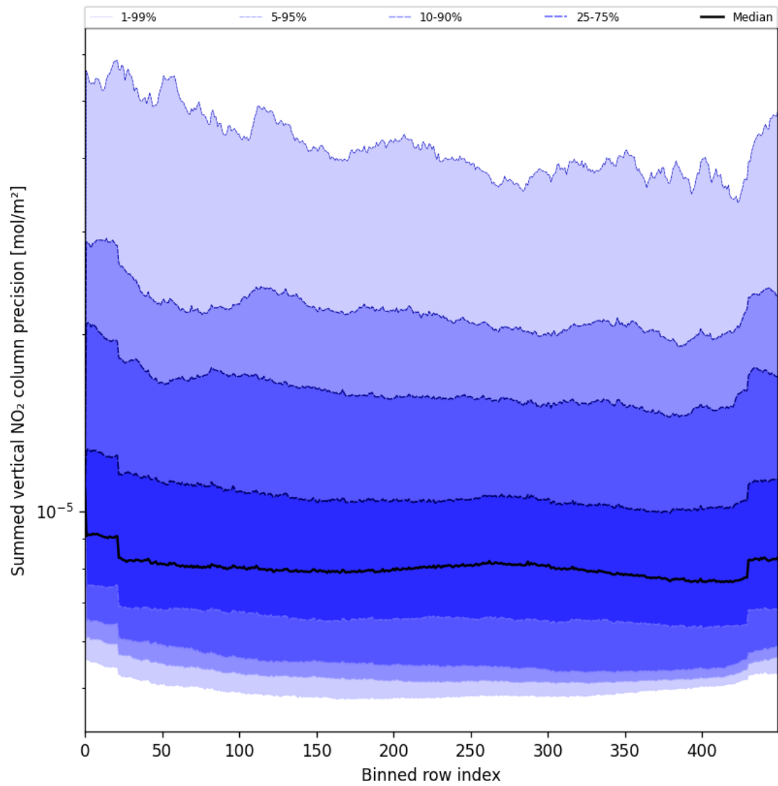
Figure 56: Along track statistics of “Summed vertical NO 2 column precision” for 2025-06-29 to 2025-06-30
