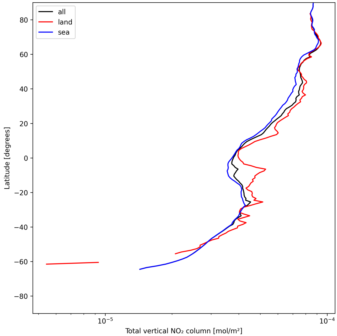
Figure 19: Zonal average of “Total vertical NO 2 column” for 2025-06-29 to 2025-06-30.
