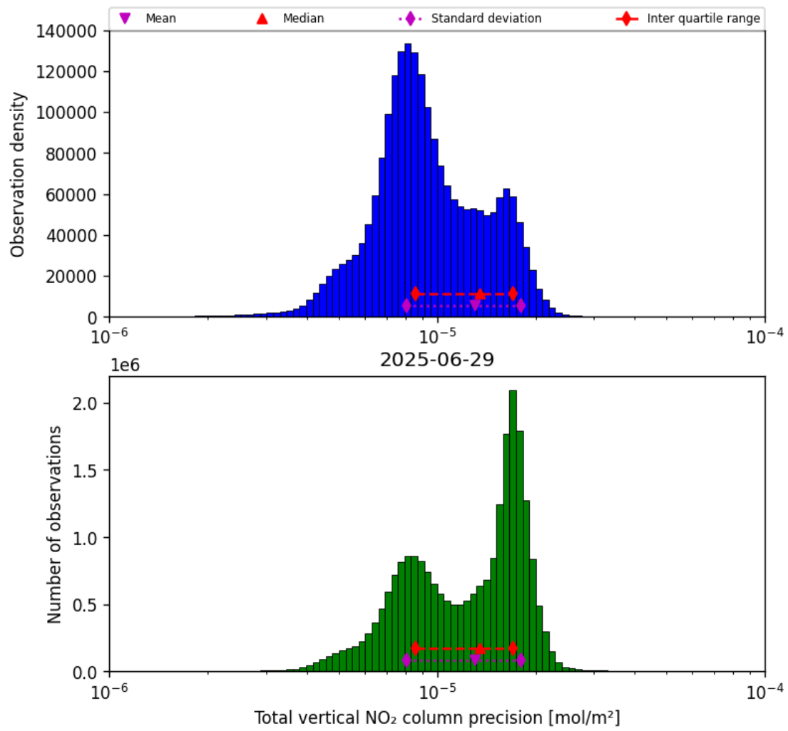
Figure 37: Histogram of "Total vertical NO 2 column precision" for 2025-06-29 to 2025-06-30
