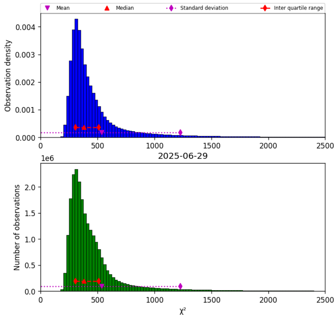
Figure 40: Histogram of “ \chi^2 ” for 2025-06-29 to 2025-06-30
