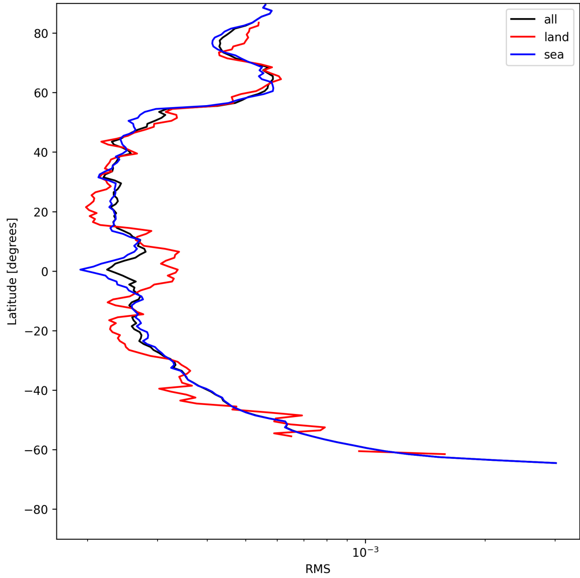
Figure 24: Zonal average of “RMS” for 2025-06-29 to 2025-06-30.
