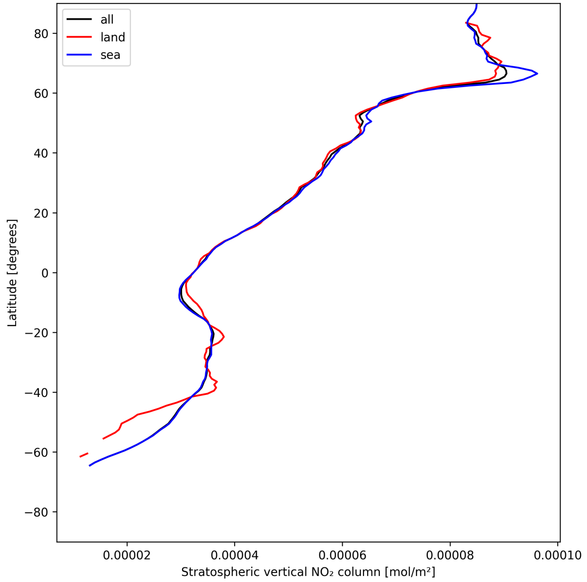
Figure 17: Zonal average of “Stratospheric vertical NO 2 column” for 2025-06-29 to 2025-06-30.
