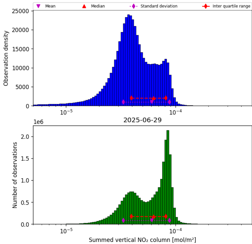
Figure 38: Histogram of “Summed vertical NO 2 column” for 2025-06-29 to 2025-06-30
