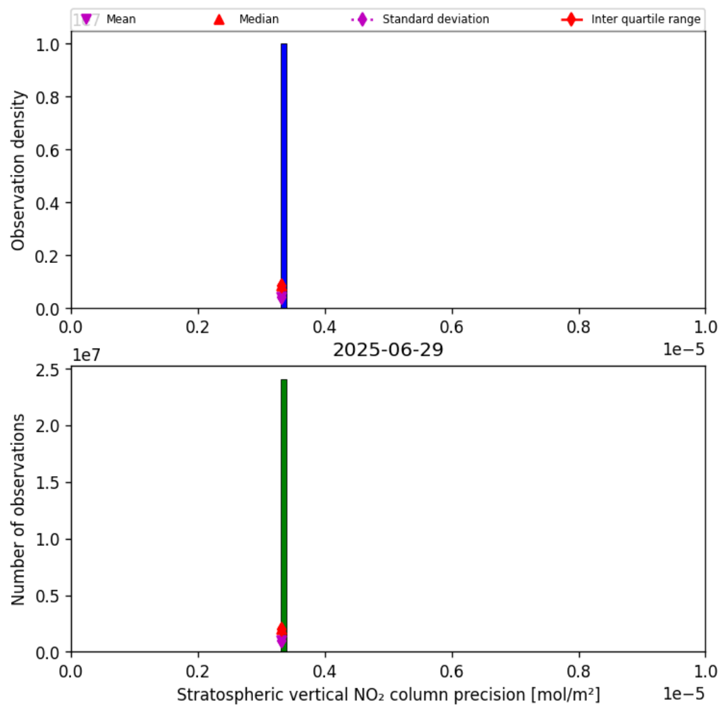
Figure 35: Histogram of “Stratospheric vertical NO 2 column precision” for 2025-06-29 to 2025-06-30
