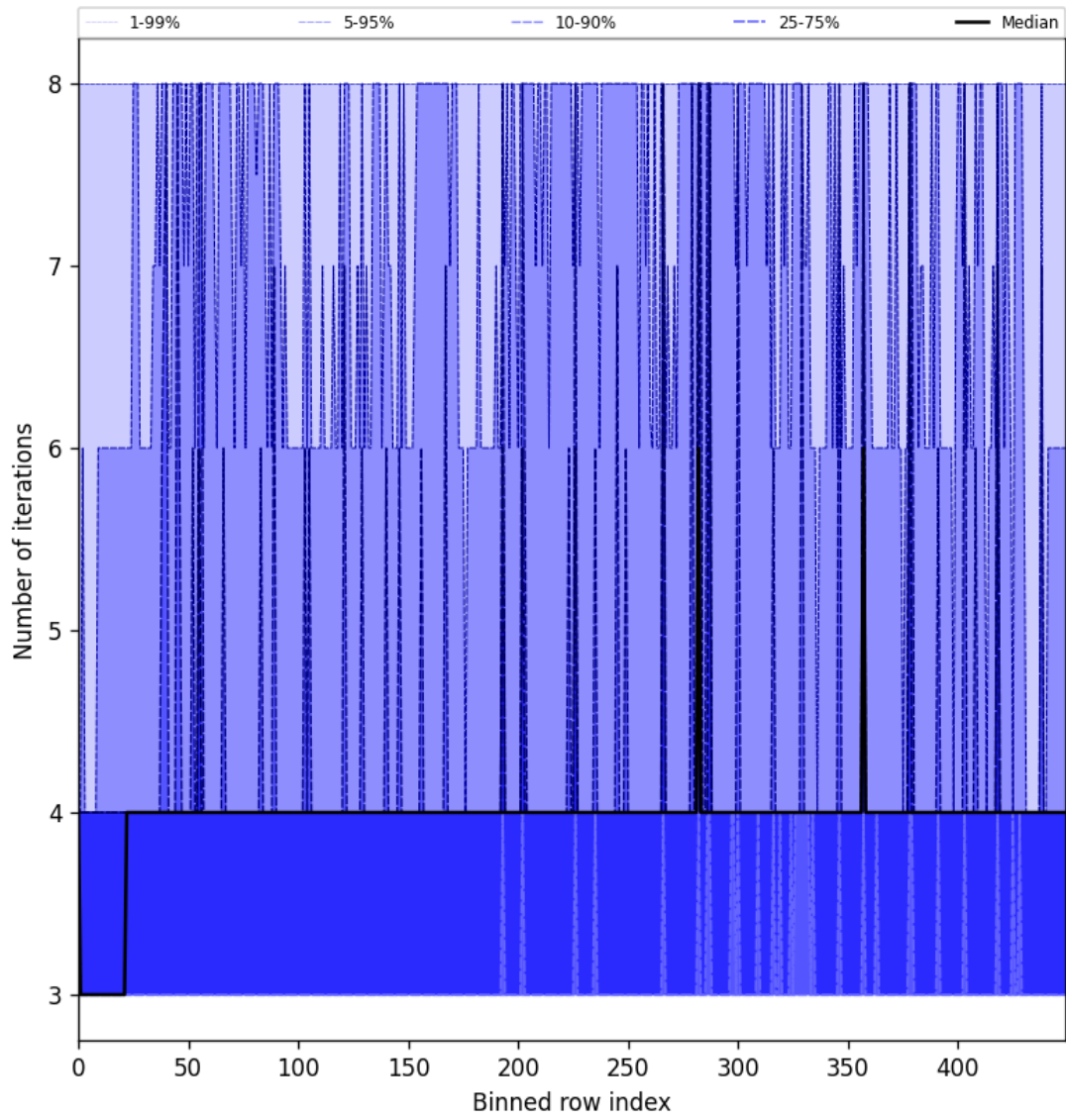
Figure 49: Along track statistics of “Number of iterations” for 2025-06-29 to 2025-06-30
