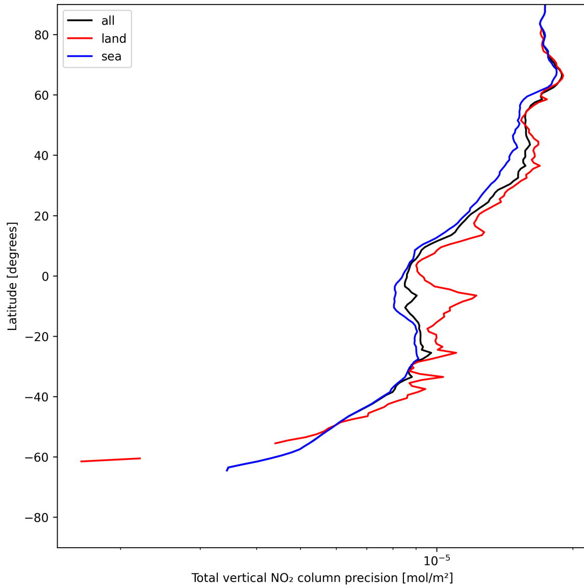
Figure 20: Zonal average of “Total vertical NO 2 column precision” for 2025-06-29 to 2025-06-30.
