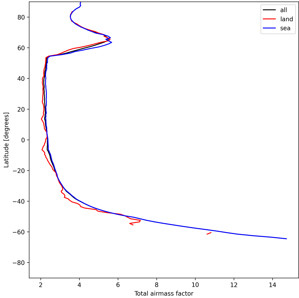
Figure 13: Zonal average of “Total airmass factor” for 2025-06-29 to 2025-06-30.
