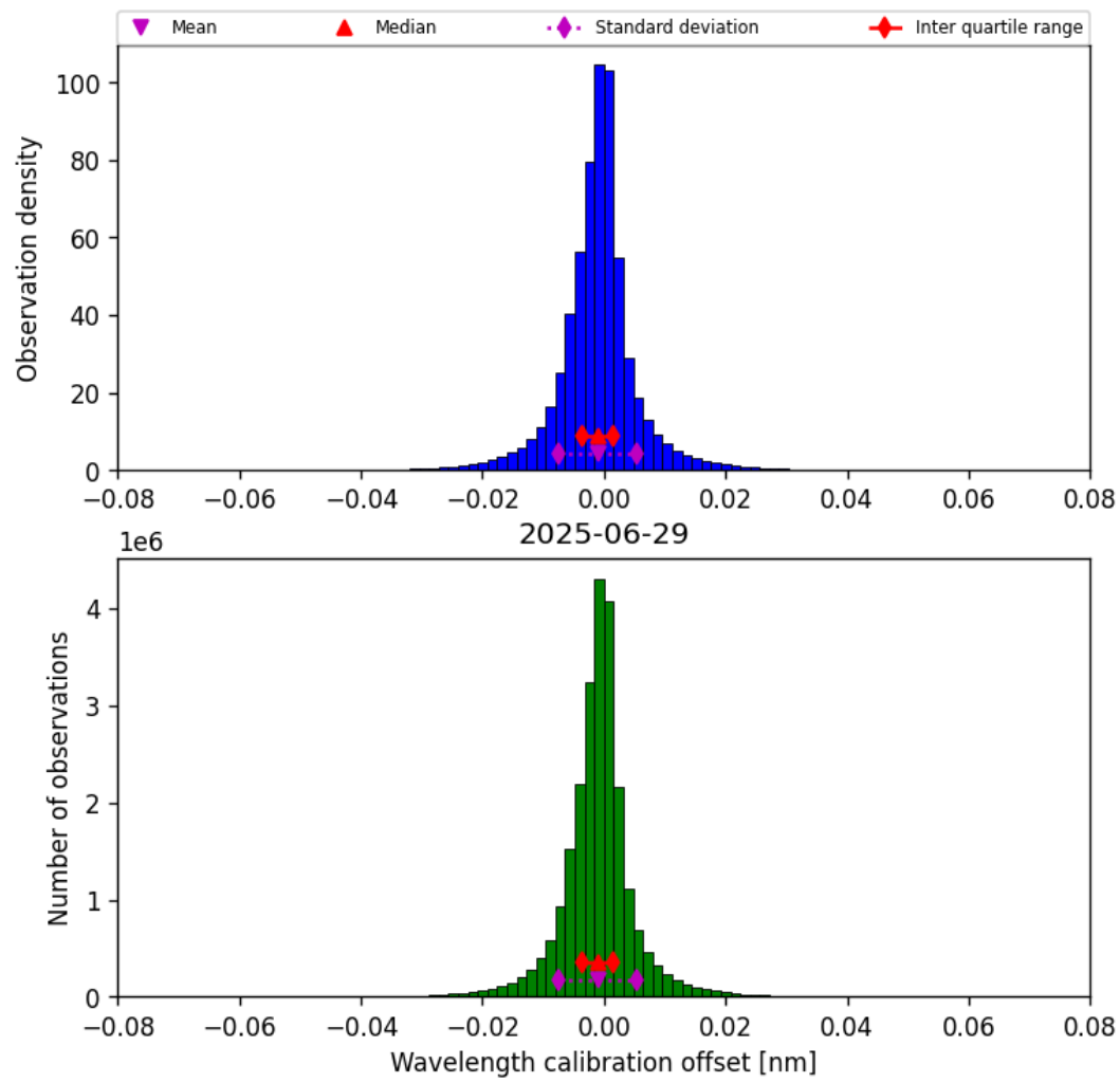
Figure 33: Histogram of “Wavelength calibration offset” for 2025-06-29 to 2025-06-30
