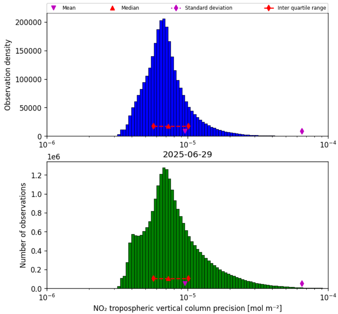
Figure 28: Histogram of “NO 2 tropospheric vertical column precision” for 2025-06-29 to 2025-06-30
