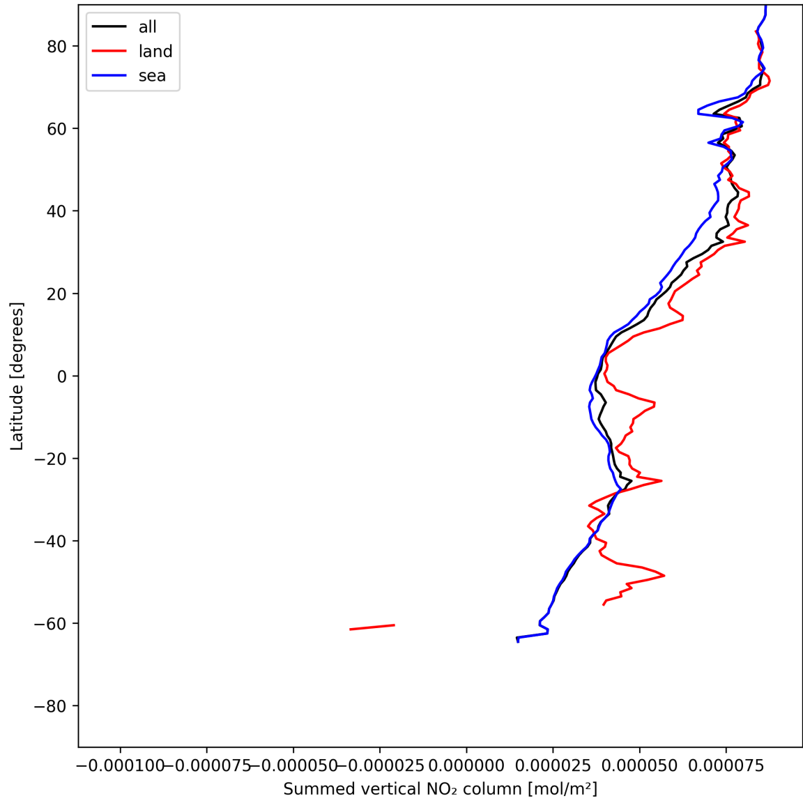
Figure 21: Zonal average of “Summed vertical NO 2 column” for 2025-06-29 to 2025-06-30.
