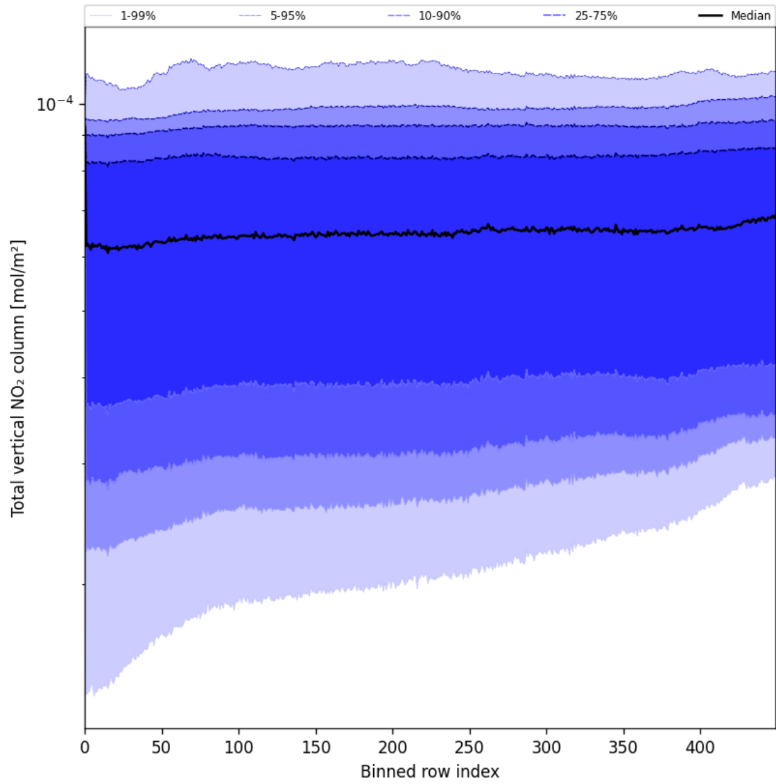
Figure 53: Along track statistics of “Total vertical NO 2 column” for 2025-06-29 to 2025-06-30
