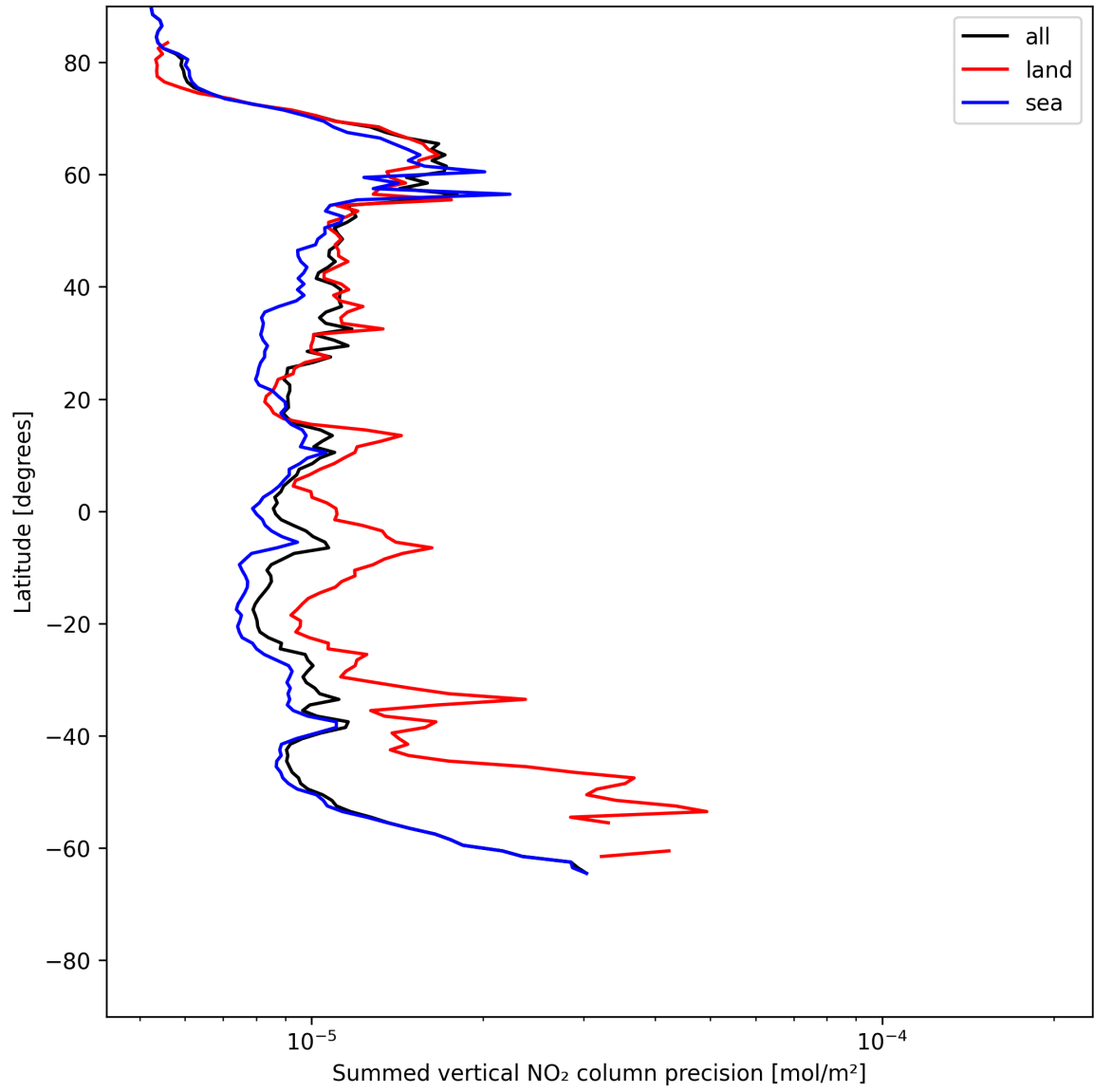
Figure 22: Zonal average of "Summed vertical NO 2 column precision" for 2025-06-29 to 2025-06-30.
