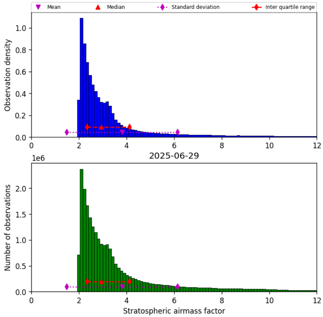
Figure 42: Histogram of “Stratospheric airmass factor” for 2025-06-29 to 2025-06-30
