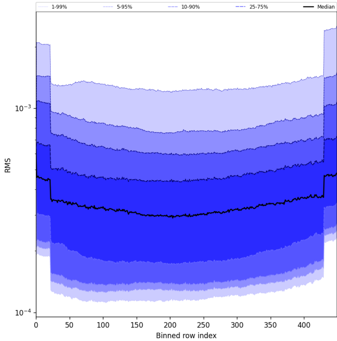
Figure 58: Along track statistics of “RMS” for 2025-06-29 to 2025-06-30
