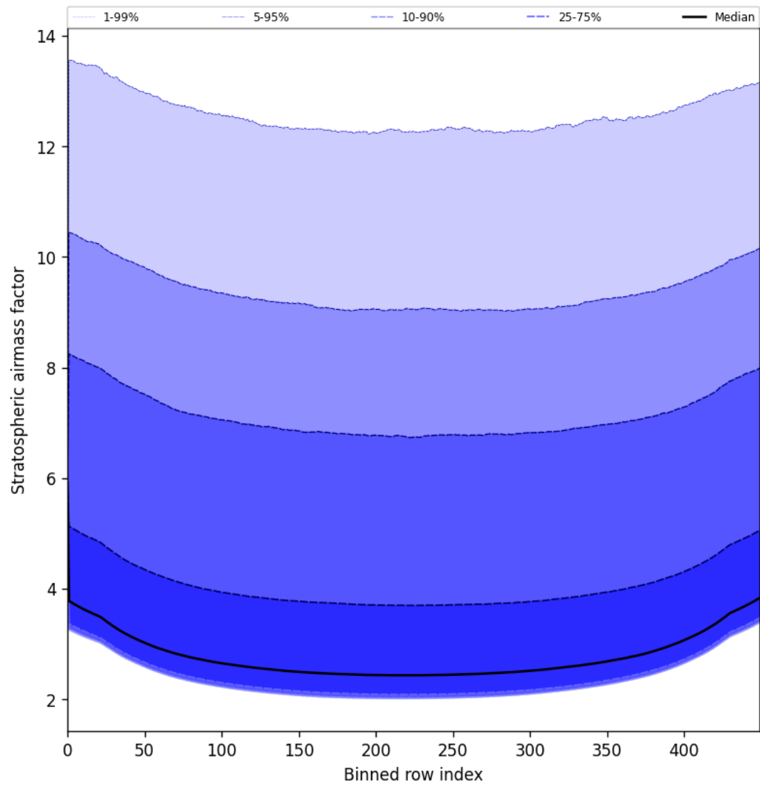
Figure 59: Along track statistics of “Stratospheric airmass factor” for 2025-06-29 to 2025-06-30
