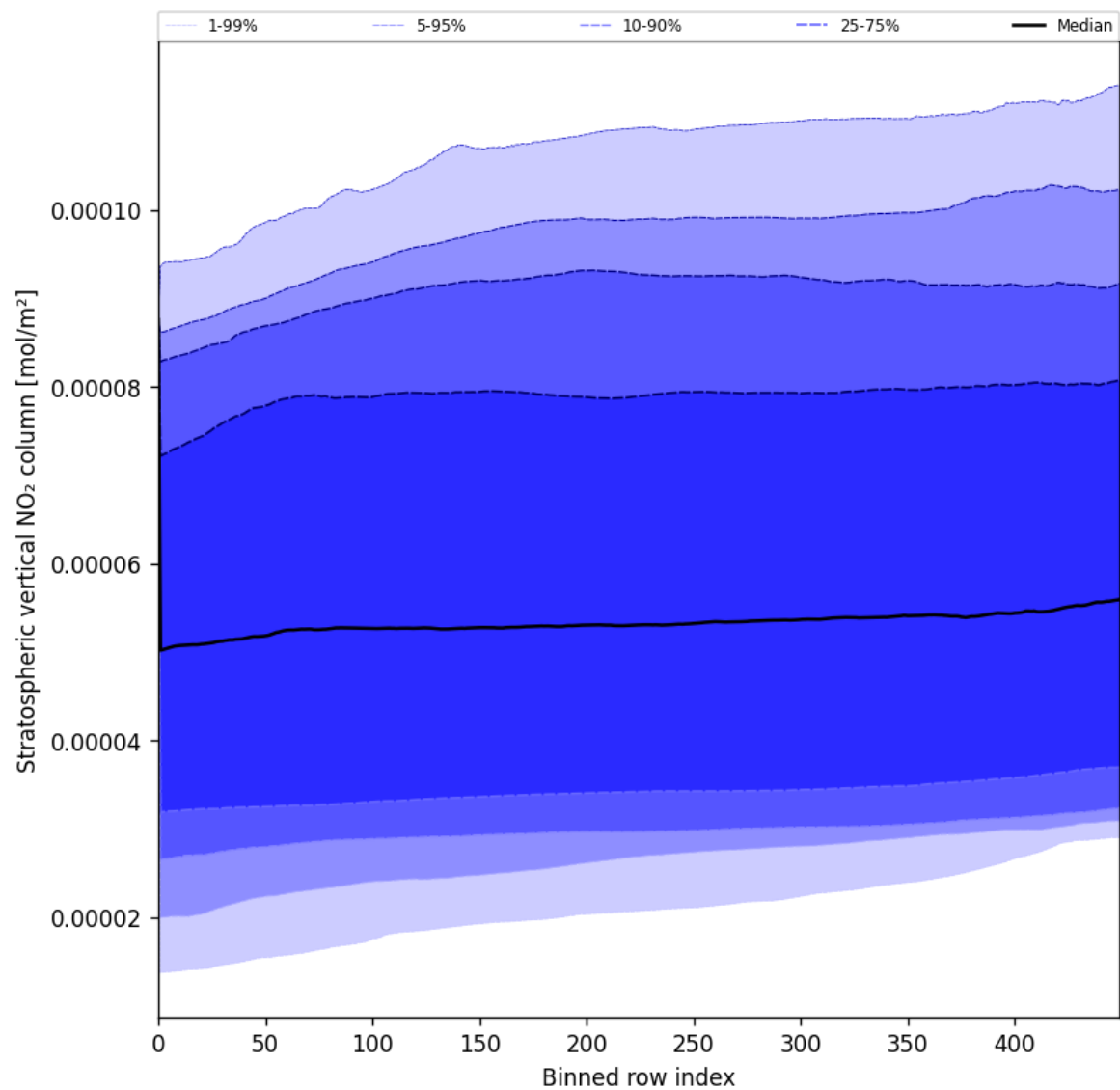
Figure 51: Along track statistics of “Stratospheric vertical NO 2 column” for 2025-06-29 to 2025-06-30
