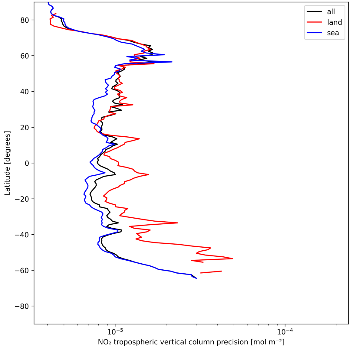
Figure 11: Zonal average of “NO 2 tropospheric vertical column precision” for 2025-06-29 to 2025-06-30.
