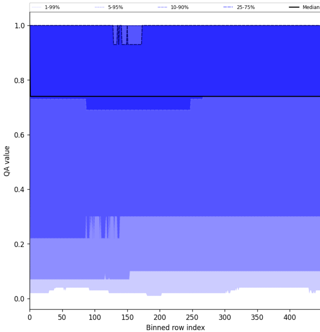
Figure 43: Along track statistics of “QA value” for 2025-06-29 to 2025-06-30
