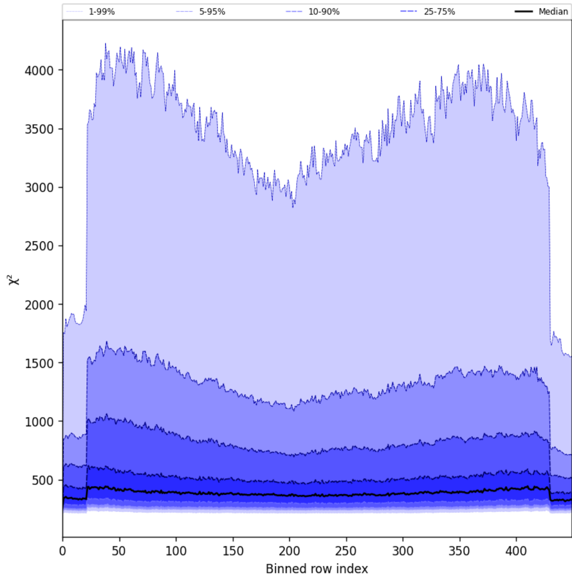
Figure 57: Along track statistics of “ \chi^2 ” for 2025-06-29 to 2025-06-30
