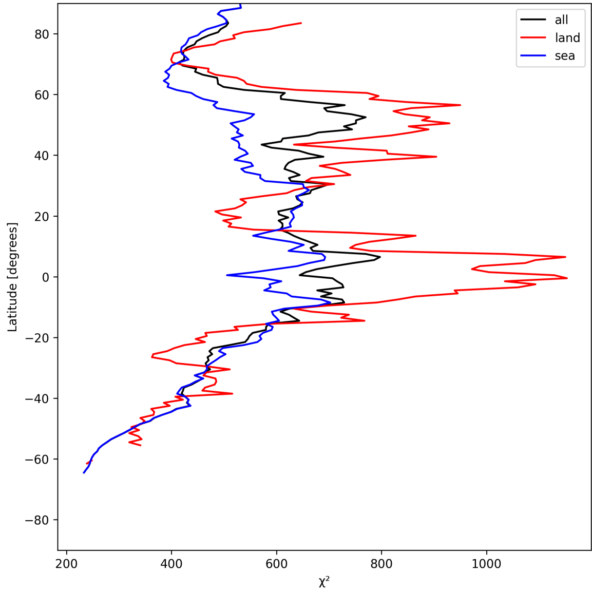
Figure 23: Zonal average of “ \chi^2 ” for 2025-06-29 to 2025-06-30.
