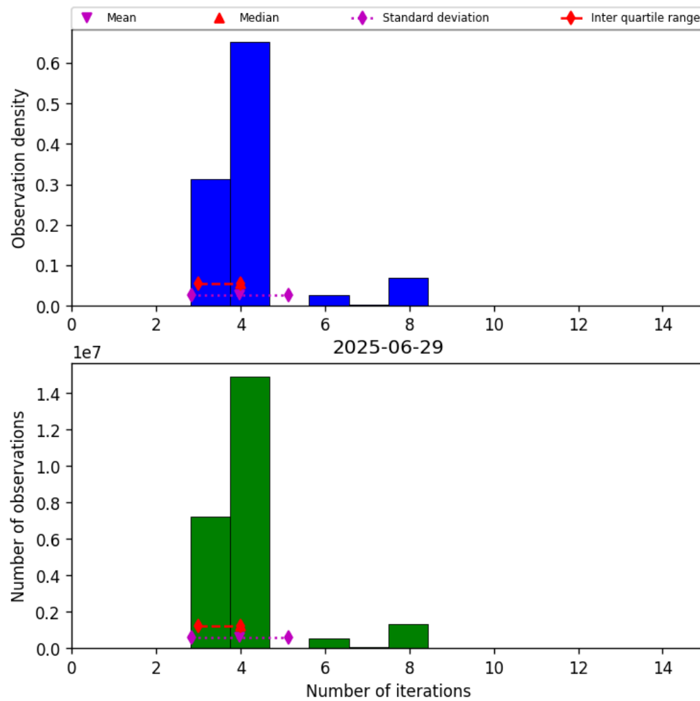
Figure 32: Histogram of “Number of iterations” for 2025-06-29 to 2025-06-30
