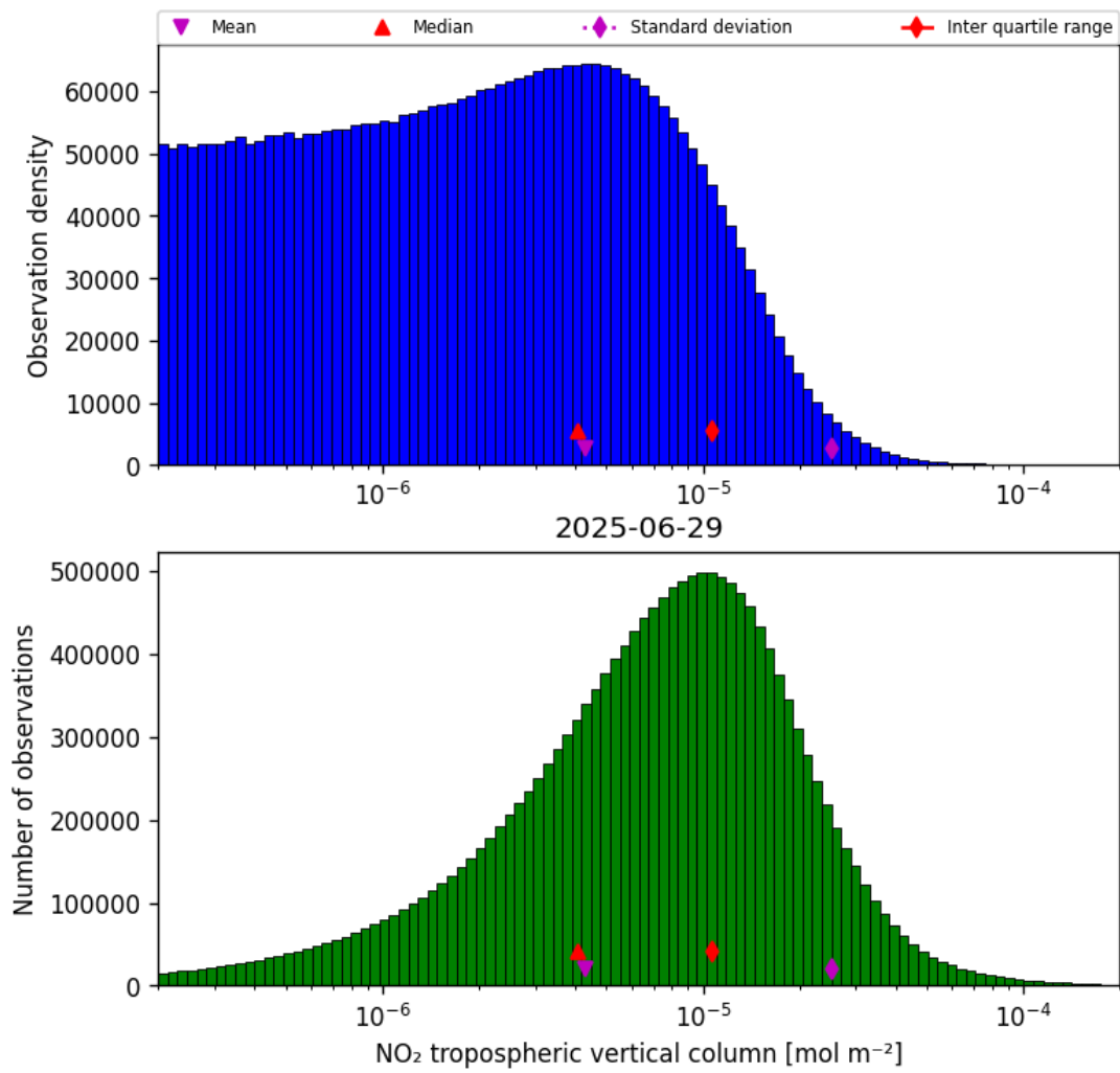
Figure 27: Histogram of “NO 2 tropospheric vertical column” for 2025-06-29 to 2025-06-30
