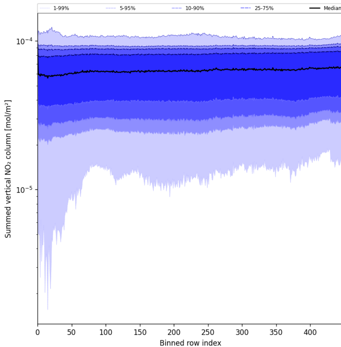
Figure 55: Along track statistics of “Summed vertical NO 2 column” for 2025-06-29 to 2025-06-30
