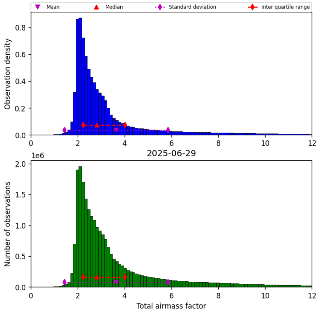
Figure 30: Histogram of “Total airmass factor” for 2025-06-29 to 2025-06-30
