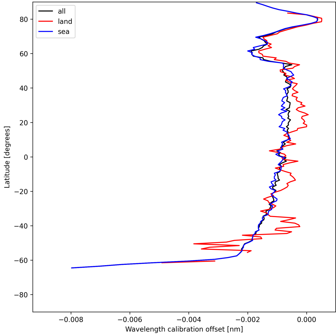
Figure 16: Zonal average of “Wavelength calibration offset” for 2025-06-29 to 2025-06-30.
