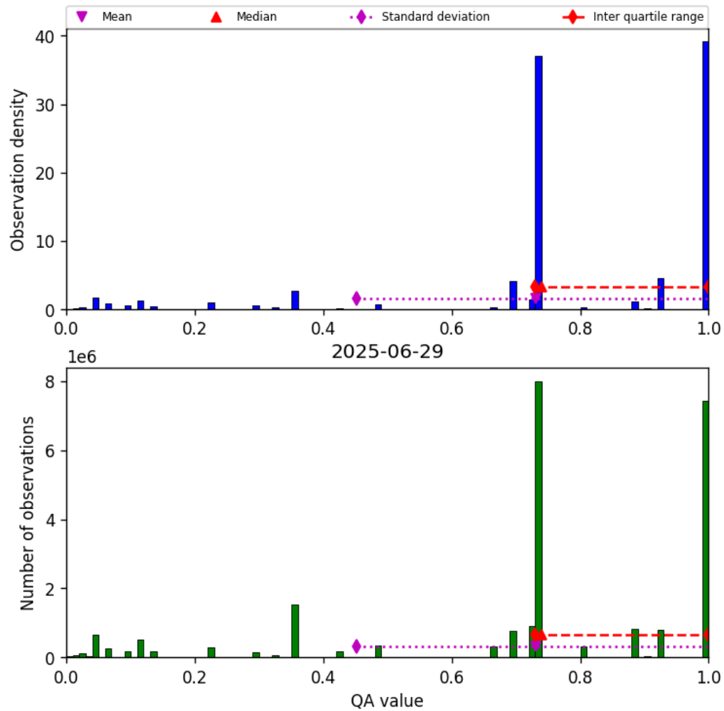
Figure 26: Histogram of “QA value” for 2025-06-29 to 2025-06-30
