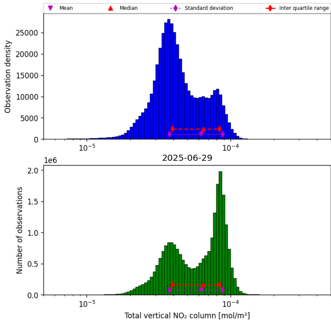
Figure 36: Histogram of “Total vertical NO 2 column” for 2025-06-29 to 2025-06-30
