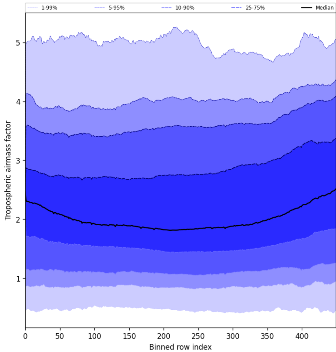
Figure 46: Along track statistics of “Tropospheric airmass factor” for 2025-06-29 to 2025-06-30
