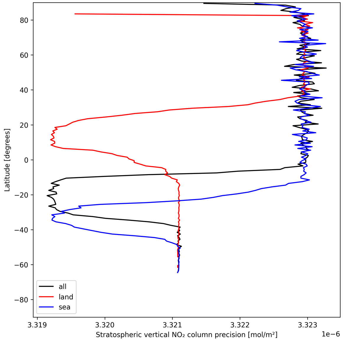
Figure 18: Zonal average of “Stratospheric vertical NO 2 column precision” for 2025-06-29 to 2025-06-30.
