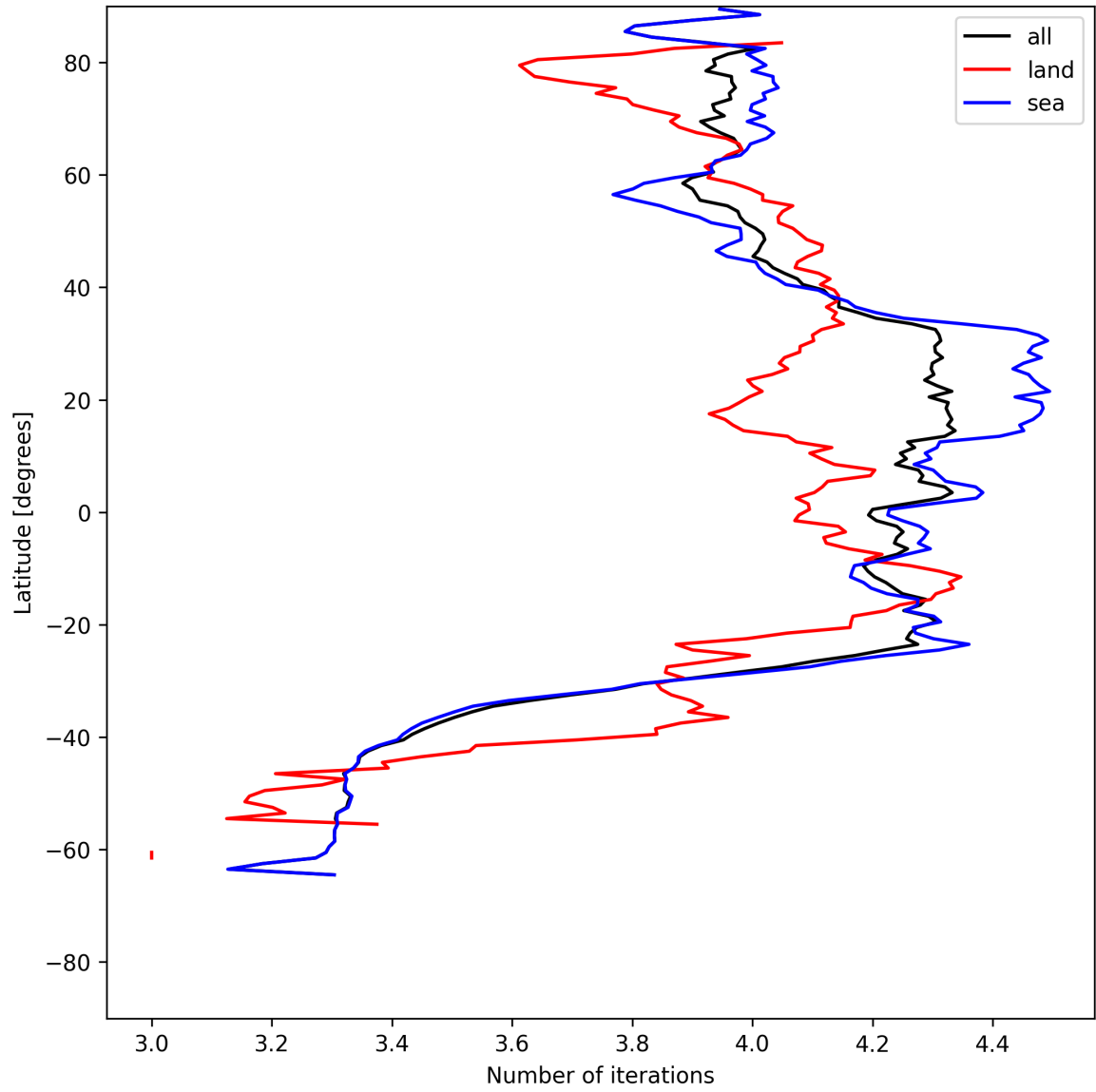
Figure 15: Zonal average of “Number of iterations” for 2025-06-29 to 2025-06-30.
