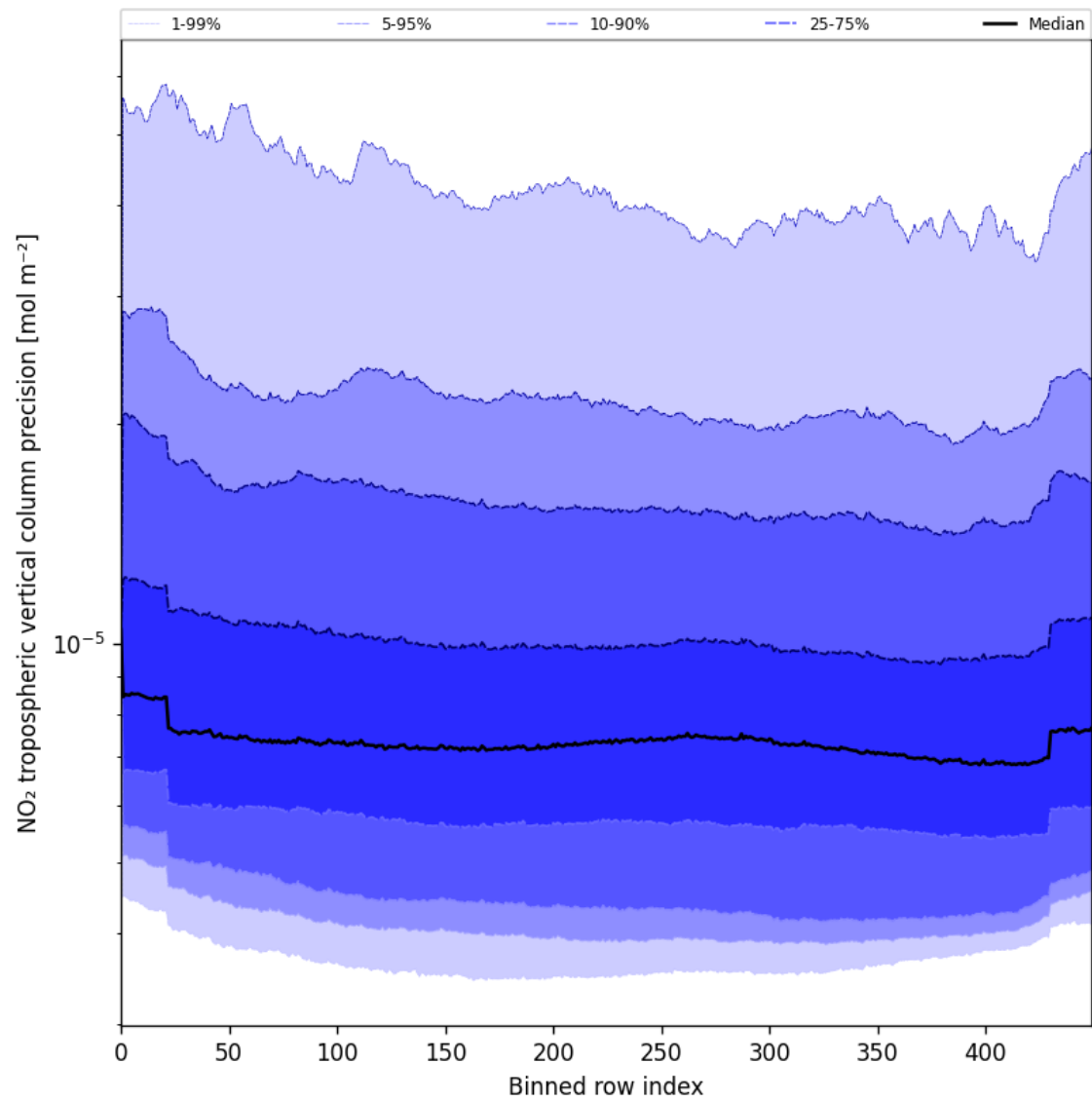
Figure 45: Along track statistics of “NO 2 tropospheric vertical column precision” for 2025-06-29 to 2025-06-30
