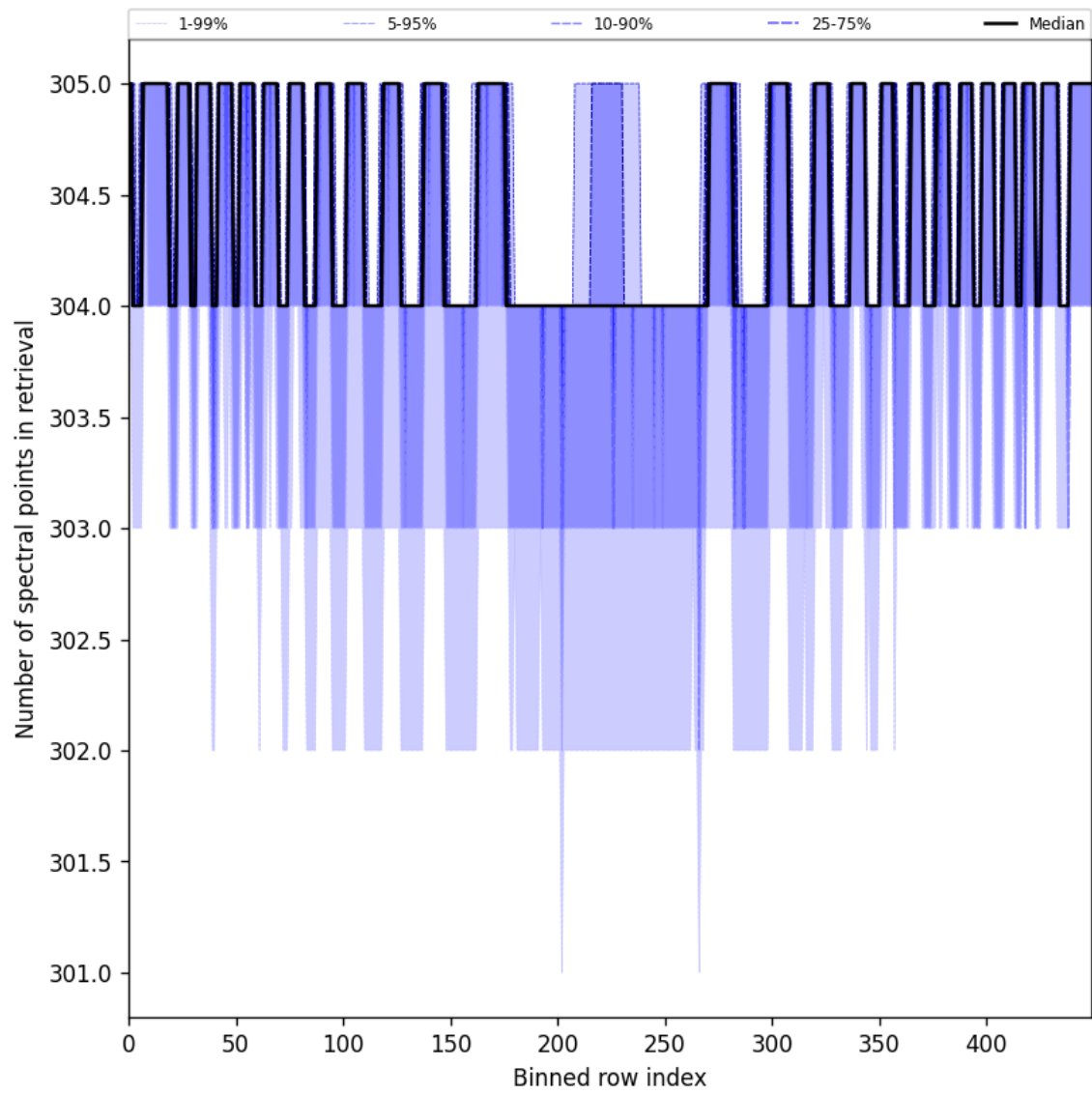
Figure 48: Along track statistics of “Number of spectral points in retrieval” for 2025-06-29 to 2025-06-30
