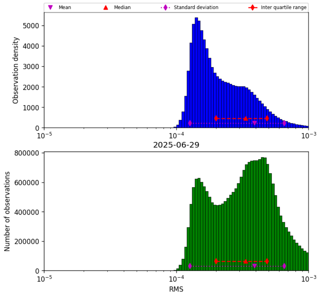
Figure 41: Histogram of “RMS” for 2025-06-29 to 2025-06-30
