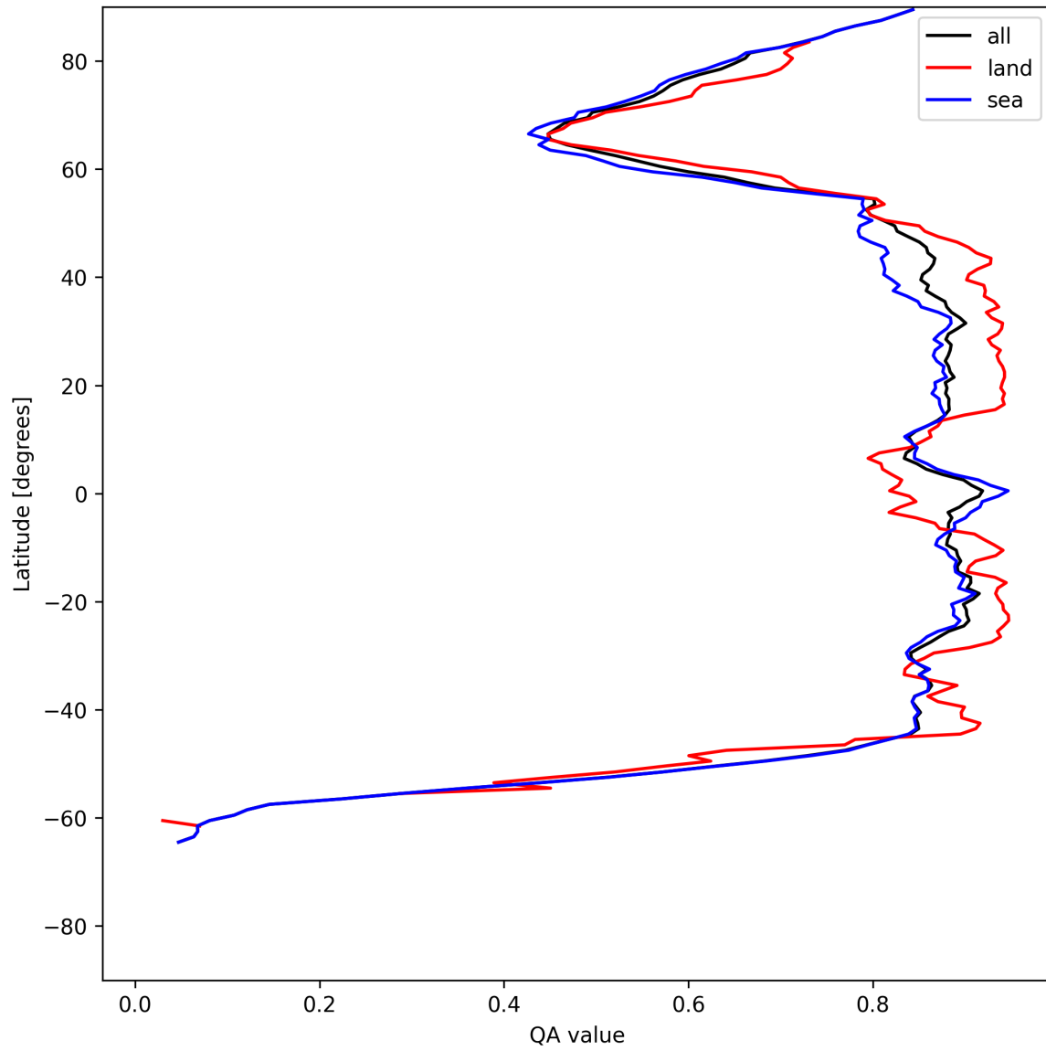
Figure 9: Zonal average of “QA value” for 2025-06-29 to 2025-06-30.
