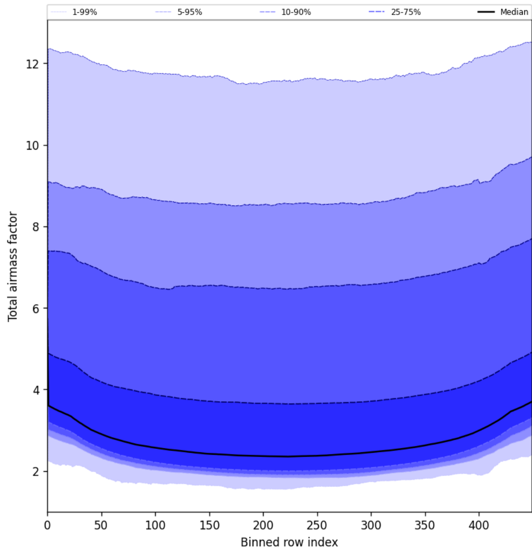
Figure 47: Along track statistics of “Total airmass factor” for 2025-06-29 to 2025-06-30
