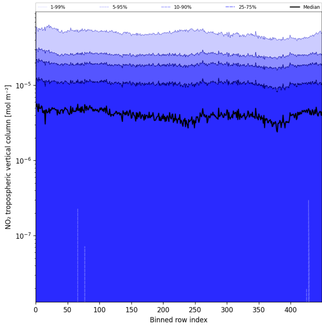
Figure 44: Along track statistics of “NO 2 tropospheric vertical column” for 2025-06-29 to 2025-06-30
