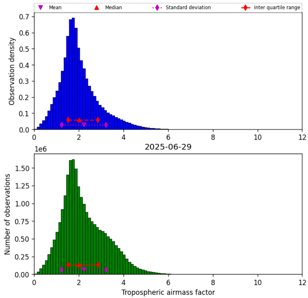
Figure 29: Histogram of “Tropospheric airmass factor” for 2025-06-29 to 2025-06-30
