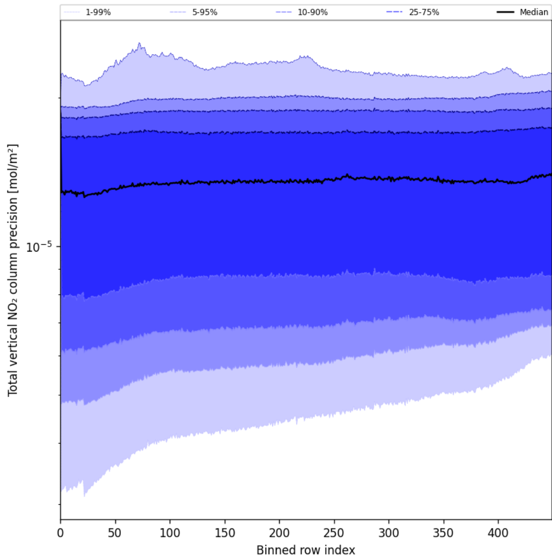
Figure 54: Along track statistics of “Total vertical NO 2 column precision” for 2025-06-29 to 2025-06-30
