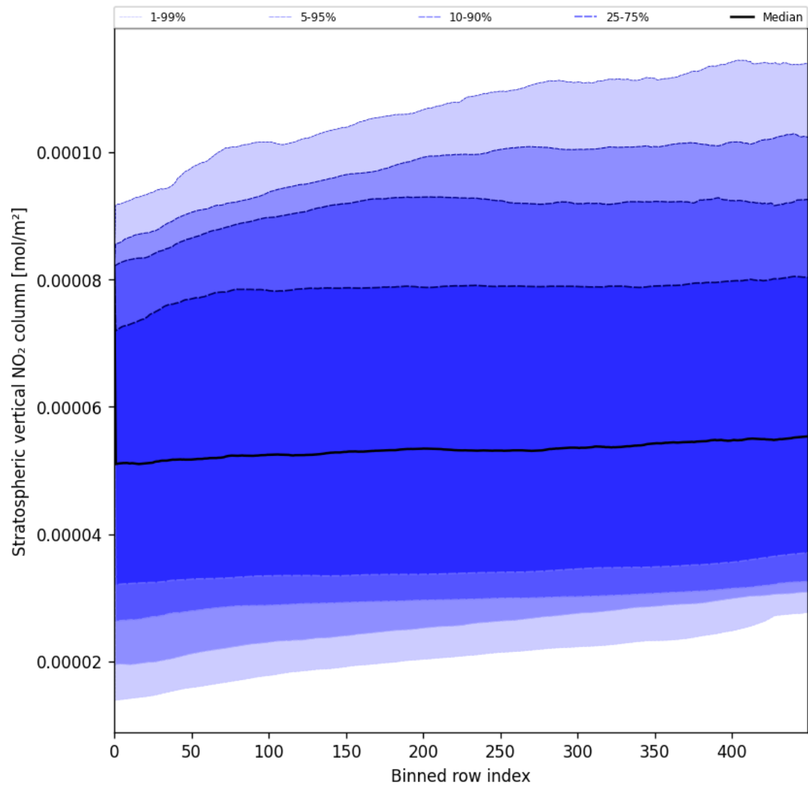
Figure 51: Along track statistics of “Stratospheric vertical NO 2 column” for 2025-06-30 to 2025-06-30
