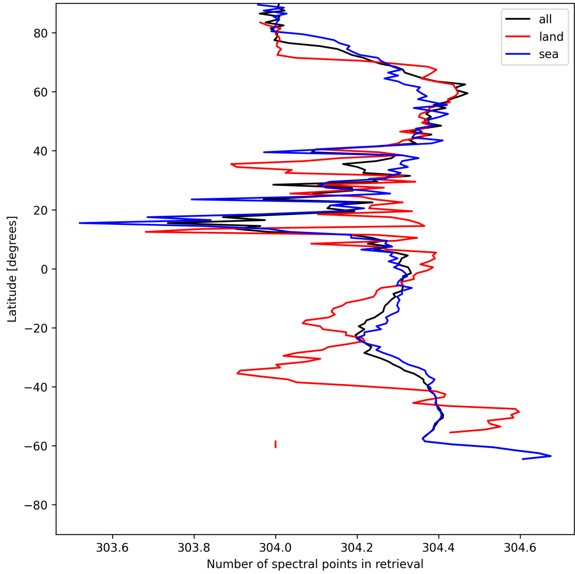
Figure 14: Zonal average of “Number of spectral points in retrieval” for 2025-06-30 to 2025-06-30.
