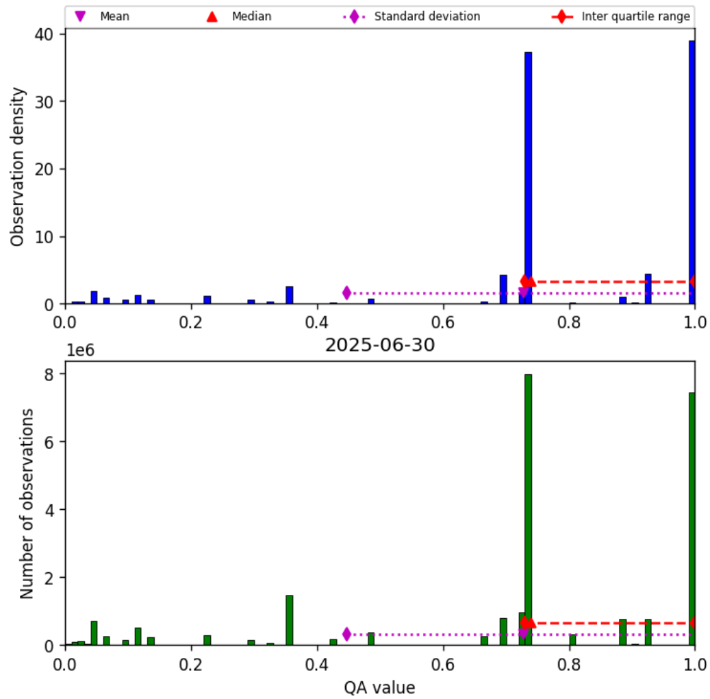
Figure 26: Histogram of “QA value” for 2025-06-30 to 2025-06-30
