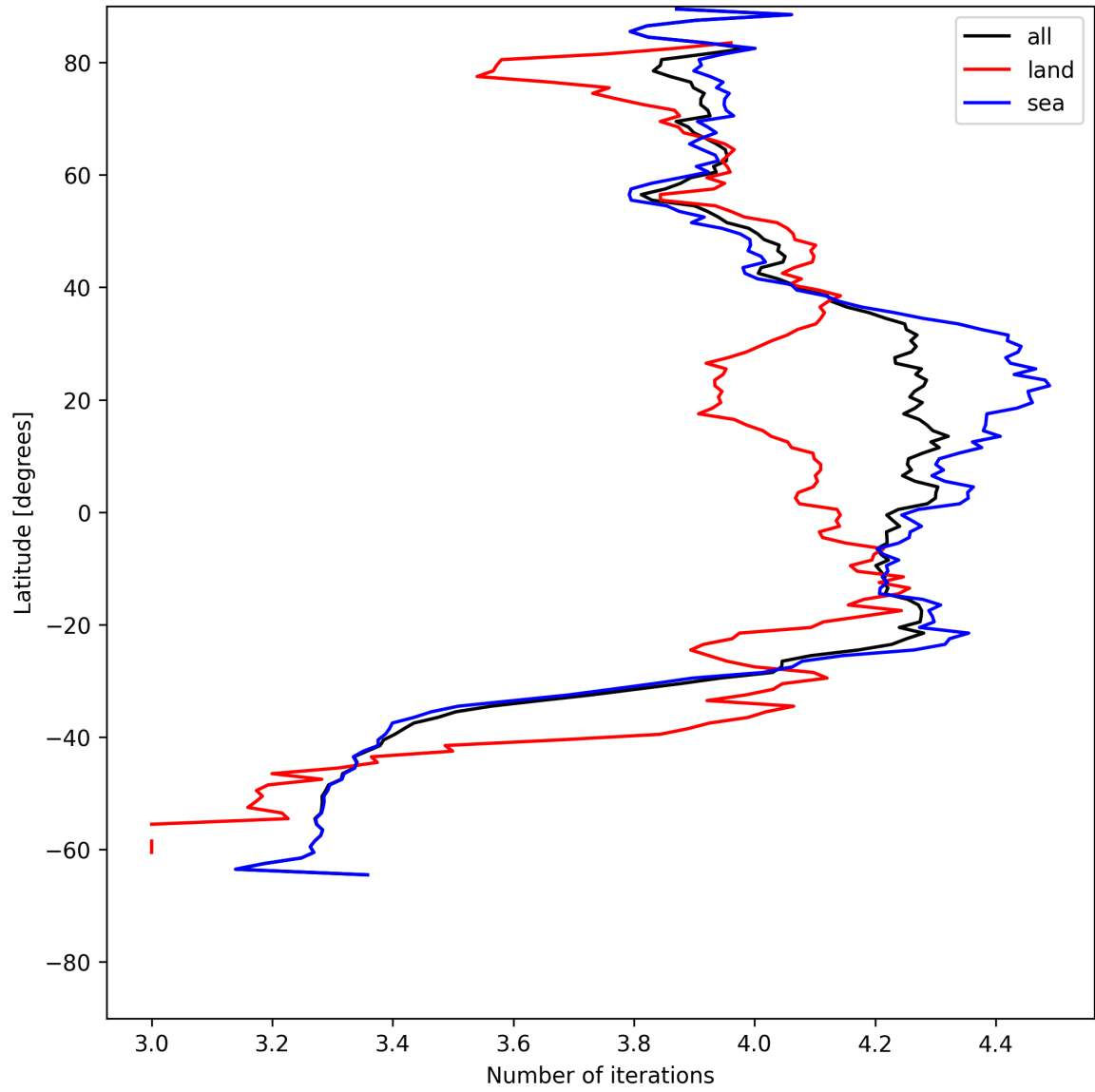
Figure 15: Zonal average of “Number of iterations” for 2025-06-30 to 2025-06-30.
