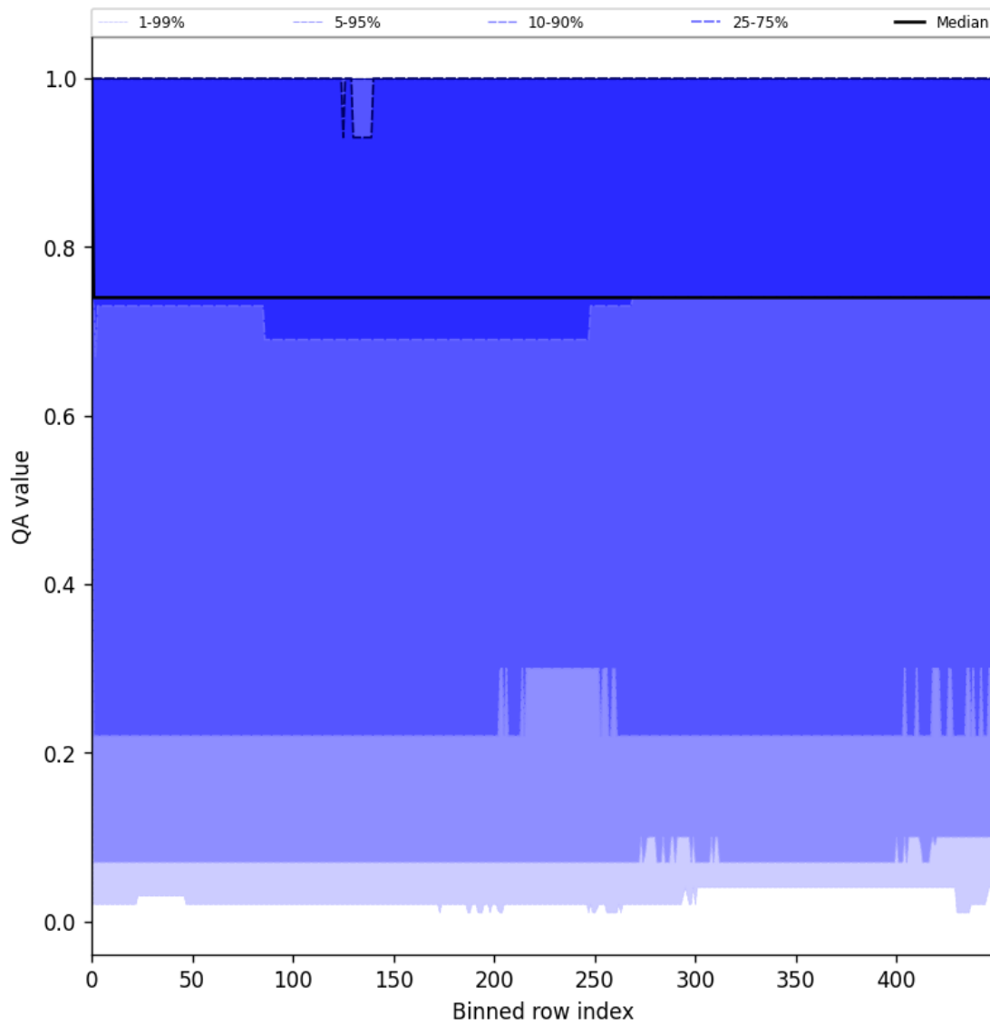
Figure 43: Along track statistics of “QA value” for 2025-06-30 to 2025-06-30
