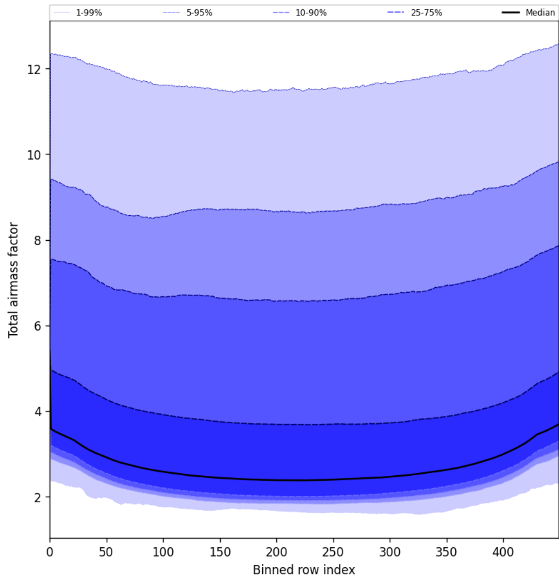
Figure 47: Along track statistics of “Total airmass factor” for 2025-06-30 to 2025-06-30
