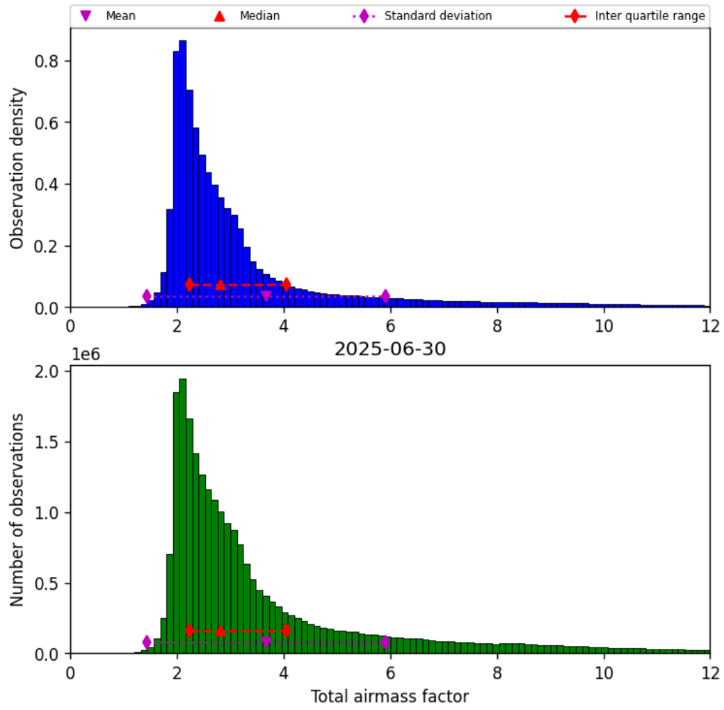
Figure 30: Histogram of “Total airmass factor” for 2025-06-30 to 2025-06-30
