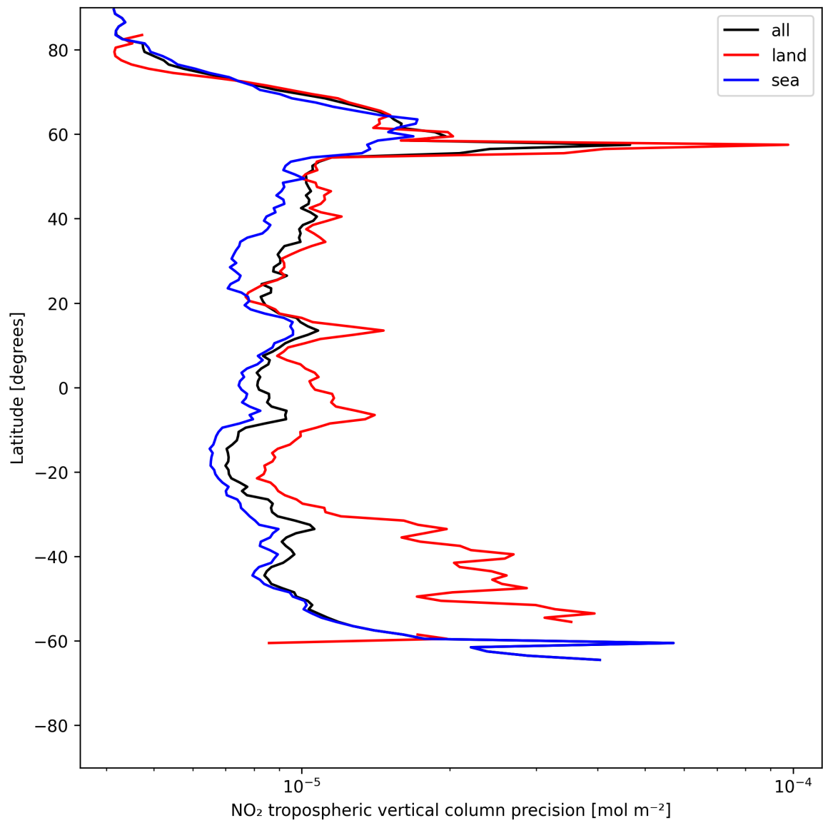
Figure 11: Zonal average of “NO 2 tropospheric vertical column precision” for 2025-06-30 to 2025-06-30.
