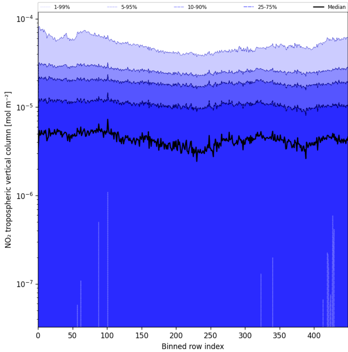
Figure 44: Along track statistics of "NO 2 tropospheric vertical column" for 2025-06-30 to 2025-06-30
