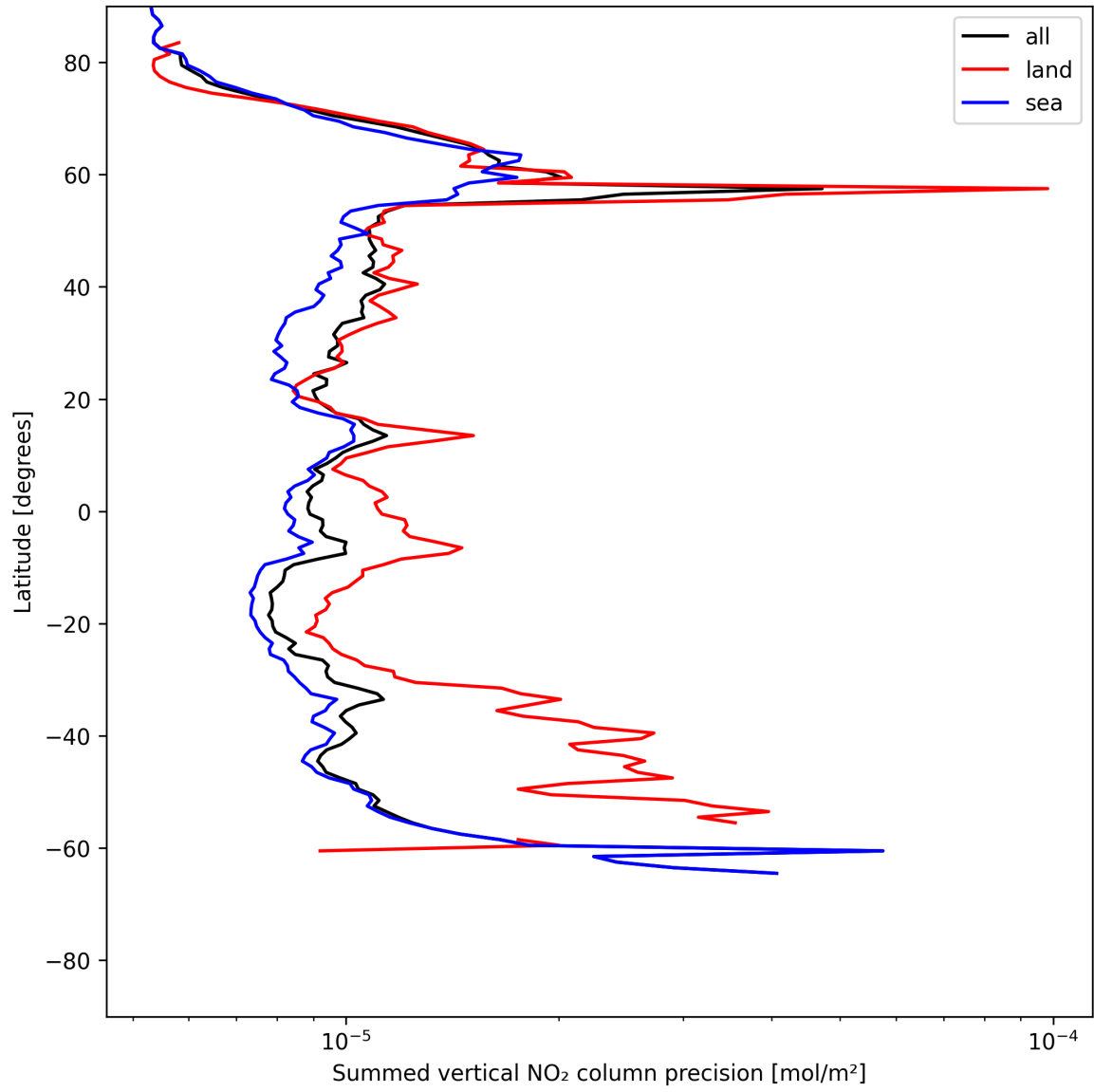
Figure 22: Zonal average of “Summed vertical NO 2 column precision” for 2025-06-30 to 2025-06-30.
