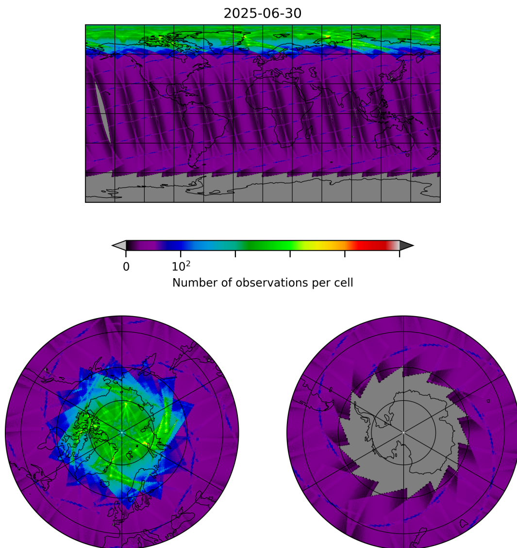
Figure 8: Map of the number of observations for 2025-06-30 to 2025-06-30
