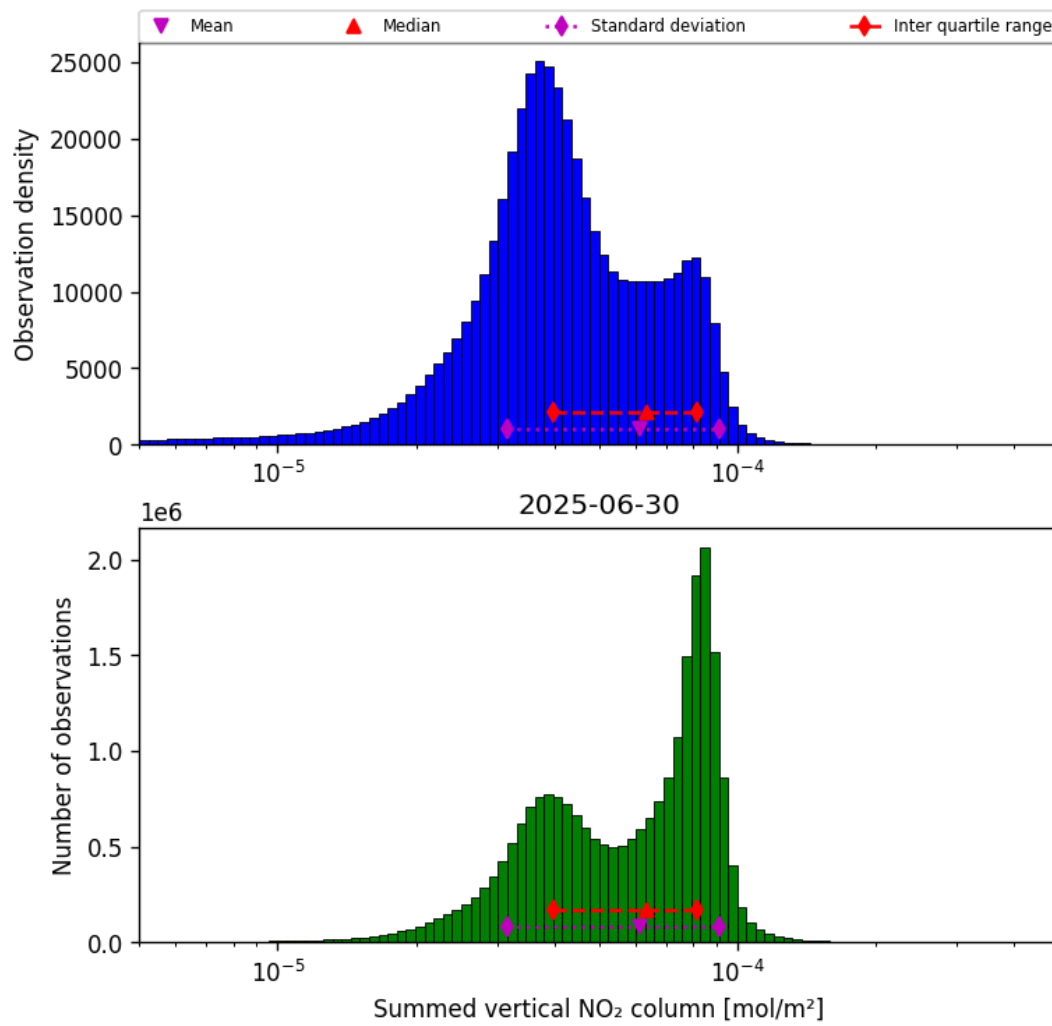
Figure 38: Histogram of “Summed vertical NO 2 column” for 2025-06-30 to 2025-06-30
