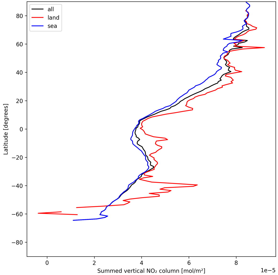
Figure 21: Zonal average of “Summed vertical NO 2 column” for 2025-06-30 to 2025-06-30.
