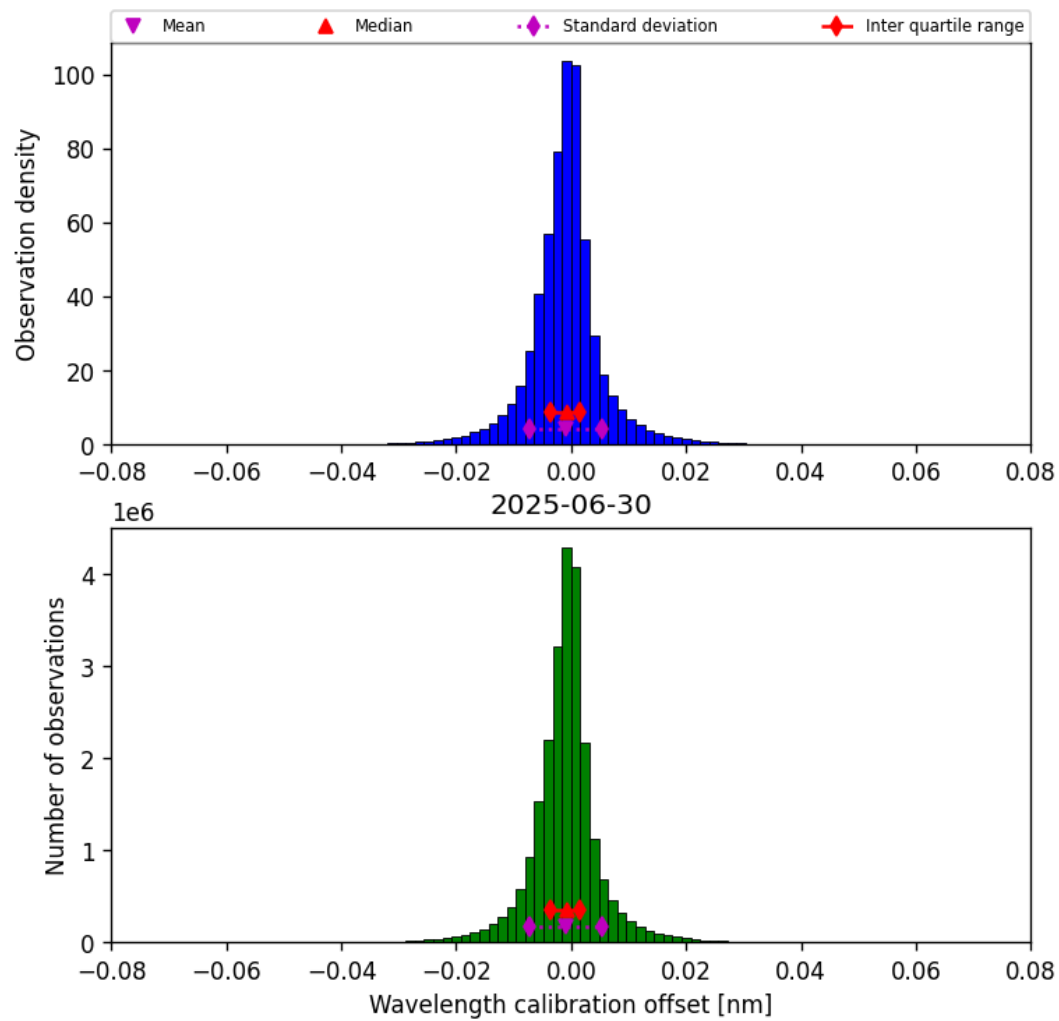
Figure 33: Histogram of “Wavelength calibration offset” for 2025-06-30 to 2025-06-30
