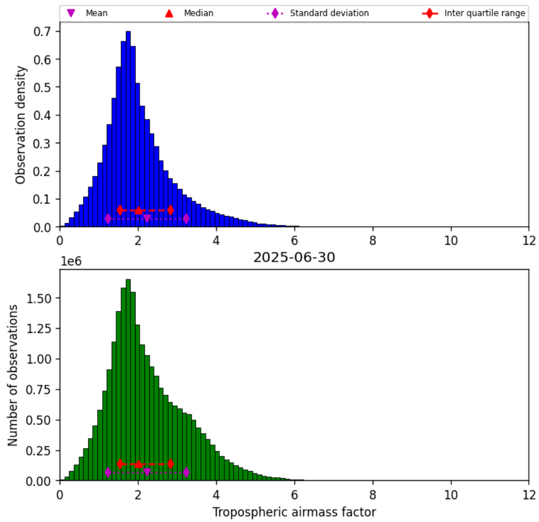
Figure 29: Histogram of “Tropospheric airmass factor” for 2025-06-30 to 2025-06-30
