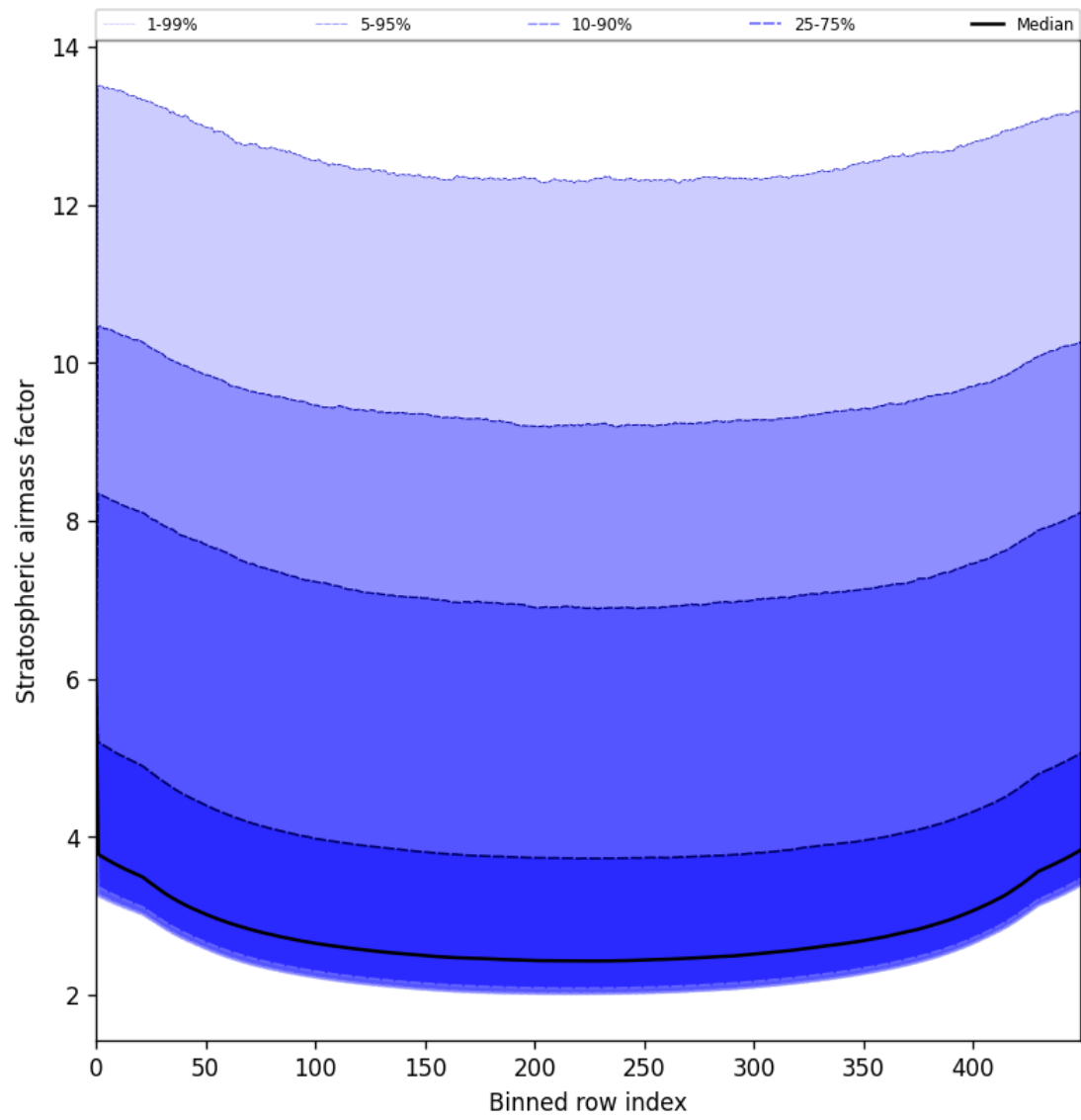
Figure 59: Along track statistics of “Stratospheric airmass factor” for 2025-06-30 to 2025-06-30
