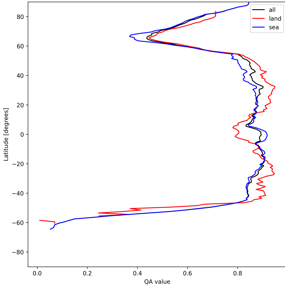
Figure 9: Zonal average of “QA value” for 2025-06-30 to 2025-06-30.
