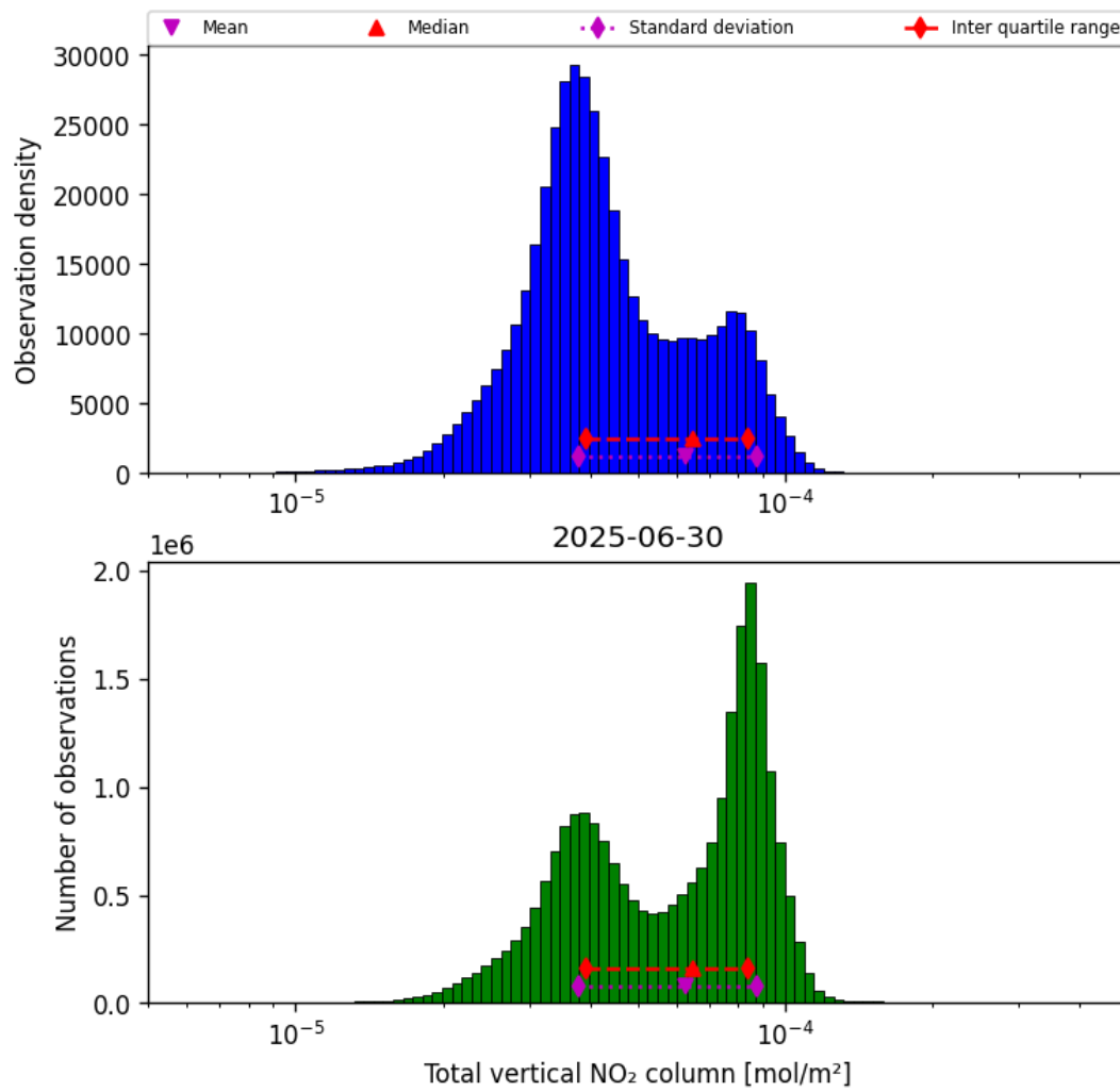
Figure 36: Histogram of "Total vertical NO 2 column" for 2025-06-30 to 2025-06-30
