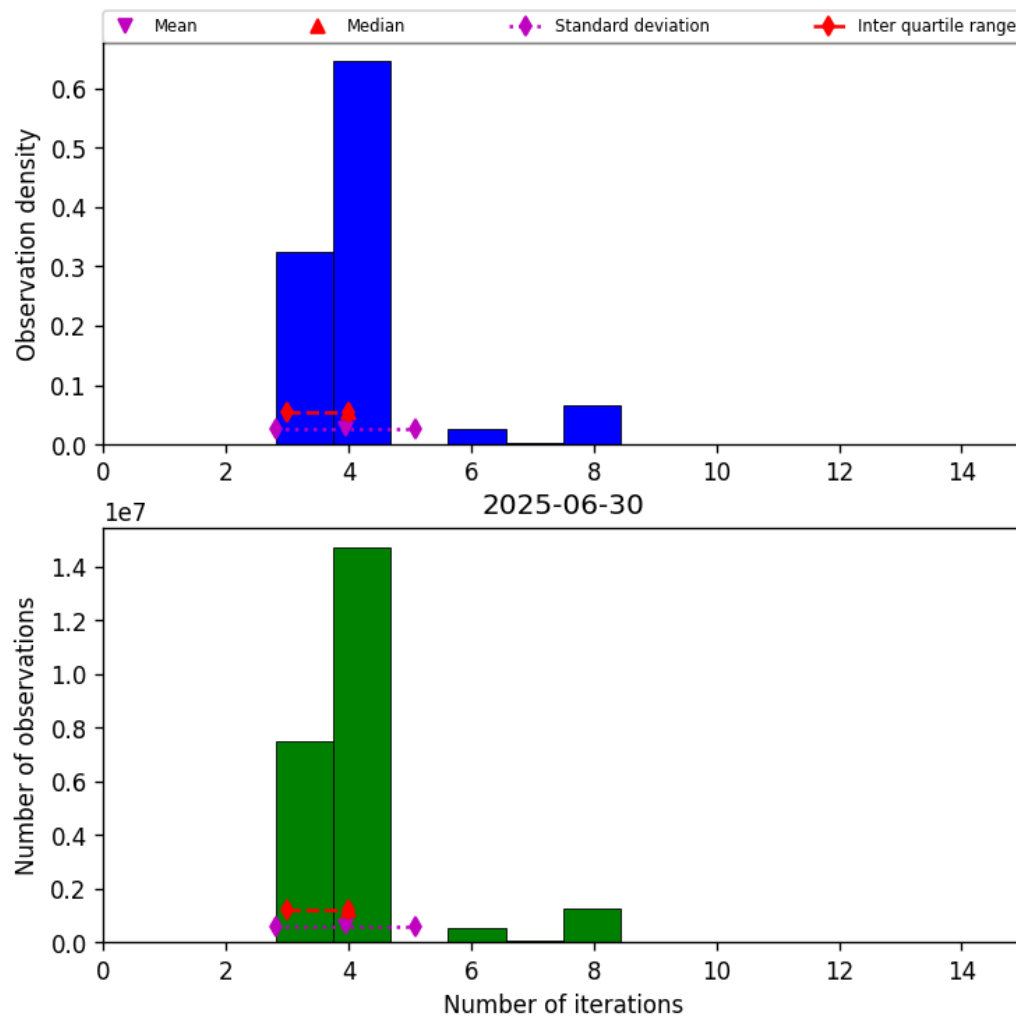
Figure 32: Histogram of “Number of iterations” for 2025-06-30 to 2025-06-30
