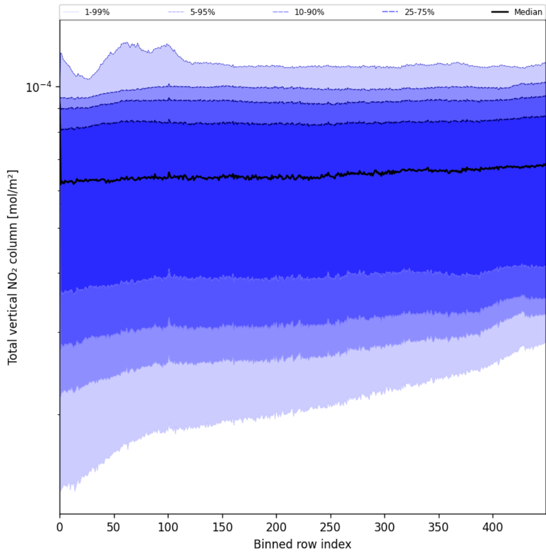
Figure 53: Along track statistics of “Total vertical NO 2 column” for 2025-06-30 to 2025-06-30
