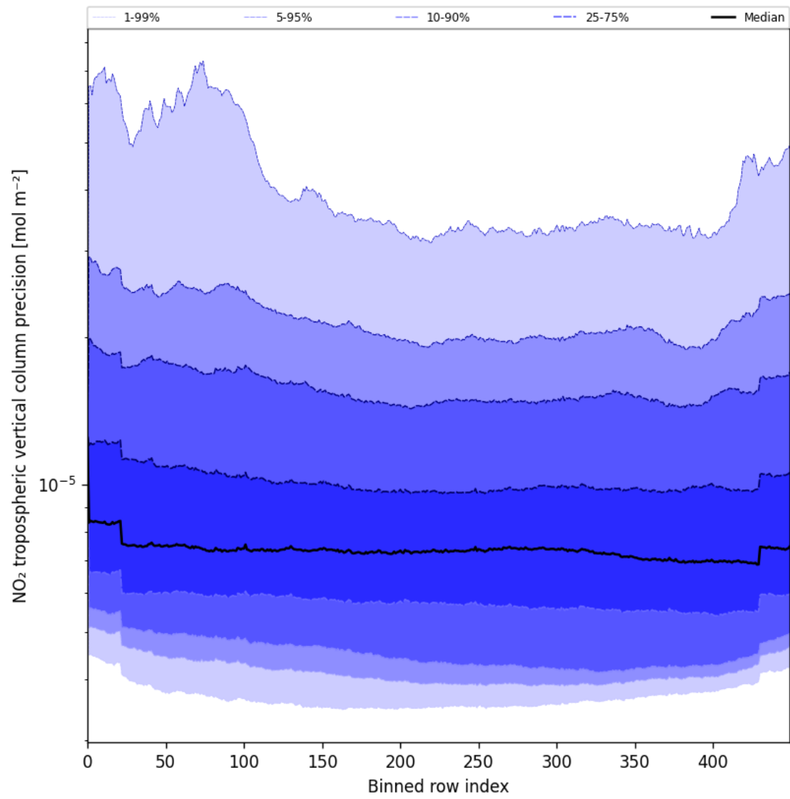
Figure 45: Along track statistics of “NO 2 tropospheric vertical column precision” for 2025-06-30 to 2025-06-30
