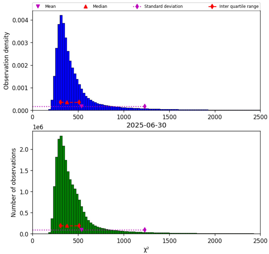
Figure 40: Histogram of “ \chi^2 ” for 2025-06-30 to 2025-06-30
