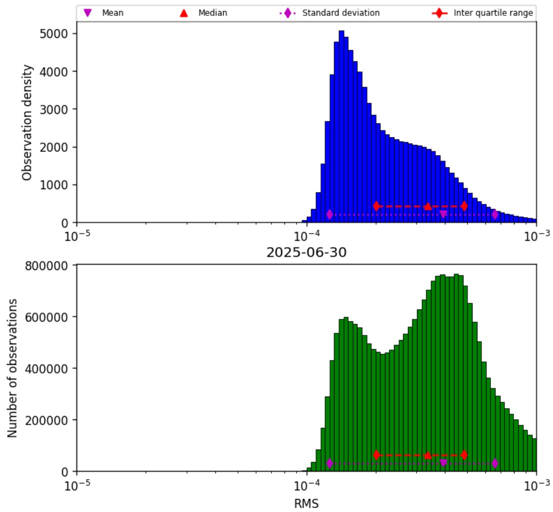
Figure 41: Histogram of “RMS” for 2025-06-30 to 2025-06-30
