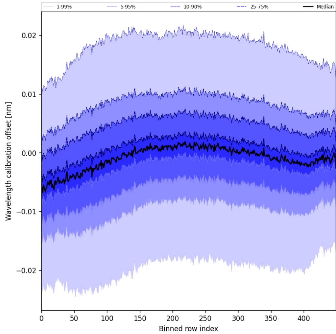
Figure 50: Along track statistics of “Wavelength calibration offset” for 2025-06-30 to 2025-06-30
