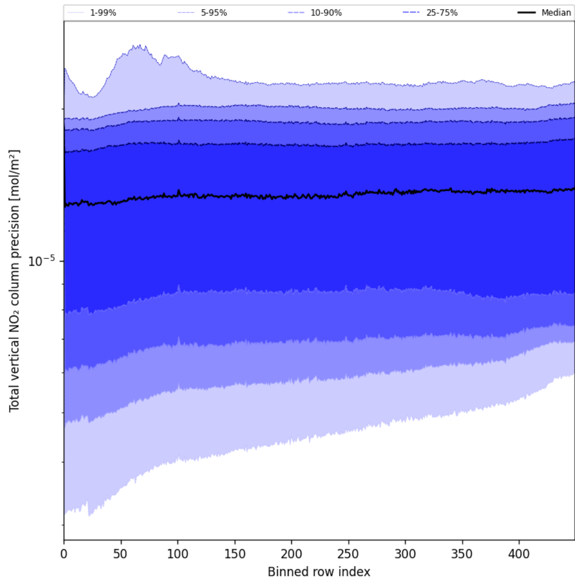
Figure 54: Along track statistics of “Total vertical NO 2 column precision” for 2025-06-30 to 2025-06-30
