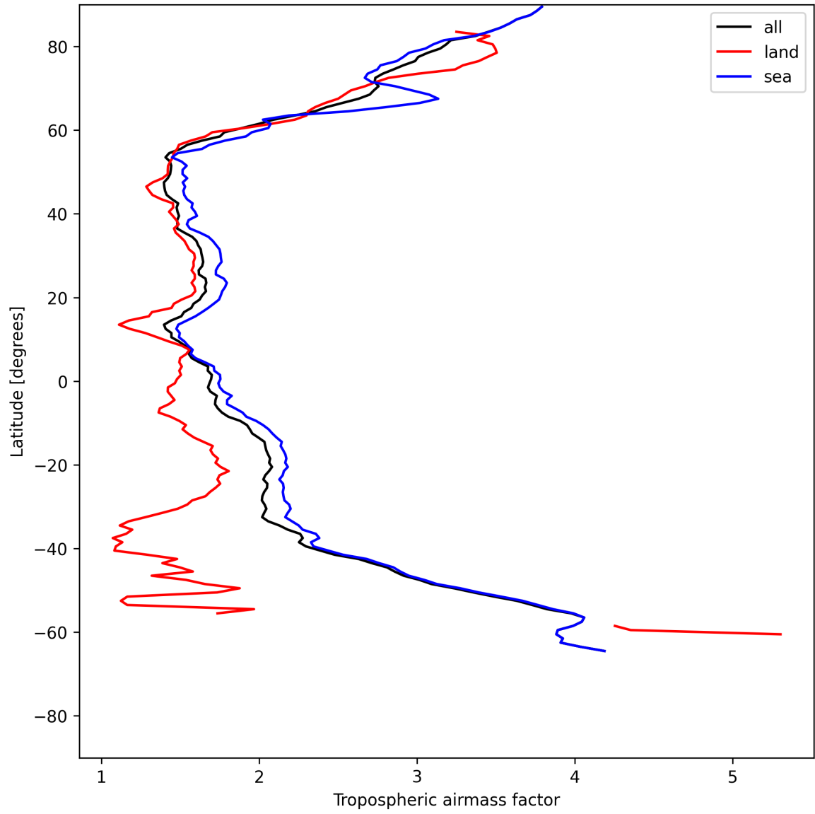
Figure 12: Zonal average of “Tropospheric airmass factor” for 2025-06-30 to 2025-06-30.
