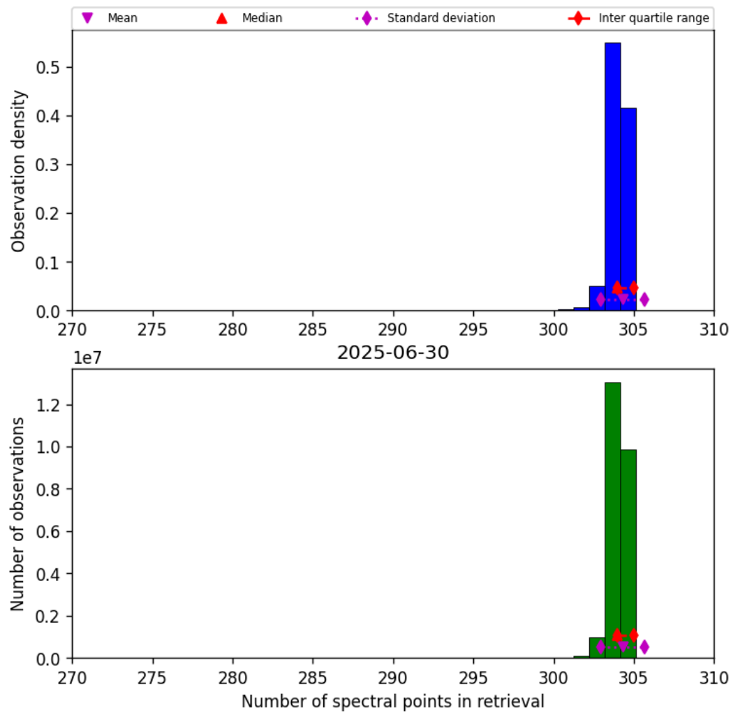
Figure 31: Histogram of “Number of spectral points in retrieval” for 2025-06-30 to 2025-06-30
