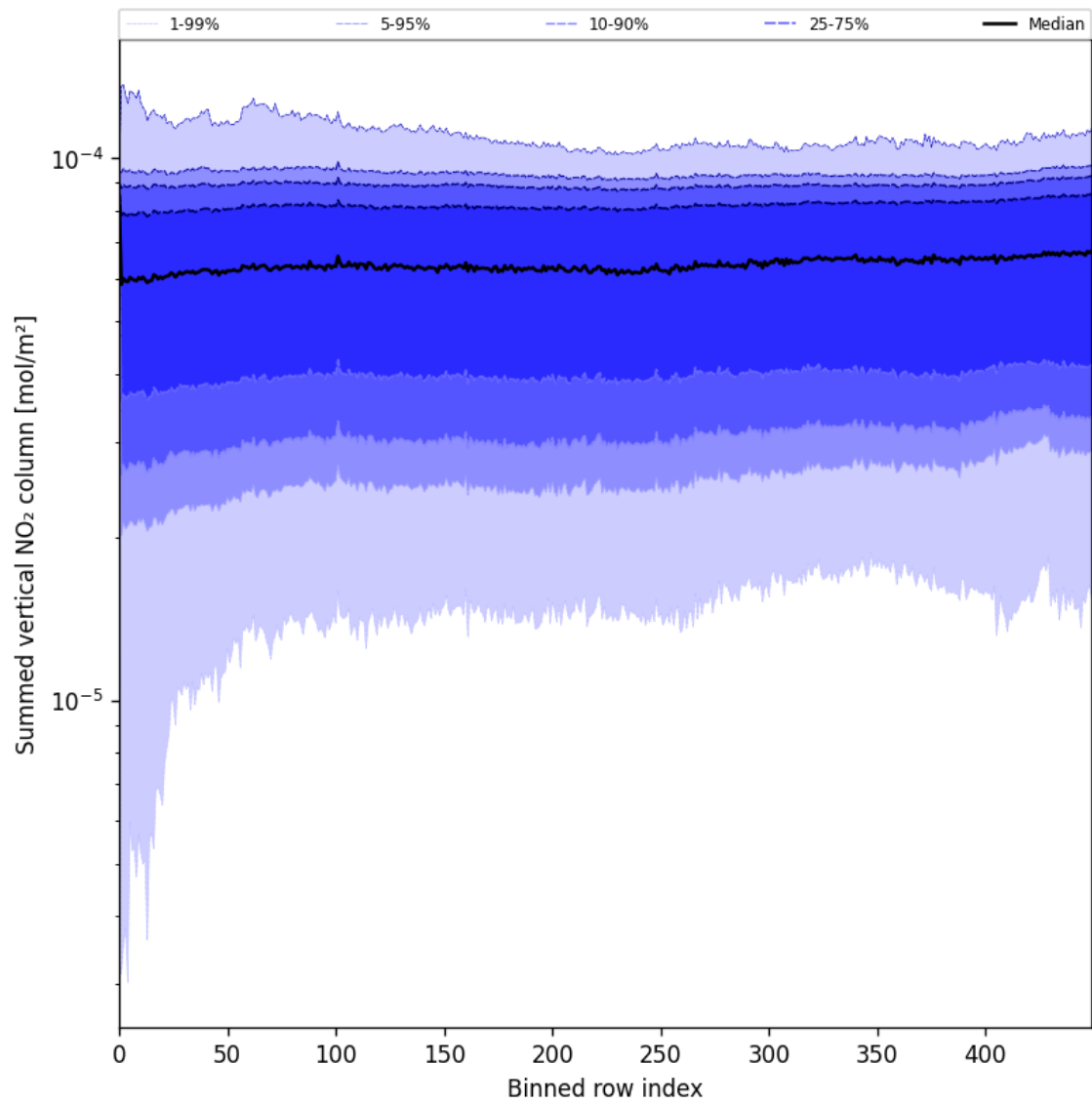
Figure 55: Along track statistics of “Summed vertical NO 2 column” for 2025-06-30 to 2025-06-30
