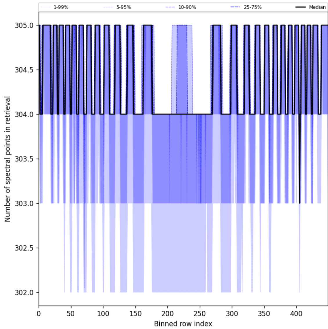
Figure 48: Along track statistics of “Number of spectral points in retrieval” for 2025-06-30 to 2025-06-30
