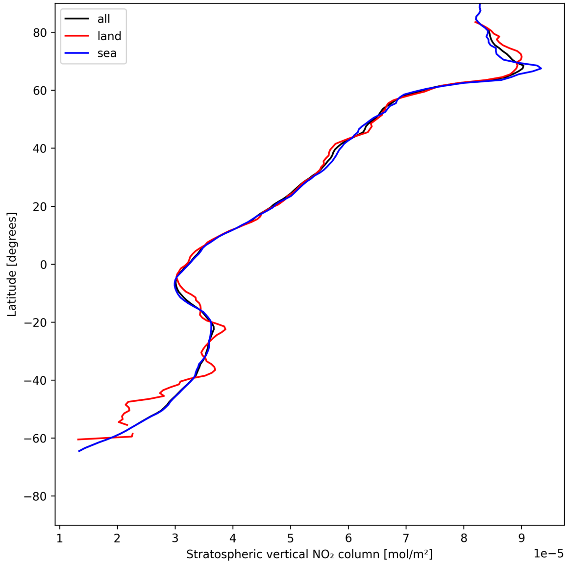
Figure 17: Zonal average of “Stratospheric vertical NO 2 column” for 2025-06-30 to 2025-06-30.
