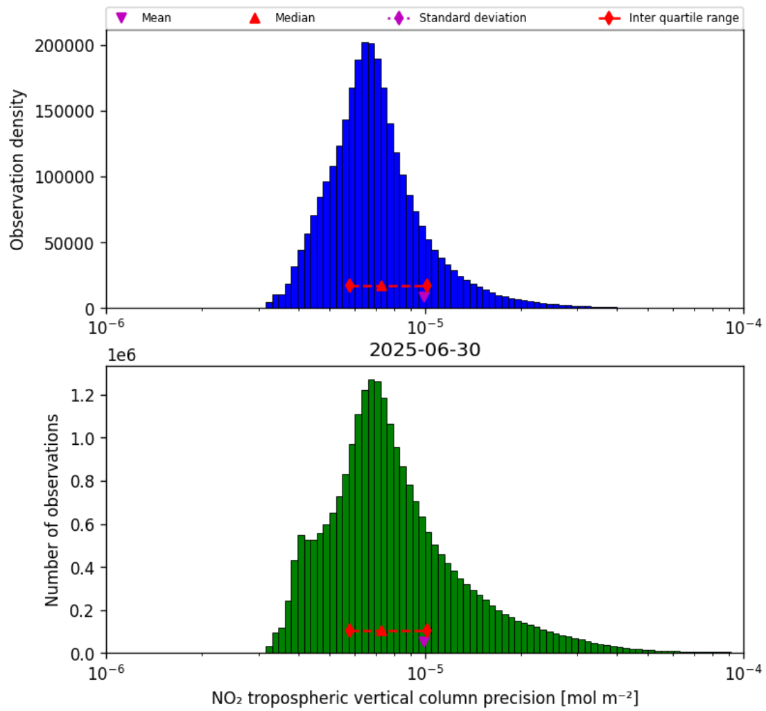
Figure 28: Histogram of "NO 2 tropospheric vertical column precision" for 2025-06-30 to 2025-06-30
