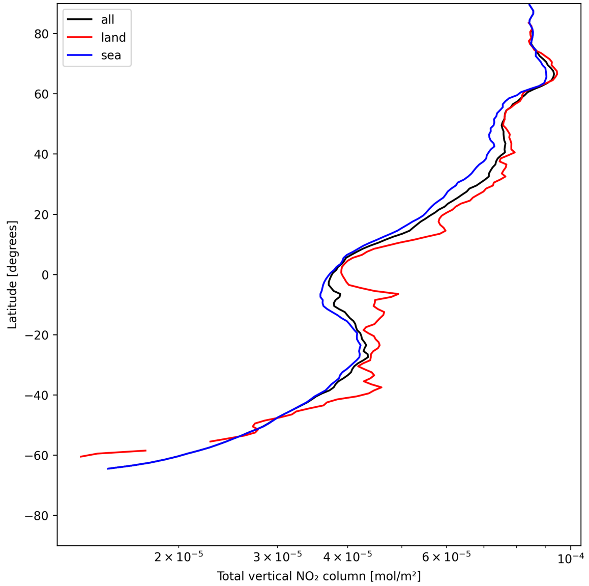
Figure 19: Zonal average of “Total vertical NO 2 column” for 2025-06-30 to 2025-06-30.
