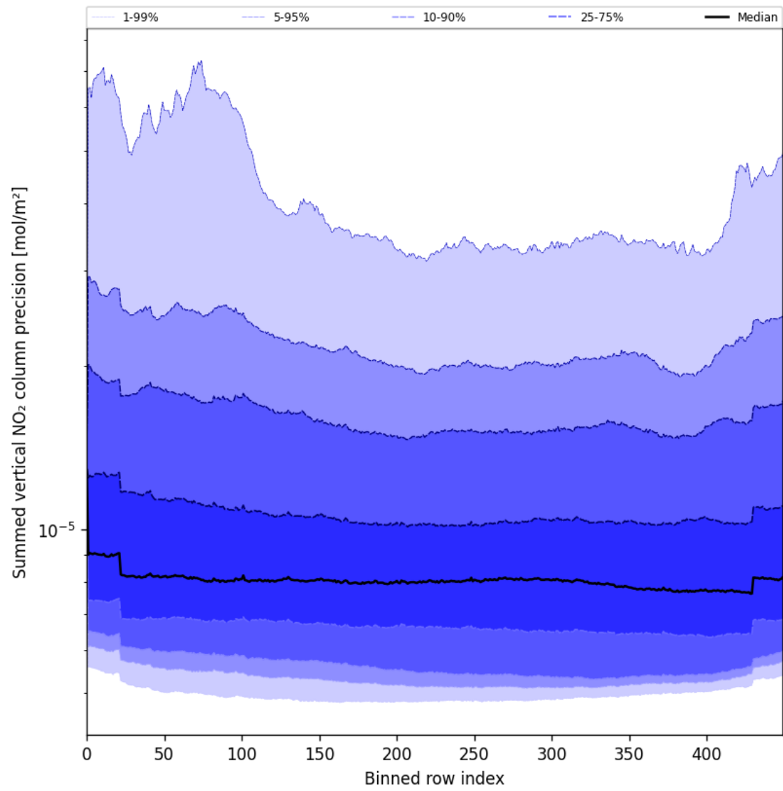
Figure 56: Along track statistics of “Summed vertical NO 2 column precision” for 2025-06-30 to 2025-06-30
