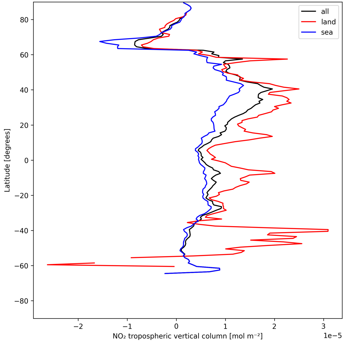
Figure 10: Zonal average of “NO 2 tropospheric vertical column” for 2025-06-30 to 2025-06-30.
