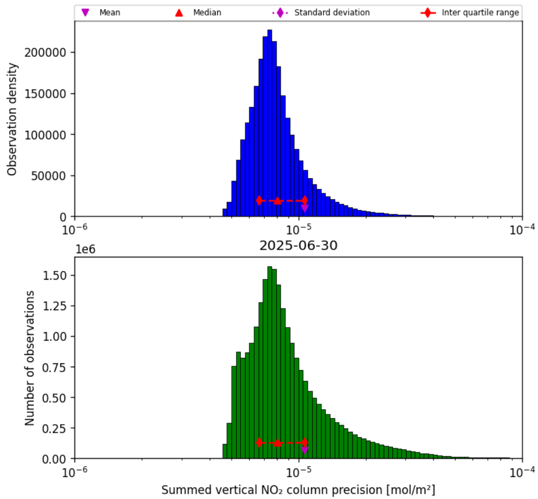
Figure 39: Histogram of "Summed vertical NO 2 column precision" for 2025-06-30 to 2025-06-30
