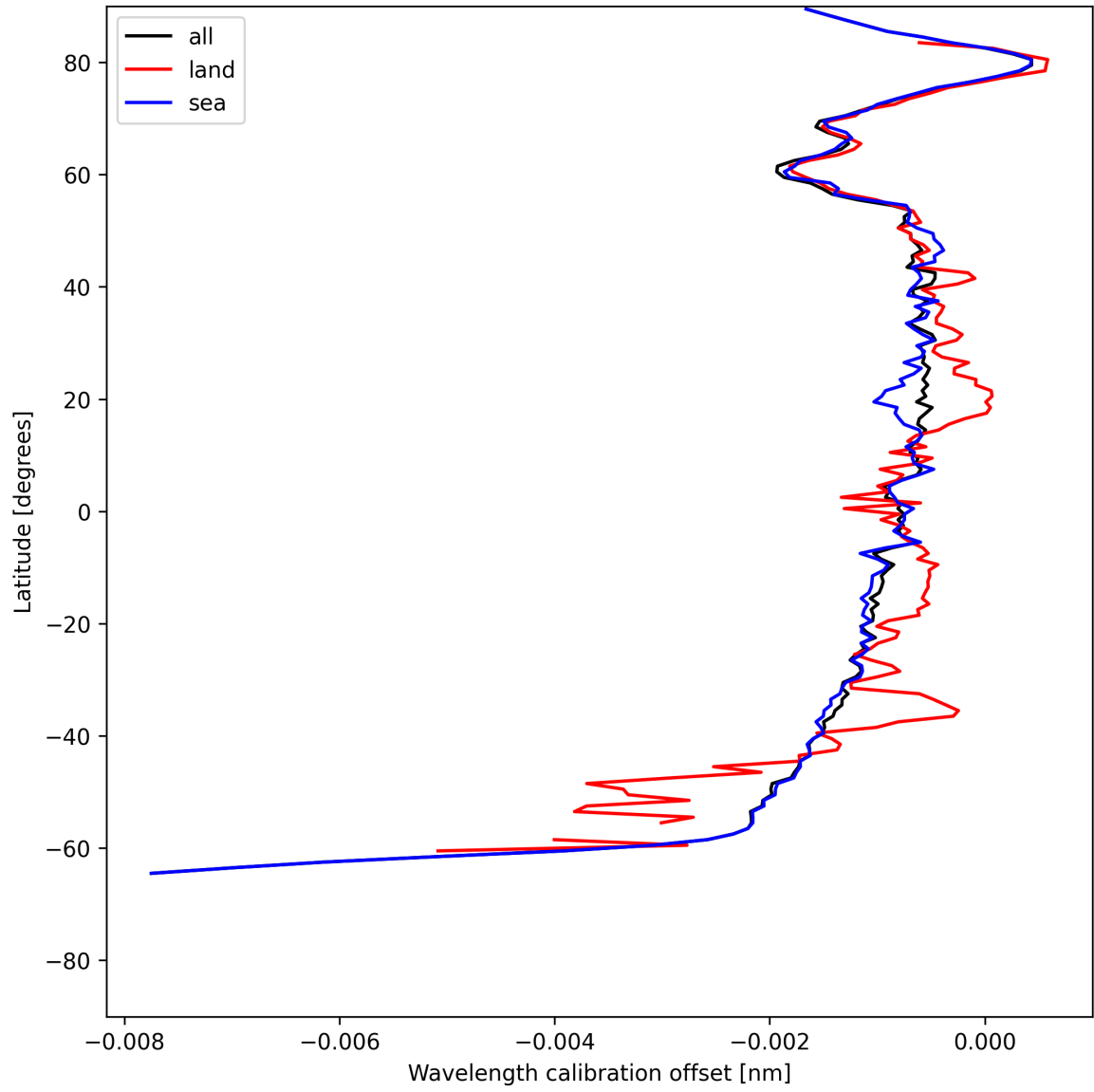
Figure 16: Zonal average of “Wavelength calibration offset” for 2025-06-30 to 2025-06-30.
