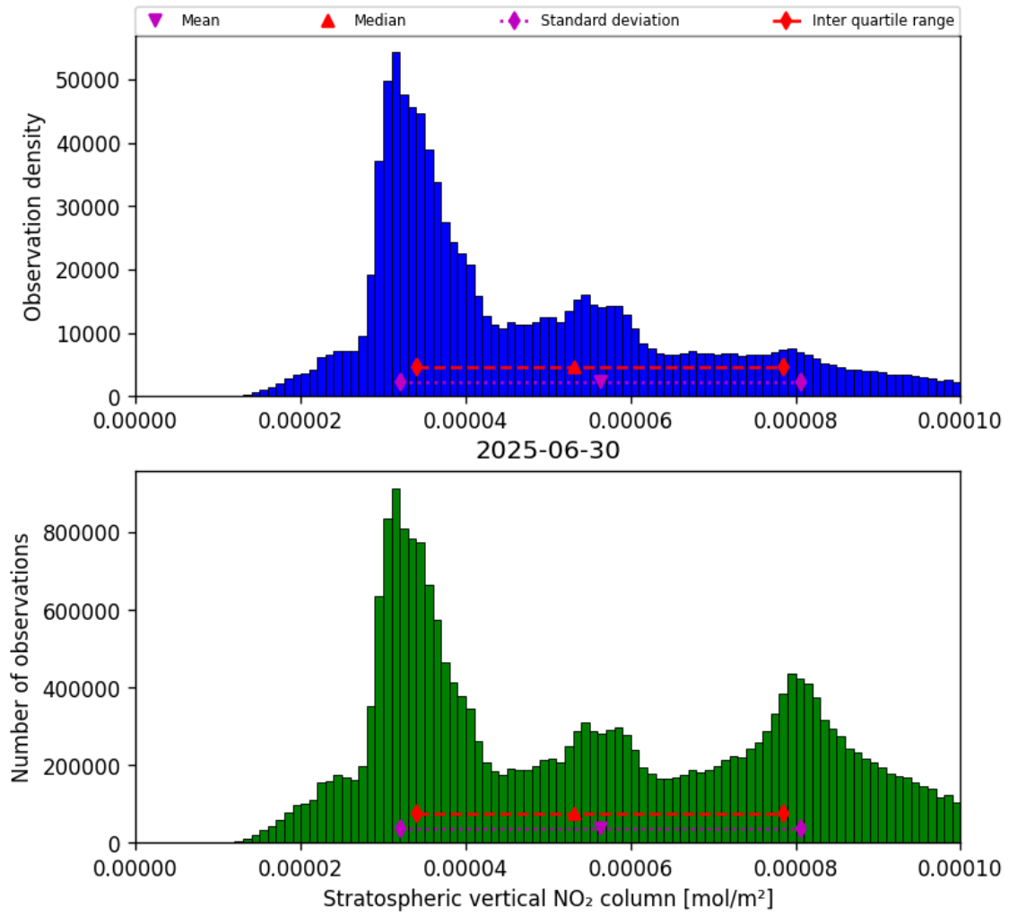
Figure 34: Histogram of “Stratospheric vertical NO 2 column” for 2025-06-30 to 2025-06-30
