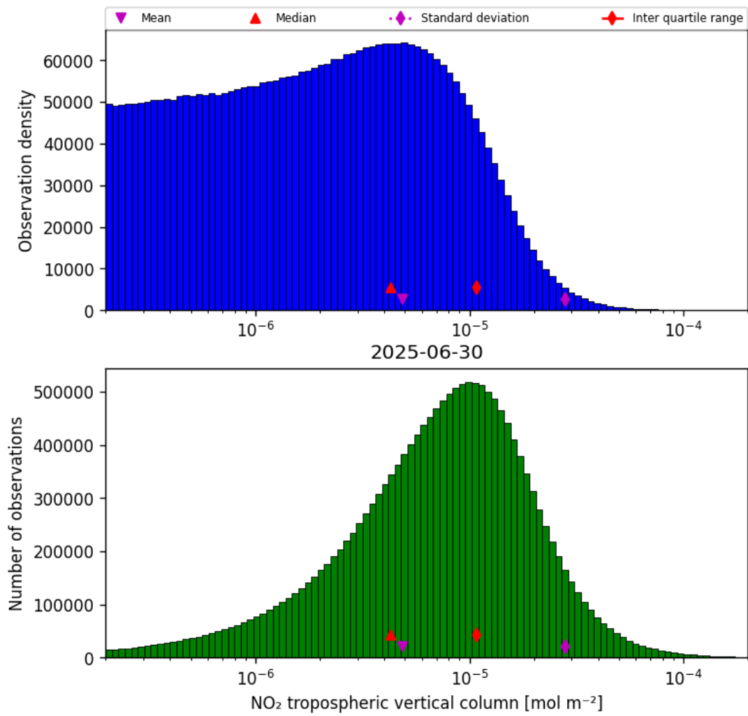
Figure 27: Histogram of “NO 2 tropospheric vertical column” for 2025-06-30 to 2025-06-30
