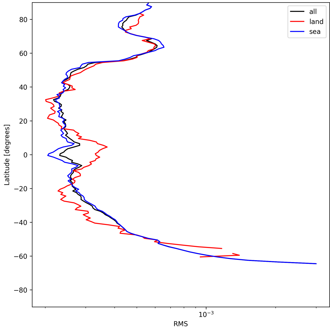
Figure 24: Zonal average of “RMS” for 2025-06-30 to 2025-06-30.
