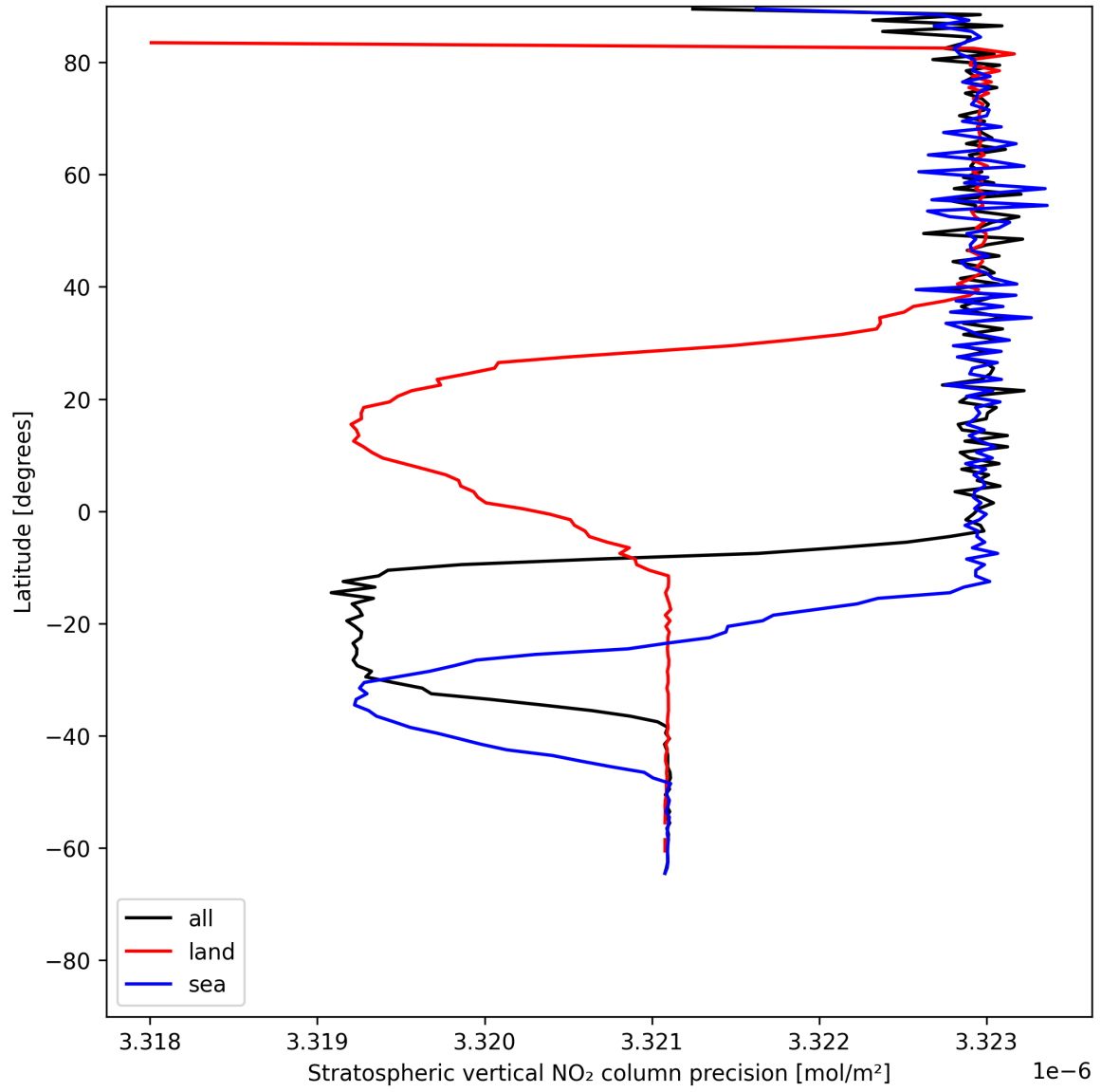
Figure 18: Zonal average of “Stratospheric vertical NO 2 column precision” for 2025-06-30 to 2025-06-30.
