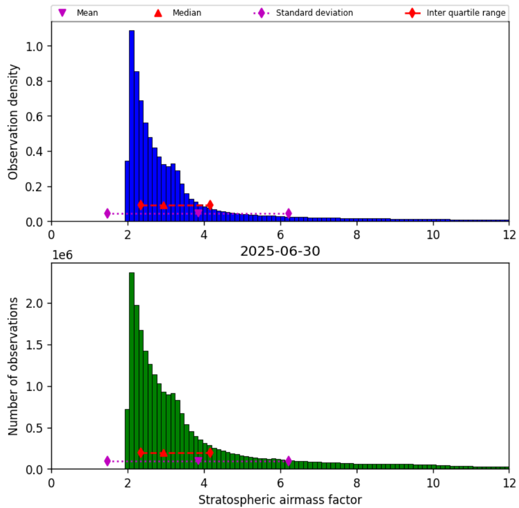
Figure 42: Histogram of “Stratospheric airmass factor” for 2025-06-30 to 2025-06-30
