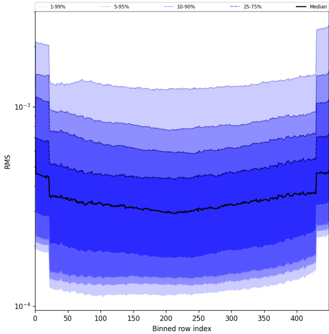
Figure 58: Along track statistics of “RMS” for 2025-06-30 to 2025-06-30
