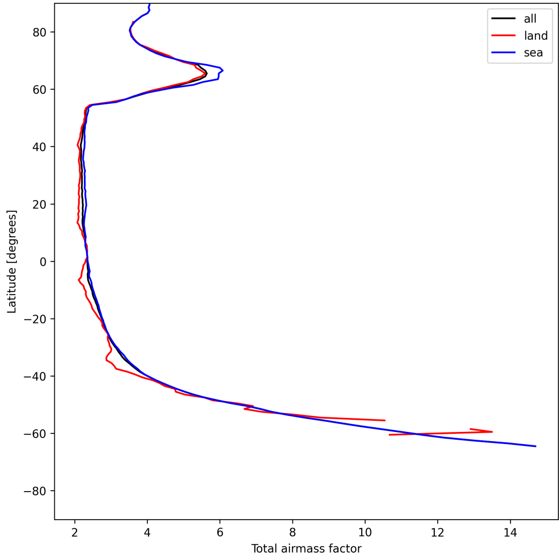
Figure 13: Zonal average of “Total airmass factor” for 2025-06-30 to 2025-06-30.
