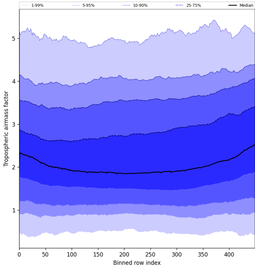
Figure 46: Along track statistics of “Tropospheric airmass factor” for 2025-06-30 to 2025-06-30
