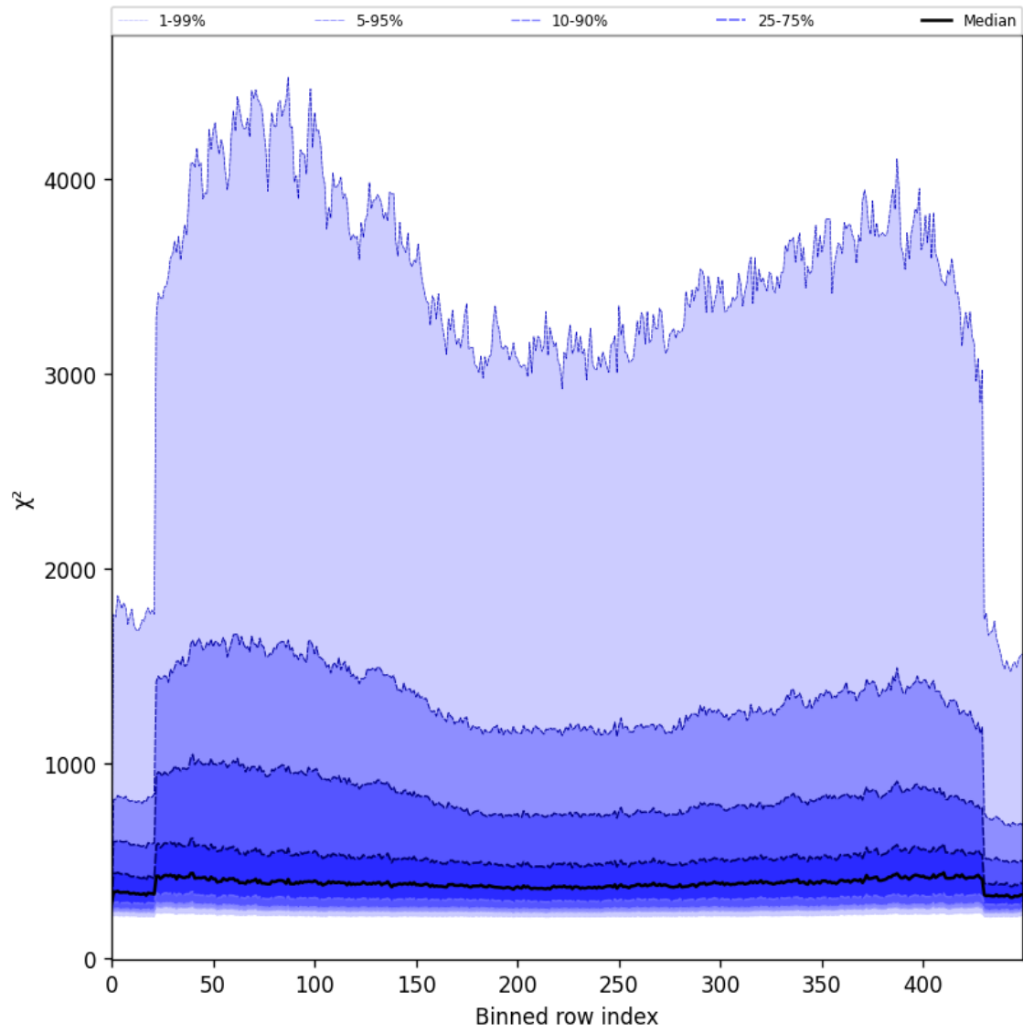
Figure 57: Along track statistics of “ \chi^2 ” for 2025-06-30 to 2025-06-30
