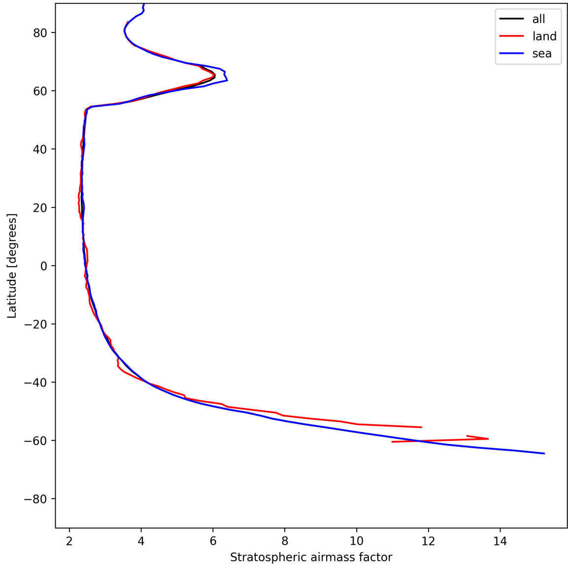
Figure 25: Zonal average of “Stratospheric air mass factor” for 2025-06-30 to 2025-06-30.
