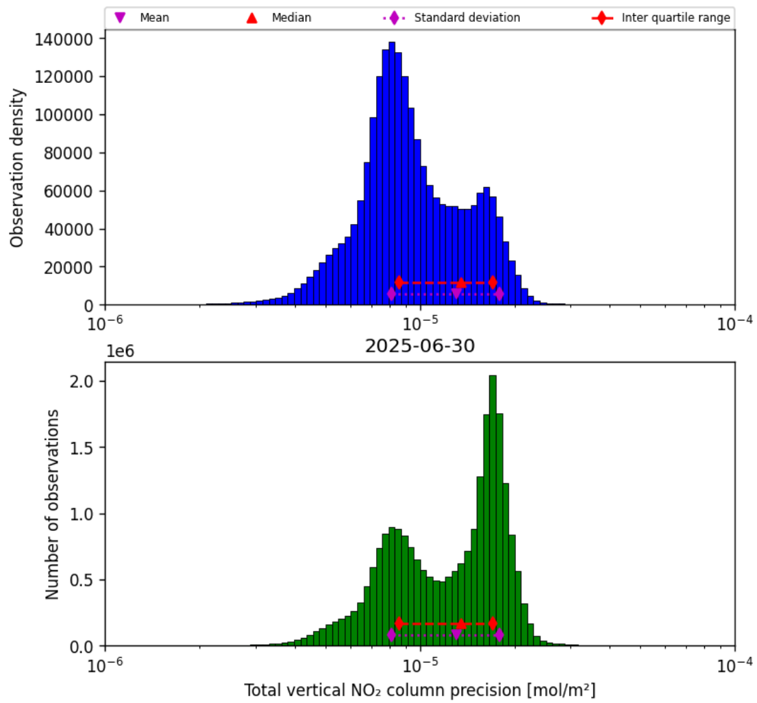
Figure 37: Histogram of "Total vertical NO 2 column precision" for 2025-06-30 to 2025-06-30
