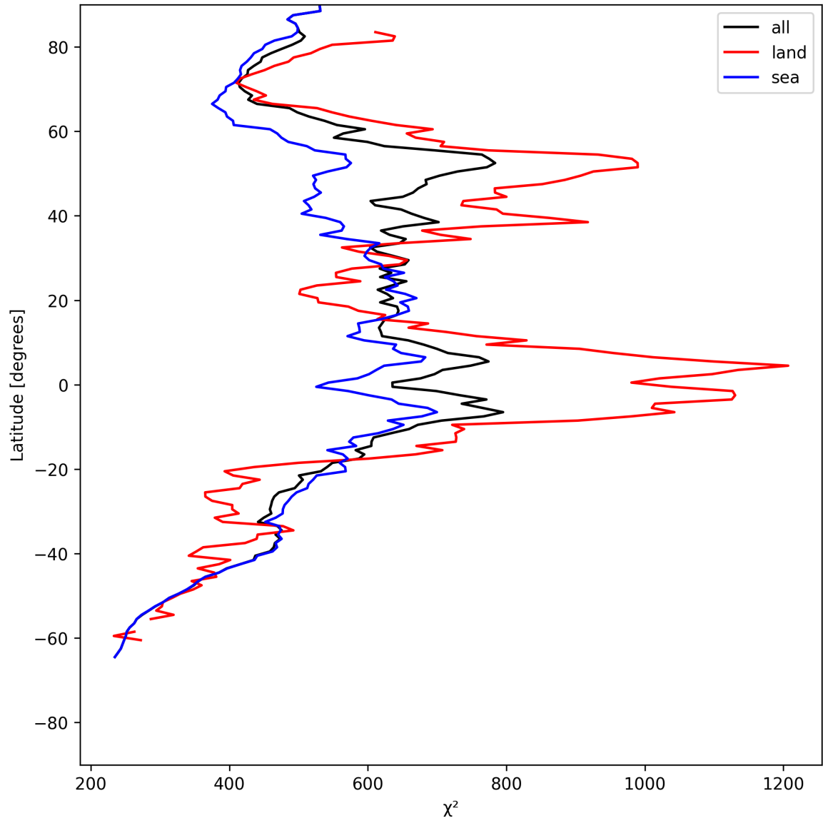
Figure 23: Zonal average of “ \chi^2 ” for 2025-06-30 to 2025-06-30.
