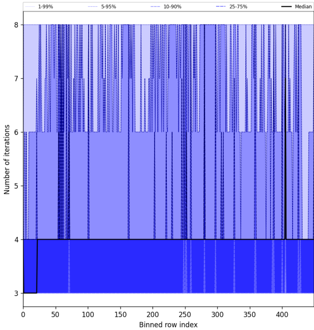
Figure 49: Along track statistics of “Number of iterations” for 2025-06-30 to 2025-06-30
