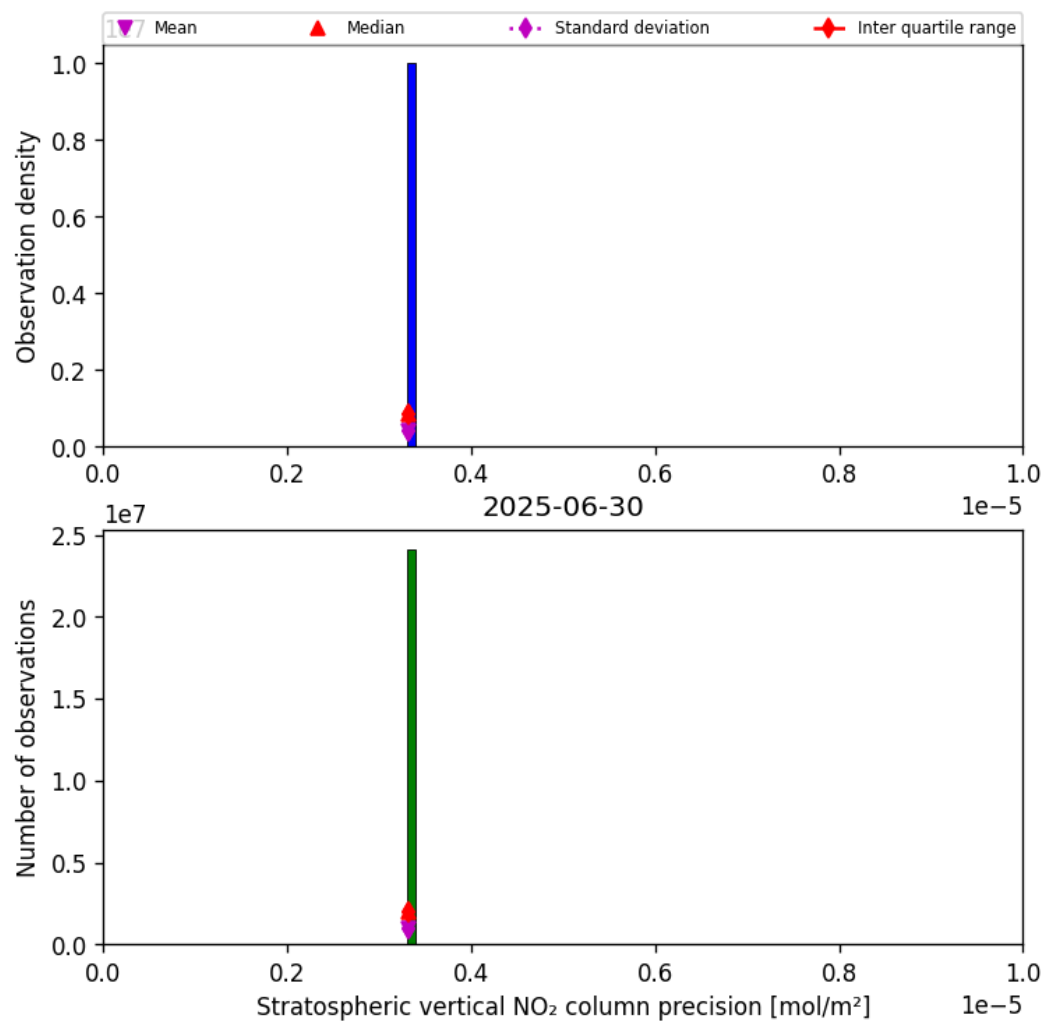
Figure 35: Histogram of “Stratospheric vertical NO 2 column precision” for 2025-06-30 to 2025-06-30
