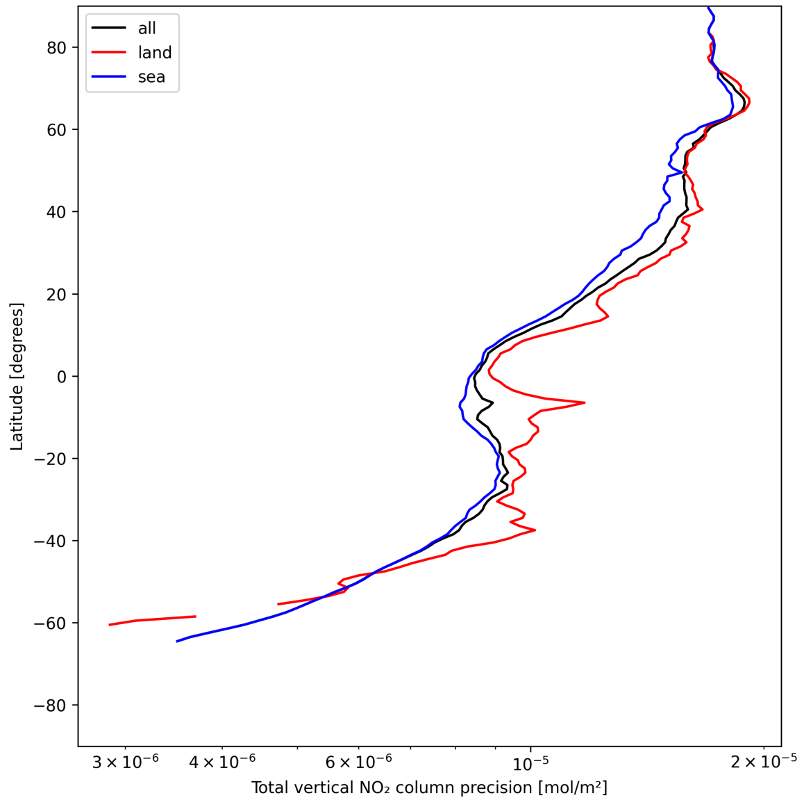
Figure 20: Zonal average of “Total vertical NO 2 column precision” for 2025-06-30 to 2025-06-30.
