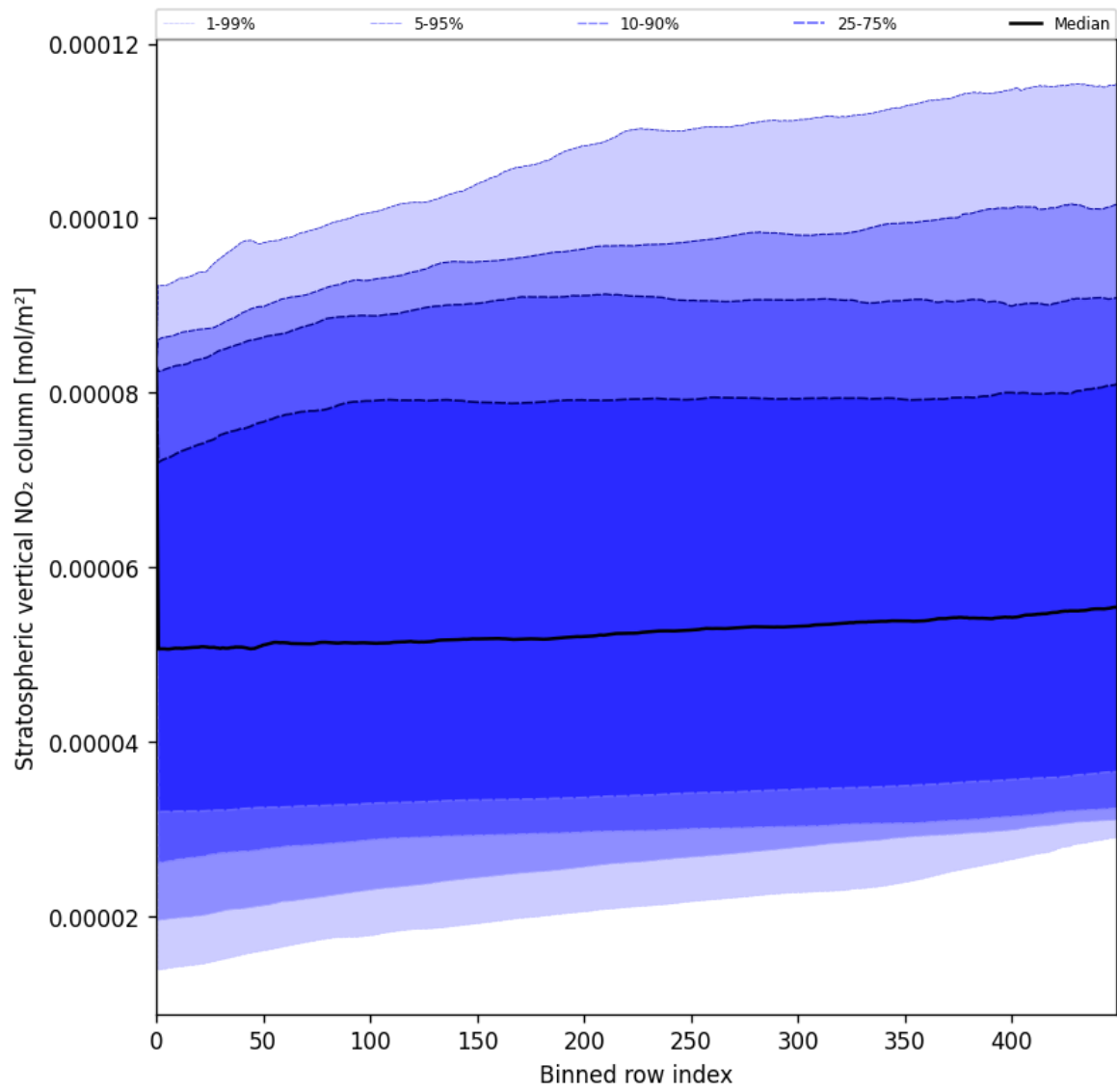
Figure 51: Along track statistics of “Stratospheric vertical NO 2 column” for 2025-07-01 to 2025-07-02
