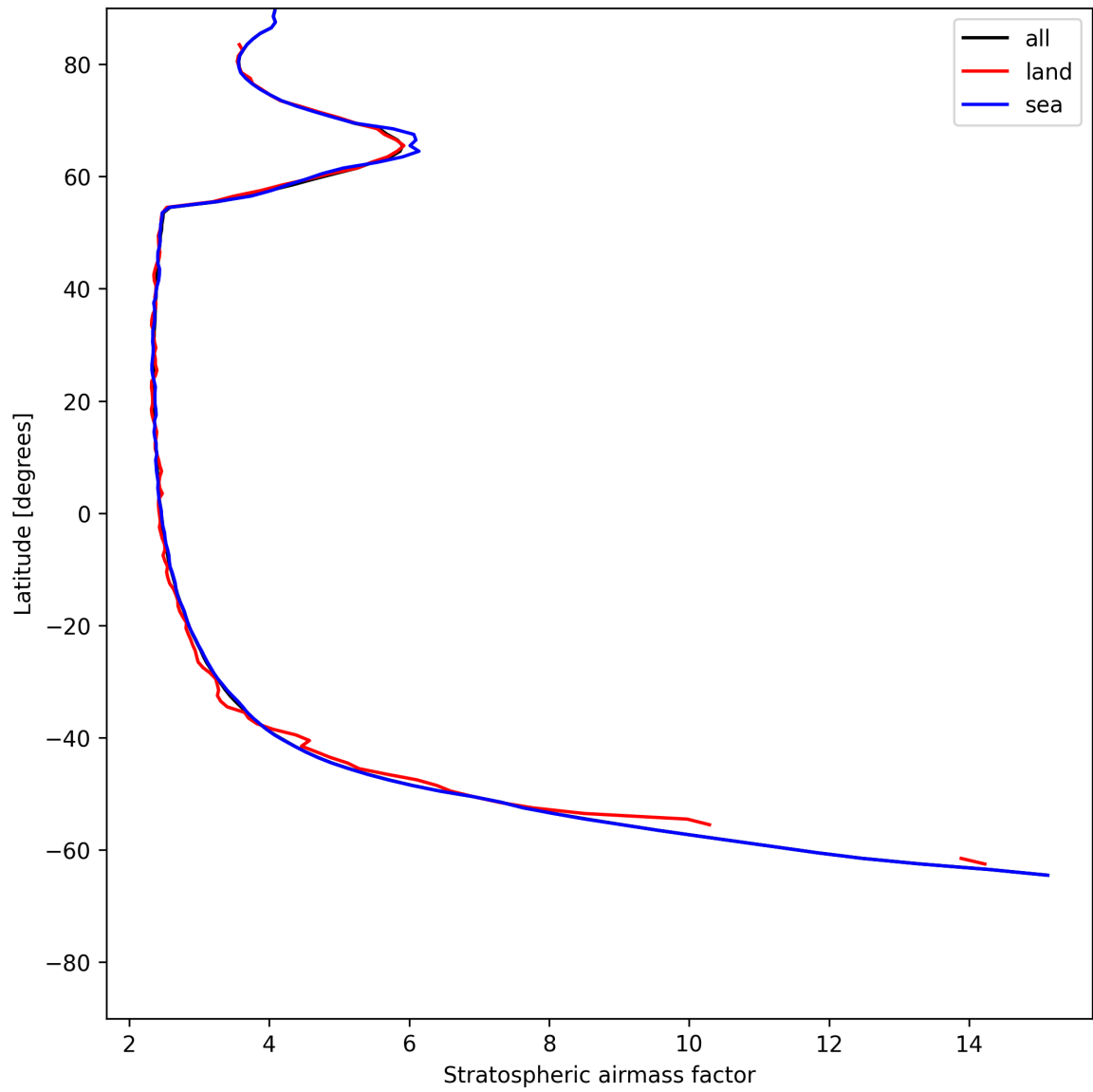
Figure 25: Zonal average of “Stratospheric air mass factor” for 2025-07-01 to 2025-07-02.
