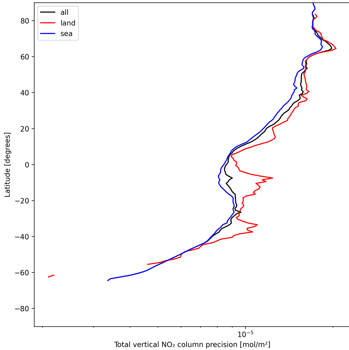
Figure 20: Zonal average of “Total vertical NO 2 column precision” for 2025-07-01 to 2025-07-02.
