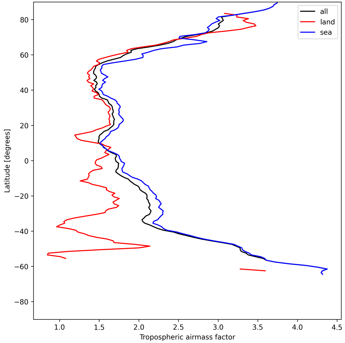
Figure 12: Zonal average of “Tropospheric airmass factor” for 2025-07-01 to 2025-07-02.
