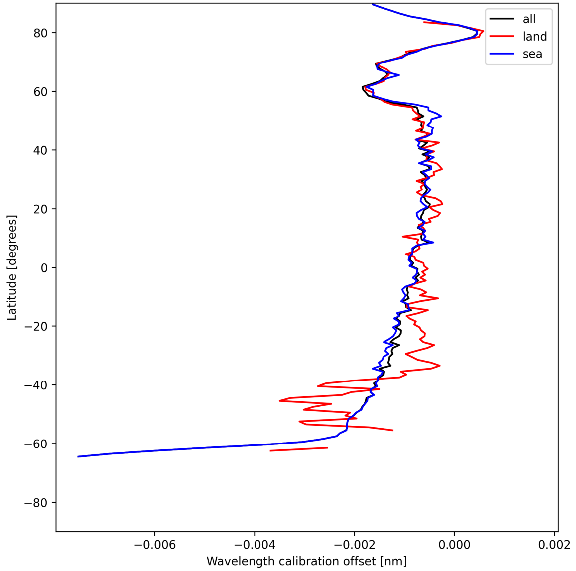
Figure 16: Zonal average of “Wavelength calibration offset” for 2025-07-01 to 2025-07-02.
