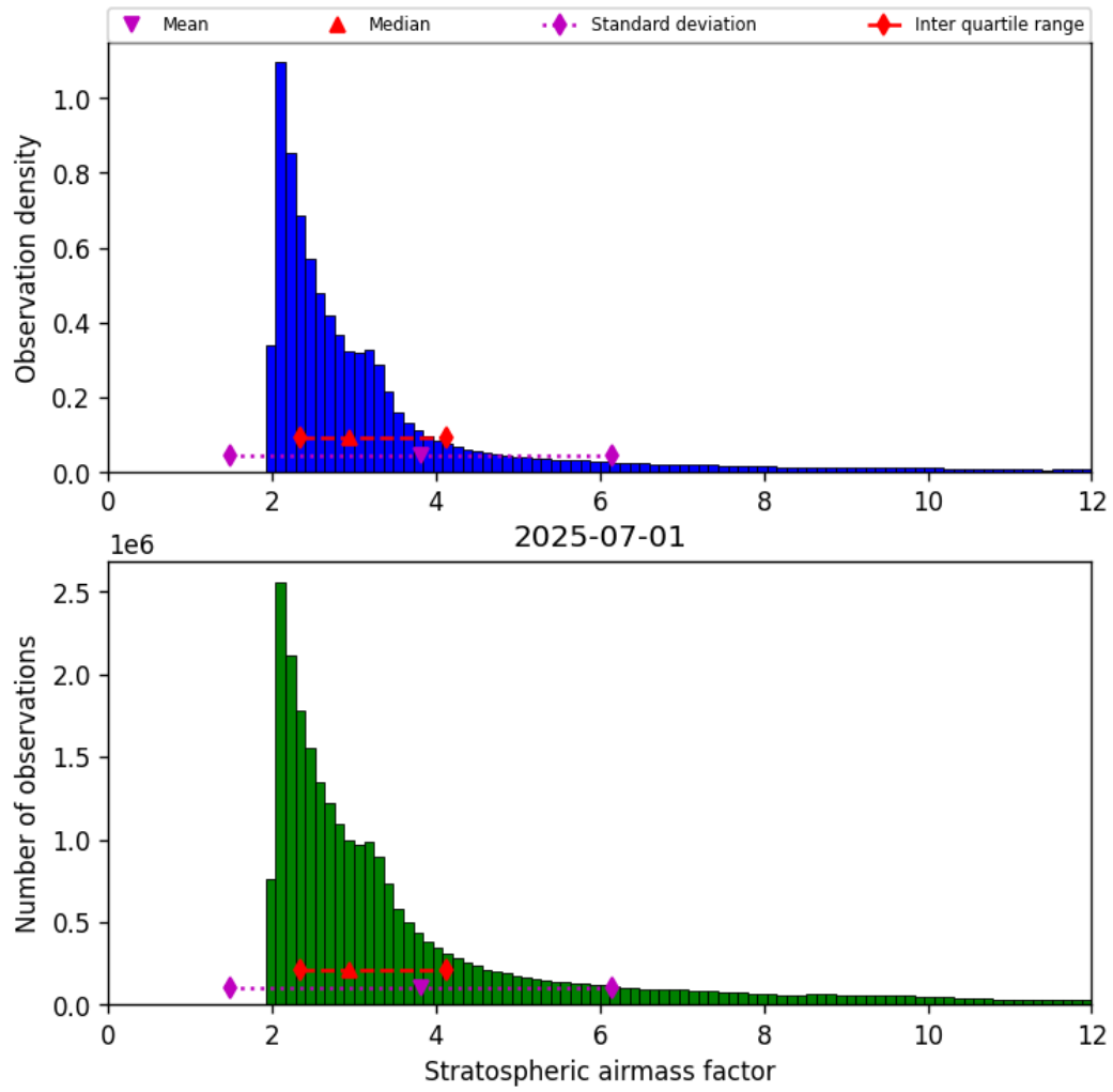
Figure 42: Histogram of “Stratospheric airmass factor” for 2025-07-01 to 2025-07-02
