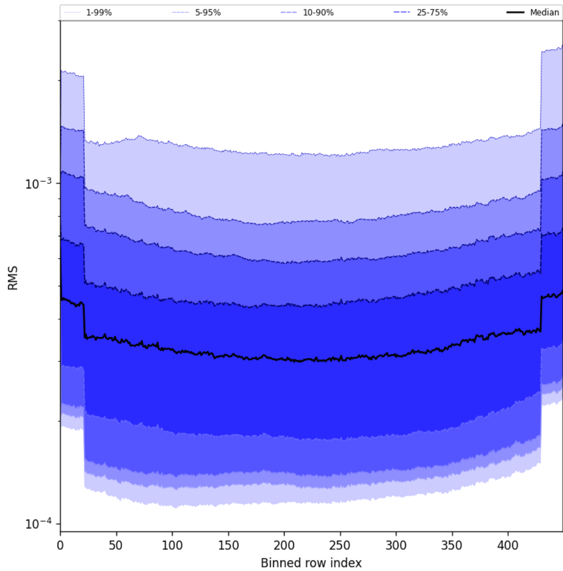
Figure 58: Along track statistics of “RMS” for 2025-07-01 to 2025-07-02
