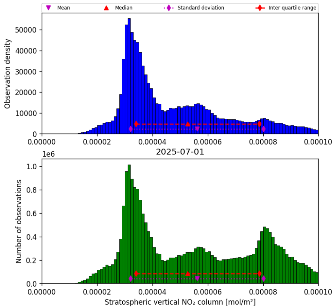
Figure 34: Histogram of “Stratospheric vertical NO 2 column” for 2025-07-01 to 2025-07-02
