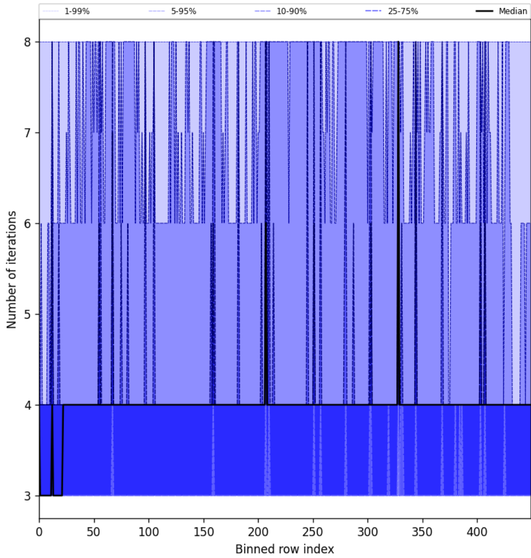
Figure 49: Along track statistics of “Number of iterations” for 2025-07-01 to 2025-07-02
