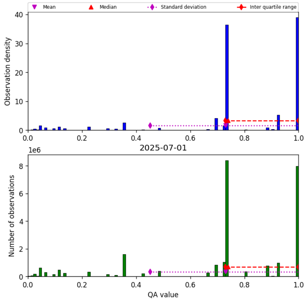
Figure 26: Histogram of “QA value” for 2025-07-01 to 2025-07-02
