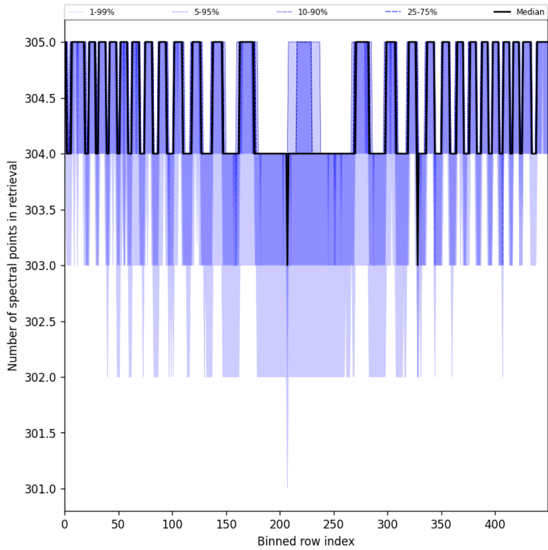
Figure 48: Along track statistics of “Number of spectral points in retrieval” for 2025-07-01 to 2025-07-02
