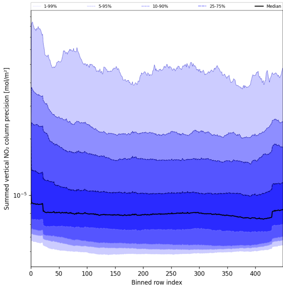
Figure 56: Along track statistics of “Summed vertical NO 2 column precision” for 2025-07-01 to 2025-07-02
