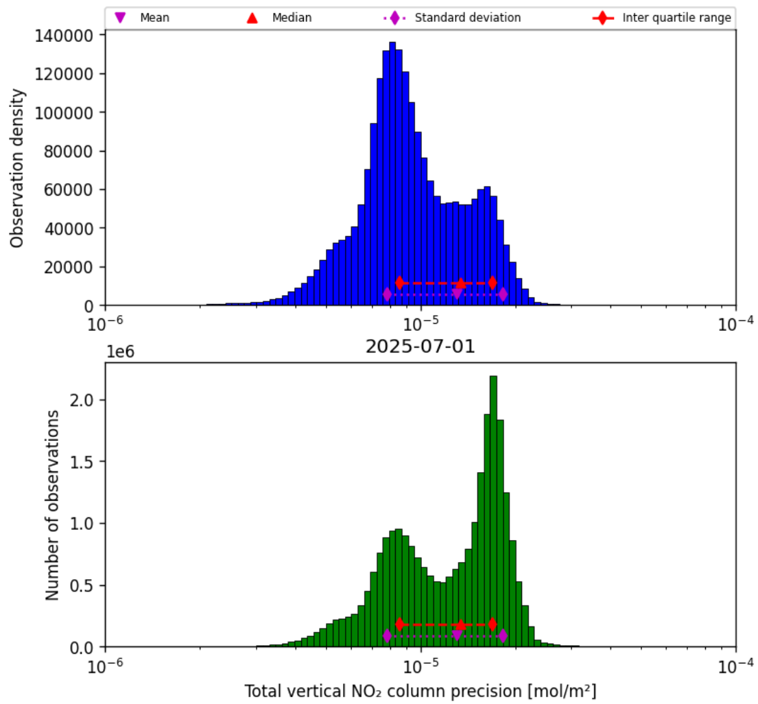
Figure 37: Histogram of “Total vertical NO 2 column precision” for 2025-07-01 to 2025-07-02
