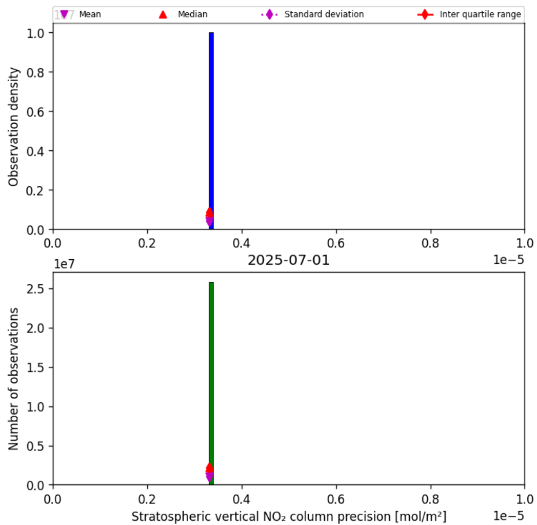
Figure 35: Histogram of “Stratospheric vertical NO 2 column precision” for 2025-07-01 to 2025-07-02
