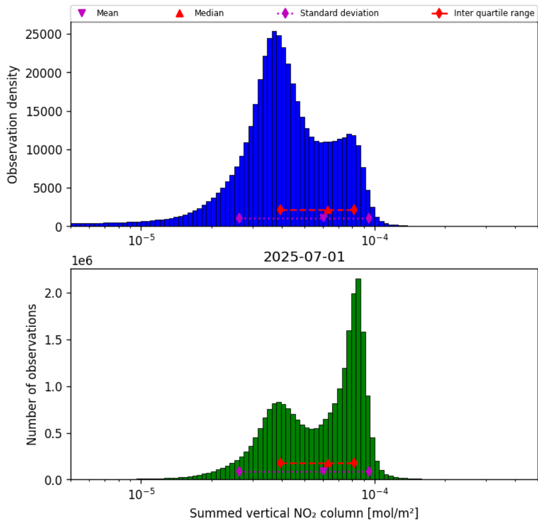
Figure 38: Histogram of “Summed vertical NO 2 column” for 2025-07-01 to 2025-07-02
