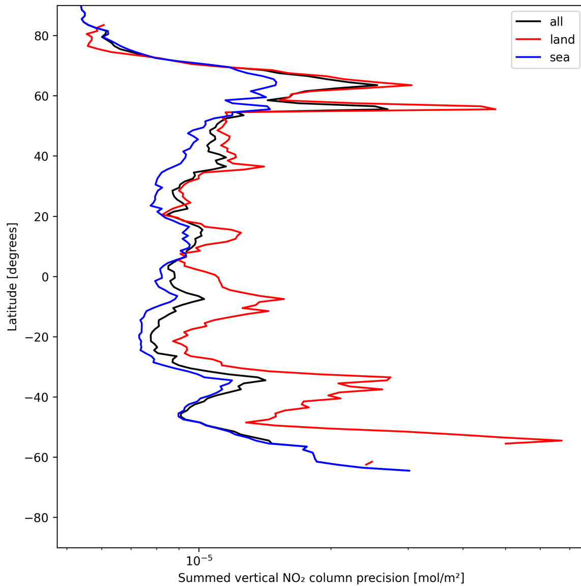
Figure 22: Zonal average of “Summed vertical NO 2 column precision” for 2025-07-01 to 2025-07-02.
