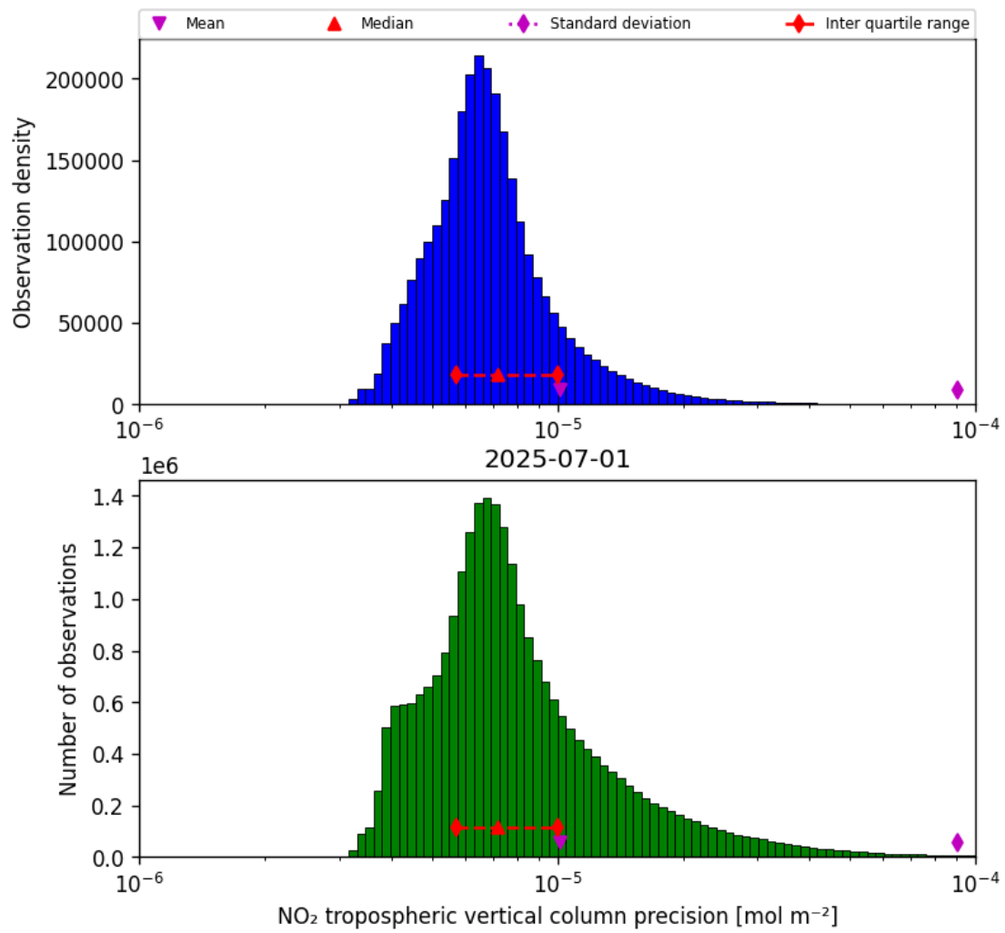
Figure 28: Histogram of “NO 2 tropospheric vertical column precision” for 2025-07-01 to 2025-07-02
