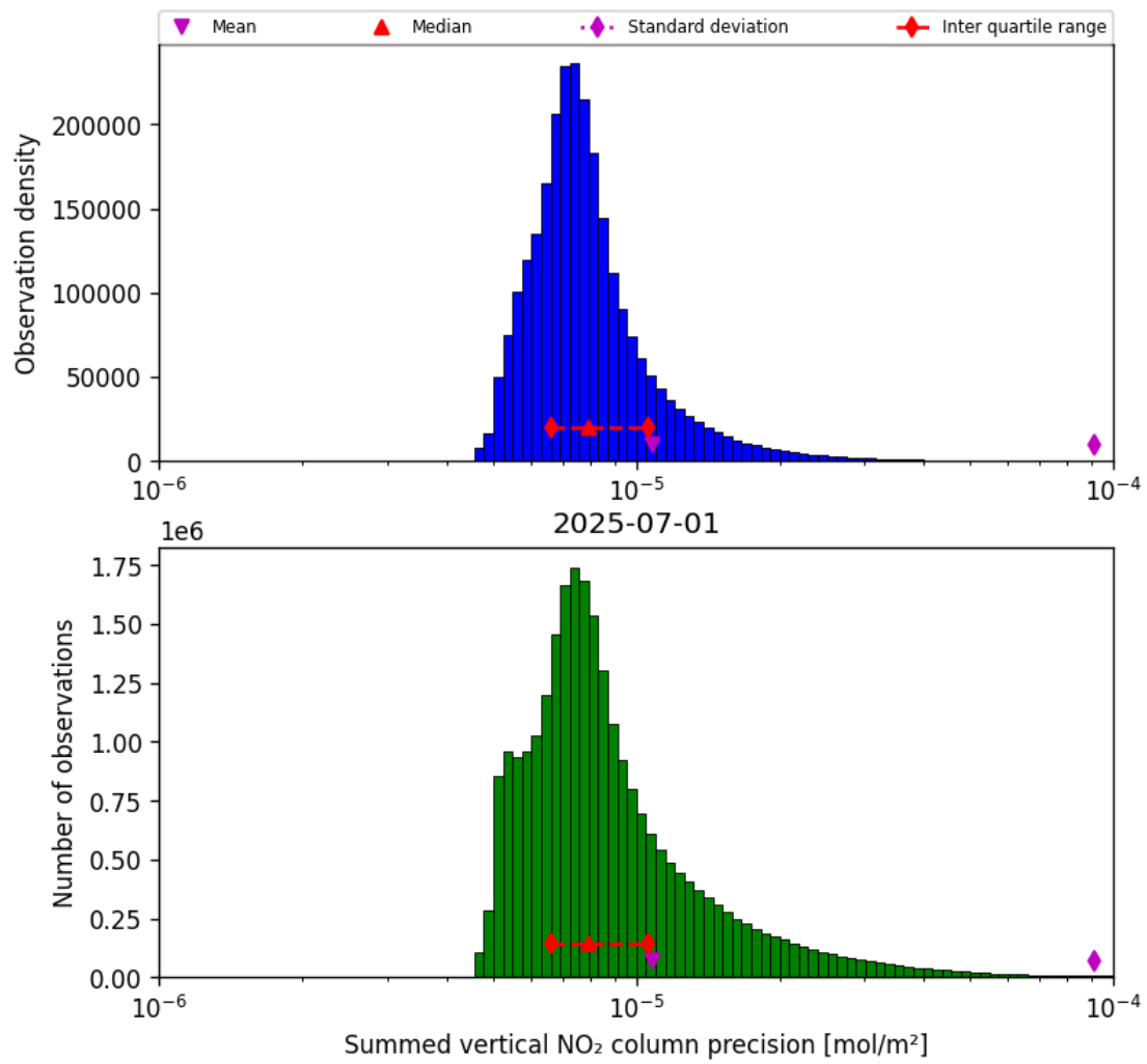
Figure 39: Histogram of “Summed vertical NO 2 column precision” for 2025-07-01 to 2025-07-02
