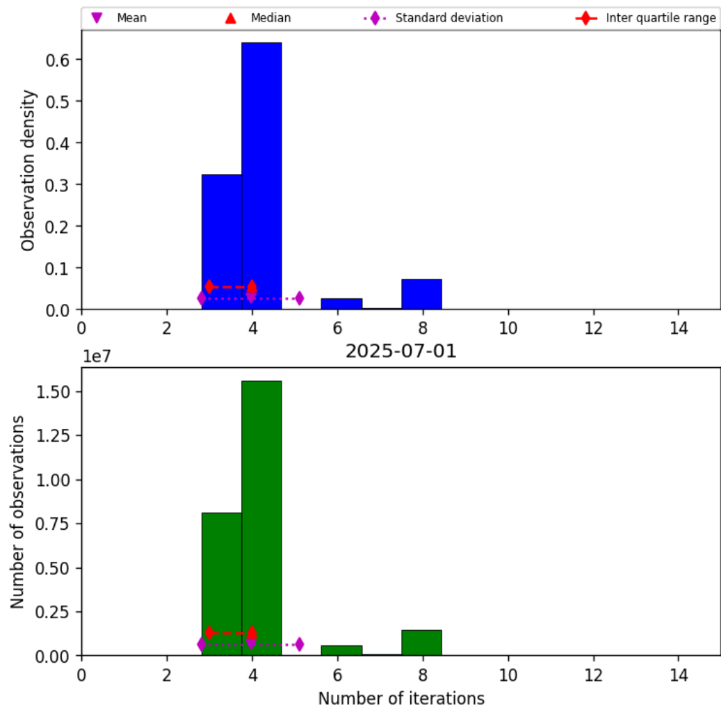
Figure 32: Histogram of “Number of iterations” for 2025-07-01 to 2025-07-02
