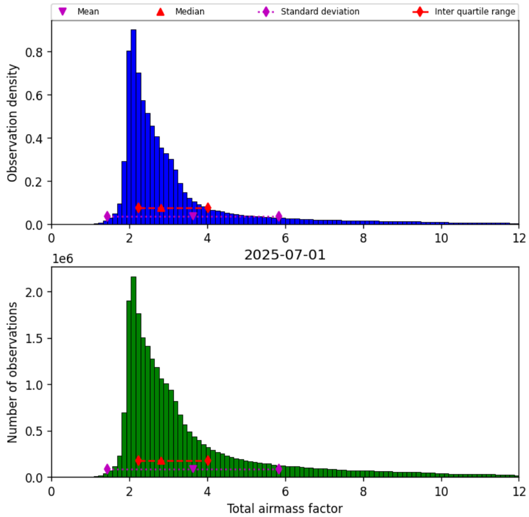
Figure 30: Histogram of “Total airmass factor” for 2025-07-01 to 2025-07-02
