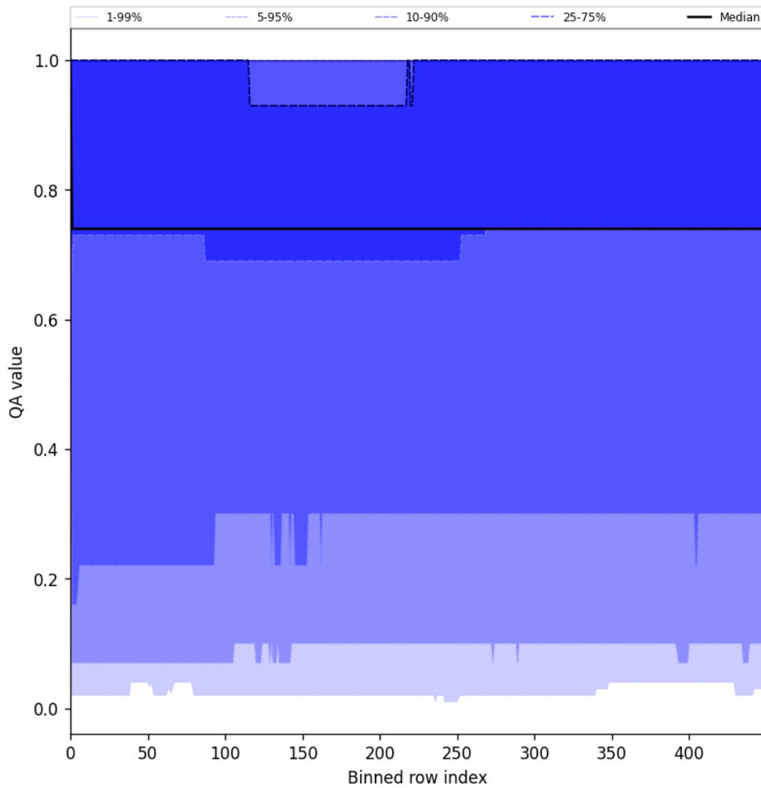
Figure 43: Along track statistics of “QA value” for 2025-07-01 to 2025-07-02
