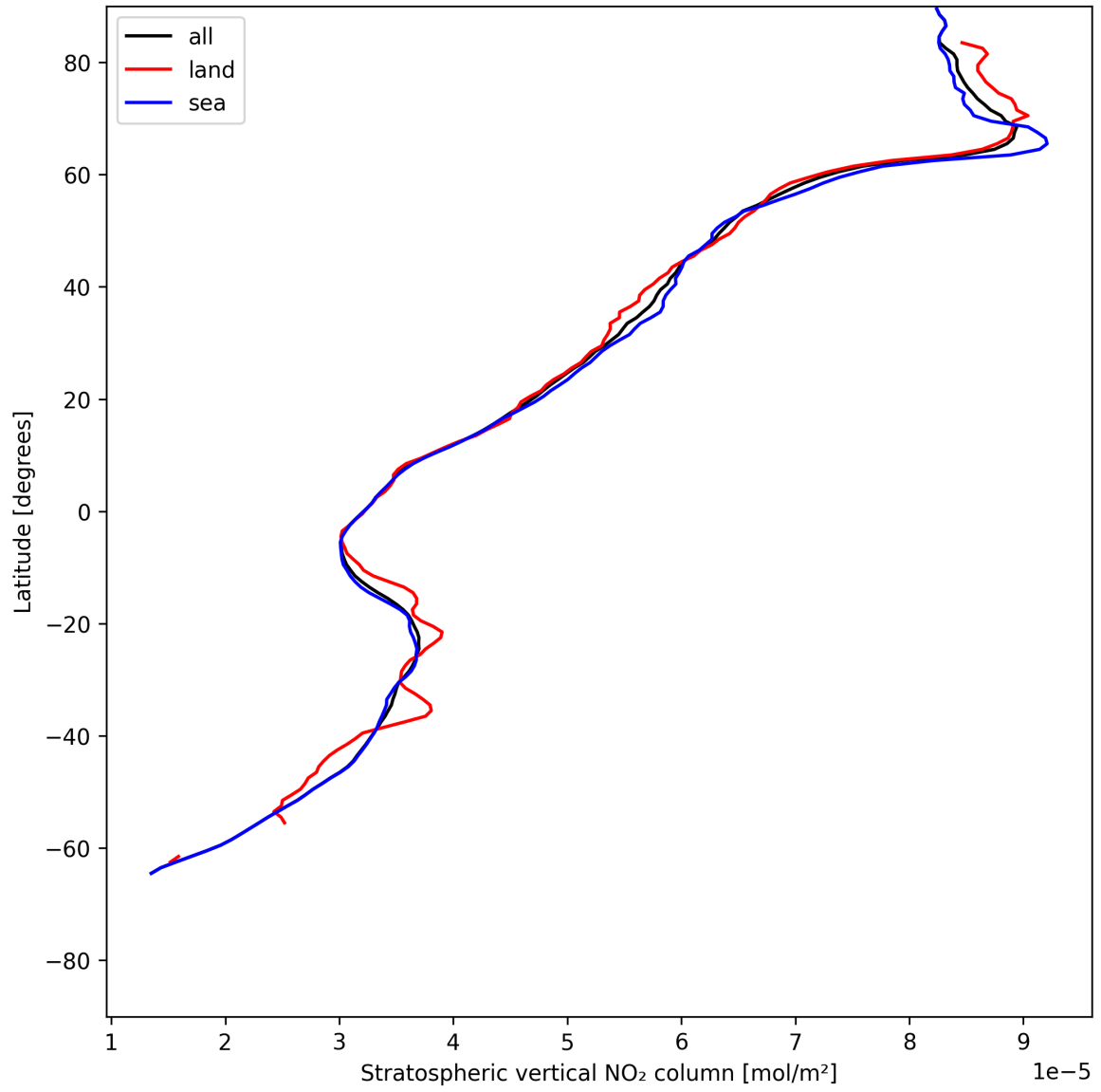
Figure 17: Zonal average of “Stratospheric vertical NO 2 column” for 2025-07-01 to 2025-07-02.
