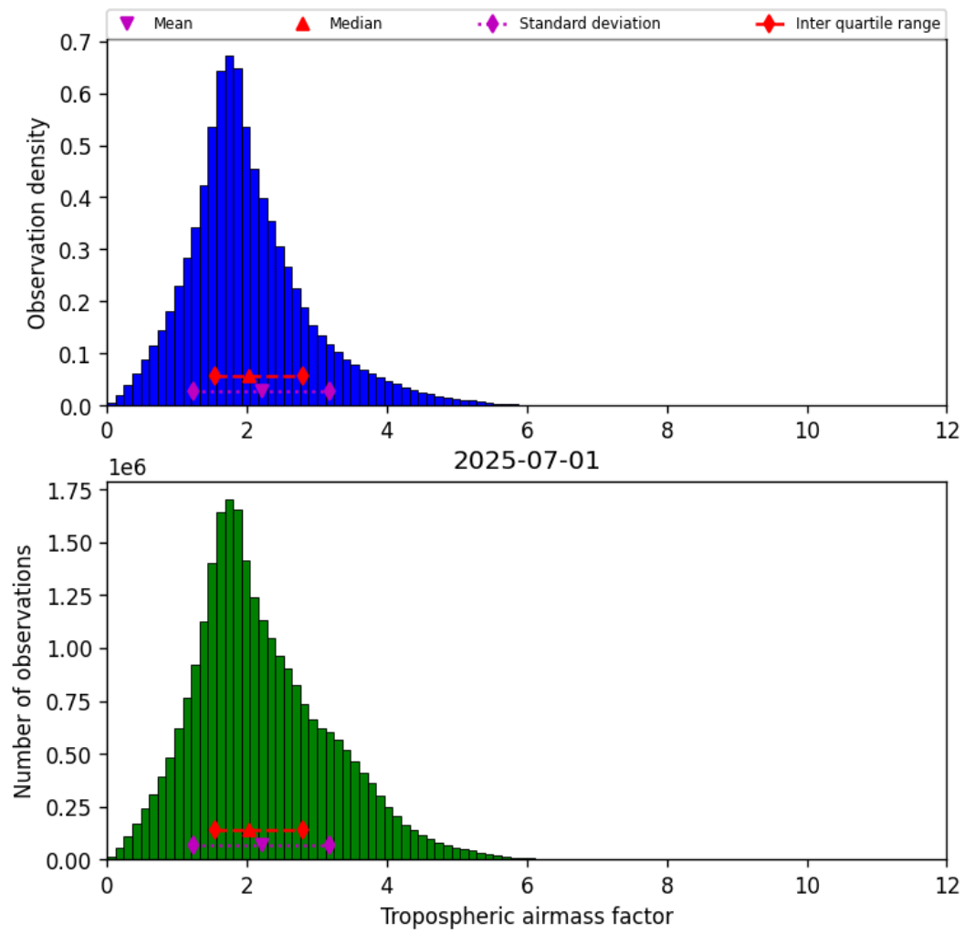
Figure 29: Histogram of “Tropospheric airmass factor” for 2025-07-01 to 2025-07-02
