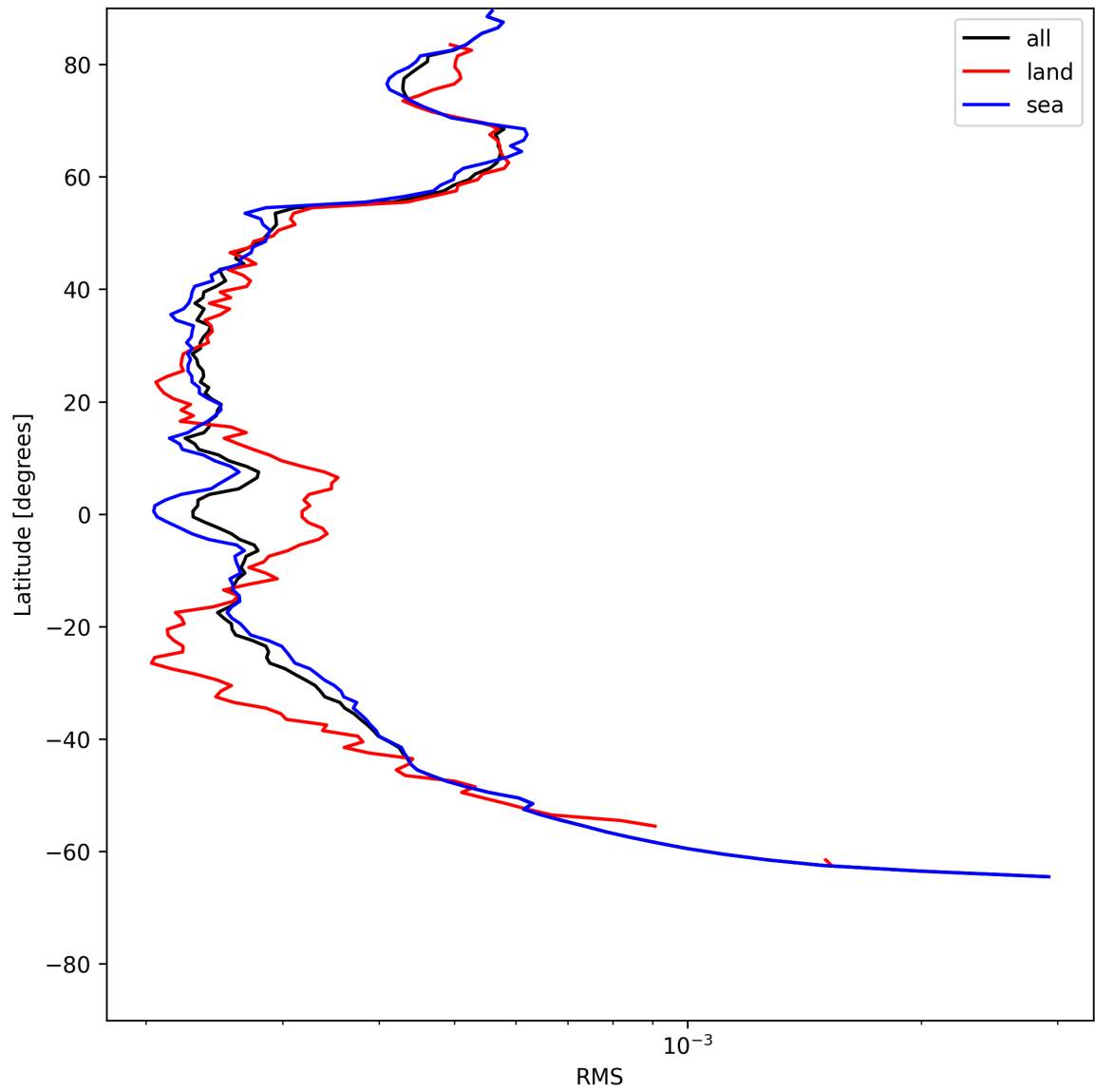
Figure 24: Zonal average of “RMS” for 2025-07-01 to 2025-07-02.
