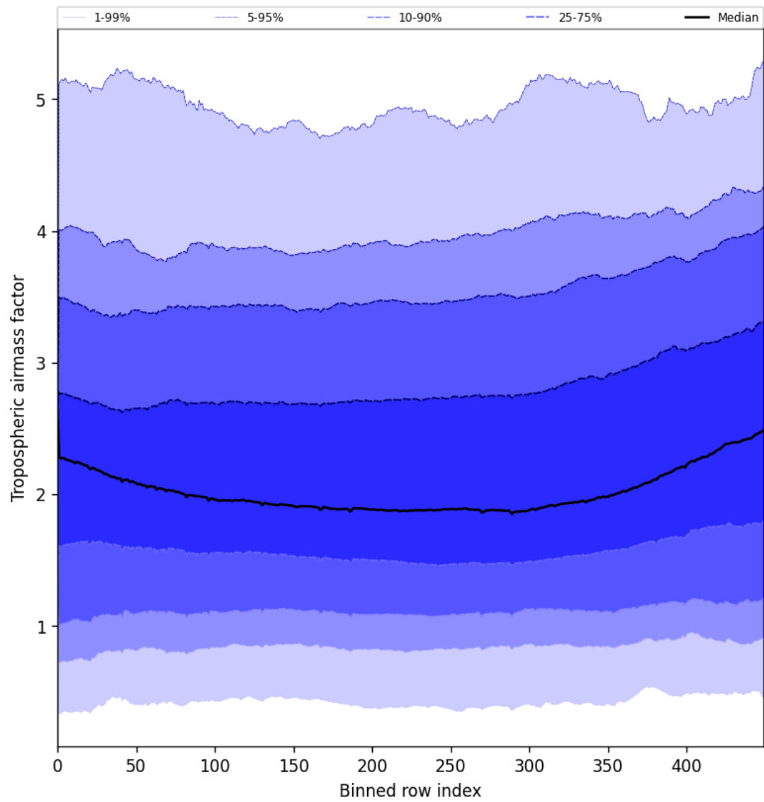
Figure 46: Along track statistics of “Tropospheric airmass factor” for 2025-07-01 to 2025-07-02
