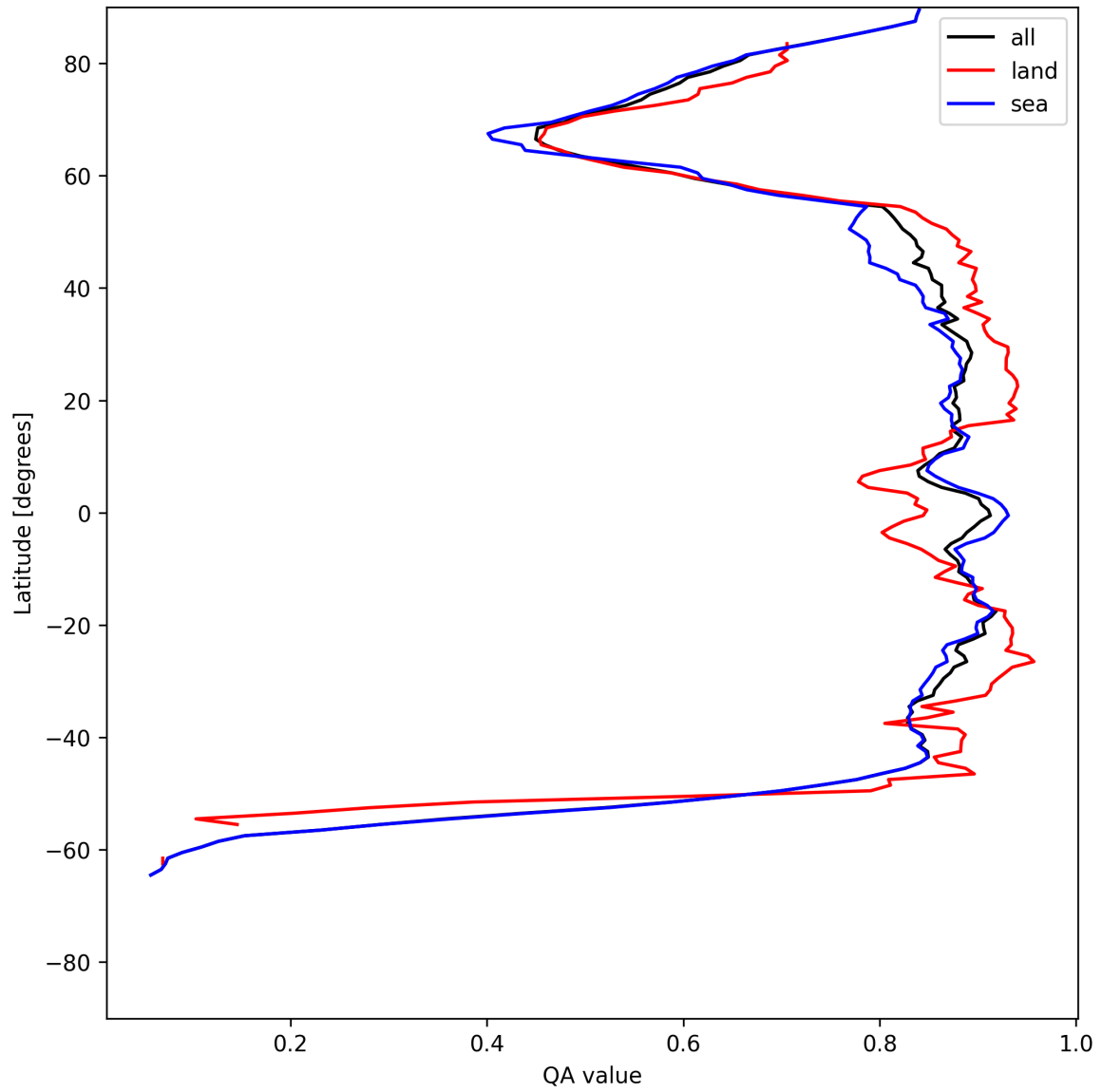
Figure 9: Zonal average of “QA value” for 2025-07-01 to 2025-07-02.
