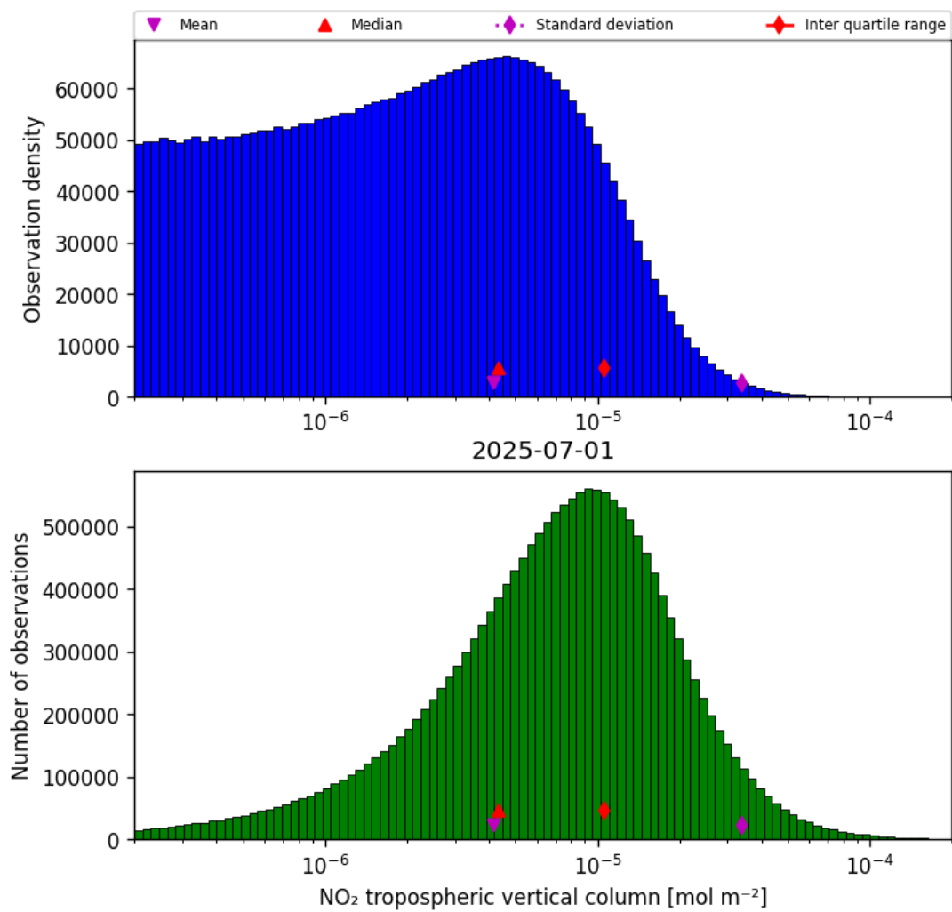
Figure 27: Histogram of “NO 2 tropospheric vertical column” for 2025-07-01 to 2025-07-02
