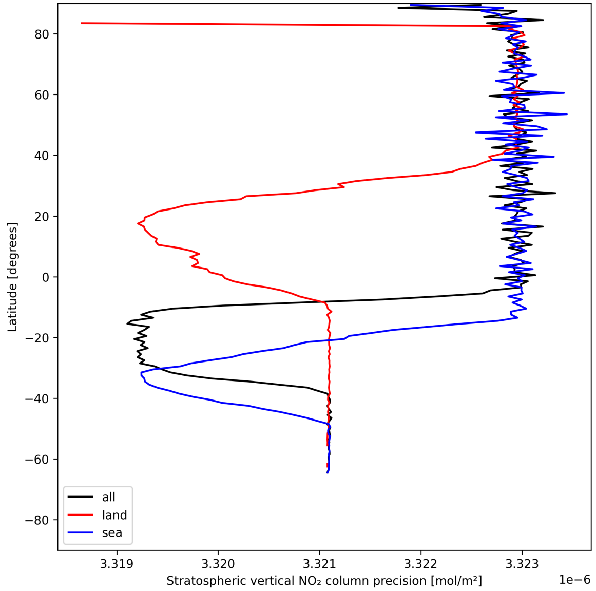
Figure 18: Zonal average of “Stratospheric vertical NO 2 column precision” for 2025-07-01 to 2025-07-02.
