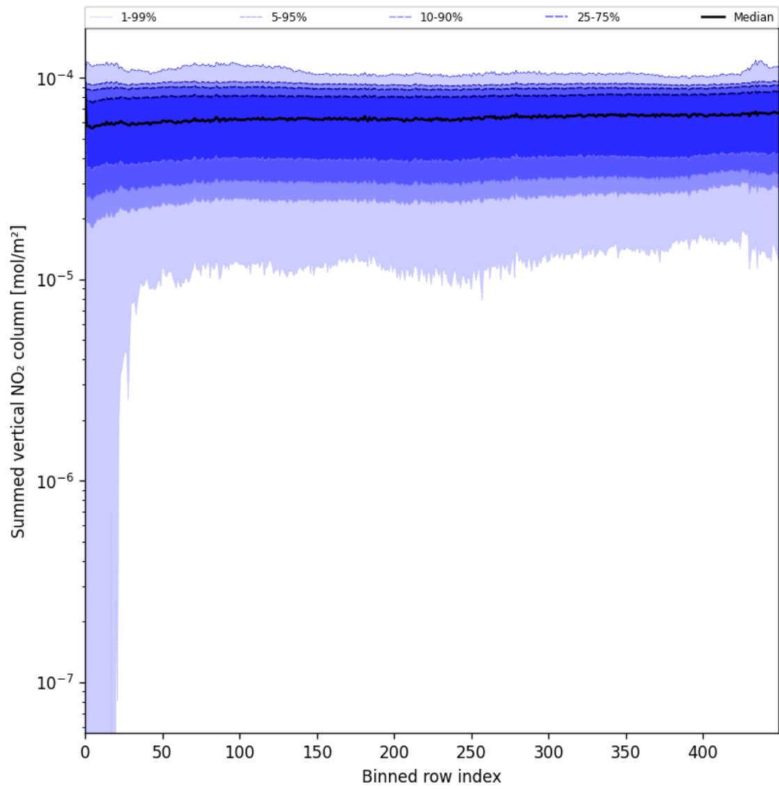
Figure 55: Along track statistics of “Summed vertical NO 2 column” for 2025-07-01 to 2025-07-02
