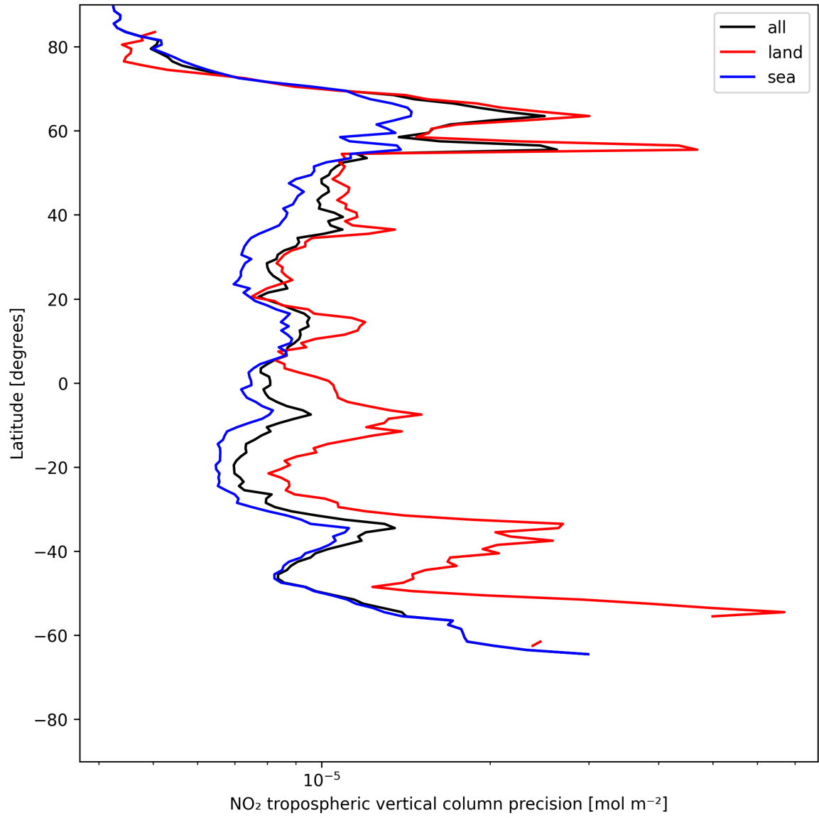
Figure 11: Zonal average of “NO 2 tropospheric vertical column precision” for 2025-07-01 to 2025-07-02.
