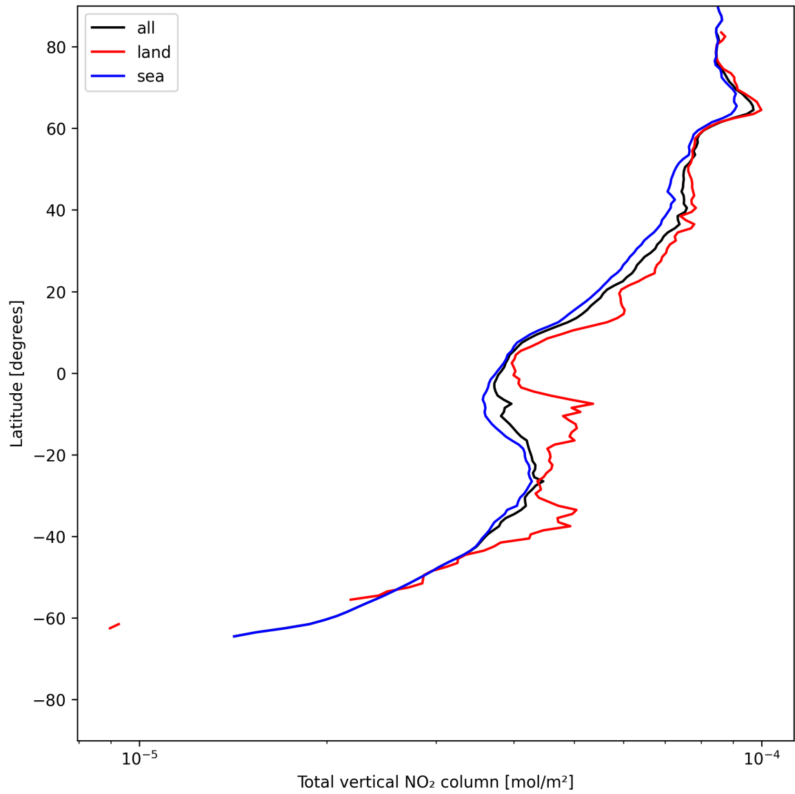
Figure 19: Zonal average of “Total vertical NO 2 column” for 2025-07-01 to 2025-07-02.
