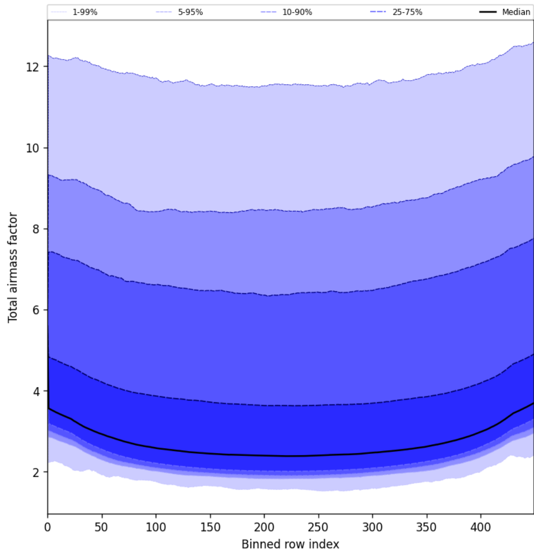
Figure 47: Along track statistics of “Total airmass factor” for 2025-07-01 to 2025-07-02
