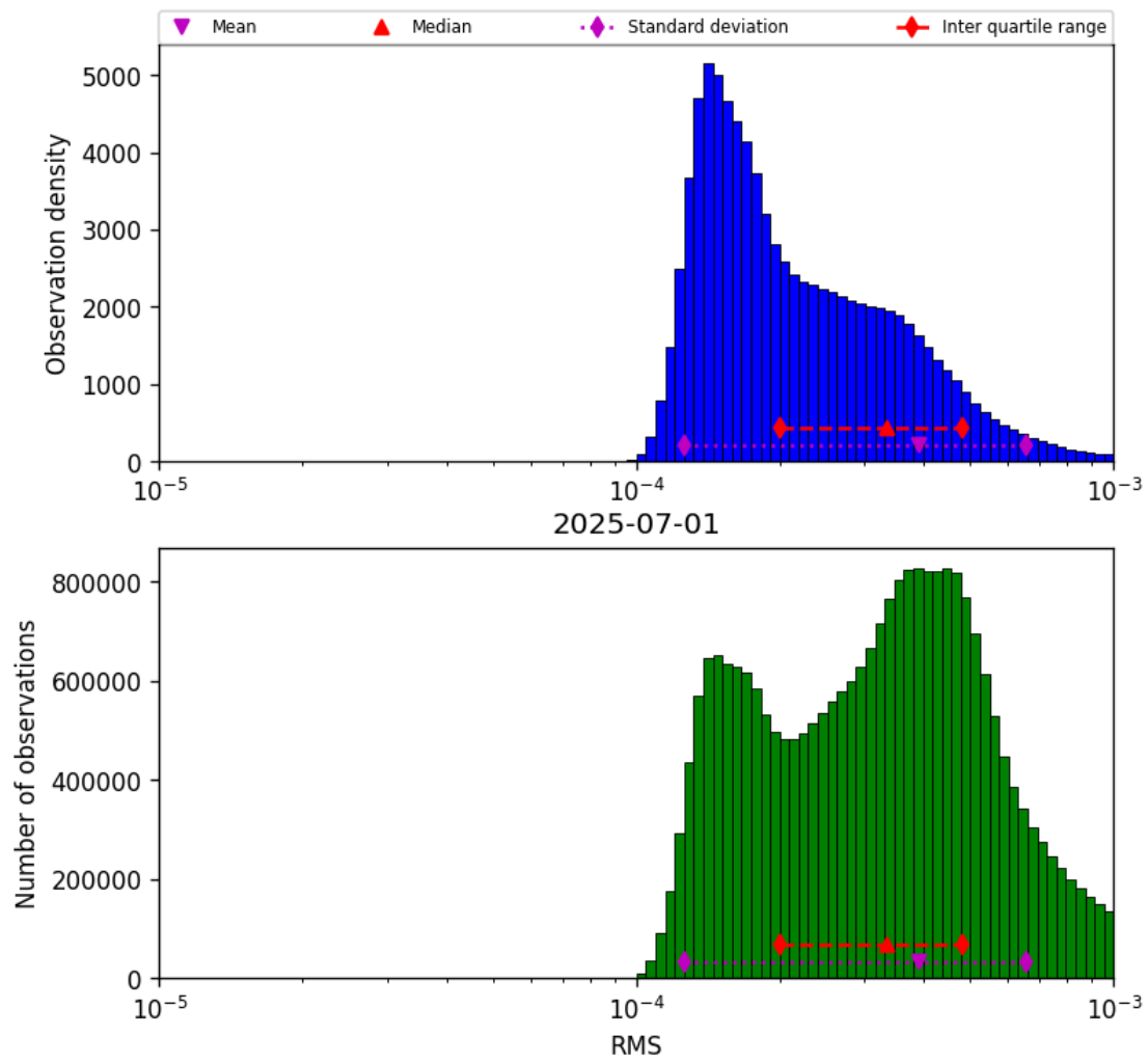
Figure 41: Histogram of “RMS” for 2025-07-01 to 2025-07-02
