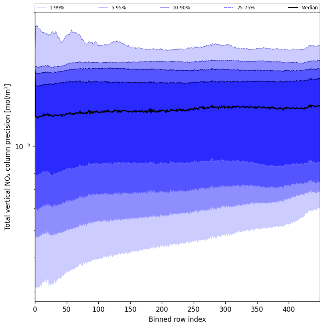
Figure 54: Along track statistics of “Total vertical NO 2 column precision” for 2025-07-01 to 2025-07-02
