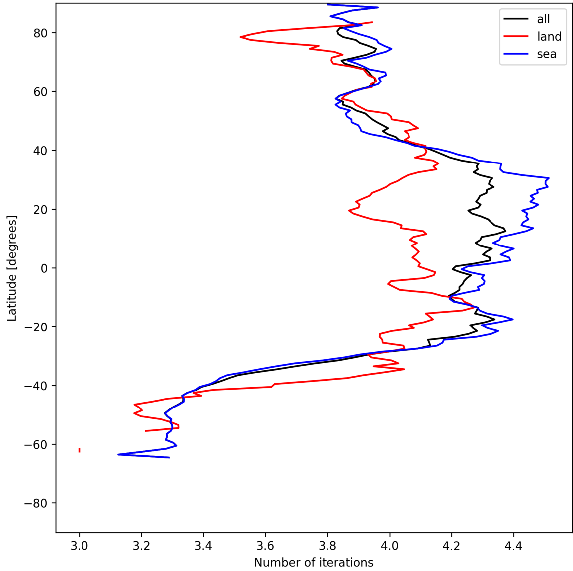
Figure 15: Zonal average of “Number of iterations” for 2025-07-01 to 2025-07-02.
