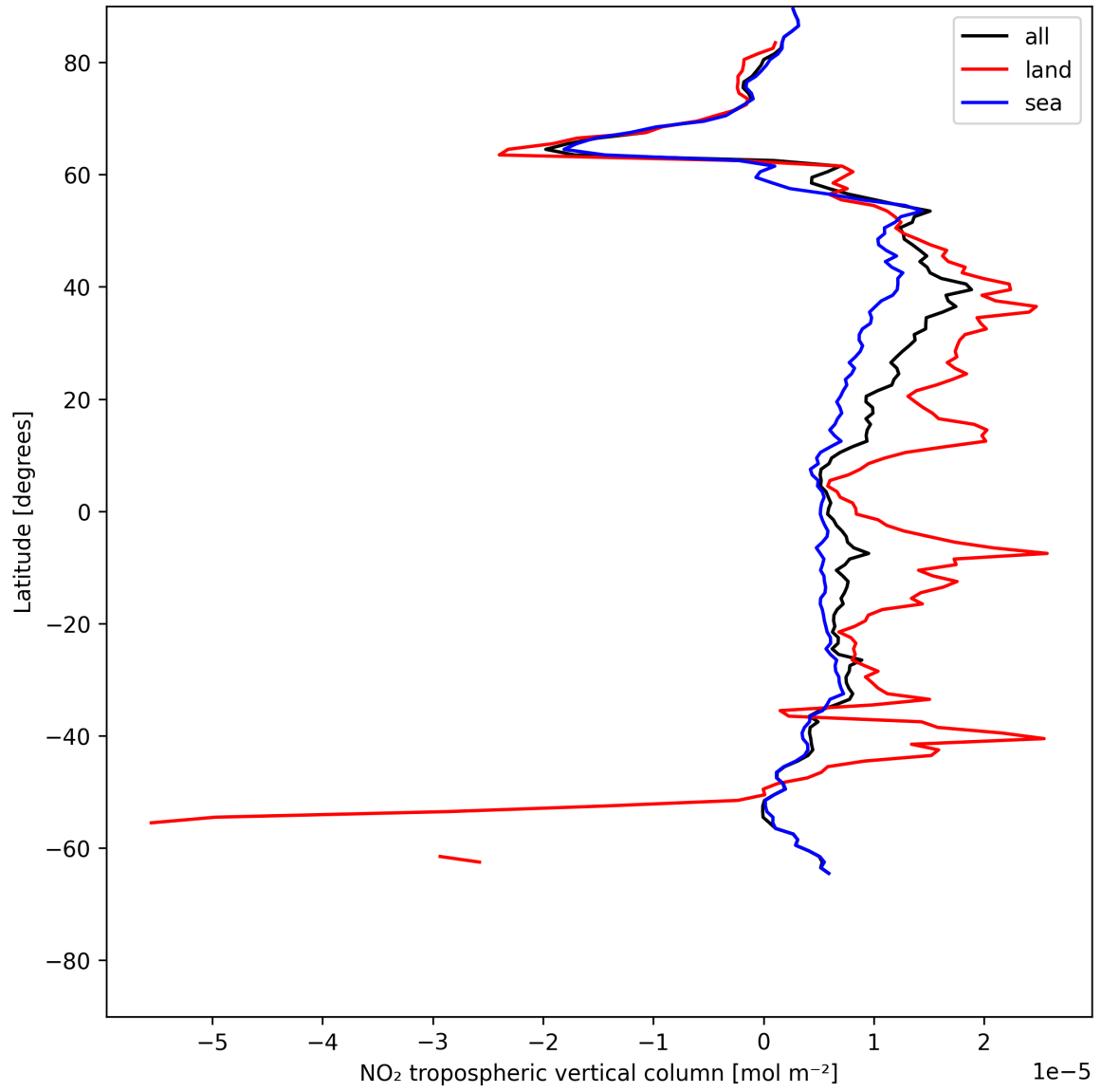
Figure 10: Zonal average of “NO 2 tropospheric vertical column” for 2025-07-01 to 2025-07-02.
