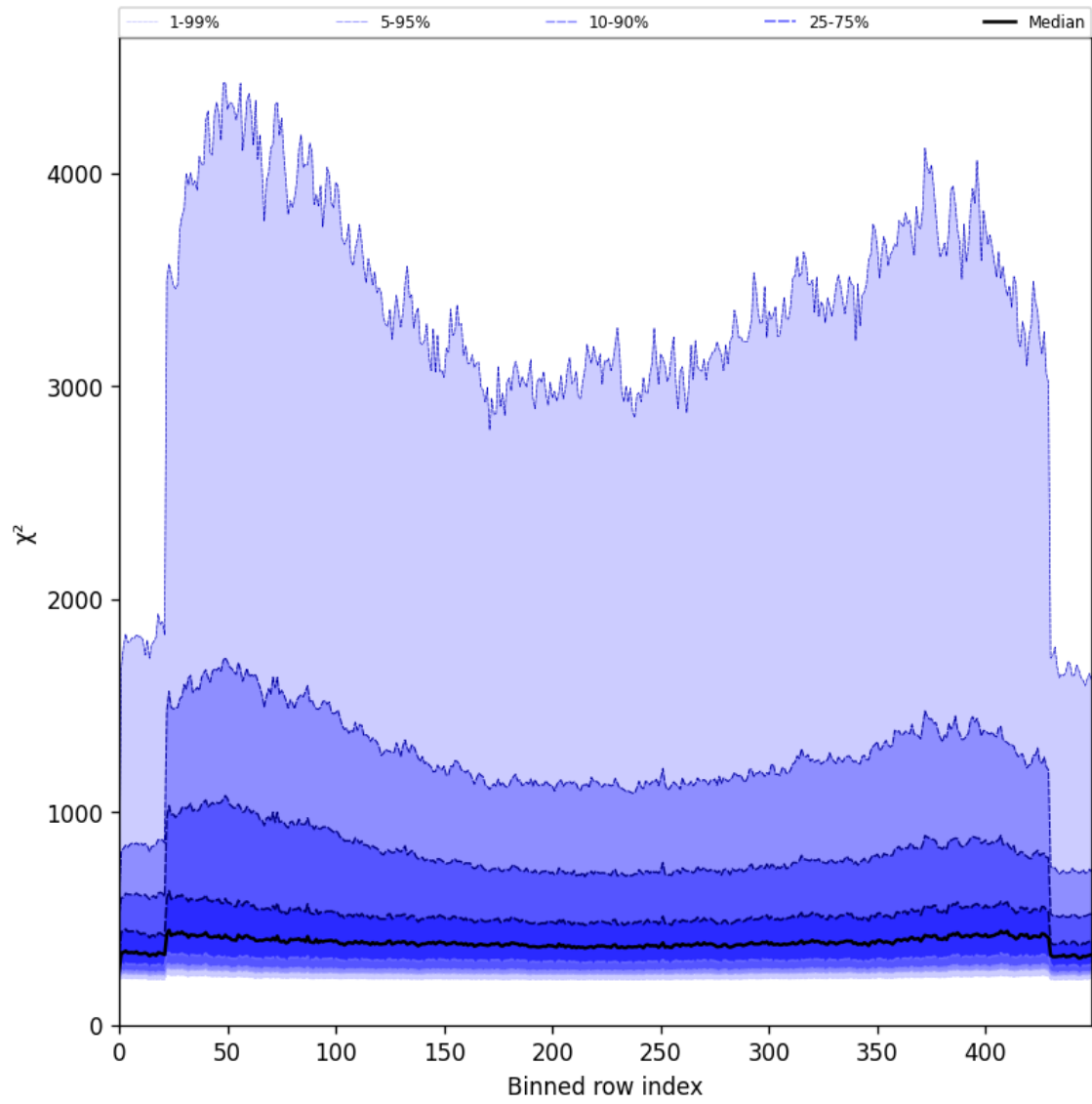
Figure 57: Along track statistics of “ \chi^2 ” for 2025-07-01 to 2025-07-02
