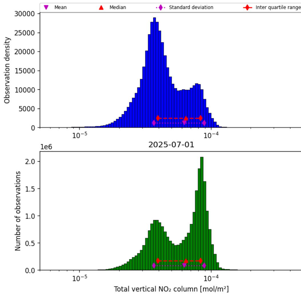
Figure 36: Histogram of “Total vertical NO 2 column” for 2025-07-01 to 2025-07-02
