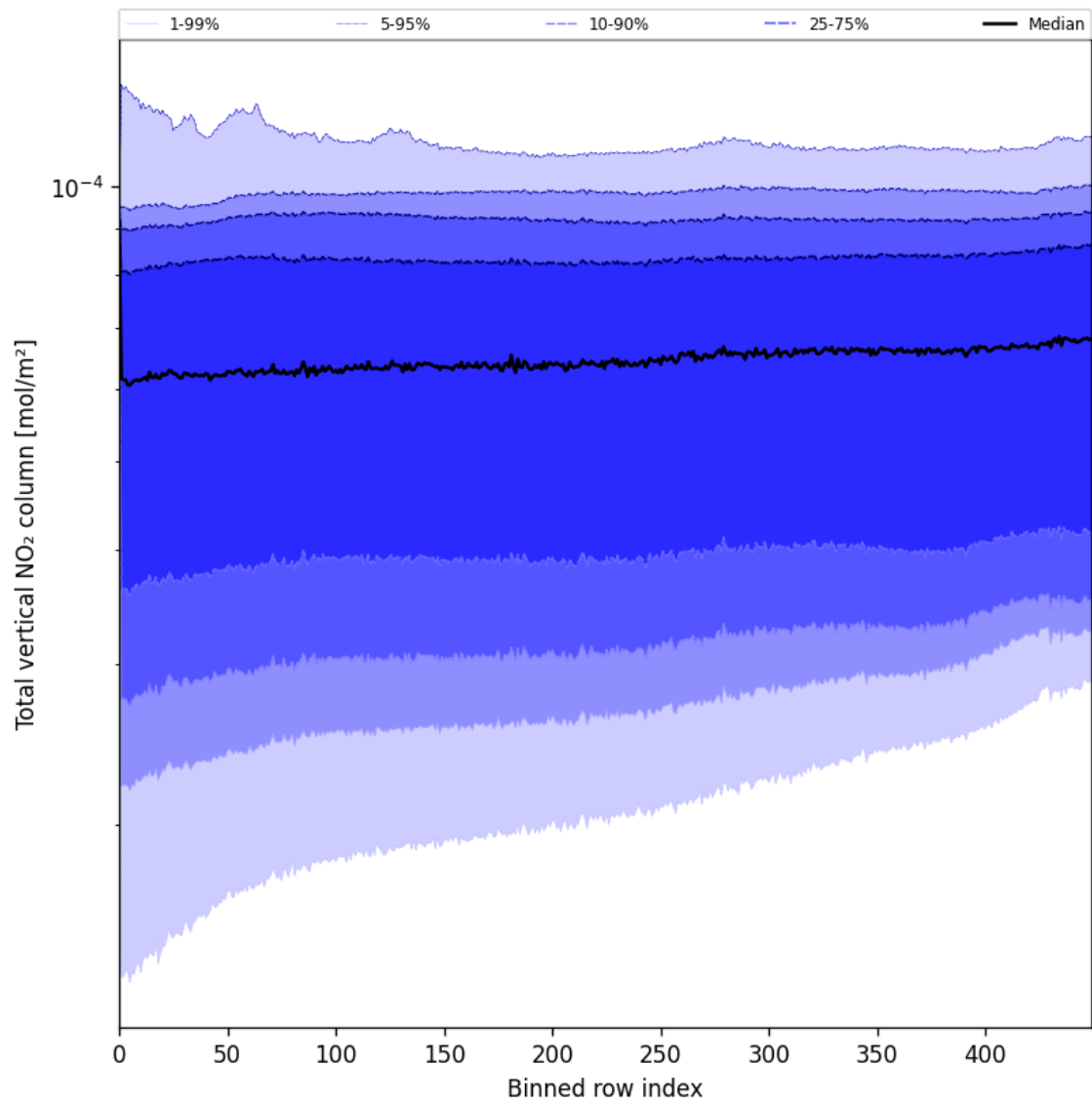
Figure 53: Along track statistics of “Total vertical NO 2 column” for 2025-07-01 to 2025-07-02
