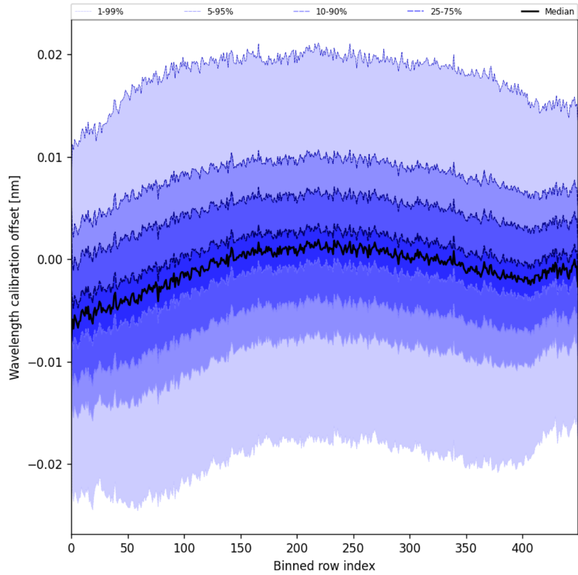
Figure 50: Along track statistics of “Wavelength calibration offset” for 2025-07-01 to 2025-07-02
