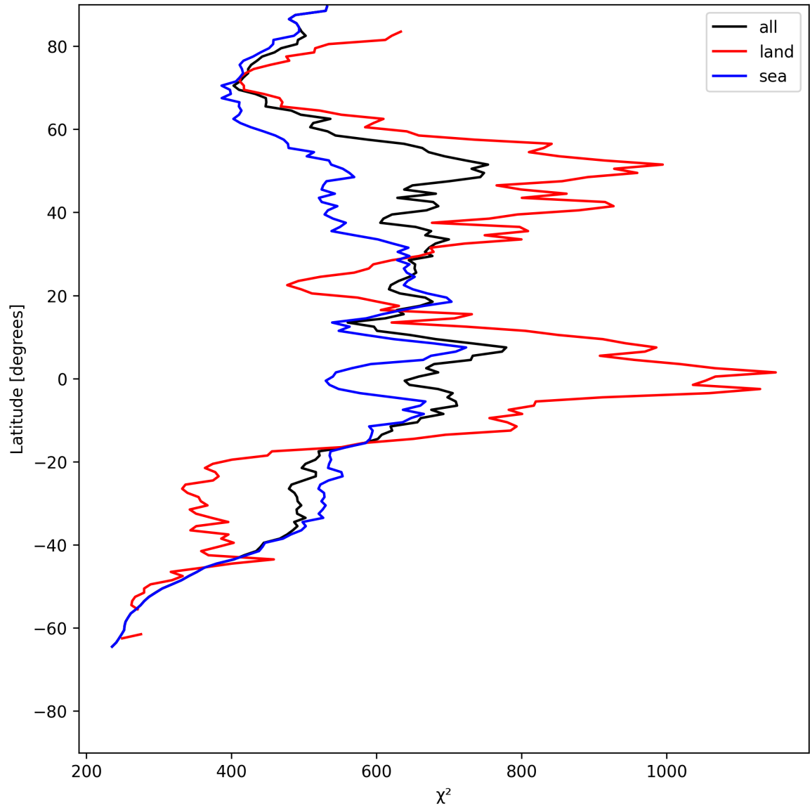
Figure 23: Zonal average of “ \chi^2 ” for 2025-07-01 to 2025-07-02.
