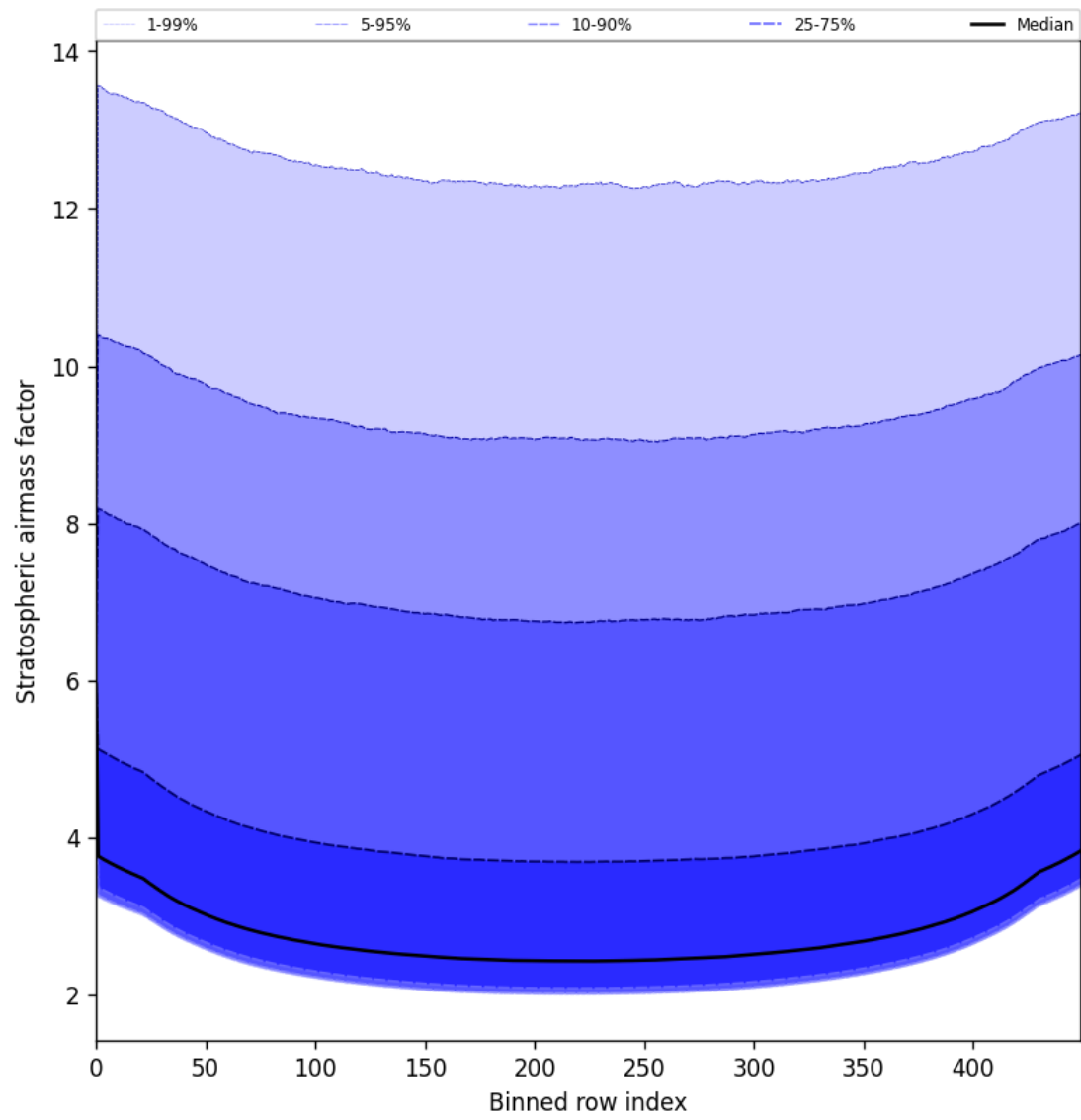
Figure 59: Along track statistics of “Stratospheric airmass factor” for 2025-07-01 to 2025-07-02
