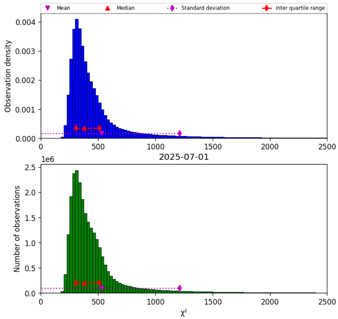
Figure 40: Histogram of “ \chi^2 ” for 2025-07-01 to 2025-07-02
