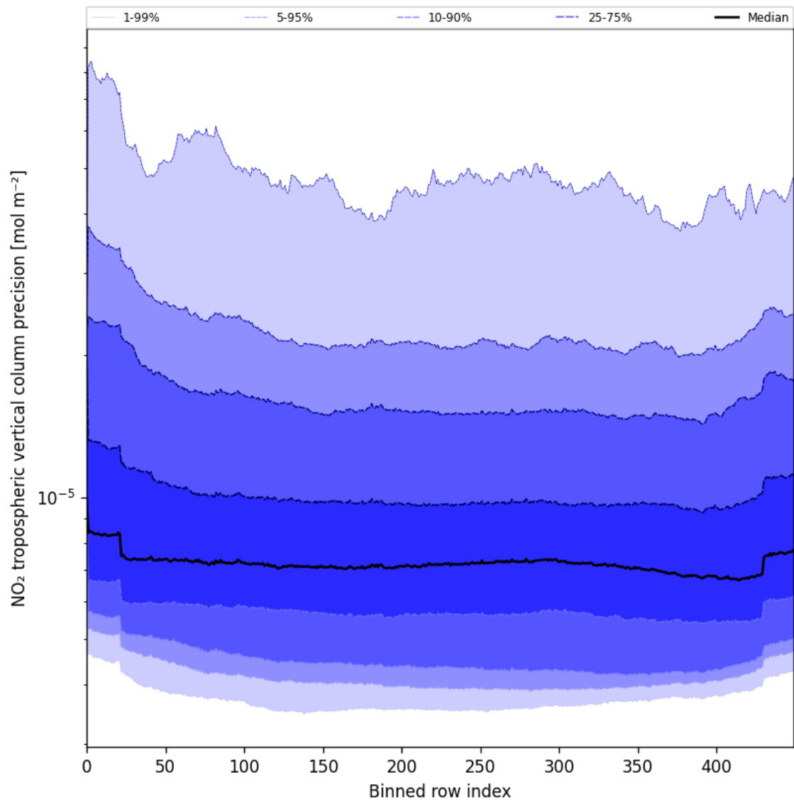
Figure 45: Along track statistics of “NO 2 tropospheric vertical column precision” for 2025-07-01 to 2025-07-02
