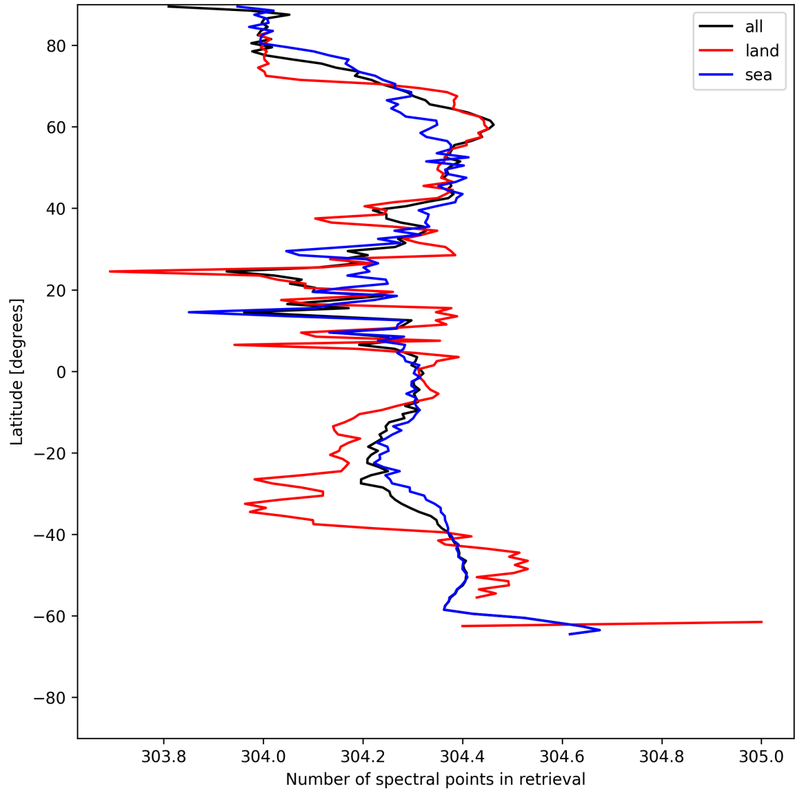
Figure 14: Zonal average of “Number of spectral points in retrieval” for 2025-07-01 to 2025-07-02.
