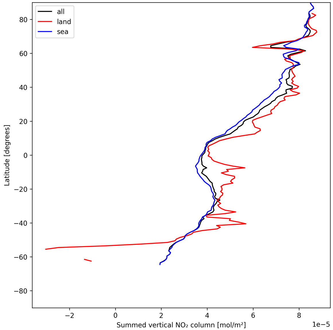
Figure 21: Zonal average of “Summed vertical NO 2 column” for 2025-07-01 to 2025-07-02.
