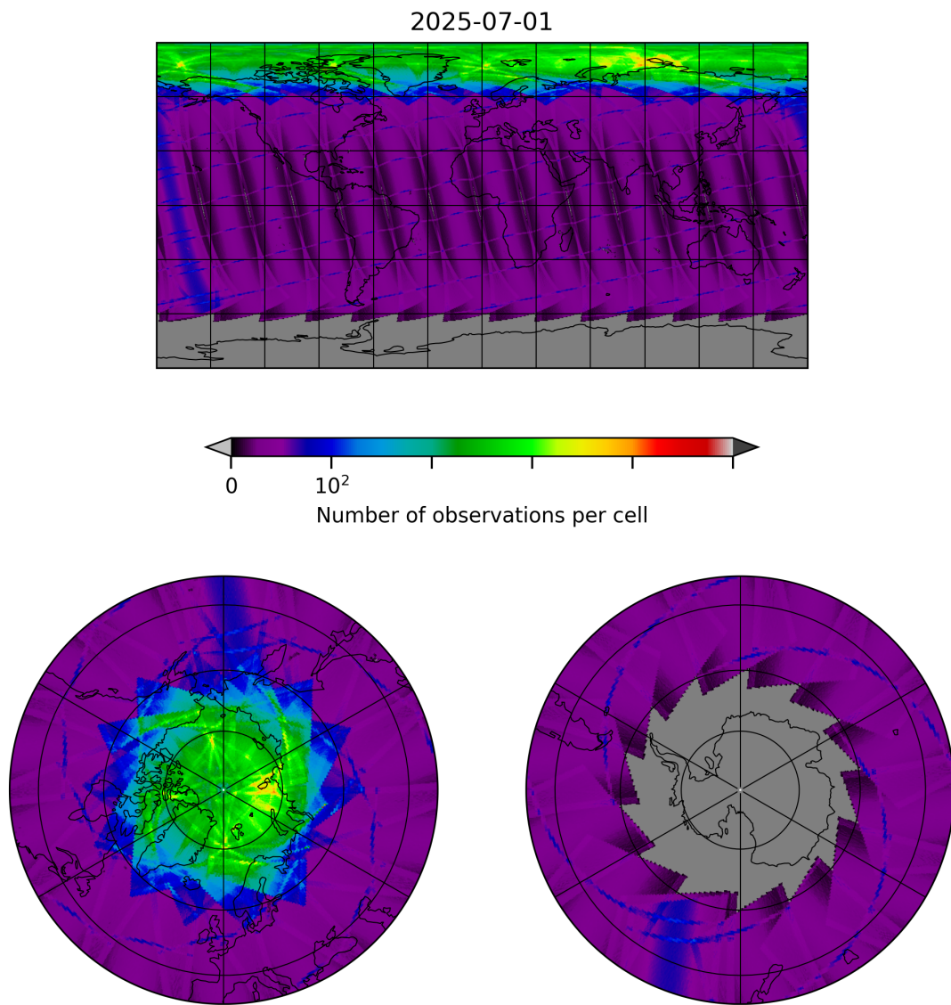
Figure 8: Map of the number of observations for 2025-07-01 to 2025-07-02
