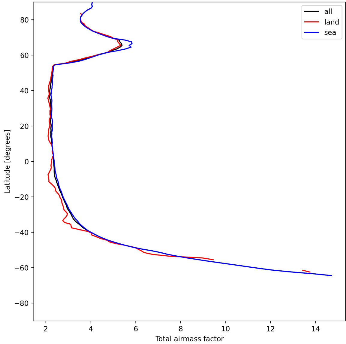
Figure 13: Zonal average of “Total airmass factor” for 2025-07-01 to 2025-07-02.
