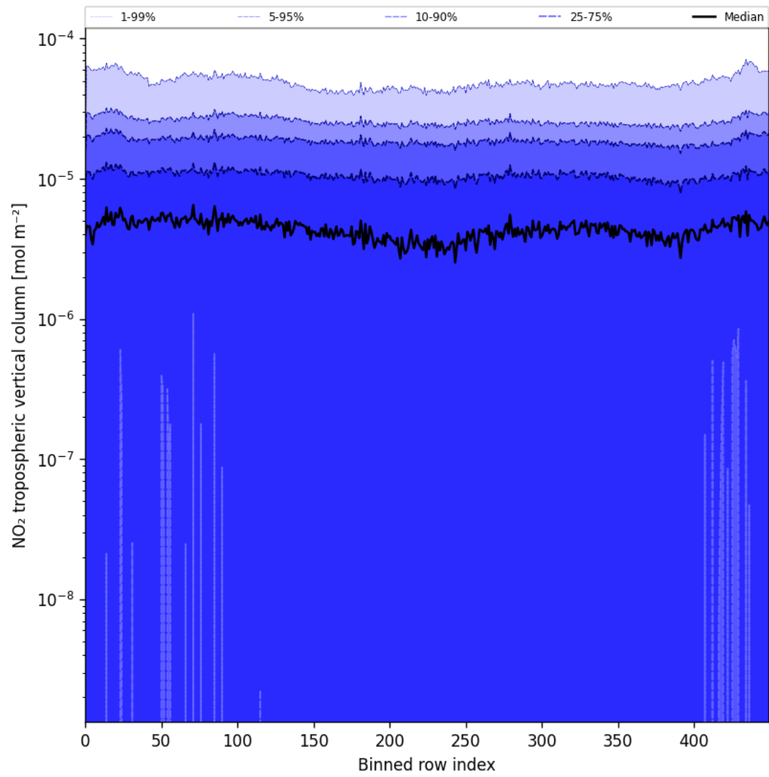
Figure 44: Along track statistics of “NO 2 tropospheric vertical column” for 2025-07-01 to 2025-07-02
