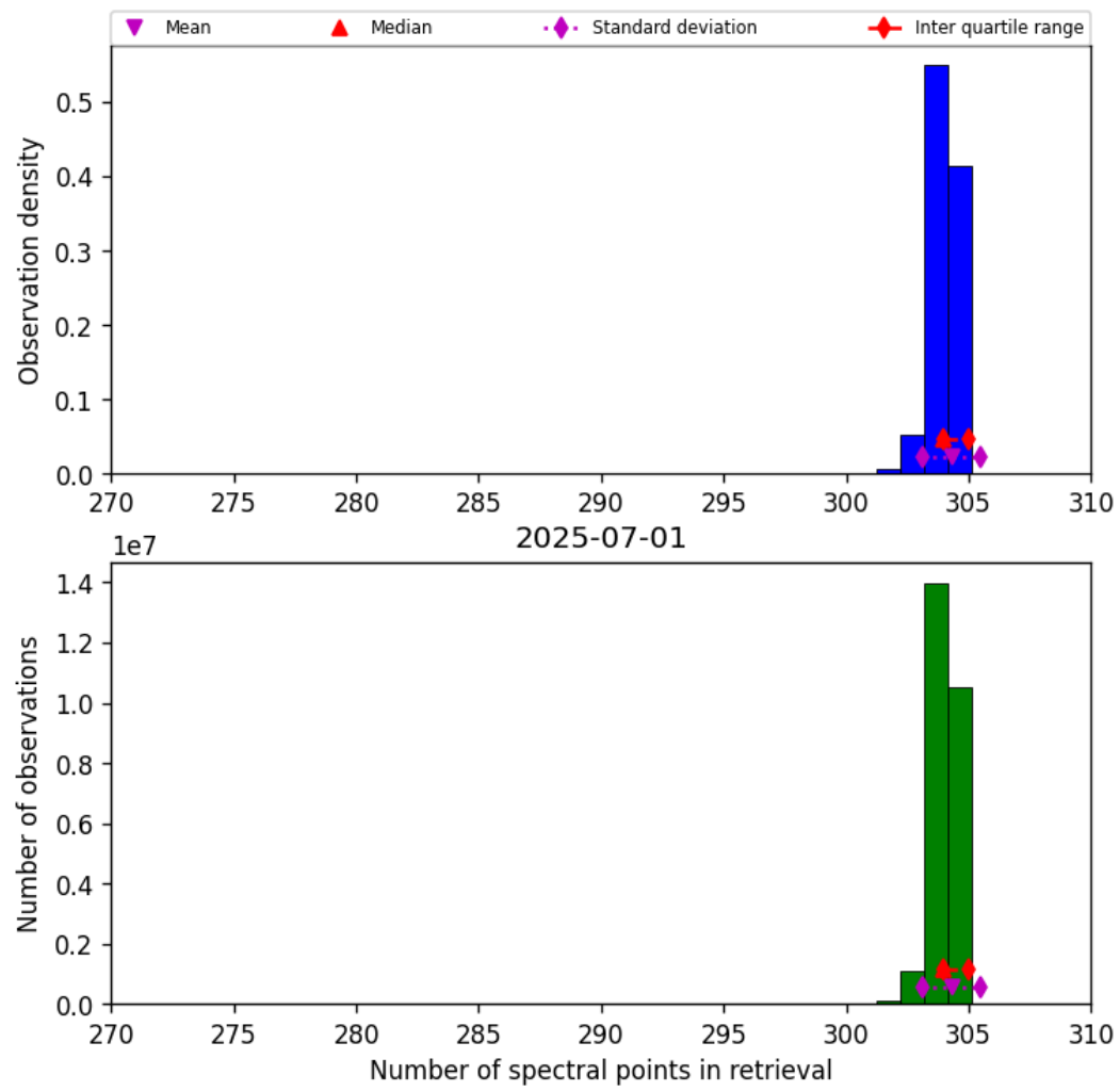
Figure 31: Histogram of “Number of spectral points in retrieval” for 2025-07-01 to 2025-07-02
