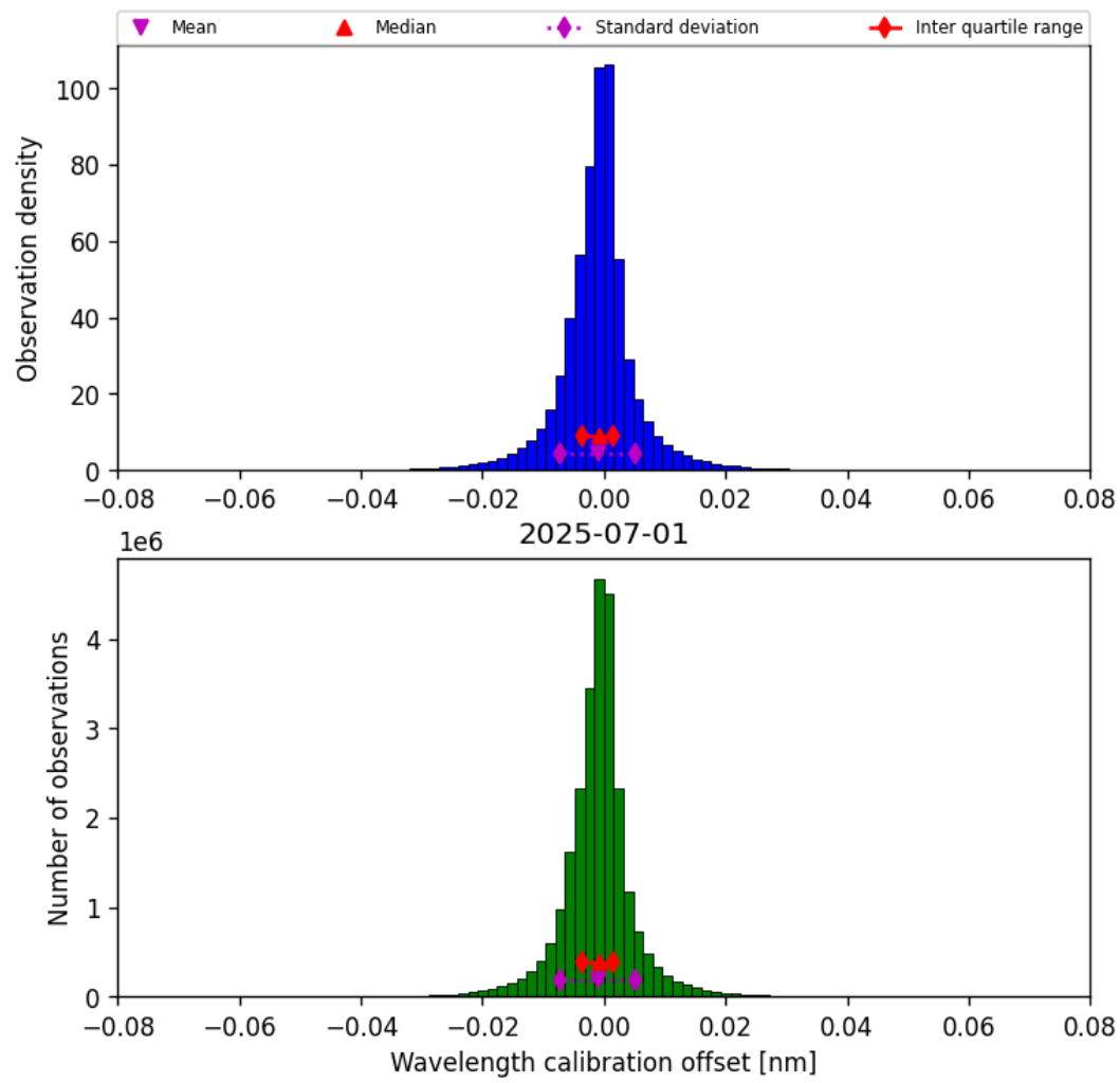
Figure 33: Histogram of “Wavelength calibration offset” for 2025-07-01 to 2025-07-02
