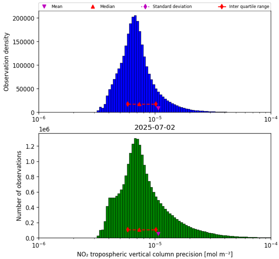
Figure 28: Histogram of “NO 2 tropospheric vertical column precision” for 2025-07-02 to 2025-07-03
