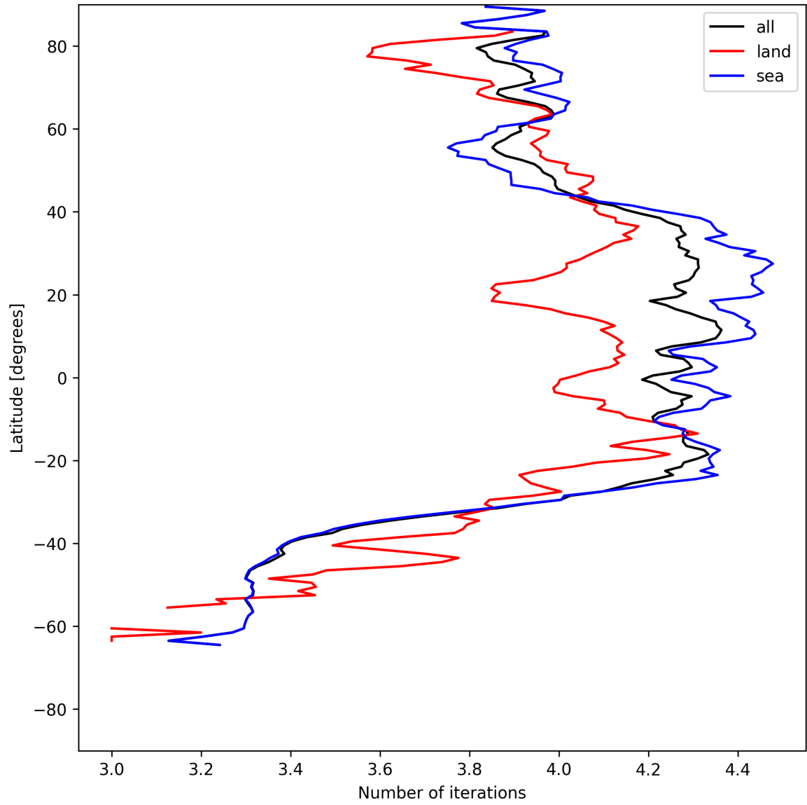
Figure 15: Zonal average of “Number of iterations” for 2025-07-02 to 2025-07-03.
