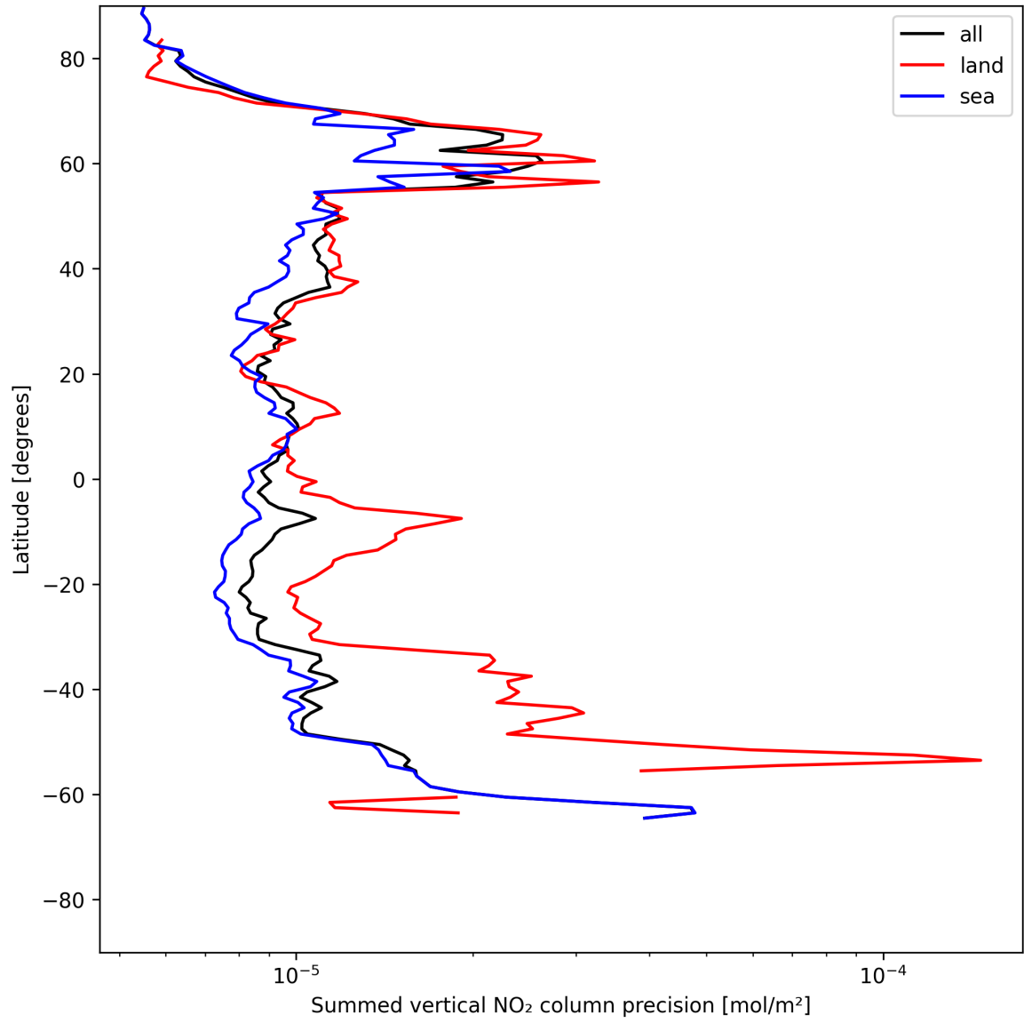
Figure 22: Zonal average of “Summed vertical NO 2 column precision” for 2025-07-02 to 2025-07-03.
