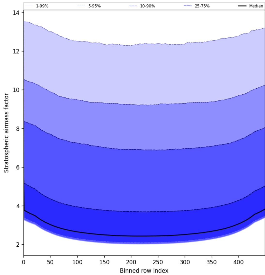
Figure 59: Along track statistics of “Stratospheric airmass factor” for 2025-07-02 to 2025-07-03
