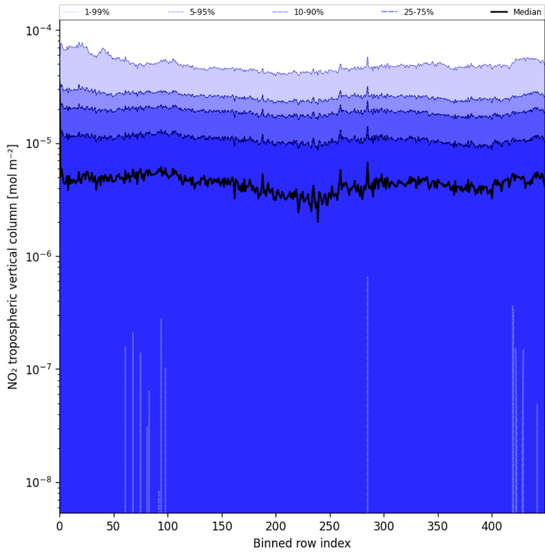
Figure 44: Along track statistics of “ \text{NO}_2 tropospheric vertical column” for 2025-07-02 to 2025-07-03
