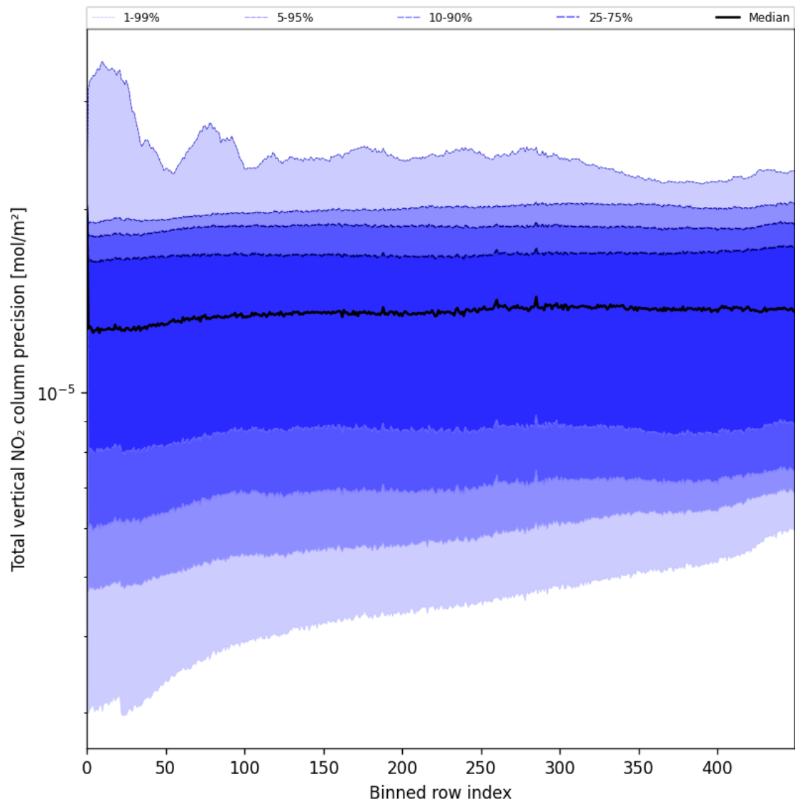
Figure 54: Along track statistics of “Total vertical NO 2 column precision” for 2025-07-02 to 2025-07-03
