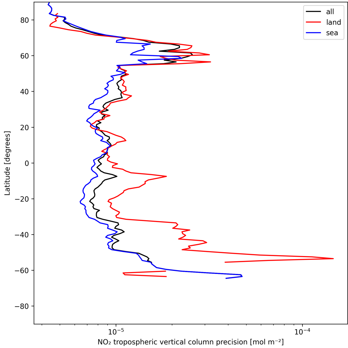
Figure 11: Zonal average of “NO 2 tropospheric vertical column precision” for 2025-07-02 to 2025-07-03.
