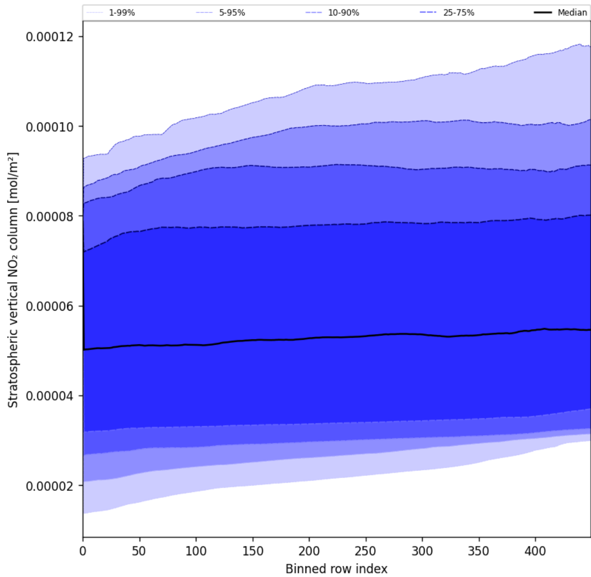
Figure 51: Along track statistics of “Stratospheric vertical NO 2 column” for 2025-07-02 to 2025-07-03
