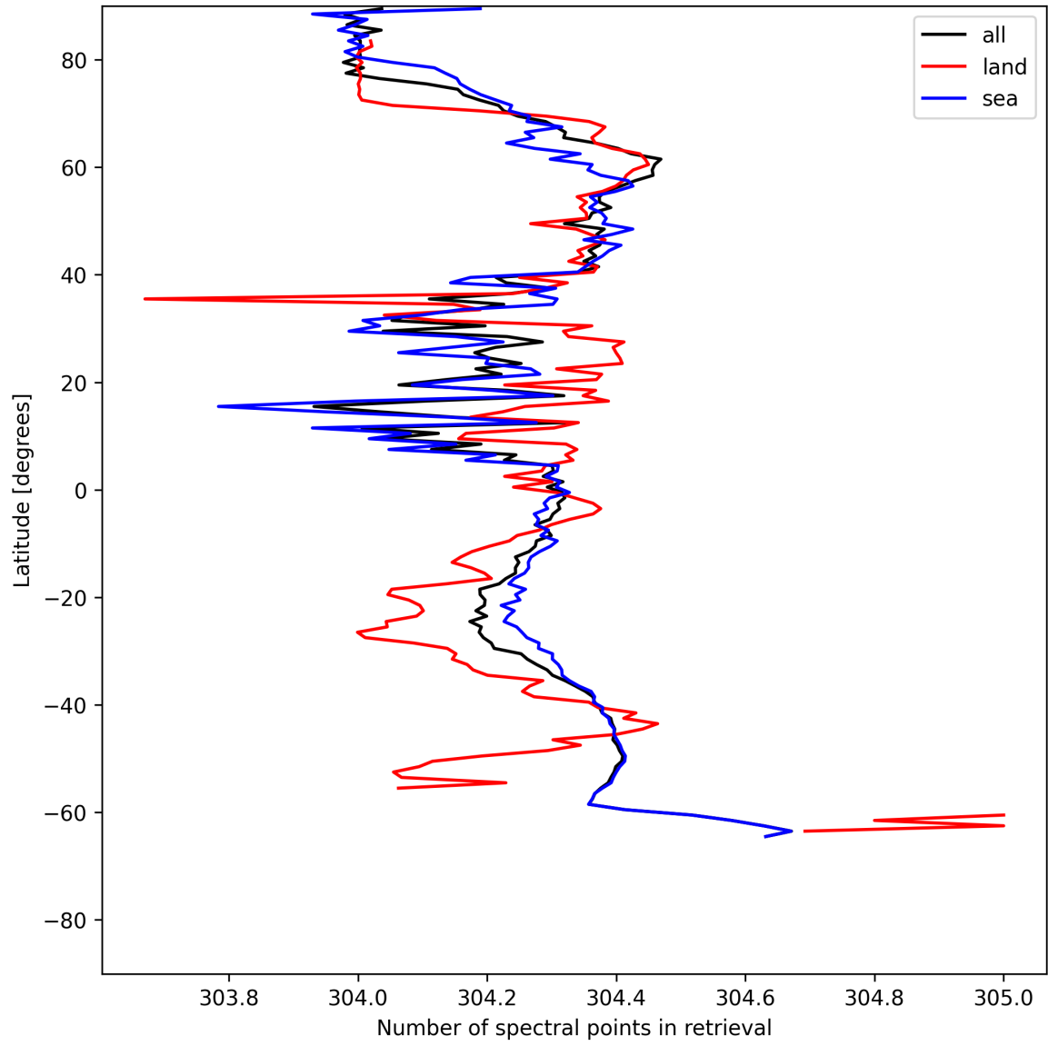
Figure 14: Zonal average of “Number of spectral points in retrieval” for 2025-07-02 to 2025-07-03.
