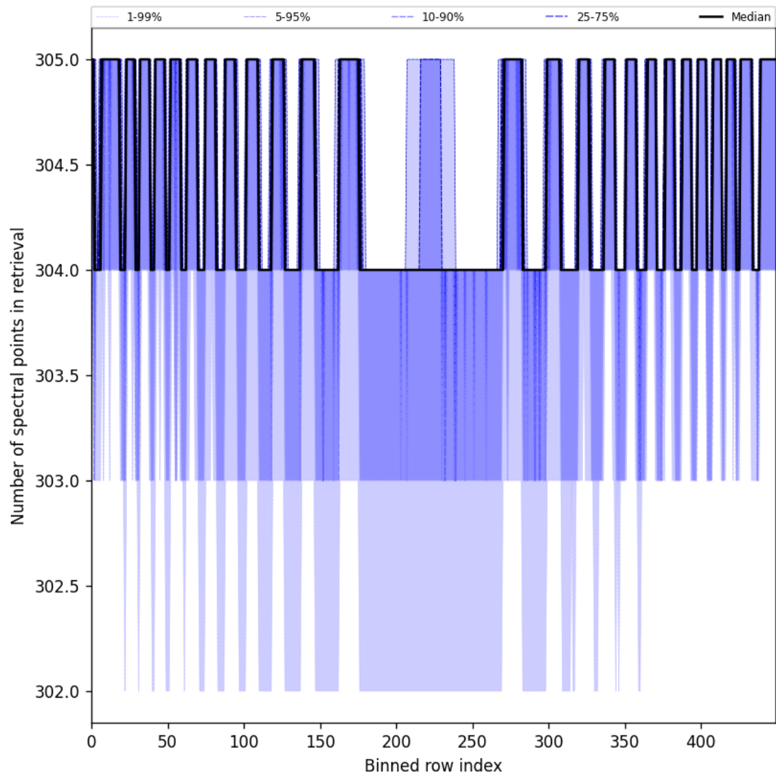
Figure 48: Along track statistics of “Number of spectral points in retrieval” for 2025-07-02 to 2025-07-03
