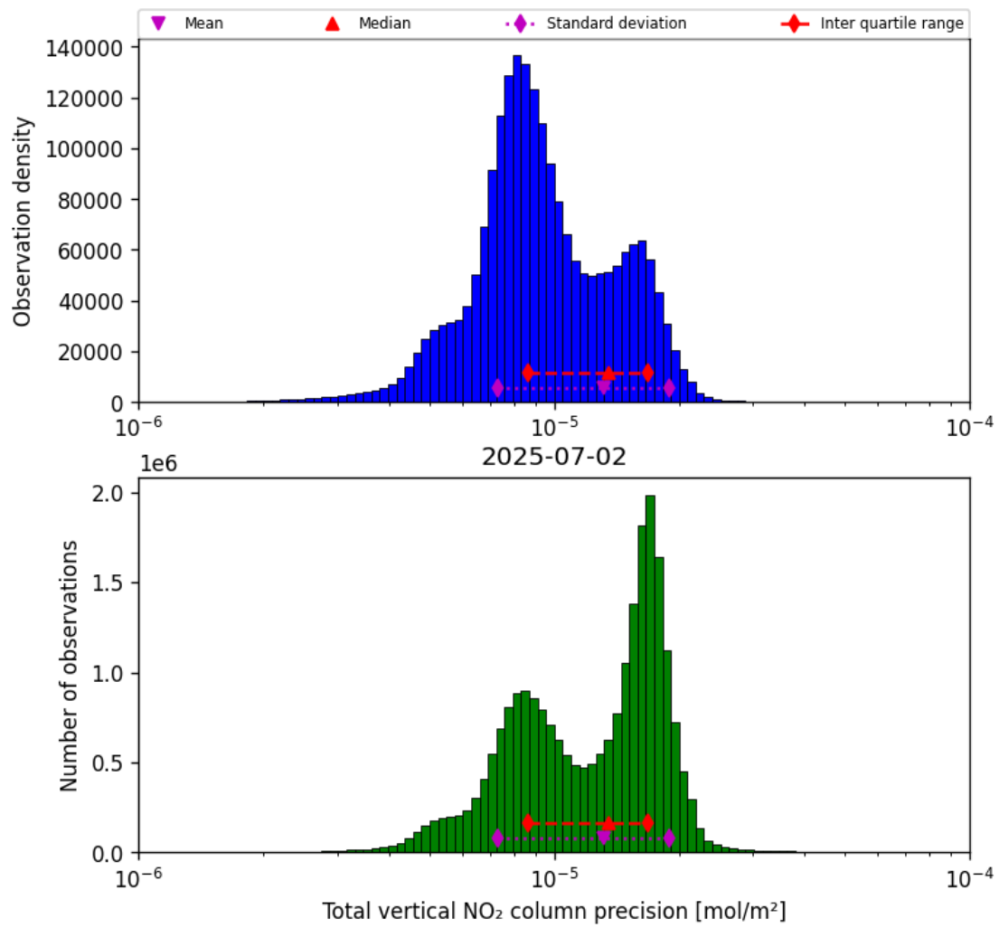
Figure 37: Histogram of “Total vertical NO 2 column precision” for 2025-07-02 to 2025-07-03
