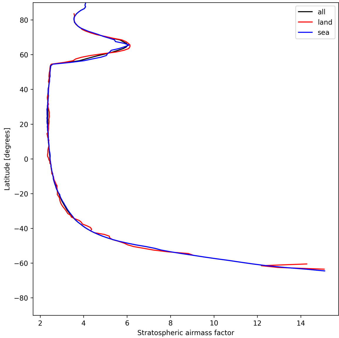
Figure 25: Zonal average of “Stratospheric air mass factor” for 2025-07-02 to 2025-07-03.
