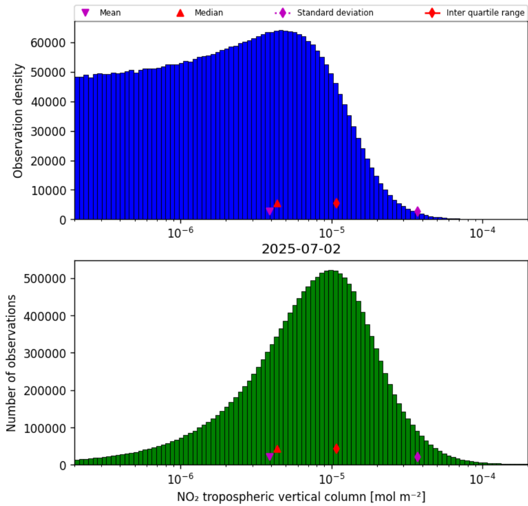
Figure 27: Histogram of “NO 2 tropospheric vertical column” for 2025-07-02 to 2025-07-03
