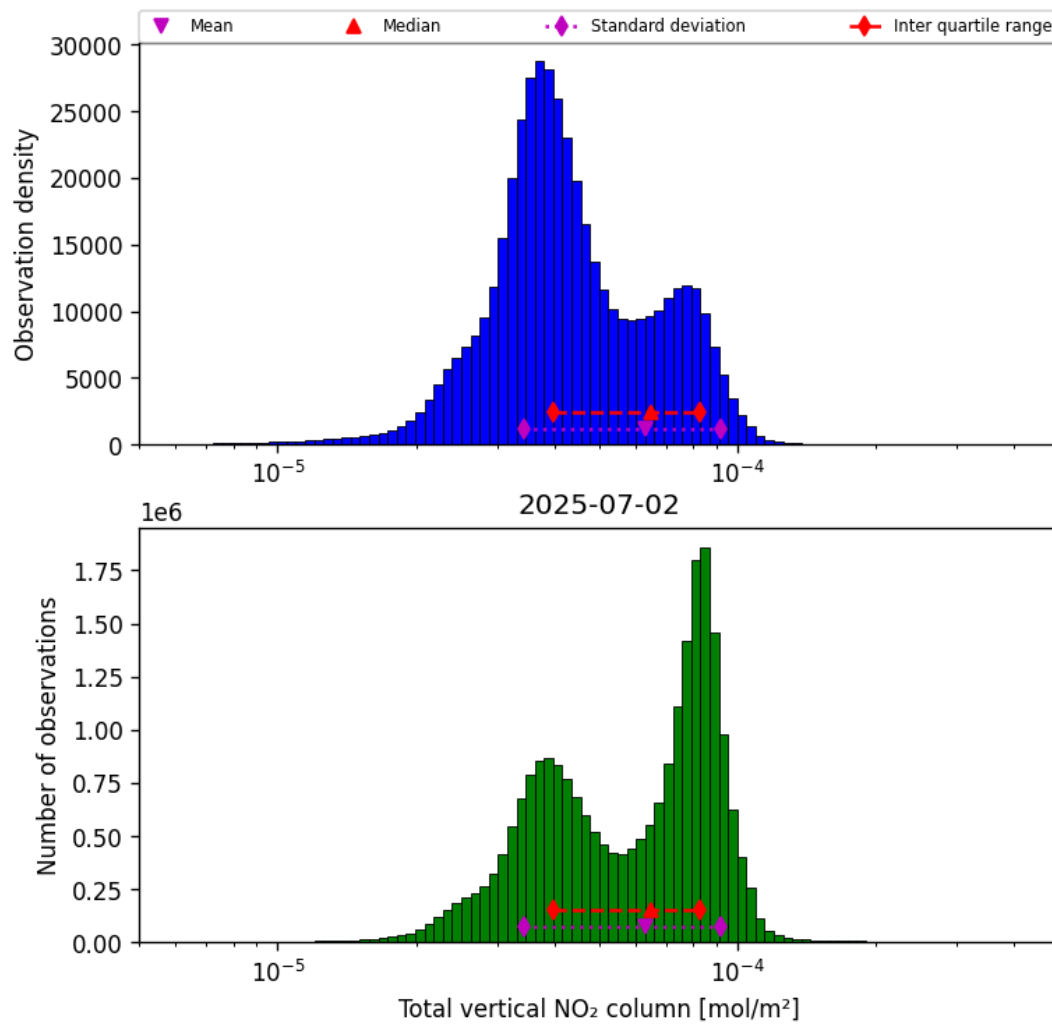
Figure 36: Histogram of “Total vertical NO 2 column” for 2025-07-02 to 2025-07-03
