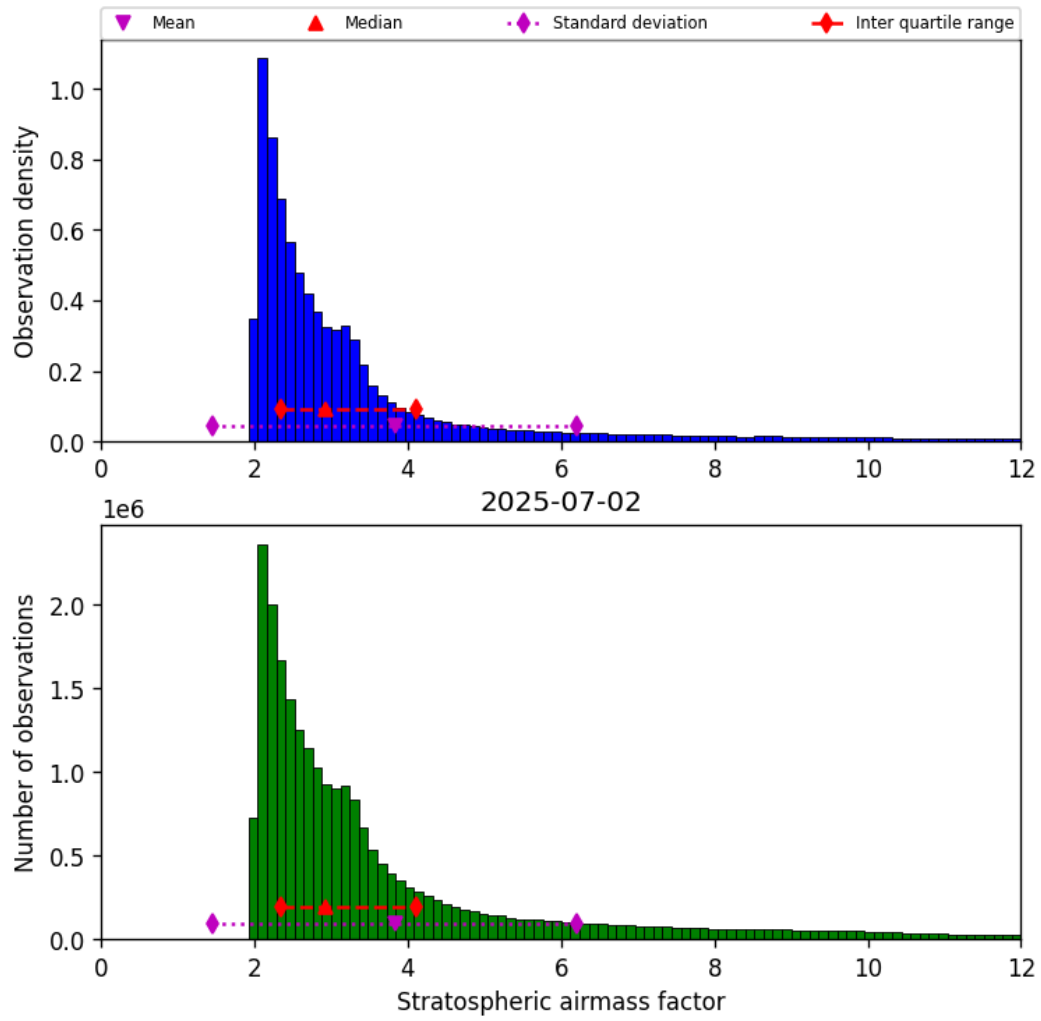
Figure 42: Histogram of “Stratospheric airmass factor” for 2025-07-02 to 2025-07-03
