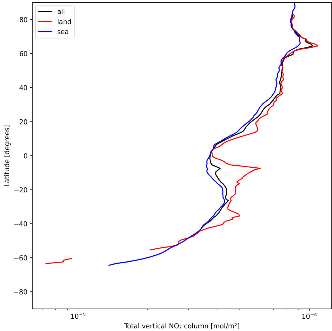
Figure 19: Zonal average of “Total vertical NO 2 column” for 2025-07-02 to 2025-07-03.
