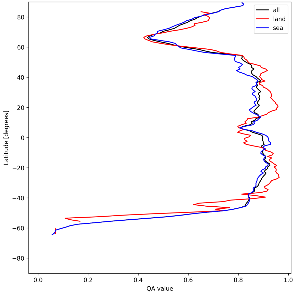
Figure 9: Zonal average of “QA value” for 2025-07-02 to 2025-07-03.
