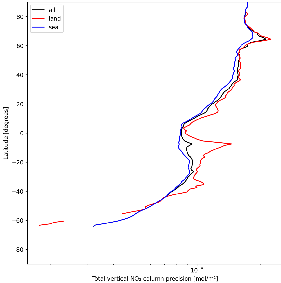
Figure 20: Zonal average of “Total vertical NO 2 column precision” for 2025-07-02 to 2025-07-03.
