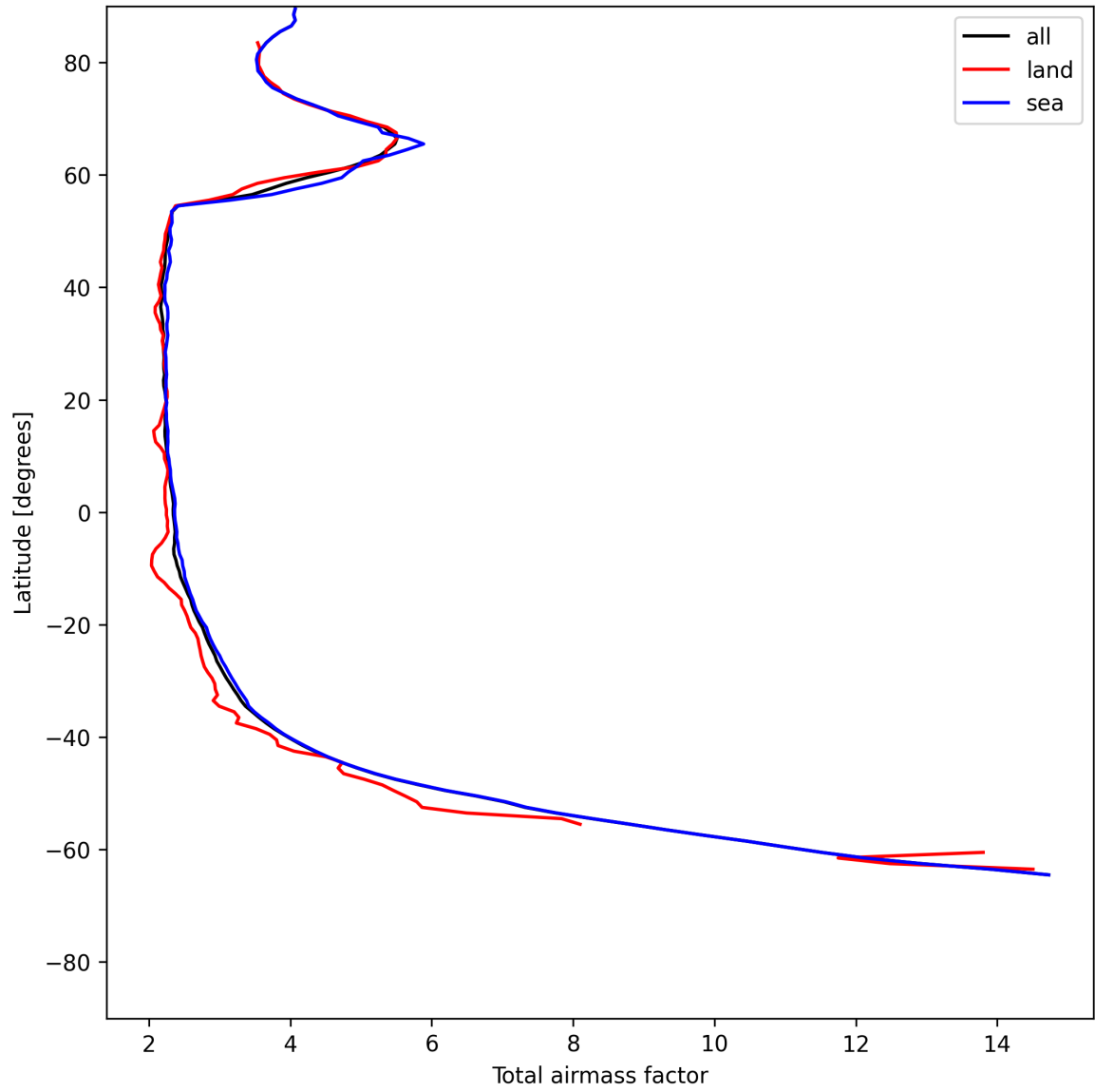
Figure 13: Zonal average of “Total airmass factor” for 2025-07-02 to 2025-07-03.
