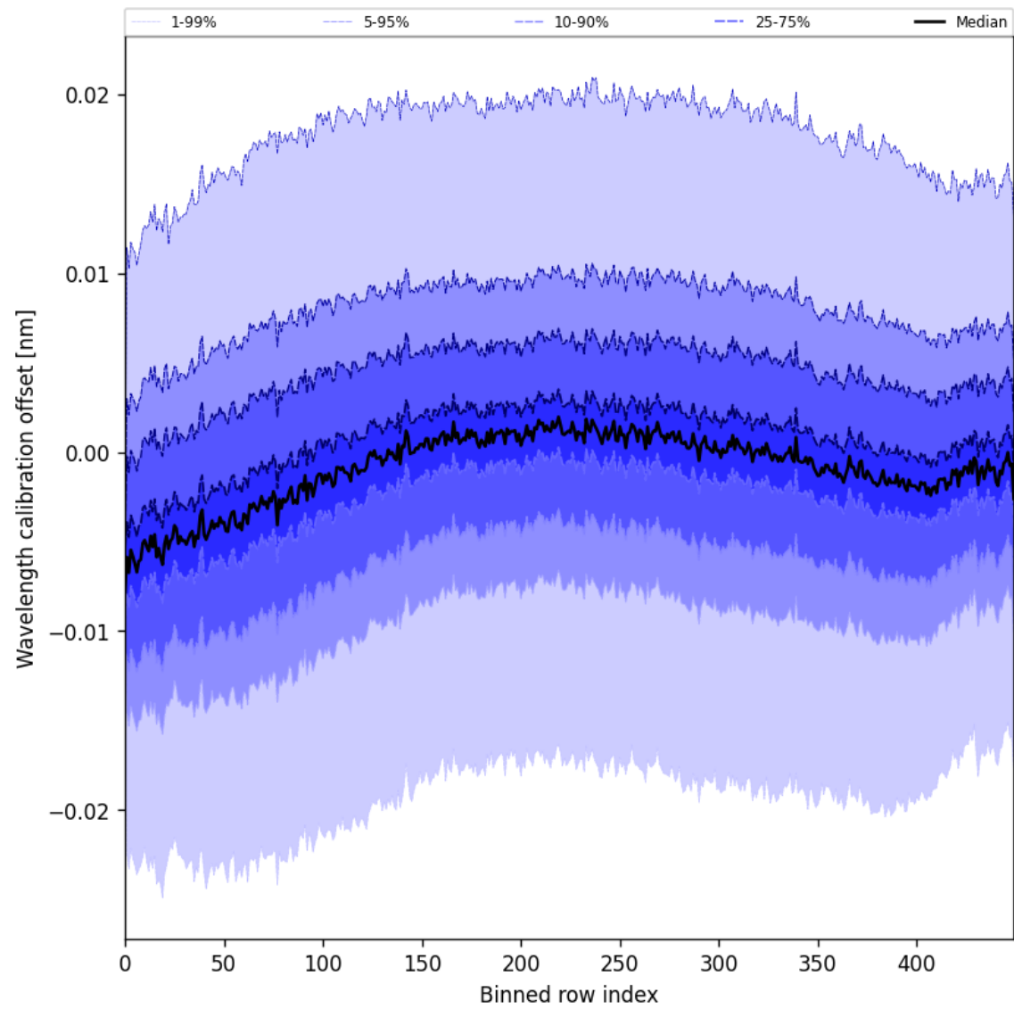
Figure 50: Along track statistics of “Wavelength calibration offset” for 2025-07-02 to 2025-07-03
