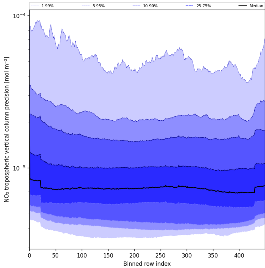
Figure 45: Along track statistics of “NO 2 tropospheric vertical column precision” for 2025-07-02 to 2025-07-03
