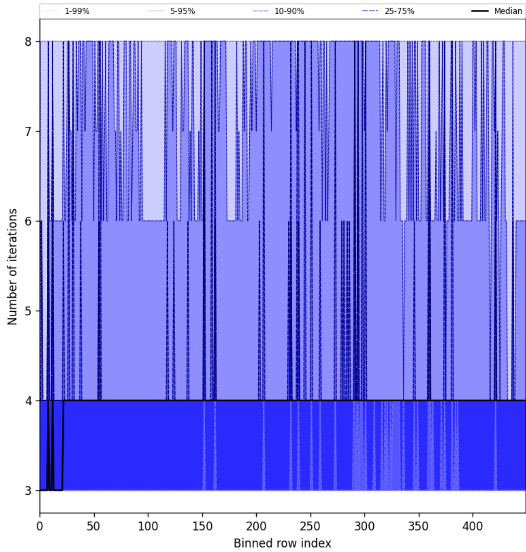
Figure 49: Along track statistics of “Number of iterations” for 2025-07-02 to 2025-07-03
