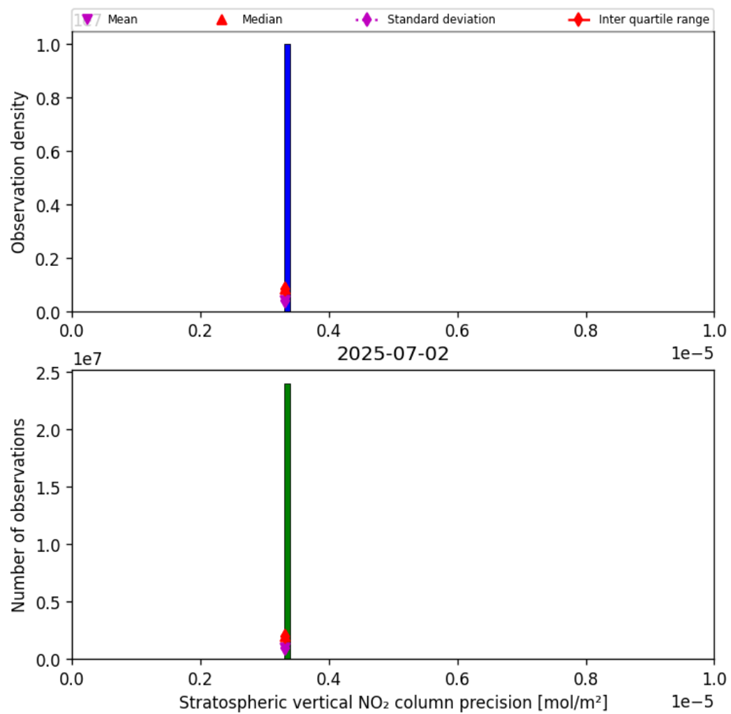
Figure 35: Histogram of “Stratospheric vertical NO 2 column precision” for 2025-07-02 to 2025-07-03
