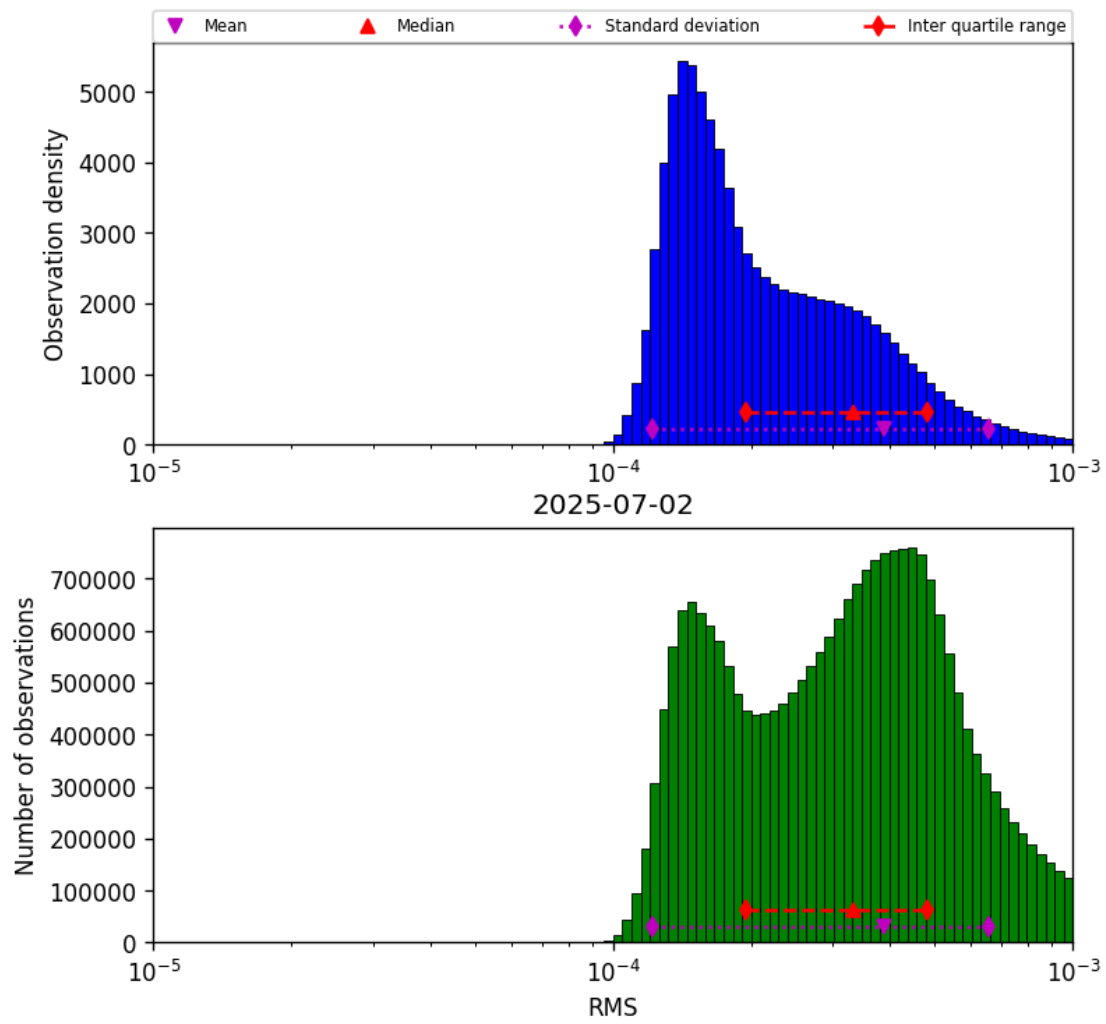
Figure 41: Histogram of “RMS” for 2025-07-02 to 2025-07-03
