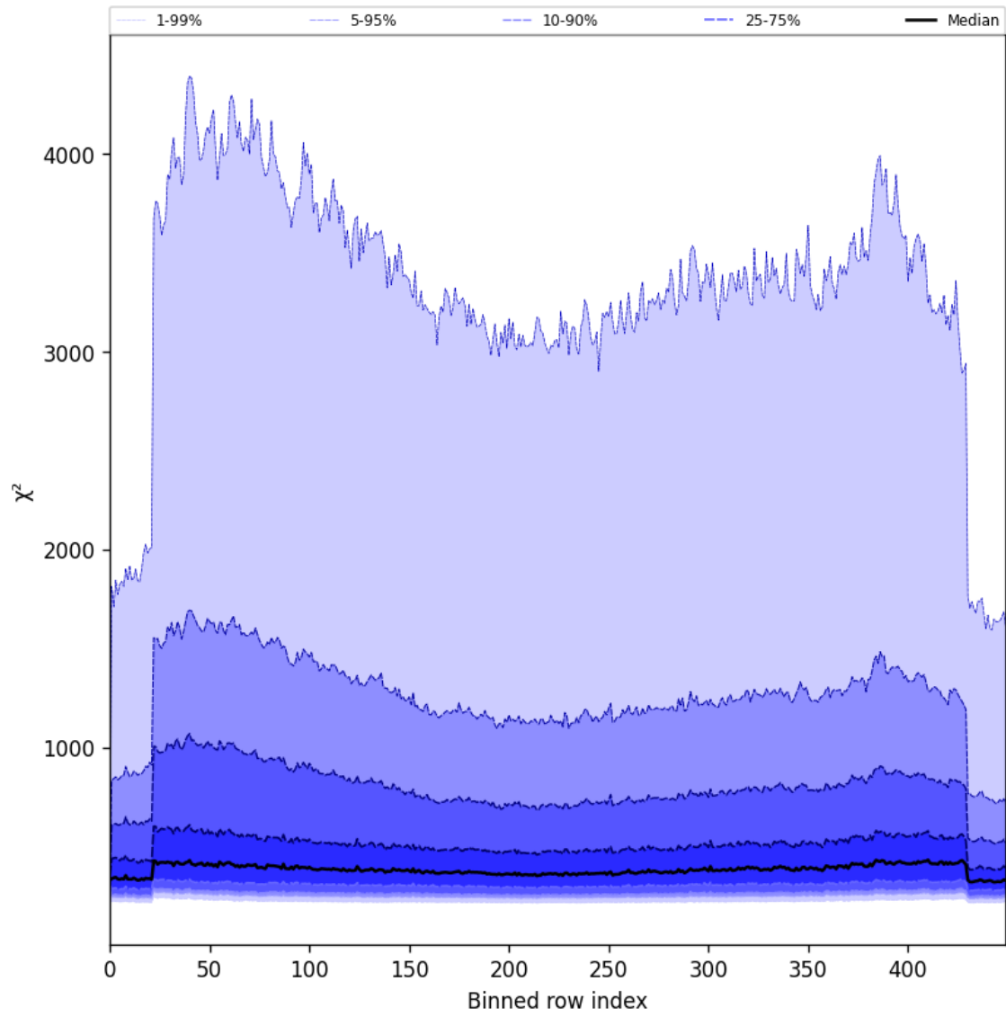
Figure 57: Along track statistics of “ \chi^2 ” for 2025-07-02 to 2025-07-03
