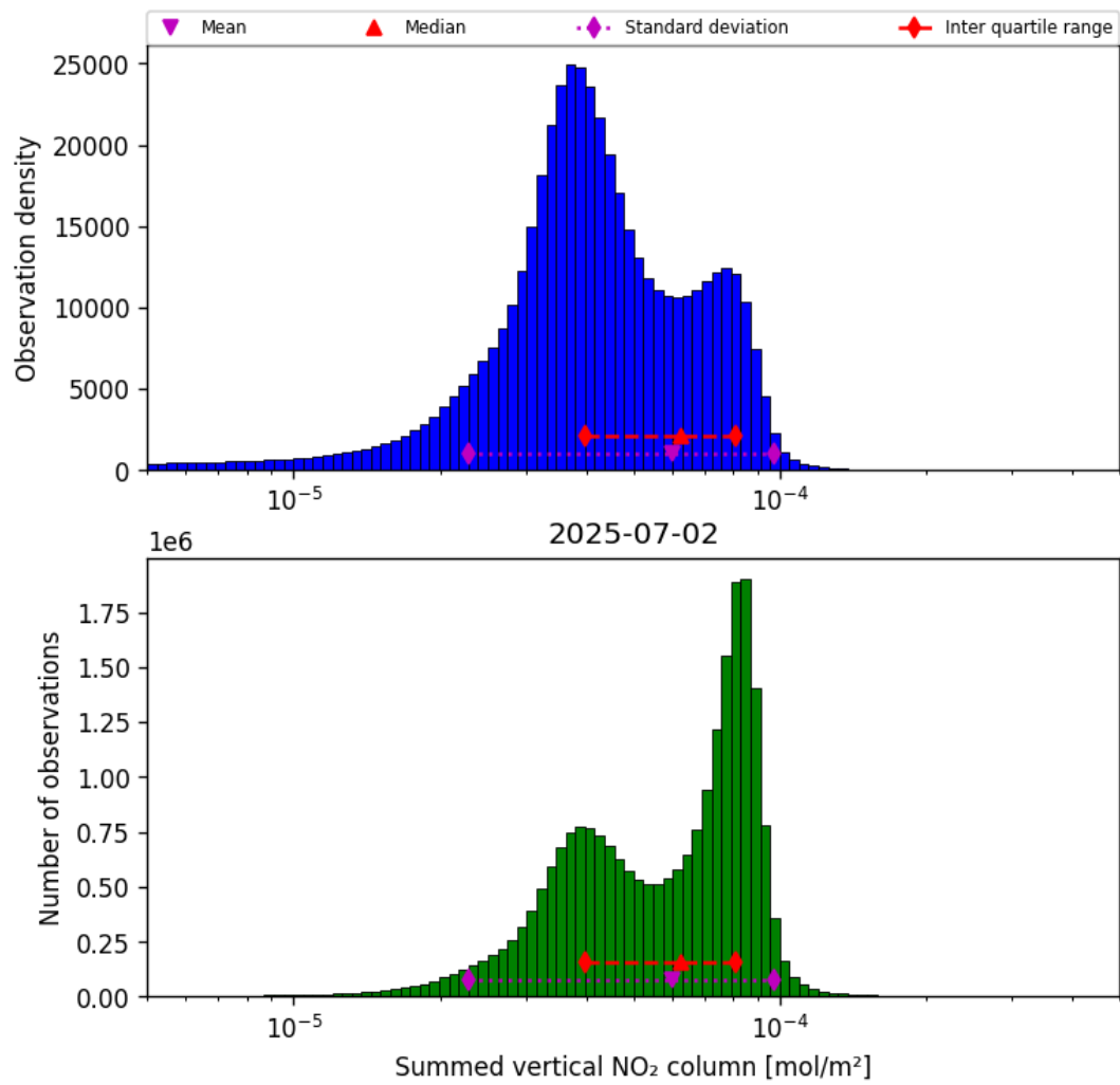
Figure 38: Histogram of “Summed vertical NO 2 column” for 2025-07-02 to 2025-07-03
