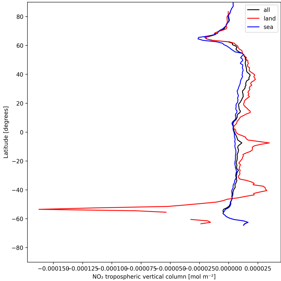
Figure 10: Zonal average of “NO 2 tropospheric vertical column” for 2025-07-02 to 2025-07-03.
