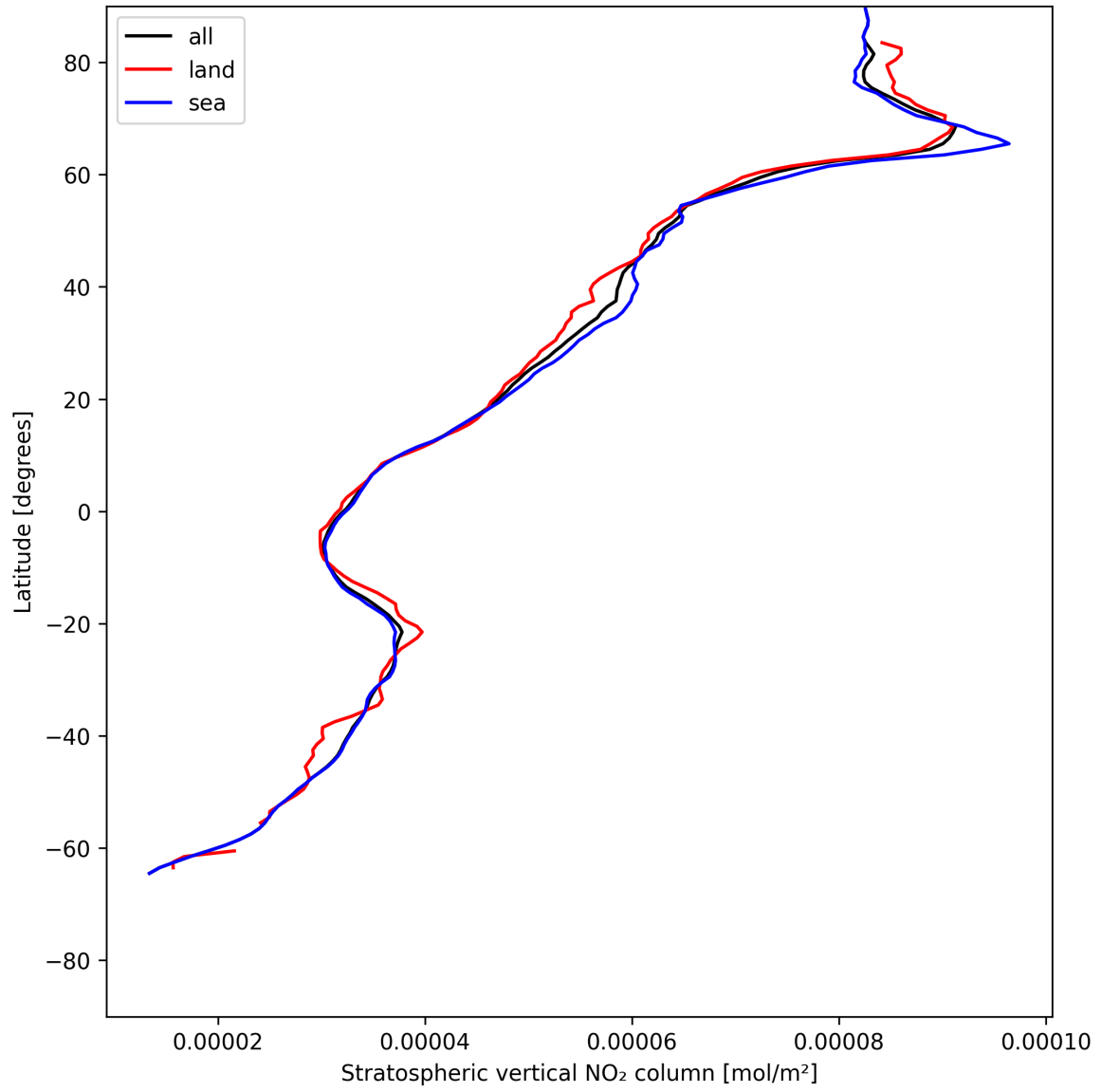
Figure 17: Zonal average of “Stratospheric vertical NO 2 column” for 2025-07-02 to 2025-07-03.
