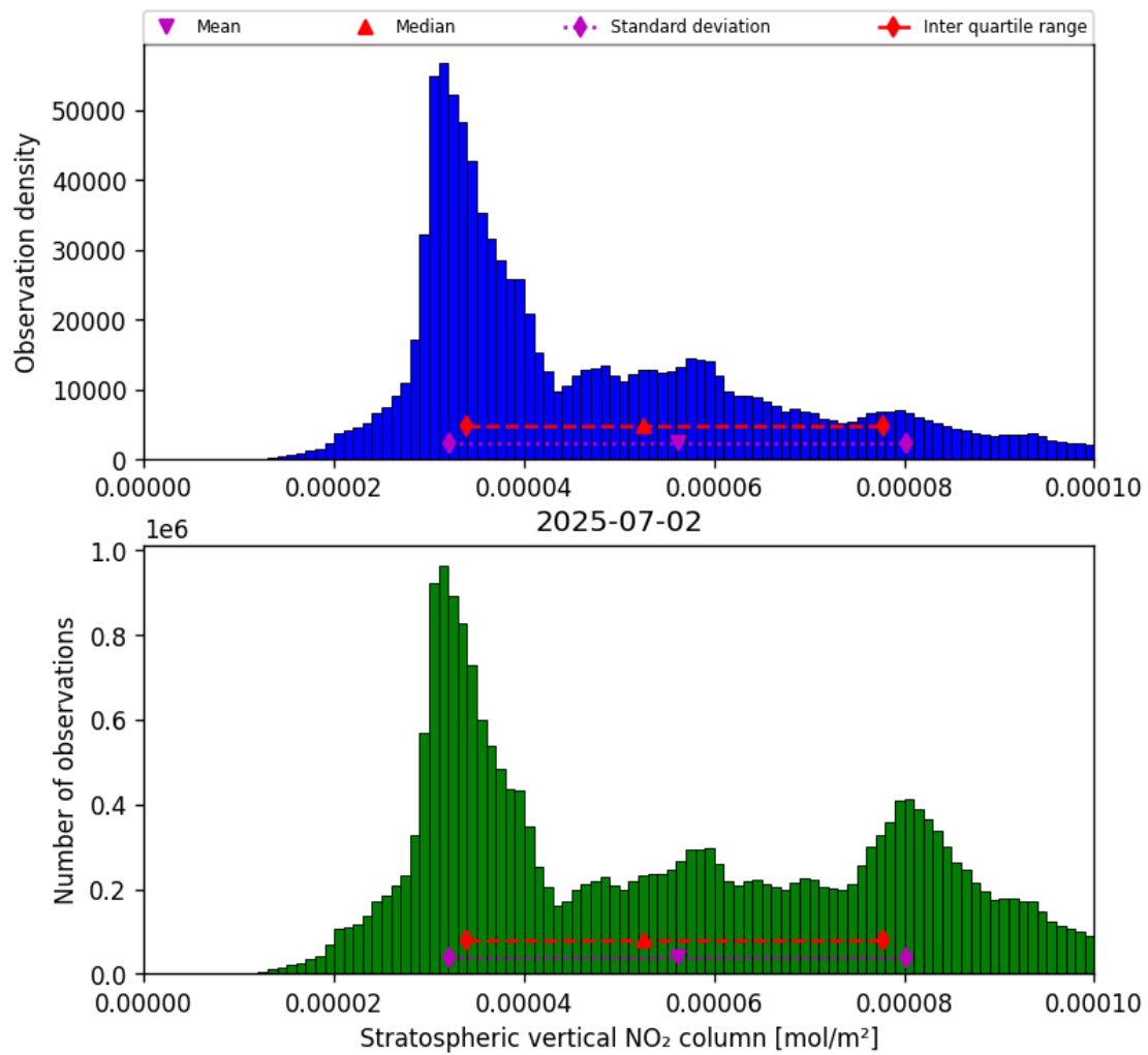
Figure 34: Histogram of “Stratospheric vertical NO 2 column” for 2025-07-02 to 2025-07-03
