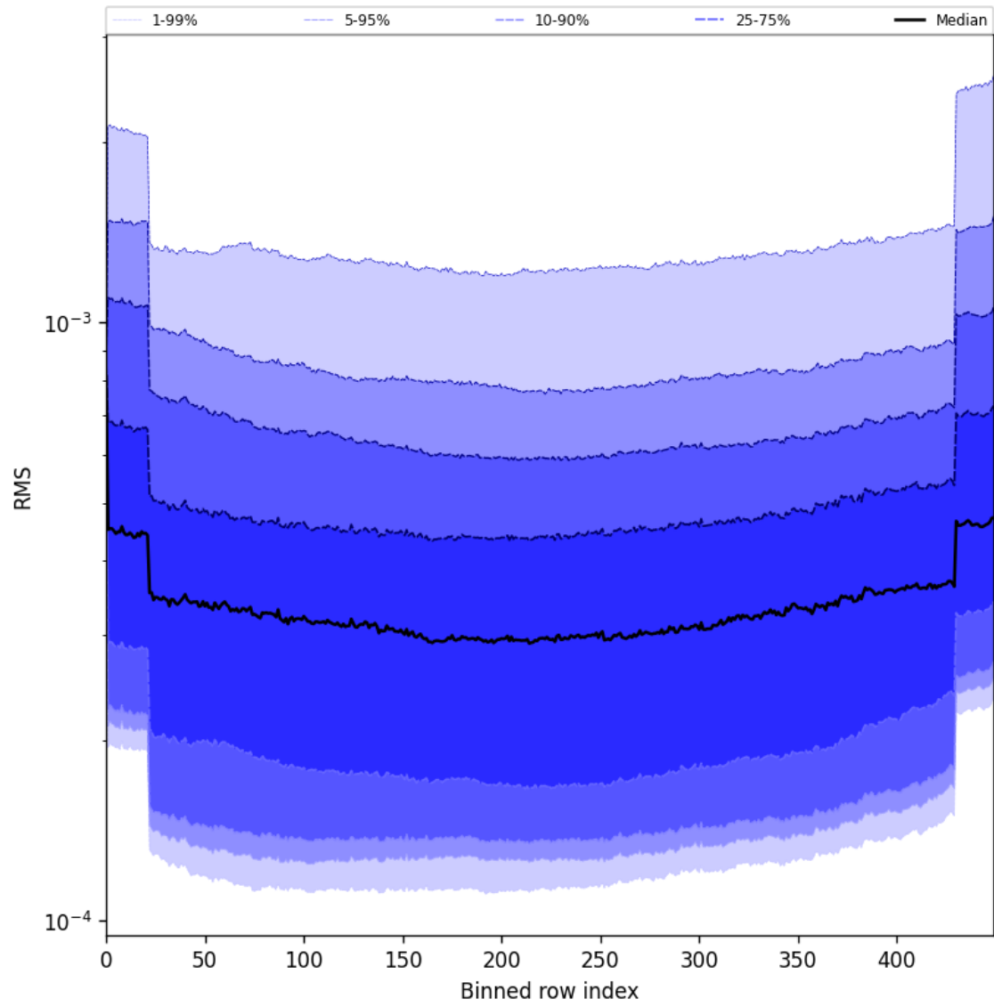
Figure 58: Along track statistics of “RMS” for 2025-07-02 to 2025-07-03
