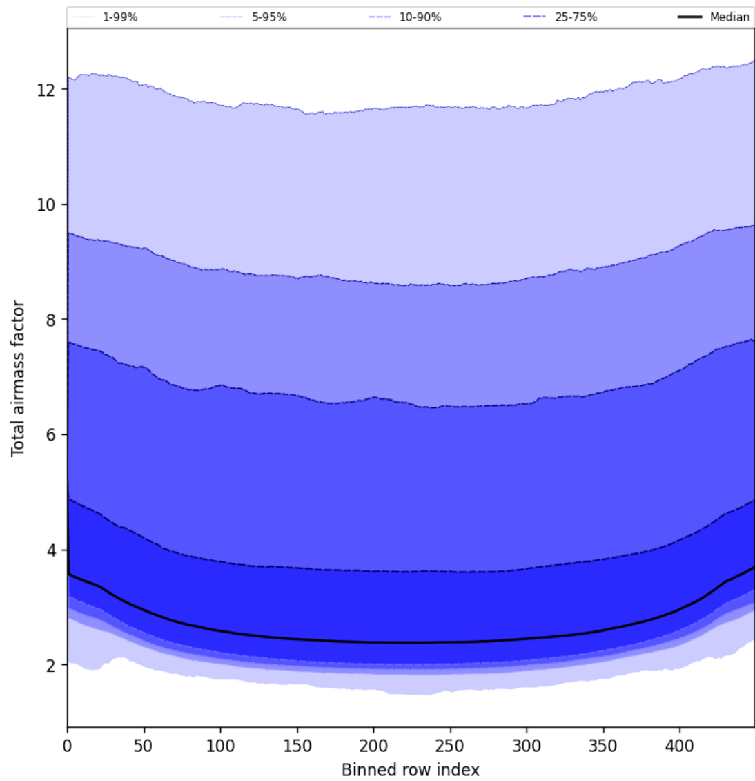
Figure 47: Along track statistics of “Total airmass factor” for 2025-07-02 to 2025-07-03
