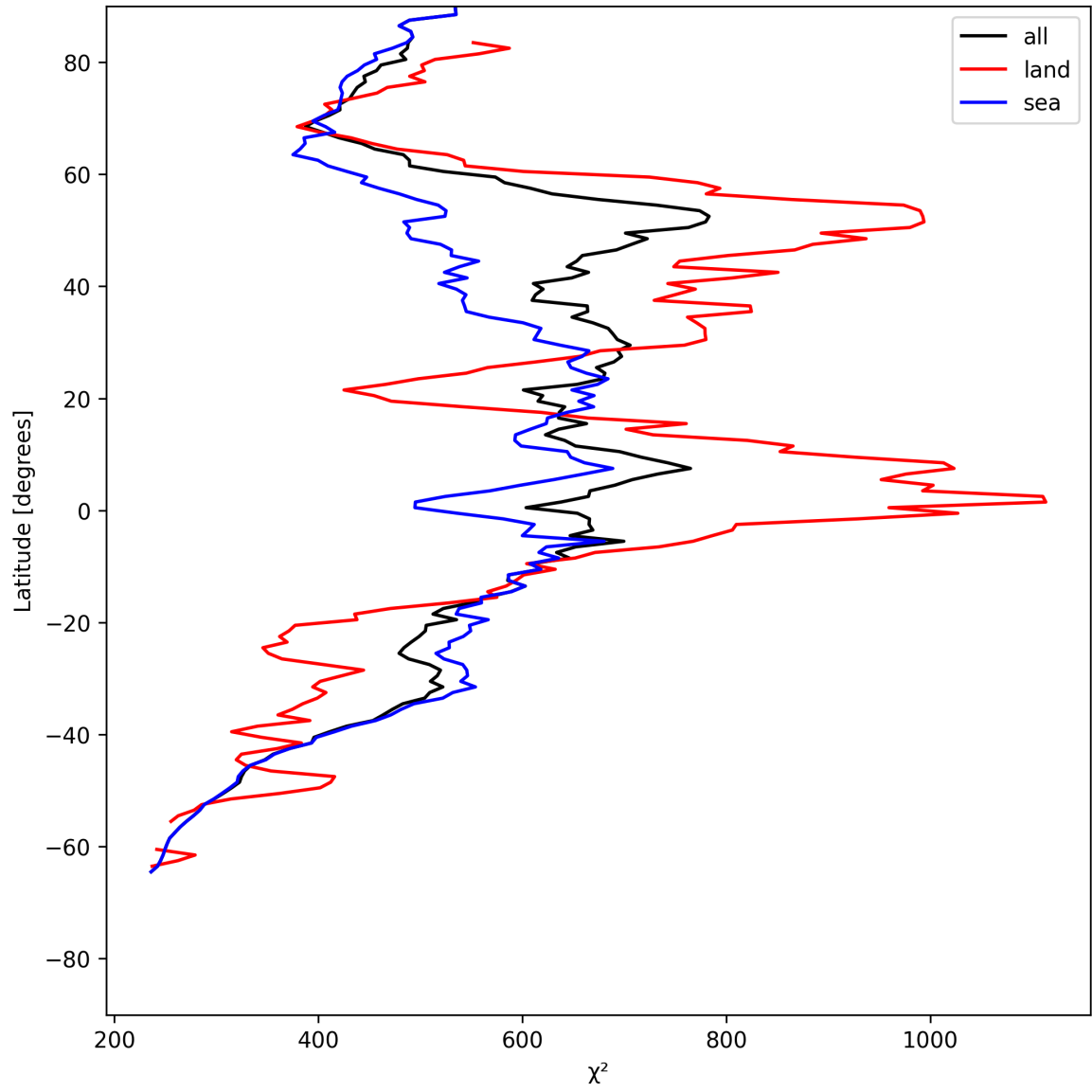
Figure 23: Zonal average of “ \chi^2 ” for 2025-07-02 to 2025-07-03.
