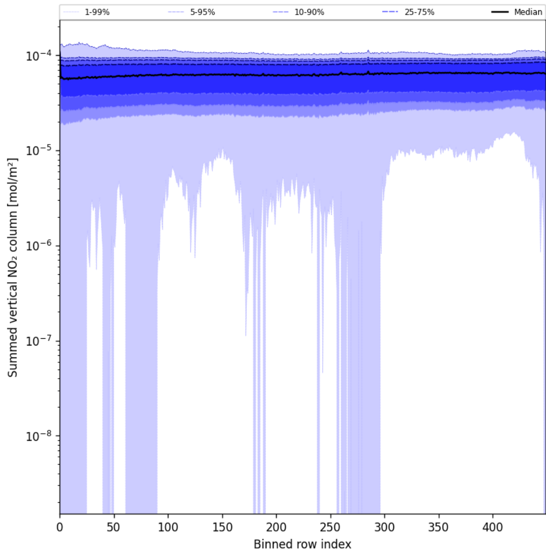
Figure 55: Along track statistics of “Summed vertical NO 2 column” for 2025-07-02 to 2025-07-03
