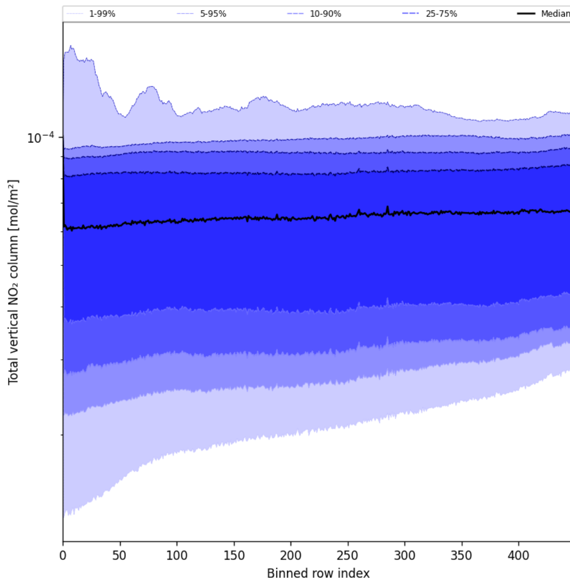
Figure 53: Along track statistics of “Total vertical NO 2 column” for 2025-07-02 to 2025-07-03
