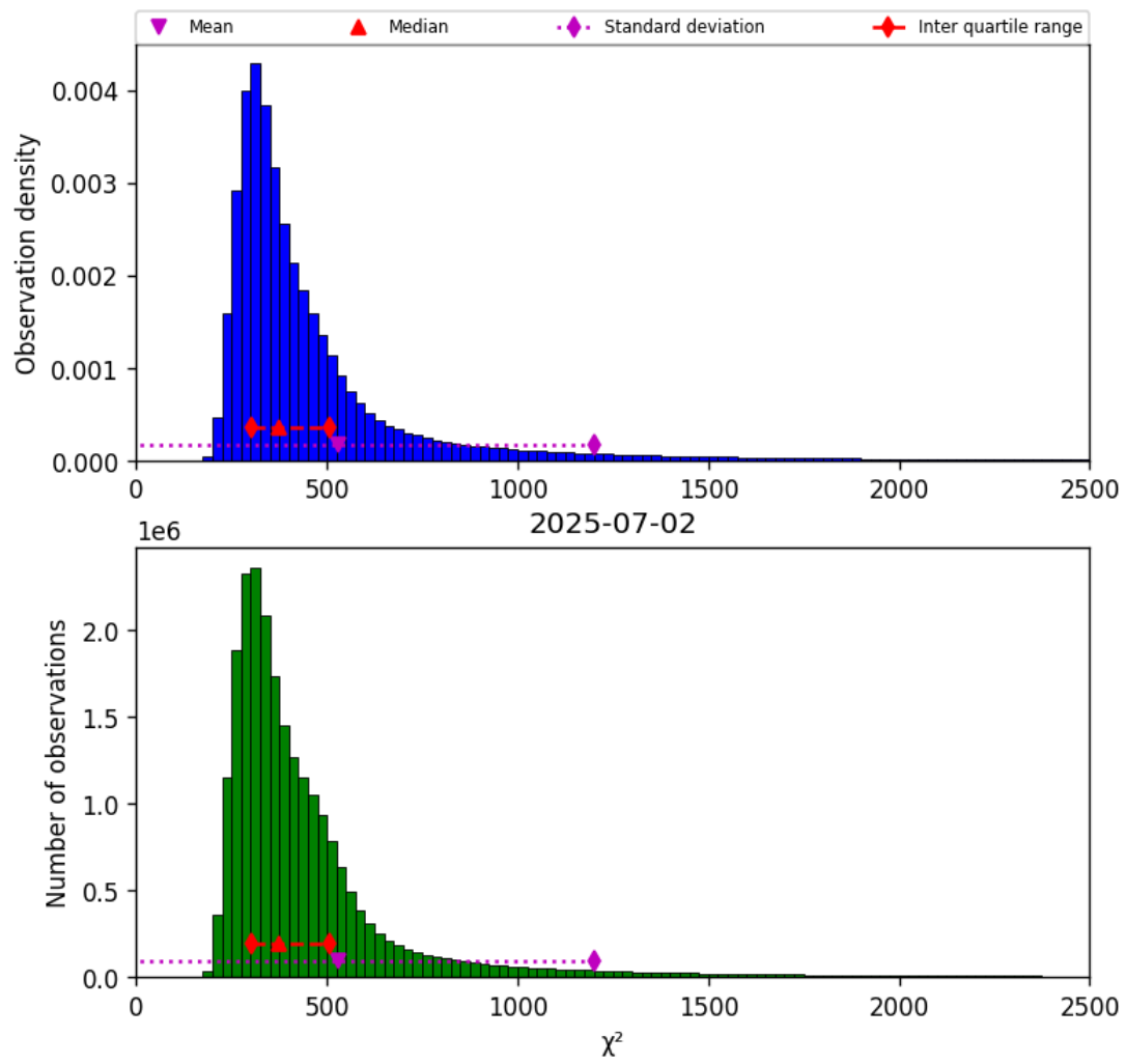
Figure 40: Histogram of “ \chi^2 ” for 2025-07-02 to 2025-07-03
