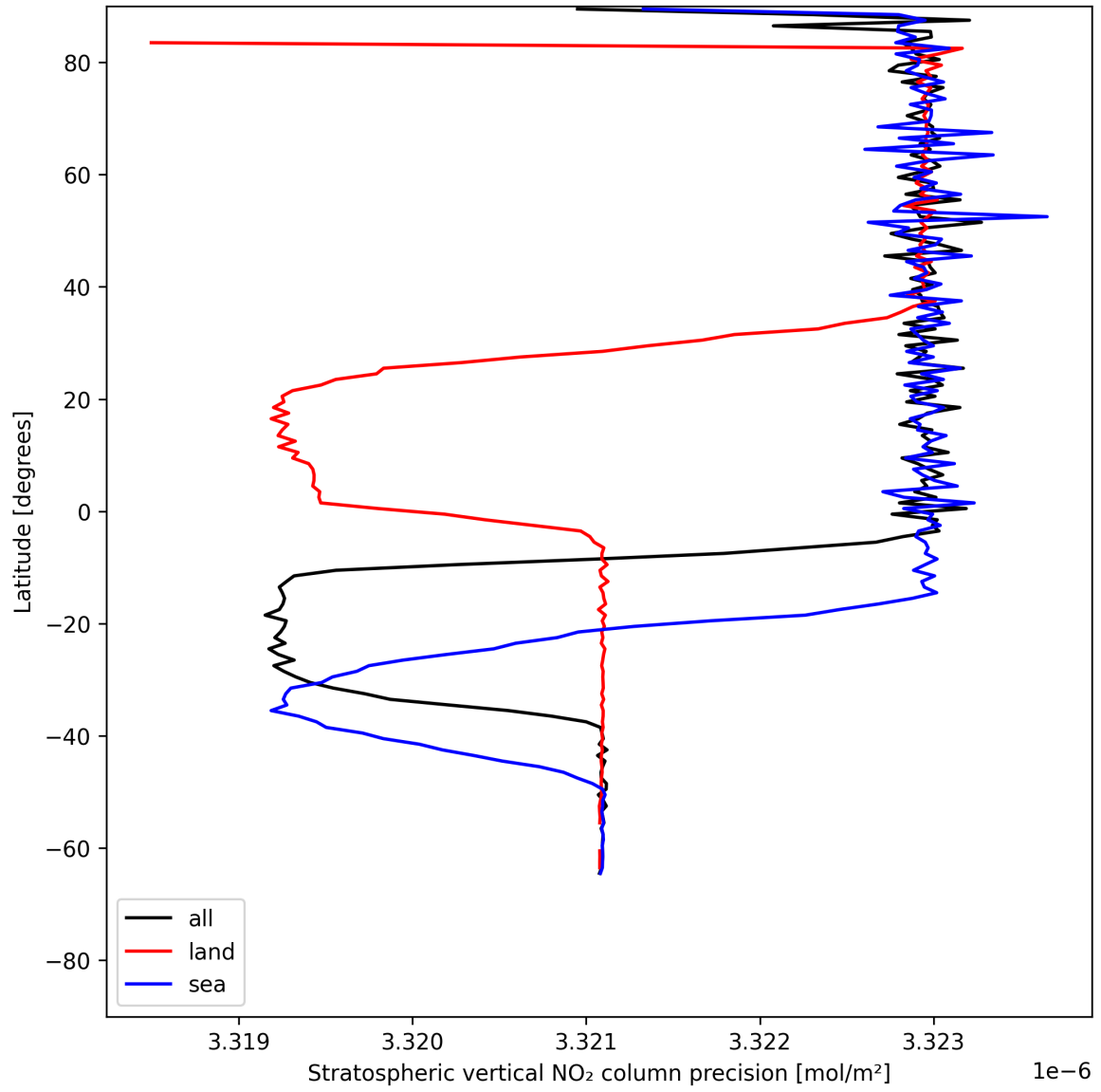
Figure 18: Zonal average of “Stratospheric vertical NO 2 column precision” for 2025-07-02 to 2025-07-03.
