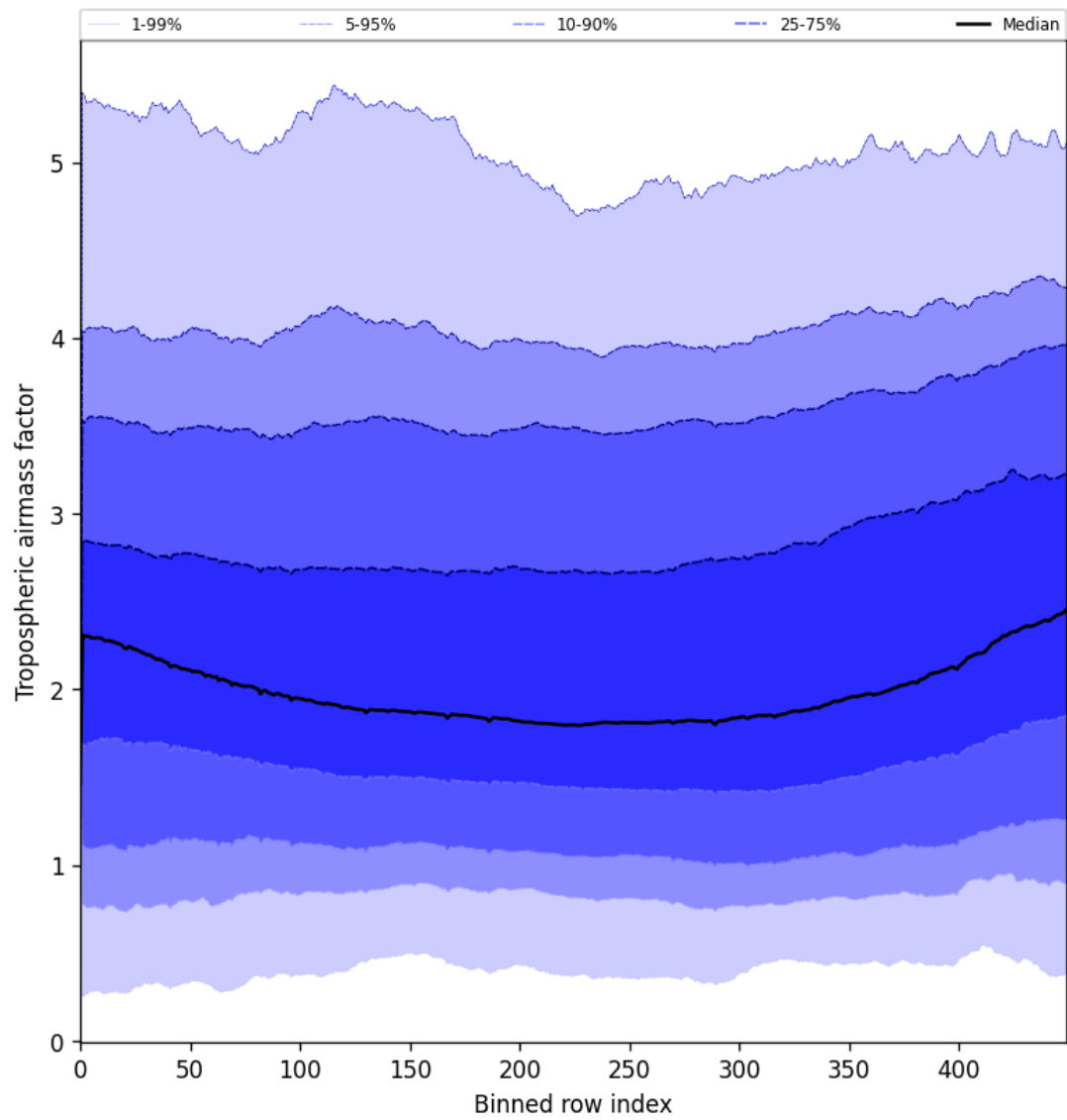
Figure 46: Along track statistics of “Tropospheric airmass factor” for 2025-07-02 to 2025-07-03
