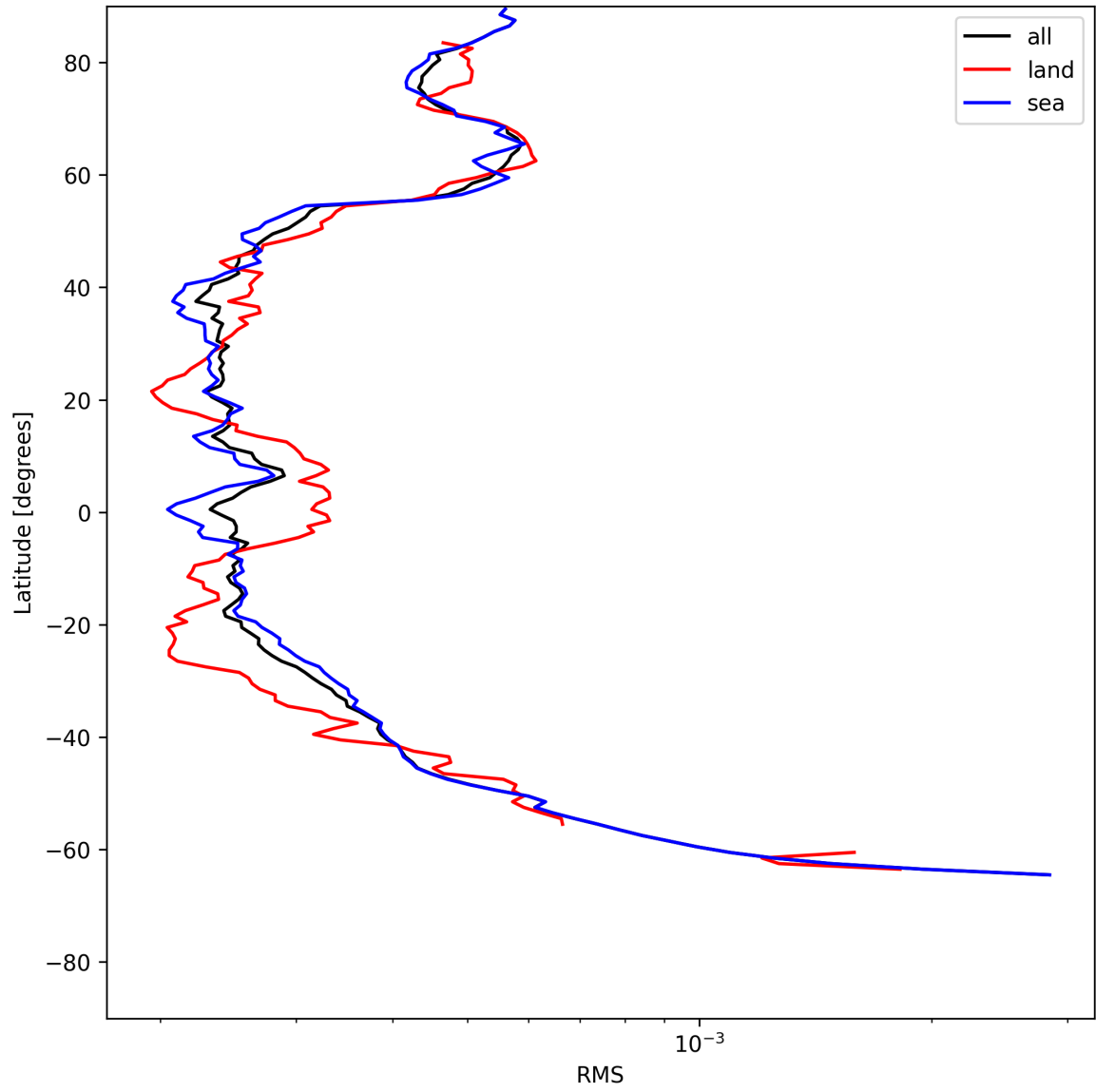
Figure 24: Zonal average of “RMS” for 2025-07-02 to 2025-07-03.
