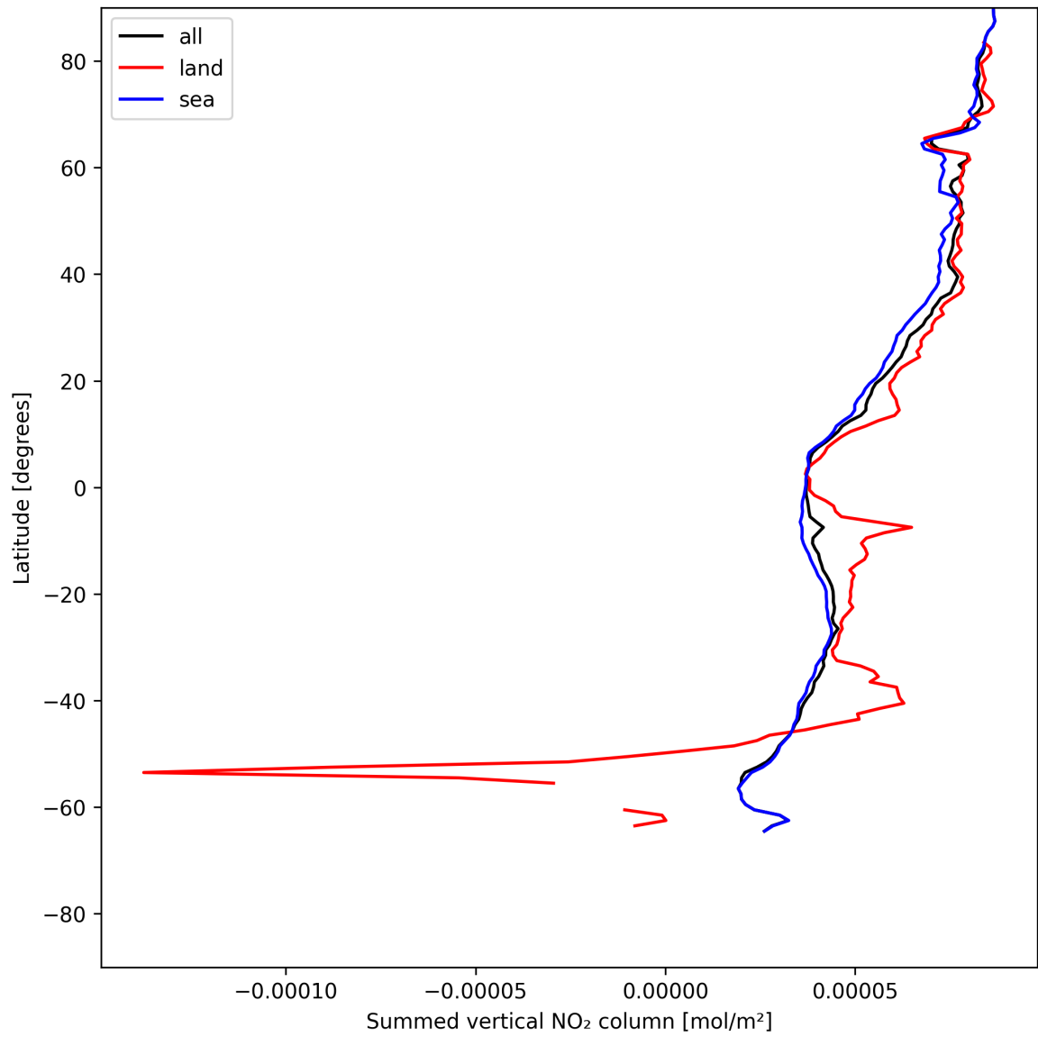
Figure 21: Zonal average of “Summed vertical NO 2 column” for 2025-07-02 to 2025-07-03.
