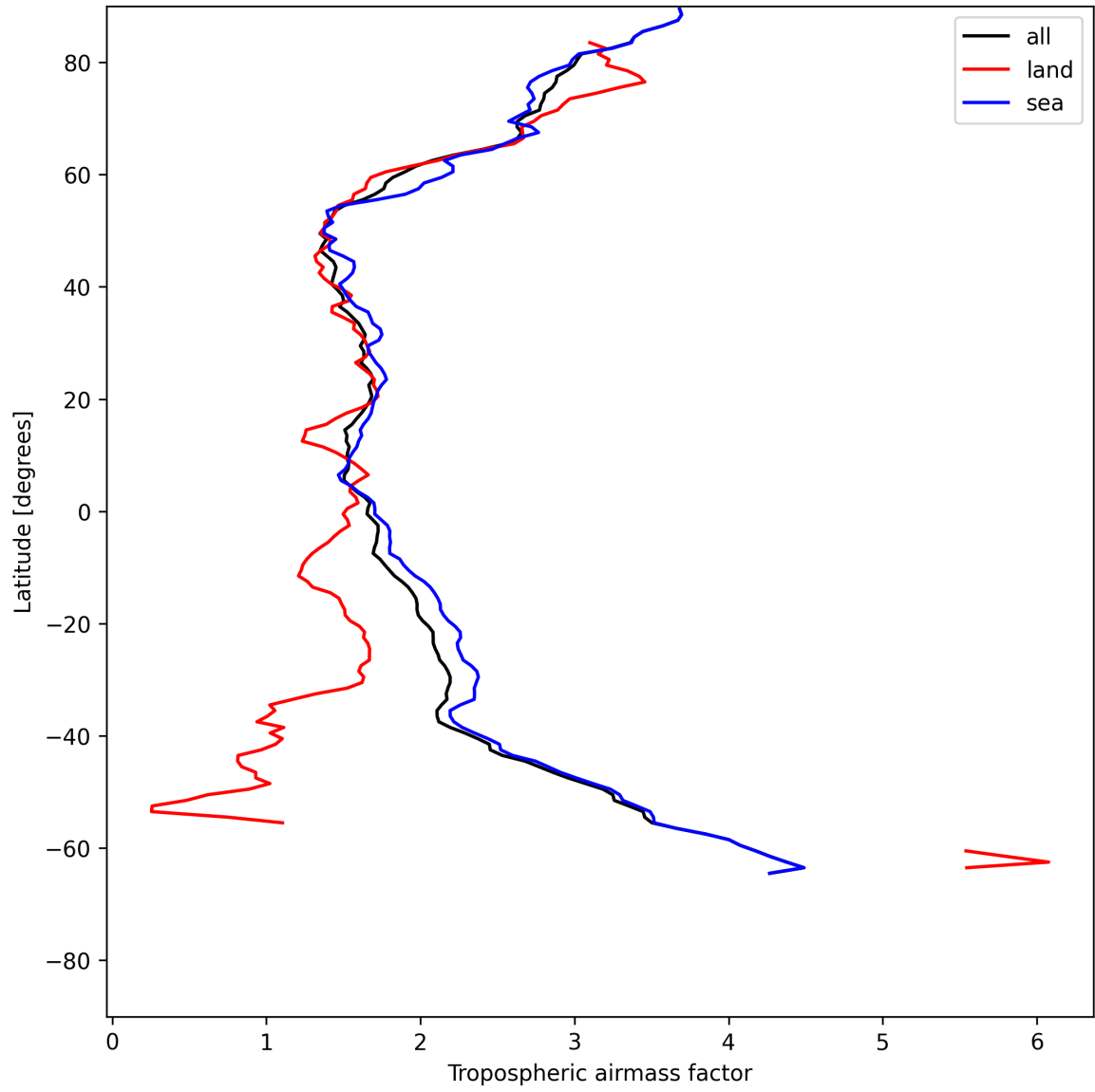
Figure 12: Zonal average of “Tropospheric airmass factor” for 2025-07-02 to 2025-07-03.
