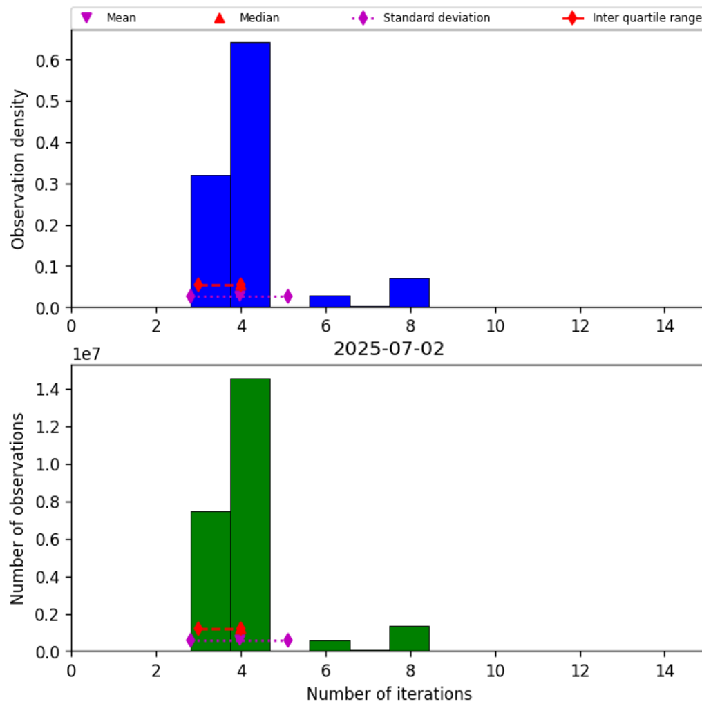
Figure 32: Histogram of “Number of iterations” for 2025-07-02 to 2025-07-03
