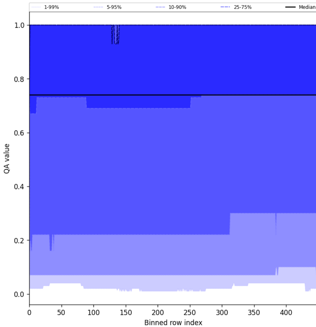
Figure 43: Along track statistics of “QA value” for 2025-07-02 to 2025-07-03
