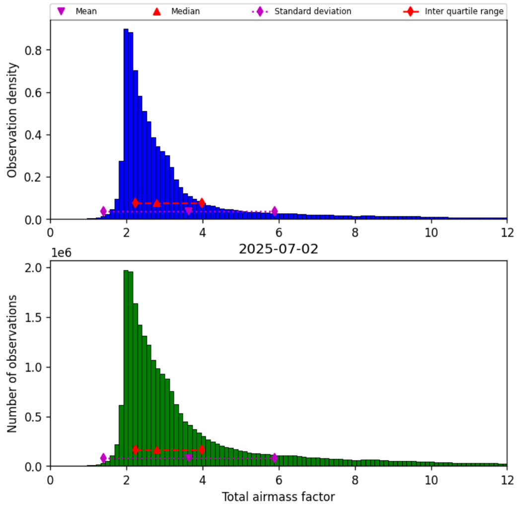
Figure 30: Histogram of “Total airmass factor” for 2025-07-02 to 2025-07-03
