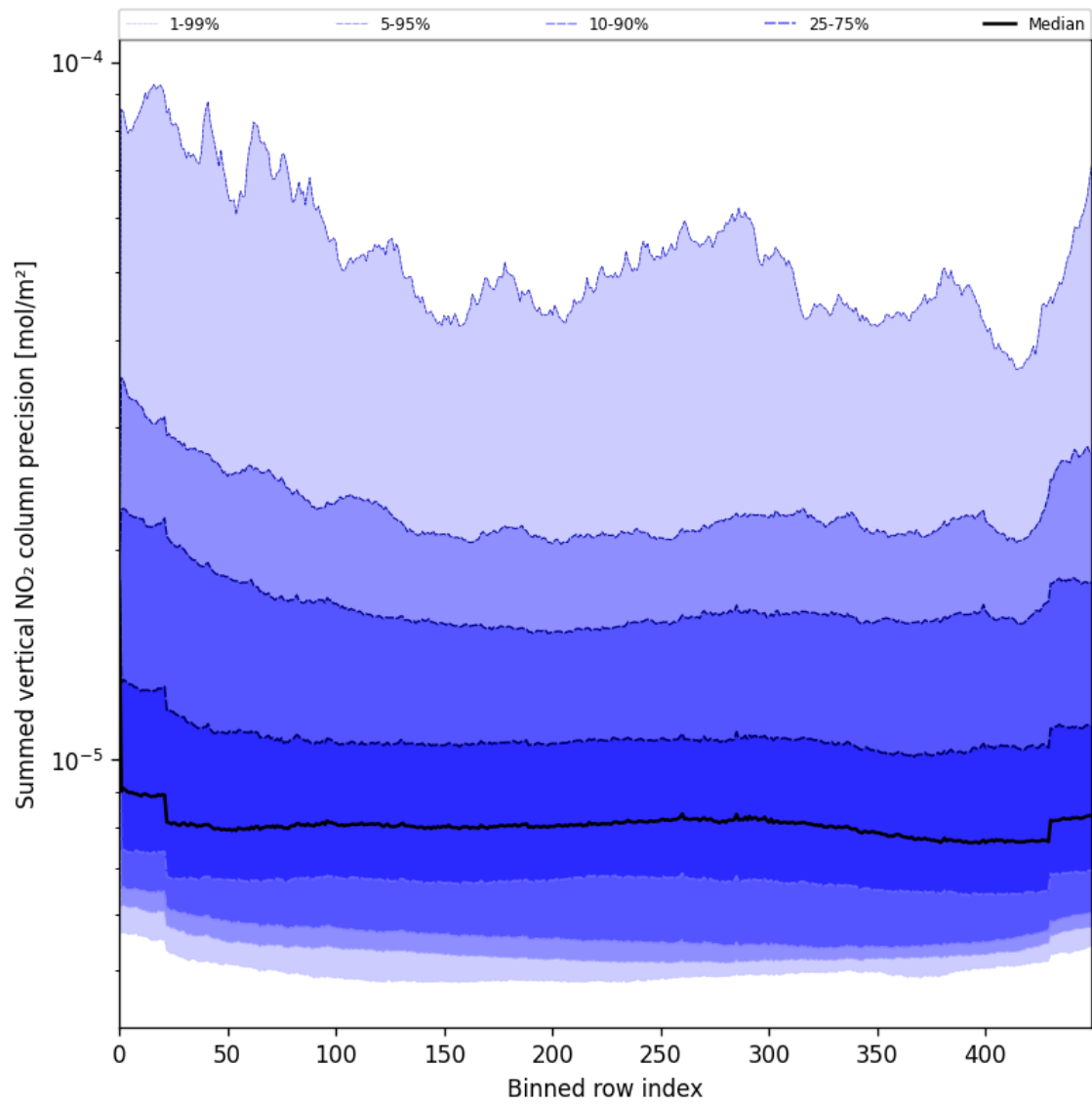
Figure 56: Along track statistics of “Summed vertical NO 2 column precision” for 2025-07-02 to 2025-07-03
