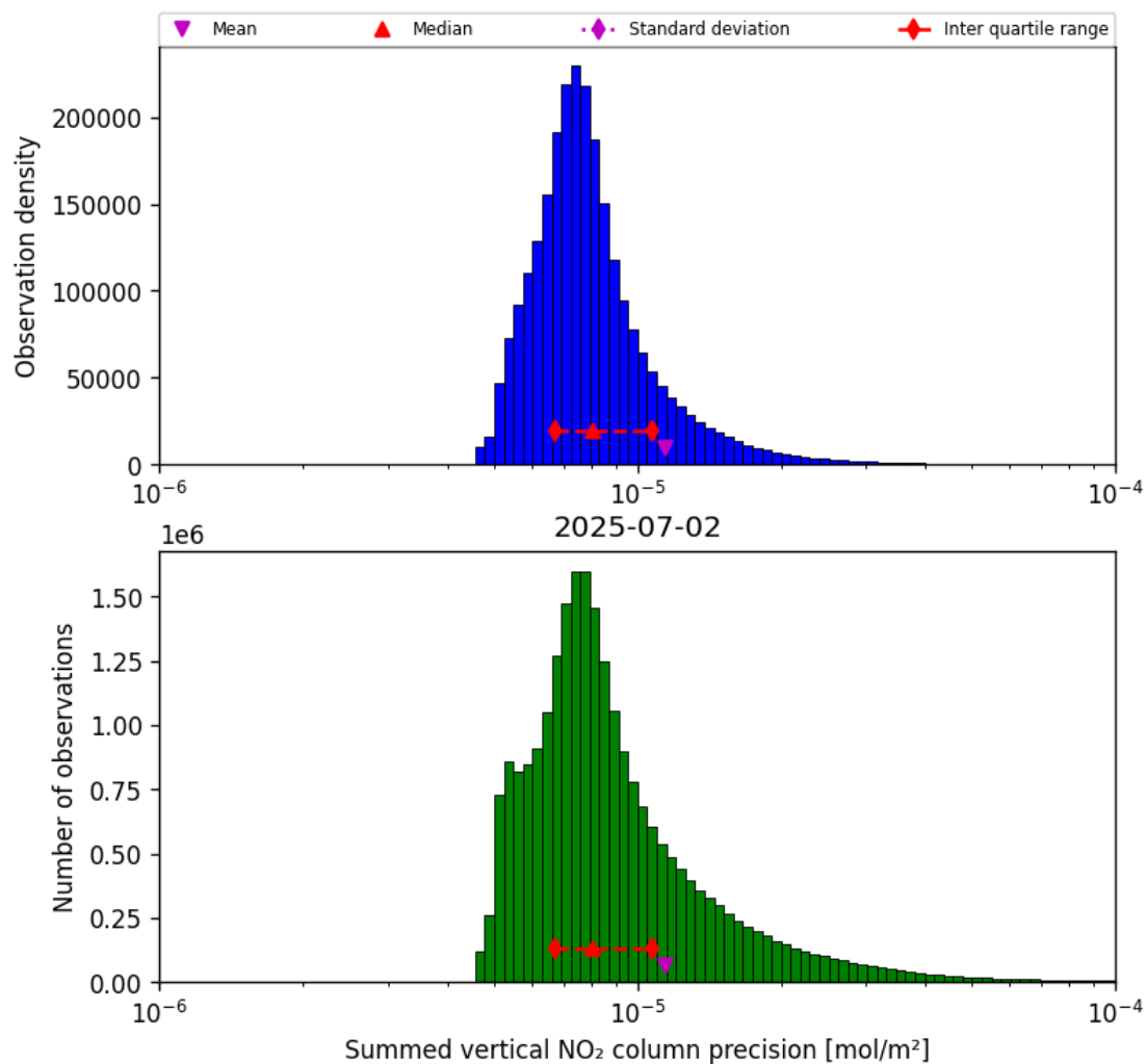
Figure 39: Histogram of "Summed vertical NO 2 column precision" for 2025-07-02 to 2025-07-03
