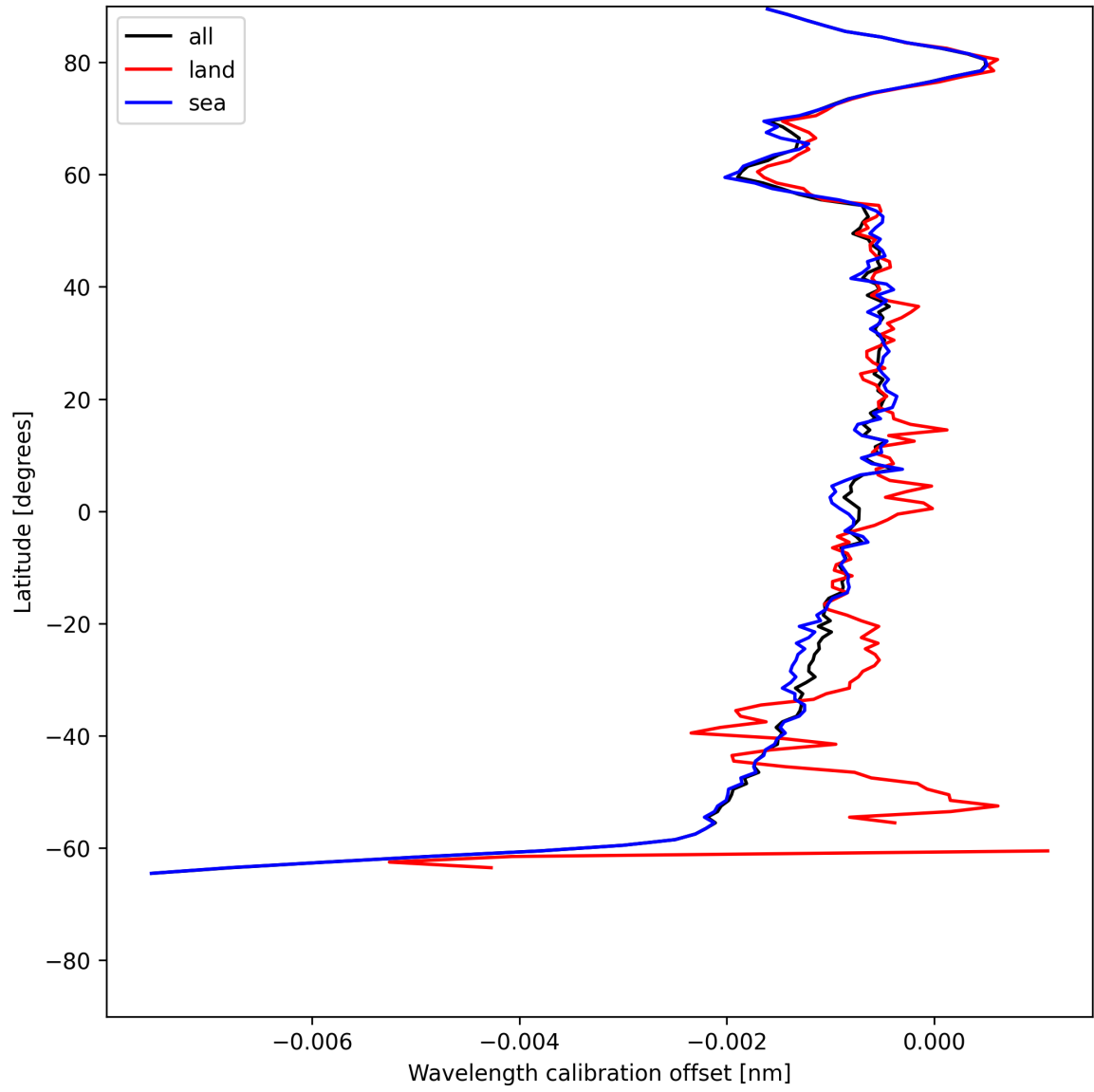
Figure 16: Zonal average of “Wavelength calibration offset” for 2025-07-02 to 2025-07-03.
