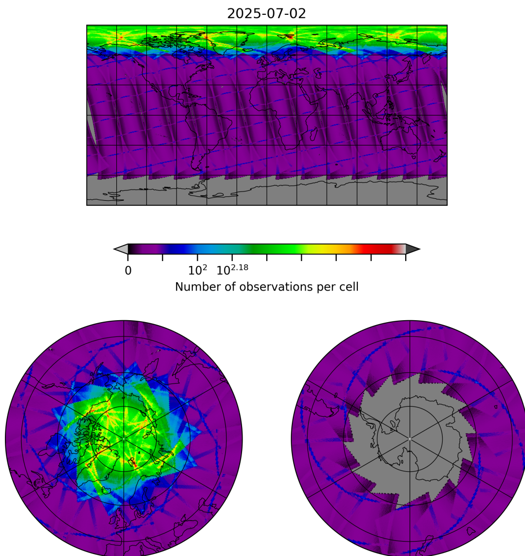
Figure 8: Map of the number of observations for 2025-07-02 to 2025-07-03
