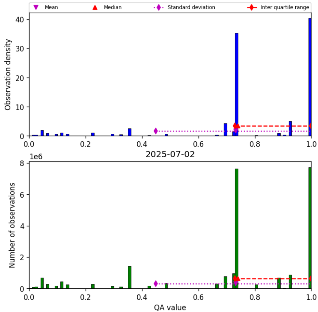
Figure 26: Histogram of “QA value” for 2025-07-02 to 2025-07-03
