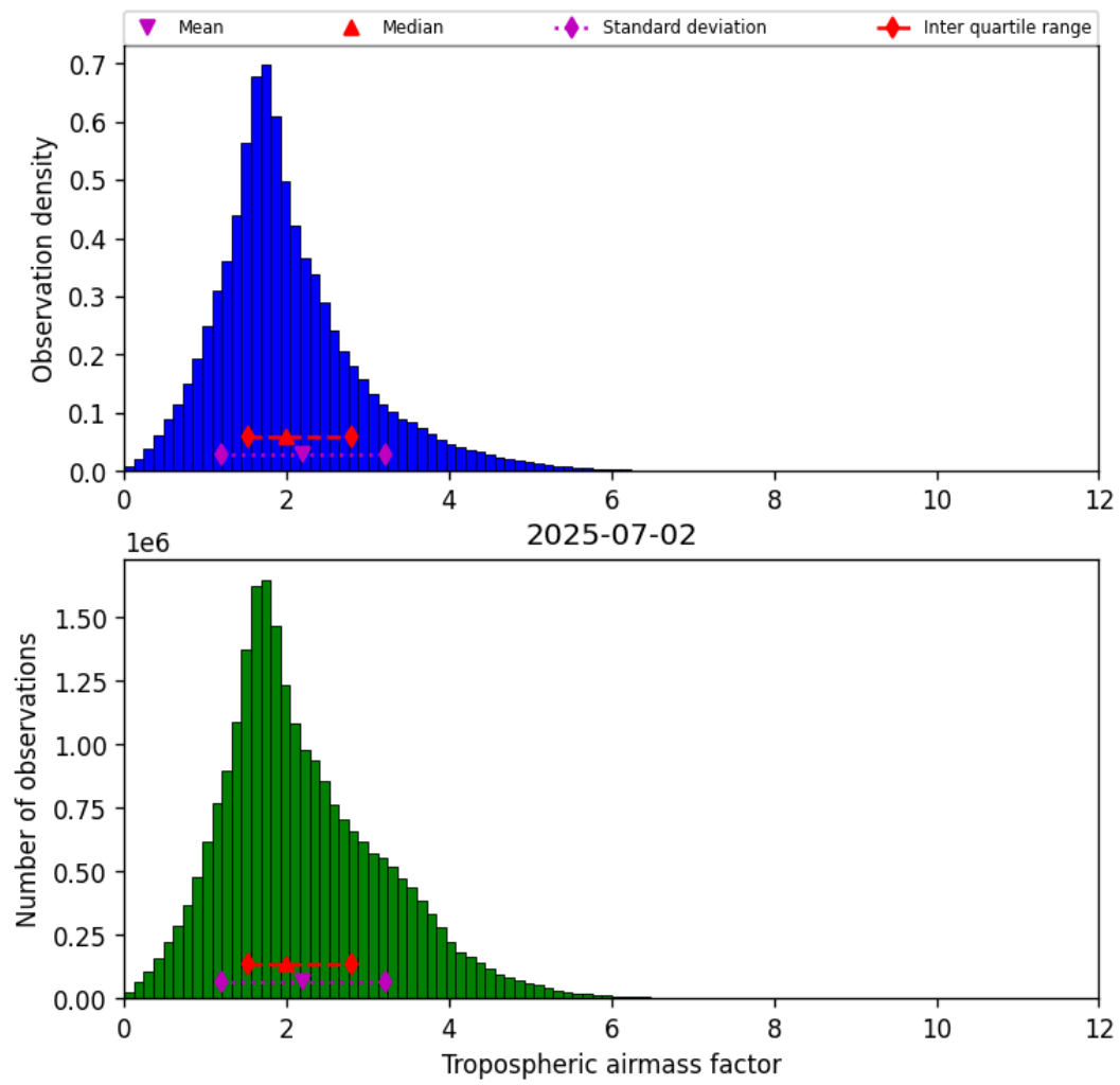
Figure 29: Histogram of “Tropospheric airmass factor” for 2025-07-02 to 2025-07-03
