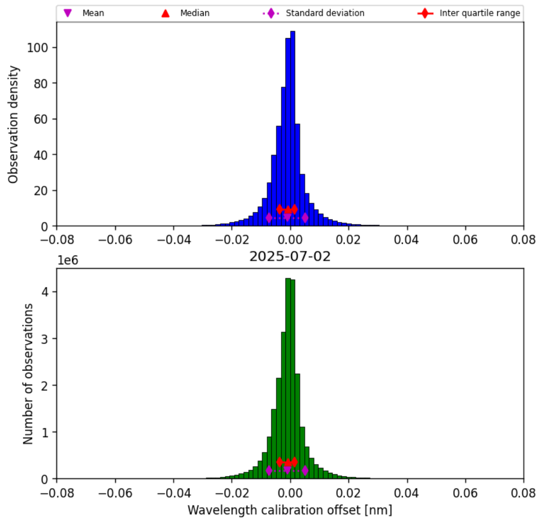
Figure 33: Histogram of “Wavelength calibration offset” for 2025-07-02 to 2025-07-03
