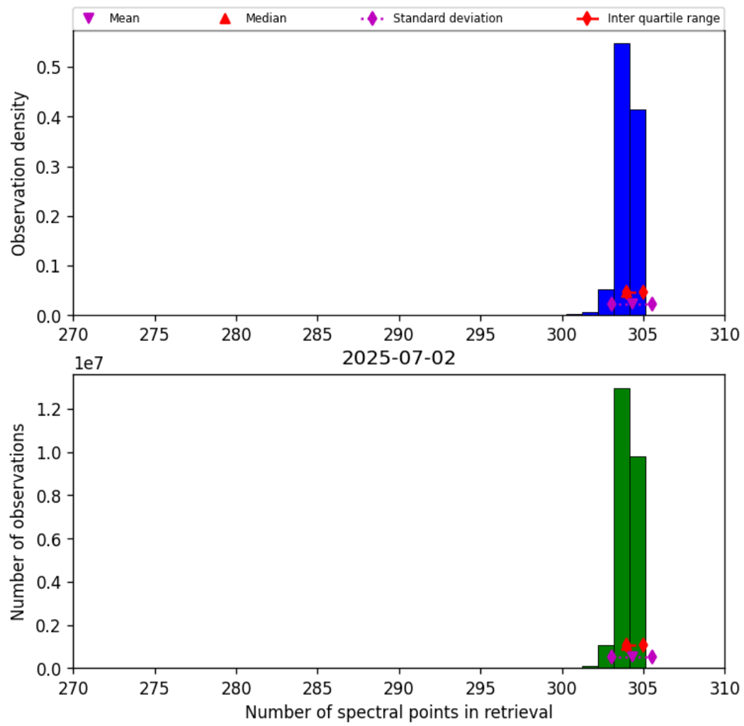
Figure 31: Histogram of “Number of spectral points in retrieval” for 2025-07-02 to 2025-07-03
