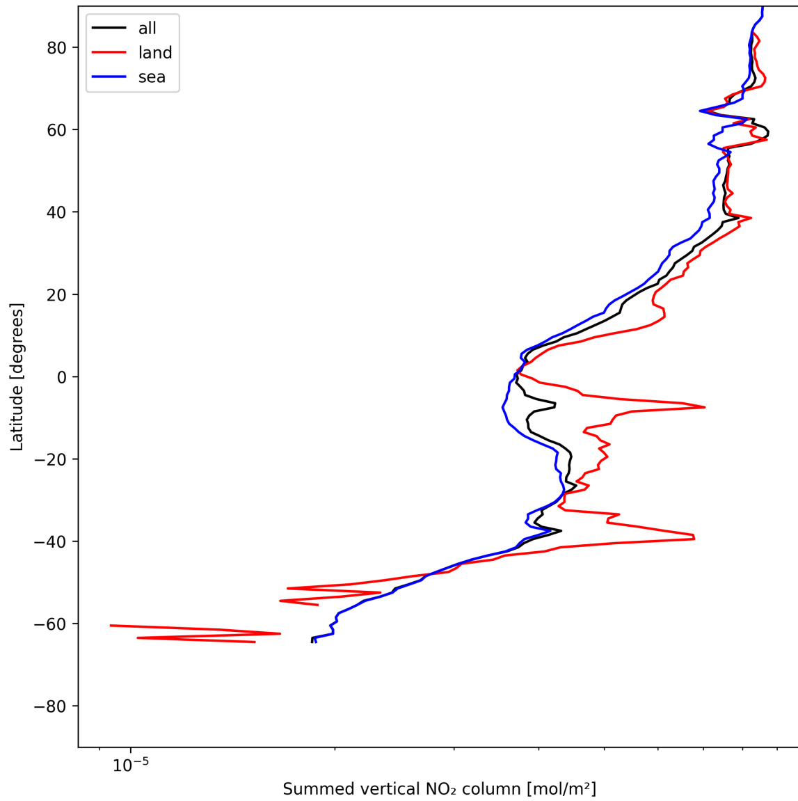
Figure 21: Zonal average of “Summed vertical NO 2 column” for 2025-07-03 to 2025-07-04.
