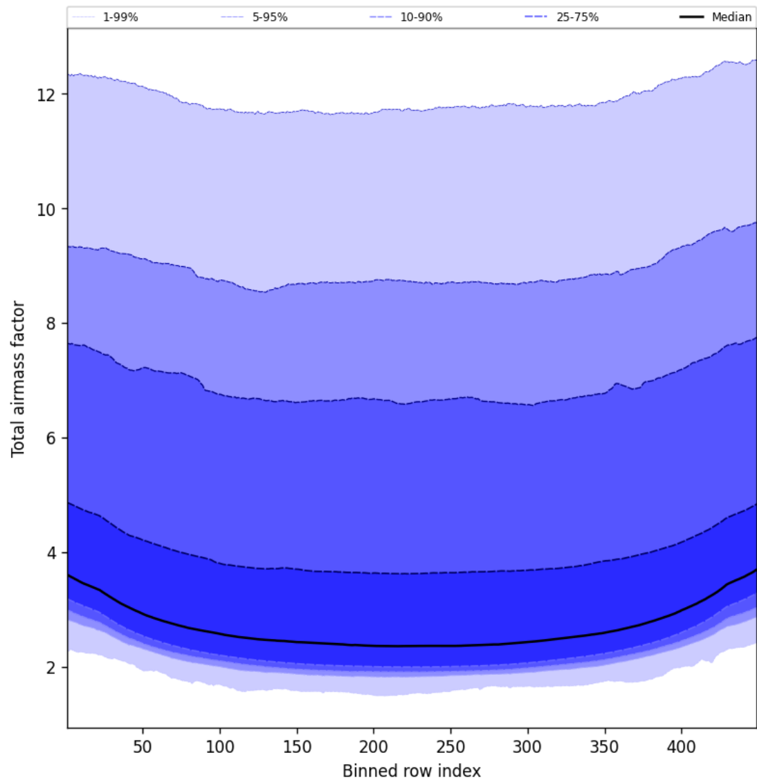
Figure 47: Along track statistics of “Total airmass factor” for 2025-07-03 to 2025-07-04
