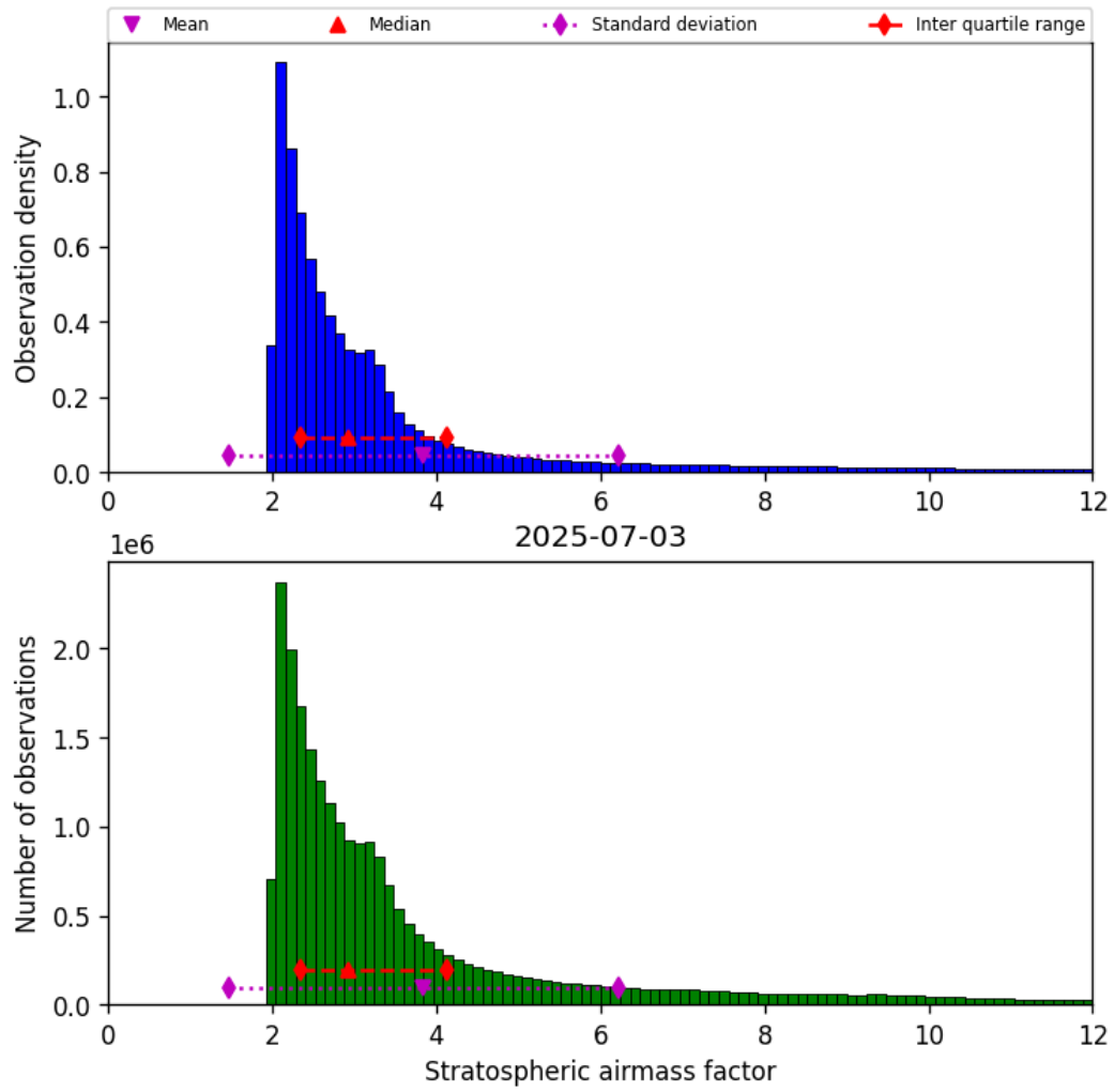
Figure 42: Histogram of “Stratospheric airmass factor” for 2025-07-03 to 2025-07-04
