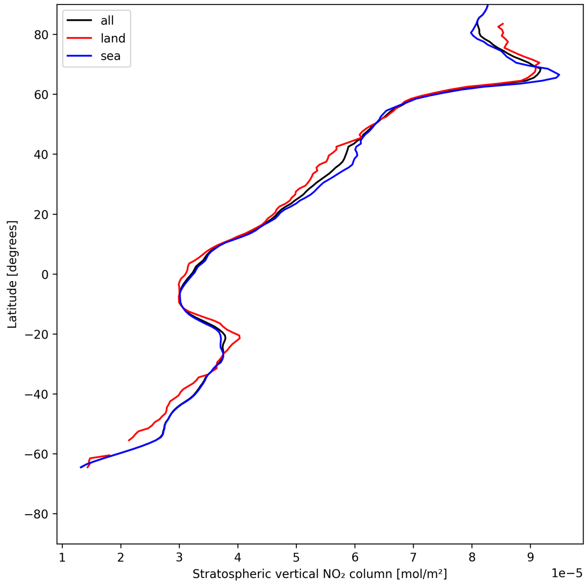
Figure 17: Zonal average of “Stratospheric vertical NO 2 column” for 2025-07-03 to 2025-07-04.
