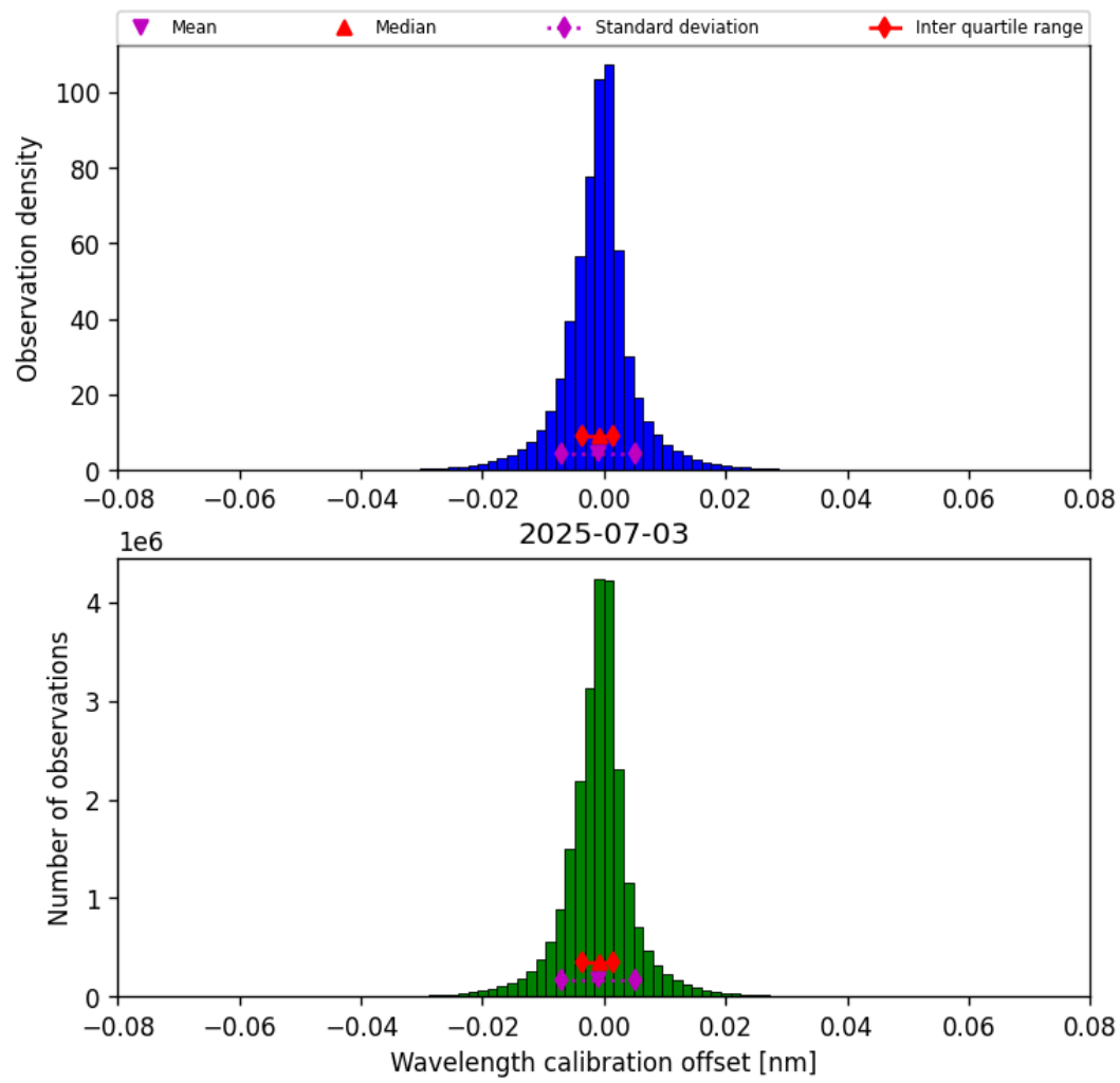
Figure 33: Histogram of “Wavelength calibration offset” for 2025-07-03 to 2025-07-04
