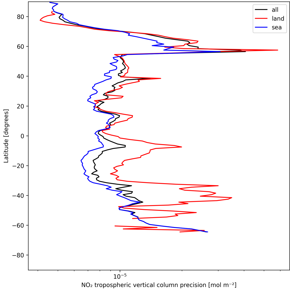
Figure 11: Zonal average of “NO 2 tropospheric vertical column precision” for 2025-07-03 to 2025-07-04.
