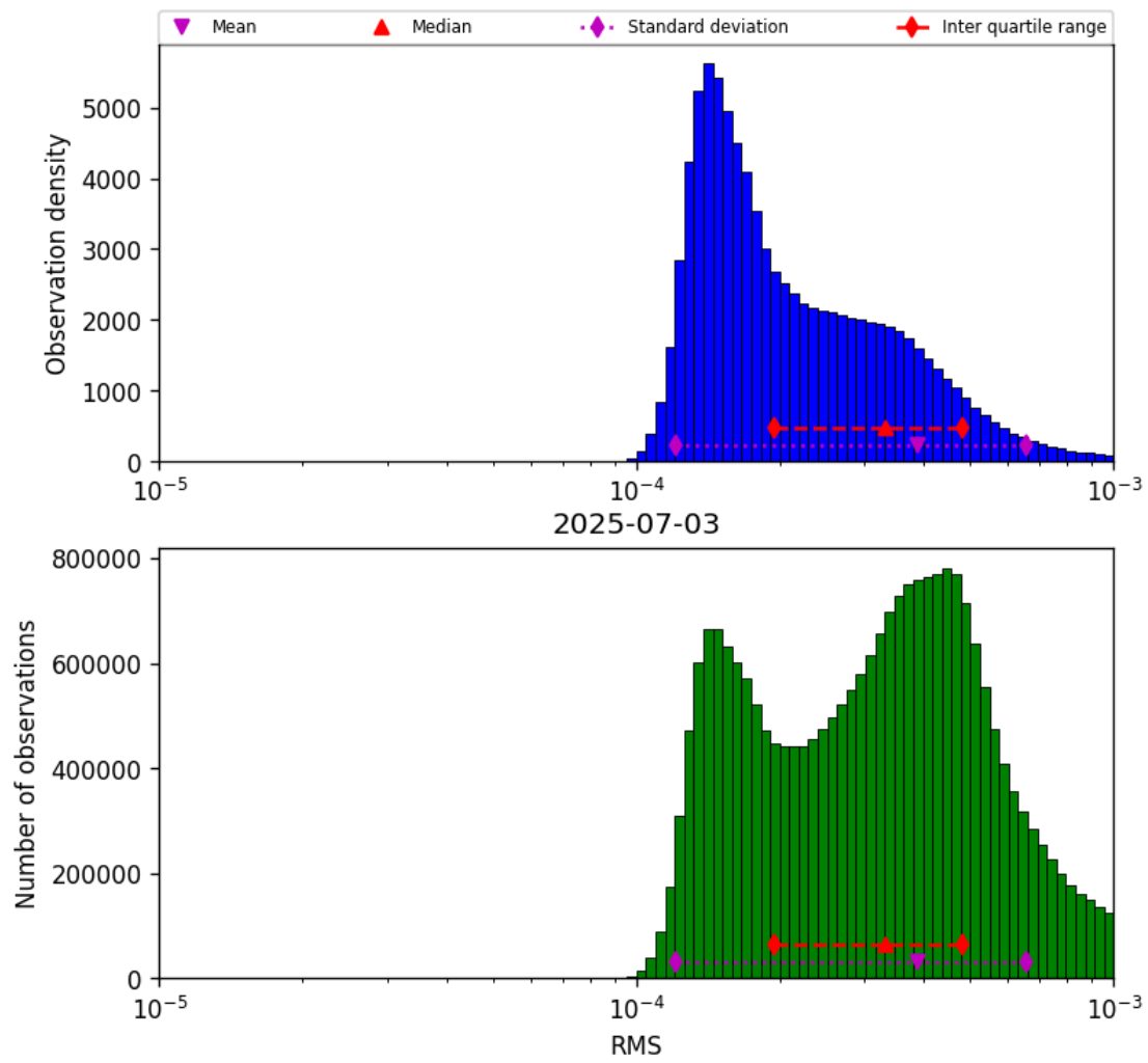
Figure 41: Histogram of “RMS” for 2025-07-03 to 2025-07-04
