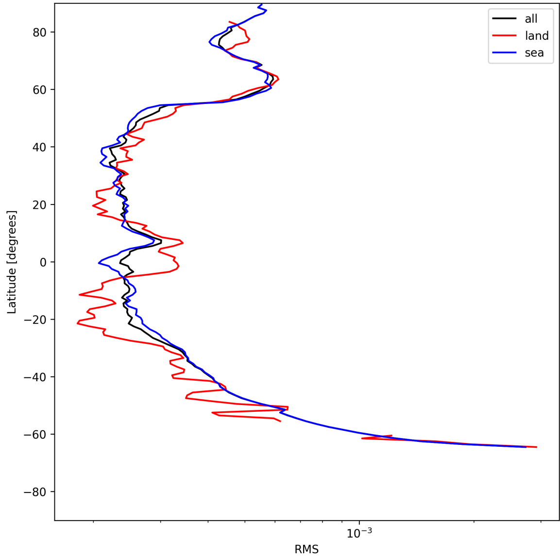
Figure 24: Zonal average of “RMS” for 2025-07-03 to 2025-07-04.
