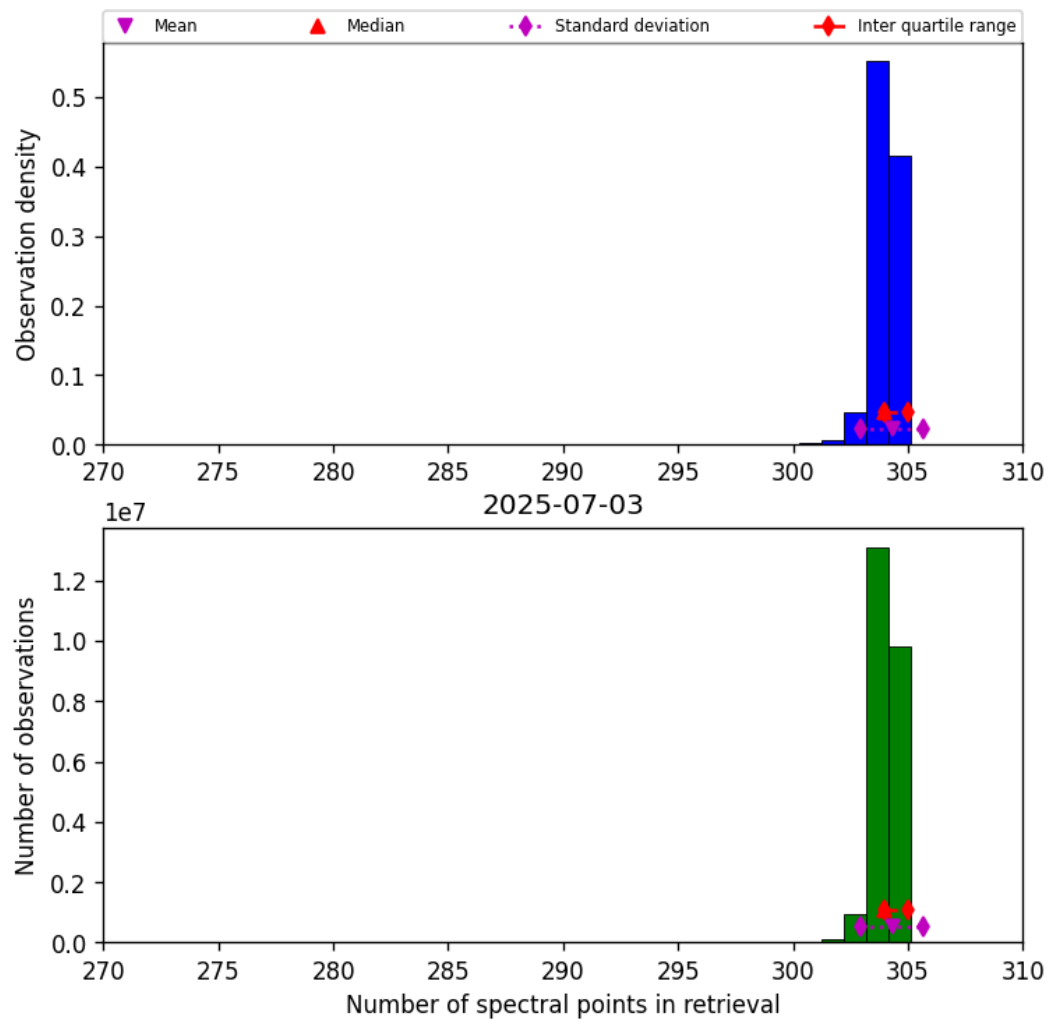
Figure 31: Histogram of “Number of spectral points in retrieval” for 2025-07-03 to 2025-07-04
