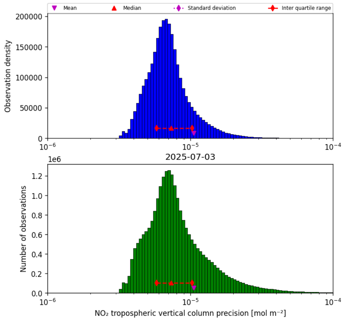
Figure 28: Histogram of “NO 2 tropospheric vertical column precision” for 2025-07-03 to 2025-07-04
