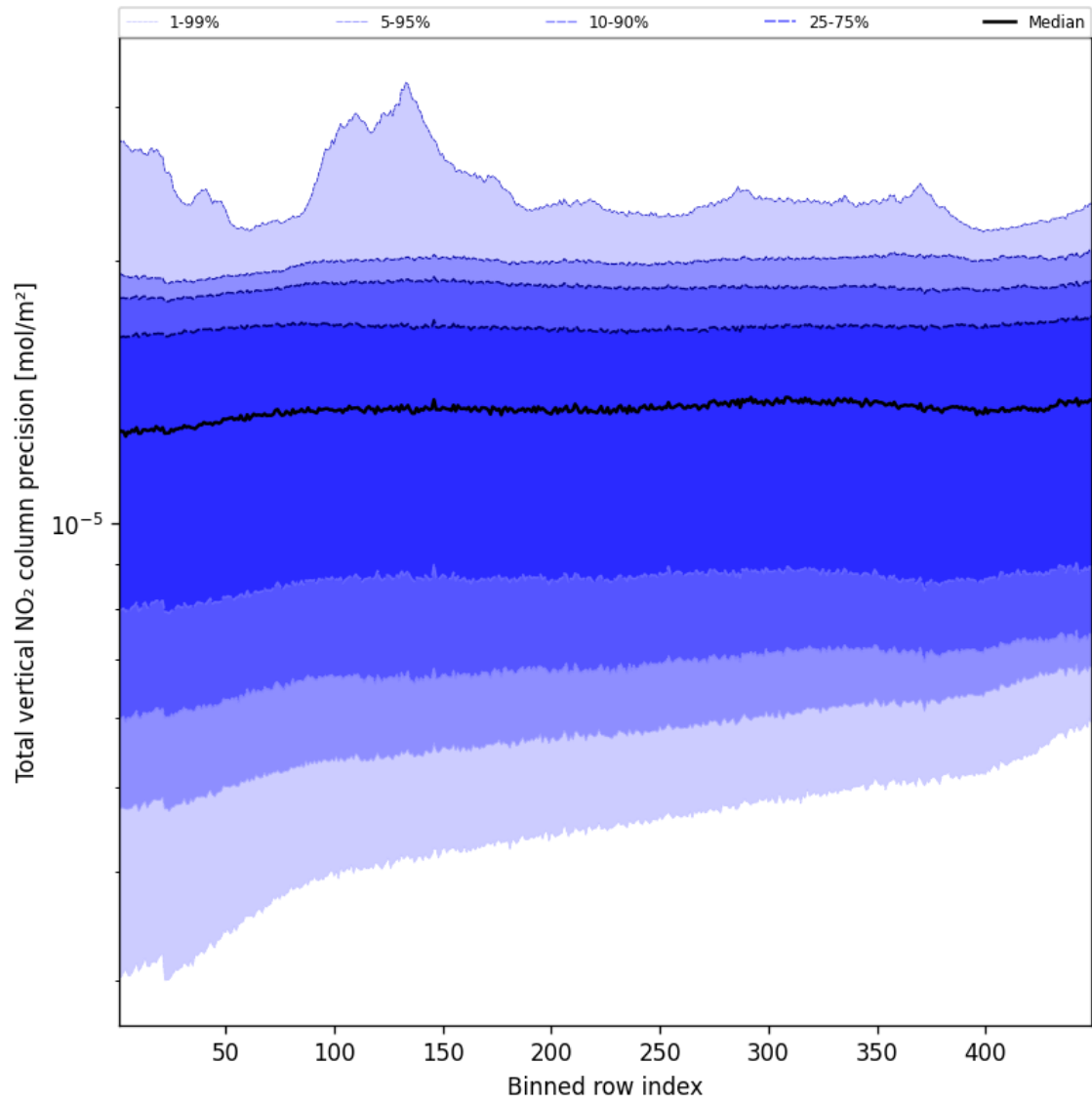
Figure 54: Along track statistics of “Total vertical NO 2 column precision” for 2025-07-03 to 2025-07-04
