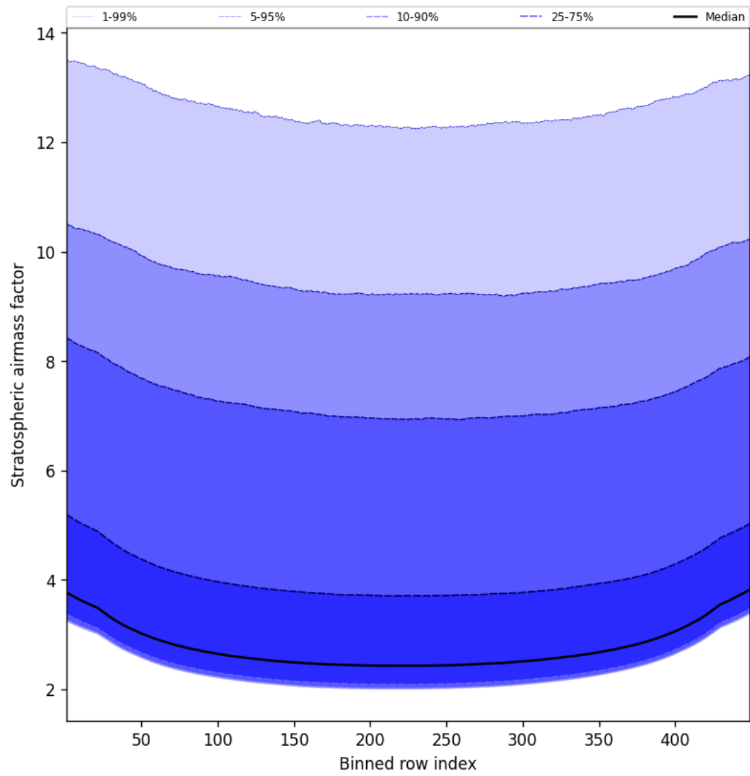
Figure 59: Along track statistics of “Stratospheric airmass factor” for 2025-07-03 to 2025-07-04
