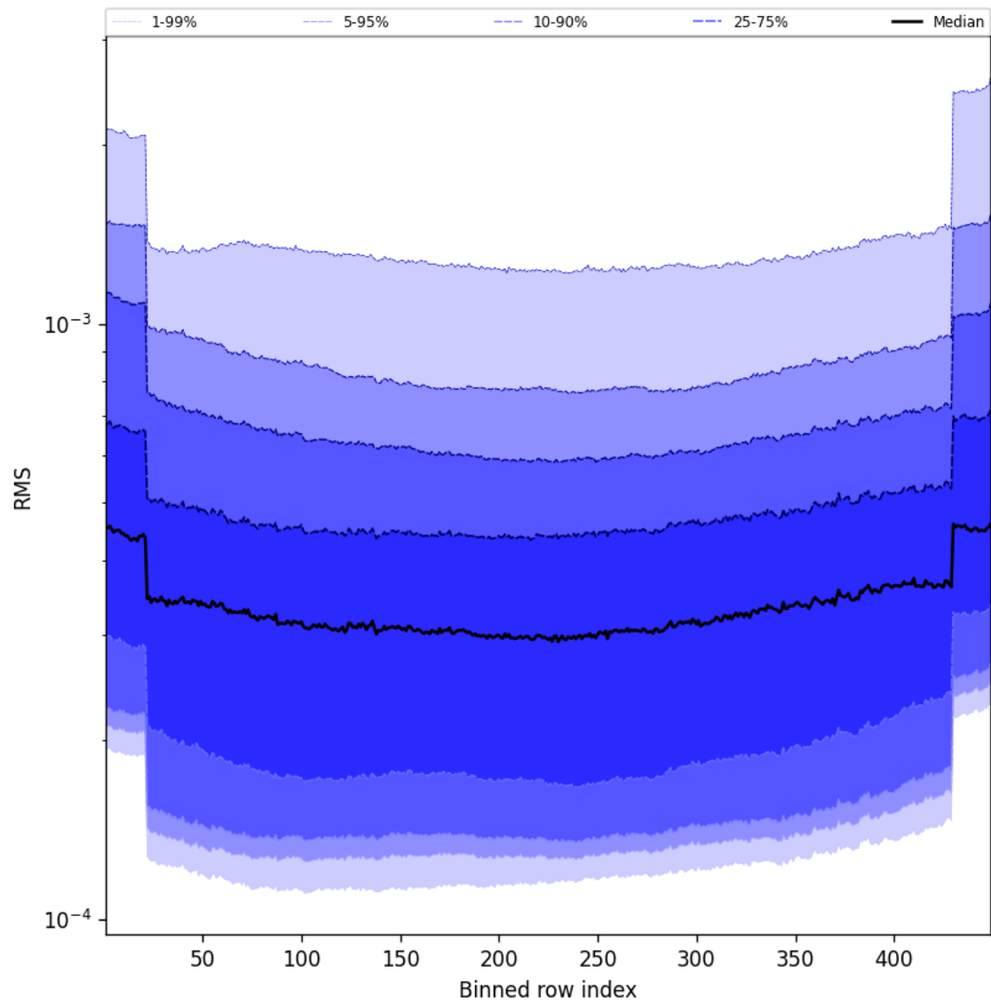
Figure 58: Along track statistics of “RMS” for 2025-07-03 to 2025-07-04
