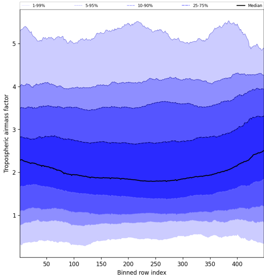
Figure 46: Along track statistics of “Tropospheric airmass factor” for 2025-07-03 to 2025-07-04
