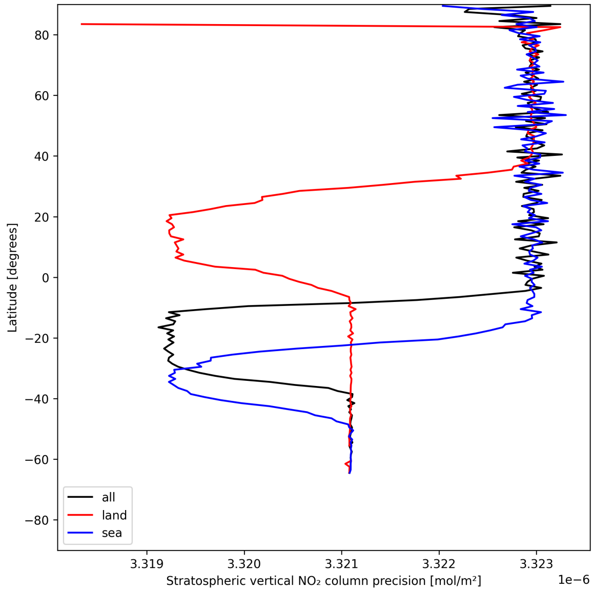
Figure 18: Zonal average of “Stratospheric vertical NO 2 column precision” for 2025-07-03 to 2025-07-04.
