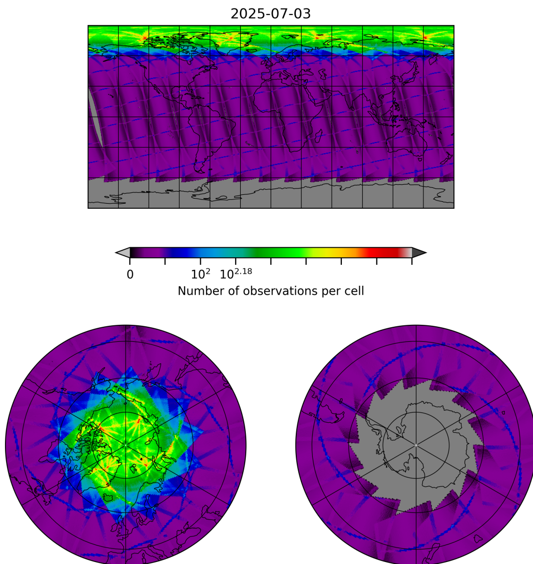
Figure 8: Map of the number of observations for 2025-07-03 to 2025-07-04
