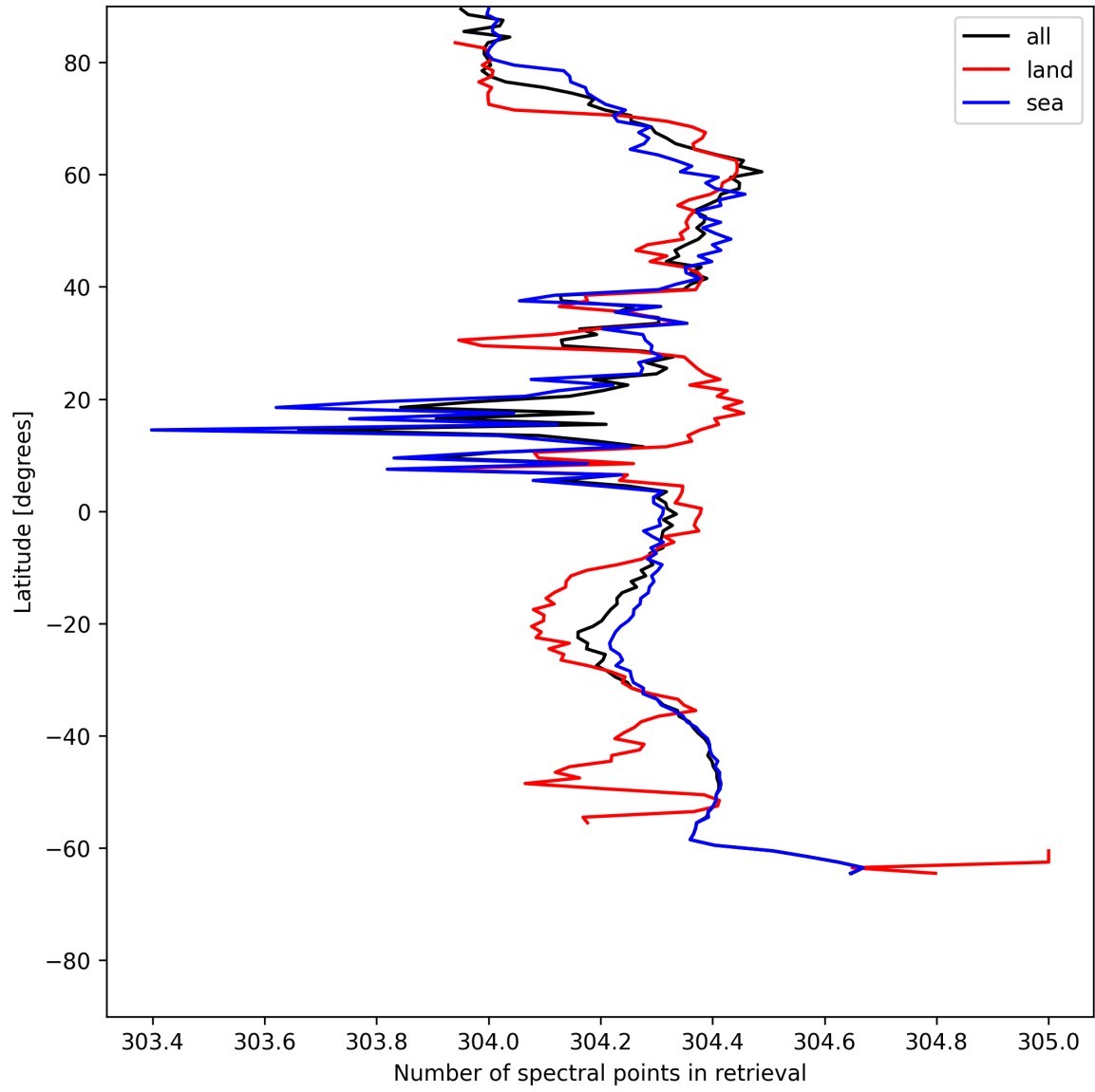
Figure 14: Zonal average of “Number of spectral points in retrieval” for 2025-07-03 to 2025-07-04.
