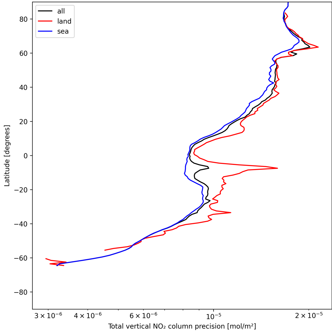
Figure 20: Zonal average of “Total vertical NO 2 column precision” for 2025-07-03 to 2025-07-04.
