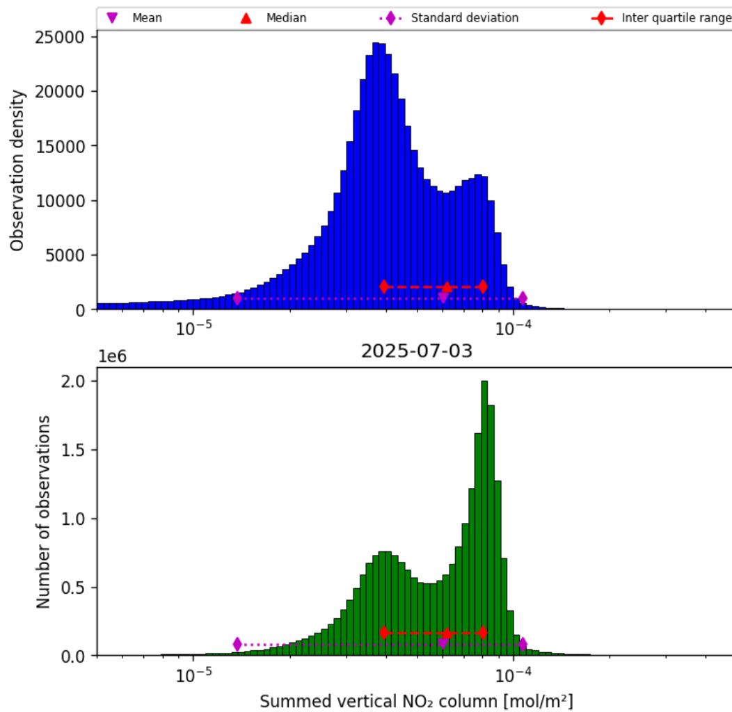
Figure 38: Histogram of "Summed vertical NO 2 column" for 2025-07-03 to 2025-07-04
