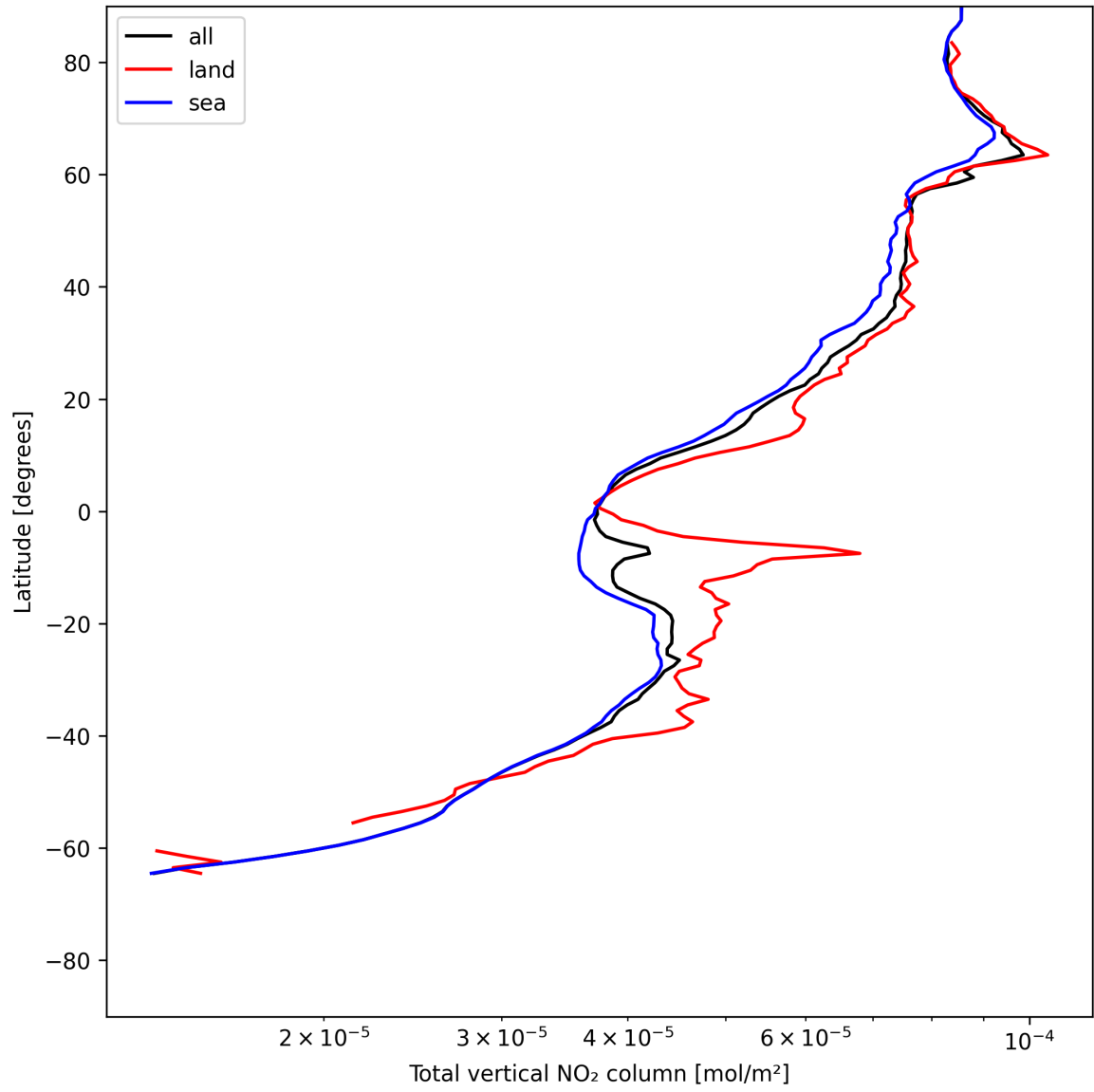
Figure 19: Zonal average of “Total vertical NO 2 column” for 2025-07-03 to 2025-07-04.
