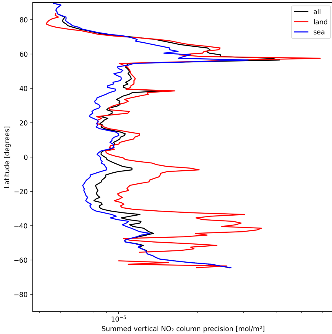
Figure 22: Zonal average of “Summed vertical NO 2 column precision” for 2025-07-03 to 2025-07-04.
