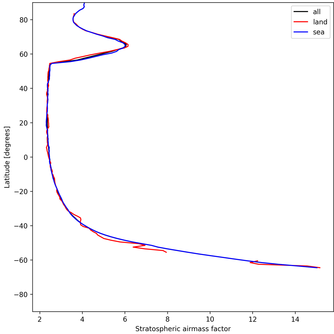
Figure 25: Zonal average of “Stratospheric air mass factor” for 2025-07-03 to 2025-07-04.
