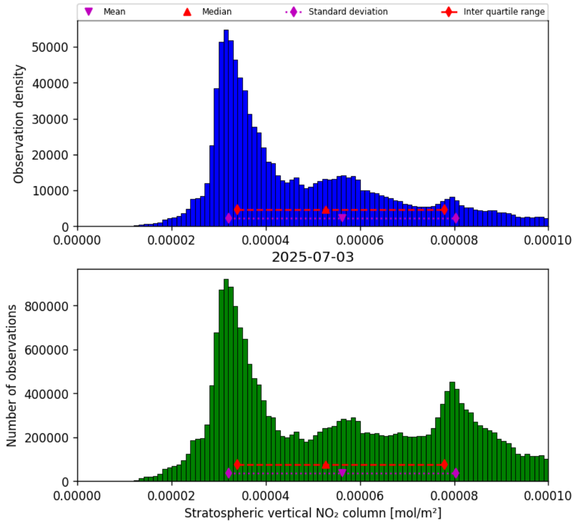
Figure 34: Histogram of “Stratospheric vertical NO 2 column” for 2025-07-03 to 2025-07-04
