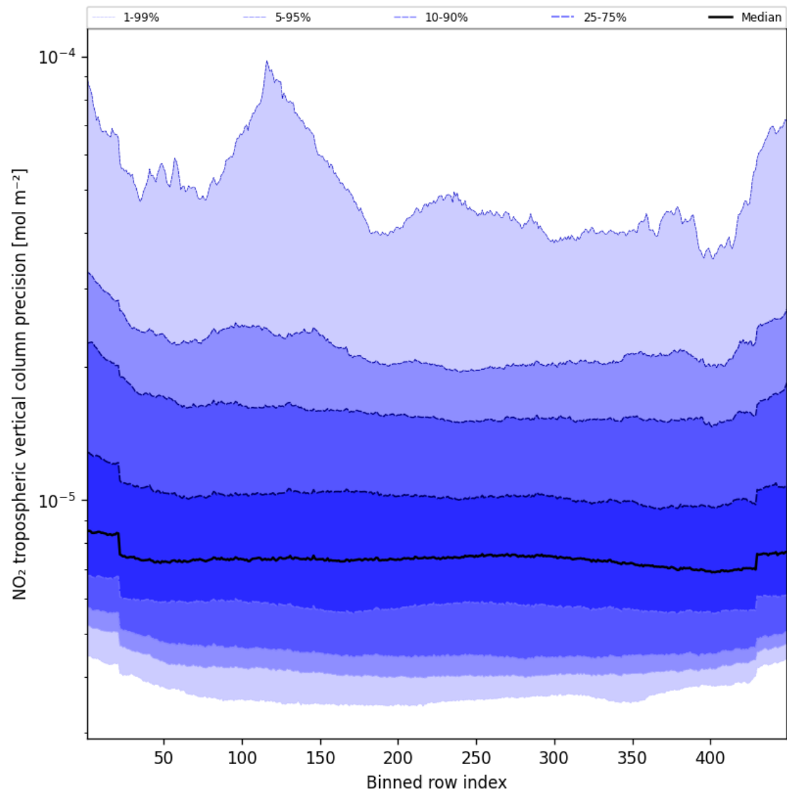
Figure 45: Along track statistics of “NO 2 tropospheric vertical column precision” for 2025-07-03 to 2025-07-04
