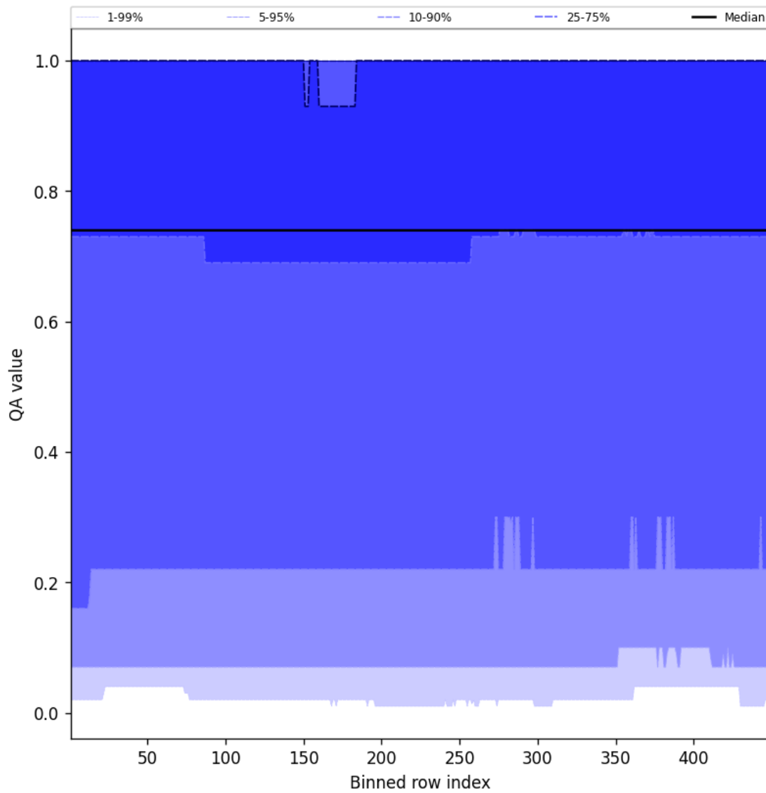
Figure 43: Along track statistics of “QA value” for 2025-07-03 to 2025-07-04
