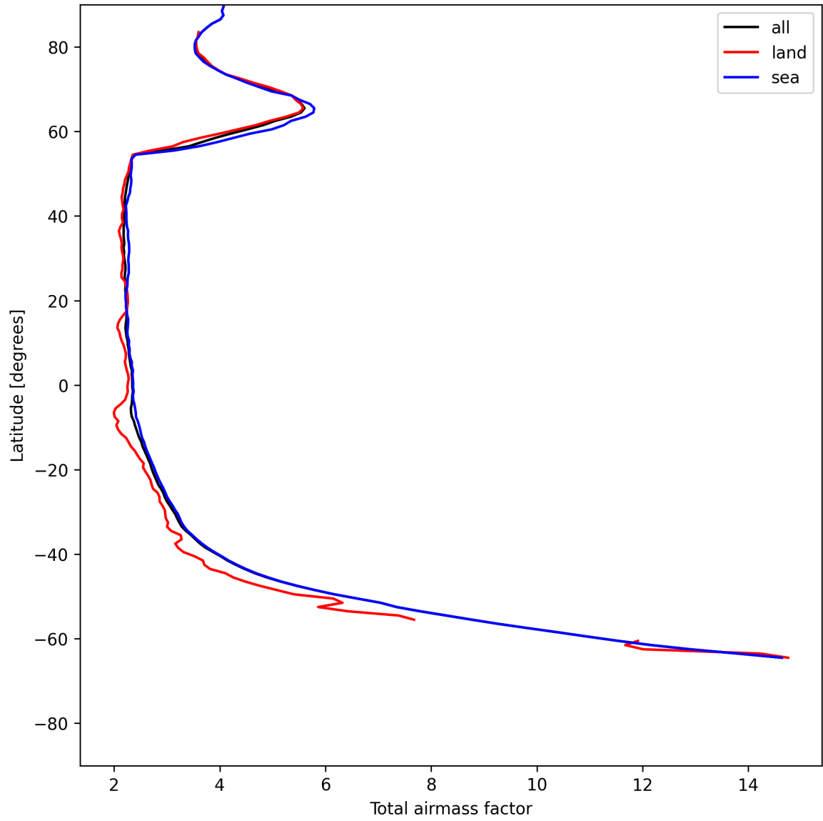
Figure 13: Zonal average of “Total airmass factor” for 2025-07-03 to 2025-07-04.
