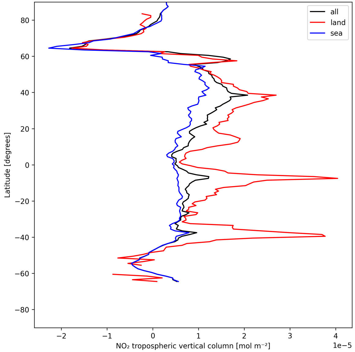
Figure 10: Zonal average of “NO 2 tropospheric vertical column” for 2025-07-03 to 2025-07-04.
