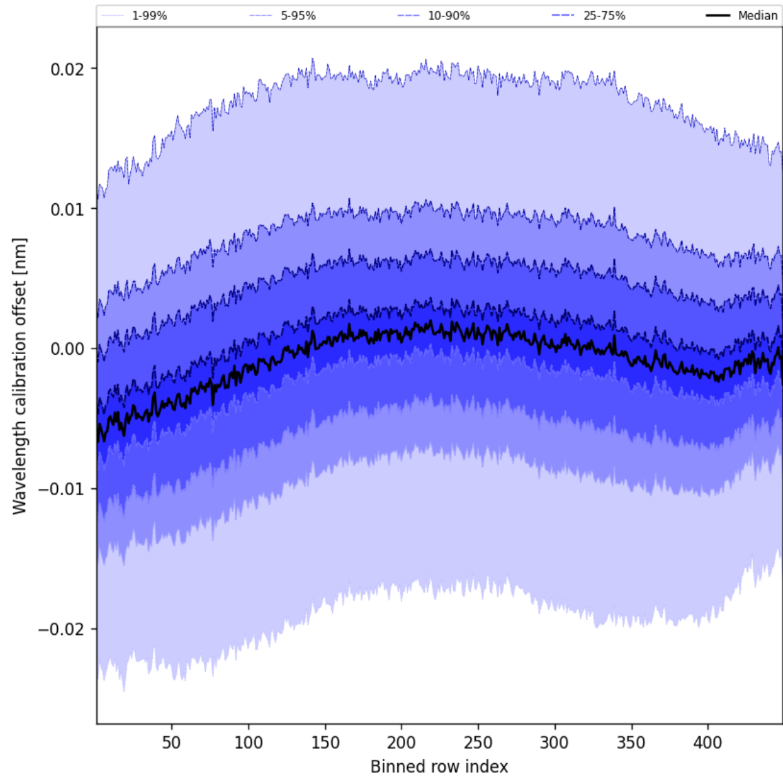
Figure 50: Along track statistics of “Wavelength calibration offset” for 2025-07-03 to 2025-07-04
