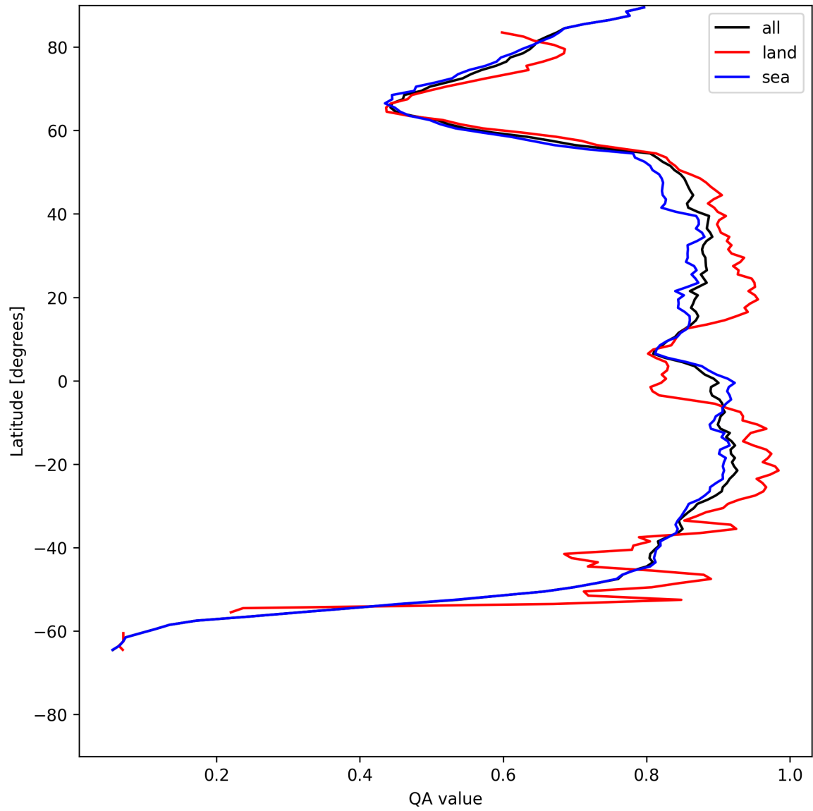
Figure 9: Zonal average of “QA value” for 2025-07-03 to 2025-07-04.
