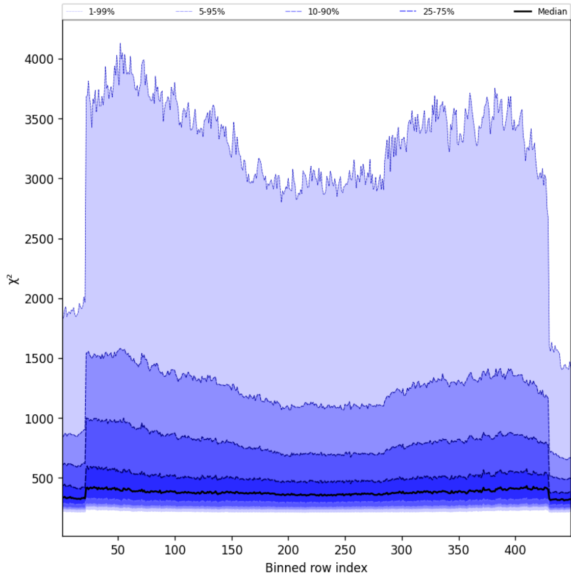
Figure 57: Along track statistics of " \chi^2 " for 2025-07-03 to 2025-07-04
