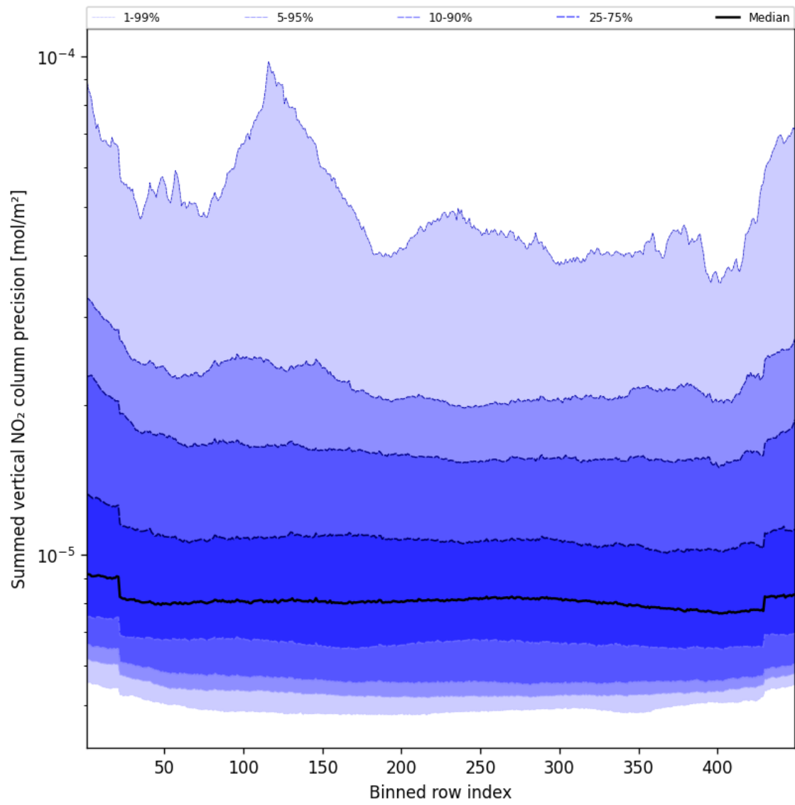
Figure 56: Along track statistics of “Summed vertical NO 2 column precision” for 2025-07-03 to 2025-07-04
