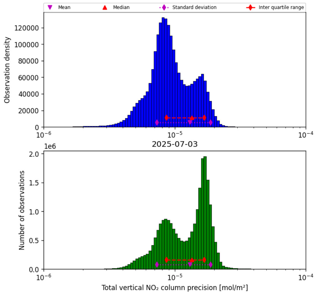
Figure 37: Histogram of “Total vertical NO 2 column precision” for 2025-07-03 to 2025-07-04
