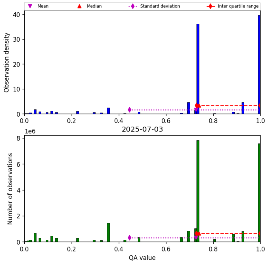
Figure 26: Histogram of “QA value” for 2025-07-03 to 2025-07-04
