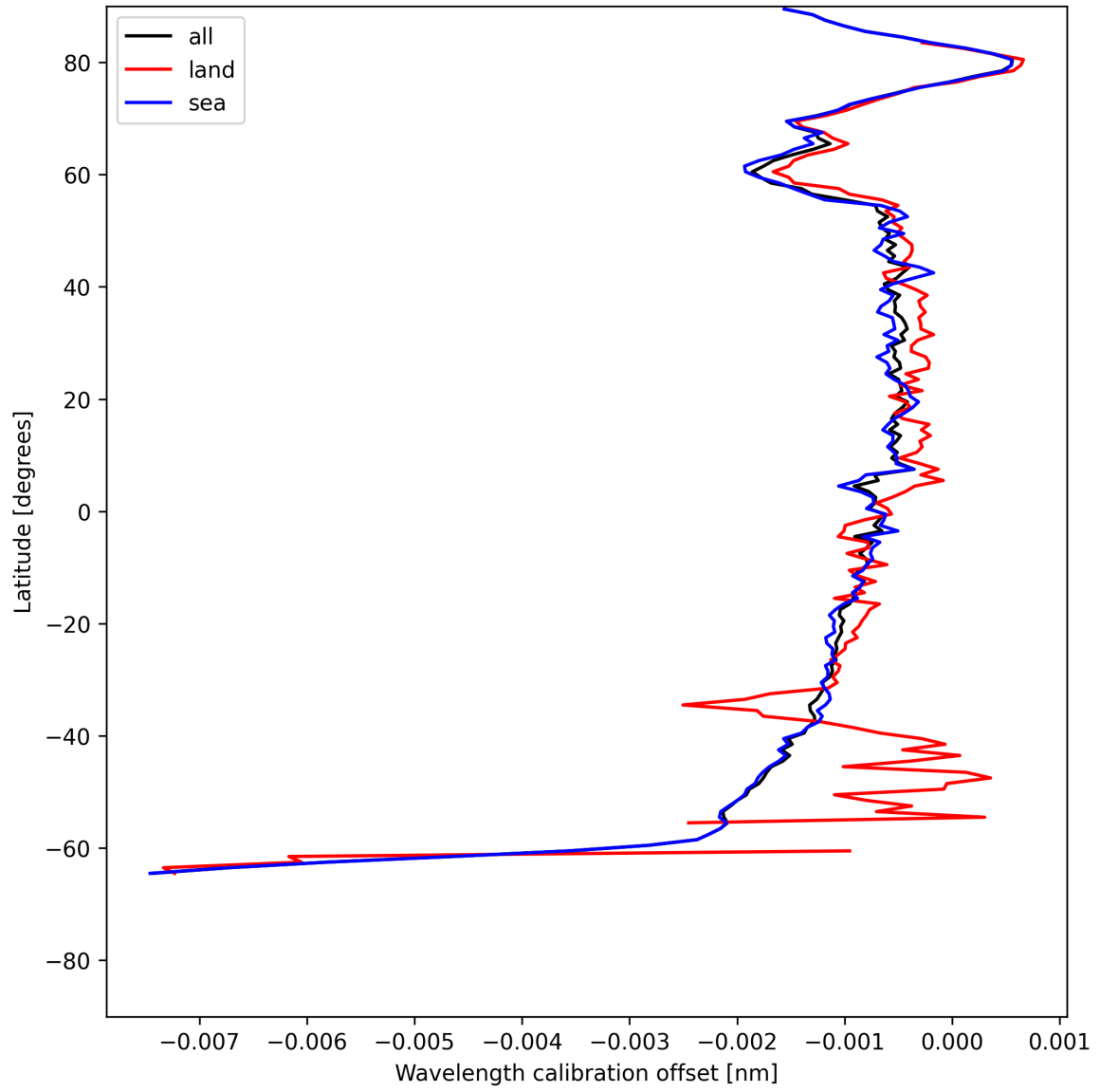
Figure 16: Zonal average of “Wavelength calibration offset” for 2025-07-03 to 2025-07-04.
