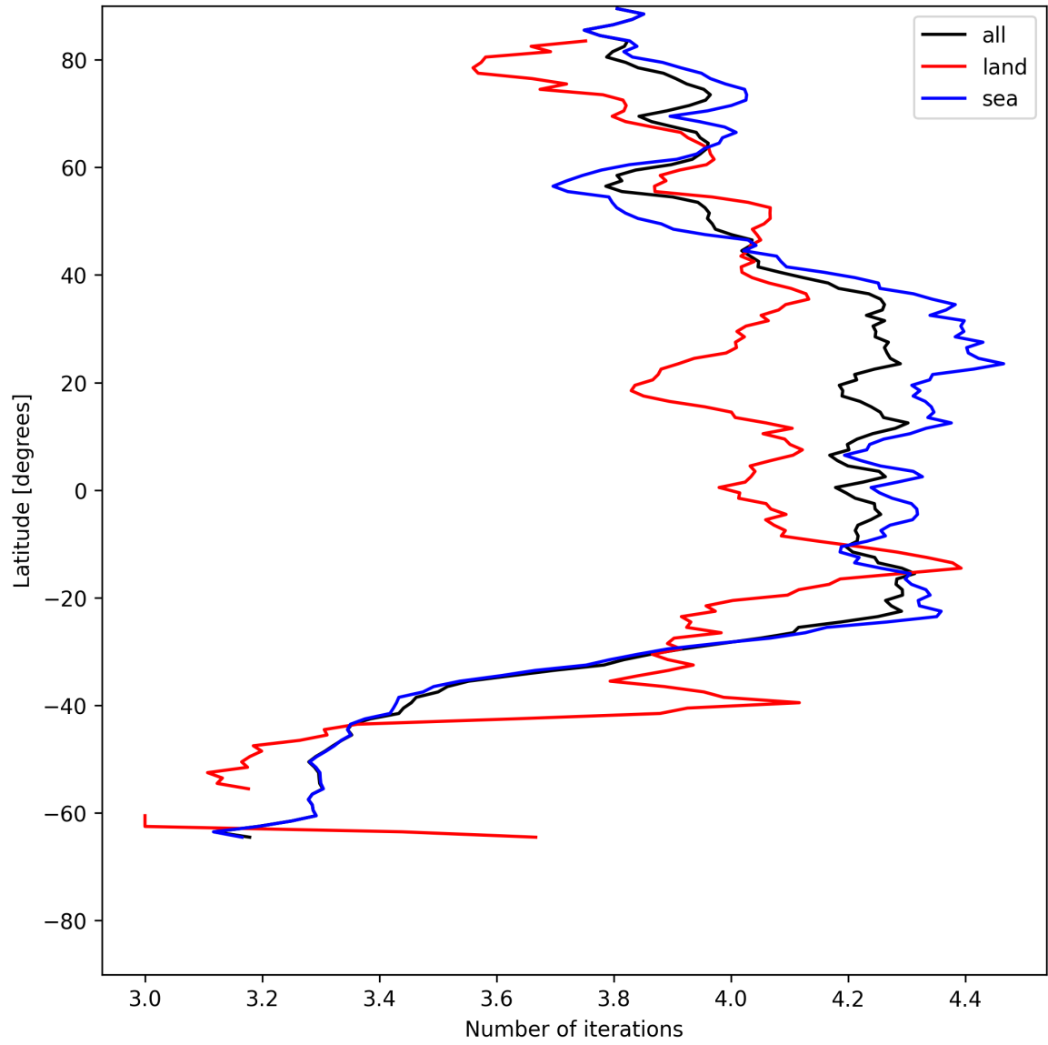
Figure 15: Zonal average of “Number of iterations” for 2025-07-03 to 2025-07-04.
