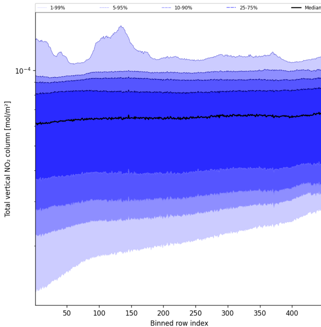
Figure 53: Along track statistics of “Total vertical NO 2 column” for 2025-07-03 to 2025-07-04
