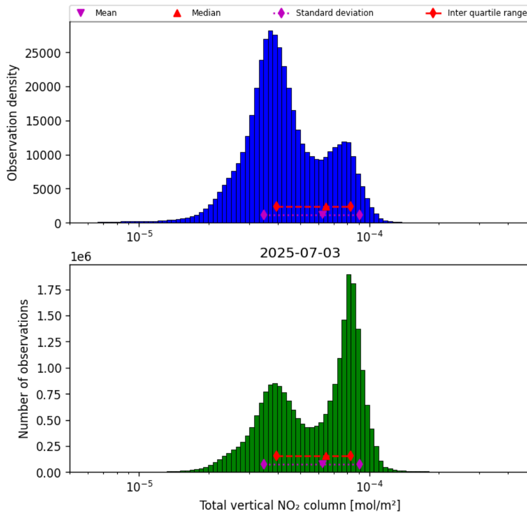
Figure 36: Histogram of “Total vertical NO 2 column” for 2025-07-03 to 2025-07-04
