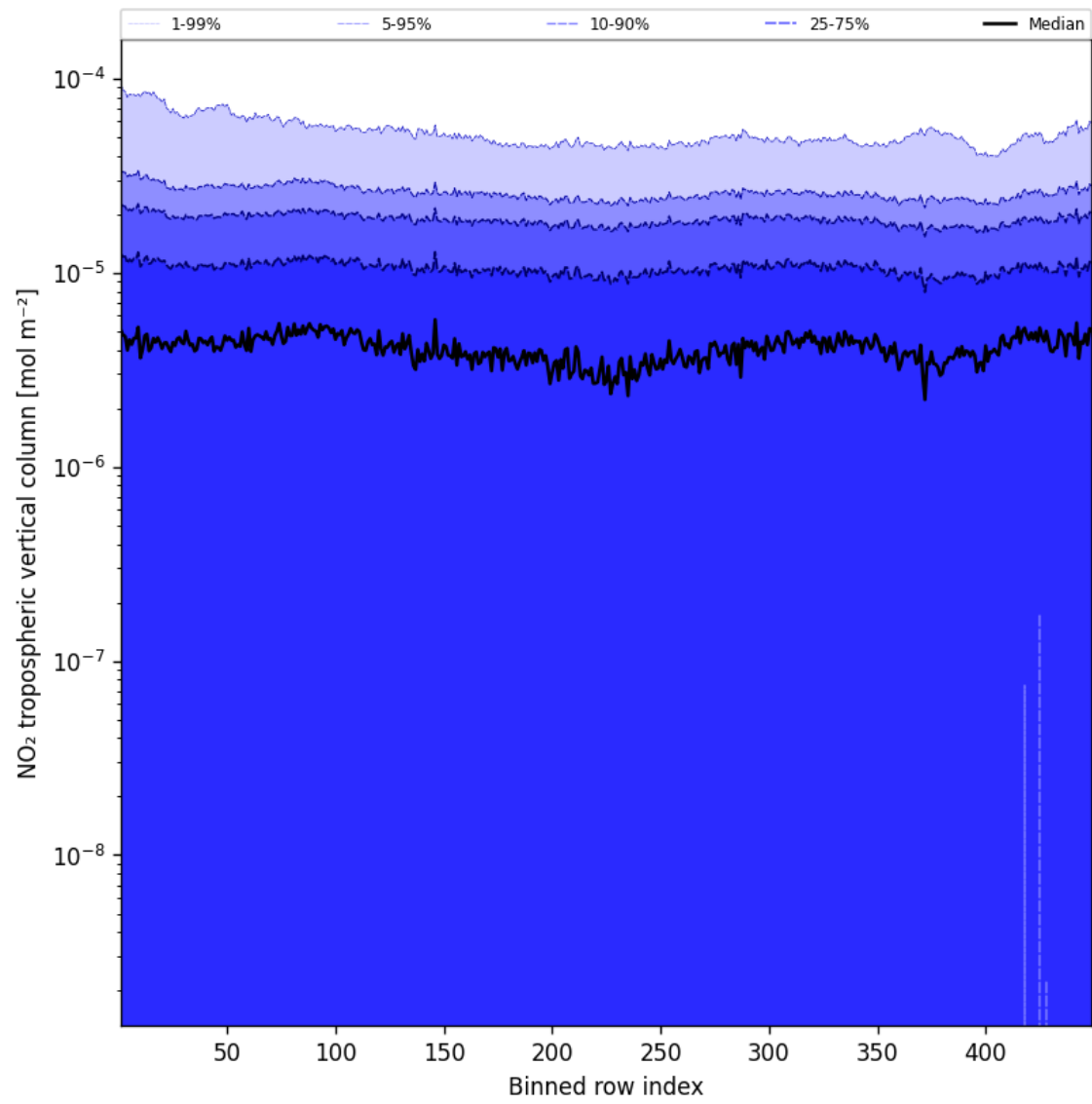
Figure 44: Along track statistics of “NO 2 tropospheric vertical column” for 2025-07-03 to 2025-07-04
