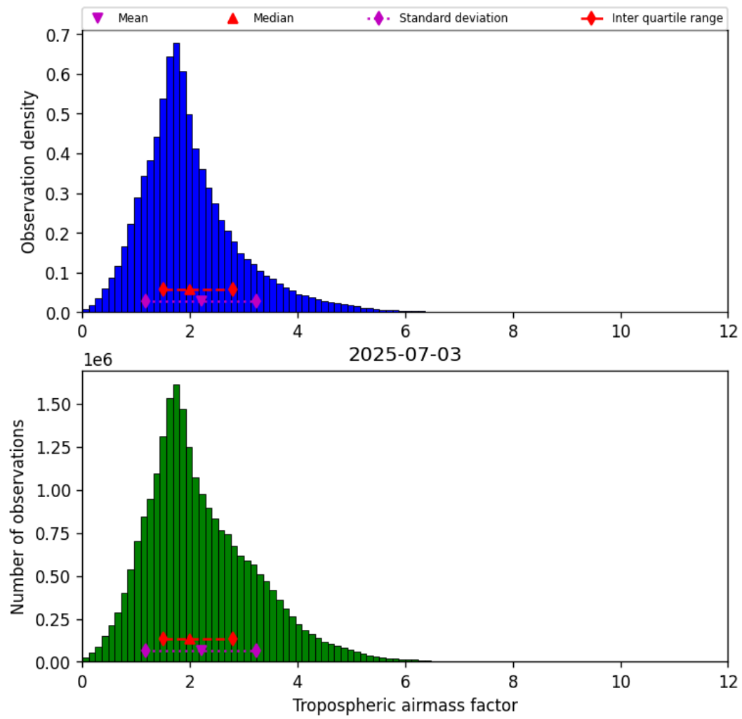
Figure 29: Histogram of “Tropospheric airmass factor” for 2025-07-03 to 2025-07-04
