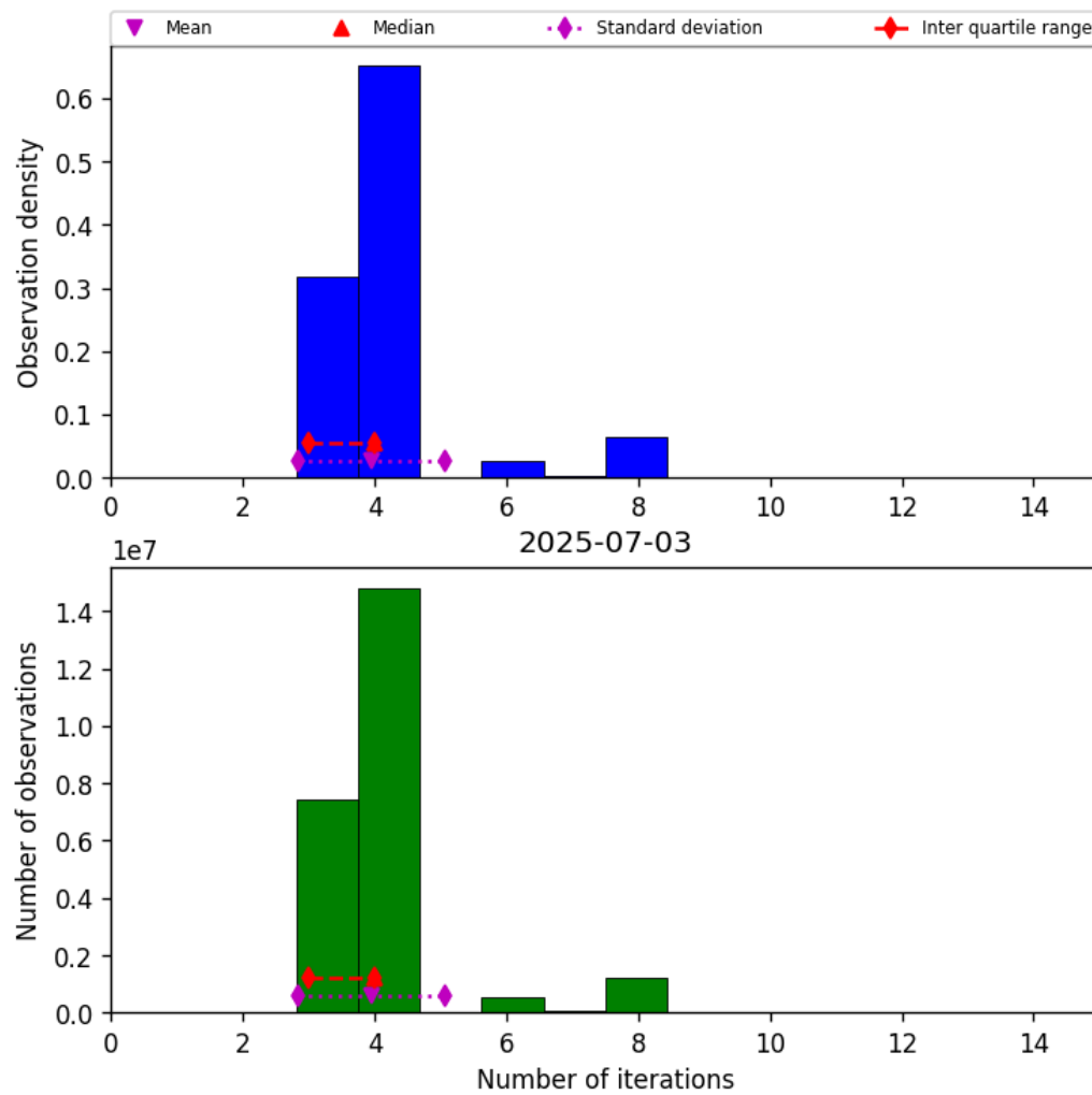
Figure 32: Histogram of “Number of iterations” for 2025-07-03 to 2025-07-04
