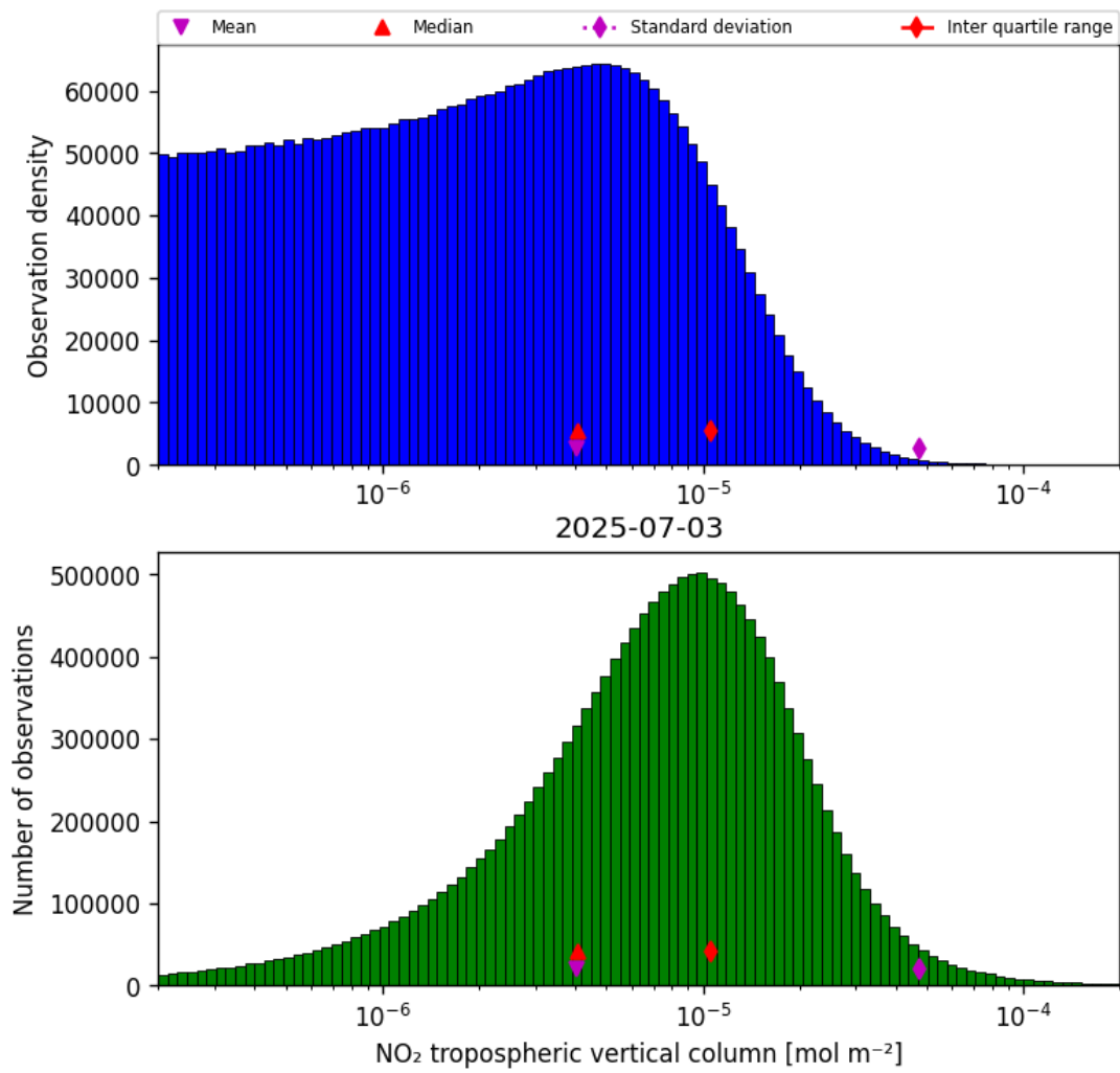
Figure 27: Histogram of “NO 2 tropospheric vertical column” for 2025-07-03 to 2025-07-04
