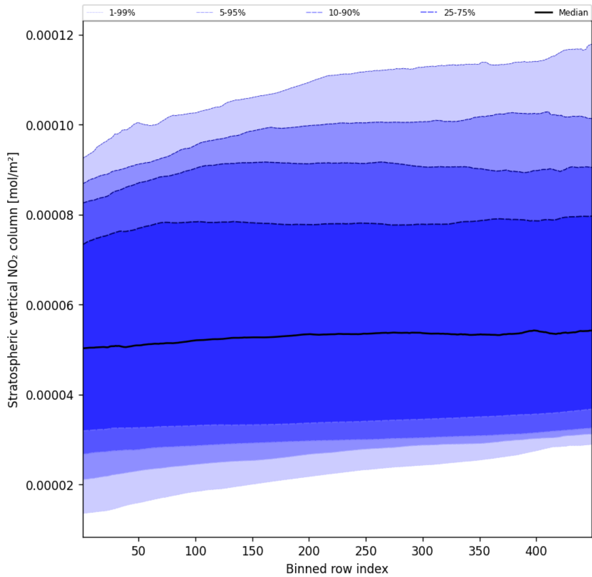
Figure 51: Along track statistics of “Stratospheric vertical NO 2 column” for 2025-07-03 to 2025-07-04
