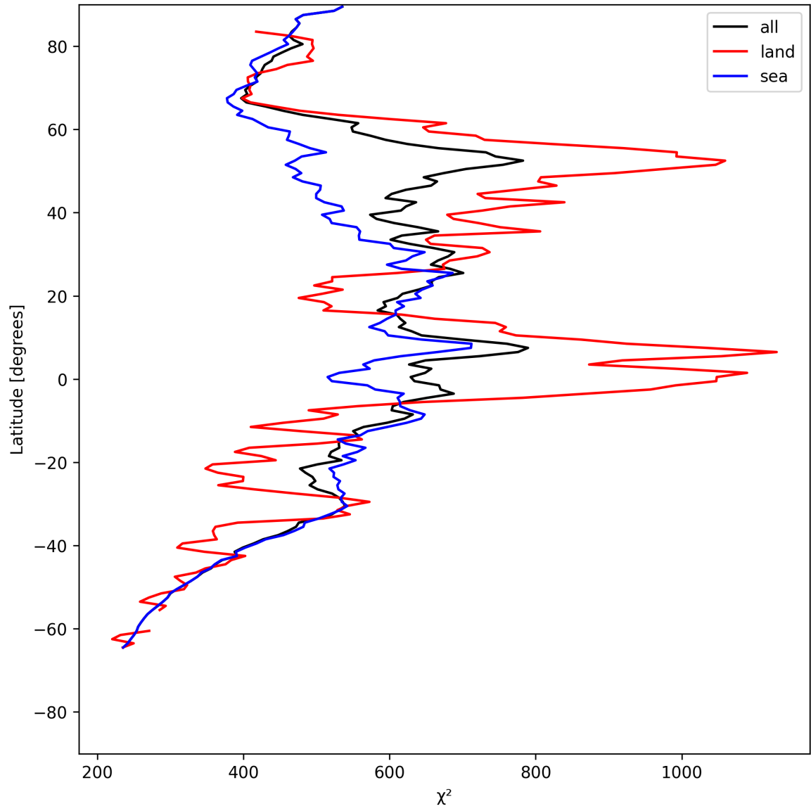
Figure 23: Zonal average of “ \chi^2 ” for 2025-07-03 to 2025-07-04.
