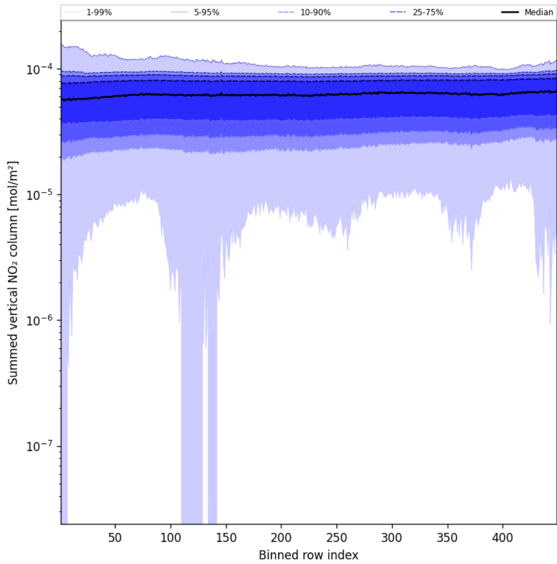
Figure 55: Along track statistics of “Summed vertical NO 2 column” for 2025-07-03 to 2025-07-04
