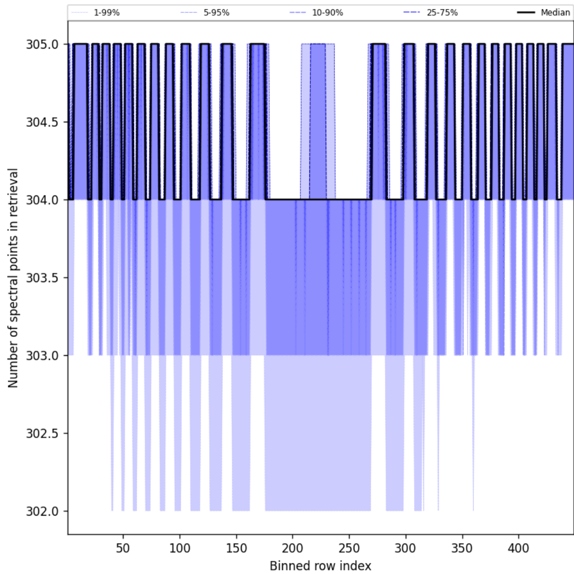
Figure 48: Along track statistics of “Number of spectral points in retrieval” for 2025-07-03 to 2025-07-04
