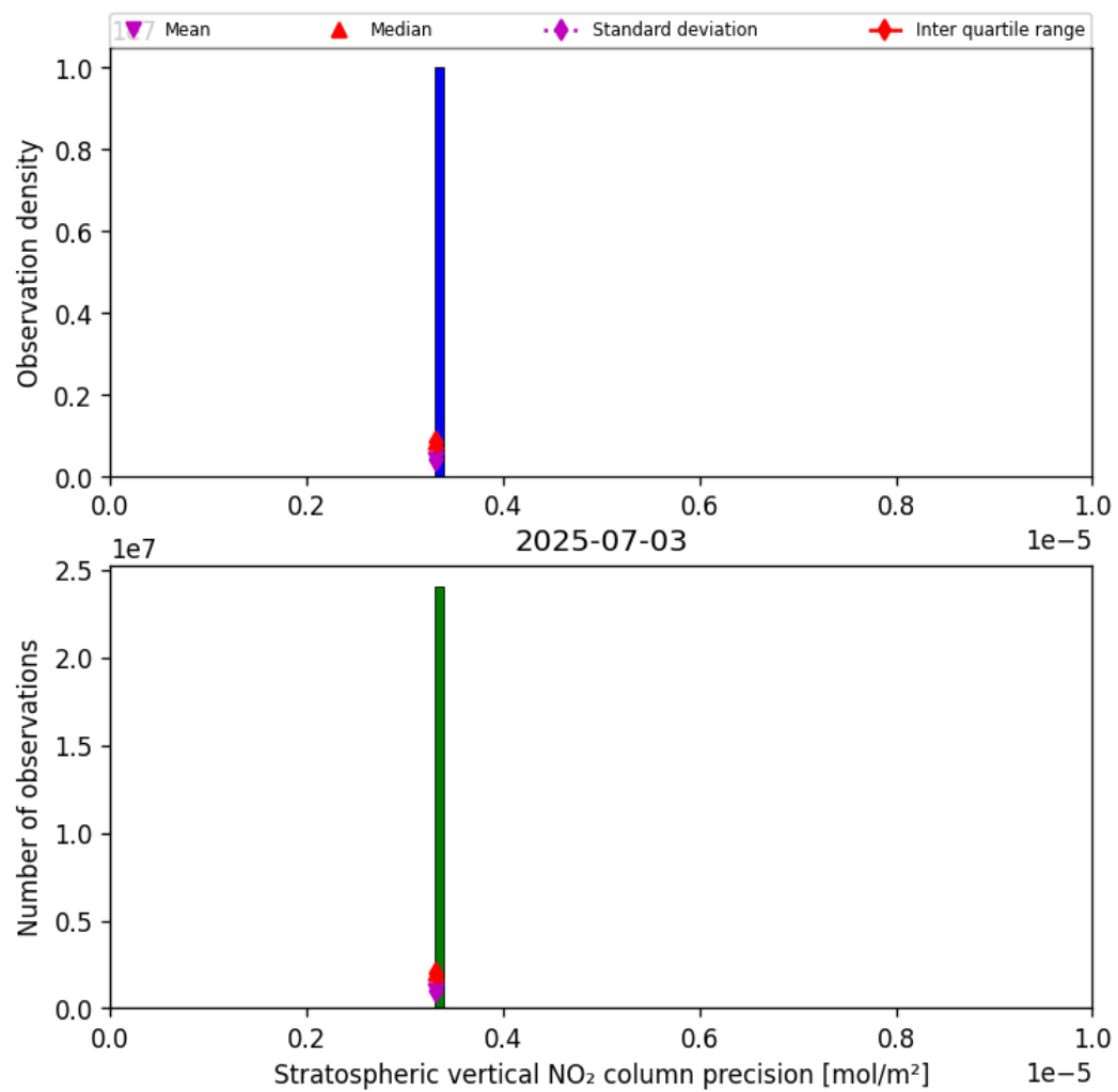
Figure 35: Histogram of “Stratospheric vertical NO 2 column precision” for 2025-07-03 to 2025-07-04
