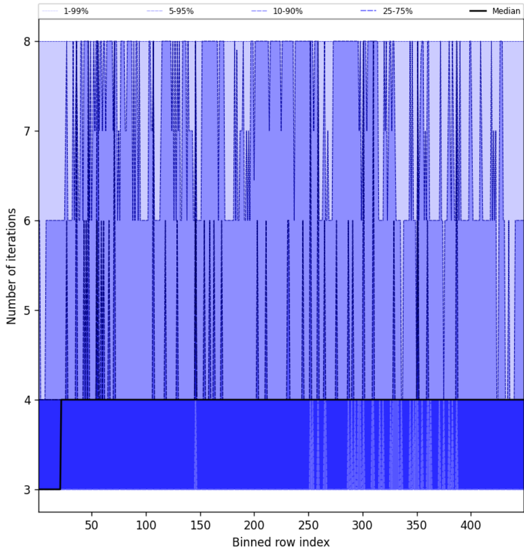
Figure 49: Along track statistics of “Number of iterations” for 2025-07-03 to 2025-07-04
