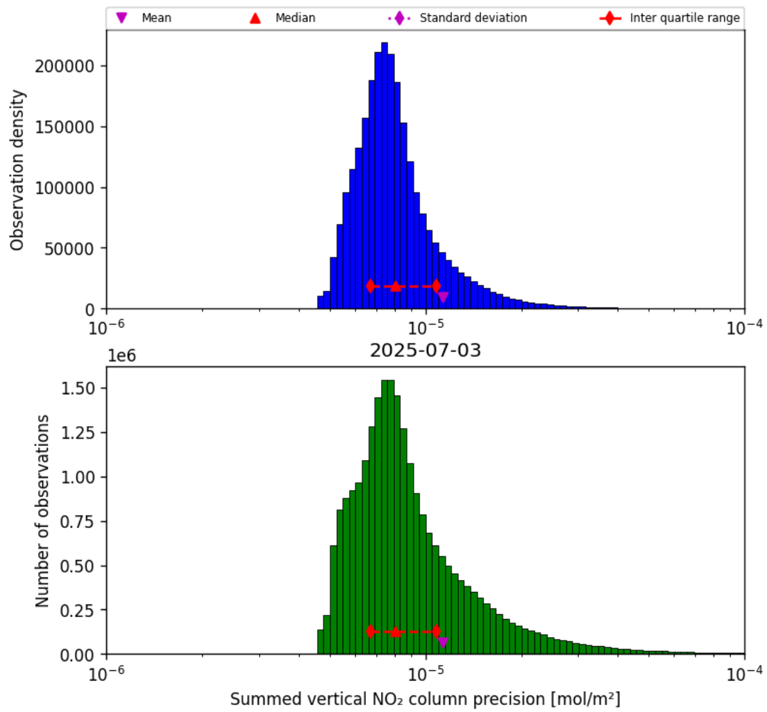
Figure 39: Histogram of "Summed vertical NO 2 column precision" for 2025-07-03 to 2025-07-04
