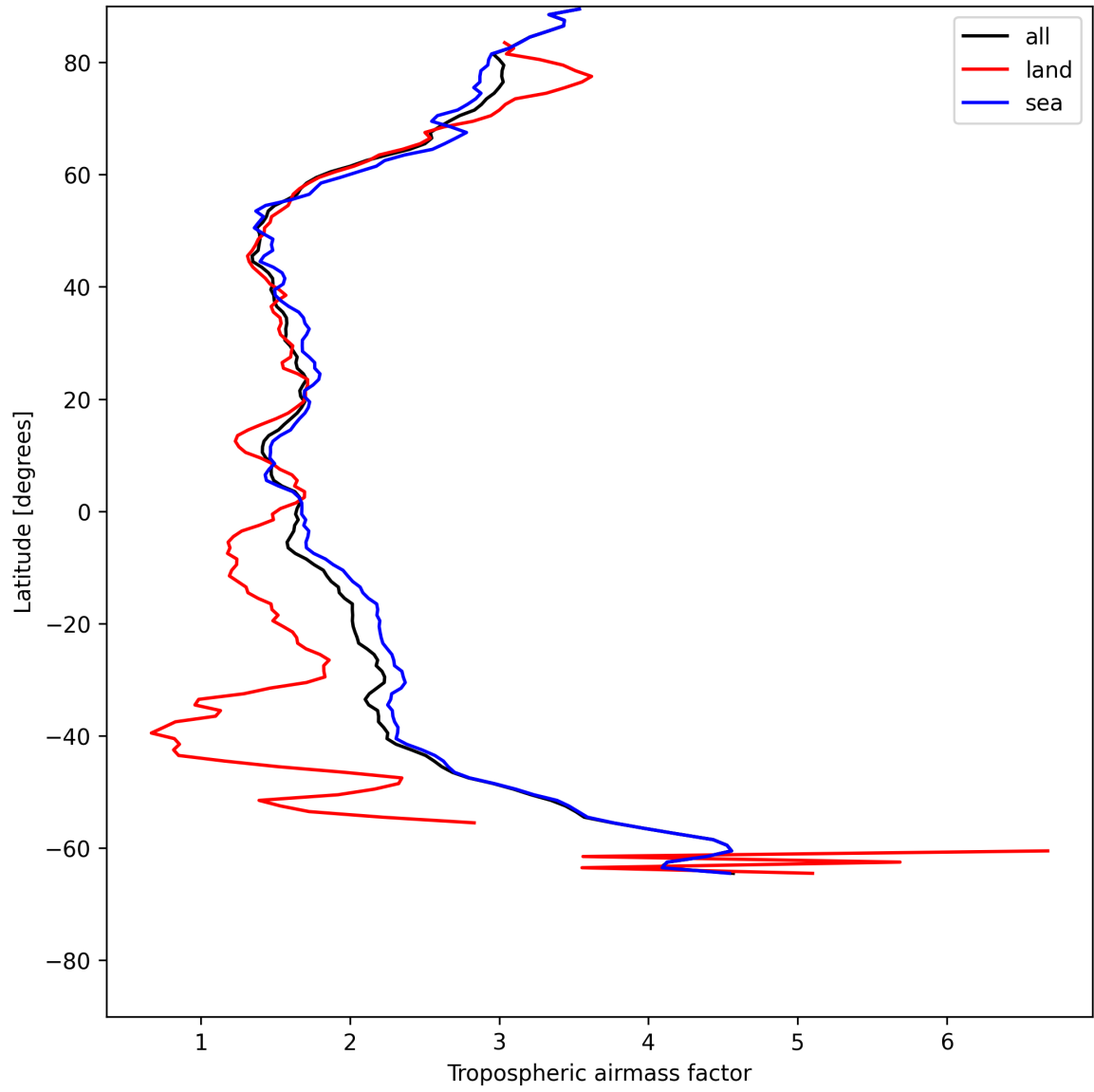
Figure 12: Zonal average of “Tropospheric airmass factor” for 2025-07-03 to 2025-07-04.
