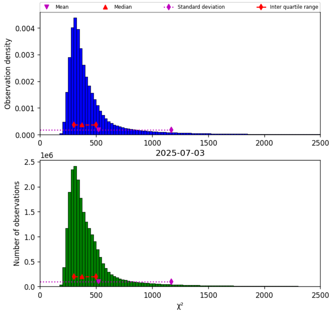
Figure 40: Histogram of “ \chi^2 ” for 2025-07-03 to 2025-07-04
