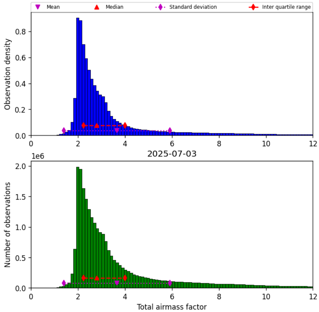
Figure 30: Histogram of “Total airmass factor” for 2025-07-03 to 2025-07-04
