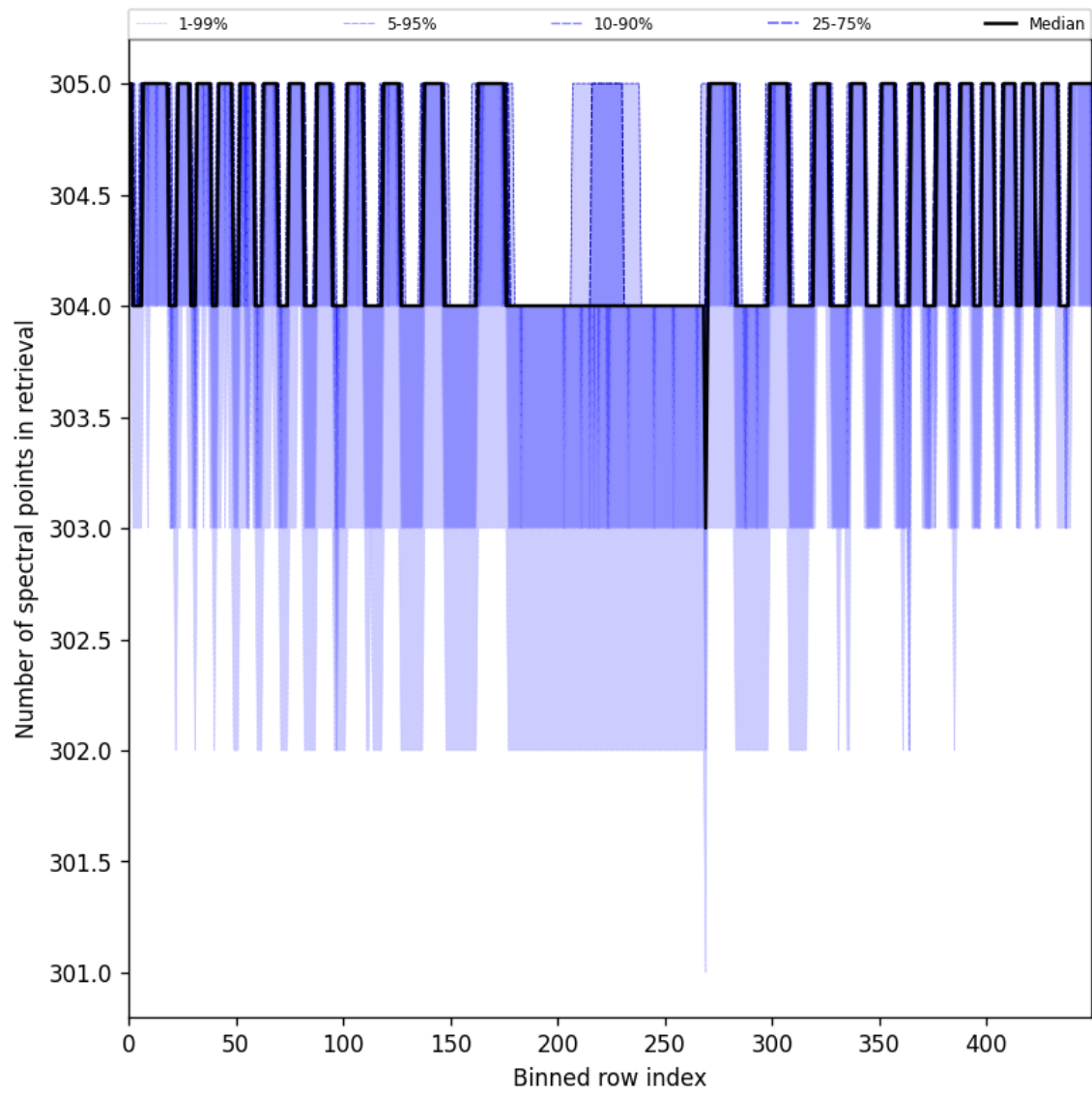
Figure 48: Along track statistics of “Number of spectral points in retrieval” for 2025-07-04 to 2025-07-05
