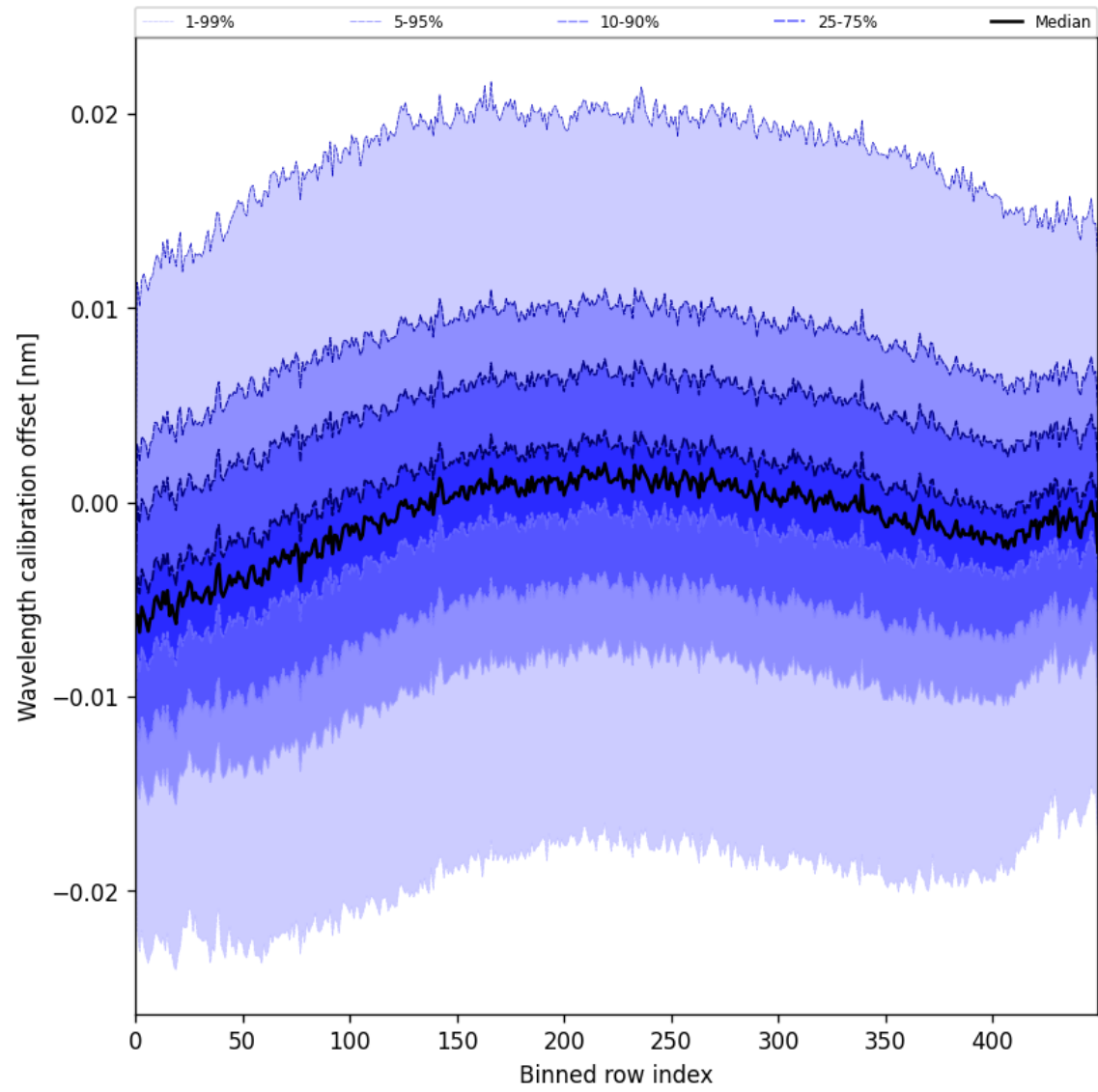
Figure 50: Along track statistics of “Wavelength calibration offset” for 2025-07-04 to 2025-07-05
