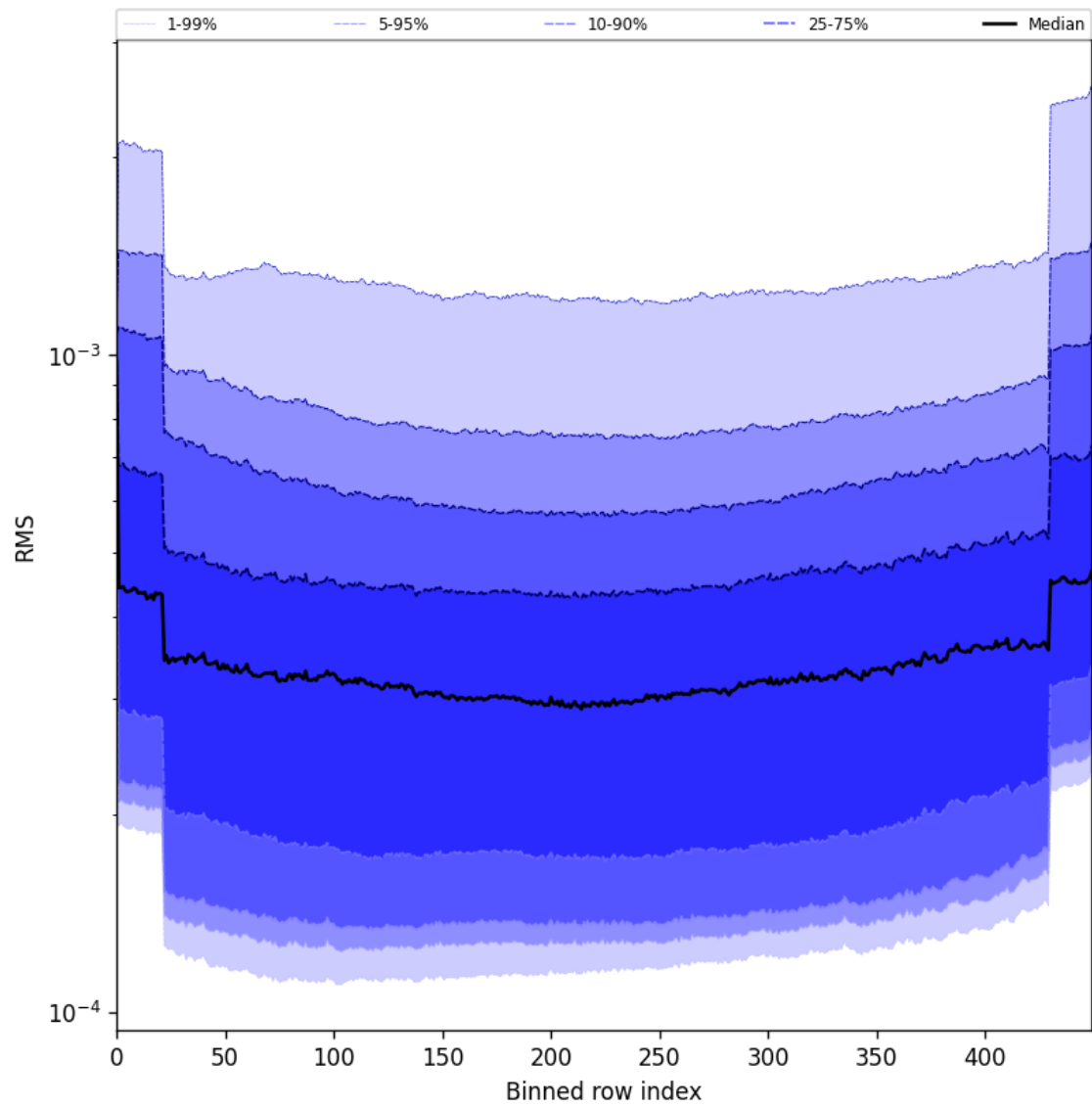
Figure 58: Along track statistics of “RMS” for 2025-07-04 to 2025-07-05
