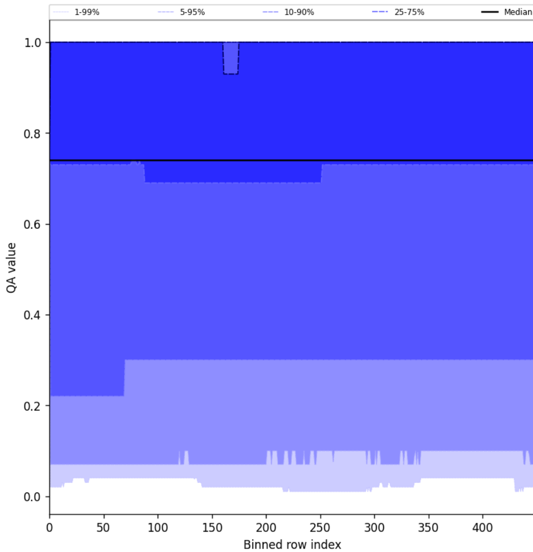
Figure 43: Along track statistics of “QA value” for 2025-07-04 to 2025-07-05
