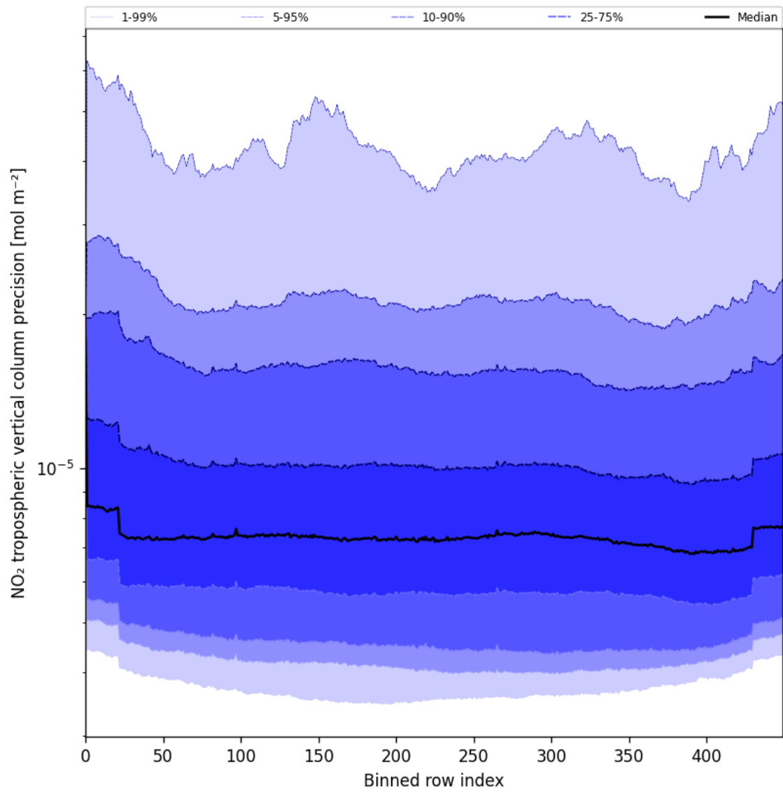
Figure 45: Along track statistics of “NO 2 tropospheric vertical column precision” for 2025-07-04 to 2025-07-05
