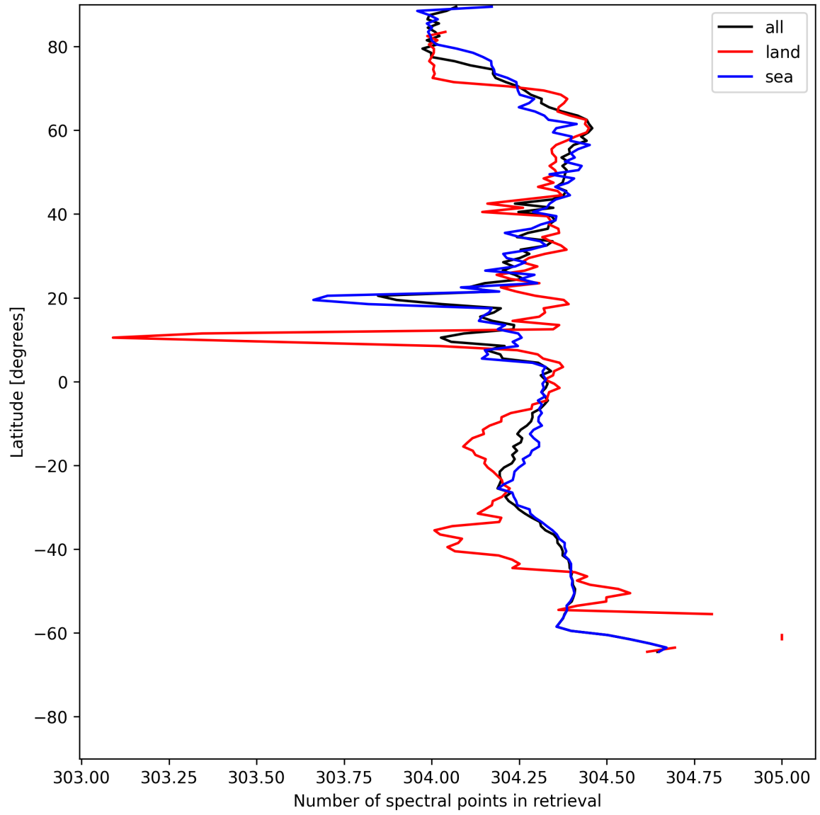
Figure 14: Zonal average of “Number of spectral points in retrieval” for 2025-07-04 to 2025-07-05.
