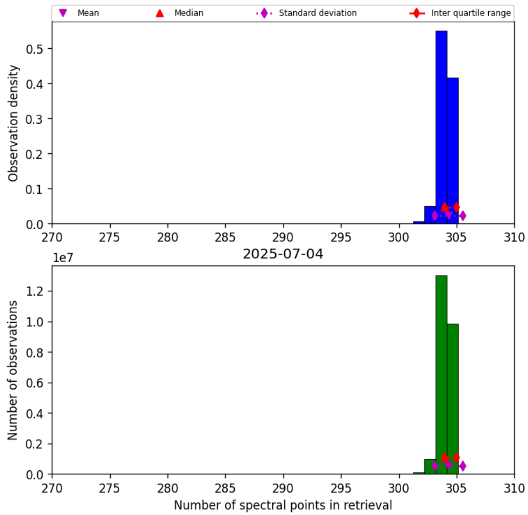
Figure 31: Histogram of “Number of spectral points in retrieval” for 2025-07-04 to 2025-07-05
