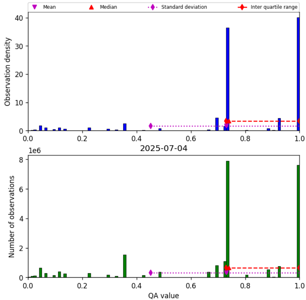
Figure 26: Histogram of “QA value” for 2025-07-04 to 2025-07-05
