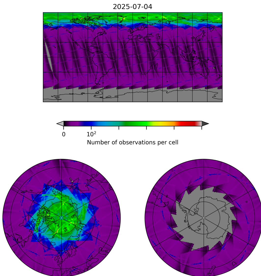
Figure 8: Map of the number of observations for 2025-07-04 to 2025-07-05
