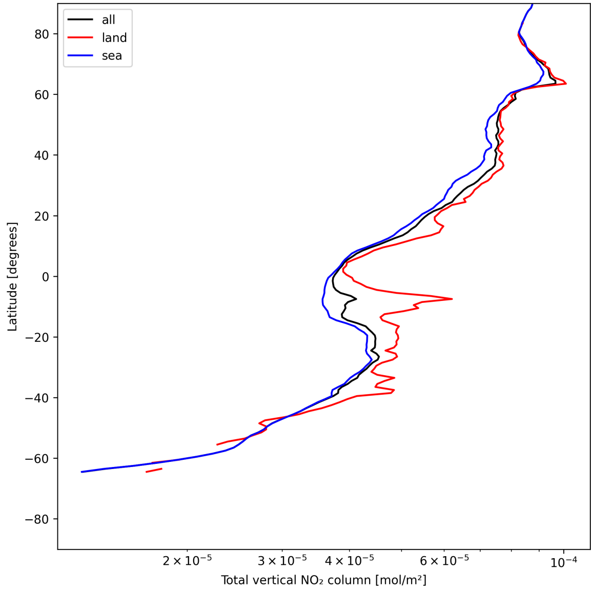
Figure 19: Zonal average of “Total vertical NO 2 column” for 2025-07-04 to 2025-07-05.
