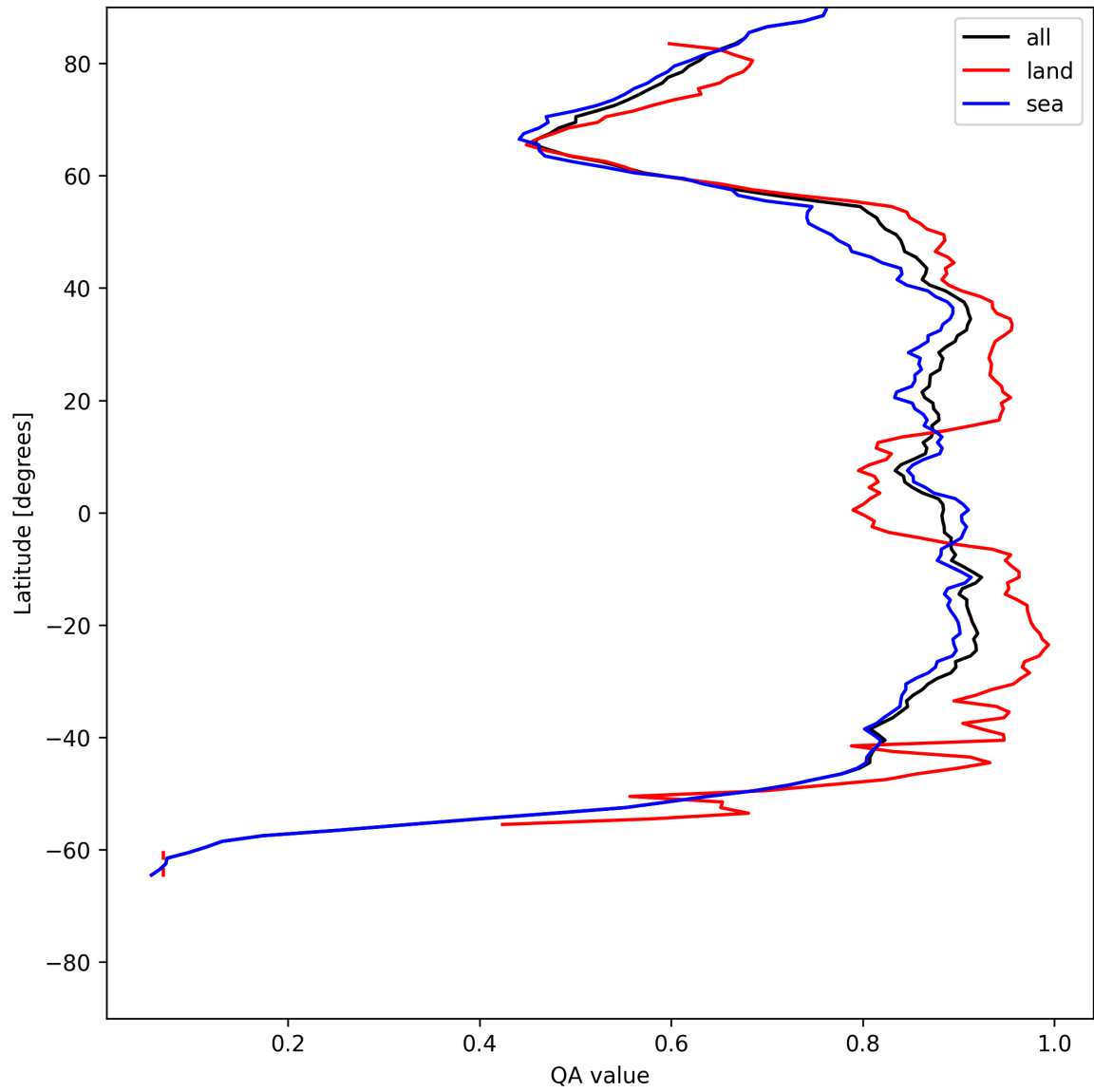
Figure 9: Zonal average of “QA value” for 2025-07-04 to 2025-07-05.
