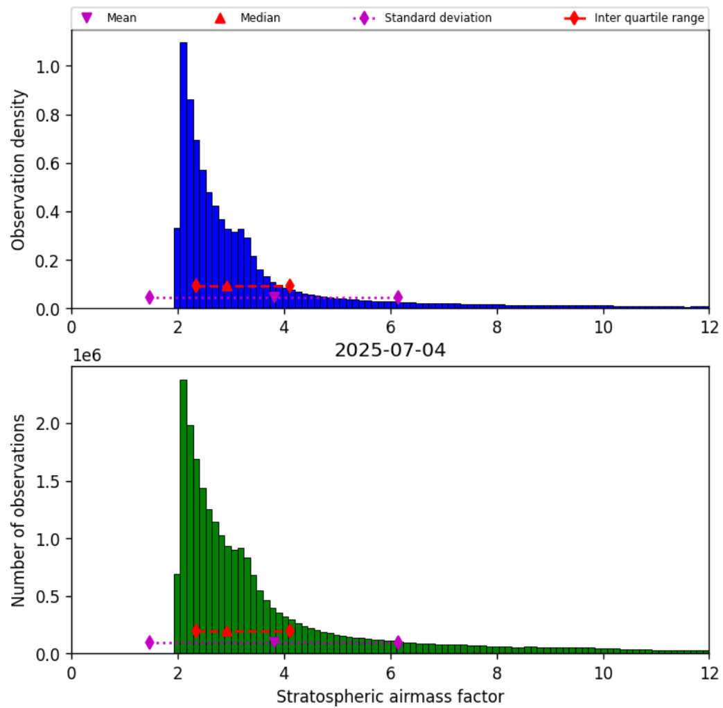
Figure 42: Histogram of “Stratospheric airmass factor” for 2025-07-04 to 2025-07-05
