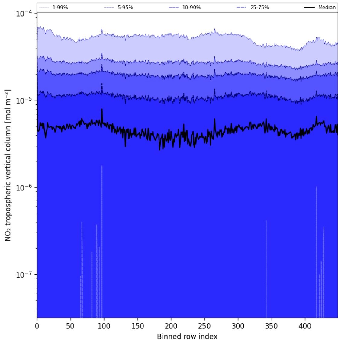
Figure 44: Along track statistics of “NO 2 tropospheric vertical column” for 2025-07-04 to 2025-07-05
