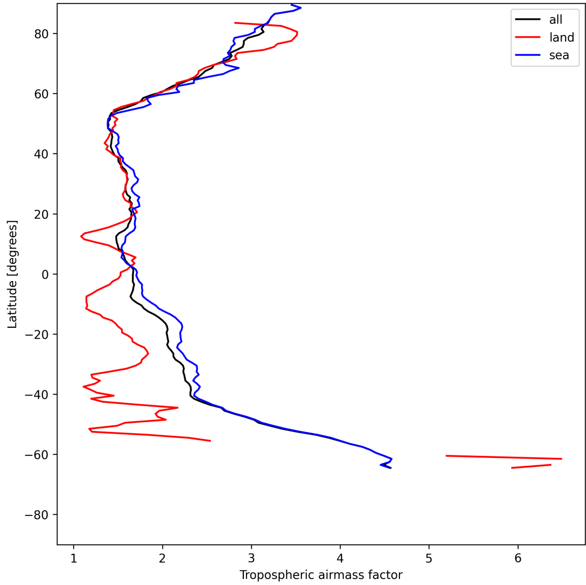
Figure 12: Zonal average of “Tropospheric airmass factor” for 2025-07-04 to 2025-07-05.
