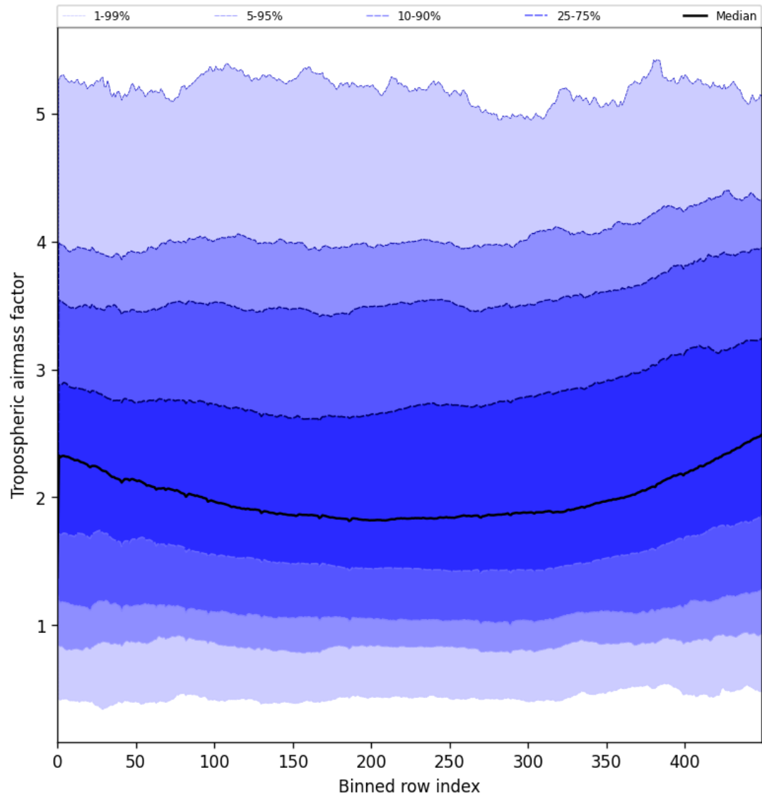
Figure 46: Along track statistics of “Tropospheric airmass factor” for 2025-07-04 to 2025-07-05
