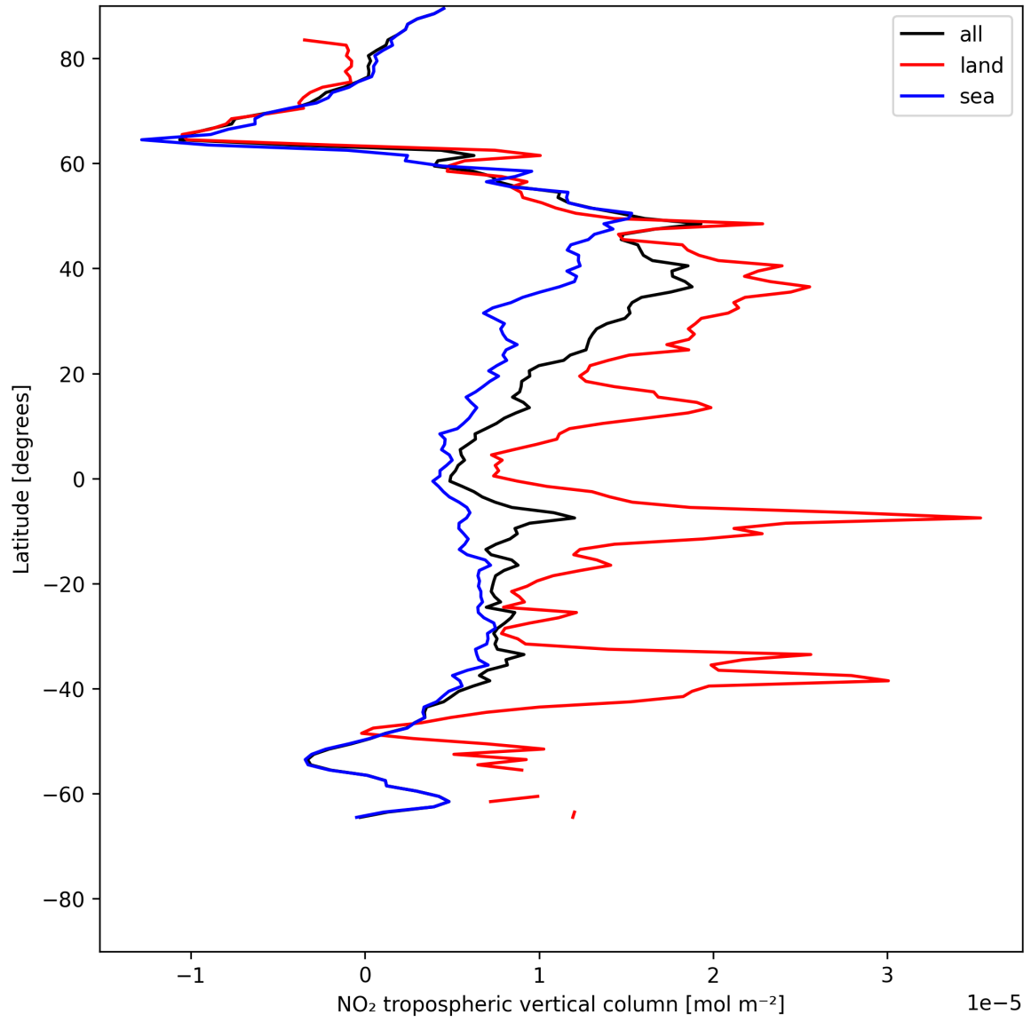
Figure 10: Zonal average of “NO 2 tropospheric vertical column” for 2025-07-04 to 2025-07-05.
