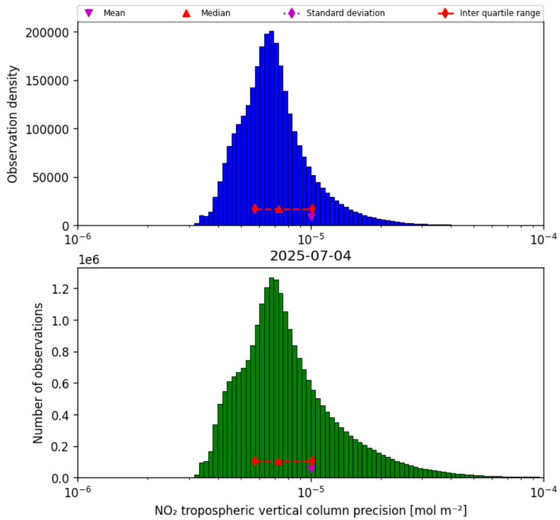
Figure 28: Histogram of “NO 2 tropospheric vertical column precision” for 2025-07-04 to 2025-07-05
