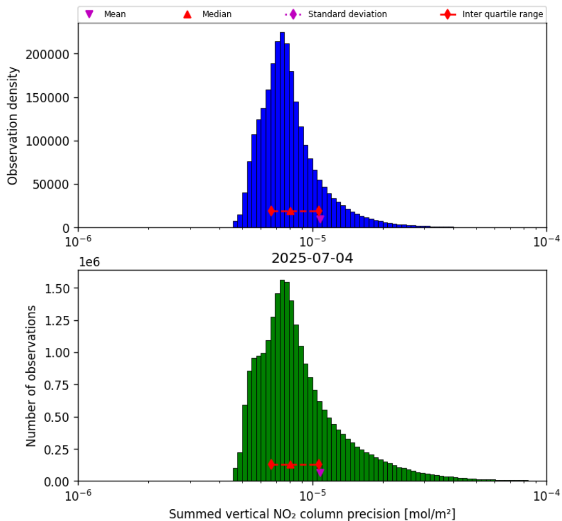
Figure 39: Histogram of "Summed vertical NO 2 column precision" for 2025-07-04 to 2025-07-05
