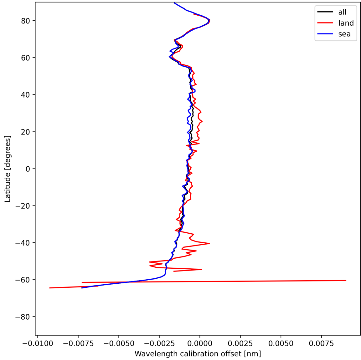
Figure 16: Zonal average of “Wavelength calibration offset” for 2025-07-04 to 2025-07-05.
