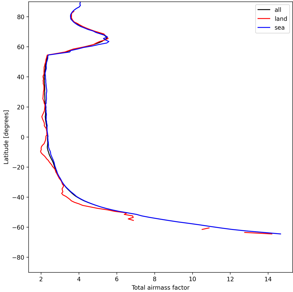
Figure 13: Zonal average of “Total airmass factor” for 2025-07-04 to 2025-07-05.
