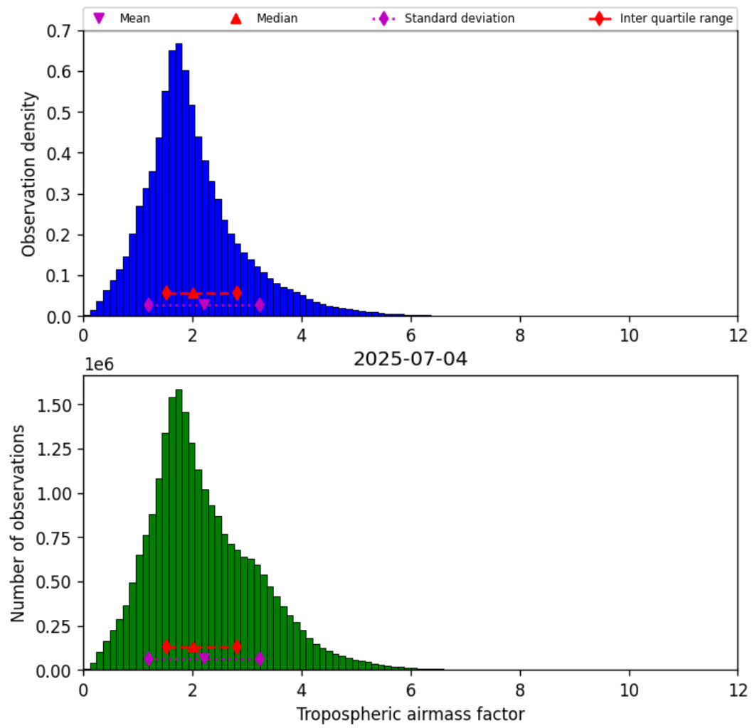
Figure 29: Histogram of “Tropospheric airmass factor” for 2025-07-04 to 2025-07-05
