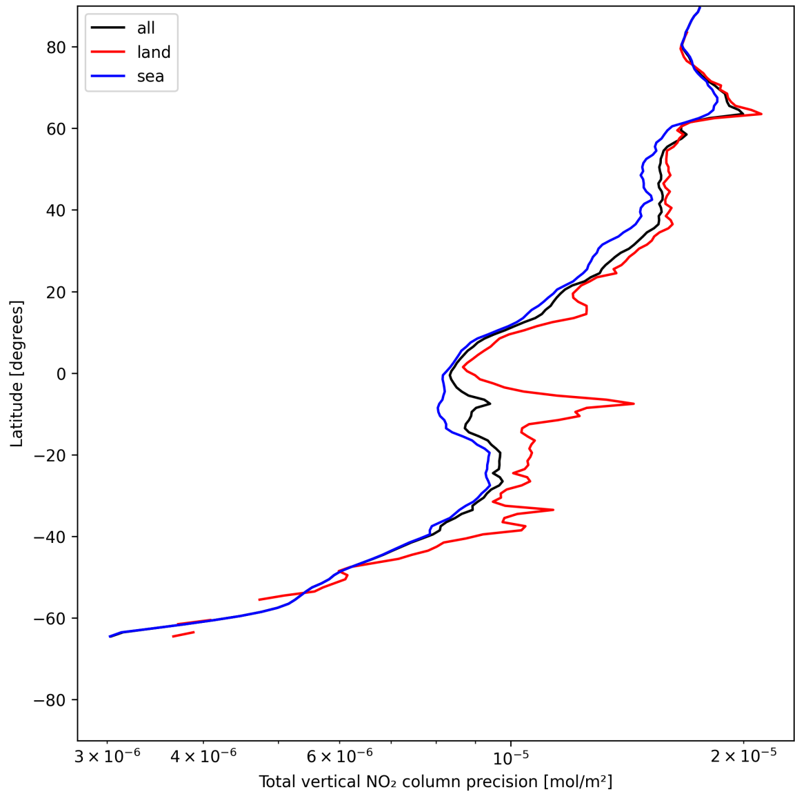
Figure 20: Zonal average of “Total vertical NO 2 column precision” for 2025-07-04 to 2025-07-05.
