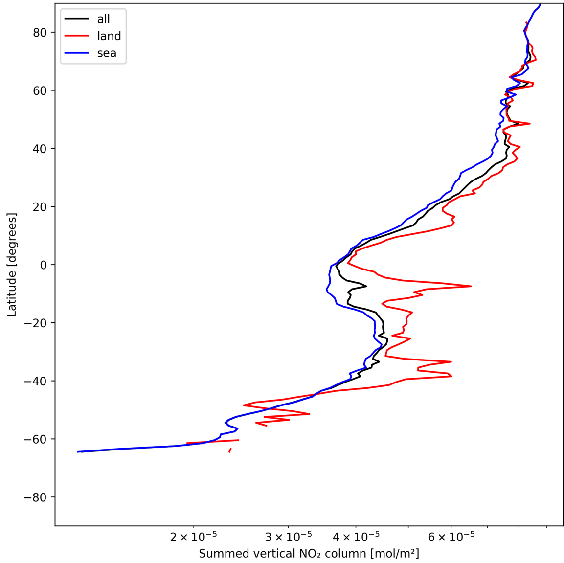
Figure 21: Zonal average of “Summed vertical NO 2 column” for 2025-07-04 to 2025-07-05.
