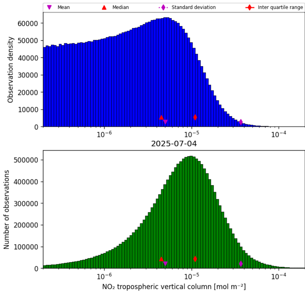
Figure 27: Histogram of “NO 2 tropospheric vertical column” for 2025-07-04 to 2025-07-05
