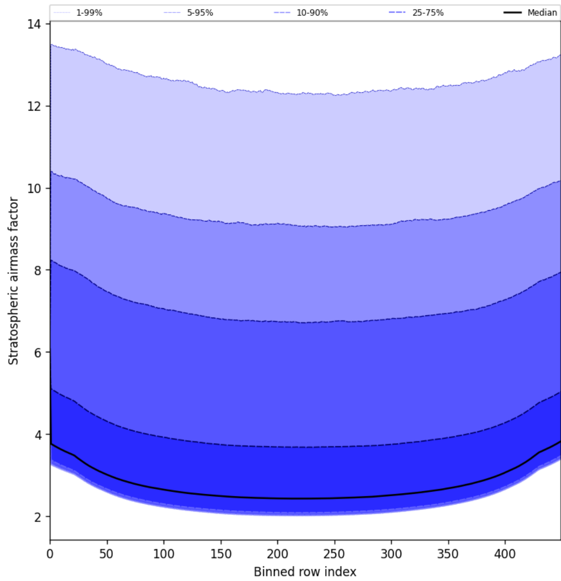
Figure 59: Along track statistics of “Stratospheric airmass factor” for 2025-07-04 to 2025-07-05
