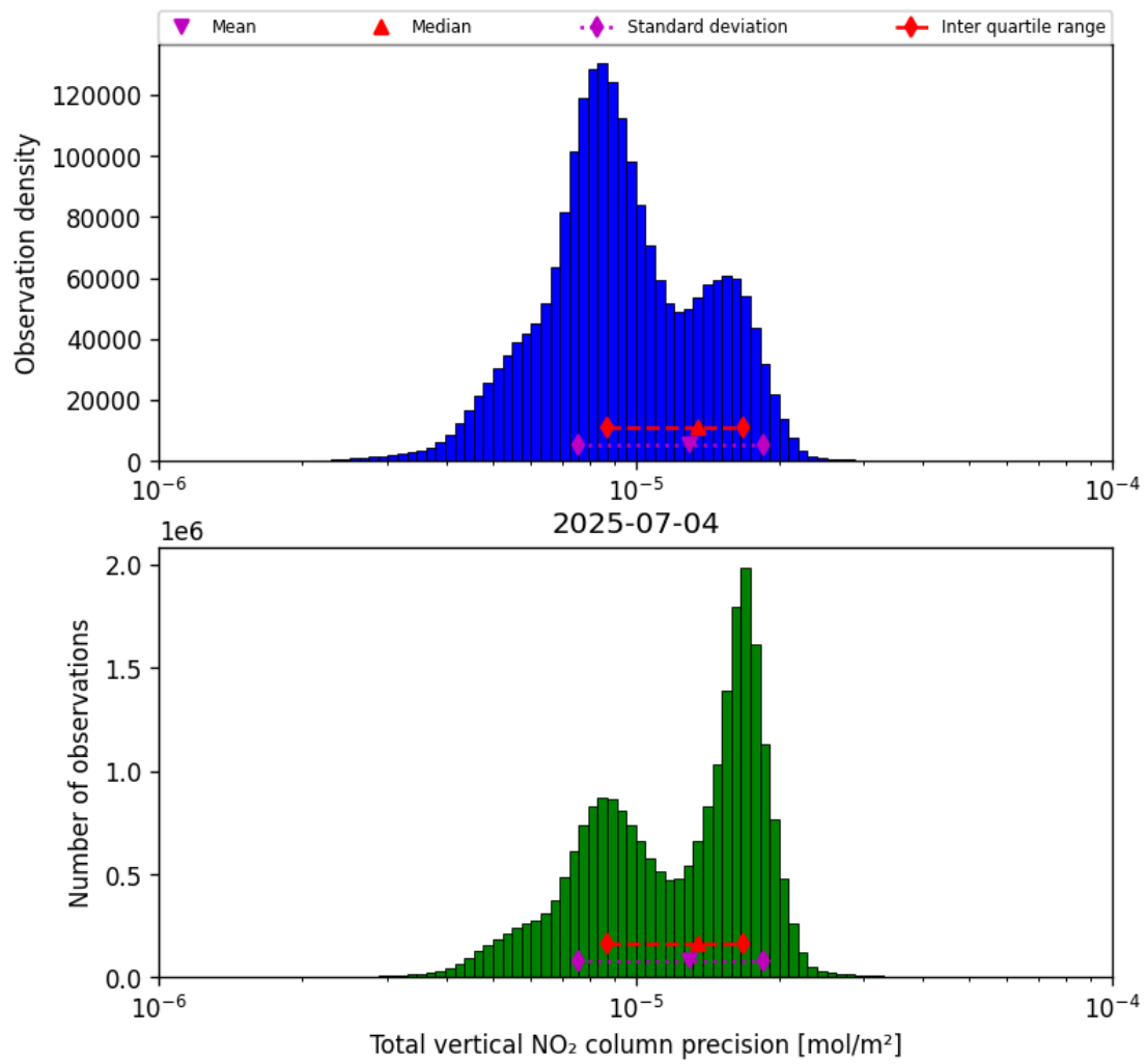
Figure 37: Histogram of “Total vertical NO 2 column precision” for 2025-07-04 to 2025-07-05
