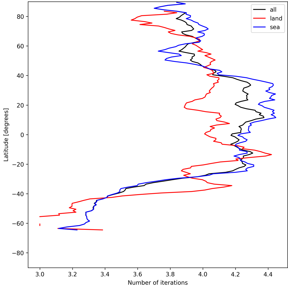
Figure 15: Zonal average of “Number of iterations” for 2025-07-04 to 2025-07-05.
