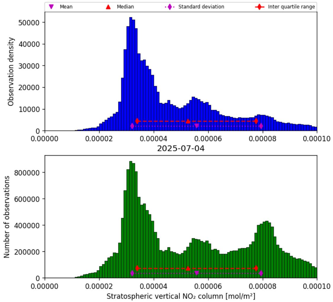
Figure 34: Histogram of “Stratospheric vertical NO 2 column” for 2025-07-04 to 2025-07-05
