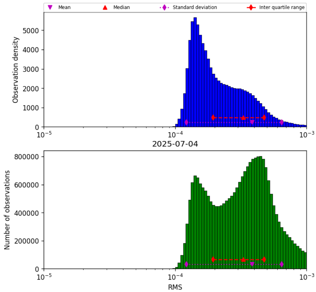
Figure 41: Histogram of “RMS” for 2025-07-04 to 2025-07-05
