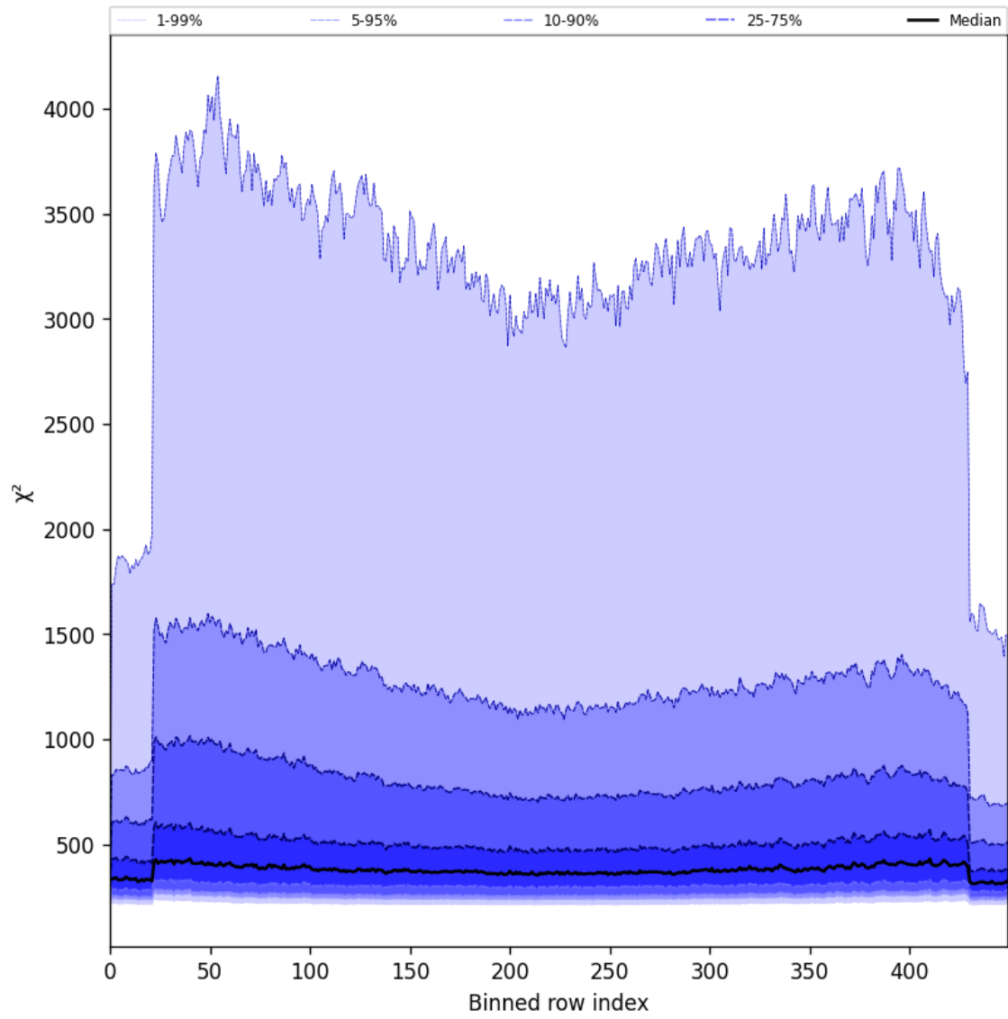
Figure 57: Along track statistics of “ \chi^2 ” for 2025-07-04 to 2025-07-05
