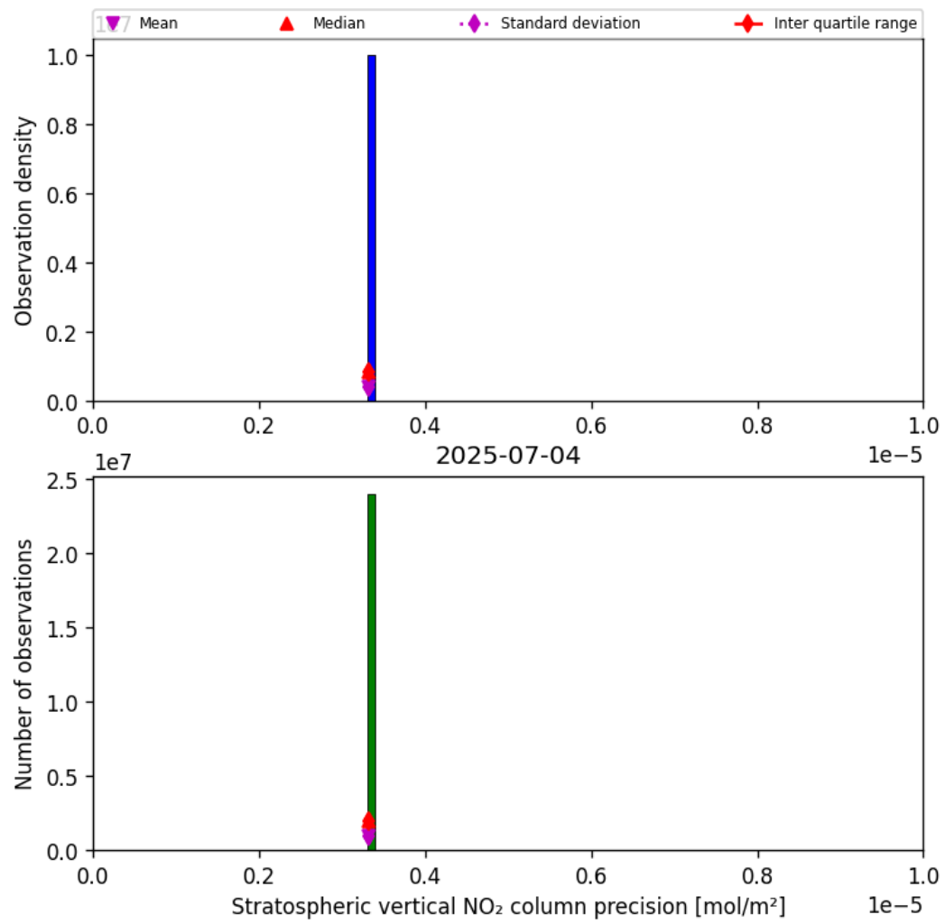
Figure 35: Histogram of “Stratospheric vertical NO 2 column precision” for 2025-07-04 to 2025-07-05
