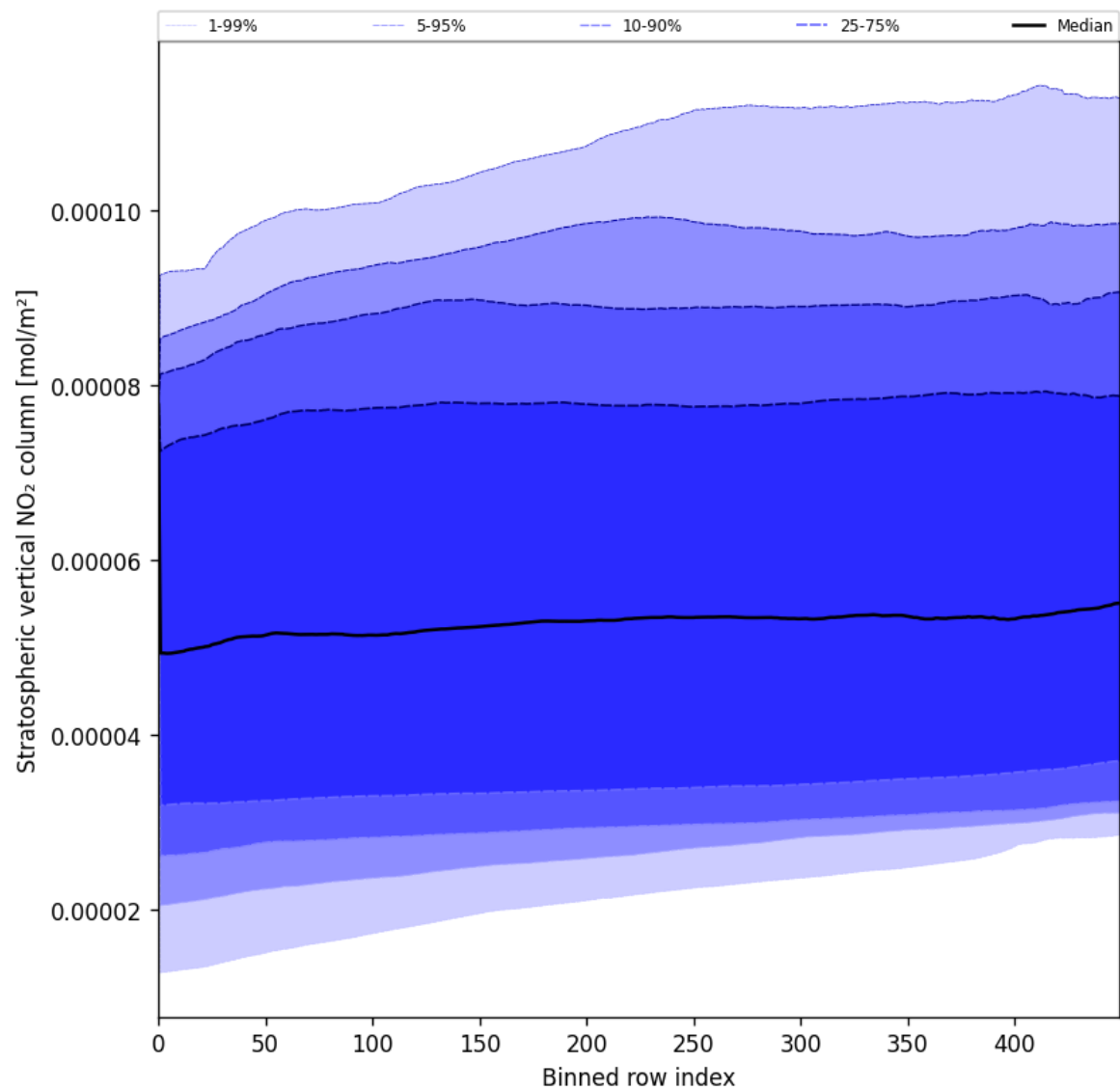
Figure 51: Along track statistics of “Stratospheric vertical NO 2 column” for 2025-07-04 to 2025-07-05
