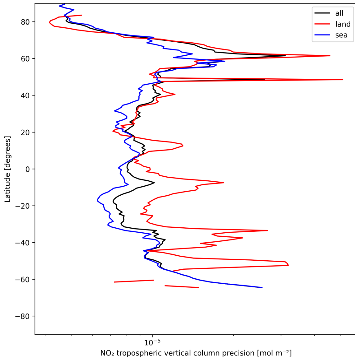
Figure 11: Zonal average of “NO 2 tropospheric vertical column precision” for 2025-07-04 to 2025-07-05.
