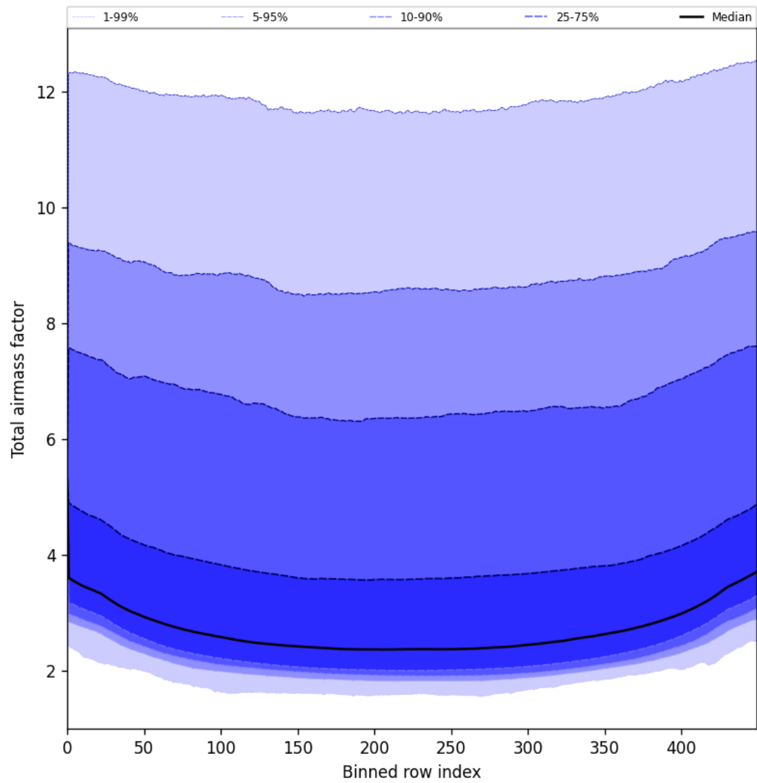
Figure 47: Along track statistics of “Total airmass factor” for 2025-07-04 to 2025-07-05
