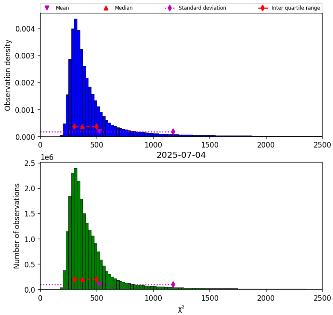
Figure 40: Histogram of “ \chi^2 ” for 2025-07-04 to 2025-07-05
