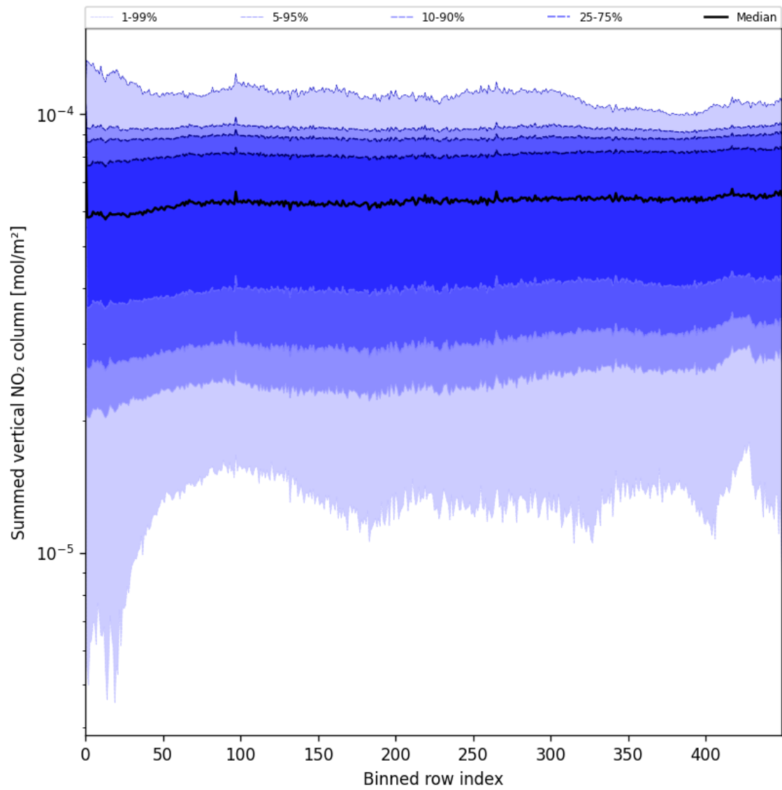
Figure 55: Along track statistics of “Summed vertical NO 2 column” for 2025-07-04 to 2025-07-05
