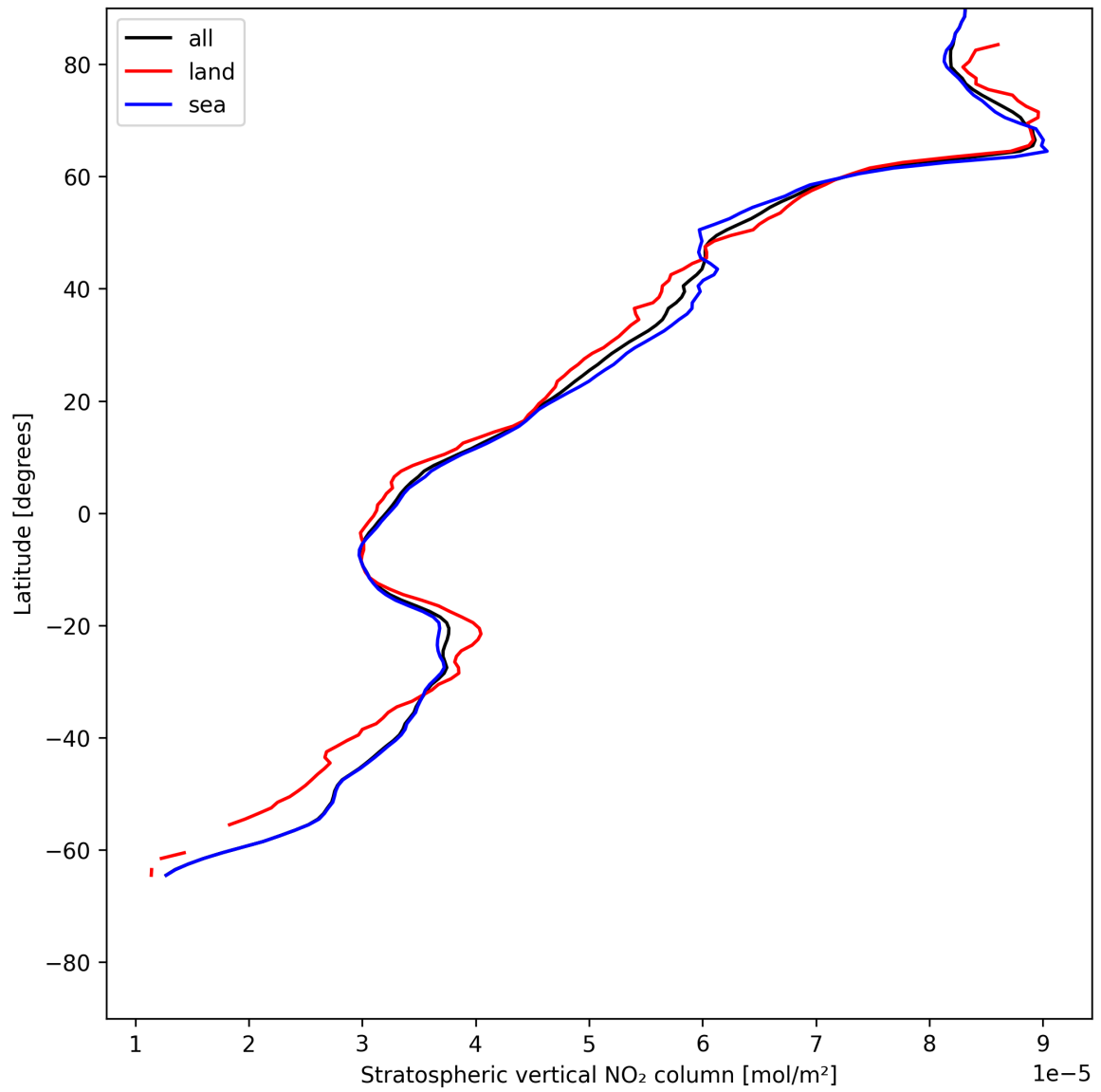
Figure 17: Zonal average of “Stratospheric vertical NO 2 column” for 2025-07-04 to 2025-07-05.
