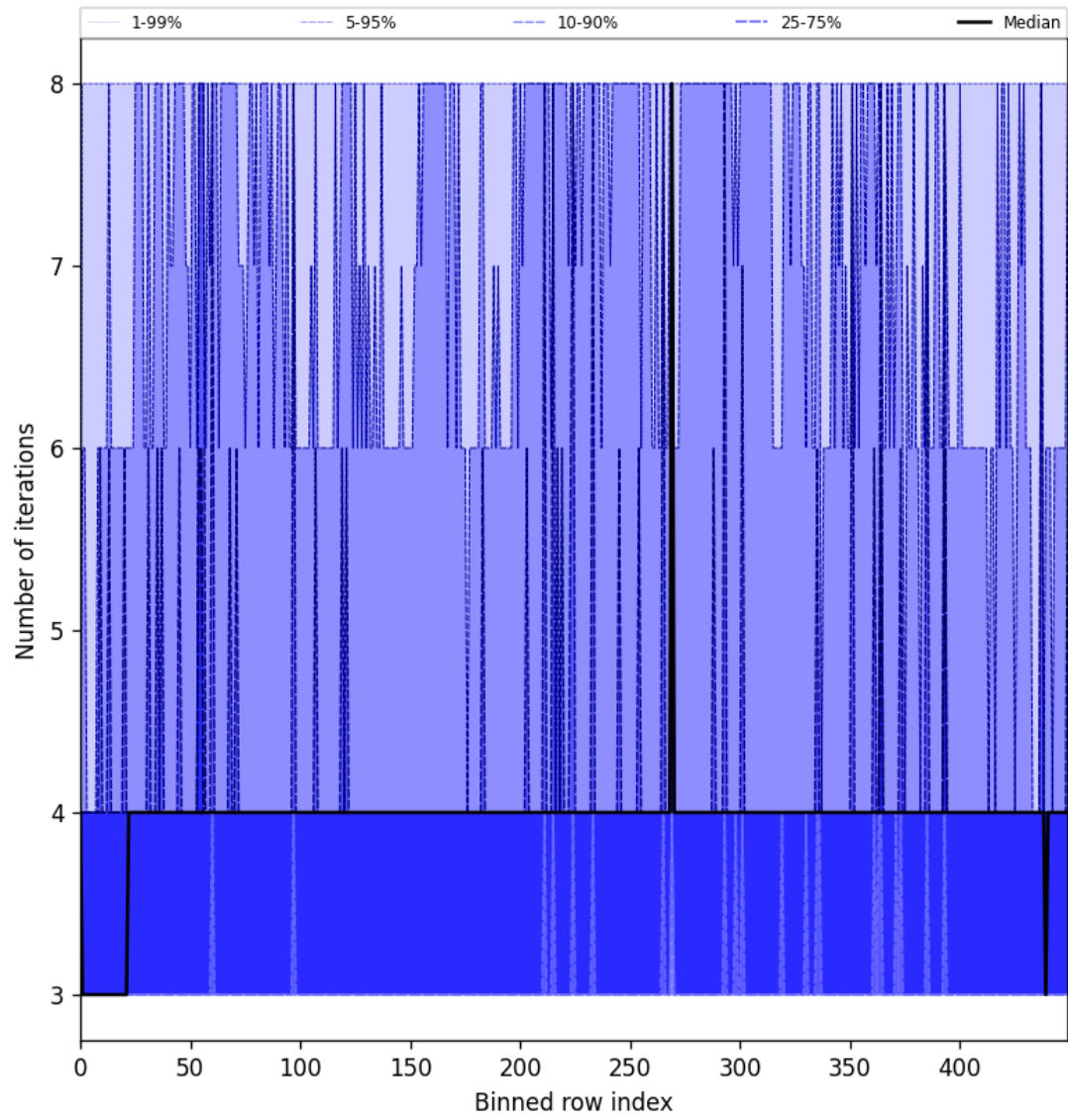
Figure 49: Along track statistics of “Number of iterations” for 2025-07-04 to 2025-07-05
