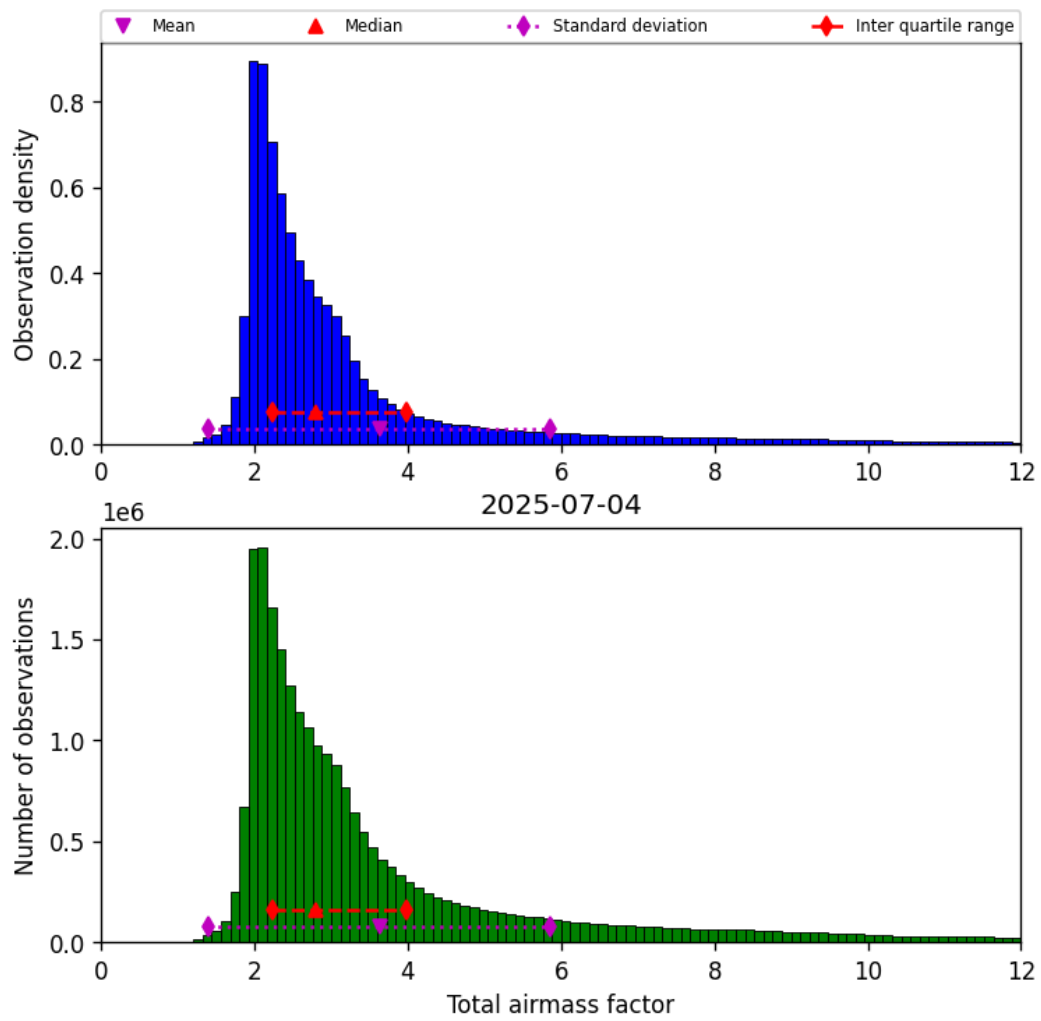
Figure 30: Histogram of “Total airmass factor” for 2025-07-04 to 2025-07-05
