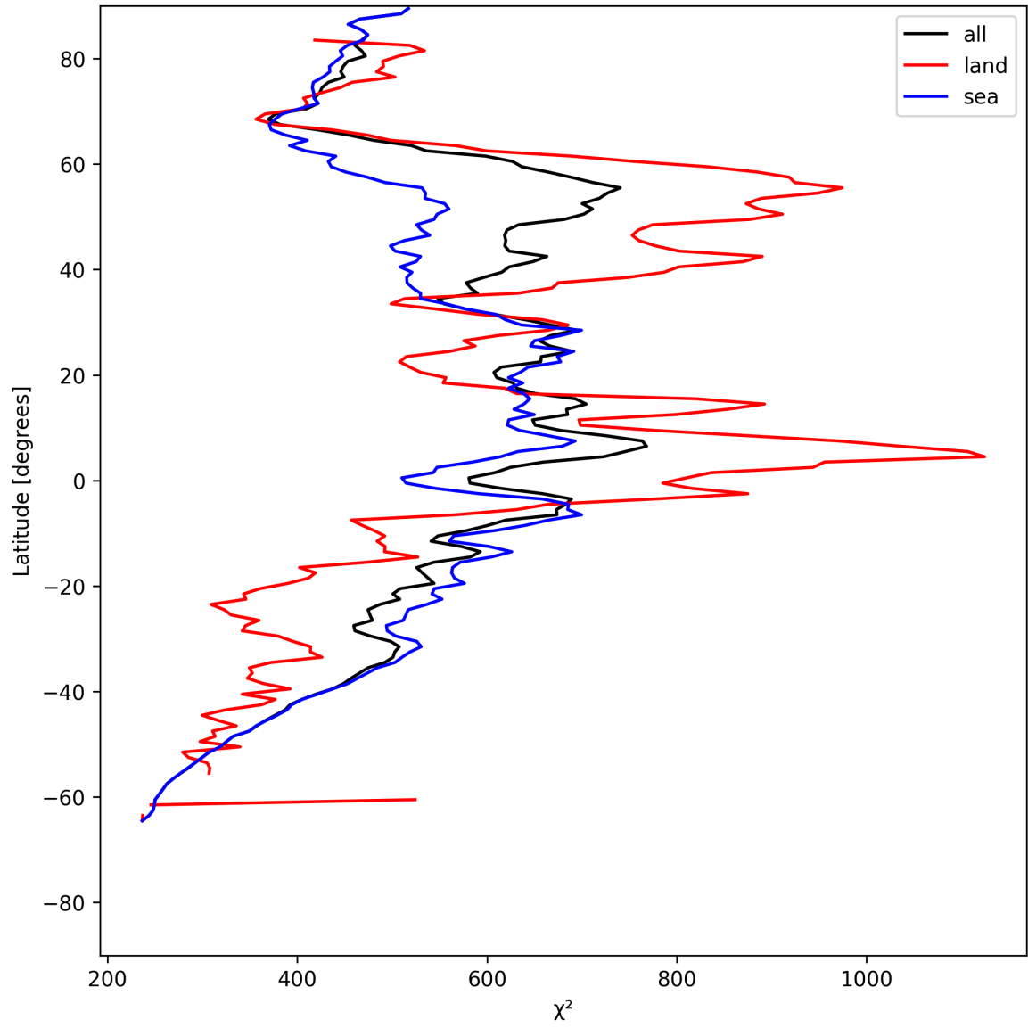
Figure 23: Zonal average of “ \chi^2 ” for 2025-07-04 to 2025-07-05.
