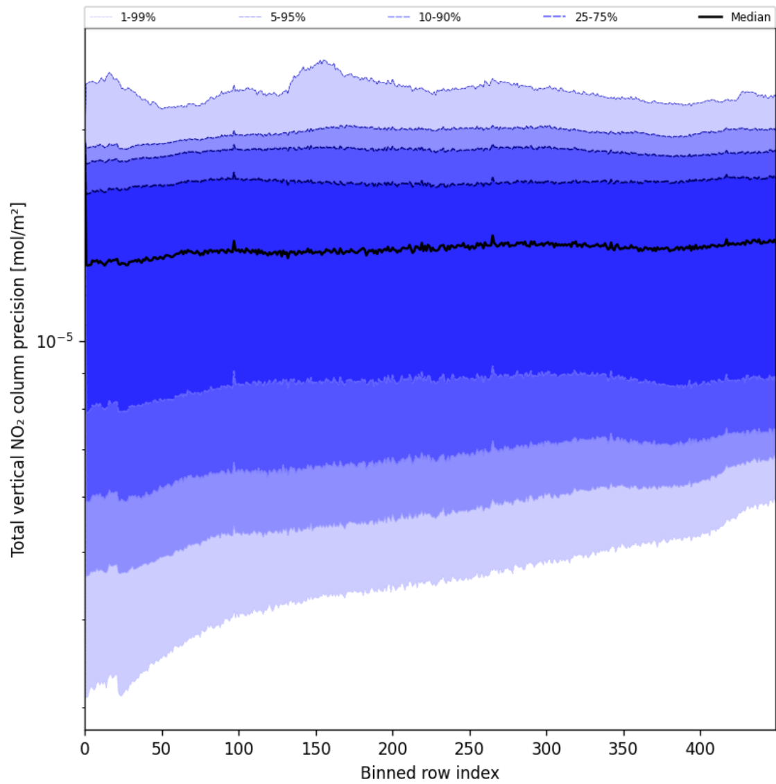
Figure 54: Along track statistics of “Total vertical NO 2 column precision” for 2025-07-04 to 2025-07-05
