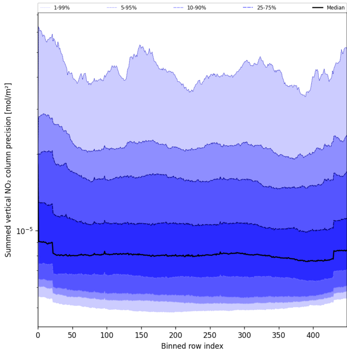
Figure 56: Along track statistics of “Summed vertical NO 2 column precision” for 2025-07-04 to 2025-07-05
