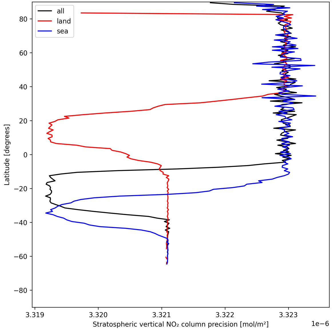
Figure 18: Zonal average of “Stratospheric vertical NO 2 column precision” for 2025-07-04 to 2025-07-05.
