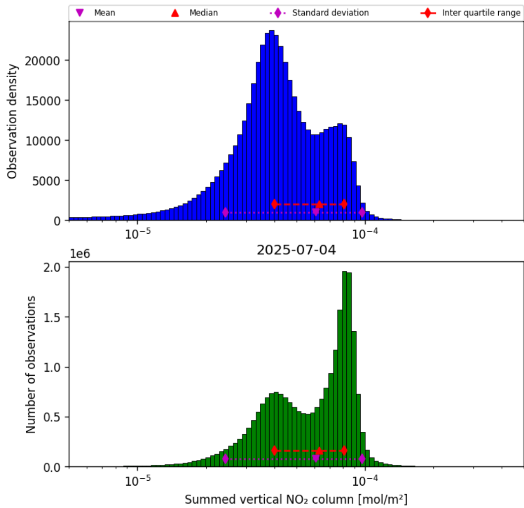
Figure 38: Histogram of “Summed vertical NO 2 column” for 2025-07-04 to 2025-07-05
