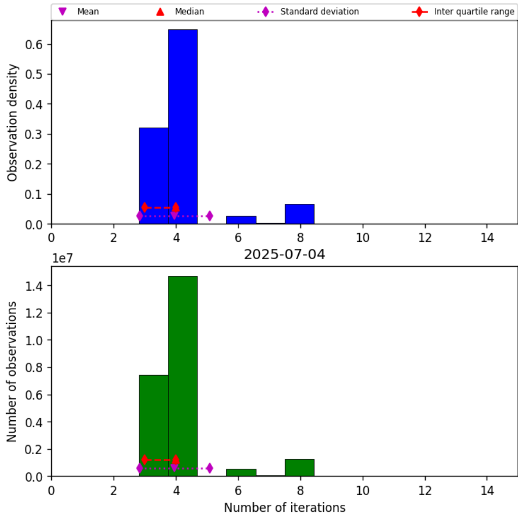
Figure 32: Histogram of “Number of iterations” for 2025-07-04 to 2025-07-05
