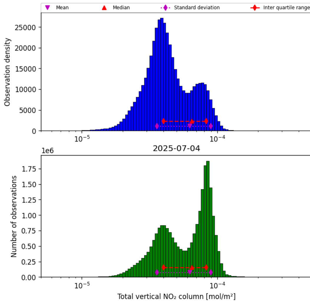
Figure 36: Histogram of “Total vertical NO 2 column” for 2025-07-04 to 2025-07-05
