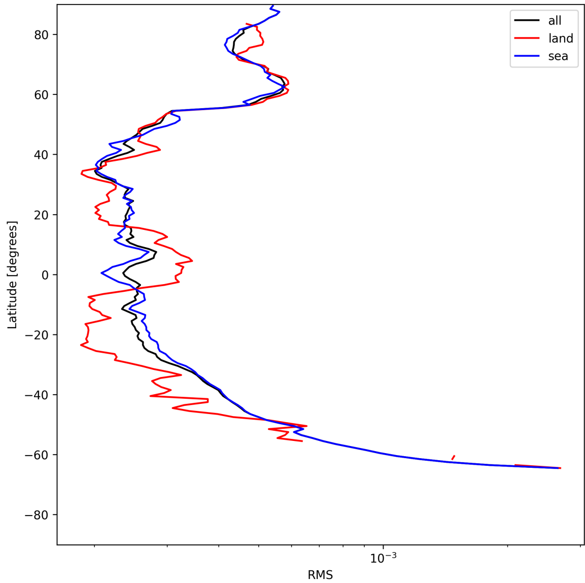
Figure 24: Zonal average of “RMS” for 2025-07-04 to 2025-07-05.
