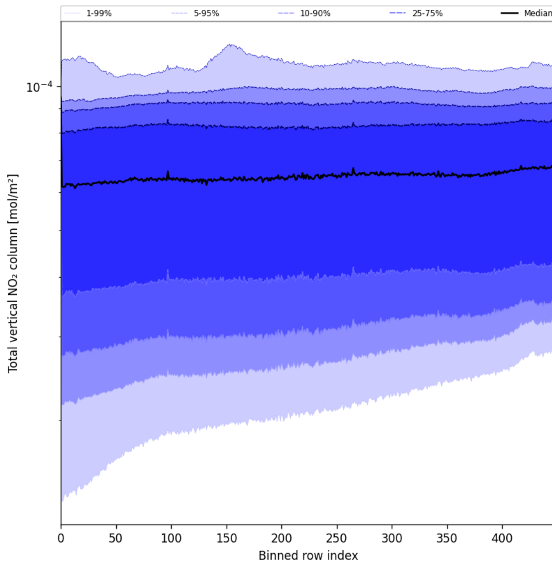
Figure 53: Along track statistics of “Total vertical NO 2 column” for 2025-07-04 to 2025-07-05
