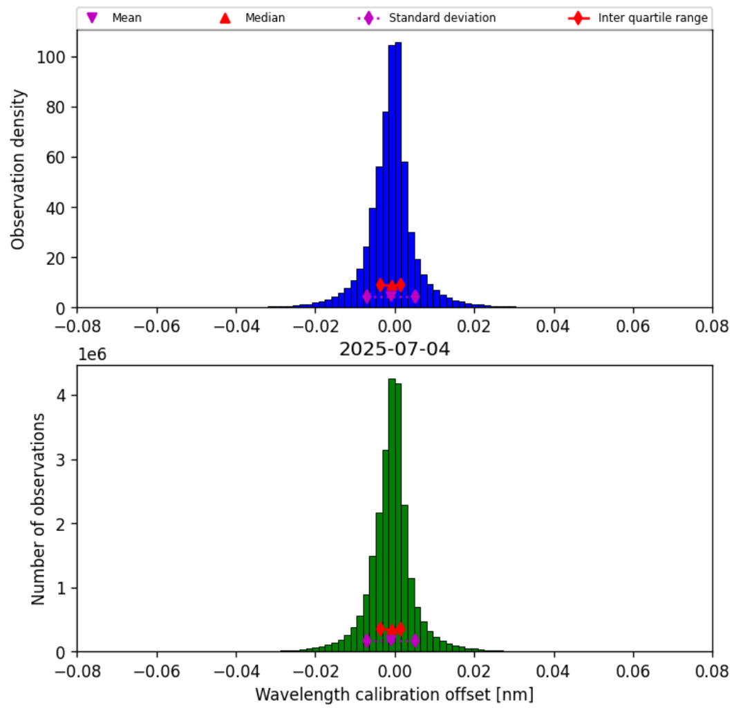
Figure 33: Histogram of “Wavelength calibration offset” for 2025-07-04 to 2025-07-05
