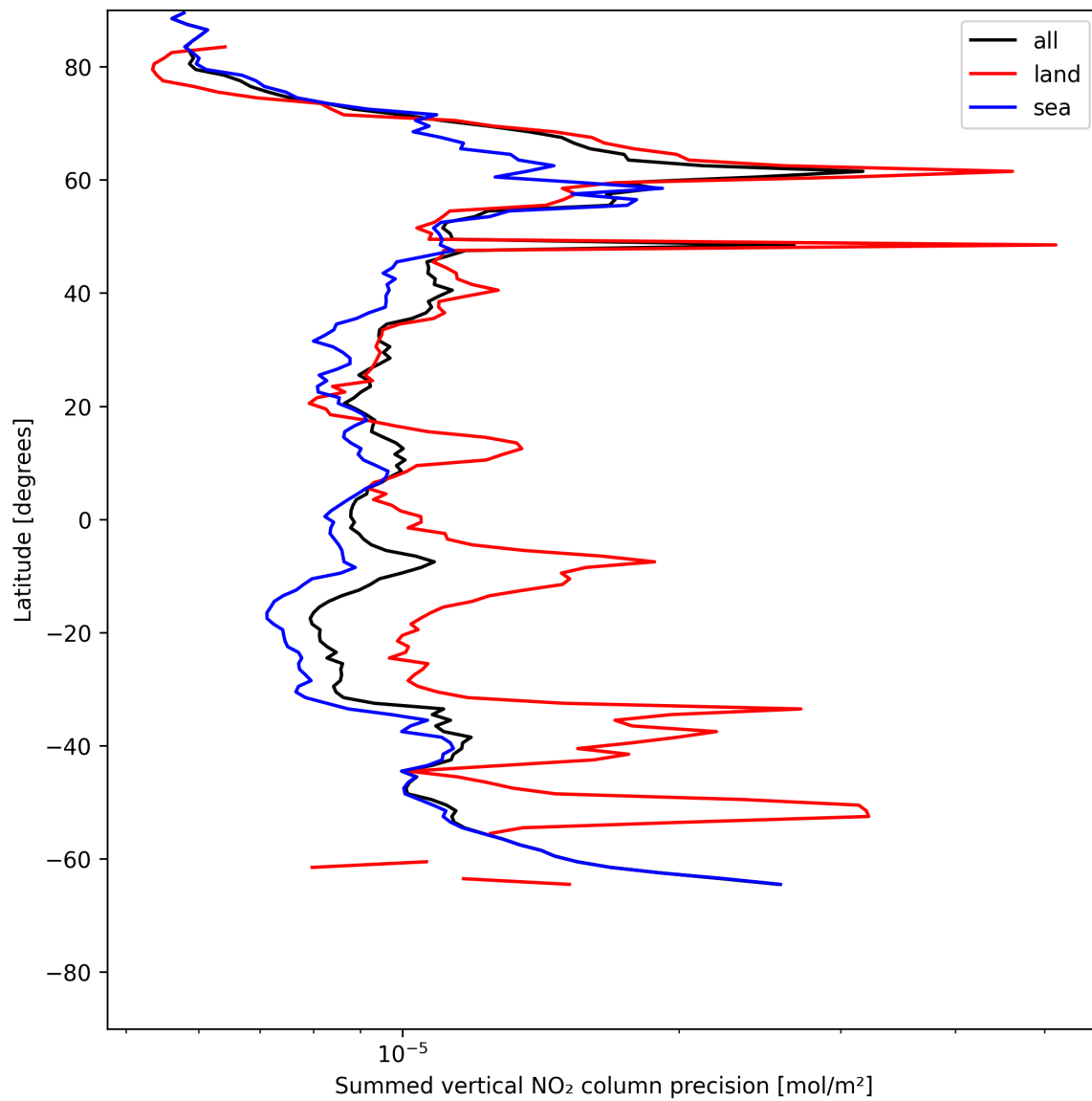
Figure 22: Zonal average of “Summed vertical NO 2 column precision” for 2025-07-04 to 2025-07-05.
