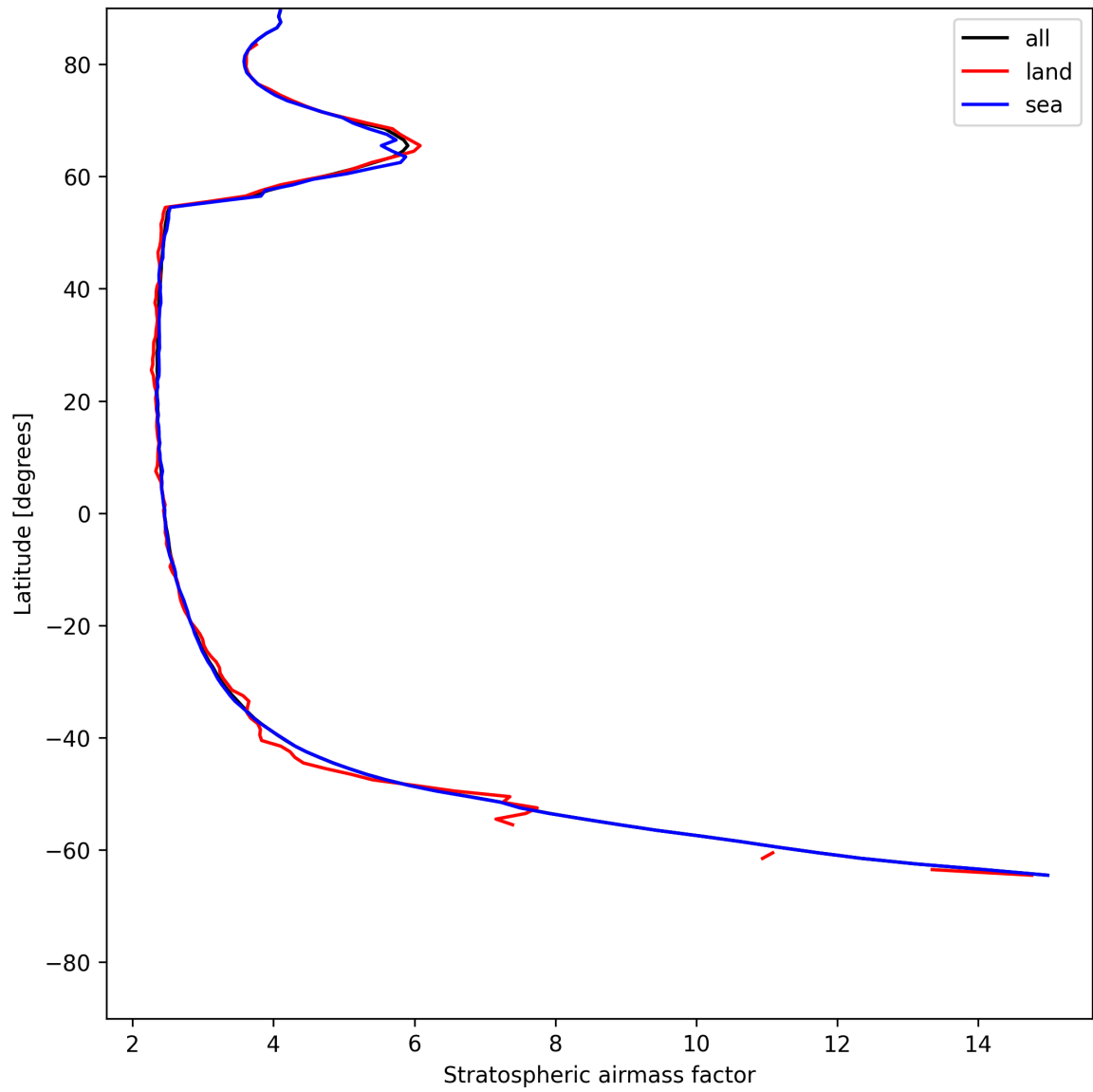
Figure 25: Zonal average of “Stratospheric airmass factor” for 2025-07-04 to 2025-07-05.
