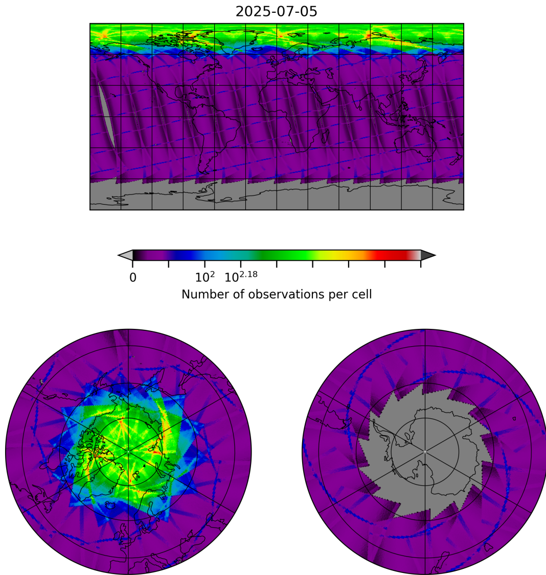
Figure 8: Map of the number of observations for 2025-07-05 to 2025-07-06
