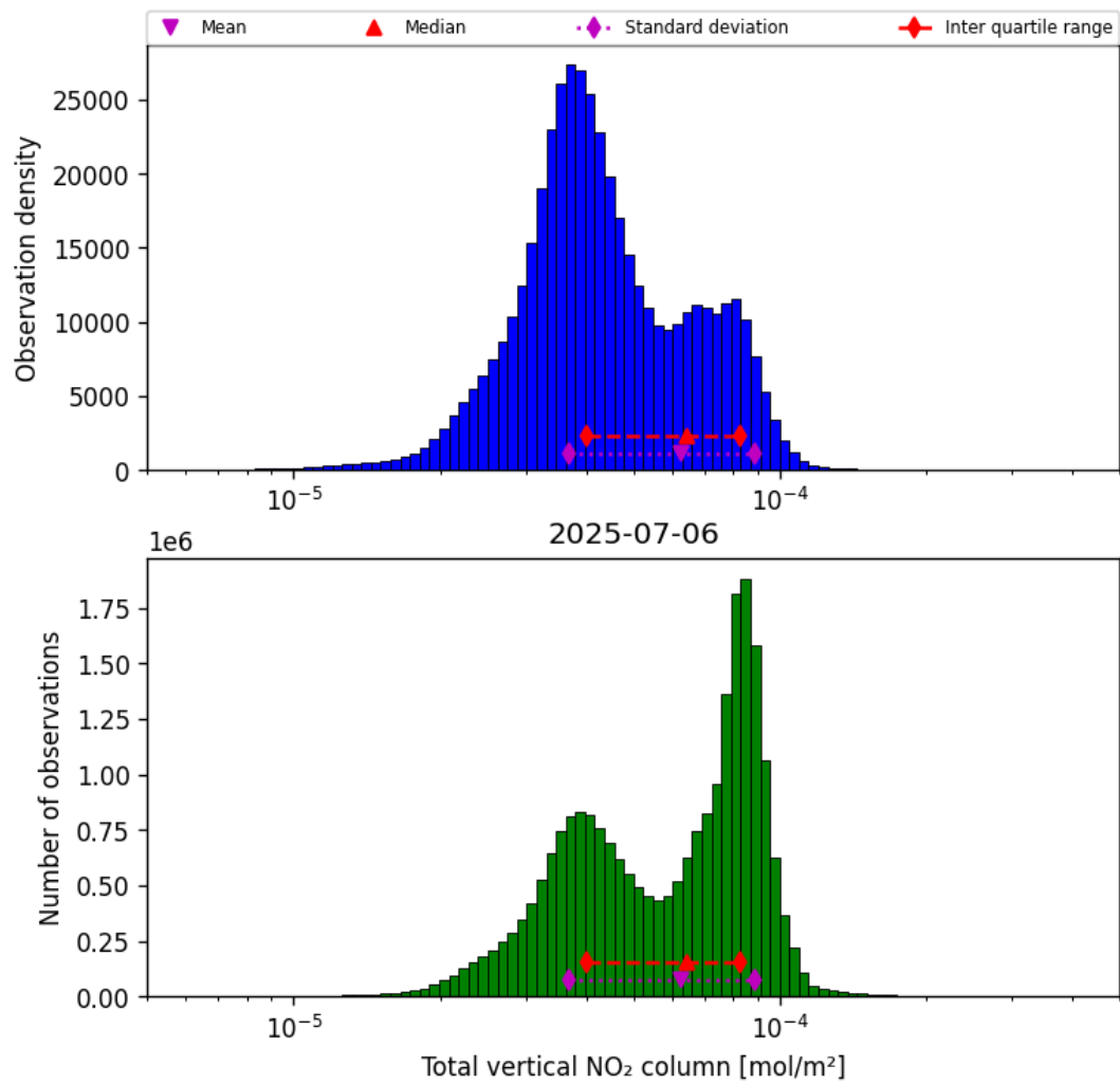
Figure 36: Histogram of “Total vertical NO 2 column” for 2025-07-06 to 2025-07-06
