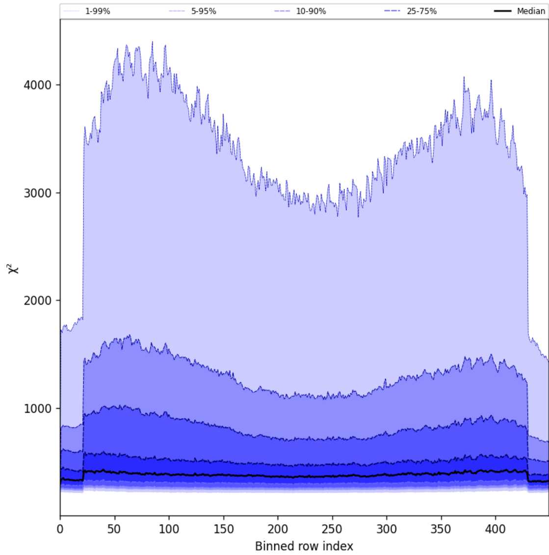
Figure 57: Along track statistics of “ \chi^2 ” for 2025-07-06 to 2025-07-06
