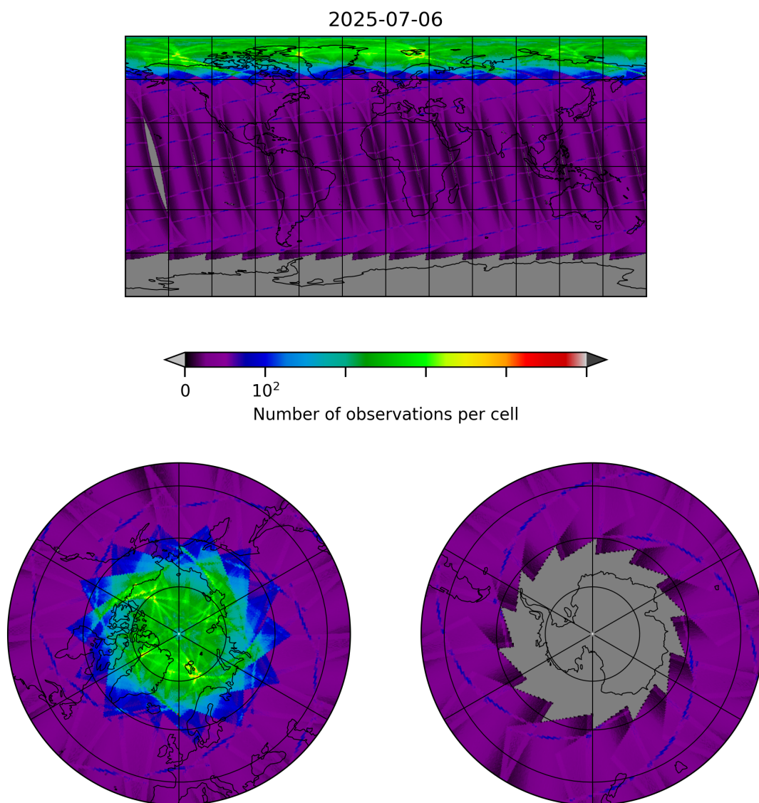
Figure 8: Map of the number of observations for 2025-07-06 to 2025-07-06
