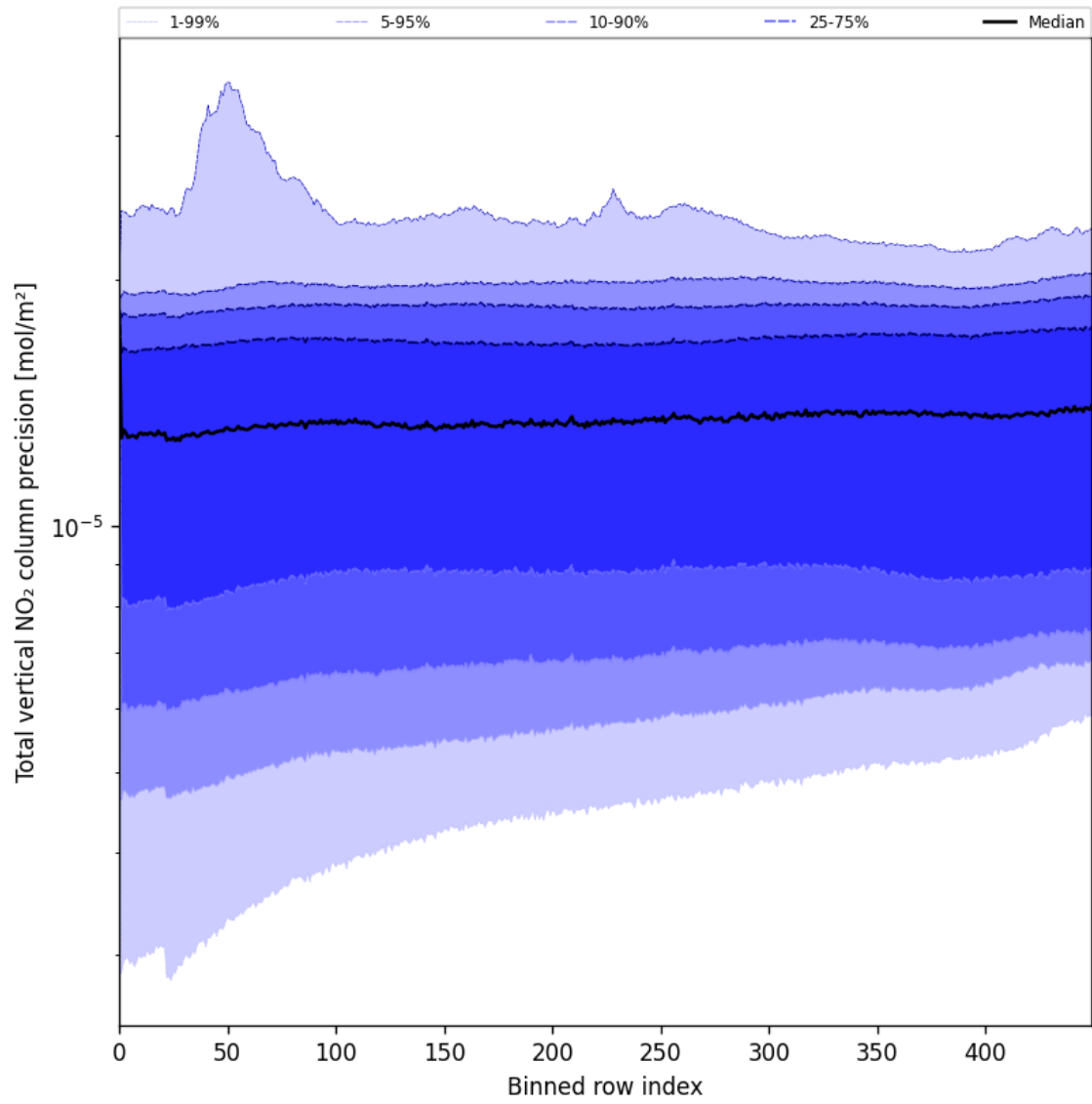
Figure 54: Along track statistics of “Total vertical NO 2 column precision” for 2025-07-06 to 2025-07-06
