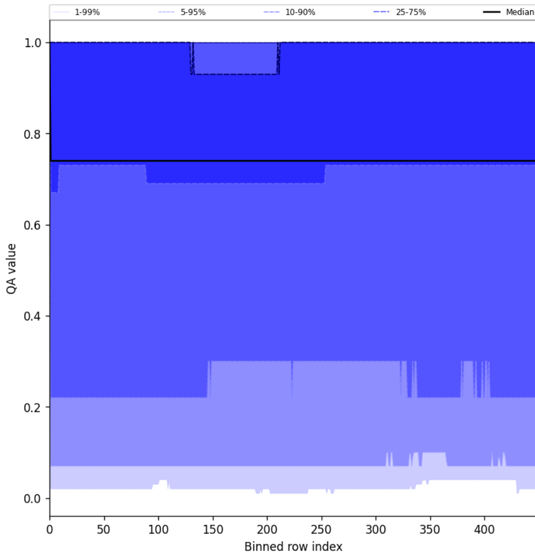
Figure 43: Along track statistics of “QA value” for 2025-07-06 to 2025-07-06
