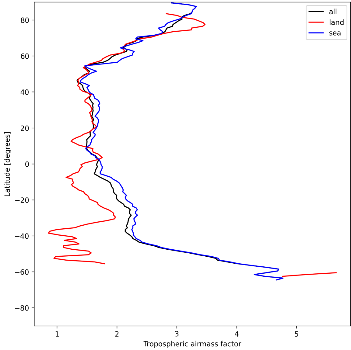
Figure 12: Zonal average of “Tropospheric airmass factor” for 2025-07-06 to 2025-07-06.
