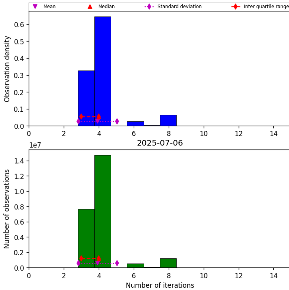
Figure 32: Histogram of “Number of iterations” for 2025-07-06 to 2025-07-06
