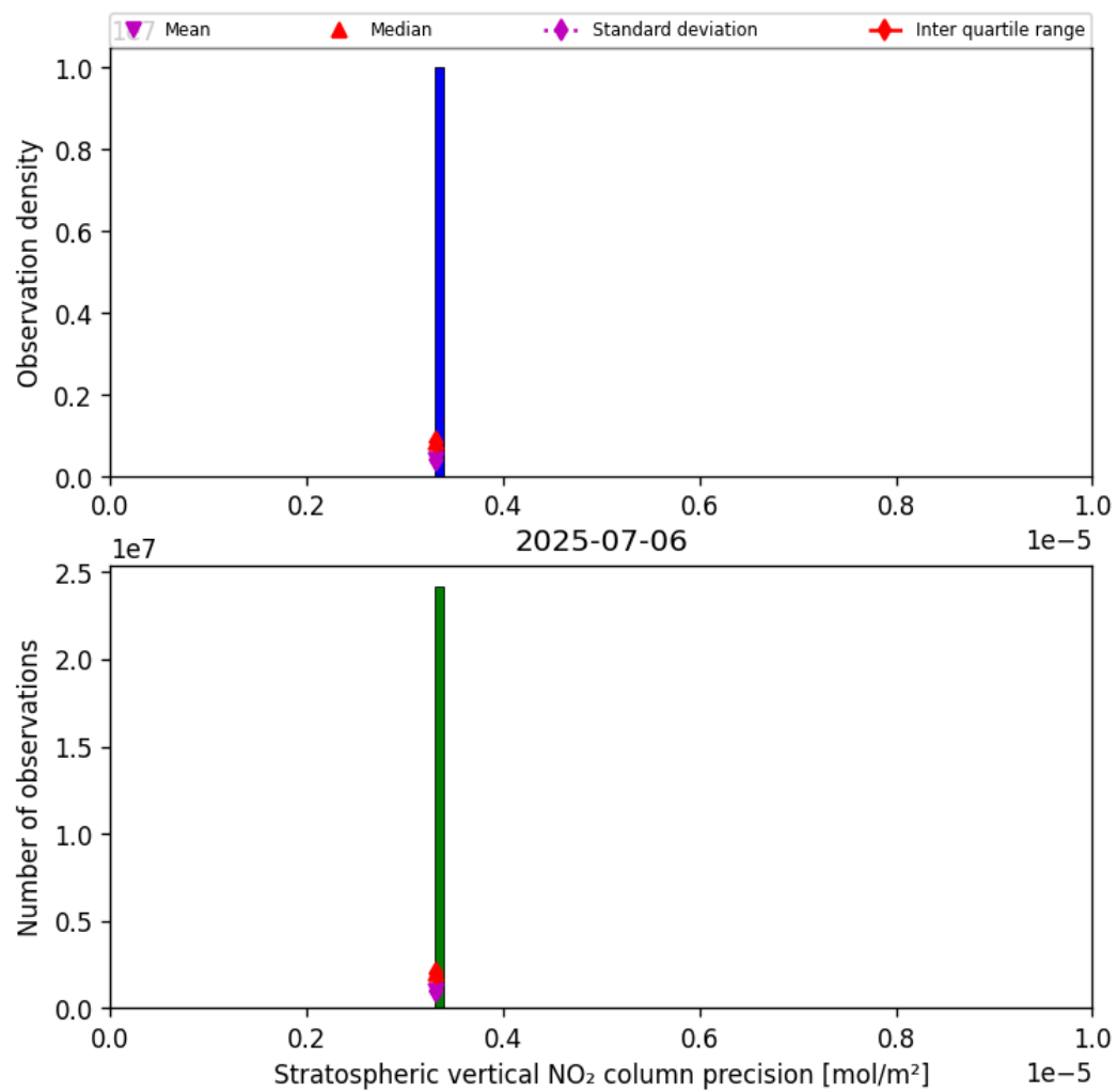
Figure 35: Histogram of “Stratospheric vertical NO 2 column precision” for 2025-07-06 to 2025-07-06
