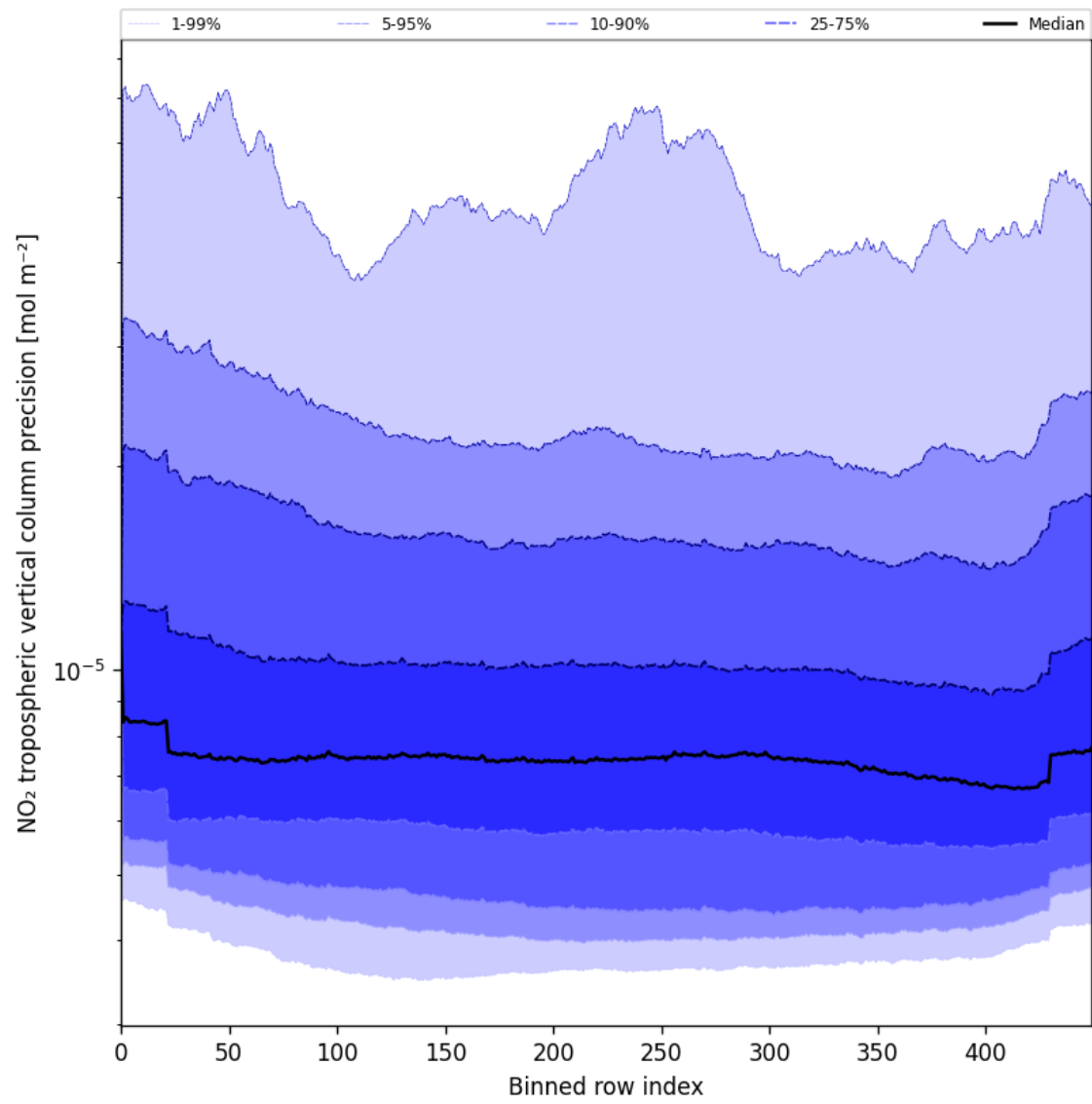
Figure 45: Along track statistics of “NO 2 tropospheric vertical column precision” for 2025-07-06 to 2025-07-06
