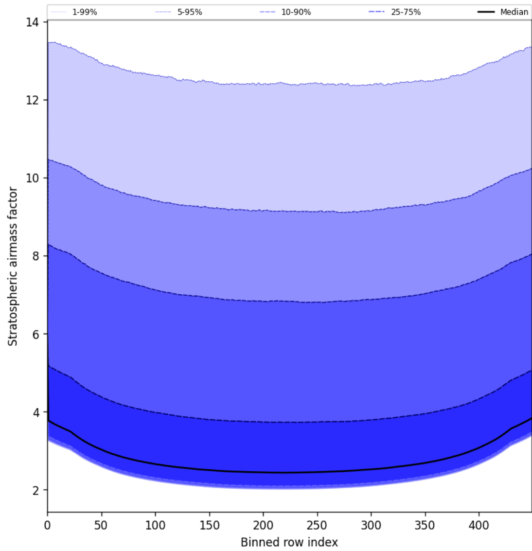
Figure 59: Along track statistics of “Stratospheric airmass factor” for 2025-07-06 to 2025-07-06
