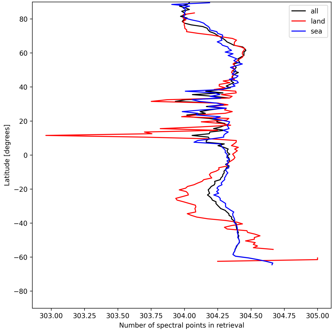
Figure 14: Zonal average of “Number of spectral points in retrieval” for 2025-07-06 to 2025-07-06.
