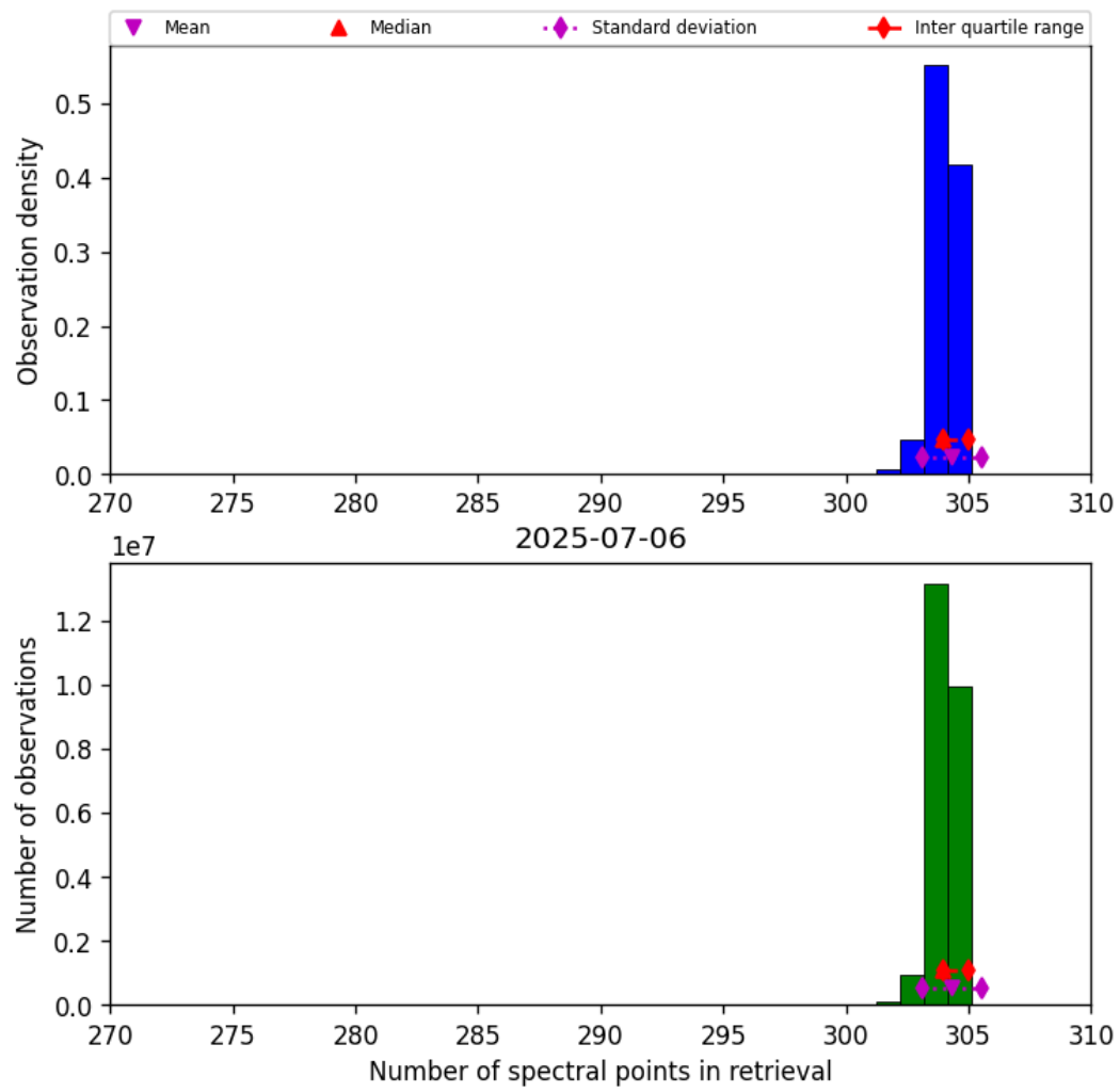
Figure 31: Histogram of “Number of spectral points in retrieval” for 2025-07-06 to 2025-07-06
