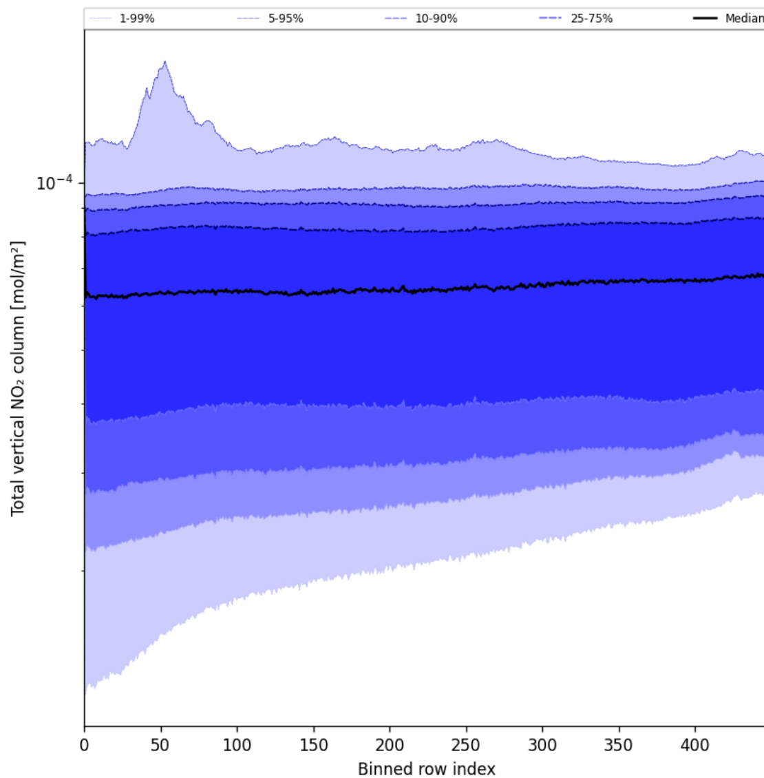
Figure 53: Along track statistics of “Total vertical NO 2 column” for 2025-07-06 to 2025-07-06
