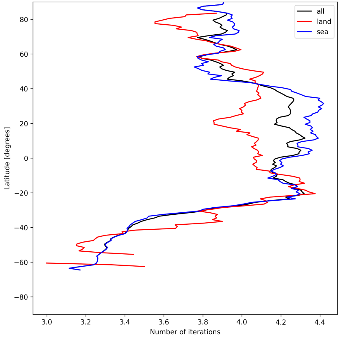
Figure 15: Zonal average of “Number of iterations” for 2025-07-06 to 2025-07-06.
