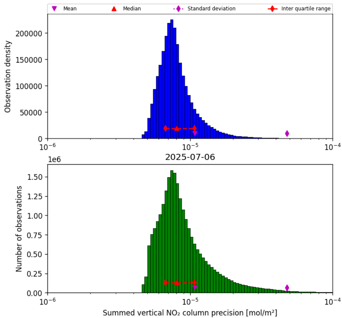
Figure 39: Histogram of "Summed vertical NO 2 column precision" for 2025-07-06 to 2025-07-06
