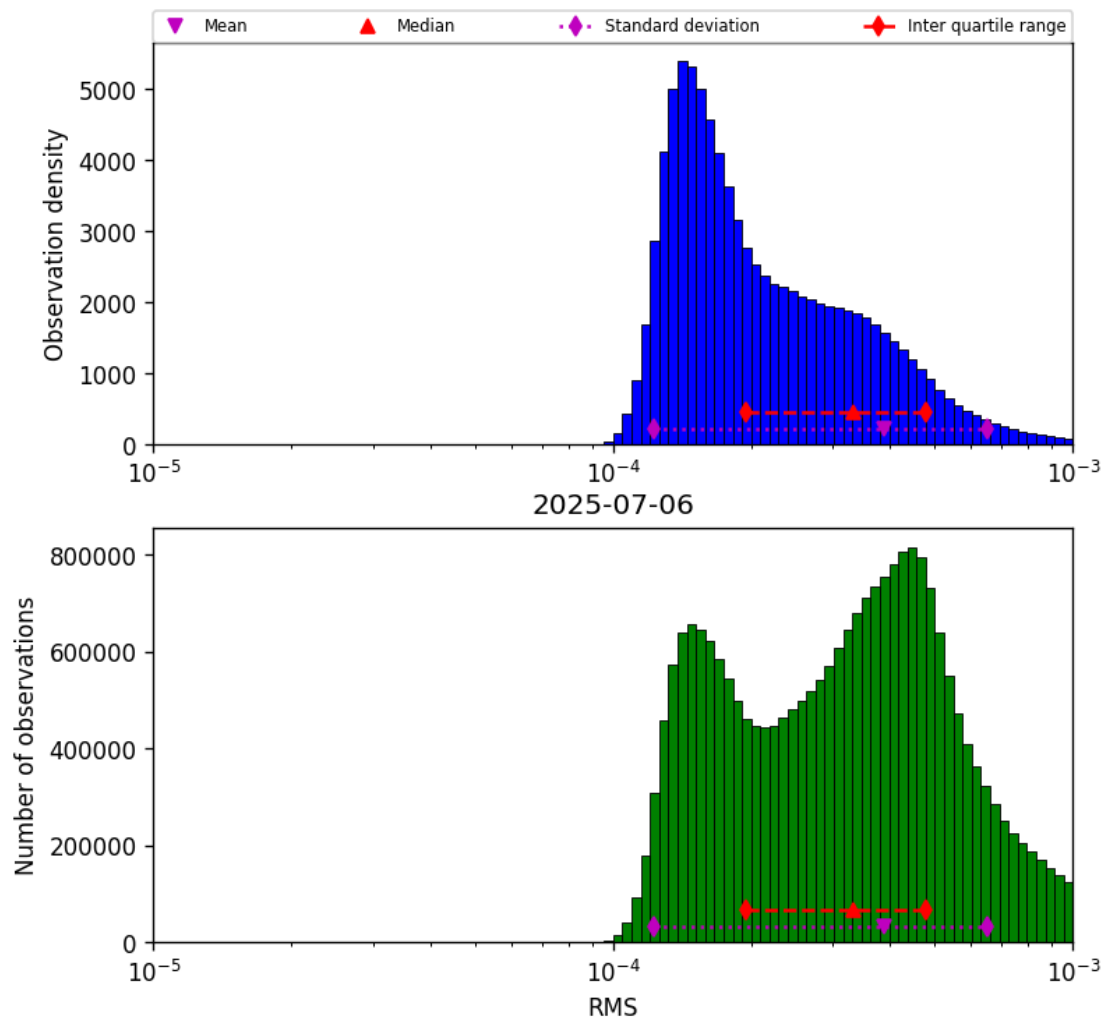
Figure 41: Histogram of “RMS” for 2025-07-06 to 2025-07-06
