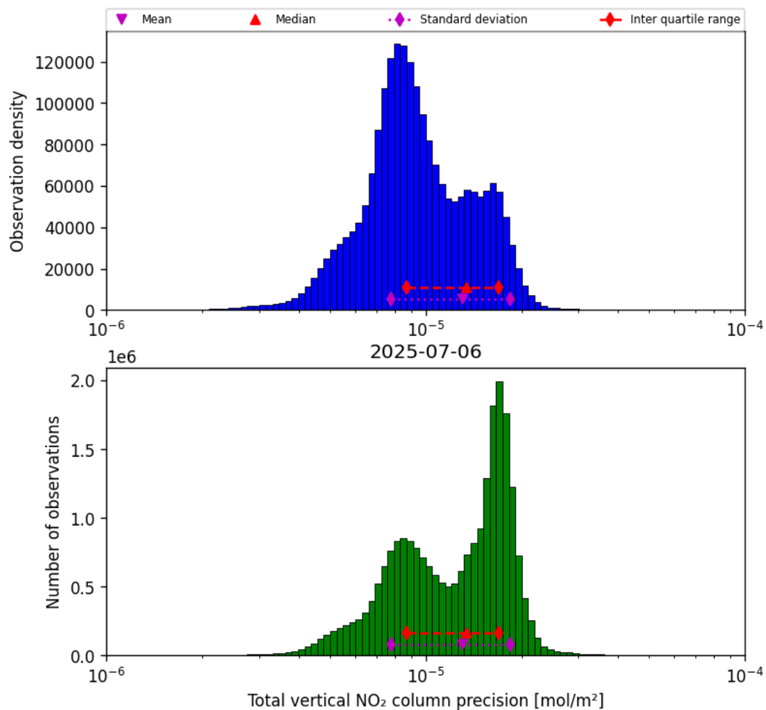
Figure 37: Histogram of "Total vertical NO 2 column precision" for 2025-07-06 to 2025-07-06
