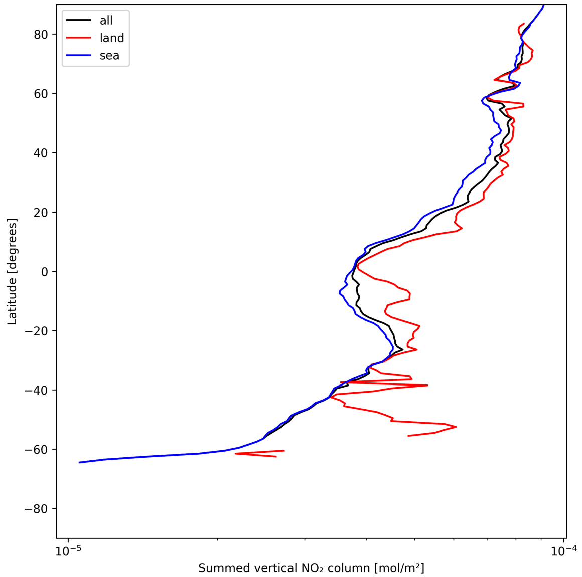
Figure 21: Zonal average of “Summed vertical NO 2 column” for 2025-07-06 to 2025-07-06.
