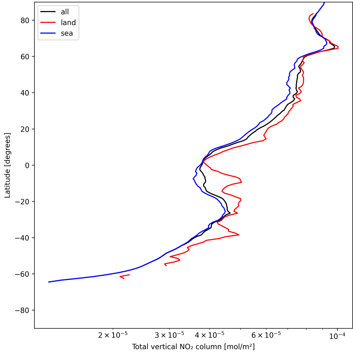
Figure 19: Zonal average of “Total vertical NO 2 column” for 2025-07-06 to 2025-07-06.
