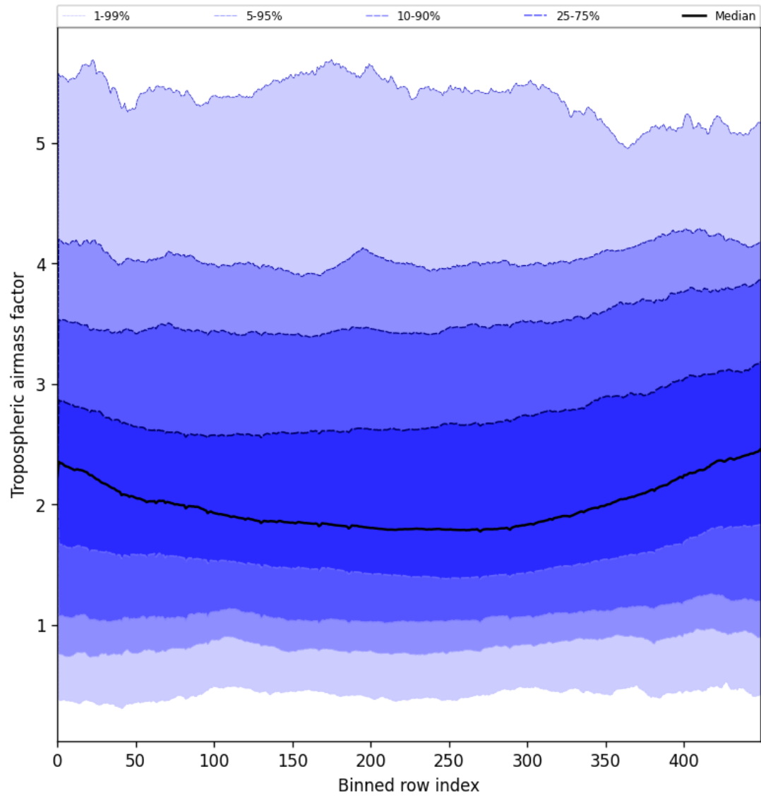
Figure 46: Along track statistics of “Tropospheric airmass factor” for 2025-07-06 to 2025-07-06
