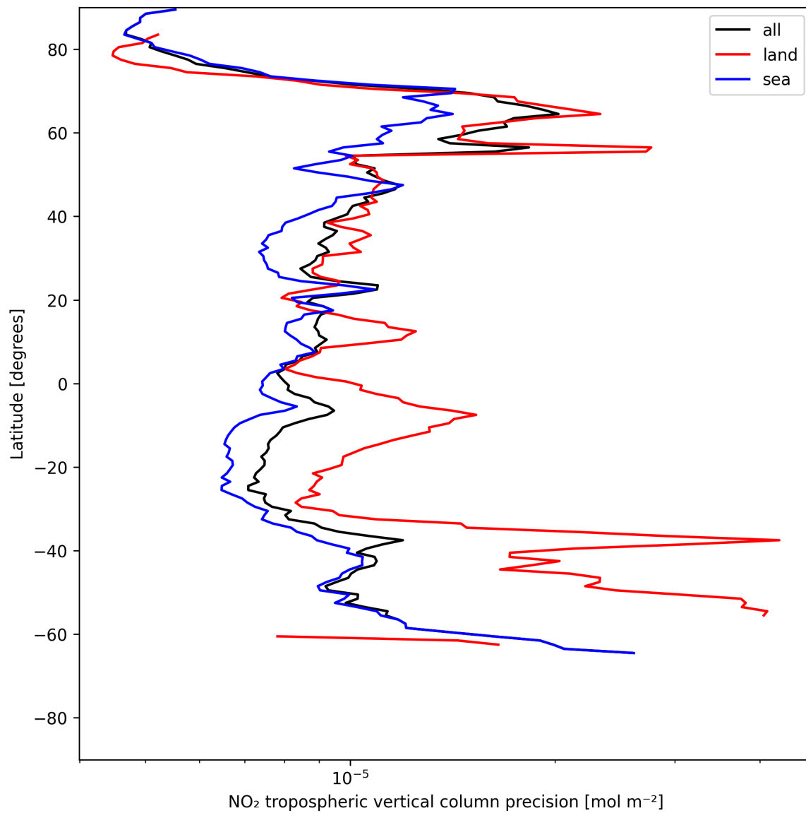
Figure 11: Zonal average of “NO 2 tropospheric vertical column precision” for 2025-07-06 to 2025-07-06.
