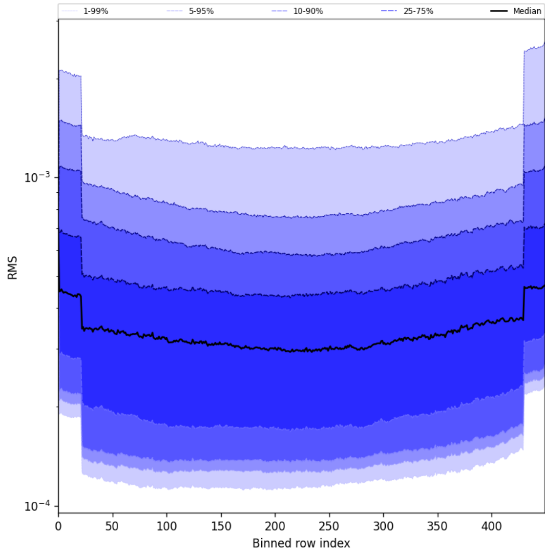
Figure 58: Along track statistics of “RMS” for 2025-07-06 to 2025-07-06
