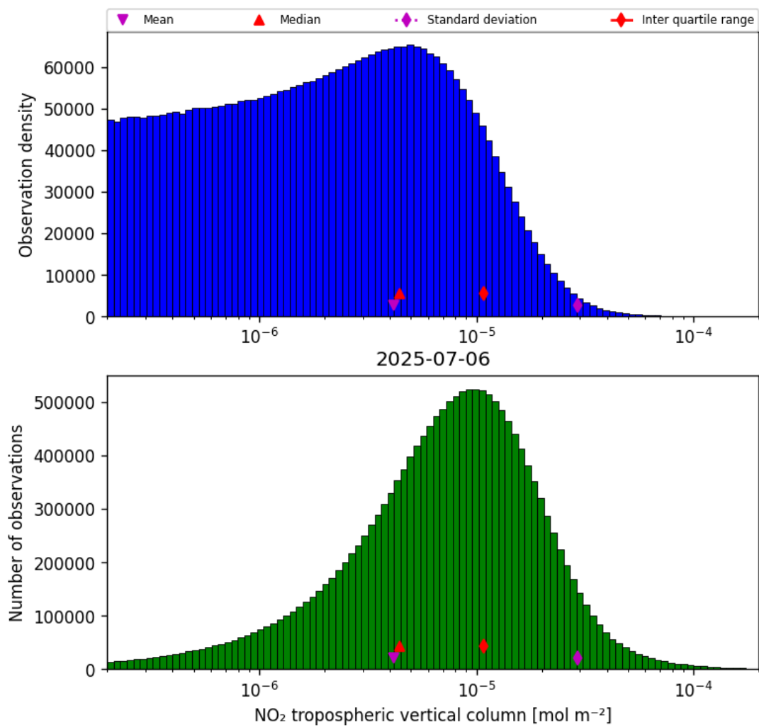
Figure 27: Histogram of “NO 2 tropospheric vertical column” for 2025-07-06 to 2025-07-06
