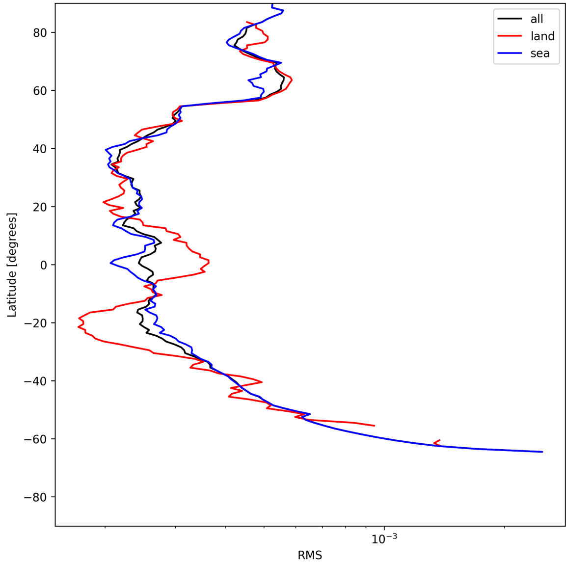
Figure 24: Zonal average of “RMS” for 2025-07-06 to 2025-07-06.
