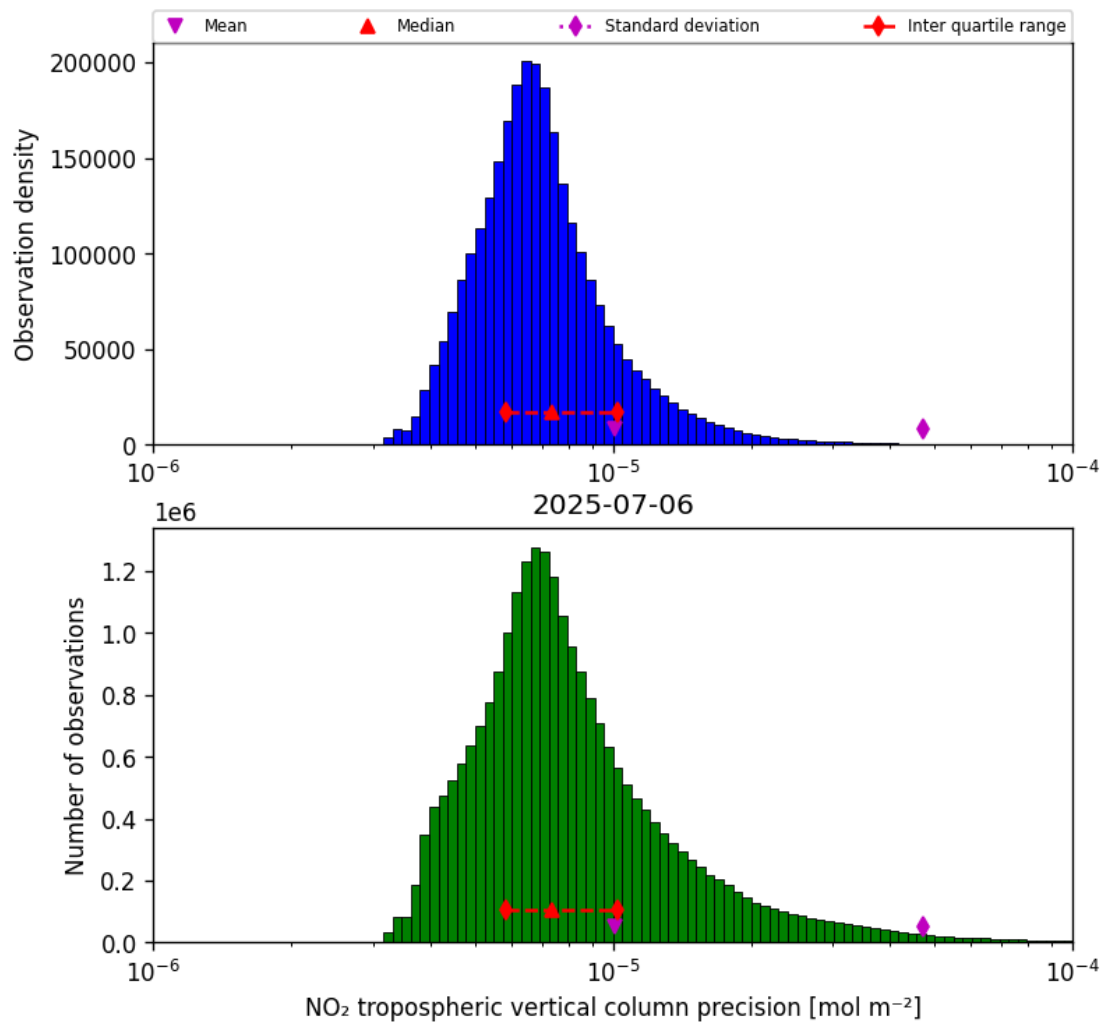
Figure 28: Histogram of "NO 2 tropospheric vertical column precision" for 2025-07-06 to 2025-07-06
