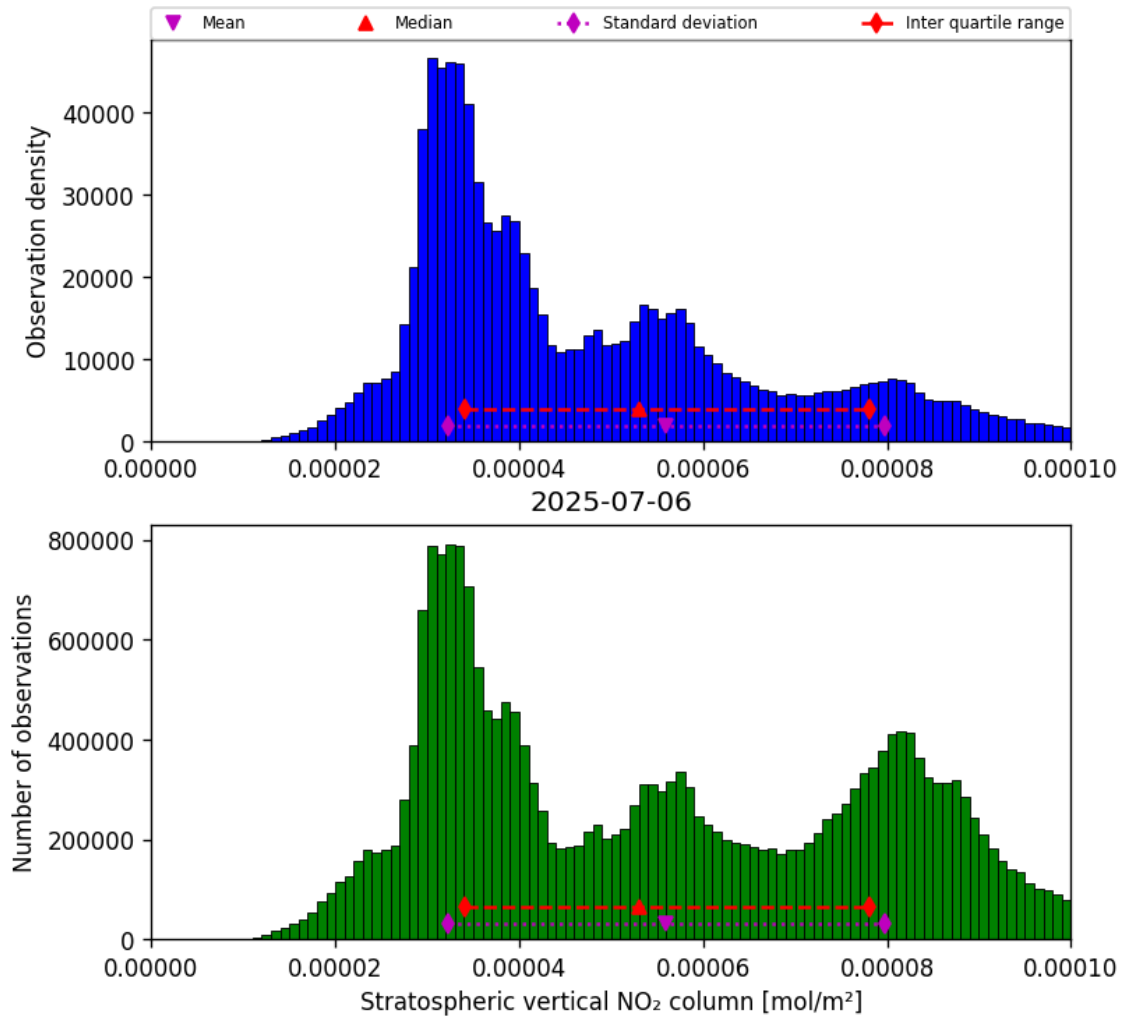
Figure 34: Histogram of “Stratospheric vertical NO 2 column” for 2025-07-06 to 2025-07-06
