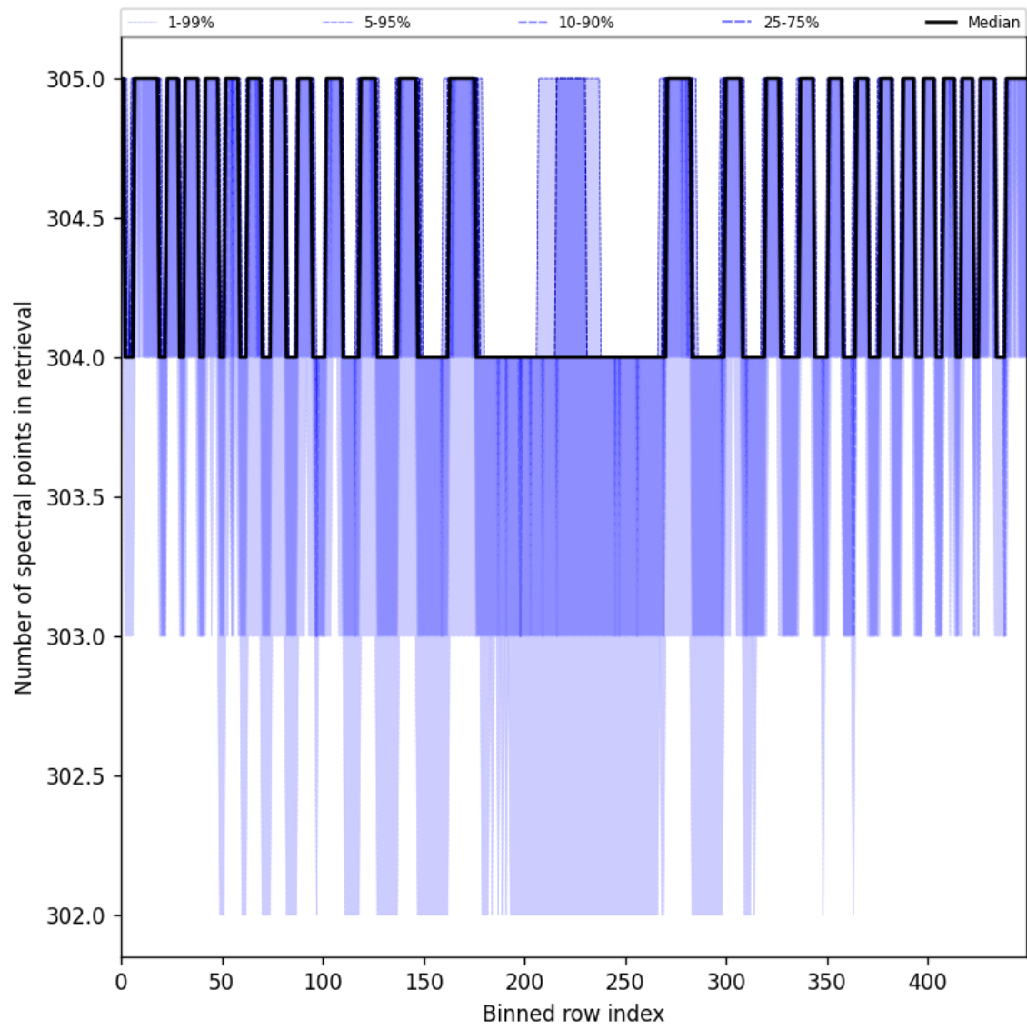
Figure 48: Along track statistics of “Number of spectral points in retrieval” for 2025-07-06 to 2025-07-06
