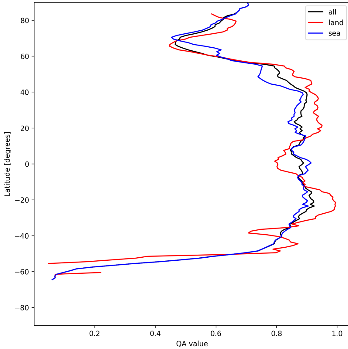
Figure 9: Zonal average of “QA value” for 2025-07-06 to 2025-07-06.
