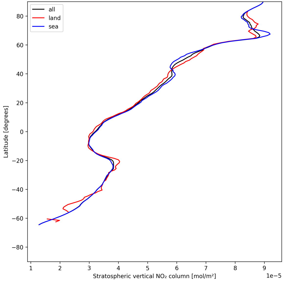
Figure 17: Zonal average of “Stratospheric vertical NO 2 column” for 2025-07-06 to 2025-07-06.
