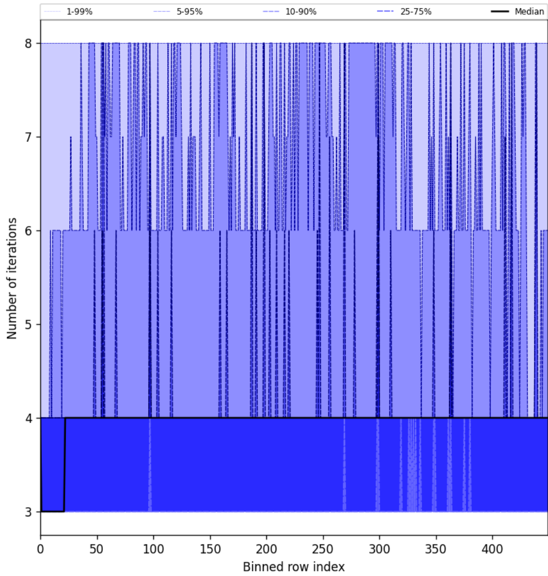
Figure 49: Along track statistics of “Number of iterations” for 2025-07-06 to 2025-07-06
