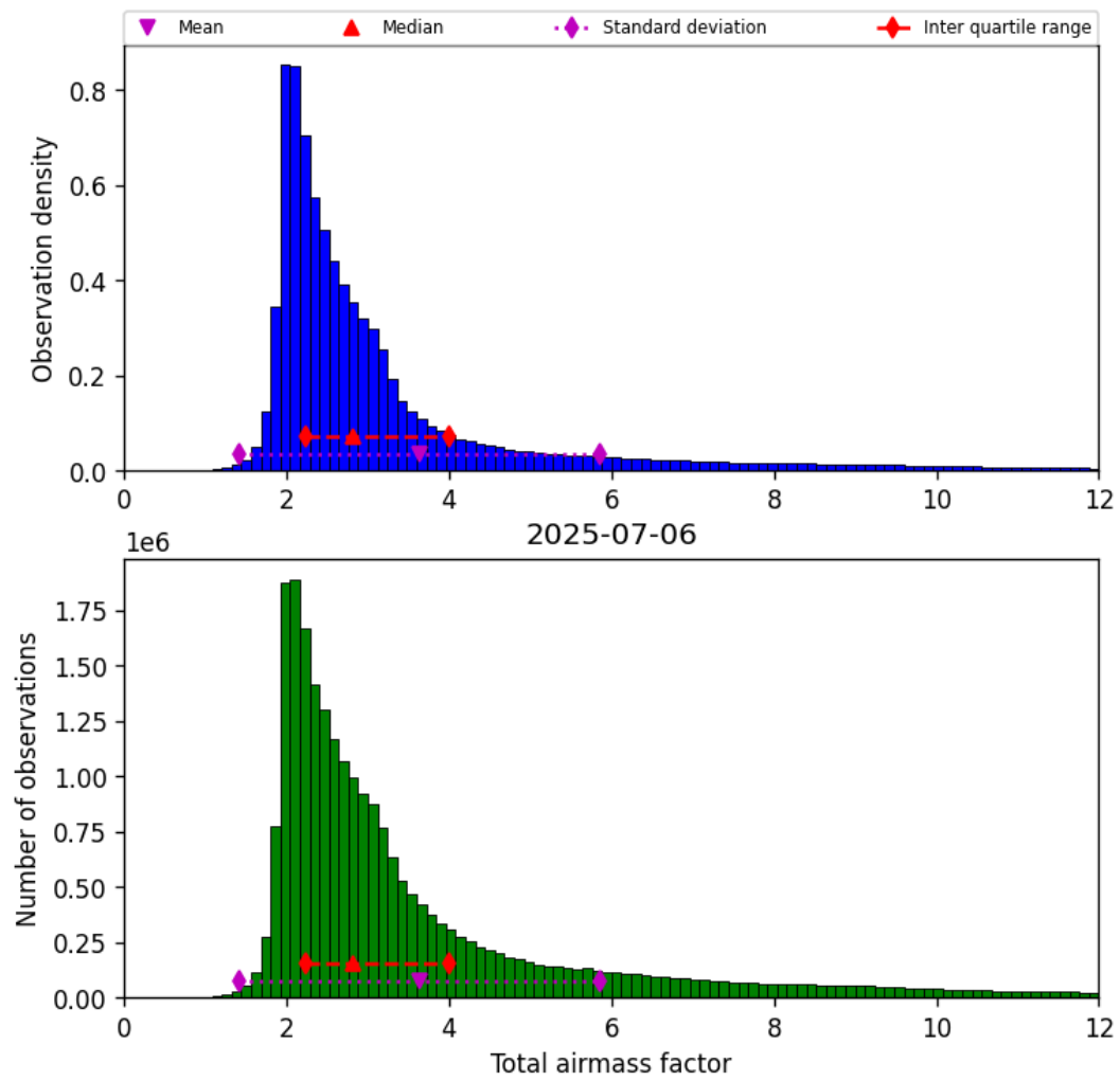
Figure 30: Histogram of “Total airmass factor” for 2025-07-06 to 2025-07-06
