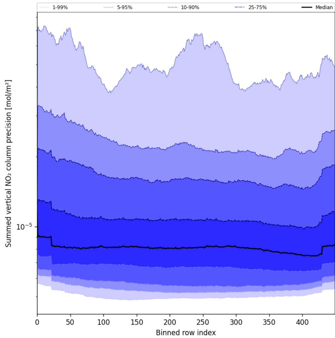
Figure 56: Along track statistics of “Summed vertical NO 2 column precision” for 2025-07-06 to 2025-07-06
