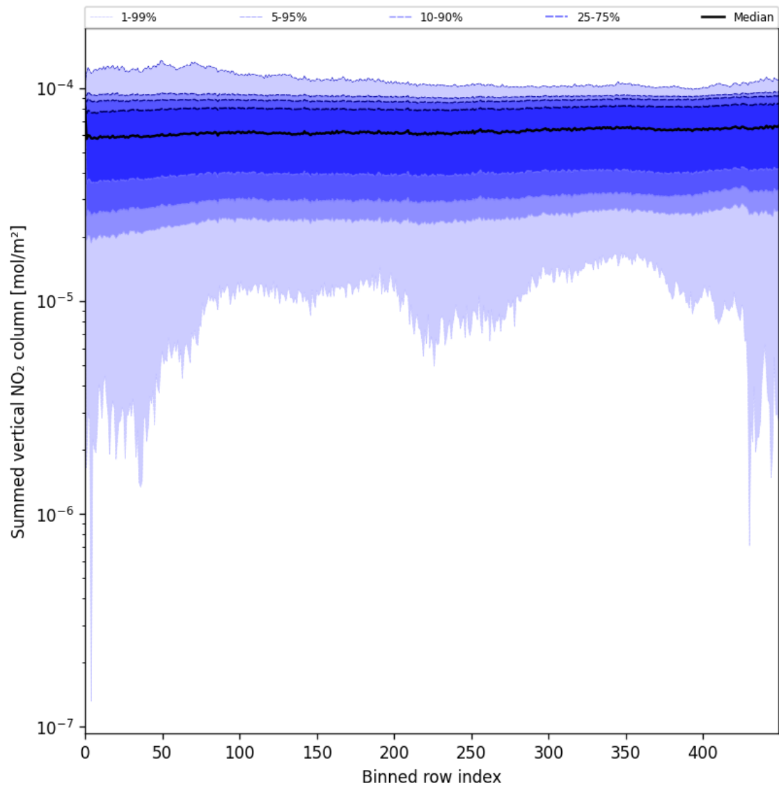
Figure 55: Along track statistics of “Summed vertical NO 2 column” for 2025-07-06 to 2025-07-06
