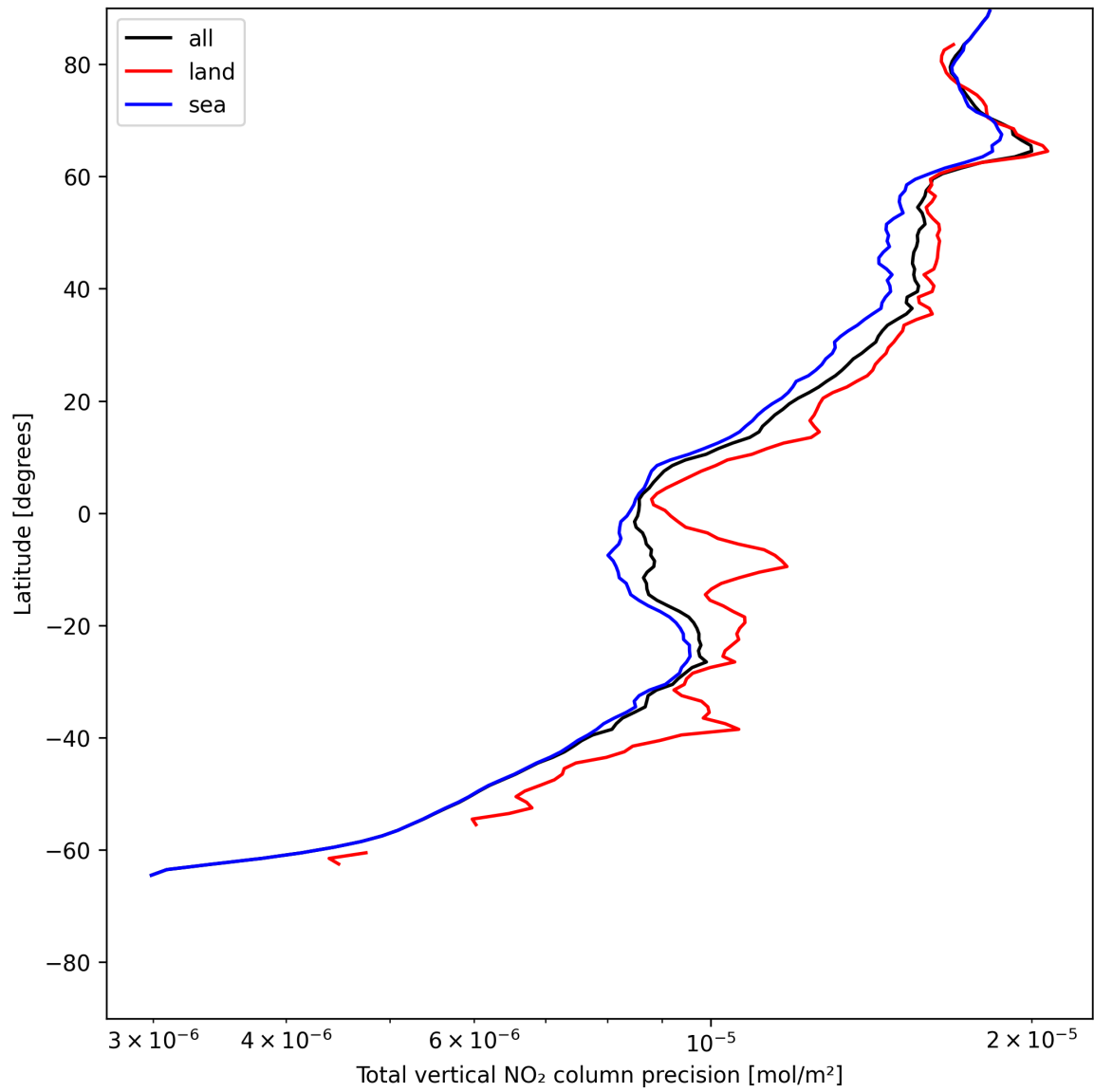
Figure 20: Zonal average of “Total vertical NO 2 column precision” for 2025-07-06 to 2025-07-06.
