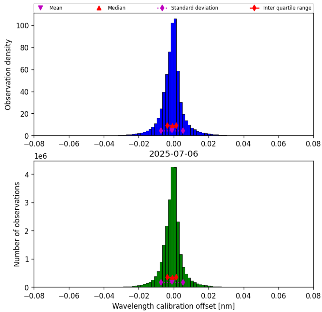
Figure 33: Histogram of “Wavelength calibration offset” for 2025-07-06 to 2025-07-06
