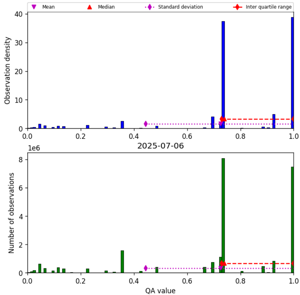
Figure 26: Histogram of “QA value” for 2025-07-06 to 2025-07-06
