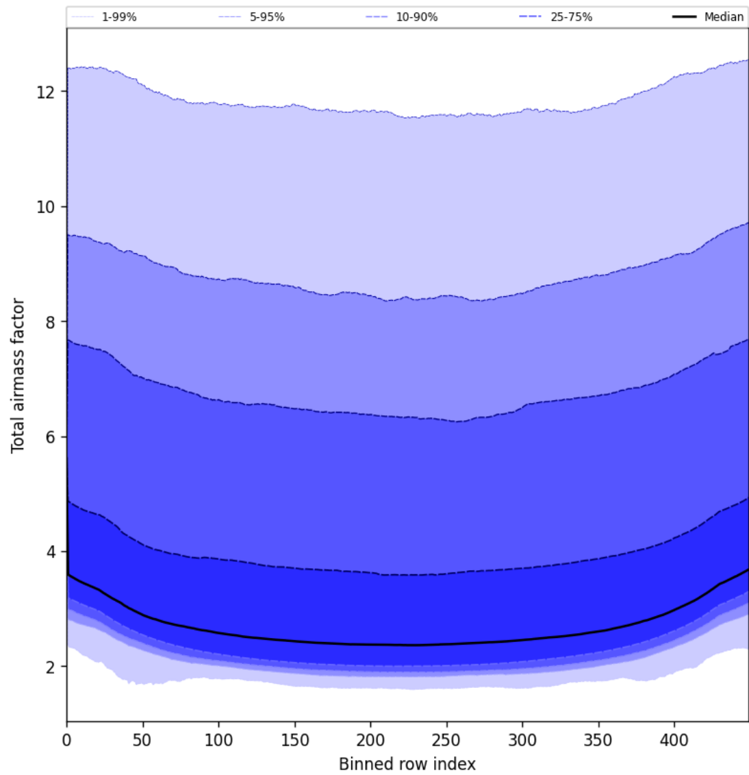
Figure 47: Along track statistics of “Total airmass factor” for 2025-07-06 to 2025-07-06
