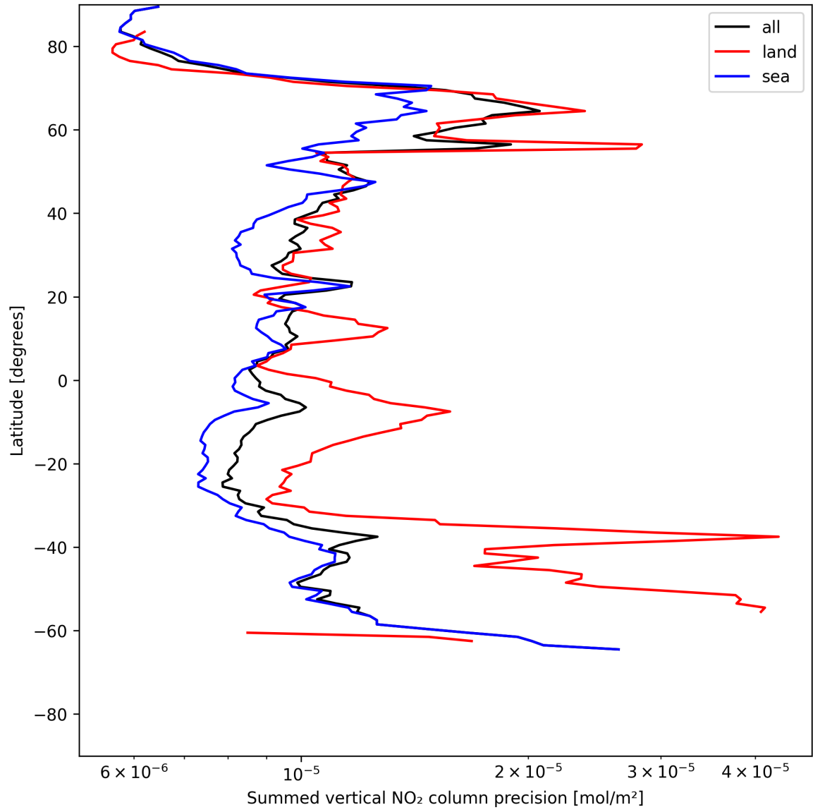
Figure 22: Zonal average of “Summed vertical NO 2 column precision” for 2025-07-06 to 2025-07-06.
