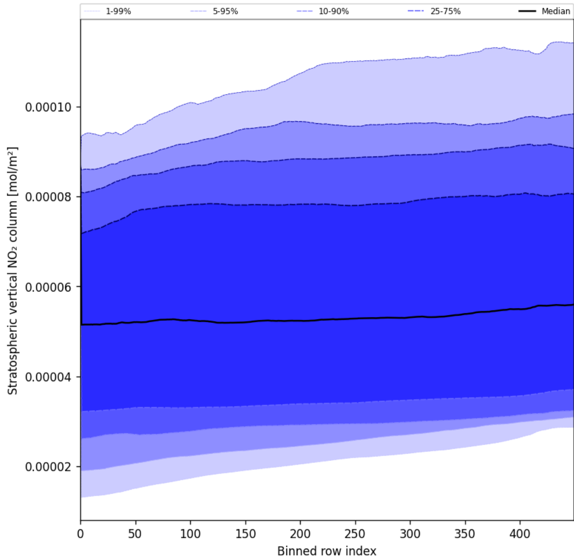
Figure 51: Along track statistics of “Stratospheric vertical NO 2 column” for 2025-07-06 to 2025-07-06
