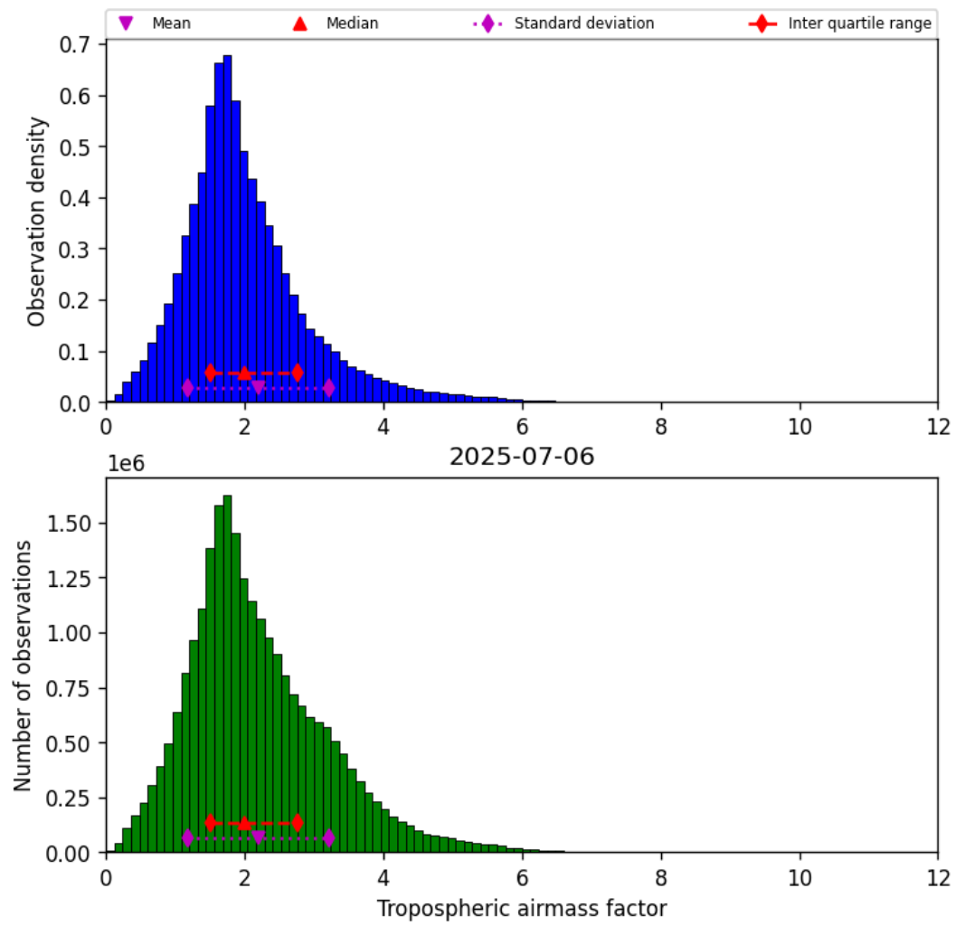
Figure 29: Histogram of “Tropospheric airmass factor” for 2025-07-06 to 2025-07-06
