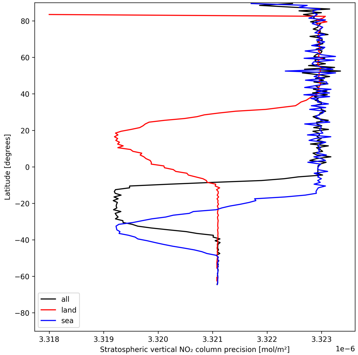
Figure 18: Zonal average of “Stratospheric vertical NO 2 column precision” for 2025-07-06 to 2025-07-06.
