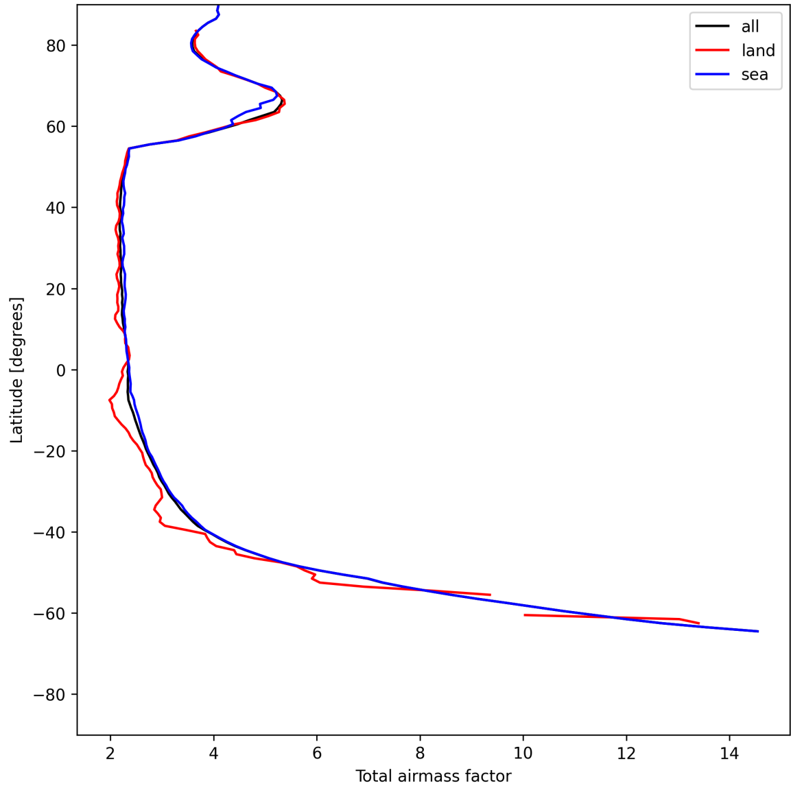
Figure 13: Zonal average of “Total airmass factor” for 2025-07-06 to 2025-07-06.
