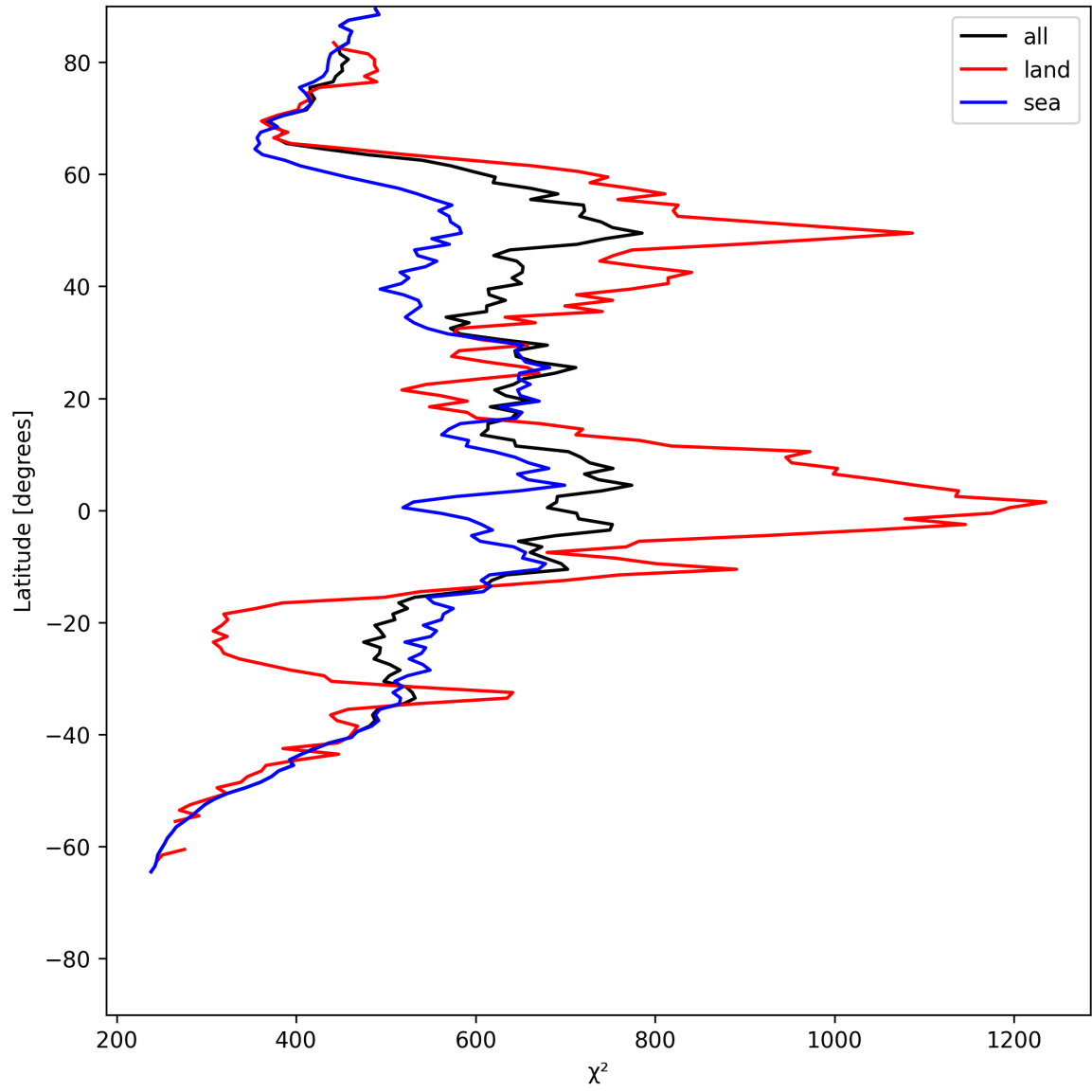
Figure 23: Zonal average of “ \chi^2 ” for 2025-07-06 to 2025-07-06.
