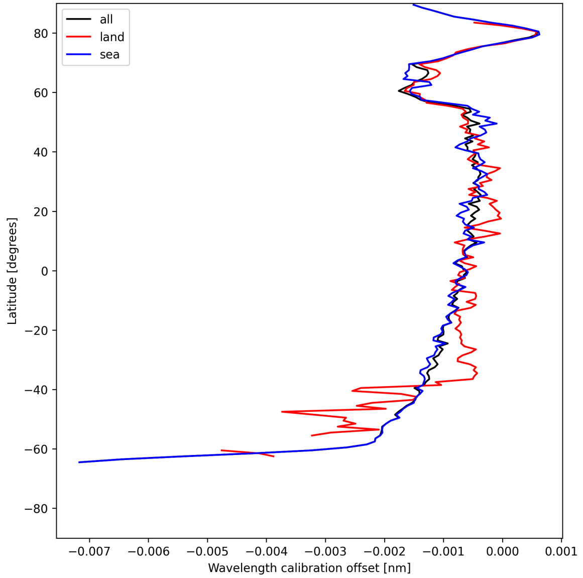
Figure 16: Zonal average of “Wavelength calibration offset” for 2025-07-06 to 2025-07-06.
