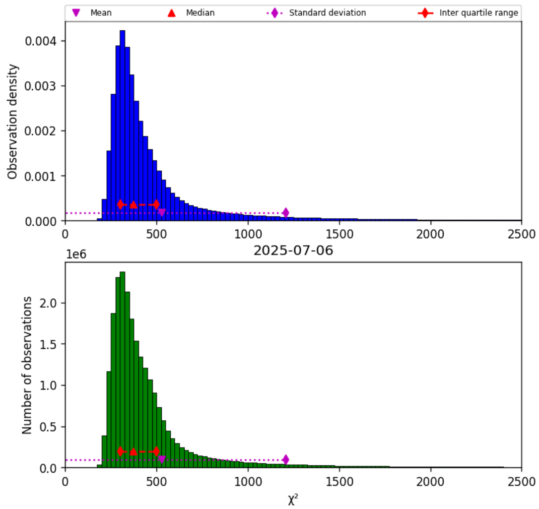
Figure 40: Histogram of “ \chi^2 ” for 2025-07-06 to 2025-07-06
