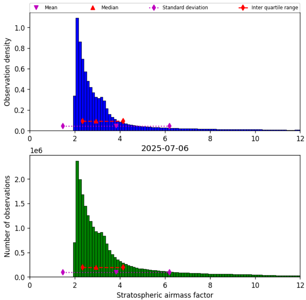
Figure 42: Histogram of “Stratospheric airmass factor” for 2025-07-06 to 2025-07-06
