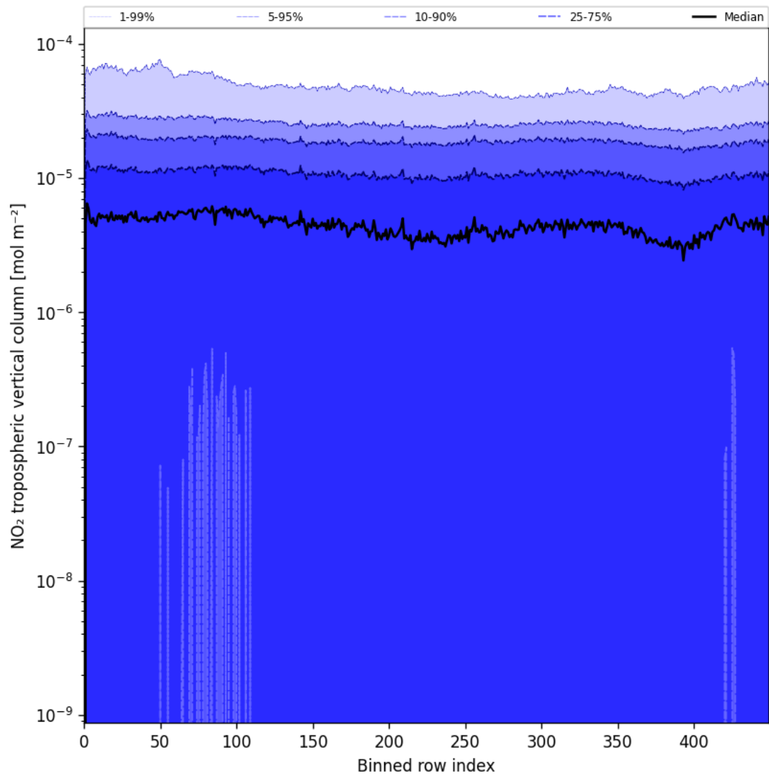
Figure 44: Along track statistics of "NO 2 tropospheric vertical column" for 2025-07-06 to 2025-07-06
