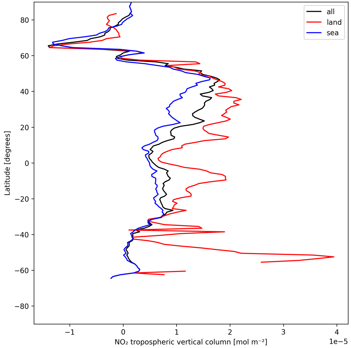
Figure 10: Zonal average of “NO 2 tropospheric vertical column” for 2025-07-06 to 2025-07-06.
