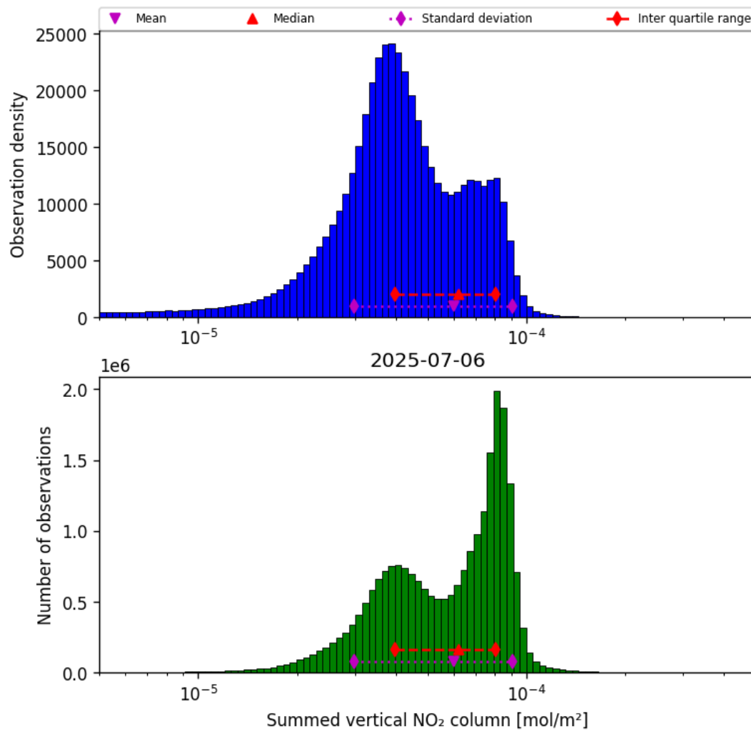
Figure 38: Histogram of "Summed vertical NO 2 column" for 2025-07-06 to 2025-07-06
