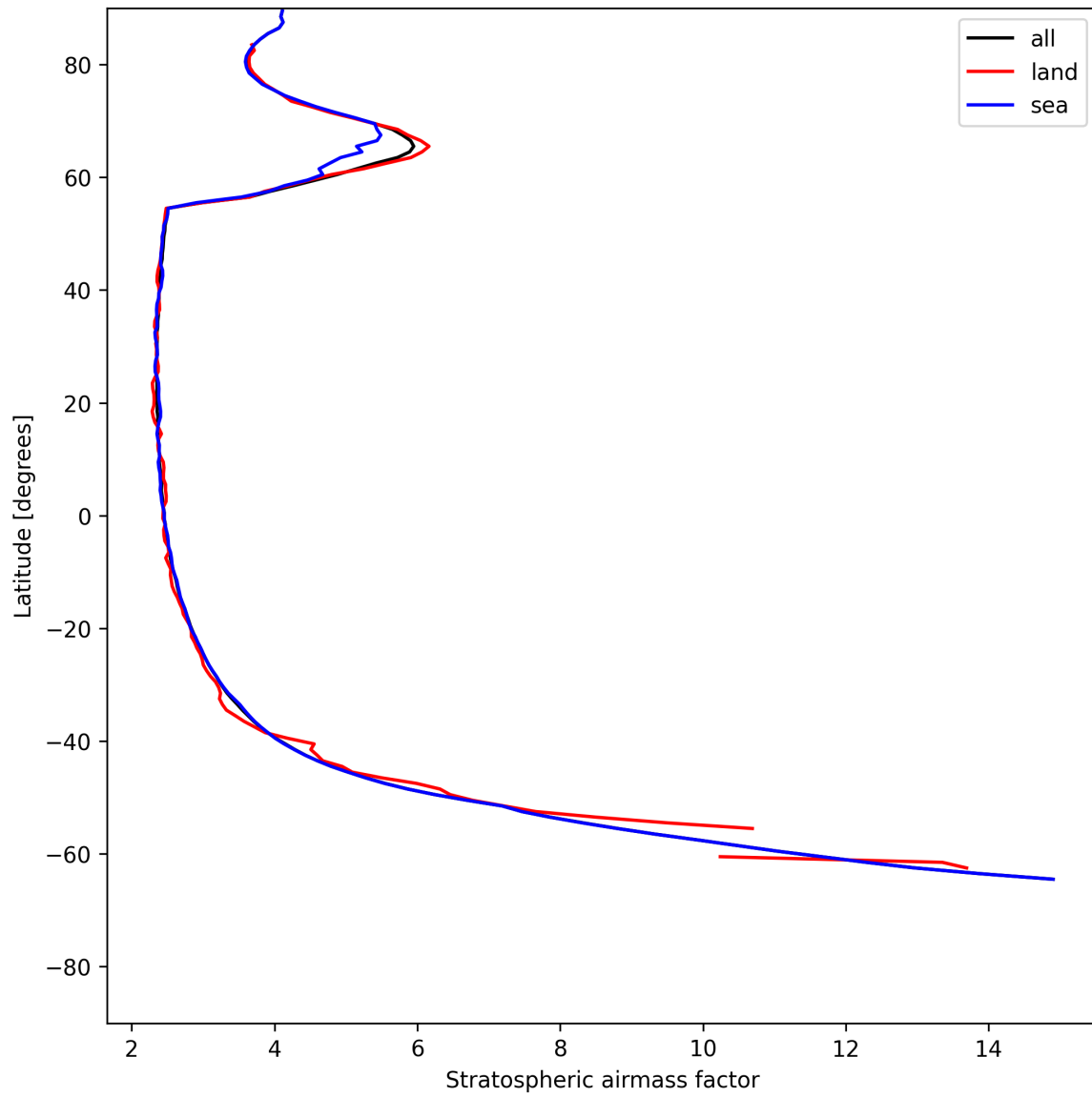
Figure 25: Zonal average of “Stratospheric air mass factor” for 2025-07-06 to 2025-07-06.
