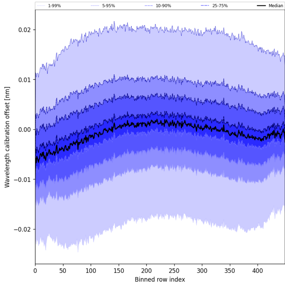
Figure 50: Along track statistics of “Wavelength calibration offset” for 2025-07-06 to 2025-07-06
