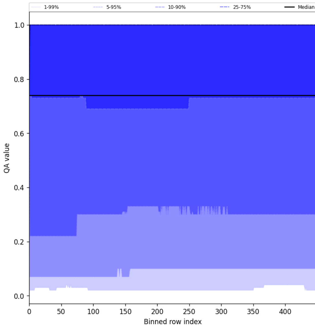
Figure 43: Along track statistics of “QA value” for 2025-07-08 to 2025-07-09
