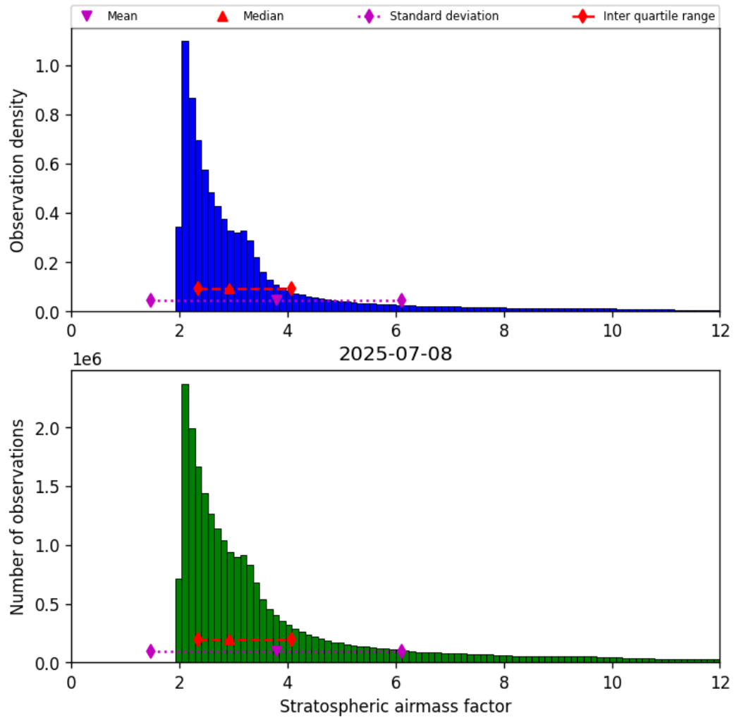
Figure 42: Histogram of “Stratospheric airmass factor” for 2025-07-08 to 2025-07-09
