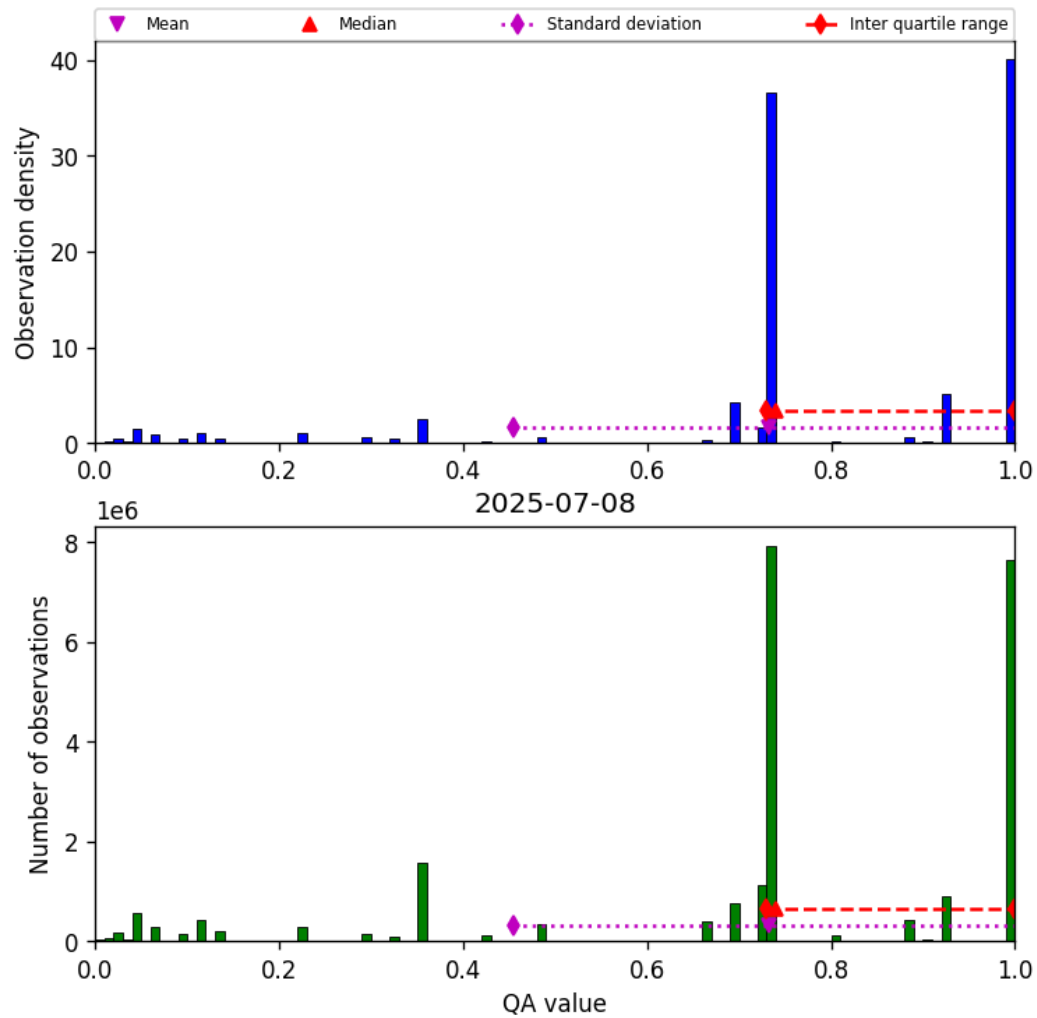
Figure 26: Histogram of “QA value” for 2025-07-08 to 2025-07-09
