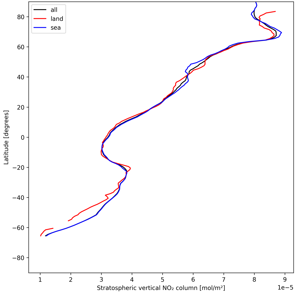
Figure 17: Zonal average of “Stratospheric vertical NO 2 column” for 2025-07-08 to 2025-07-09.
