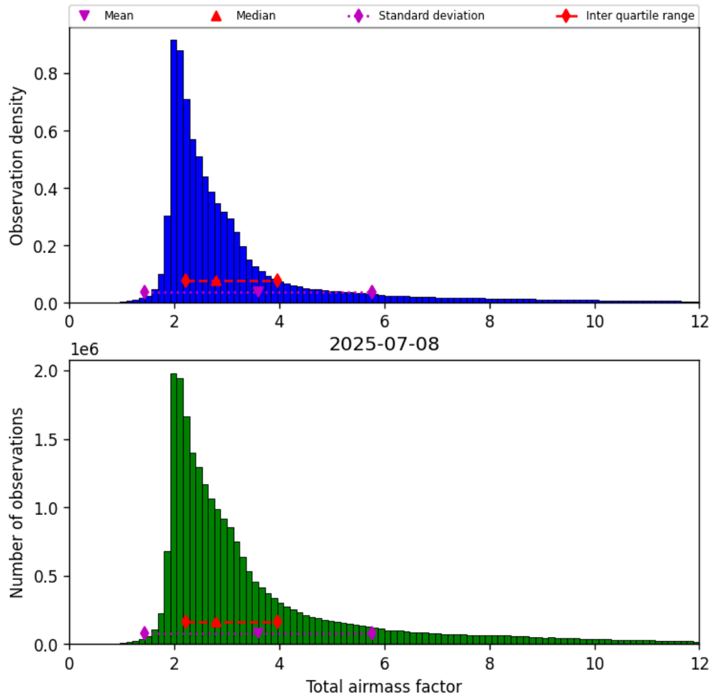
Figure 30: Histogram of “Total airmass factor” for 2025-07-08 to 2025-07-09
