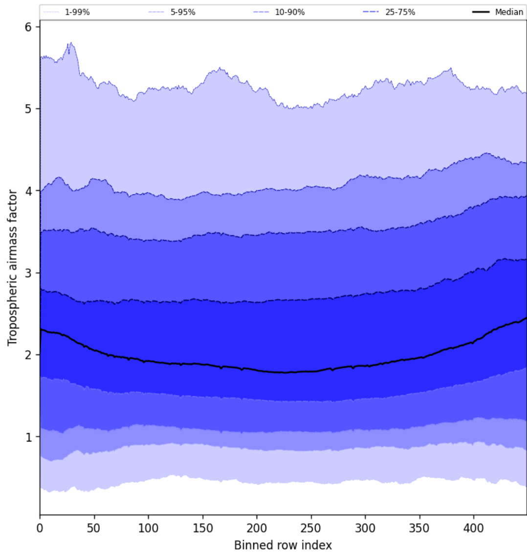
Figure 46: Along track statistics of “Tropospheric airmass factor” for 2025-07-08 to 2025-07-09
