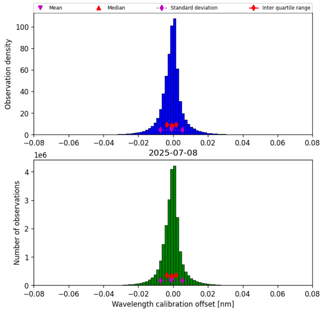
Figure 33: Histogram of “Wavelength calibration offset” for 2025-07-08 to 2025-07-09
