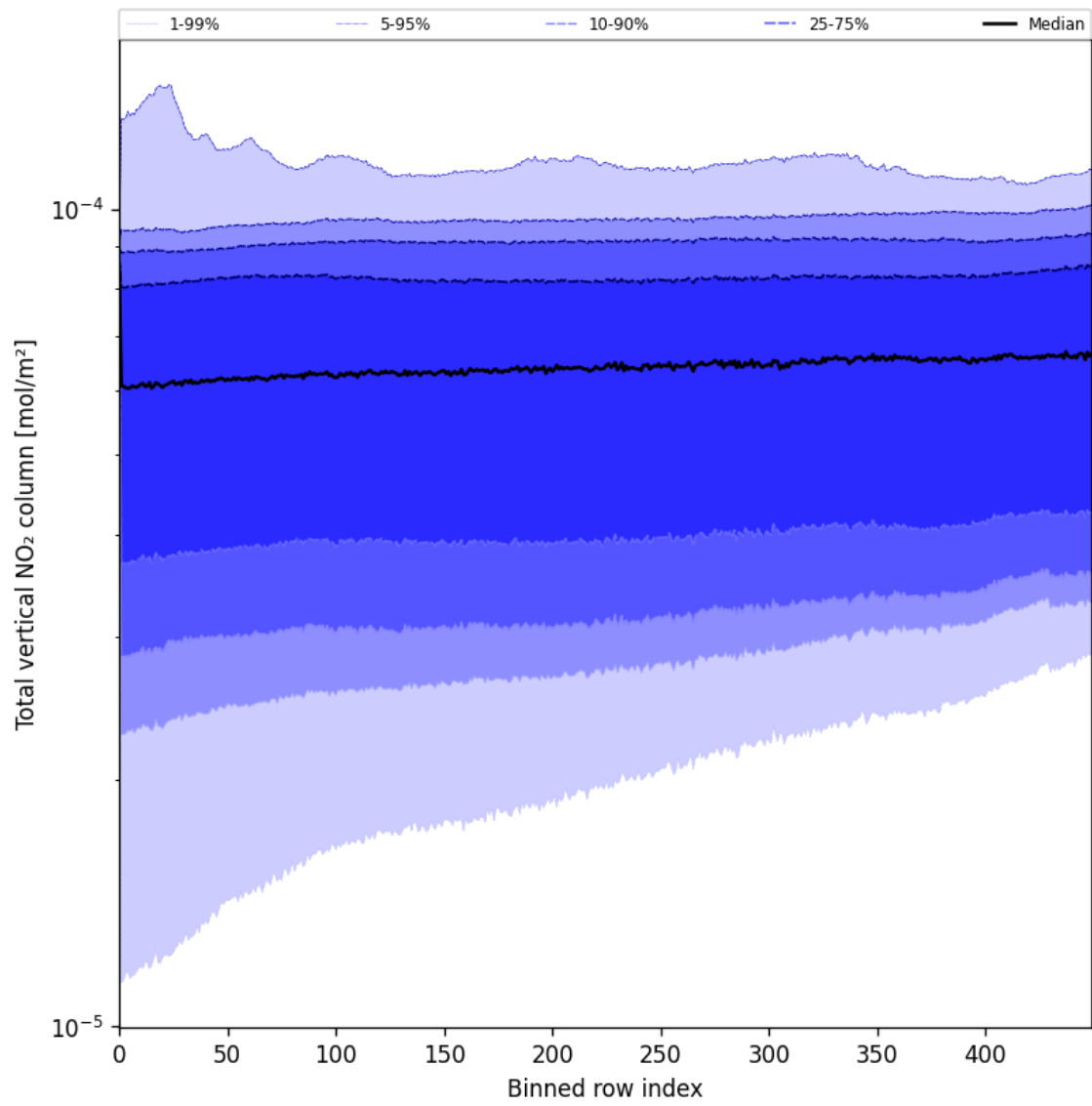
Figure 53: Along track statistics of “Total vertical NO 2 column” for 2025-07-08 to 2025-07-09
