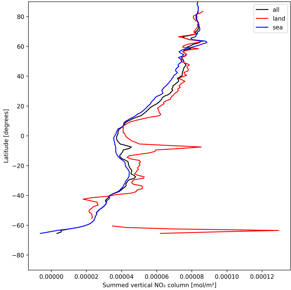
Figure 21: Zonal average of “Summed vertical NO 2 column” for 2025-07-08 to 2025-07-09.
