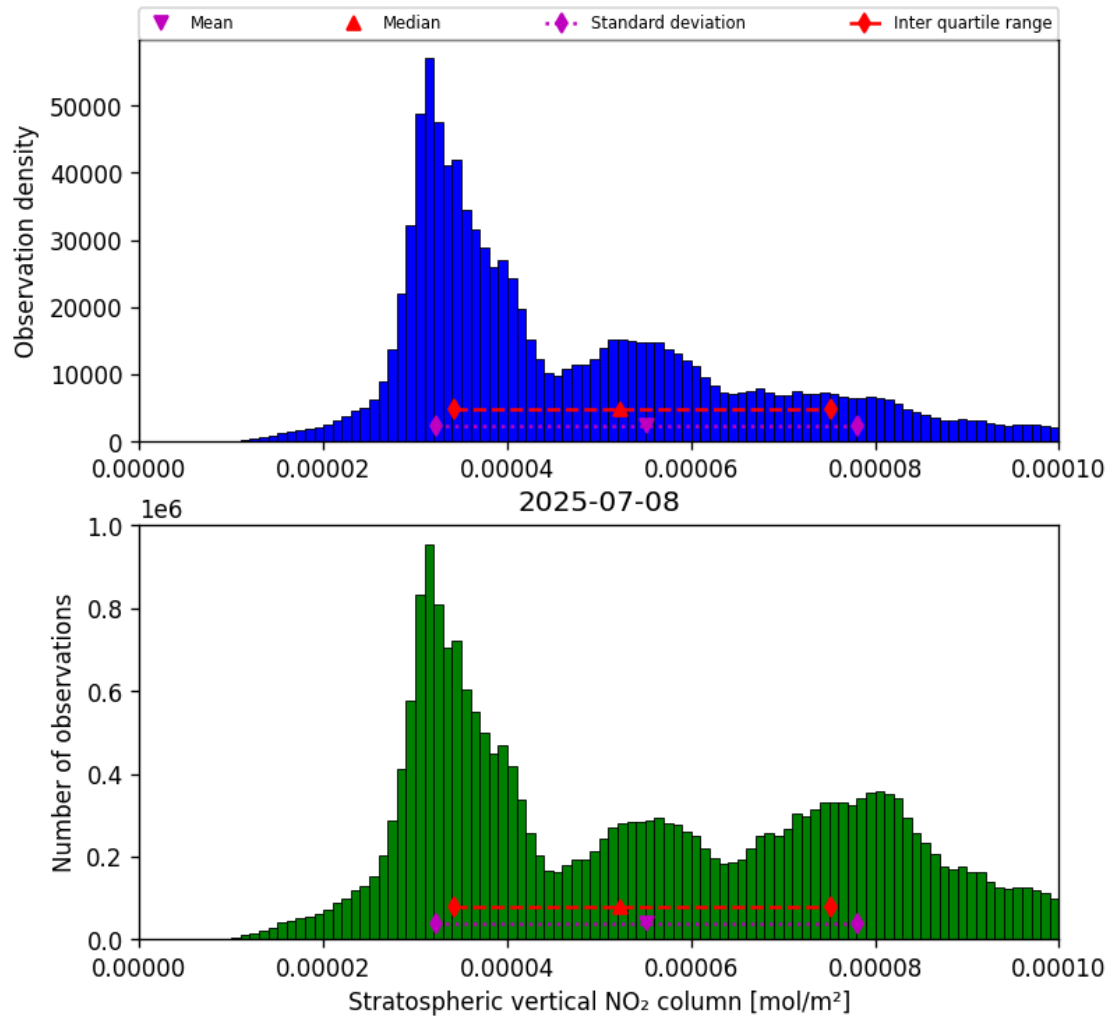
Figure 34: Histogram of “Stratospheric vertical NO 2 column” for 2025-07-08 to 2025-07-09
