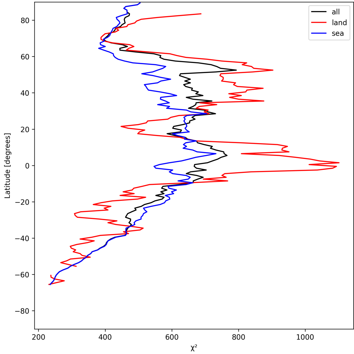
Figure 23: Zonal average of “ \chi^2 ” for 2025-07-08 to 2025-07-09.
