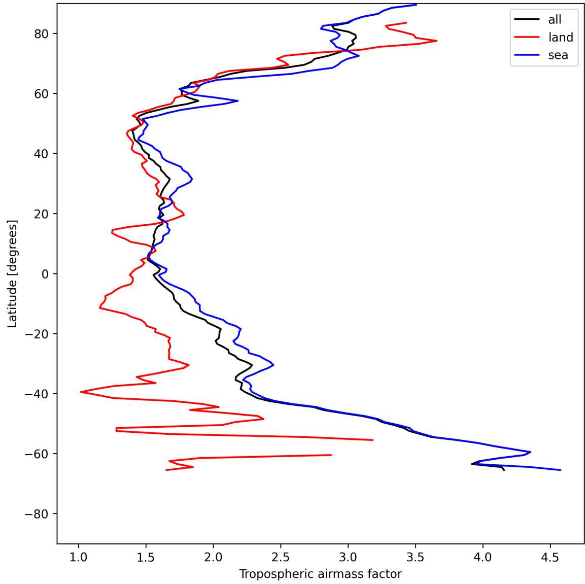
Figure 12: Zonal average of “Tropospheric airmass factor” for 2025-07-08 to 2025-07-09.
