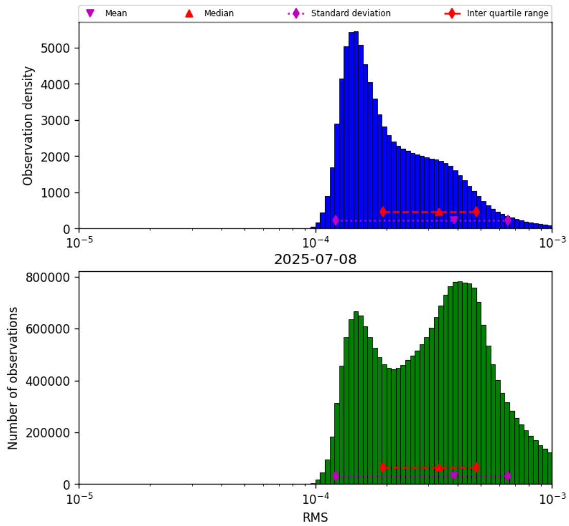
Figure 41: Histogram of “RMS” for 2025-07-08 to 2025-07-09
