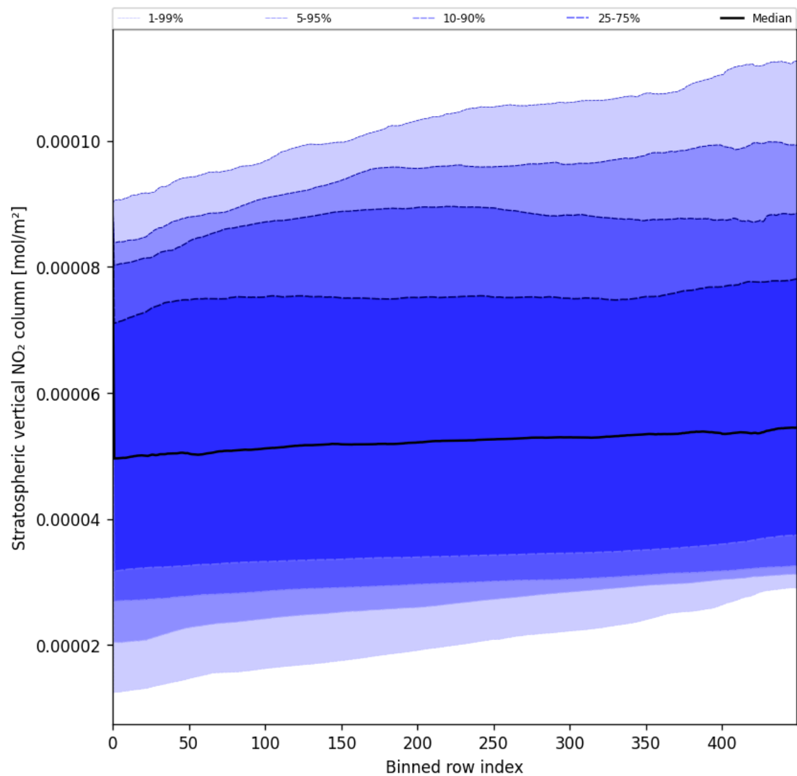
Figure 51: Along track statistics of “Stratospheric vertical NO 2 column” for 2025-07-08 to 2025-07-09
