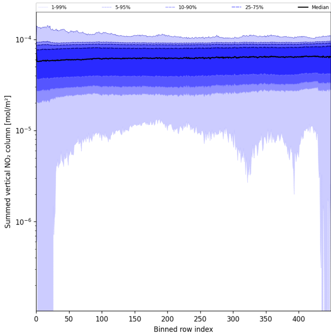
Figure 55: Along track statistics of “Summed vertical NO 2 column” for 2025-07-08 to 2025-07-09
