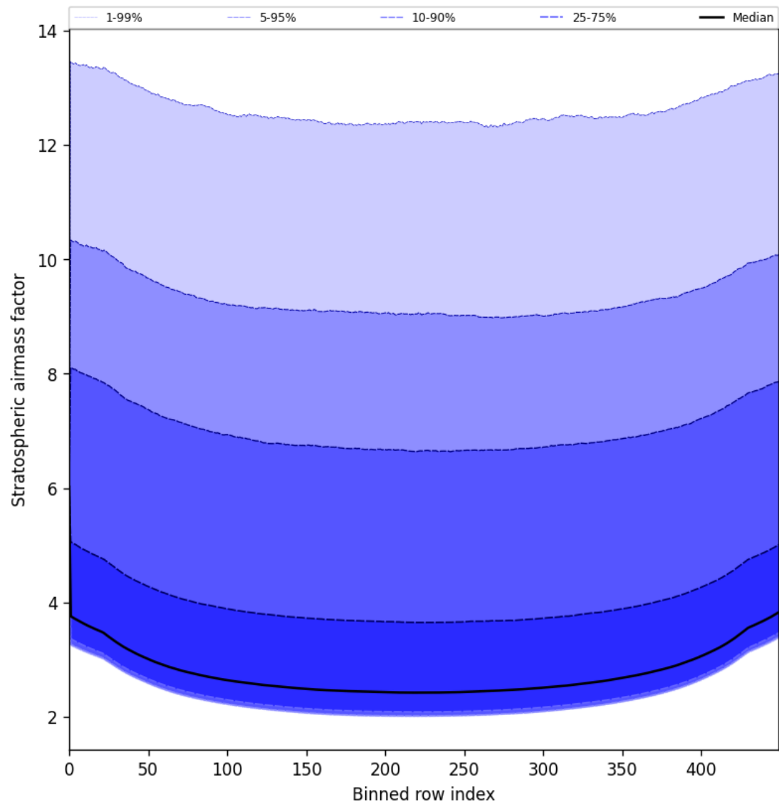
Figure 59: Along track statistics of “Stratospheric airmass factor” for 2025-07-08 to 2025-07-09
