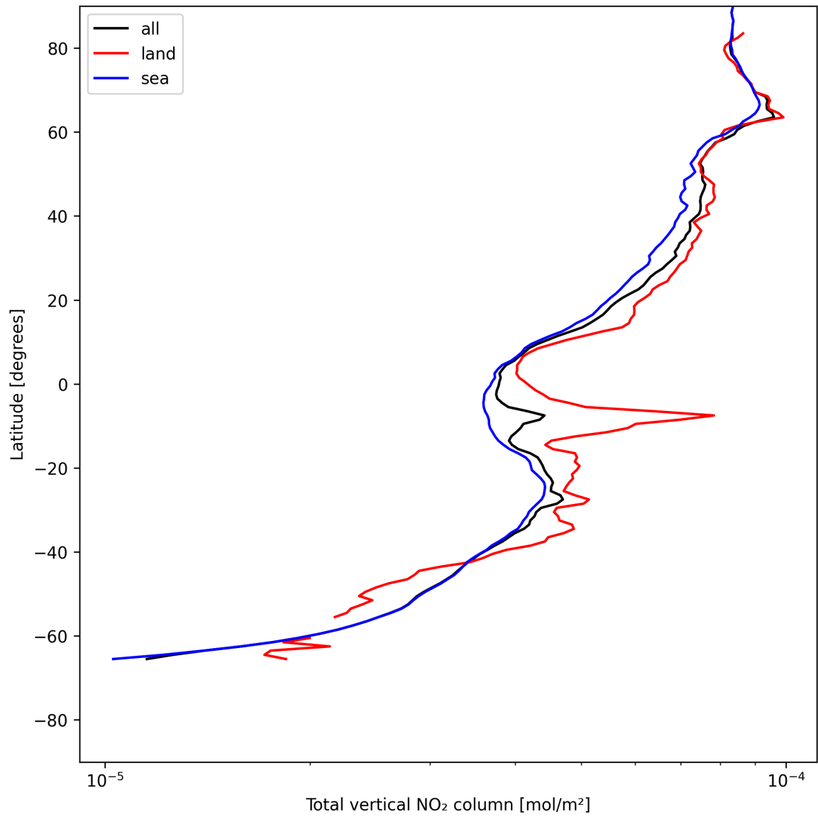
Figure 19: Zonal average of “Total vertical NO 2 column” for 2025-07-08 to 2025-07-09.
