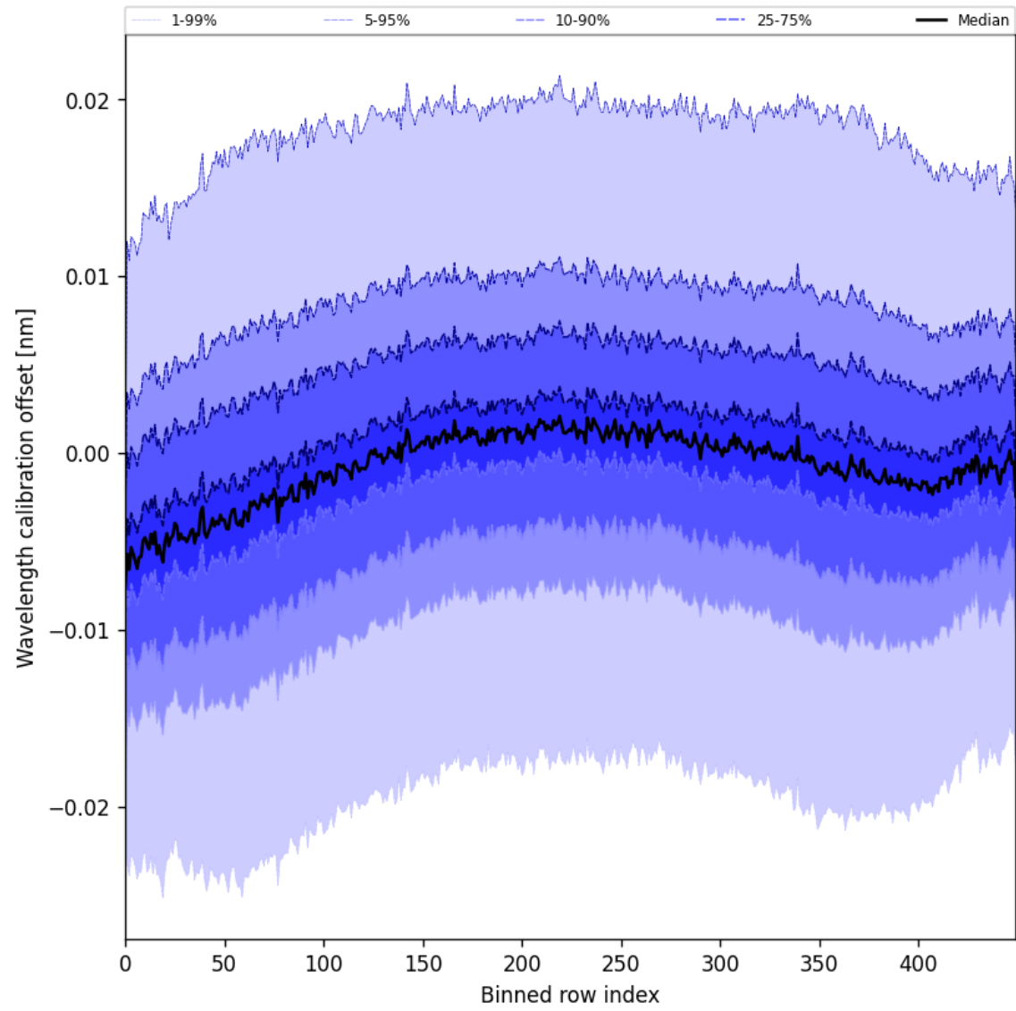
Figure 50: Along track statistics of “Wavelength calibration offset” for 2025-07-08 to 2025-07-09
