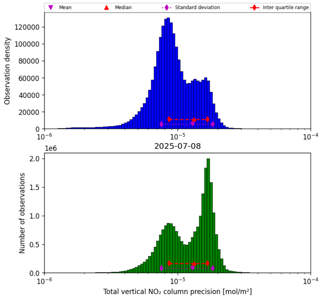
Figure 37: Histogram of “Total vertical NO 2 column precision” for 2025-07-08 to 2025-07-09
