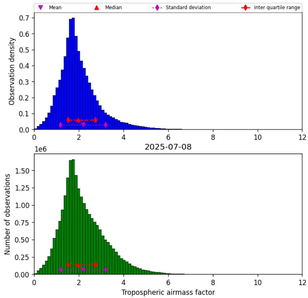
Figure 29: Histogram of “Tropospheric airmass factor” for 2025-07-08 to 2025-07-09
