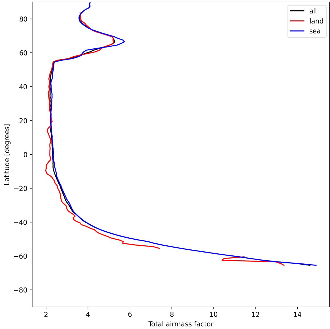
Figure 13: Zonal average of “Total airmass factor” for 2025-07-08 to 2025-07-09.
