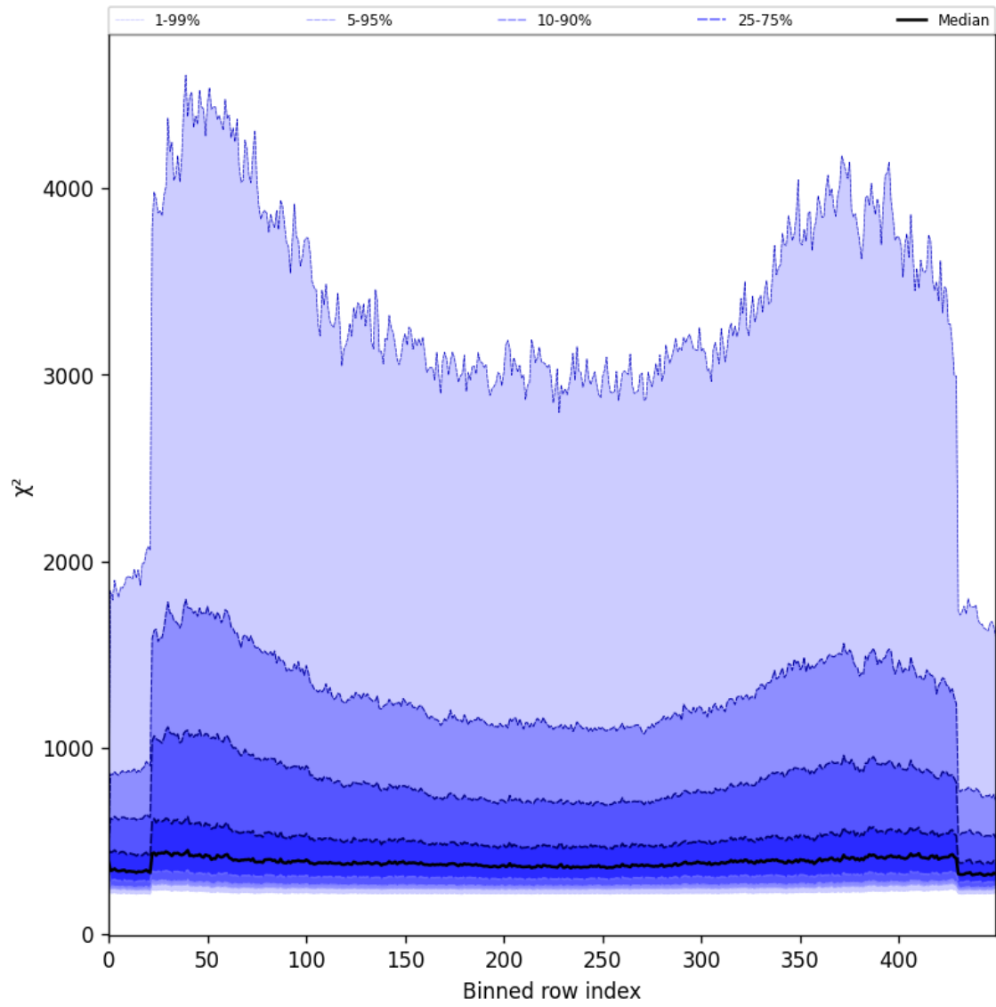
Figure 57: Along track statistics of “ \chi^2 ” for 2025-07-08 to 2025-07-09
