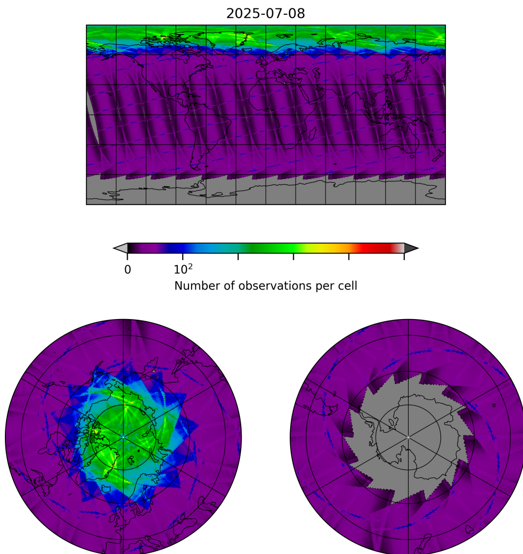
Figure 8: Map of the number of observations for 2025-07-08 to 2025-07-09
