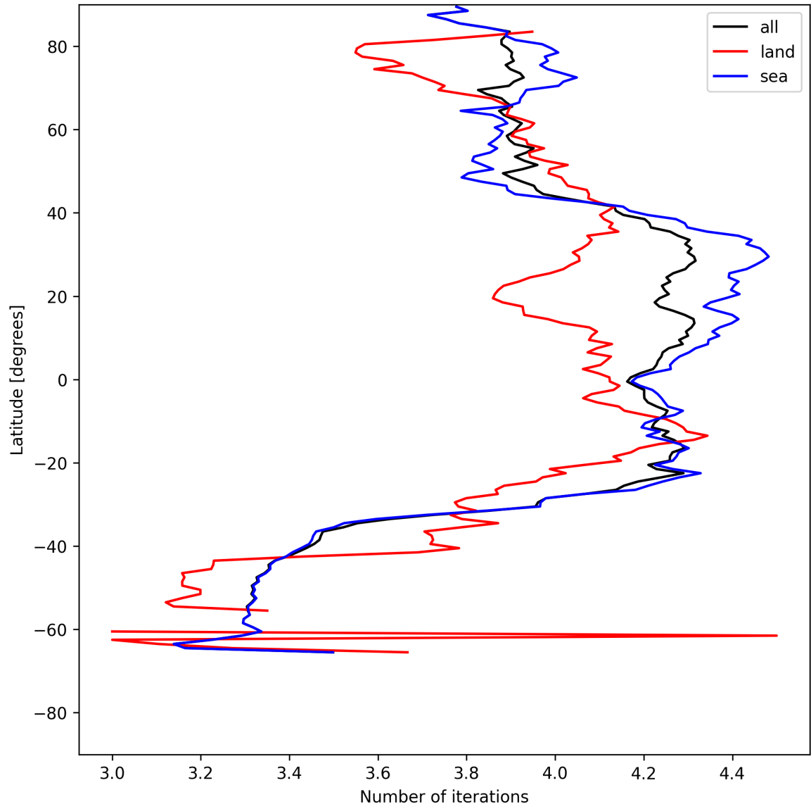
Figure 15: Zonal average of “Number of iterations” for 2025-07-08 to 2025-07-09.
