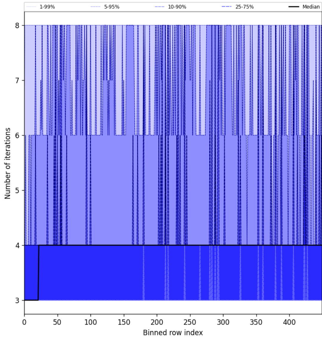
Figure 49: Along track statistics of “Number of iterations” for 2025-07-08 to 2025-07-09
