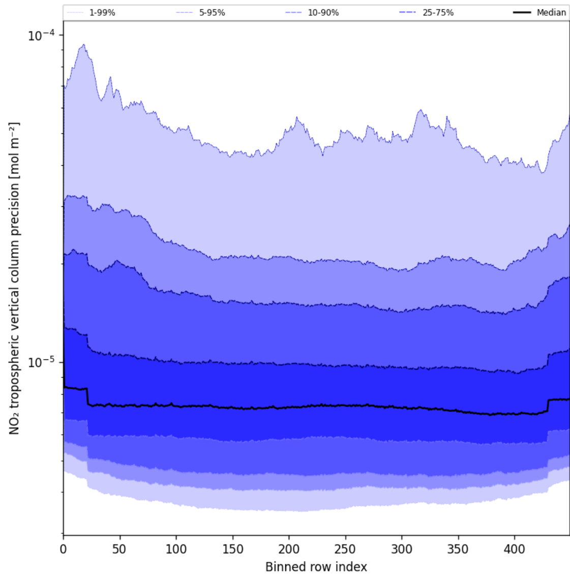
Figure 45: Along track statistics of “NO 2 tropospheric vertical column precision” for 2025-07-08 to 2025-07-09
