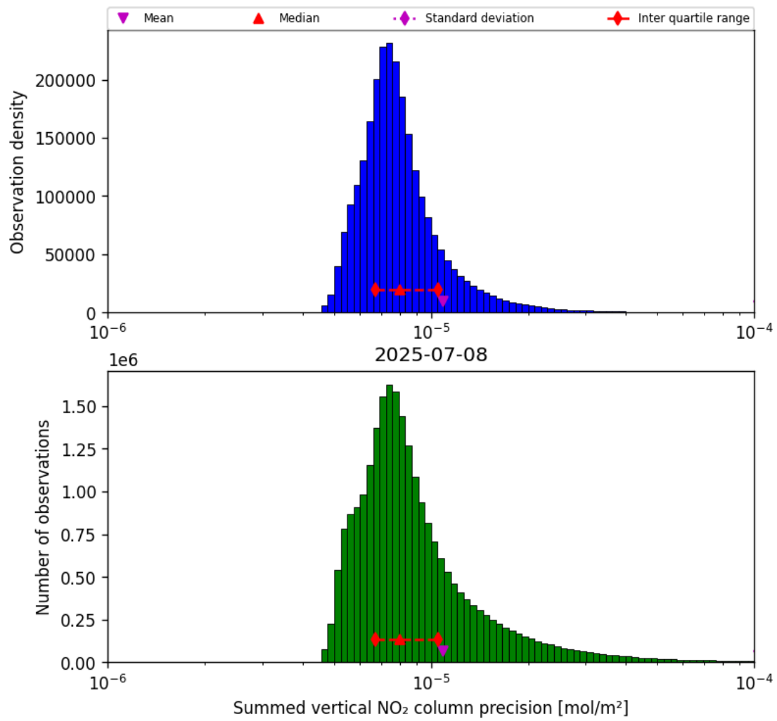
Figure 39: Histogram of “Summed vertical NO 2 column precision” for 2025-07-08 to 2025-07-09
