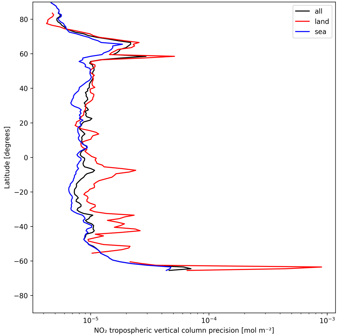
Figure 11: Zonal average of “NO 2 tropospheric vertical column precision” for 2025-07-08 to 2025-07-09.
