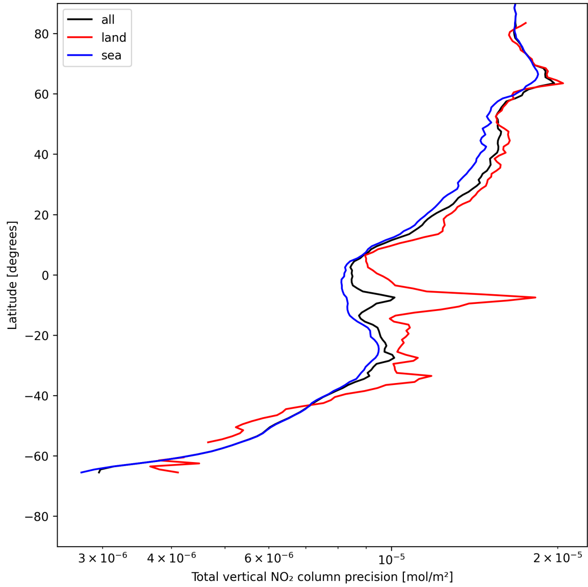
Figure 20: Zonal average of “Total vertical NO 2 column precision” for 2025-07-08 to 2025-07-09.
