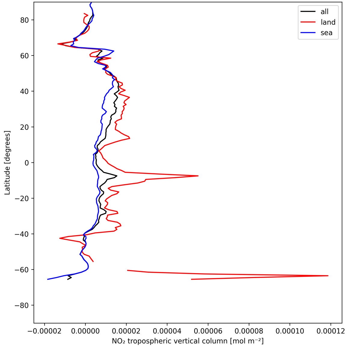
Figure 10: Zonal average of “NO 2 tropospheric vertical column” for 2025-07-08 to 2025-07-09.
