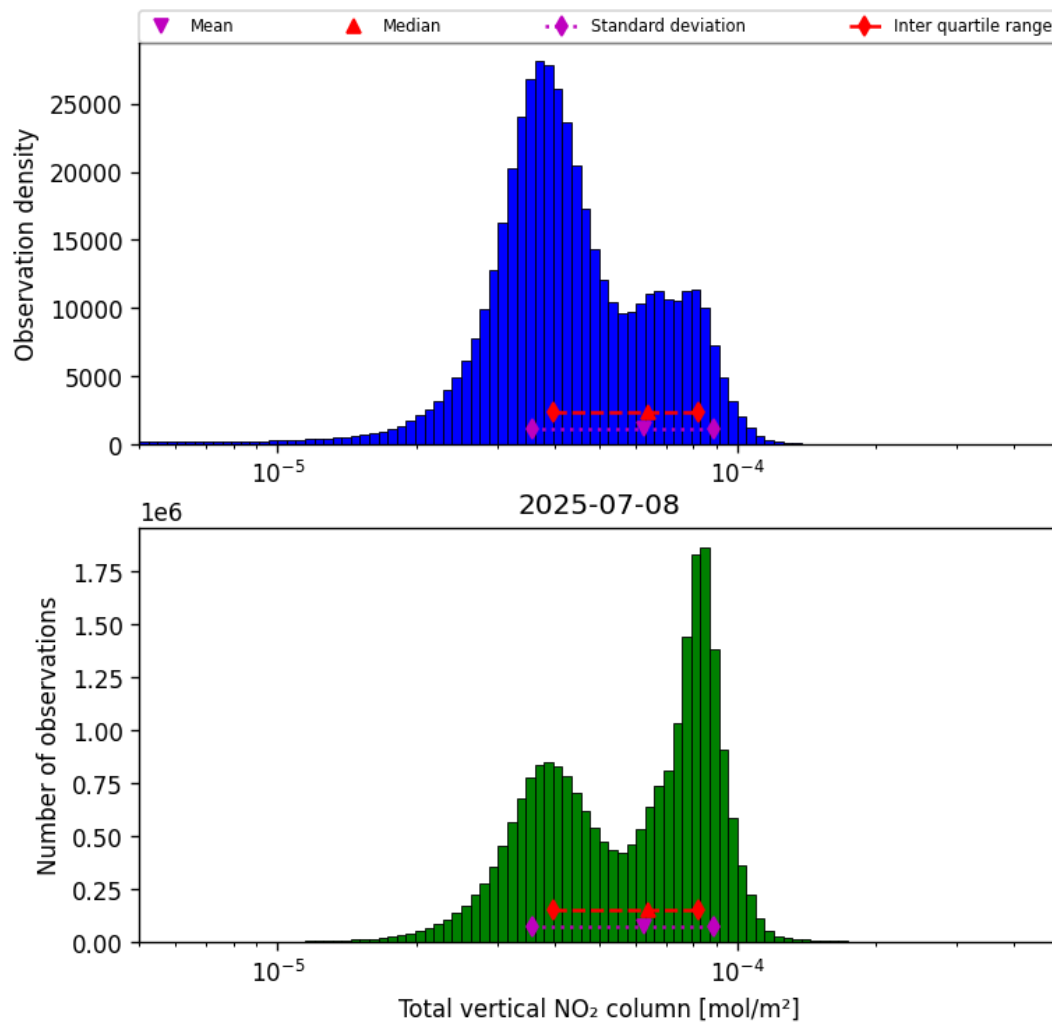
Figure 36: Histogram of “Total vertical NO 2 column” for 2025-07-08 to 2025-07-09
