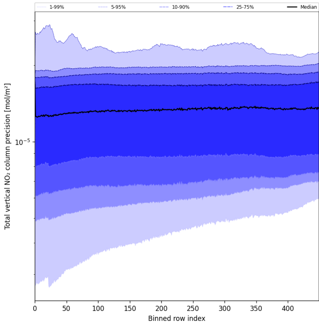
Figure 54: Along track statistics of “Total vertical NO 2 column precision” for 2025-07-08 to 2025-07-09
