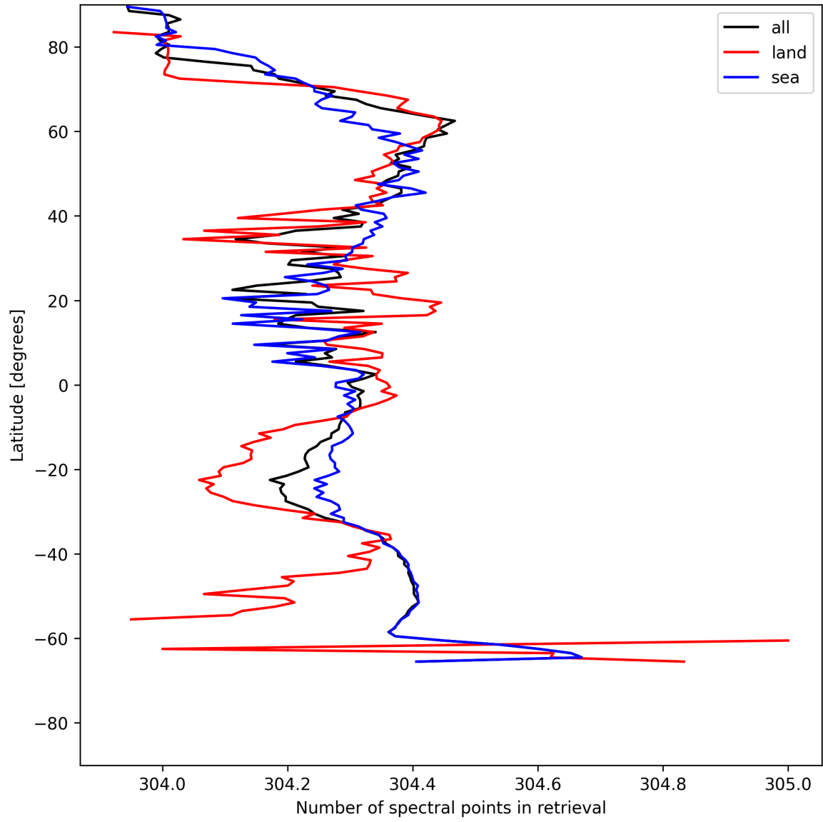
Figure 14: Zonal average of “Number of spectral points in retrieval” for 2025-07-08 to 2025-07-09.
