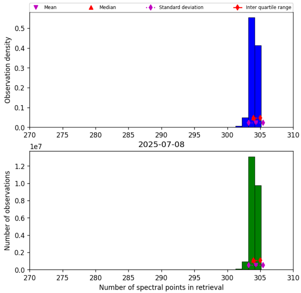
Figure 31: Histogram of “Number of spectral points in retrieval” for 2025-07-08 to 2025-07-09
