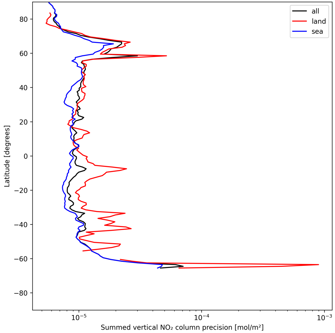
Figure 22: Zonal average of “Summed vertical NO 2 column precision” for 2025-07-08 to 2025-07-09.
