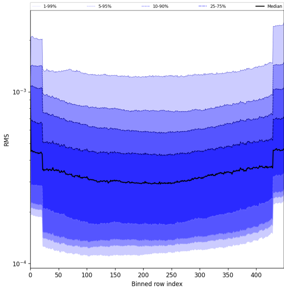
Figure 58: Along track statistics of “RMS” for 2025-07-08 to 2025-07-09
