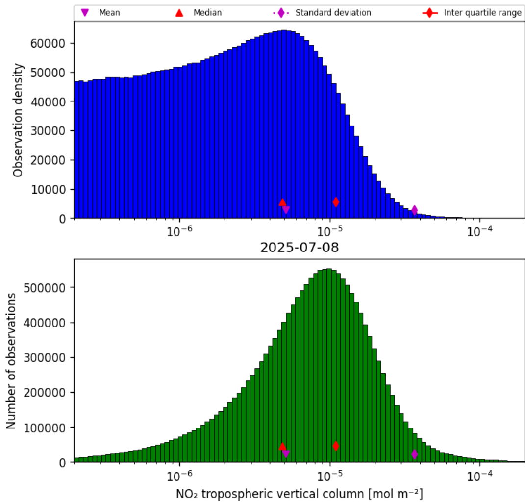
Figure 27: Histogram of “NO 2 tropospheric vertical column” for 2025-07-08 to 2025-07-09
