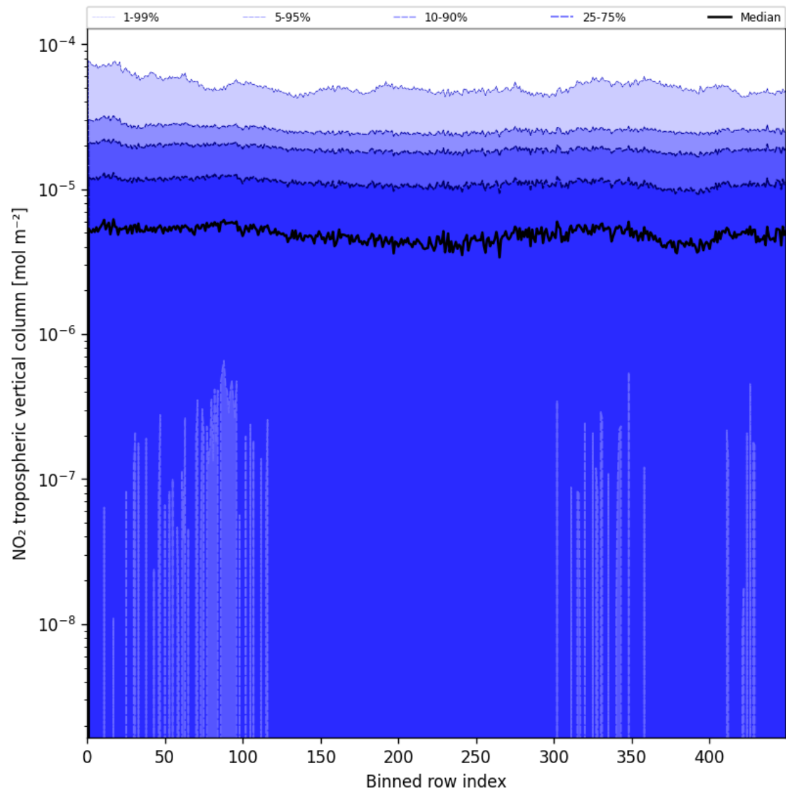
Figure 44: Along track statistics of “NO 2 tropospheric vertical column” for 2025-07-08 to 2025-07-09
