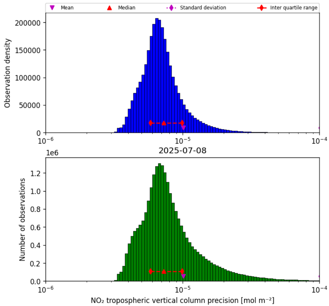
Figure 28: Histogram of “NO 2 tropospheric vertical column precision” for 2025-07-08 to 2025-07-09
