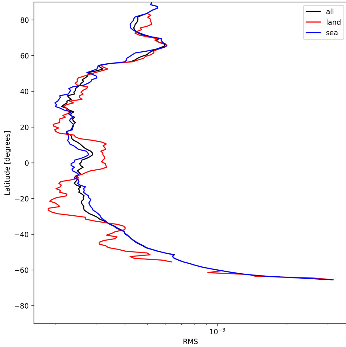
Figure 24: Zonal average of “RMS” for 2025-07-08 to 2025-07-09.
