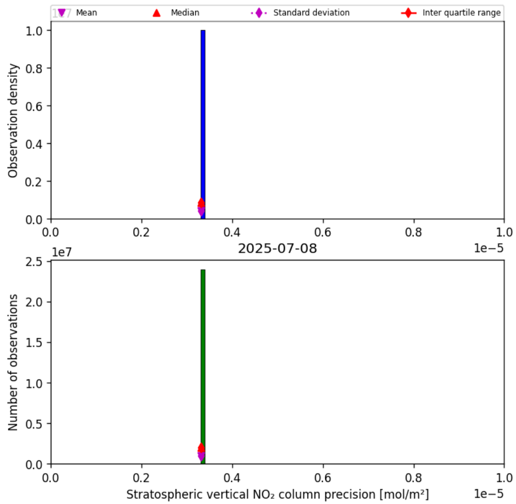
Figure 35: Histogram of “Stratospheric vertical NO 2 column precision” for 2025-07-08 to 2025-07-09
