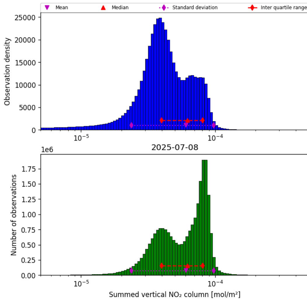
Figure 38: Histogram of “Summed vertical NO 2 column” for 2025-07-08 to 2025-07-09
