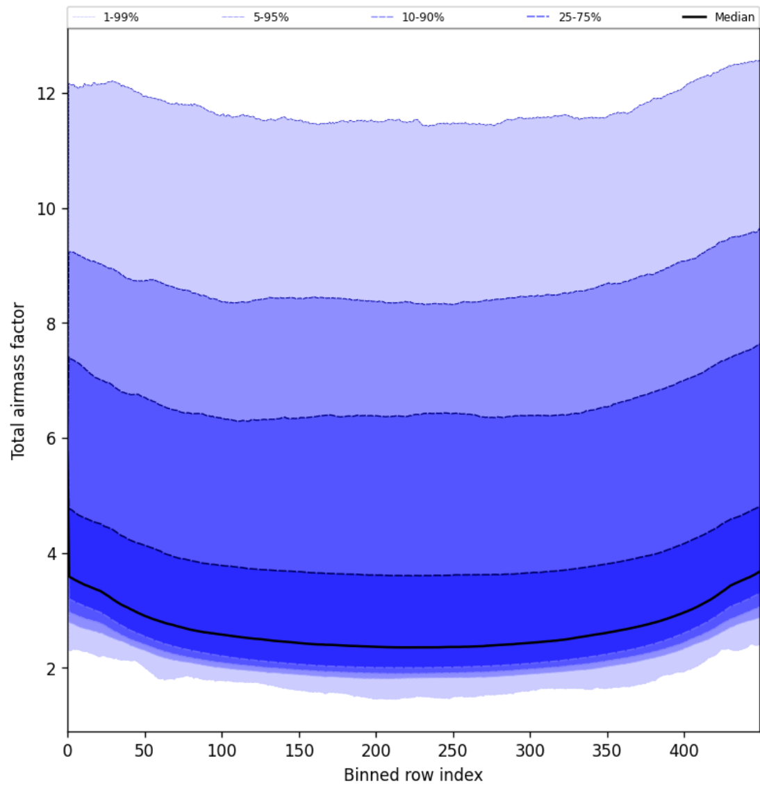
Figure 47: Along track statistics of “Total airmass factor” for 2025-07-08 to 2025-07-09
