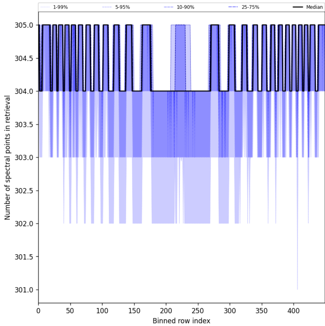
Figure 48: Along track statistics of “Number of spectral points in retrieval” for 2025-07-08 to 2025-07-09
