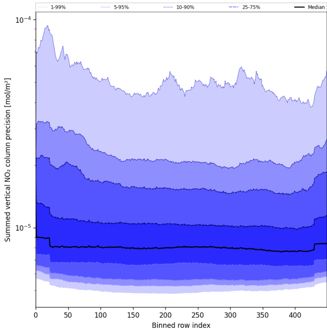
Figure 56: Along track statistics of “Summed vertical NO 2 column precision” for 2025-07-08 to 2025-07-09
