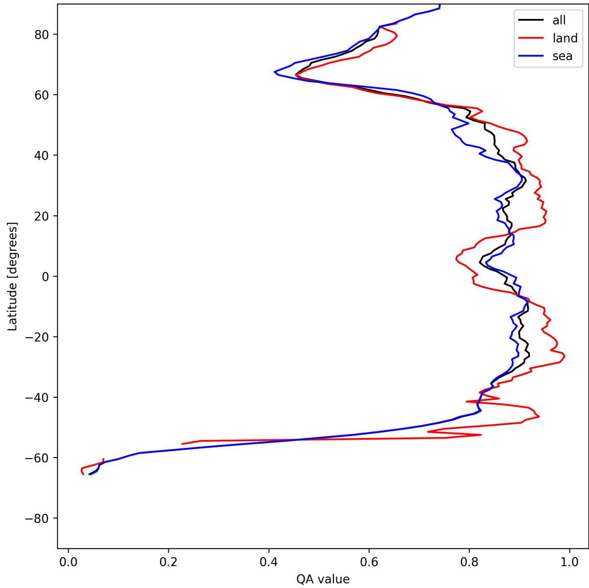
Figure 9: Zonal average of “QA value” for 2025-07-08 to 2025-07-09.
