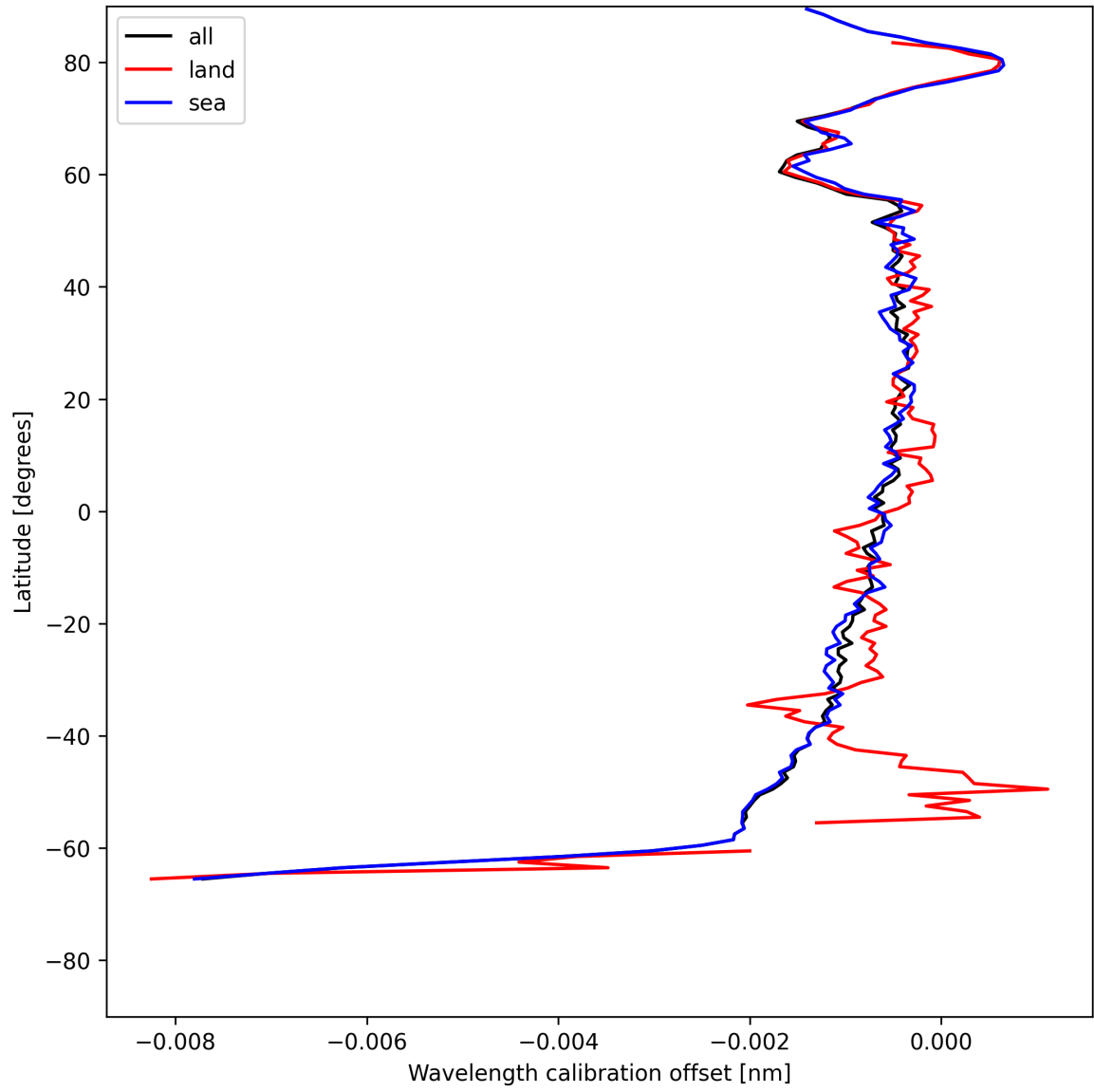
Figure 16: Zonal average of “Wavelength calibration offset” for 2025-07-08 to 2025-07-09.
