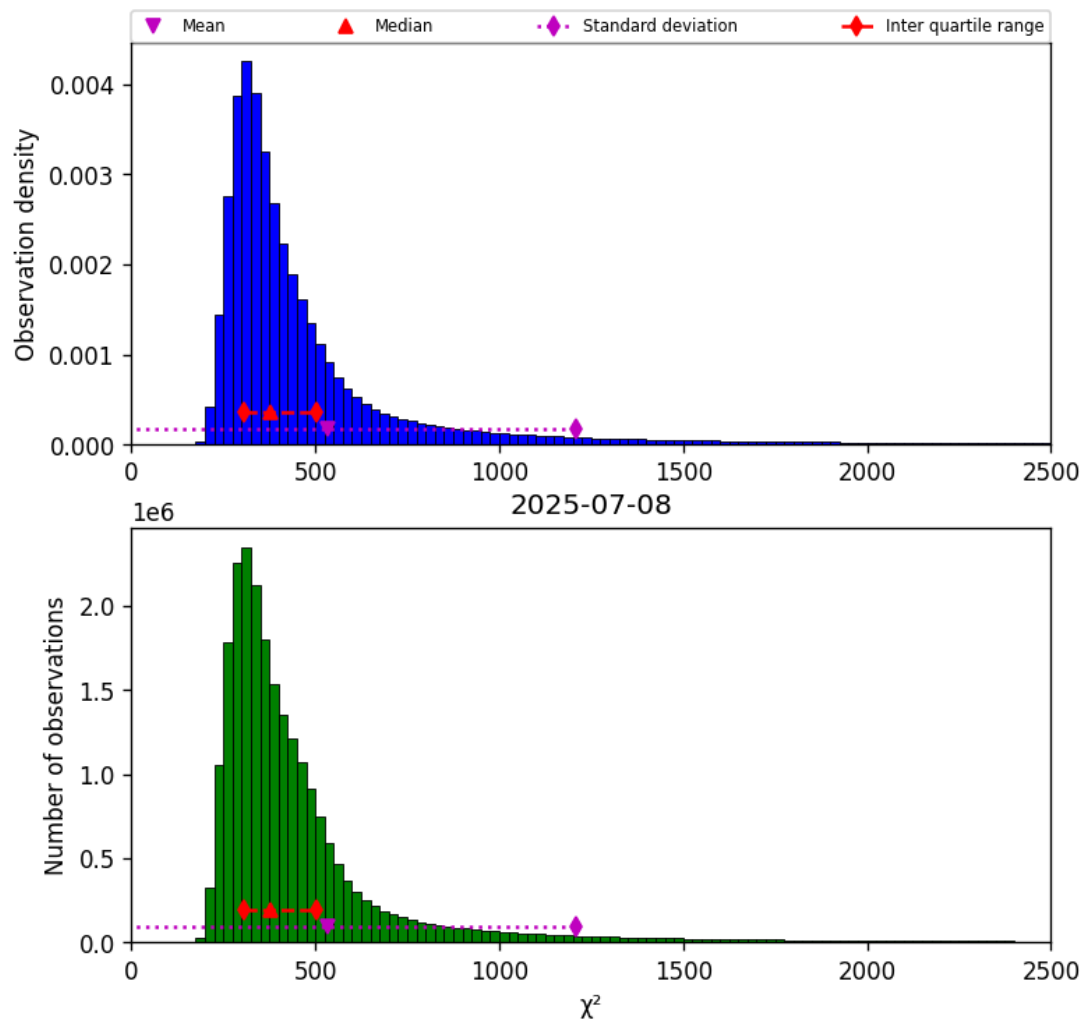
Figure 40: Histogram of “ \chi^2 ” for 2025-07-08 to 2025-07-09
