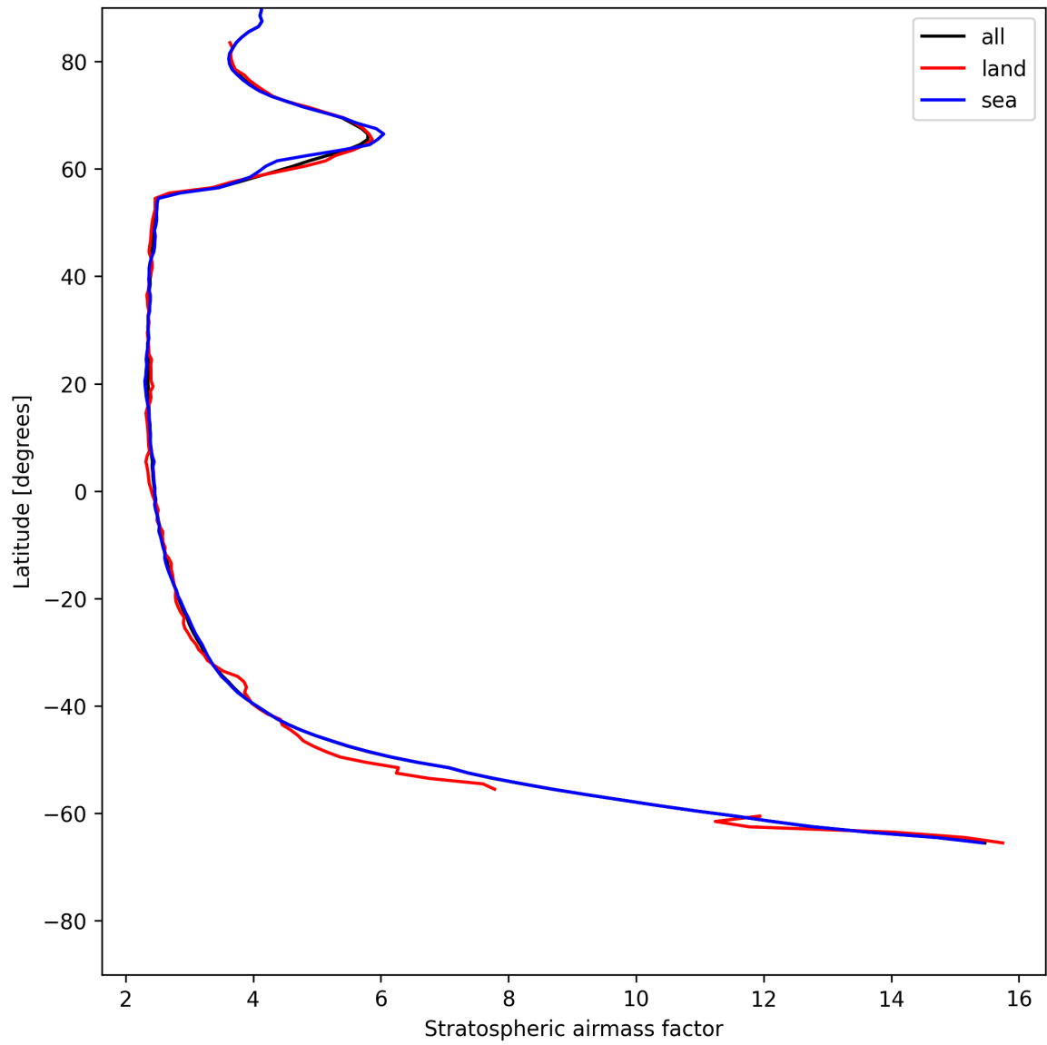
Figure 25: Zonal average of “Stratospheric air mass factor” for 2025-07-08 to 2025-07-09.
