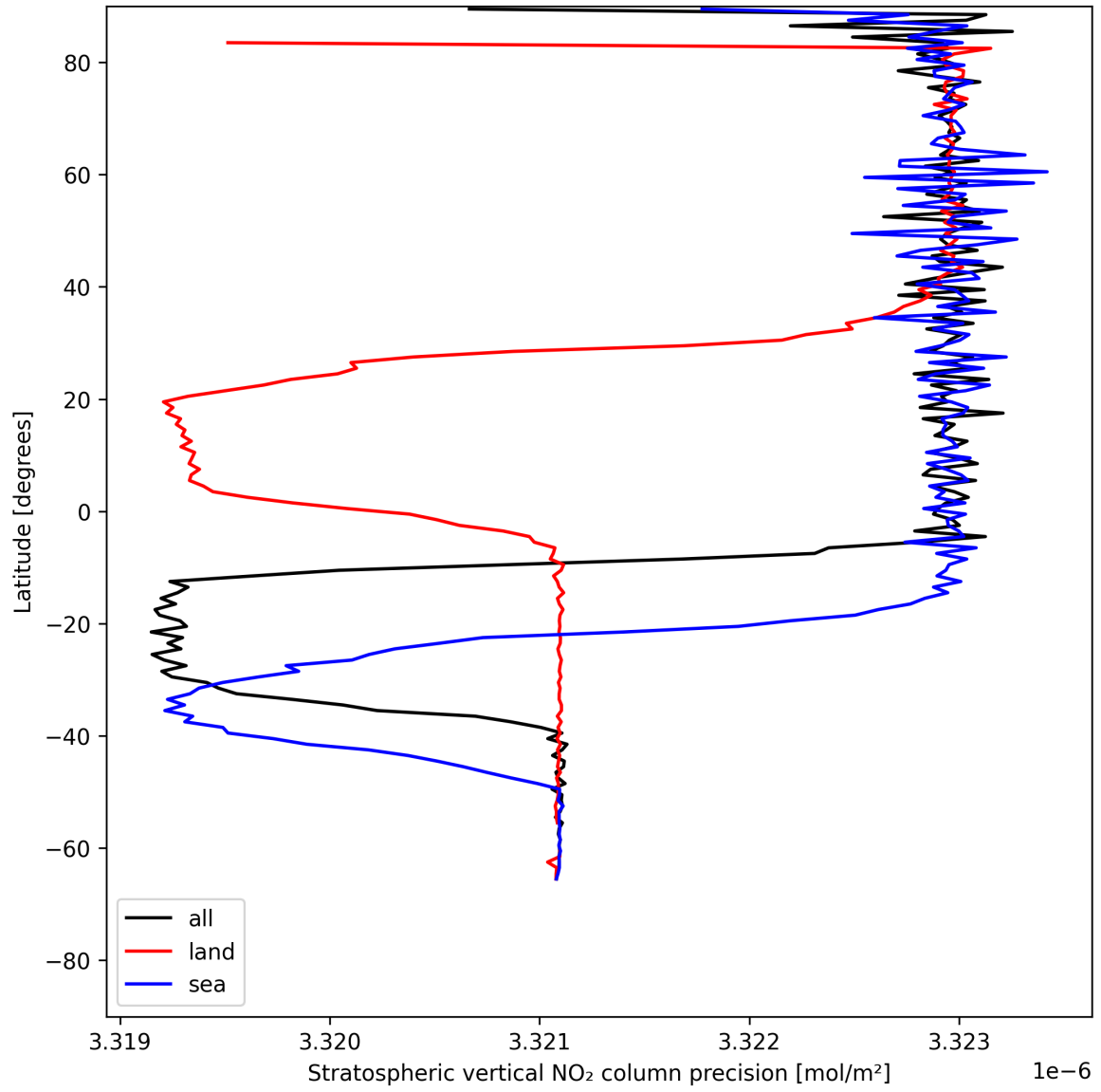
Figure 18: Zonal average of “Stratospheric vertical NO 2 column precision” for 2025-07-08 to 2025-07-09.
