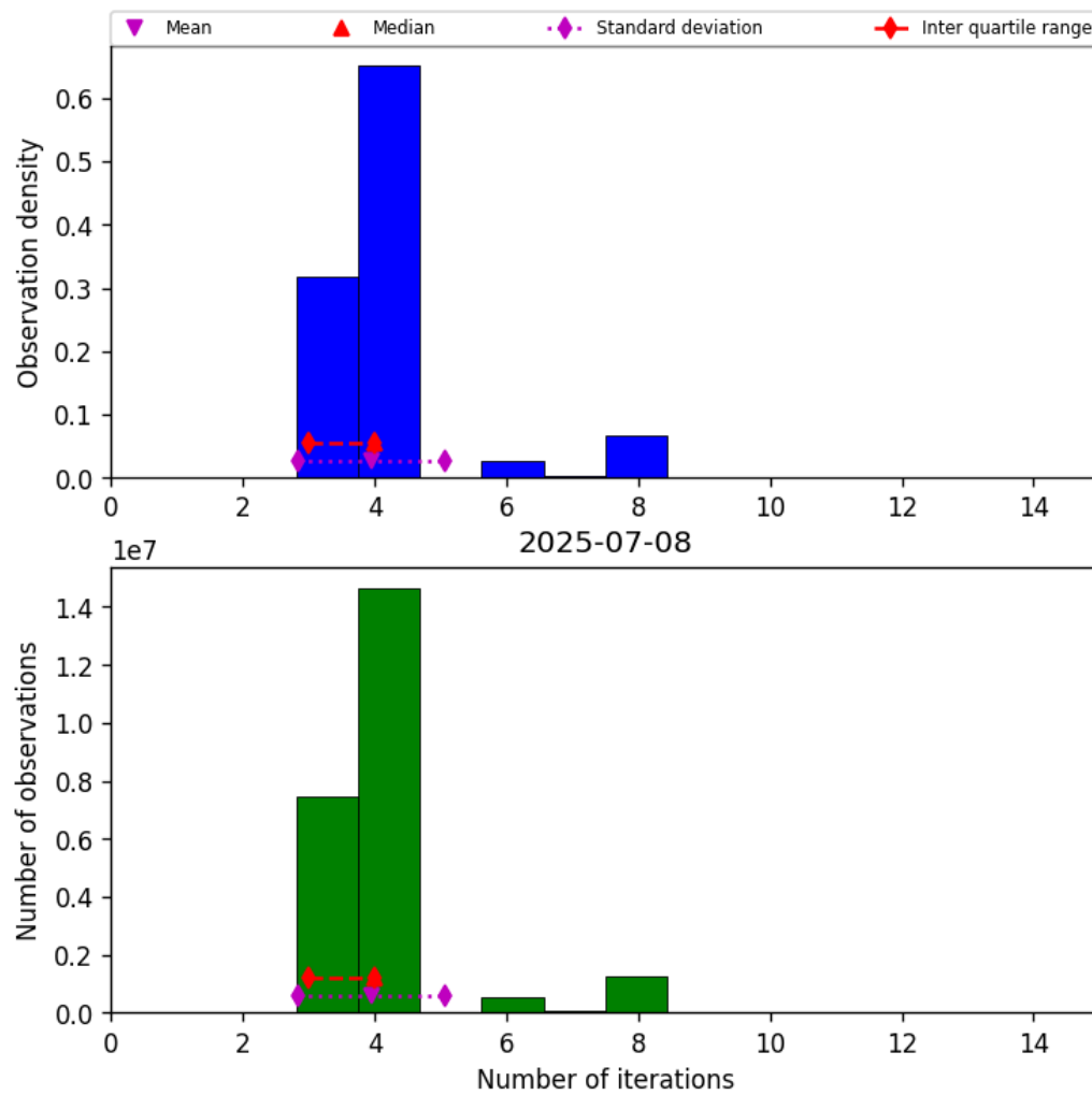
Figure 32: Histogram of “Number of iterations” for 2025-07-08 to 2025-07-09
