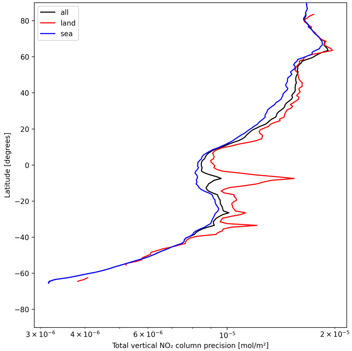
Figure 20: Zonal average of “Total vertical NO 2 column precision” for 2025-07-09 to 2025-07-10.
