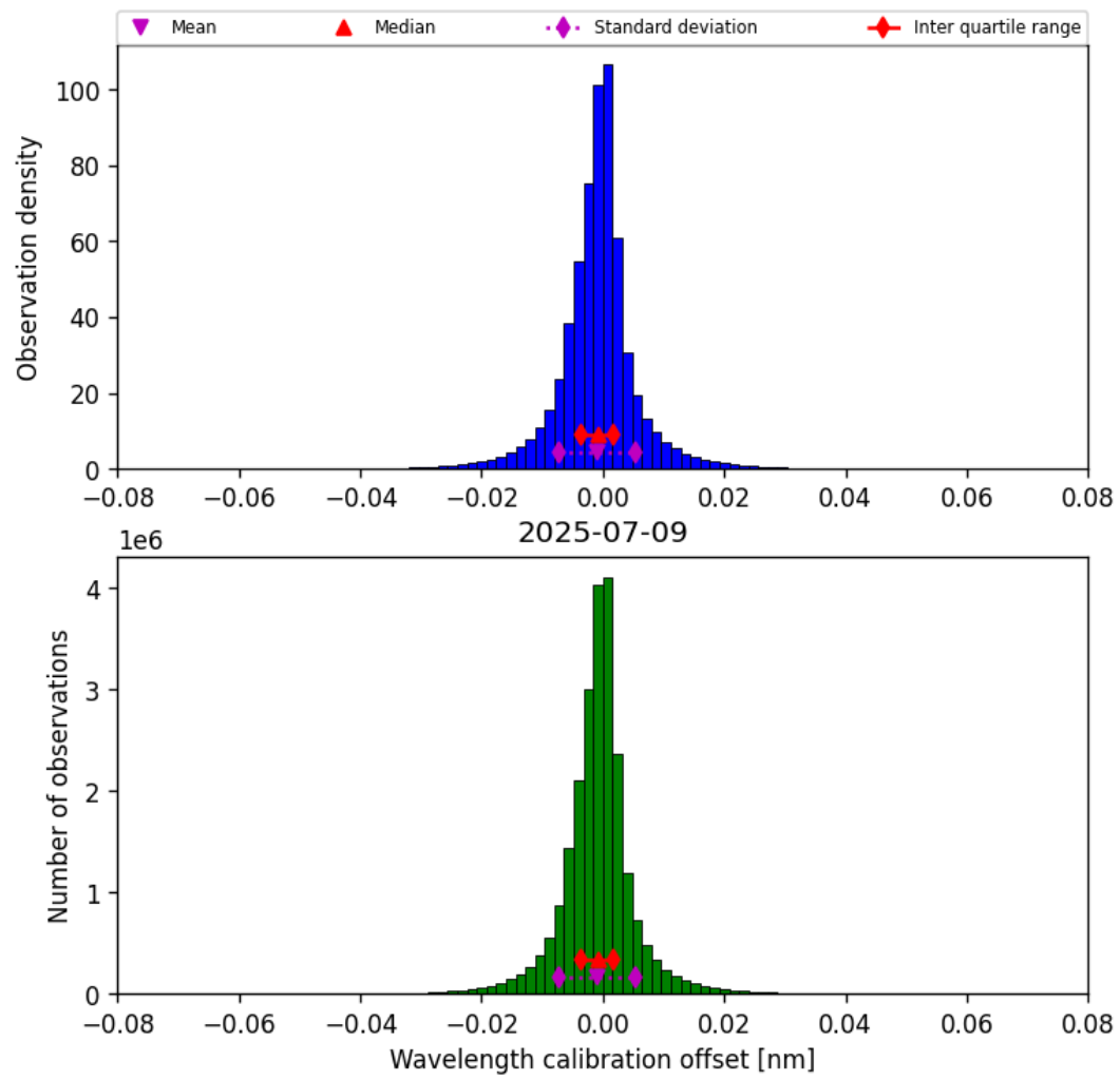
Figure 33: Histogram of “Wavelength calibration offset” for 2025-07-09 to 2025-07-10
