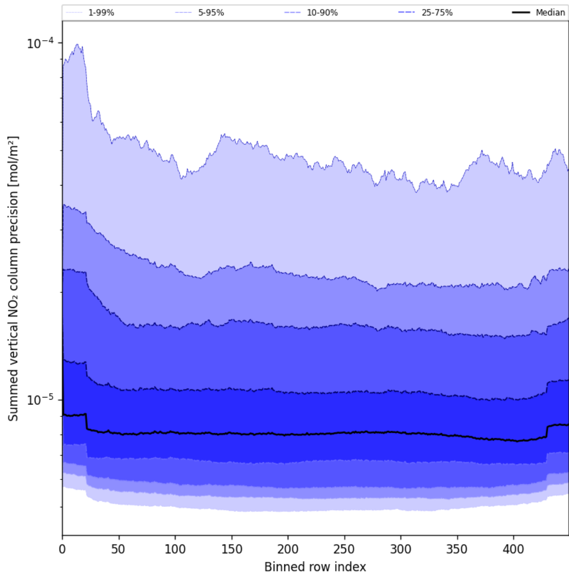
Figure 56: Along track statistics of “Summed vertical NO 2 column precision” for 2025-07-09 to 2025-07-10
