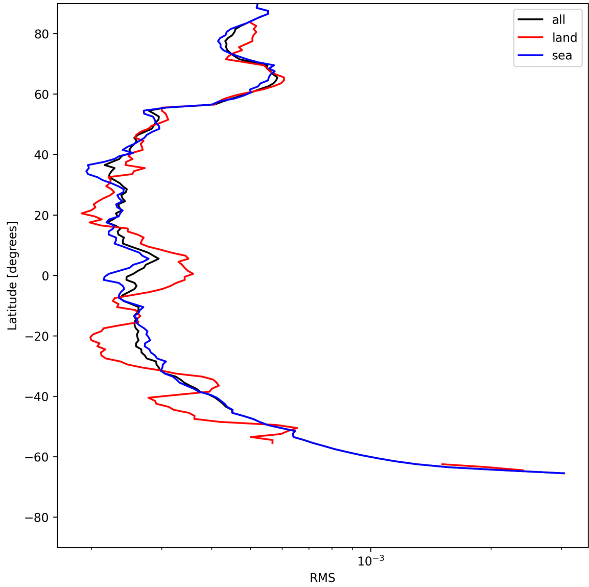
Figure 24: Zonal average of “RMS” for 2025-07-09 to 2025-07-10.
