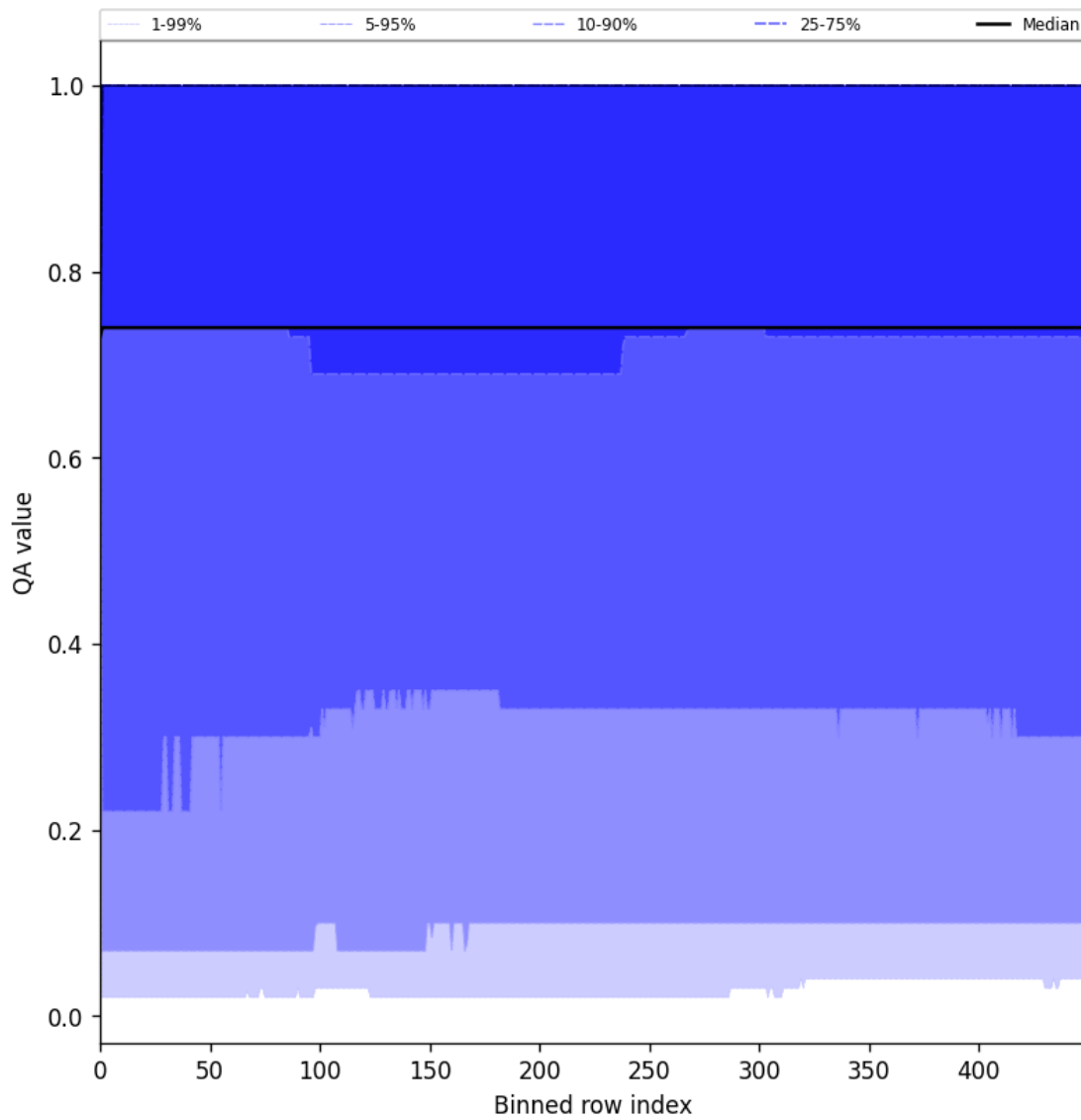
Figure 43: Along track statistics of “QA value” for 2025-07-09 to 2025-07-10
