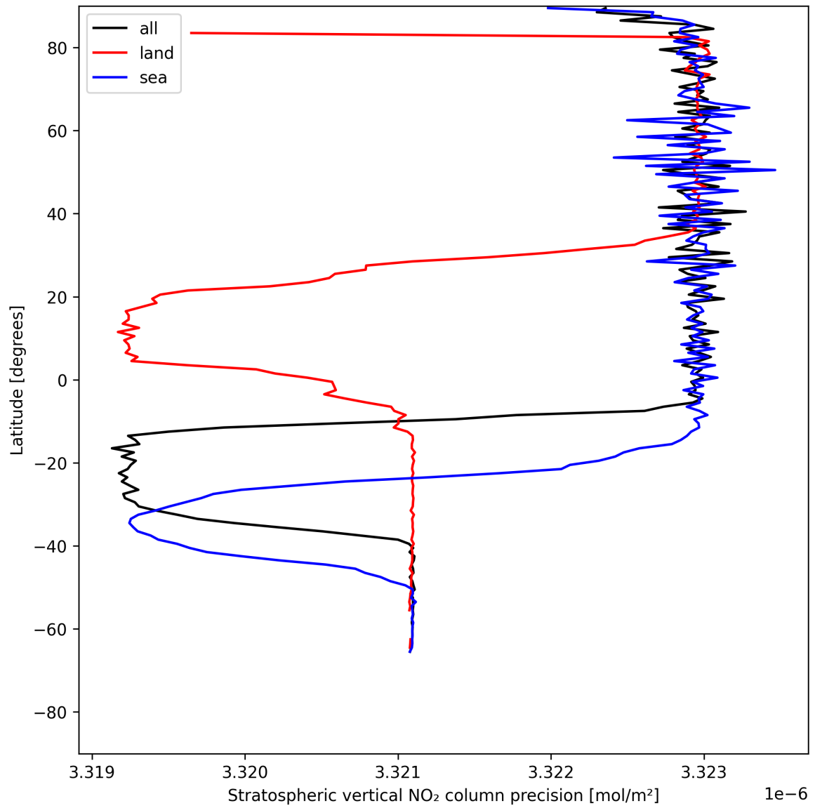
Figure 18: Zonal average of “Stratospheric vertical NO 2 column precision” for 2025-07-09 to 2025-07-10.
