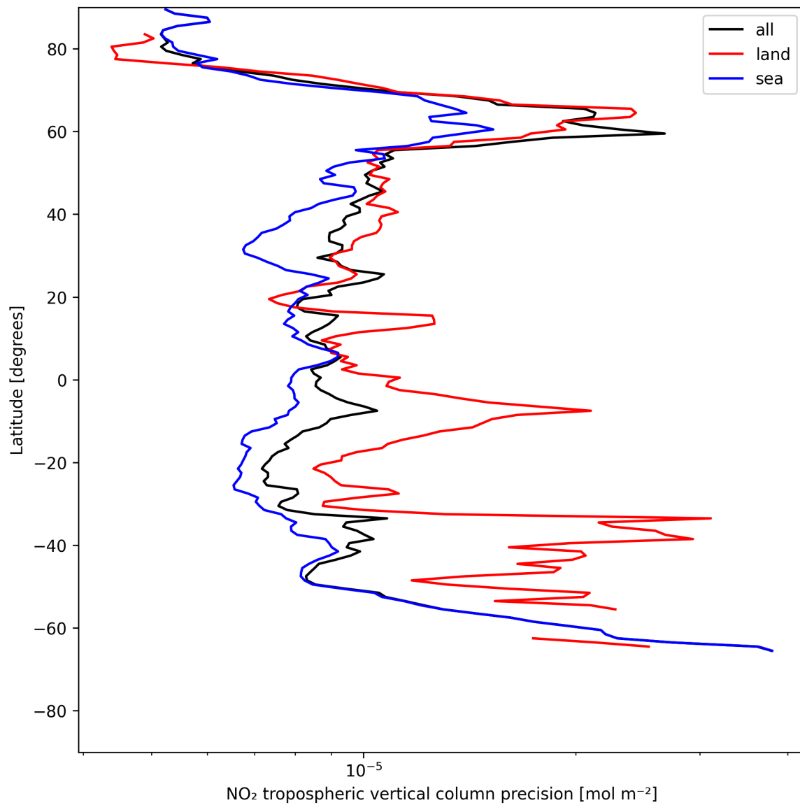
Figure 11: Zonal average of “NO 2 tropospheric vertical column precision” for 2025-07-09 to 2025-07-10.
