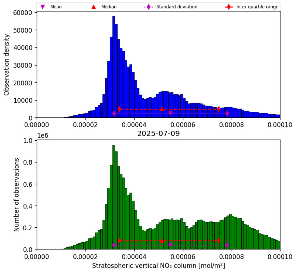
Figure 34: Histogram of “Stratospheric vertical NO 2 column” for 2025-07-09 to 2025-07-10
