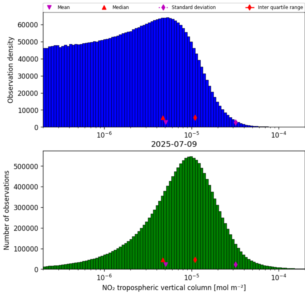
Figure 27: Histogram of “NO 2 tropospheric vertical column” for 2025-07-09 to 2025-07-10
