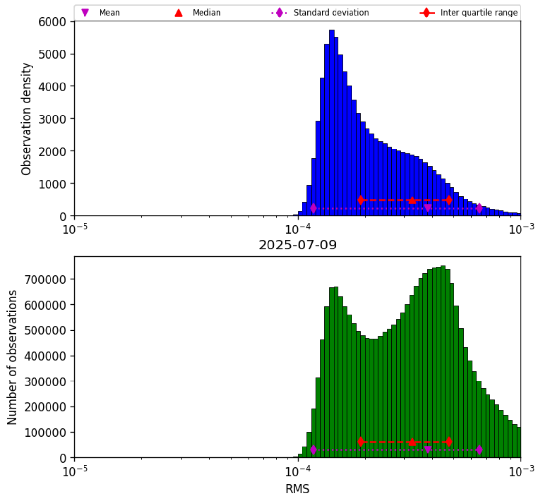
Figure 41: Histogram of “RMS” for 2025-07-09 to 2025-07-10
