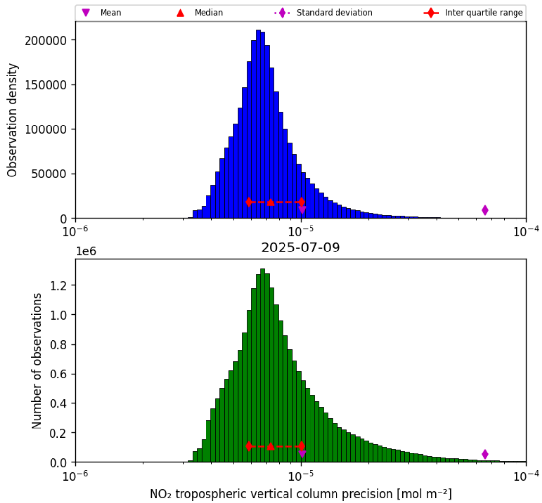
Figure 28: Histogram of “NO 2 tropospheric vertical column precision” for 2025-07-09 to 2025-07-10
