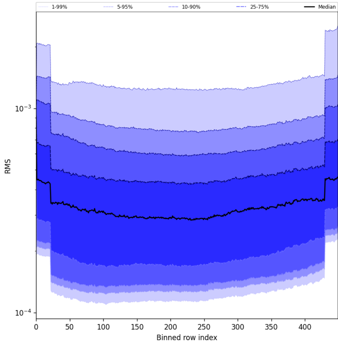
Figure 58: Along track statistics of “RMS” for 2025-07-09 to 2025-07-10
