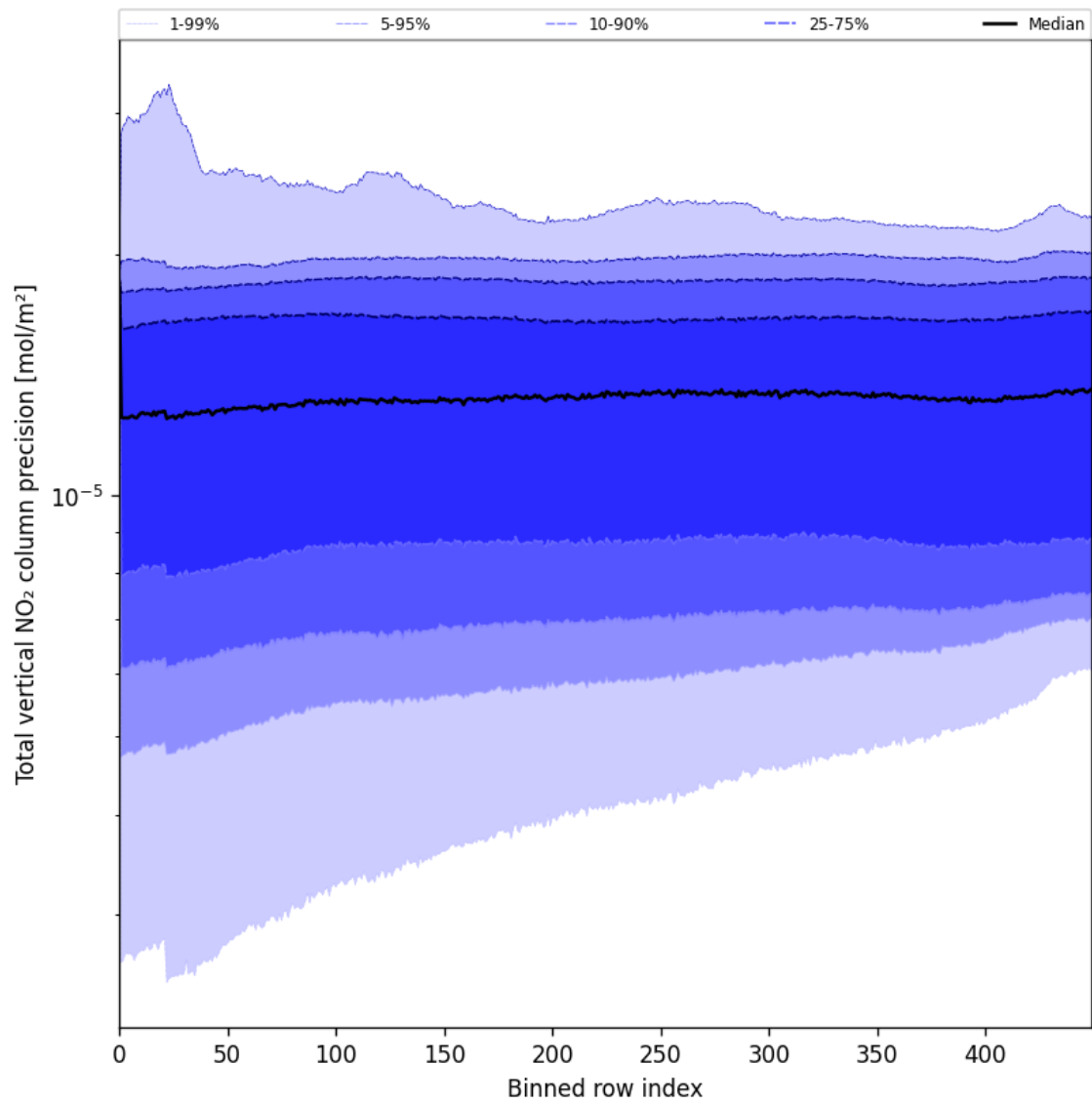
Figure 54: Along track statistics of “Total vertical NO 2 column precision” for 2025-07-09 to 2025-07-10
