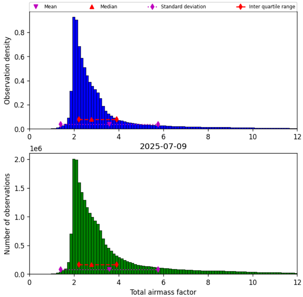
Figure 30: Histogram of “Total airmass factor” for 2025-07-09 to 2025-07-10
