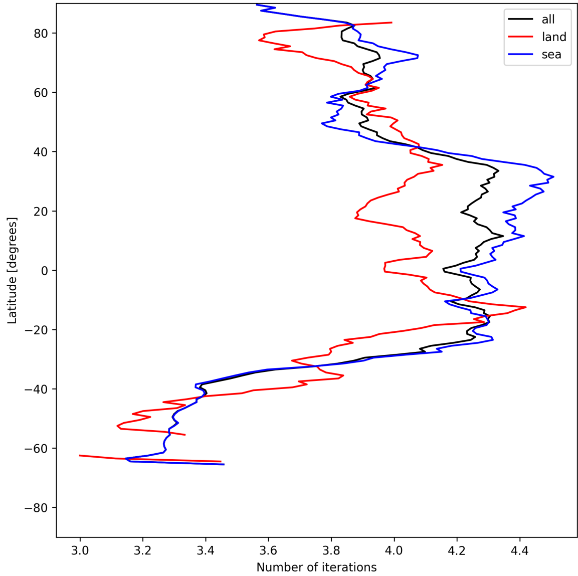
Figure 15: Zonal average of “Number of iterations” for 2025-07-09 to 2025-07-10.
