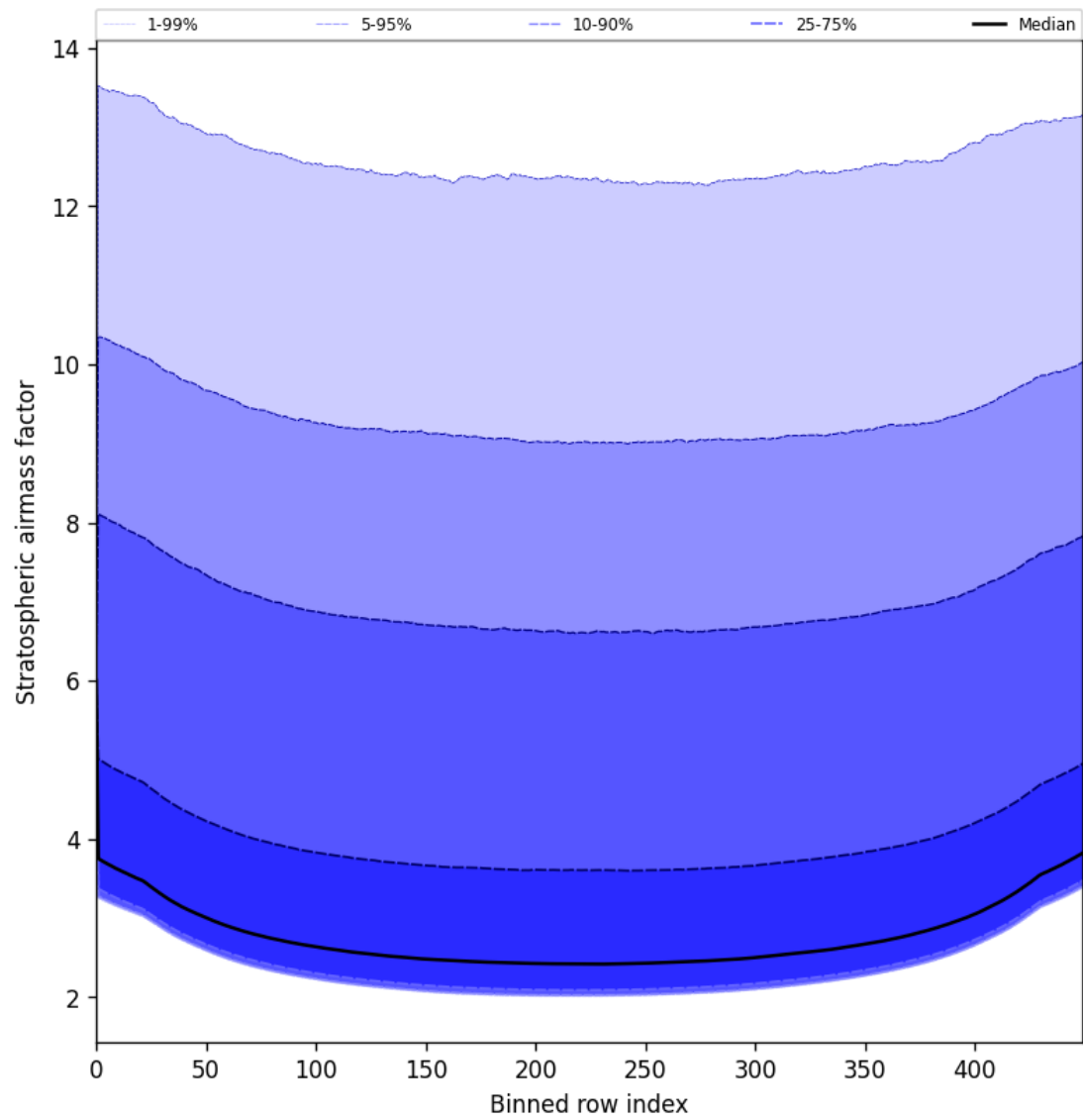
Figure 59: Along track statistics of “Stratospheric airmass factor” for 2025-07-09 to 2025-07-10
