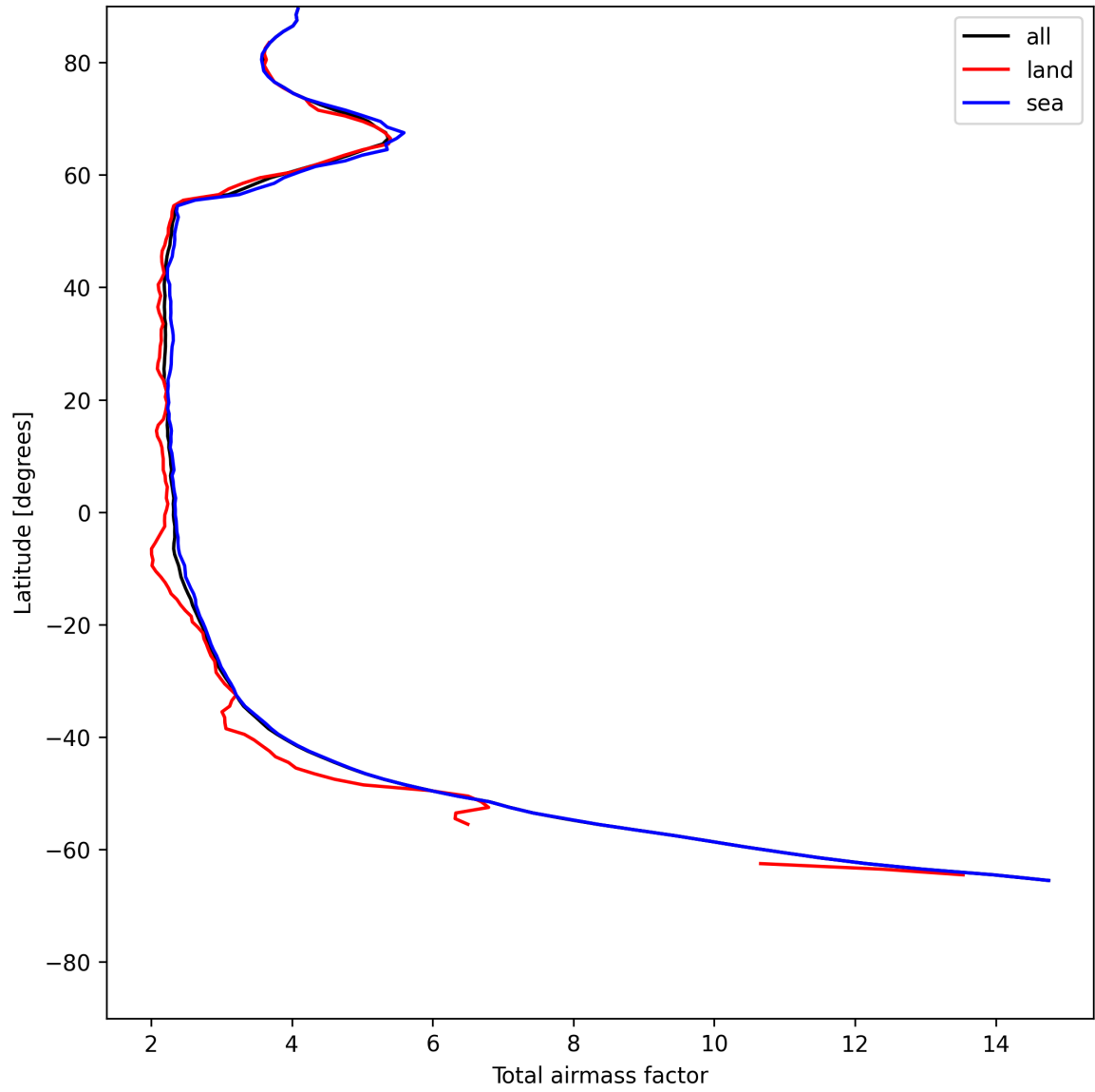
Figure 13: Zonal average of “Total airmass factor” for 2025-07-09 to 2025-07-10.
