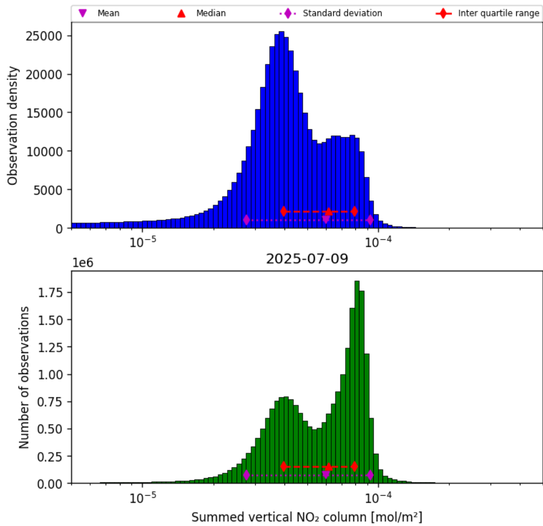
Figure 38: Histogram of “Summed vertical NO 2 column” for 2025-07-09 to 2025-07-10
