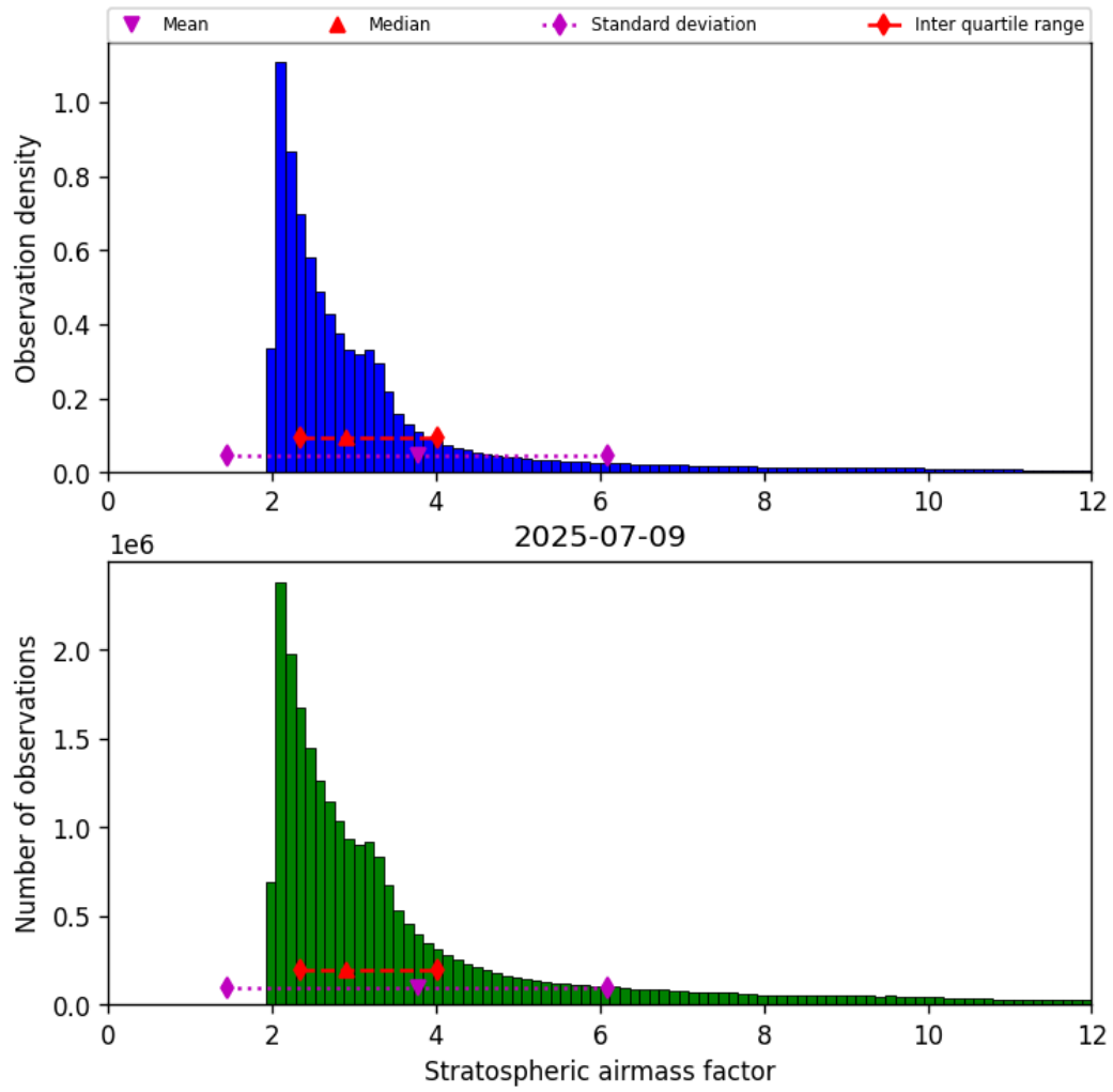
Figure 42: Histogram of “Stratospheric airmass factor” for 2025-07-09 to 2025-07-10
