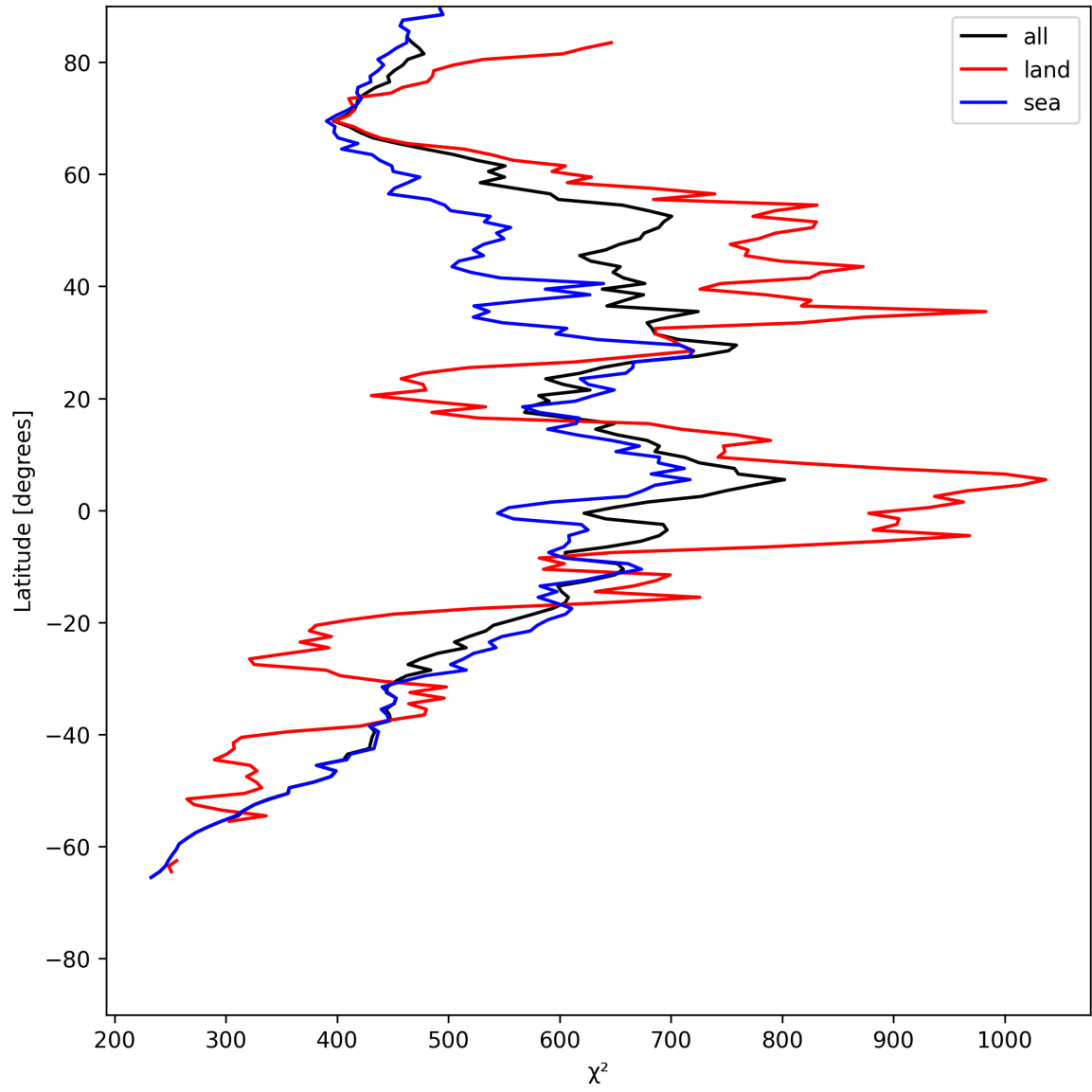
Figure 23: Zonal average of “ \chi^2 ” for 2025-07-09 to 2025-07-10.
