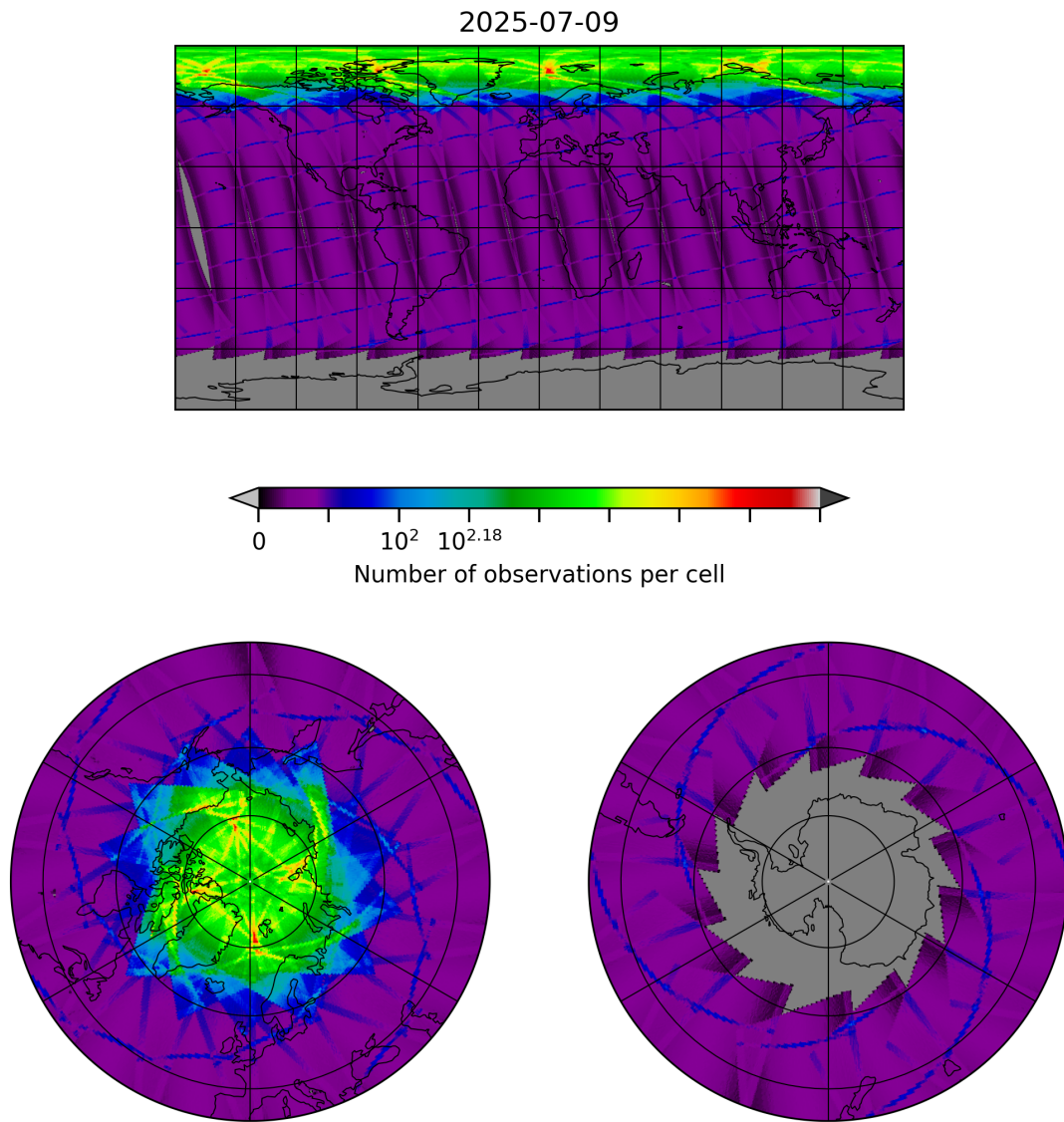
Figure 8: Map of the number of observations for 2025-07-09 to 2025-07-10
