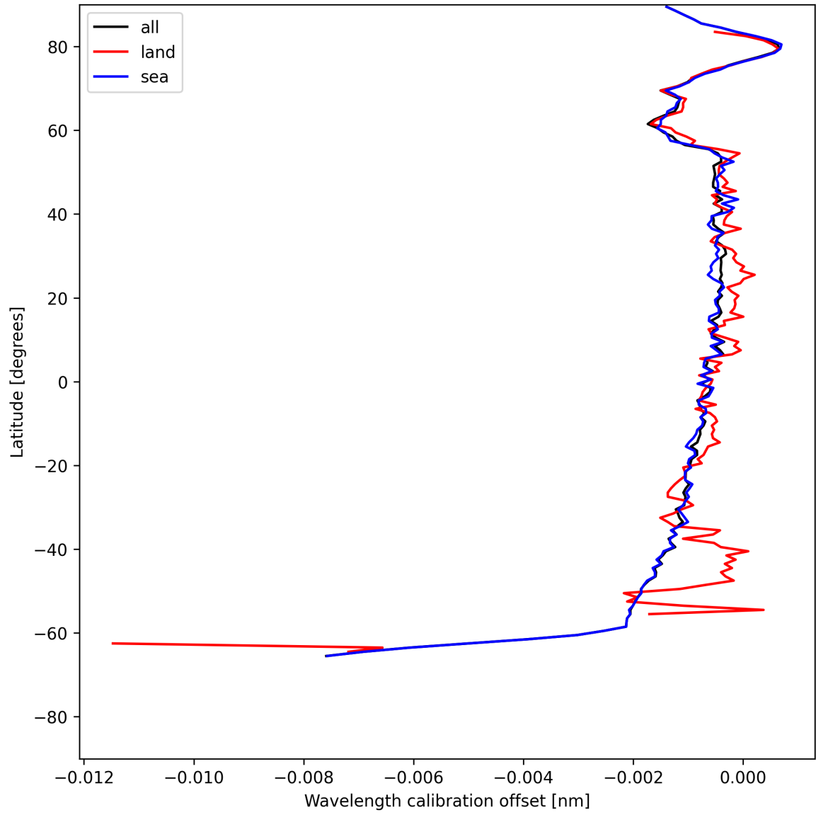
Figure 16: Zonal average of “Wavelength calibration offset” for 2025-07-09 to 2025-07-10.
