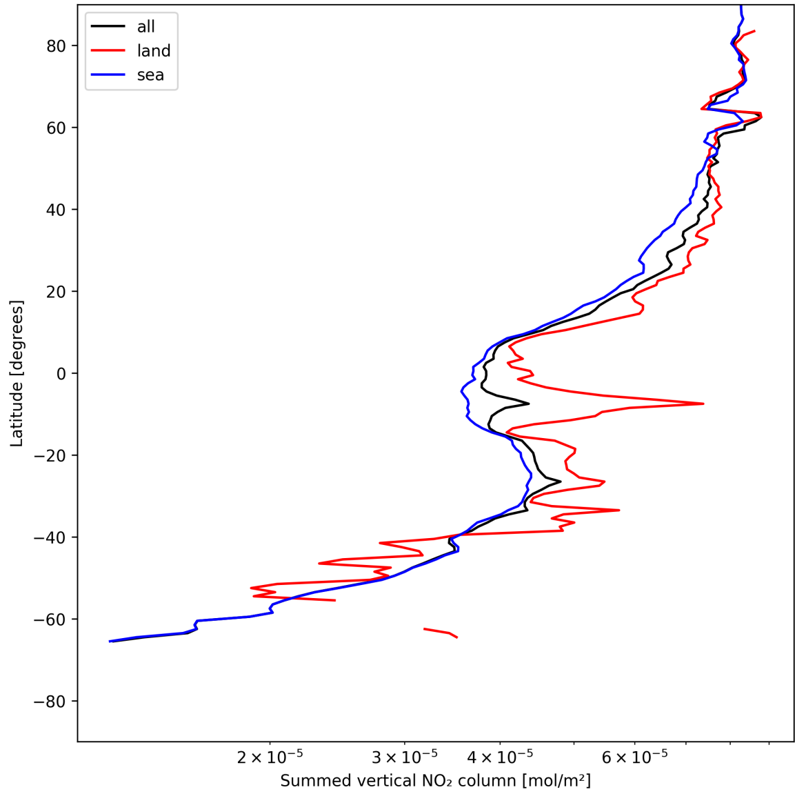
Figure 21: Zonal average of “Summed vertical NO 2 column” for 2025-07-09 to 2025-07-10.
