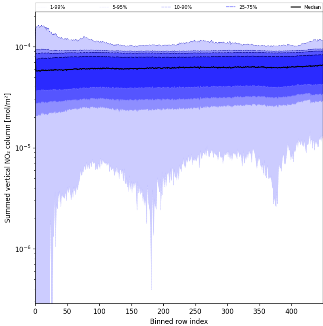
Figure 55: Along track statistics of “Summed vertical NO 2 column” for 2025-07-09 to 2025-07-10
