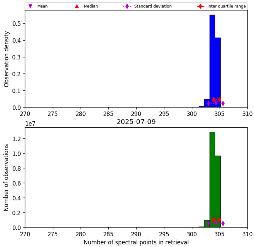
Figure 31: Histogram of “Number of spectral points in retrieval” for 2025-07-09 to 2025-07-10
