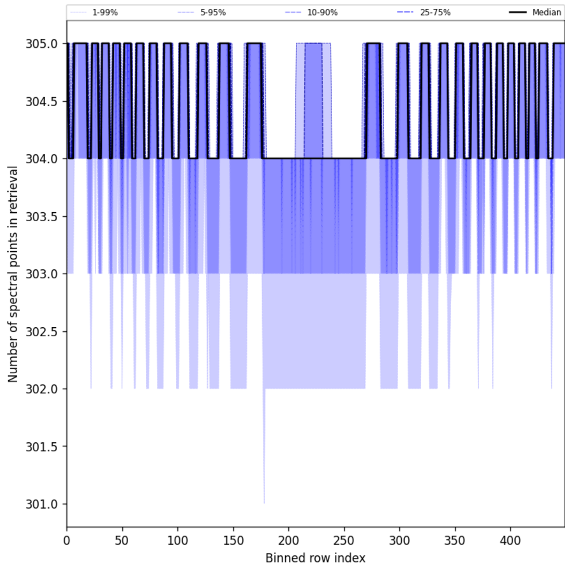
Figure 48: Along track statistics of “Number of spectral points in retrieval” for 2025-07-09 to 2025-07-10
