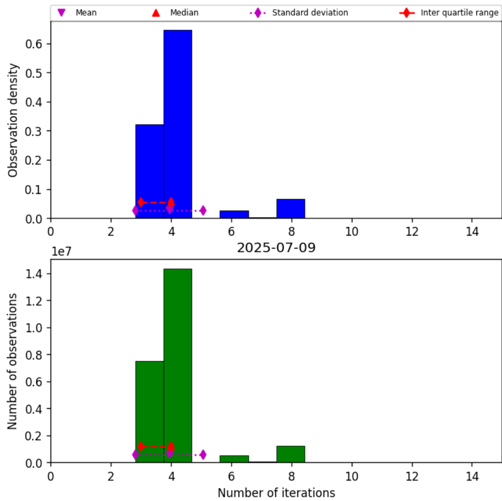
Figure 32: Histogram of “Number of iterations” for 2025-07-09 to 2025-07-10
