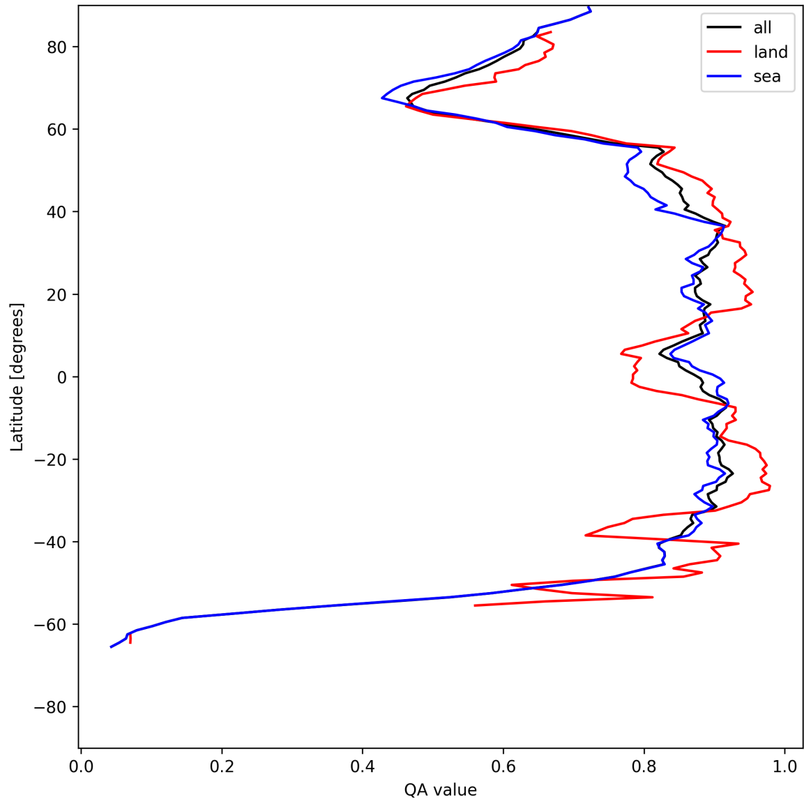
Figure 9: Zonal average of “QA value” for 2025-07-09 to 2025-07-10.
