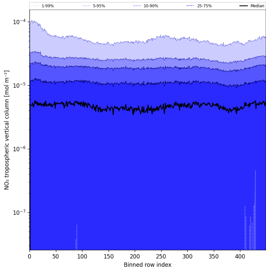
Figure 44: Along track statistics of “NO 2 tropospheric vertical column” for 2025-07-09 to 2025-07-10
