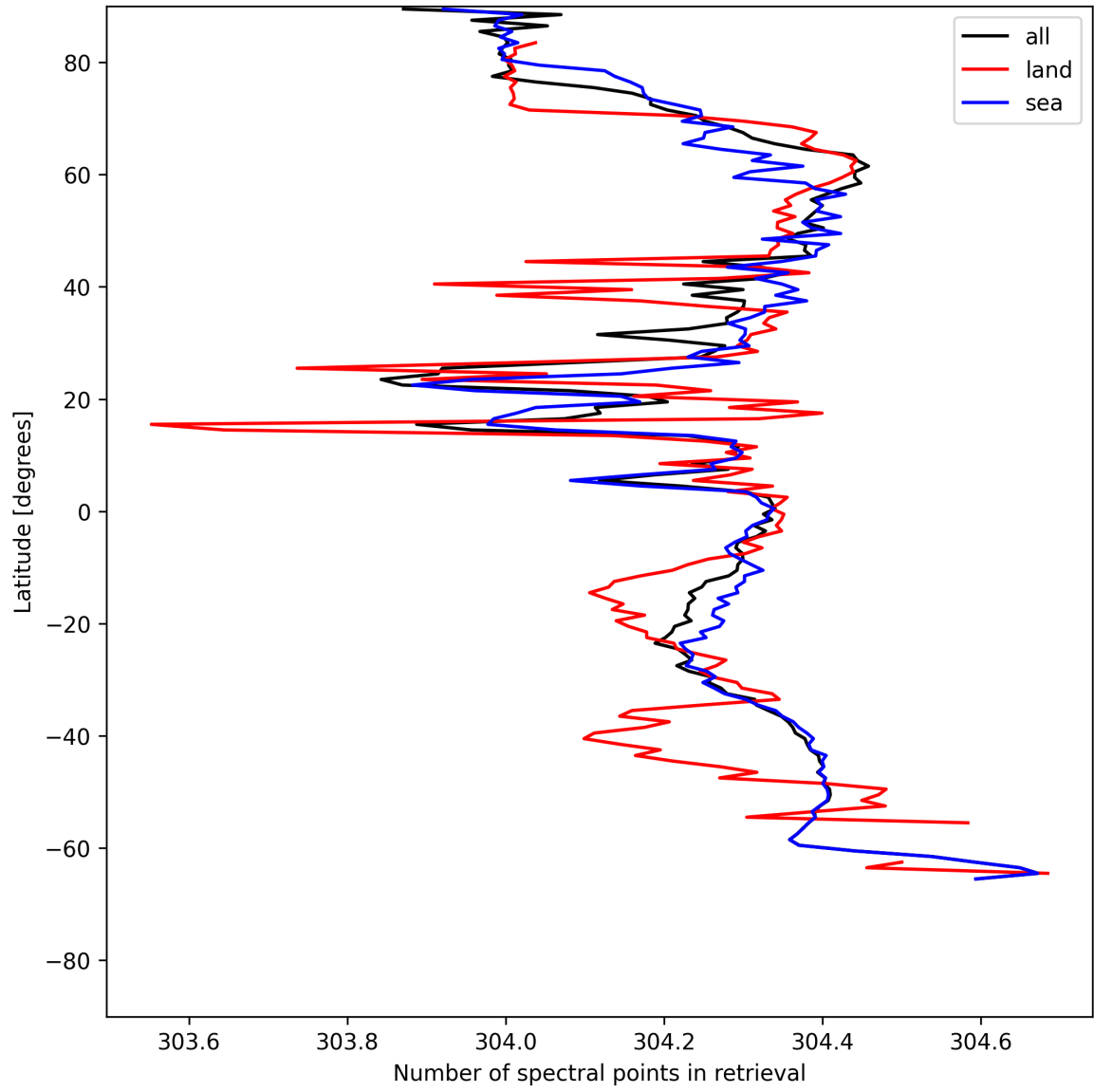
Figure 14: Zonal average of “Number of spectral points in retrieval” for 2025-07-09 to 2025-07-10.
