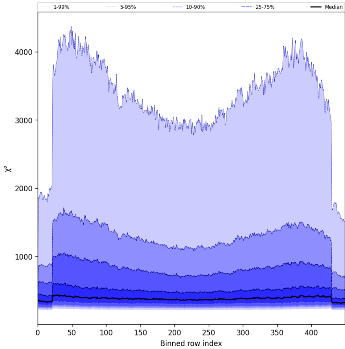
Figure 57: Along track statistics of “ \chi^2 ” for 2025-07-09 to 2025-07-10
