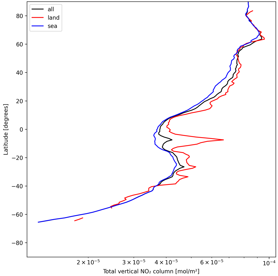
Figure 19: Zonal average of “Total vertical NO 2 column” for 2025-07-09 to 2025-07-10.
