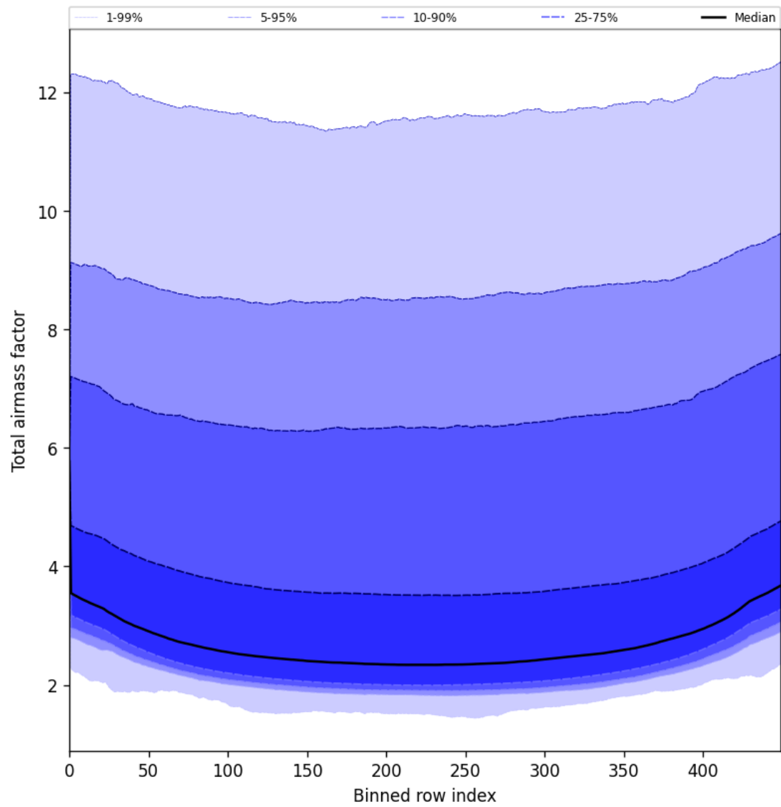
Figure 47: Along track statistics of “Total airmass factor” for 2025-07-09 to 2025-07-10
