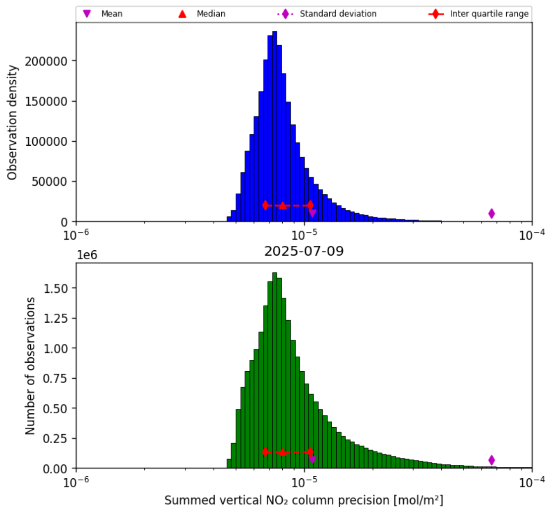
Figure 39: Histogram of “Summed vertical NO 2 column precision” for 2025-07-09 to 2025-07-10
