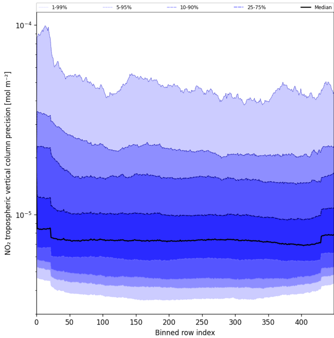
Figure 45: Along track statistics of “NO 2 tropospheric vertical column precision” for 2025-07-09 to 2025-07-10
