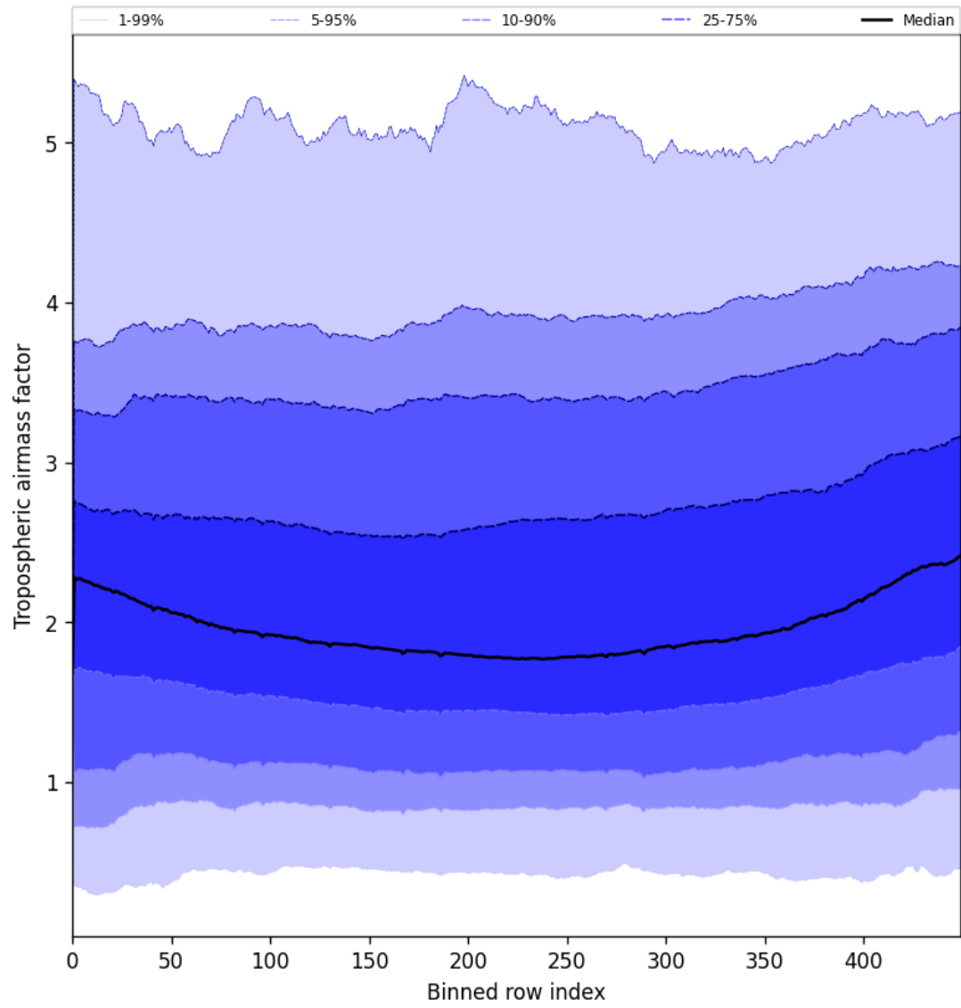
Figure 46: Along track statistics of “Tropospheric airmass factor” for 2025-07-09 to 2025-07-10
