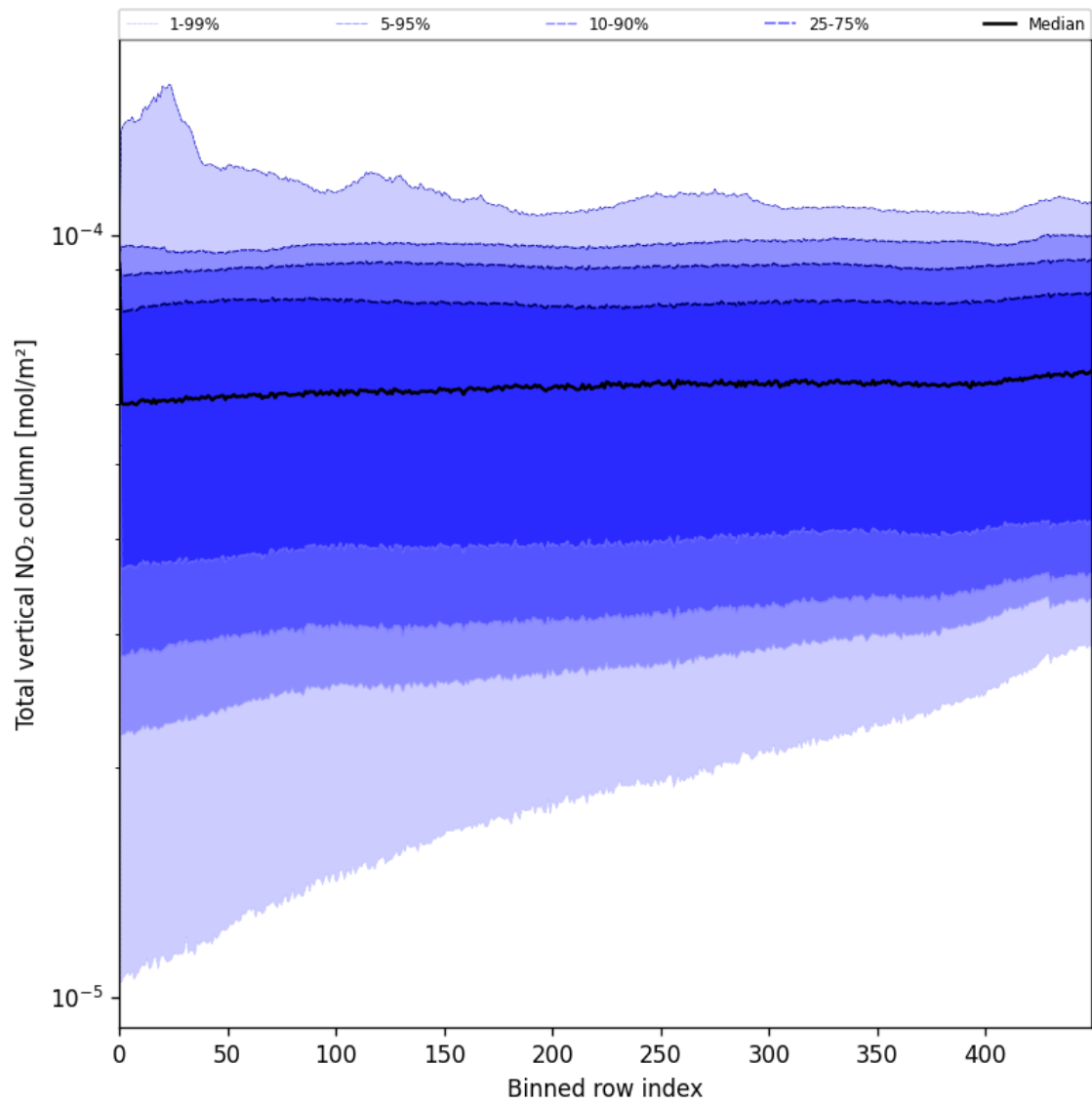
Figure 53: Along track statistics of “Total vertical NO 2 column” for 2025-07-09 to 2025-07-10
