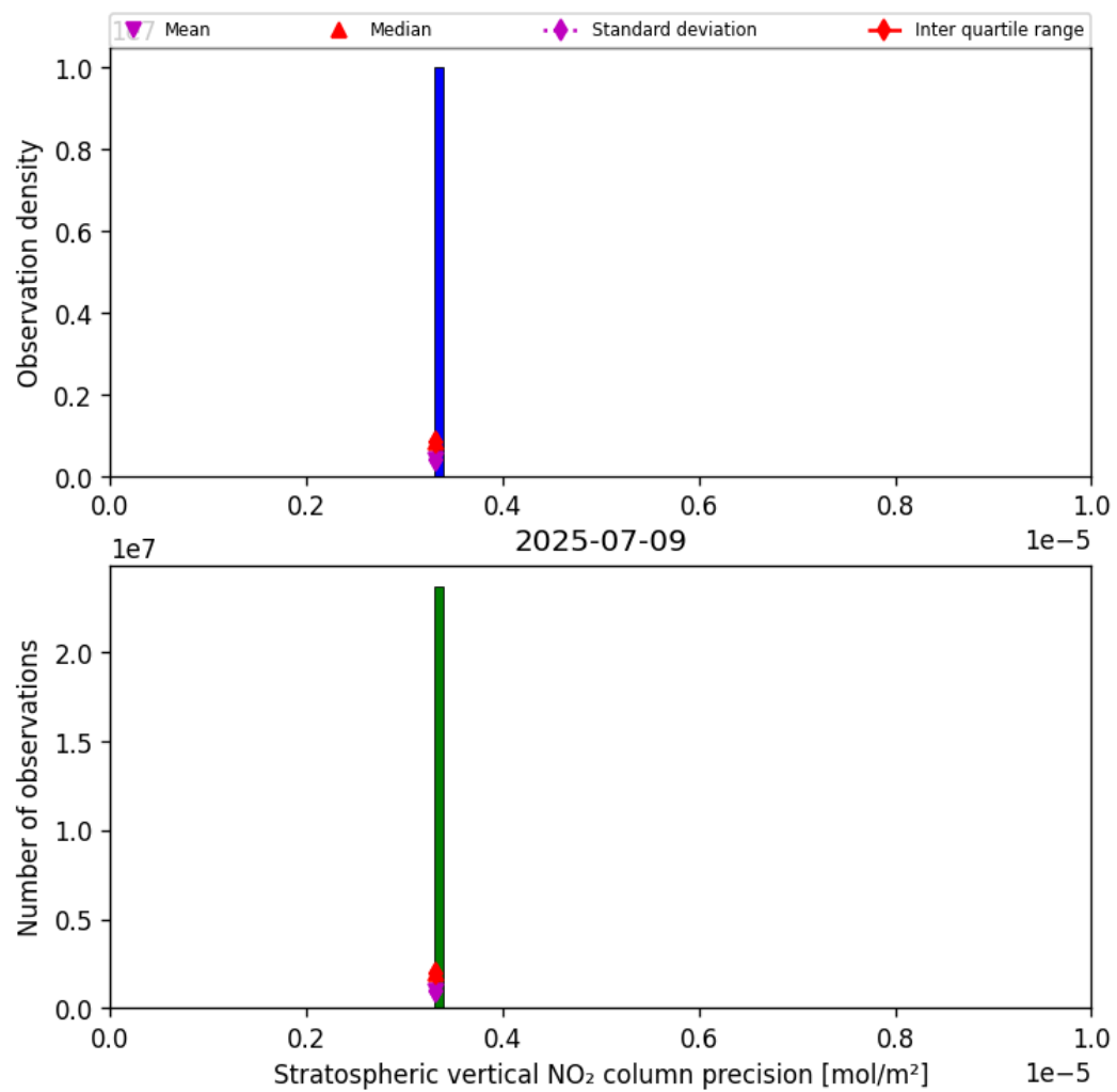
Figure 35: Histogram of “Stratospheric vertical NO 2 column precision” for 2025-07-09 to 2025-07-10
