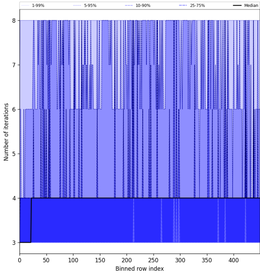
Figure 49: Along track statistics of “Number of iterations” for 2025-07-09 to 2025-07-10
