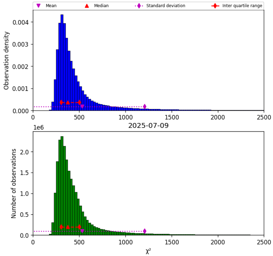
Figure 40: Histogram of “ \chi^2 ” for 2025-07-09 to 2025-07-10
