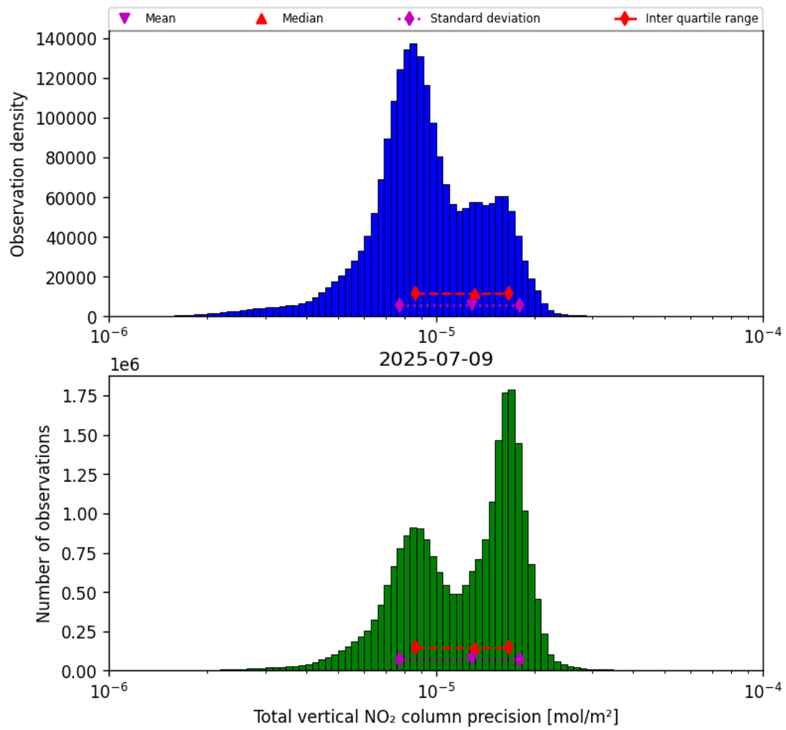
Figure 37: Histogram of “Total vertical NO 2 column precision” for 2025-07-09 to 2025-07-10
