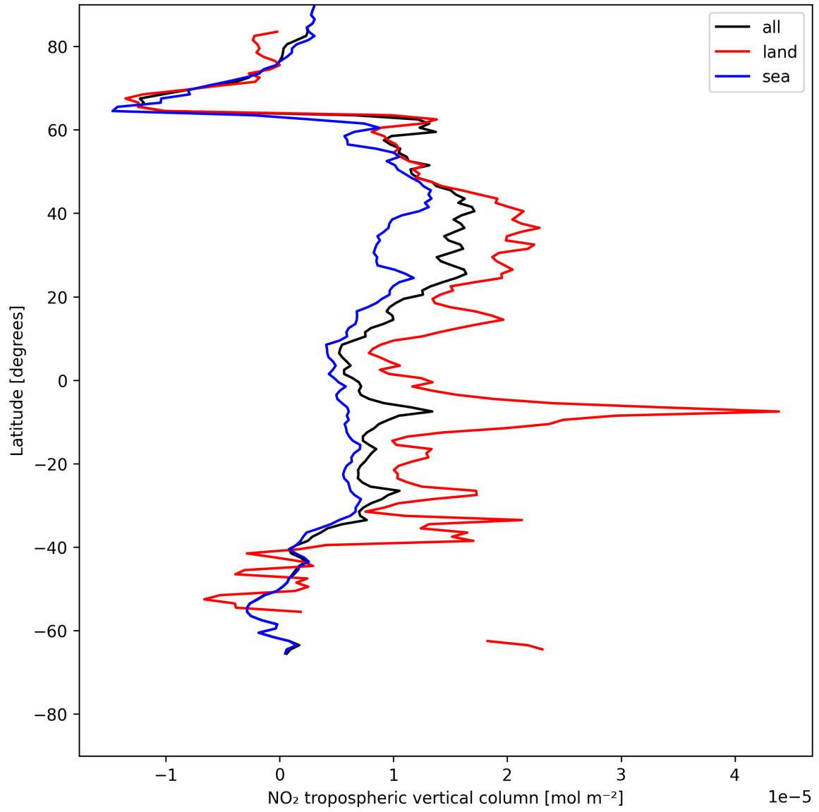
Figure 10: Zonal average of “NO 2 tropospheric vertical column” for 2025-07-09 to 2025-07-10.
