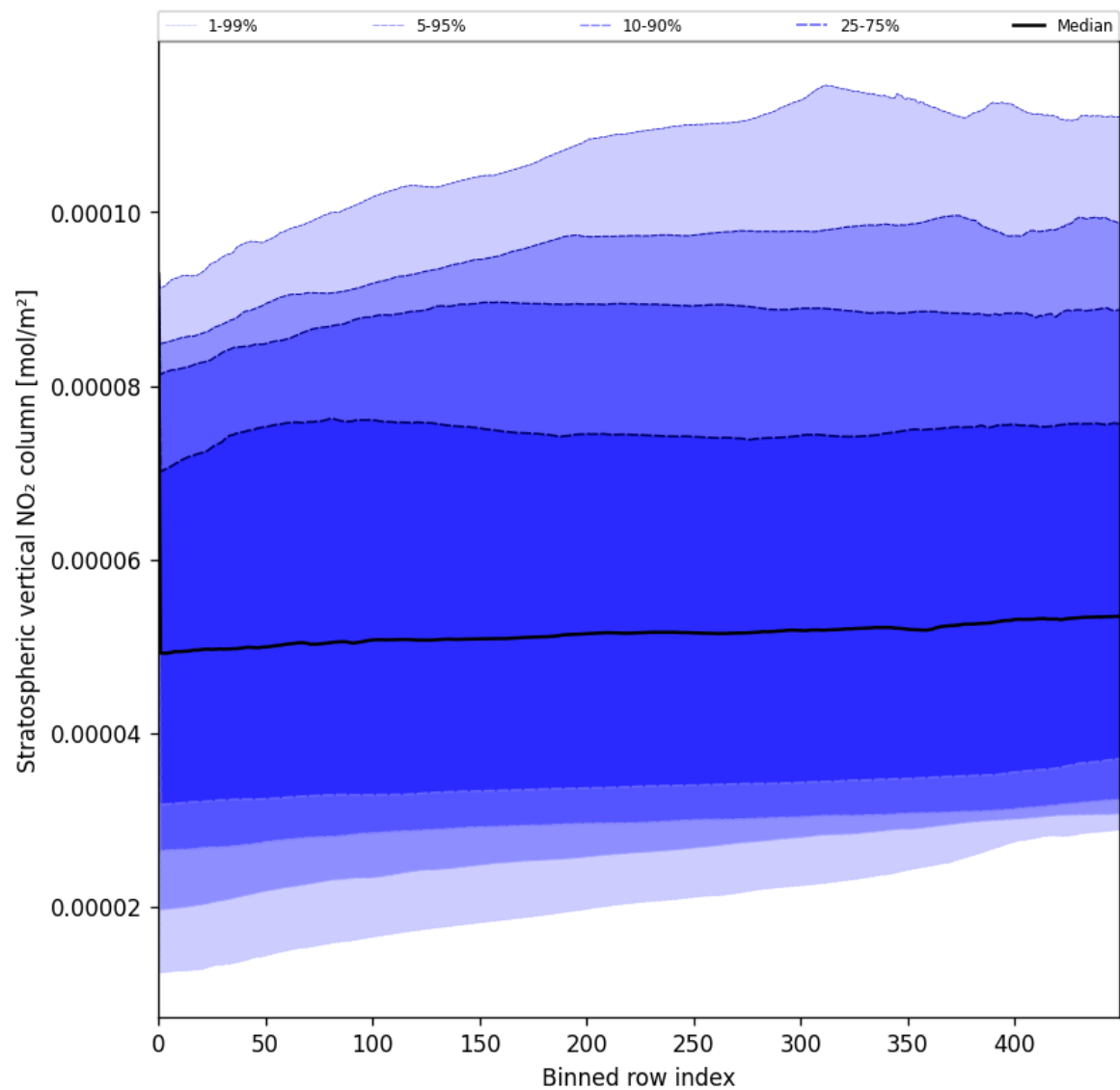
Figure 51: Along track statistics of “Stratospheric vertical NO 2 column” for 2025-07-09 to 2025-07-10
