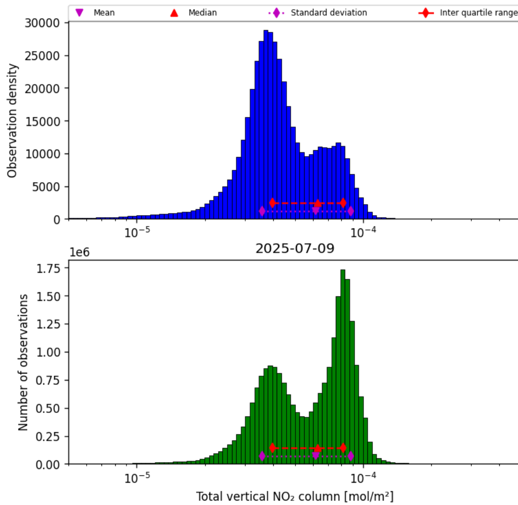
Figure 36: Histogram of "Total vertical NO 2 column" for 2025-07-09 to 2025-07-10
