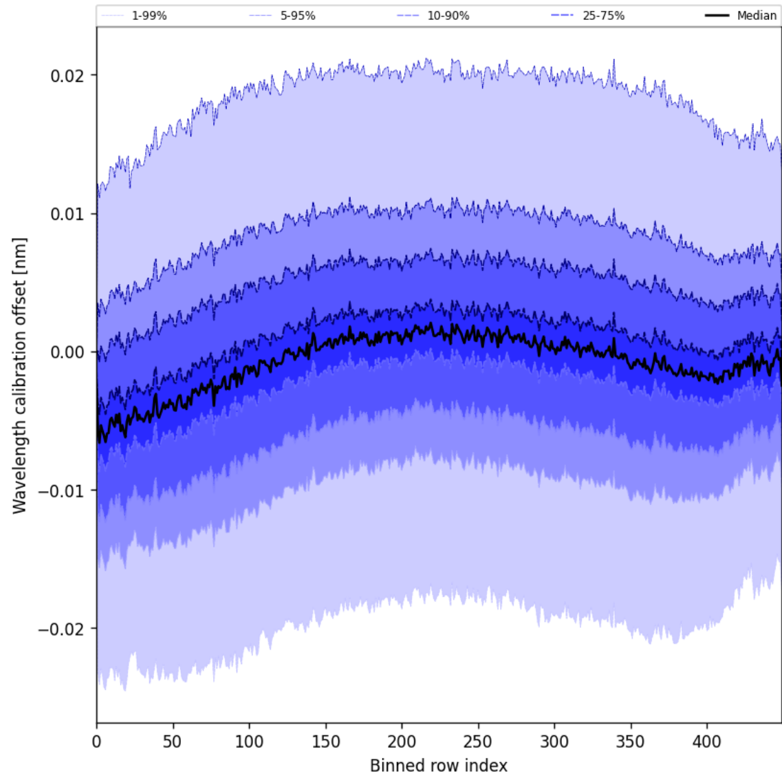
Figure 50: Along track statistics of “Wavelength calibration offset” for 2025-07-09 to 2025-07-10
