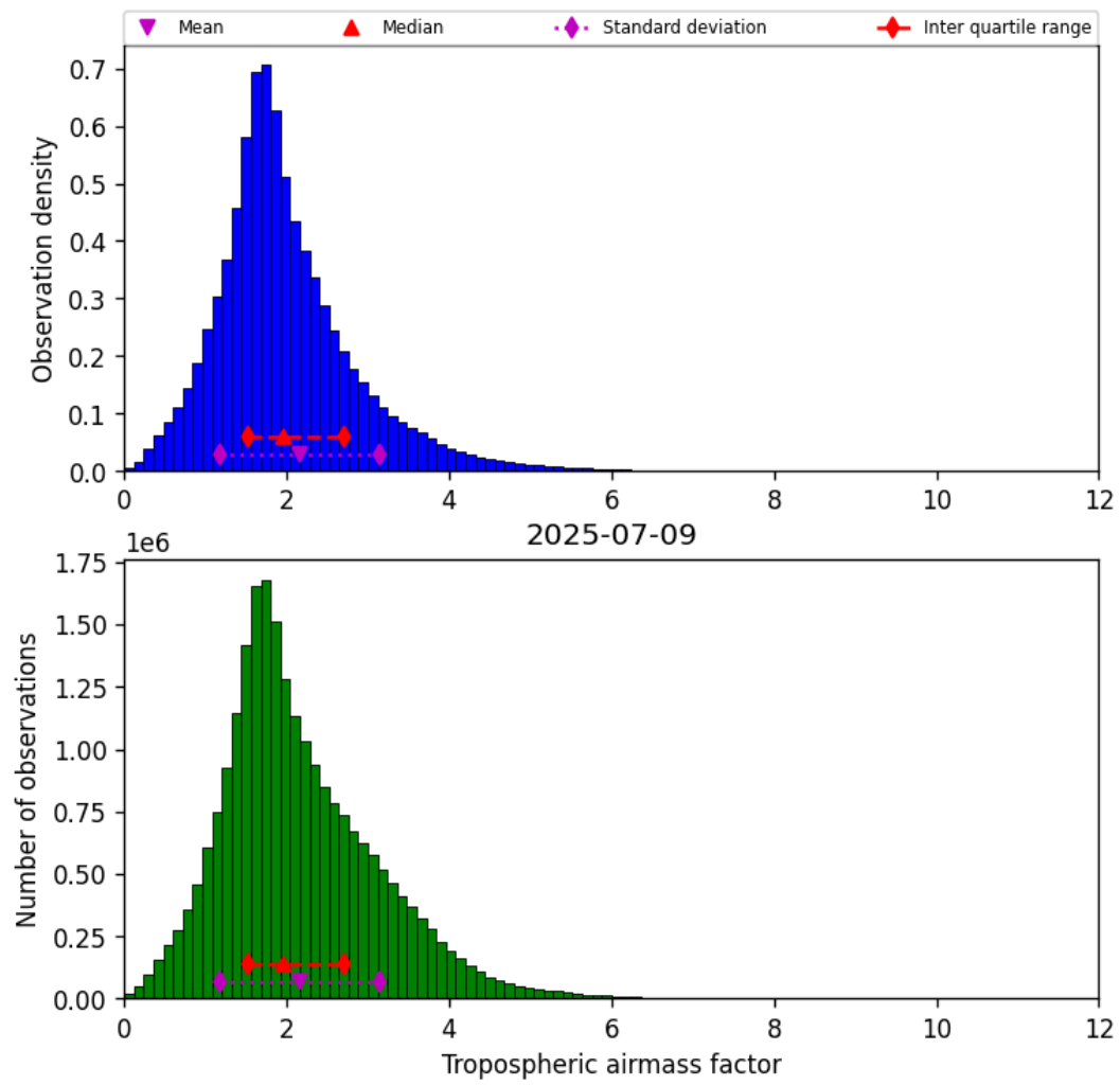
Figure 29: Histogram of “Tropospheric airmass factor” for 2025-07-09 to 2025-07-10
