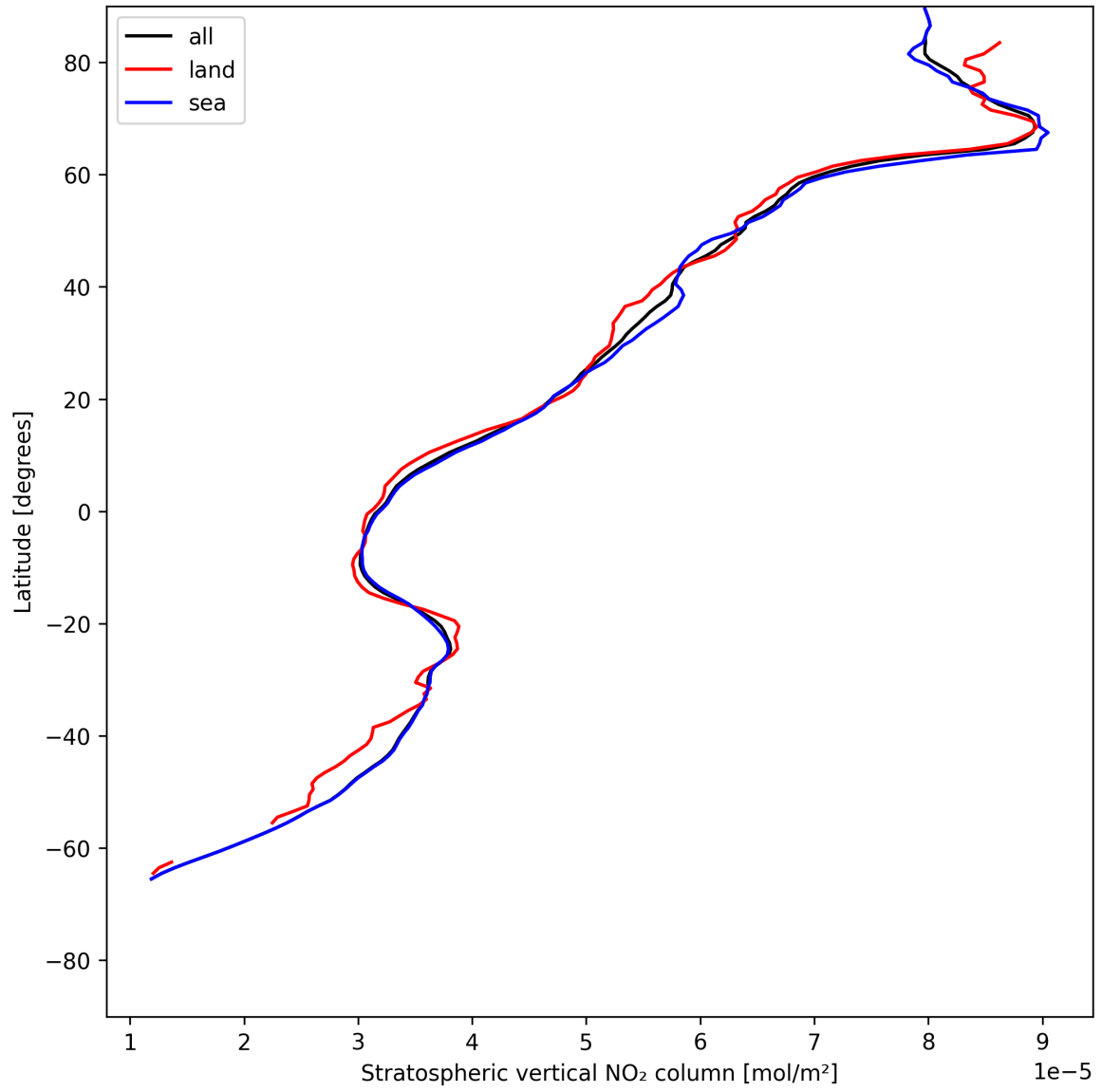
Figure 17: Zonal average of “Stratospheric vertical NO 2 column” for 2025-07-09 to 2025-07-10.
