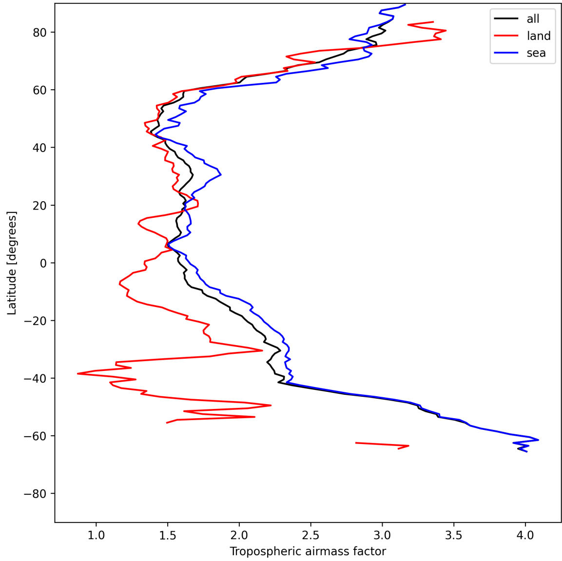
Figure 12: Zonal average of “Tropospheric airmass factor” for 2025-07-09 to 2025-07-10.
