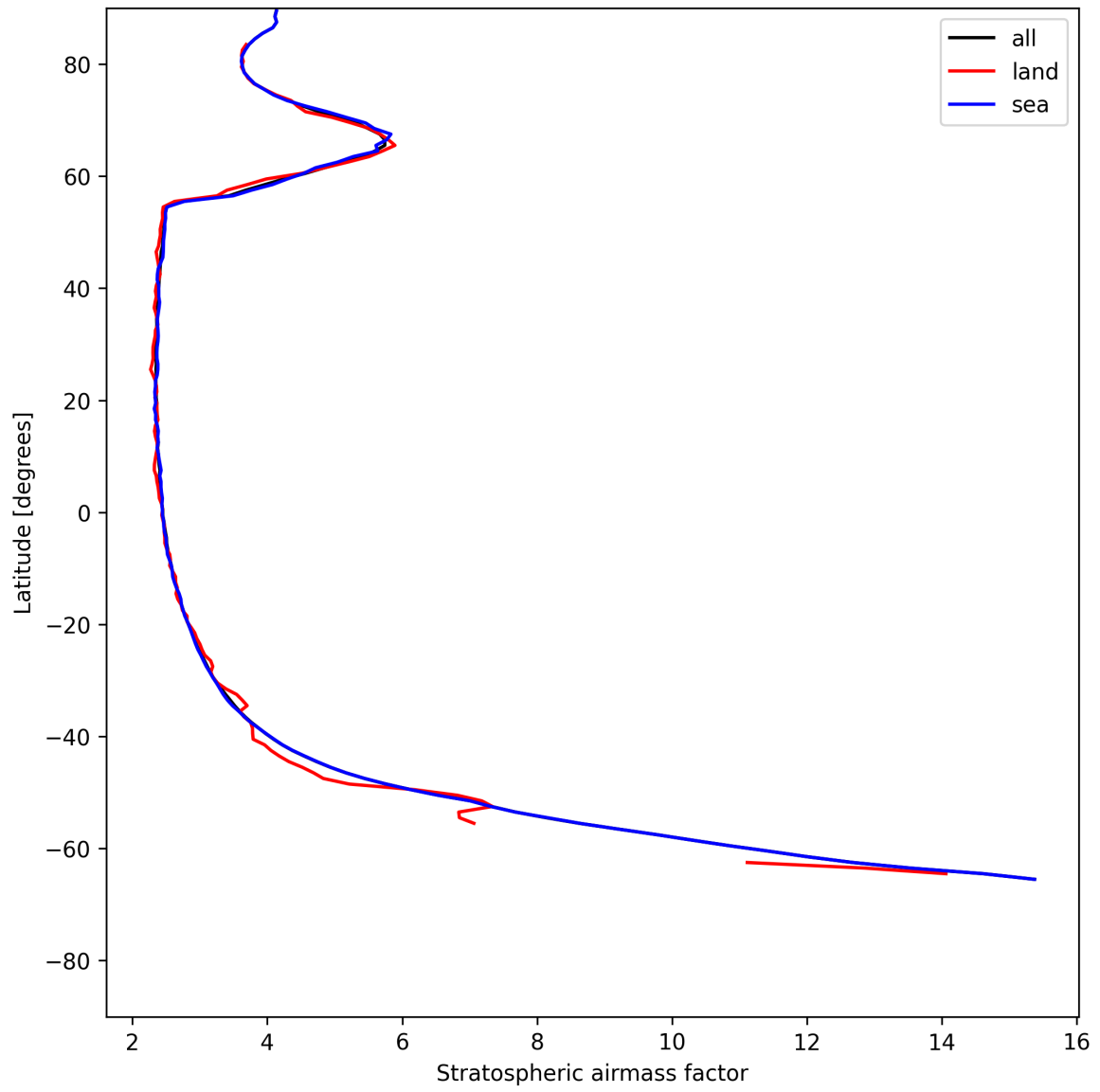
Figure 25: Zonal average of “Stratospheric airmass factor” for 2025-07-09 to 2025-07-10.
