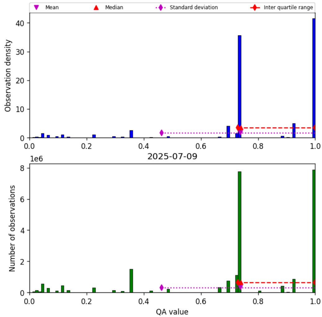
Figure 26: Histogram of “QA value” for 2025-07-09 to 2025-07-10
