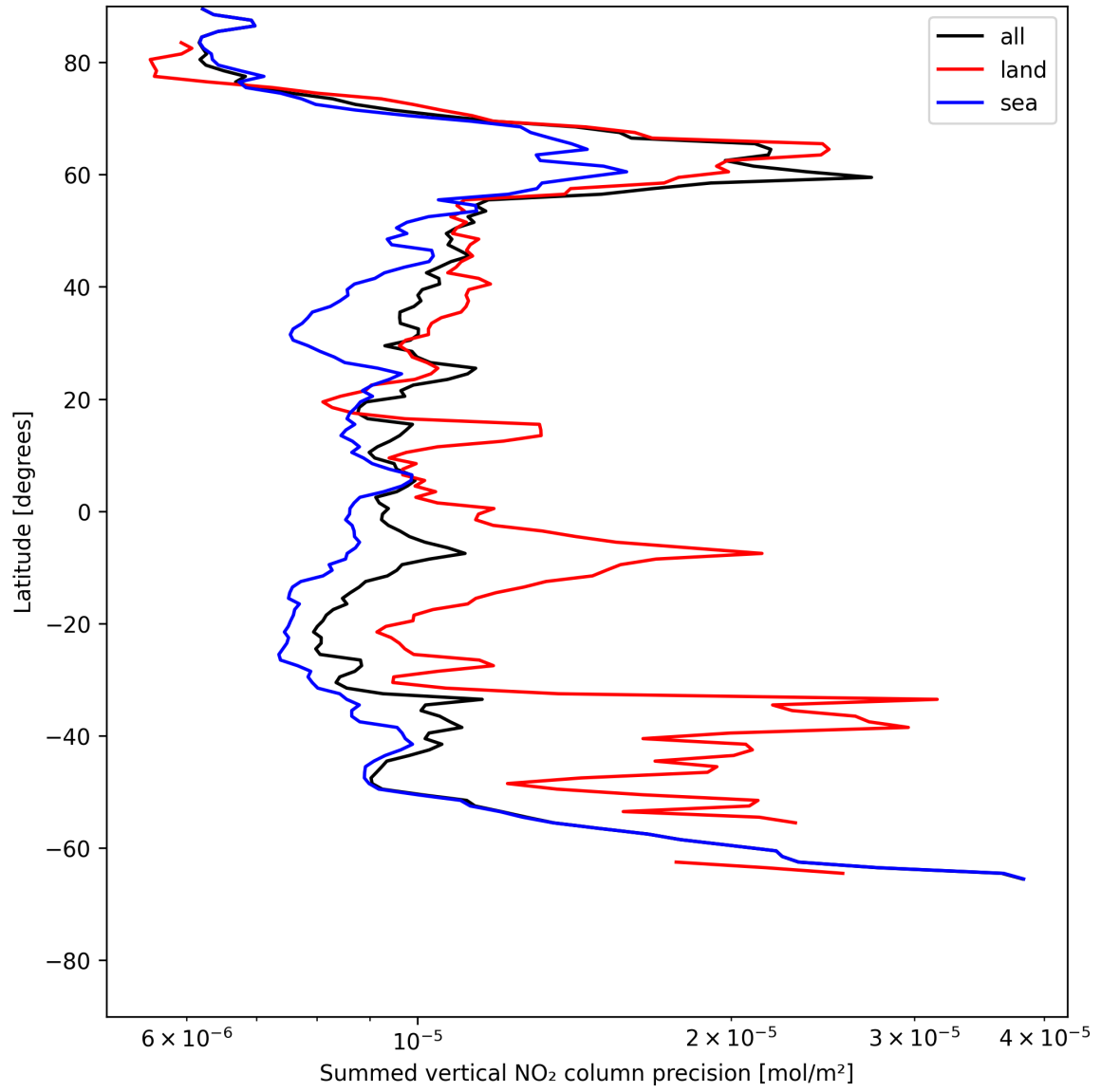
Figure 22: Zonal average of “Summed vertical NO 2 column precision” for 2025-07-09 to 2025-07-10.
