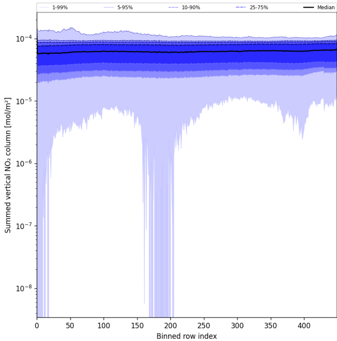
Figure 55: Along track statistics of “Summed vertical NO 2 column” for 2025-07-10 to 2025-07-11
