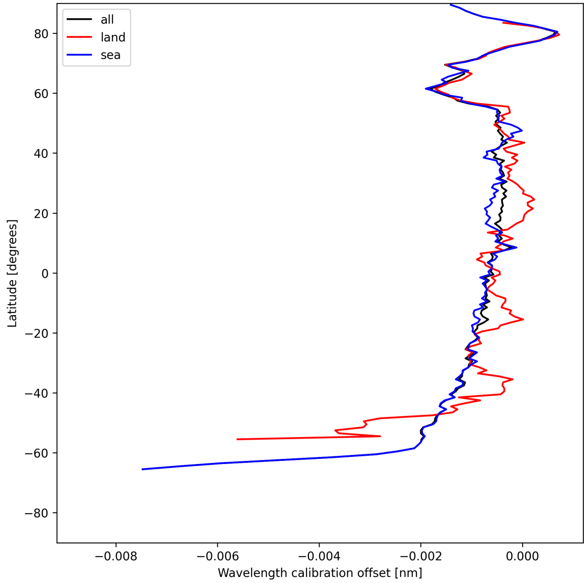
Figure 16: Zonal average of “Wavelength calibration offset” for 2025-07-10 to 2025-07-11.
