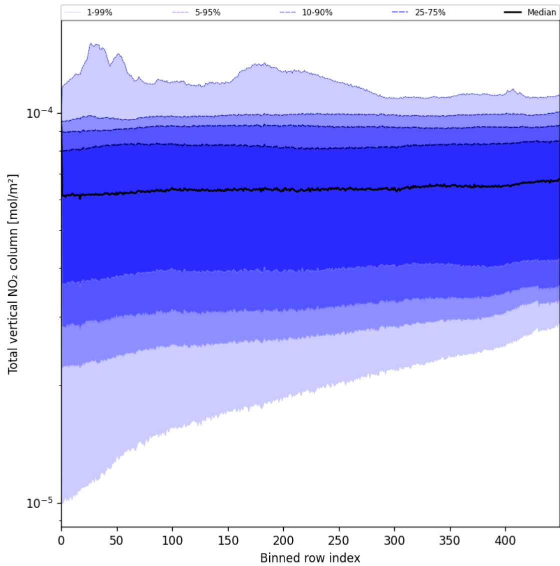
Figure 53: Along track statistics of “Total vertical NO 2 column” for 2025-07-10 to 2025-07-11
