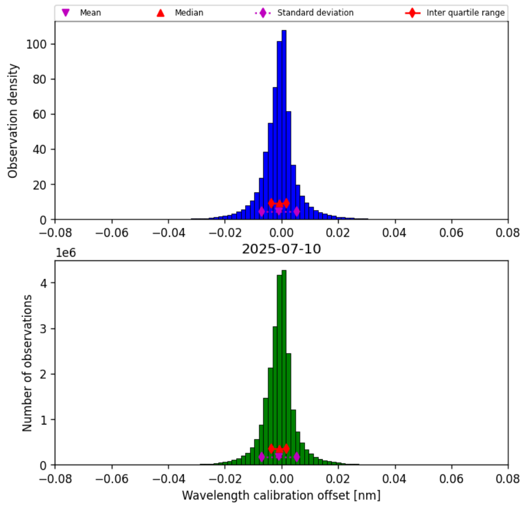
Figure 33: Histogram of “Wavelength calibration offset” for 2025-07-10 to 2025-07-11
