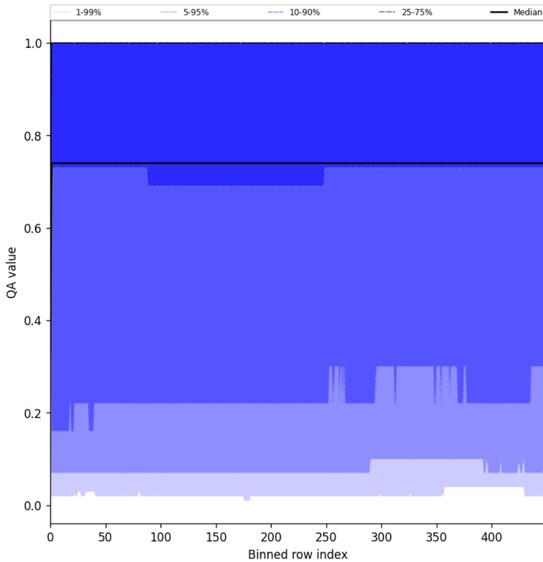
Figure 43: Along track statistics of “QA value” for 2025-07-10 to 2025-07-11
