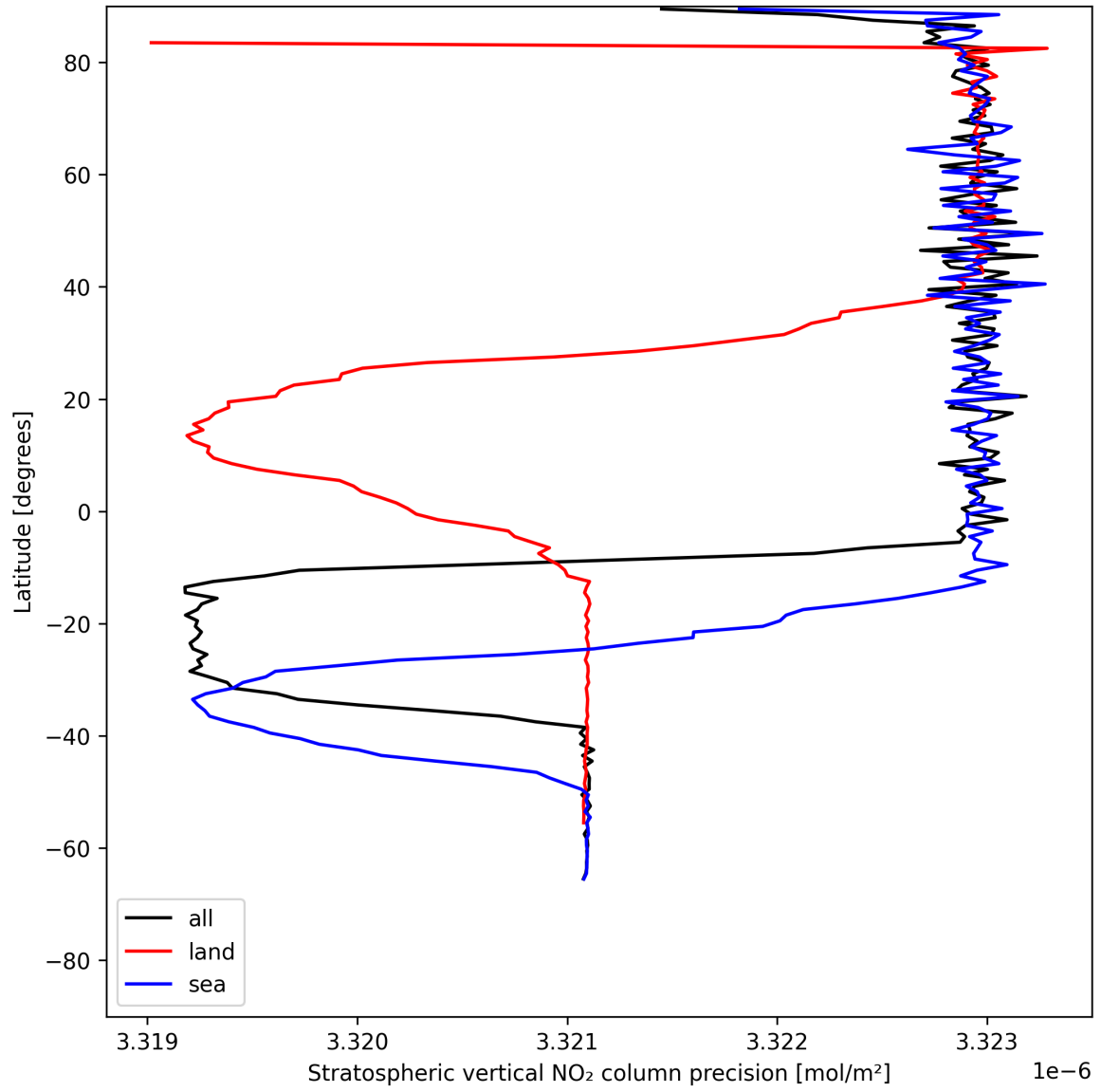
Figure 18: Zonal average of “Stratospheric vertical NO 2 column precision” for 2025-07-10 to 2025-07-11.
