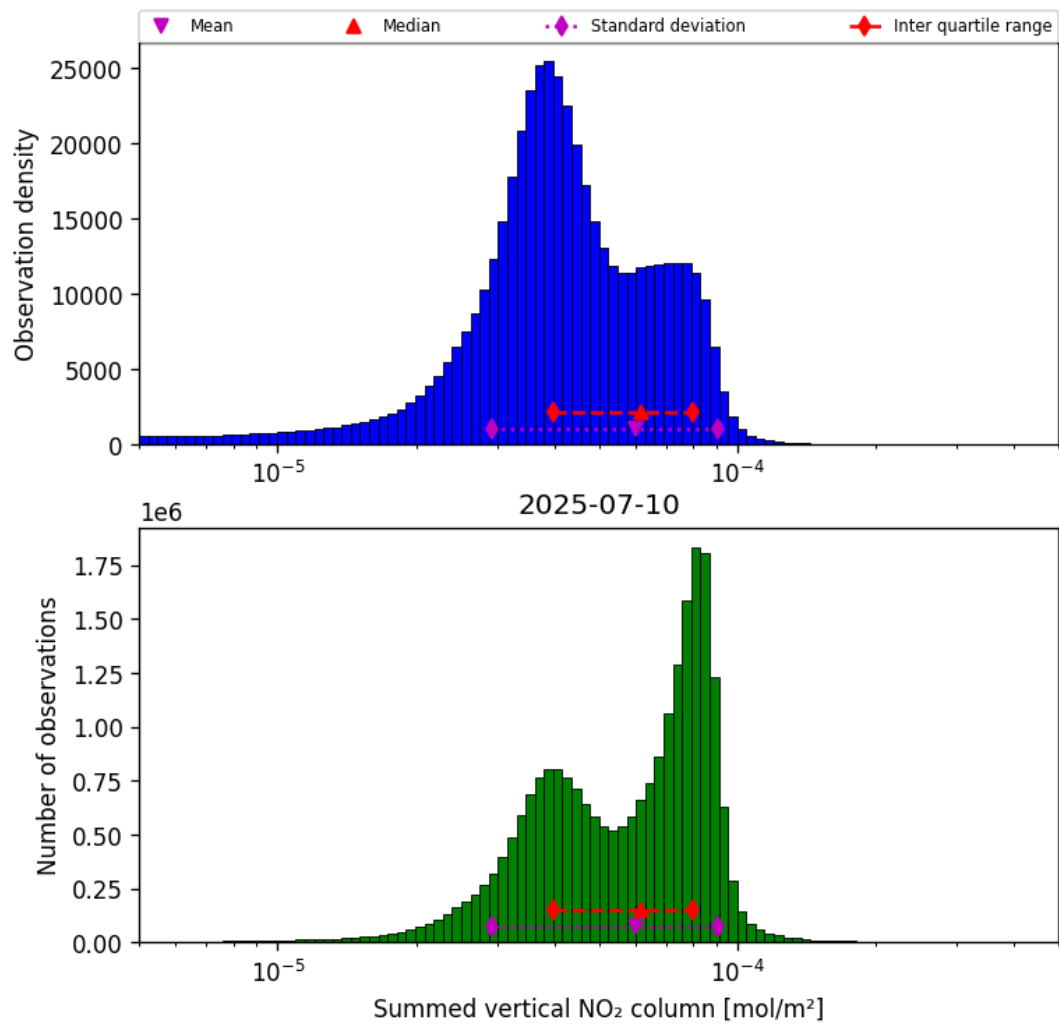
Figure 38: Histogram of “Summed vertical NO 2 column” for 2025-07-10 to 2025-07-11
