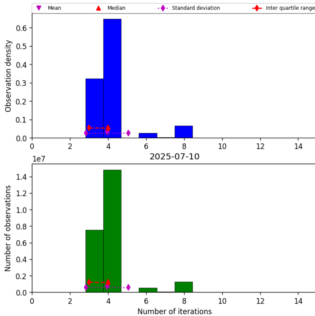
Figure 32: Histogram of “Number of iterations” for 2025-07-10 to 2025-07-11
