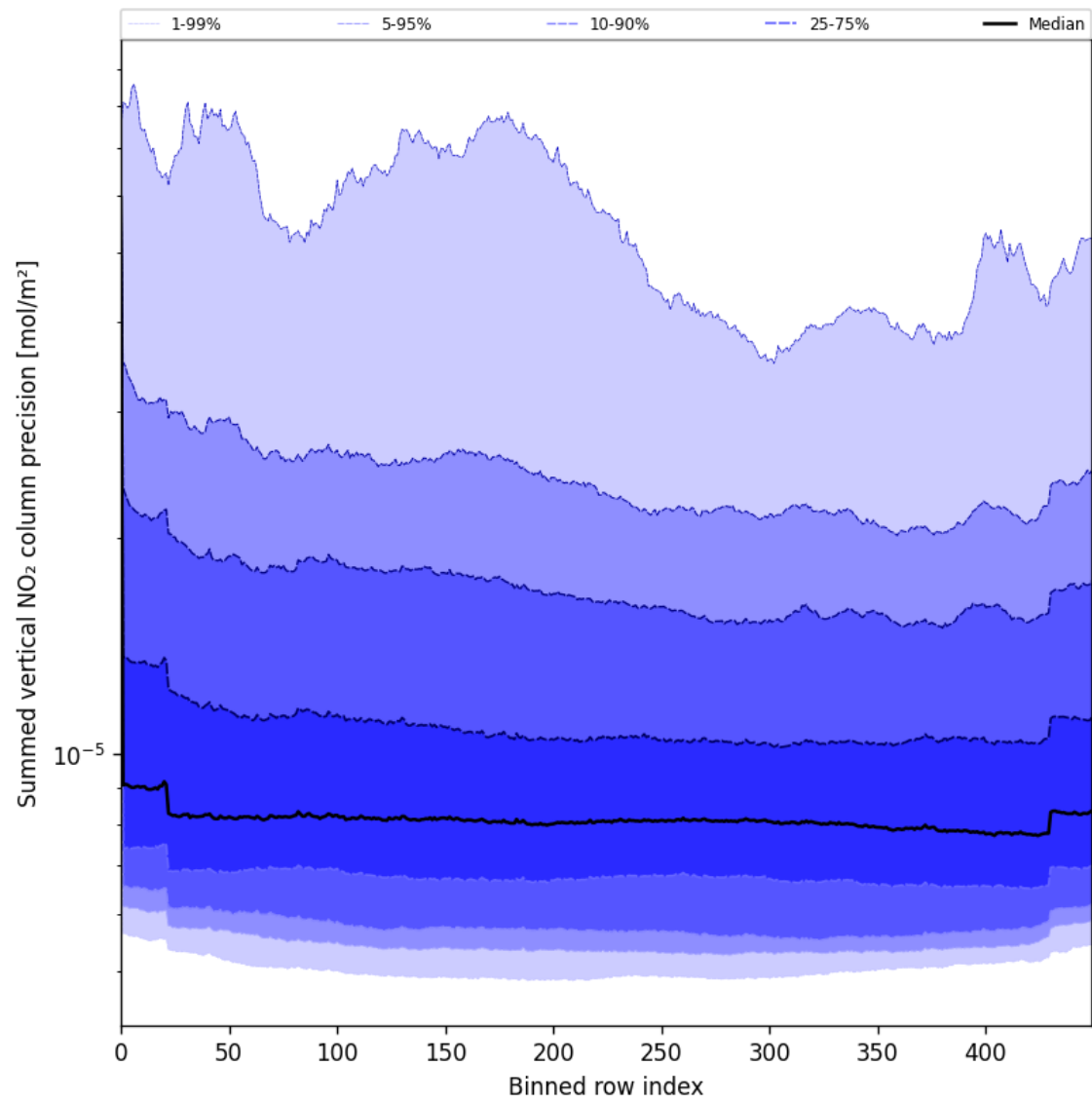
Figure 56: Along track statistics of “Summed vertical NO 2 column precision” for 2025-07-10 to 2025-07-11
