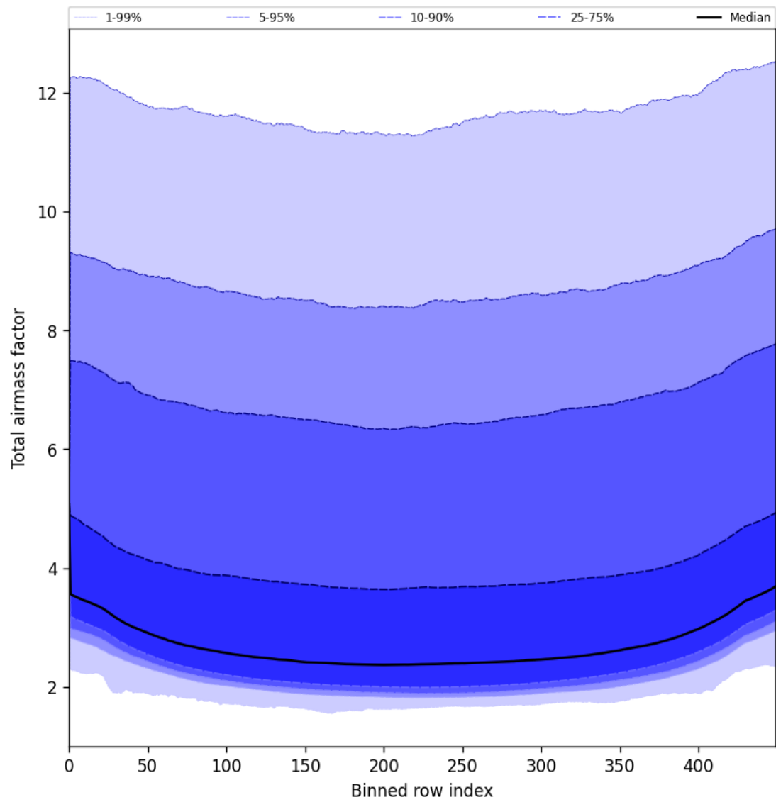
Figure 47: Along track statistics of “Total airmass factor” for 2025-07-10 to 2025-07-11
