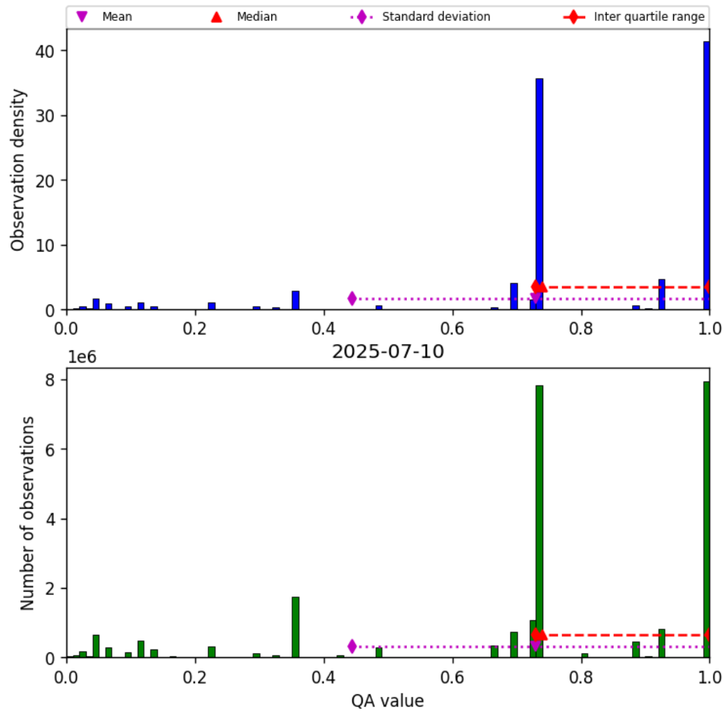
Figure 26: Histogram of “QA value” for 2025-07-10 to 2025-07-11
