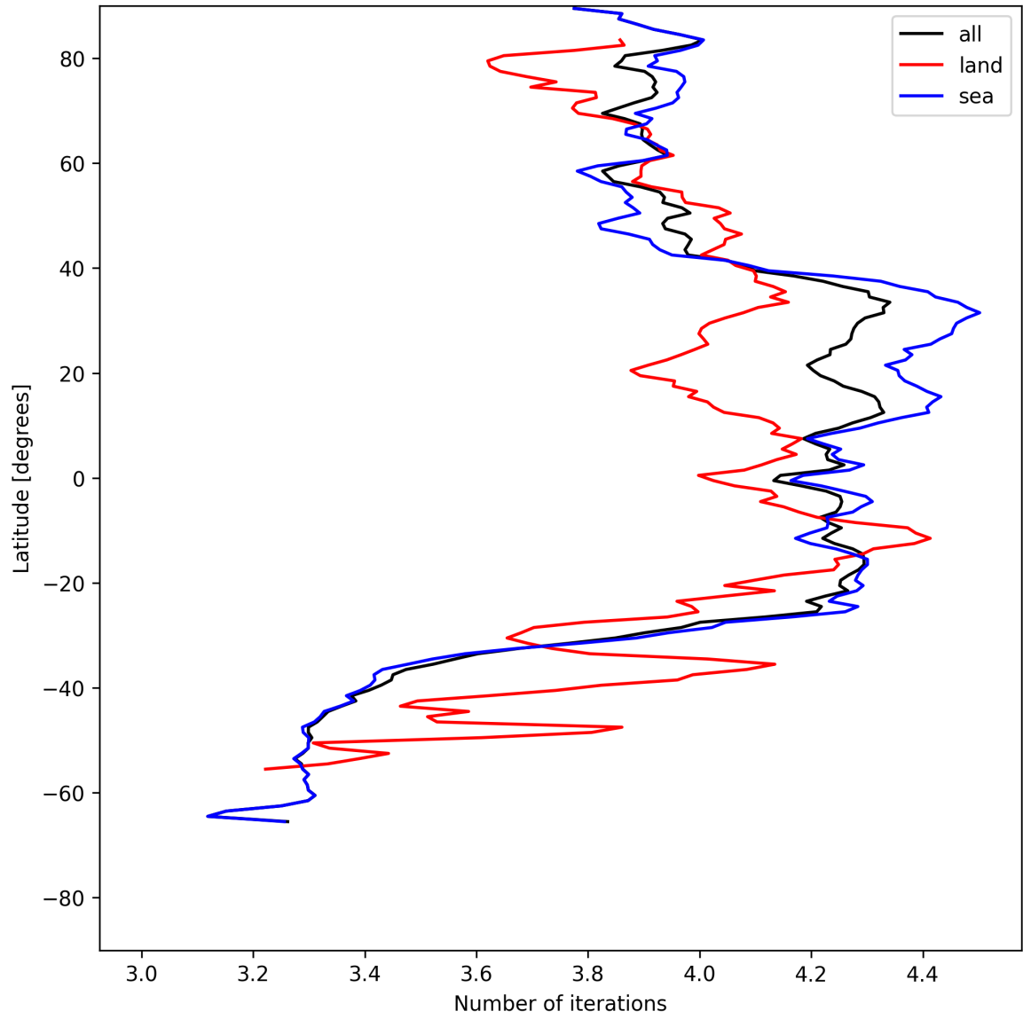
Figure 15: Zonal average of “Number of iterations” for 2025-07-10 to 2025-07-11.
