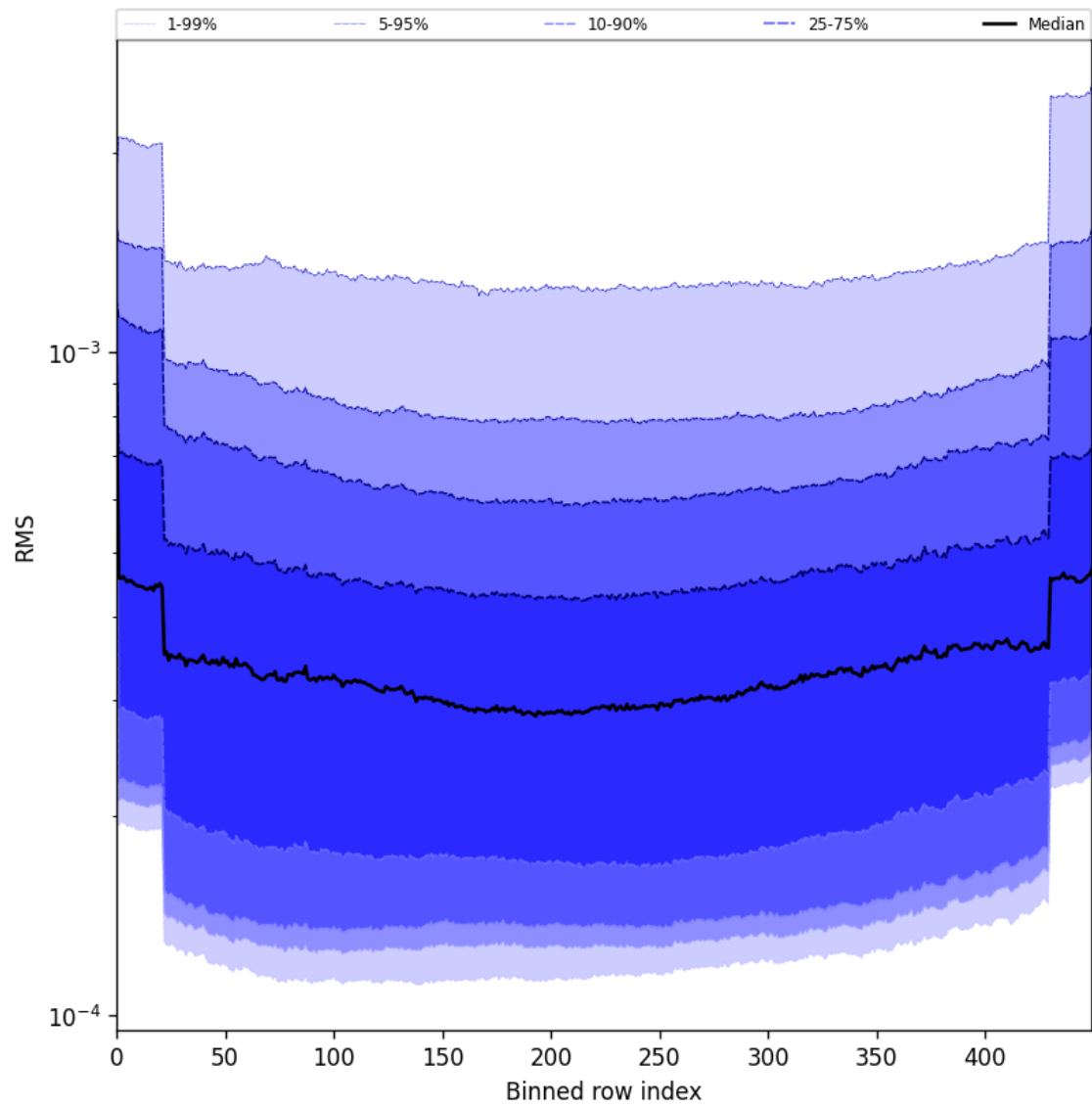
Figure 58: Along track statistics of “RMS” for 2025-07-10 to 2025-07-11
