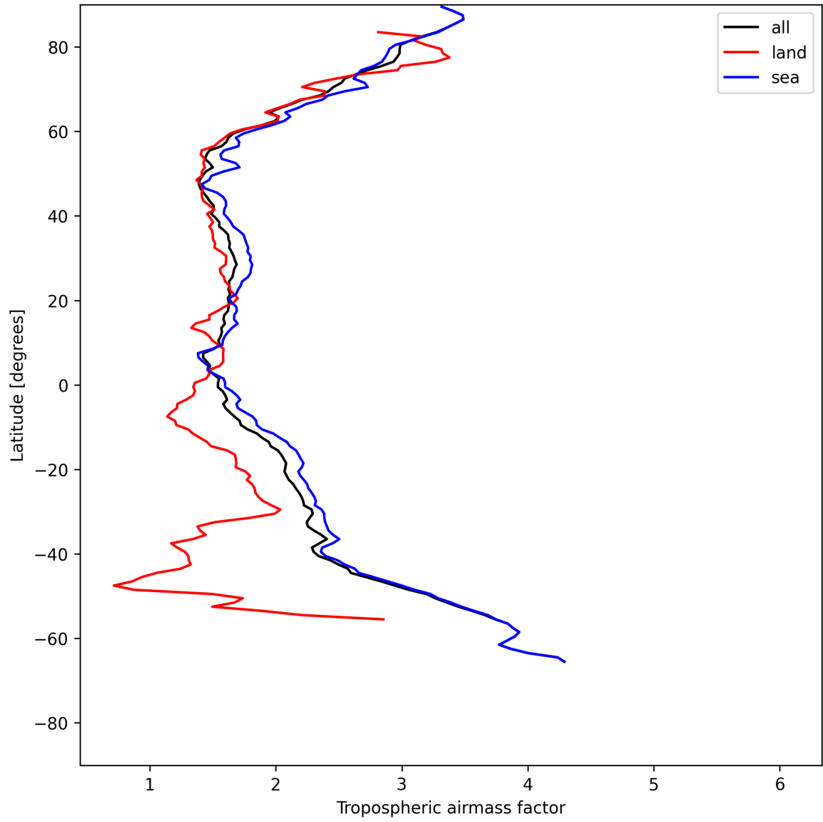
Figure 12: Zonal average of “Tropospheric airmass factor” for 2025-07-10 to 2025-07-11.
