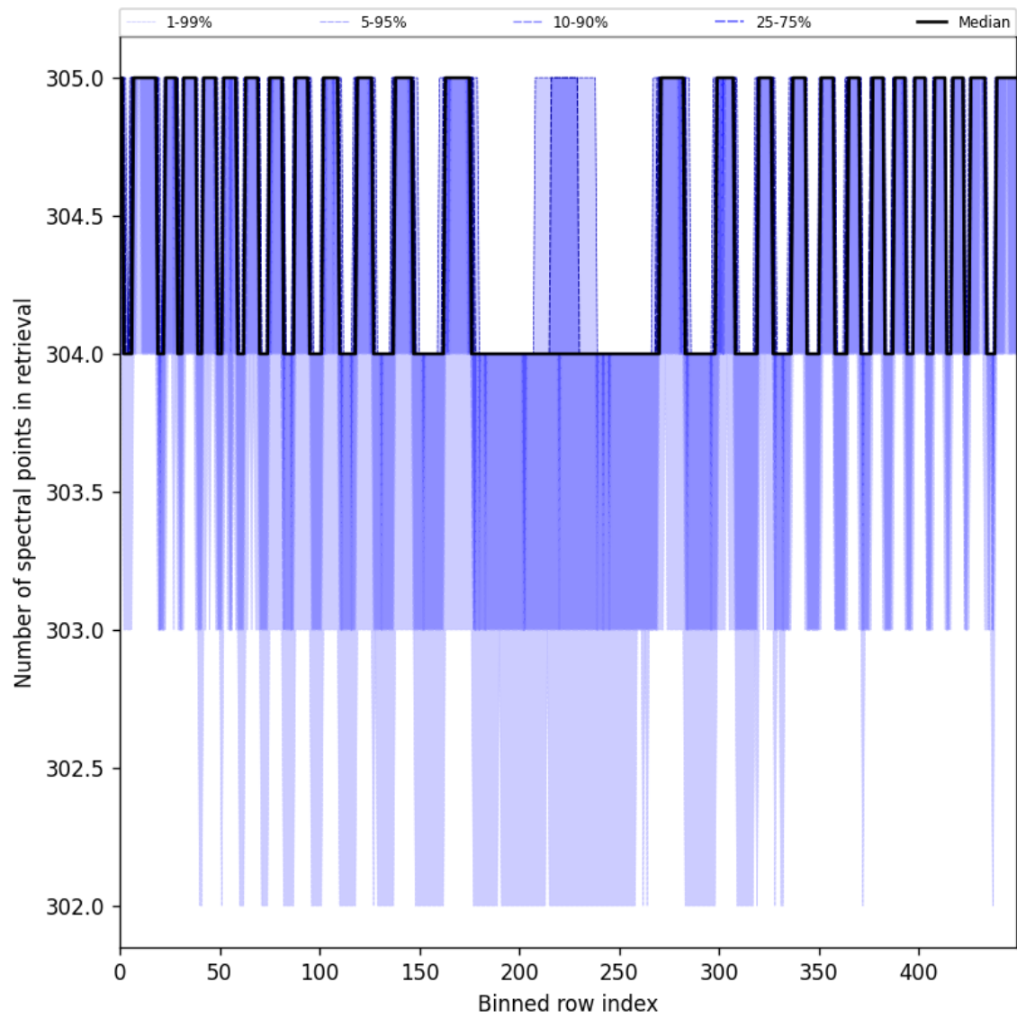
Figure 48: Along track statistics of “Number of spectral points in retrieval” for 2025-07-10 to 2025-07-11
