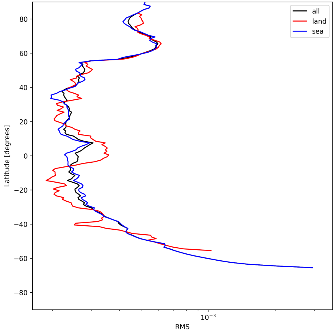
Figure 24: Zonal average of “RMS” for 2025-07-10 to 2025-07-11.
