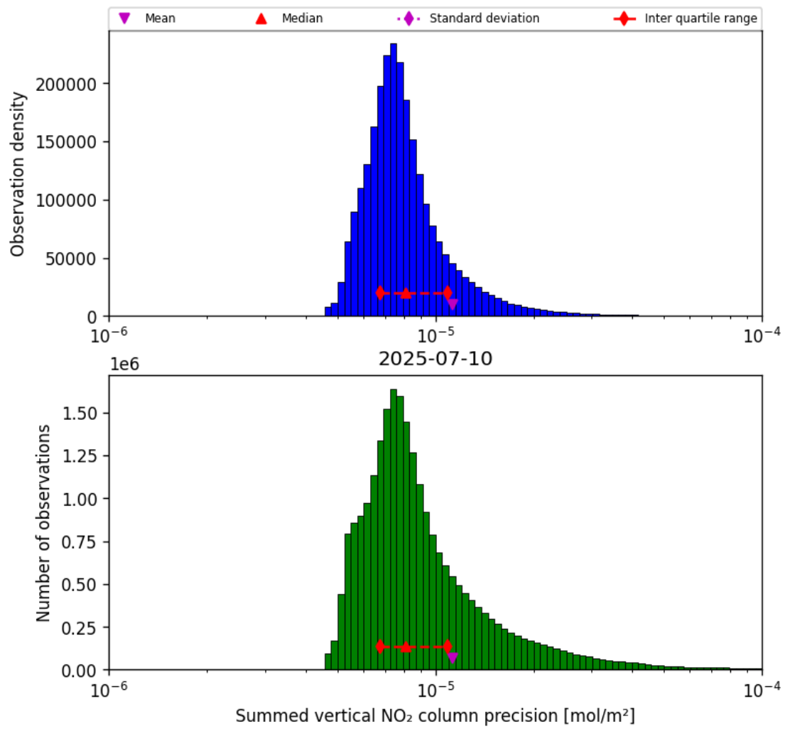
Figure 39: Histogram of “Summed vertical NO 2 column precision” for 2025-07-10 to 2025-07-11
