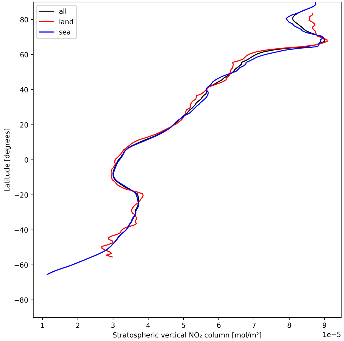
Figure 17: Zonal average of “Stratospheric vertical NO 2 column” for 2025-07-10 to 2025-07-11.
