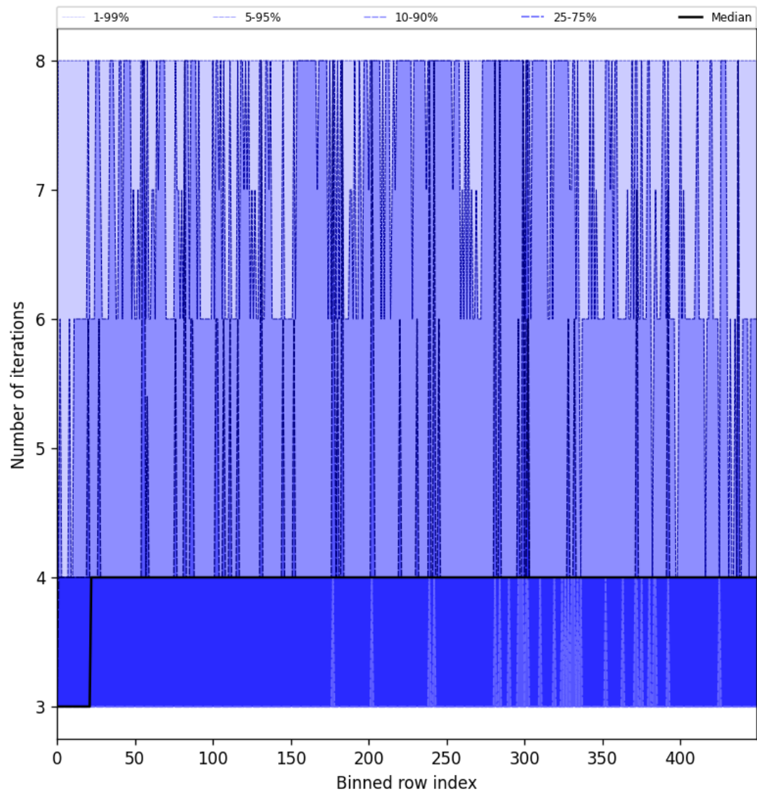
Figure 49: Along track statistics of “Number of iterations” for 2025-07-10 to 2025-07-11
