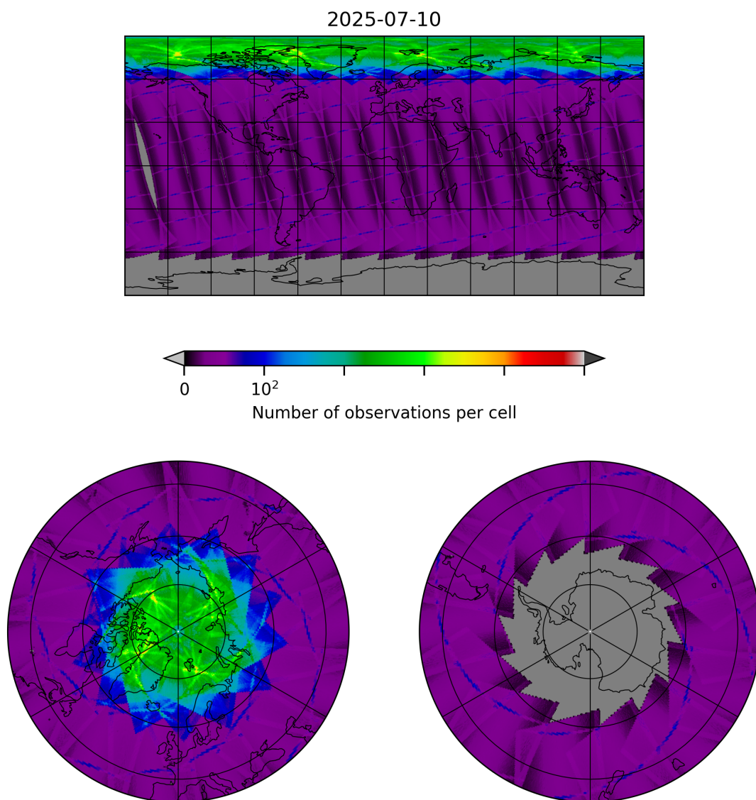
Figure 8: Map of the number of observations for 2025-07-10 to 2025-07-11
