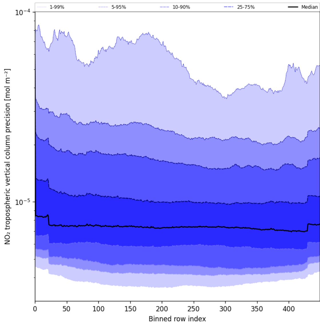
Figure 45: Along track statistics of “NO 2 tropospheric vertical column precision” for 2025-07-10 to 2025-07-11
