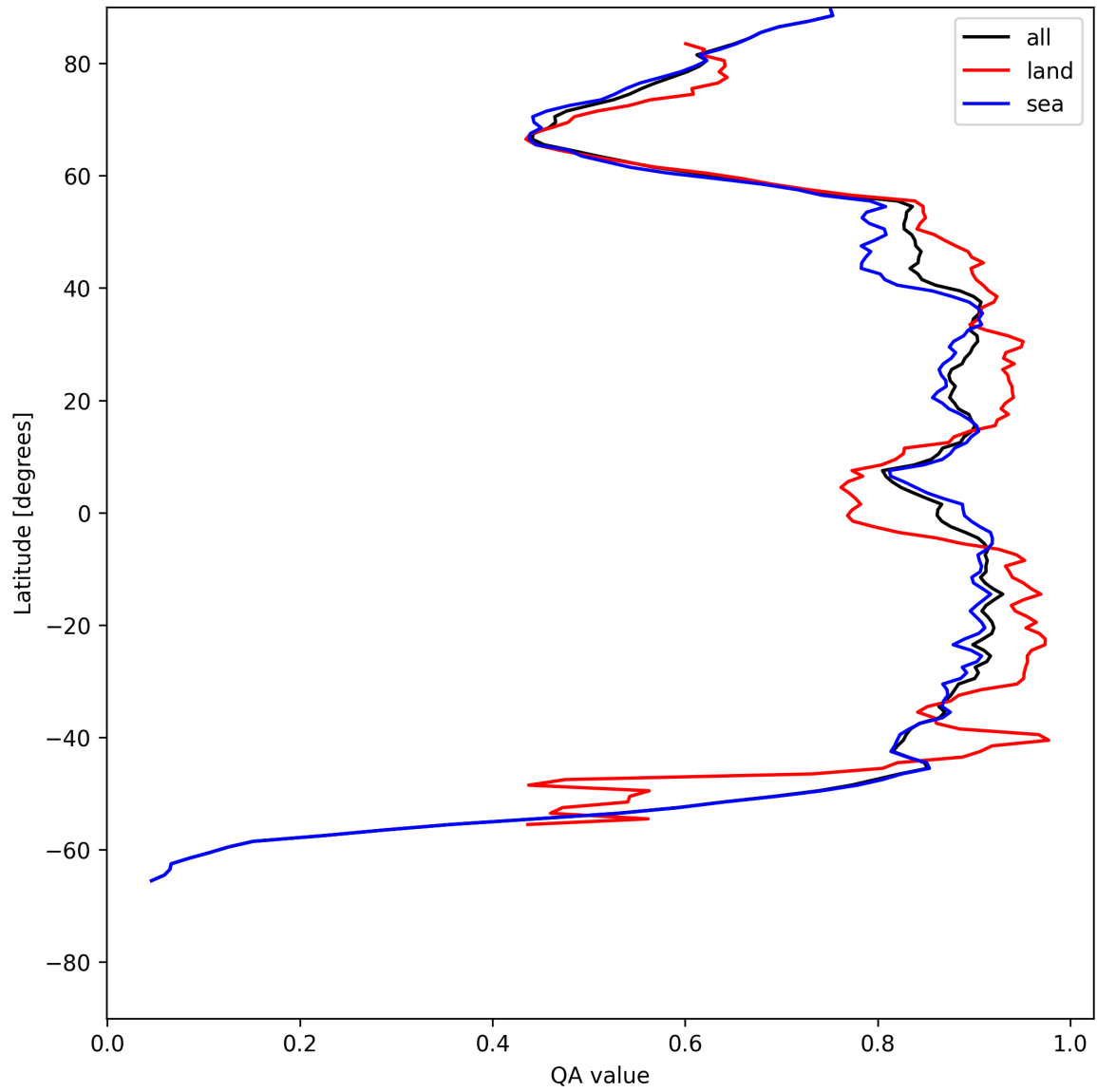
Figure 9: Zonal average of “QA value” for 2025-07-10 to 2025-07-11.
