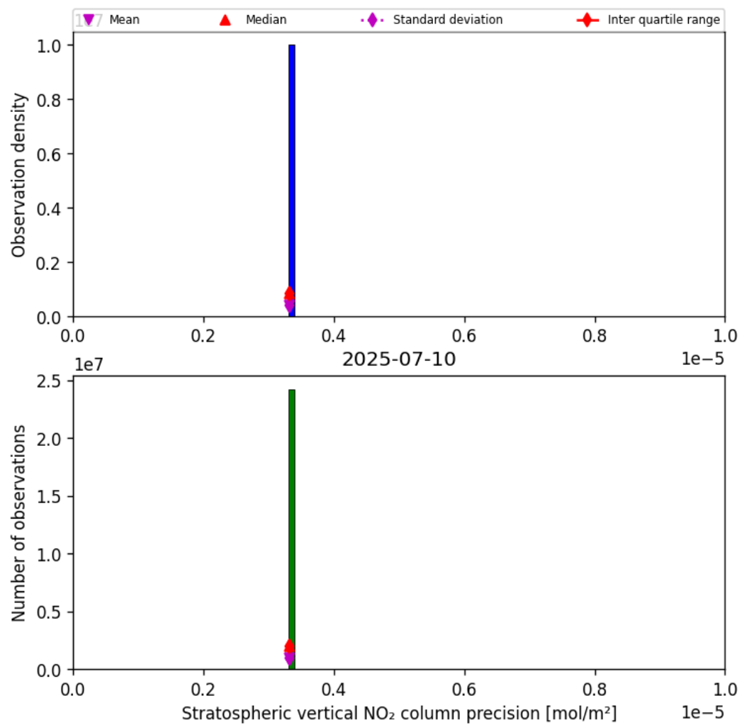
Figure 35: Histogram of “Stratospheric vertical NO 2 column precision” for 2025-07-10 to 2025-07-11
