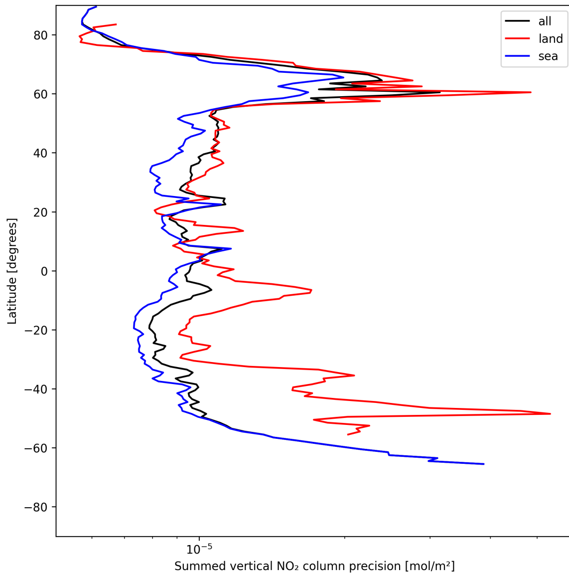
Figure 22: Zonal average of “Summed vertical NO 2 column precision” for 2025-07-10 to 2025-07-11.
