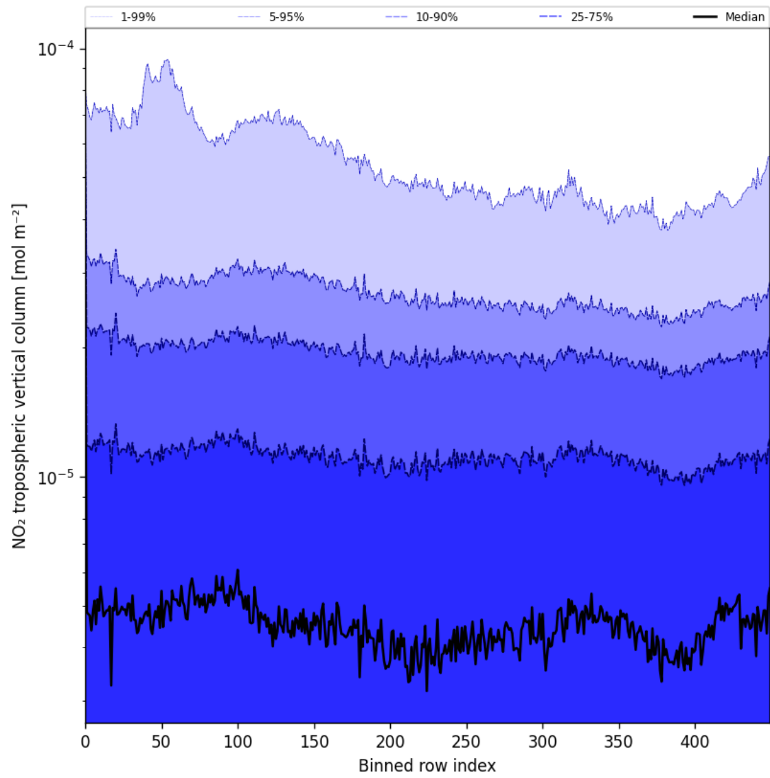
Figure 44: Along track statistics of “NO 2 tropospheric vertical column” for 2025-07-10 to 2025-07-11
