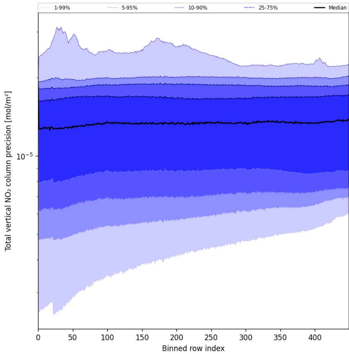
Figure 54: Along track statistics of “Total vertical NO 2 column precision” for 2025-07-10 to 2025-07-11
