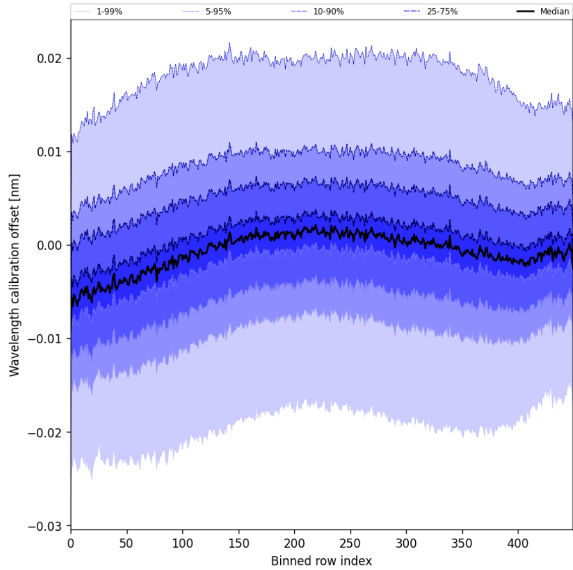
Figure 50: Along track statistics of “Wavelength calibration offset” for 2025-07-10 to 2025-07-11
