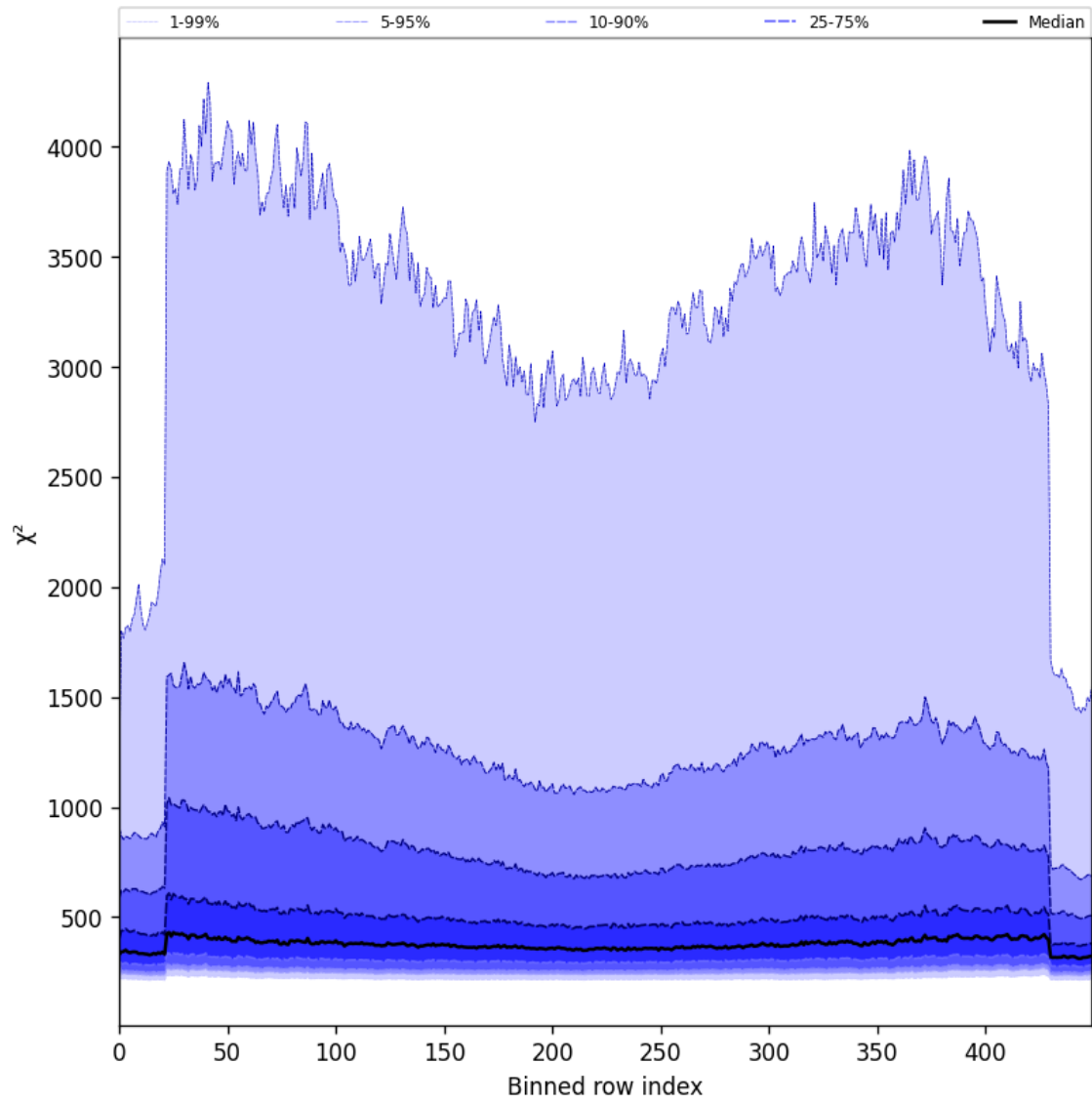
Figure 57: Along track statistics of “ \chi^2 ” for 2025-07-10 to 2025-07-11
