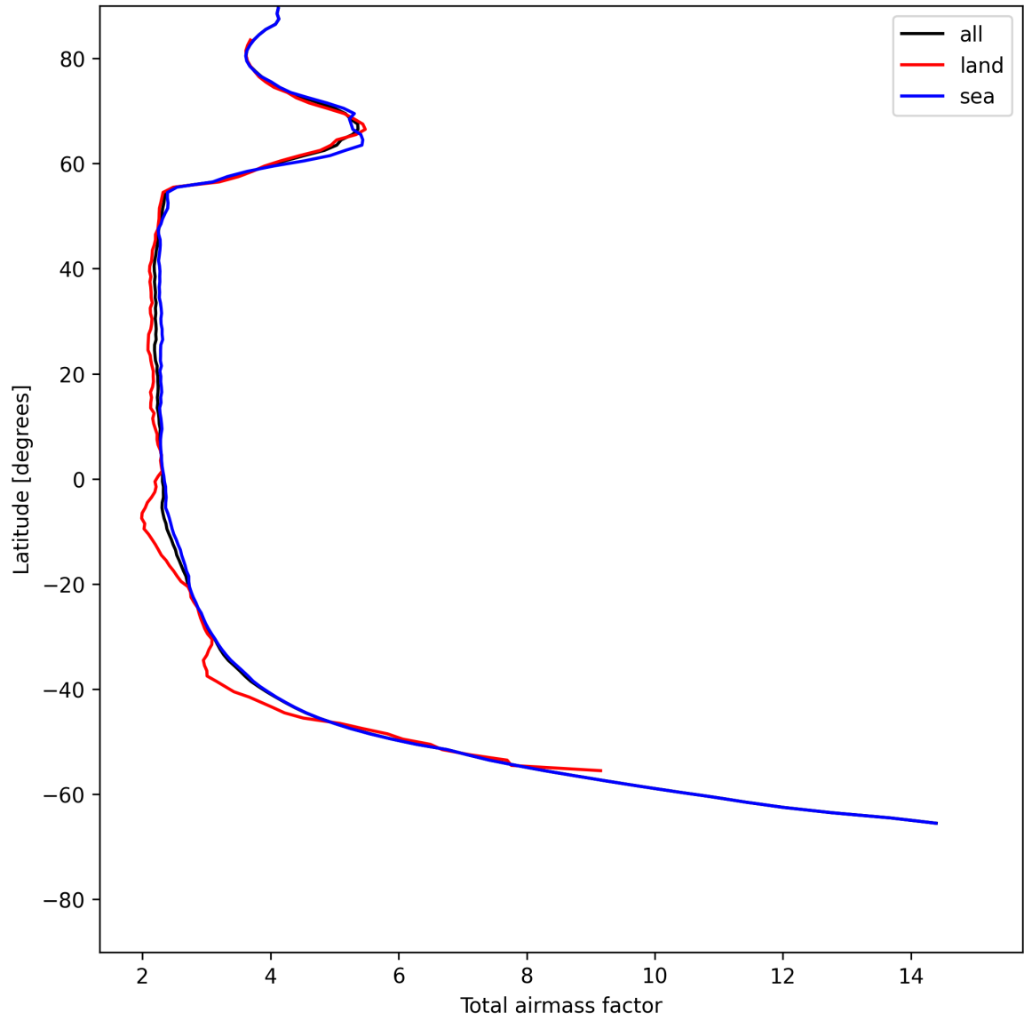
Figure 13: Zonal average of “Total airmass factor” for 2025-07-10 to 2025-07-11.
