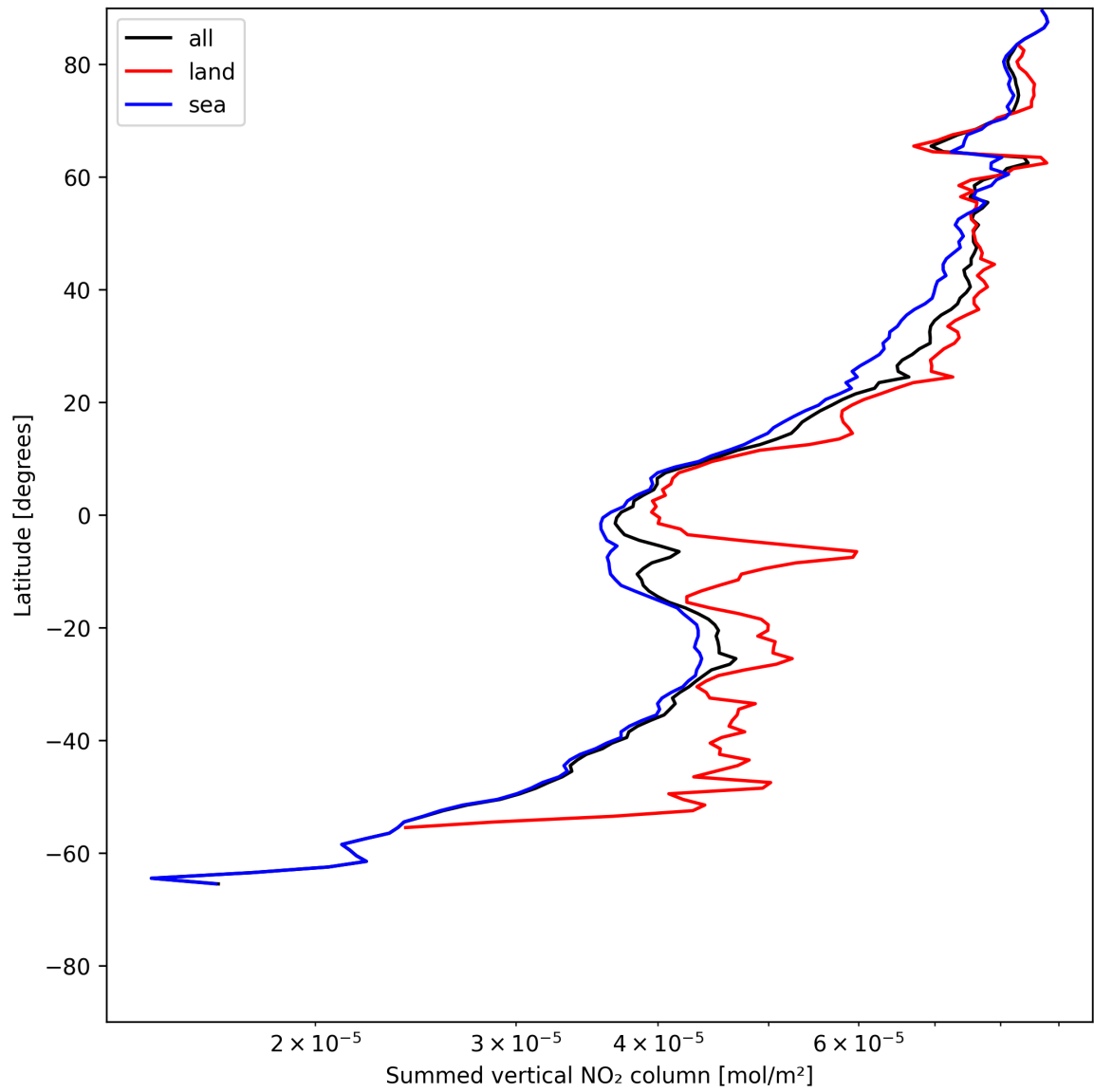
Figure 21: Zonal average of “Summed vertical NO 2 column” for 2025-07-10 to 2025-07-11.
