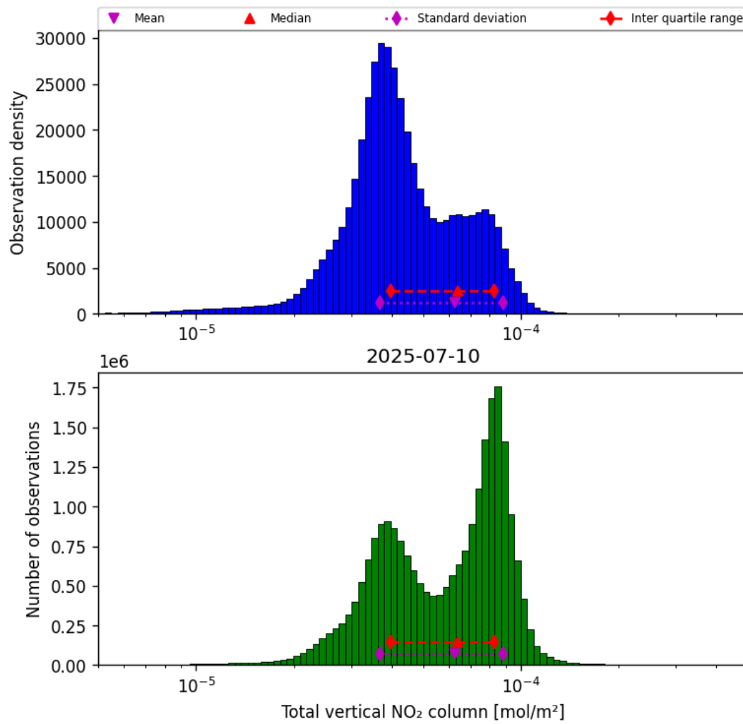
Figure 36: Histogram of “Total vertical NO 2 column” for 2025-07-10 to 2025-07-11
