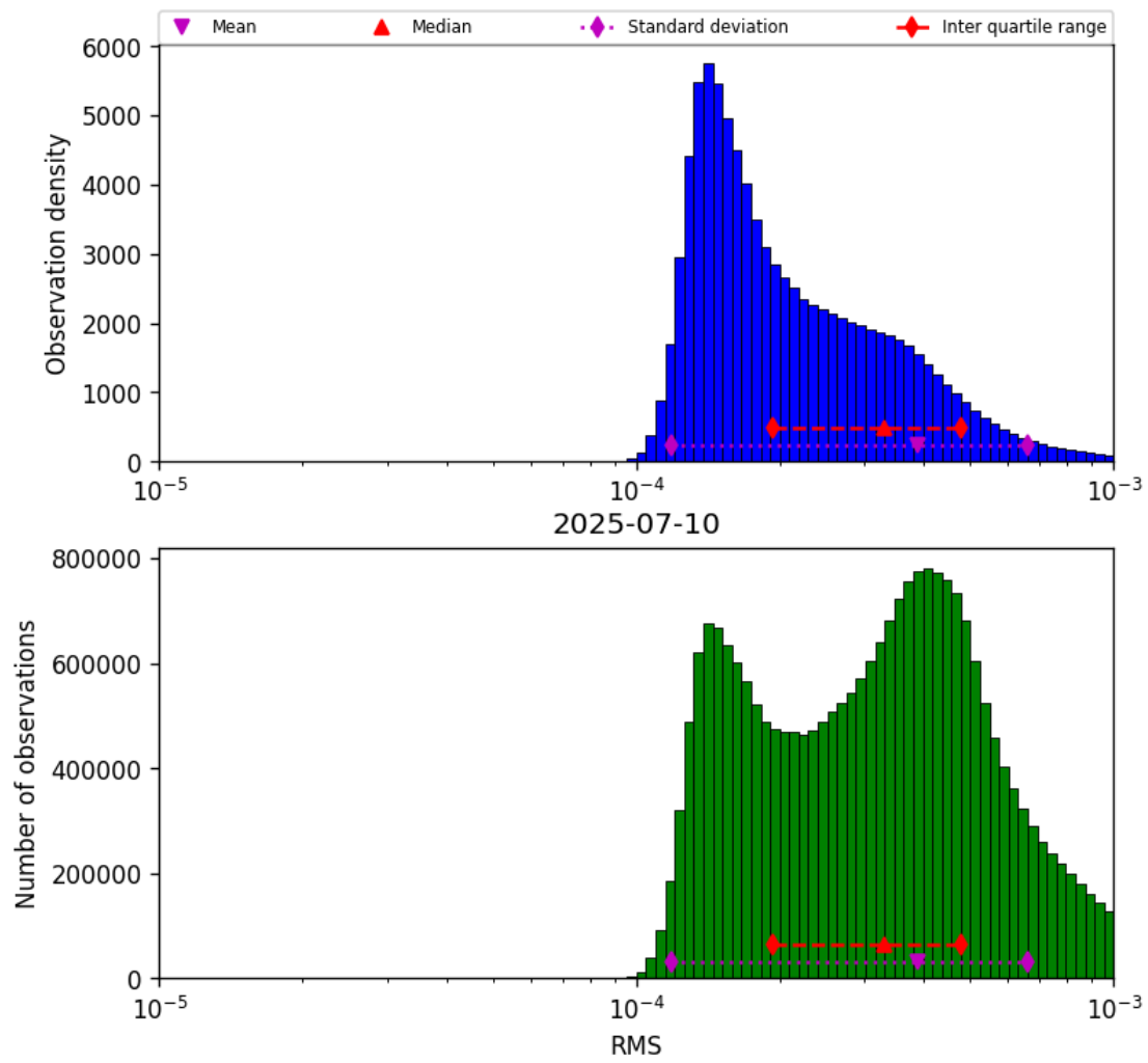
Figure 41: Histogram of “RMS” for 2025-07-10 to 2025-07-11
