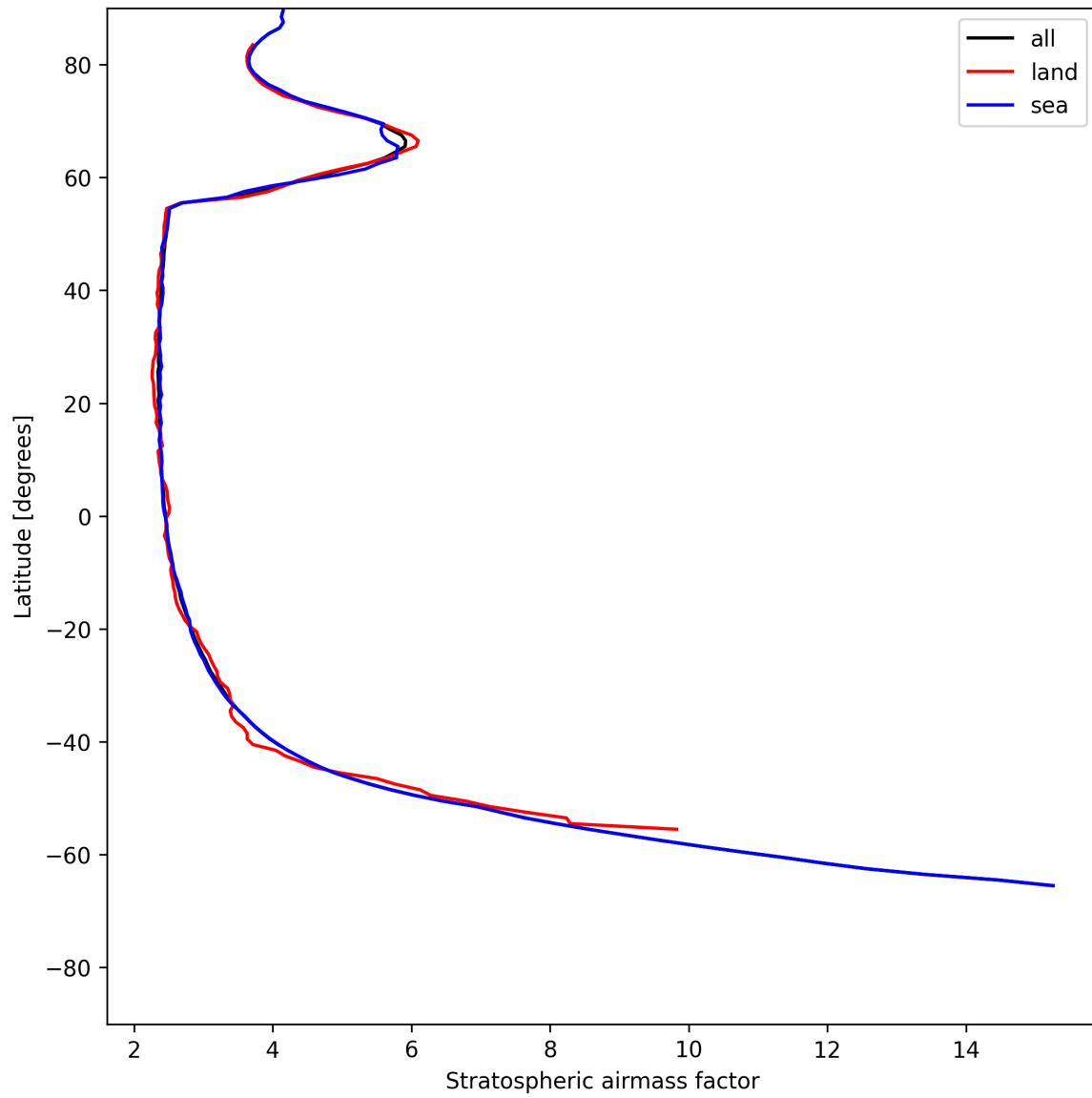
Figure 25: Zonal average of “Stratospheric air mass factor” for 2025-07-10 to 2025-07-11.
