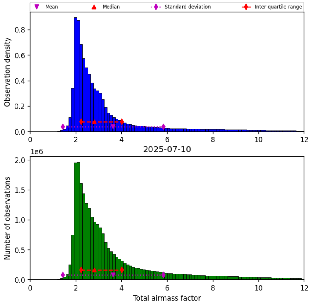
Figure 30: Histogram of “Total airmass factor” for 2025-07-10 to 2025-07-11
