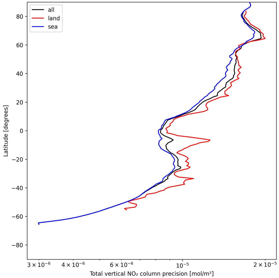
Figure 20: Zonal average of “Total vertical NO 2 column precision” for 2025-07-10 to 2025-07-11.
