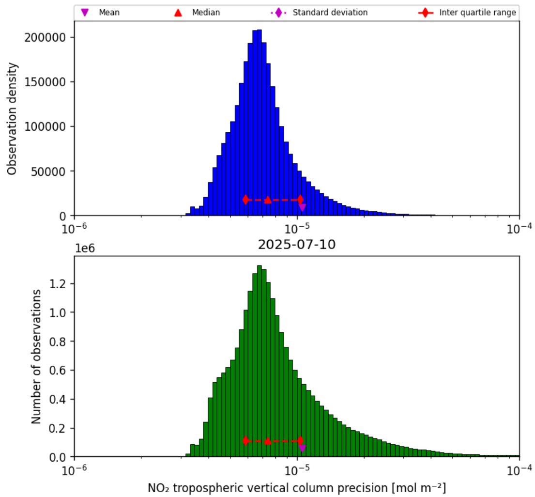
Figure 28: Histogram of “NO 2 tropospheric vertical column precision” for 2025-07-10 to 2025-07-11
