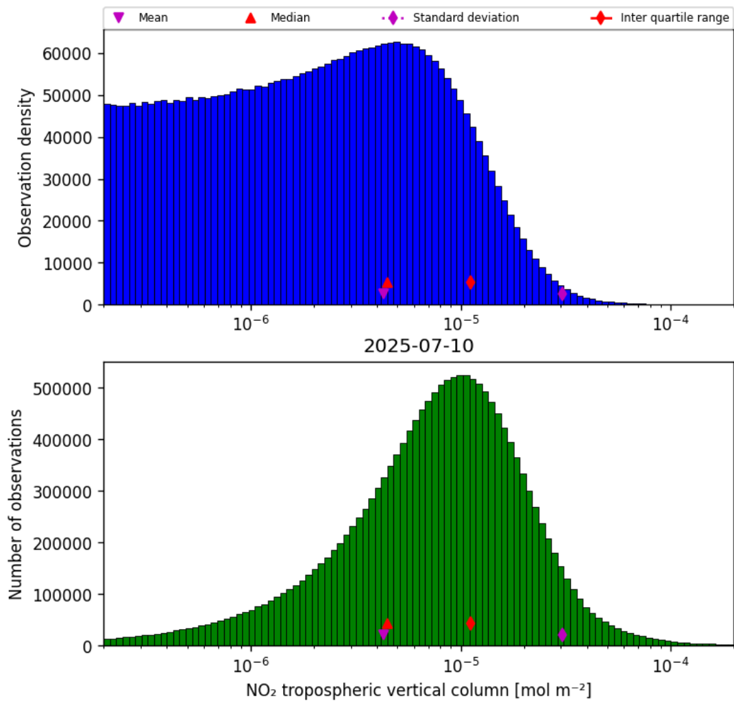
Figure 27: Histogram of “NO 2 tropospheric vertical column” for 2025-07-10 to 2025-07-11
