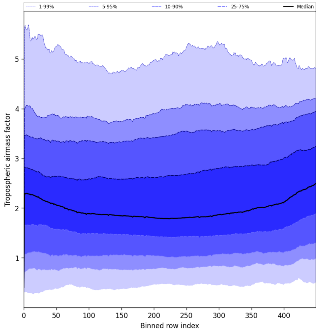
Figure 46: Along track statistics of “Tropospheric airmass factor” for 2025-07-10 to 2025-07-11
