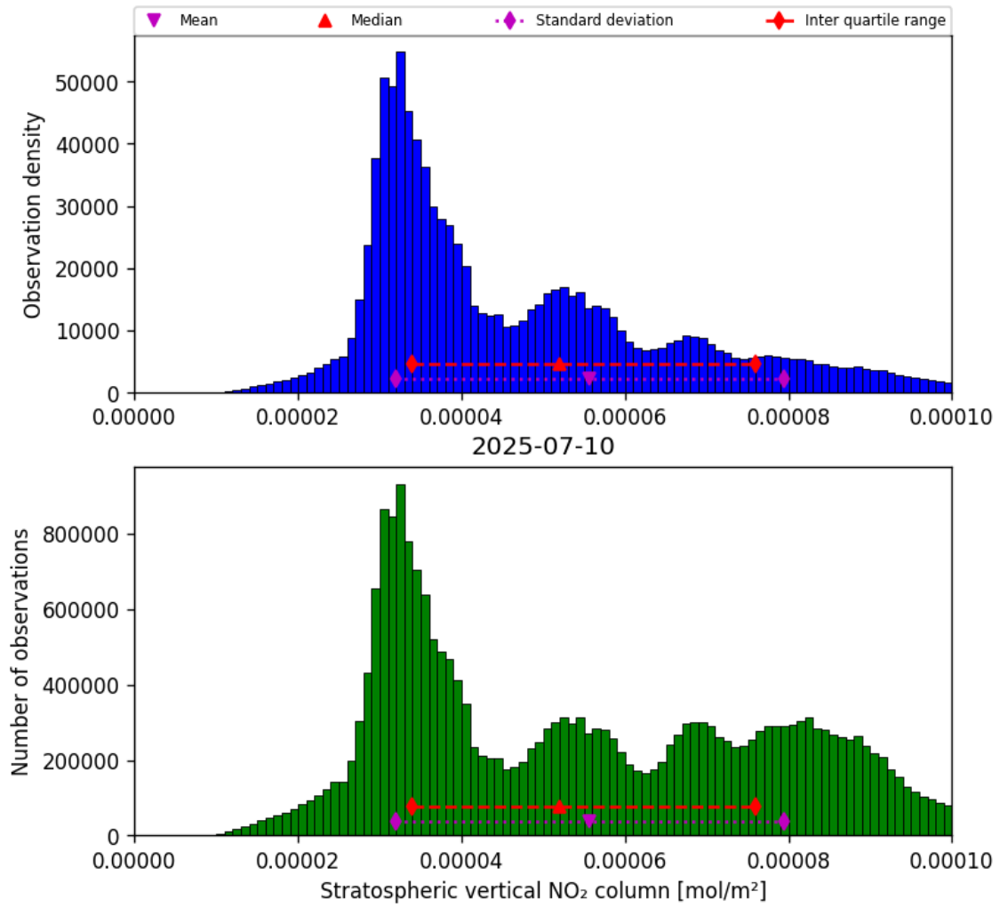
Figure 34: Histogram of “Stratospheric vertical NO 2 column” for 2025-07-10 to 2025-07-11
