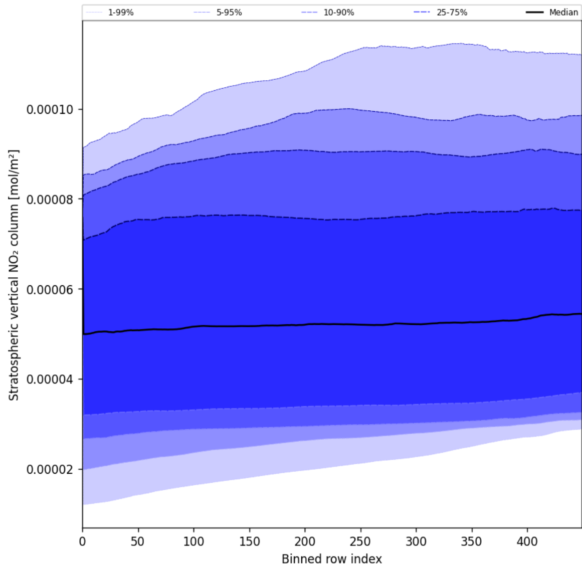
Figure 51: Along track statistics of “Stratospheric vertical NO 2 column” for 2025-07-10 to 2025-07-11
