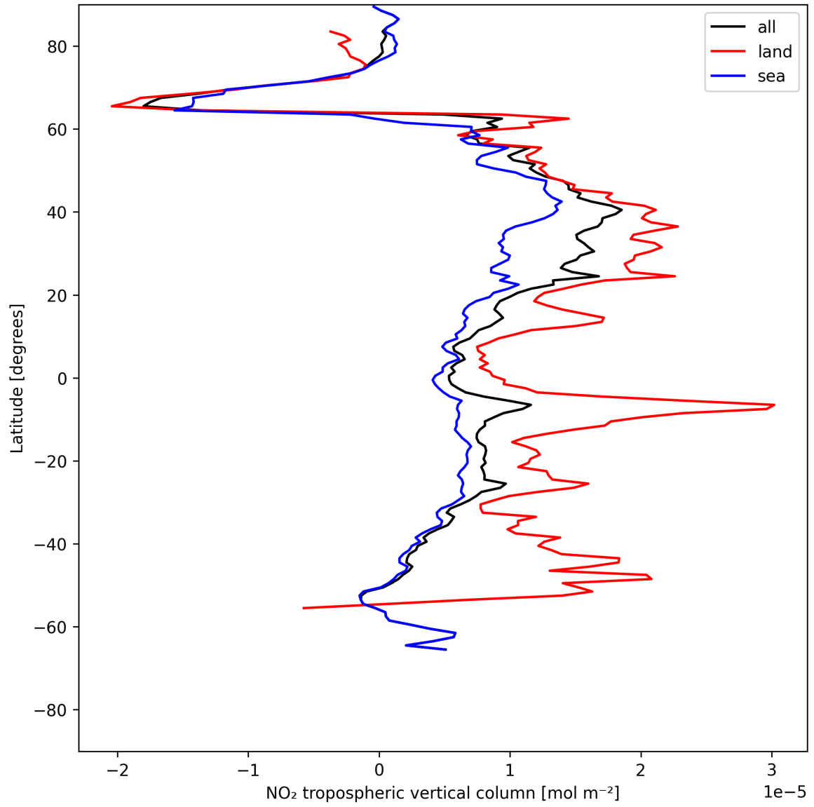
Figure 10: Zonal average of “NO 2 tropospheric vertical column” for 2025-07-10 to 2025-07-11.
