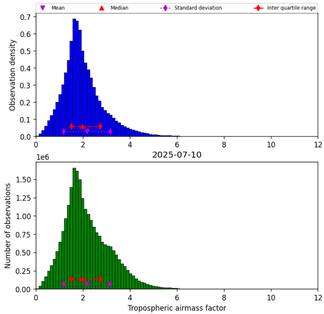
Figure 29: Histogram of “Tropospheric airmass factor” for 2025-07-10 to 2025-07-11
