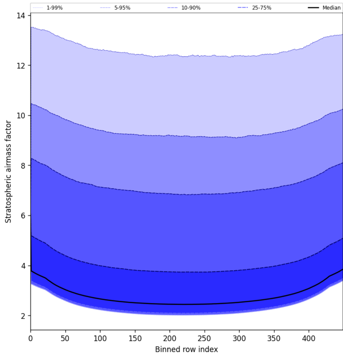
Figure 59: Along track statistics of “Stratospheric airmass factor” for 2025-07-10 to 2025-07-11
