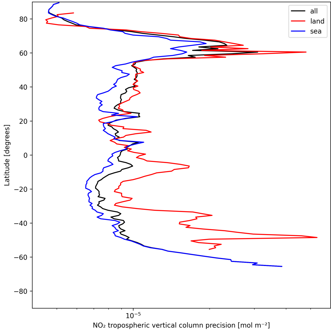
Figure 11: Zonal average of “NO 2 tropospheric vertical column precision” for 2025-07-10 to 2025-07-11.
