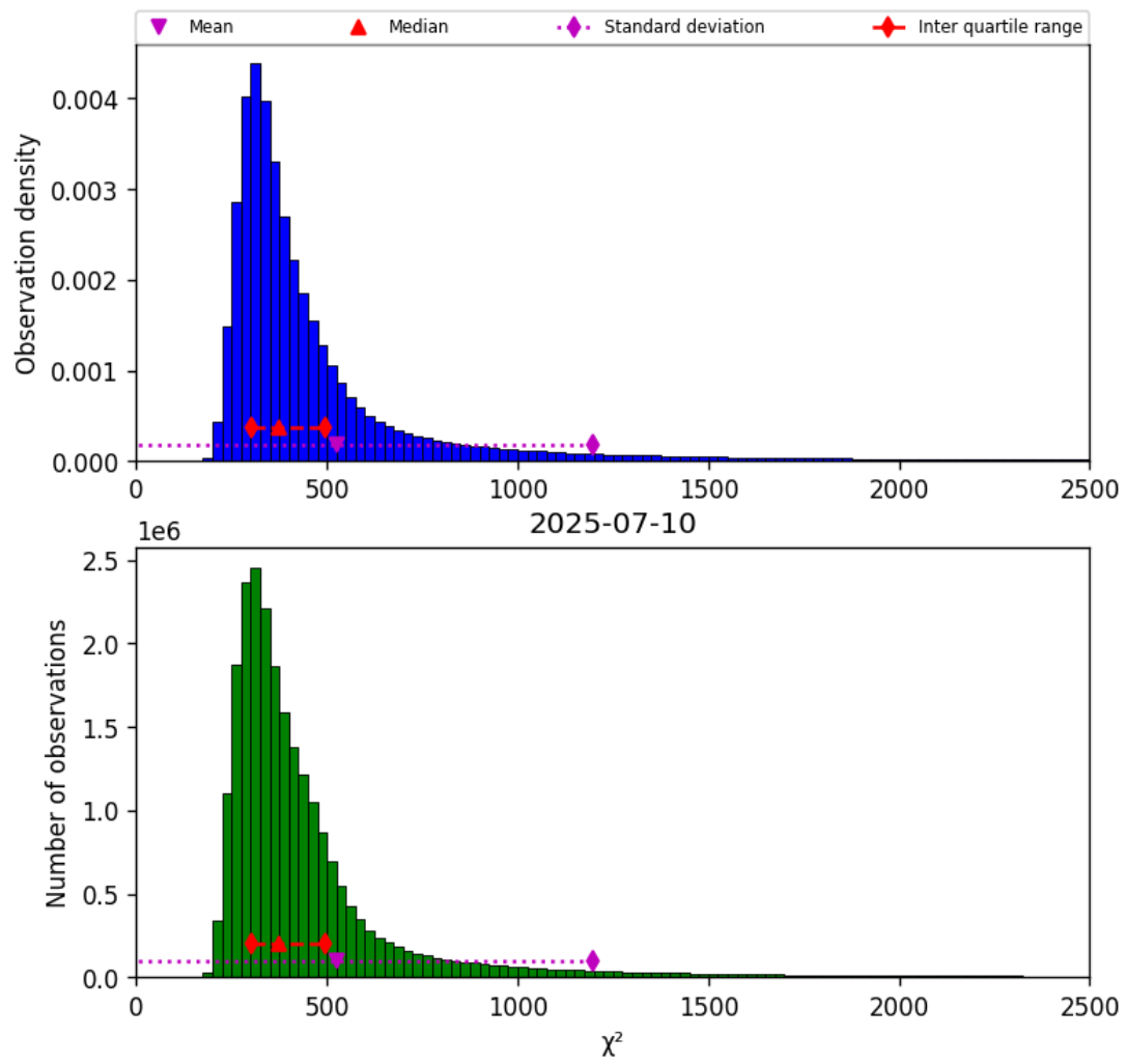
Figure 40: Histogram of " \chi^2 " for 2025-07-10 to 2025-07-11
