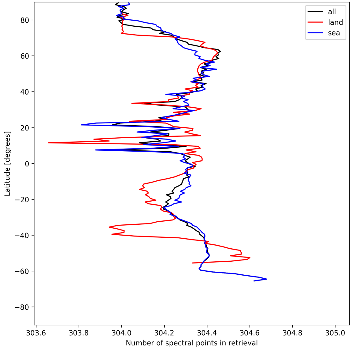
Figure 14: Zonal average of “Number of spectral points in retrieval” for 2025-07-10 to 2025-07-11.
