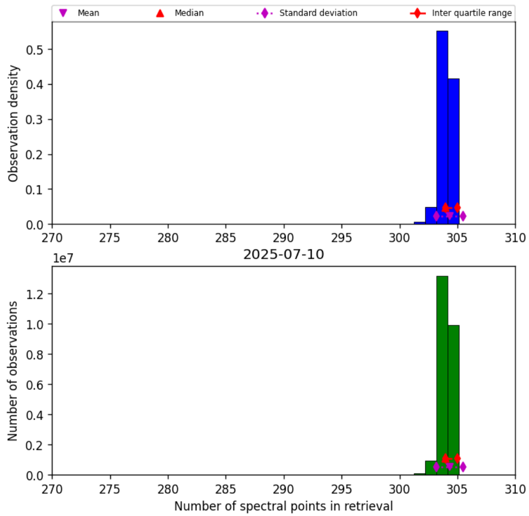
Figure 31: Histogram of “Number of spectral points in retrieval” for 2025-07-10 to 2025-07-11
