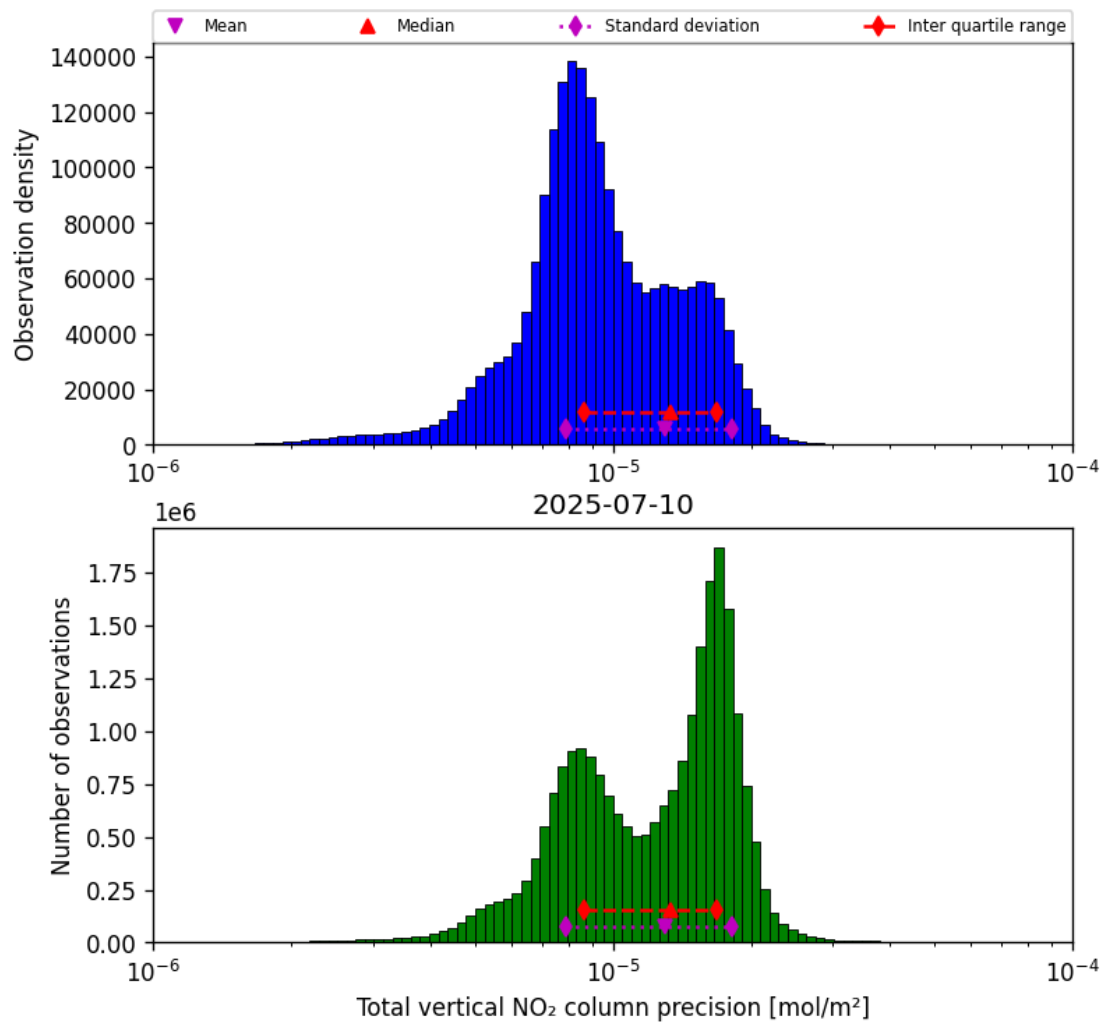
Figure 37: Histogram of “Total vertical NO 2 column precision” for 2025-07-10 to 2025-07-11
