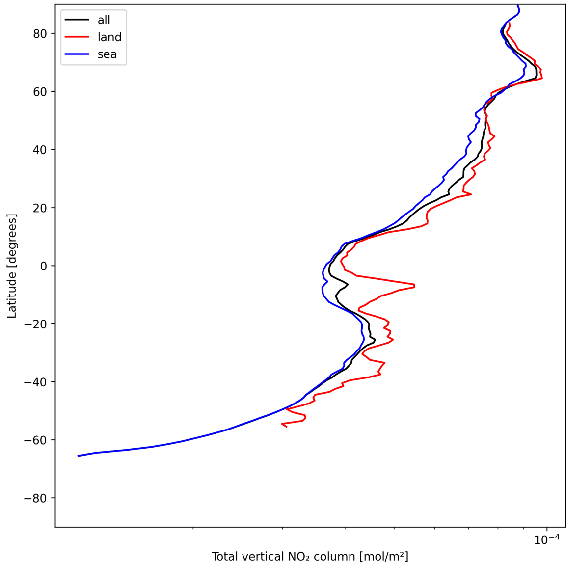
Figure 19: Zonal average of “Total vertical NO 2 column” for 2025-07-10 to 2025-07-11.
