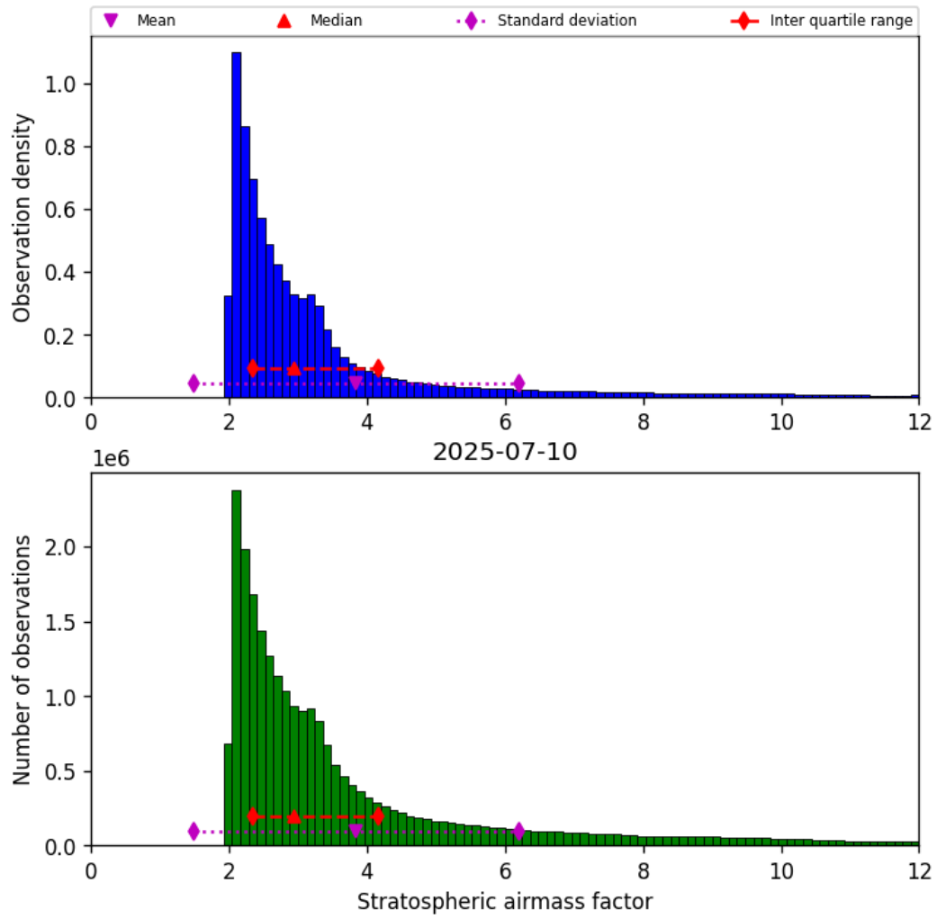
Figure 42: Histogram of “Stratospheric airmass factor” for 2025-07-10 to 2025-07-11
