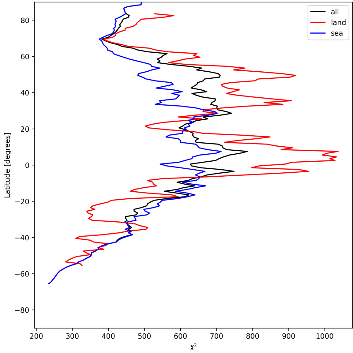
Figure 23: Zonal average of “ \chi^2 ” for 2025-07-10 to 2025-07-11.
