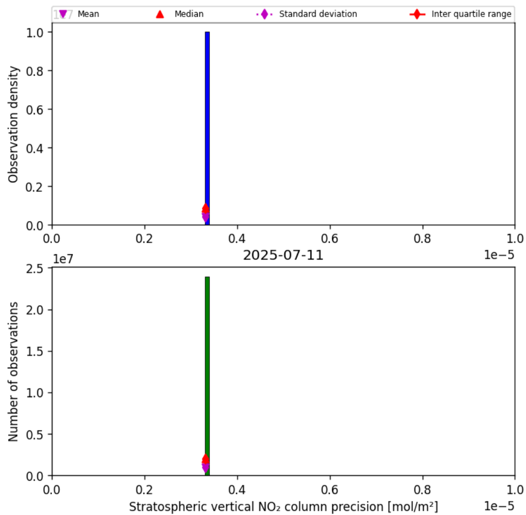
Figure 35: Histogram of “Stratospheric vertical NO 2 column precision” for 2025-07-11 to 2025-07-11
