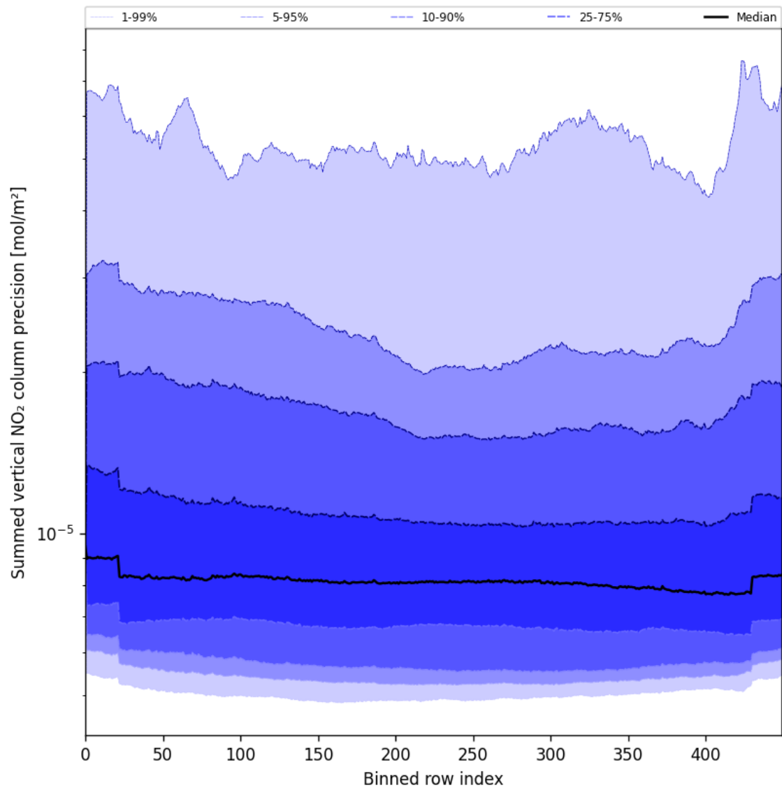
Figure 56: Along track statistics of “Summed vertical NO 2 column precision” for 2025-07-11 to 2025-07-11
