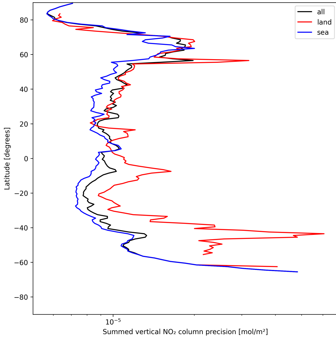
Figure 22: Zonal average of “Summed vertical NO 2 column precision” for 2025-07-11 to 2025-07-11.
