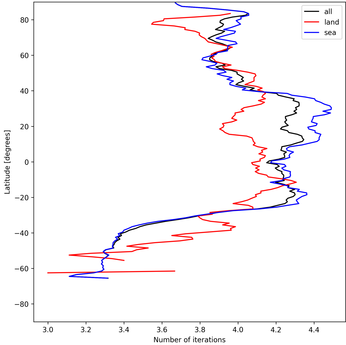
Figure 15: Zonal average of “Number of iterations” for 2025-07-11 to 2025-07-11.
