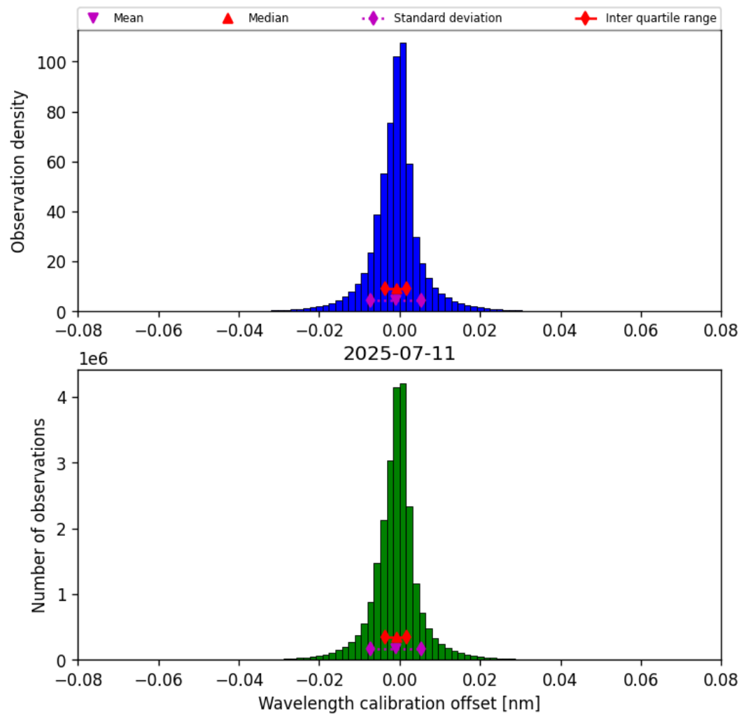
Figure 33: Histogram of “Wavelength calibration offset” for 2025-07-11 to 2025-07-11
