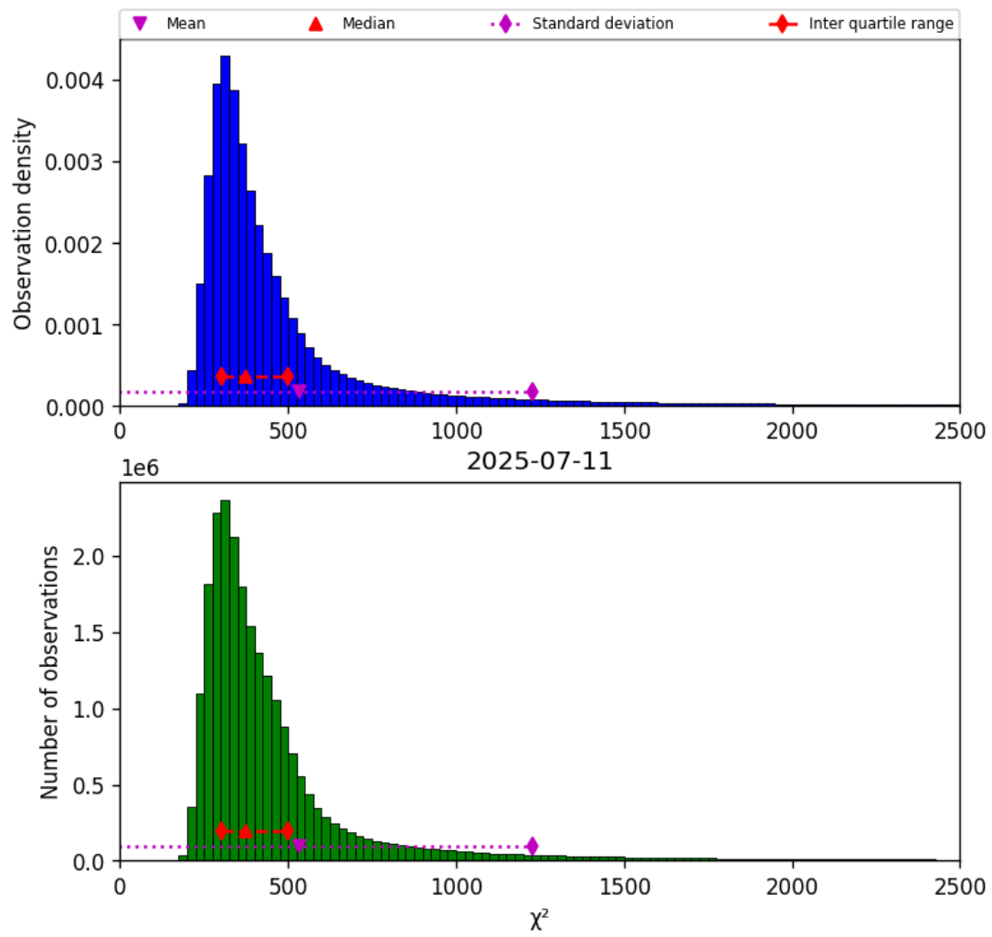
Figure 40: Histogram of “ \chi^2 ” for 2025-07-11 to 2025-07-11
