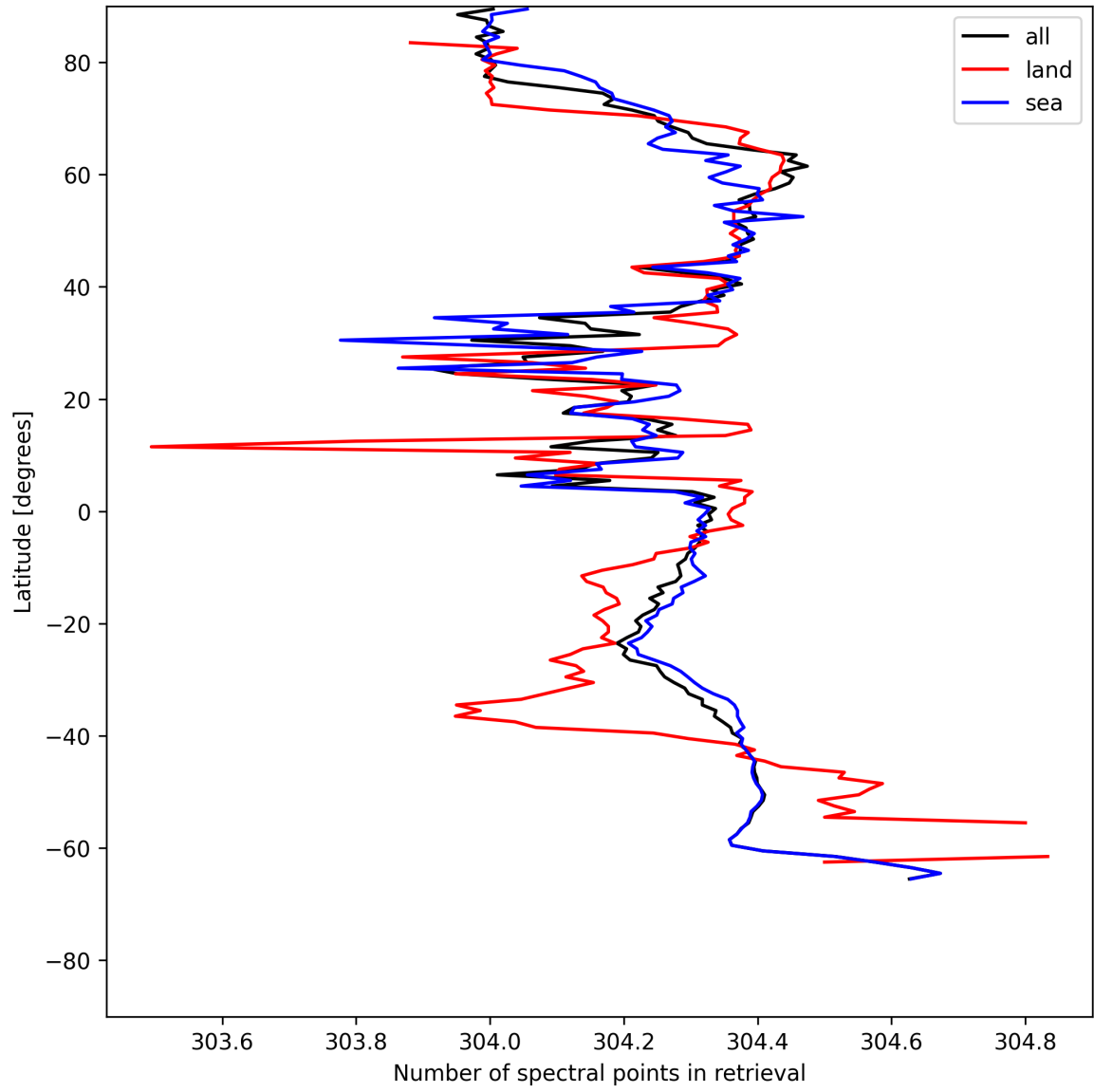
Figure 14: Zonal average of “Number of spectral points in retrieval” for 2025-07-11 to 2025-07-11.
