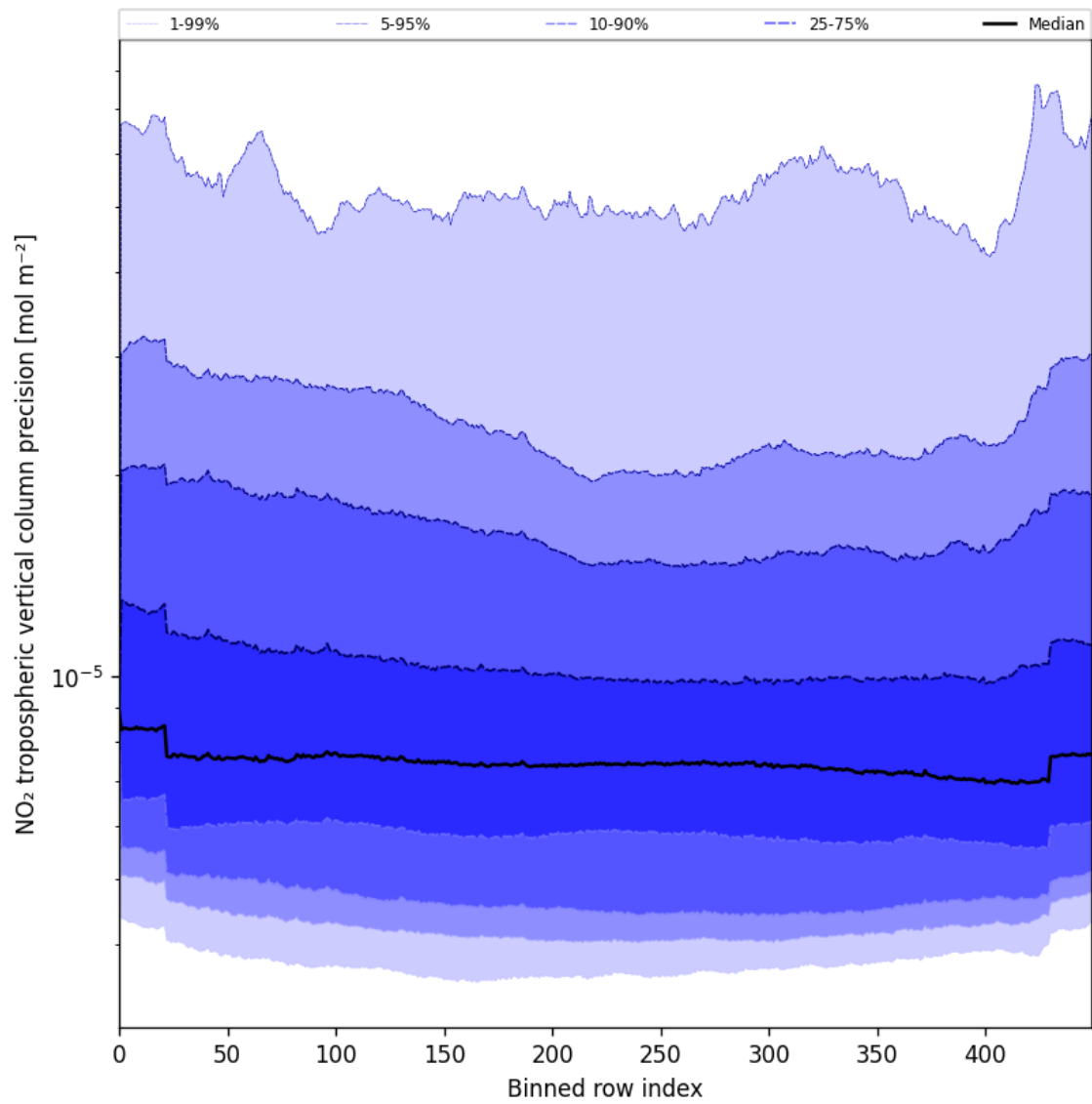
Figure 45: Along track statistics of “NO 2 tropospheric vertical column precision” for 2025-07-11 to 2025-07-11
