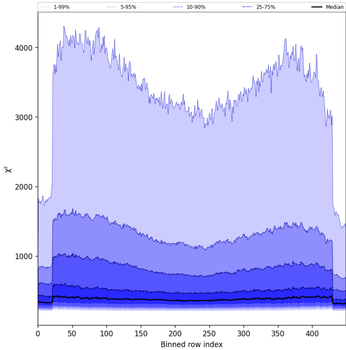
Figure 57: Along track statistics of “ \chi^2 ” for 2025-07-11 to 2025-07-11
