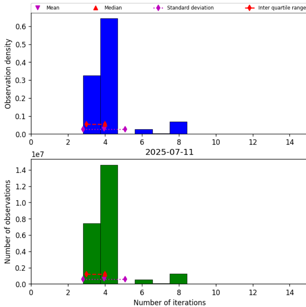
Figure 32: Histogram of “Number of iterations” for 2025-07-11 to 2025-07-11
