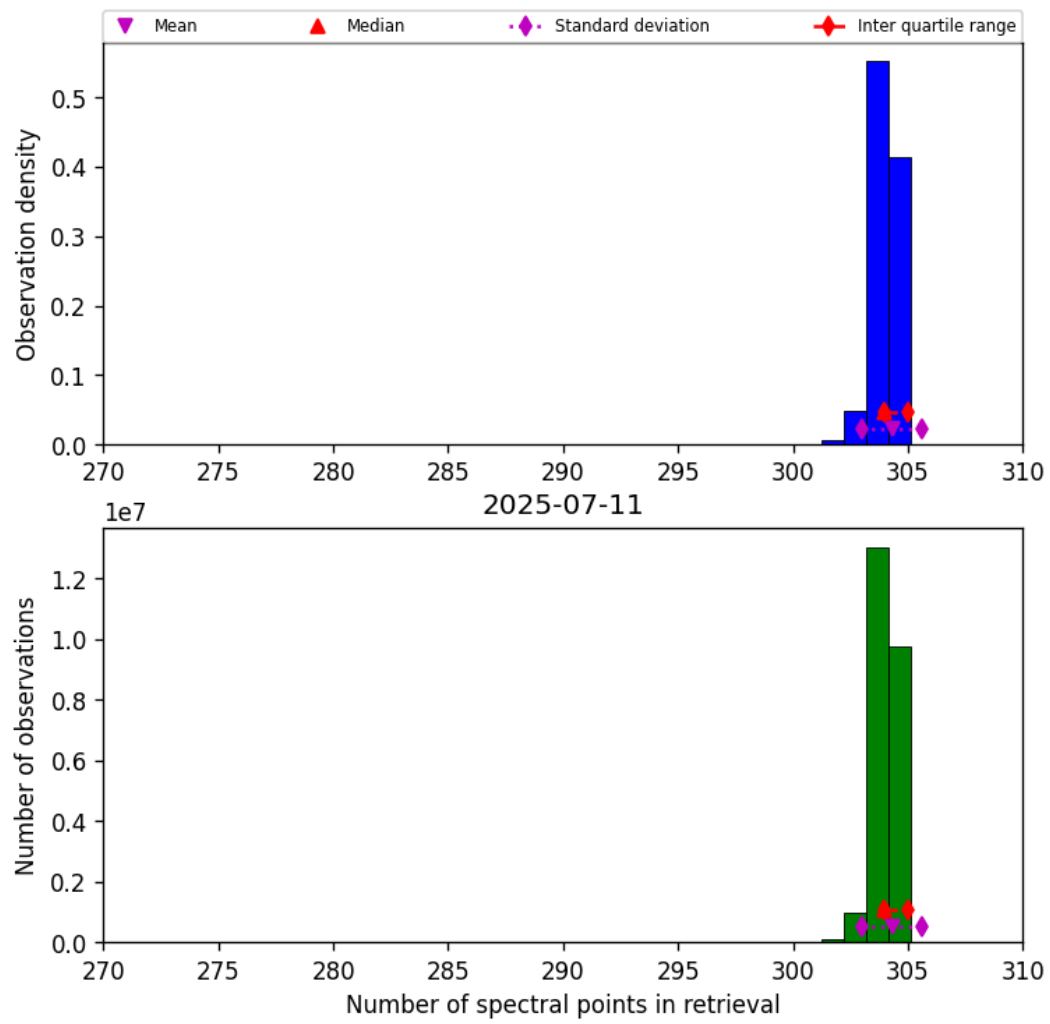
Figure 31: Histogram of “Number of spectral points in retrieval” for 2025-07-11 to 2025-07-11
