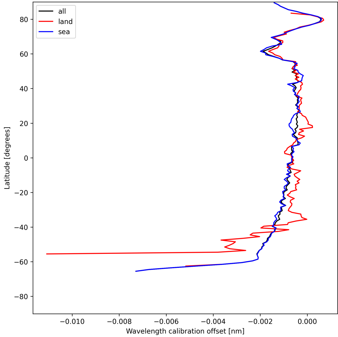
Figure 16: Zonal average of “Wavelength calibration offset” for 2025-07-11 to 2025-07-11.
