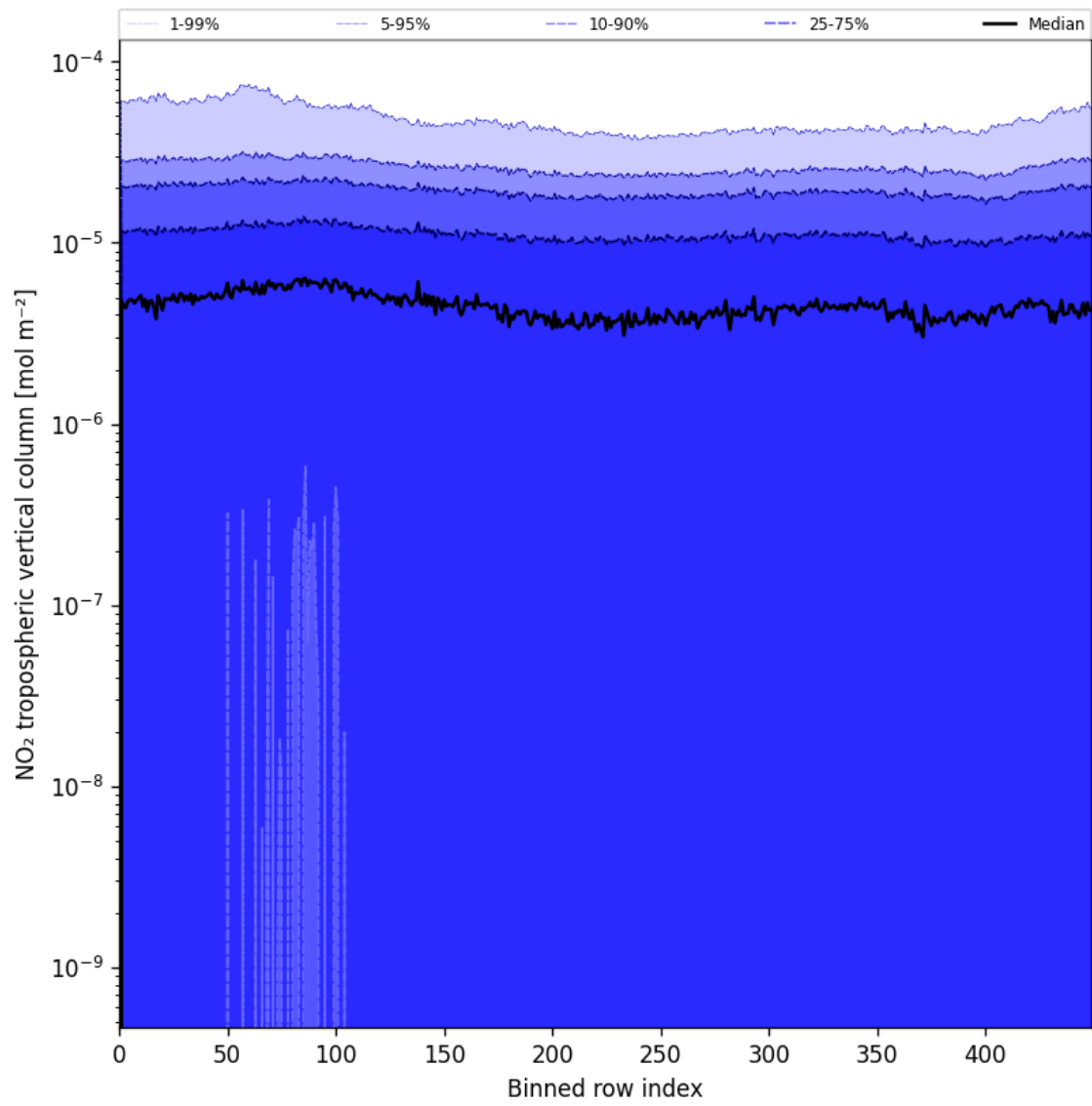
Figure 44: Along track statistics of "NO 2 tropospheric vertical column" for 2025-07-11 to 2025-07-11
