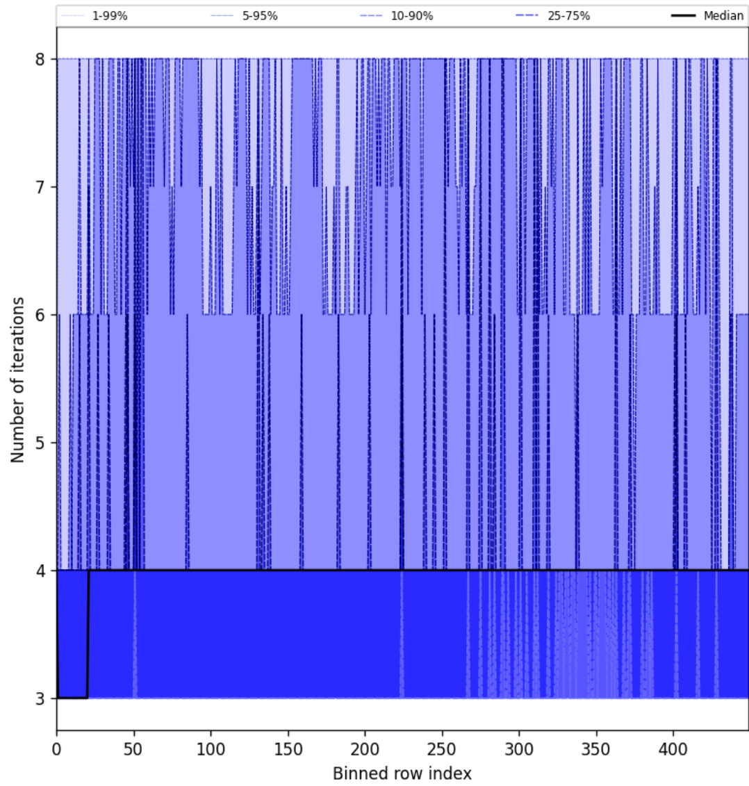
Figure 49: Along track statistics of “Number of iterations” for 2025-07-11 to 2025-07-11
