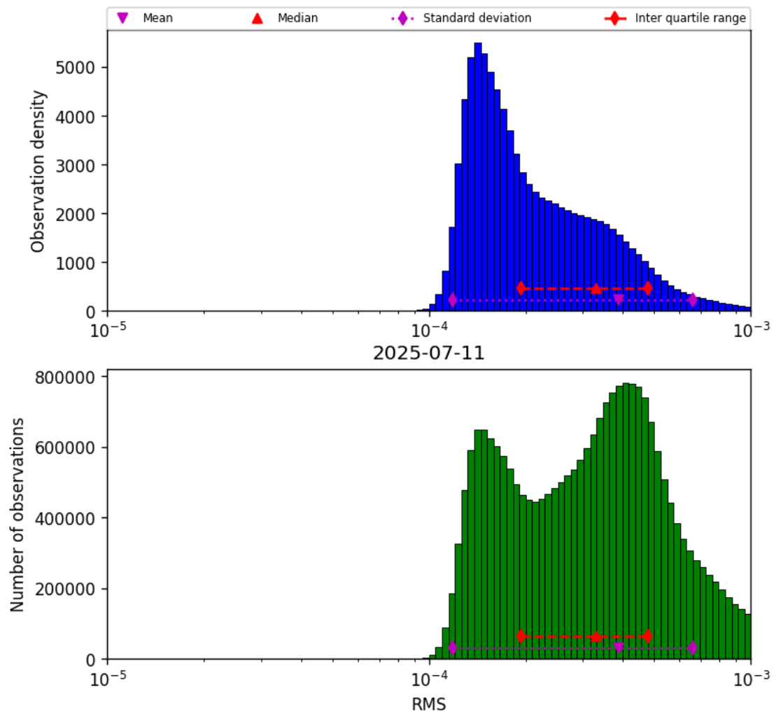
Figure 41: Histogram of “RMS” for 2025-07-11 to 2025-07-11
