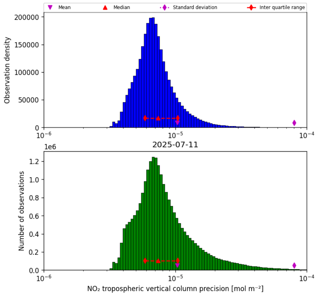
Figure 28: Histogram of "NO 2 tropospheric vertical column precision" for 2025-07-11 to 2025-07-11
