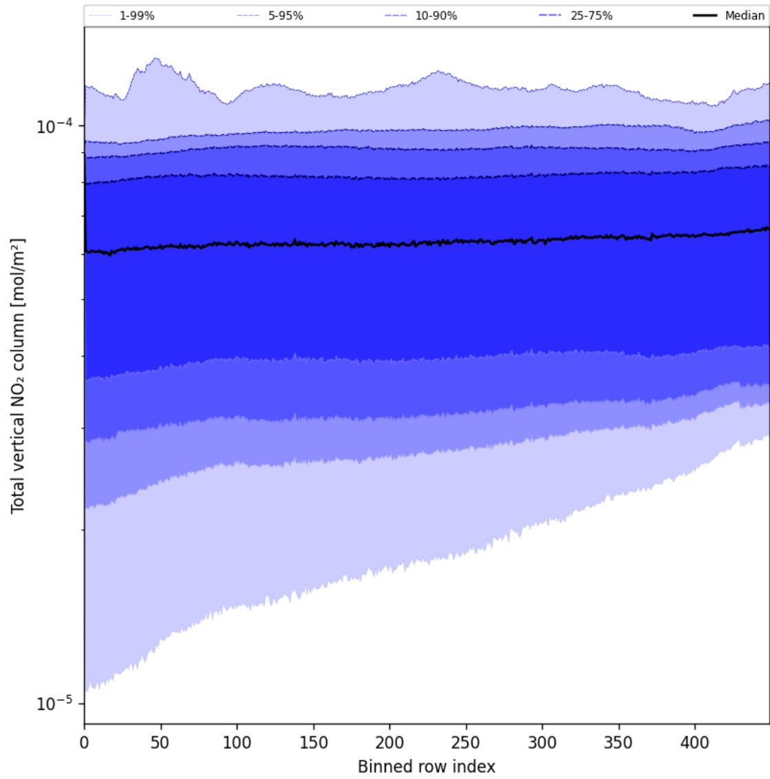
Figure 53: Along track statistics of “Total vertical NO 2 column” for 2025-07-11 to 2025-07-11
