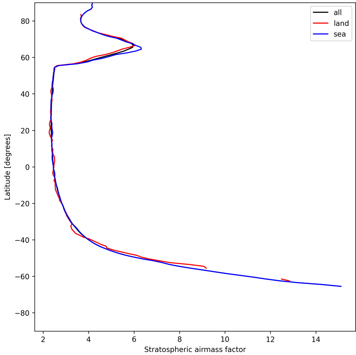
Figure 25: Zonal average of “Stratospheric air mass factor” for 2025-07-11 to 2025-07-11.
