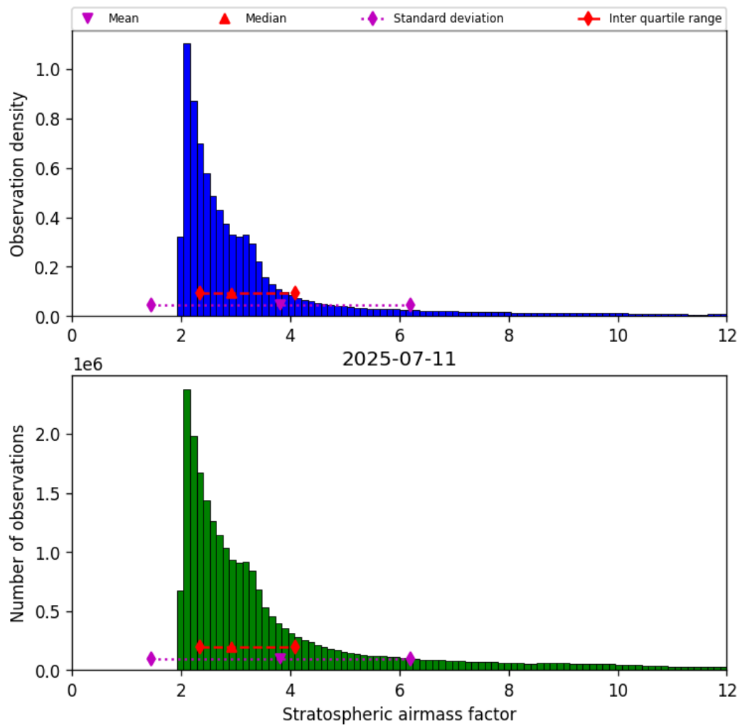
Figure 42: Histogram of “Stratospheric airmass factor” for 2025-07-11 to 2025-07-11
