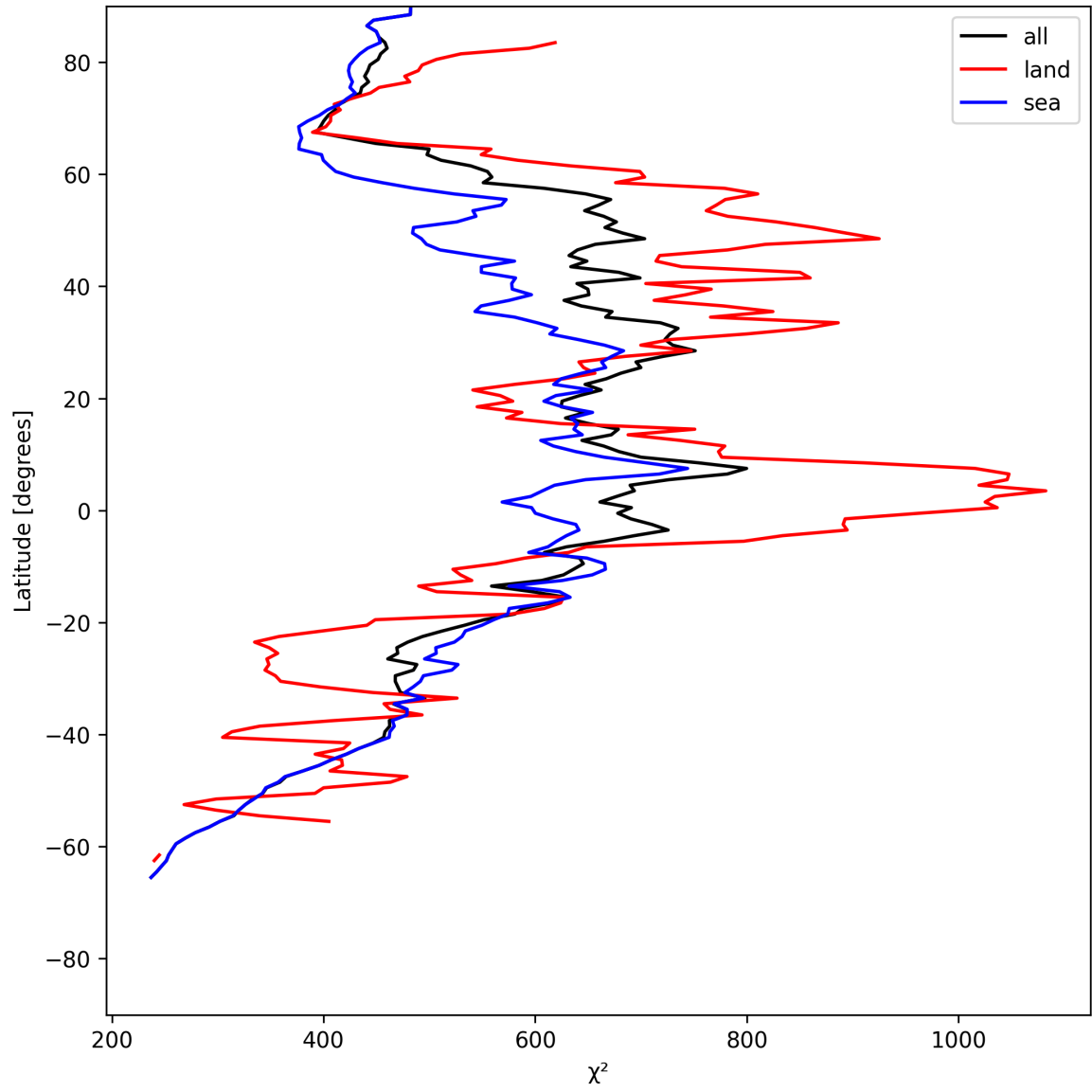
Figure 23: Zonal average of “ \chi^2 ” for 2025-07-11 to 2025-07-11.
