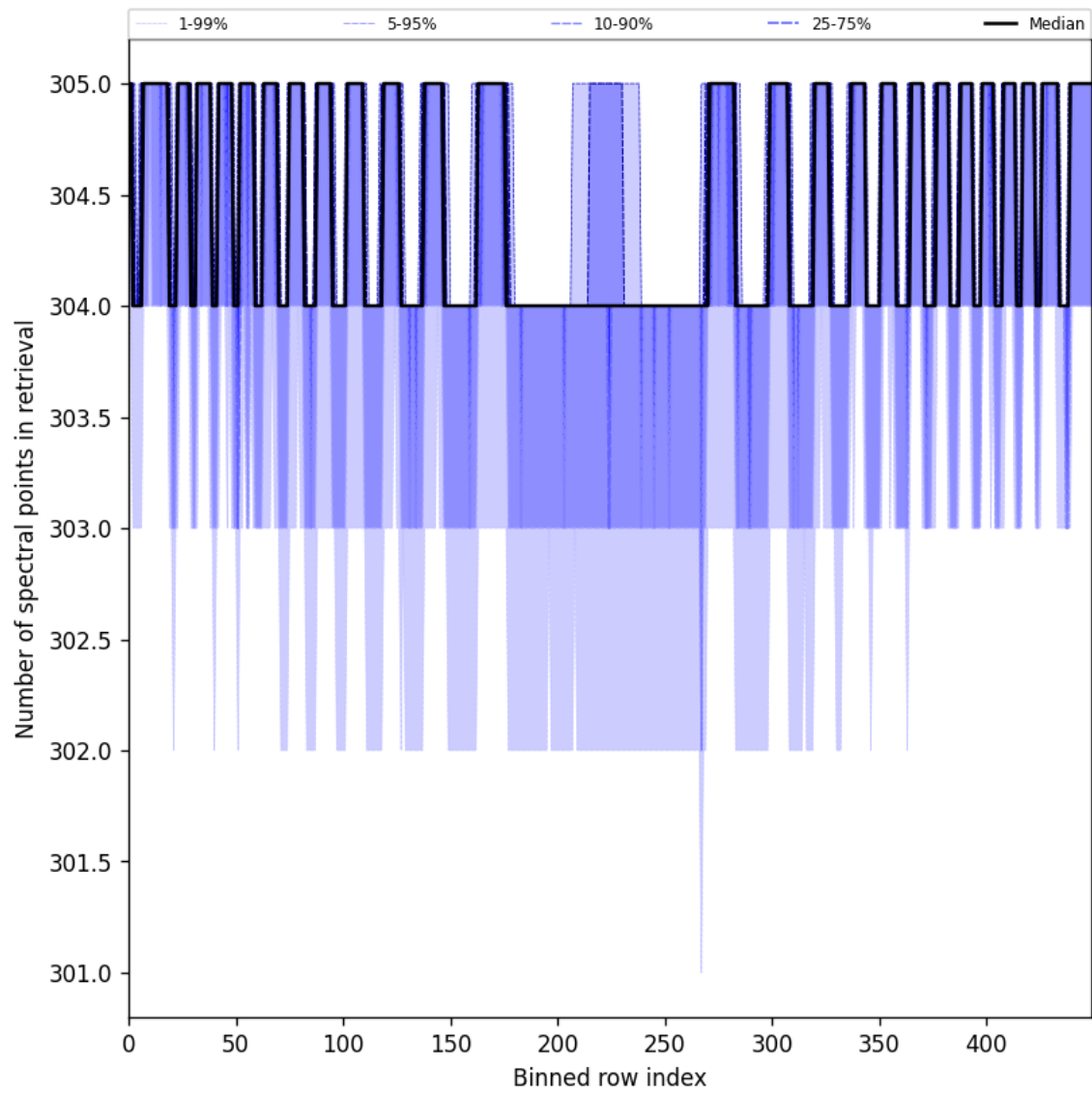
Figure 48: Along track statistics of “Number of spectral points in retrieval” for 2025-07-11 to 2025-07-11
