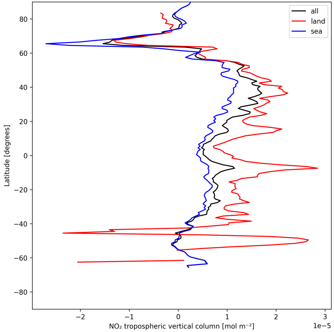
Figure 10: Zonal average of “NO 2 tropospheric vertical column” for 2025-07-11 to 2025-07-11.
