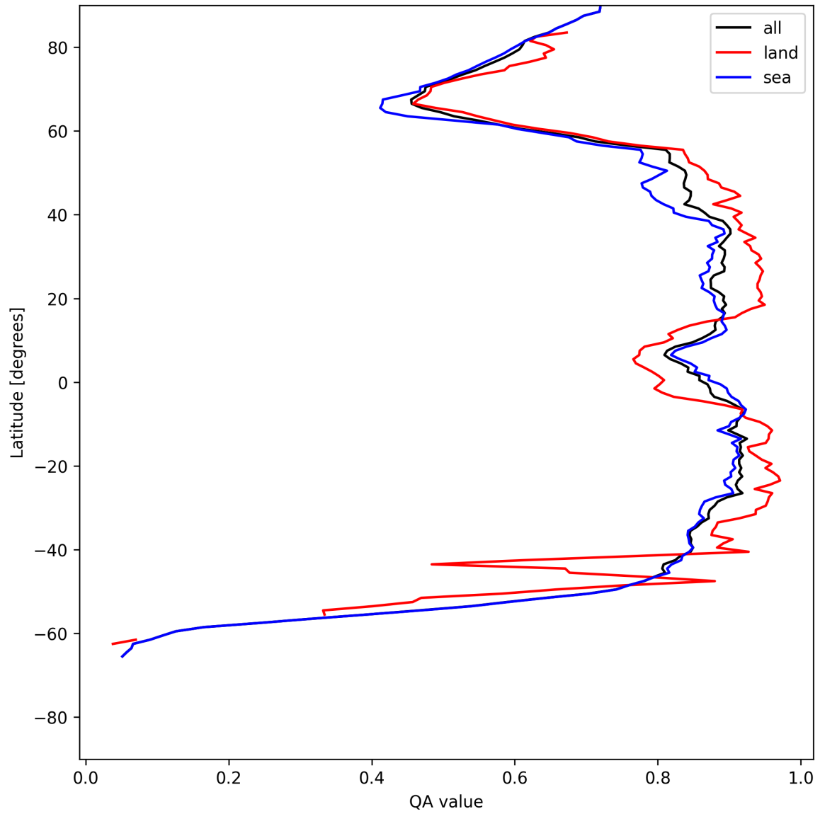
Figure 9: Zonal average of “QA value” for 2025-07-11 to 2025-07-11.
