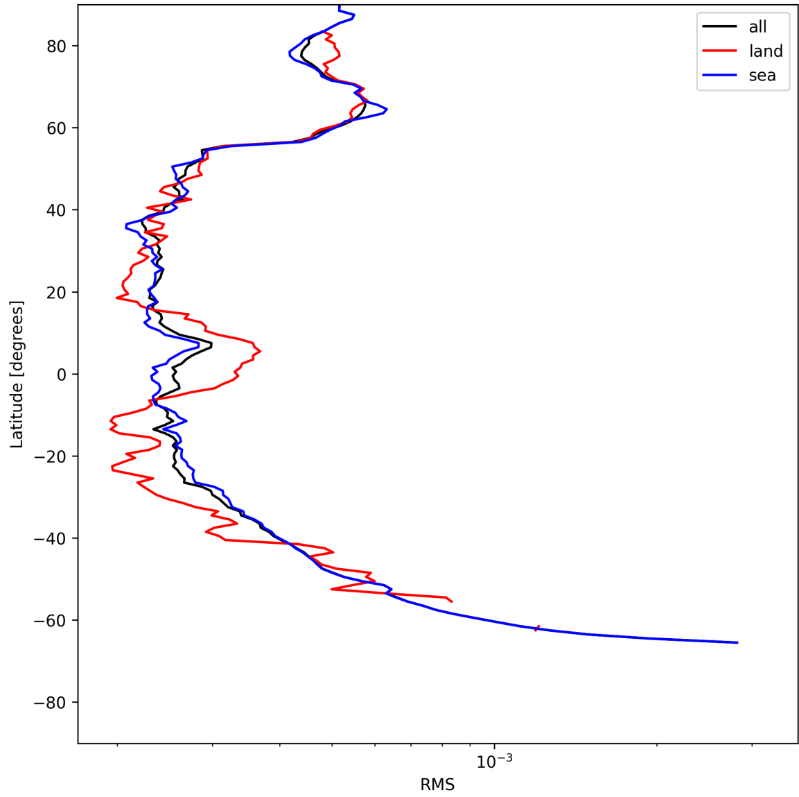
Figure 24: Zonal average of “RMS” for 2025-07-11 to 2025-07-11.
