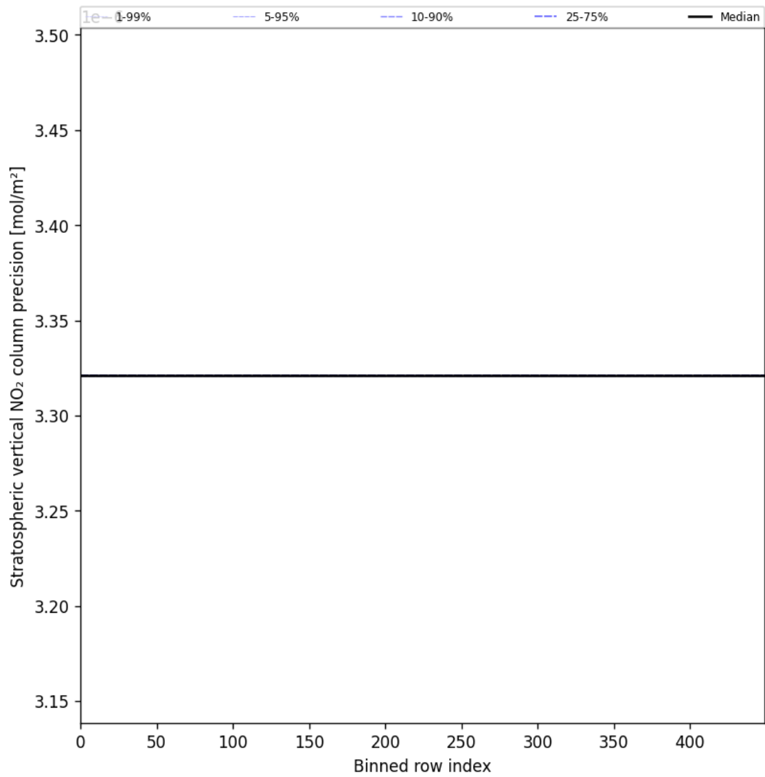
Figure 52: Along track statistics of “Stratospheric vertical NO 2 column precision” for 2025-07-11 to 2025-07-11
