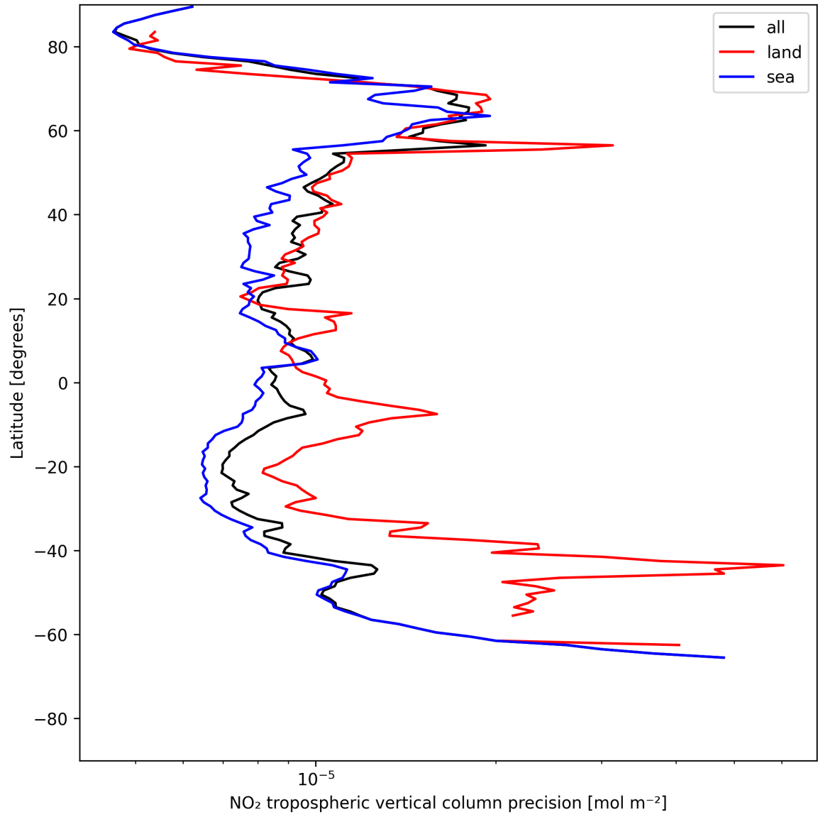
Figure 11: Zonal average of “NO 2 tropospheric vertical column precision” for 2025-07-11 to 2025-07-11.
