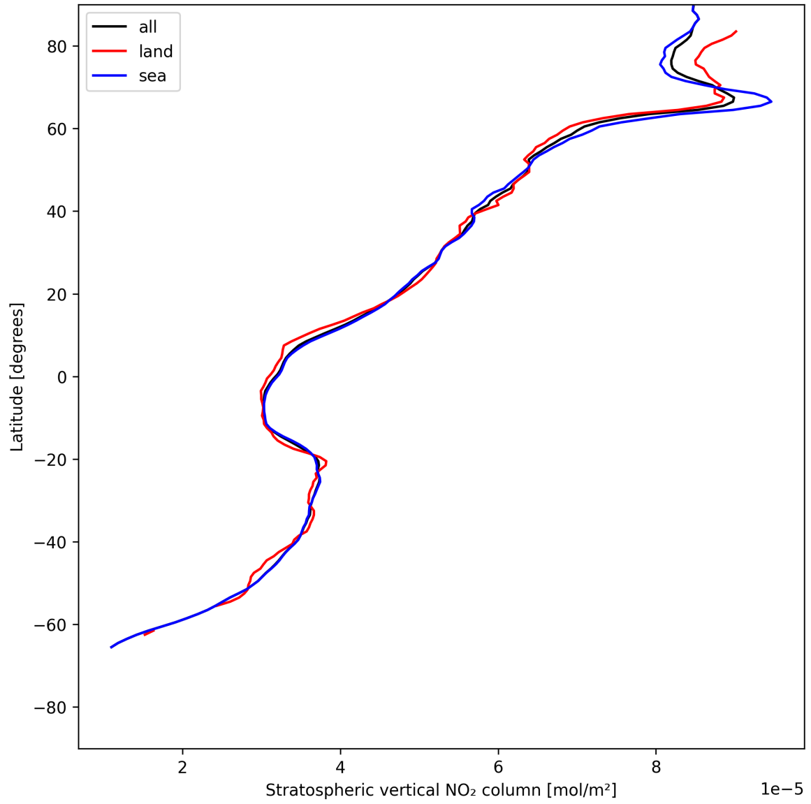
Figure 17: Zonal average of “Stratospheric vertical NO 2 column” for 2025-07-11 to 2025-07-11.
