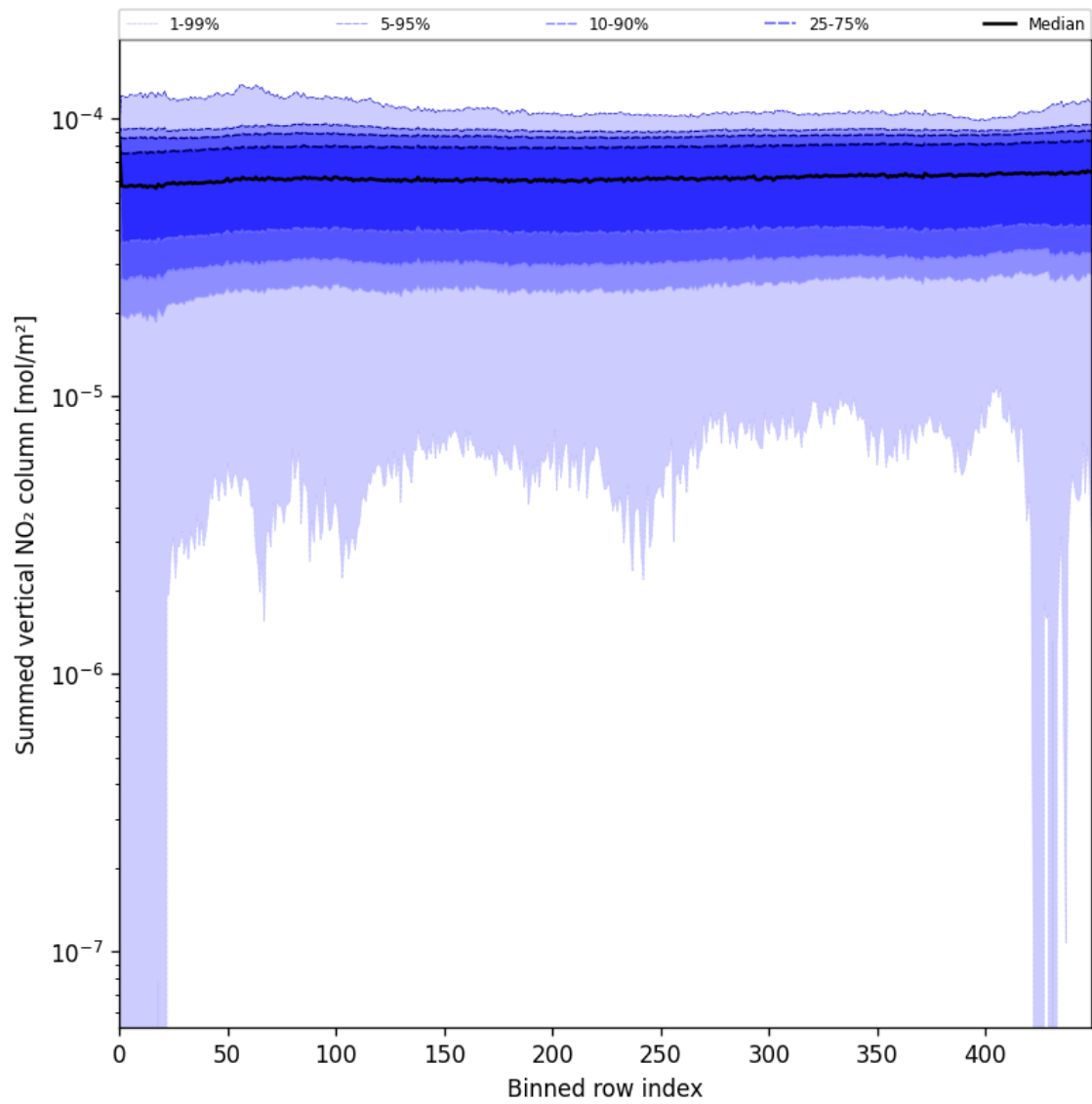
Figure 55: Along track statistics of “Summed vertical NO 2 column” for 2025-07-11 to 2025-07-11
