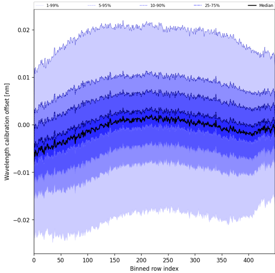
Figure 50: Along track statistics of “Wavelength calibration offset” for 2025-07-11 to 2025-07-11
