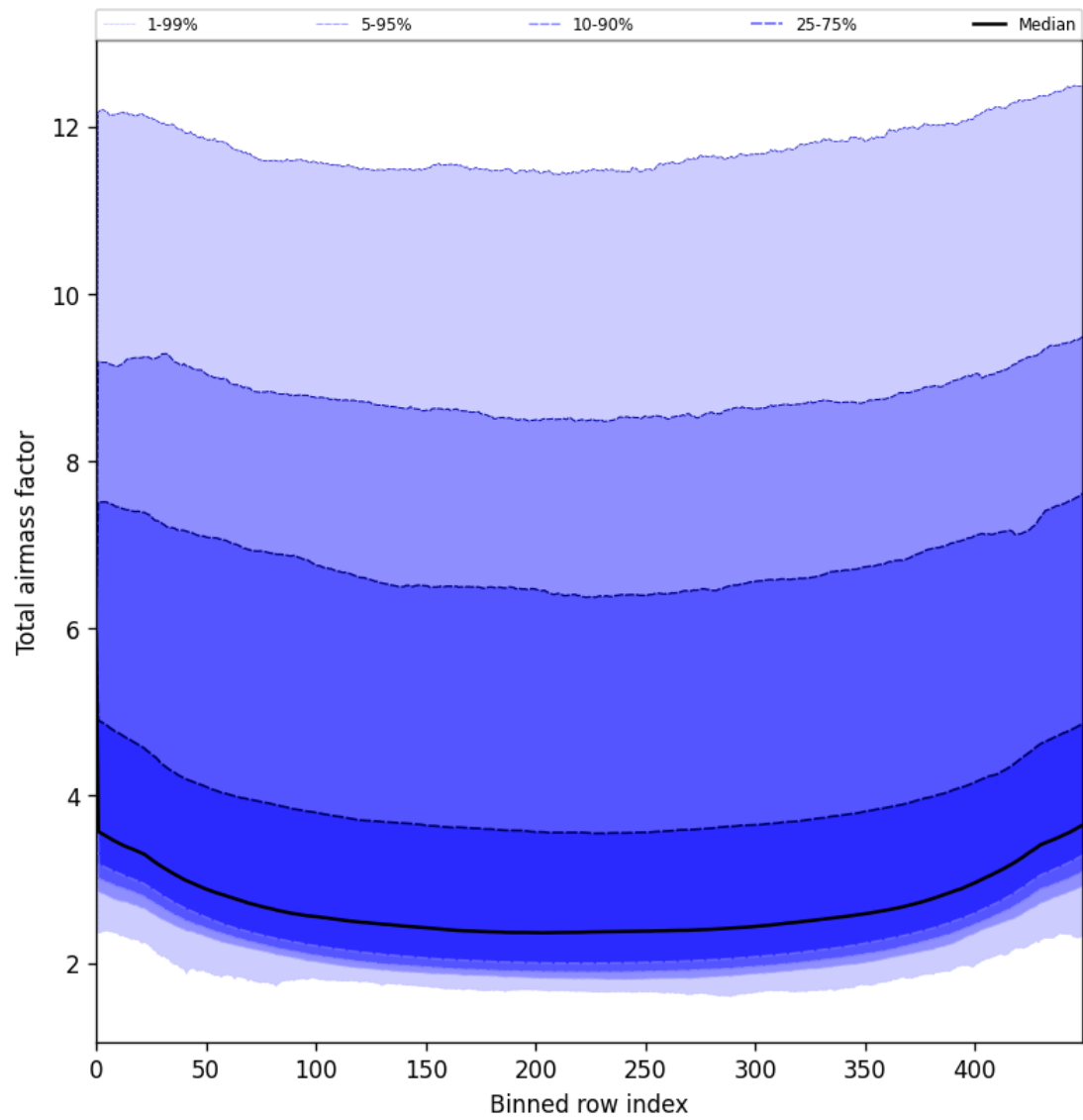
Figure 47: Along track statistics of “Total airmass factor” for 2025-07-11 to 2025-07-11
