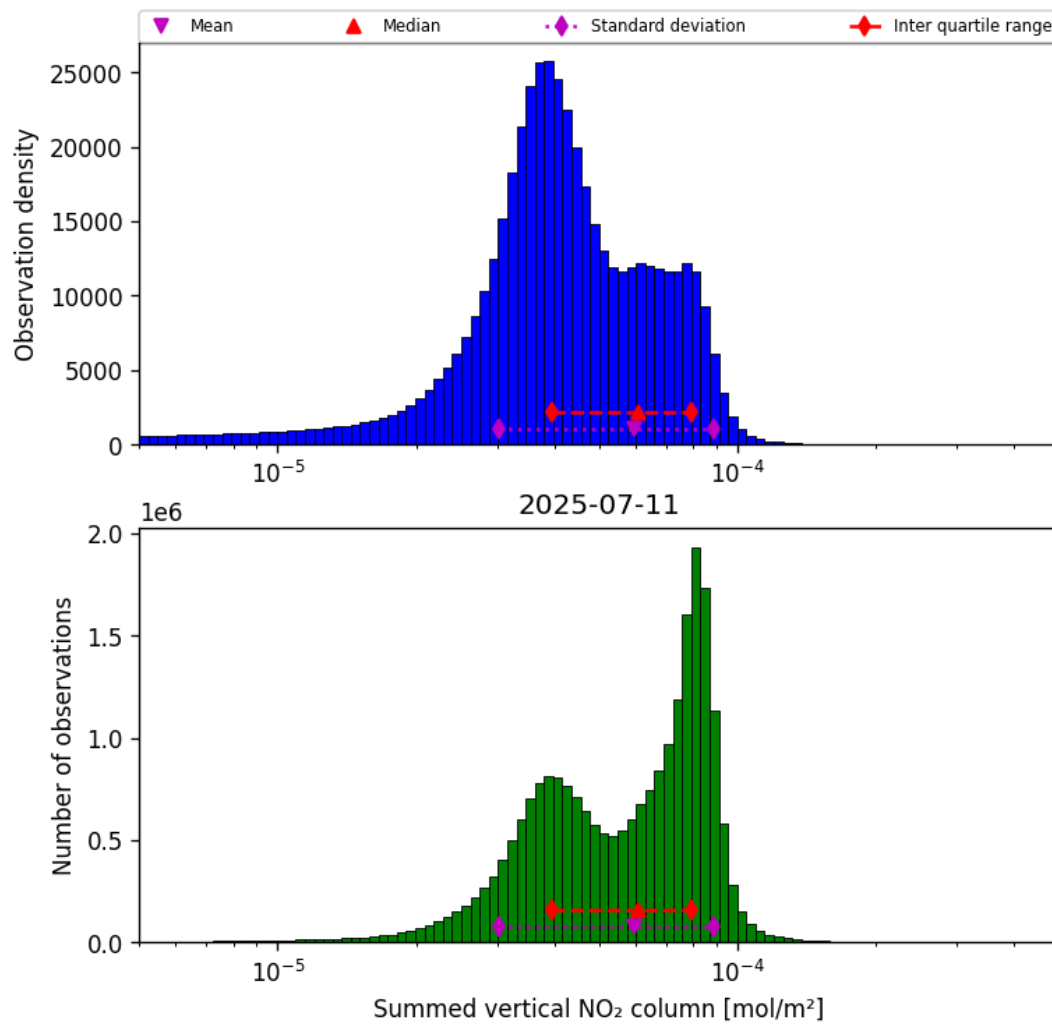
Figure 38: Histogram of "Summed vertical NO 2 column" for 2025-07-11 to 2025-07-11
