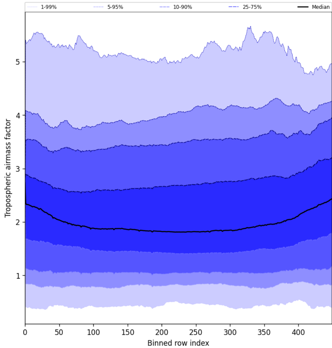
Figure 46: Along track statistics of “Tropospheric airmass factor” for 2025-07-11 to 2025-07-11
