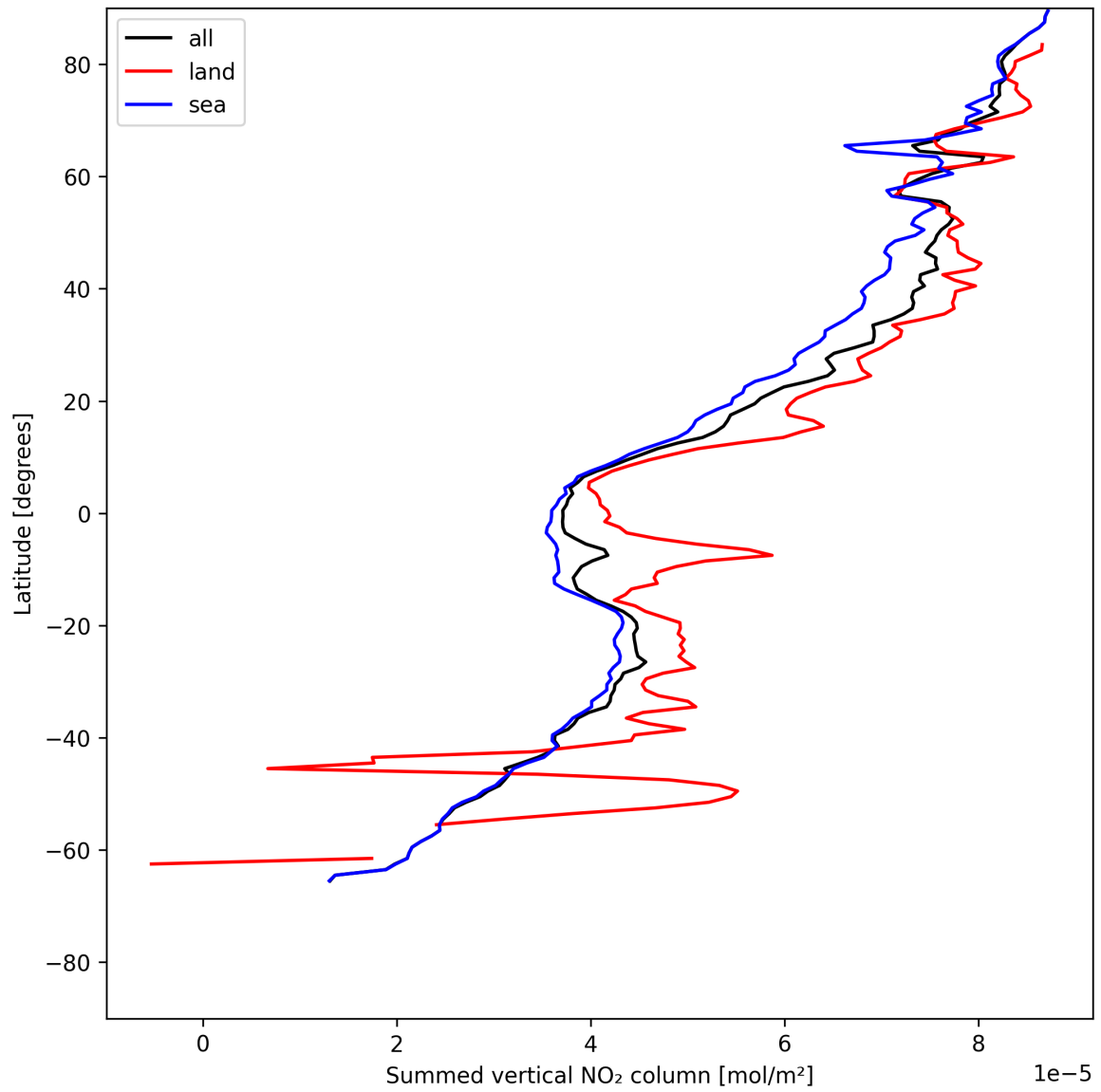
Figure 21: Zonal average of “Summed vertical NO 2 column” for 2025-07-11 to 2025-07-11.
