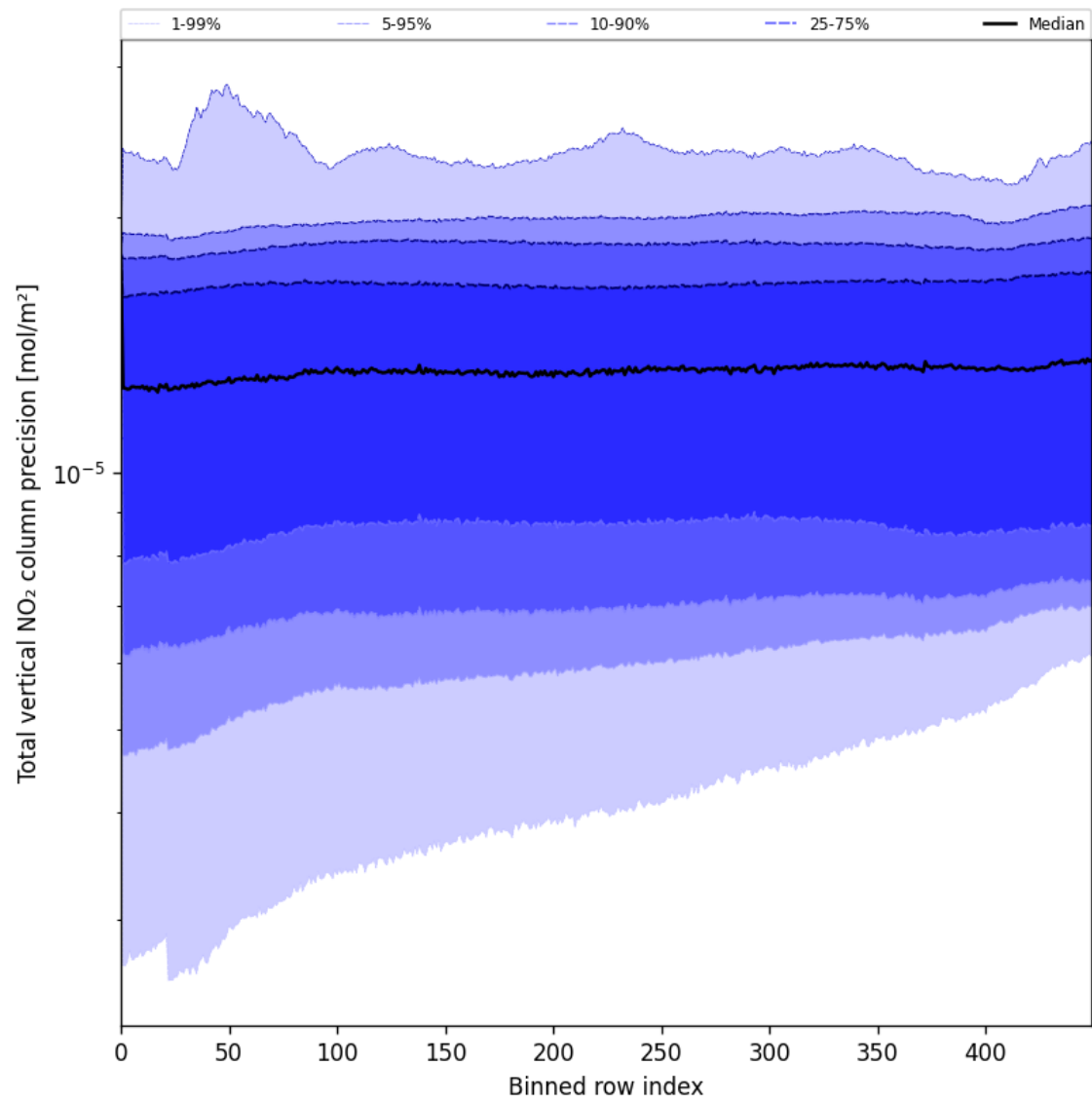
Figure 54: Along track statistics of “Total vertical NO 2 column precision” for 2025-07-11 to 2025-07-11
