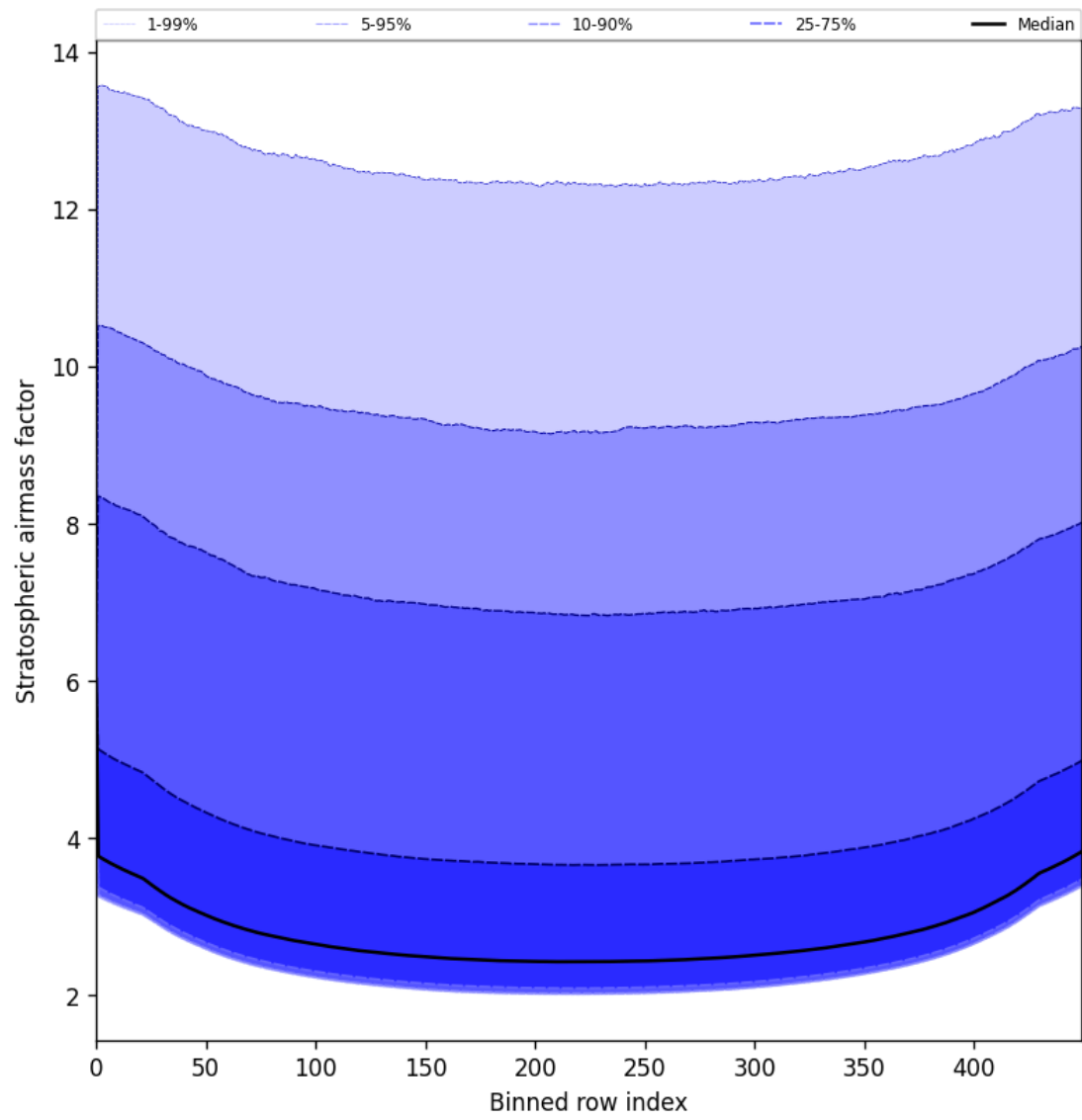
Figure 59: Along track statistics of “Stratospheric airmass factor” for 2025-07-11 to 2025-07-11
