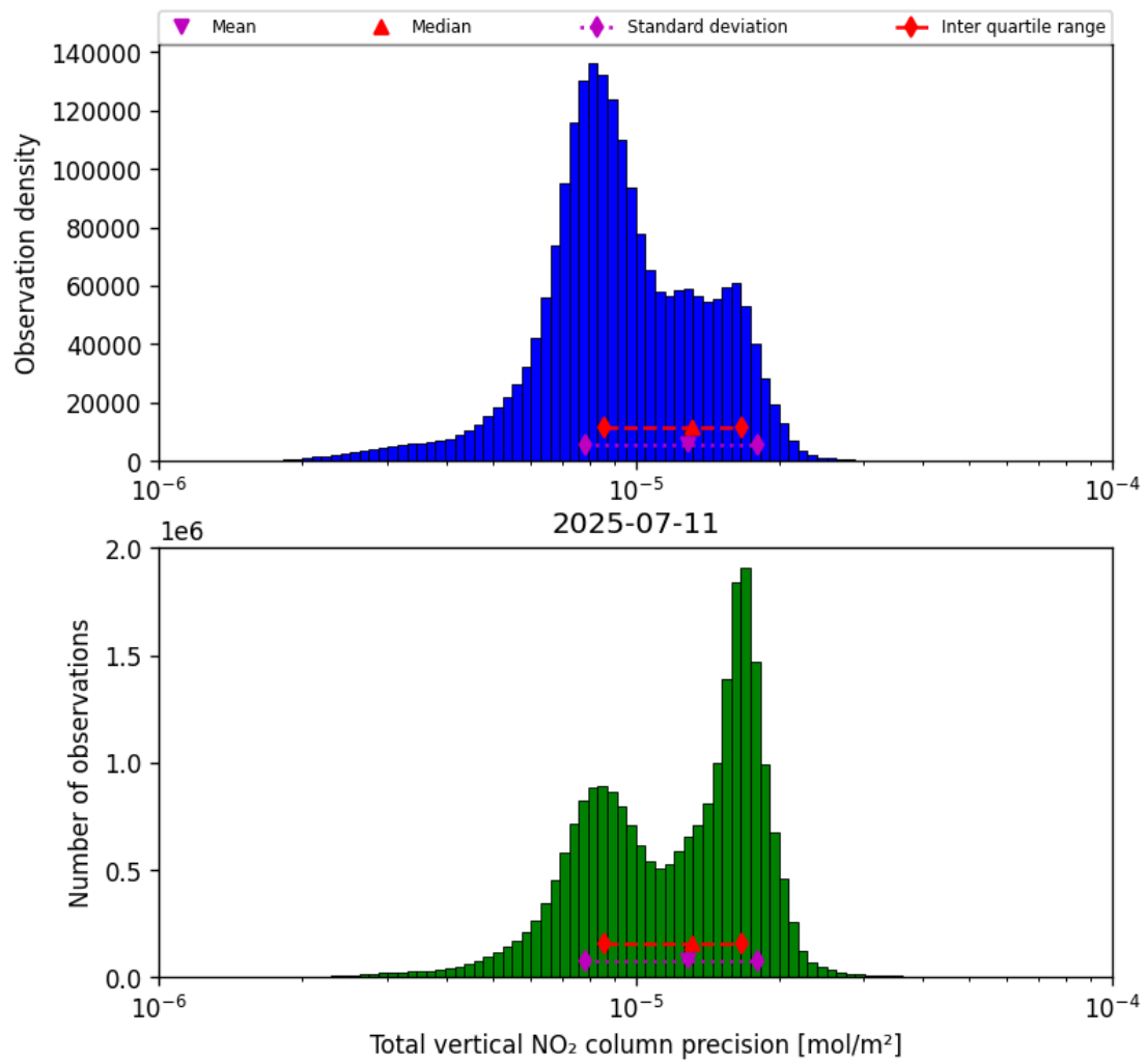
Figure 37: Histogram of "Total vertical NO 2 column precision" for 2025-07-11 to 2025-07-11
