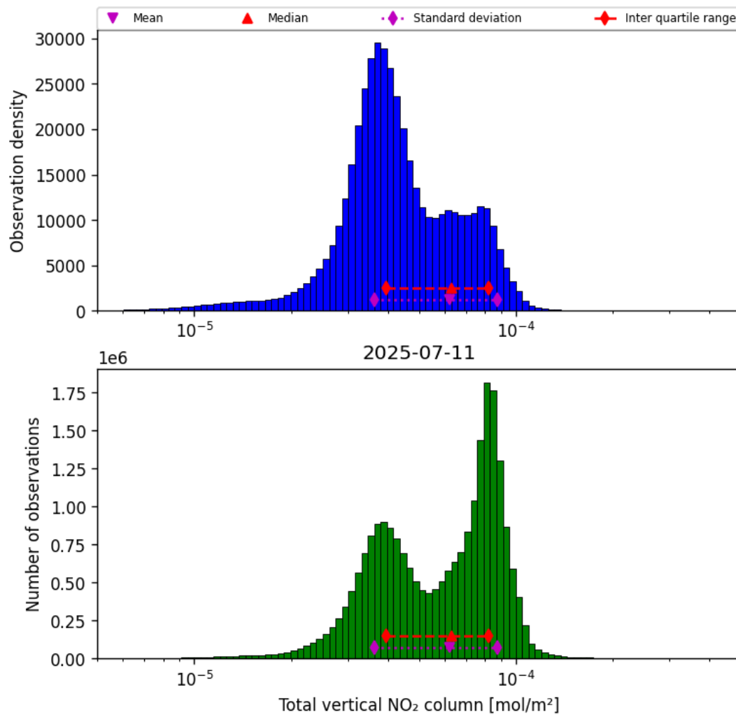
Figure 36: Histogram of "Total vertical NO 2 column" for 2025-07-11 to 2025-07-11
