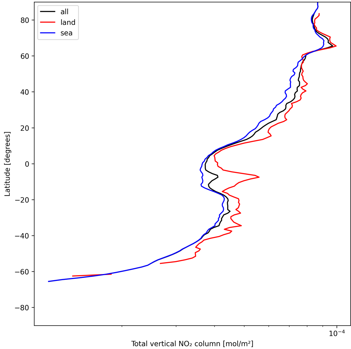
Figure 19: Zonal average of “Total vertical NO 2 column” for 2025-07-11 to 2025-07-11.
