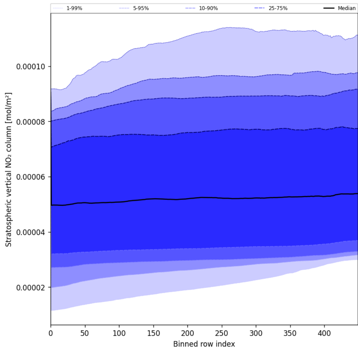
Figure 51: Along track statistics of “Stratospheric vertical NO 2 column” for 2025-07-11 to 2025-07-11
