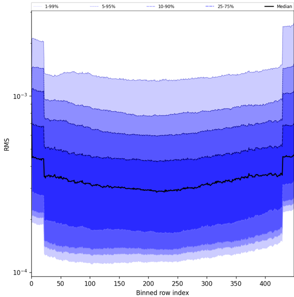
Figure 58: Along track statistics of “RMS” for 2025-07-11 to 2025-07-11
