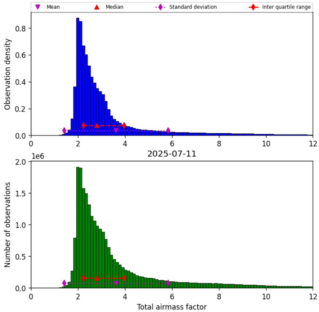
Figure 30: Histogram of “Total airmass factor” for 2025-07-11 to 2025-07-11
