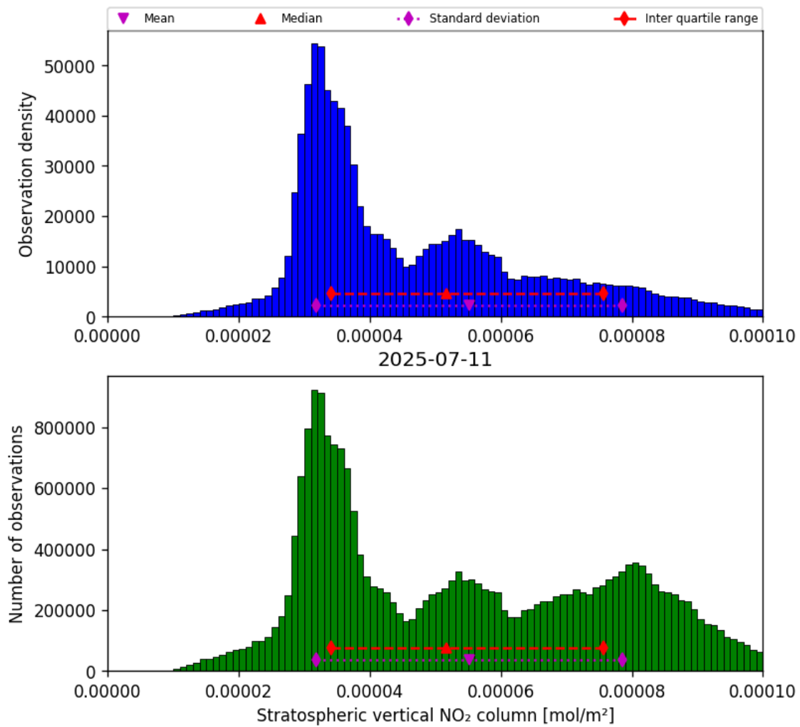
Figure 34: Histogram of “Stratospheric vertical NO 2 column” for 2025-07-11 to 2025-07-11
