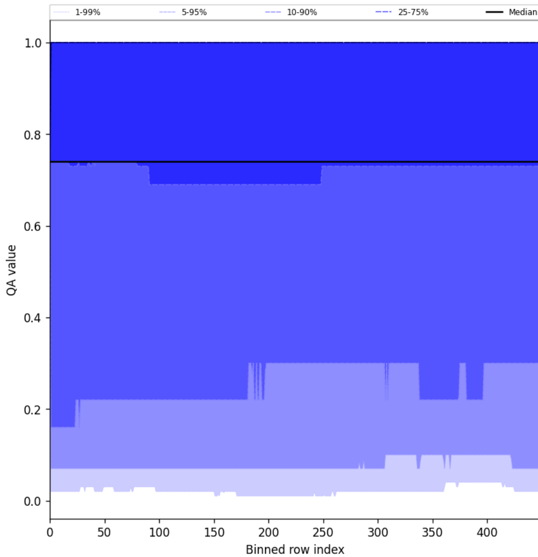
Figure 43: Along track statistics of “QA value” for 2025-07-11 to 2025-07-11
