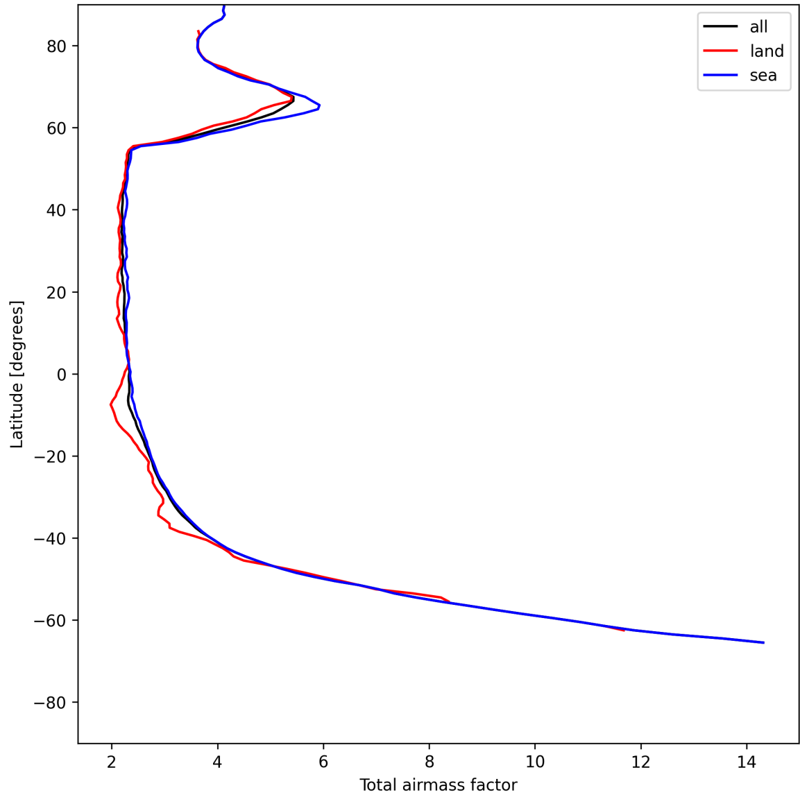
Figure 13: Zonal average of “Total airmass factor” for 2025-07-11 to 2025-07-11.
