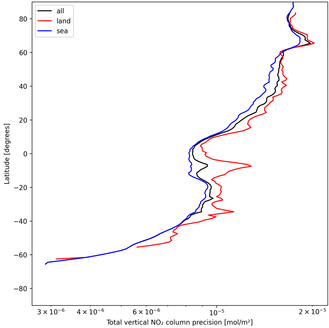
Figure 20: Zonal average of “Total vertical NO 2 column precision” for 2025-07-11 to 2025-07-11.
