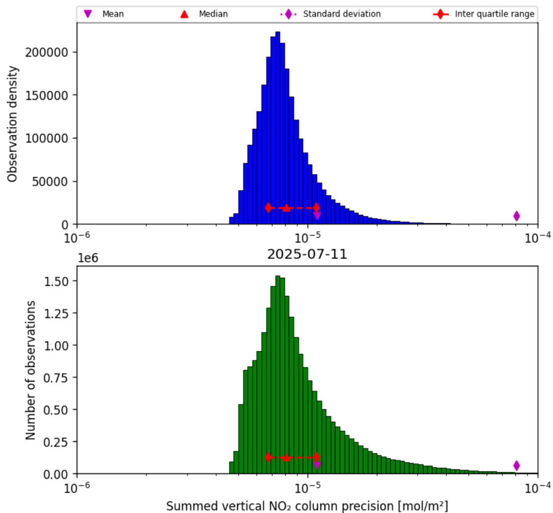
Figure 39: Histogram of "Summed vertical NO 2 column precision" for 2025-07-11 to 2025-07-11
