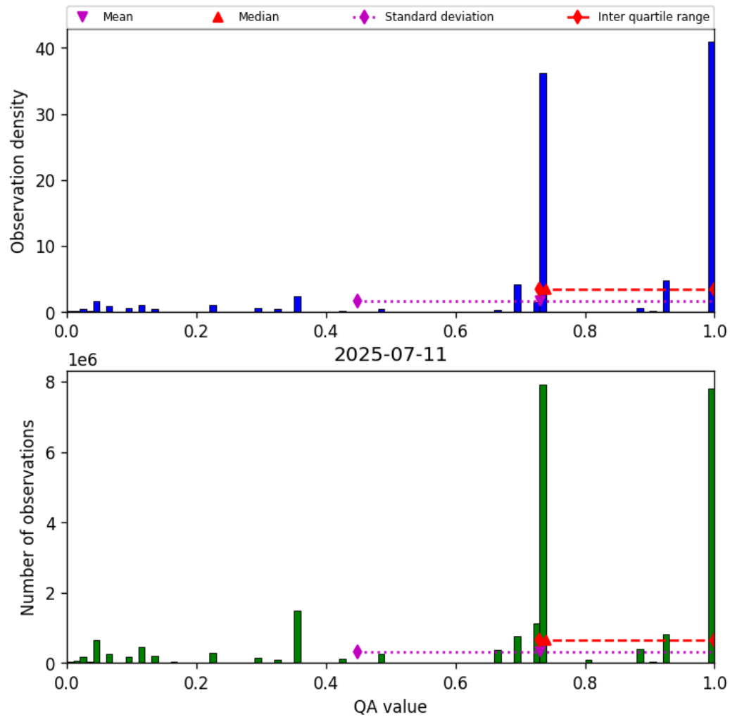
Figure 26: Histogram of “QA value” for 2025-07-11 to 2025-07-11
