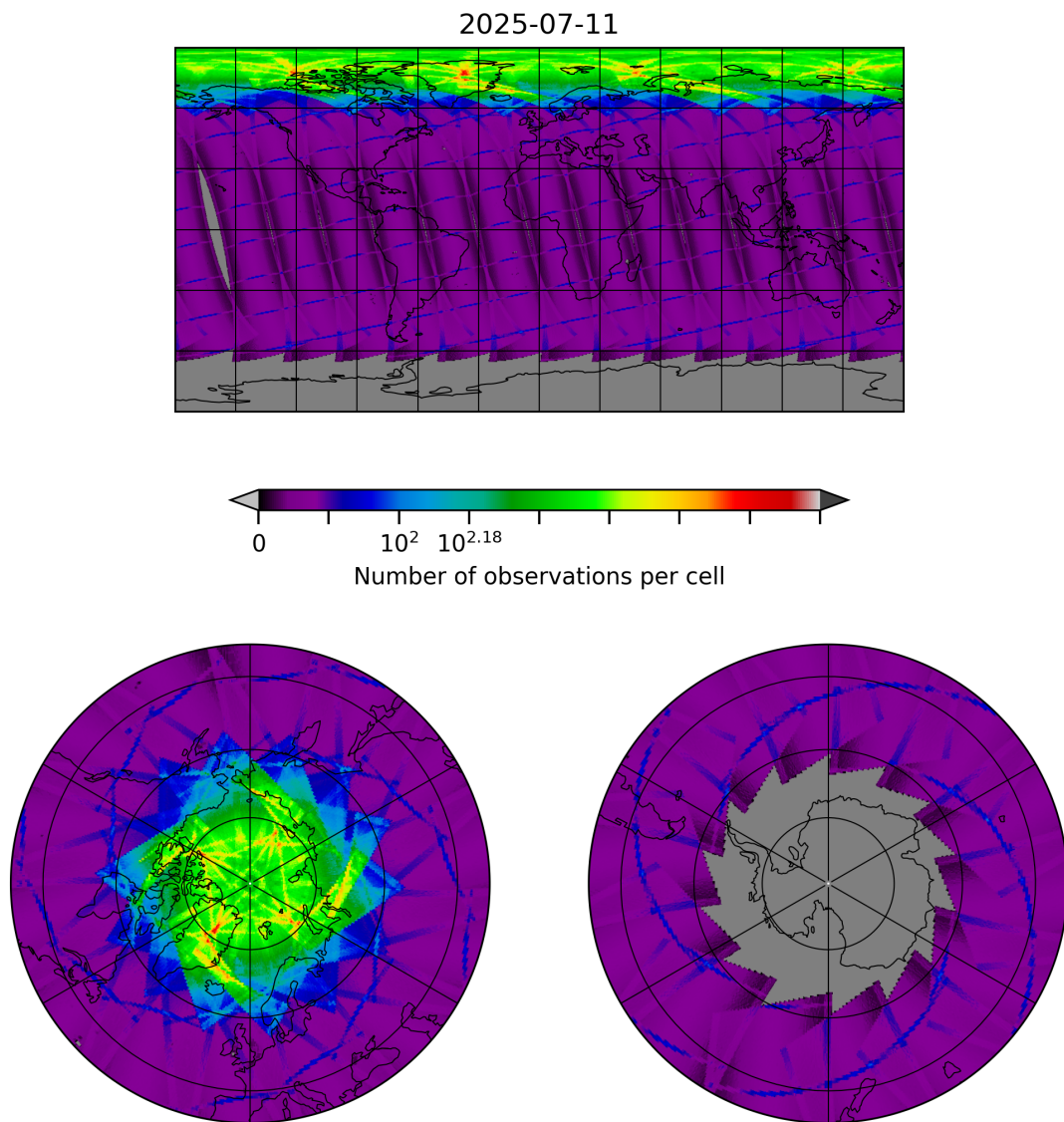
Figure 8: Map of the number of observations for 2025-07-11 to 2025-07-11
