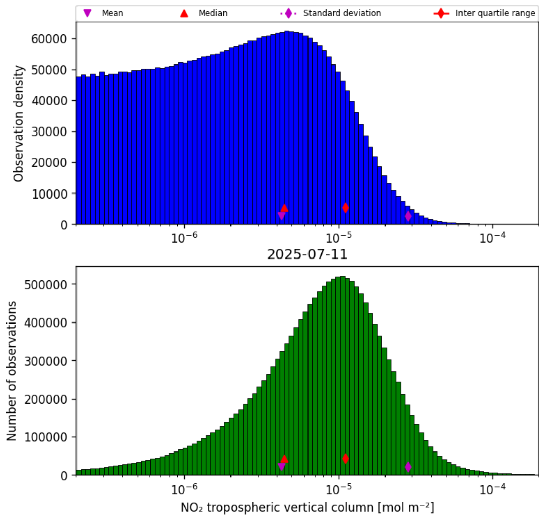
Figure 27: Histogram of “NO 2 tropospheric vertical column” for 2025-07-11 to 2025-07-11
