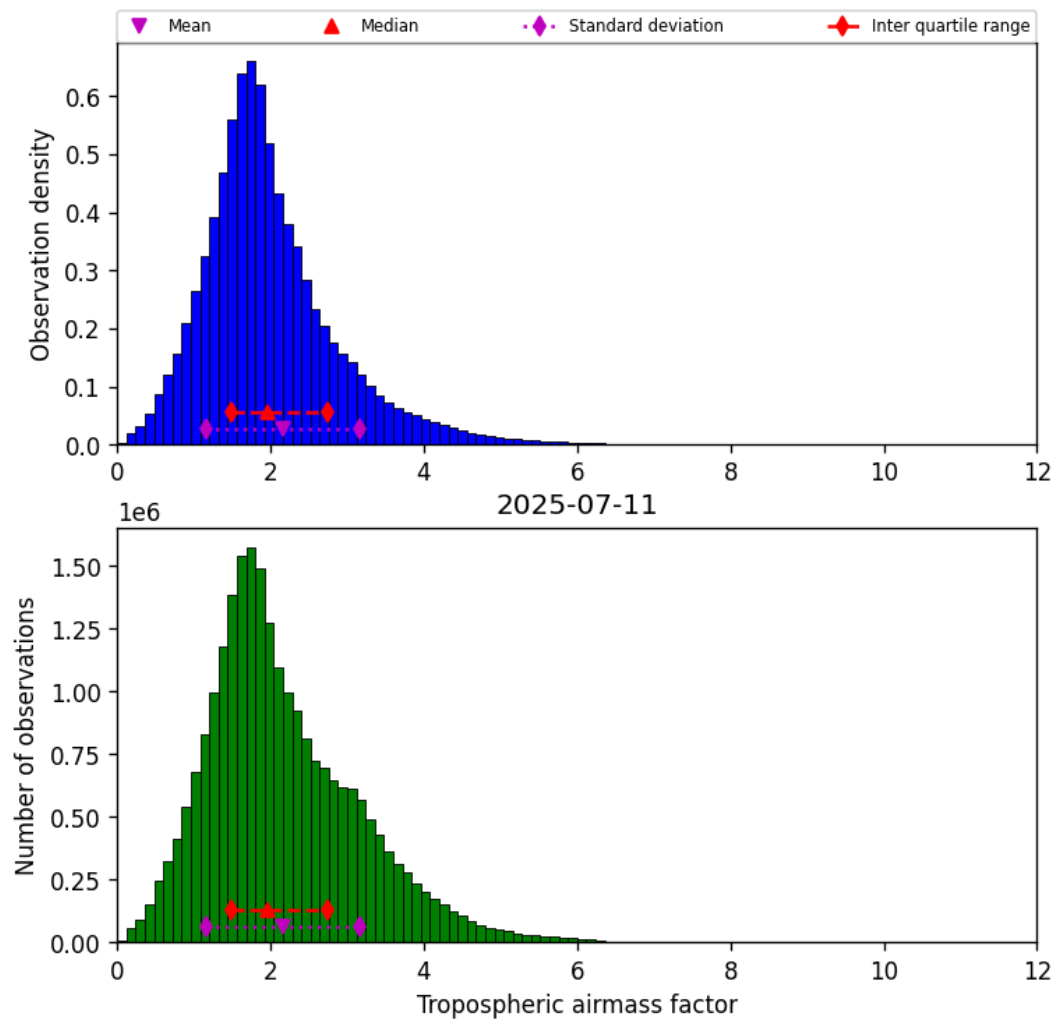
Figure 29: Histogram of “Tropospheric airmass factor” for 2025-07-11 to 2025-07-11
