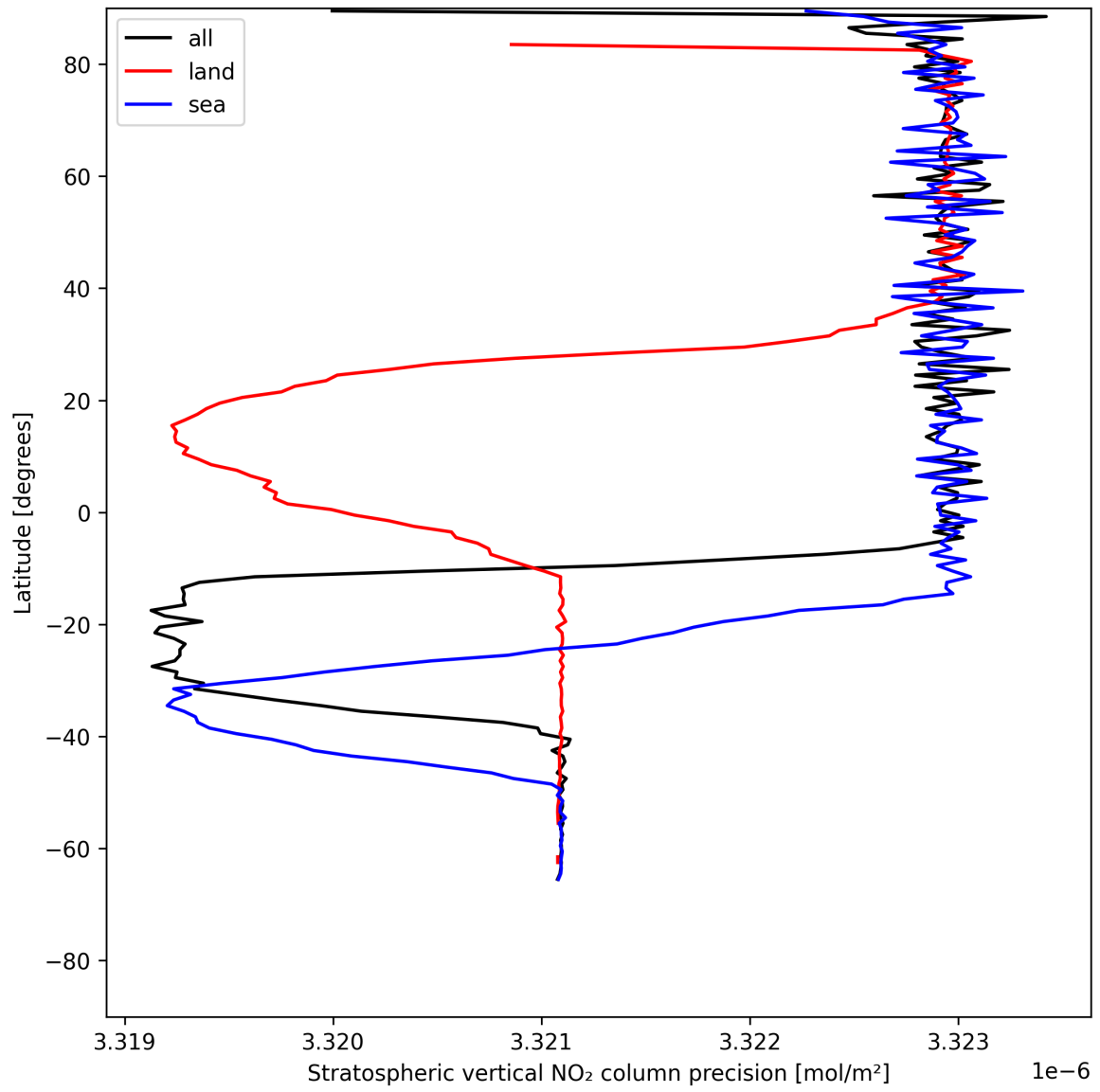
Figure 18: Zonal average of “Stratospheric vertical NO 2 column precision” for 2025-07-11 to 2025-07-11.
