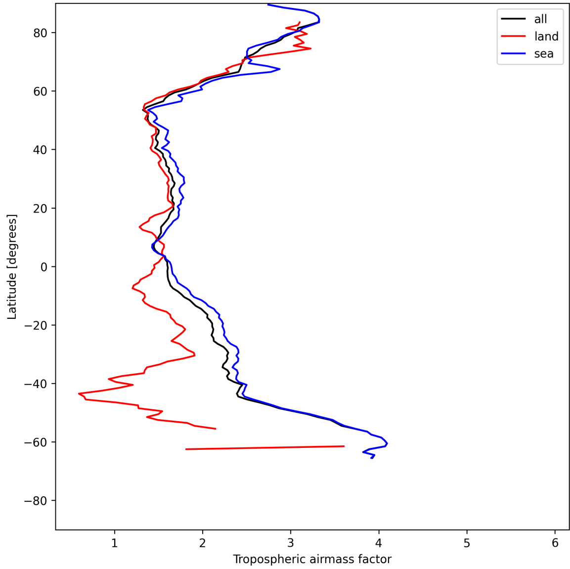
Figure 12: Zonal average of “Tropospheric airmass factor” for 2025-07-11 to 2025-07-11.
