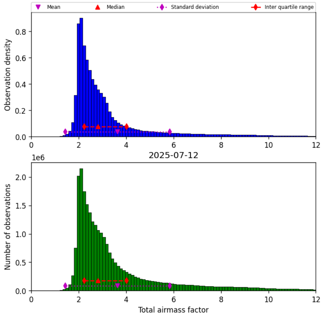
Figure 30: Histogram of “Total airmass factor” for 2025-07-12 to 2025-07-13
