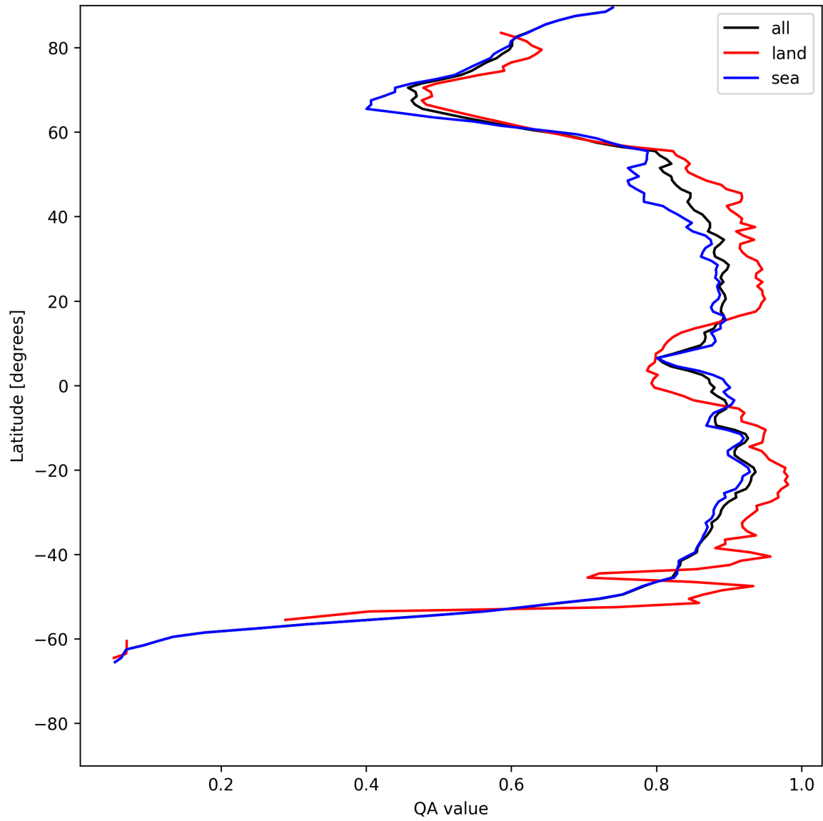
Figure 9: Zonal average of “QA value” for 2025-07-12 to 2025-07-13.
