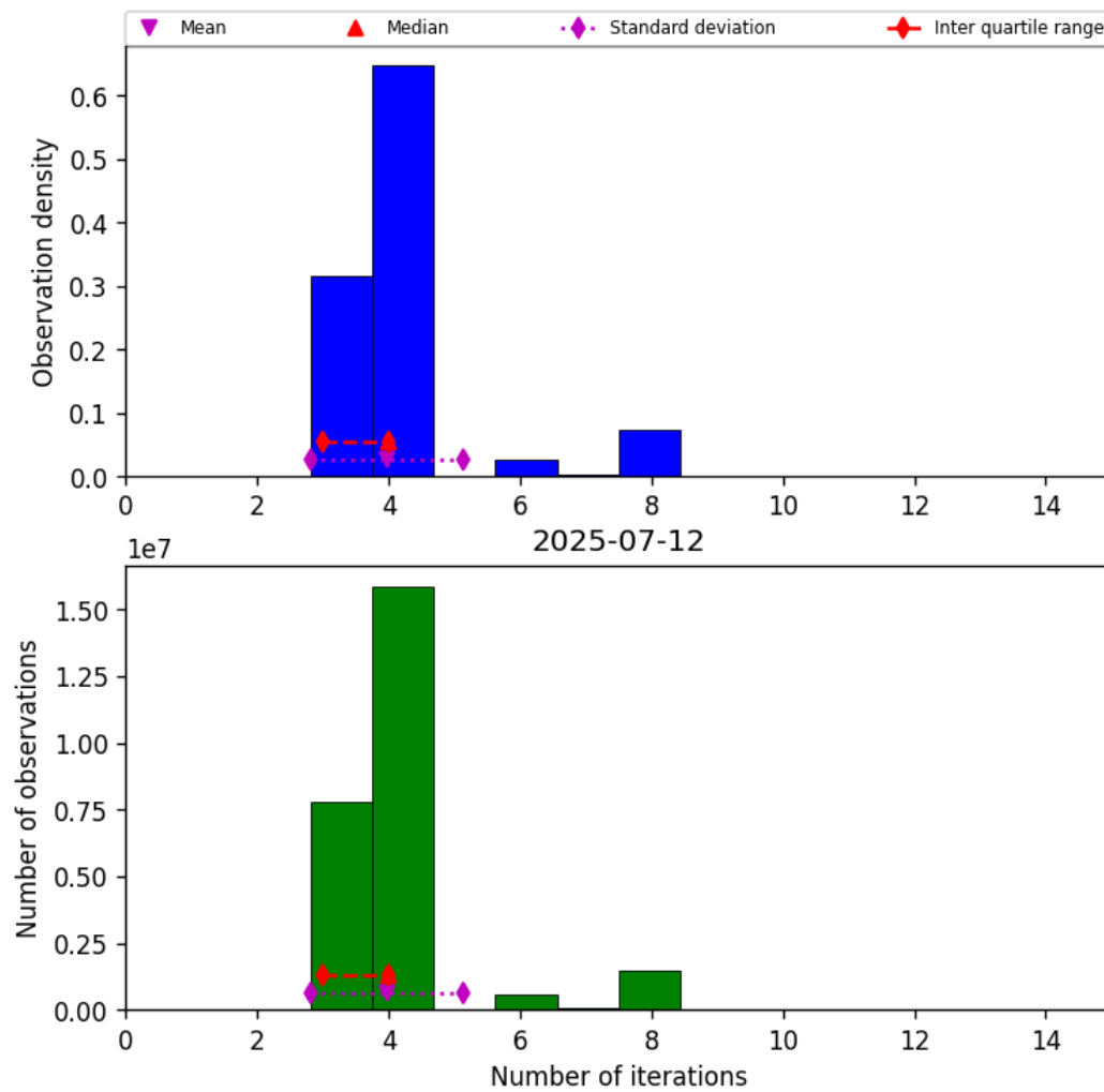
Figure 32: Histogram of “Number of iterations” for 2025-07-12 to 2025-07-13
