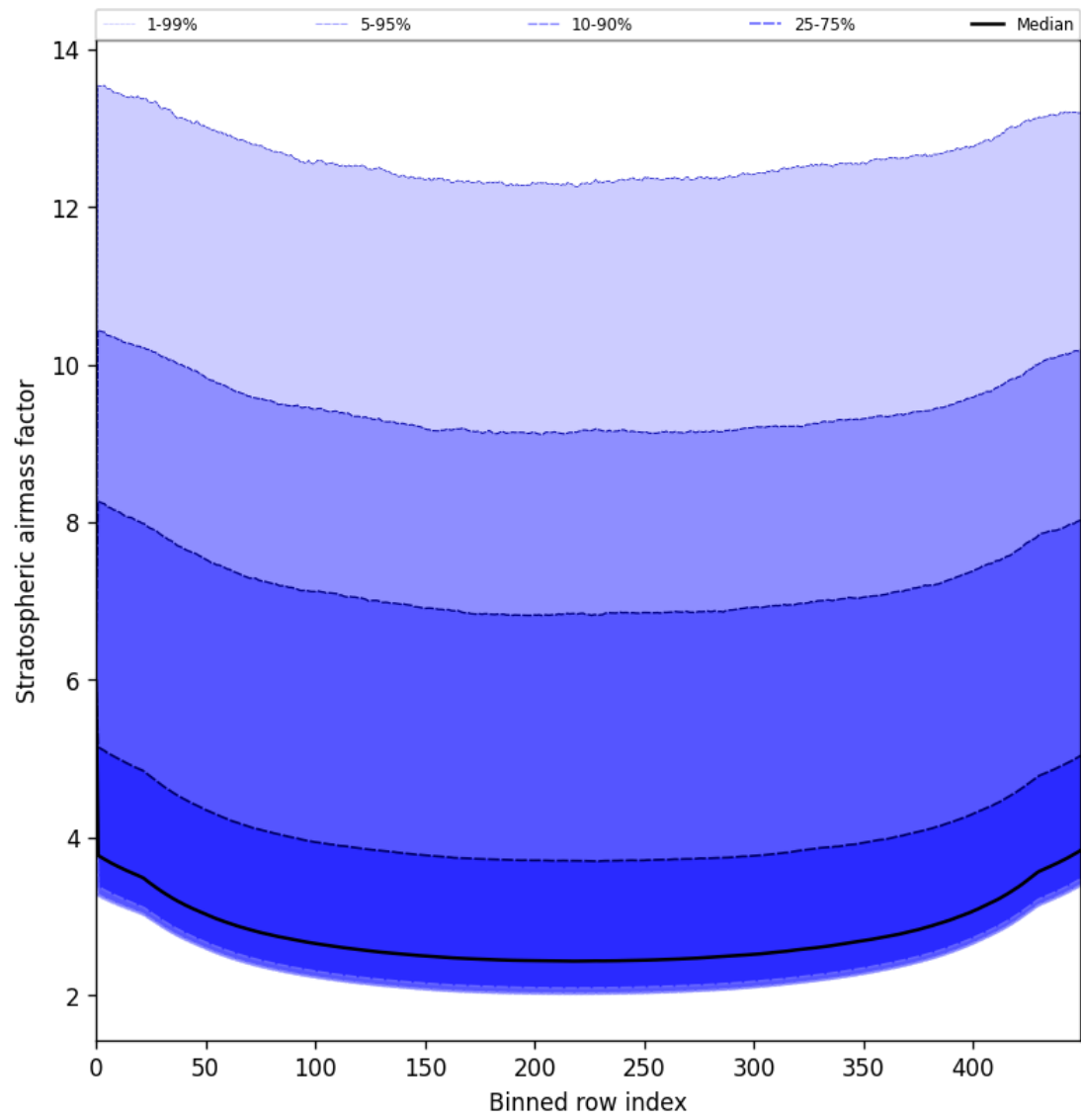
Figure 59: Along track statistics of “Stratospheric airmass factor” for 2025-07-12 to 2025-07-13
