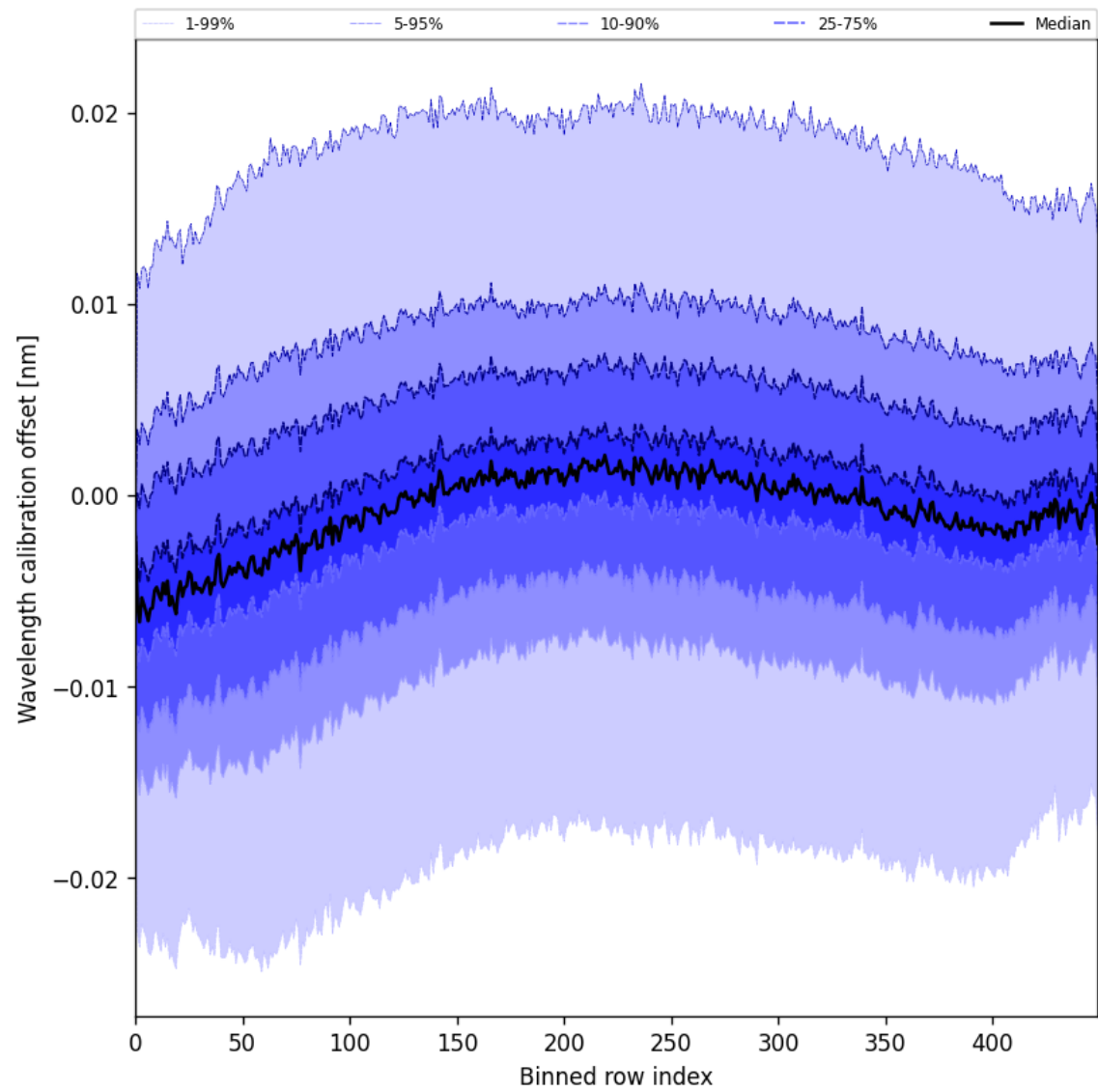
Figure 50: Along track statistics of “Wavelength calibration offset” for 2025-07-12 to 2025-07-13
