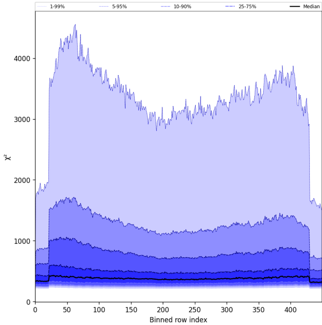
Figure 57: Along track statistics of “ \chi^2 ” for 2025-07-12 to 2025-07-13
