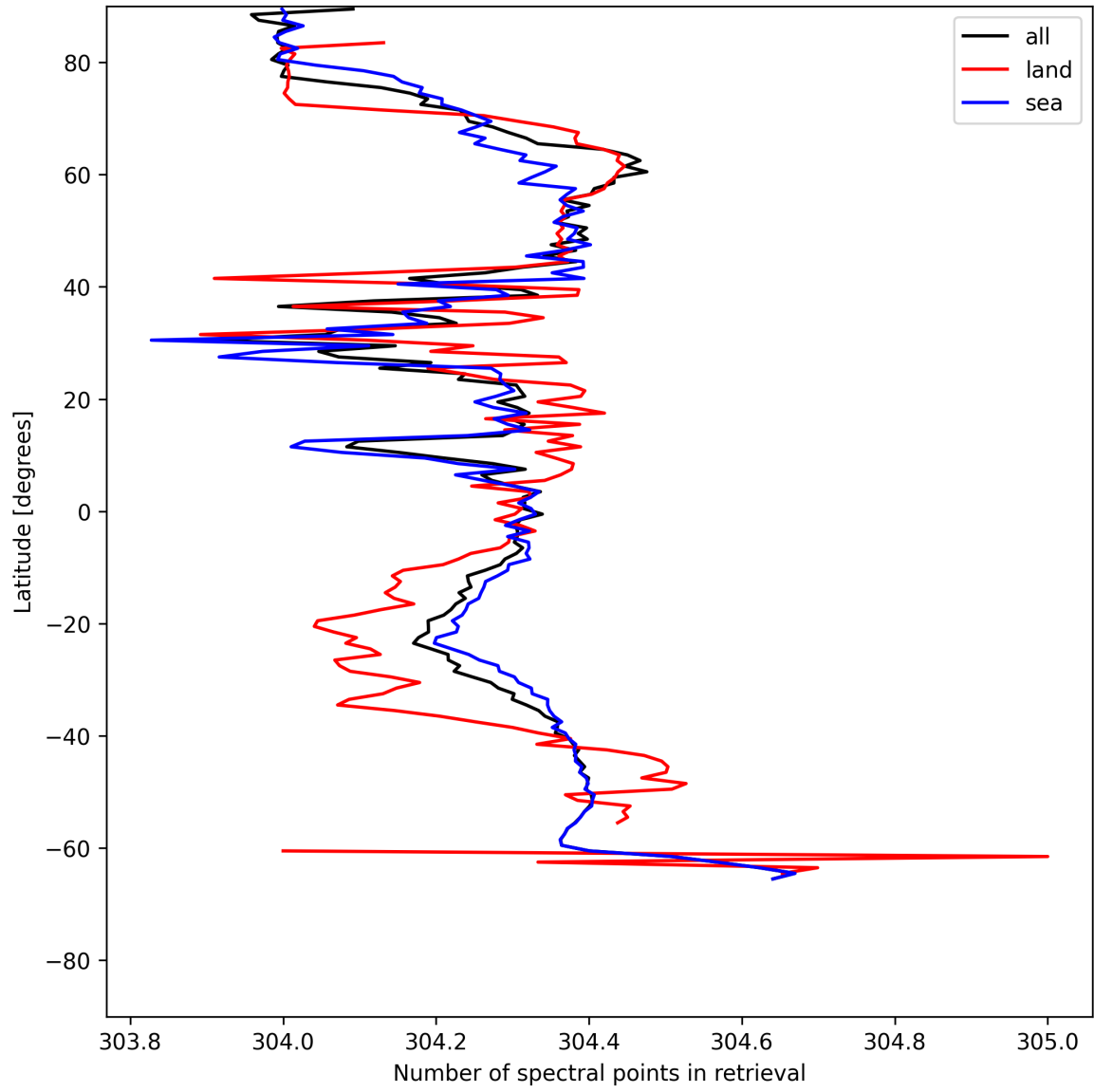
Figure 14: Zonal average of “Number of spectral points in retrieval” for 2025-07-12 to 2025-07-13.
