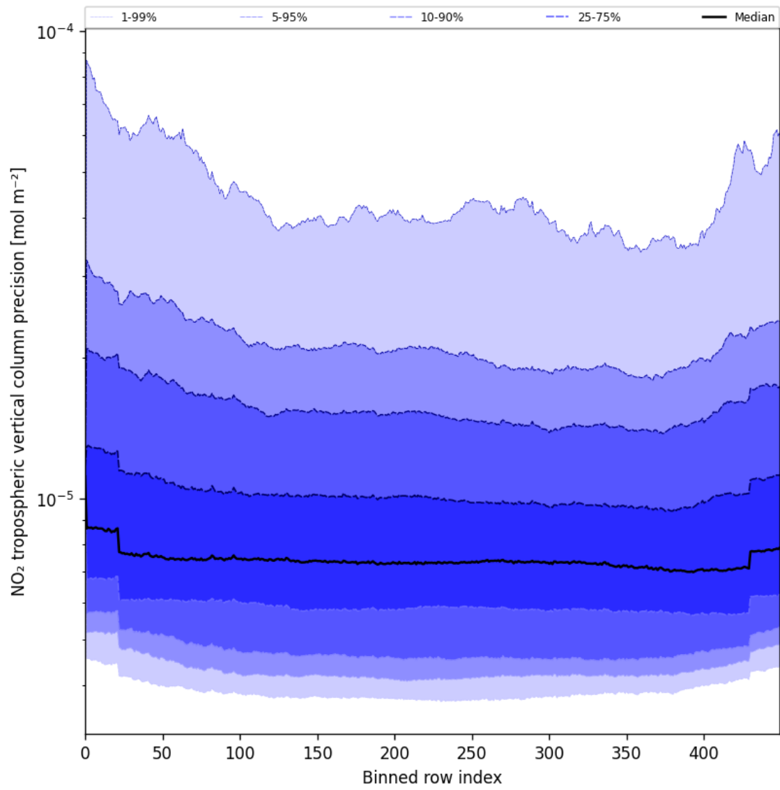
Figure 45: Along track statistics of “NO 2 tropospheric vertical column precision” for 2025-07-12 to 2025-07-13
