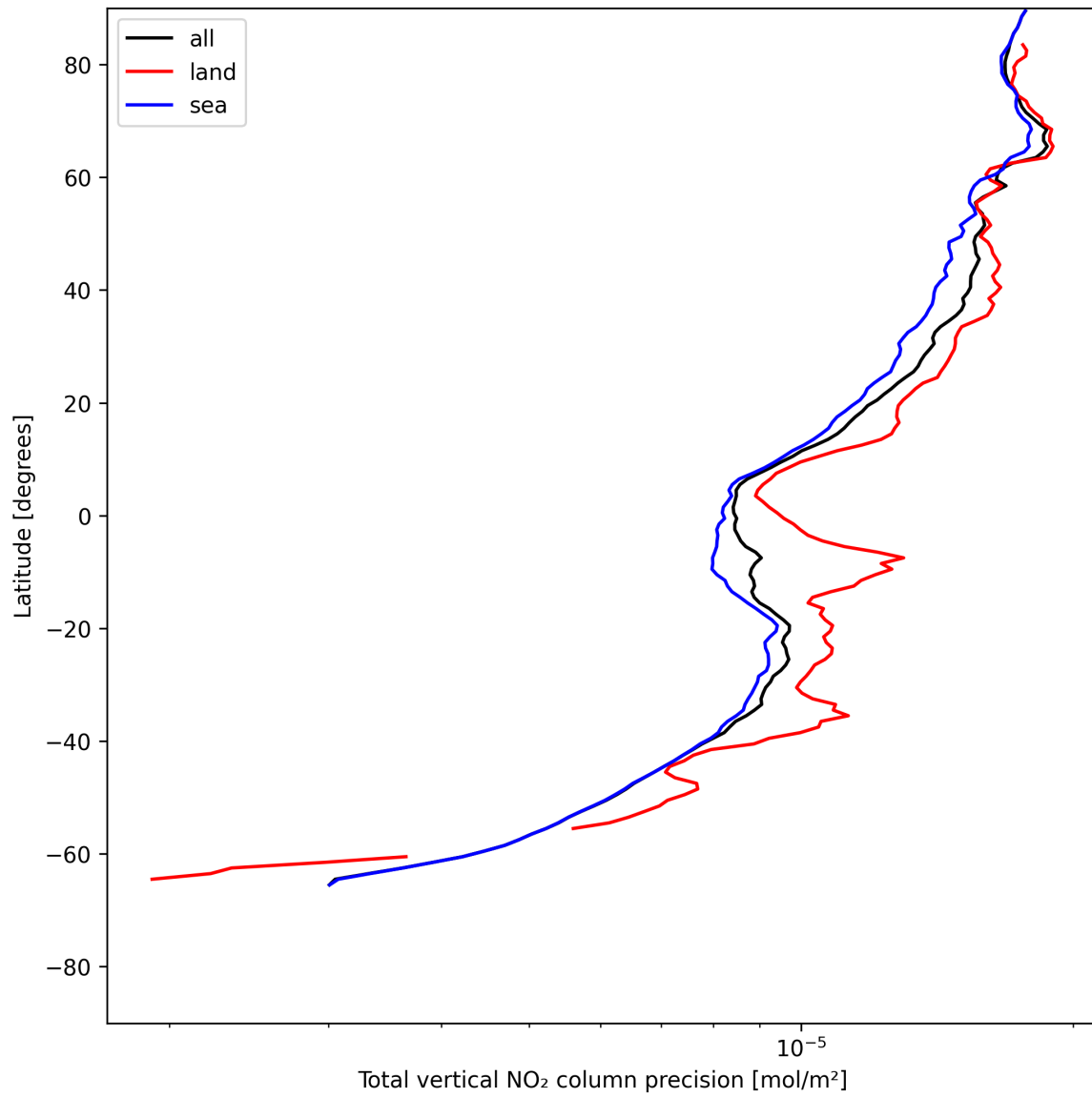
Figure 20: Zonal average of “Total vertical NO 2 column precision” for 2025-07-12 to 2025-07-13.
