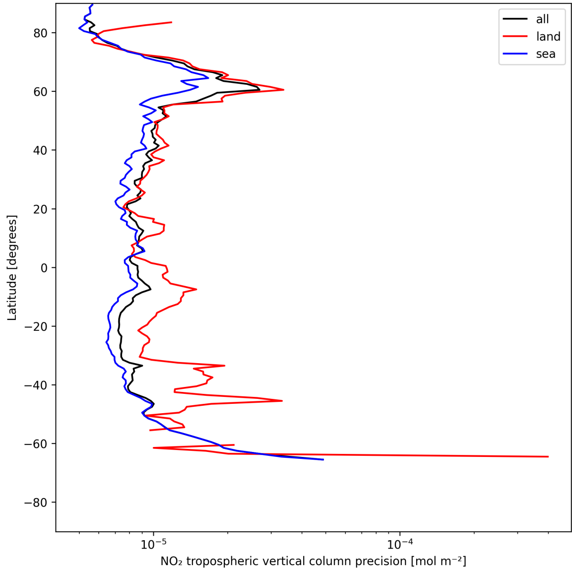
Figure 11: Zonal average of “NO 2 tropospheric vertical column precision” for 2025-07-12 to 2025-07-13.
