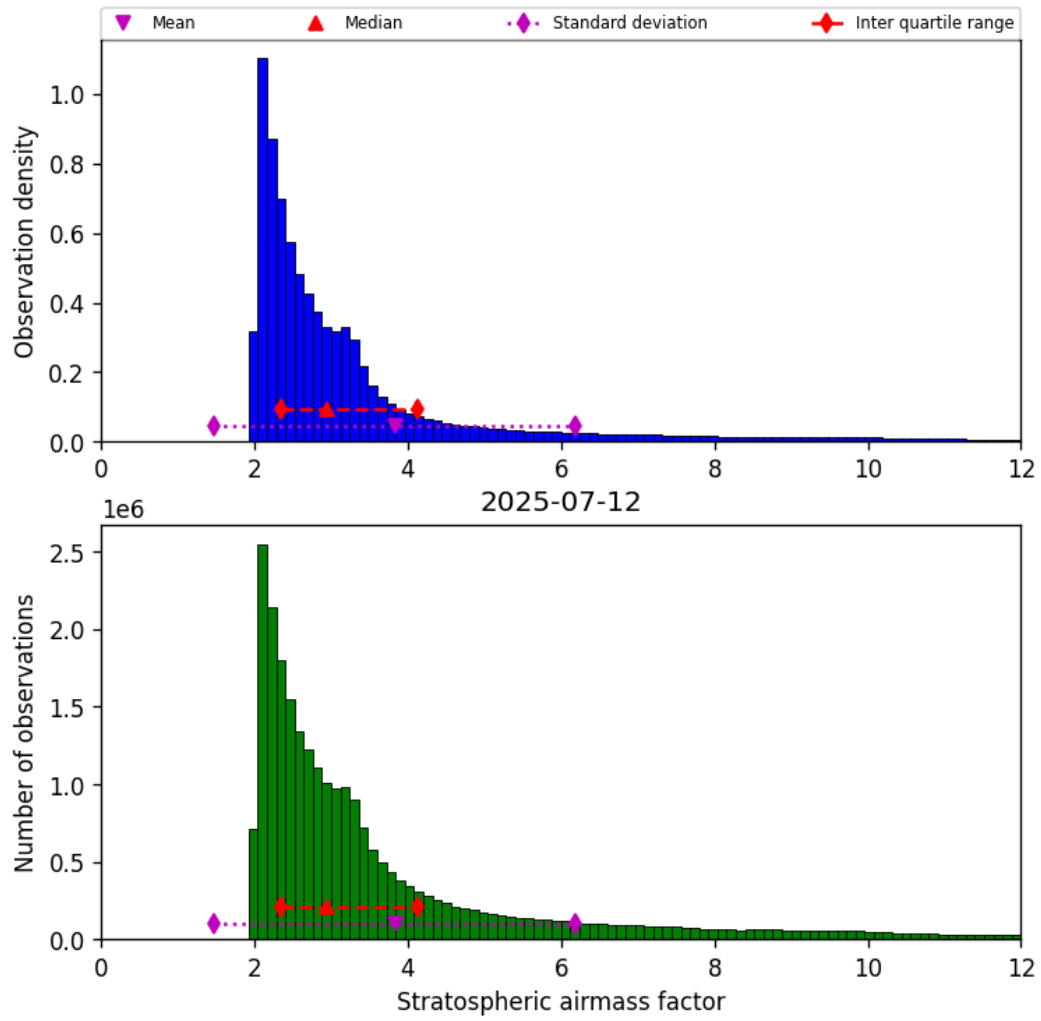
Figure 42: Histogram of “Stratospheric airmass factor” for 2025-07-12 to 2025-07-13
