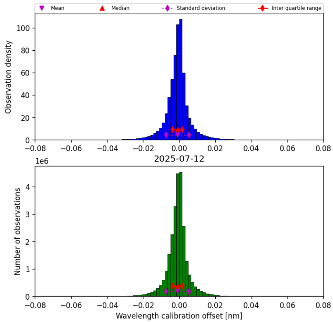
Figure 33: Histogram of “Wavelength calibration offset” for 2025-07-12 to 2025-07-13
