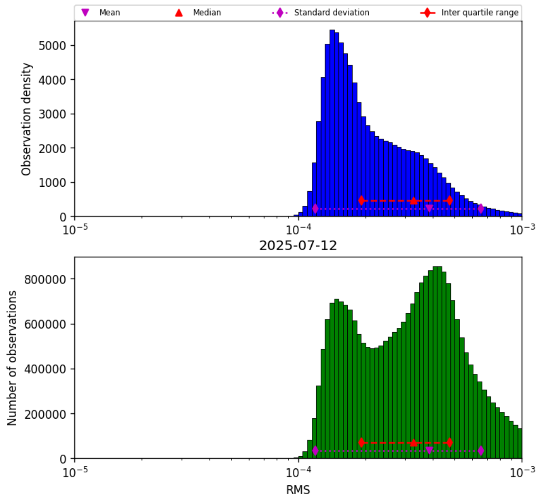
Figure 41: Histogram of “RMS” for 2025-07-12 to 2025-07-13
