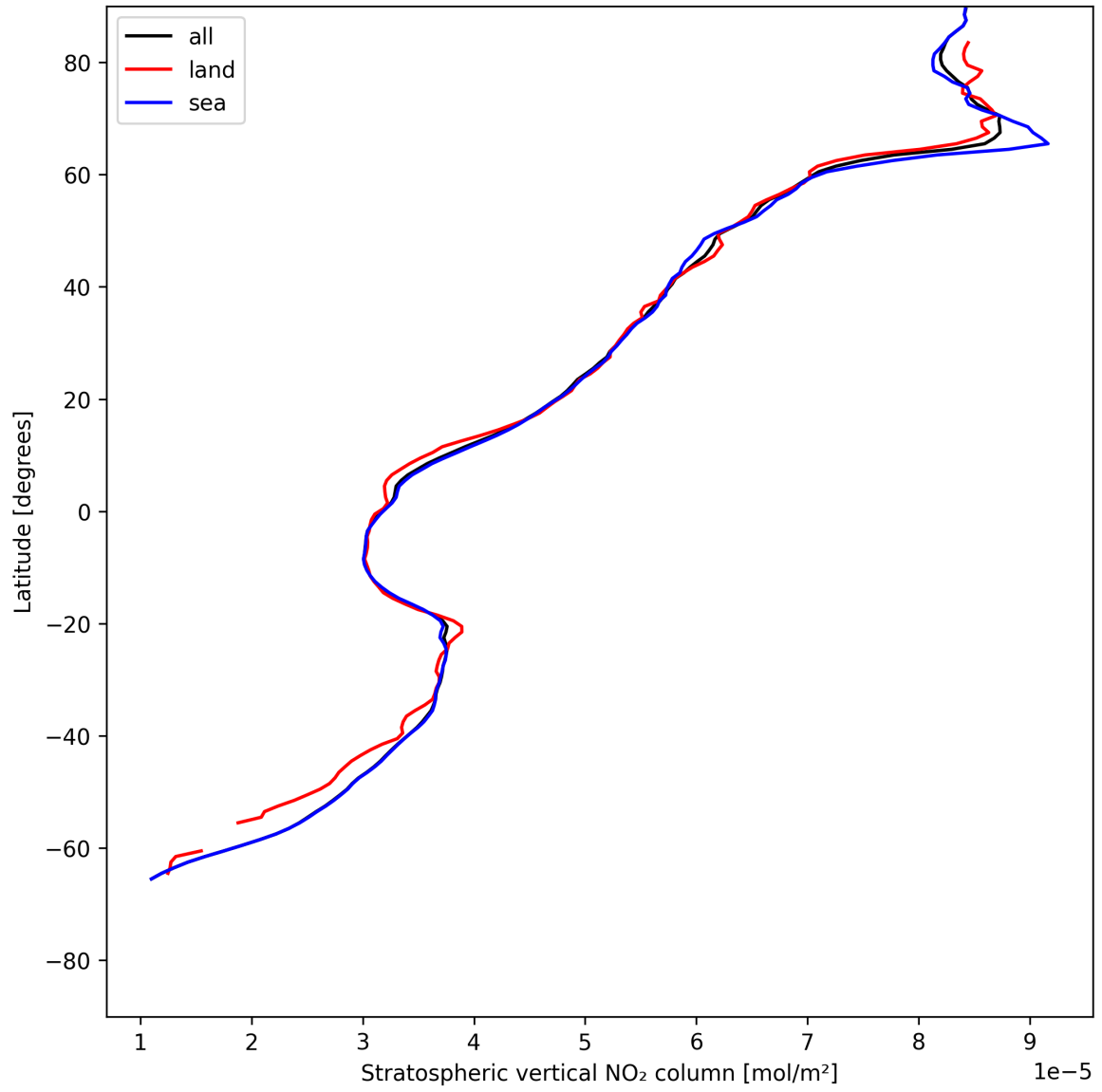
Figure 17: Zonal average of “Stratospheric vertical NO 2 column” for 2025-07-12 to 2025-07-13.
