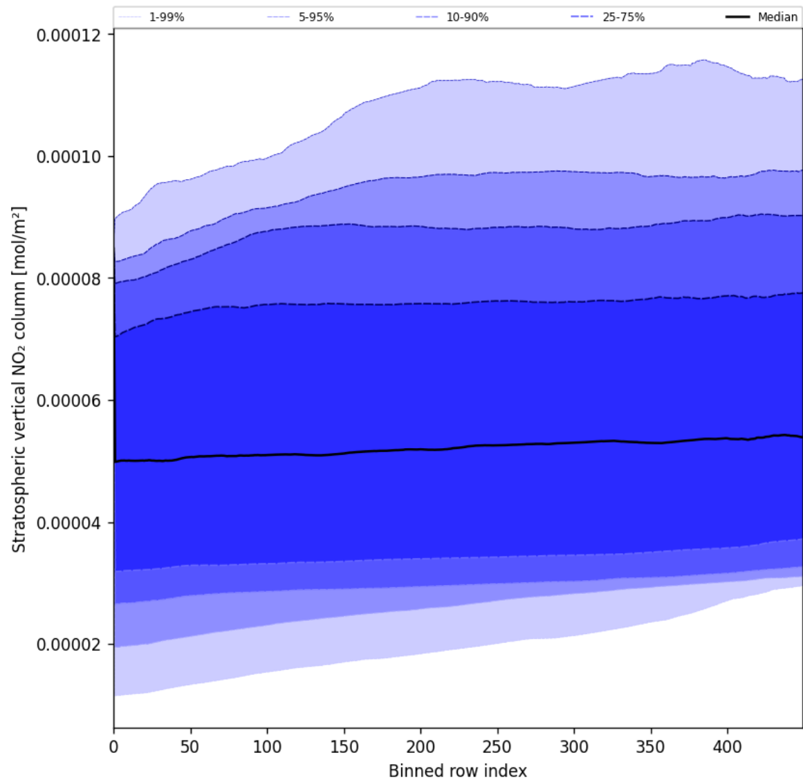
Figure 51: Along track statistics of “Stratospheric vertical NO 2 column” for 2025-07-12 to 2025-07-13
