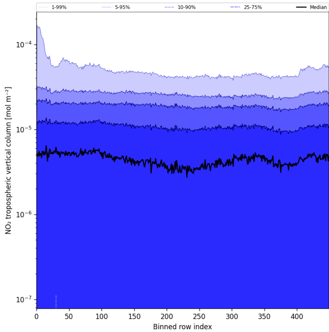
Figure 44: Along track statistics of “NO 2 tropospheric vertical column” for 2025-07-12 to 2025-07-13
