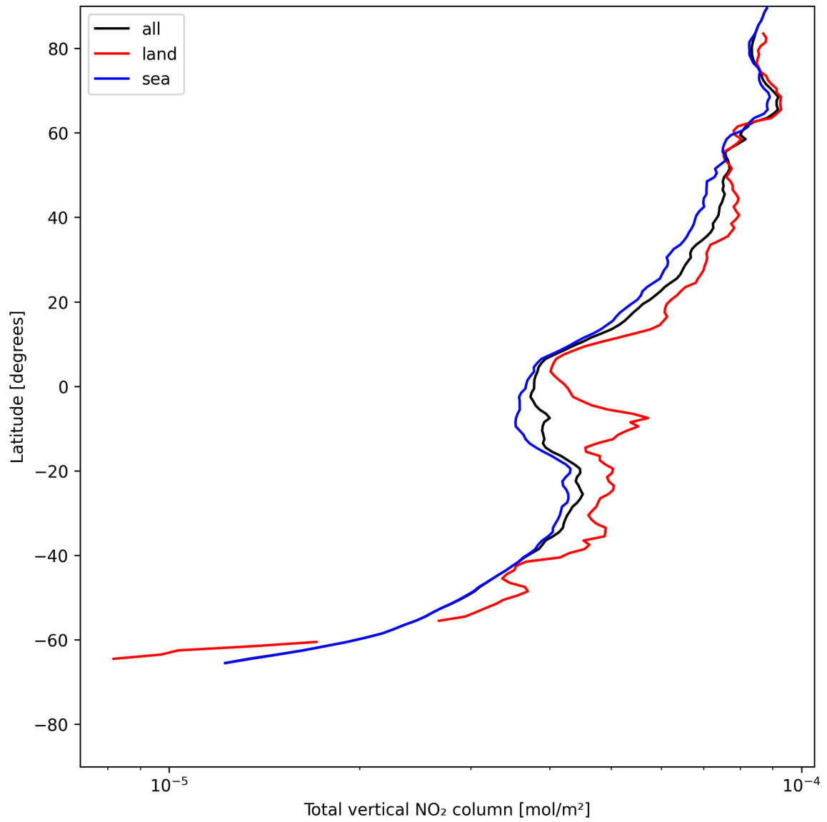
Figure 19: Zonal average of “Total vertical NO 2 column” for 2025-07-12 to 2025-07-13.
