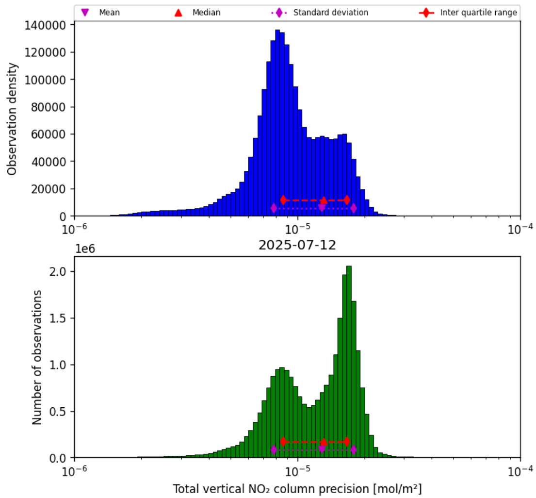
Figure 37: Histogram of “Total vertical NO 2 column precision” for 2025-07-12 to 2025-07-13
