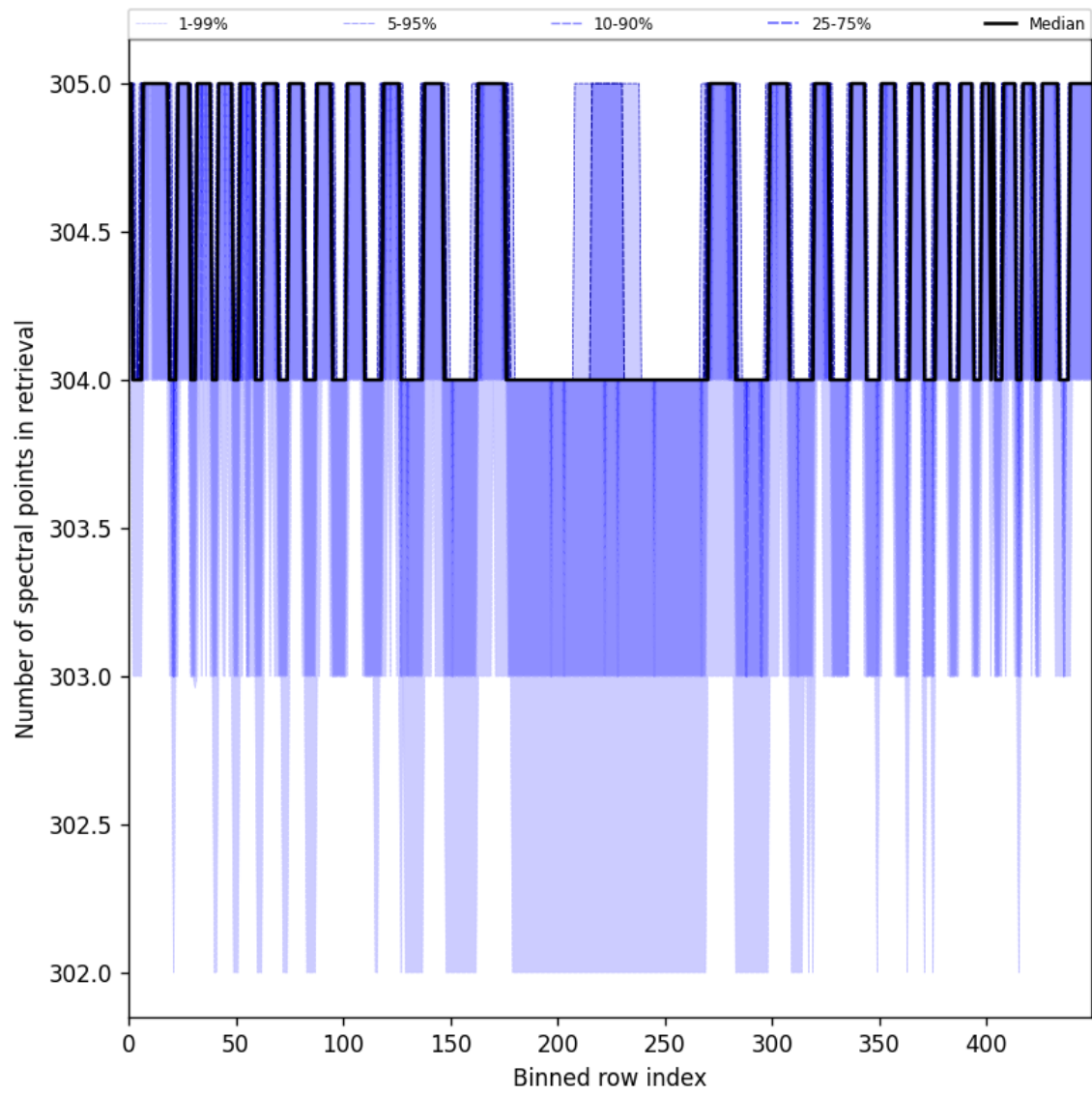
Figure 48: Along track statistics of “Number of spectral points in retrieval” for 2025-07-12 to 2025-07-13
