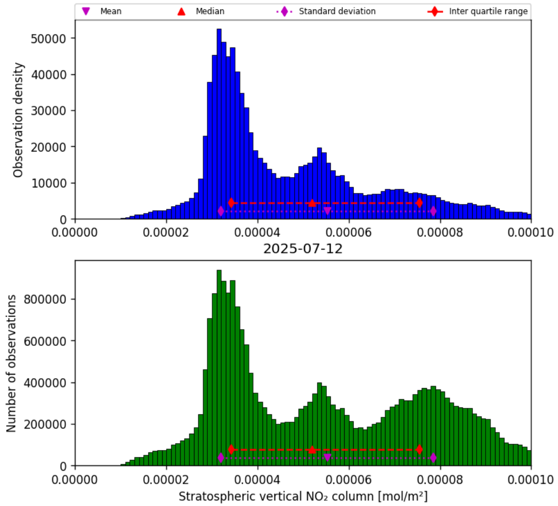
Figure 34: Histogram of “Stratospheric vertical NO 2 column” for 2025-07-12 to 2025-07-13
