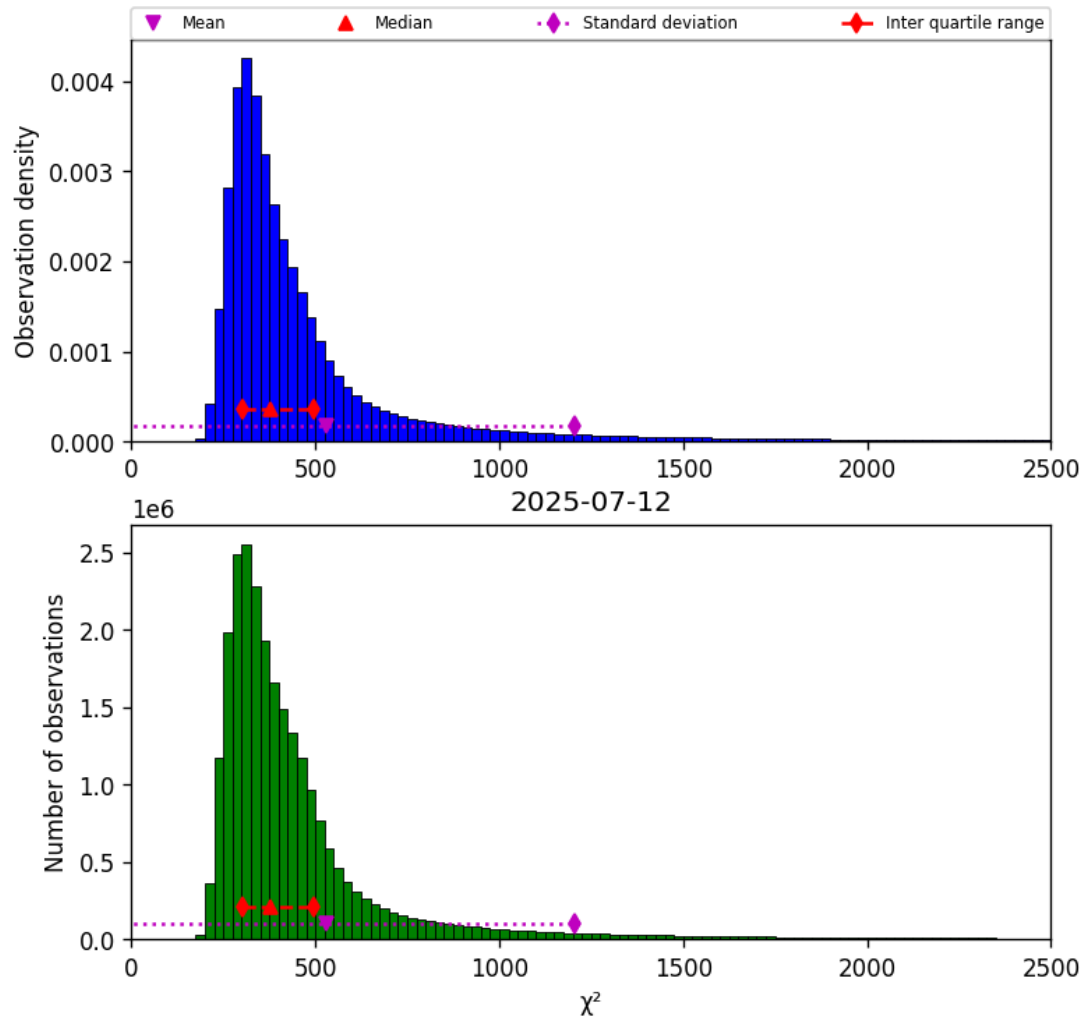
Figure 40: Histogram of “ \chi^2 ” for 2025-07-12 to 2025-07-13
