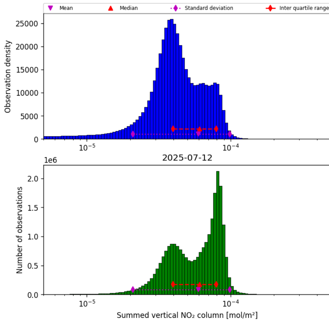
Figure 38: Histogram of “Summed vertical NO 2 column” for 2025-07-12 to 2025-07-13
