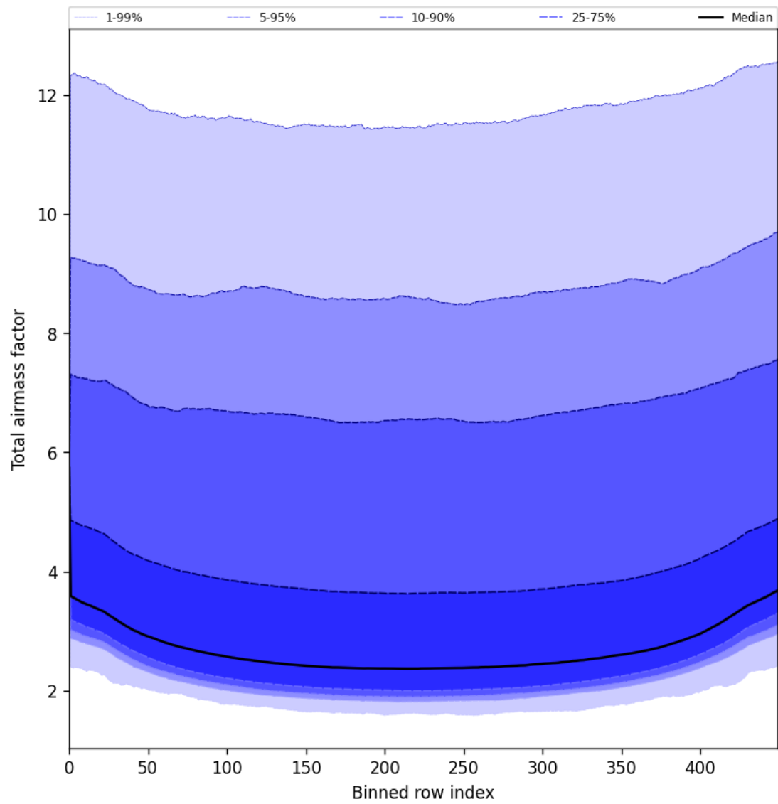
Figure 47: Along track statistics of “Total airmass factor” for 2025-07-12 to 2025-07-13
