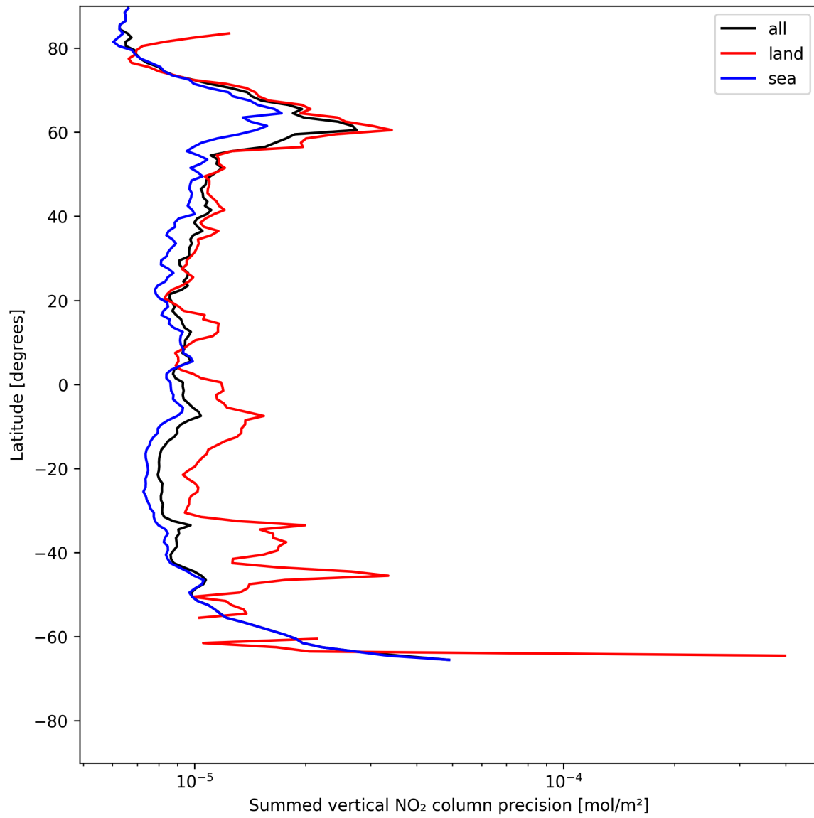
Figure 22: Zonal average of “Summed vertical NO 2 column precision” for 2025-07-12 to 2025-07-13.
