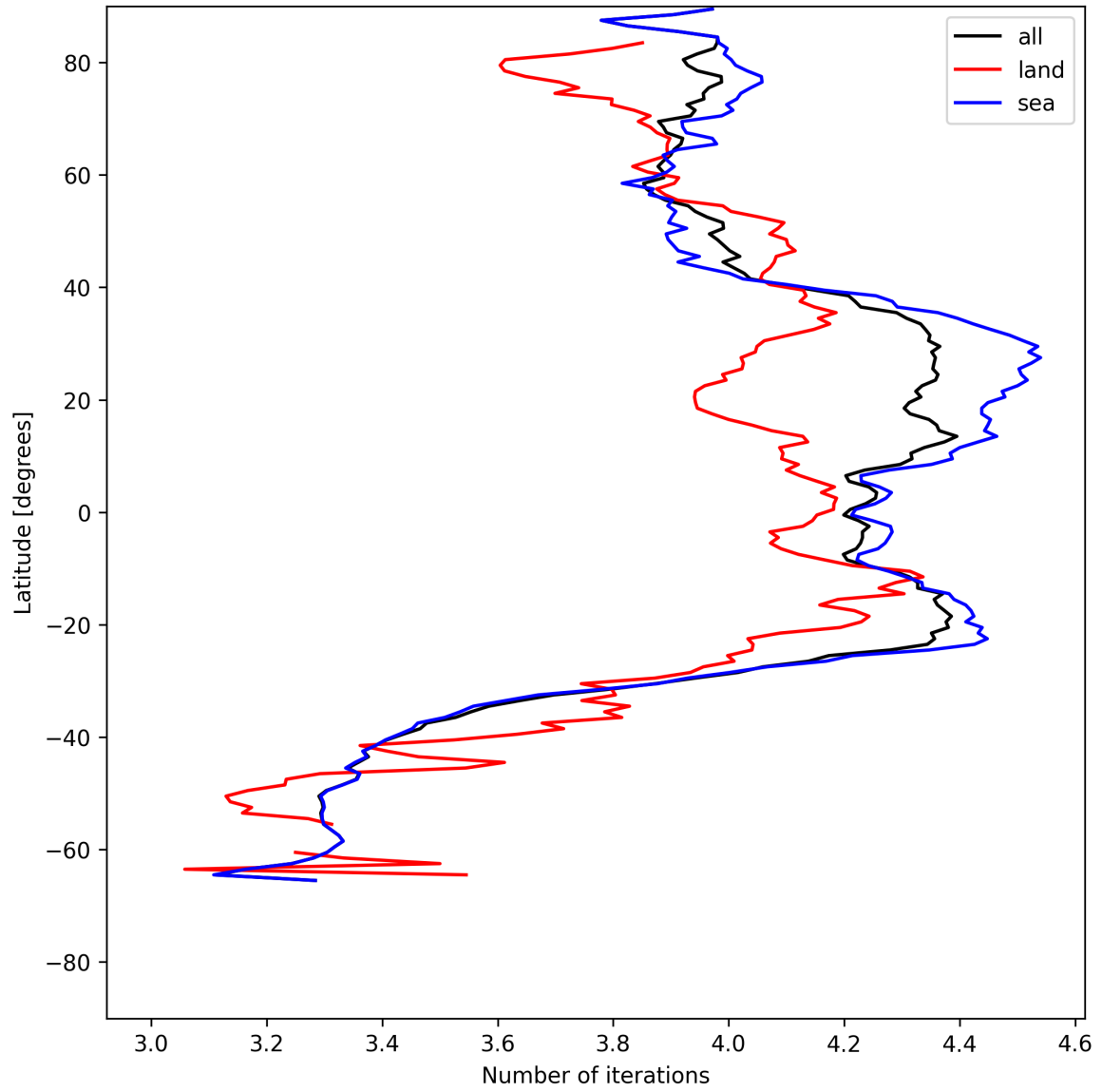
Figure 15: Zonal average of “Number of iterations” for 2025-07-12 to 2025-07-13.
