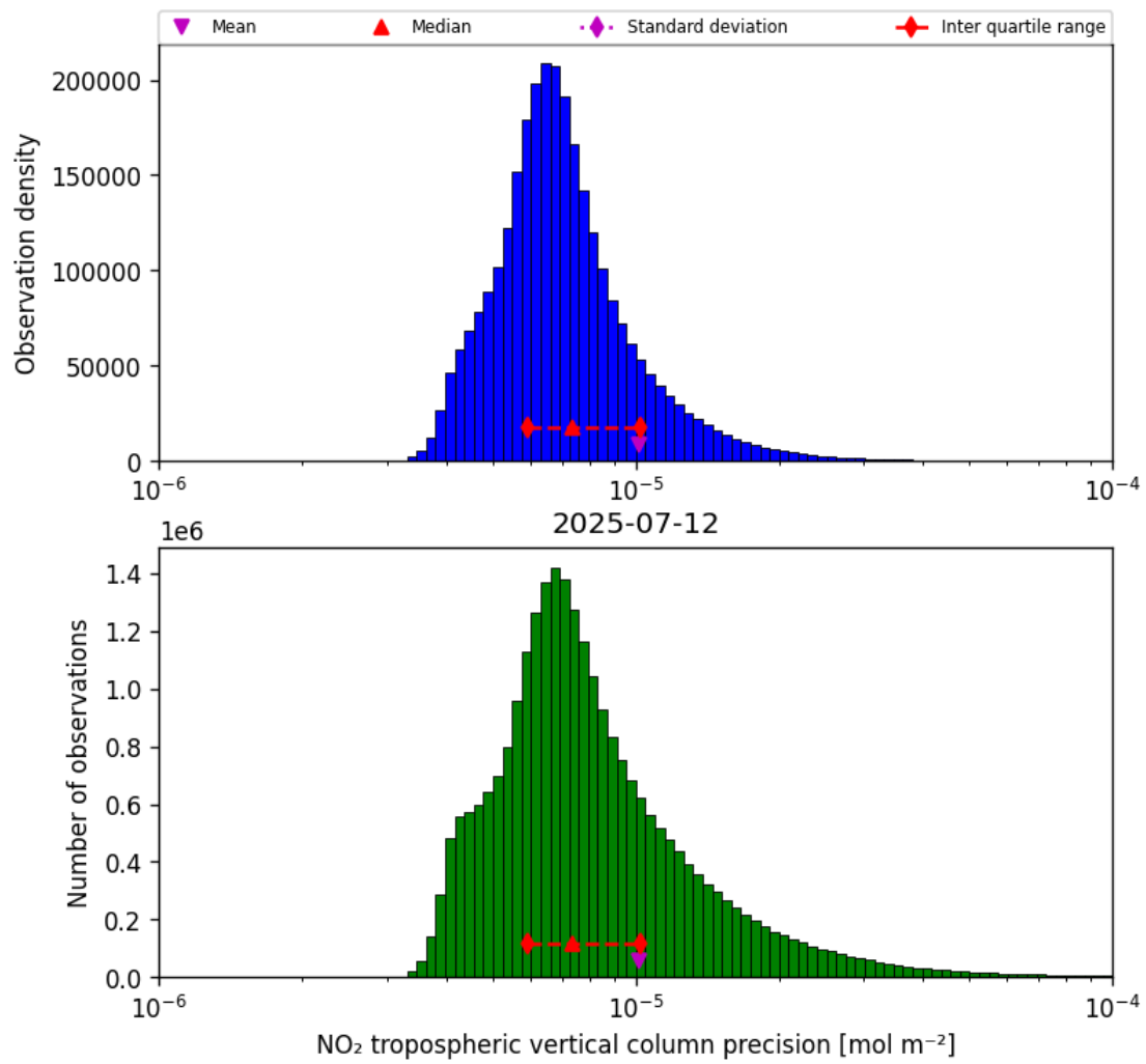
Figure 28: Histogram of “NO 2 tropospheric vertical column precision” for 2025-07-12 to 2025-07-13
