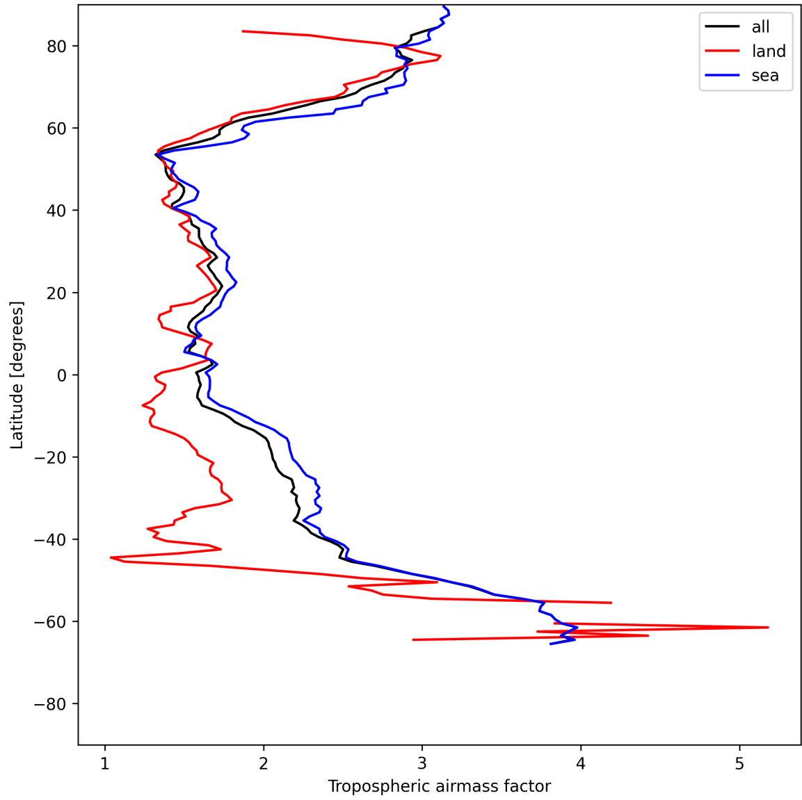
Figure 12: Zonal average of “Tropospheric airmass factor” for 2025-07-12 to 2025-07-13.
