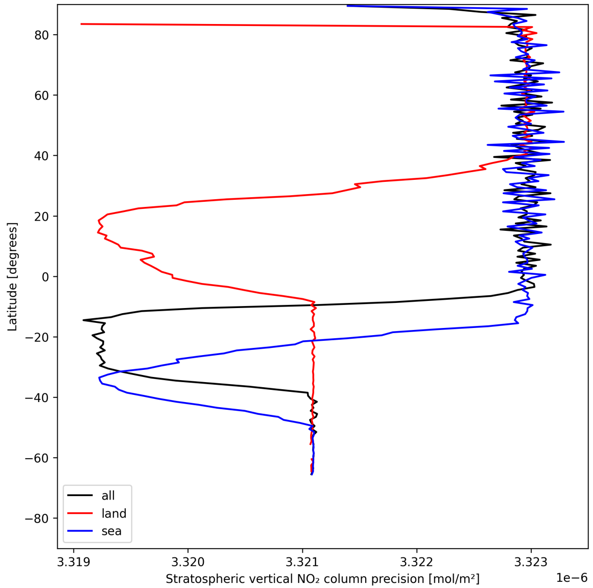
Figure 18: Zonal average of “Stratospheric vertical NO 2 column precision” for 2025-07-12 to 2025-07-13.
