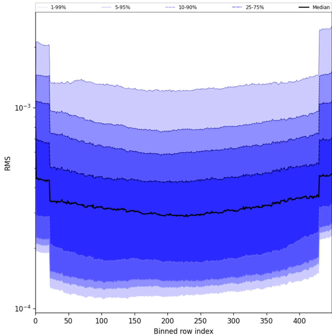
Figure 58: Along track statistics of “RMS” for 2025-07-12 to 2025-07-13
