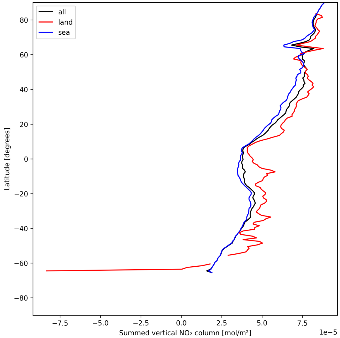
Figure 21: Zonal average of “Summed vertical NO 2 column” for 2025-07-12 to 2025-07-13.
