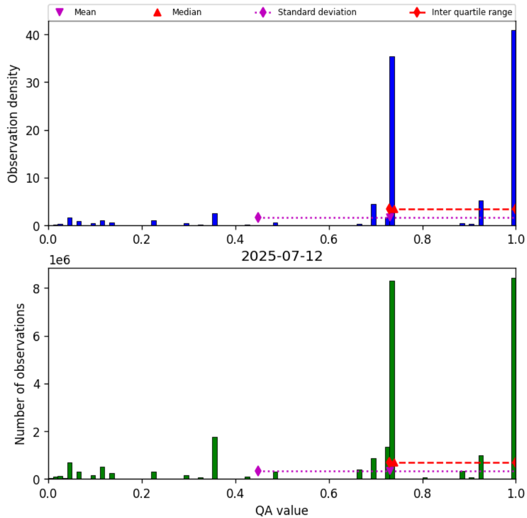
Figure 26: Histogram of “QA value” for 2025-07-12 to 2025-07-13
