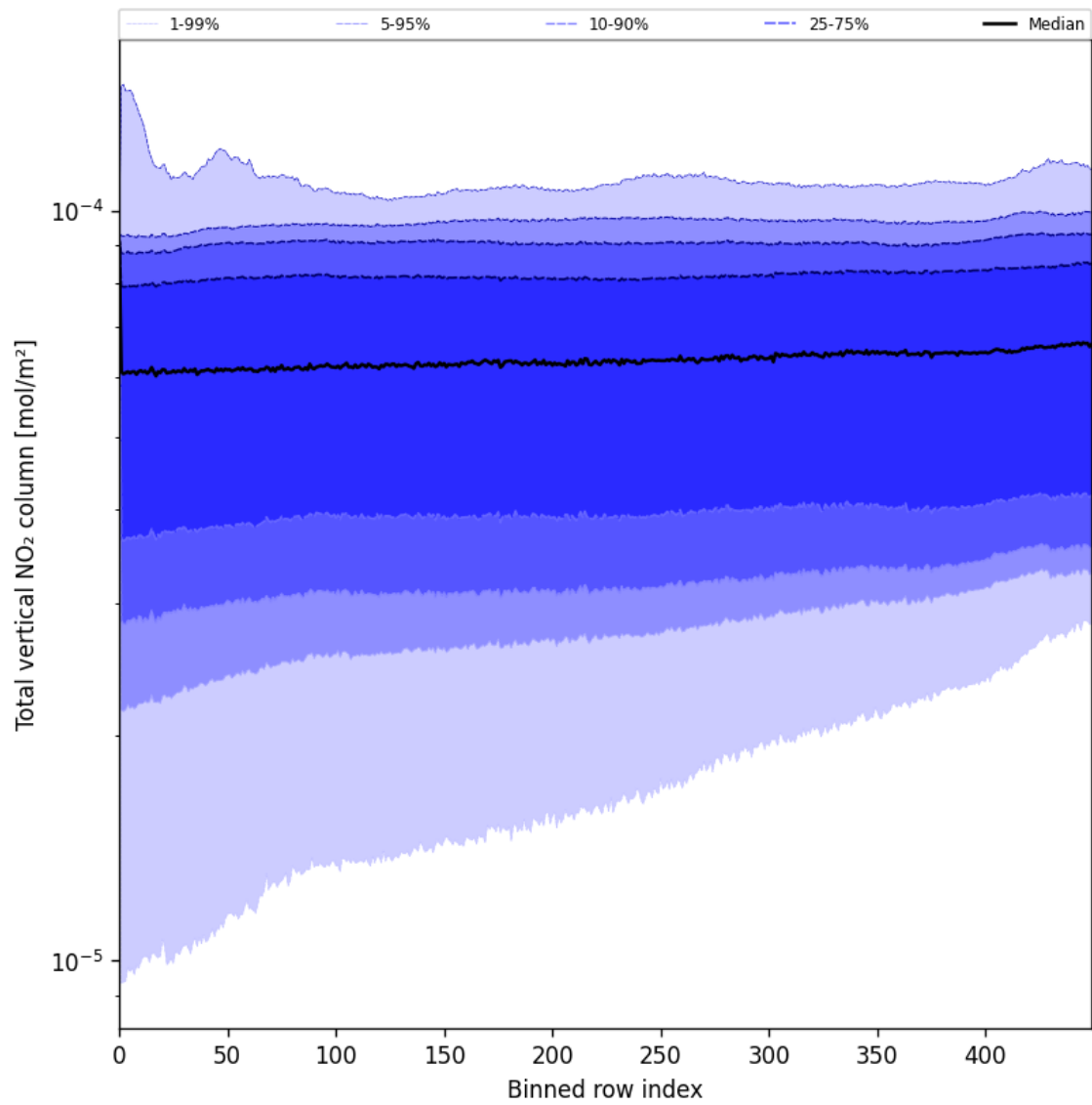
Figure 53: Along track statistics of “Total vertical NO 2 column” for 2025-07-12 to 2025-07-13
