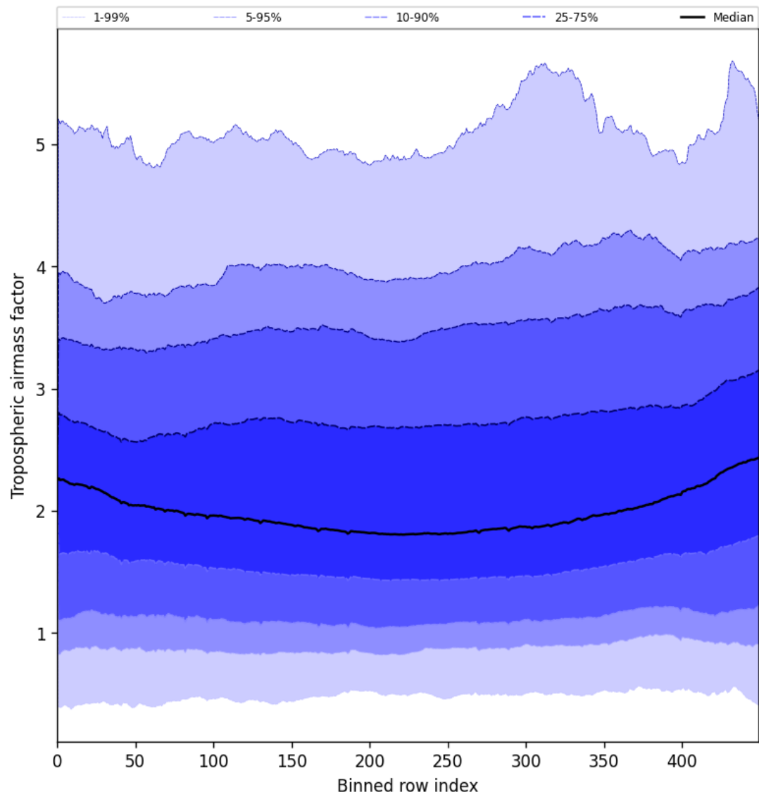
Figure 46: Along track statistics of “Tropospheric airmass factor” for 2025-07-12 to 2025-07-13
