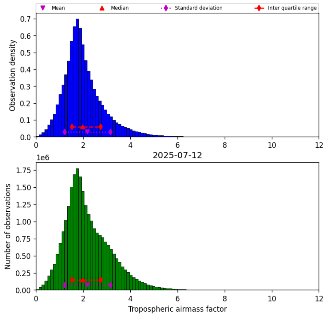
Figure 29: Histogram of “Tropospheric airmass factor” for 2025-07-12 to 2025-07-13
