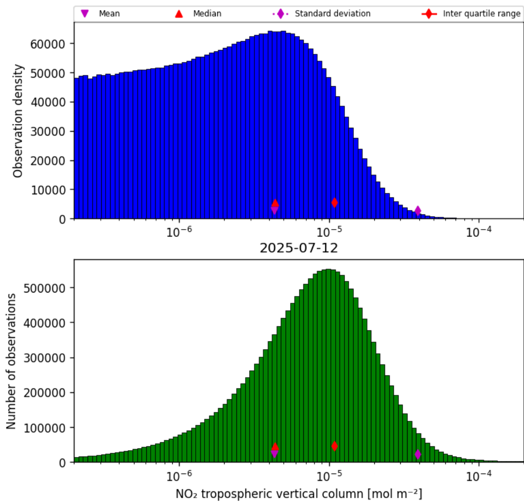
Figure 27: Histogram of “NO 2 tropospheric vertical column” for 2025-07-12 to 2025-07-13
