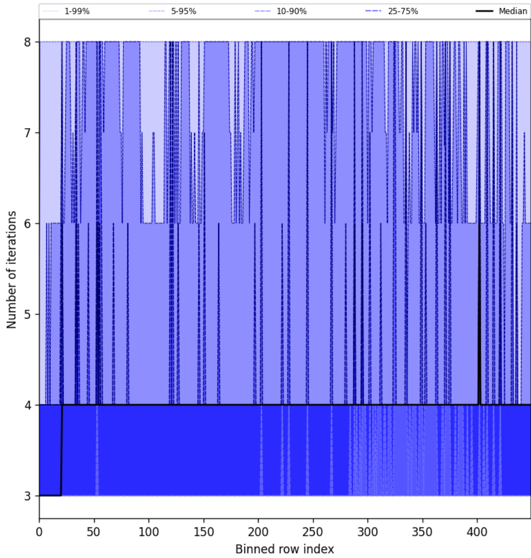
Figure 49: Along track statistics of “Number of iterations” for 2025-07-12 to 2025-07-13
