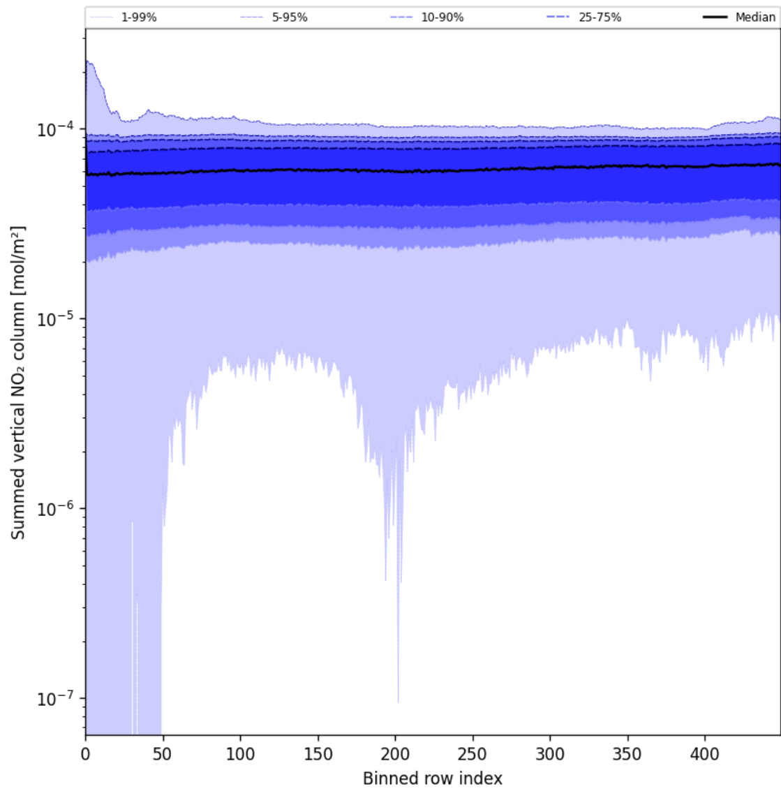
Figure 55: Along track statistics of “Summed vertical NO 2 column” for 2025-07-12 to 2025-07-13
