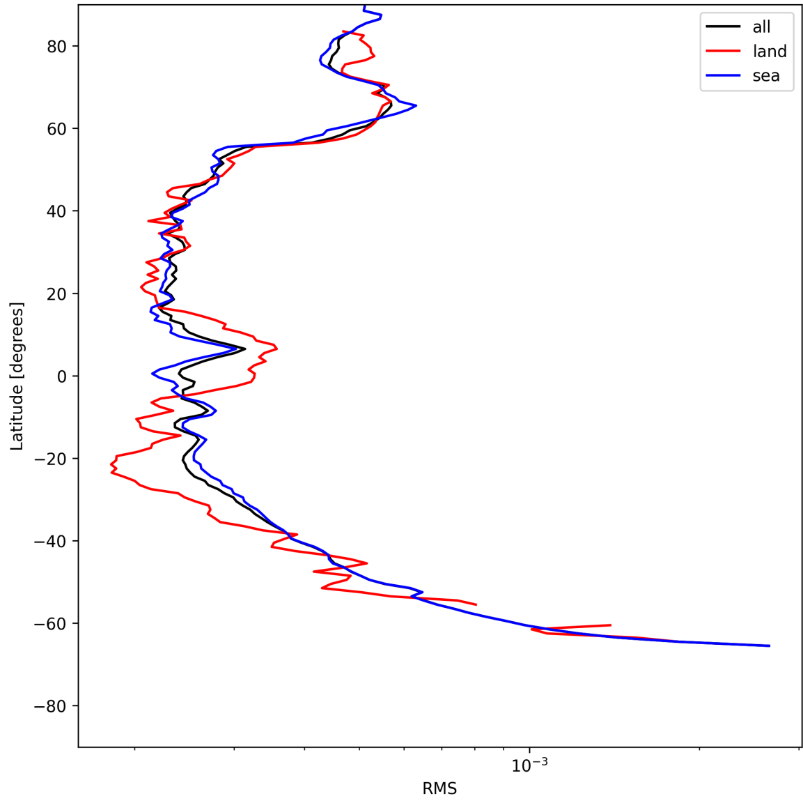
Figure 24: Zonal average of “RMS” for 2025-07-12 to 2025-07-13.
