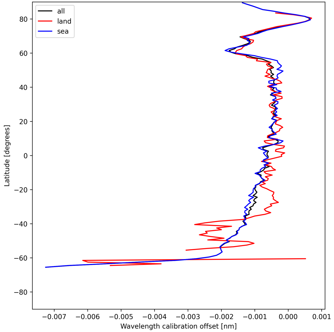
Figure 16: Zonal average of “Wavelength calibration offset” for 2025-07-12 to 2025-07-13.
