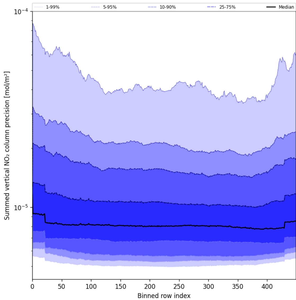
Figure 56: Along track statistics of “Summed vertical NO 2 column precision” for 2025-07-12 to 2025-07-13
