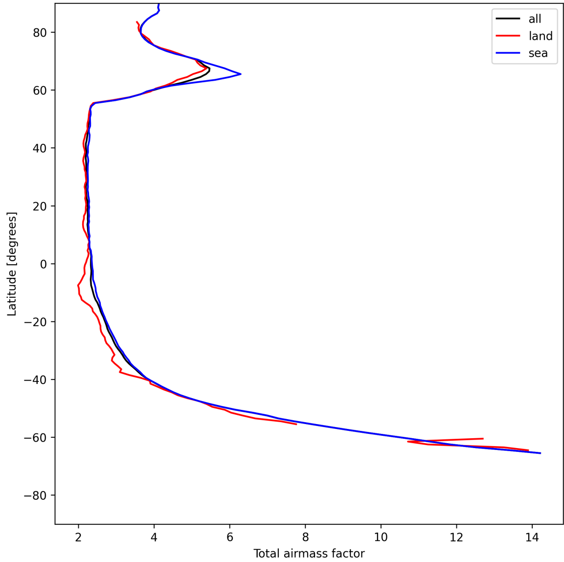
Figure 13: Zonal average of “Total airmass factor” for 2025-07-12 to 2025-07-13.
