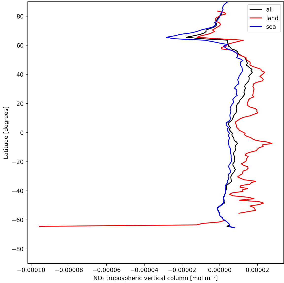
Figure 10: Zonal average of “NO 2 tropospheric vertical column” for 2025-07-12 to 2025-07-13.
