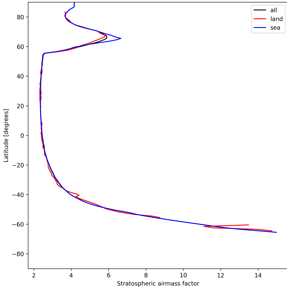
Figure 25: Zonal average of “Stratospheric airmass factor” for 2025-07-12 to 2025-07-13.
