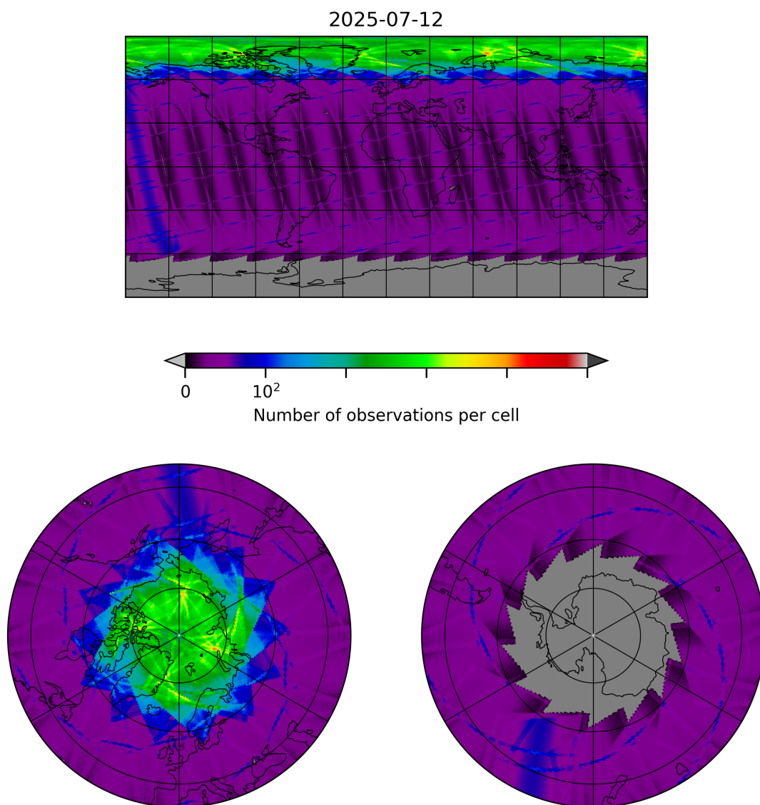
Figure 8: Map of the number of observations for 2025-07-12 to 2025-07-13
