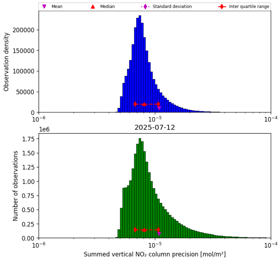
Figure 39: Histogram of "Summed vertical NO 2 column precision" for 2025-07-12 to 2025-07-13
