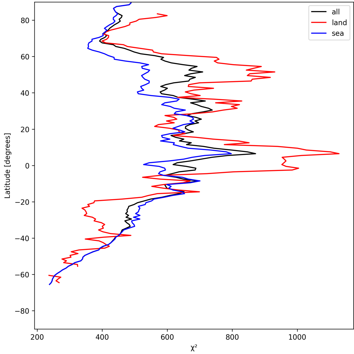
Figure 23: Zonal average of “ \chi^2 ” for 2025-07-12 to 2025-07-13.
