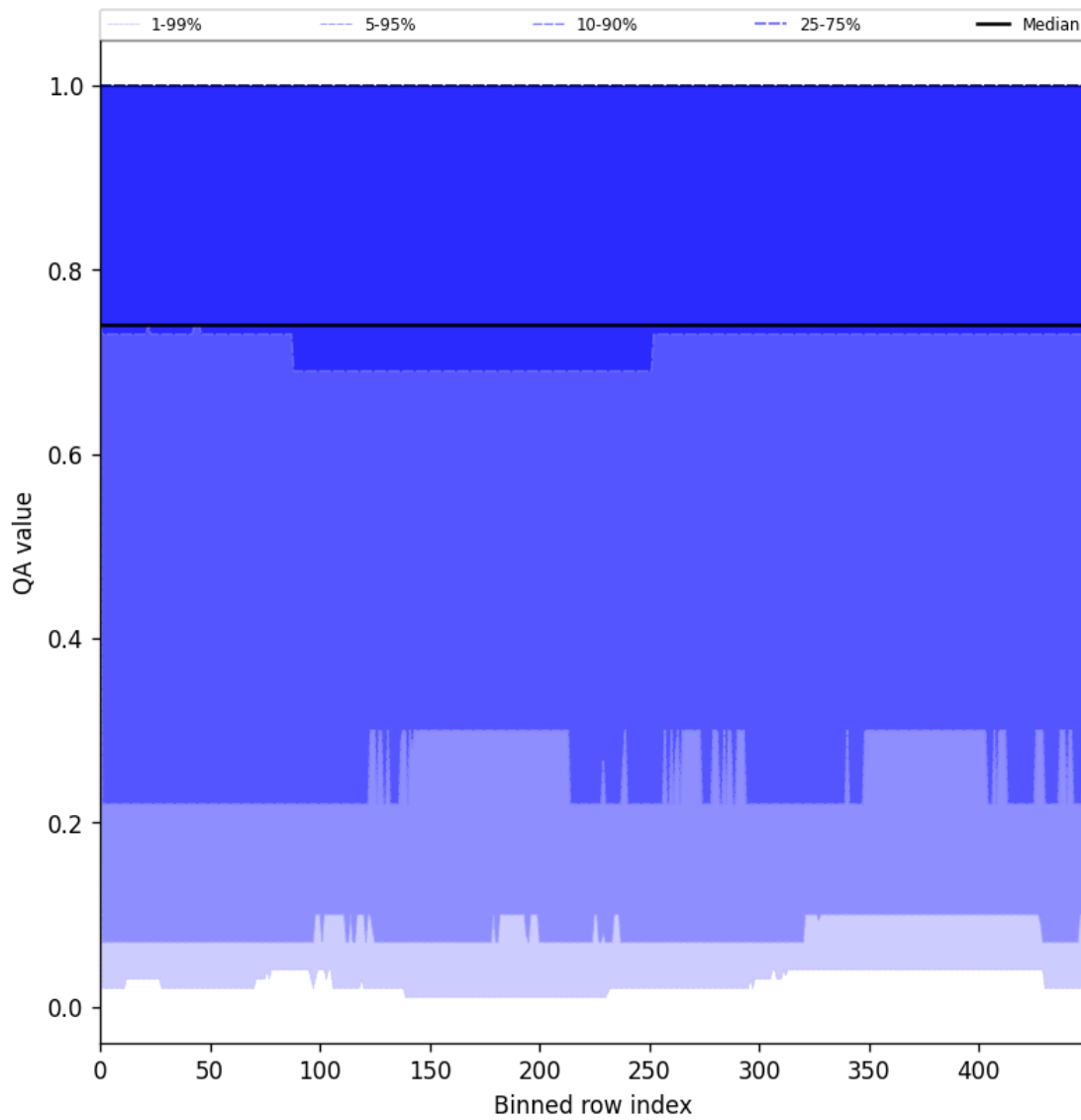
Figure 43: Along track statistics of “QA value” for 2025-07-12 to 2025-07-13
