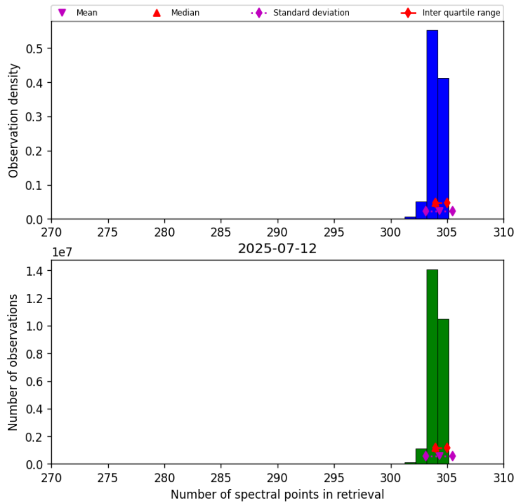
Figure 31: Histogram of “Number of spectral points in retrieval” for 2025-07-12 to 2025-07-13
