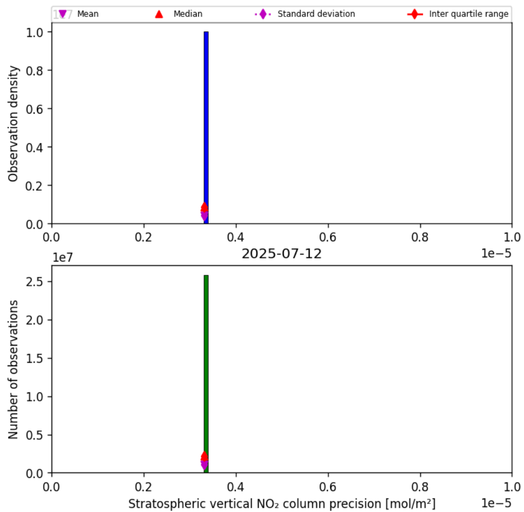
Figure 35: Histogram of “Stratospheric vertical NO 2 column precision” for 2025-07-12 to 2025-07-13
