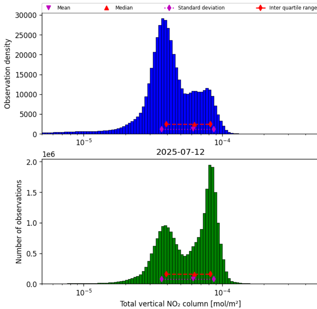
Figure 36: Histogram of "Total vertical NO 2 column" for 2025-07-12 to 2025-07-13
