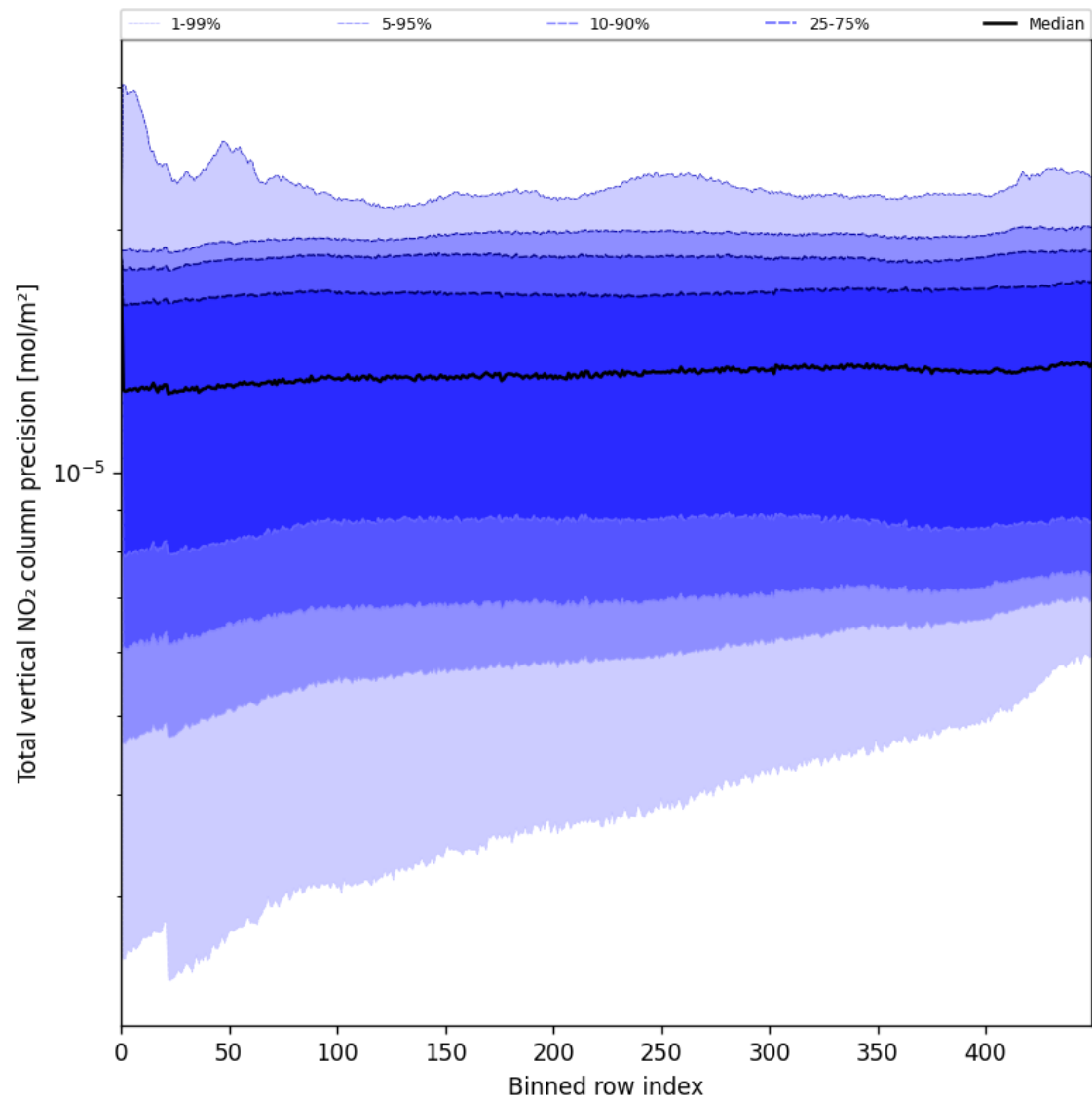
Figure 54: Along track statistics of “Total vertical NO 2 column precision” for 2025-07-12 to 2025-07-13
