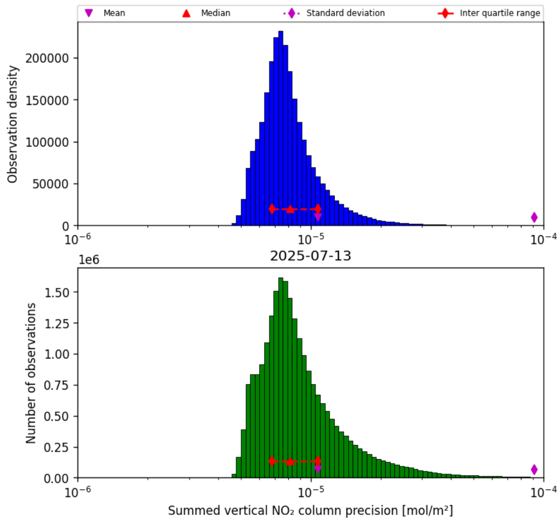
Figure 39: Histogram of "Summed vertical NO 2 column precision" for 2025-07-13 to 2025-07-14
