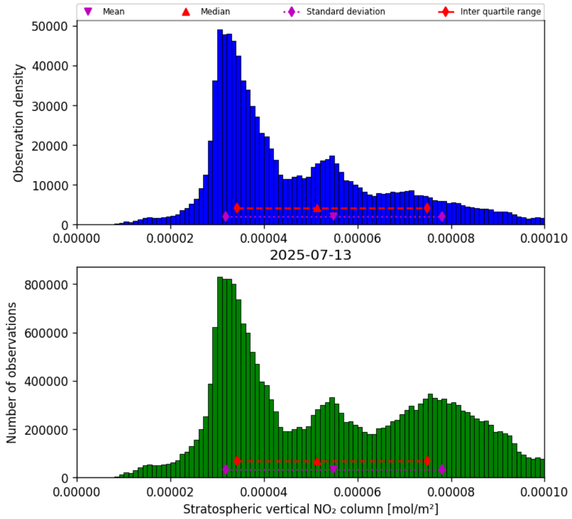
Figure 34: Histogram of “Stratospheric vertical NO 2 column” for 2025-07-13 to 2025-07-14
