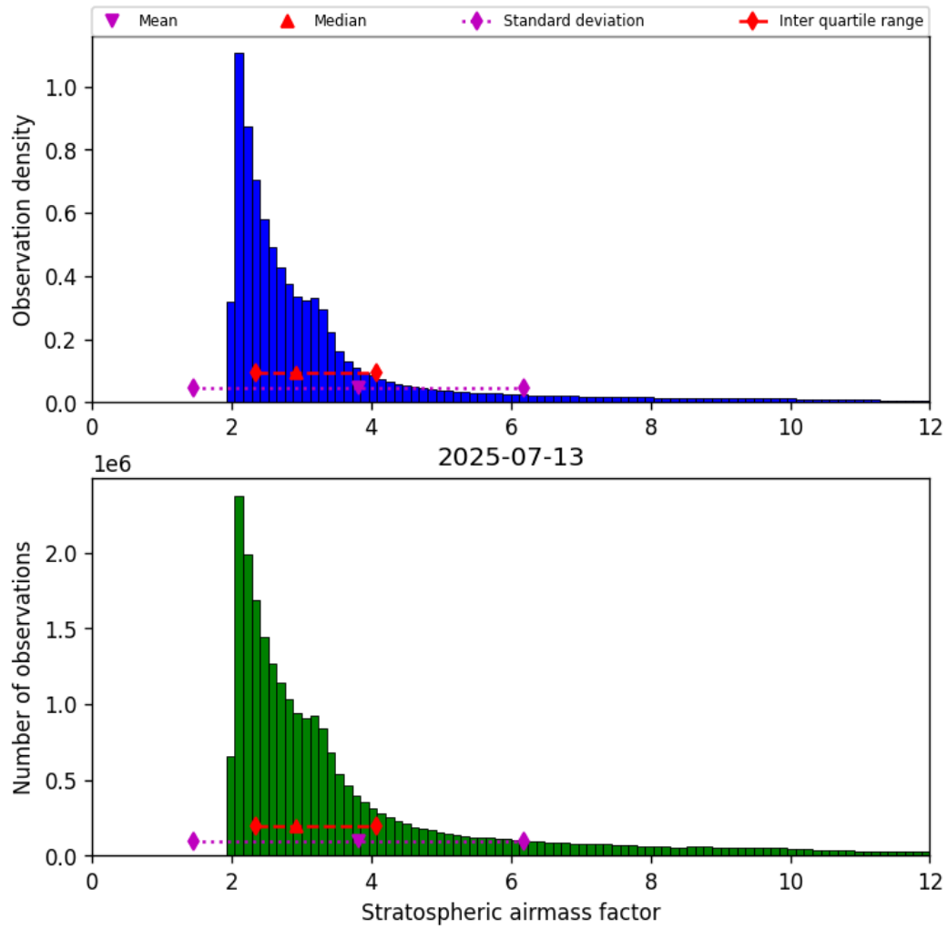
Figure 42: Histogram of “Stratospheric airmass factor” for 2025-07-13 to 2025-07-14
