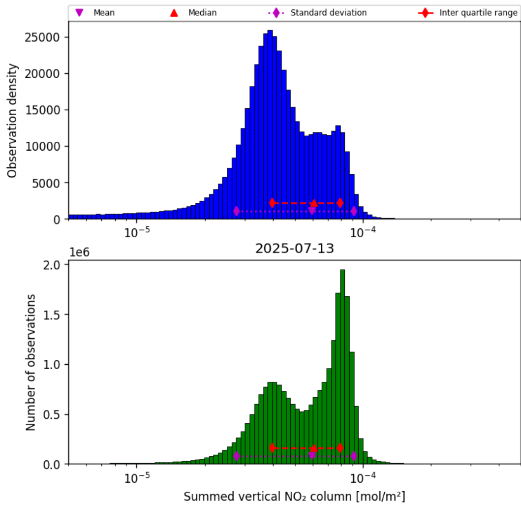
Figure 38: Histogram of “Summed vertical NO 2 column” for 2025-07-13 to 2025-07-14
