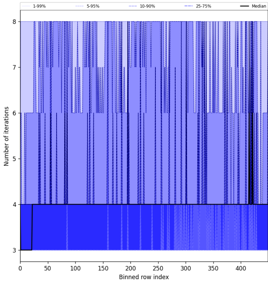
Figure 49: Along track statistics of “Number of iterations” for 2025-07-13 to 2025-07-14
