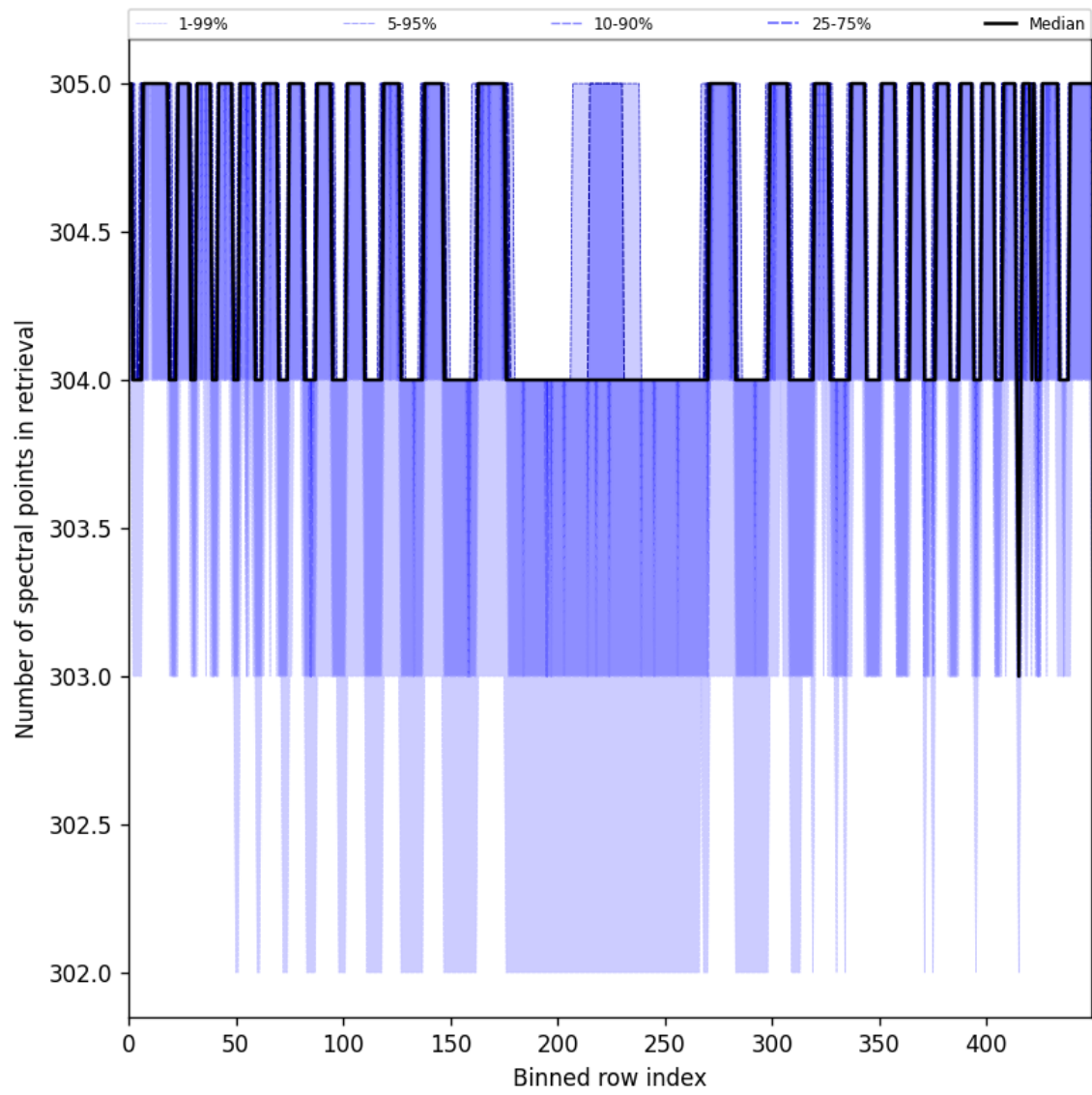
Figure 48: Along track statistics of “Number of spectral points in retrieval” for 2025-07-13 to 2025-07-14
