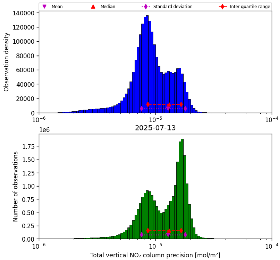
Figure 37: Histogram of “Total vertical NO 2 column precision” for 2025-07-13 to 2025-07-14
