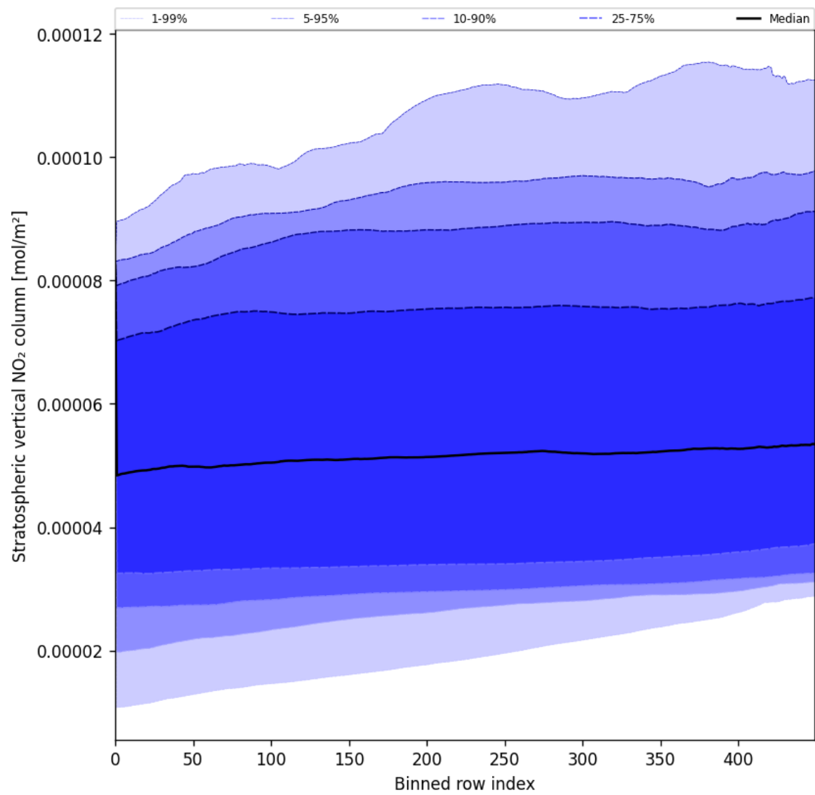
Figure 51: Along track statistics of “Stratospheric vertical NO 2 column” for 2025-07-13 to 2025-07-14
