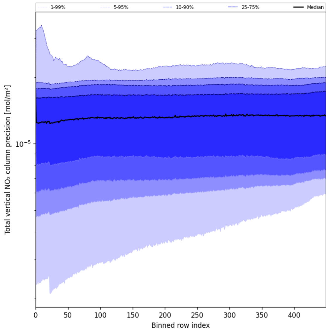
Figure 54: Along track statistics of “Total vertical NO 2 column precision” for 2025-07-13 to 2025-07-14
