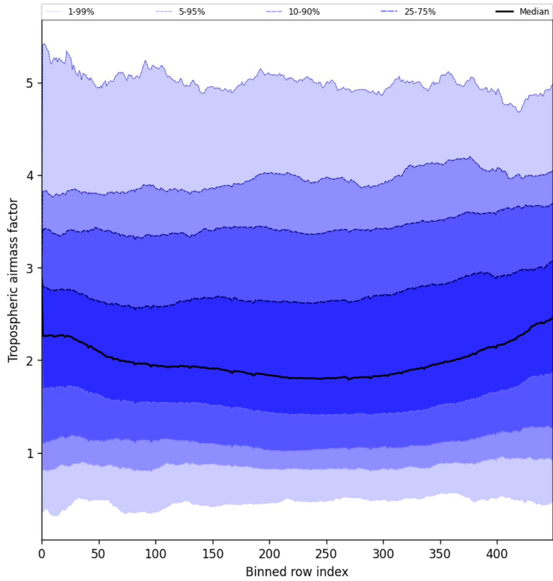
Figure 46: Along track statistics of “Tropospheric airmass factor” for 2025-07-13 to 2025-07-14
