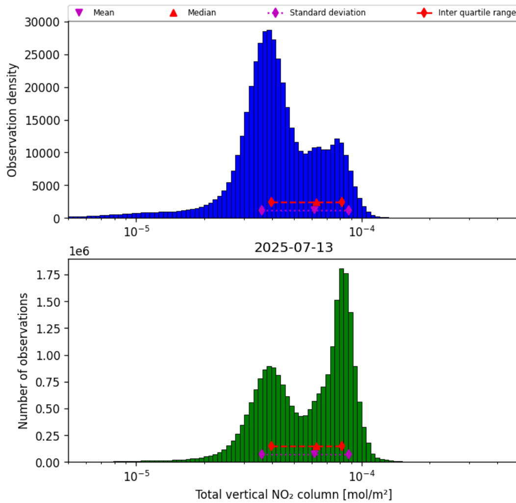
Figure 36: Histogram of “Total vertical NO 2 column” for 2025-07-13 to 2025-07-14
