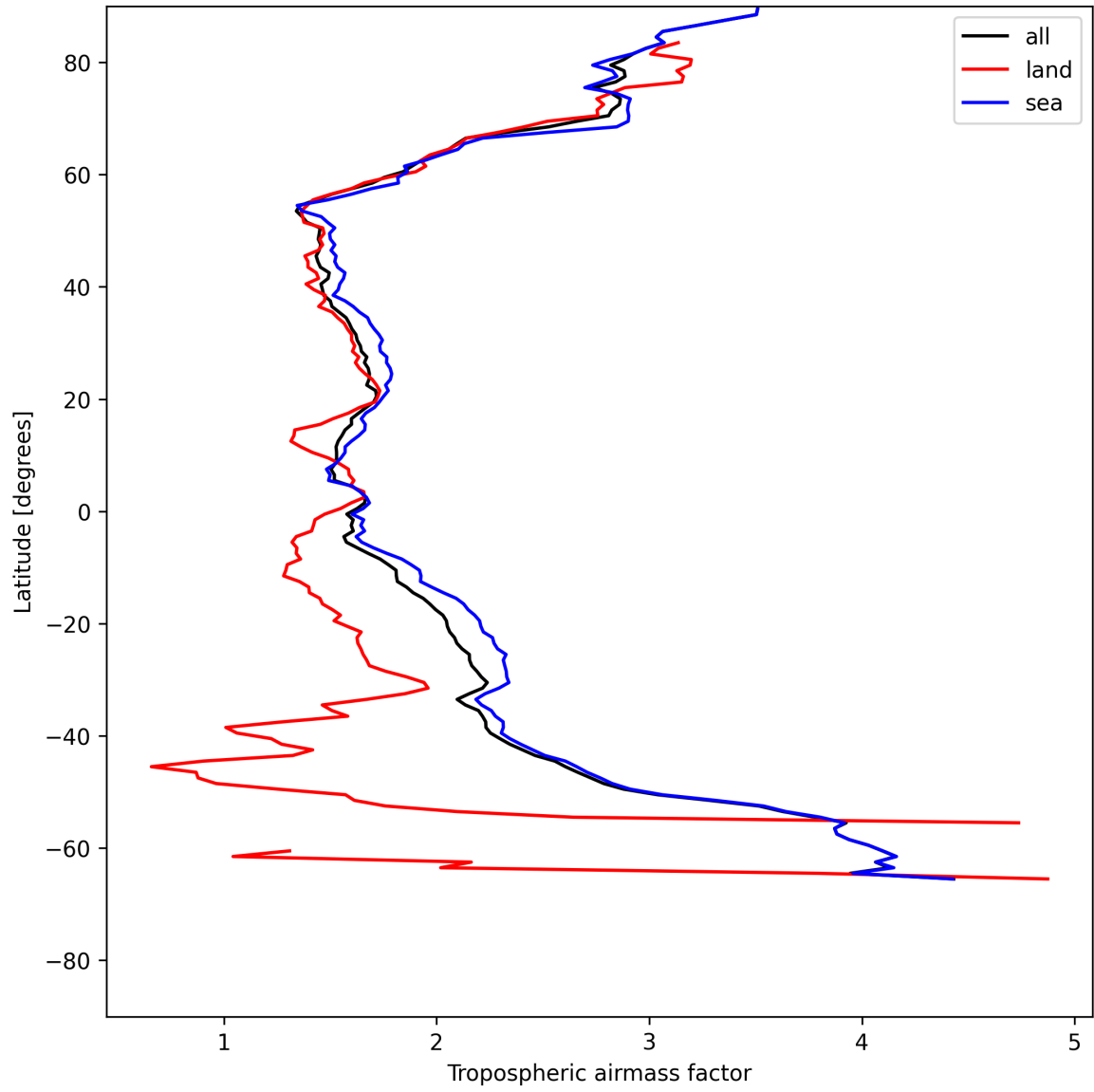
Figure 12: Zonal average of “Tropospheric airmass factor” for 2025-07-13 to 2025-07-14.
