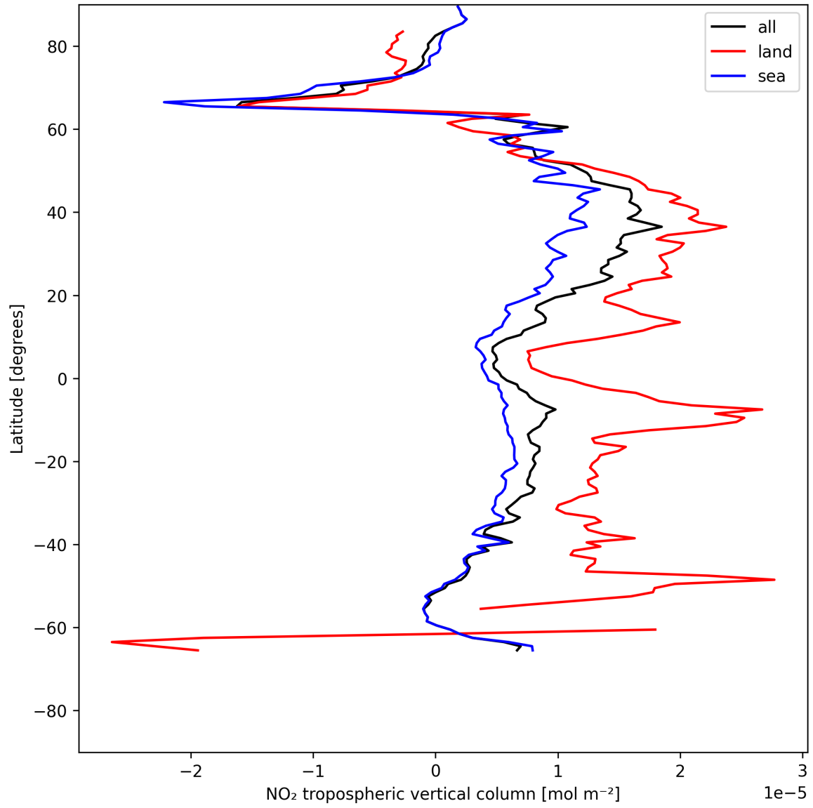
Figure 10: Zonal average of “NO 2 tropospheric vertical column” for 2025-07-13 to 2025-07-14.
