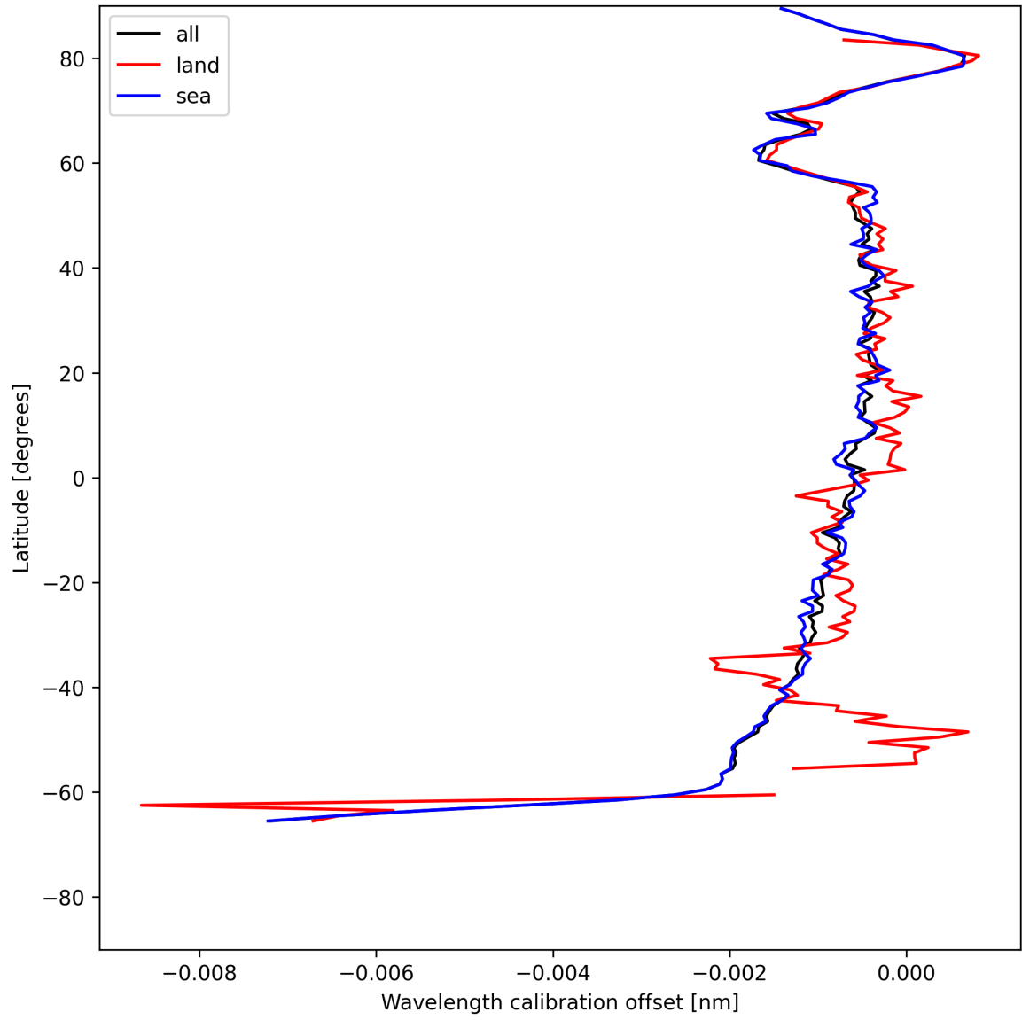
Figure 16: Zonal average of “Wavelength calibration offset” for 2025-07-13 to 2025-07-14.
