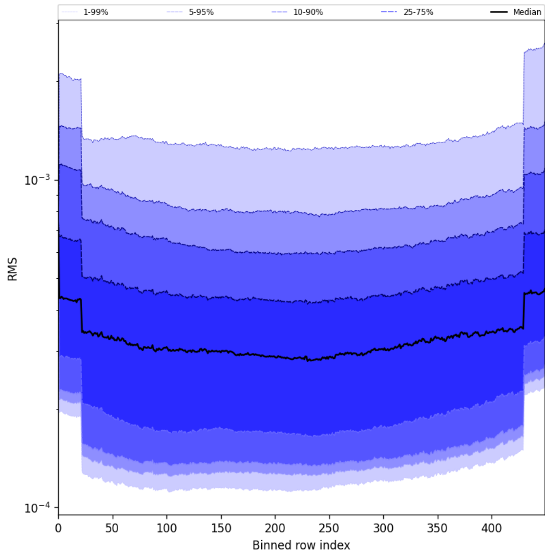
Figure 58: Along track statistics of “RMS” for 2025-07-13 to 2025-07-14
