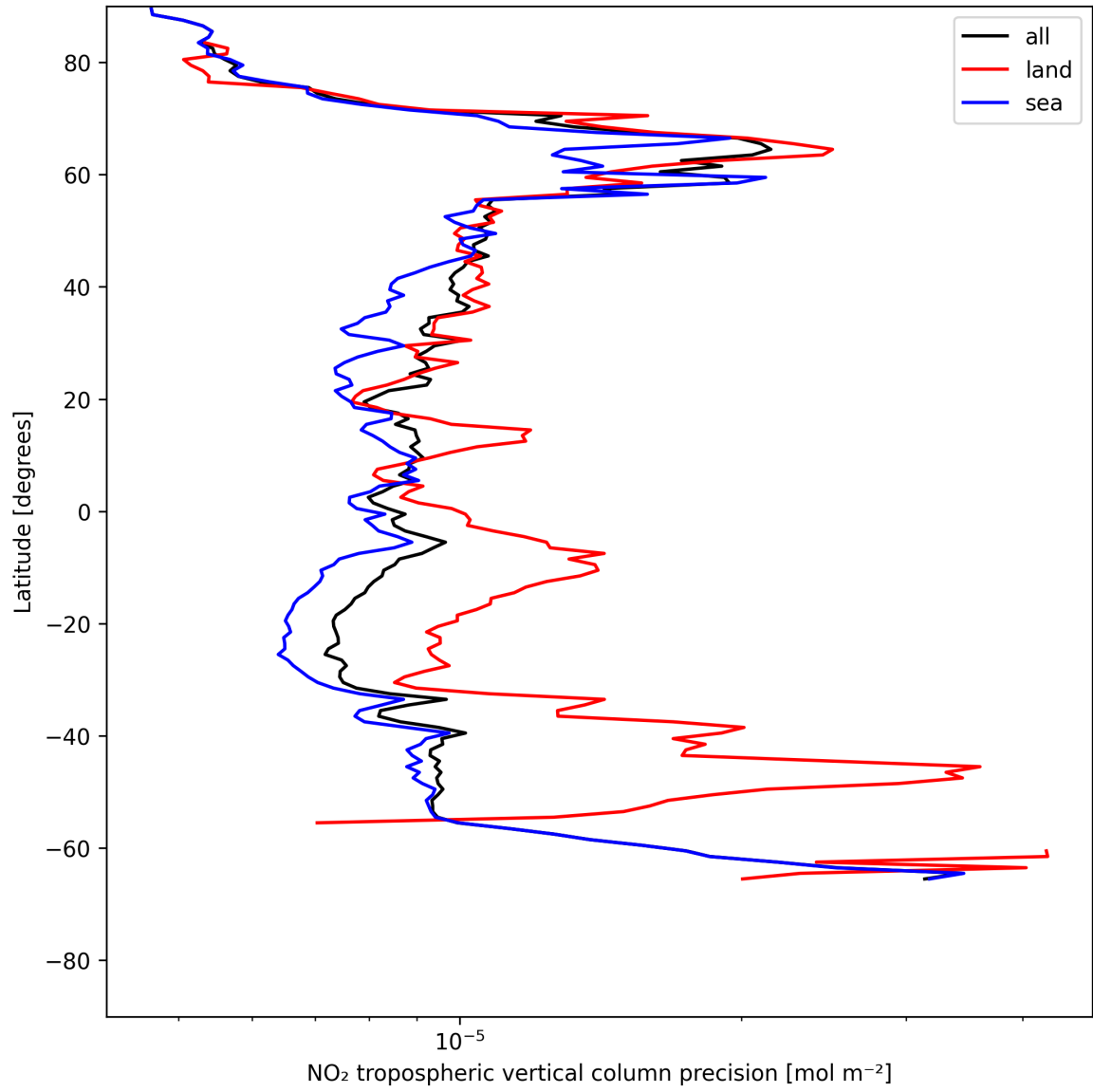
Figure 11: Zonal average of “NO 2 tropospheric vertical column precision” for 2025-07-13 to 2025-07-14.
