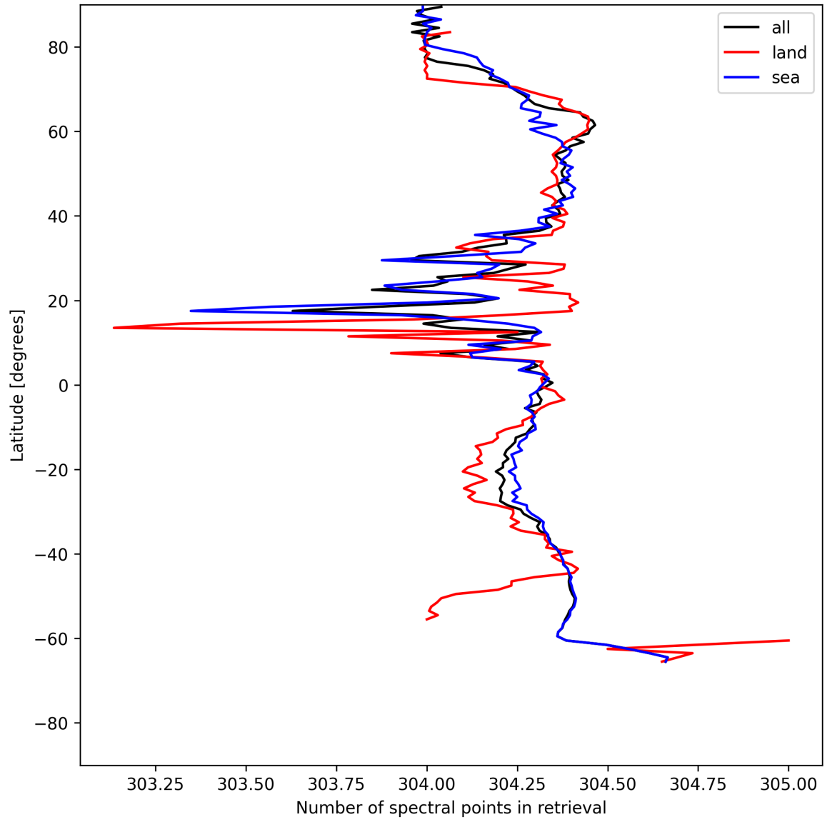
Figure 14: Zonal average of “Number of spectral points in retrieval” for 2025-07-13 to 2025-07-14.
