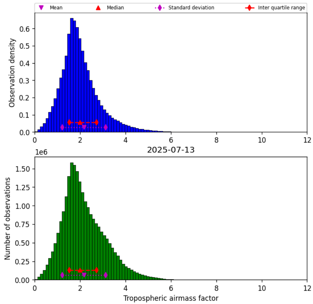
Figure 29: Histogram of “Tropospheric airmass factor” for 2025-07-13 to 2025-07-14
