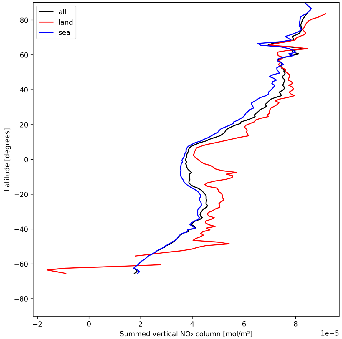
Figure 21: Zonal average of “Summed vertical NO 2 column” for 2025-07-13 to 2025-07-14.
