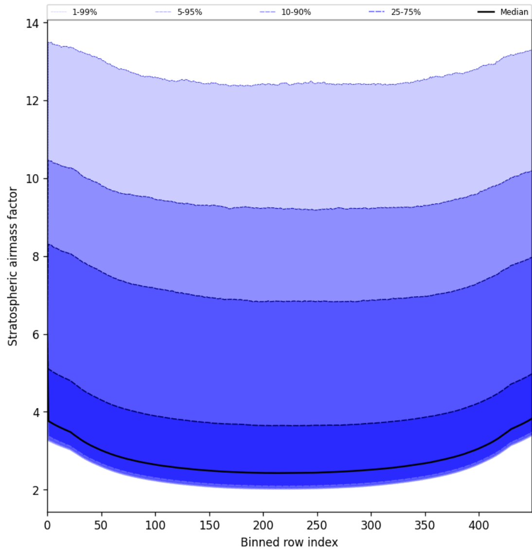
Figure 59: Along track statistics of “Stratospheric airmass factor” for 2025-07-13 to 2025-07-14
