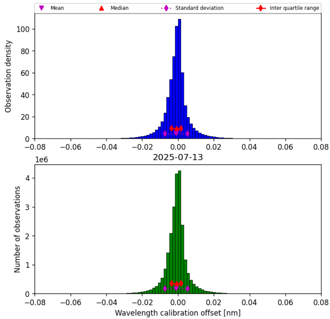
Figure 33: Histogram of “Wavelength calibration offset” for 2025-07-13 to 2025-07-14
