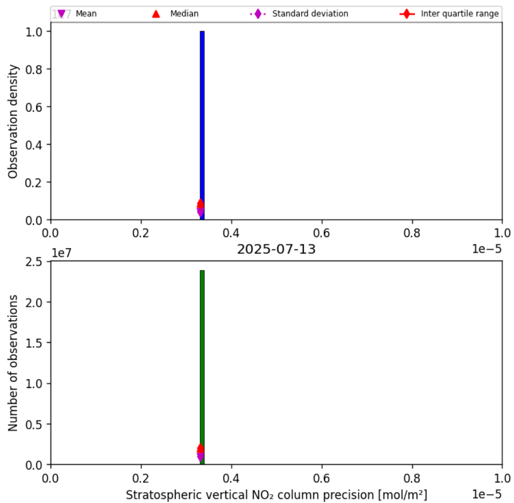
Figure 35: Histogram of “Stratospheric vertical NO 2 column precision” for 2025-07-13 to 2025-07-14
