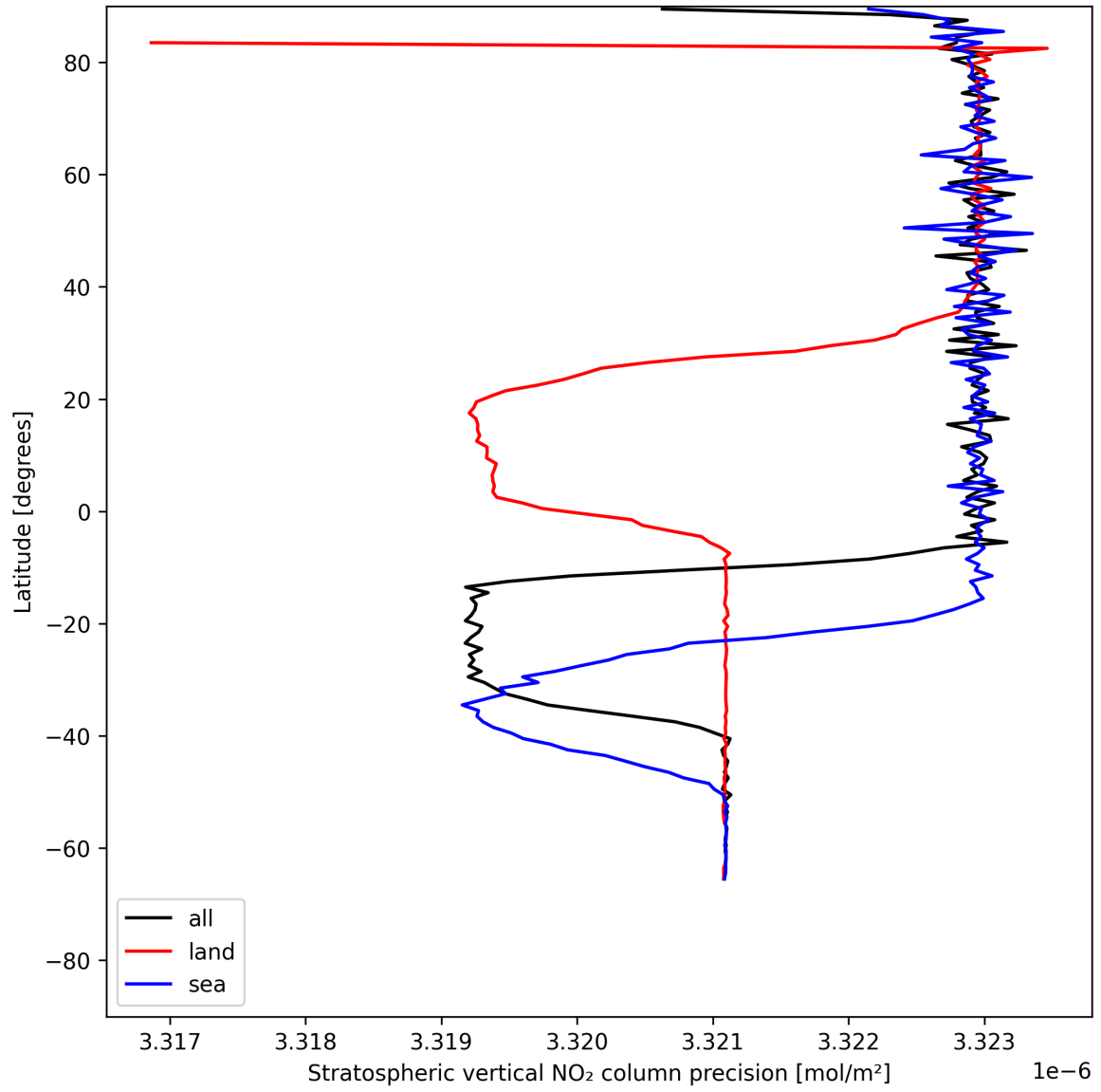
Figure 18: Zonal average of “Stratospheric vertical NO 2 column precision” for 2025-07-13 to 2025-07-14.
