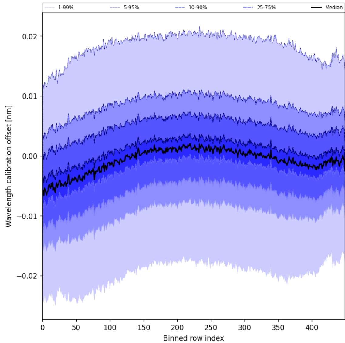
Figure 50: Along track statistics of “Wavelength calibration offset” for 2025-07-13 to 2025-07-14
