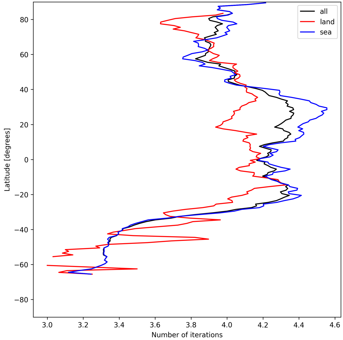
Figure 15: Zonal average of “Number of iterations” for 2025-07-13 to 2025-07-14.
