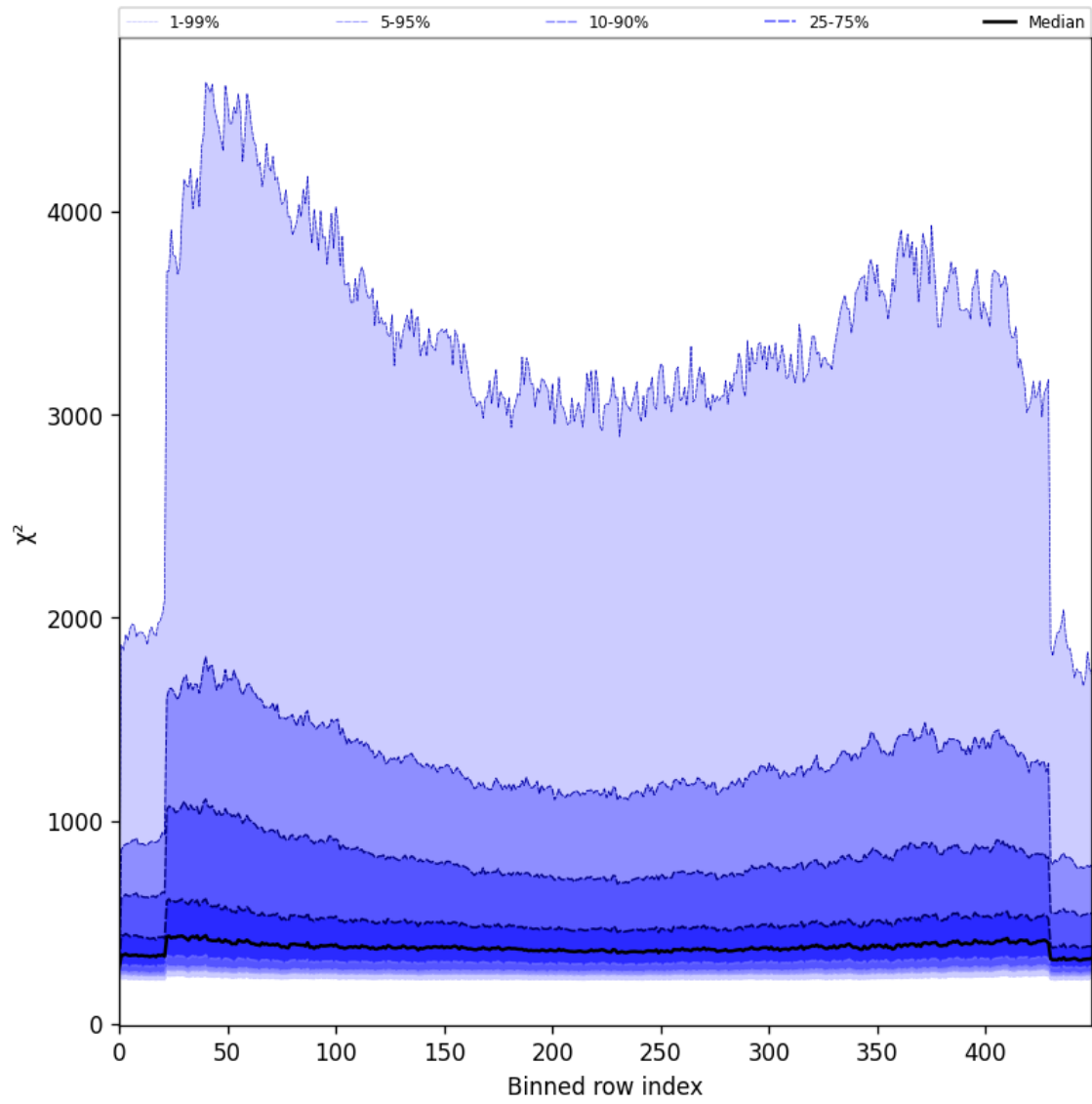
Figure 57: Along track statistics of “ \chi^2 ” for 2025-07-13 to 2025-07-14
