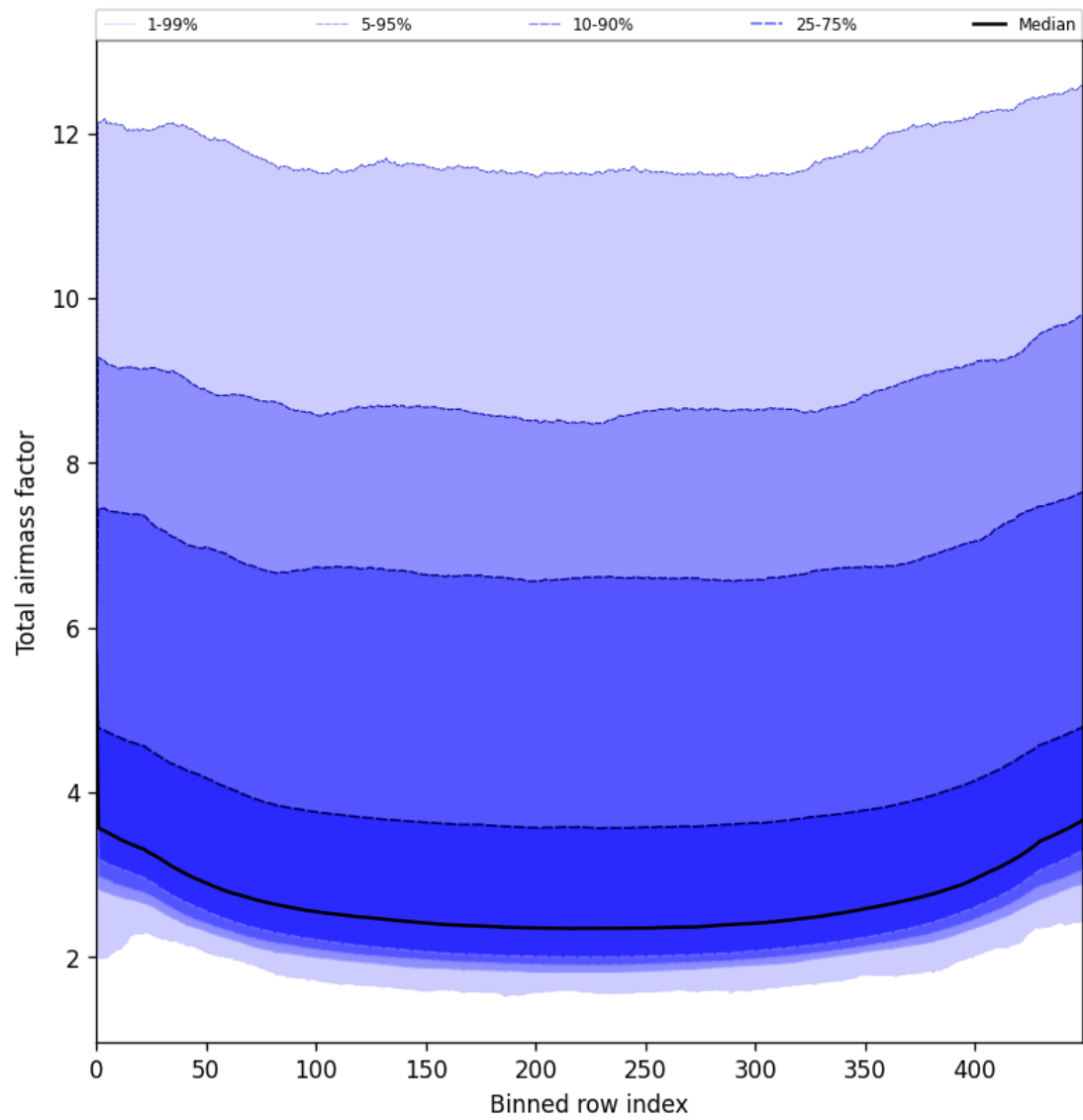
Figure 47: Along track statistics of “Total airmass factor” for 2025-07-13 to 2025-07-14
