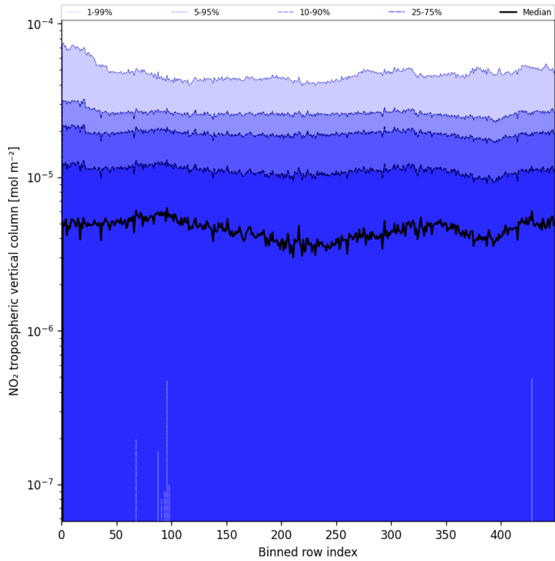
Figure 44: Along track statistics of “NO 2 tropospheric vertical column” for 2025-07-13 to 2025-07-14
