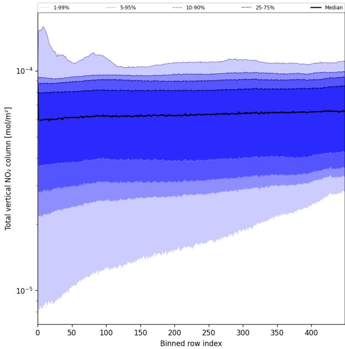
Figure 53: Along track statistics of “Total vertical NO 2 column” for 2025-07-13 to 2025-07-14
