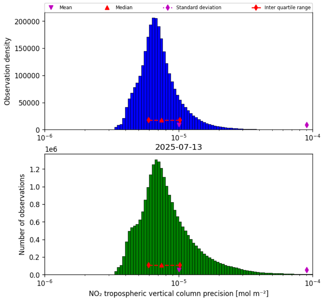
Figure 28: Histogram of “NO 2 tropospheric vertical column precision” for 2025-07-13 to 2025-07-14
