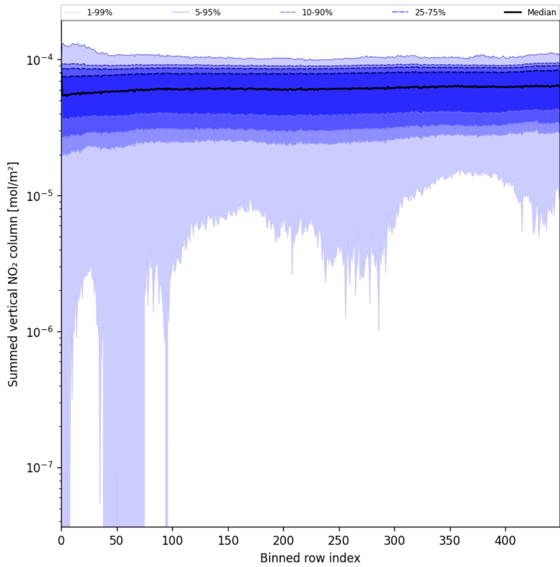
Figure 55: Along track statistics of “Summed vertical NO 2 column” for 2025-07-13 to 2025-07-14
