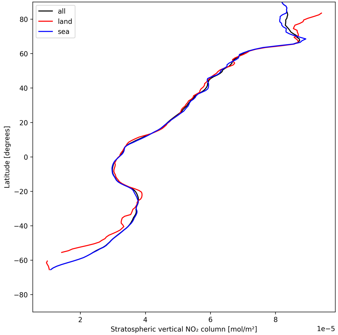
Figure 17: Zonal average of “Stratospheric vertical NO 2 column” for 2025-07-13 to 2025-07-14.
