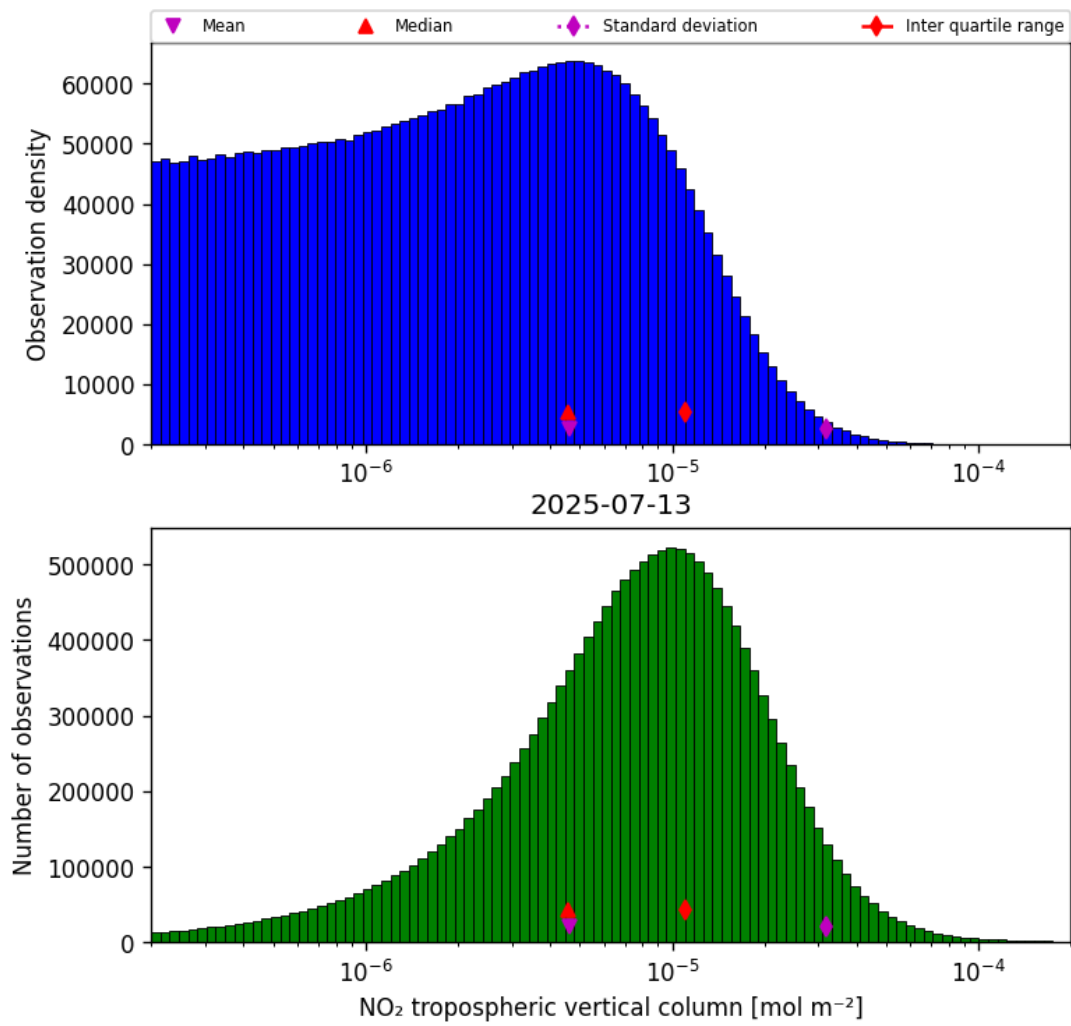
Figure 27: Histogram of “NO 2 tropospheric vertical column” for 2025-07-13 to 2025-07-14
