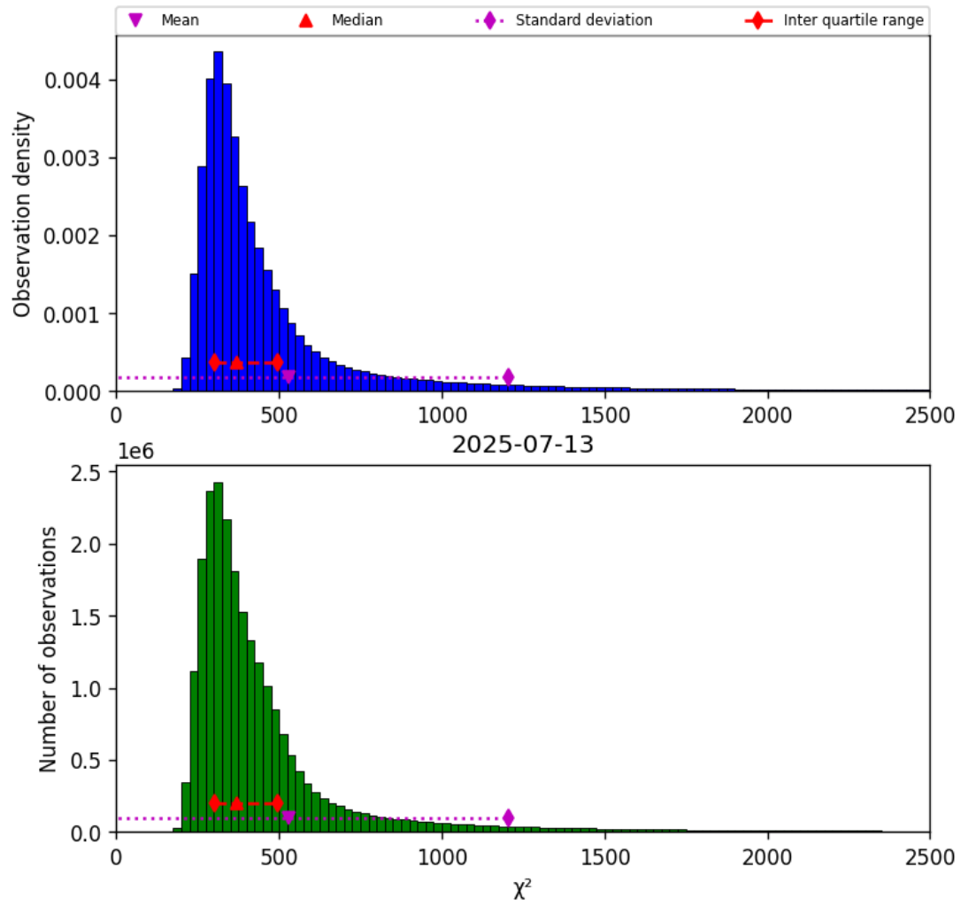
Figure 40: Histogram of “ \chi^2 ” for 2025-07-13 to 2025-07-14
