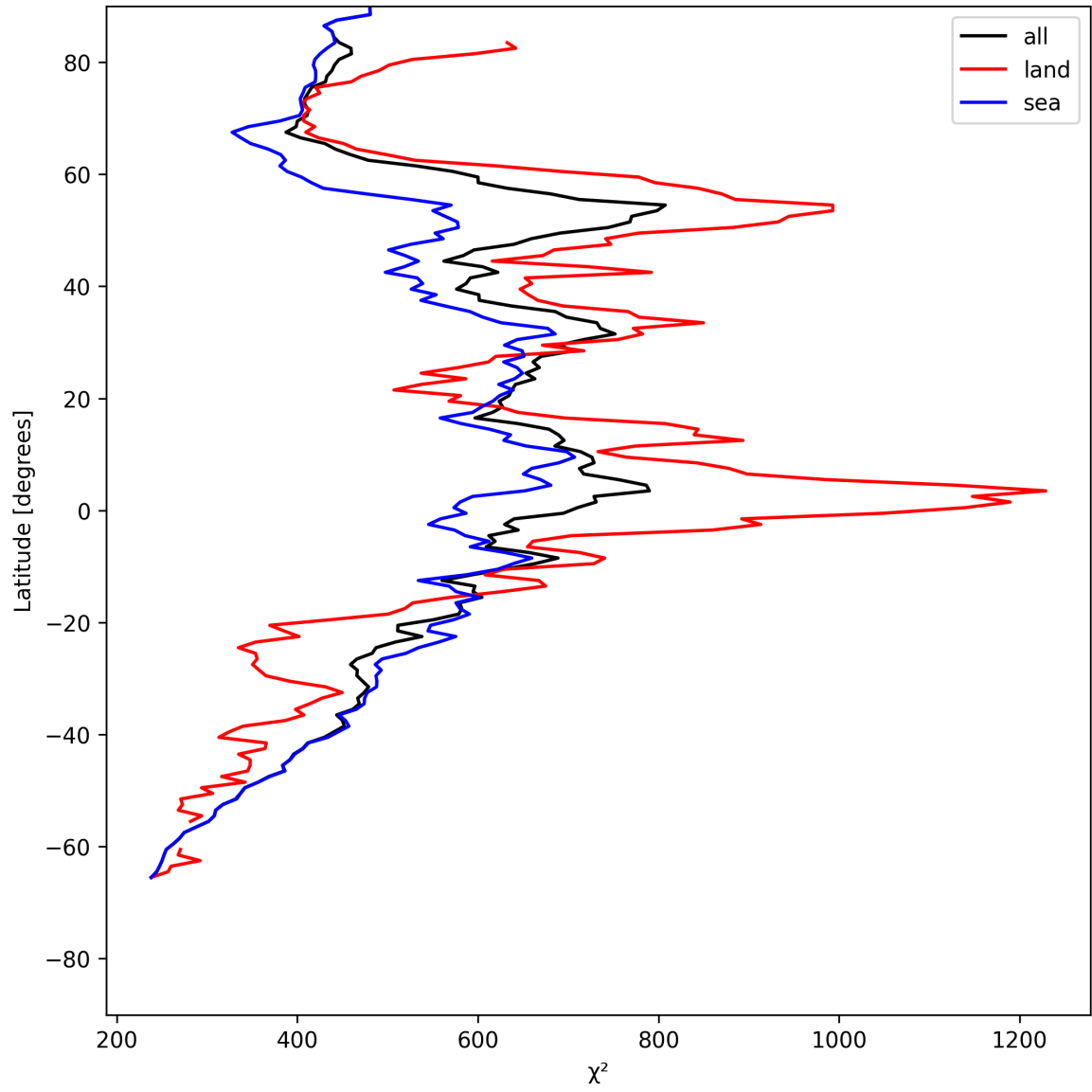
Figure 23: Zonal average of “ \chi^2 ” for 2025-07-13 to 2025-07-14.
