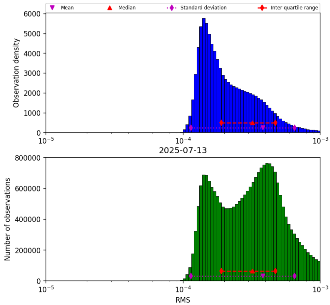
Figure 41: Histogram of “RMS” for 2025-07-13 to 2025-07-14
