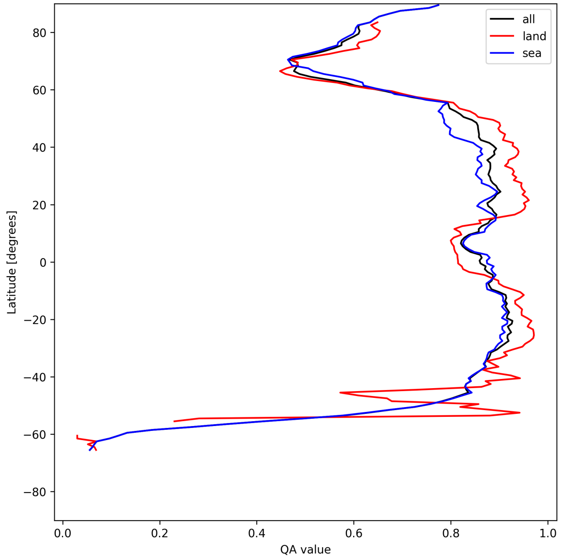
Figure 9: Zonal average of “QA value” for 2025-07-13 to 2025-07-14.
