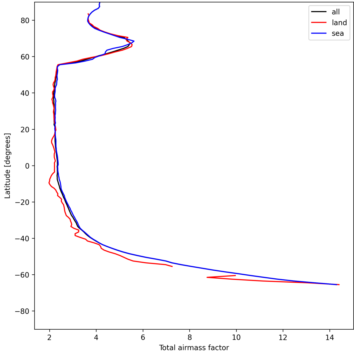
Figure 13: Zonal average of “Total airmass factor” for 2025-07-13 to 2025-07-14.
