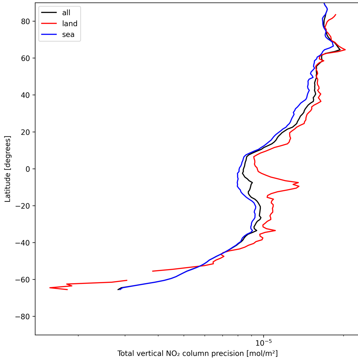
Figure 20: Zonal average of “Total vertical NO 2 column precision” for 2025-07-13 to 2025-07-14.
