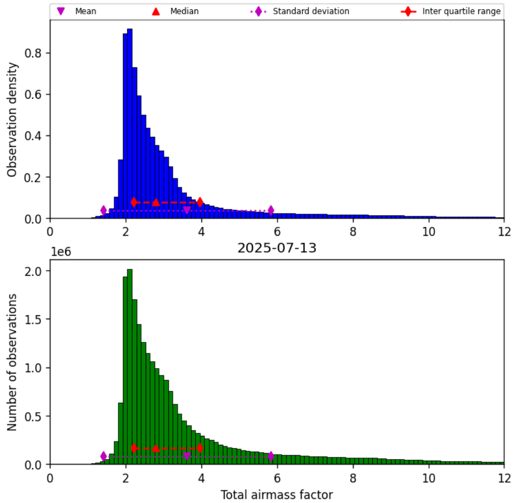
Figure 30: Histogram of “Total airmass factor” for 2025-07-13 to 2025-07-14
