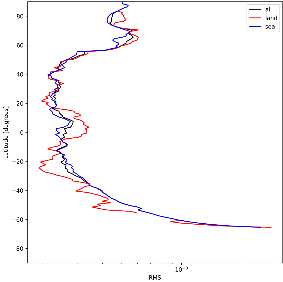
Figure 24: Zonal average of “RMS” for 2025-07-13 to 2025-07-14.
