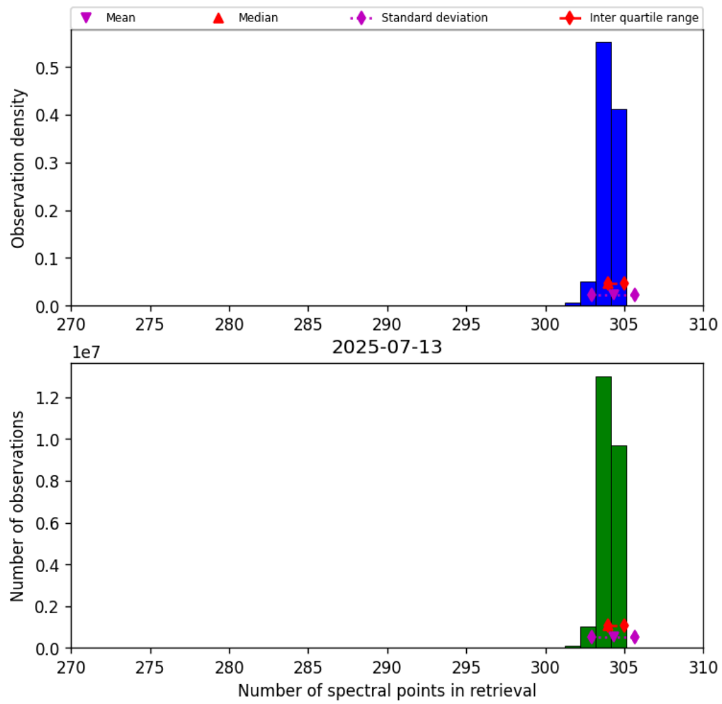
Figure 31: Histogram of “Number of spectral points in retrieval” for 2025-07-13 to 2025-07-14
