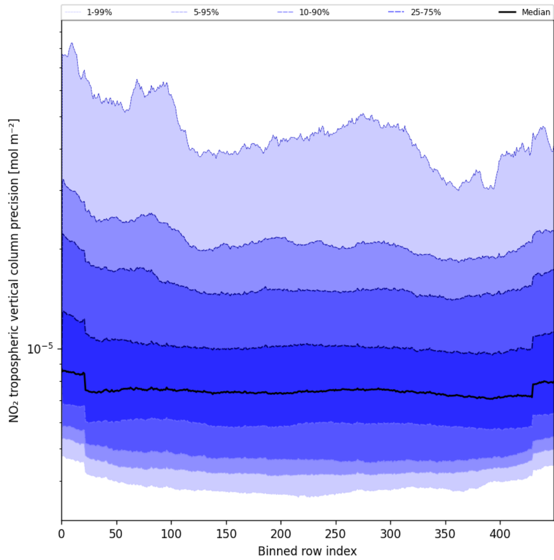
Figure 45: Along track statistics of “NO 2 tropospheric vertical column precision” for 2025-07-13 to 2025-07-14
