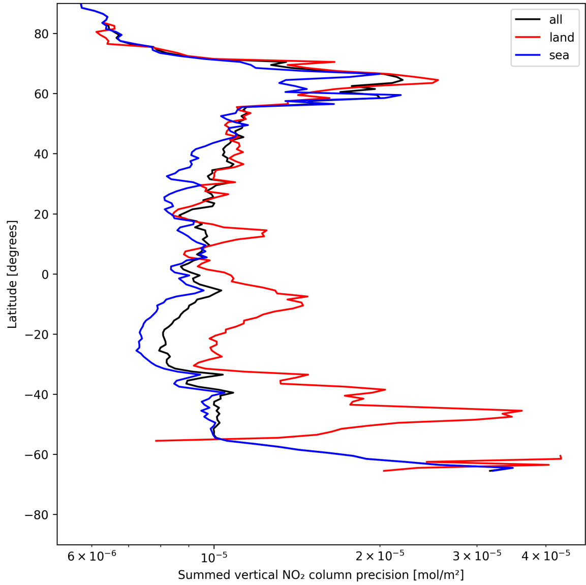
Figure 22: Zonal average of “Summed vertical NO 2 column precision” for 2025-07-13 to 2025-07-14.
