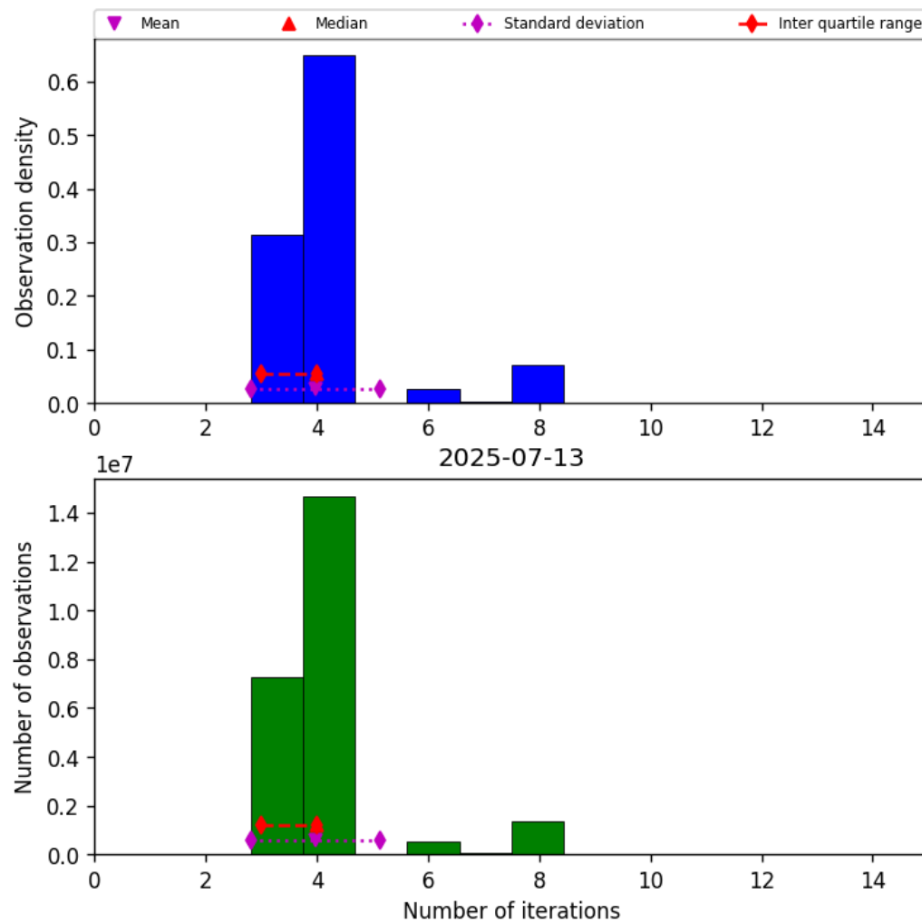
Figure 32: Histogram of “Number of iterations” for 2025-07-13 to 2025-07-14
