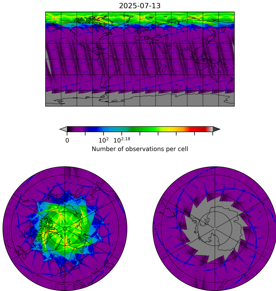
Figure 8: Map of the number of observations for 2025-07-13 to 2025-07-14
