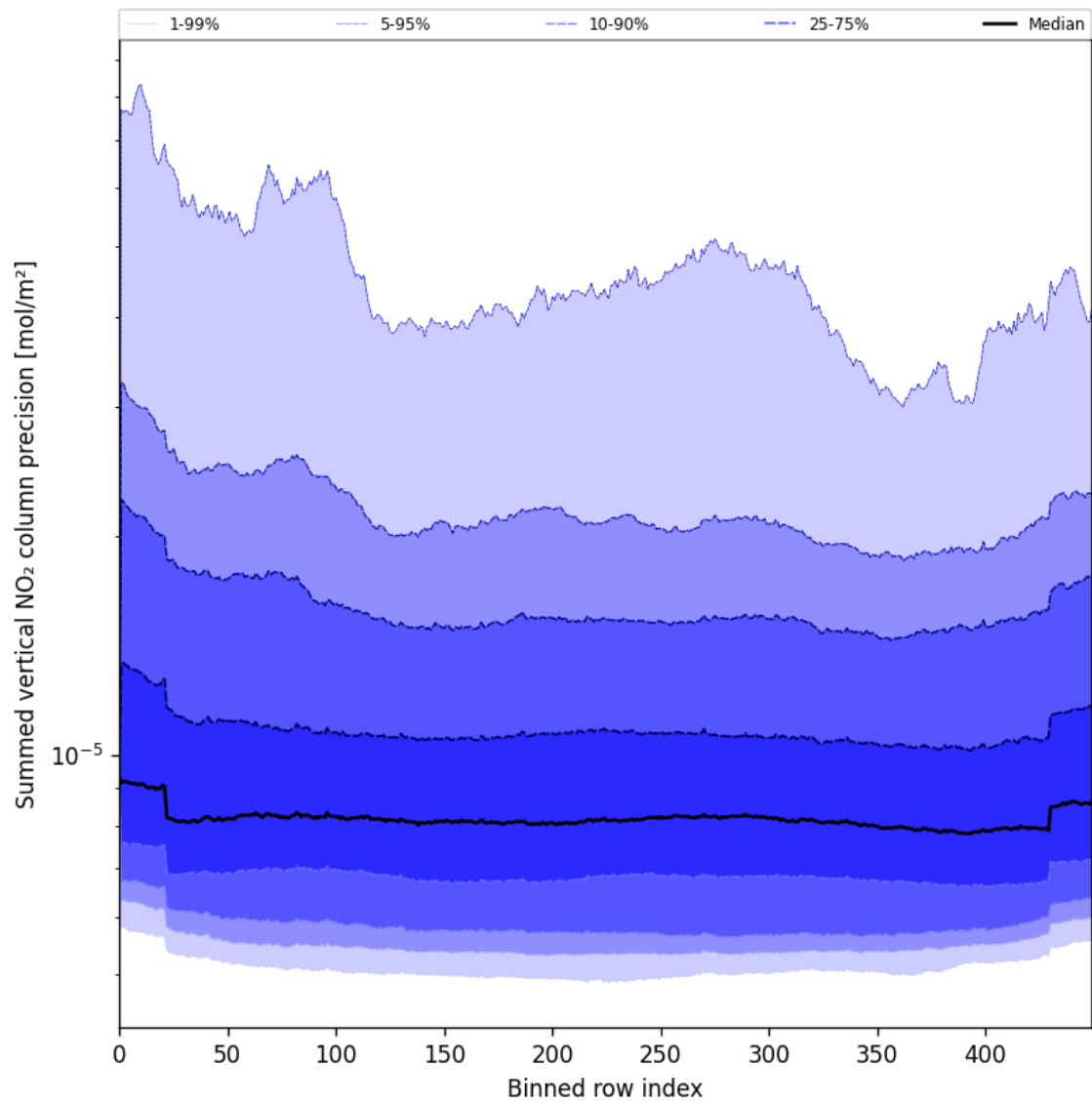
Figure 56: Along track statistics of “Summed vertical NO 2 column precision” for 2025-07-13 to 2025-07-14
