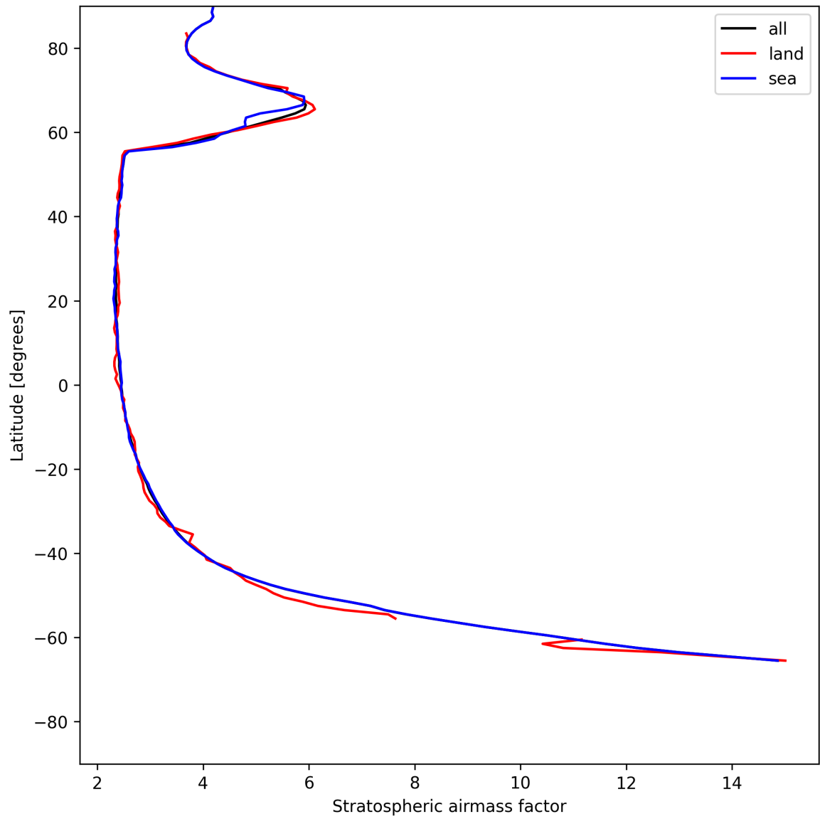
Figure 25: Zonal average of “Stratospheric airmass factor” for 2025-07-13 to 2025-07-14.
