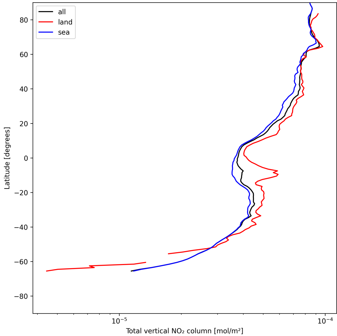
Figure 19: Zonal average of “Total vertical NO 2 column” for 2025-07-13 to 2025-07-14.
