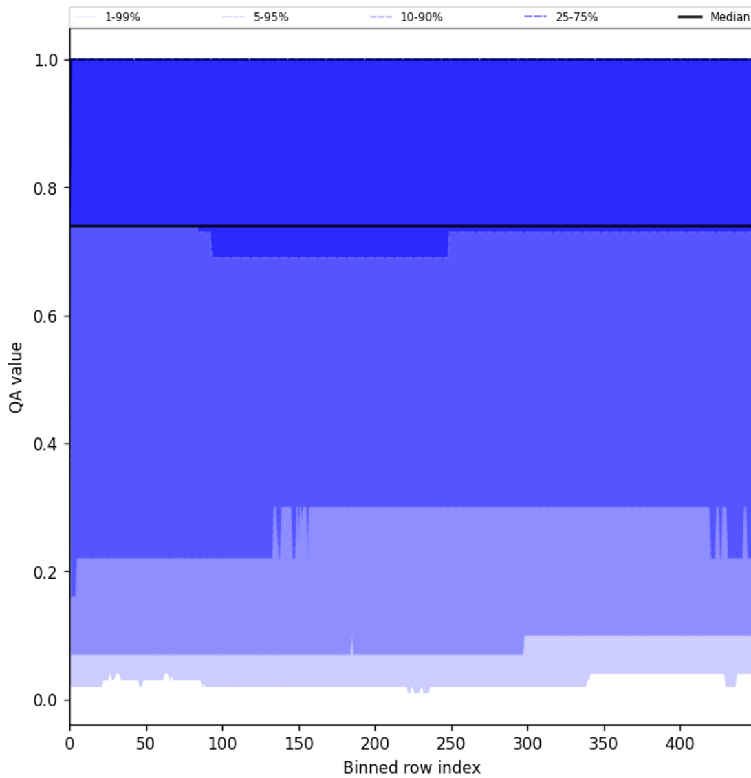
Figure 43: Along track statistics of "QA value" for 2025-07-13 to 2025-07-14
