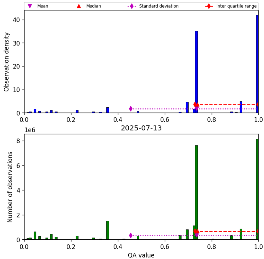
Figure 26: Histogram of “QA value” for 2025-07-13 to 2025-07-14
