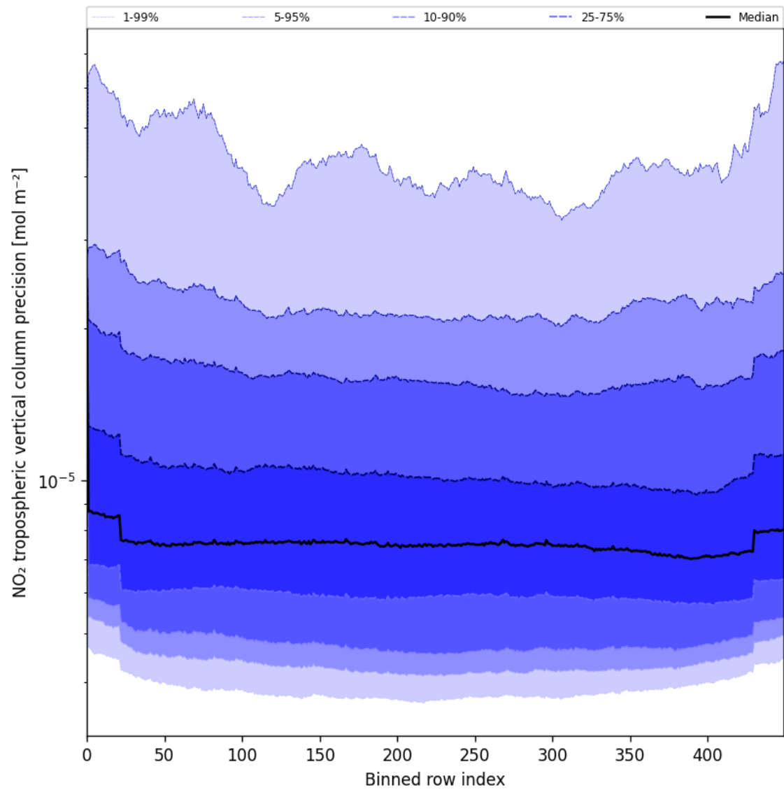
Figure 45: Along track statistics of “NO 2 tropospheric vertical column precision” for 2025-07-15 to 2025-07-16
