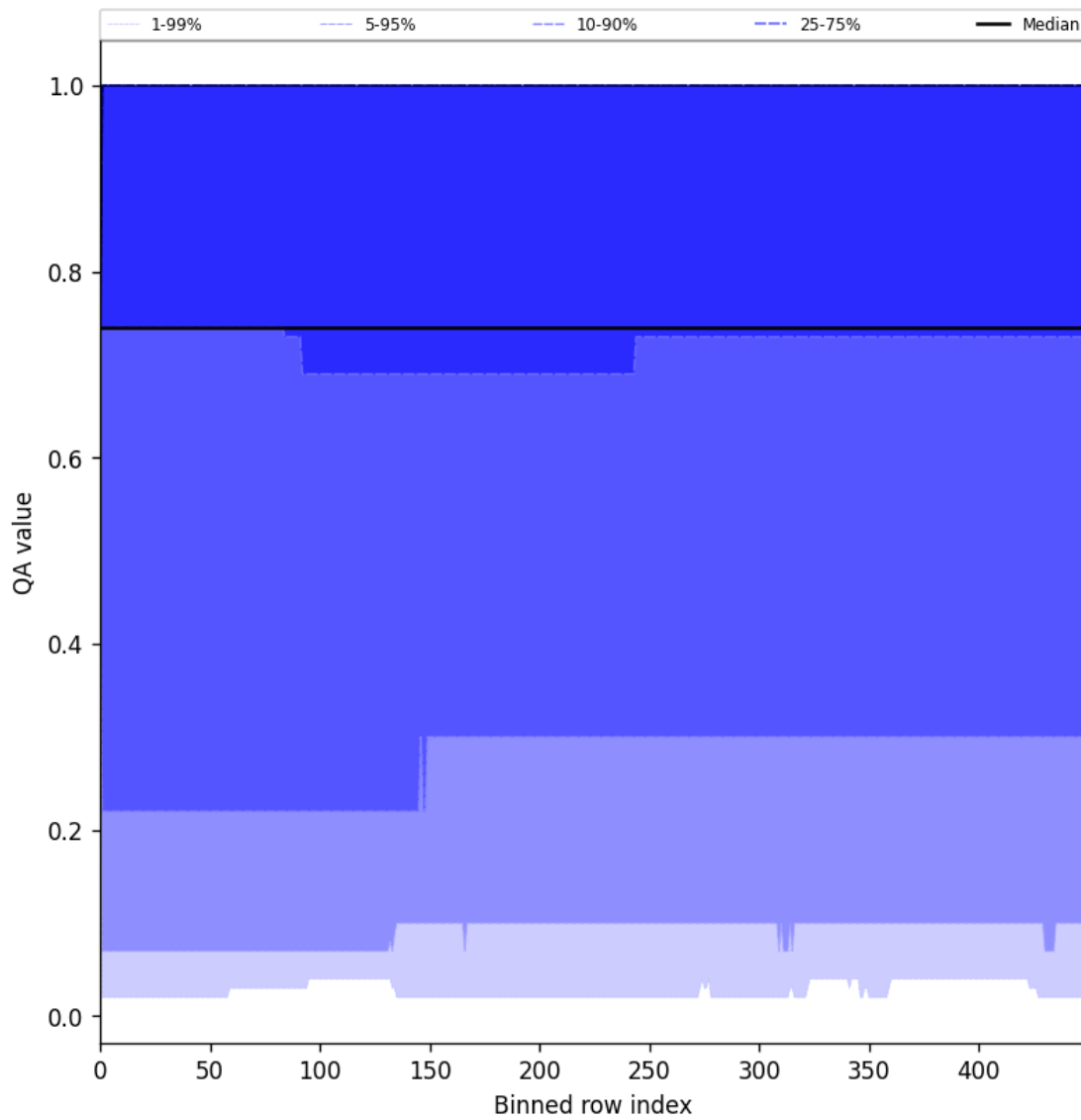
Figure 43: Along track statistics of “QA value” for 2025-07-15 to 2025-07-16
