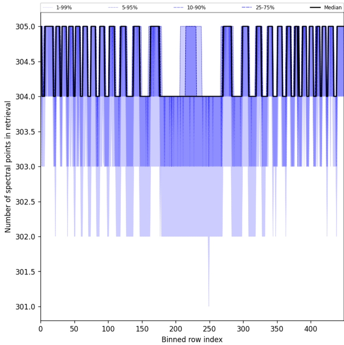
Figure 48: Along track statistics of “Number of spectral points in retrieval” for 2025-07-15 to 2025-07-16
