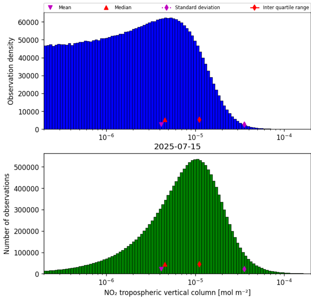
Figure 27: Histogram of “NO 2 tropospheric vertical column” for 2025-07-15 to 2025-07-16
