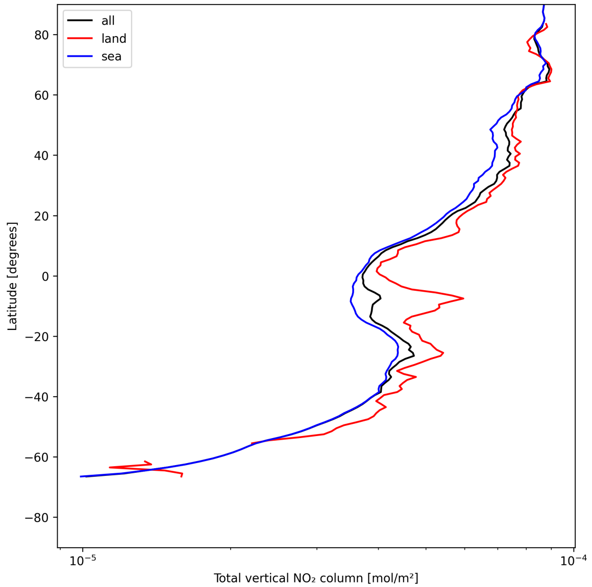
Figure 19: Zonal average of “Total vertical NO 2 column” for 2025-07-15 to 2025-07-16.
