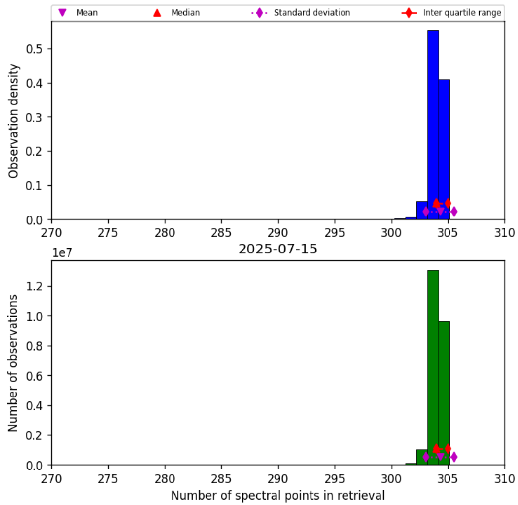
Figure 31: Histogram of “Number of spectral points in retrieval” for 2025-07-15 to 2025-07-16
