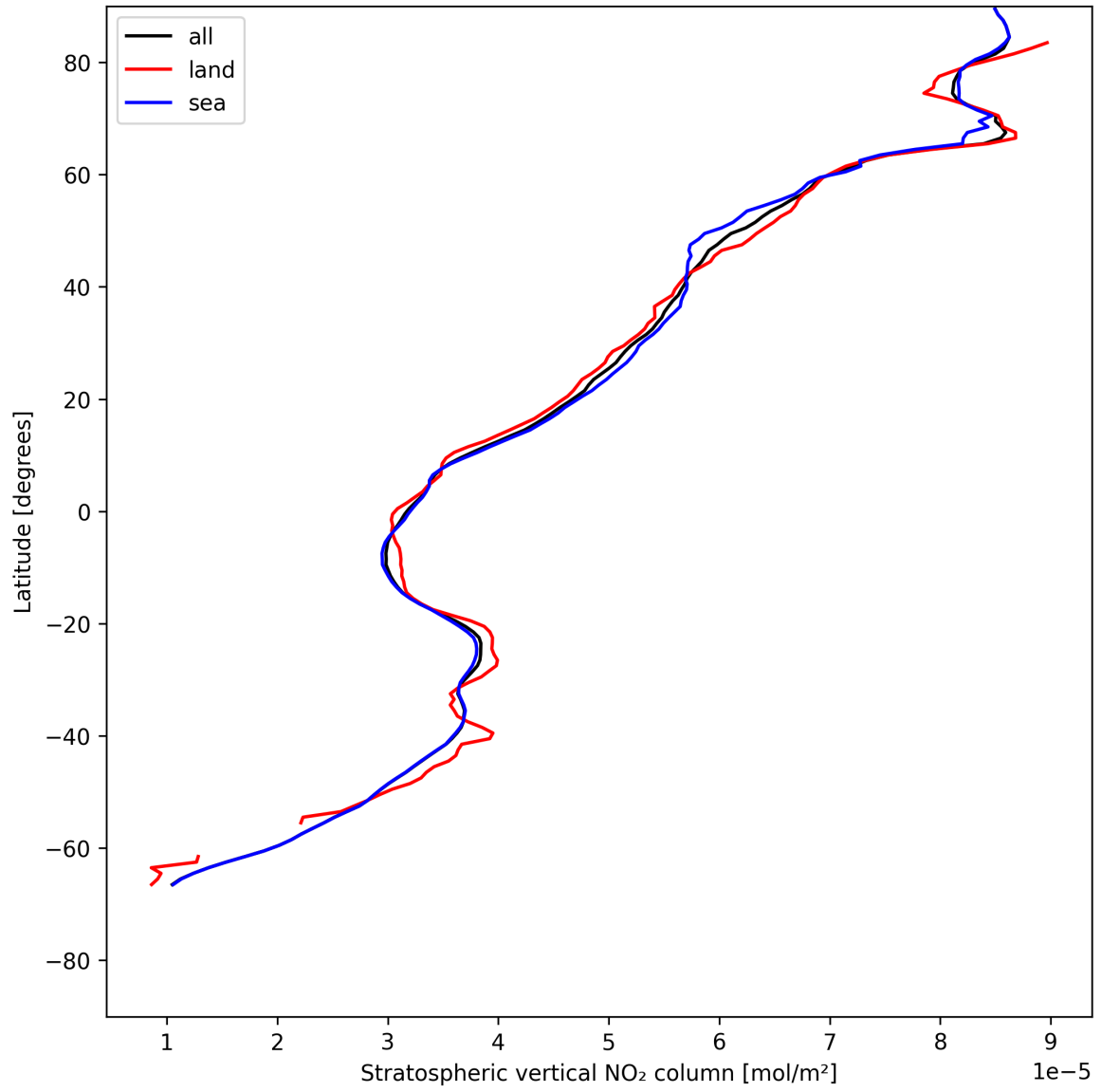
Figure 17: Zonal average of “Stratospheric vertical NO 2 column” for 2025-07-15 to 2025-07-16.
