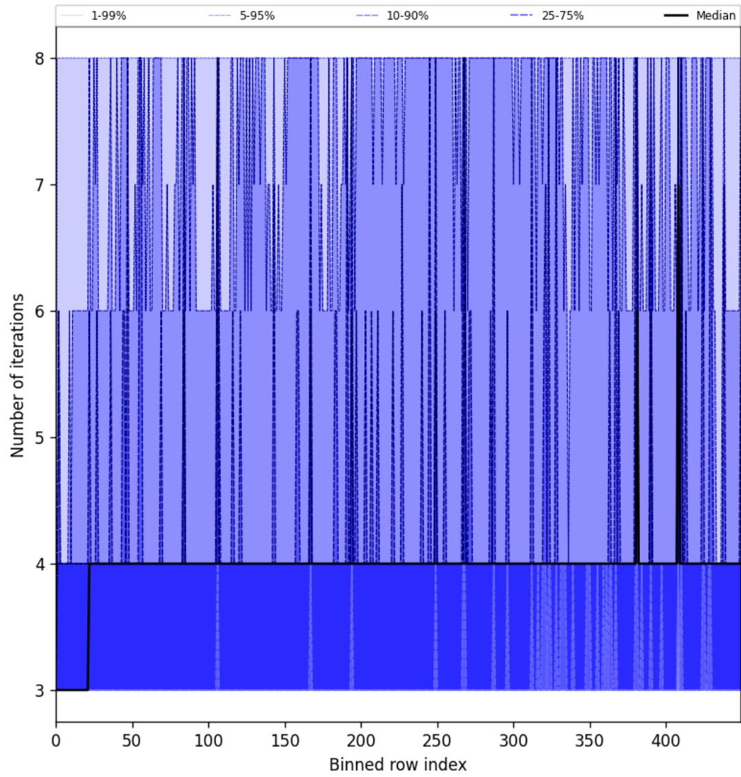
Figure 49: Along track statistics of “Number of iterations” for 2025-07-15 to 2025-07-16
