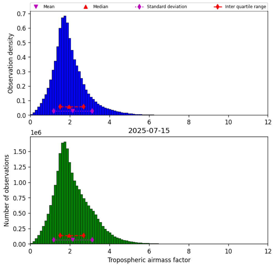
Figure 29: Histogram of “Tropospheric airmass factor” for 2025-07-15 to 2025-07-16
