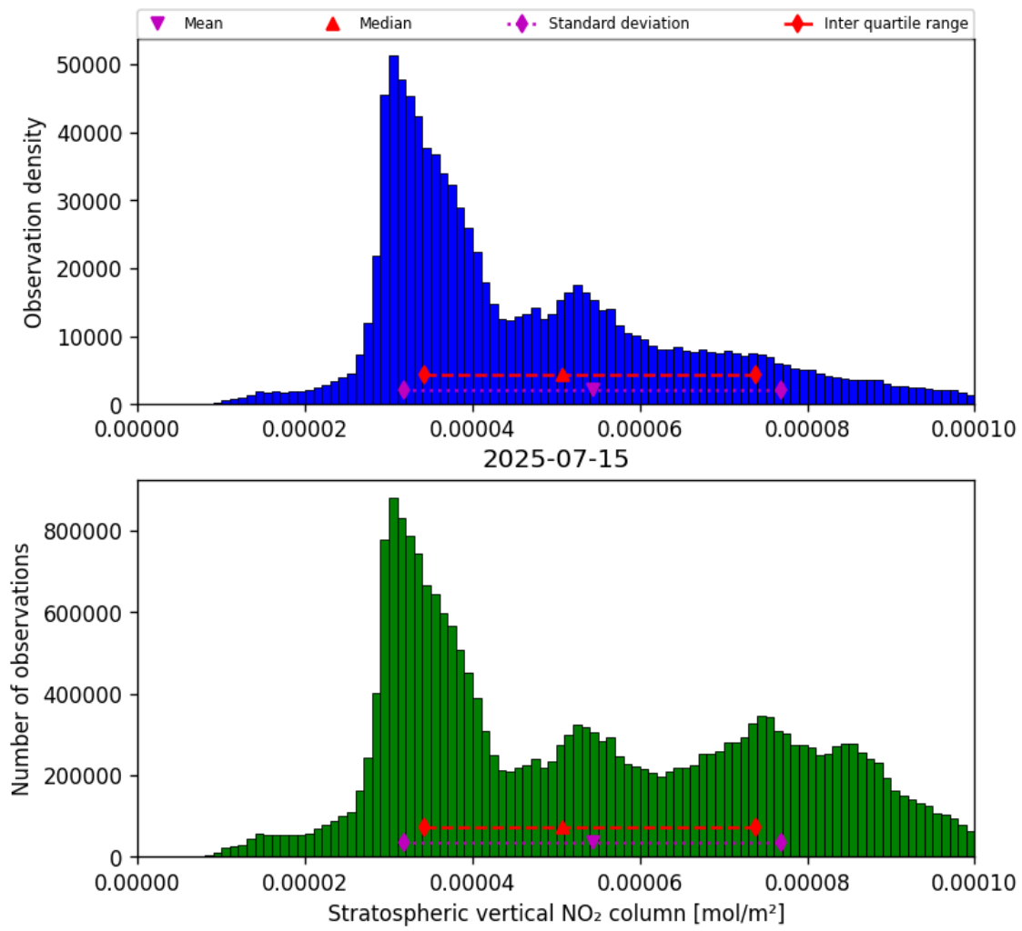
Figure 34: Histogram of “Stratospheric vertical NO 2 column” for 2025-07-15 to 2025-07-16
