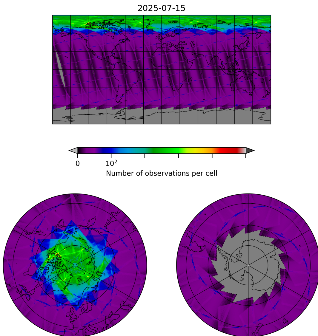
Figure 8: Map of the number of observations for 2025-07-15 to 2025-07-16
