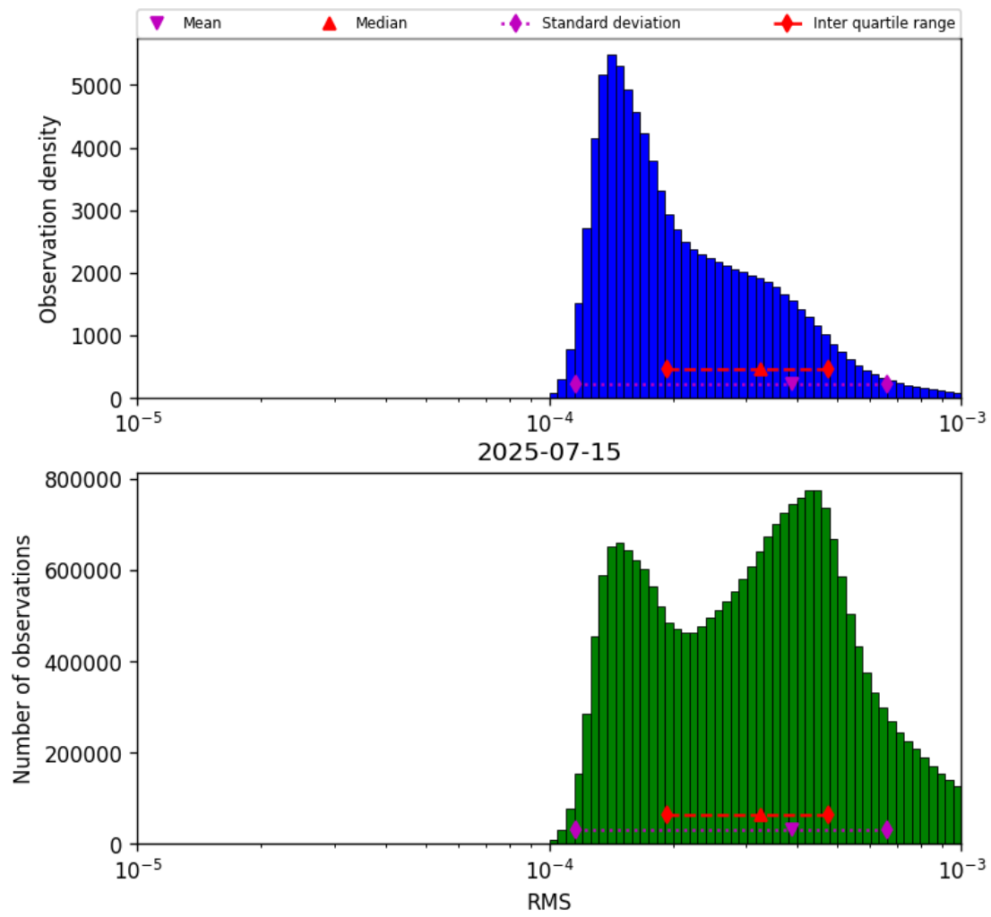
Figure 41: Histogram of “RMS” for 2025-07-15 to 2025-07-16
