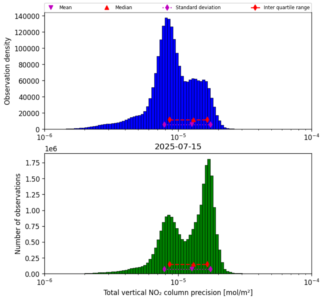
Figure 37: Histogram of “Total vertical NO 2 column precision” for 2025-07-15 to 2025-07-16
