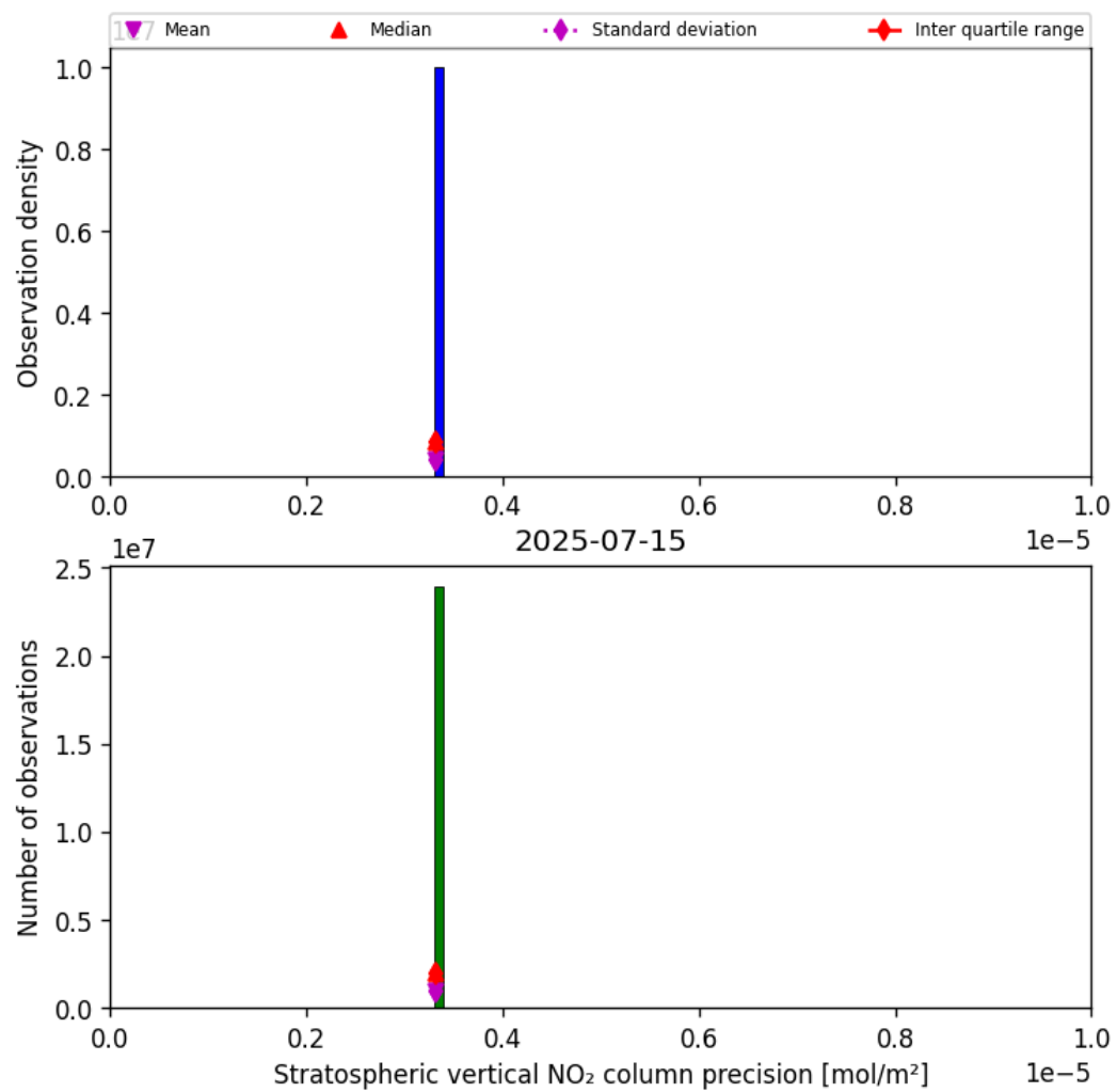
Figure 35: Histogram of “Stratospheric vertical NO 2 column precision” for 2025-07-15 to 2025-07-16
