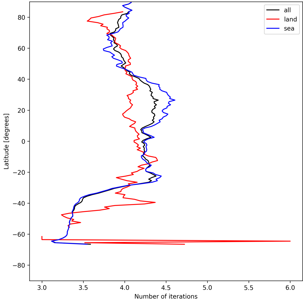
Figure 15: Zonal average of “Number of iterations” for 2025-07-15 to 2025-07-16.
