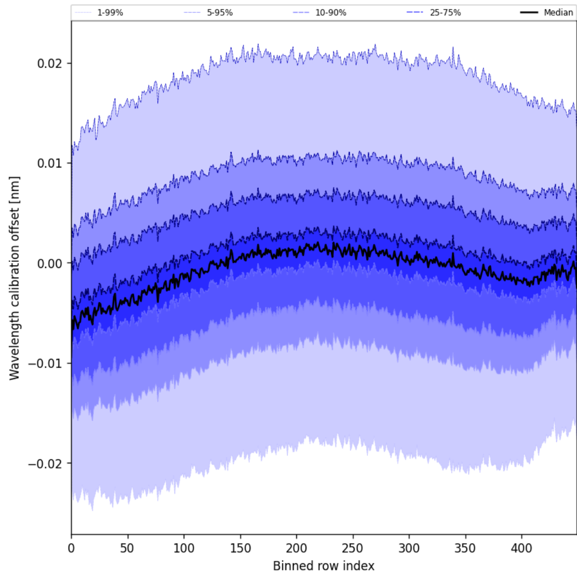
Figure 50: Along track statistics of “Wavelength calibration offset” for 2025-07-15 to 2025-07-16
