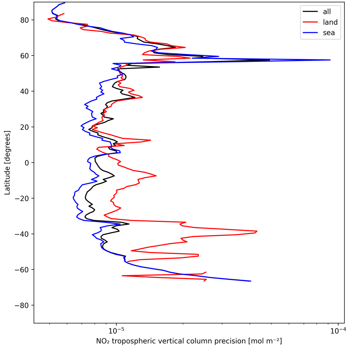
Figure 11: Zonal average of “NO 2 tropospheric vertical column precision” for 2025-07-15 to 2025-07-16.
