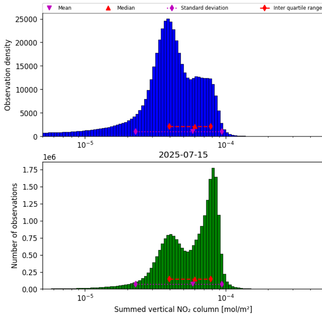
Figure 38: Histogram of "Summed vertical NO 2 column" for 2025-07-15 to 2025-07-16
