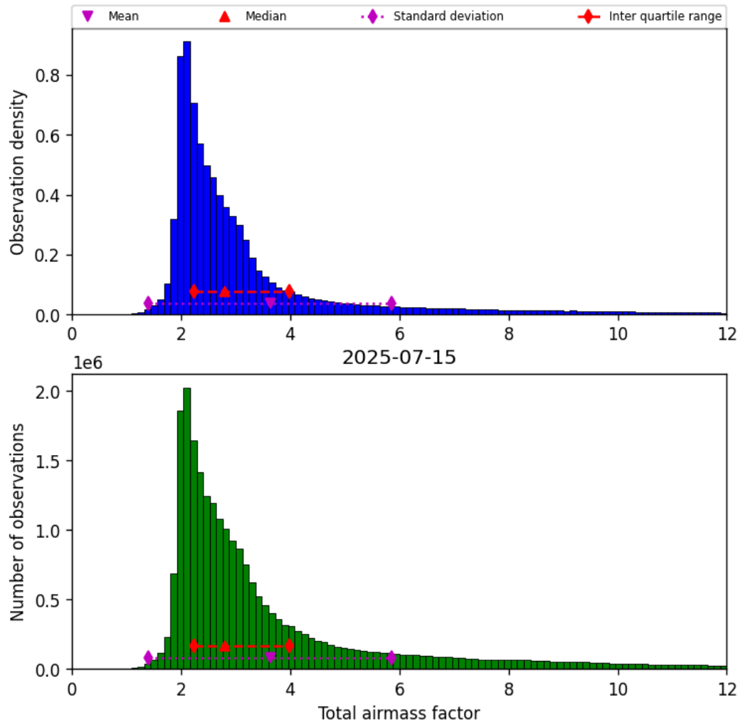
Figure 30: Histogram of “Total airmass factor” for 2025-07-15 to 2025-07-16
