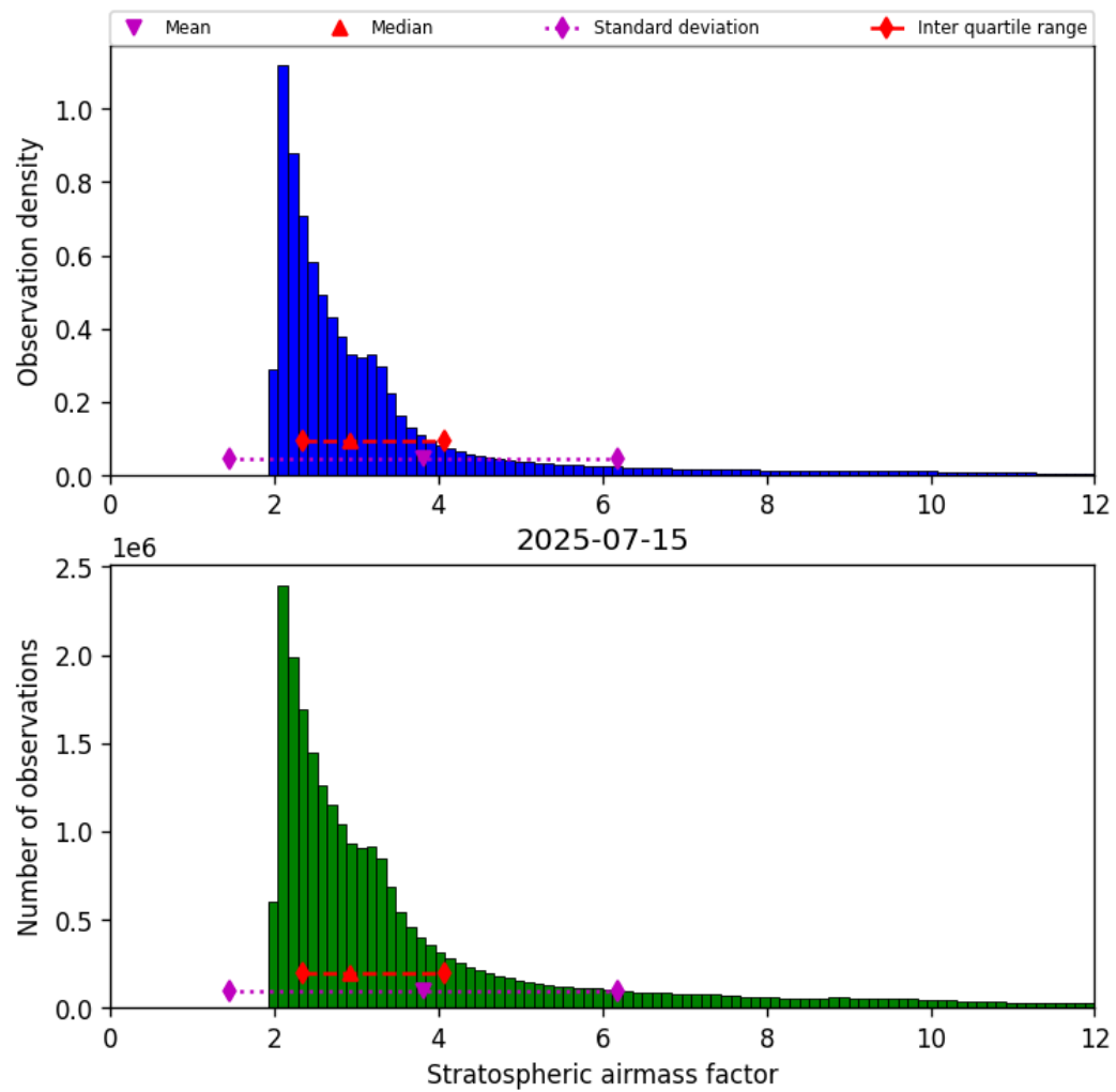
Figure 42: Histogram of “Stratospheric airmass factor” for 2025-07-15 to 2025-07-16
