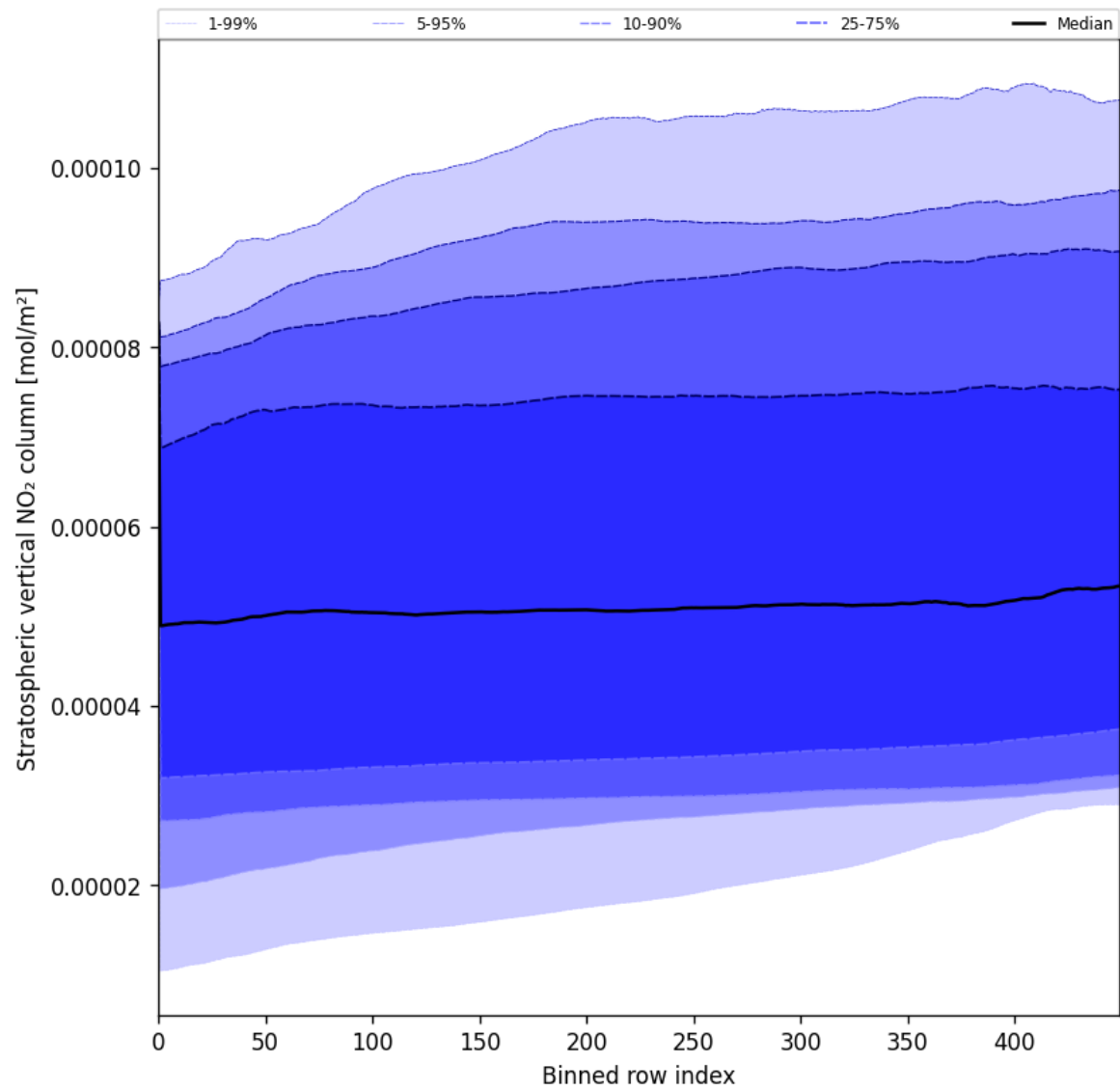
Figure 51: Along track statistics of “Stratospheric vertical NO 2 column” for 2025-07-15 to 2025-07-16
