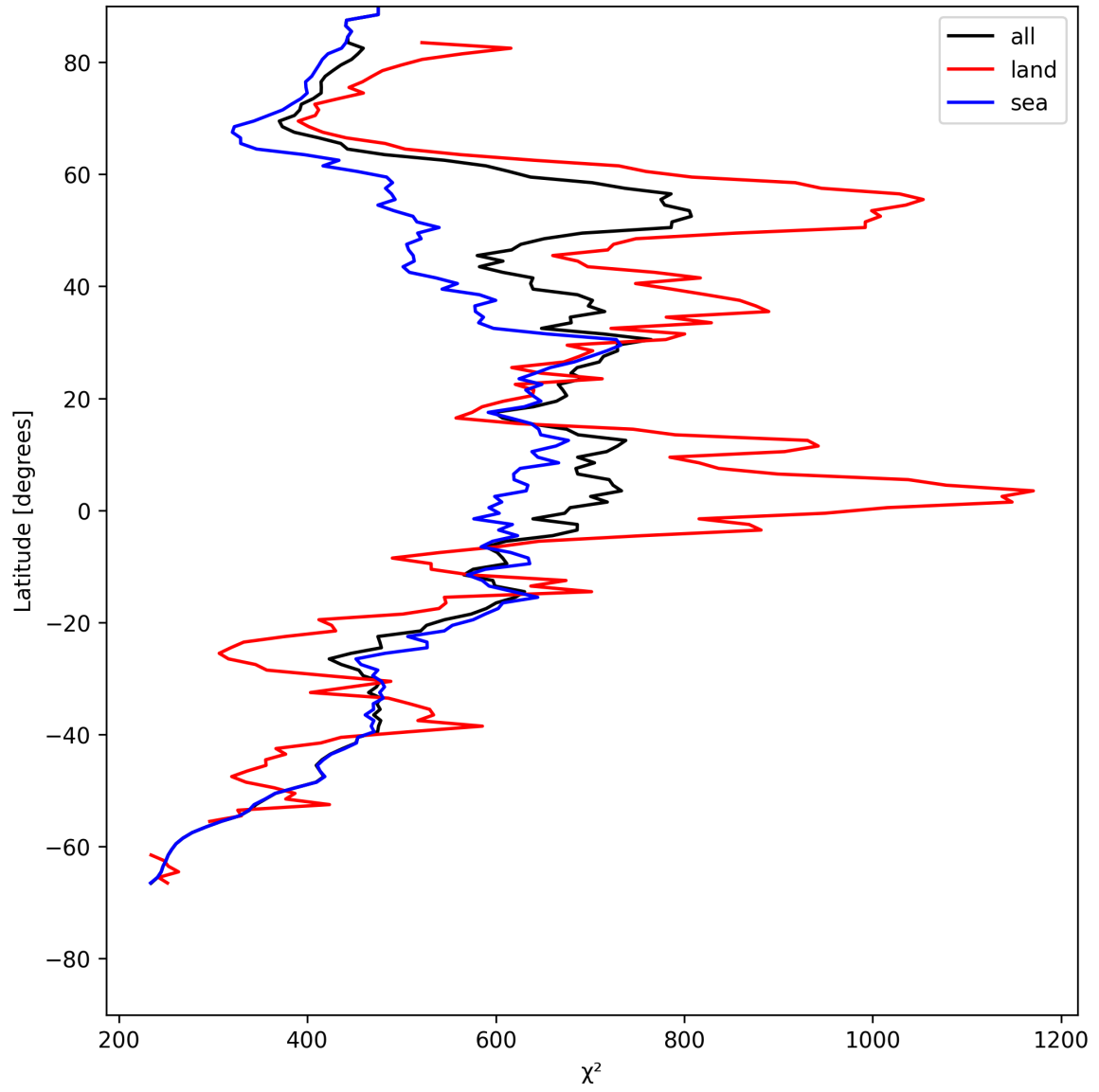
Figure 23: Zonal average of “ \chi^2 ” for 2025-07-15 to 2025-07-16.
