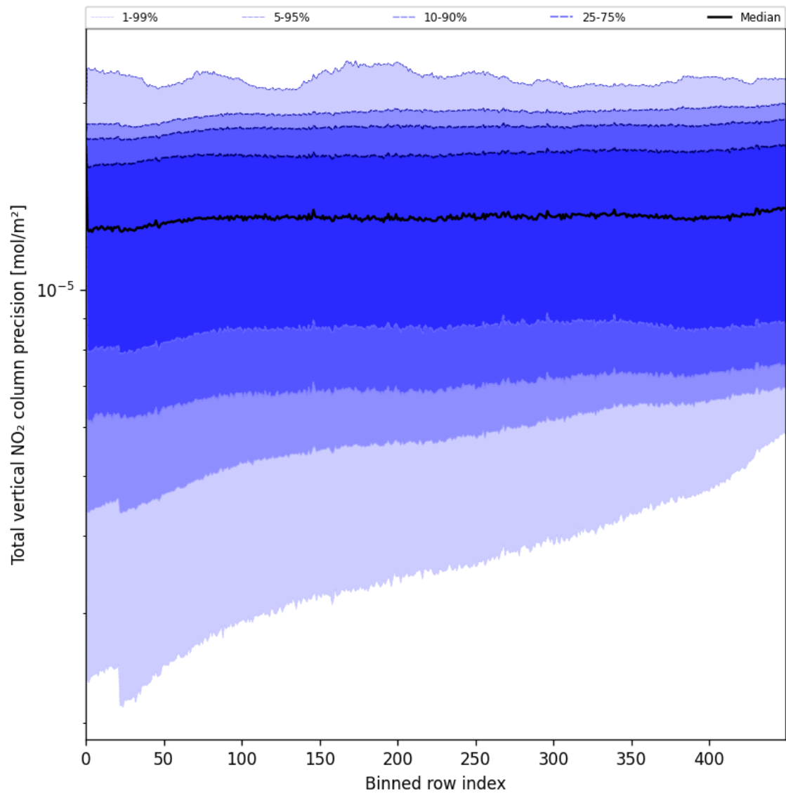
Figure 54: Along track statistics of “Total vertical NO 2 column precision” for 2025-07-15 to 2025-07-16
