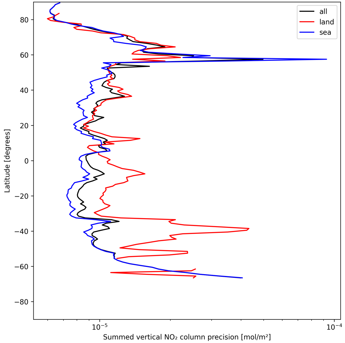
Figure 22: Zonal average of “Summed vertical NO 2 column precision” for 2025-07-15 to 2025-07-16.
