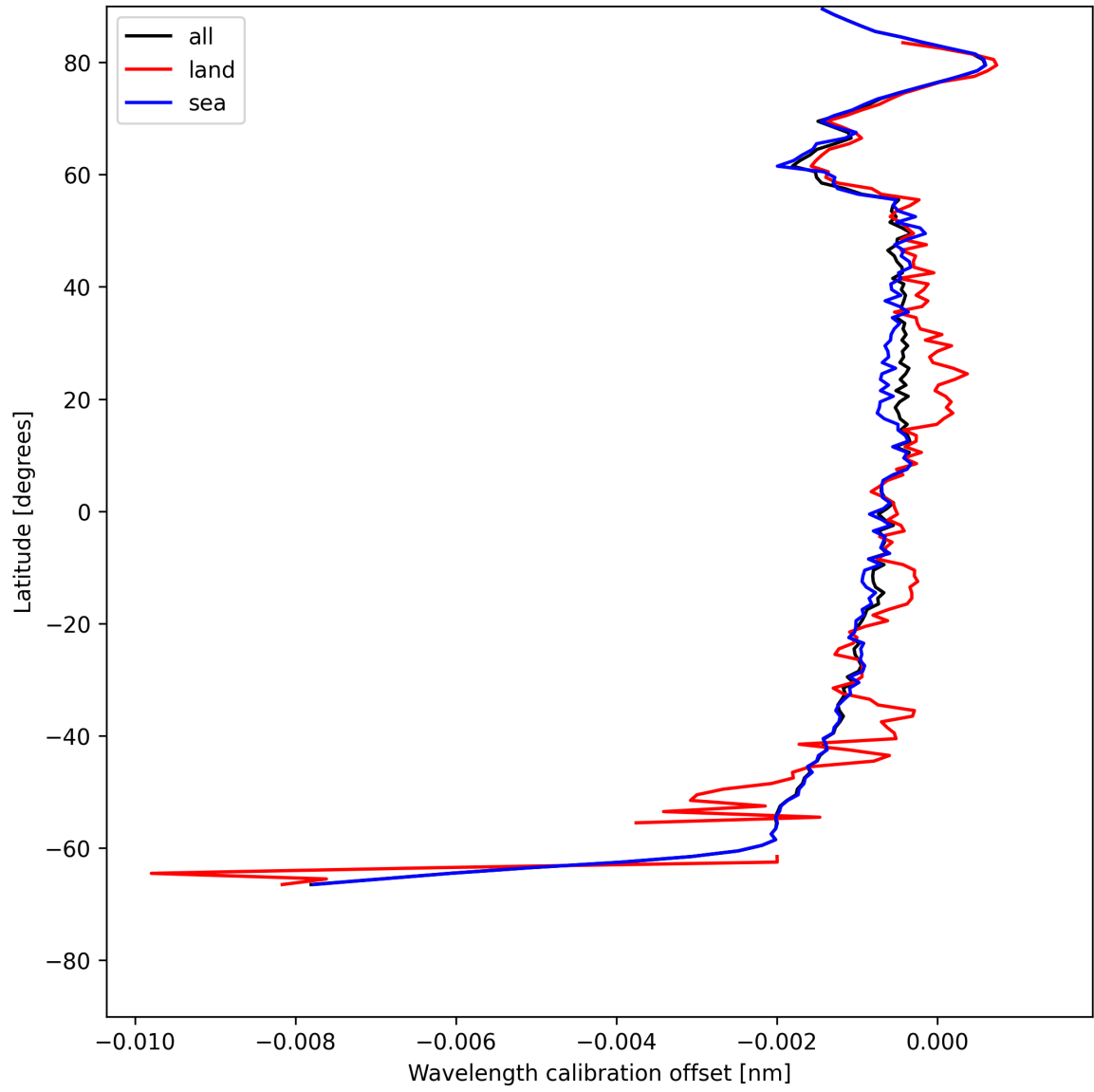
Figure 16: Zonal average of “Wavelength calibration offset” for 2025-07-15 to 2025-07-16.
