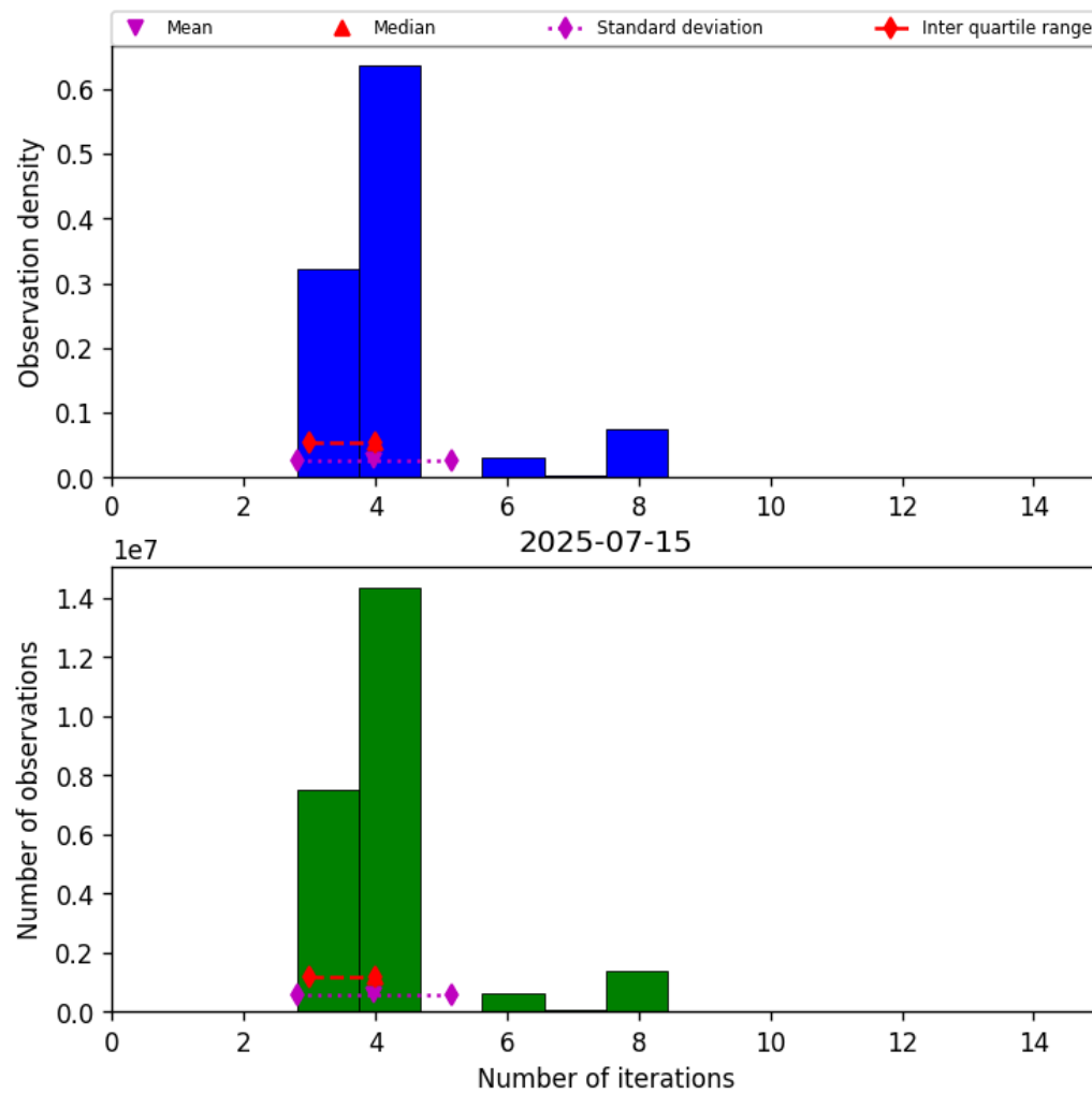
Figure 32: Histogram of “Number of iterations” for 2025-07-15 to 2025-07-16
