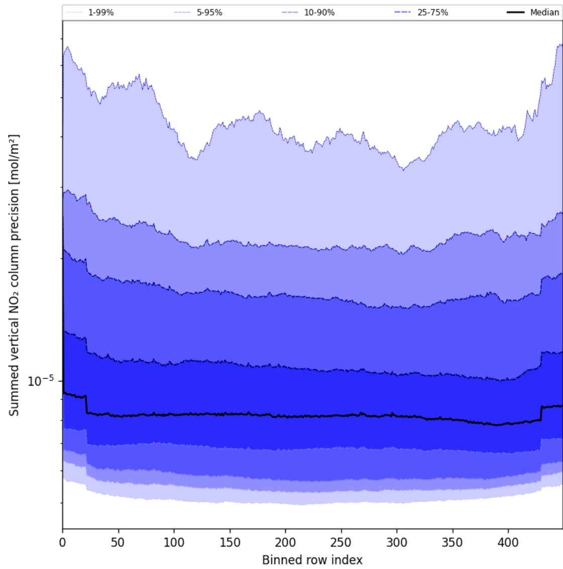
Figure 56: Along track statistics of “Summed vertical NO 2 column precision” for 2025-07-15 to 2025-07-16
