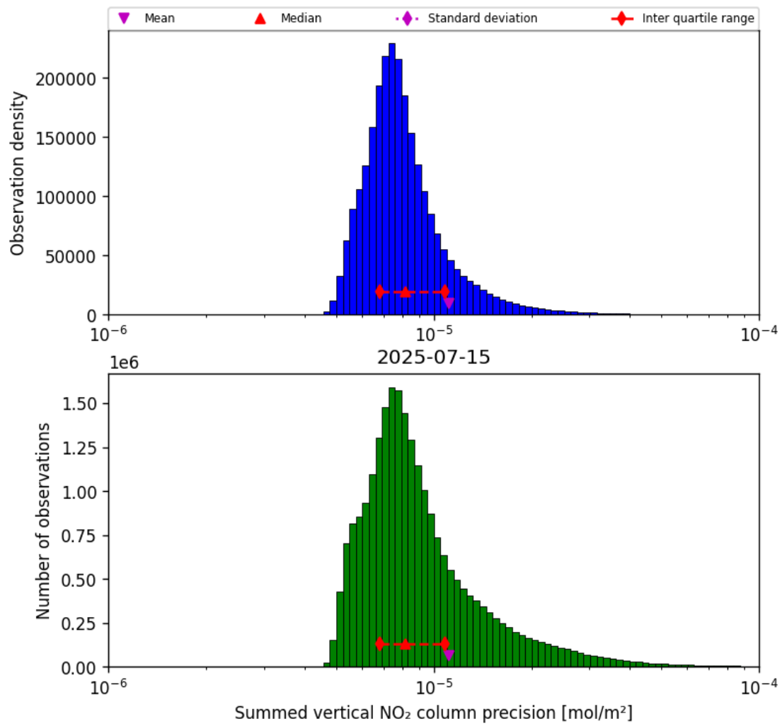
Figure 39: Histogram of "Summed vertical NO 2 column precision" for 2025-07-15 to 2025-07-16
