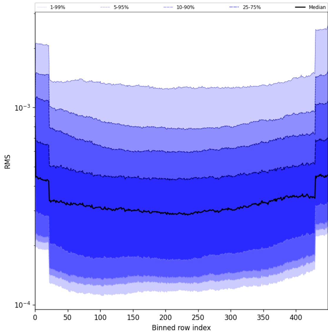
Figure 58: Along track statistics of “RMS” for 2025-07-15 to 2025-07-16
