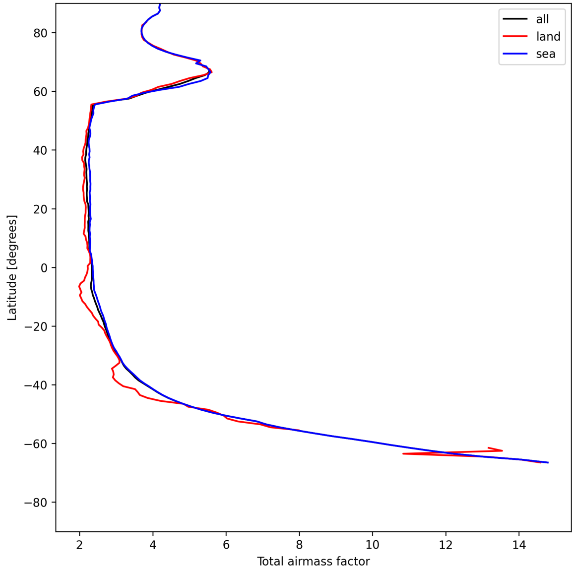
Figure 13: Zonal average of “Total airmass factor” for 2025-07-15 to 2025-07-16.
