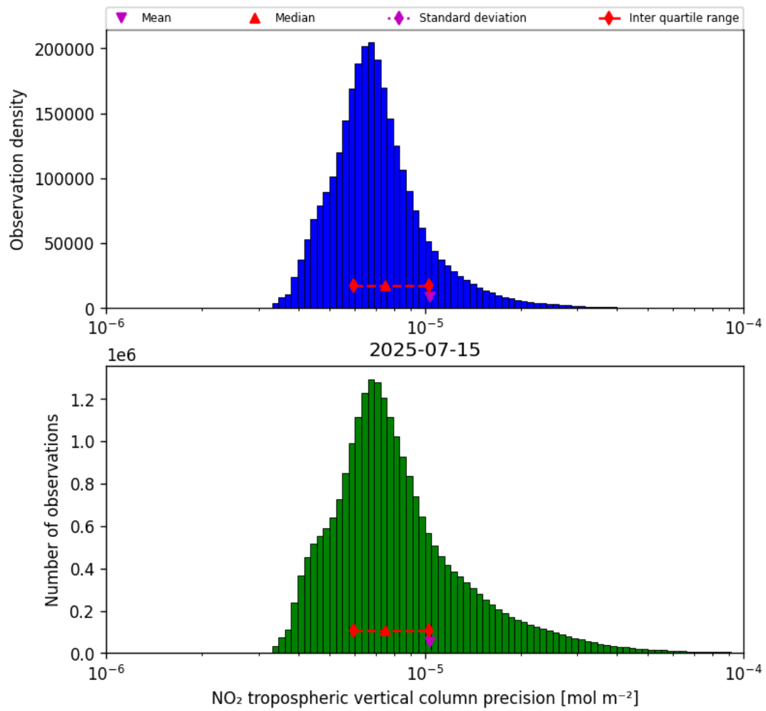
Figure 28: Histogram of “NO 2 tropospheric vertical column precision” for 2025-07-15 to 2025-07-16
