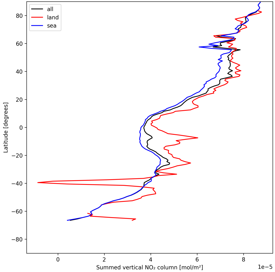
Figure 21: Zonal average of “Summed vertical NO 2 column” for 2025-07-15 to 2025-07-16.
