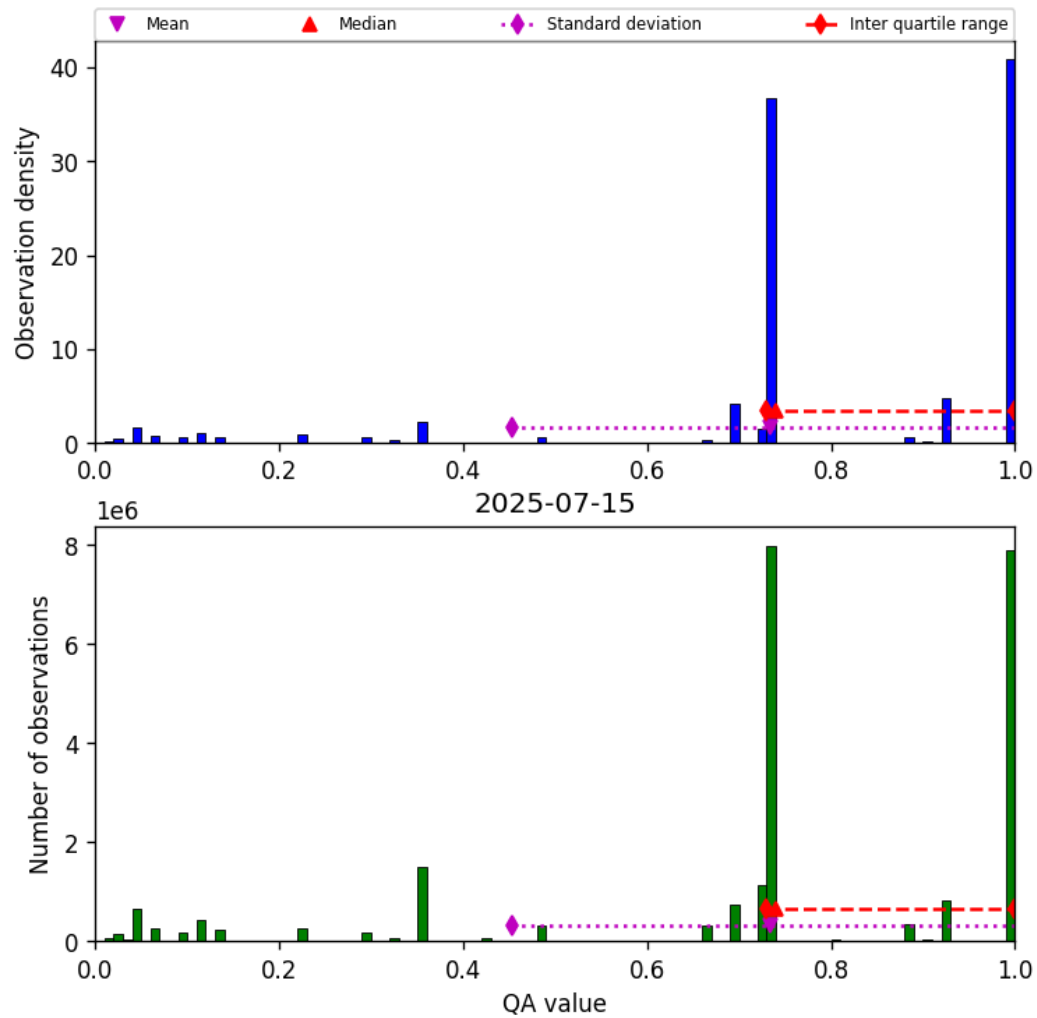
Figure 26: Histogram of “QA value” for 2025-07-15 to 2025-07-16
