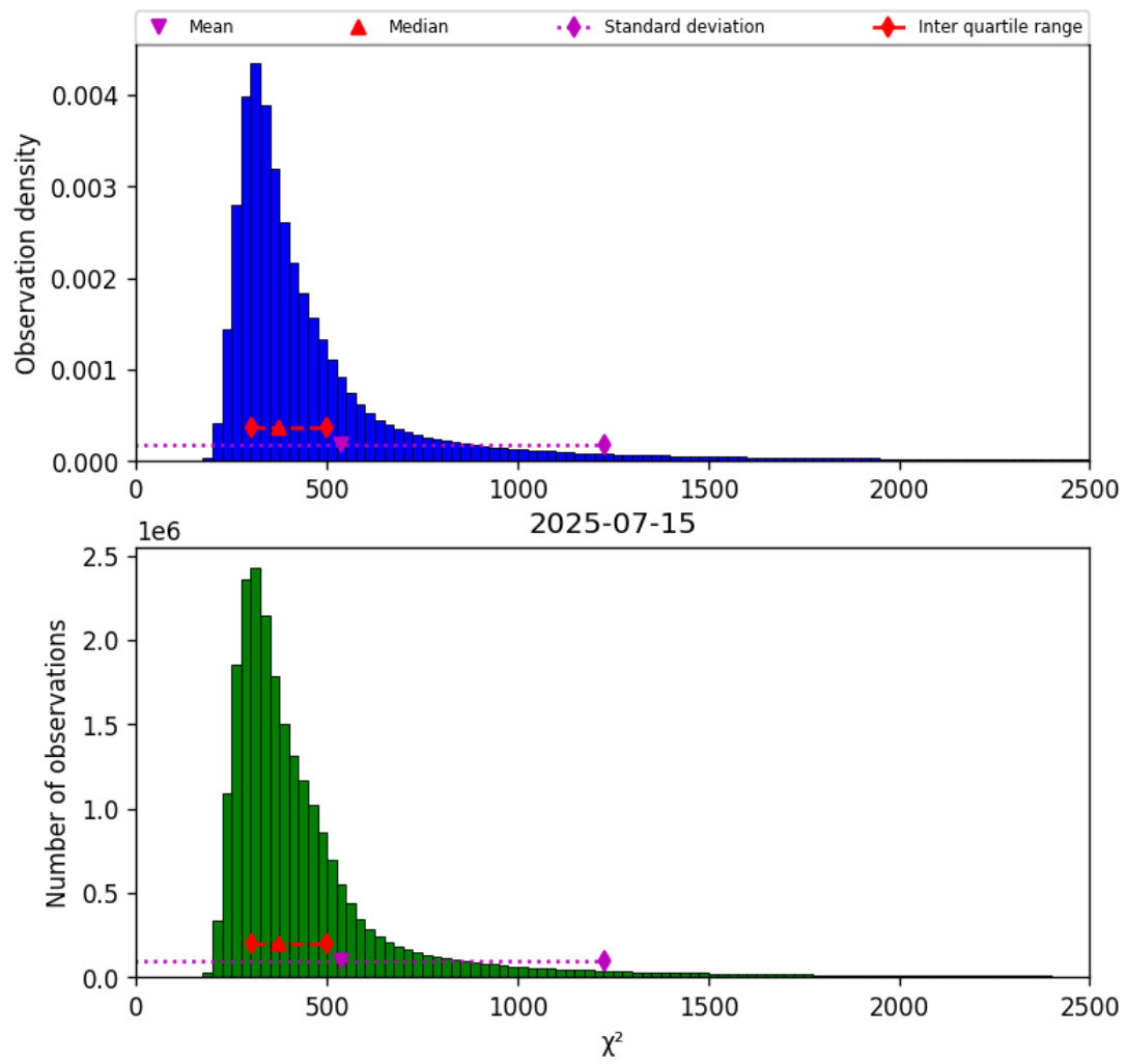
Figure 40: Histogram of “ \chi^2 ” for 2025-07-15 to 2025-07-16
