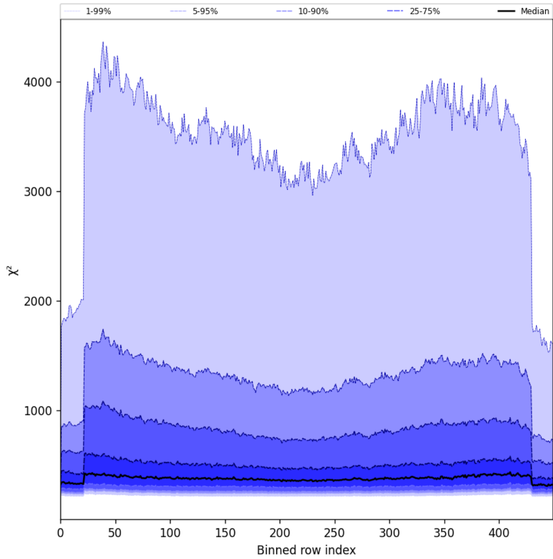
Figure 57: Along track statistics of “ \chi^2 ” for 2025-07-15 to 2025-07-16
