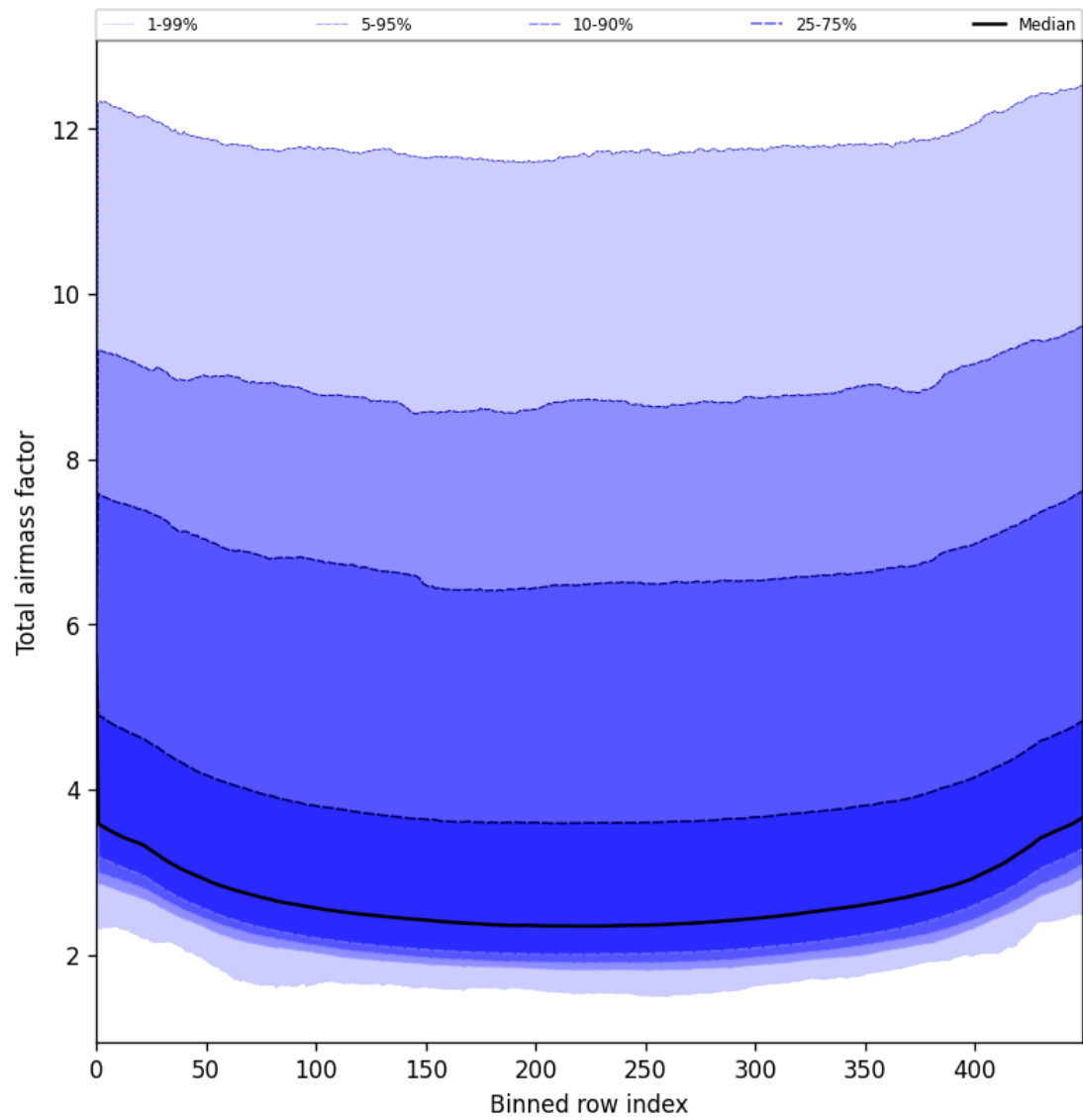
Figure 47: Along track statistics of “Total airmass factor” for 2025-07-15 to 2025-07-16
