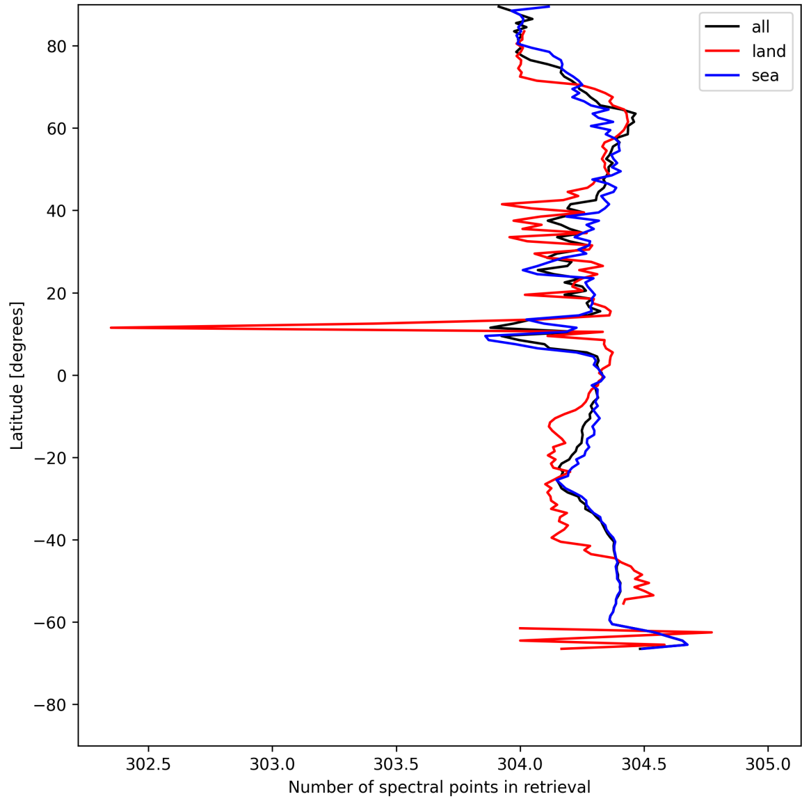
Figure 14: Zonal average of “Number of spectral points in retrieval” for 2025-07-15 to 2025-07-16.
