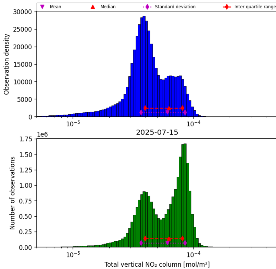
Figure 36: Histogram of "Total vertical NO 2 column" for 2025-07-15 to 2025-07-16
