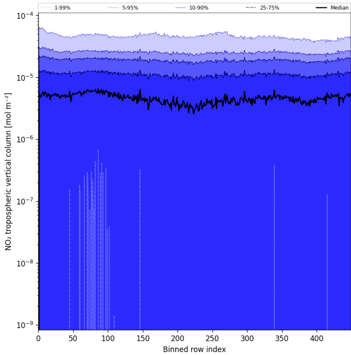
Figure 44: Along track statistics of "NO 2 tropospheric vertical column" for 2025-07-15 to 2025-07-16
