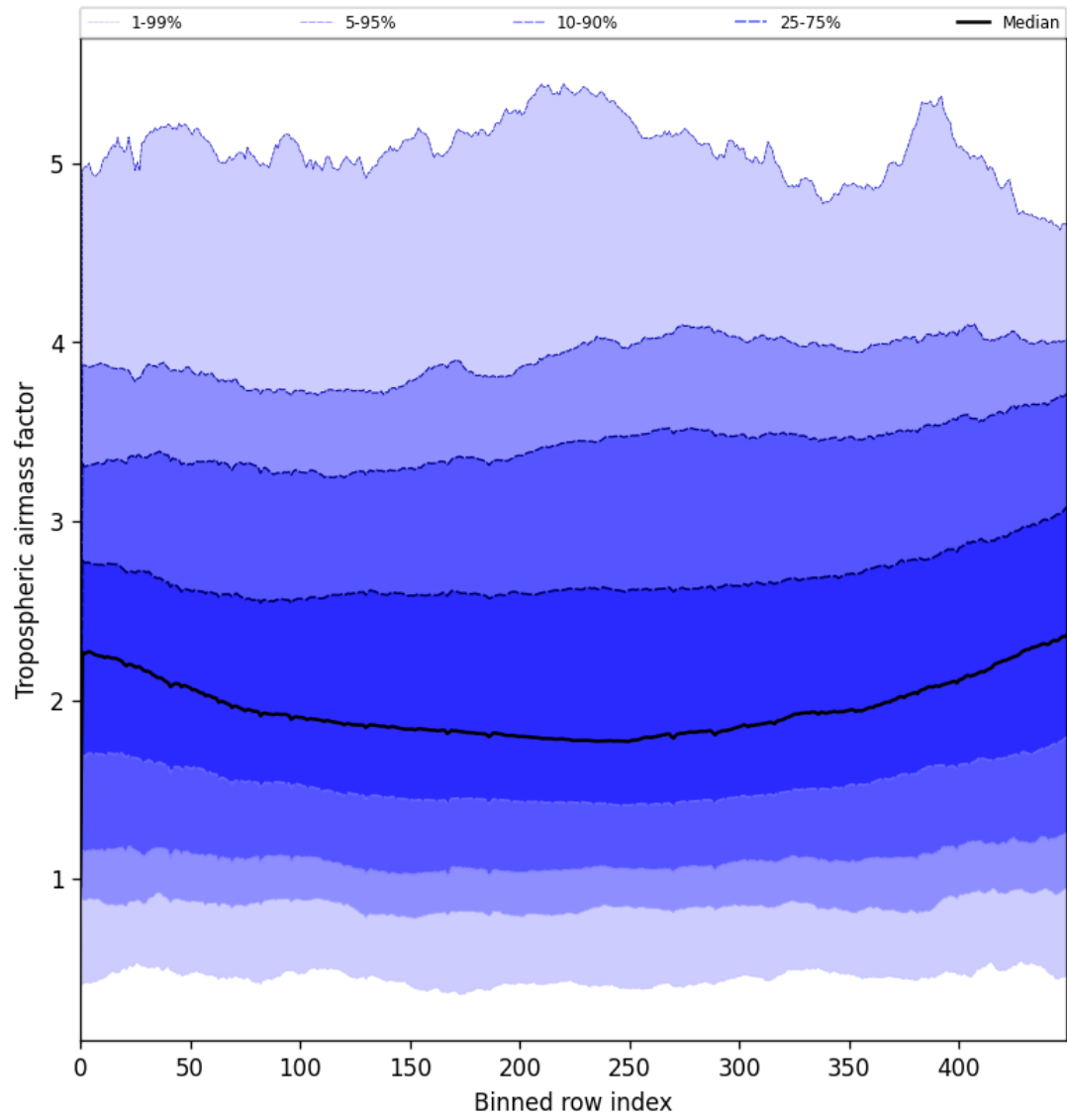
Figure 46: Along track statistics of “Tropospheric airmass factor” for 2025-07-15 to 2025-07-16
