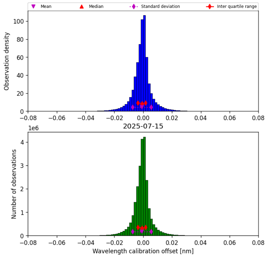
Figure 33: Histogram of “Wavelength calibration offset” for 2025-07-15 to 2025-07-16
