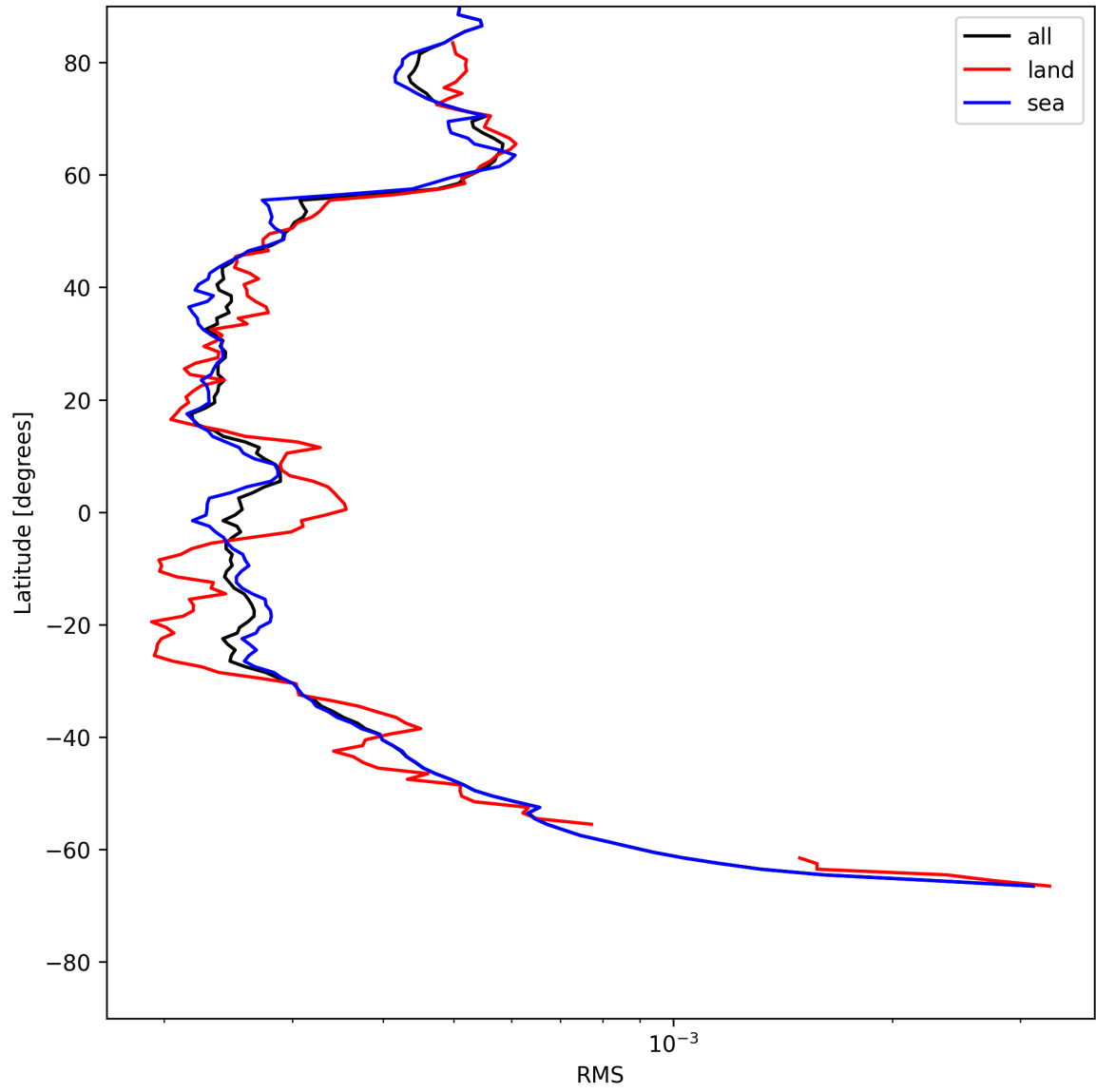
Figure 24: Zonal average of “RMS” for 2025-07-15 to 2025-07-16.
