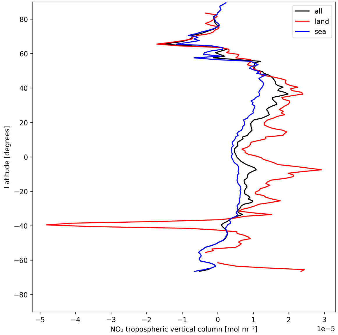
Figure 10: Zonal average of “NO 2 tropospheric vertical column” for 2025-07-15 to 2025-07-16.
