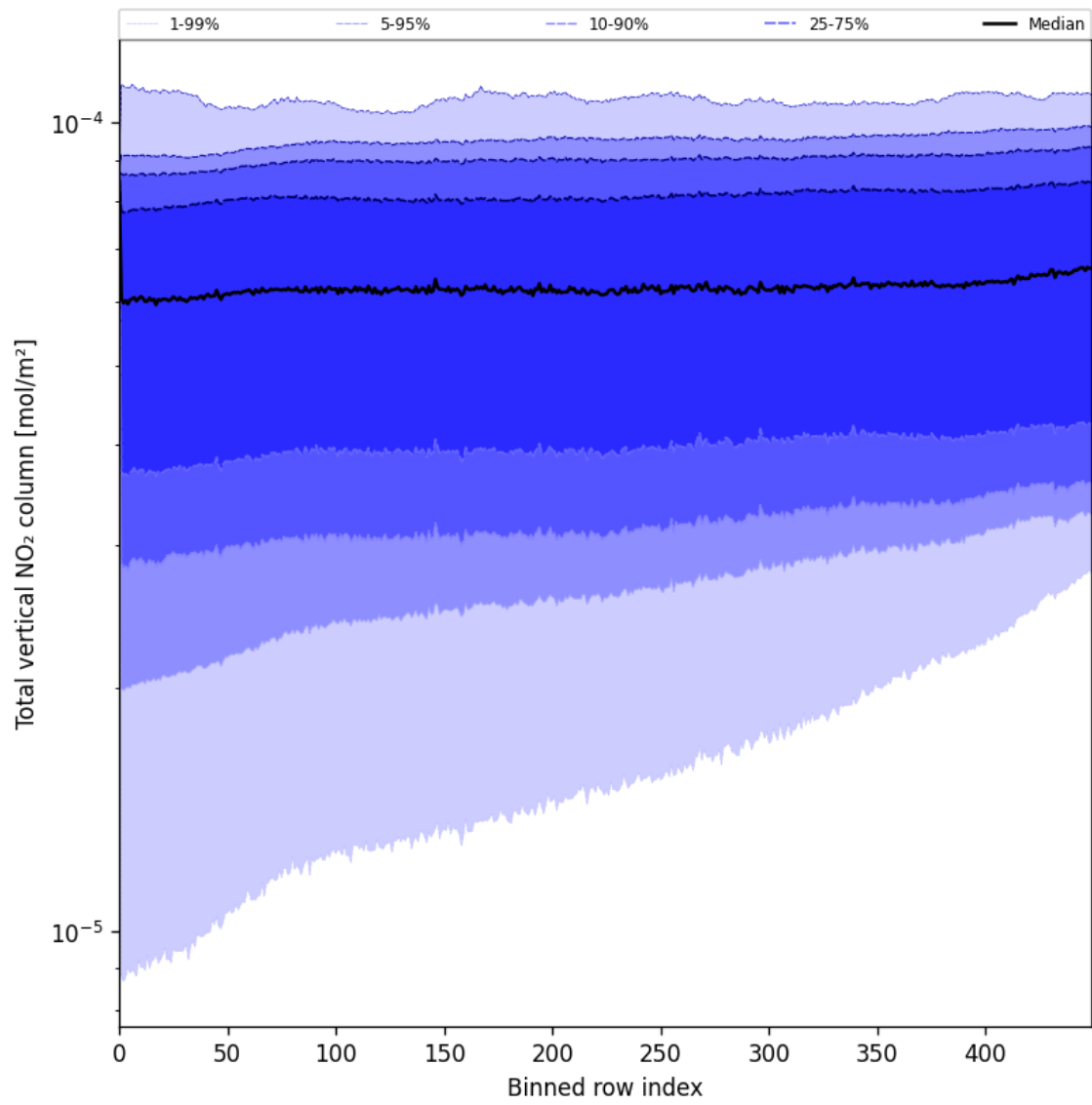
Figure 53: Along track statistics of “Total vertical NO 2 column” for 2025-07-15 to 2025-07-16
