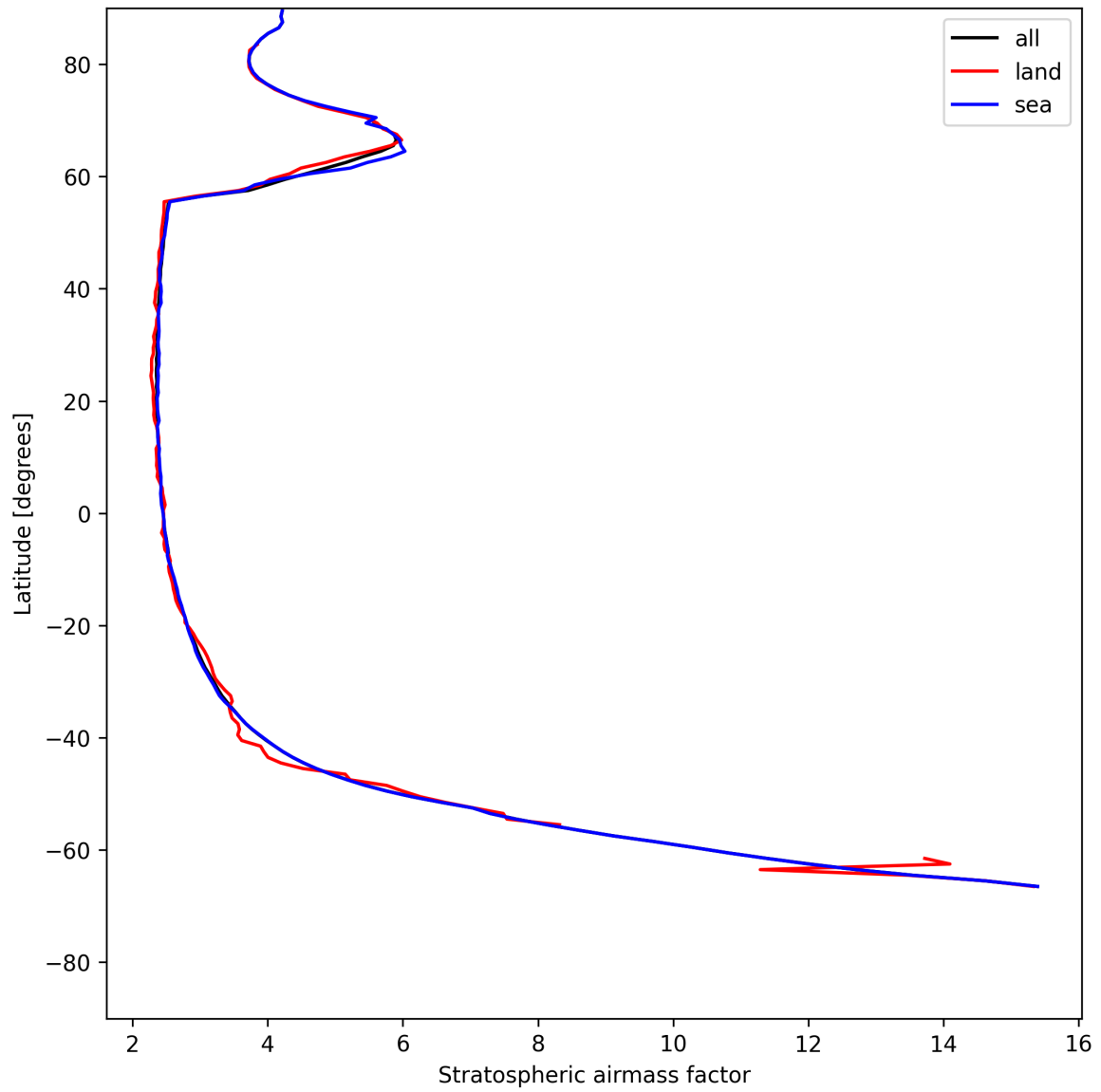
Figure 25: Zonal average of “Stratospheric airmass factor” for 2025-07-15 to 2025-07-16.
