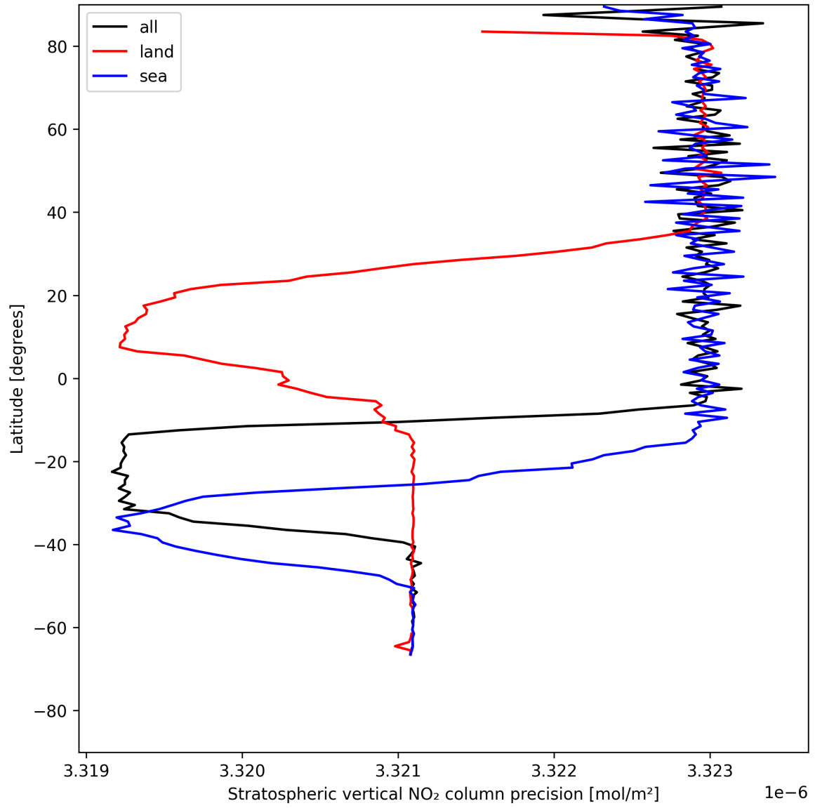
Figure 18: Zonal average of “Stratospheric vertical NO 2 column precision” for 2025-07-15 to 2025-07-16.
