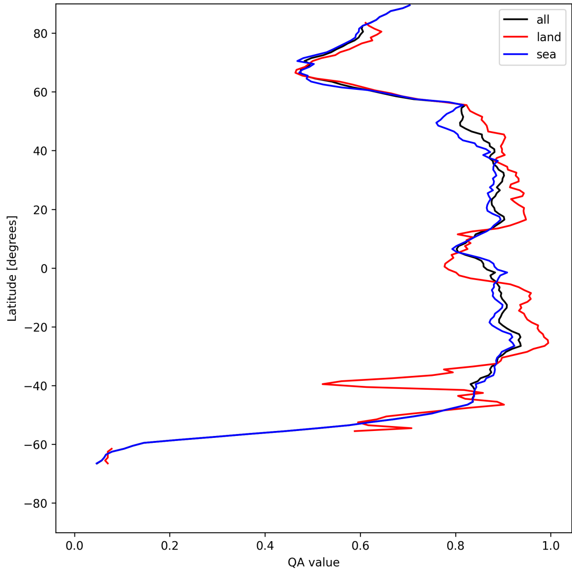
Figure 9: Zonal average of “QA value” for 2025-07-15 to 2025-07-16.
