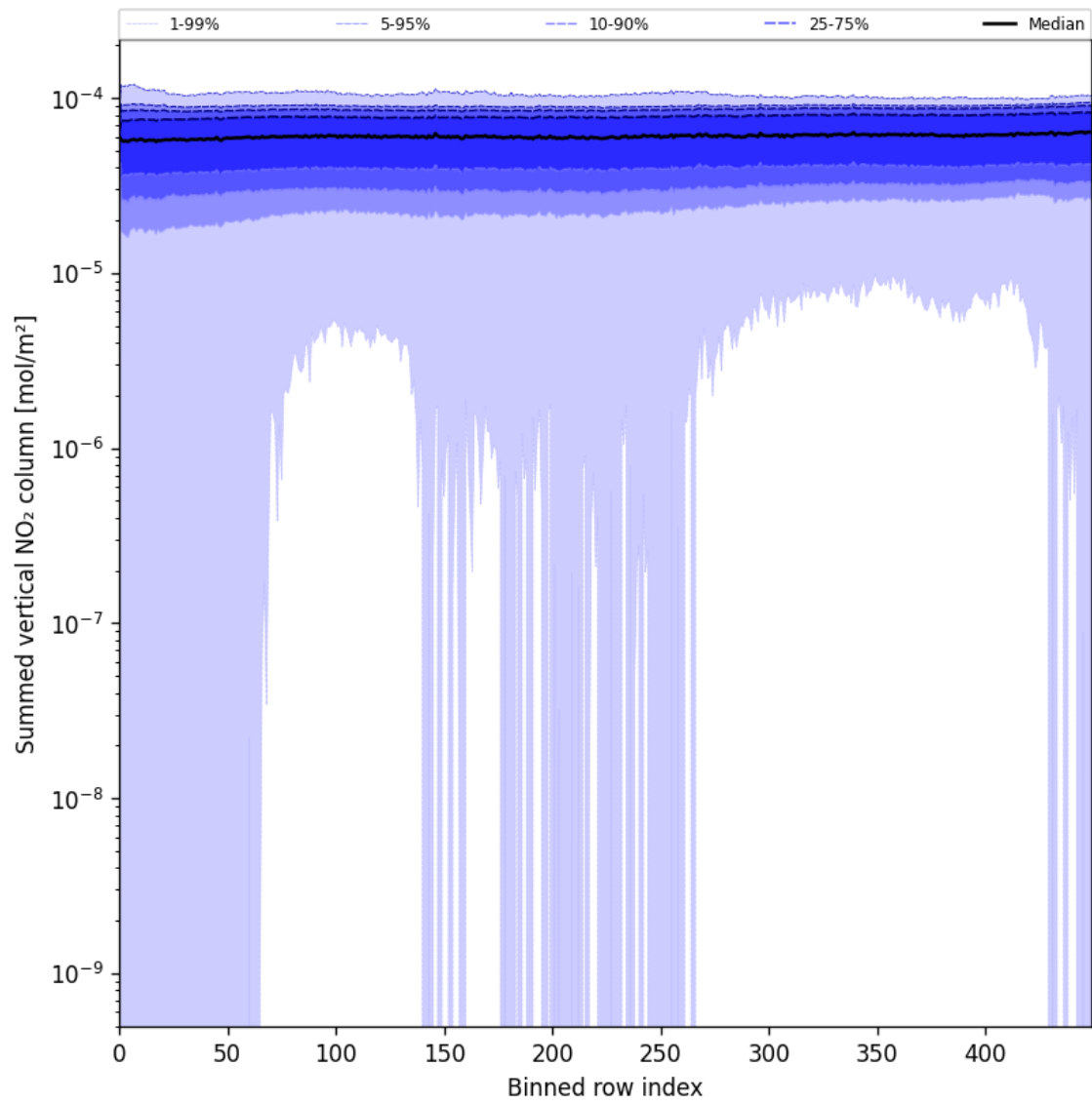
Figure 55: Along track statistics of “Summed vertical NO 2 column” for 2025-07-15 to 2025-07-16
