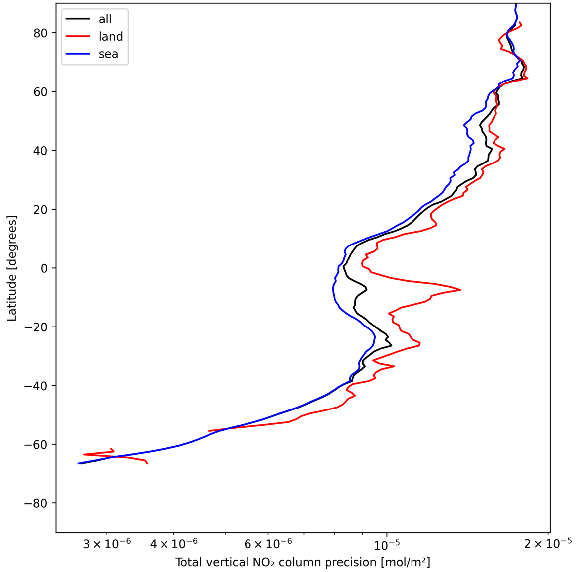
Figure 20: Zonal average of “Total vertical NO 2 column precision” for 2025-07-15 to 2025-07-16.
