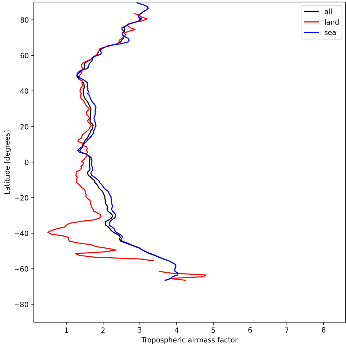
Figure 12: Zonal average of “Tropospheric airmass factor” for 2025-07-15 to 2025-07-16.
