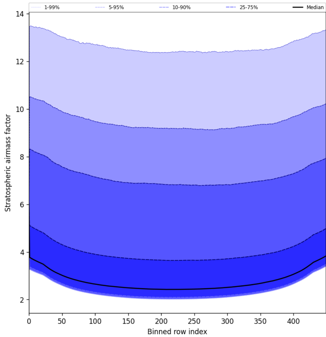
Figure 59: Along track statistics of “Stratospheric airmass factor” for 2025-07-15 to 2025-07-16
