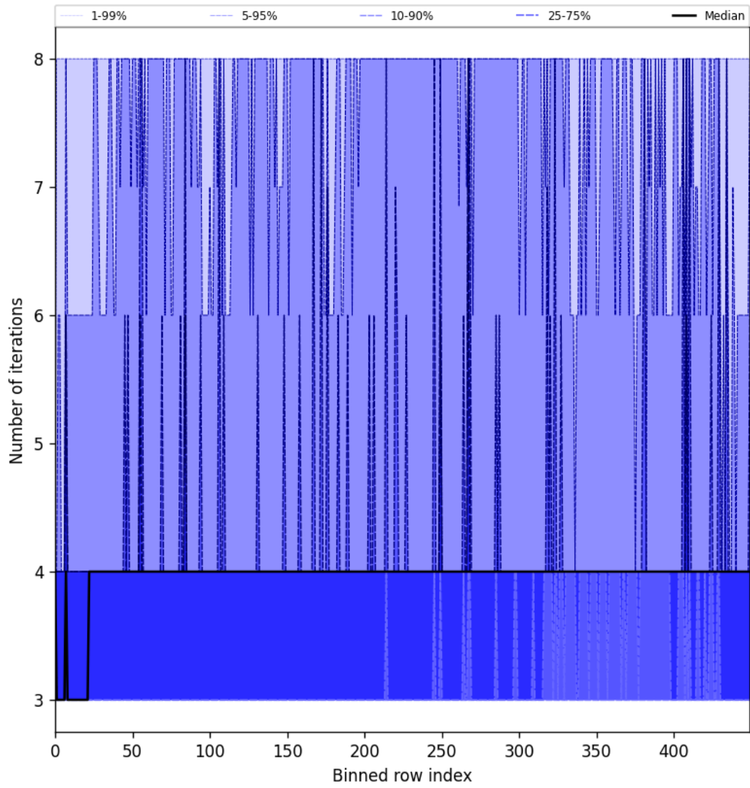
Figure 49: Along track statistics of “Number of iterations” for 2025-07-16 to 2025-07-16
