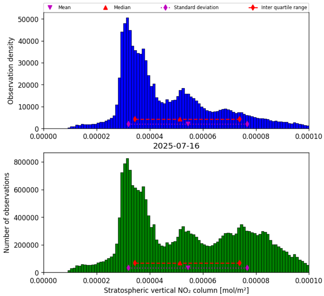
Figure 34: Histogram of “Stratospheric vertical NO 2 column” for 2025-07-16 to 2025-07-16
