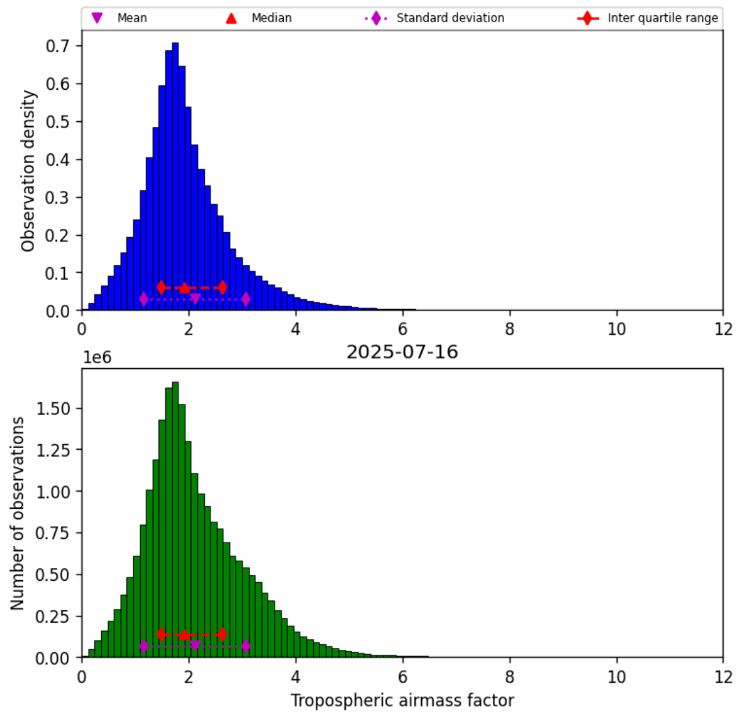
Figure 29: Histogram of “Tropospheric airmass factor” for 2025-07-16 to 2025-07-16
