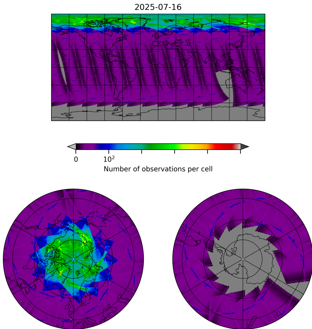
Figure 8: Map of the number of observations for 2025-07-16 to 2025-07-16
