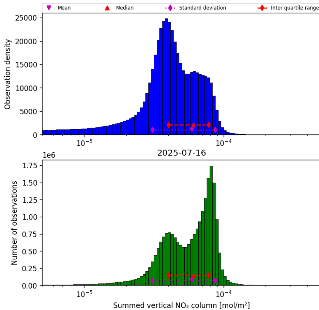
Figure 38: Histogram of “Summed vertical NO 2 column” for 2025-07-16 to 2025-07-16
