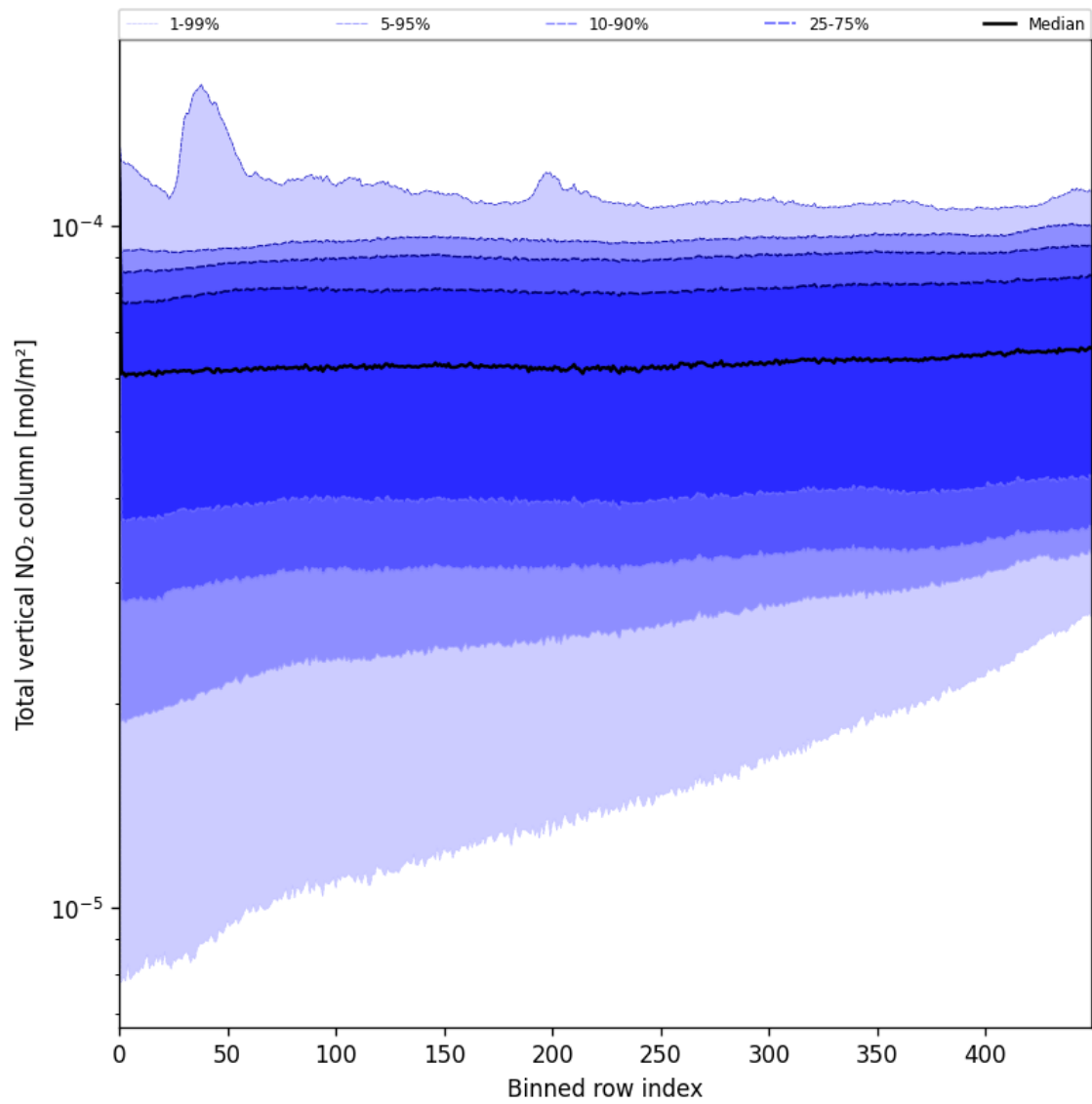
Figure 53: Along track statistics of “Total vertical NO 2 column” for 2025-07-16 to 2025-07-16
