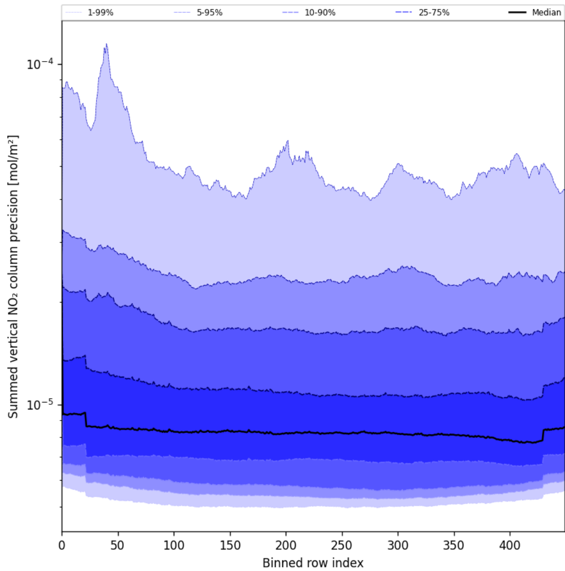
Figure 56: Along track statistics of “Summed vertical NO 2 column precision” for 2025-07-16 to 2025-07-16
