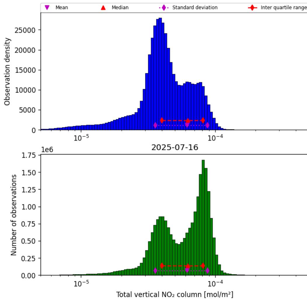
Figure 36: Histogram of “Total vertical NO 2 column” for 2025-07-16 to 2025-07-16
