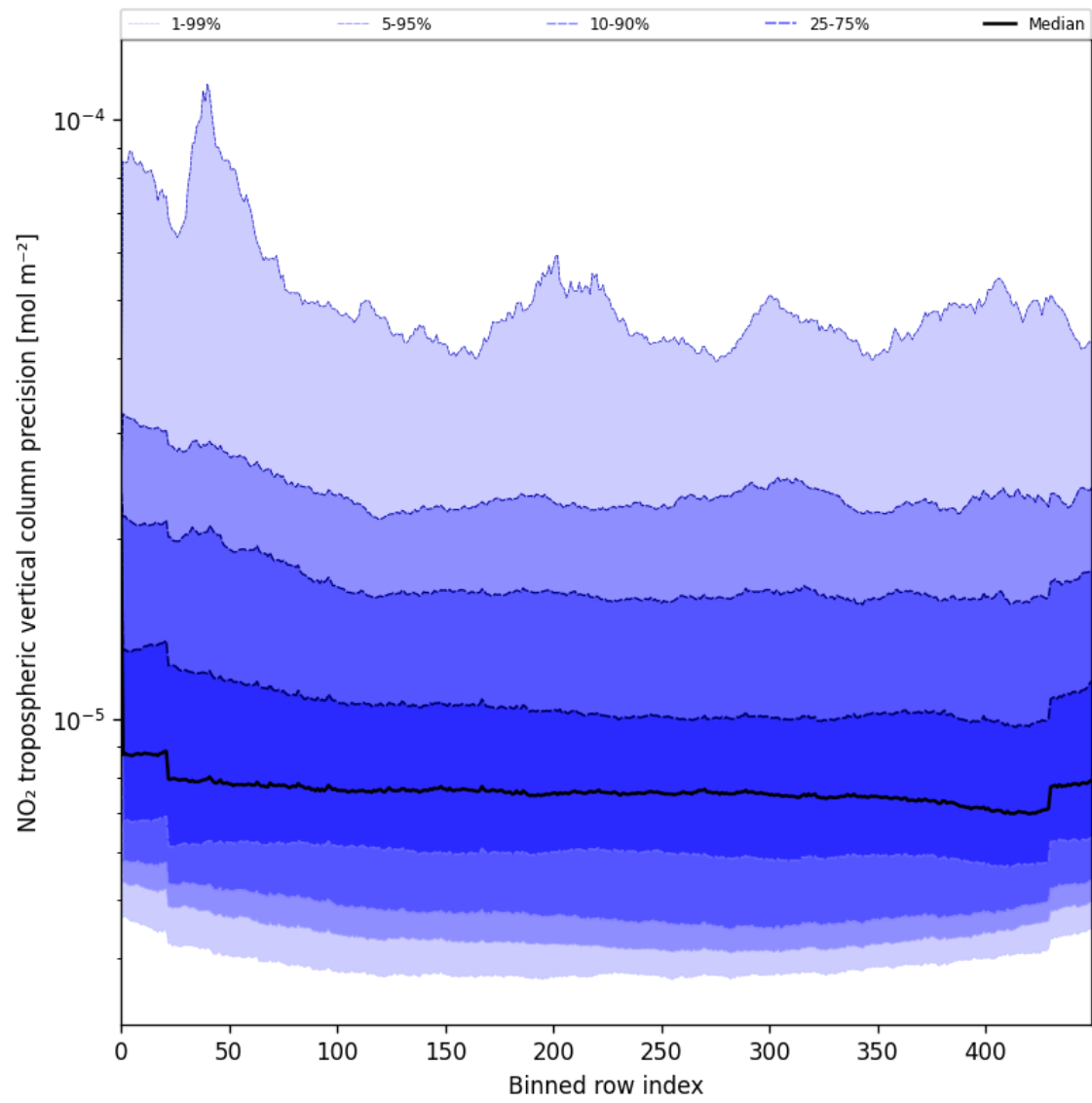
Figure 45: Along track statistics of “NO 2 tropospheric vertical column precision” for 2025-07-16 to 2025-07-16
