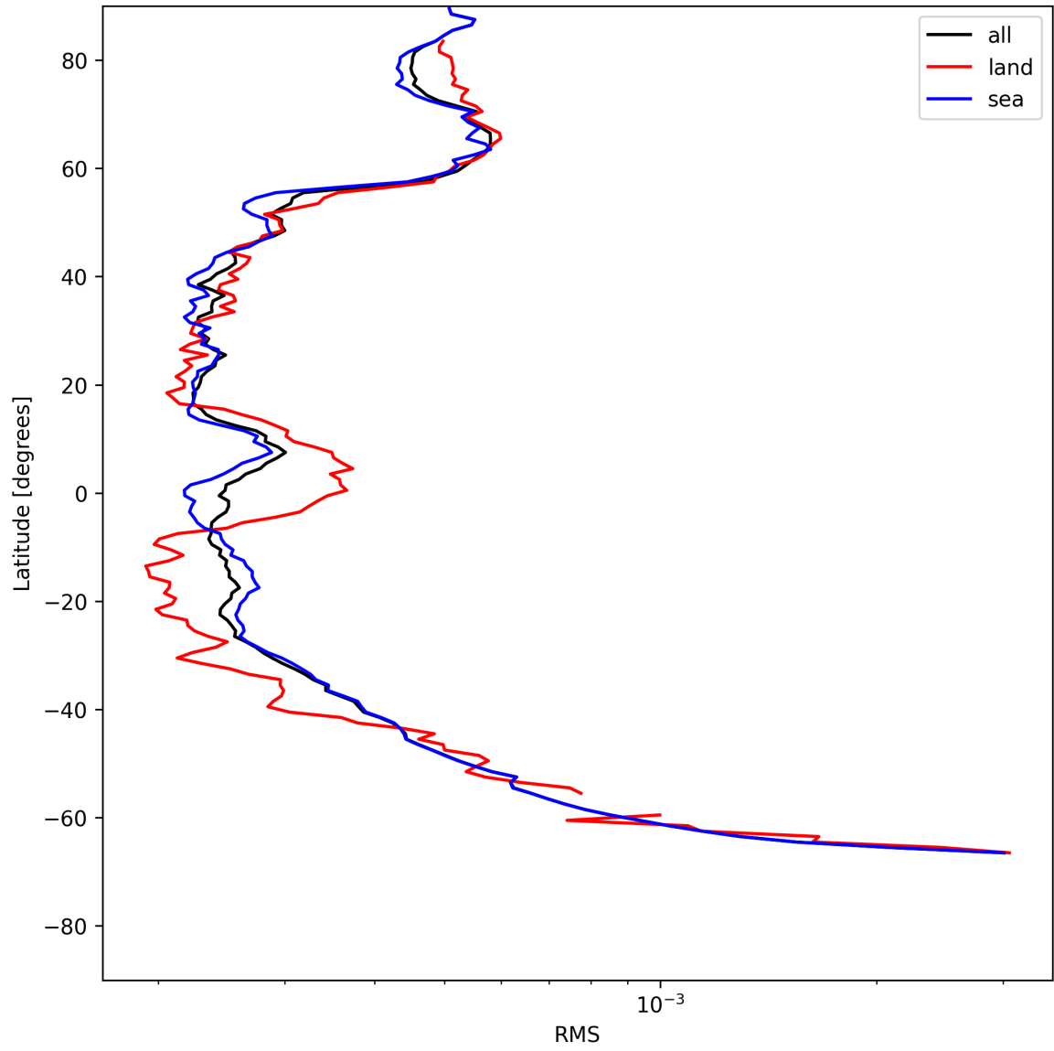
Figure 24: Zonal average of “RMS” for 2025-07-16 to 2025-07-16.
