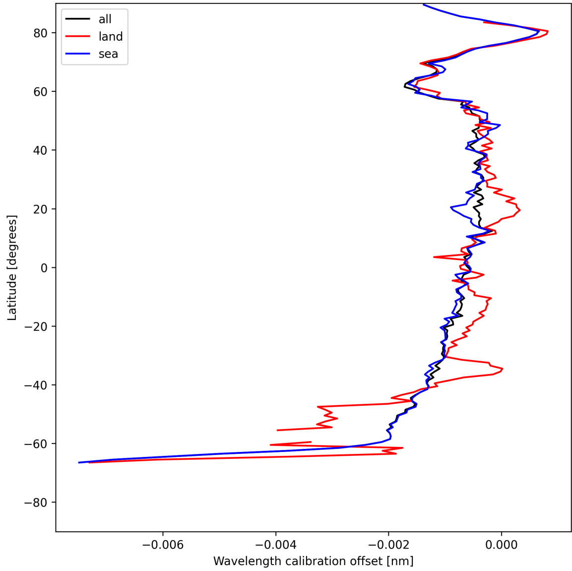
Figure 16: Zonal average of “Wavelength calibration offset” for 2025-07-16 to 2025-07-16.
