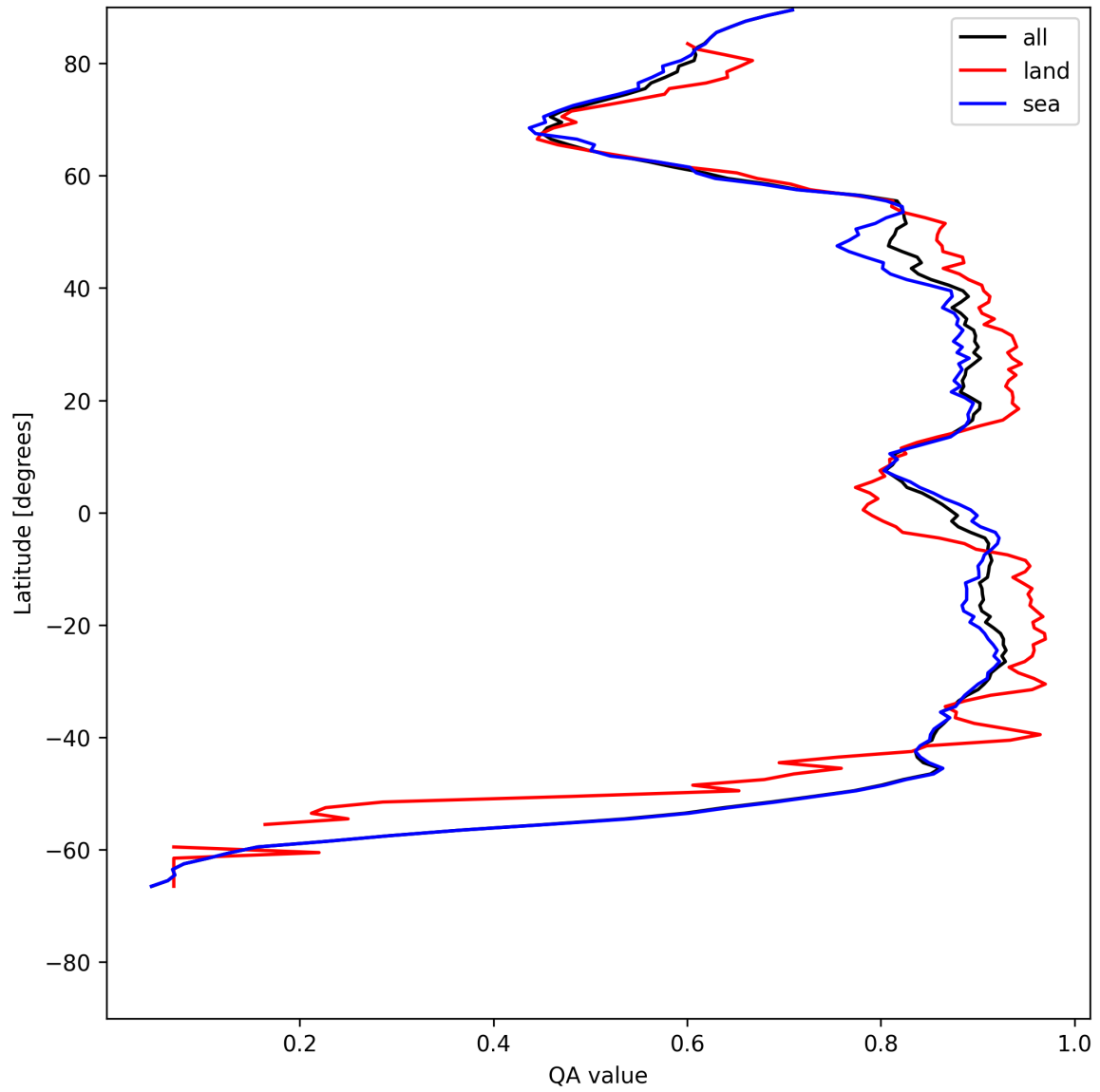
Figure 9: Zonal average of “QA value” for 2025-07-16 to 2025-07-16.
