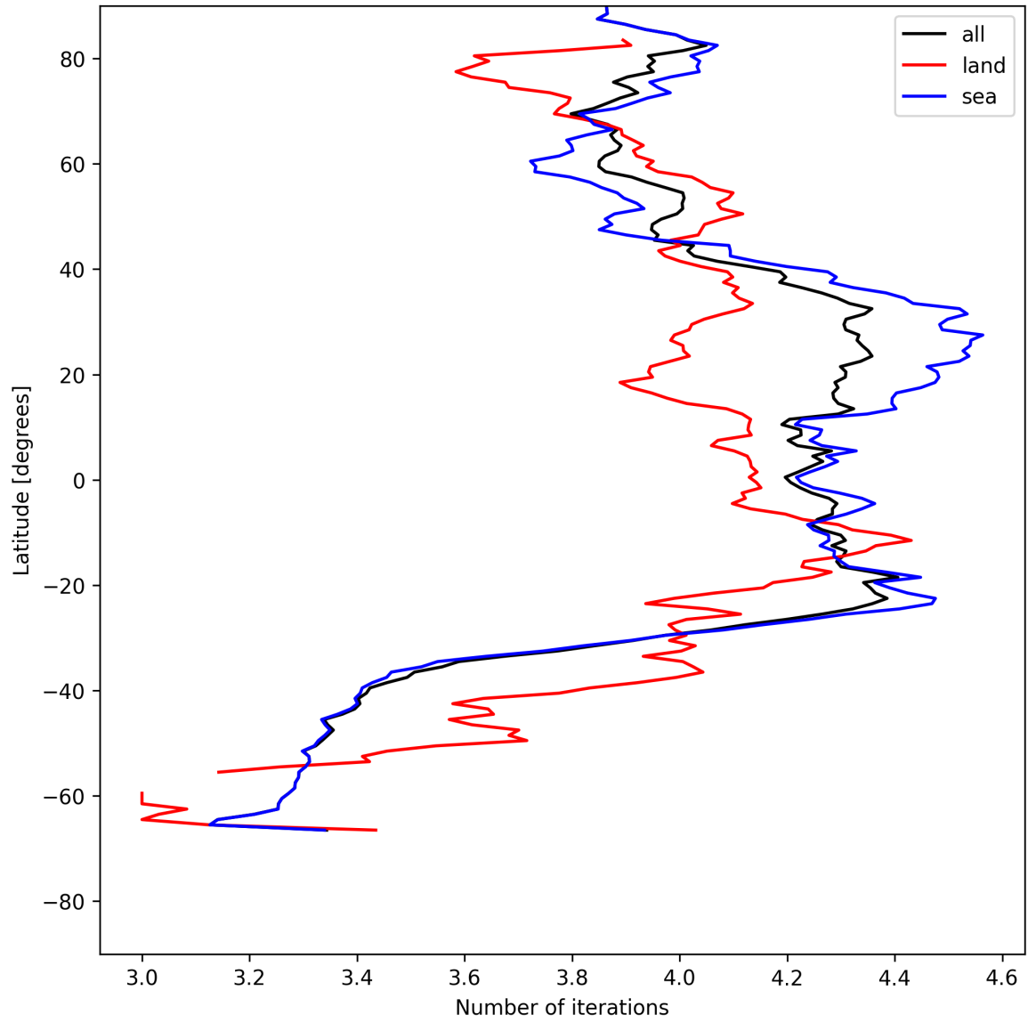
Figure 15: Zonal average of “Number of iterations” for 2025-07-16 to 2025-07-16.
