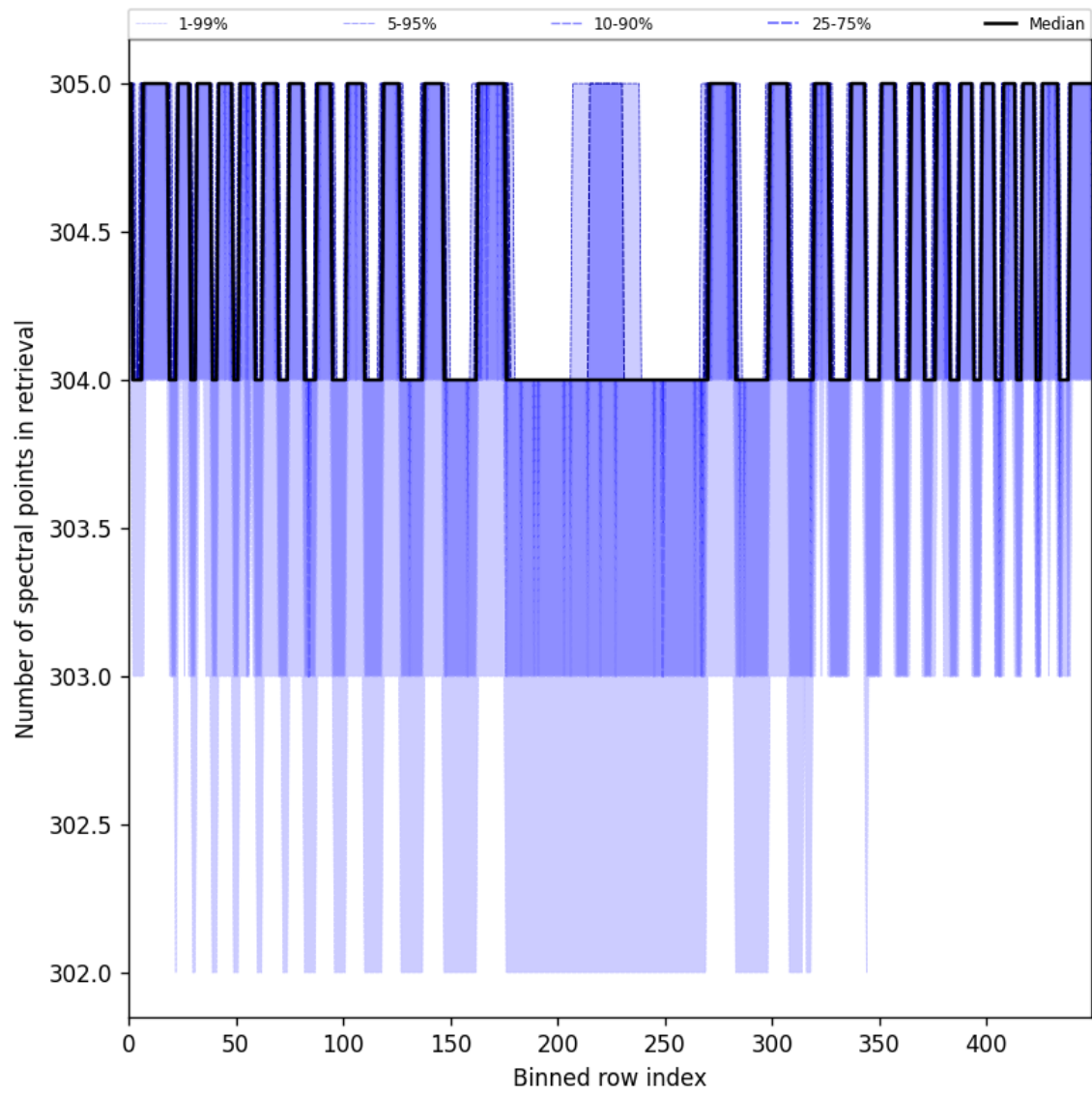
Figure 48: Along track statistics of “Number of spectral points in retrieval” for 2025-07-16 to 2025-07-16
