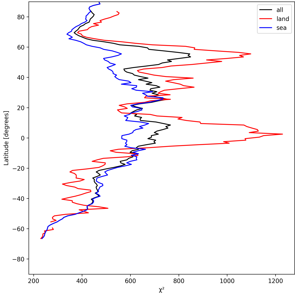
Figure 23: Zonal average of “ \chi^2 ” for 2025-07-16 to 2025-07-16.
