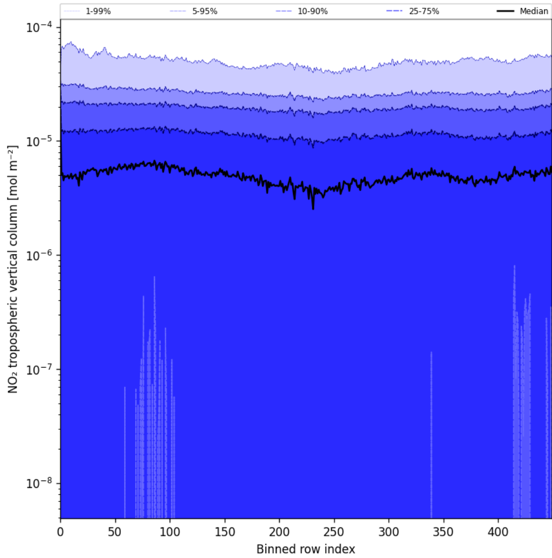
Figure 44: Along track statistics of “NO 2 tropospheric vertical column” for 2025-07-16 to 2025-07-16
