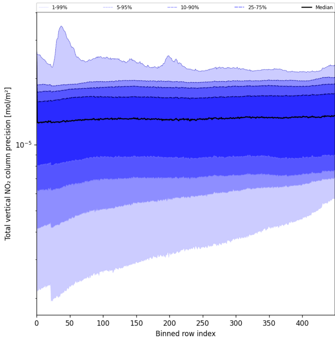
Figure 54: Along track statistics of “Total vertical NO 2 column precision” for 2025-07-16 to 2025-07-16
