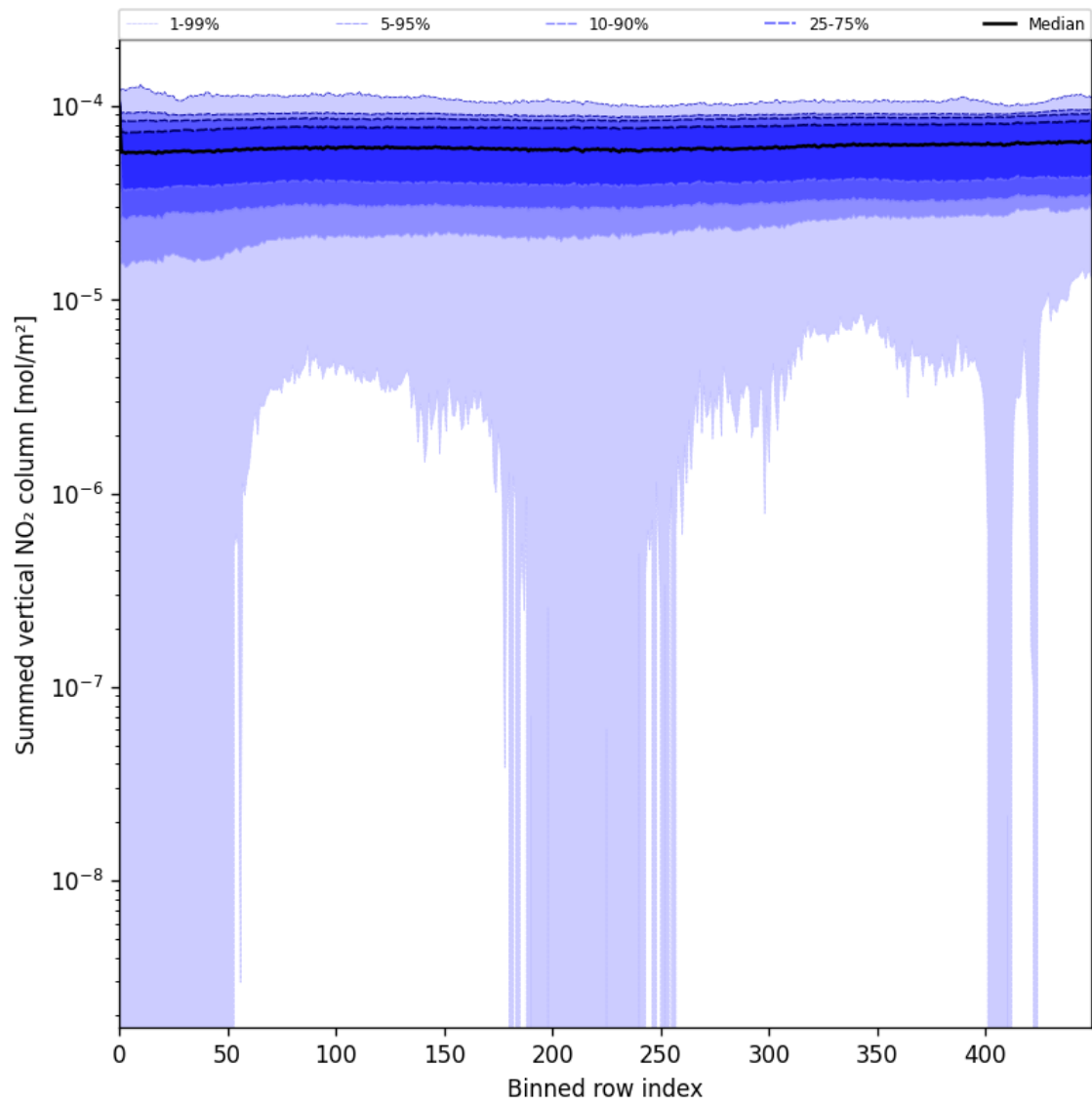
Figure 55: Along track statistics of “Summed vertical NO 2 column” for 2025-07-16 to 2025-07-16
