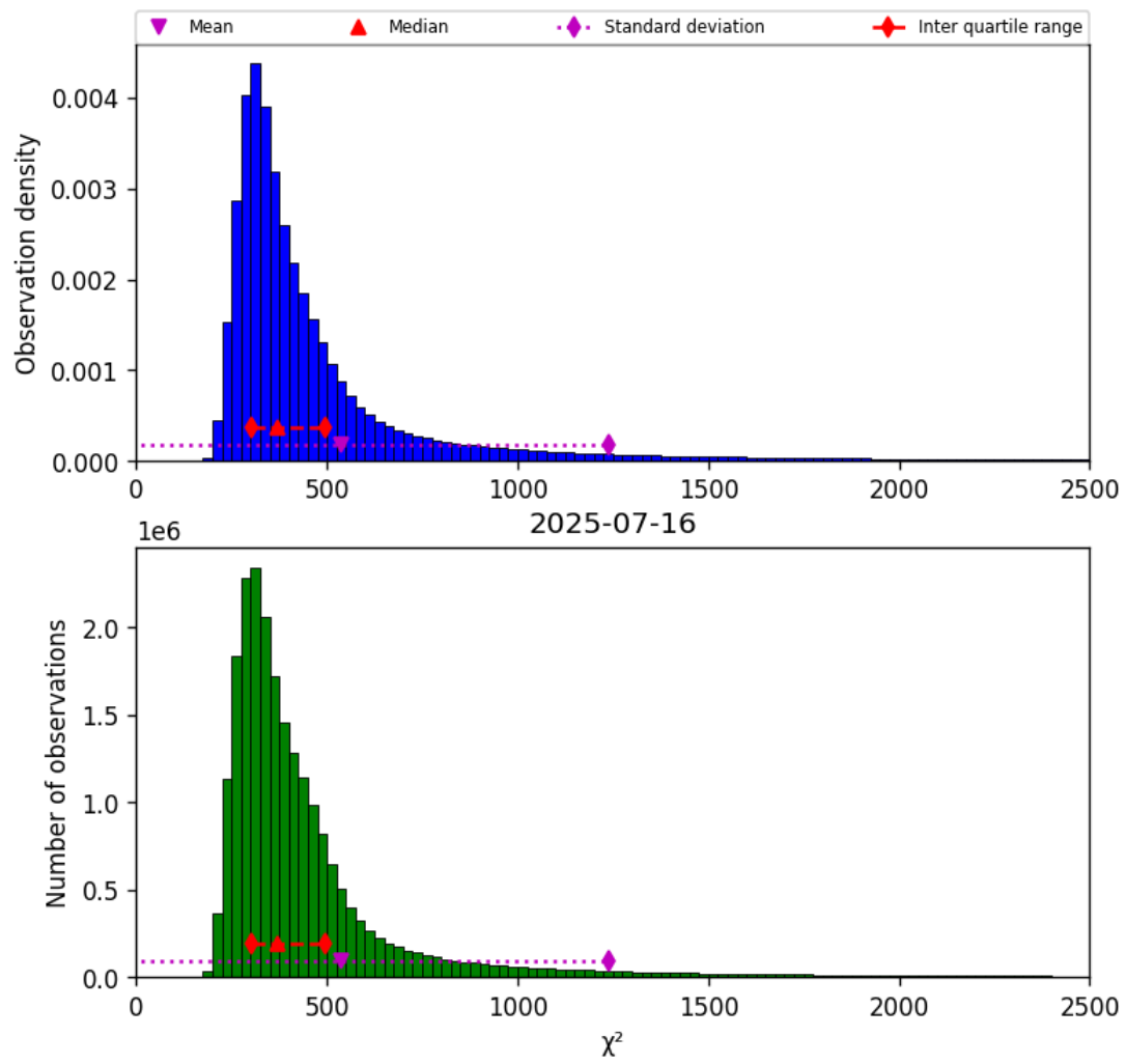
Figure 40: Histogram of “ \chi^2 ” for 2025-07-16 to 2025-07-16
