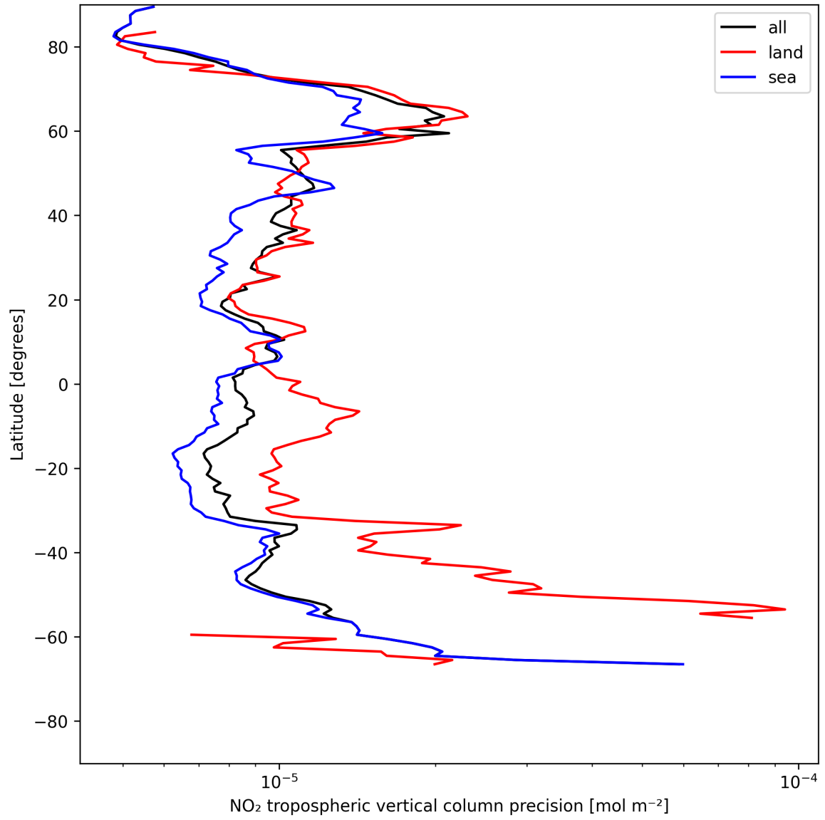
Figure 11: Zonal average of “NO 2 tropospheric vertical column precision” for 2025-07-16 to 2025-07-16.
