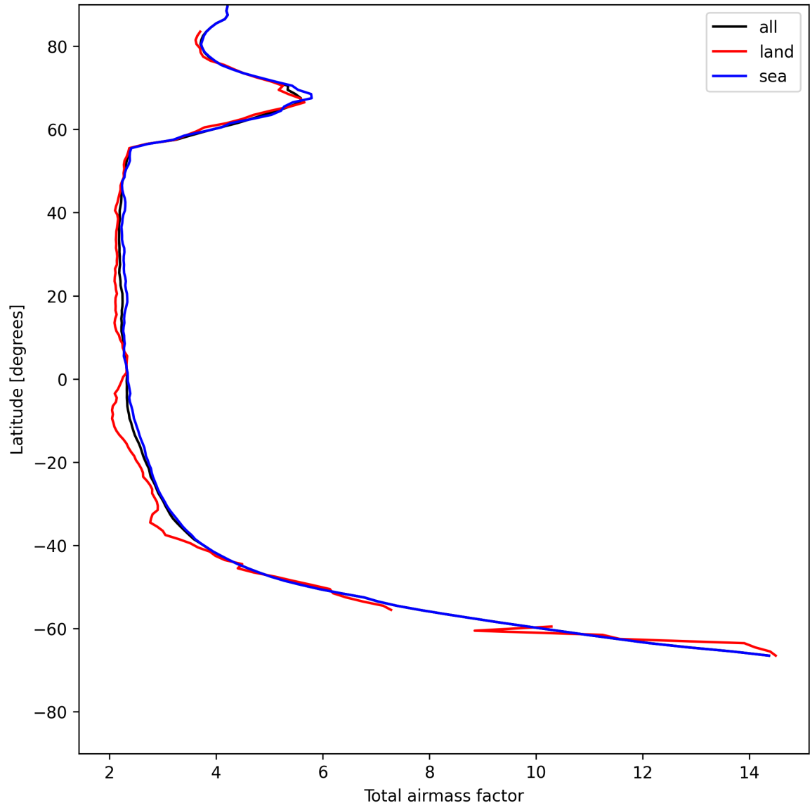
Figure 13: Zonal average of “Total airmass factor” for 2025-07-16 to 2025-07-16.
