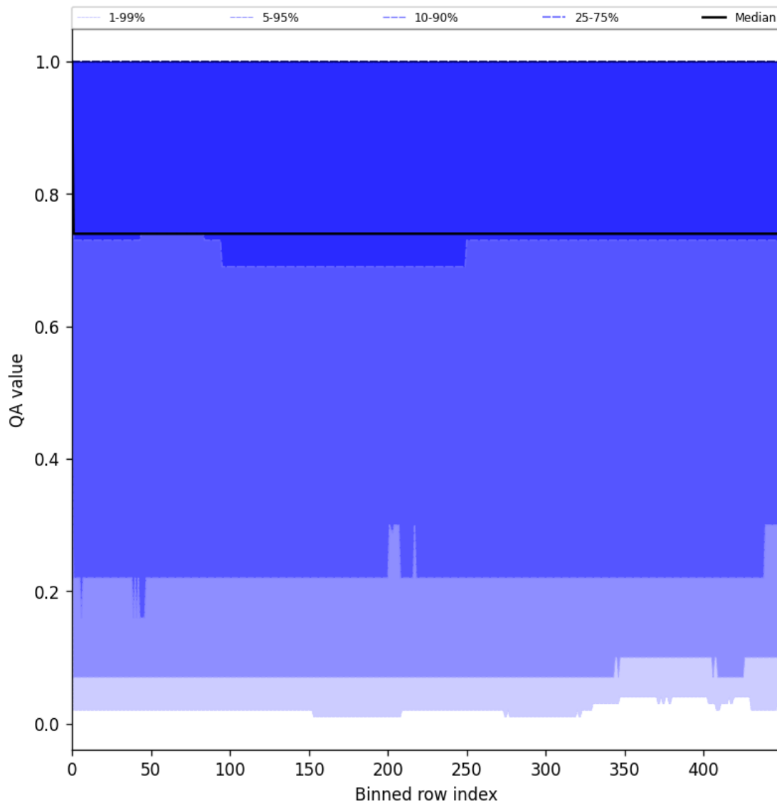
Figure 43: Along track statistics of “QA value” for 2025-07-16 to 2025-07-16
