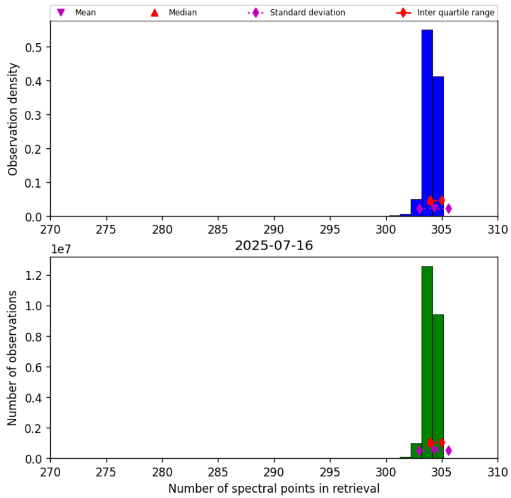
Figure 31: Histogram of “Number of spectral points in retrieval” for 2025-07-16 to 2025-07-16
