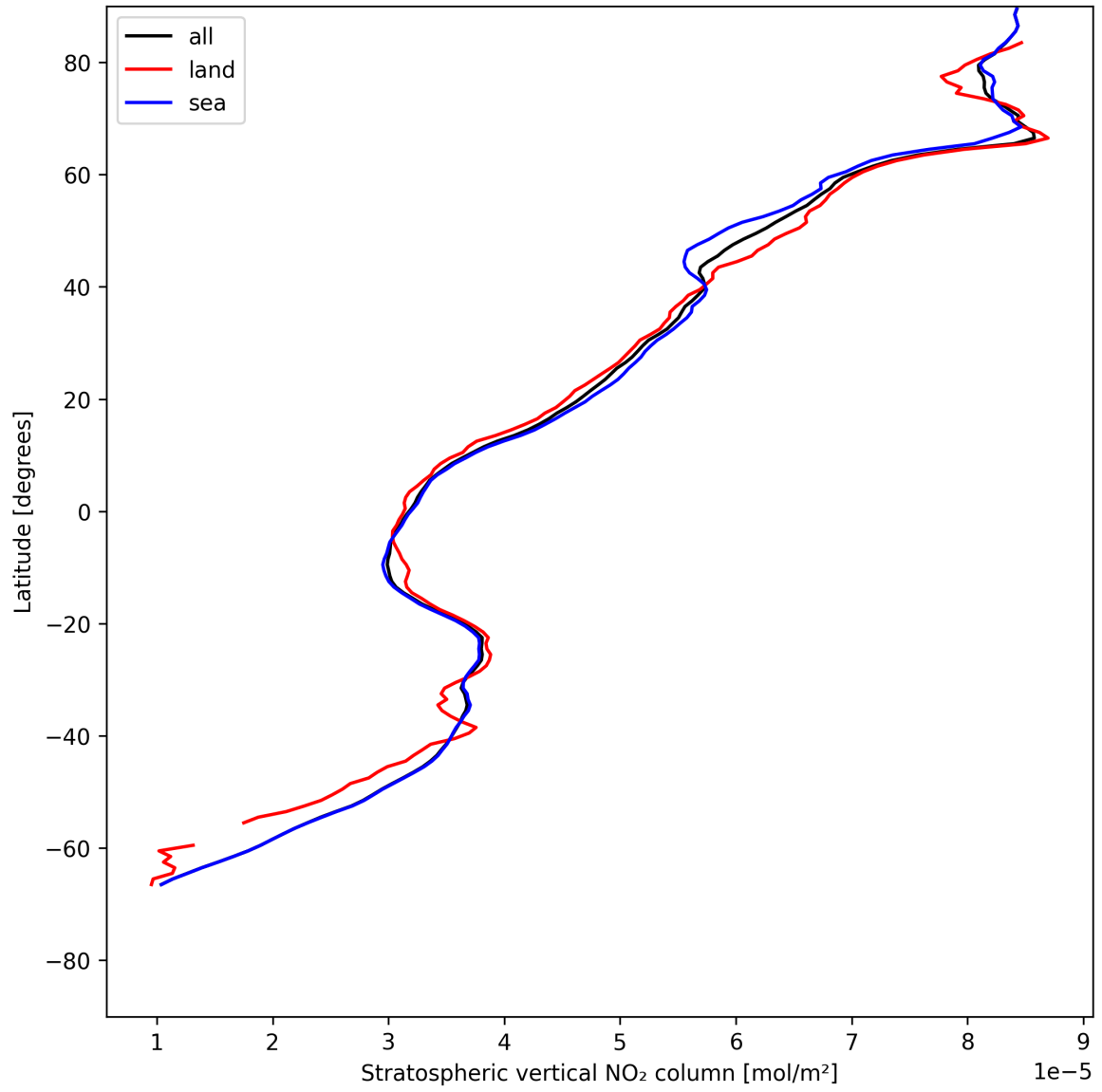
Figure 17: Zonal average of “Stratospheric vertical NO 2 column” for 2025-07-16 to 2025-07-16.
