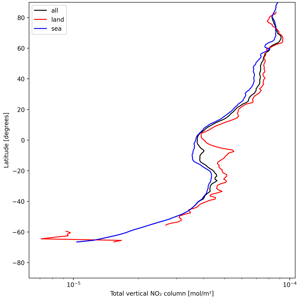
Figure 19: Zonal average of “Total vertical NO 2 column” for 2025-07-16 to 2025-07-16.
