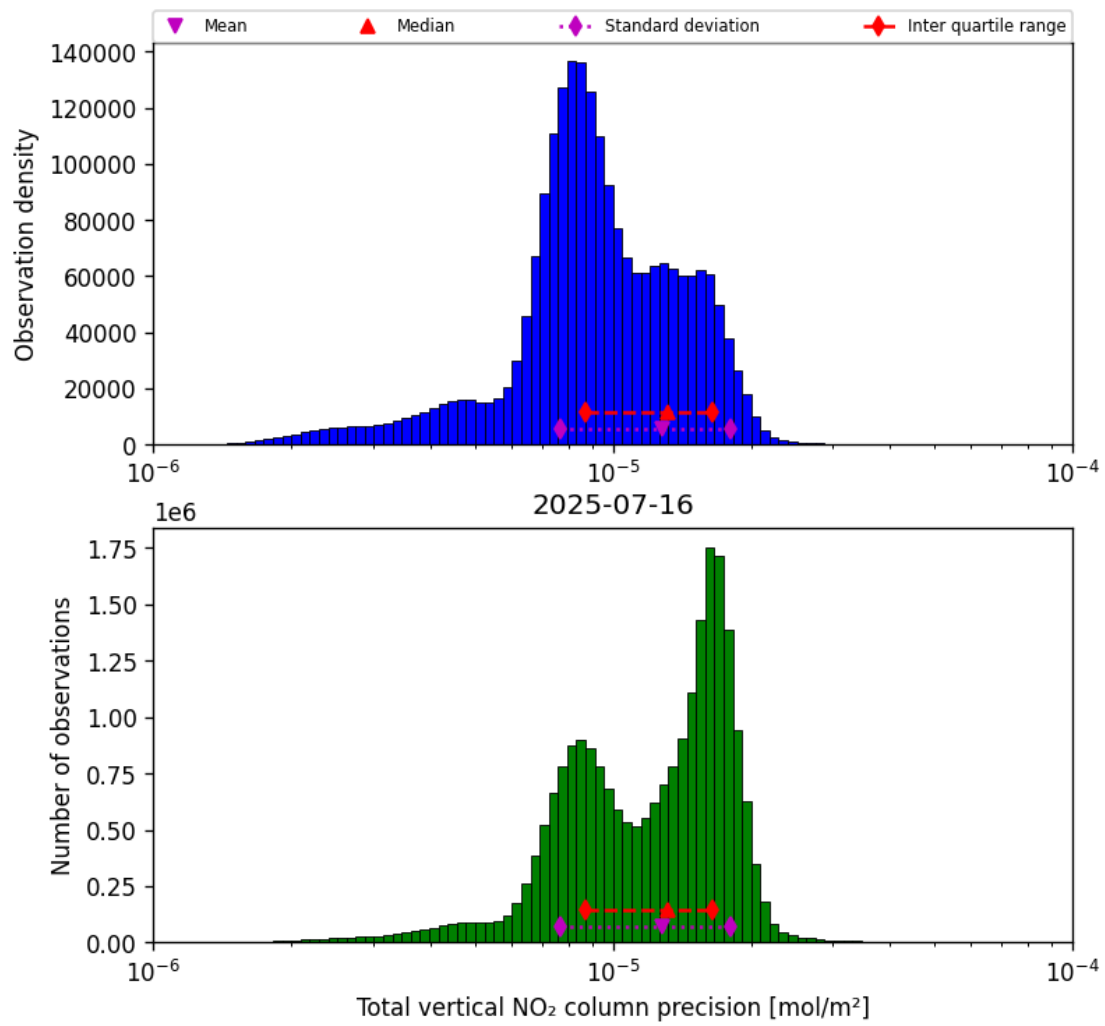
Figure 37: Histogram of “Total vertical NO 2 column precision” for 2025-07-16 to 2025-07-16
