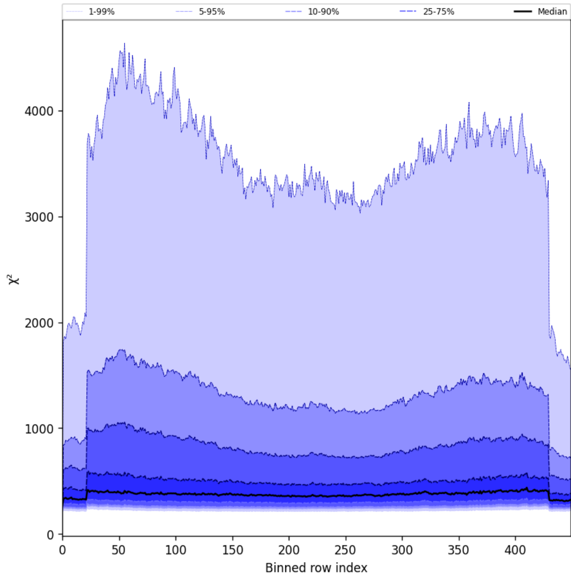
Figure 57: Along track statistics of “ \chi^2 ” for 2025-07-16 to 2025-07-16
