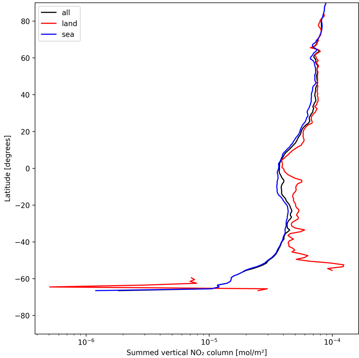
Figure 21: Zonal average of “Summed vertical NO 2 column” for 2025-07-16 to 2025-07-16.
