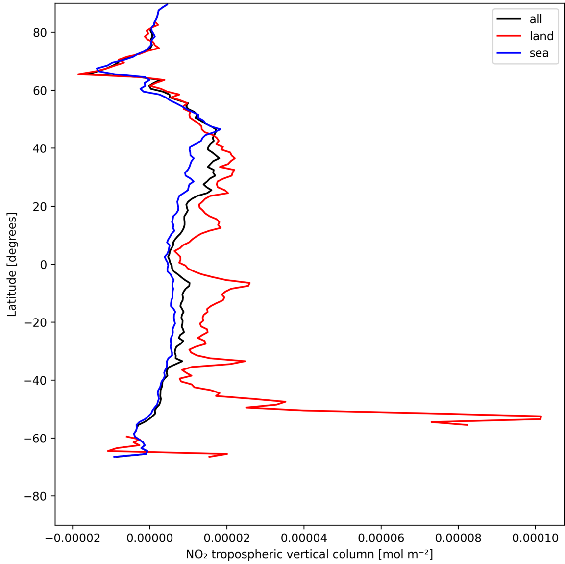
Figure 10: Zonal average of “NO 2 tropospheric vertical column” for 2025-07-16 to 2025-07-16.
