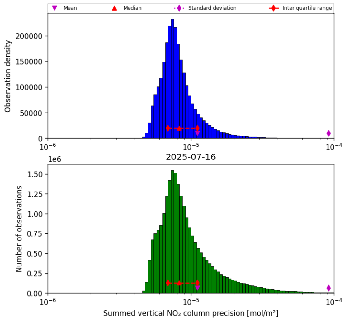
Figure 39: Histogram of "Summed vertical NO 2 column precision" for 2025-07-16 to 2025-07-16
