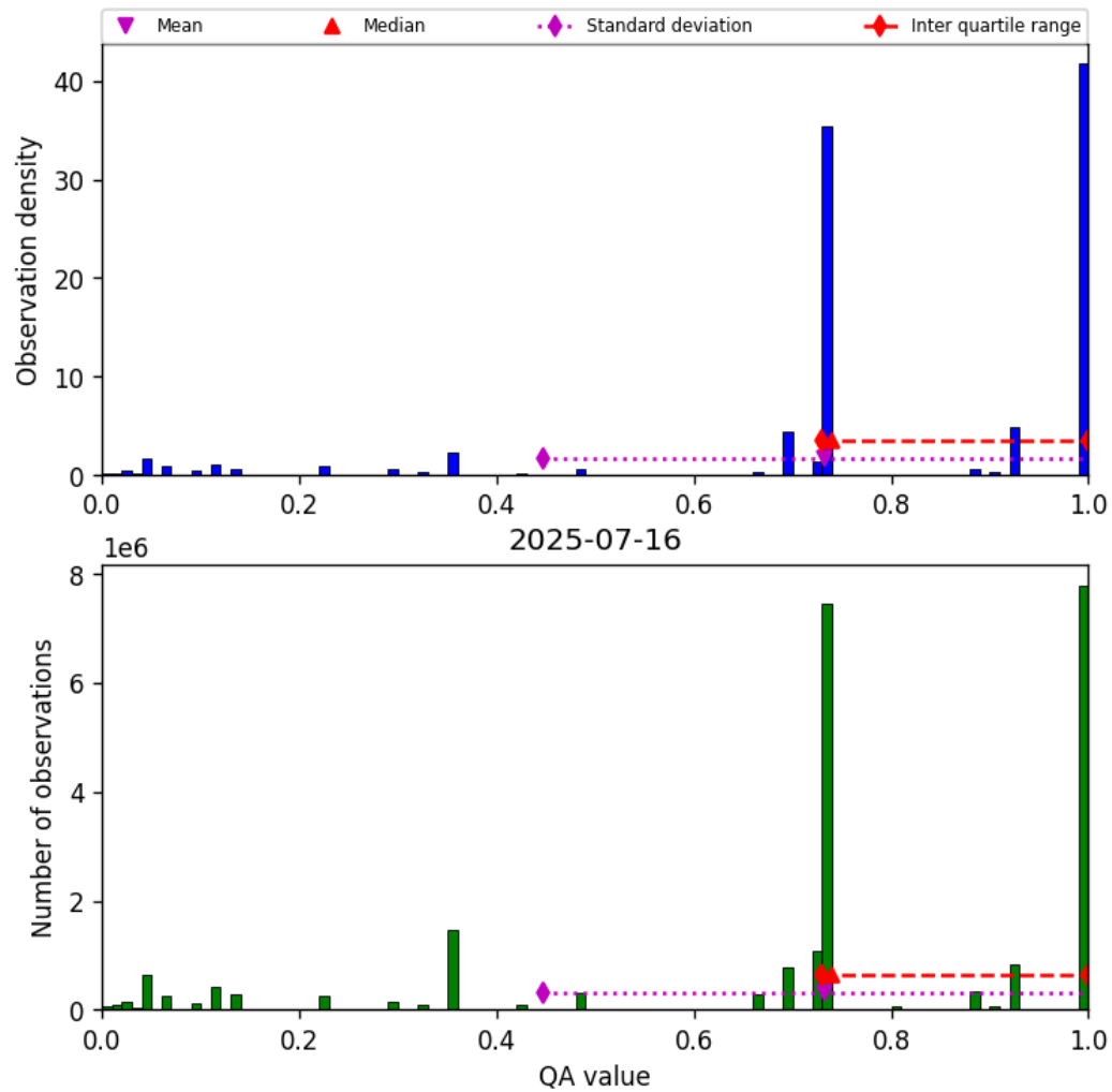
Figure 26: Histogram of “QA value” for 2025-07-16 to 2025-07-16
