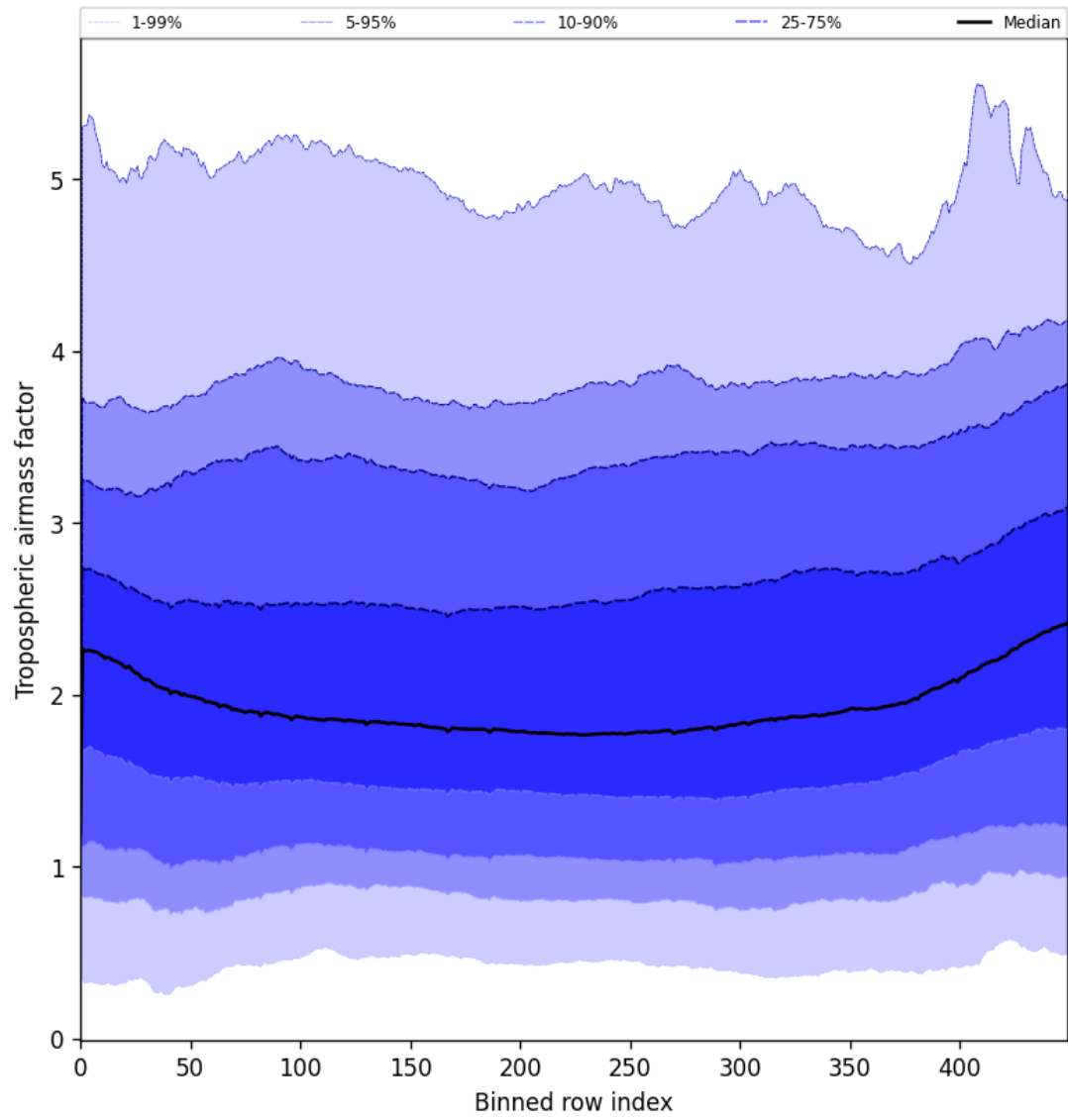
Figure 46: Along track statistics of “Tropospheric airmass factor” for 2025-07-16 to 2025-07-16
