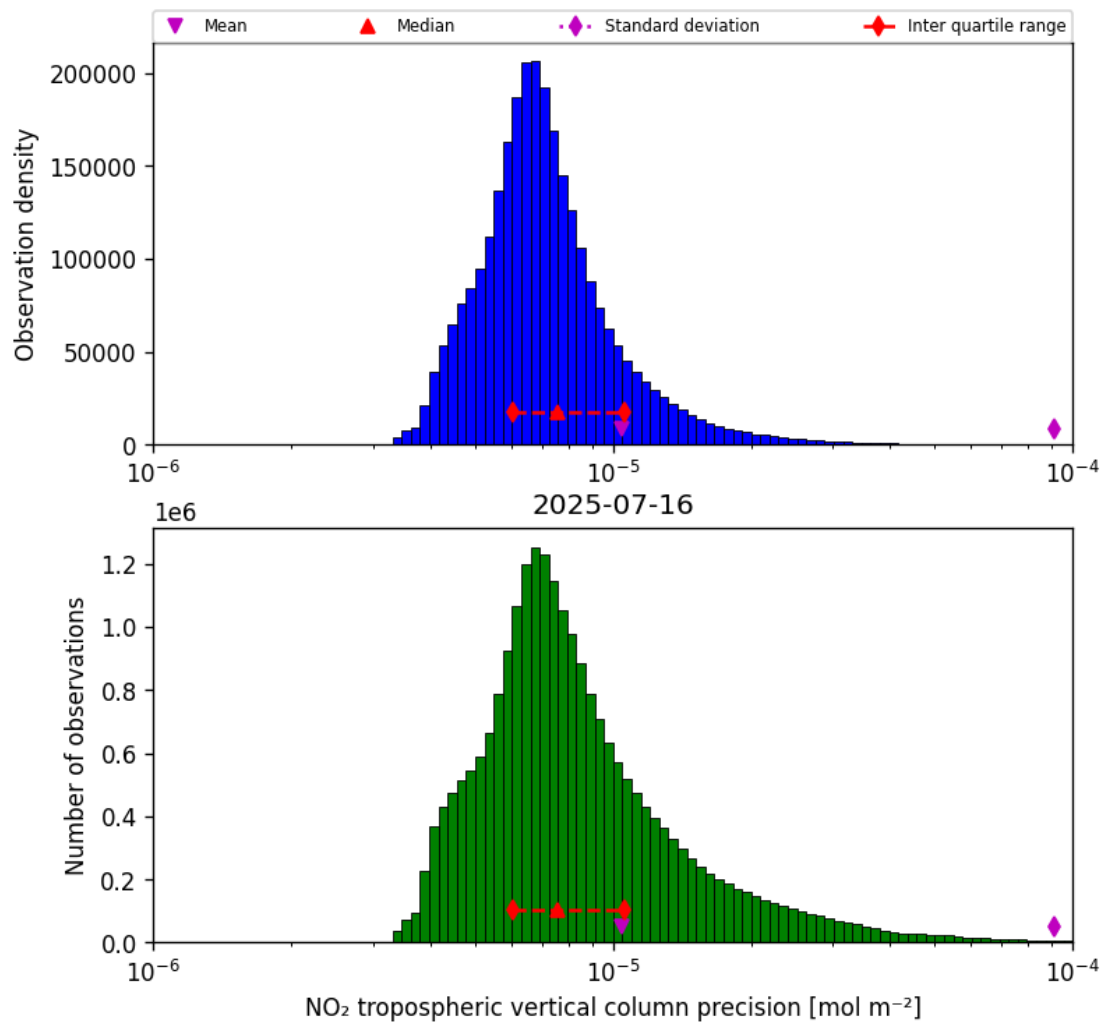
Figure 28: Histogram of "NO 2 tropospheric vertical column precision" for 2025-07-16 to 2025-07-16
