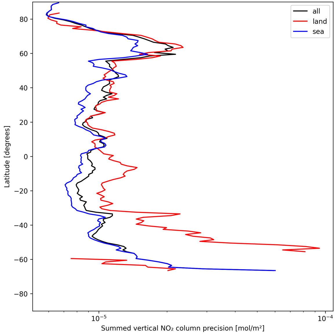
Figure 22: Zonal average of “Summed vertical NO 2 column precision” for 2025-07-16 to 2025-07-16.
