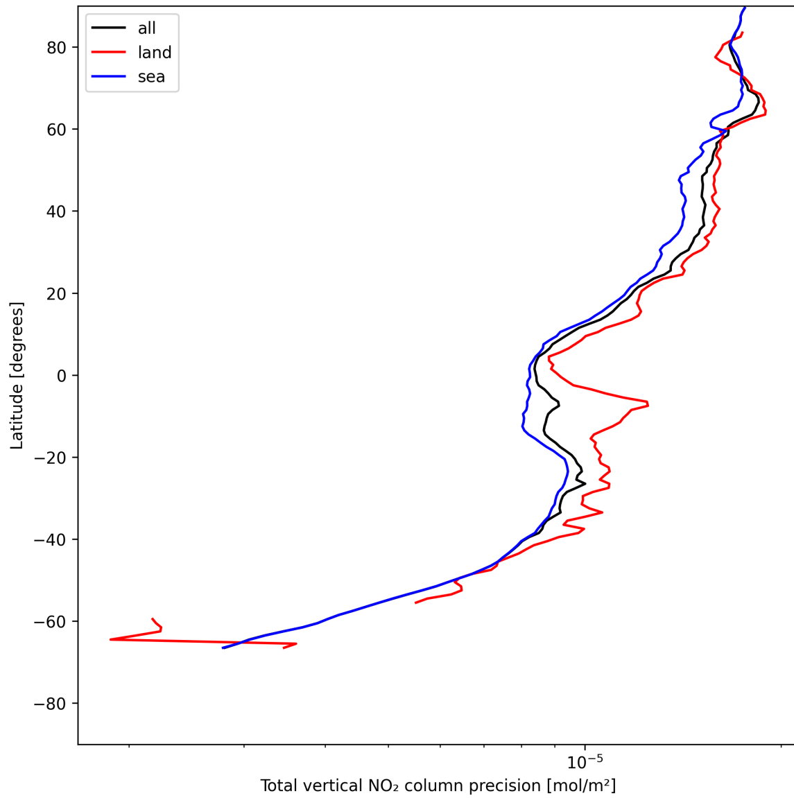
Figure 20: Zonal average of “Total vertical NO 2 column precision” for 2025-07-16 to 2025-07-16.
