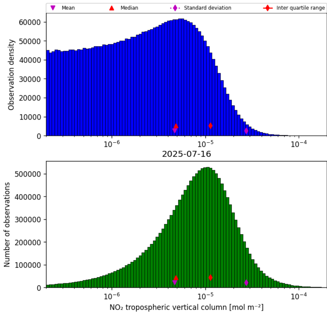
Figure 27: Histogram of “NO 2 tropospheric vertical column” for 2025-07-16 to 2025-07-16
