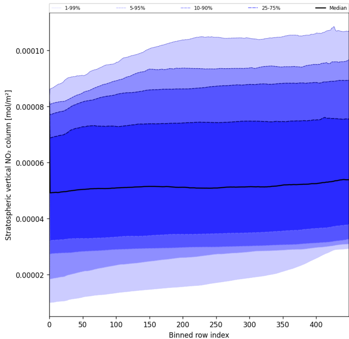
Figure 51: Along track statistics of “Stratospheric vertical NO 2 column” for 2025-07-16 to 2025-07-16
