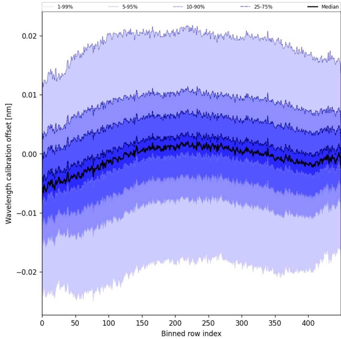
Figure 50: Along track statistics of “Wavelength calibration offset” for 2025-07-16 to 2025-07-16
