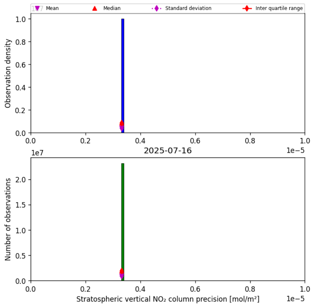
Figure 35: Histogram of “Stratospheric vertical NO 2 column precision” for 2025-07-16 to 2025-07-16
