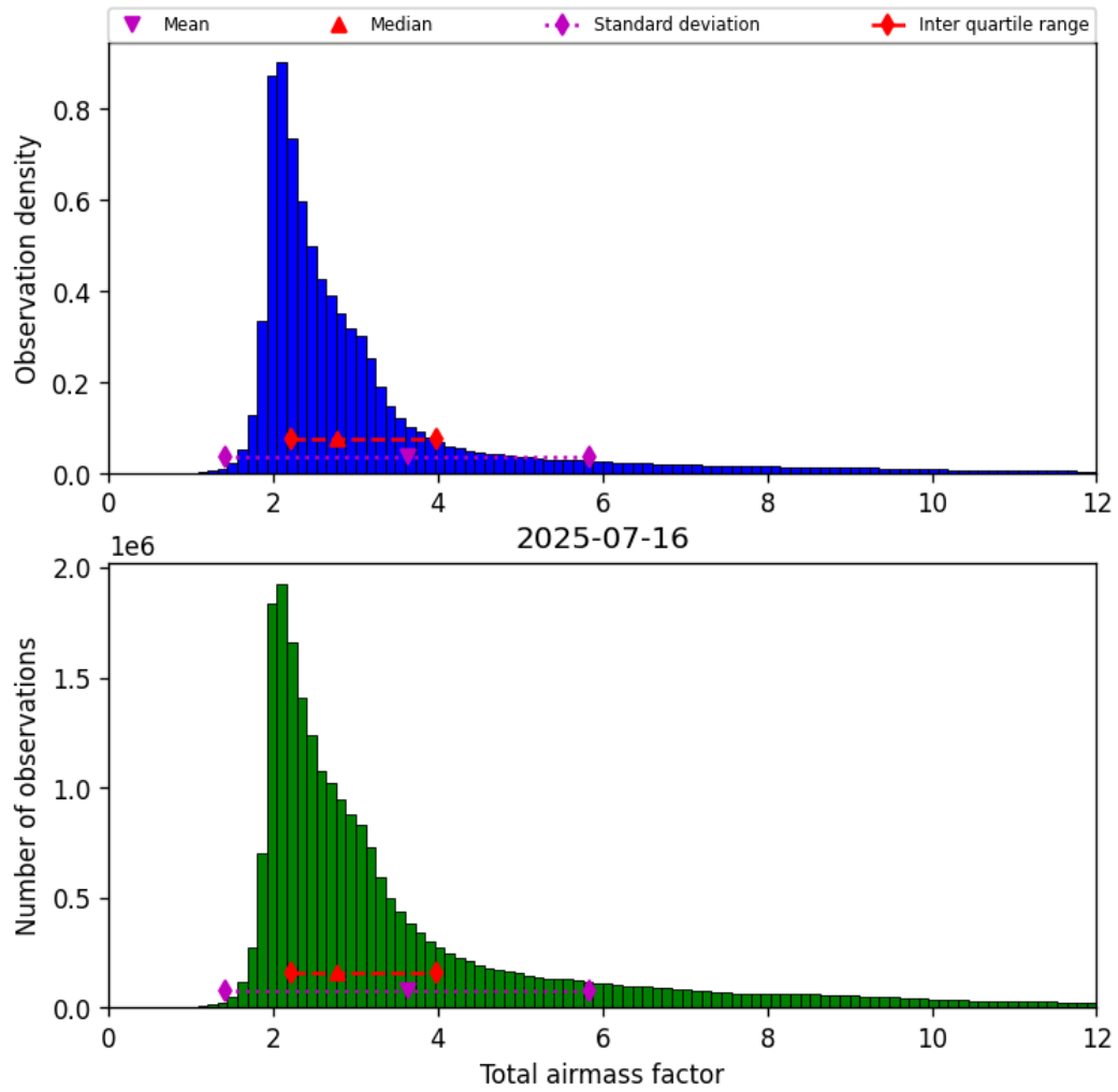
Figure 30: Histogram of “Total airmass factor” for 2025-07-16 to 2025-07-16
