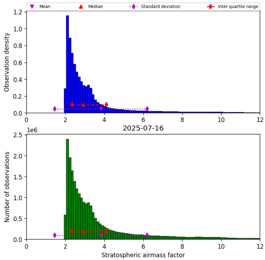
Figure 42: Histogram of “Stratospheric airmass factor” for 2025-07-16 to 2025-07-16
