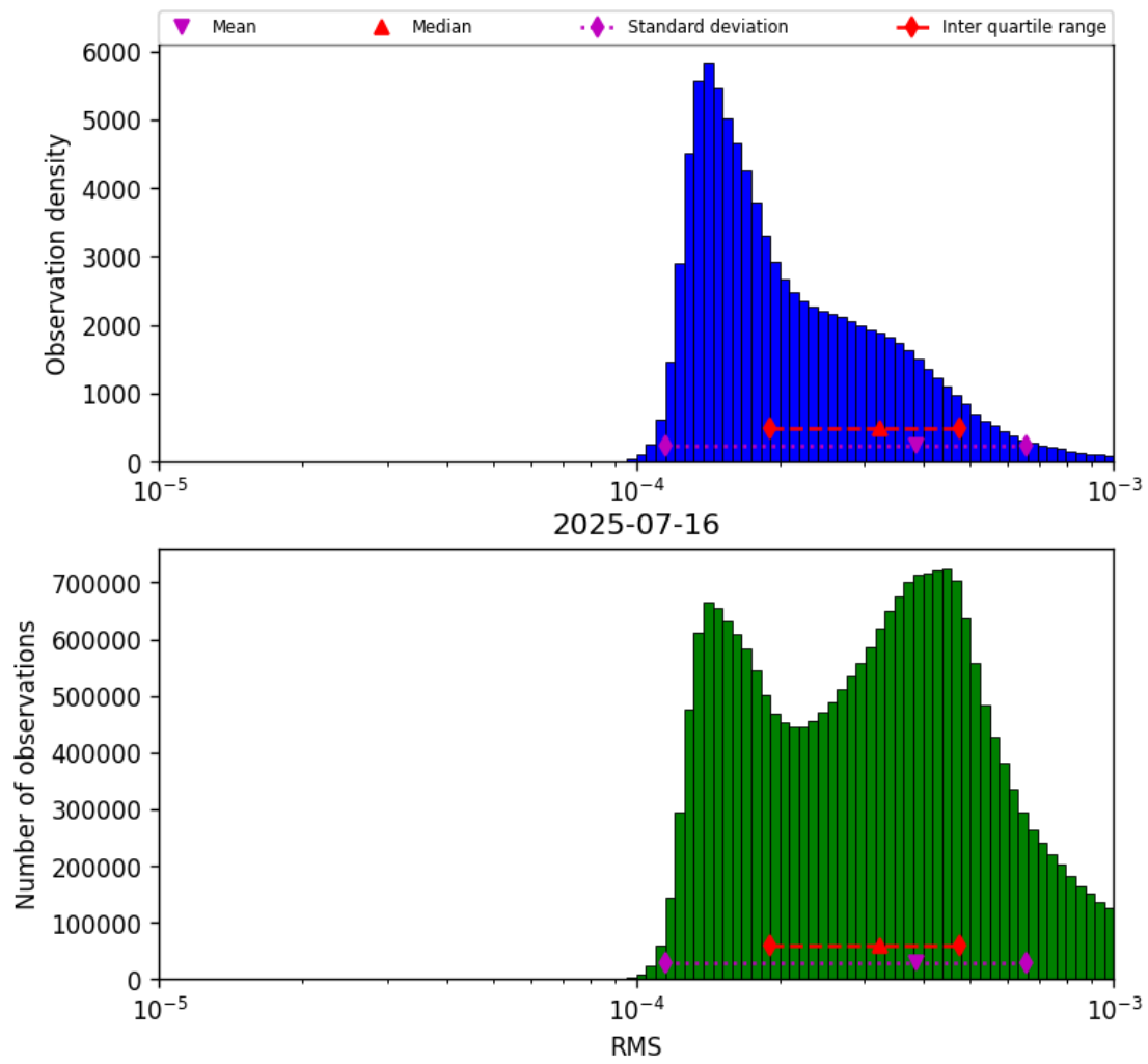
Figure 41: Histogram of “RMS” for 2025-07-16 to 2025-07-16
