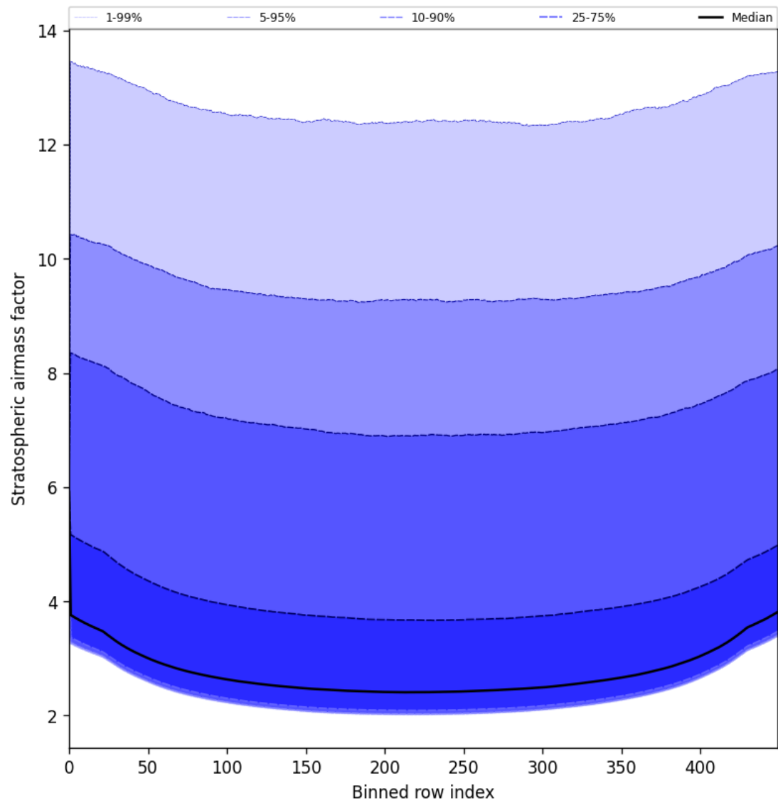
Figure 59: Along track statistics of “Stratospheric airmass factor” for 2025-07-16 to 2025-07-16
