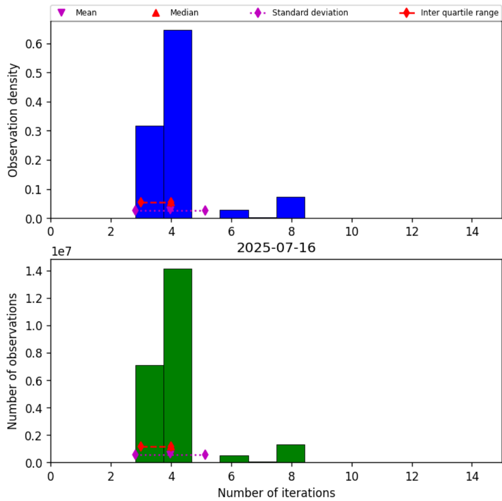
Figure 32: Histogram of “Number of iterations” for 2025-07-16 to 2025-07-16
