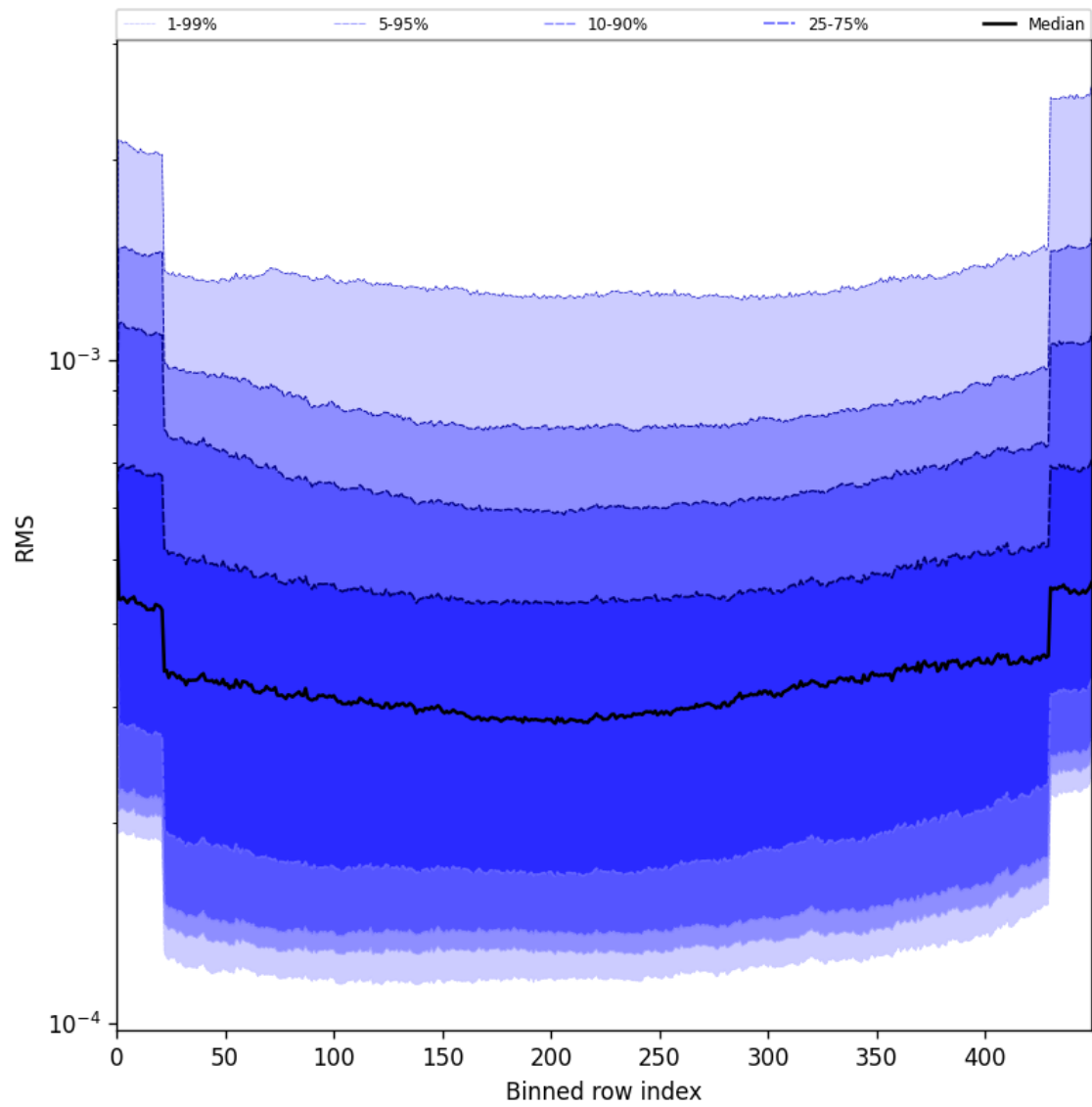
Figure 58: Along track statistics of “RMS” for 2025-07-16 to 2025-07-16
