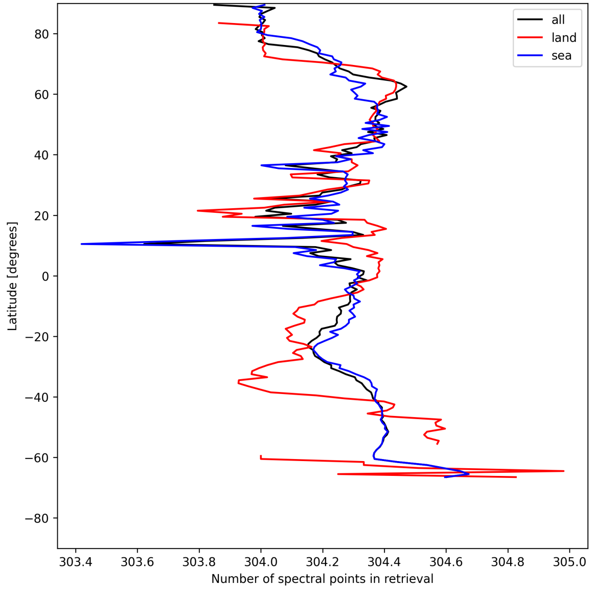
Figure 14: Zonal average of “Number of spectral points in retrieval” for 2025-07-16 to 2025-07-16.
