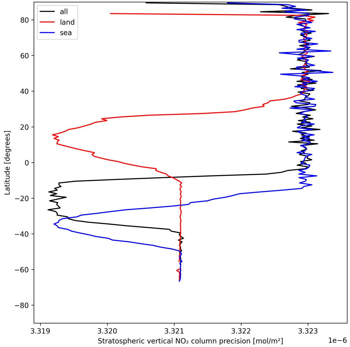
Figure 18: Zonal average of “Stratospheric vertical NO 2 column precision” for 2025-07-16 to 2025-07-16.
