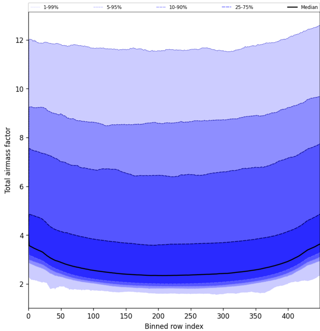
Figure 47: Along track statistics of “Total airmass factor” for 2025-07-16 to 2025-07-16
