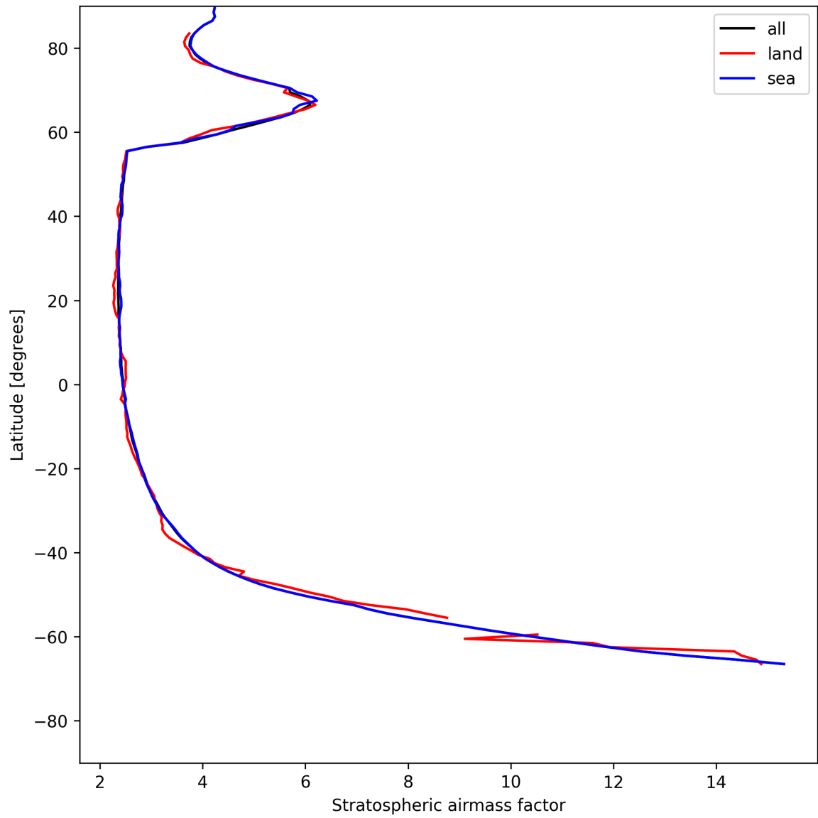
Figure 25: Zonal average of “Stratospheric air mass factor” for 2025-07-16 to 2025-07-16.
