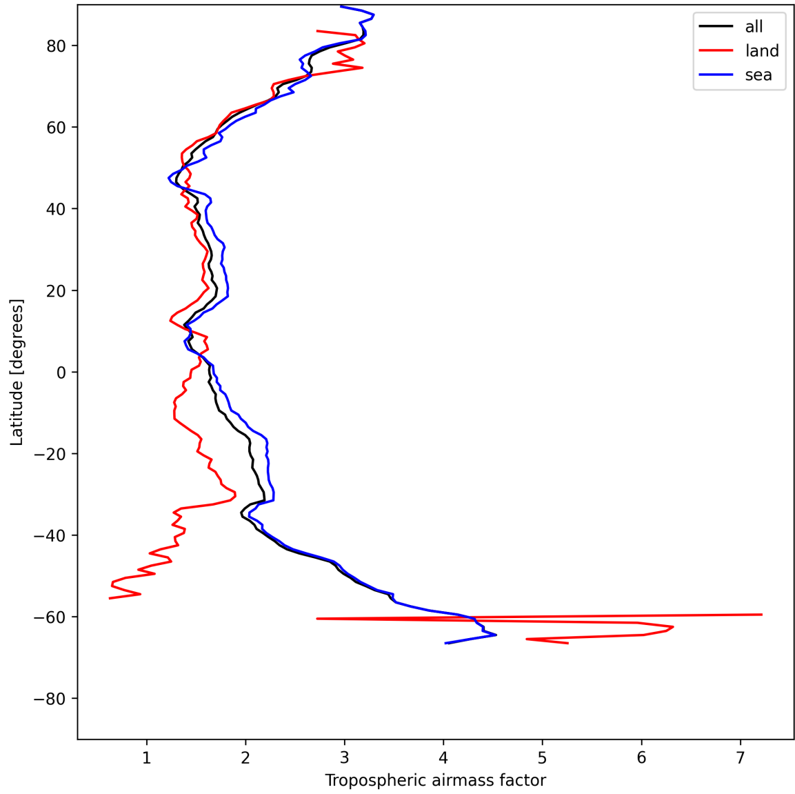
Figure 12: Zonal average of “Tropospheric air mass factor” for 2025-07-16 to 2025-07-16.
