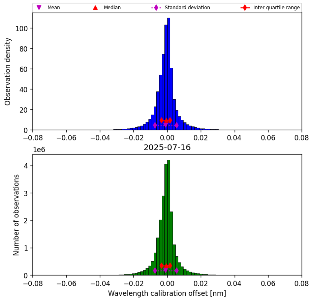
Figure 33: Histogram of “Wavelength calibration offset” for 2025-07-16 to 2025-07-16
