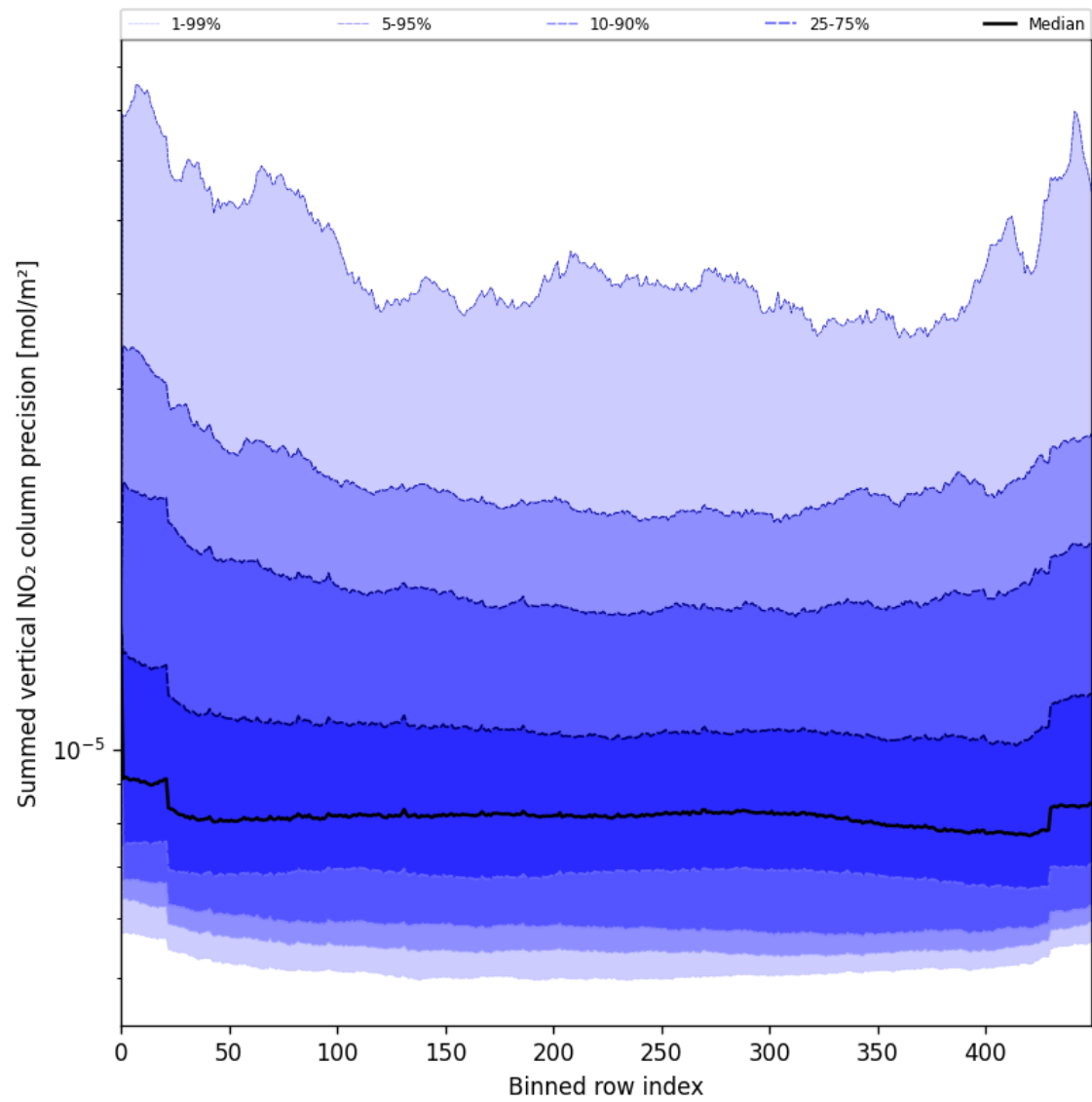
Figure 56: Along track statistics of “Summed vertical NO 2 column precision” for 2025-07-17 to 2025-07-18
