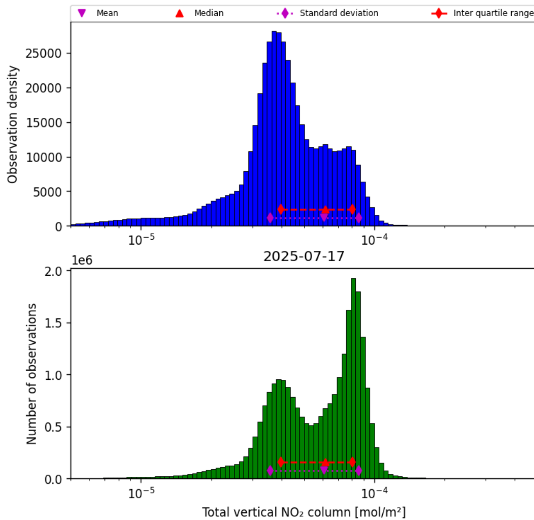
Figure 36: Histogram of “Total vertical NO 2 column” for 2025-07-17 to 2025-07-18
