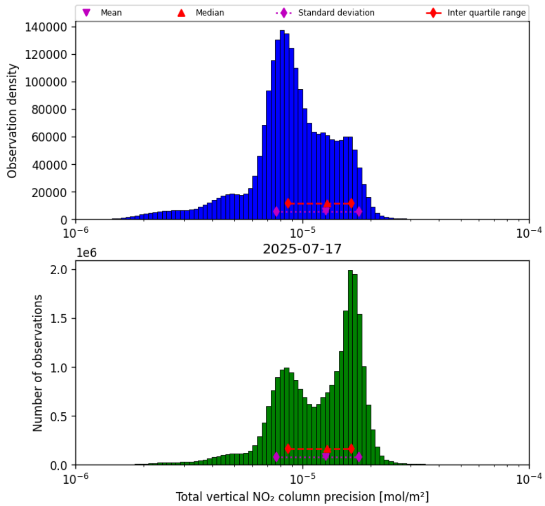
Figure 37: Histogram of “Total vertical NO 2 column precision” for 2025-07-17 to 2025-07-18
