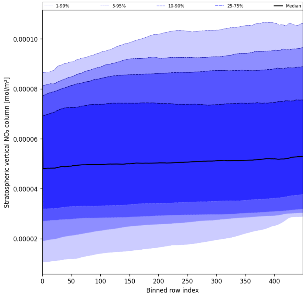
Figure 51: Along track statistics of “Stratospheric vertical NO 2 column” for 2025-07-17 to 2025-07-18
