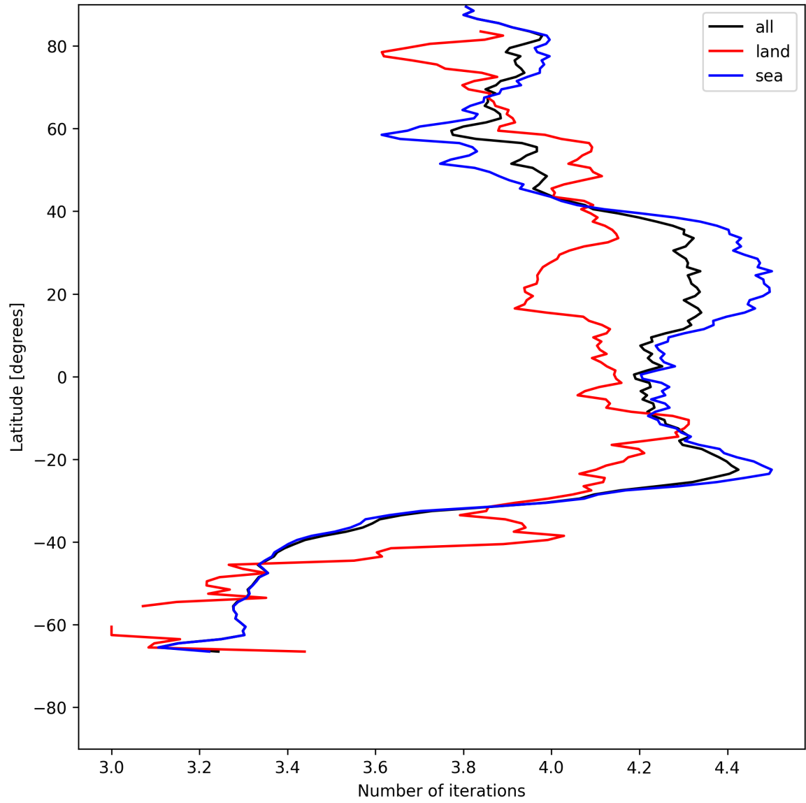
Figure 15: Zonal average of “Number of iterations” for 2025-07-17 to 2025-07-18.
