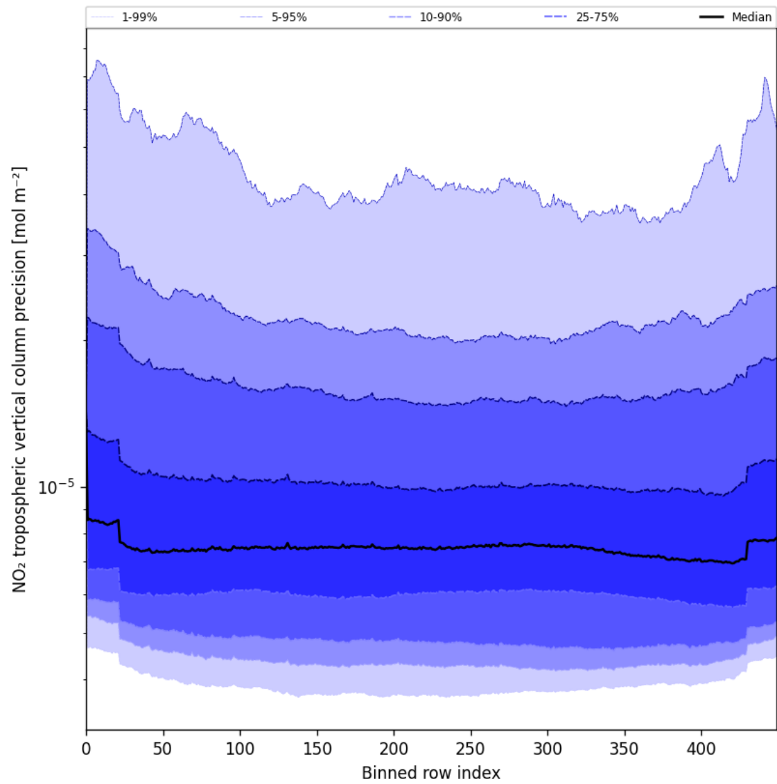
Figure 45: Along track statistics of “NO 2 tropospheric vertical column precision” for 2025-07-17 to 2025-07-18
