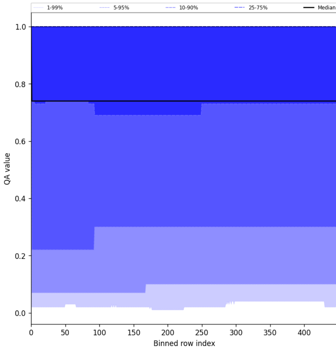
Figure 43: Along track statistics of “QA value” for 2025-07-17 to 2025-07-18
