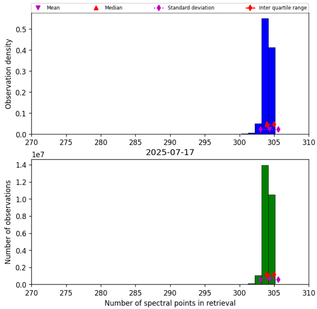
Figure 31: Histogram of “Number of spectral points in retrieval” for 2025-07-17 to 2025-07-18
