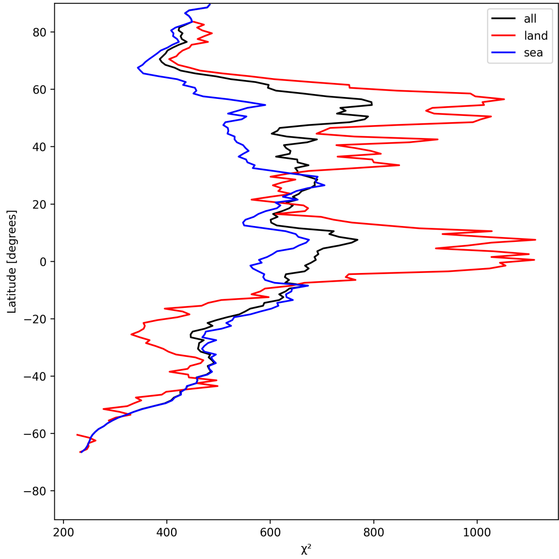
Figure 23: Zonal average of “ \chi^2 ” for 2025-07-17 to 2025-07-18.
