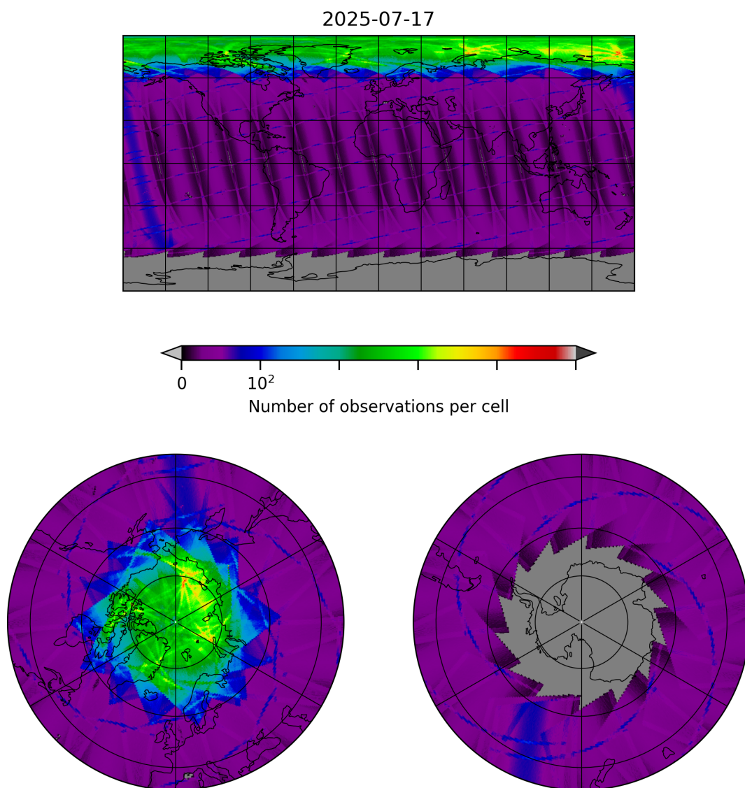
Figure 8: Map of the number of observations for 2025-07-17 to 2025-07-18
