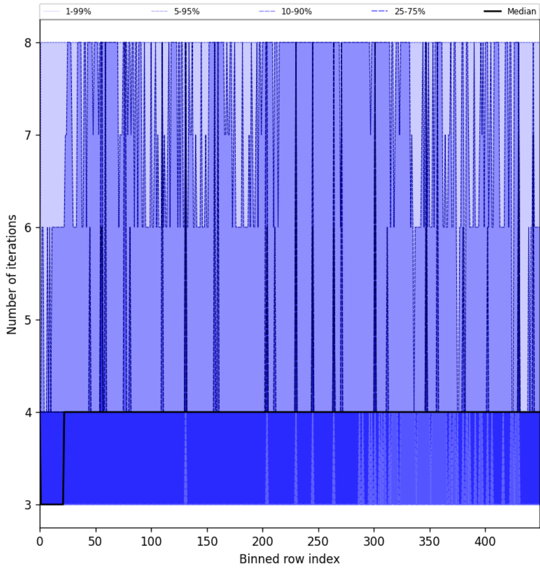
Figure 49: Along track statistics of “Number of iterations” for 2025-07-17 to 2025-07-18
