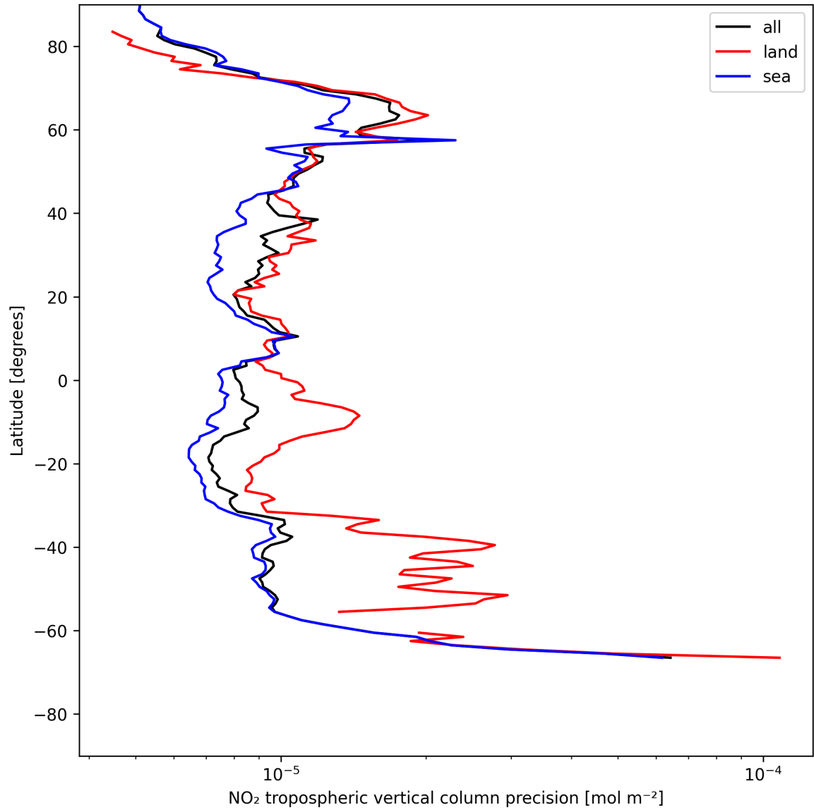
Figure 11: Zonal average of “NO 2 tropospheric vertical column precision” for 2025-07-17 to 2025-07-18.
