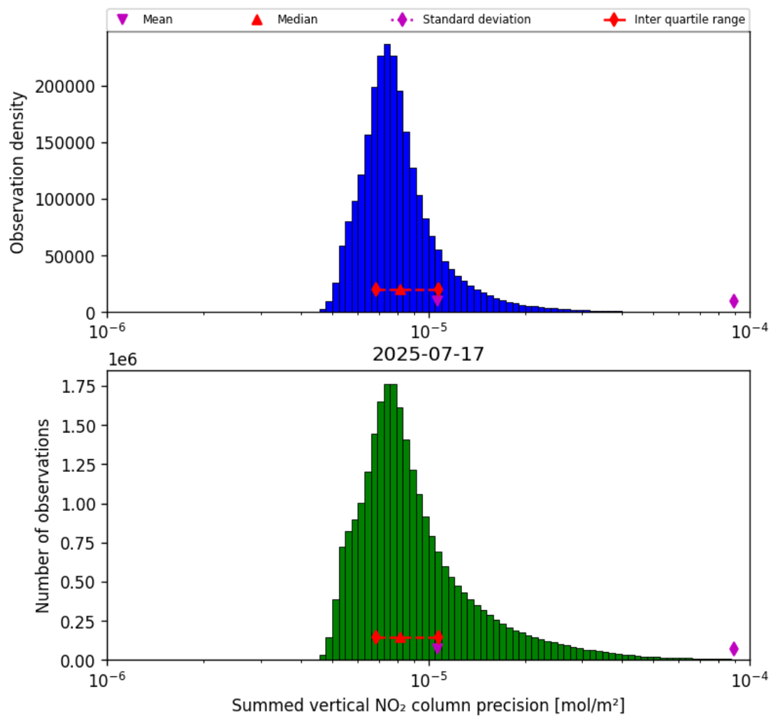
Figure 39: Histogram of "Summed vertical NO 2 column precision" for 2025-07-17 to 2025-07-18
