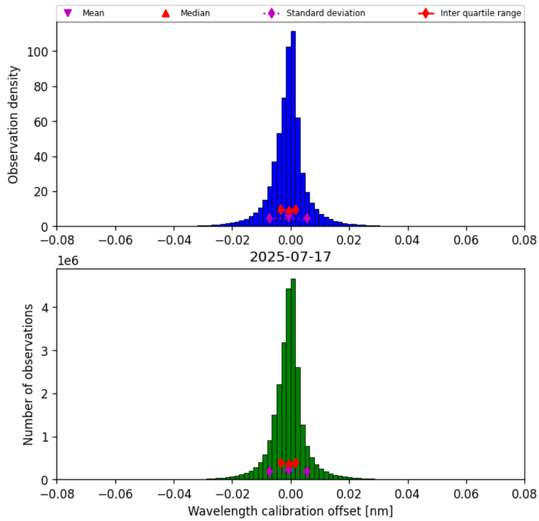
Figure 33: Histogram of “Wavelength calibration offset” for 2025-07-17 to 2025-07-18
