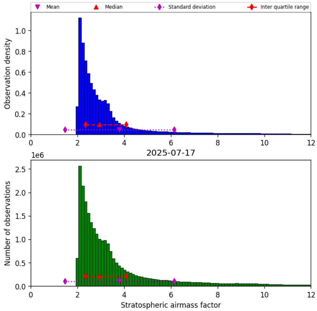
Figure 42: Histogram of “Stratospheric airmass factor” for 2025-07-17 to 2025-07-18
