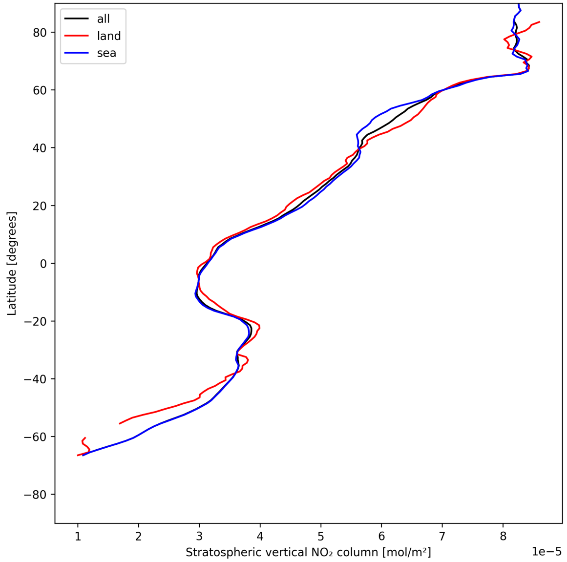
Figure 17: Zonal average of “Stratospheric vertical NO 2 column” for 2025-07-17 to 2025-07-18.
