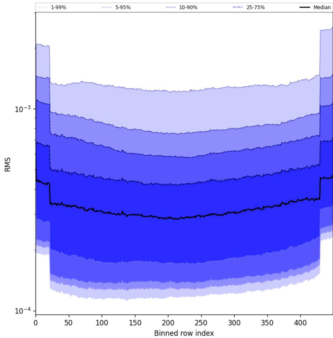
Figure 58: Along track statistics of “RMS” for 2025-07-17 to 2025-07-18
