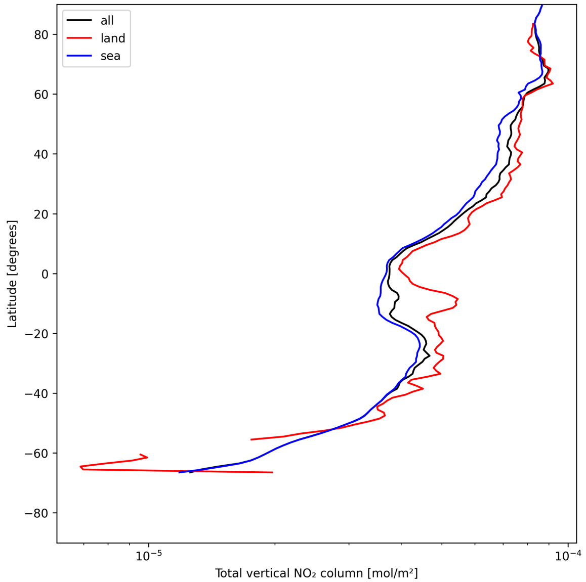
Figure 19: Zonal average of “Total vertical NO 2 column” for 2025-07-17 to 2025-07-18.
