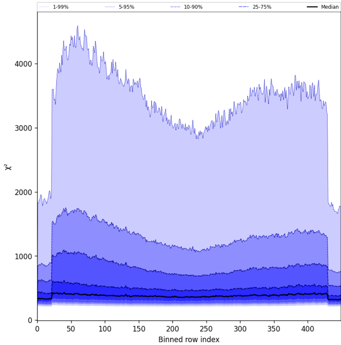
Figure 57: Along track statistics of “ \chi^2 ” for 2025-07-17 to 2025-07-18
