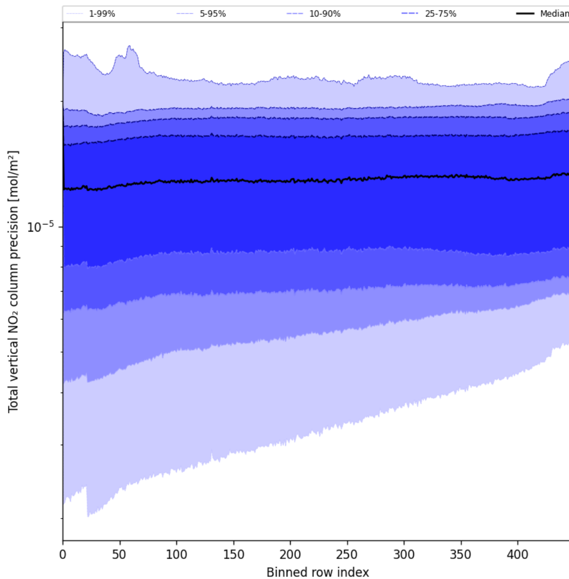
Figure 54: Along track statistics of “Total vertical NO 2 column precision” for 2025-07-17 to 2025-07-18
