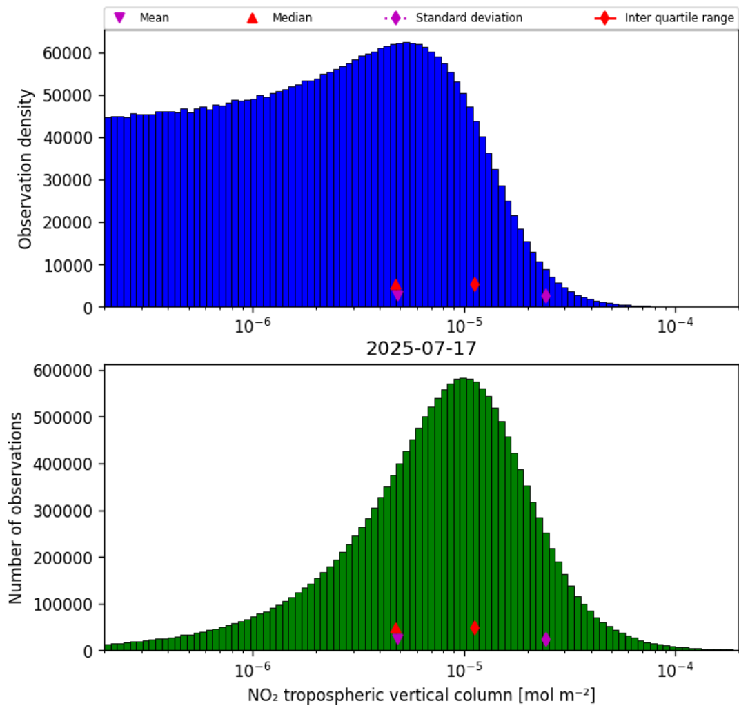
Figure 27: Histogram of “NO 2 tropospheric vertical column” for 2025-07-17 to 2025-07-18
