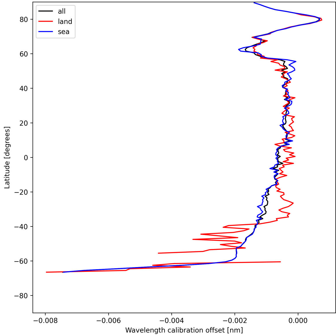
Figure 16: Zonal average of “Wavelength calibration offset” for 2025-07-17 to 2025-07-18.
