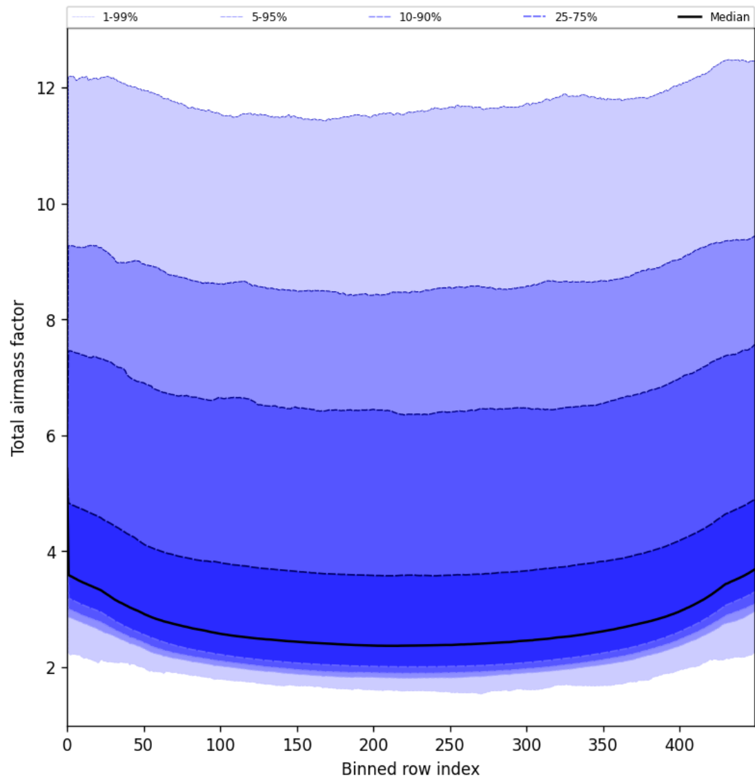
Figure 47: Along track statistics of “Total airmass factor” for 2025-07-17 to 2025-07-18
