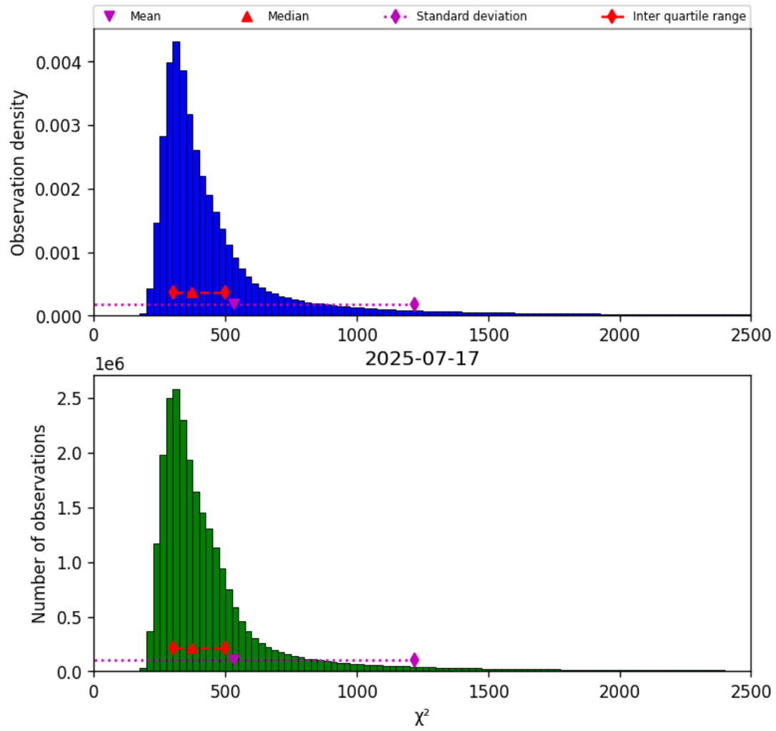
Figure 40: Histogram of “ \chi^2 ” for 2025-07-17 to 2025-07-18
