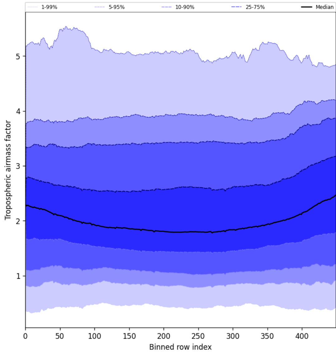
Figure 46: Along track statistics of “Tropospheric airmass factor” for 2025-07-17 to 2025-07-18
