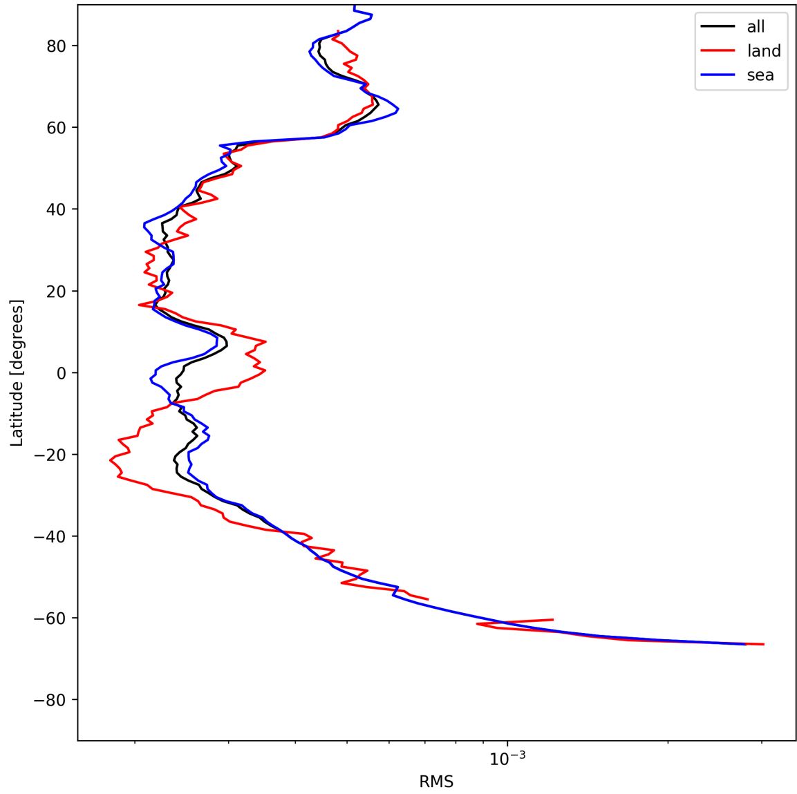
Figure 24: Zonal average of “RMS” for 2025-07-17 to 2025-07-18.
