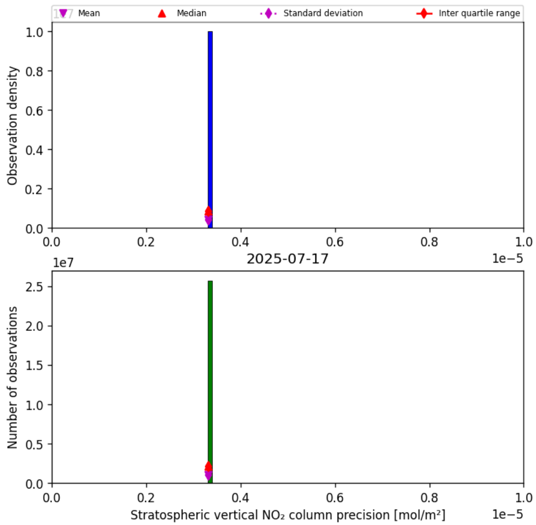
Figure 35: Histogram of “Stratospheric vertical NO 2 column precision” for 2025-07-17 to 2025-07-18
