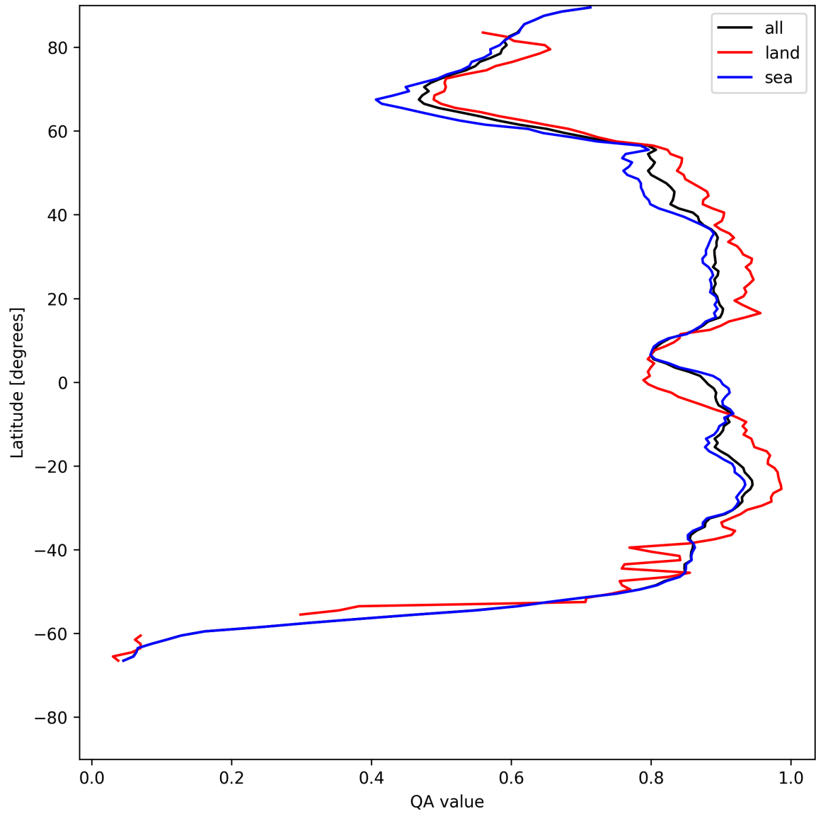
Figure 9: Zonal average of “QA value” for 2025-07-17 to 2025-07-18.
