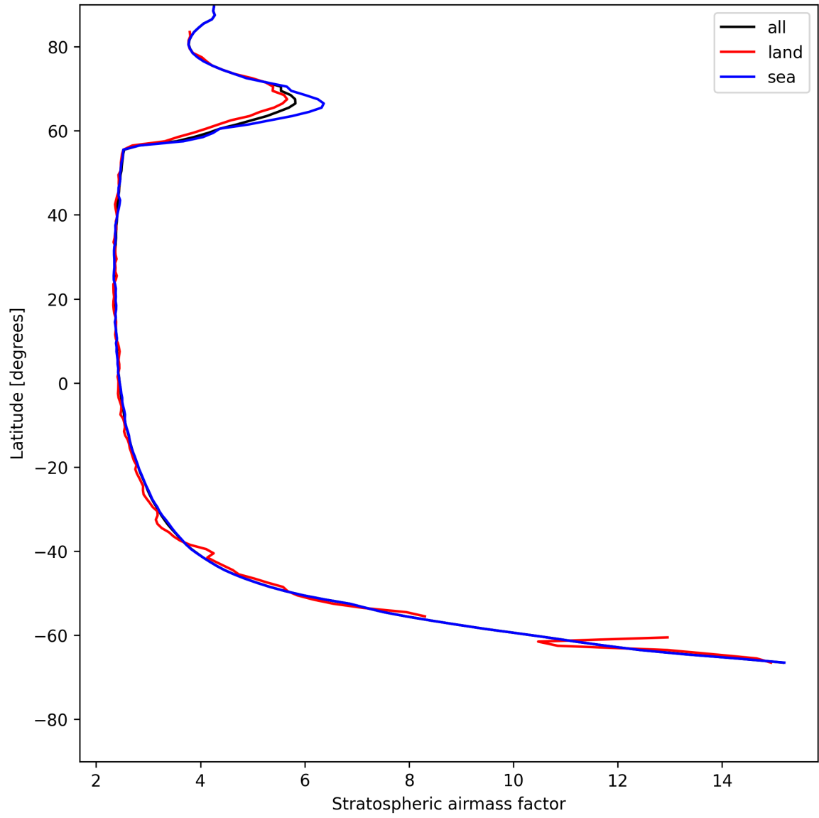
Figure 25: Zonal average of “Stratospheric air mass factor” for 2025-07-17 to 2025-07-18.
