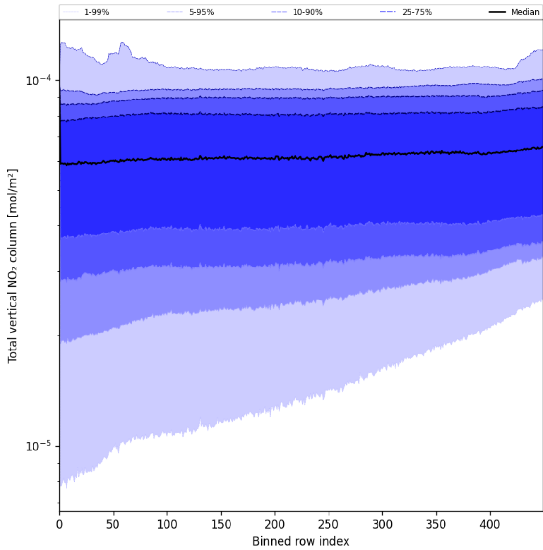
Figure 53: Along track statistics of “Total vertical NO 2 column” for 2025-07-17 to 2025-07-18
