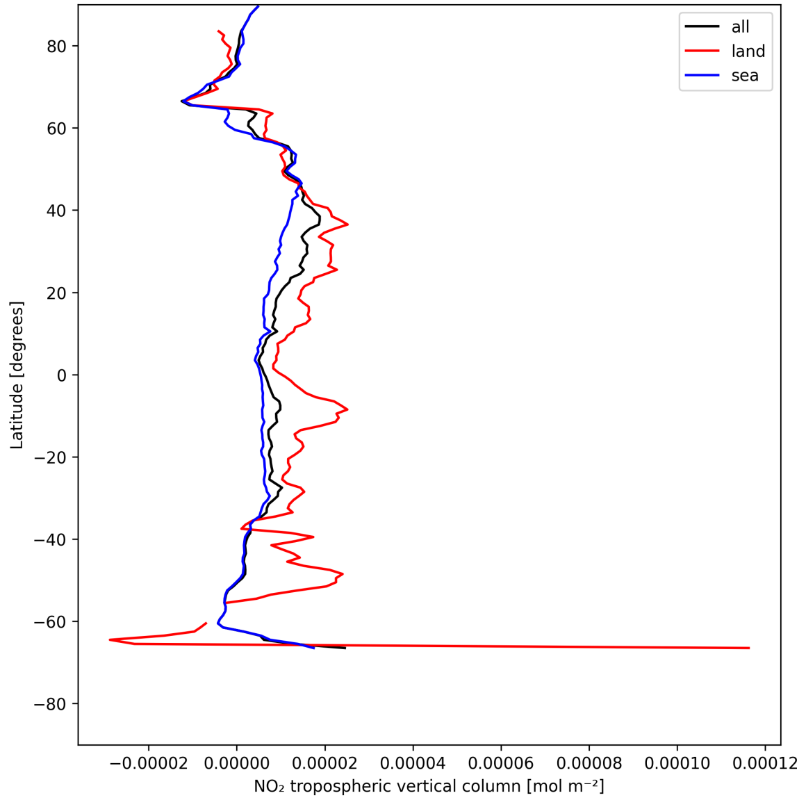
Figure 10: Zonal average of “NO 2 tropospheric vertical column” for 2025-07-17 to 2025-07-18.
