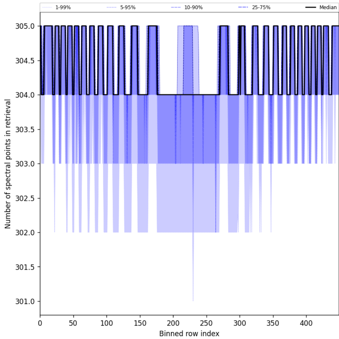
Figure 48: Along track statistics of “Number of spectral points in retrieval” for 2025-07-17 to 2025-07-18
