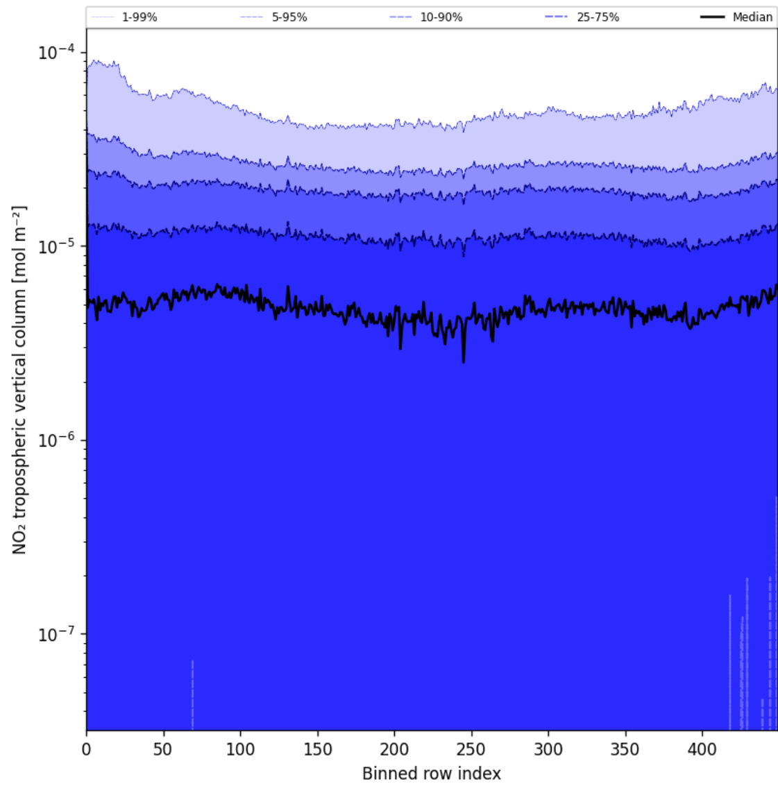
Figure 44: Along track statistics of “NO 2 tropospheric vertical column” for 2025-07-17 to 2025-07-18
