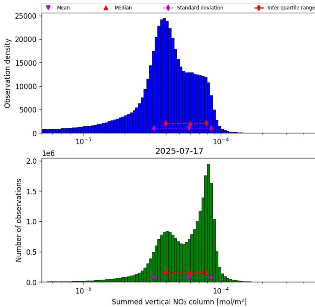
Figure 38: Histogram of "Summed vertical NO 2 column" for 2025-07-17 to 2025-07-18
