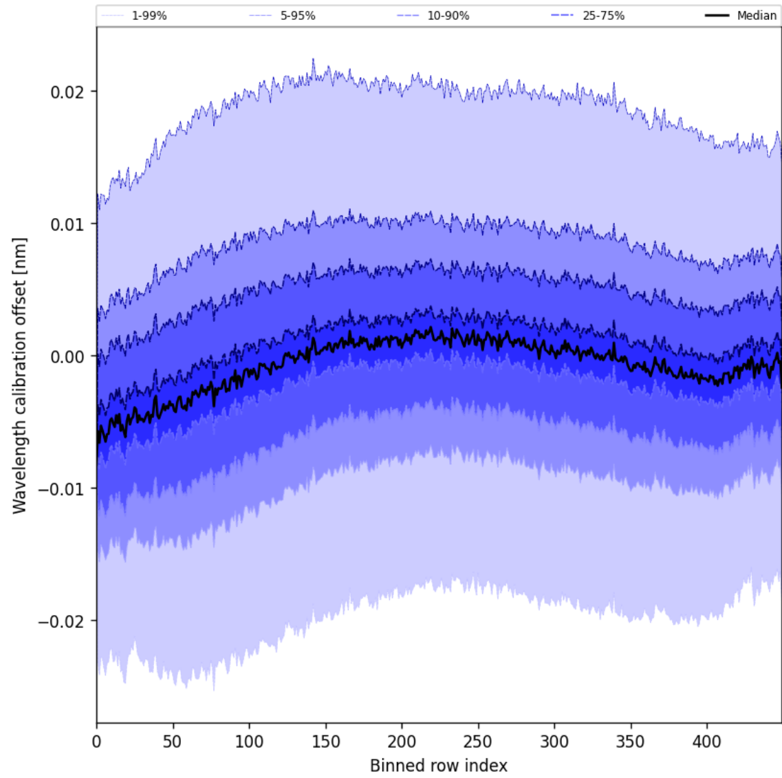
Figure 50: Along track statistics of “Wavelength calibration offset” for 2025-07-17 to 2025-07-18
