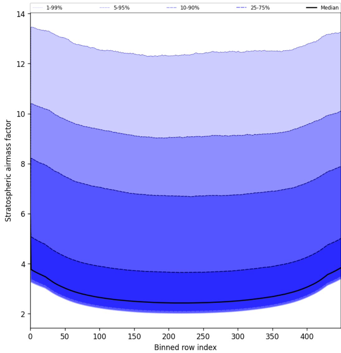
Figure 59: Along track statistics of “Stratospheric airmass factor” for 2025-07-17 to 2025-07-18
