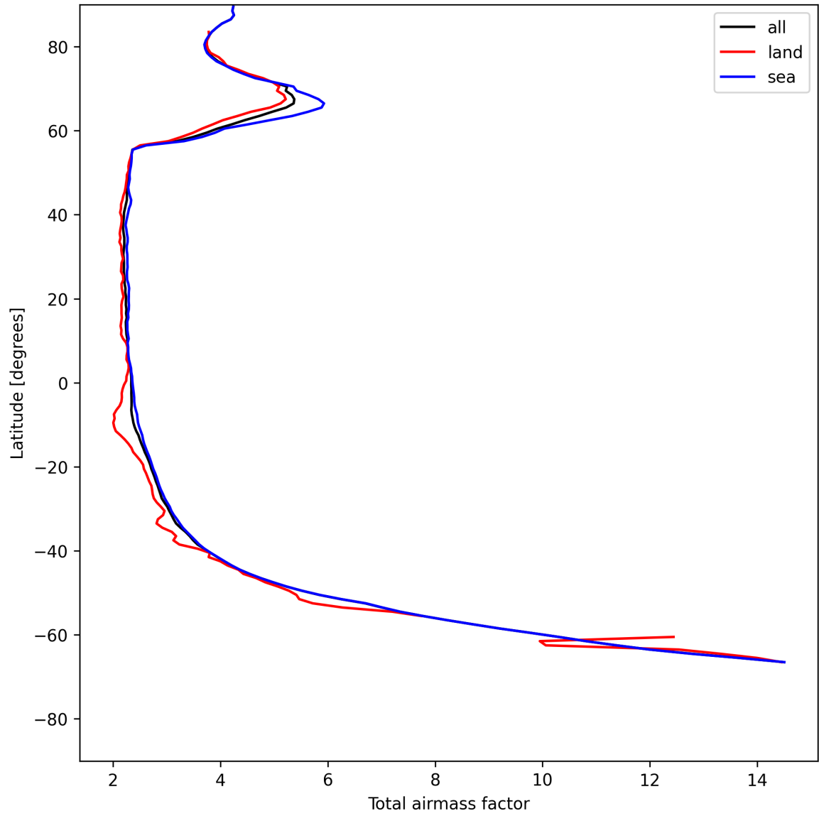
Figure 13: Zonal average of “Total airmass factor” for 2025-07-17 to 2025-07-18.
