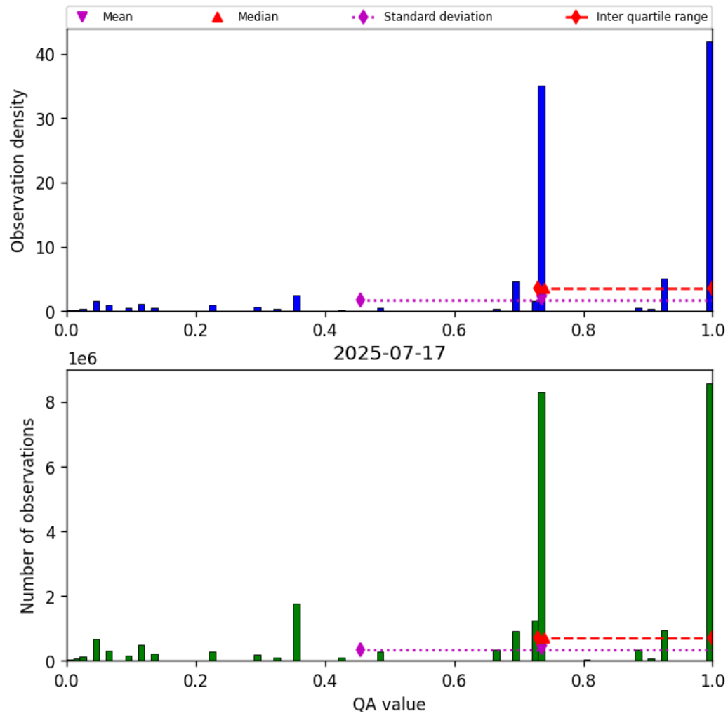
Figure 26: Histogram of “QA value” for 2025-07-17 to 2025-07-18
