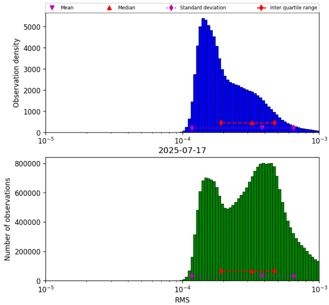
Figure 41: Histogram of “RMS” for 2025-07-17 to 2025-07-18
