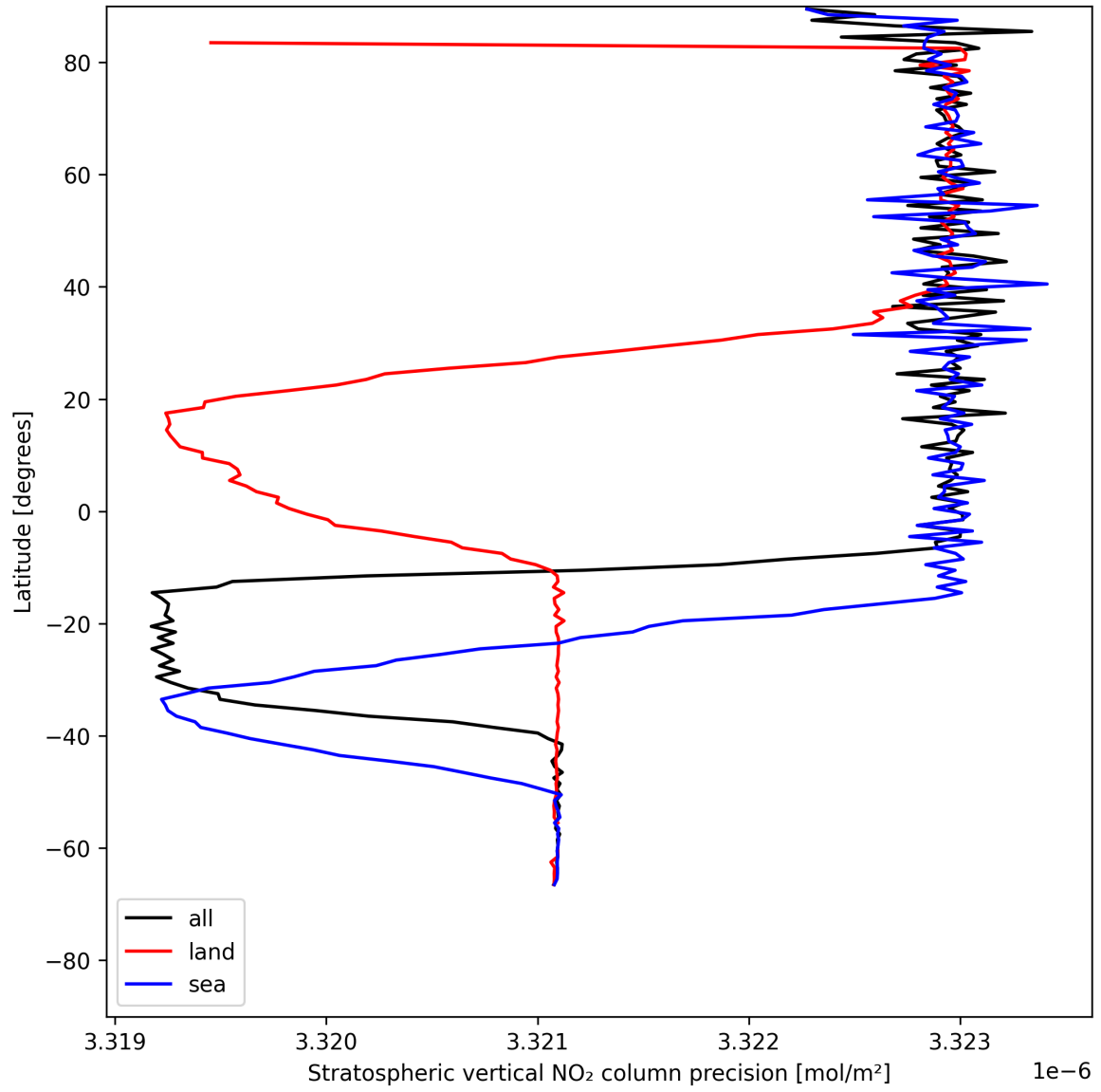
Figure 18: Zonal average of “Stratospheric vertical NO 2 column precision” for 2025-07-17 to 2025-07-18.
