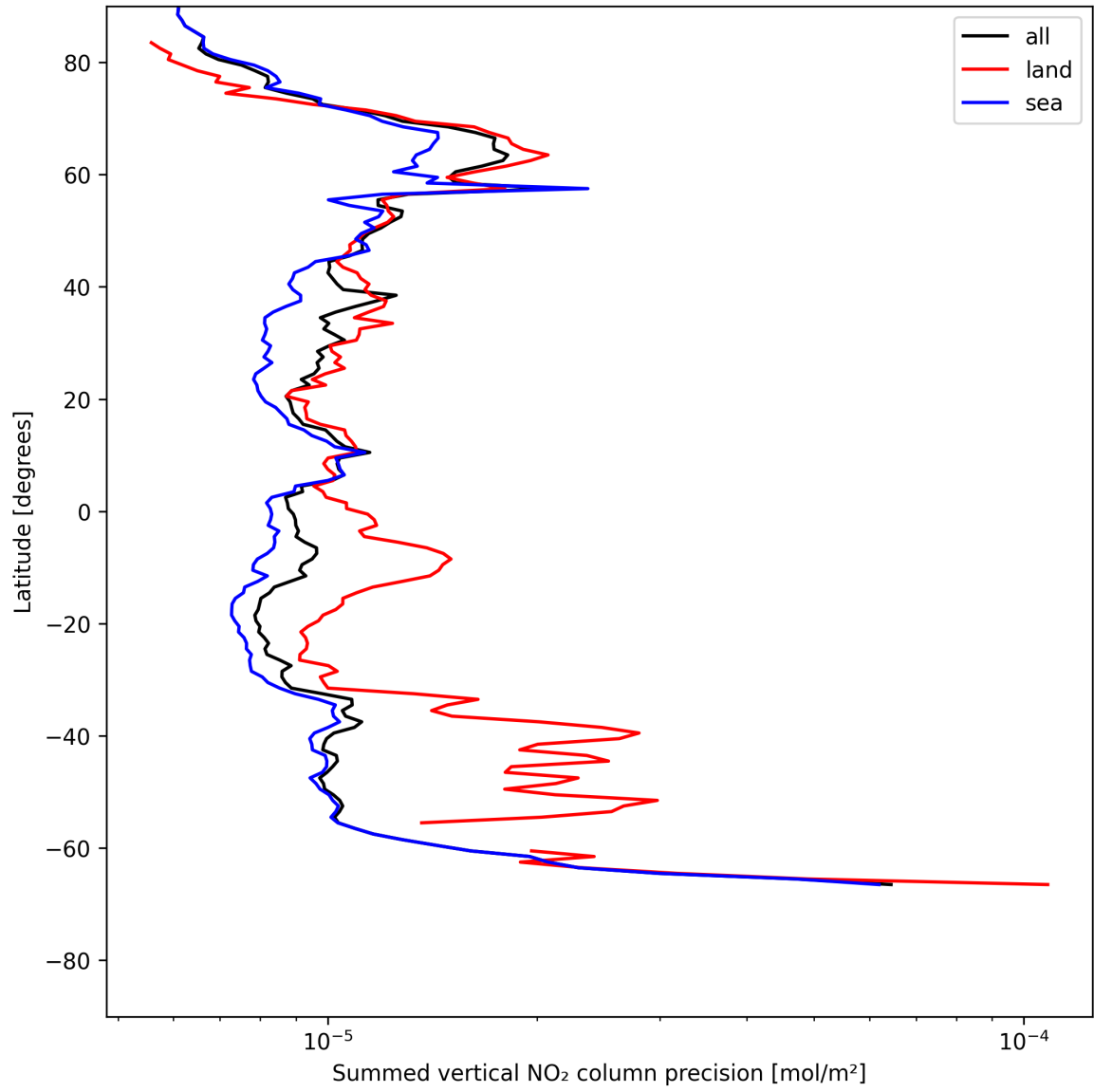
Figure 22: Zonal average of “Summed vertical NO 2 column precision” for 2025-07-17 to 2025-07-18.
