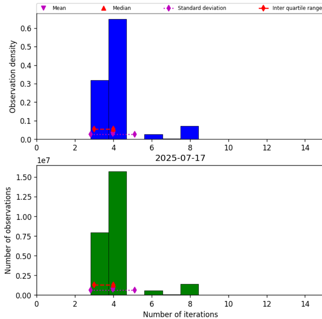
Figure 32: Histogram of “Number of iterations” for 2025-07-17 to 2025-07-18
