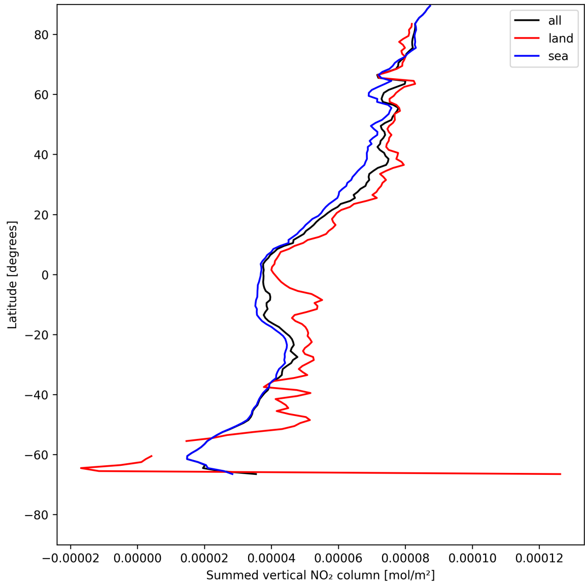
Figure 21: Zonal average of “Summed vertical NO 2 column” for 2025-07-17 to 2025-07-18.
