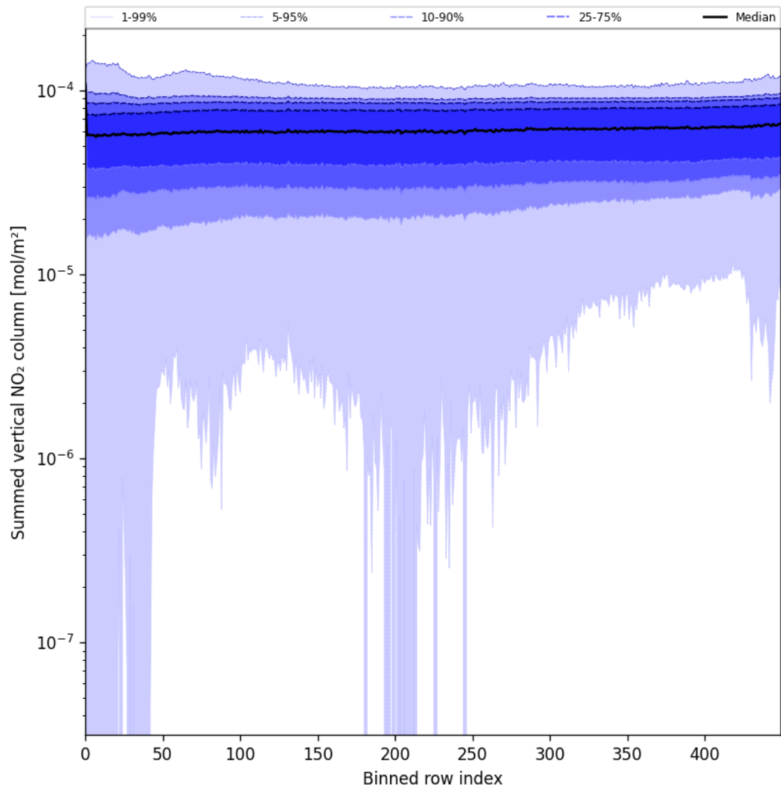
Figure 55: Along track statistics of “Summed vertical NO 2 column” for 2025-07-17 to 2025-07-18
