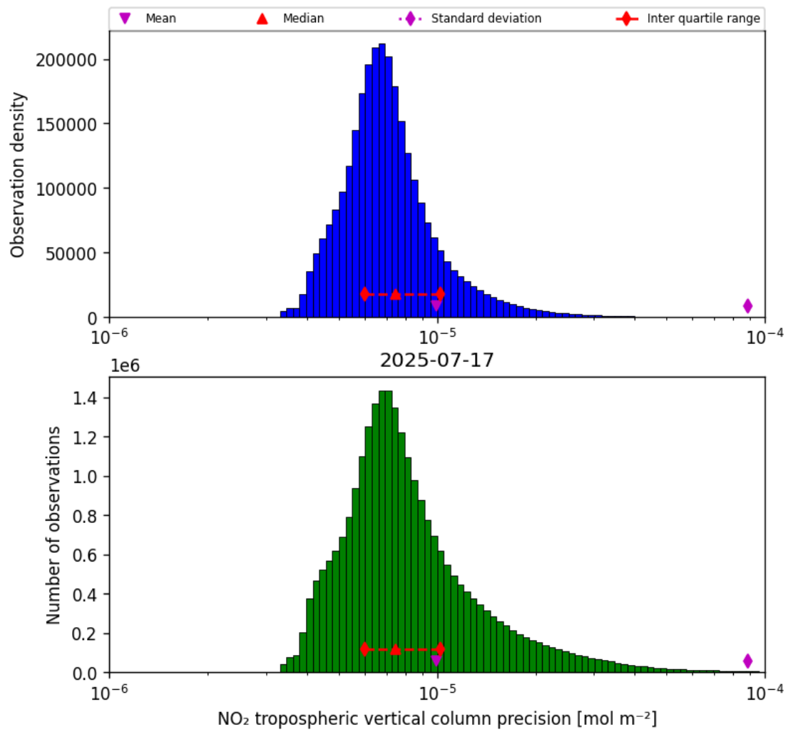
Figure 28: Histogram of “NO 2 tropospheric vertical column precision” for 2025-07-17 to 2025-07-18
