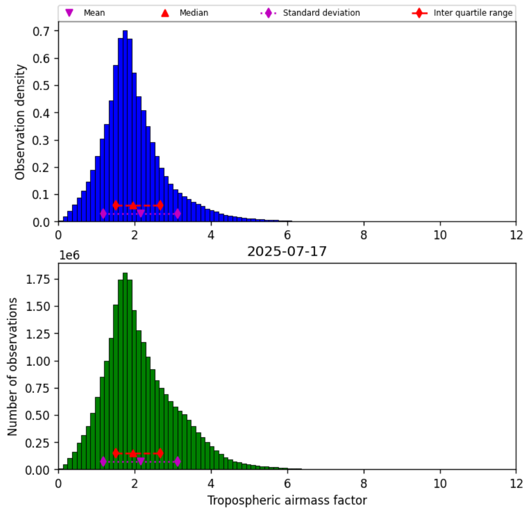
Figure 29: Histogram of “Tropospheric airmass factor” for 2025-07-17 to 2025-07-18
