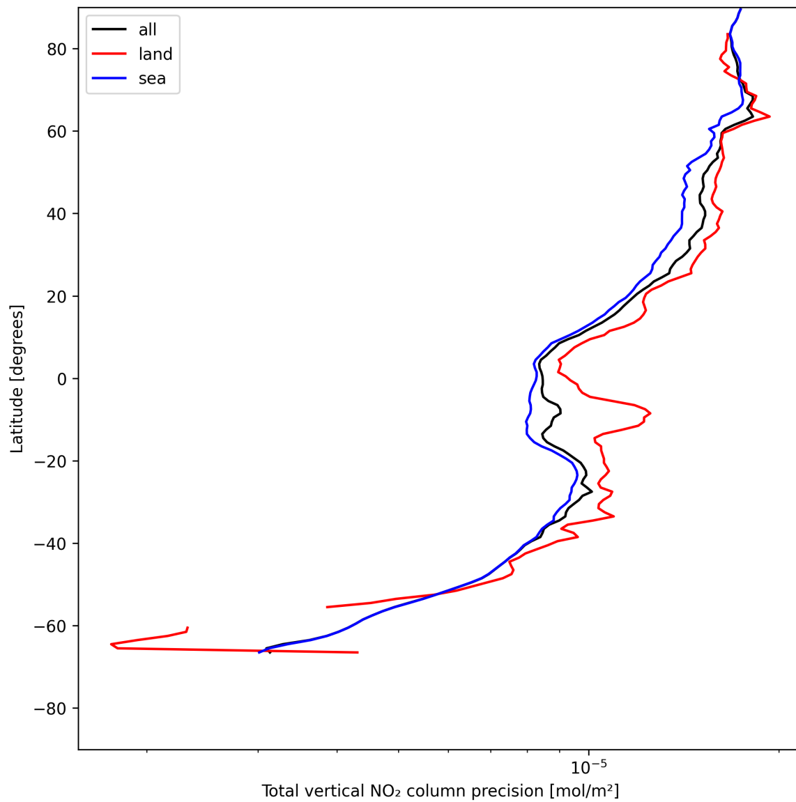
Figure 20: Zonal average of “Total vertical NO 2 column precision” for 2025-07-17 to 2025-07-18.
