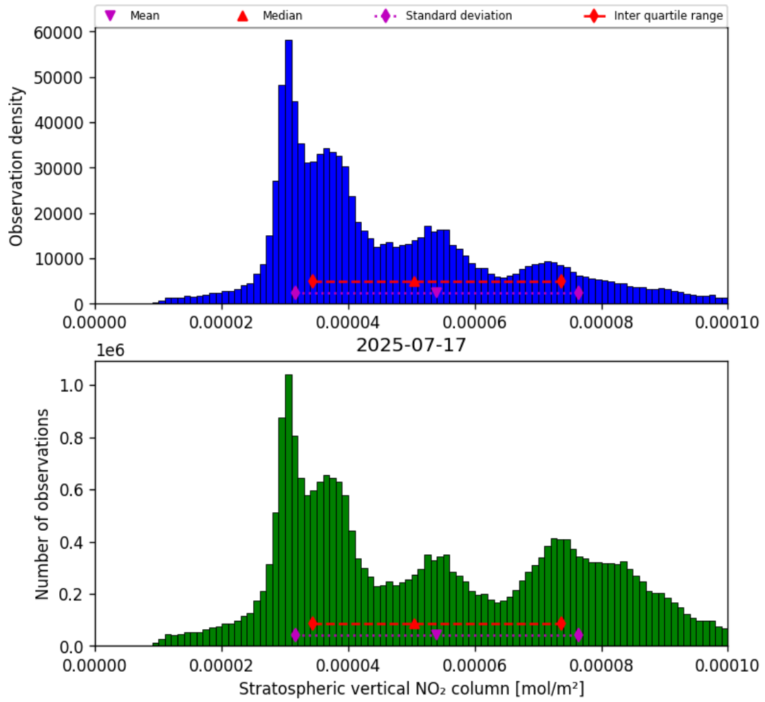
Figure 34: Histogram of “Stratospheric vertical NO 2 column” for 2025-07-17 to 2025-07-18
