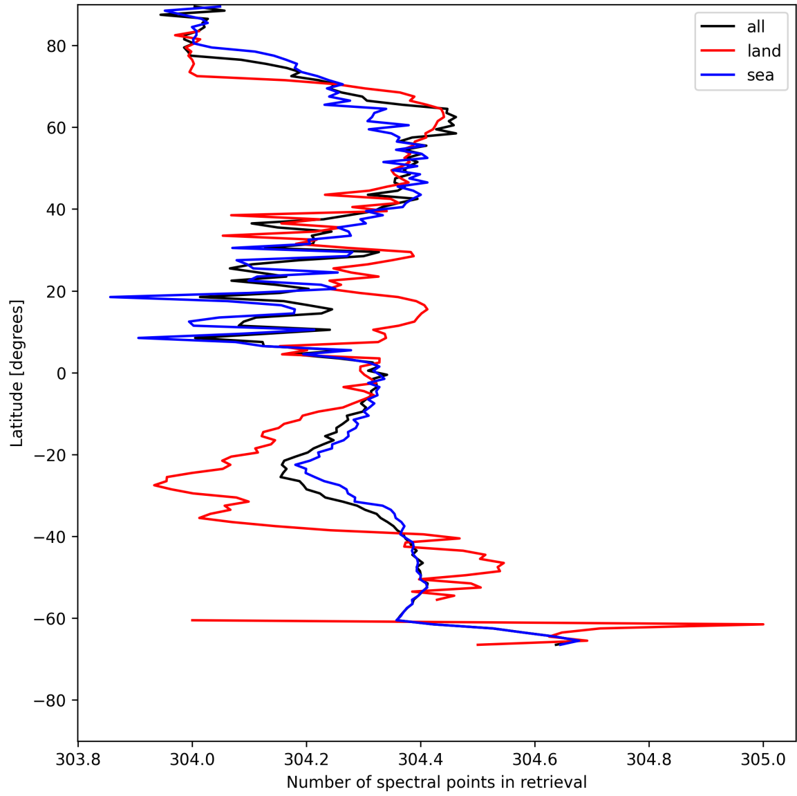
Figure 14: Zonal average of “Number of spectral points in retrieval” for 2025-07-17 to 2025-07-18.
