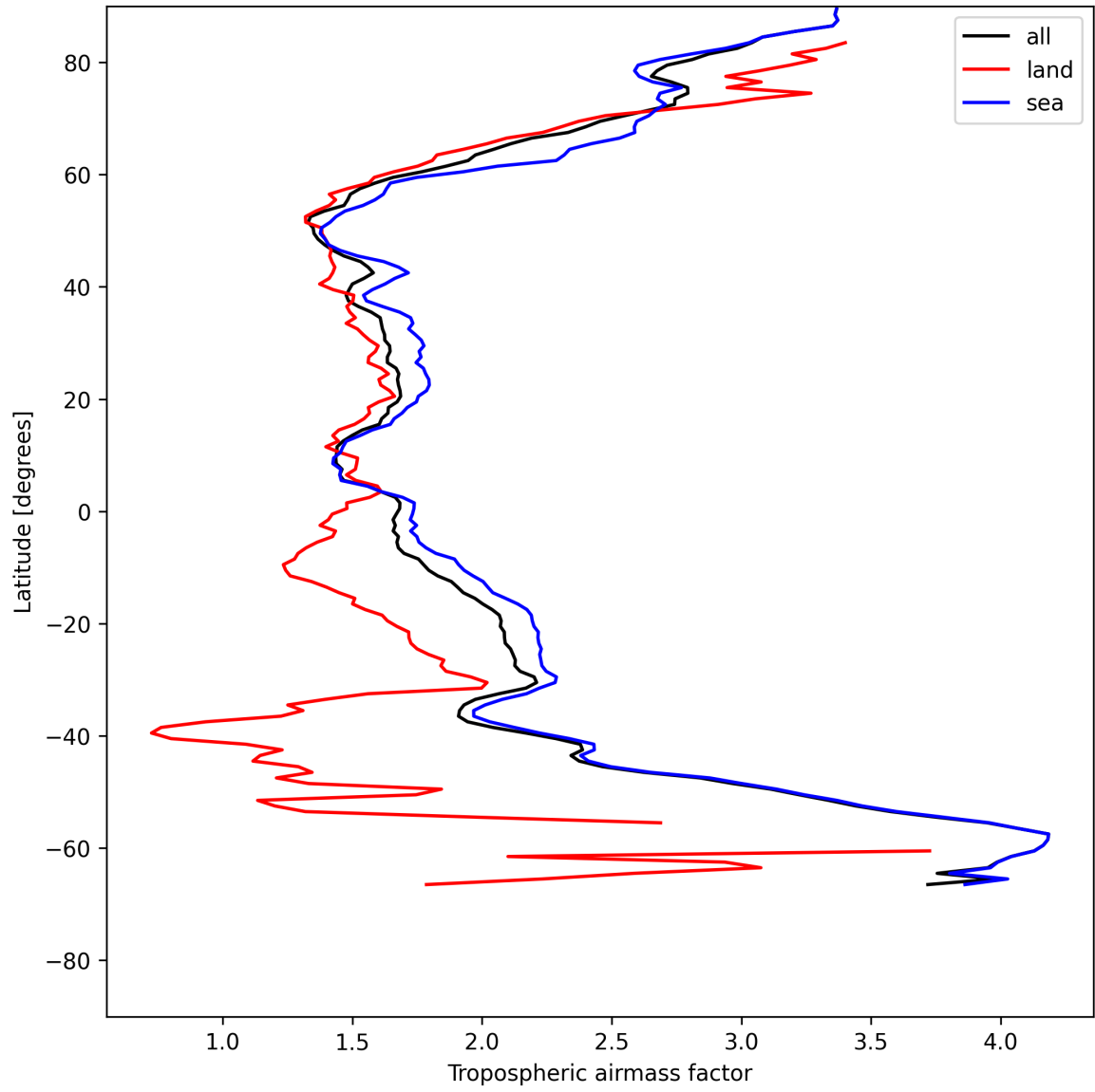
Figure 12: Zonal average of “Tropospheric airmass factor” for 2025-07-17 to 2025-07-18.
