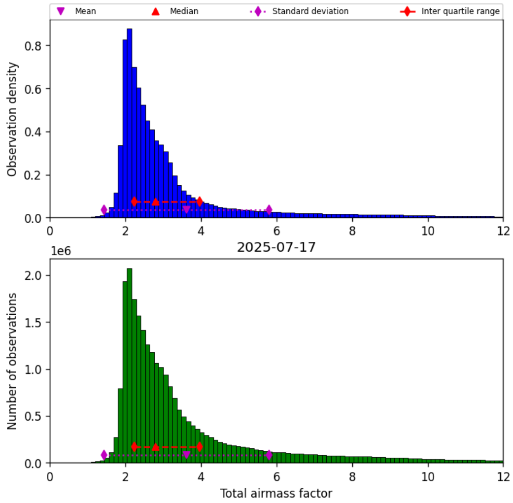
Figure 30: Histogram of “Total airmass factor” for 2025-07-17 to 2025-07-18
