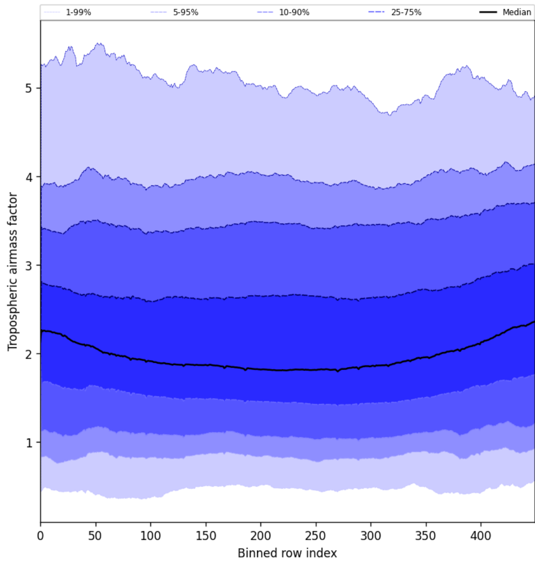
Figure 46: Along track statistics of “Tropospheric airmass factor” for 2025-07-18 to 2025-07-19
