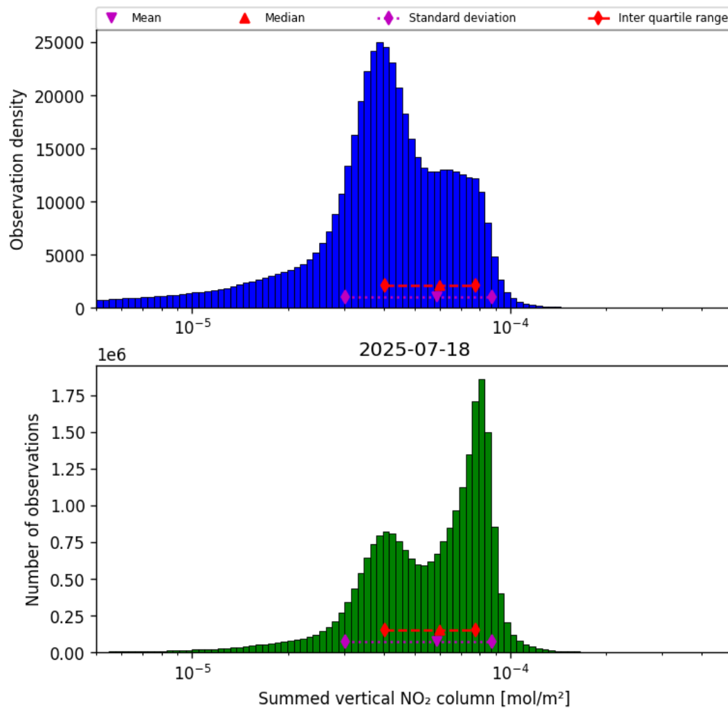
Figure 38: Histogram of "Summed vertical NO 2 column" for 2025-07-18 to 2025-07-19
