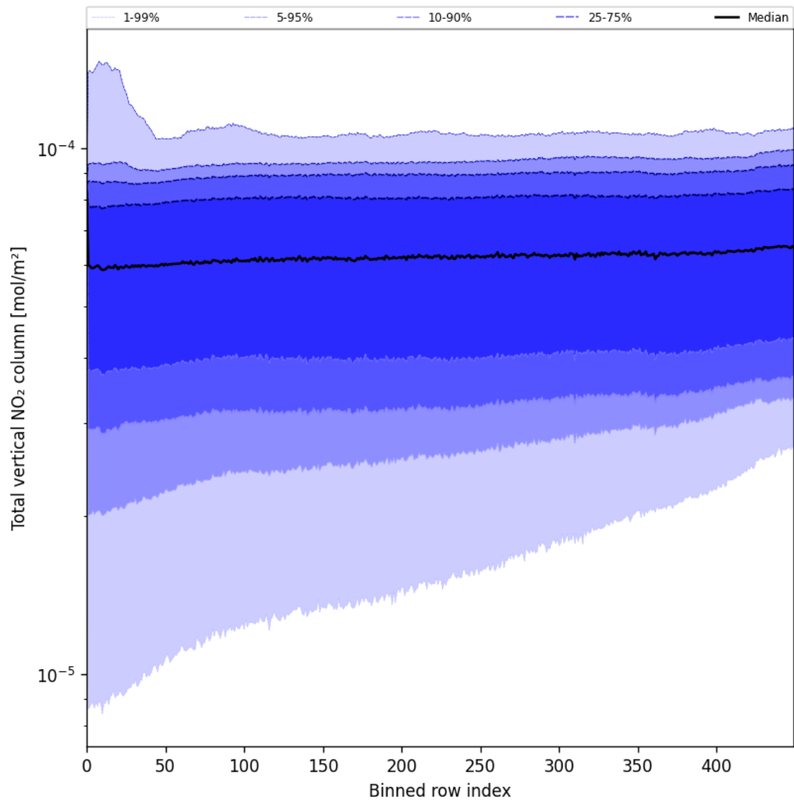
Figure 53: Along track statistics of “Total vertical NO 2 column” for 2025-07-18 to 2025-07-19
