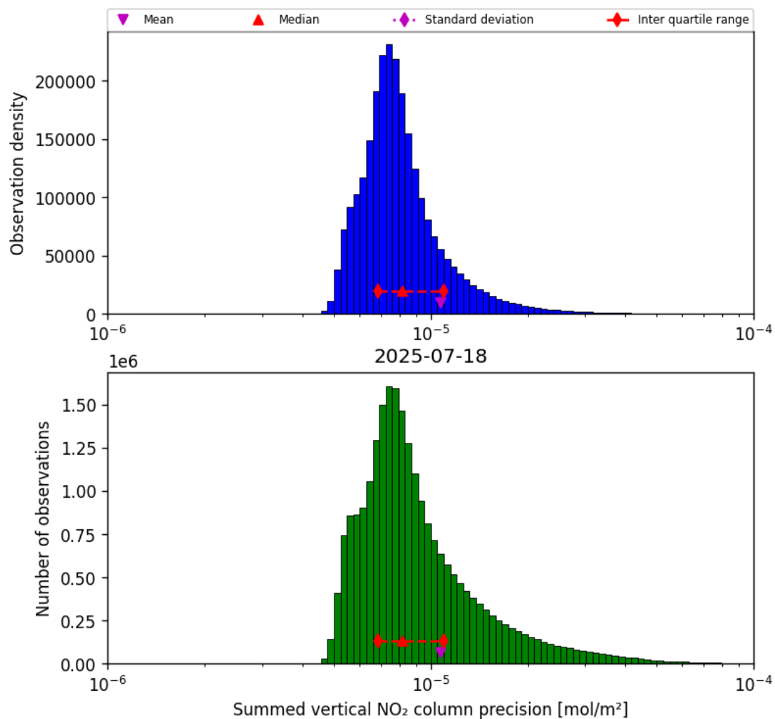
Figure 39: Histogram of “Summed vertical NO 2 column precision” for 2025-07-18 to 2025-07-19
