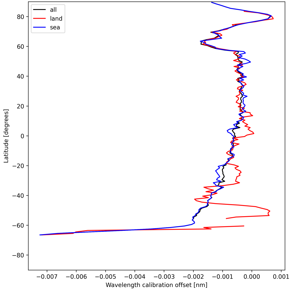
Figure 16: Zonal average of “Wavelength calibration offset” for 2025-07-18 to 2025-07-19.
