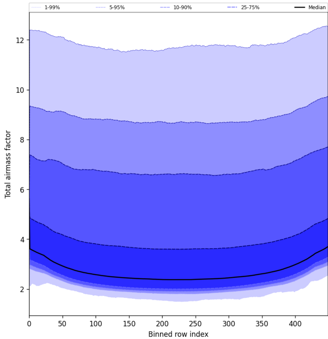
Figure 47: Along track statistics of “Total airmass factor” for 2025-07-18 to 2025-07-19
