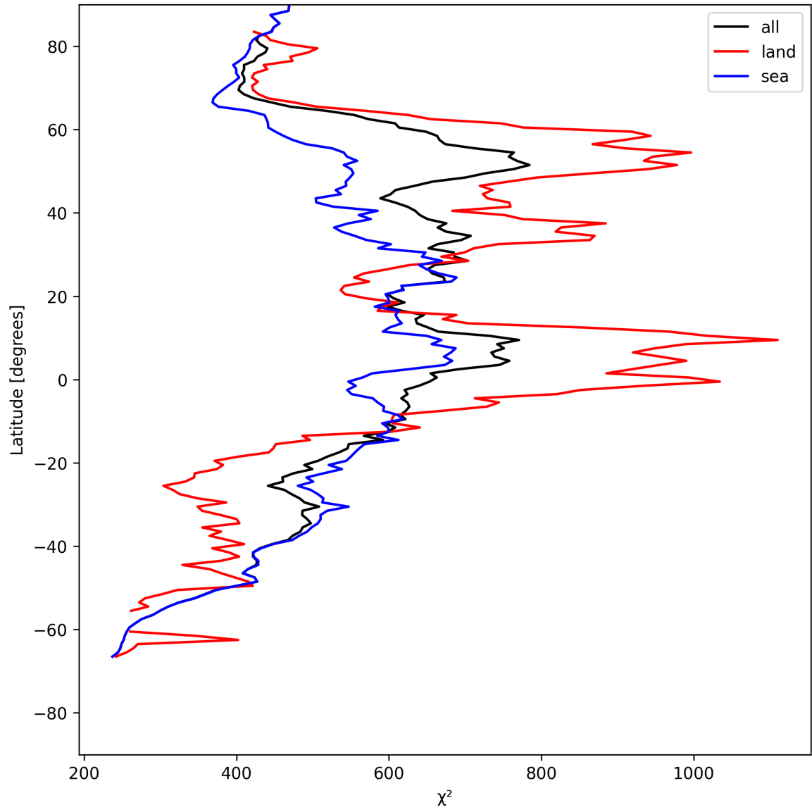
Figure 23: Zonal average of “ \chi^2 ” for 2025-07-18 to 2025-07-19.
