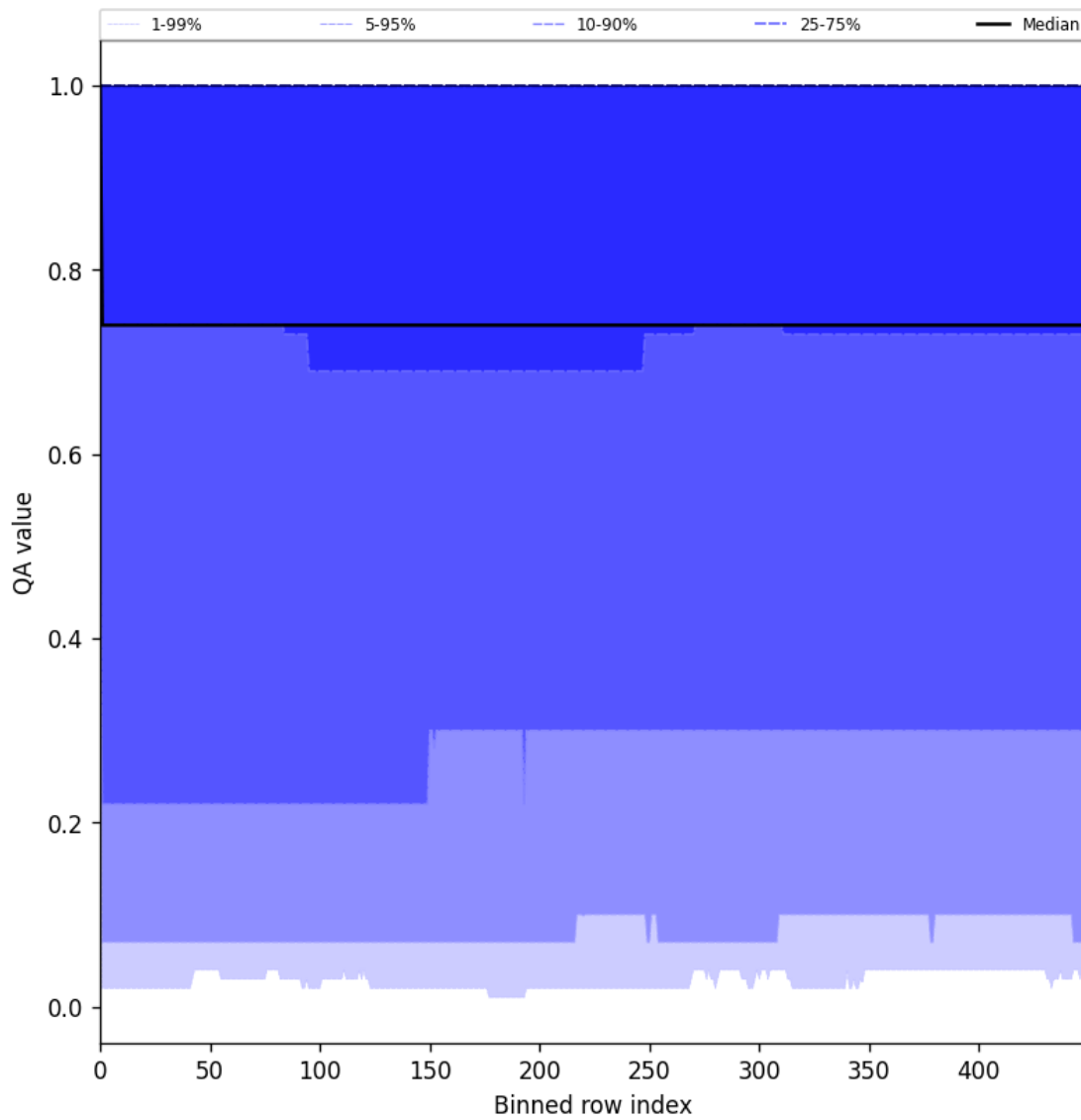
Figure 43: Along track statistics of “QA value” for 2025-07-18 to 2025-07-19
