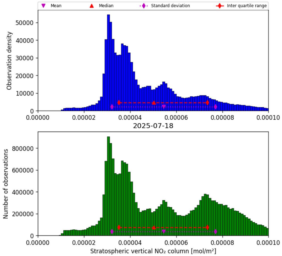
Figure 34: Histogram of “Stratospheric vertical NO 2 column” for 2025-07-18 to 2025-07-19
