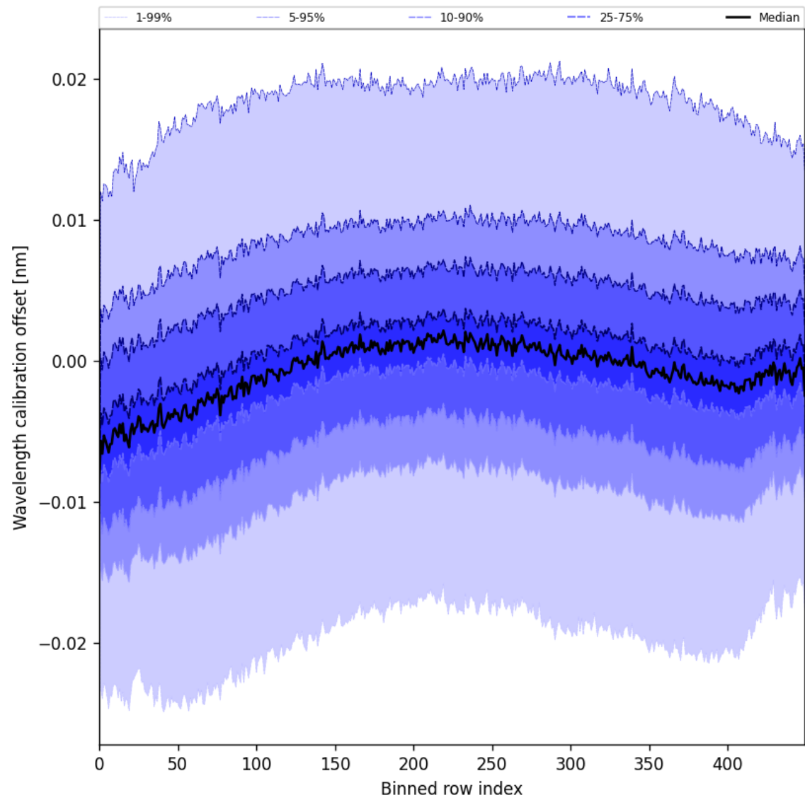
Figure 50: Along track statistics of “Wavelength calibration offset” for 2025-07-18 to 2025-07-19
