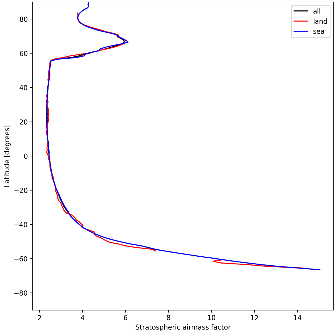
Figure 25: Zonal average of “Stratospheric air mass factor” for 2025-07-18 to 2025-07-19.
