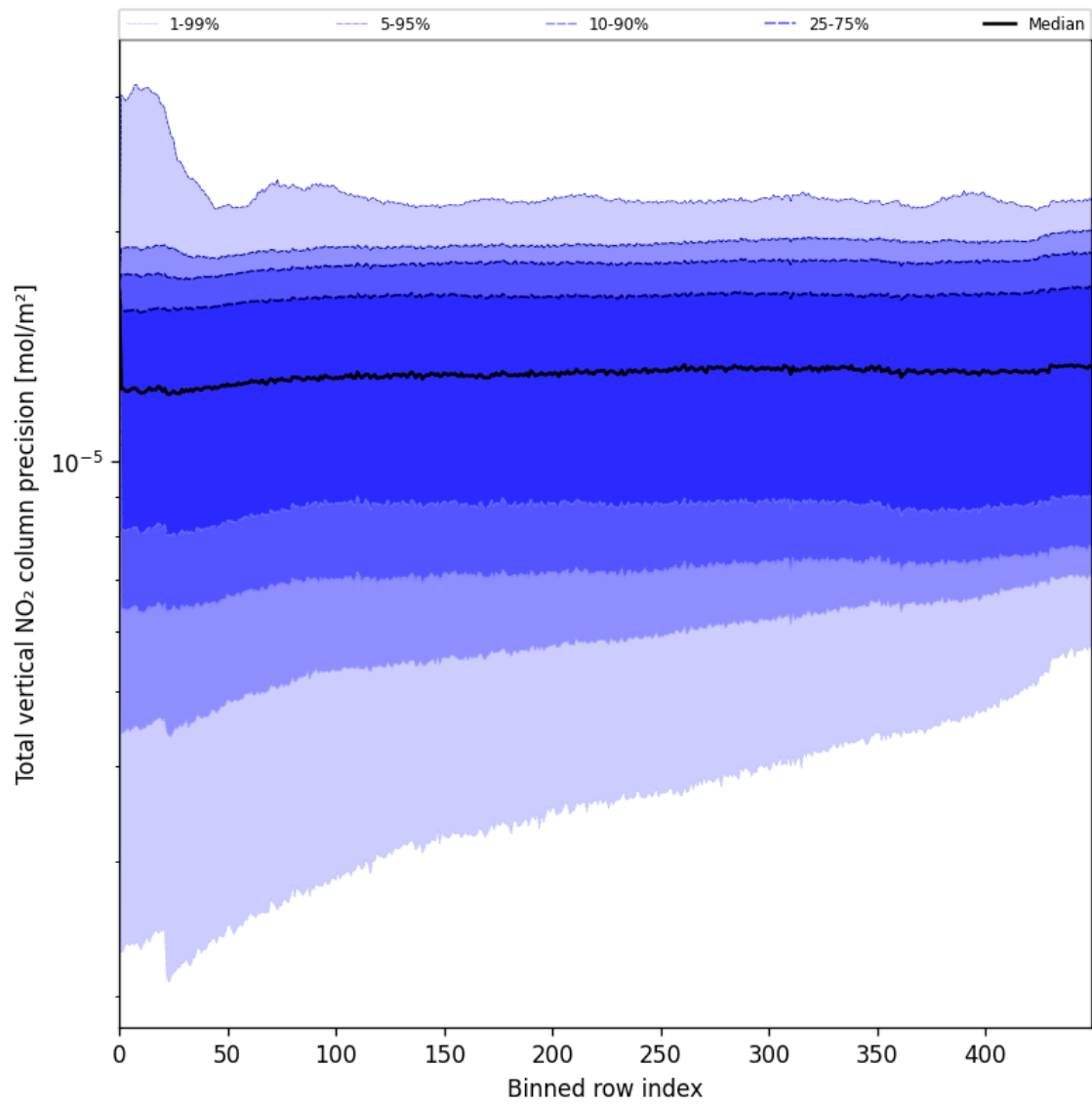
Figure 54: Along track statistics of “Total vertical NO 2 column precision” for 2025-07-18 to 2025-07-19
