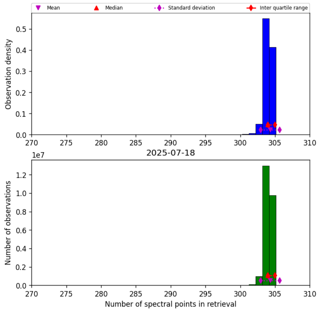
Figure 31: Histogram of “Number of spectral points in retrieval” for 2025-07-18 to 2025-07-19
