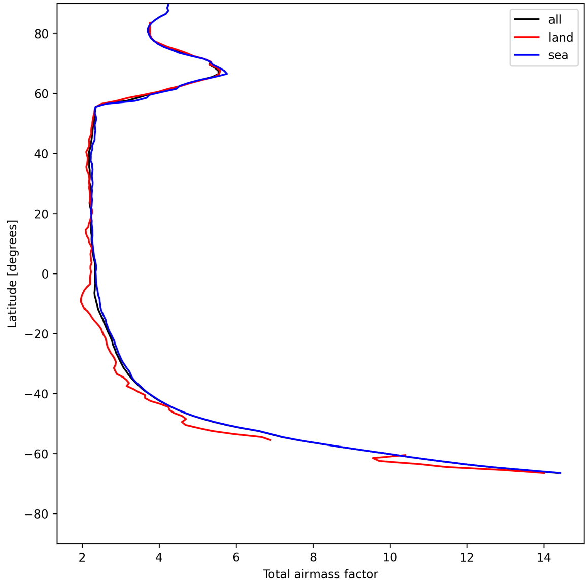
Figure 13: Zonal average of “Total airmass factor” for 2025-07-18 to 2025-07-19.
