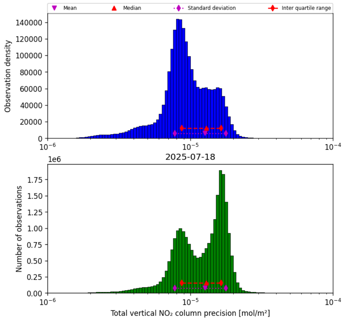
Figure 37: Histogram of “Total vertical NO 2 column precision” for 2025-07-18 to 2025-07-19
