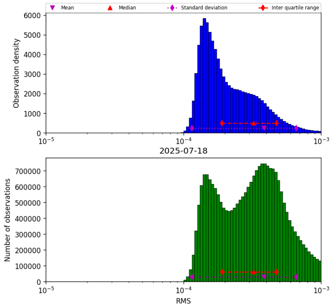
Figure 41: Histogram of “RMS” for 2025-07-18 to 2025-07-19
