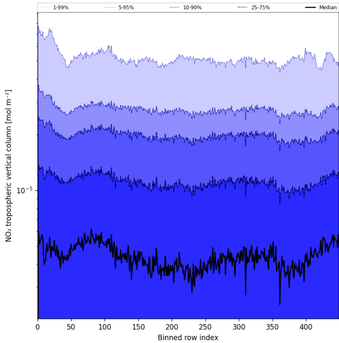
Figure 44: Along track statistics of “NO 2 tropospheric vertical column” for 2025-07-18 to 2025-07-19
