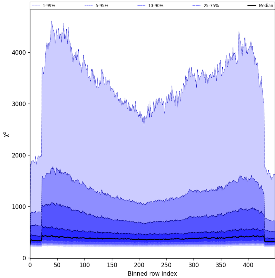
Figure 57: Along track statistics of “ \chi^2 ” for 2025-07-18 to 2025-07-19
