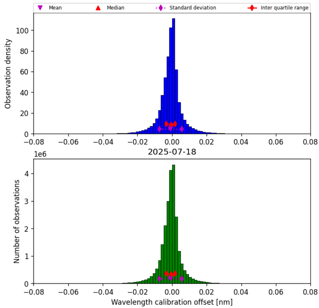
Figure 33: Histogram of “Wavelength calibration offset” for 2025-07-18 to 2025-07-19
