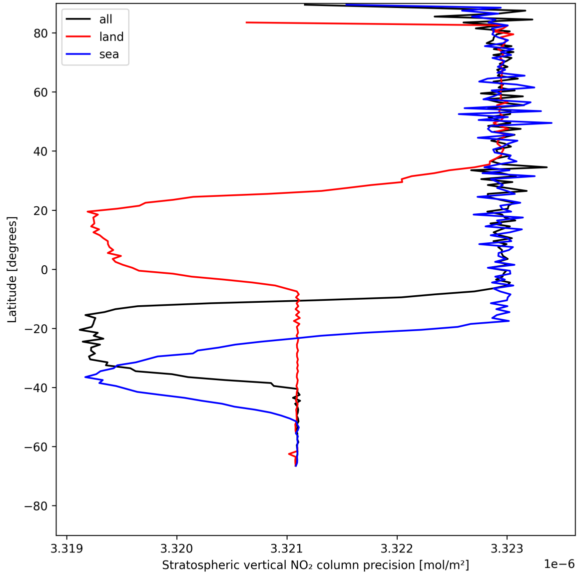
Figure 18: Zonal average of “Stratospheric vertical NO 2 column precision” for 2025-07-18 to 2025-07-19.
