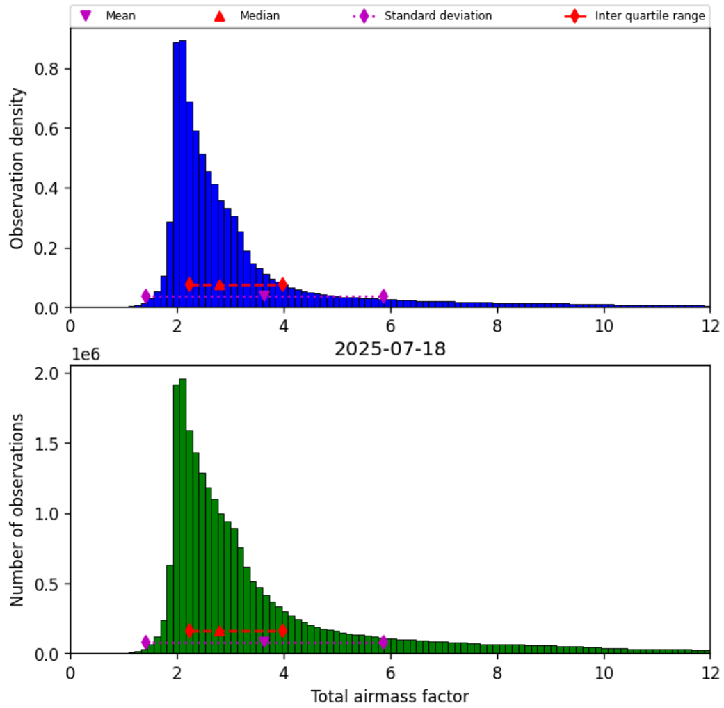
Figure 30: Histogram of “Total airmass factor” for 2025-07-18 to 2025-07-19
