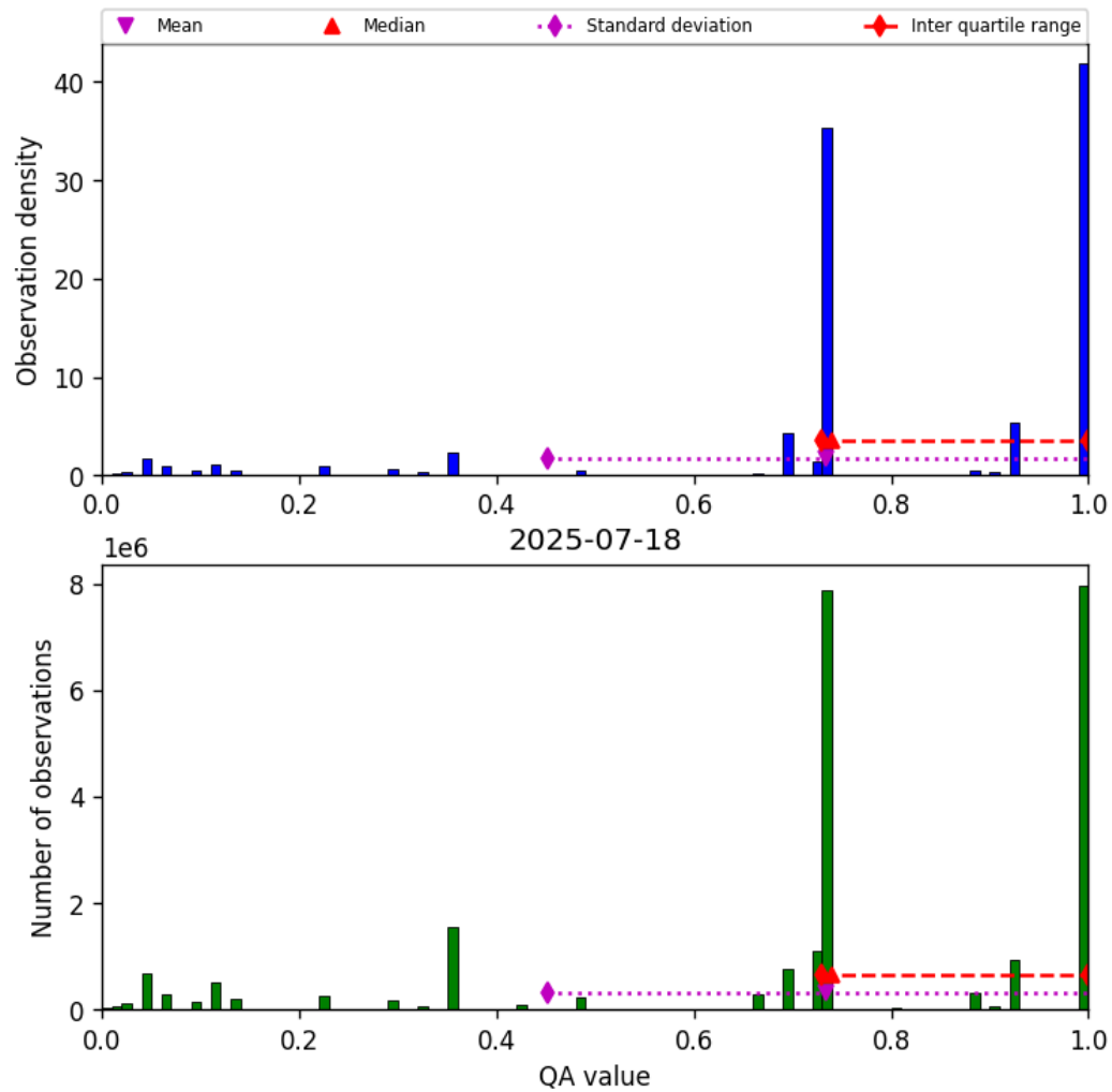
Figure 26: Histogram of “QA value” for 2025-07-18 to 2025-07-19
