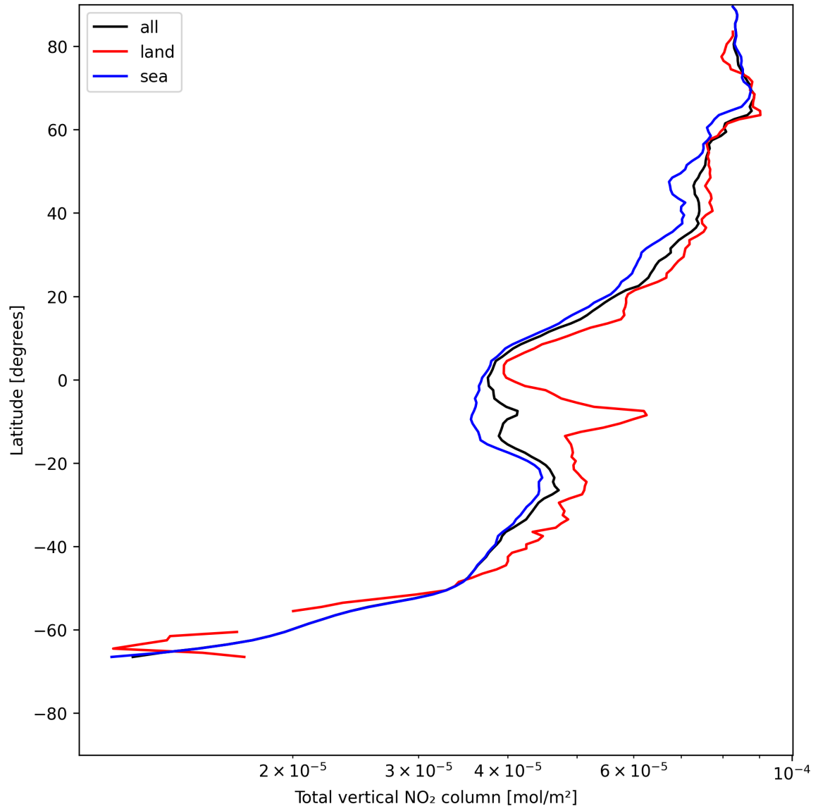
Figure 19: Zonal average of “Total vertical NO 2 column” for 2025-07-18 to 2025-07-19.
