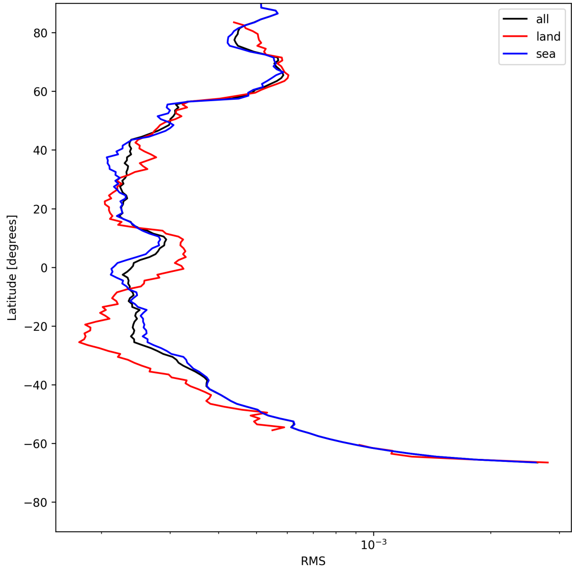
Figure 24: Zonal average of “RMS” for 2025-07-18 to 2025-07-19.
