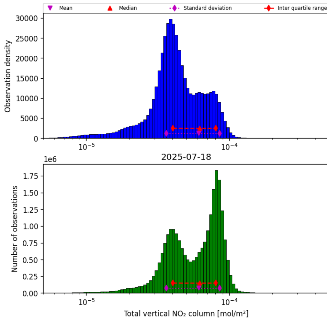
Figure 36: Histogram of “Total vertical NO 2 column” for 2025-07-18 to 2025-07-19
