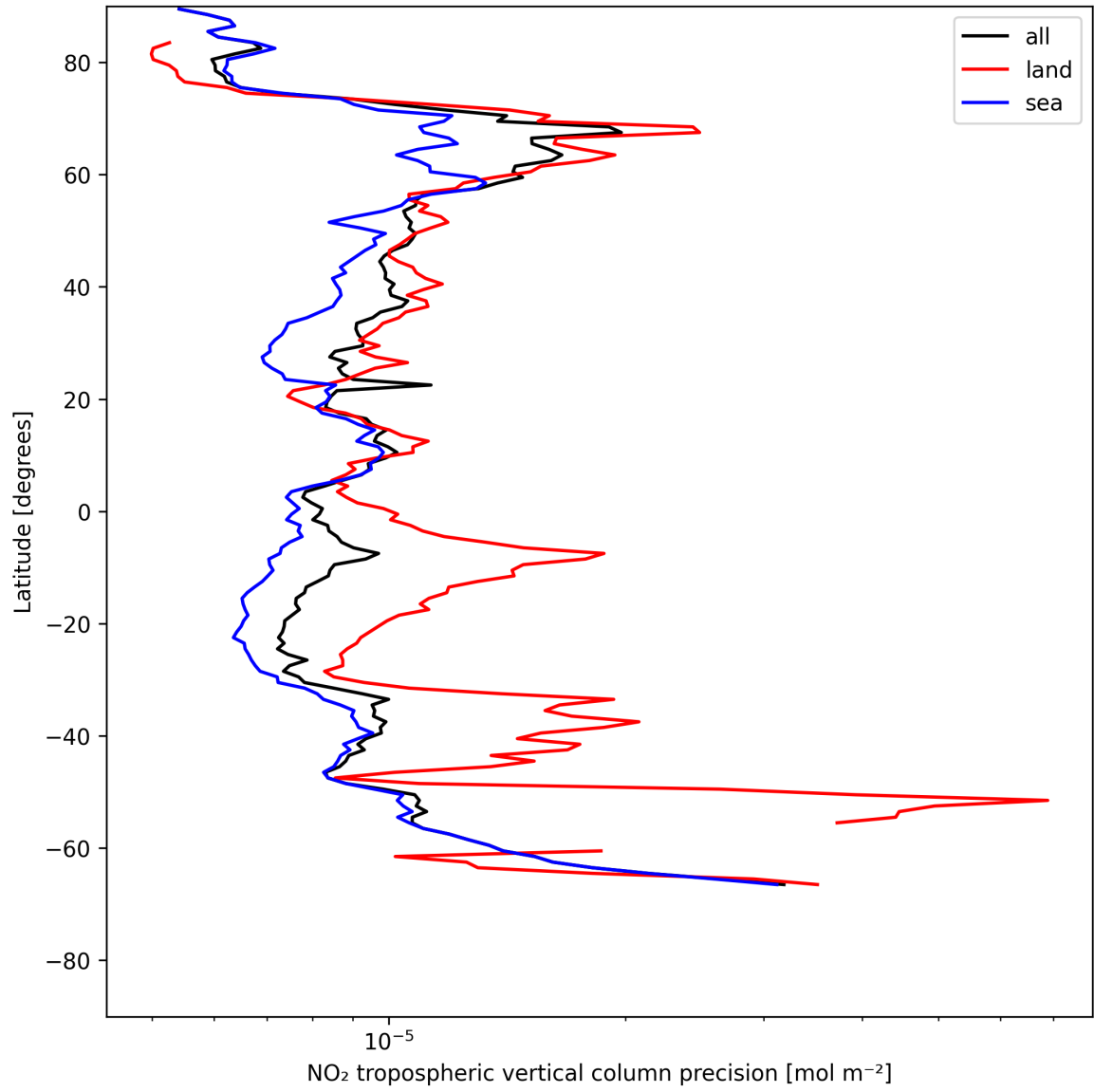
Figure 11: Zonal average of “NO 2 tropospheric vertical column precision” for 2025-07-18 to 2025-07-19.
