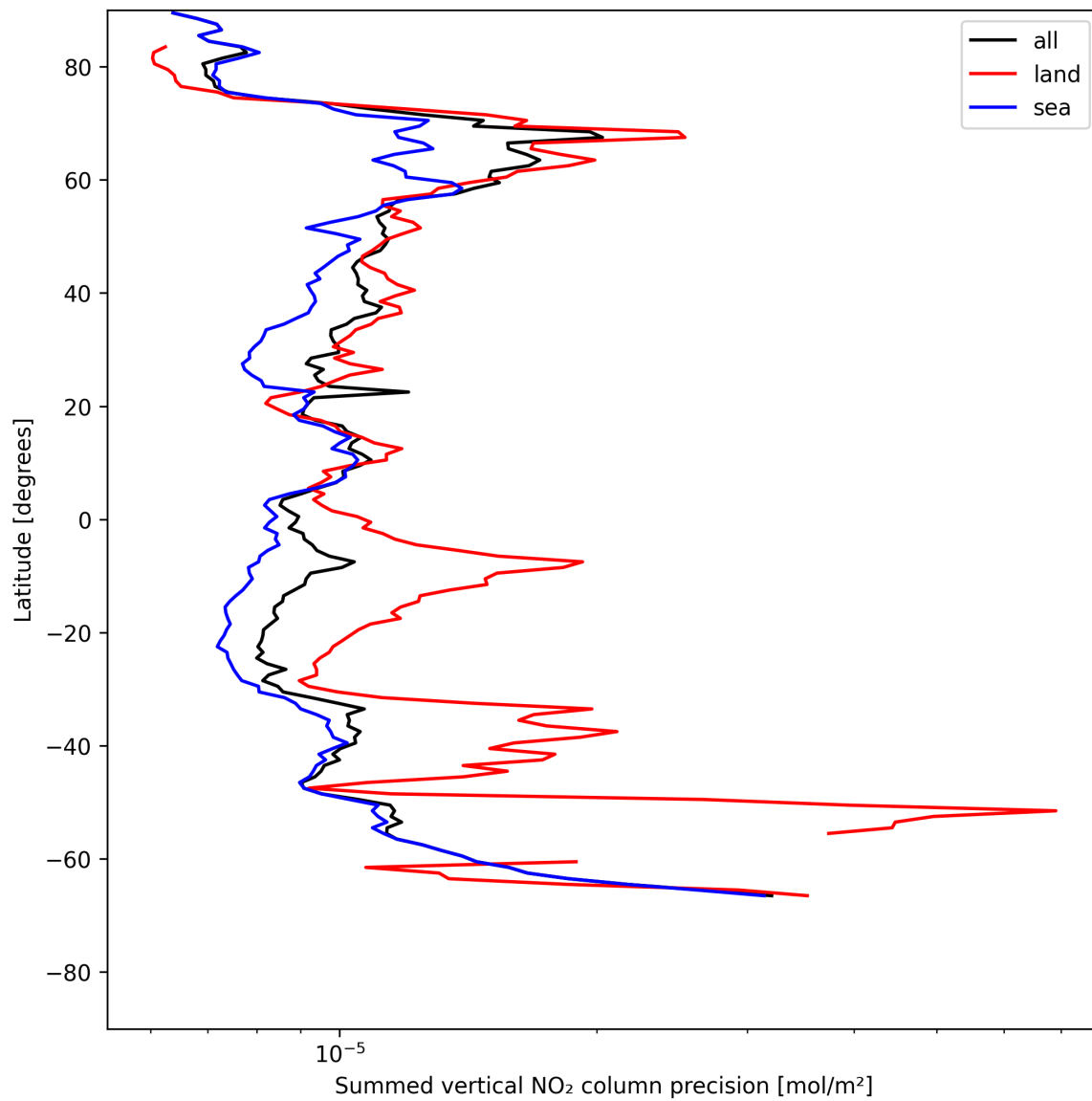
Figure 22: Zonal average of “Summed vertical NO 2 column precision” for 2025-07-18 to 2025-07-19.
