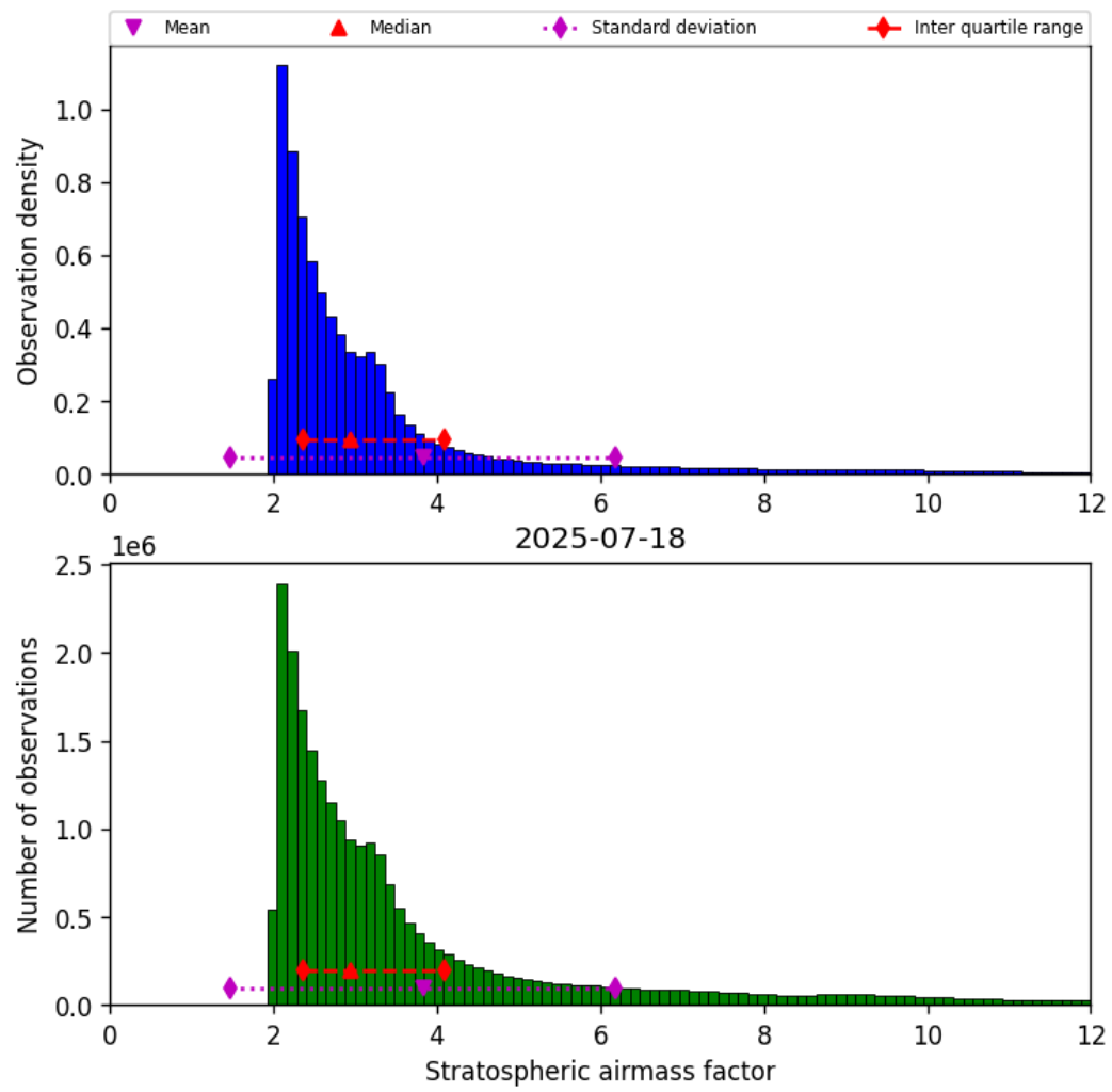
Figure 42: Histogram of “Stratospheric airmass factor” for 2025-07-18 to 2025-07-19
