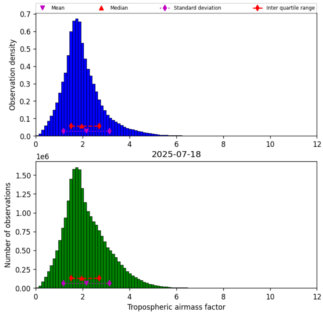
Figure 29: Histogram of “Tropospheric airmass factor” for 2025-07-18 to 2025-07-19
