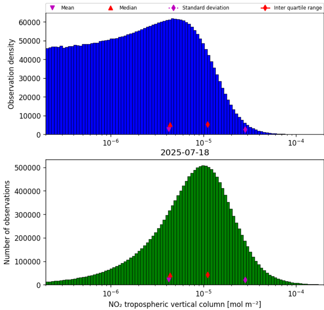
Figure 27: Histogram of “NO 2 tropospheric vertical column” for 2025-07-18 to 2025-07-19
