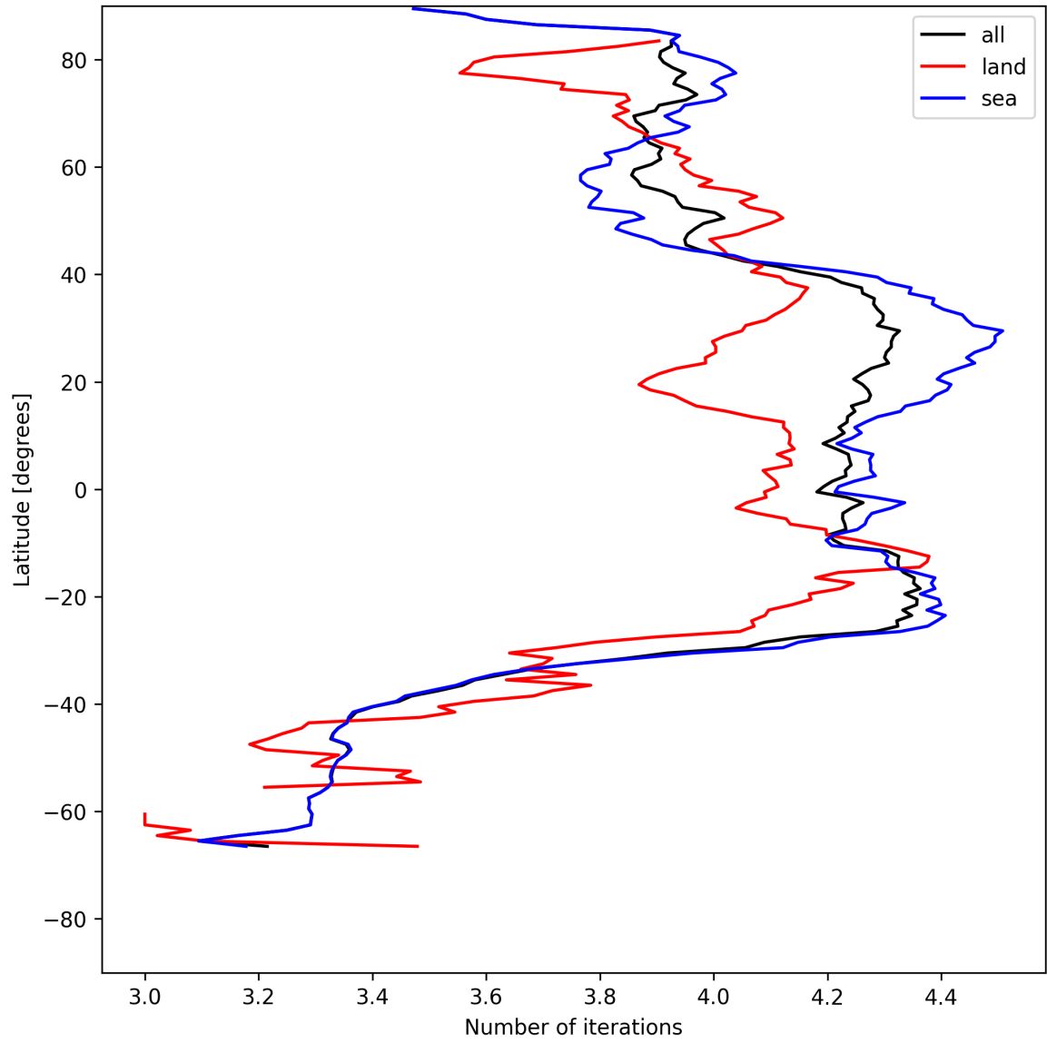
Figure 15: Zonal average of “Number of iterations” for 2025-07-18 to 2025-07-19.
