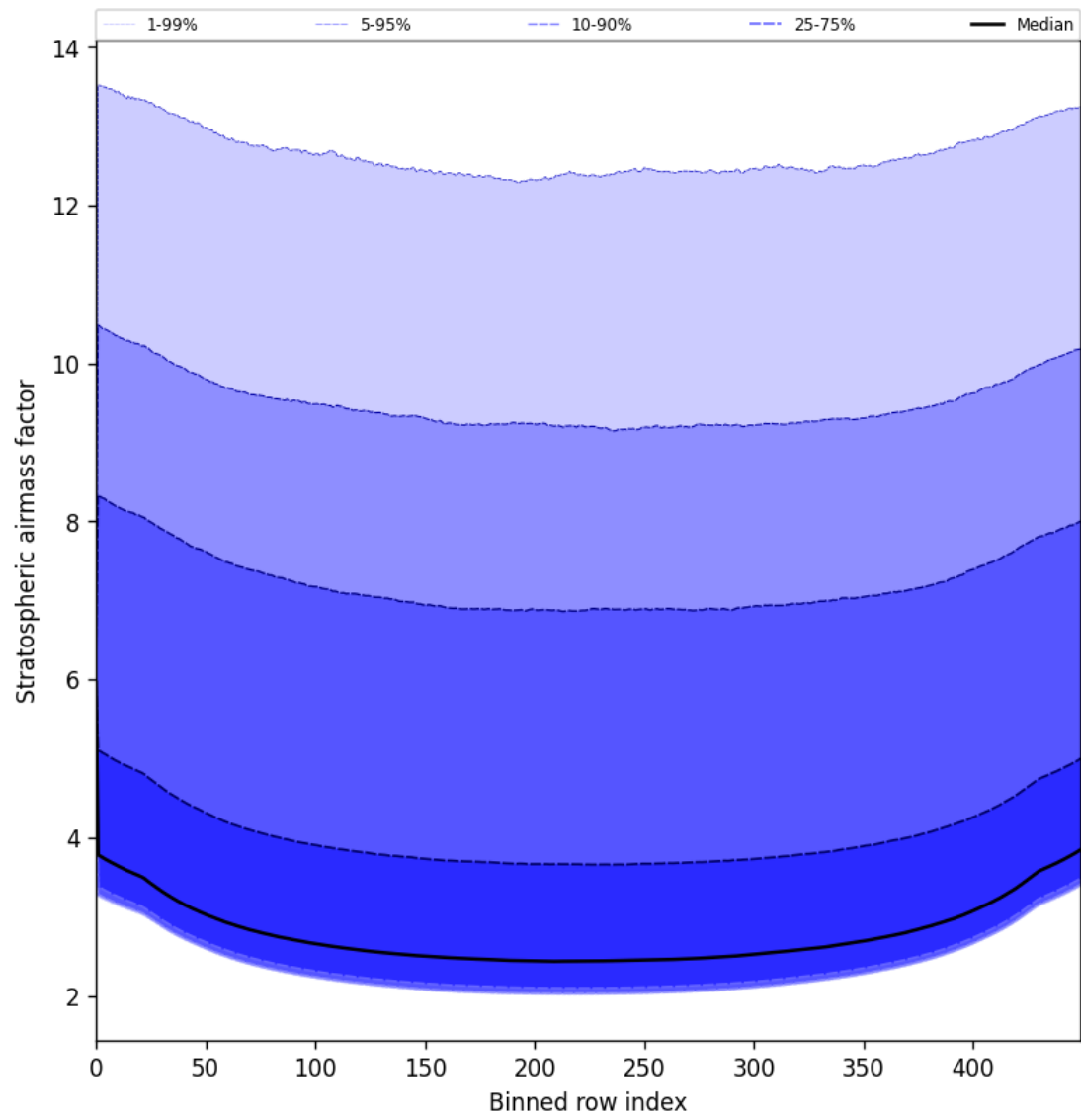
Figure 59: Along track statistics of “Stratospheric airmass factor” for 2025-07-18 to 2025-07-19
