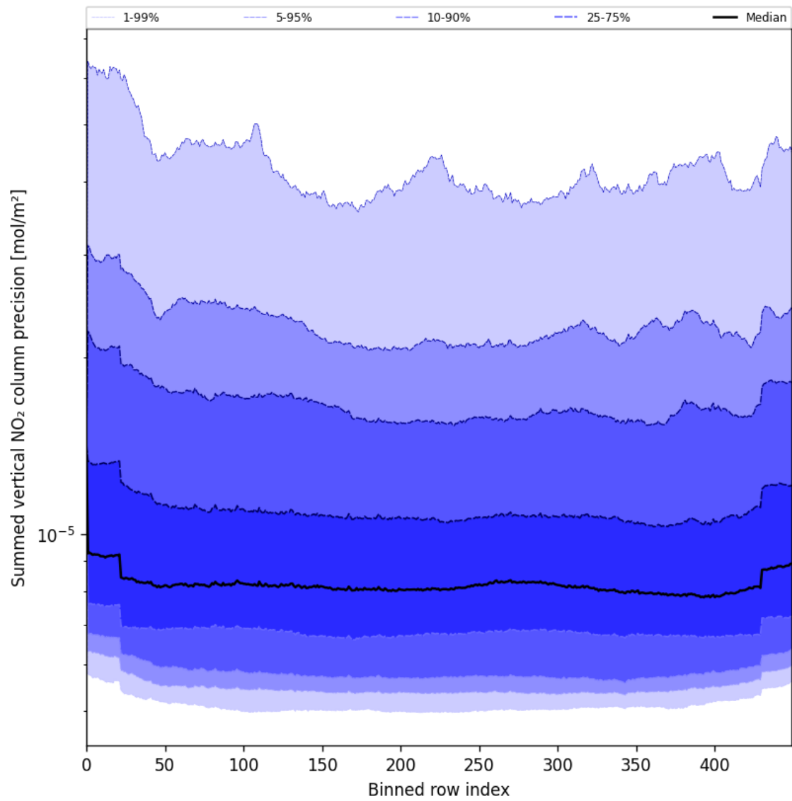
Figure 56: Along track statistics of “Summed vertical NO 2 column precision” for 2025-07-18 to 2025-07-19
