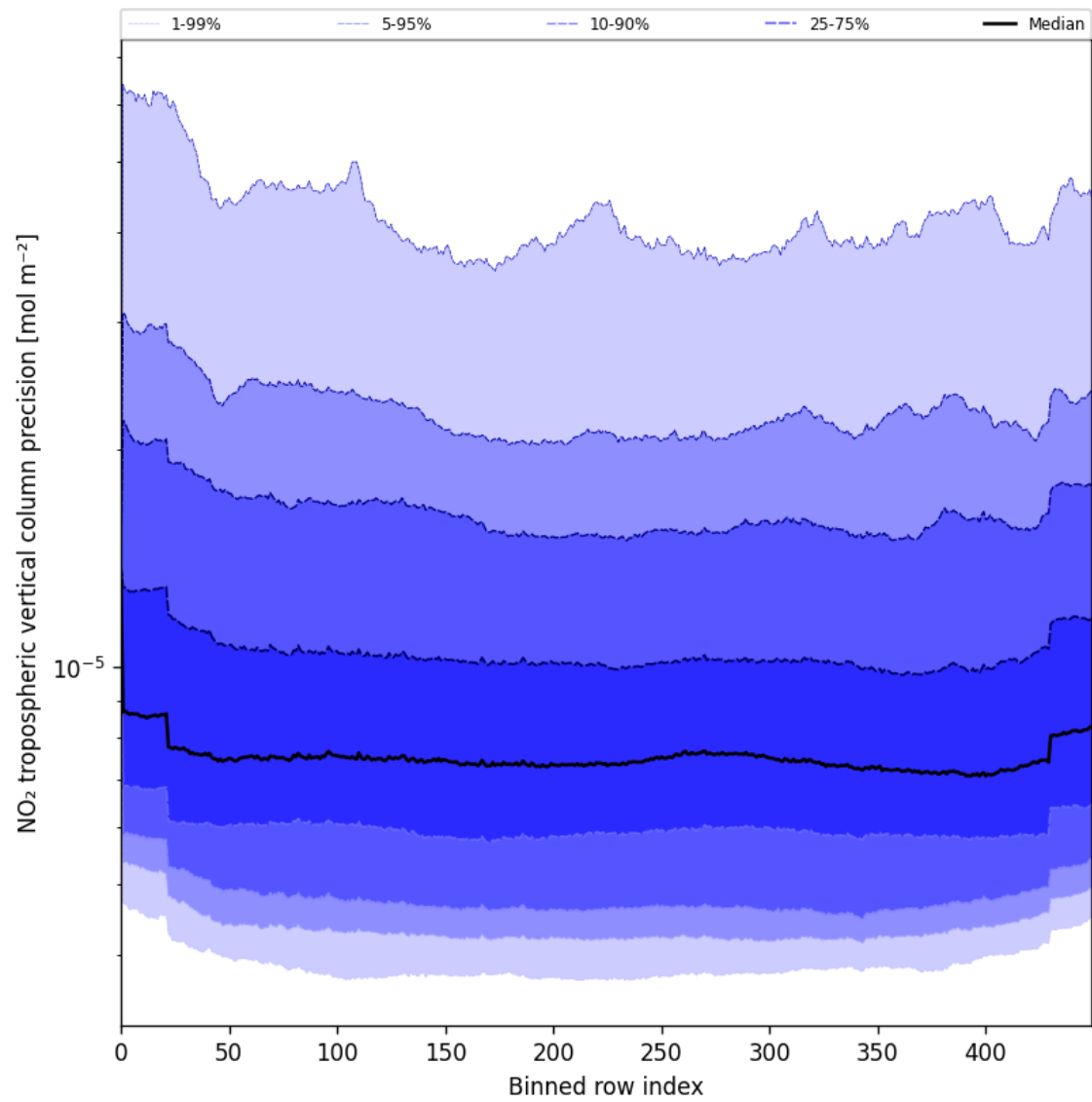
Figure 45: Along track statistics of “NO 2 tropospheric vertical column precision” for 2025-07-18 to 2025-07-19
