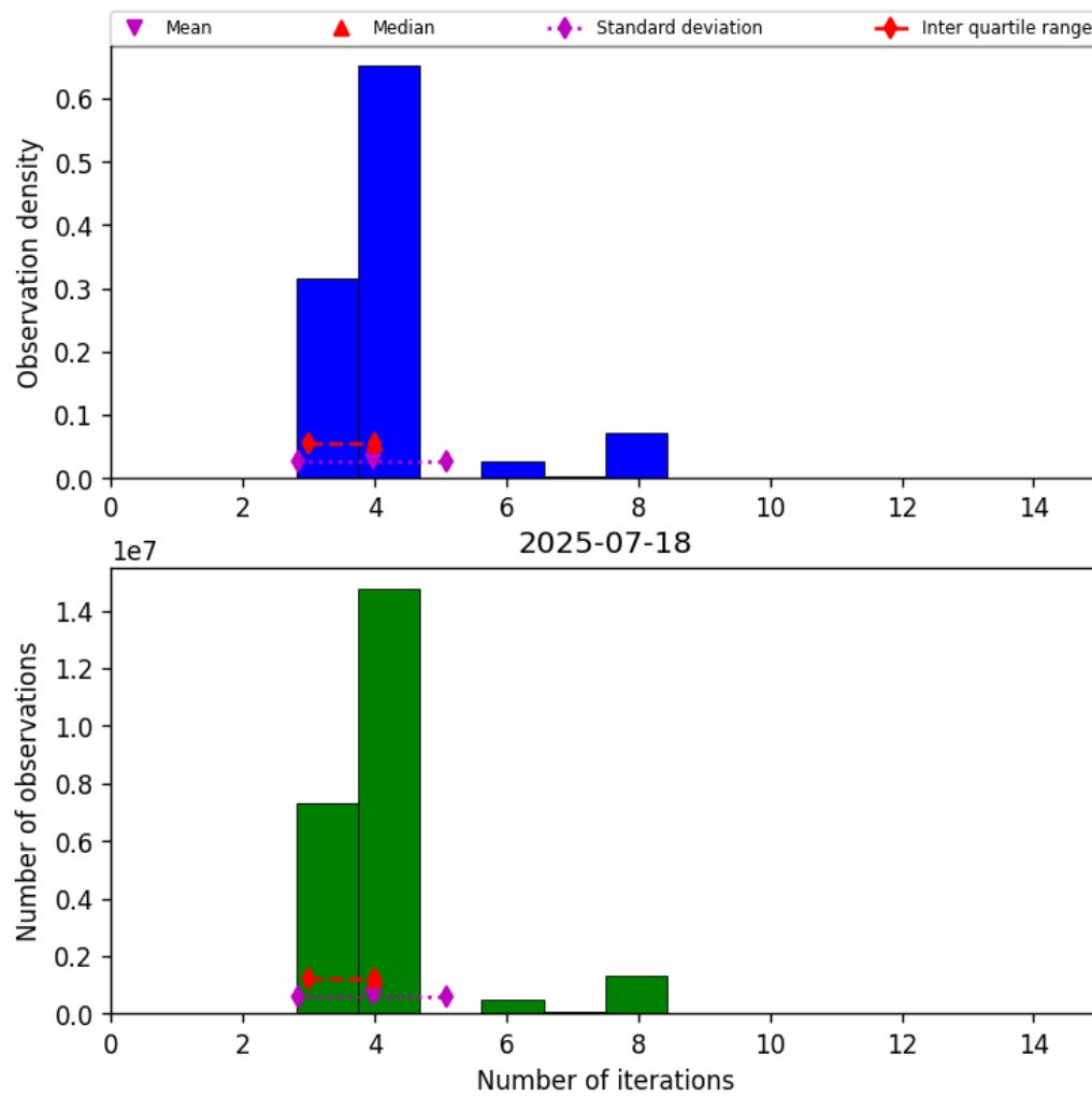
Figure 32: Histogram of “Number of iterations” for 2025-07-18 to 2025-07-19
