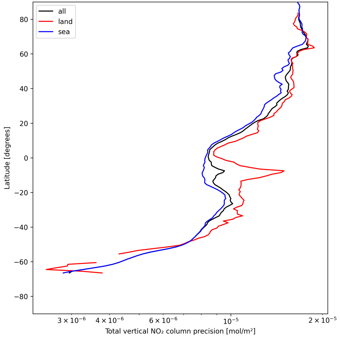
Figure 20: Zonal average of “Total vertical NO 2 column precision” for 2025-07-18 to 2025-07-19.
