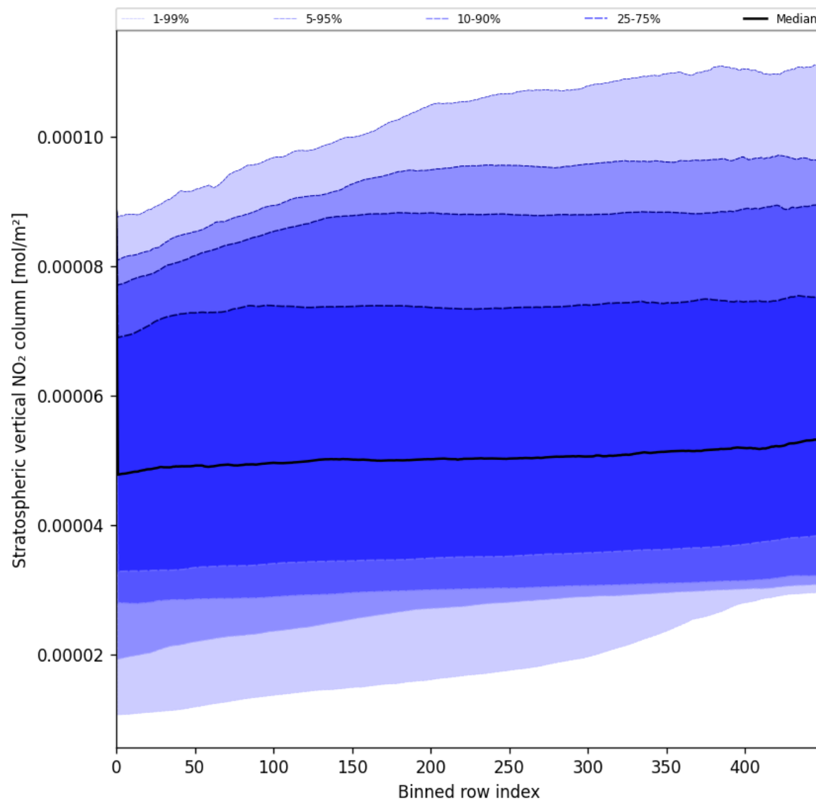
Figure 51: Along track statistics of “Stratospheric vertical NO 2 column” for 2025-07-18 to 2025-07-19
