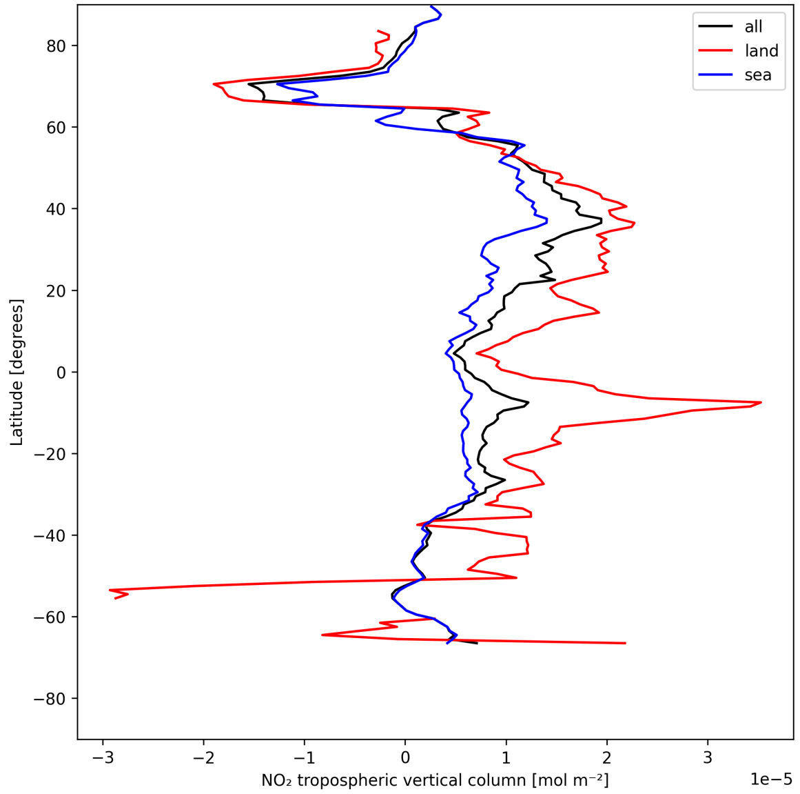
Figure 10: Zonal average of “NO 2 tropospheric vertical column” for 2025-07-18 to 2025-07-19.
