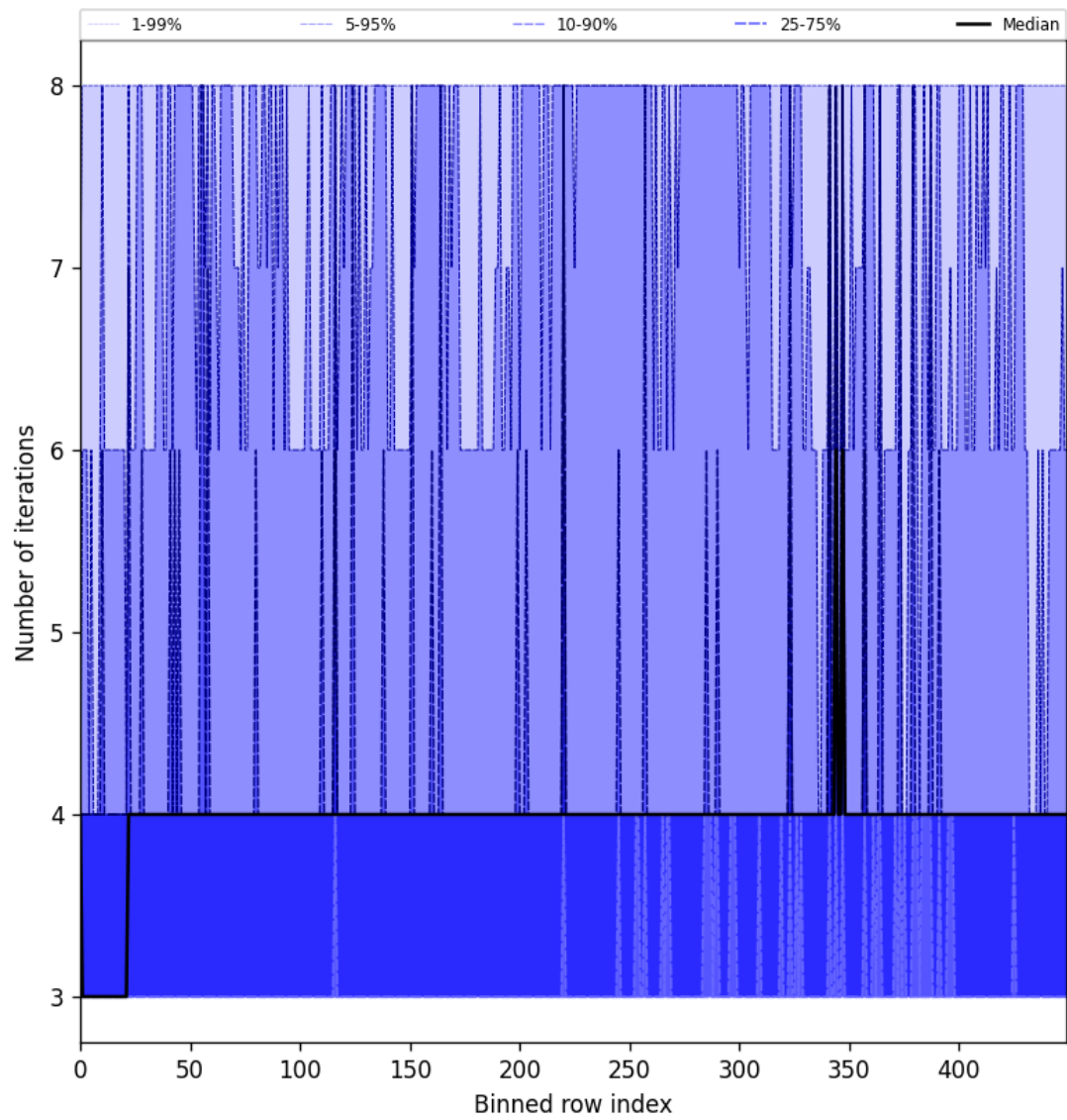
Figure 49: Along track statistics of “Number of iterations” for 2025-07-18 to 2025-07-19
