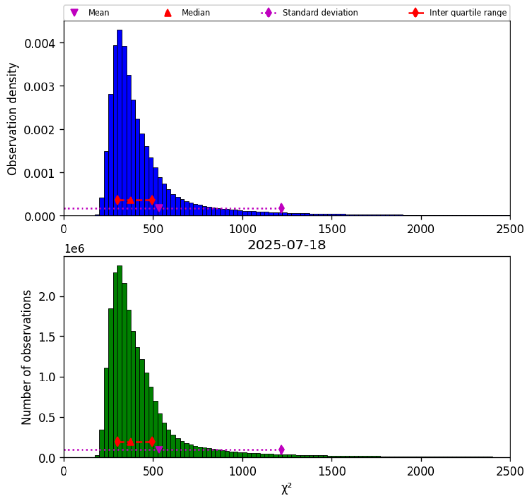
Figure 40: Histogram of “ \chi^2 ” for 2025-07-18 to 2025-07-19
