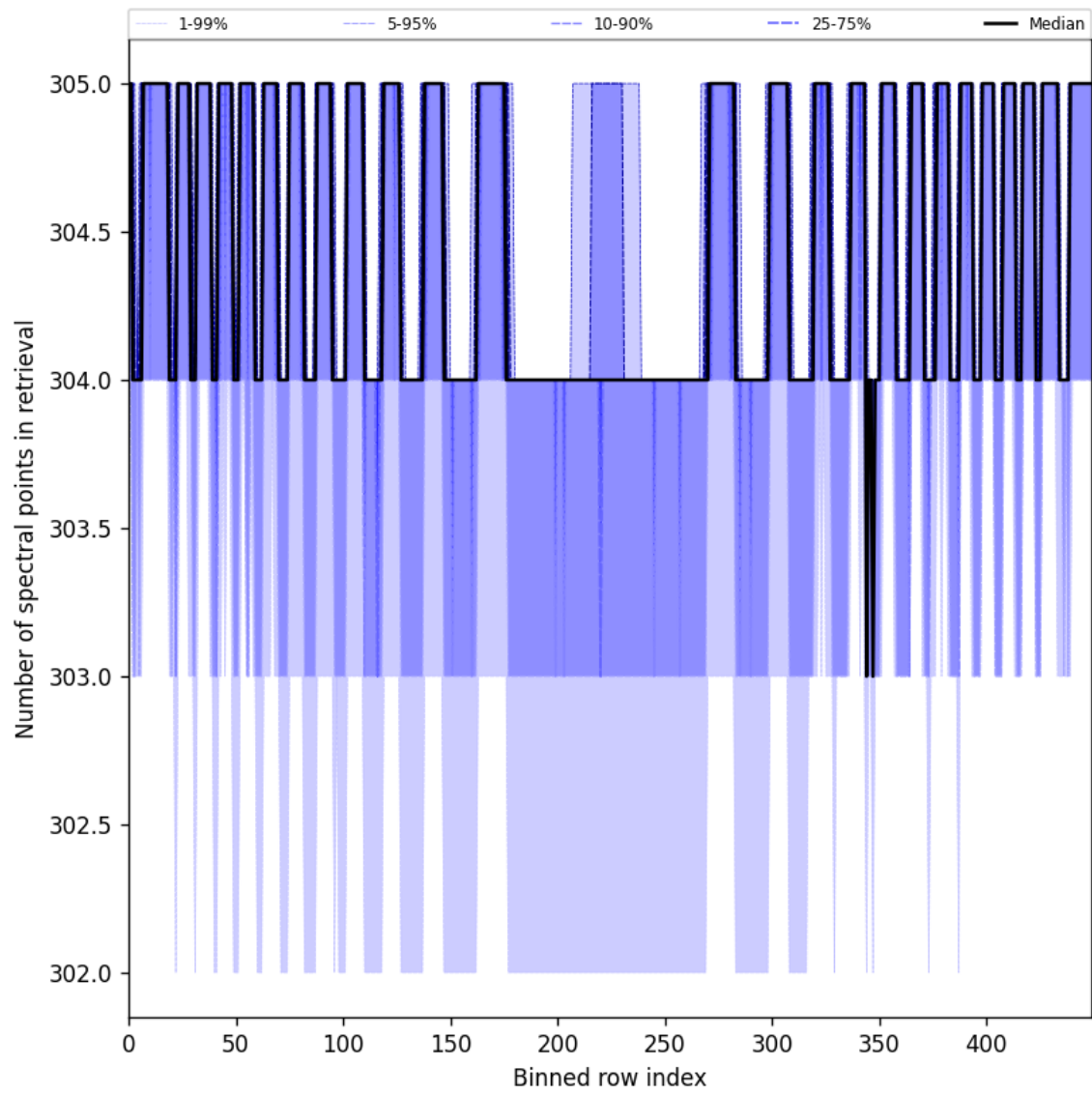
Figure 48: Along track statistics of “Number of spectral points in retrieval” for 2025-07-18 to 2025-07-19
