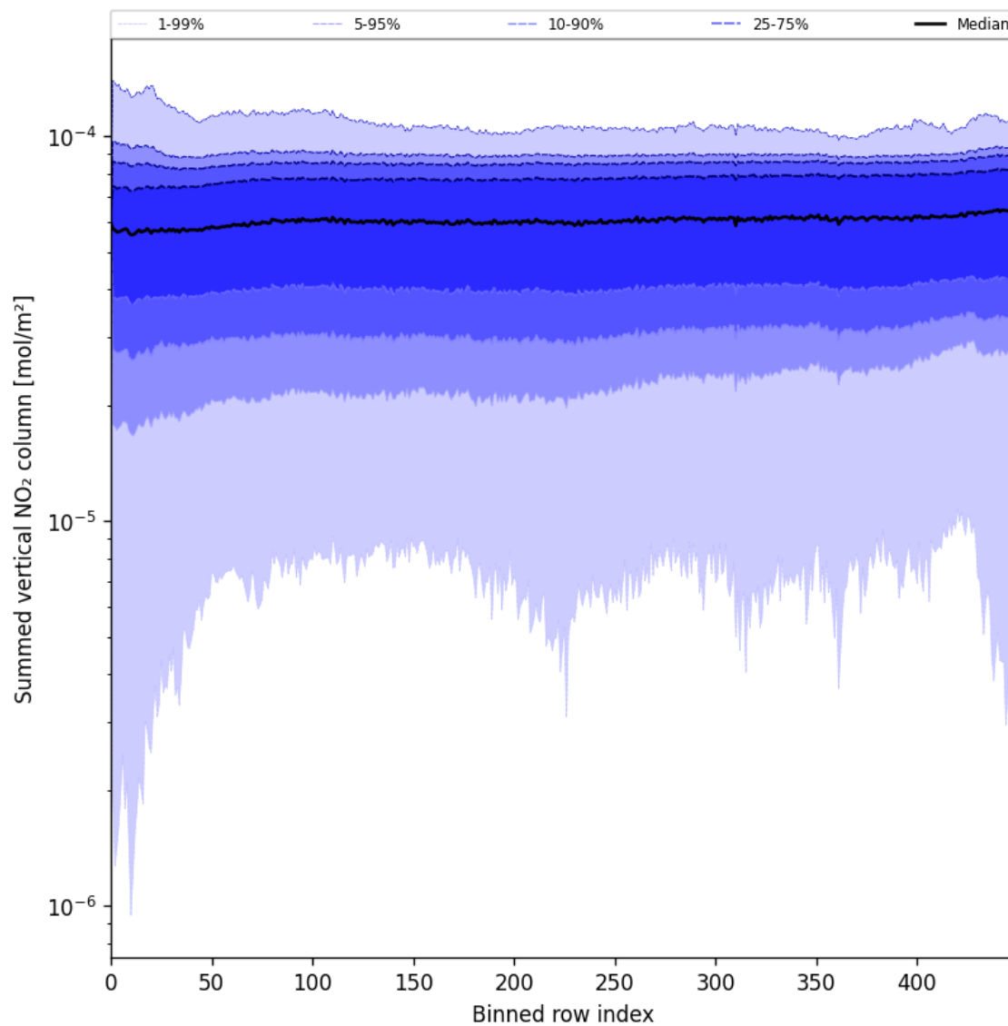
Figure 55: Along track statistics of “Summed vertical NO 2 column” for 2025-07-18 to 2025-07-19
