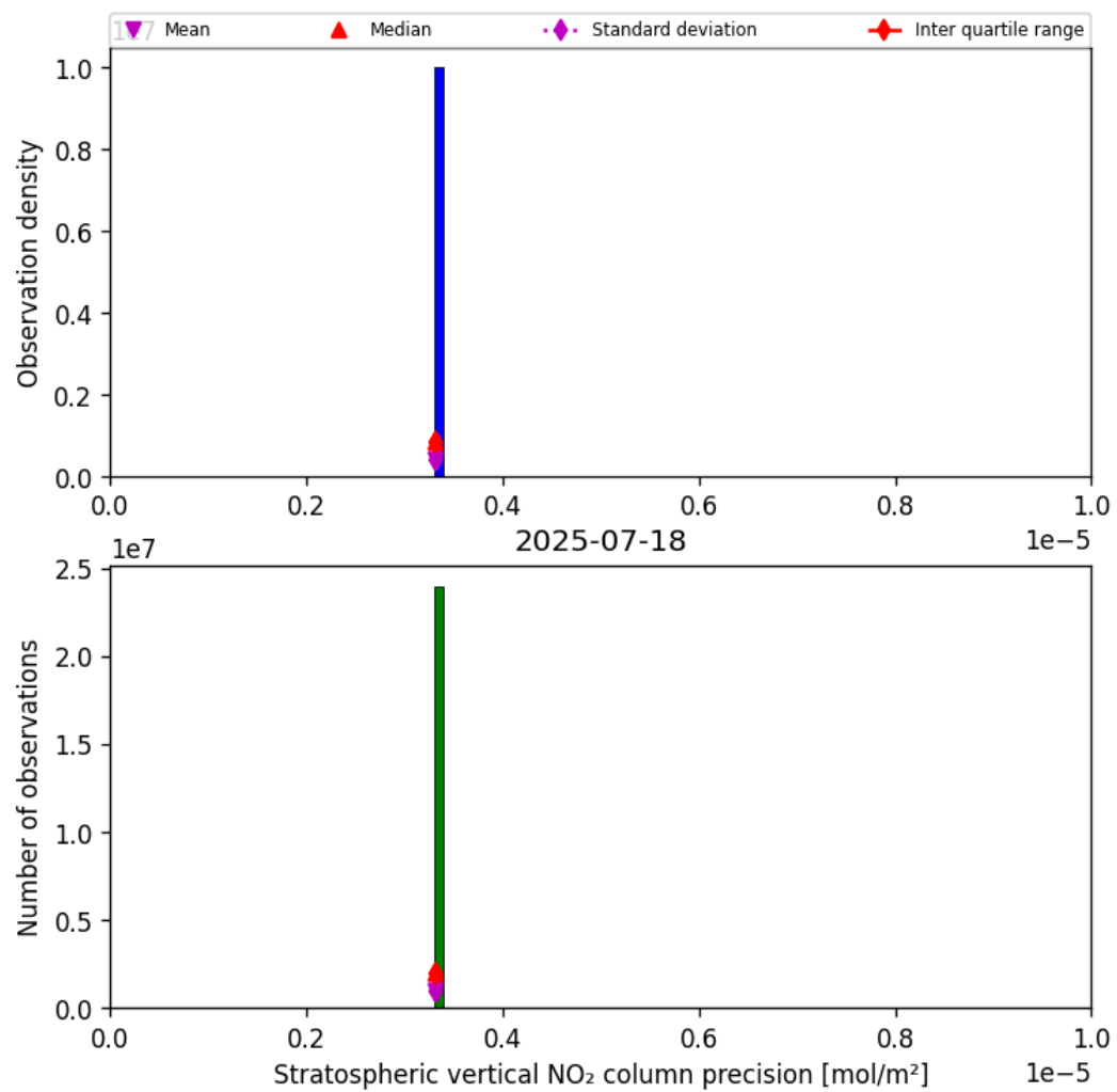
Figure 35: Histogram of “Stratospheric vertical NO 2 column precision” for 2025-07-18 to 2025-07-19
