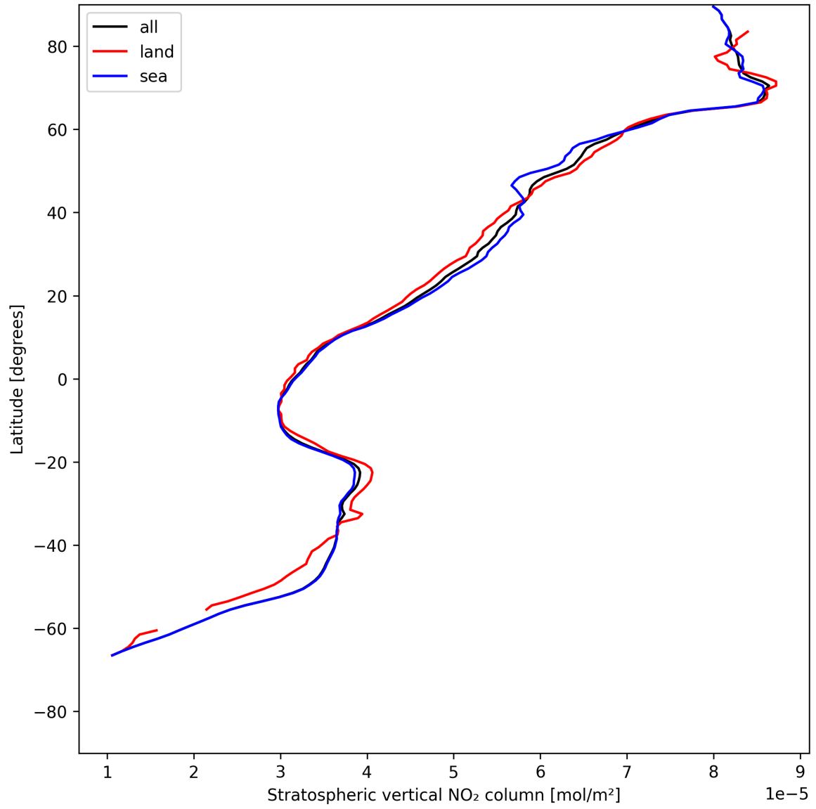
Figure 17: Zonal average of “Stratospheric vertical NO 2 column” for 2025-07-18 to 2025-07-19.
