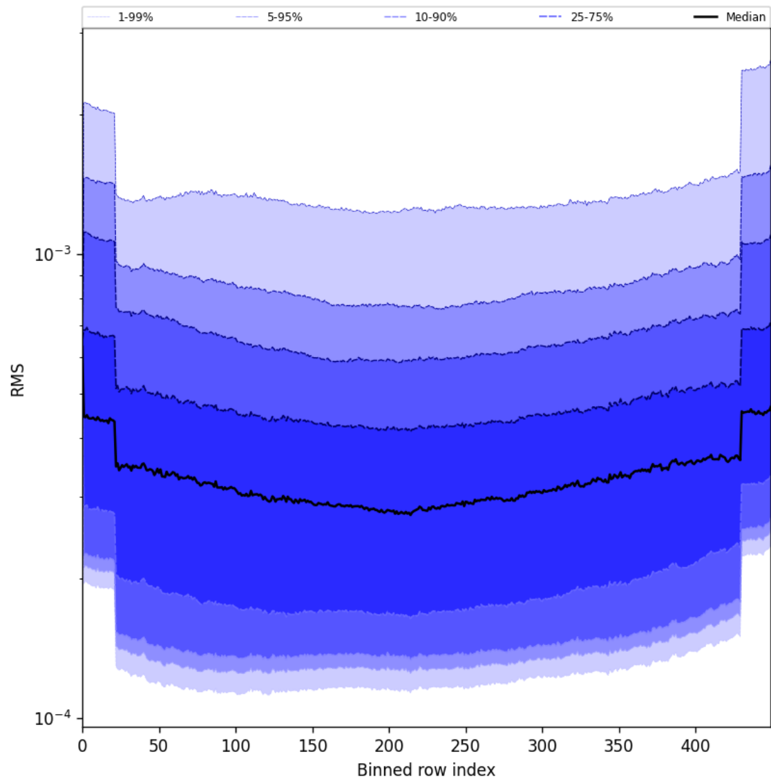
Figure 58: Along track statistics of “RMS” for 2025-07-18 to 2025-07-19
