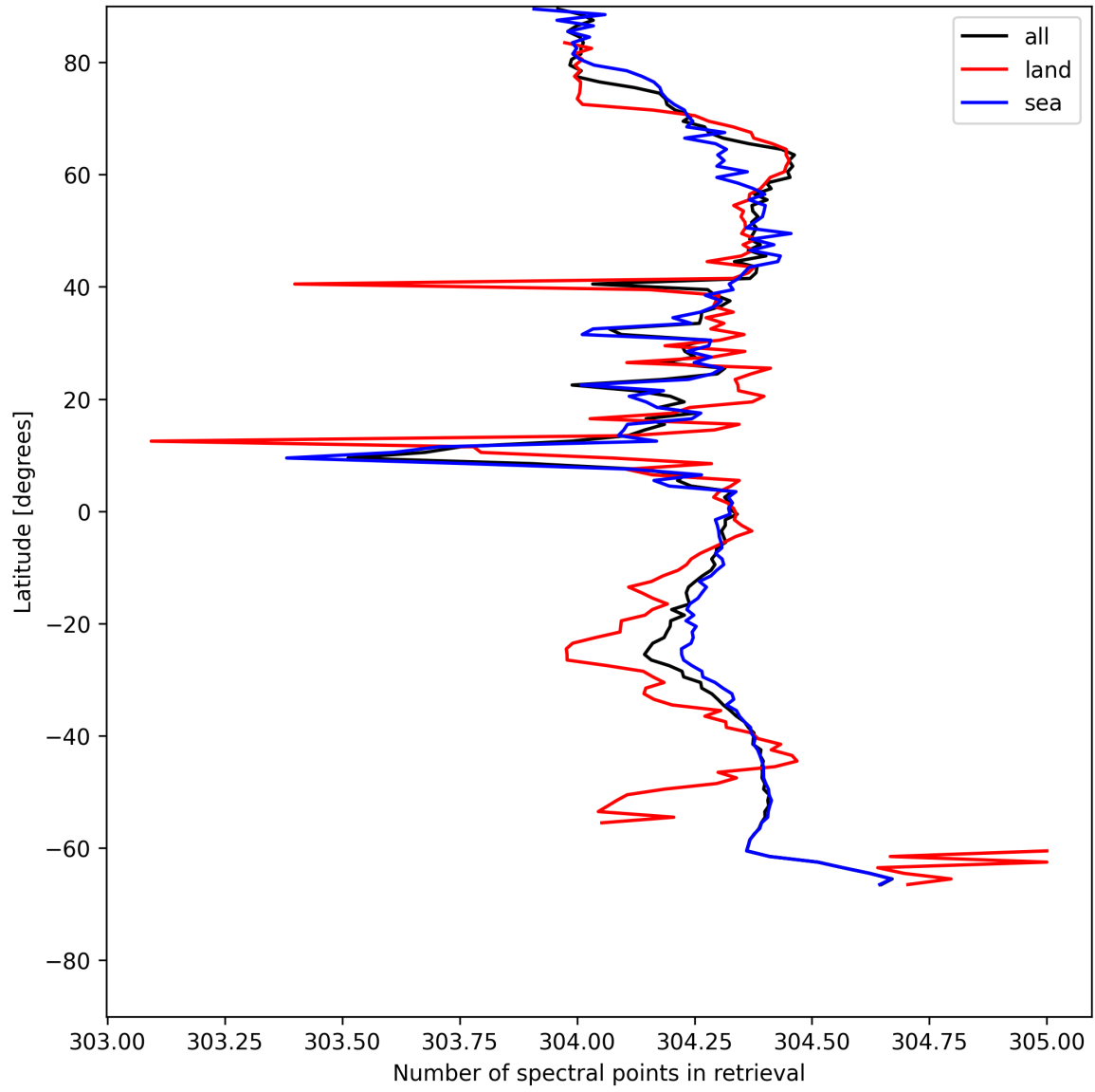
Figure 14: Zonal average of “Number of spectral points in retrieval” for 2025-07-18 to 2025-07-19.
