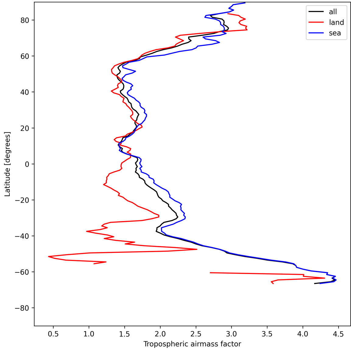
Figure 12: Zonal average of “Tropospheric airmass factor” for 2025-07-18 to 2025-07-19.
