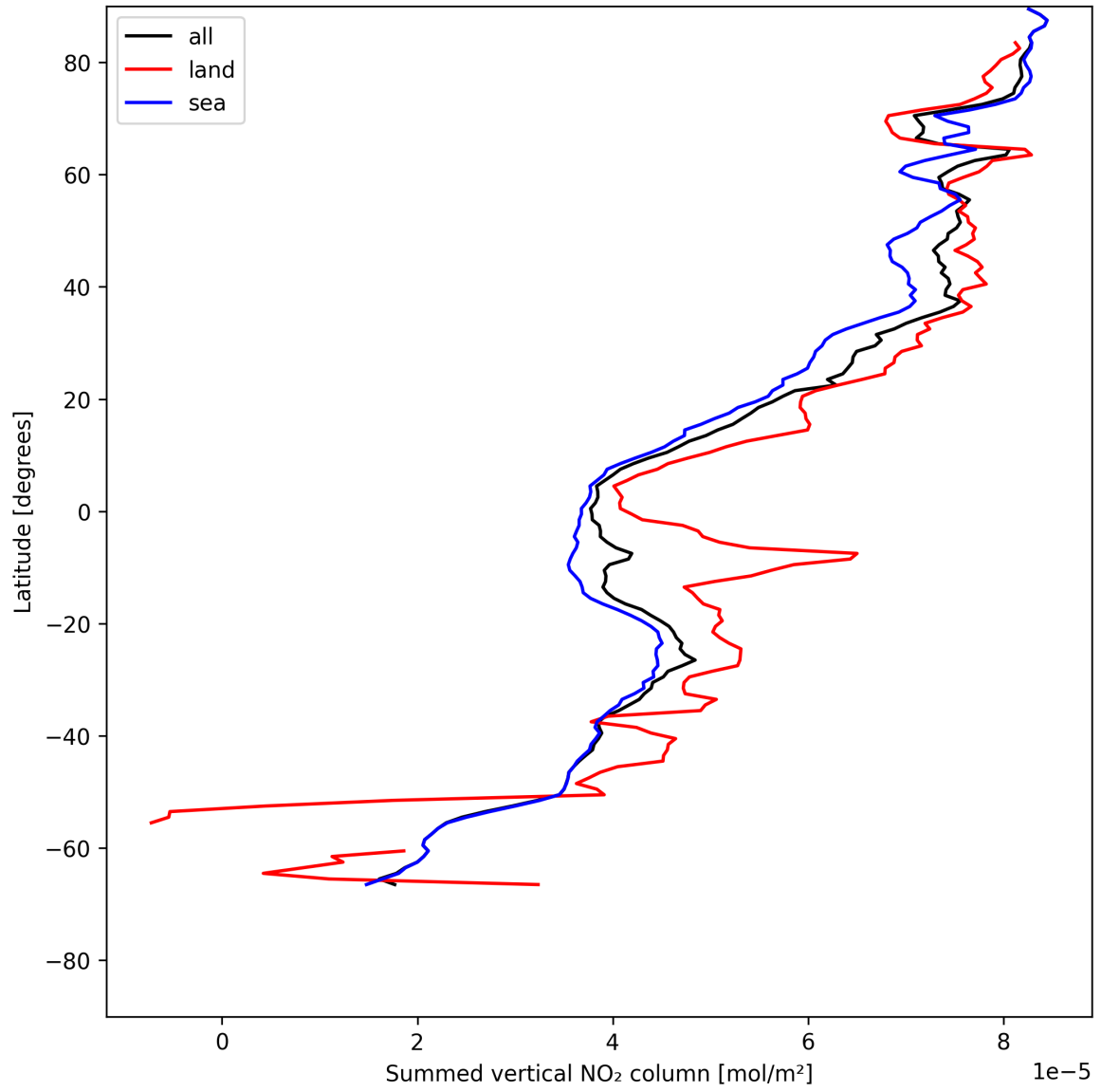
Figure 21: Zonal average of “Summed vertical NO 2 column” for 2025-07-18 to 2025-07-19.
