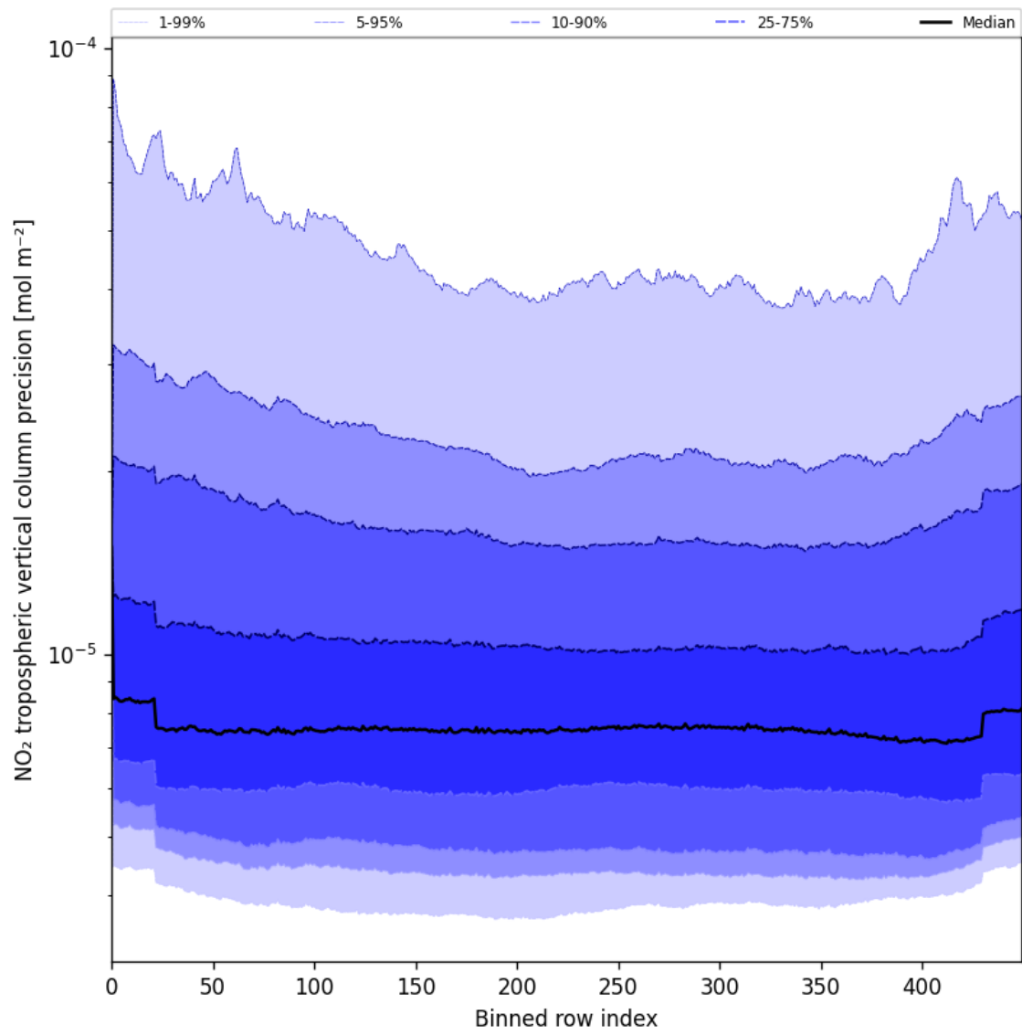
Figure 45: Along track statistics of "NO 2 tropospheric vertical column precision" for 2025-07-19 to 2025-07-20
