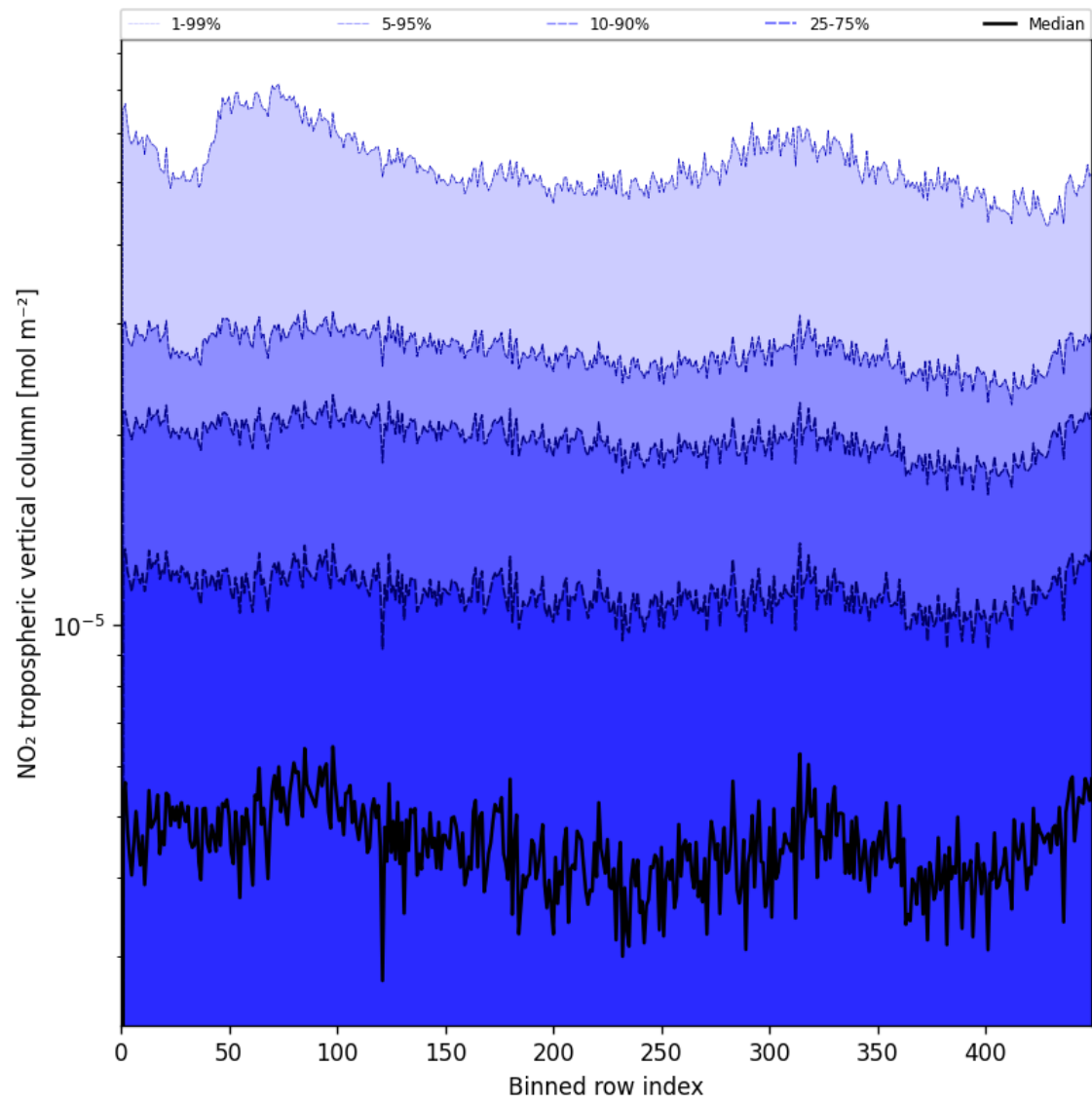
Figure 44: Along track statistics of “NO 2 tropospheric vertical column” for 2025-07-19 to 2025-07-20
