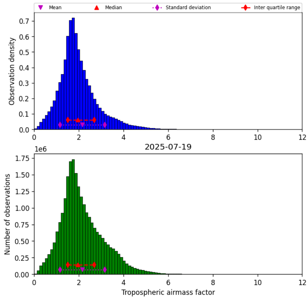
Figure 29: Histogram of “Tropospheric airmass factor” for 2025-07-19 to 2025-07-20
