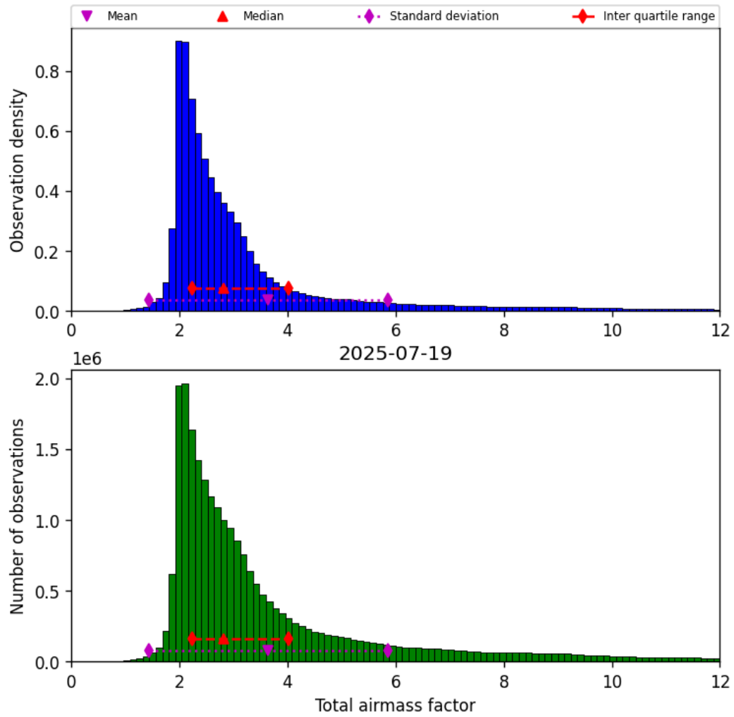
Figure 30: Histogram of “Total airmass factor” for 2025-07-19 to 2025-07-20
