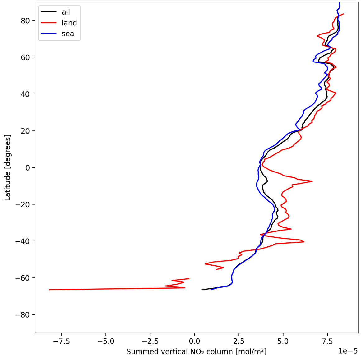
Figure 21: Zonal average of “Summed vertical NO 2 column” for 2025-07-19 to 2025-07-20.
