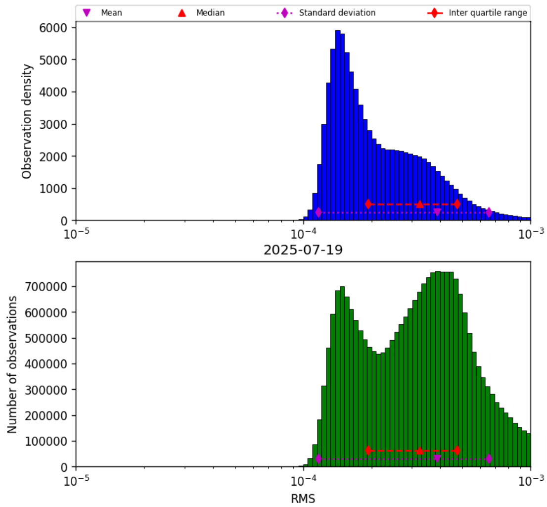
Figure 41: Histogram of “RMS” for 2025-07-19 to 2025-07-20
