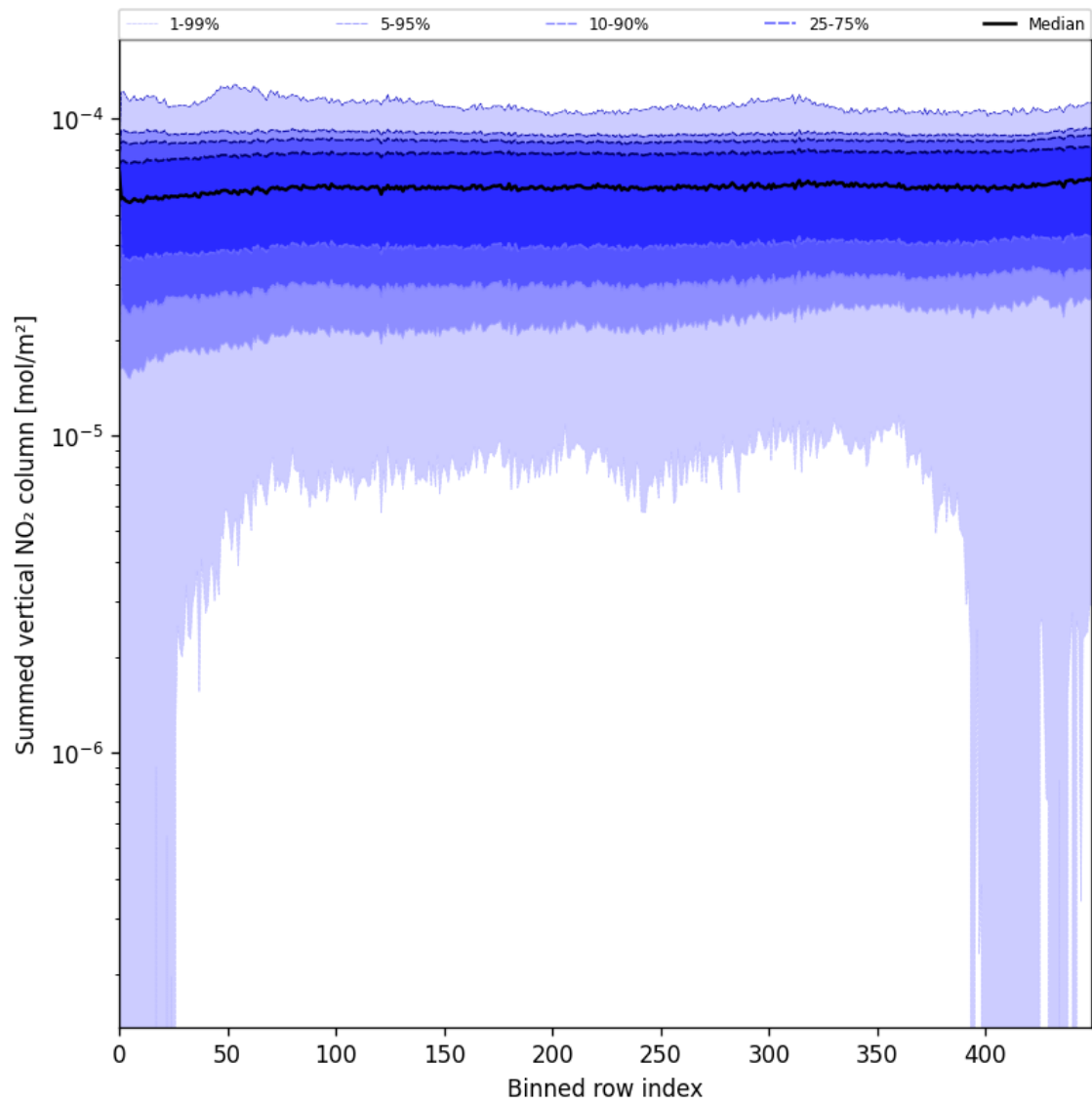
Figure 55: Along track statistics of “Summed vertical NO 2 column” for 2025-07-19 to 2025-07-20
