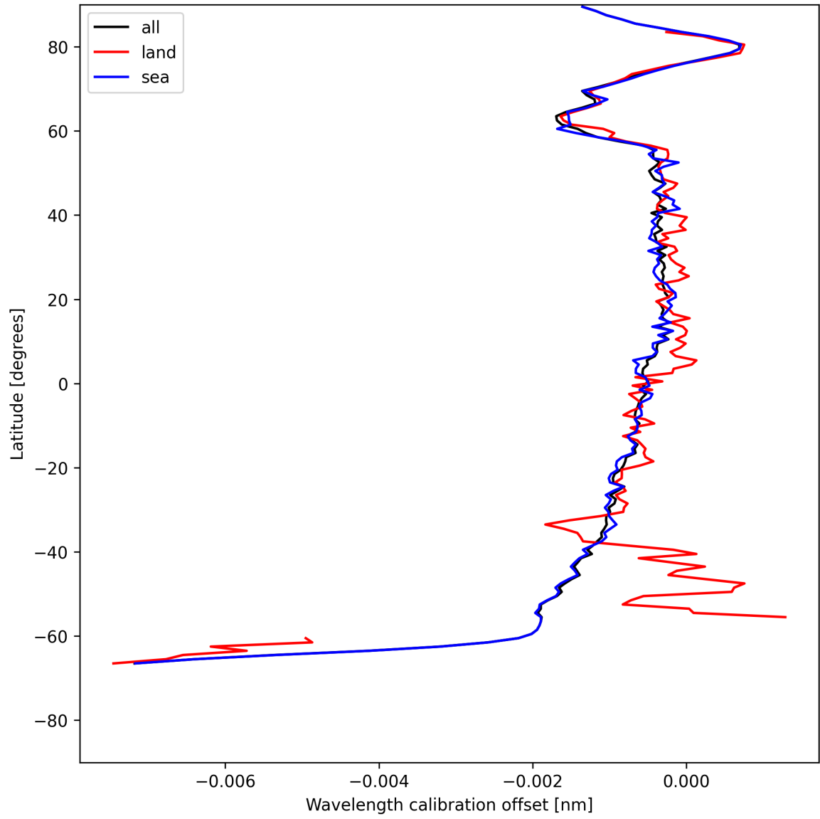
Figure 16: Zonal average of “Wavelength calibration offset” for 2025-07-19 to 2025-07-20.
