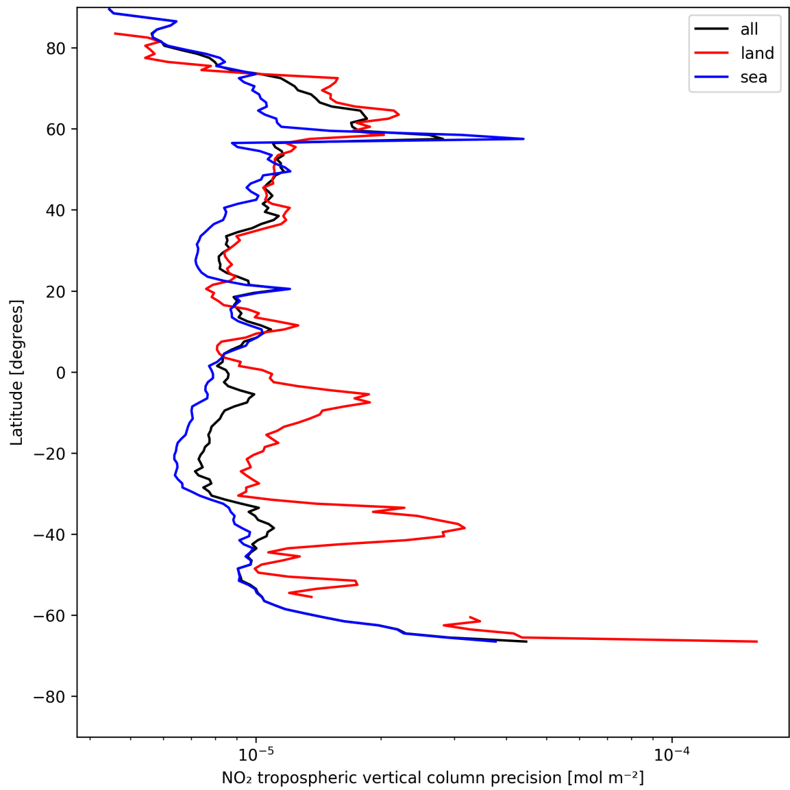
Figure 11: Zonal average of “NO 2 tropospheric vertical column precision” for 2025-07-19 to 2025-07-20.
