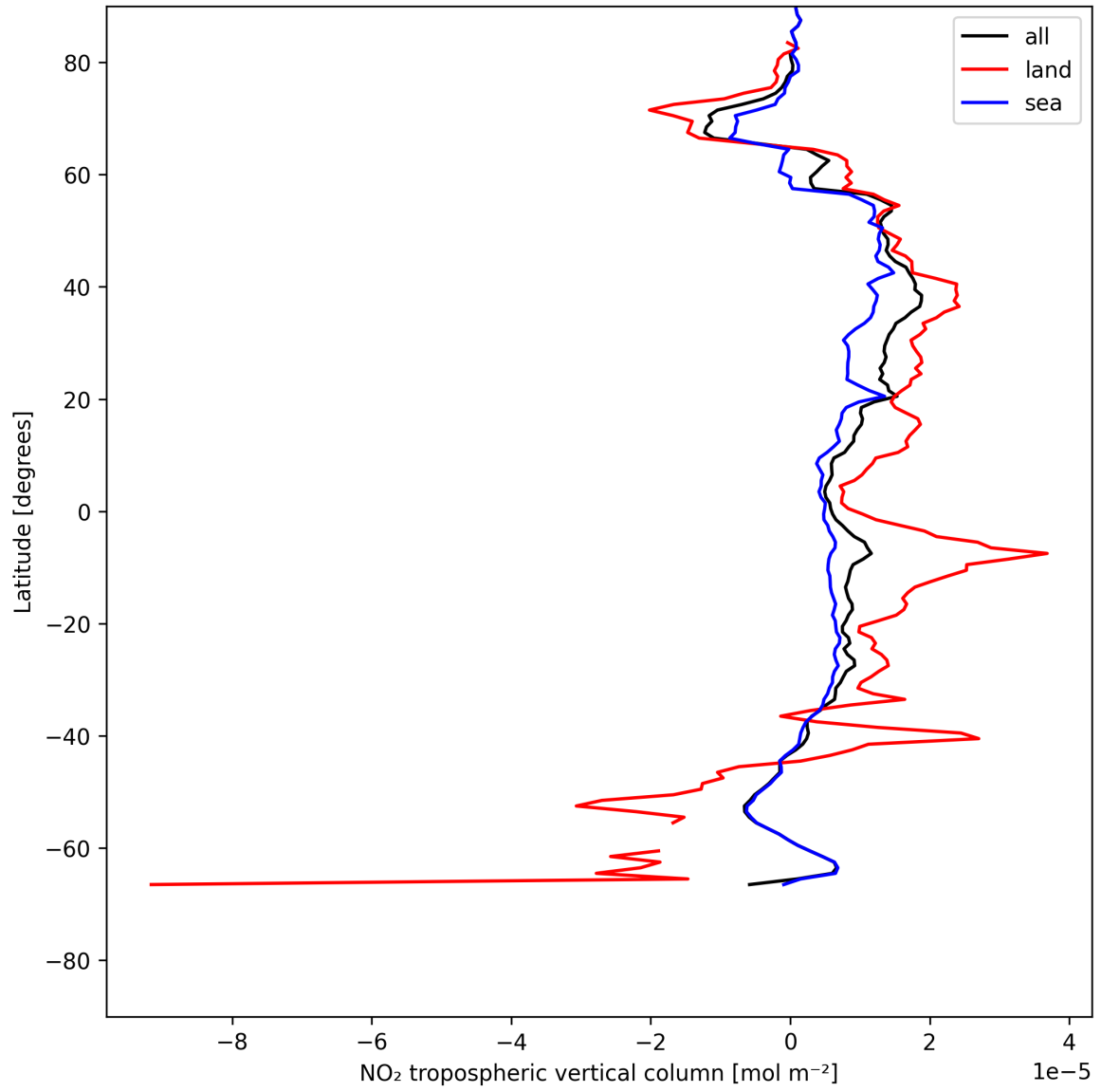
Figure 10: Zonal average of “NO 2 tropospheric vertical column” for 2025-07-19 to 2025-07-20.
