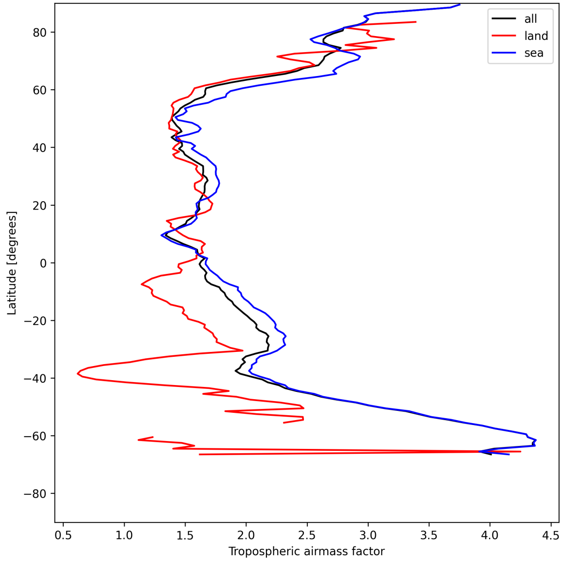
Figure 12: Zonal average of “Tropospheric airmass factor” for 2025-07-19 to 2025-07-20.
