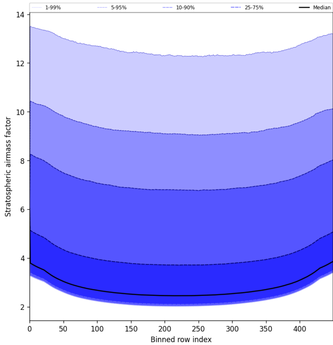
Figure 59: Along track statistics of “Stratospheric airmass factor” for 2025-07-19 to 2025-07-20
