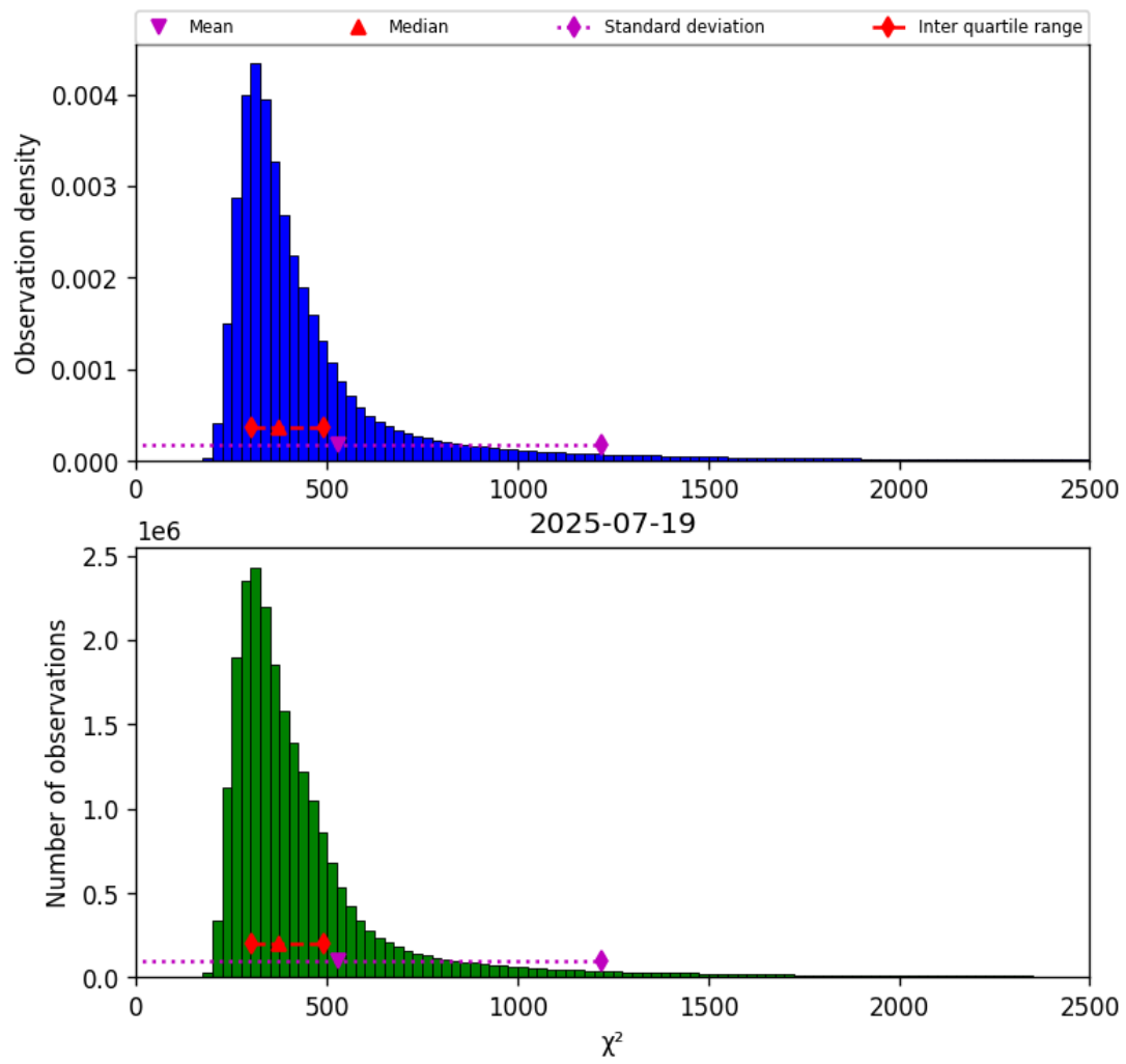
Figure 40: Histogram of “ \chi^2 ” for 2025-07-19 to 2025-07-20
