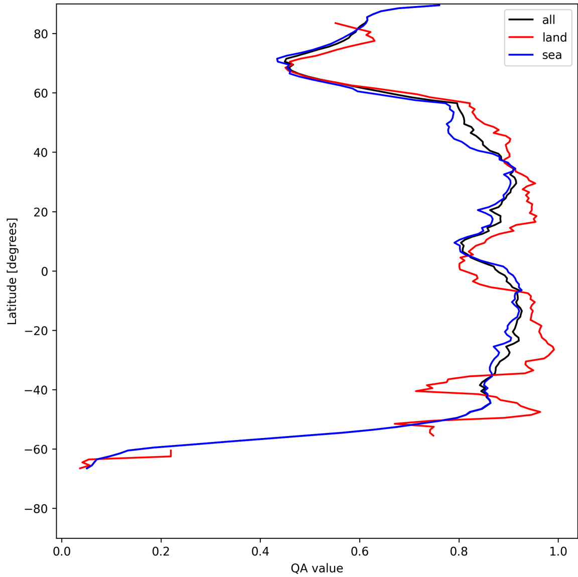
Figure 9: Zonal average of “QA value” for 2025-07-19 to 2025-07-20.
