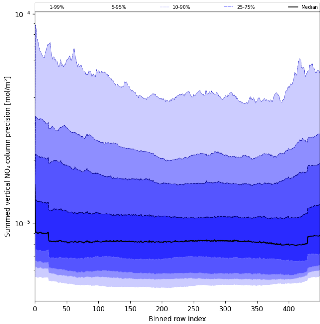
Figure 56: Along track statistics of “Summed vertical NO 2 column precision” for 2025-07-19 to 2025-07-20
