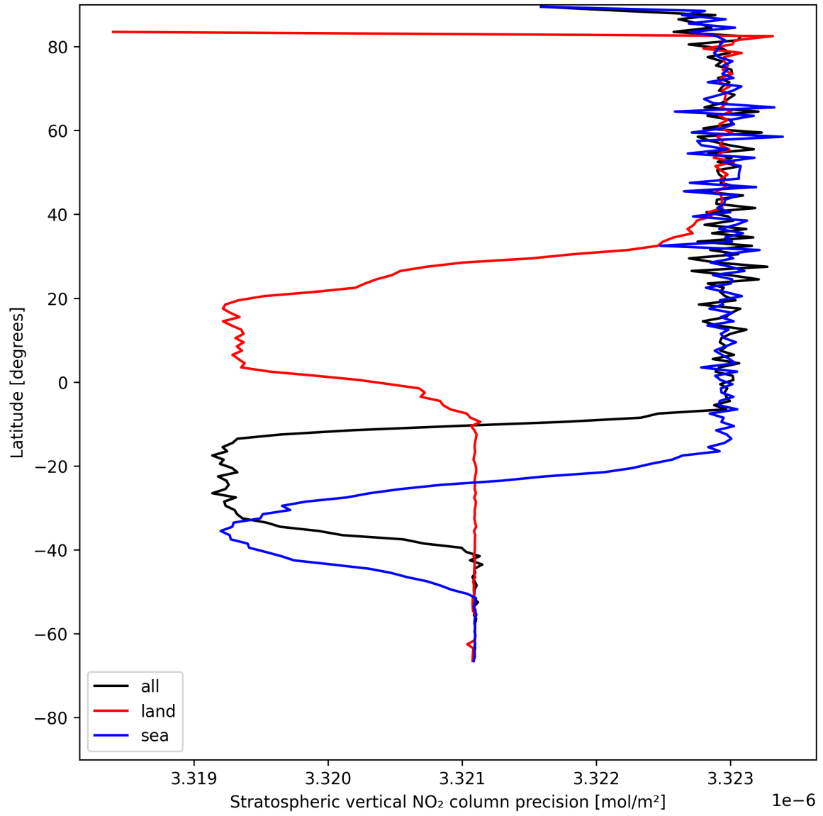
Figure 18: Zonal average of “Stratospheric vertical NO 2 column precision” for 2025-07-19 to 2025-07-20.
