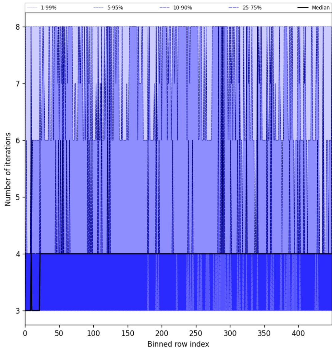
Figure 49: Along track statistics of “Number of iterations” for 2025-07-19 to 2025-07-20
