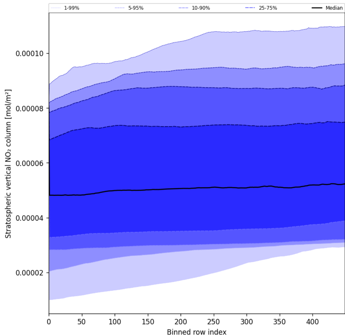
Figure 51: Along track statistics of “Stratospheric vertical NO 2 column” for 2025-07-19 to 2025-07-20
