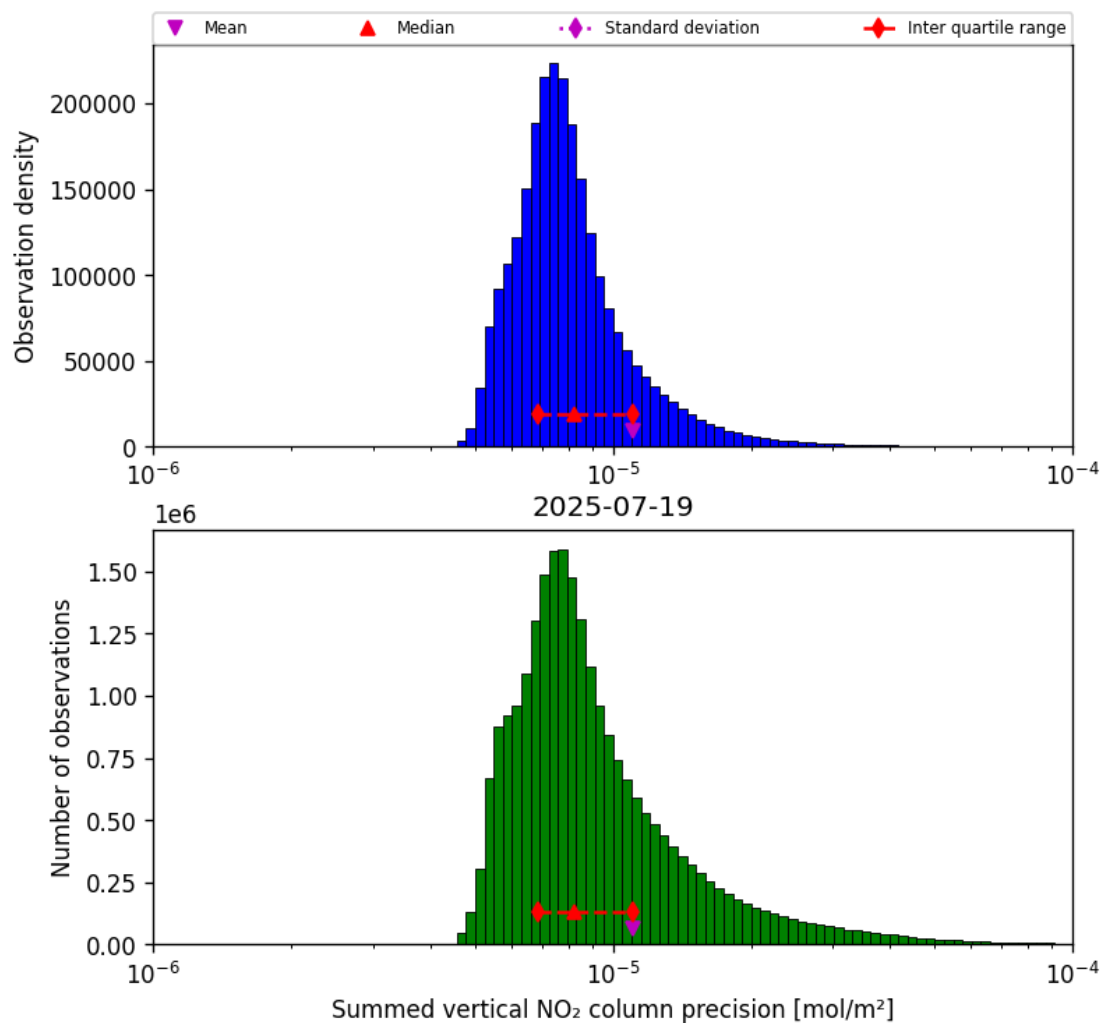
Figure 39: Histogram of "Summed vertical NO 2 column precision" for 2025-07-19 to 2025-07-20
