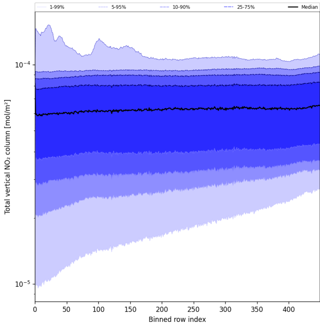
Figure 53: Along track statistics of “Total vertical NO 2 column” for 2025-07-19 to 2025-07-20
