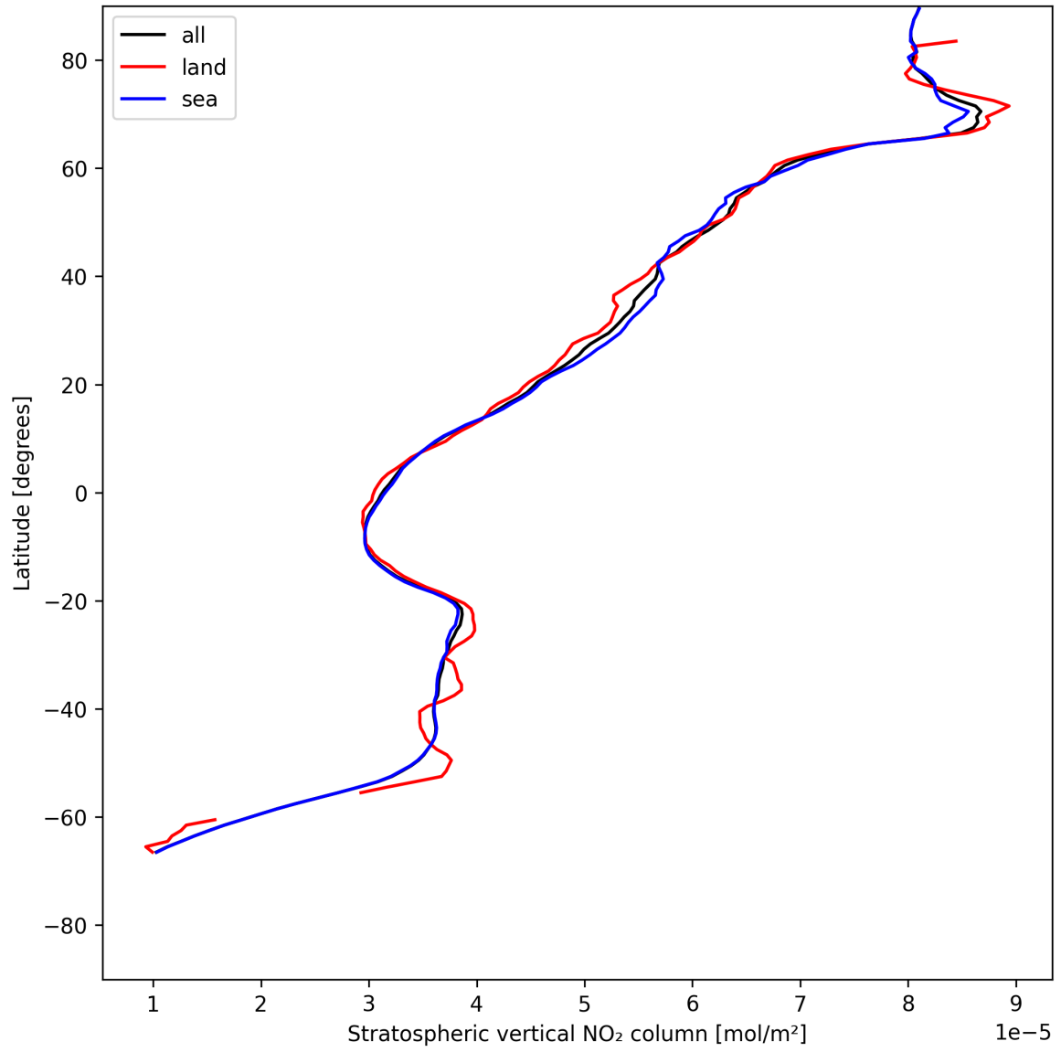
Figure 17: Zonal average of “Stratospheric vertical NO 2 column” for 2025-07-19 to 2025-07-20.
