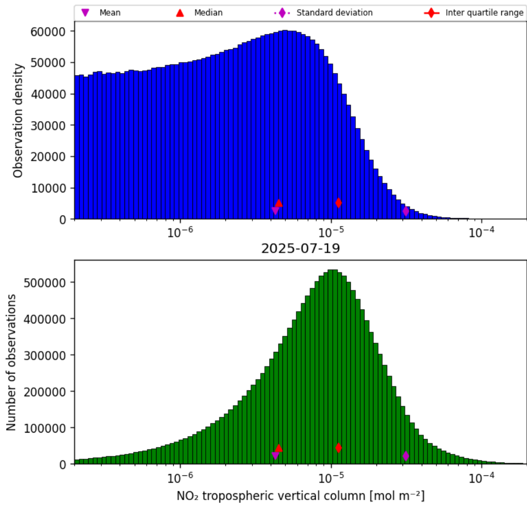
Figure 27: Histogram of “NO 2 tropospheric vertical column” for 2025-07-19 to 2025-07-20
