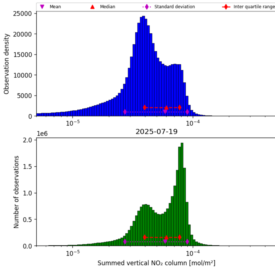
Figure 38: Histogram of “Summed vertical NO 2 column” for 2025-07-19 to 2025-07-20
