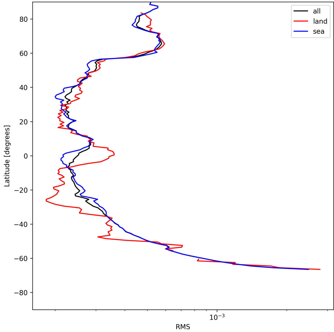
Figure 24: Zonal average of “RMS” for 2025-07-19 to 2025-07-20.
