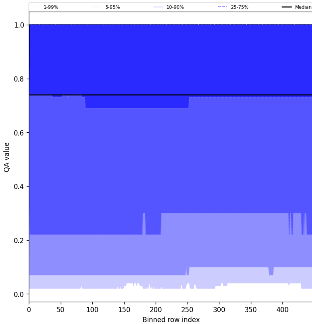
Figure 43: Along track statistics of “QA value” for 2025-07-19 to 2025-07-20
