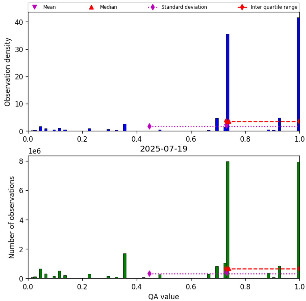
Figure 26: Histogram of “QA value” for 2025-07-19 to 2025-07-20
