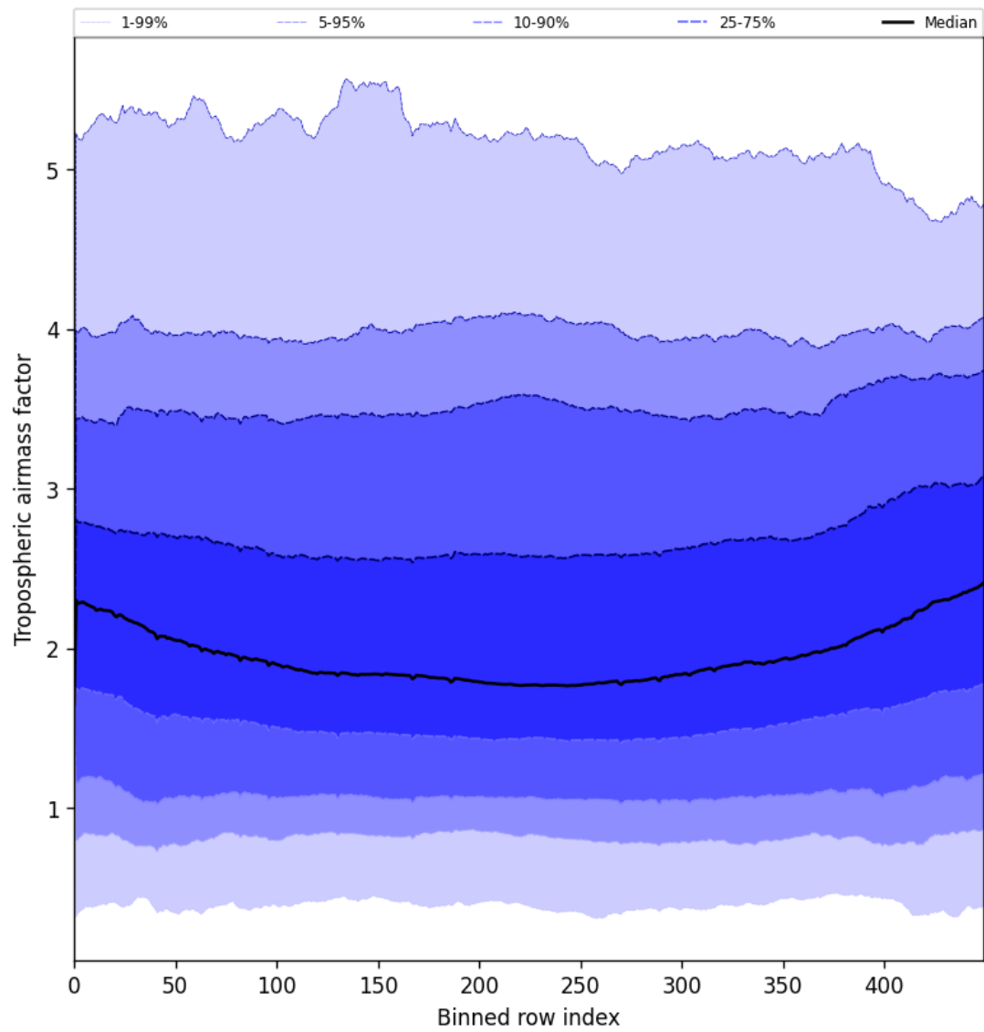
Figure 46: Along track statistics of “Tropospheric airmass factor” for 2025-07-19 to 2025-07-20
