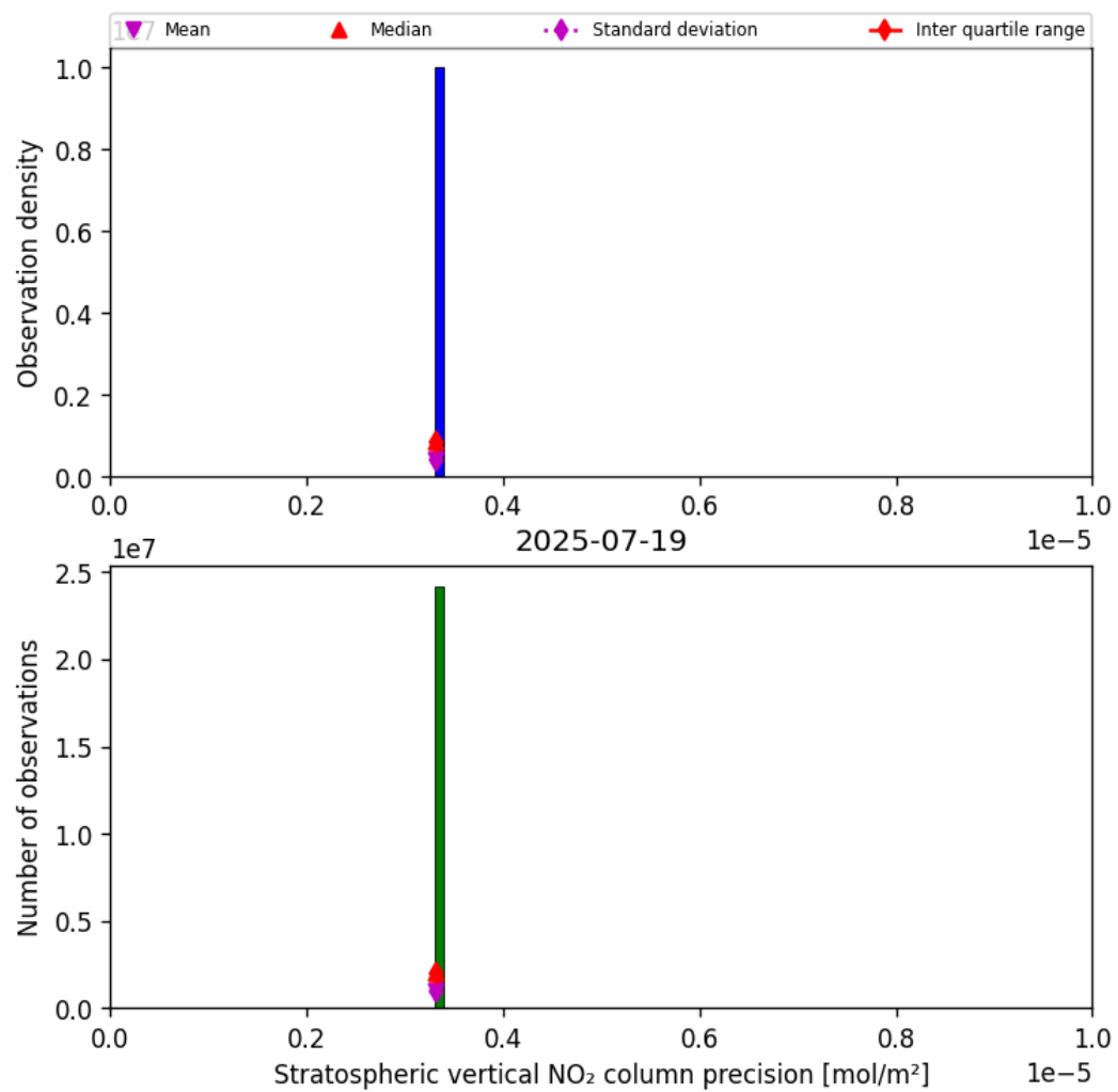
Figure 35: Histogram of “Stratospheric vertical NO 2 column precision” for 2025-07-19 to 2025-07-20
