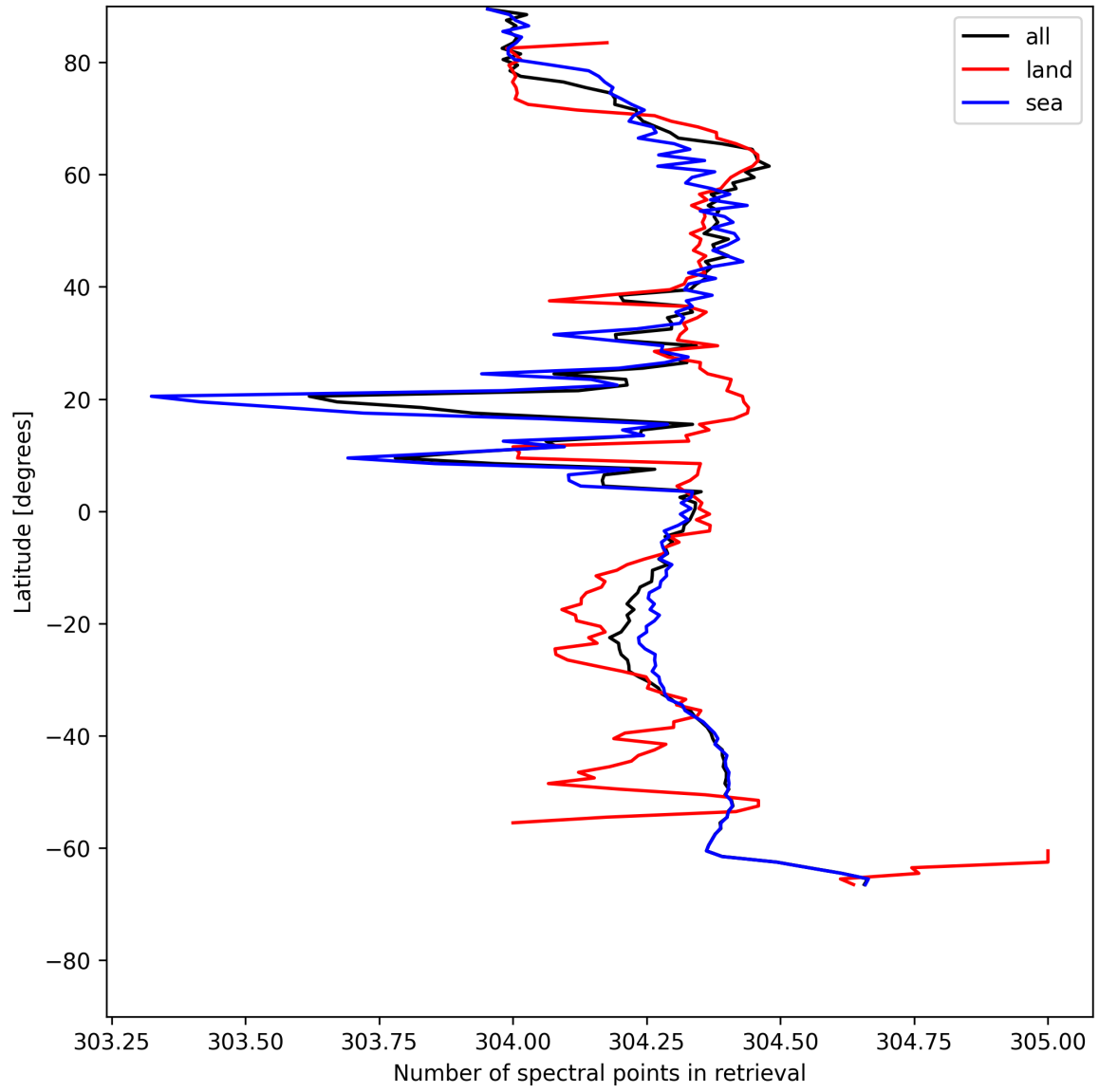
Figure 14: Zonal average of “Number of spectral points in retrieval” for 2025-07-19 to 2025-07-20.
