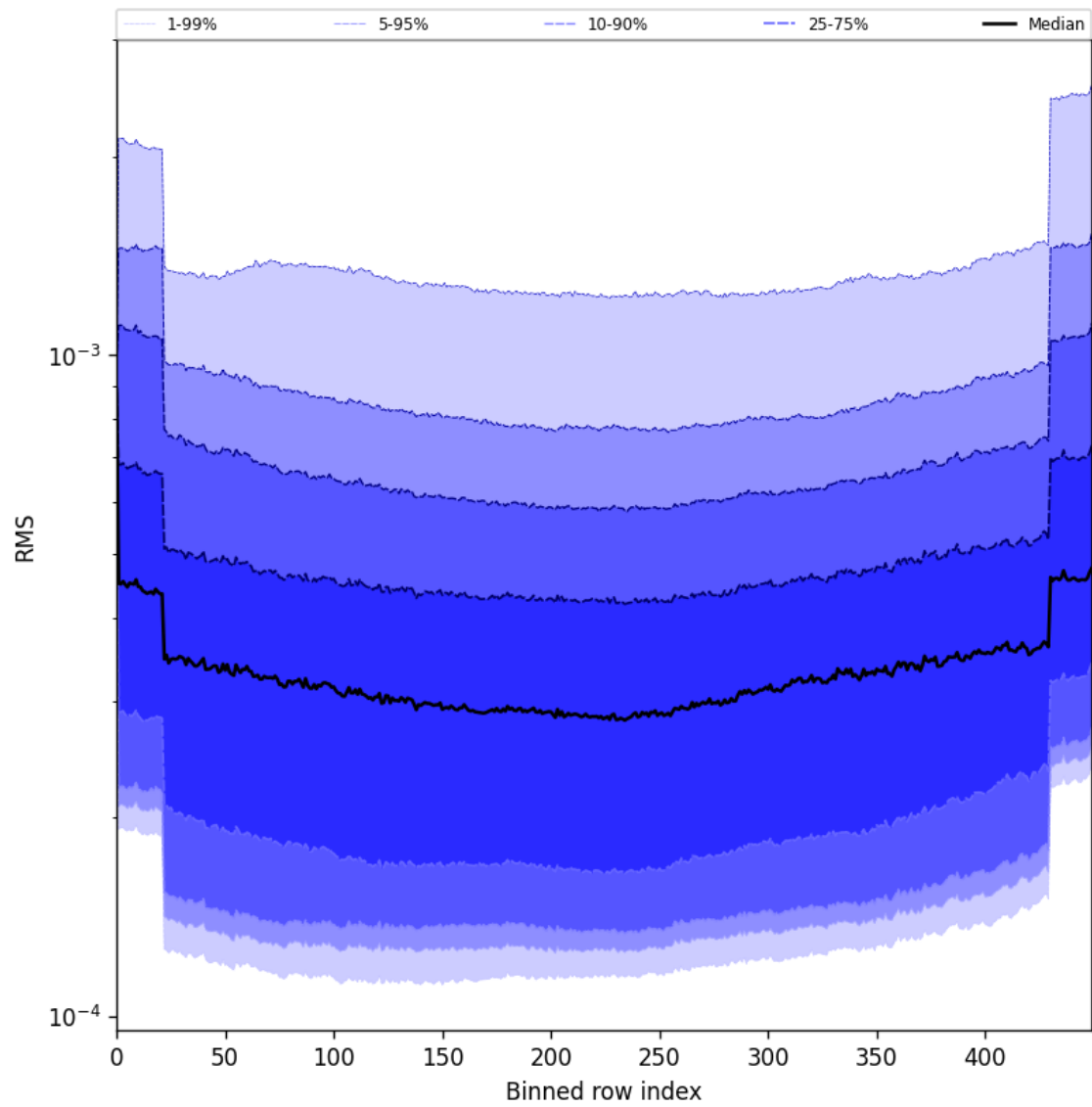
Figure 58: Along track statistics of “RMS” for 2025-07-19 to 2025-07-20
