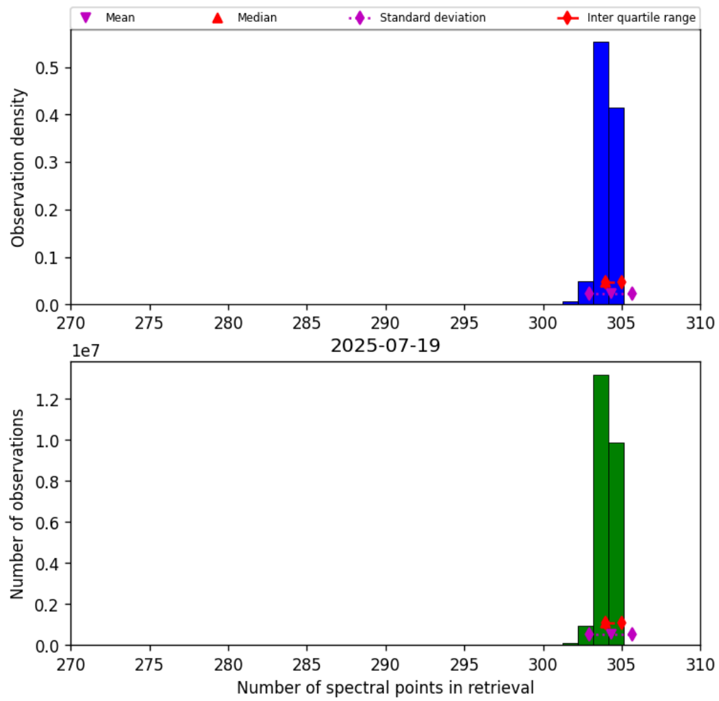
Figure 31: Histogram of “Number of spectral points in retrieval” for 2025-07-19 to 2025-07-20
