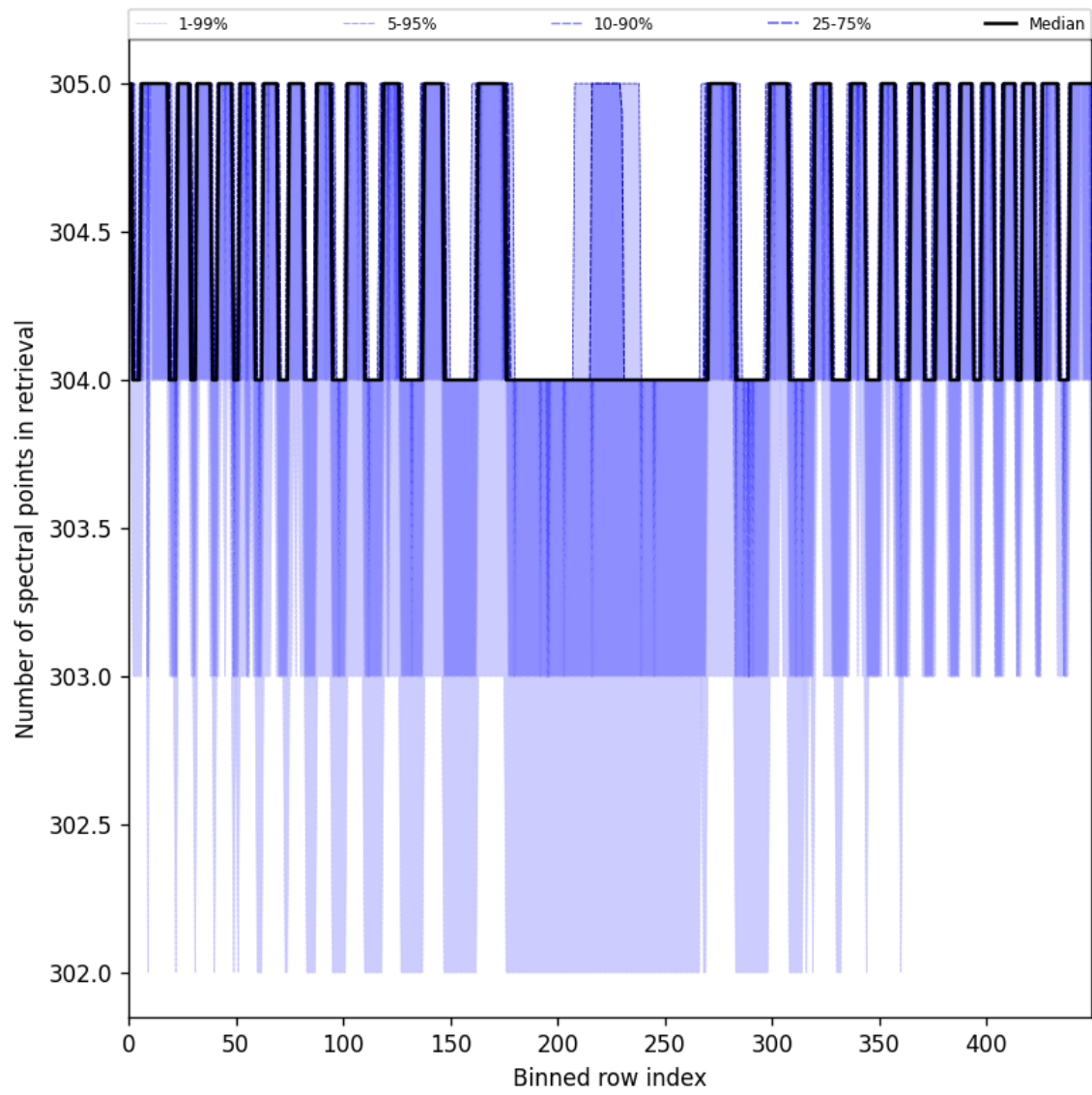
Figure 48: Along track statistics of “Number of spectral points in retrieval” for 2025-07-19 to 2025-07-20
