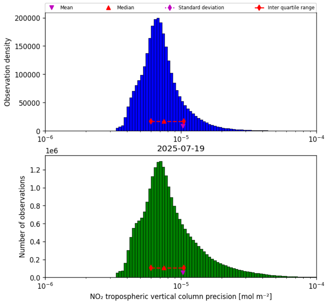
Figure 28: Histogram of “NO 2 tropospheric vertical column precision” for 2025-07-19 to 2025-07-20
