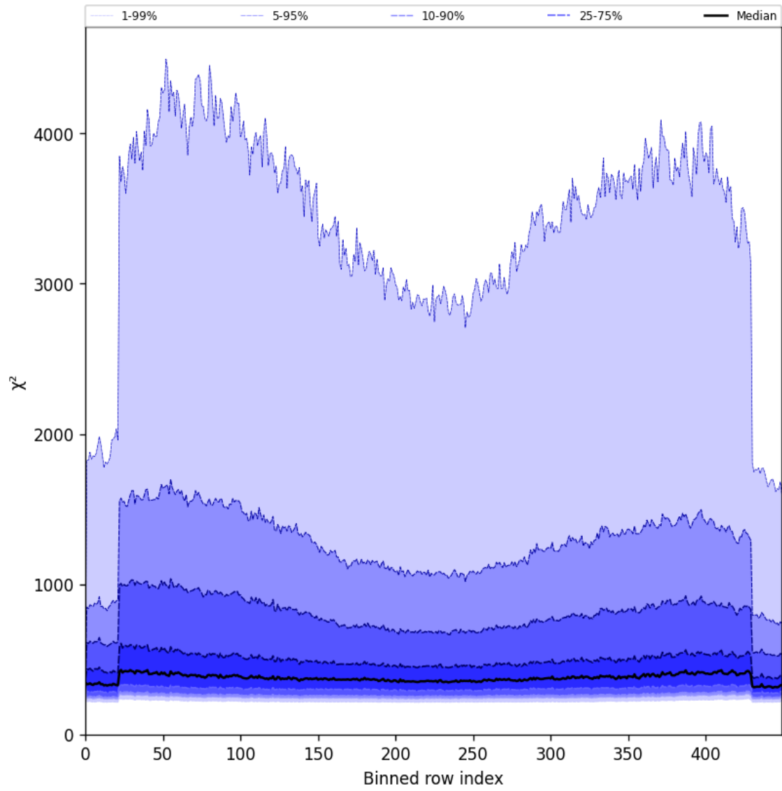
Figure 57: Along track statistics of “ \chi^2 ” for 2025-07-19 to 2025-07-20
