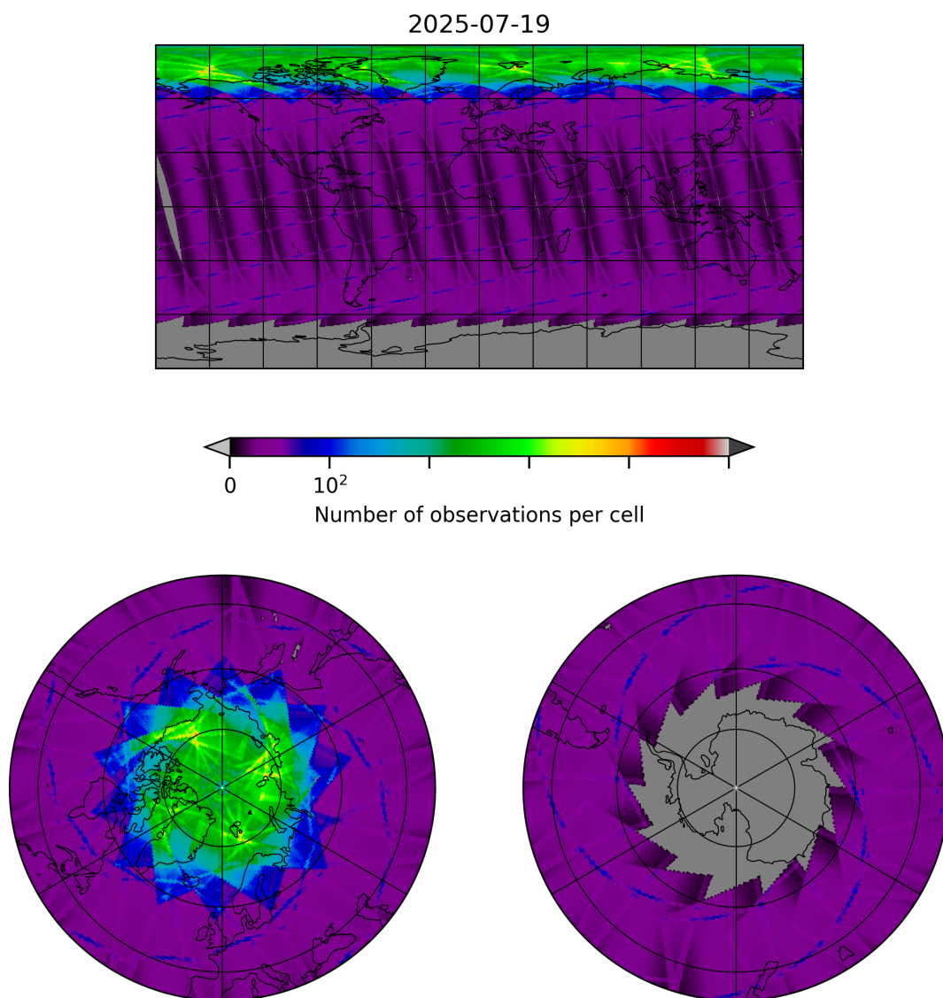
Figure 8: Map of the number of observations for 2025-07-19 to 2025-07-20
