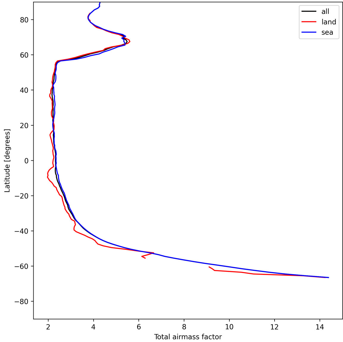
Figure 13: Zonal average of “Total airmass factor” for 2025-07-19 to 2025-07-20.
