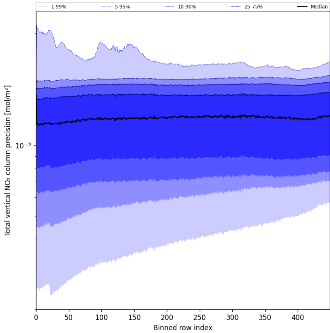
Figure 54: Along track statistics of “Total vertical NO 2 column precision” for 2025-07-19 to 2025-07-20
