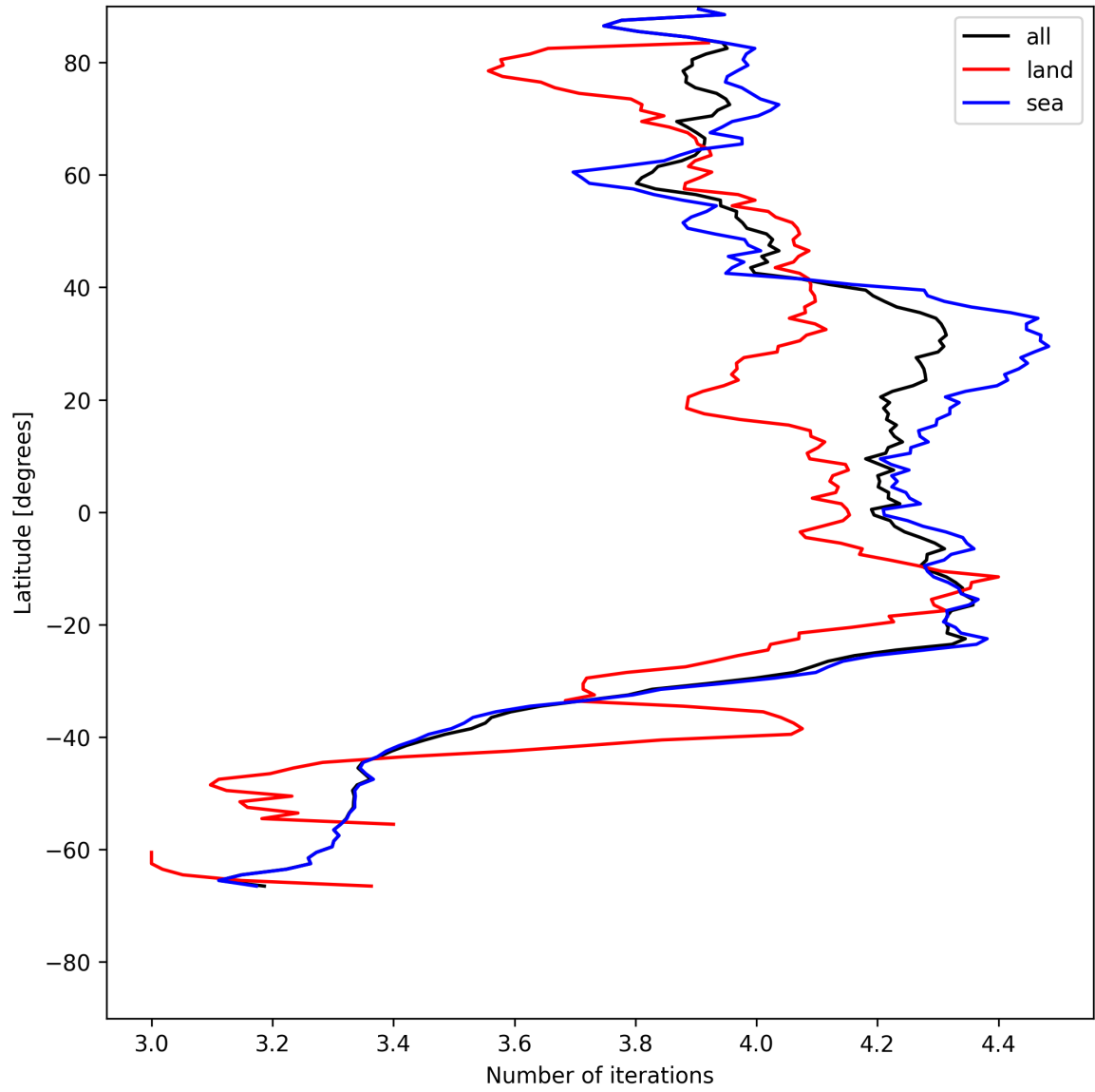
Figure 15: Zonal average of “Number of iterations” for 2025-07-19 to 2025-07-20.
