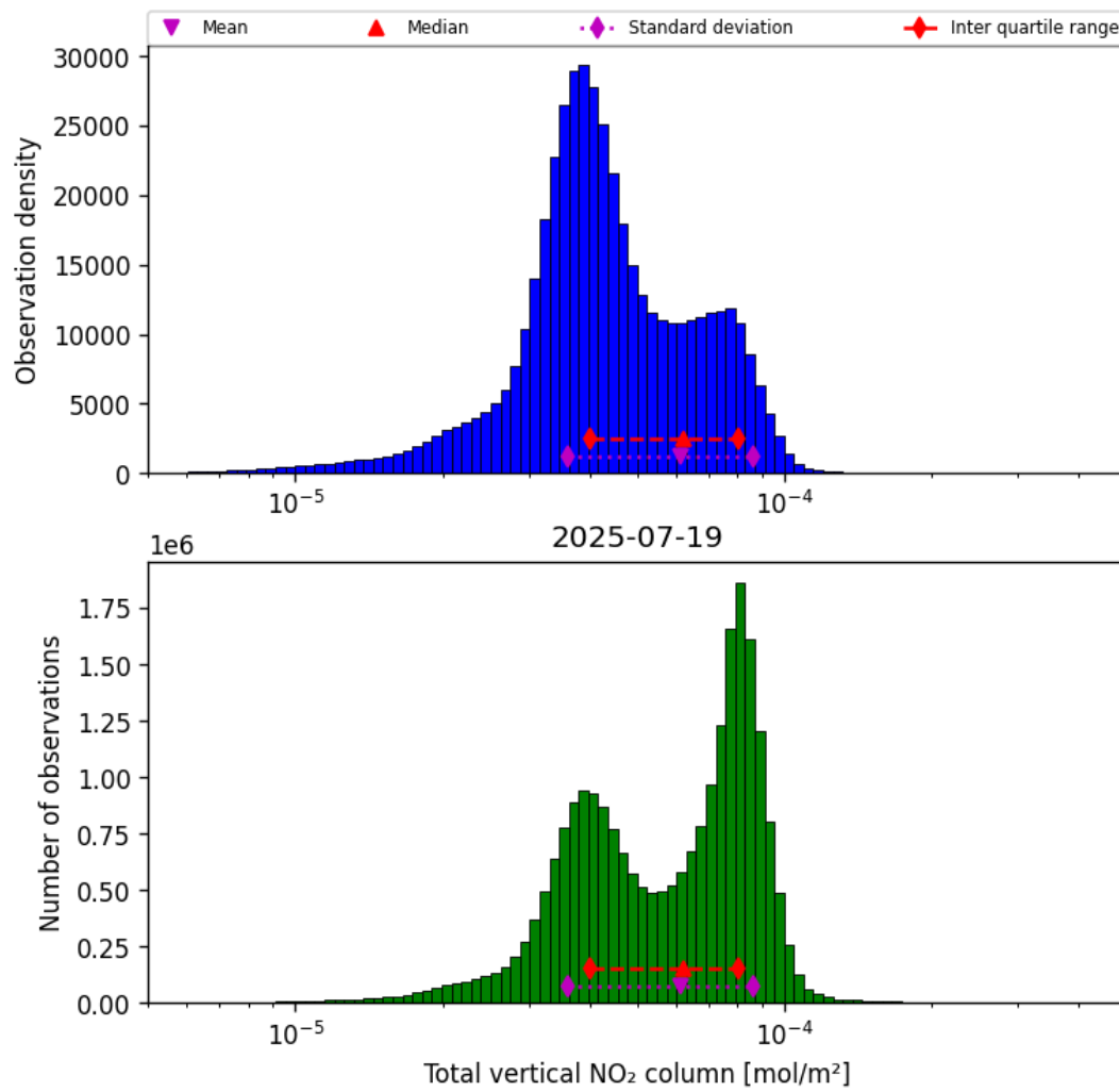
Figure 36: Histogram of “Total vertical NO 2 column” for 2025-07-19 to 2025-07-20
