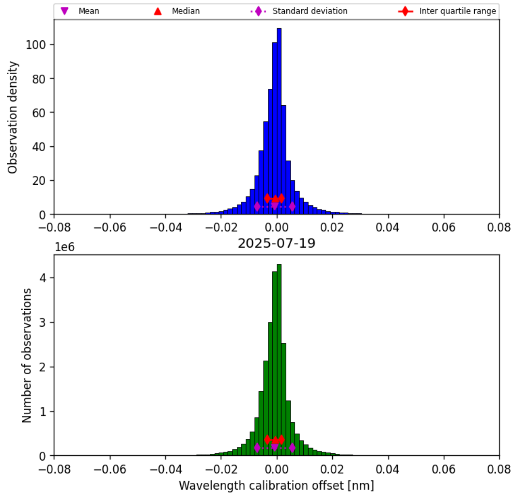
Figure 33: Histogram of “Wavelength calibration offset” for 2025-07-19 to 2025-07-20
