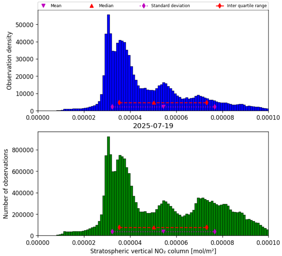
Figure 34: Histogram of “Stratospheric vertical NO 2 column” for 2025-07-19 to 2025-07-20
