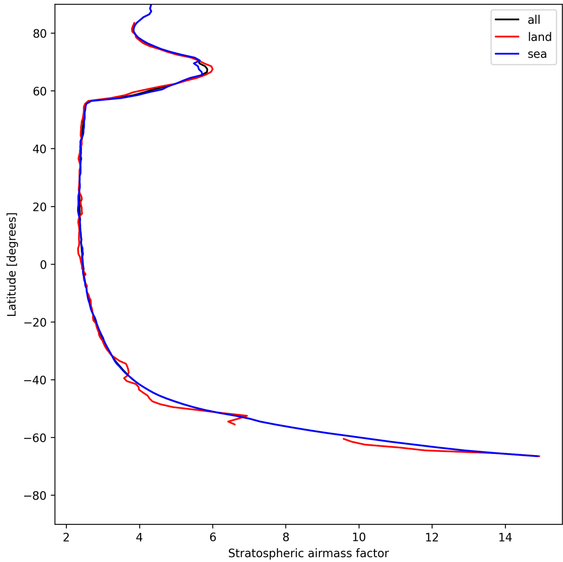
Figure 25: Zonal average of “Stratospheric airmass factor” for 2025-07-19 to 2025-07-20.
