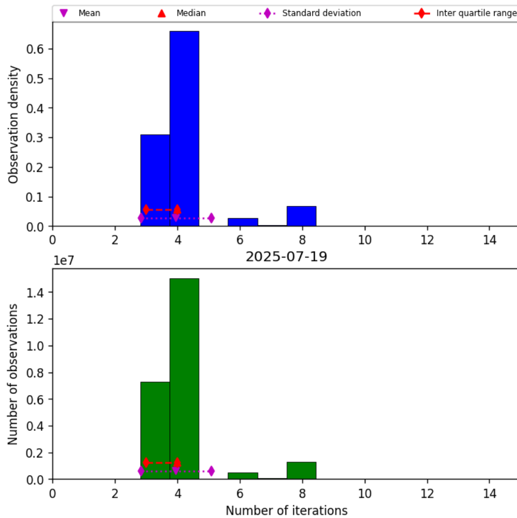
Figure 32: Histogram of “Number of iterations” for 2025-07-19 to 2025-07-20
