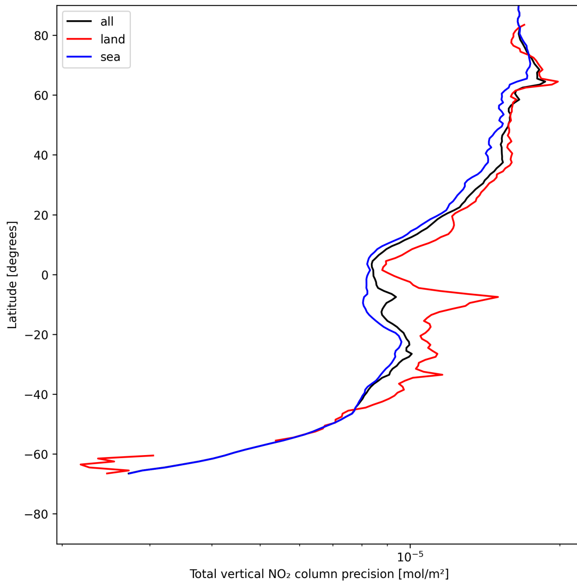
Figure 20: Zonal average of “Total vertical NO 2 column precision” for 2025-07-19 to 2025-07-20.
