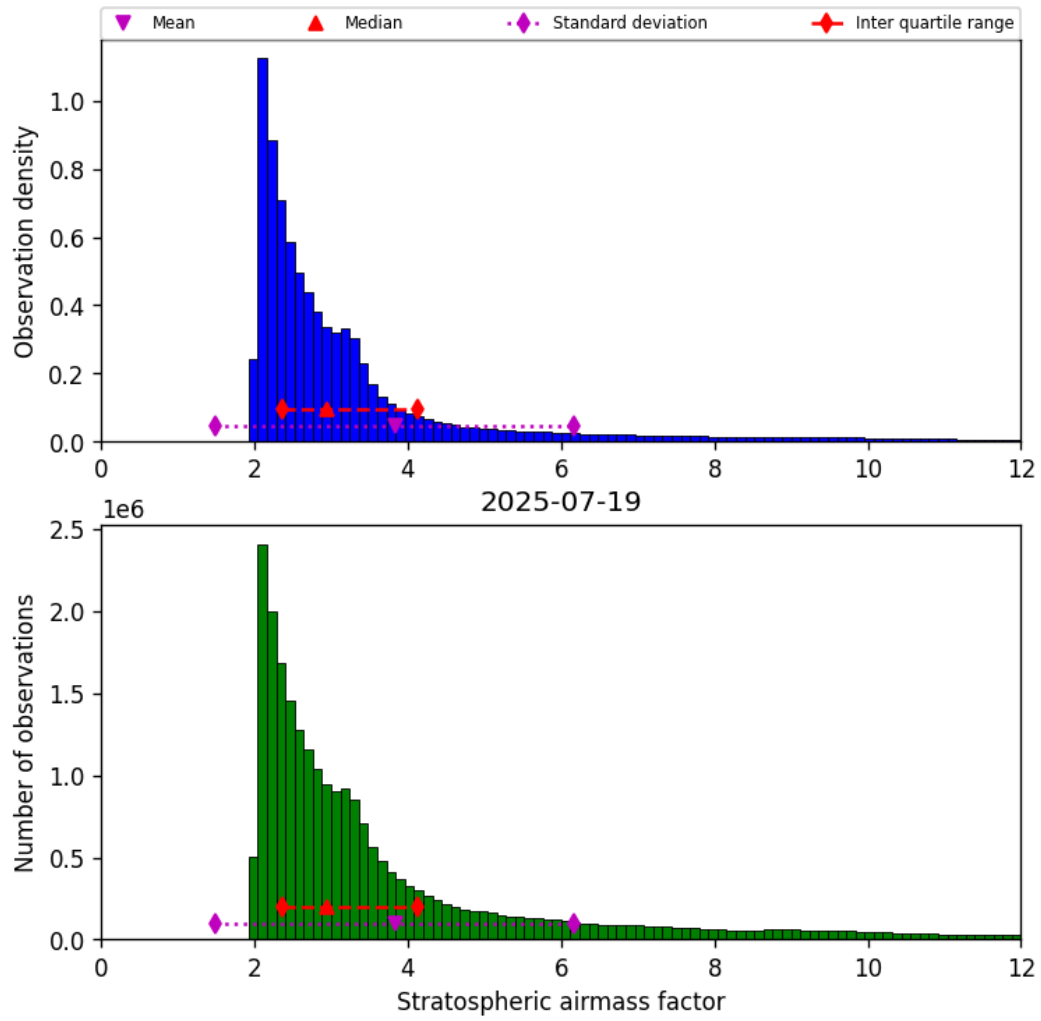
Figure 42: Histogram of “Stratospheric airmass factor” for 2025-07-19 to 2025-07-20
