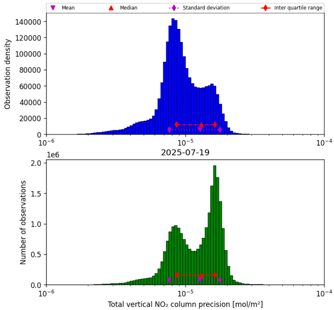
Figure 37: Histogram of “Total vertical NO 2 column precision” for 2025-07-19 to 2025-07-20
