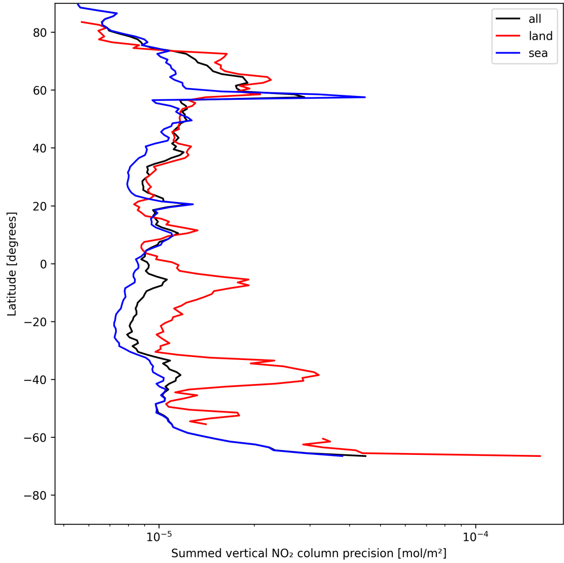
Figure 22: Zonal average of “Summed vertical NO 2 column precision” for 2025-07-19 to 2025-07-20.
