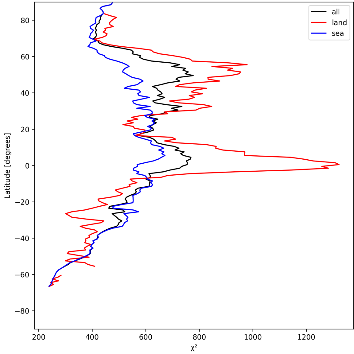
Figure 23: Zonal average of “ \chi^2 ” for 2025-07-19 to 2025-07-20.
