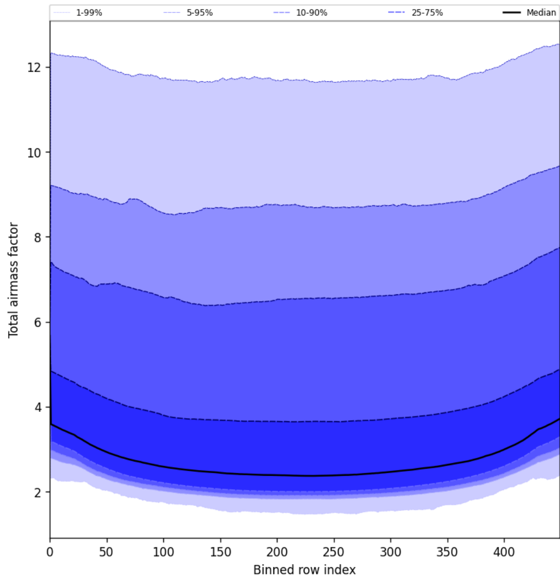
Figure 47: Along track statistics of “Total airmass factor” for 2025-07-19 to 2025-07-20
