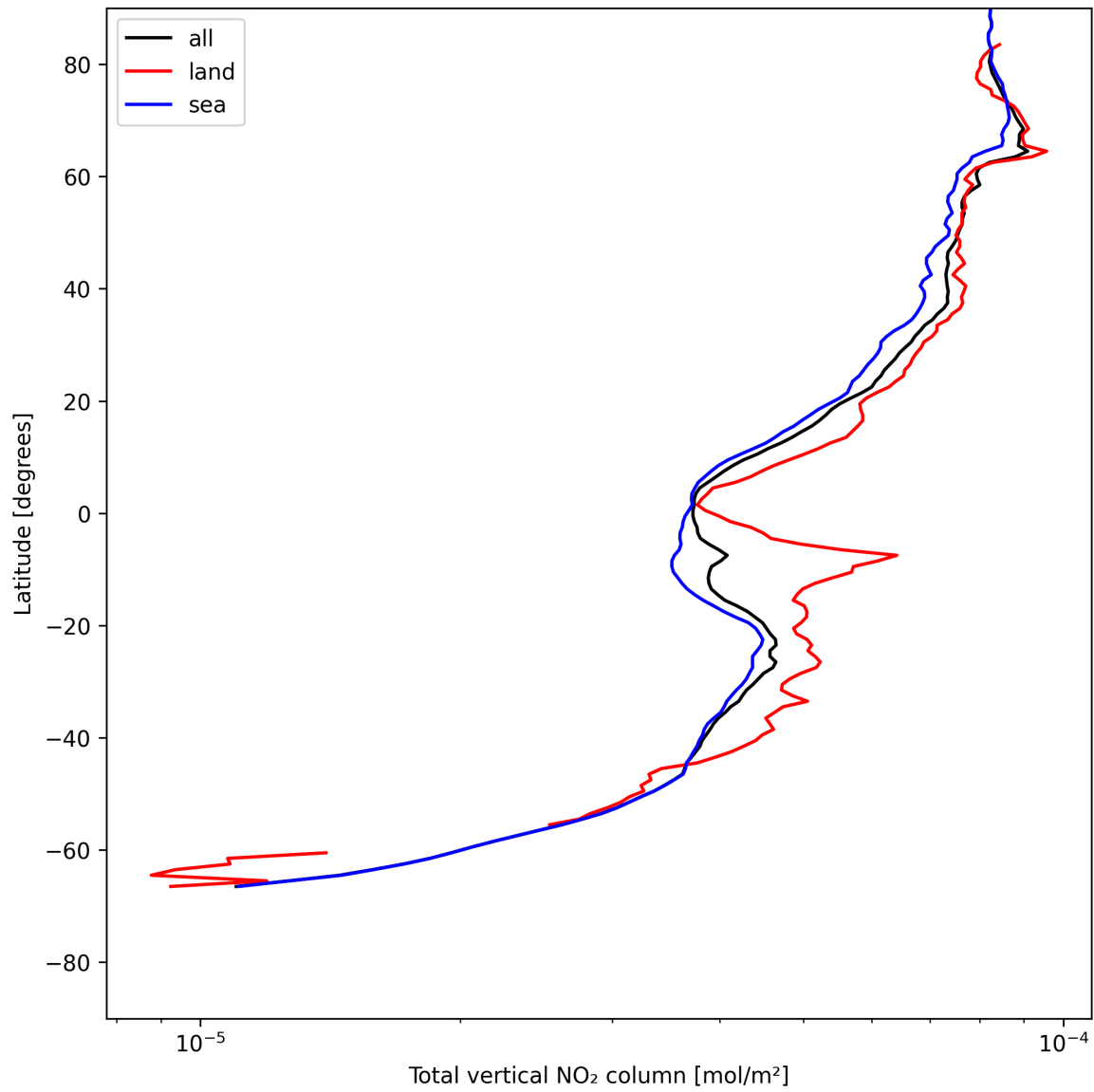
Figure 19: Zonal average of “Total vertical NO 2 column” for 2025-07-19 to 2025-07-20.
