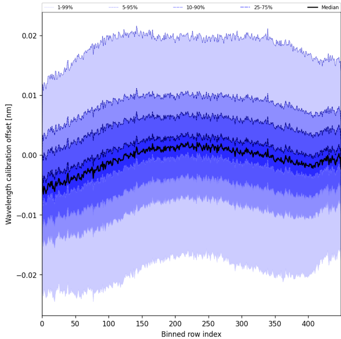
Figure 50: Along track statistics of “Wavelength calibration offset” for 2025-07-19 to 2025-07-20
