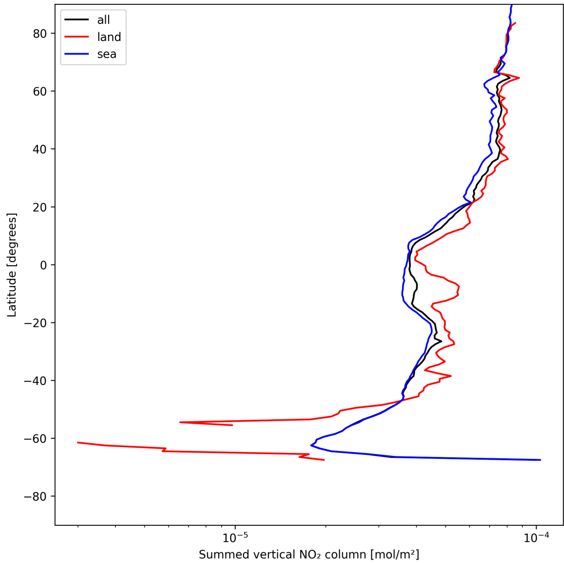
Figure 21: Zonal average of “Summed vertical NO 2 column” for 2025-07-20 to 2025-07-21.
