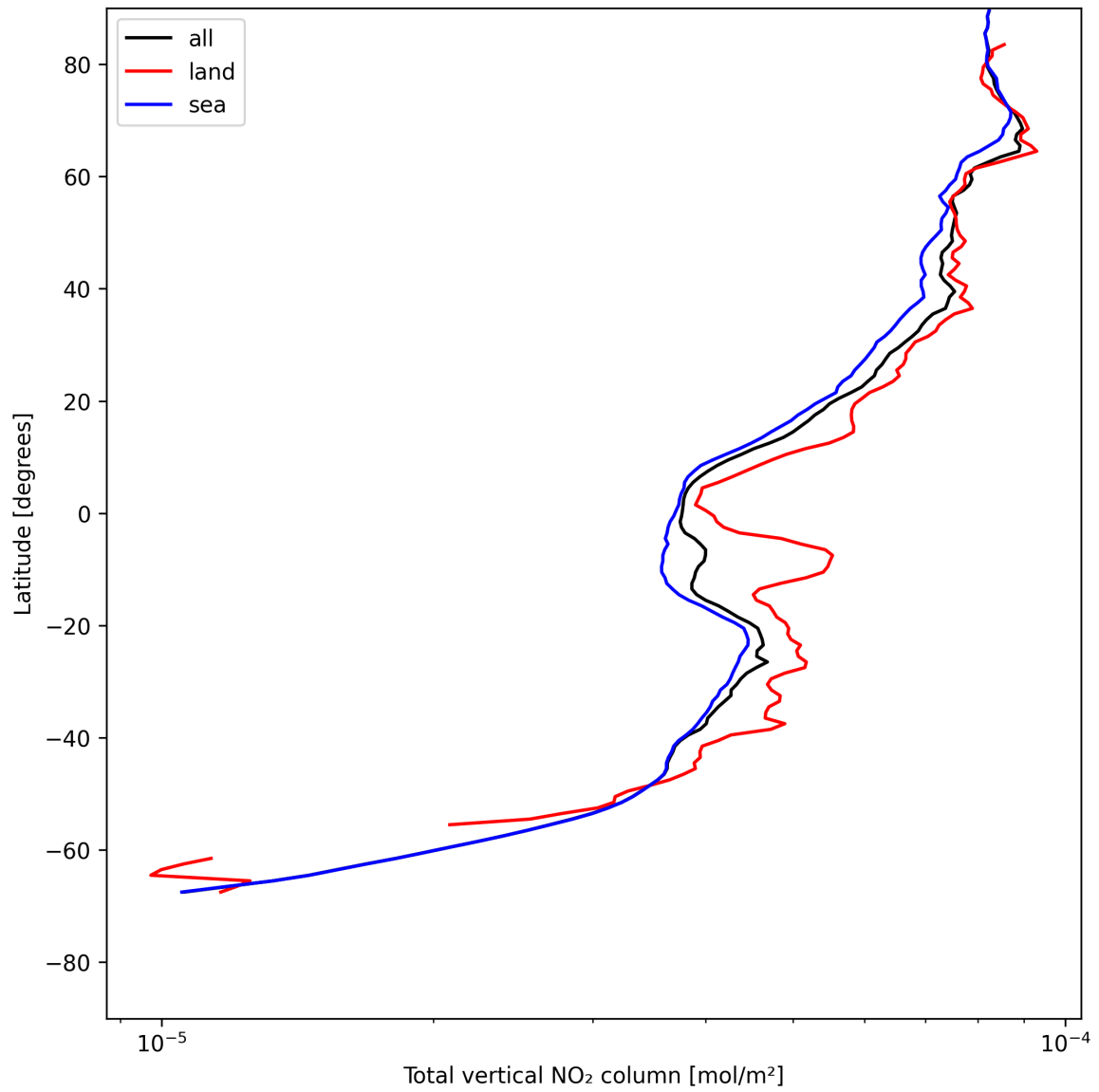
Figure 19: Zonal average of “Total vertical NO 2 column” for 2025-07-20 to 2025-07-21.
