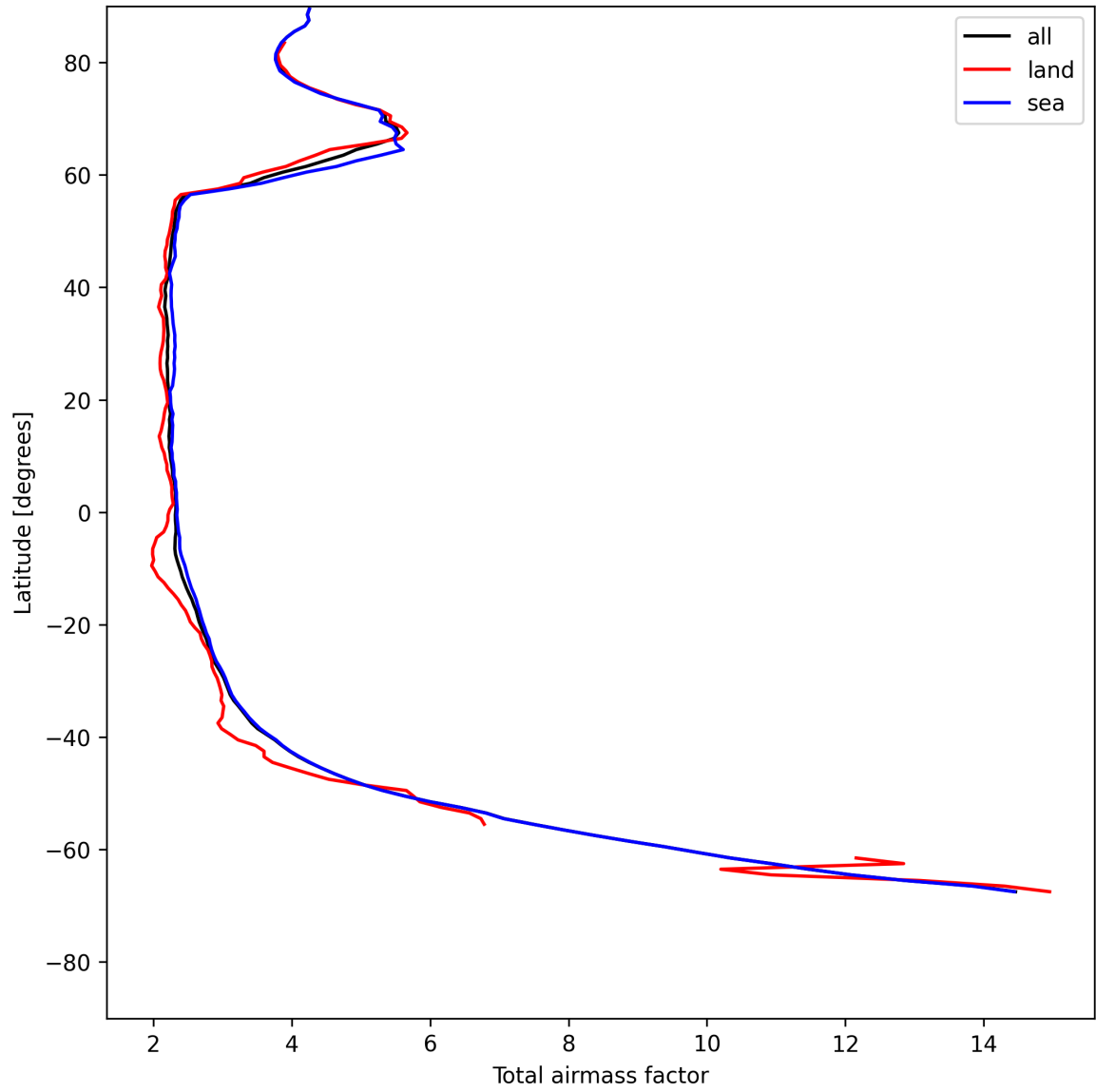
Figure 13: Zonal average of “Total airmass factor” for 2025-07-20 to 2025-07-21.
