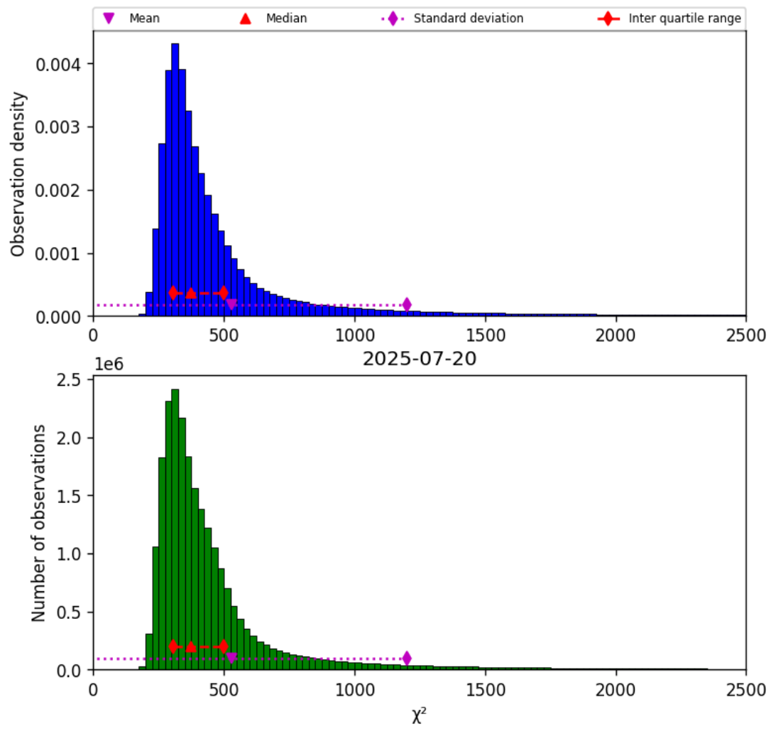
Figure 40: Histogram of “ \chi^2 ” for 2025-07-20 to 2025-07-21
