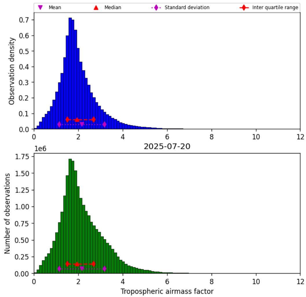
Figure 29: Histogram of “Tropospheric airmass factor” for 2025-07-20 to 2025-07-21
