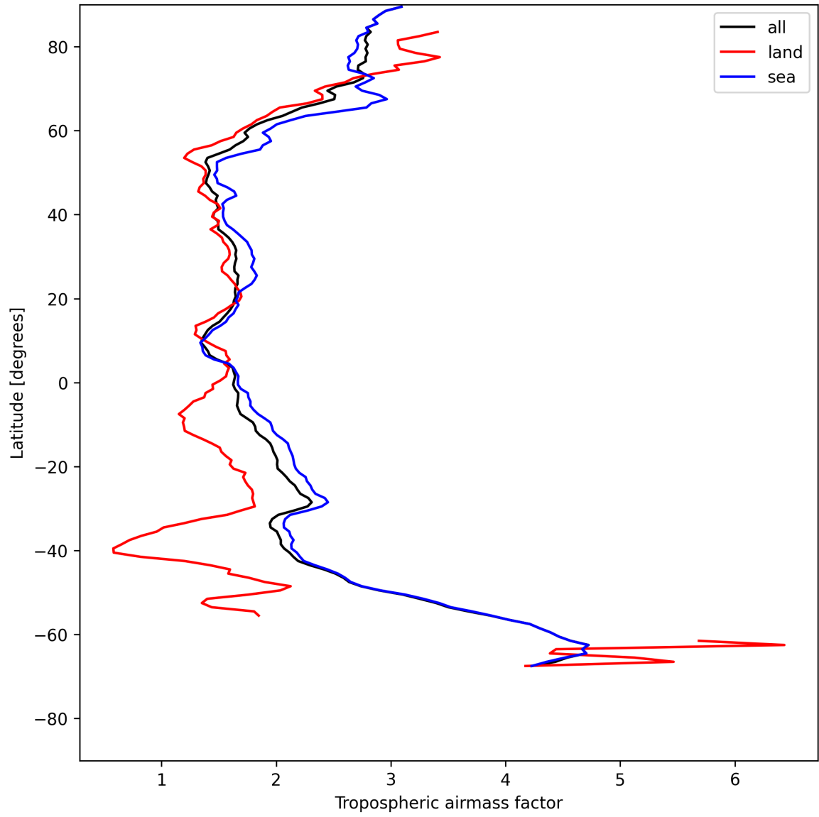
Figure 12: Zonal average of “Tropospheric airmass factor” for 2025-07-20 to 2025-07-21.
