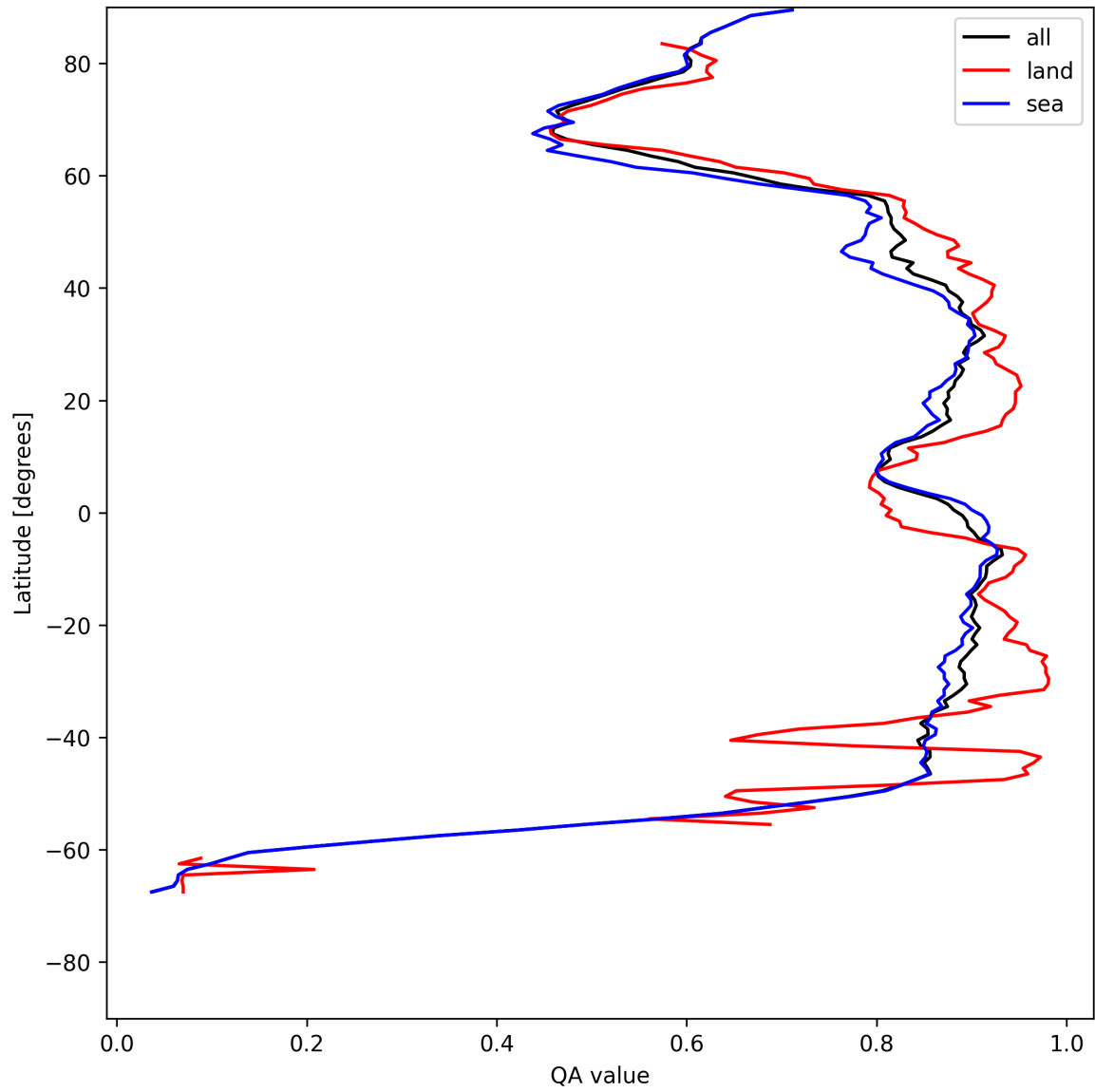
Figure 9: Zonal average of “QA value” for 2025-07-20 to 2025-07-21.
