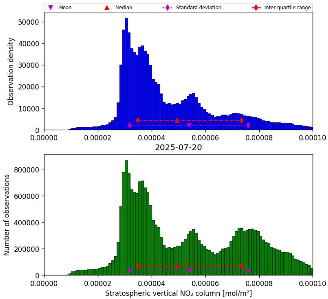
Figure 34: Histogram of “Stratospheric vertical NO 2 column” for 2025-07-20 to 2025-07-21
