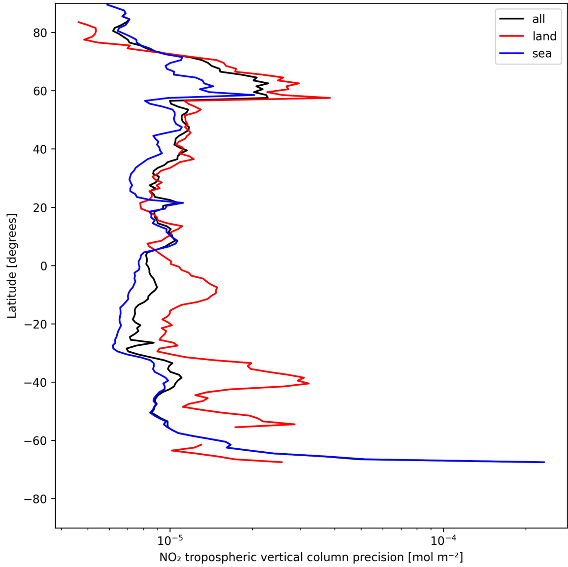
Figure 11: Zonal average of “NO 2 tropospheric vertical column precision” for 2025-07-20 to 2025-07-21.
