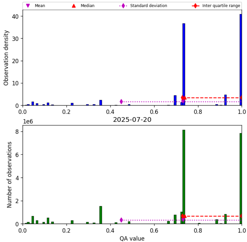
Figure 26: Histogram of “QA value” for 2025-07-20 to 2025-07-21
