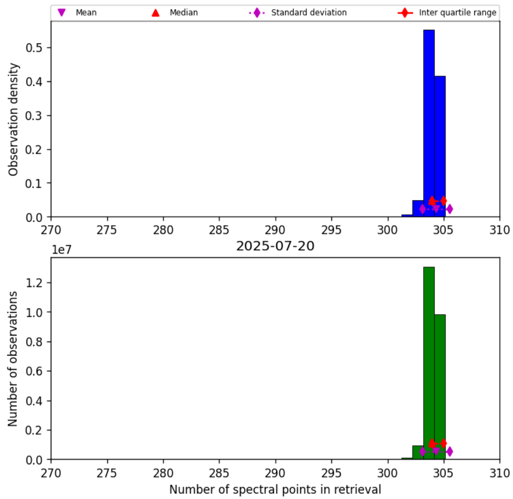
Figure 31: Histogram of “Number of spectral points in retrieval” for 2025-07-20 to 2025-07-21
