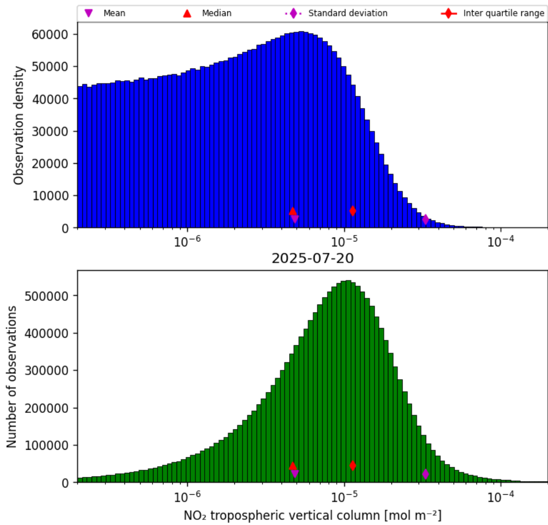
Figure 27: Histogram of “NO 2 tropospheric vertical column” for 2025-07-20 to 2025-07-21
