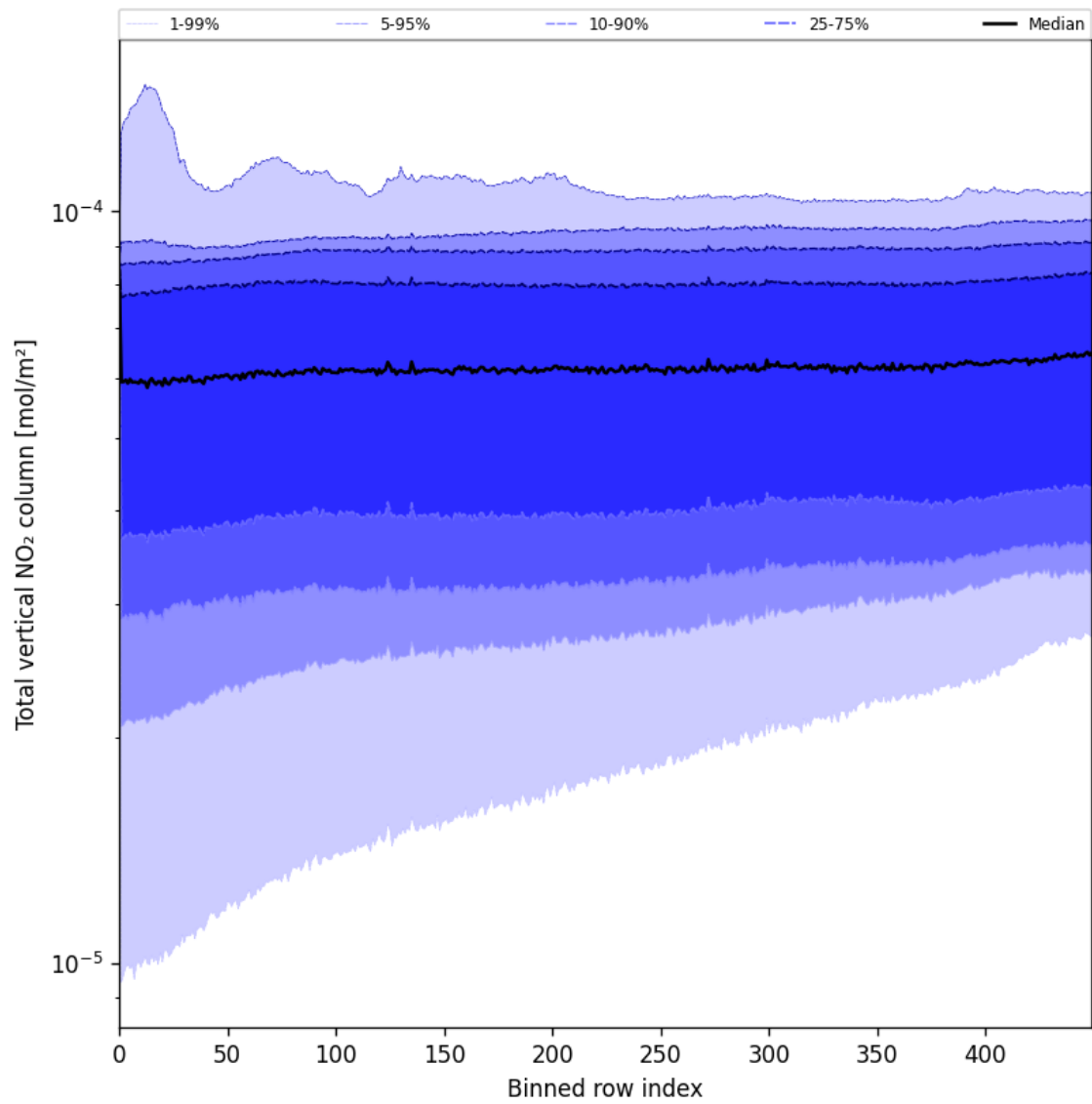
Figure 53: Along track statistics of “Total vertical NO 2 column” for 2025-07-20 to 2025-07-21
