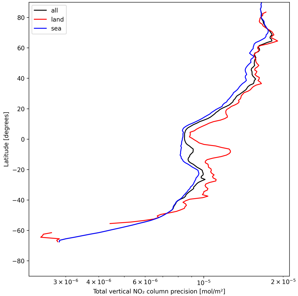
Figure 20: Zonal average of “Total vertical NO 2 column precision” for 2025-07-20 to 2025-07-21.
