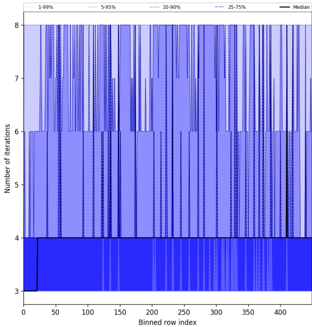
Figure 49: Along track statistics of “Number of iterations” for 2025-07-20 to 2025-07-21
