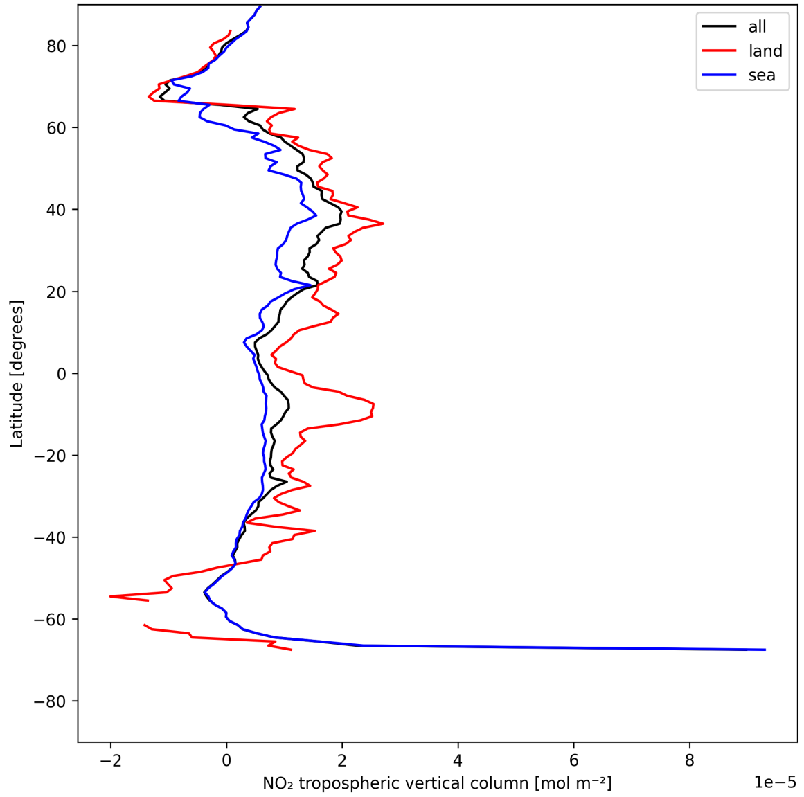
Figure 10: Zonal average of “NO 2 tropospheric vertical column” for 2025-07-20 to 2025-07-21.
