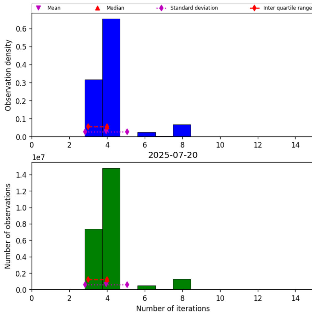
Figure 32: Histogram of “Number of iterations” for 2025-07-20 to 2025-07-21
