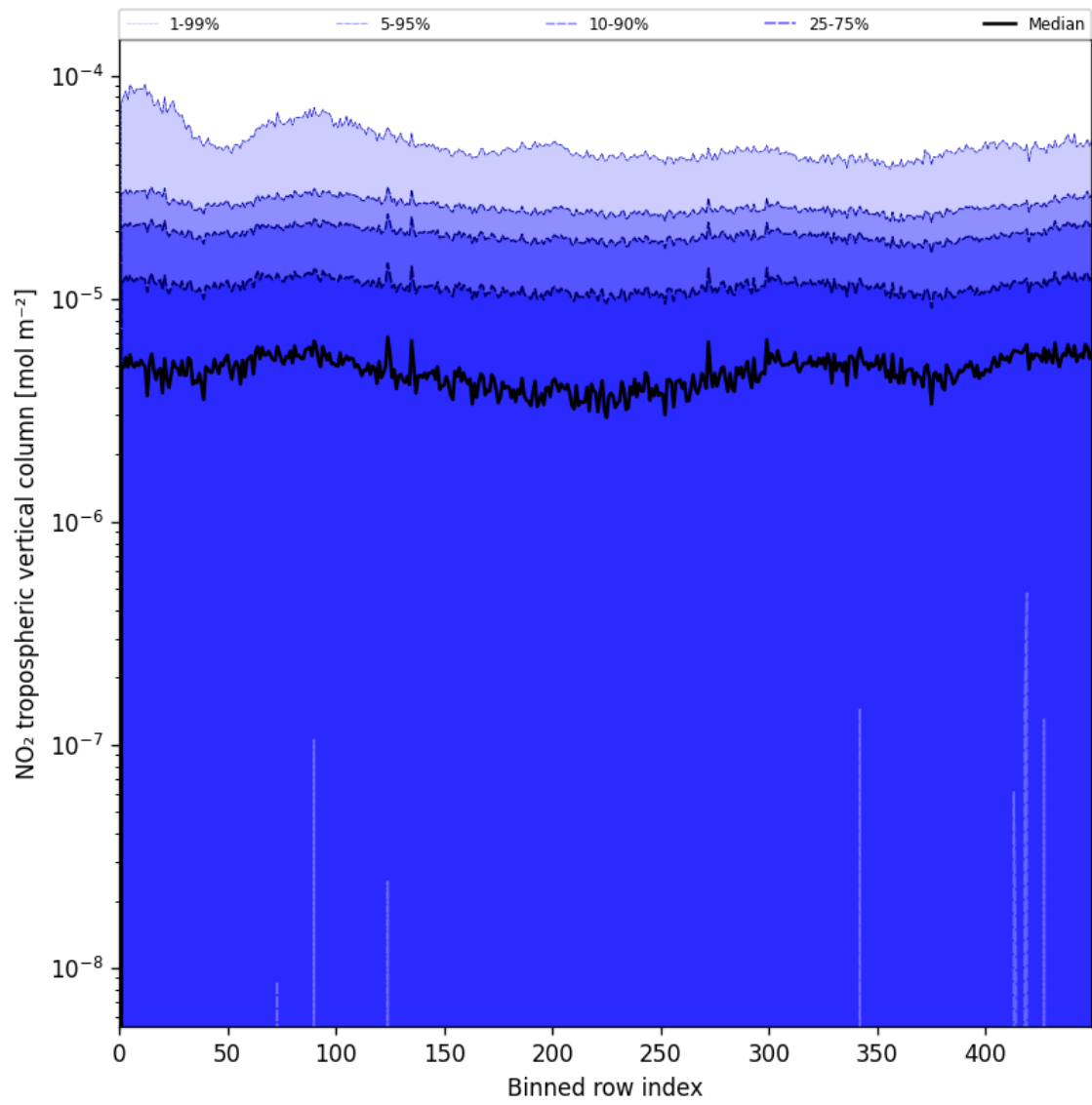
Figure 44: Along track statistics of “NO 2 tropospheric vertical column” for 2025-07-20 to 2025-07-21
