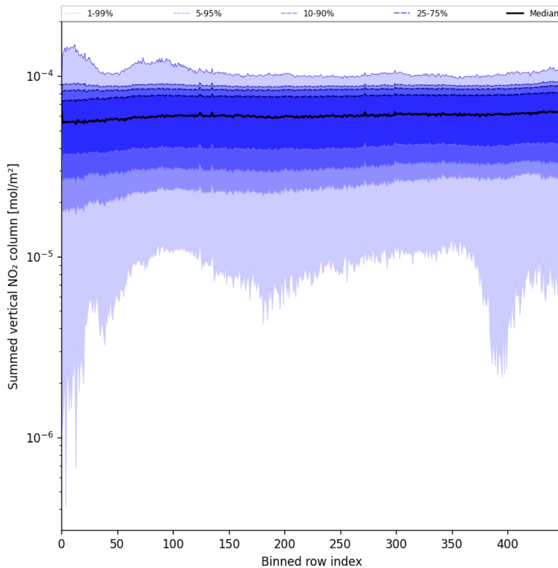
Figure 55: Along track statistics of “Summed vertical NO 2 column” for 2025-07-20 to 2025-07-21
