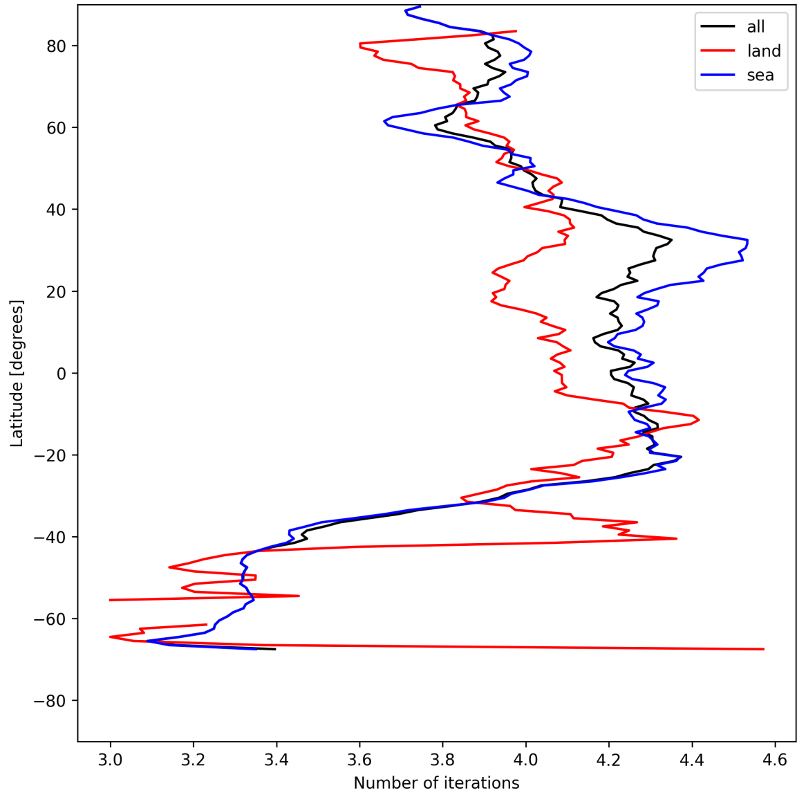
Figure 15: Zonal average of “Number of iterations” for 2025-07-20 to 2025-07-21.
