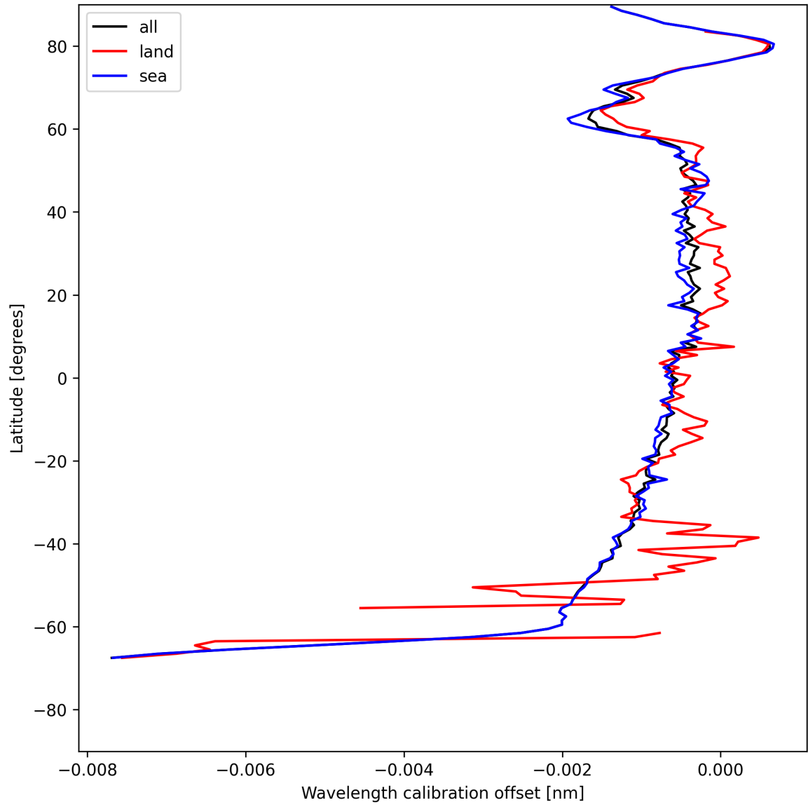
Figure 16: Zonal average of “Wavelength calibration offset” for 2025-07-20 to 2025-07-21.
