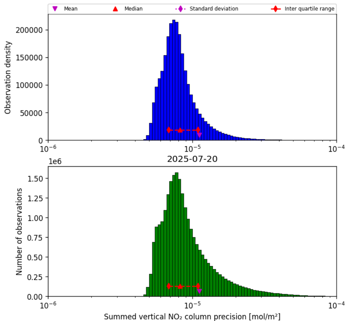
Figure 39: Histogram of “Summed vertical NO 2 column precision” for 2025-07-20 to 2025-07-21
