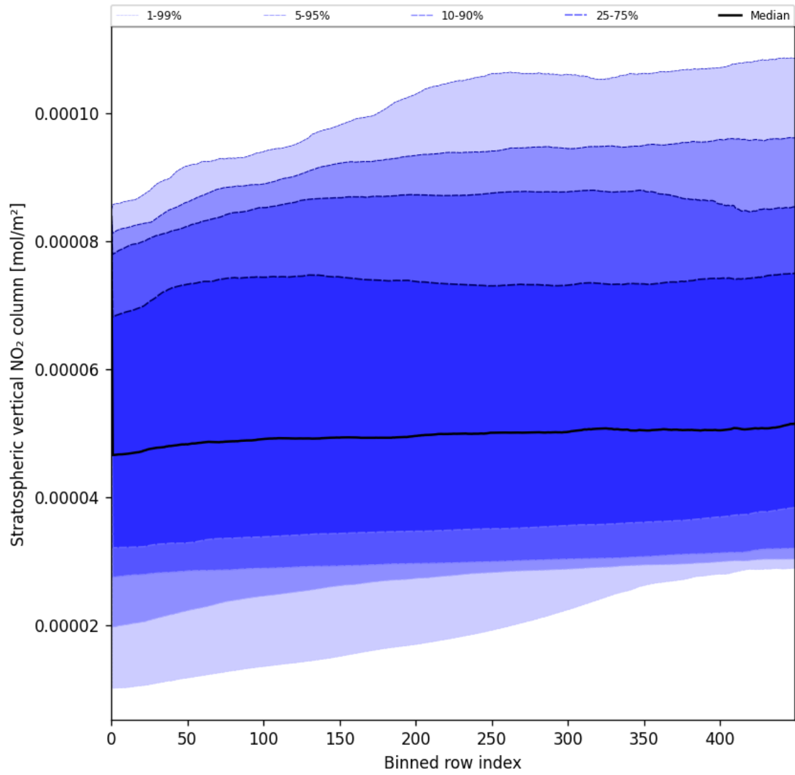
Figure 51: Along track statistics of “Stratospheric vertical NO 2 column” for 2025-07-20 to 2025-07-21
