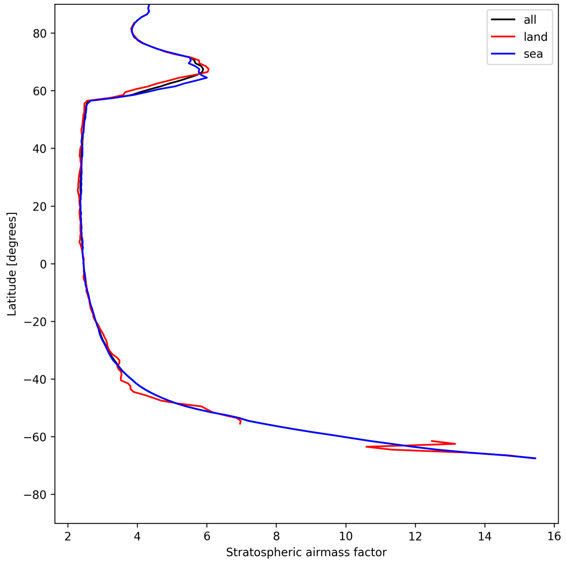
Figure 25: Zonal average of “Stratospheric airmass factor” for 2025-07-20 to 2025-07-21.
