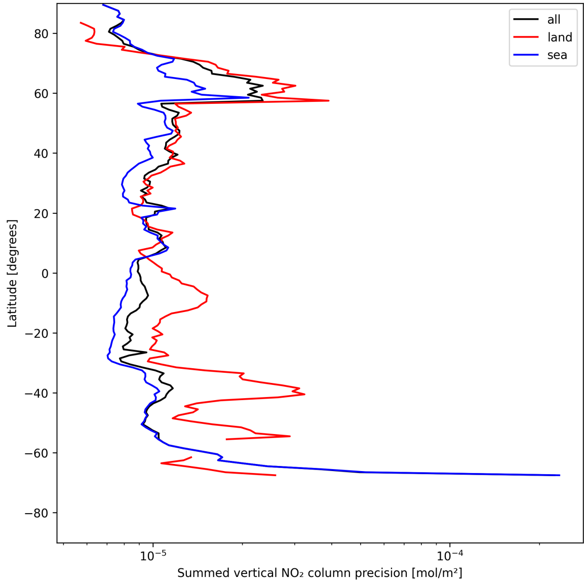
Figure 22: Zonal average of “Summed vertical NO 2 column precision” for 2025-07-20 to 2025-07-21.
