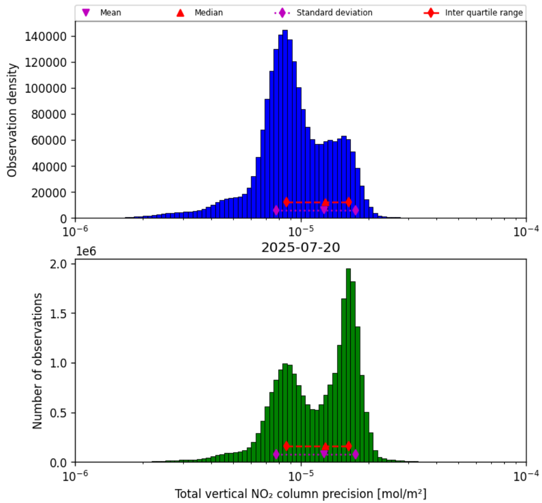
Figure 37: Histogram of “Total vertical NO 2 column precision” for 2025-07-20 to 2025-07-21
