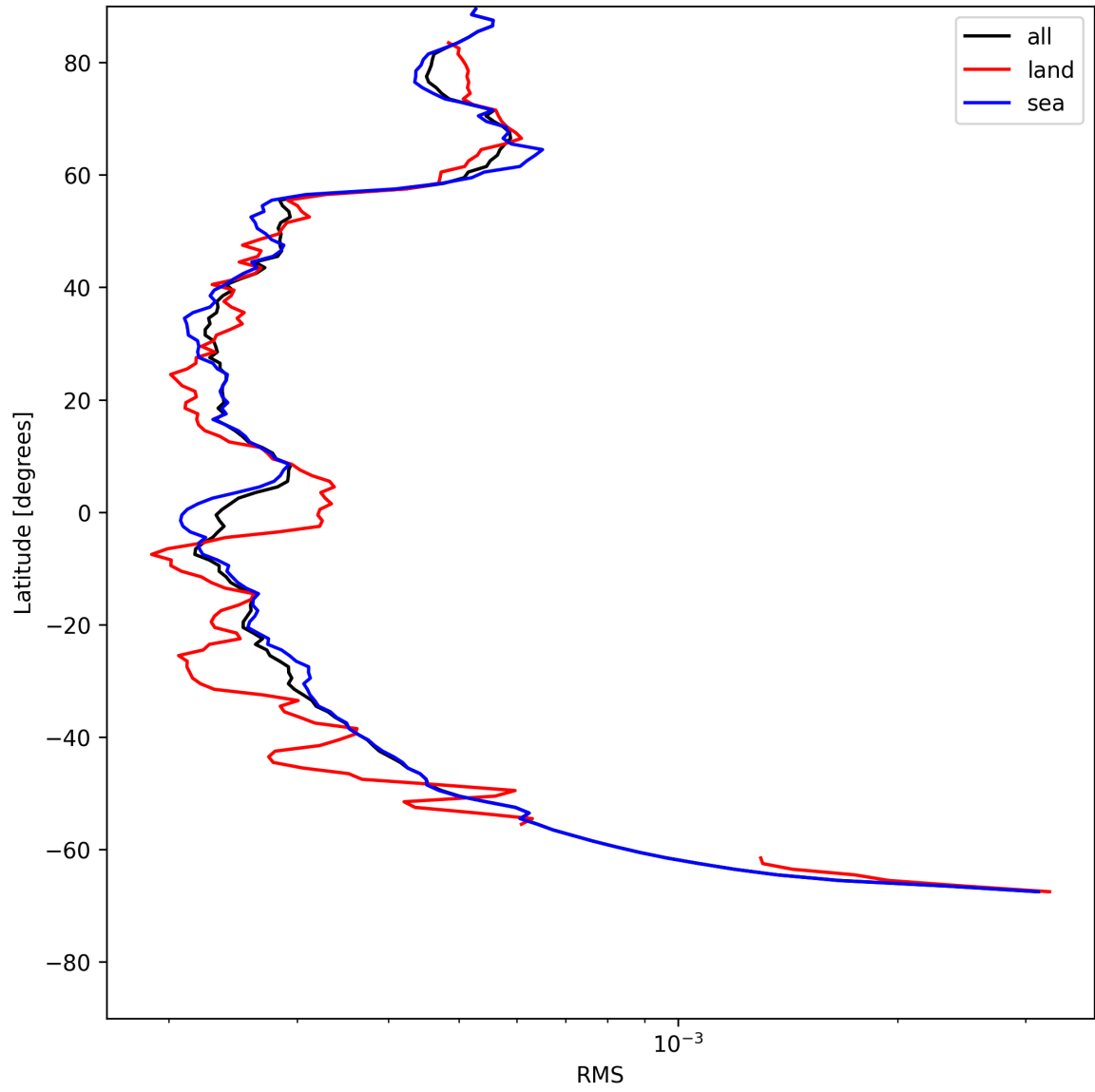
Figure 24: Zonal average of “RMS” for 2025-07-20 to 2025-07-21.
