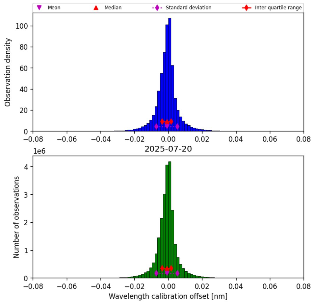
Figure 33: Histogram of “Wavelength calibration offset” for 2025-07-20 to 2025-07-21
