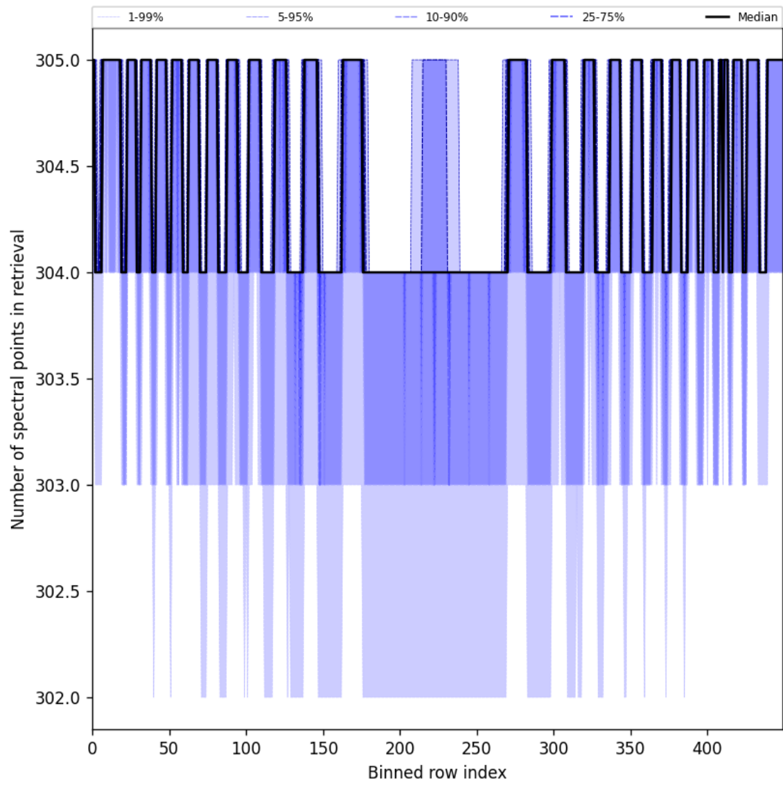
Figure 48: Along track statistics of “Number of spectral points in retrieval” for 2025-07-20 to 2025-07-21
