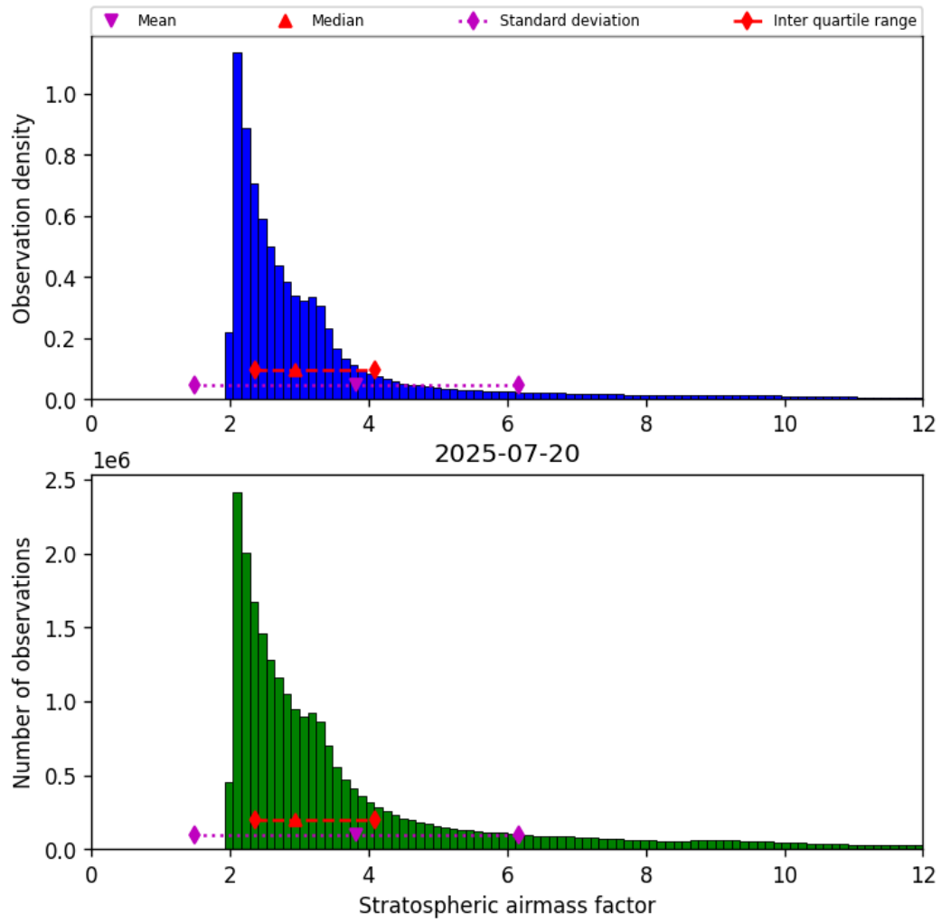
Figure 42: Histogram of “Stratospheric airmass factor” for 2025-07-20 to 2025-07-21
