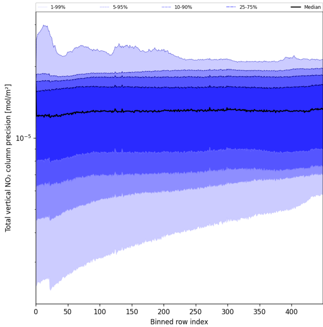
Figure 54: Along track statistics of “Total vertical NO 2 column precision” for 2025-07-20 to 2025-07-21
