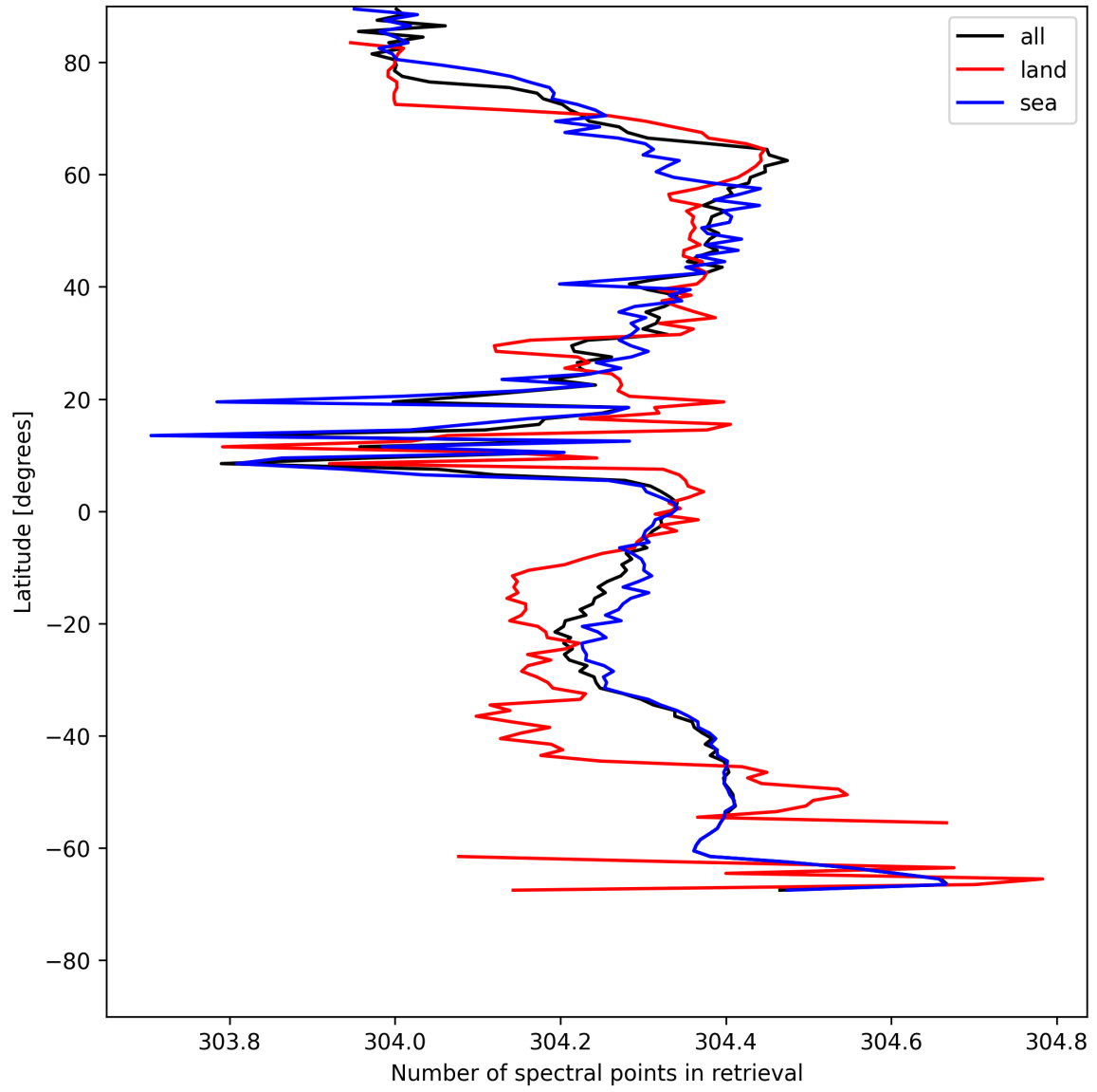
Figure 14: Zonal average of “Number of spectral points in retrieval” for 2025-07-20 to 2025-07-21.
