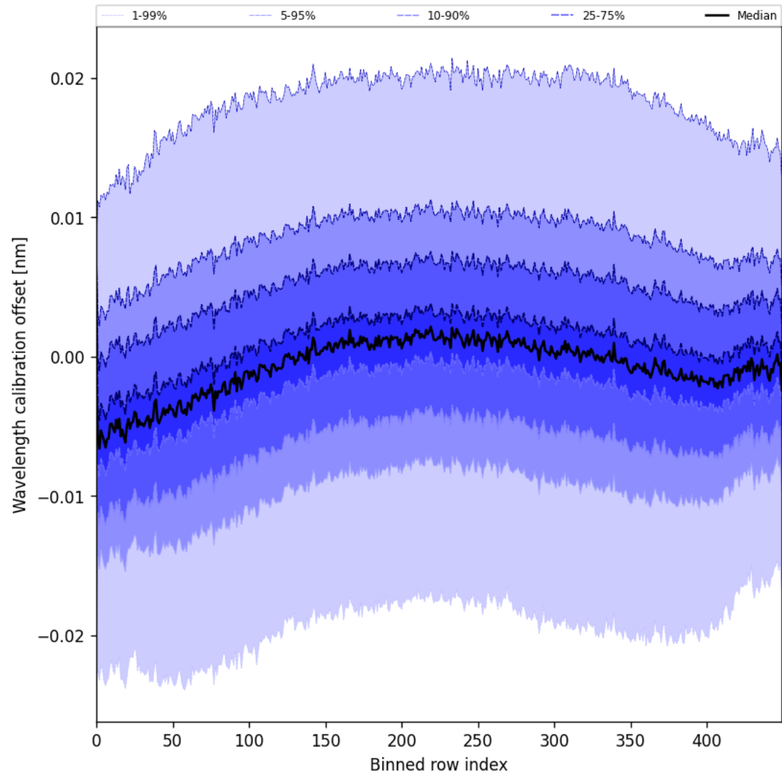
Figure 50: Along track statistics of “Wavelength calibration offset” for 2025-07-20 to 2025-07-21
