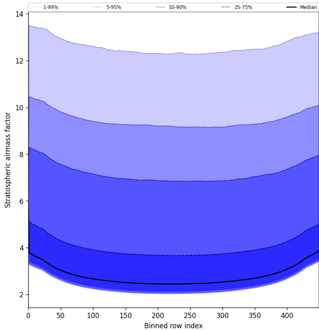
Figure 59: Along track statistics of “Stratospheric airmass factor” for 2025-07-20 to 2025-07-21
