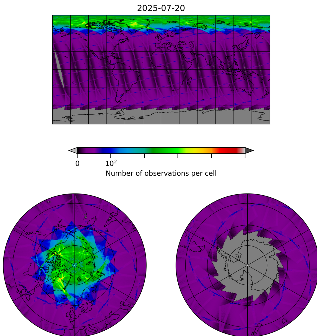
Figure 8: Map of the number of observations for 2025-07-20 to 2025-07-21
