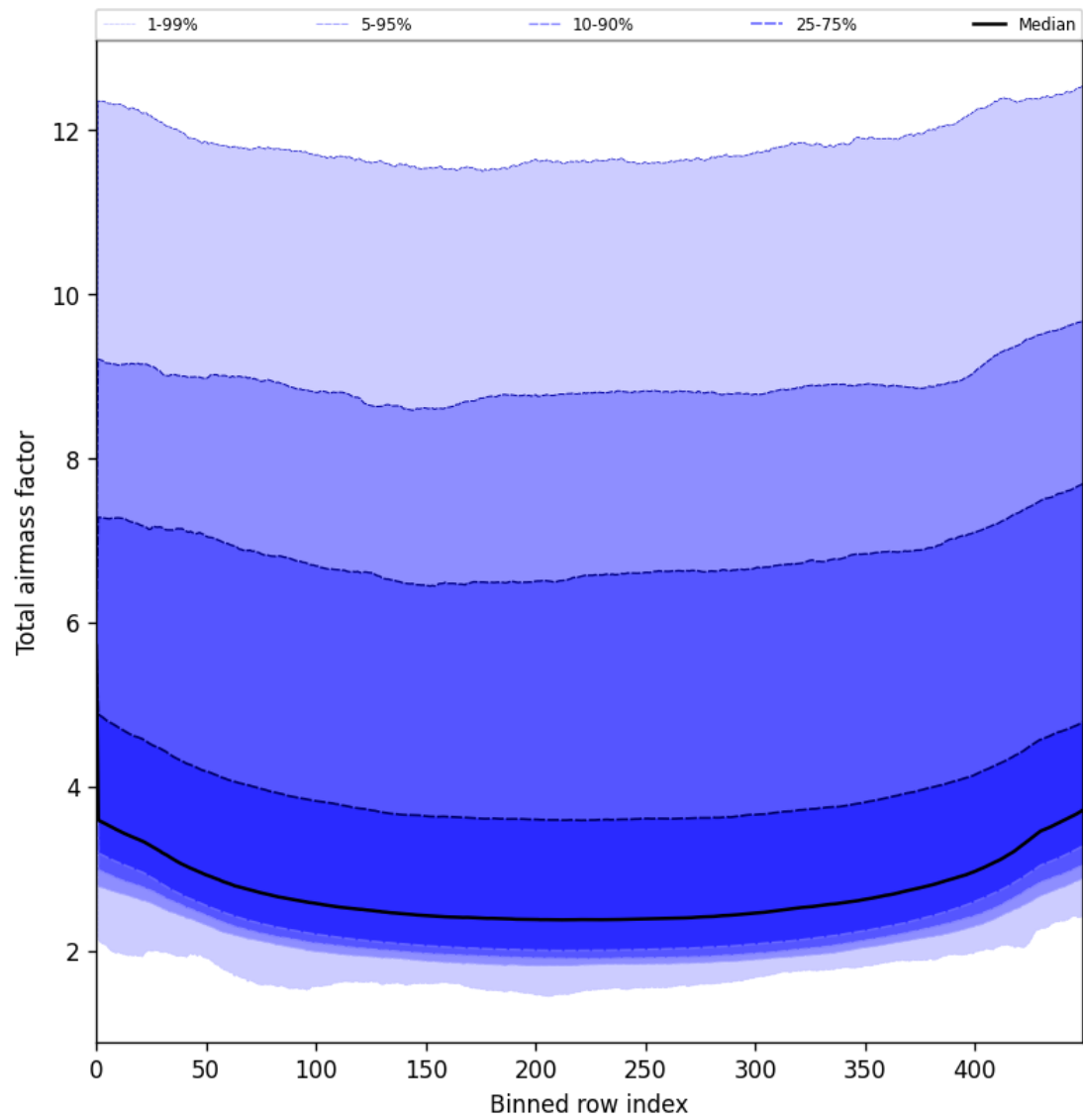
Figure 47: Along track statistics of “Total airmass factor” for 2025-07-20 to 2025-07-21
