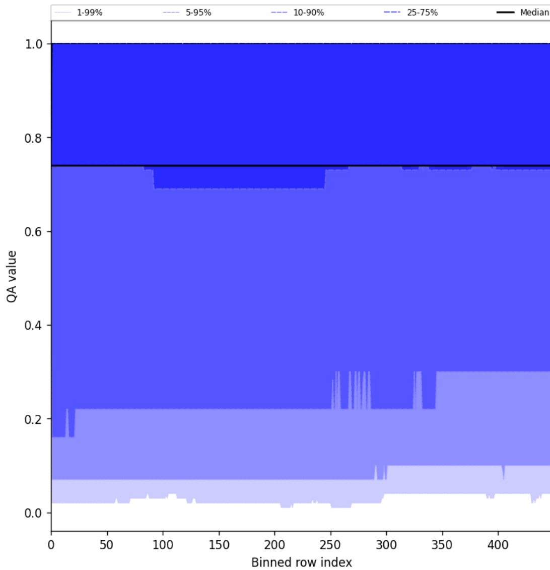
Figure 43: Along track statistics of “QA value” for 2025-07-20 to 2025-07-21
