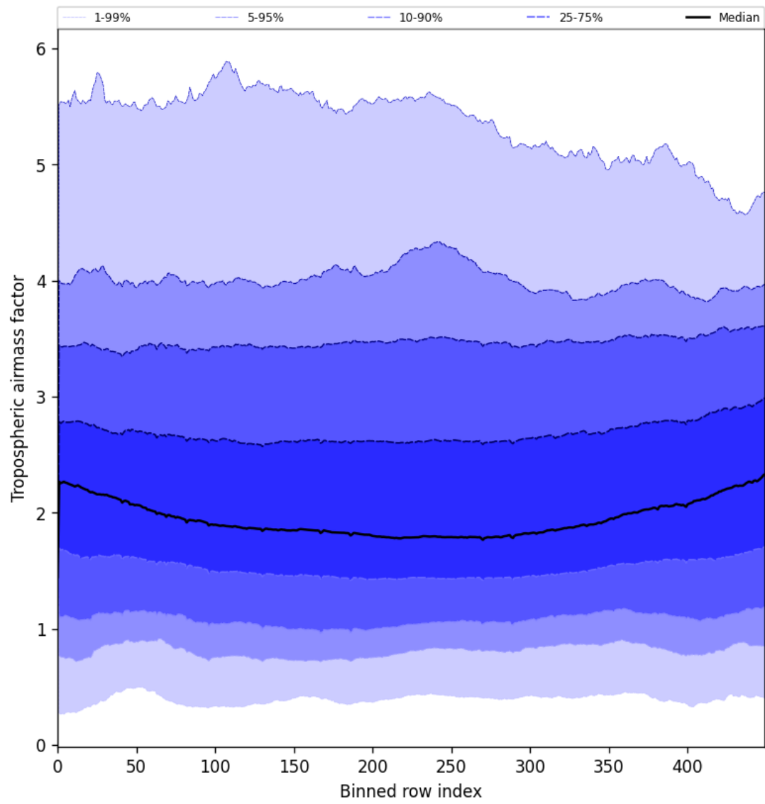
Figure 46: Along track statistics of “Tropospheric airmass factor” for 2025-07-20 to 2025-07-21
