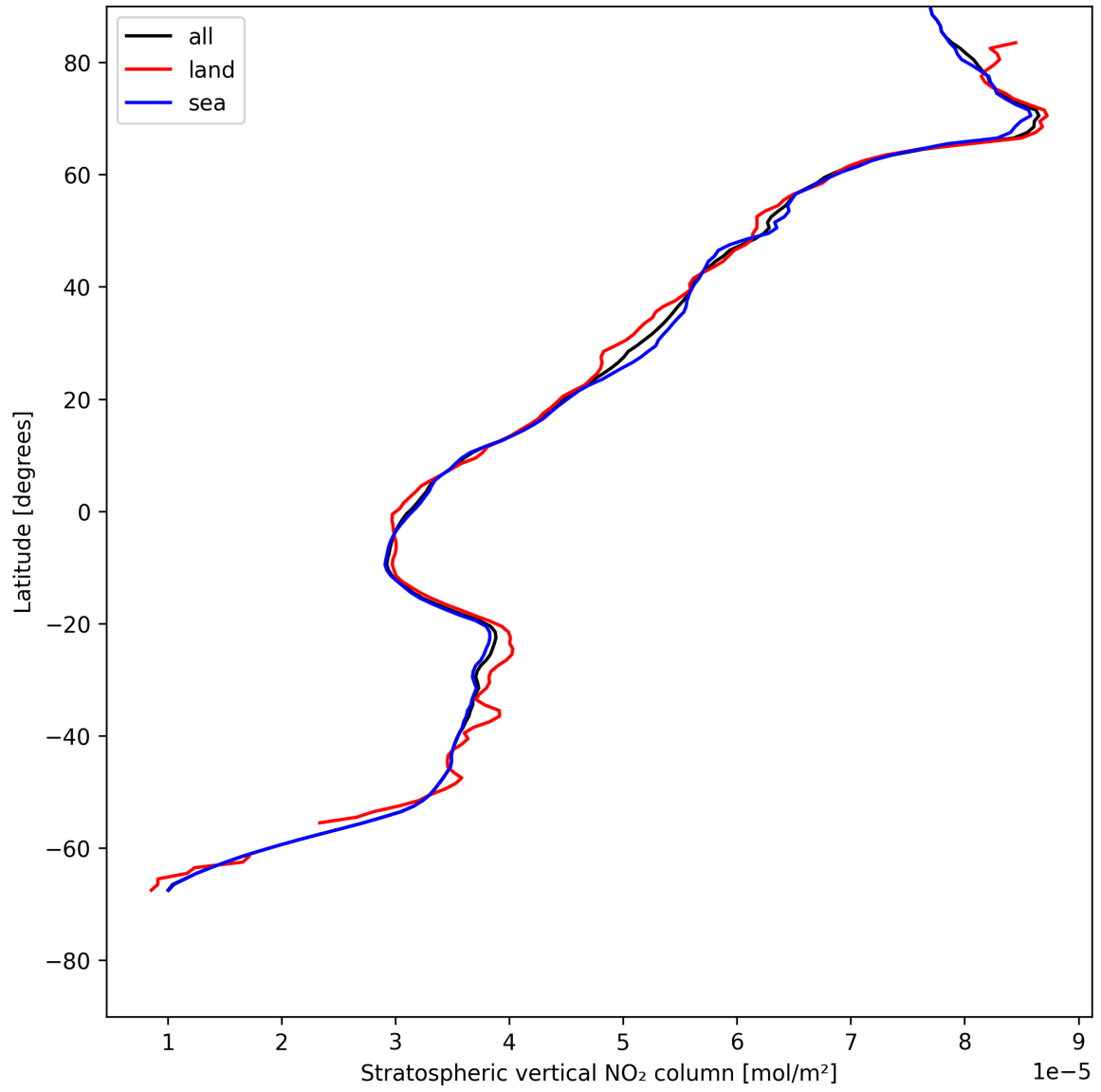
Figure 17: Zonal average of “Stratospheric vertical NO 2 column” for 2025-07-20 to 2025-07-21.
