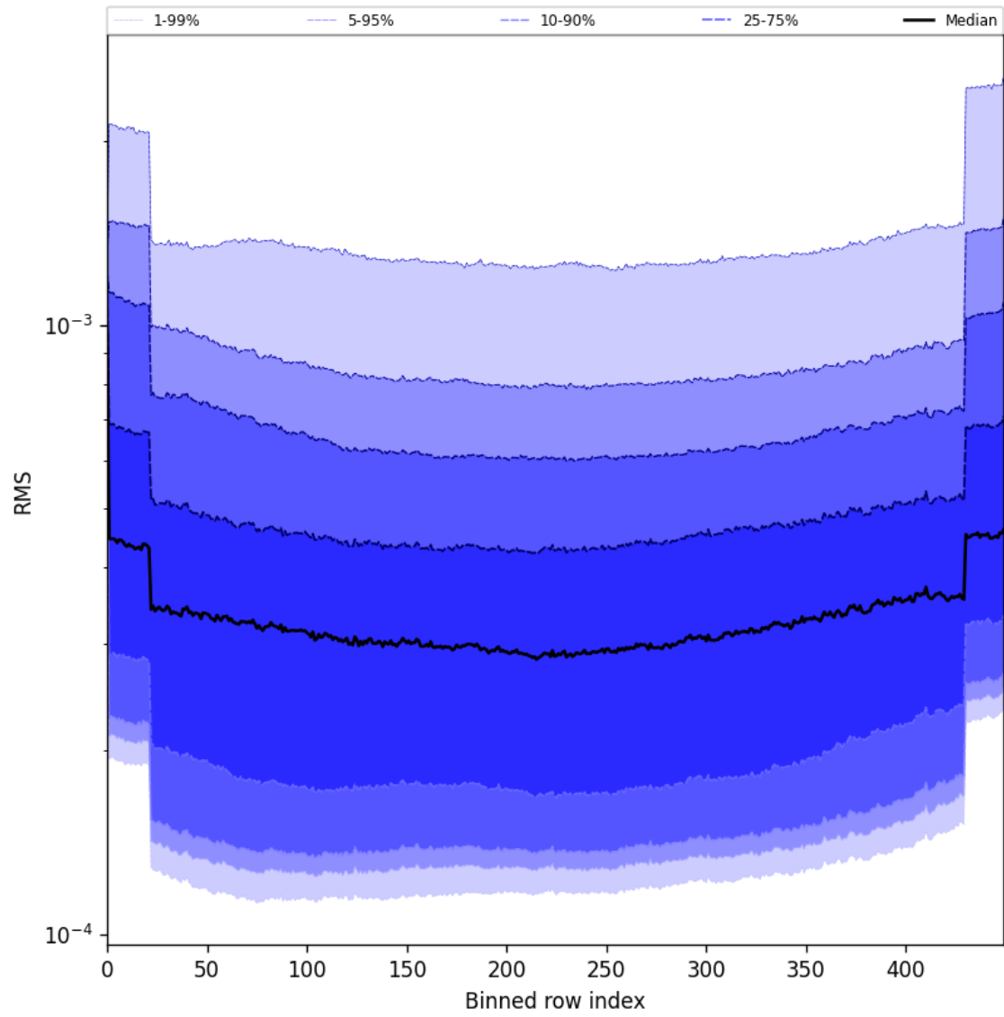
Figure 58: Along track statistics of “RMS” for 2025-07-20 to 2025-07-21
