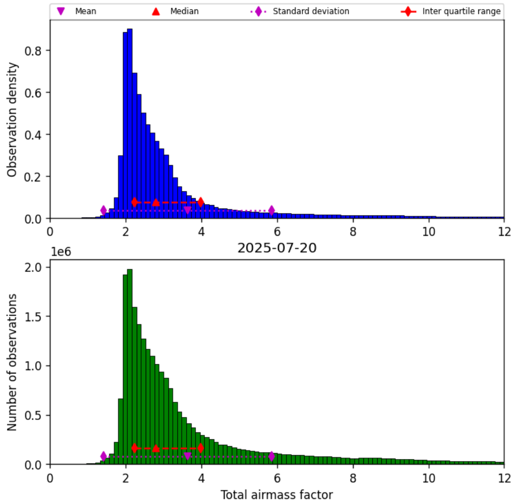
Figure 30: Histogram of “Total airmass factor” for 2025-07-20 to 2025-07-21
