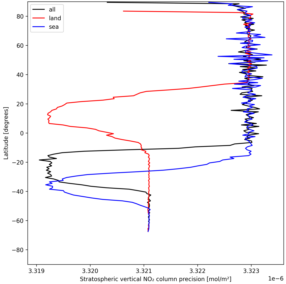
Figure 18: Zonal average of “Stratospheric vertical NO 2 column precision” for 2025-07-20 to 2025-07-21.
