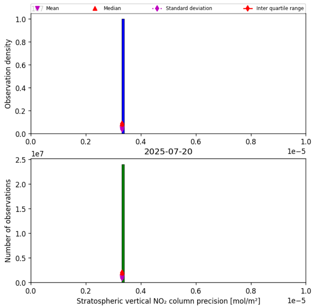
Figure 35: Histogram of “Stratospheric vertical NO 2 column precision” for 2025-07-20 to 2025-07-21
