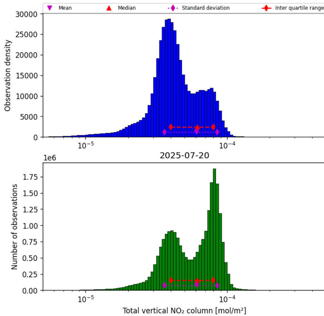
Figure 36: Histogram of "Total vertical NO 2 column" for 2025-07-20 to 2025-07-21
