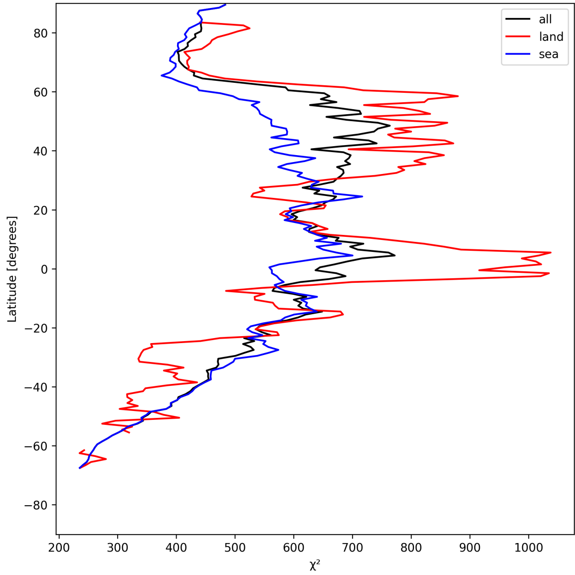
Figure 23: Zonal average of “ \chi^2 ” for 2025-07-20 to 2025-07-21.
