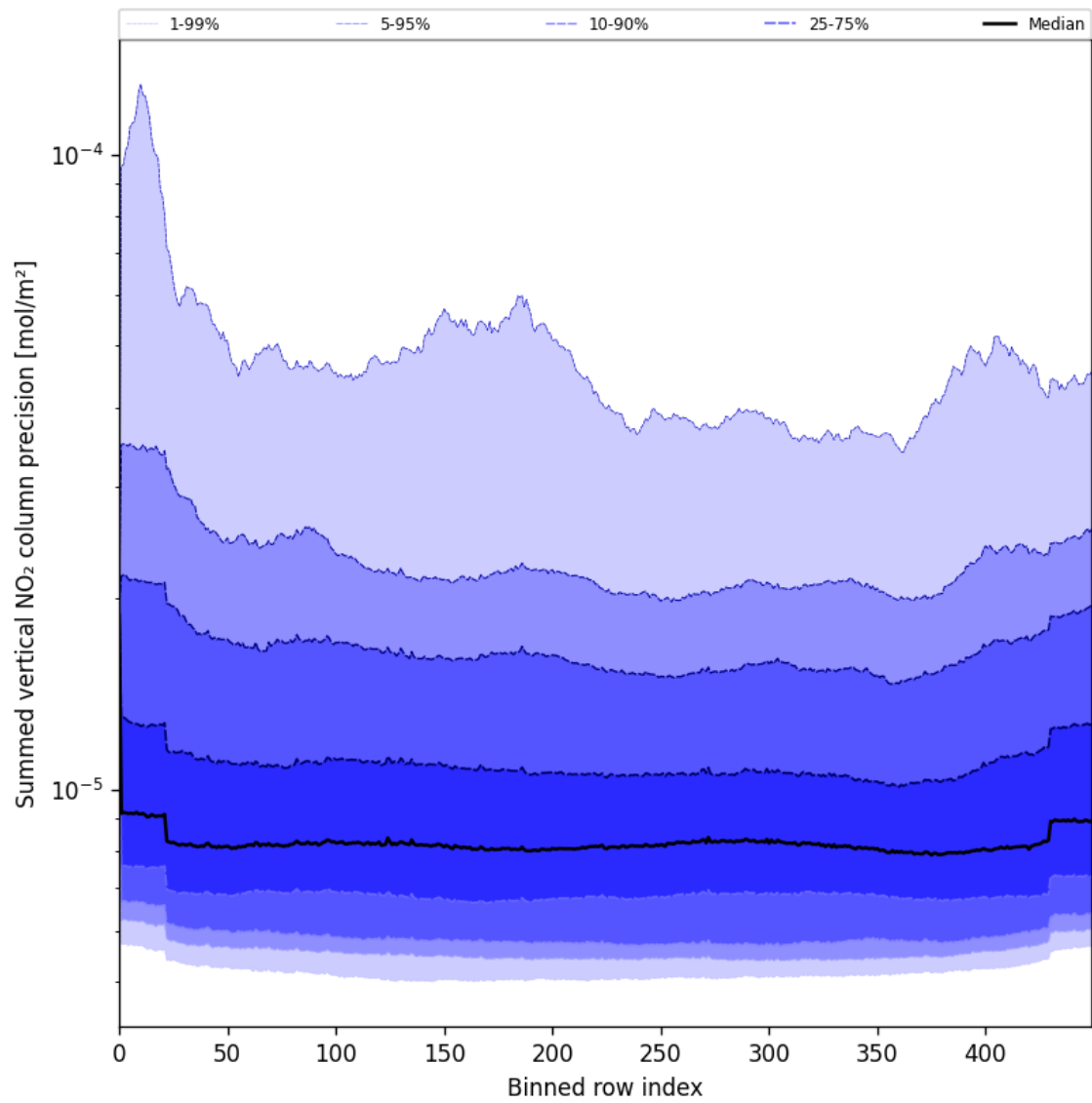
Figure 56: Along track statistics of “Summed vertical NO 2 column precision” for 2025-07-20 to 2025-07-21
