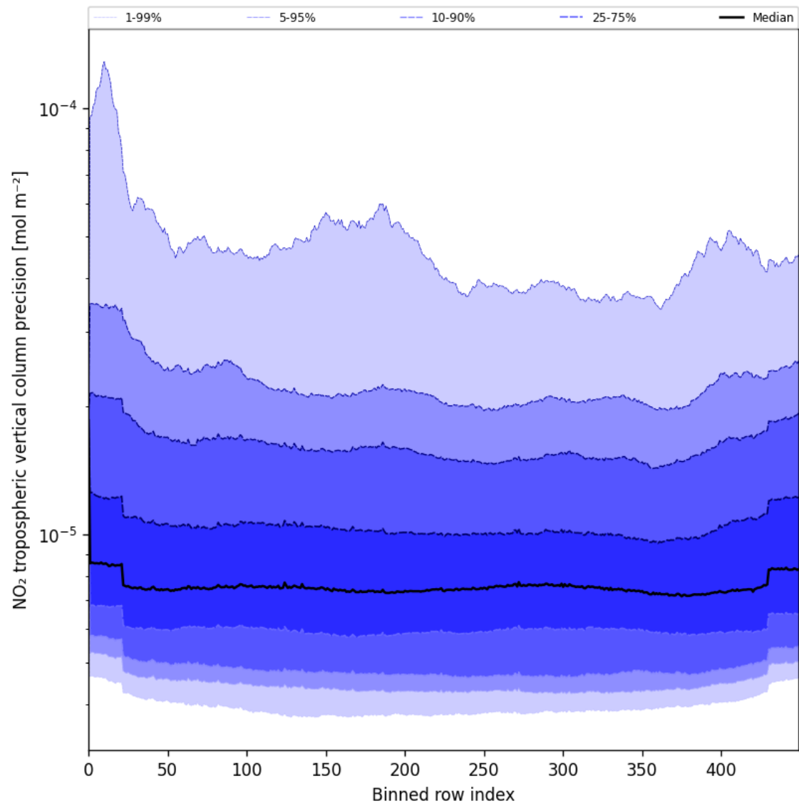
Figure 45: Along track statistics of “NO 2 tropospheric vertical column precision” for 2025-07-20 to 2025-07-21
