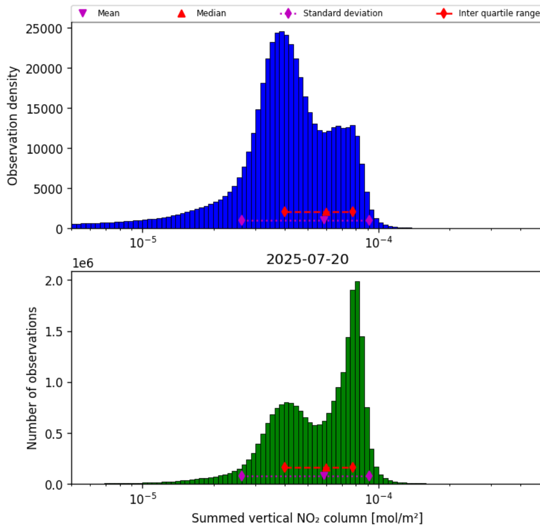
Figure 38: Histogram of “Summed vertical NO 2 column” for 2025-07-20 to 2025-07-21
