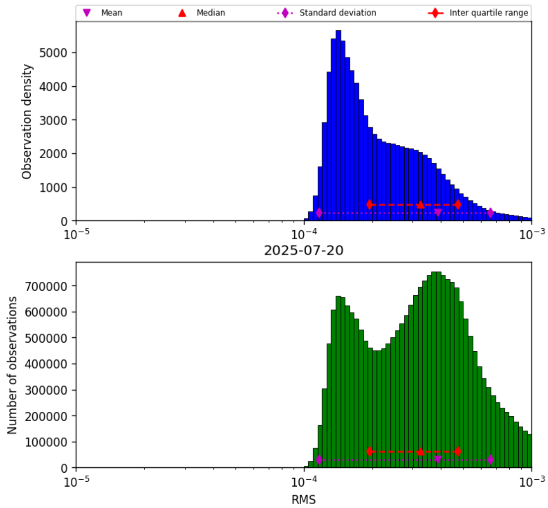
Figure 41: Histogram of “RMS” for 2025-07-20 to 2025-07-21
