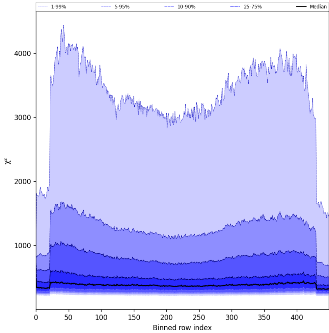
Figure 57: Along track statistics of “ \chi^2 ” for 2025-07-20 to 2025-07-21
