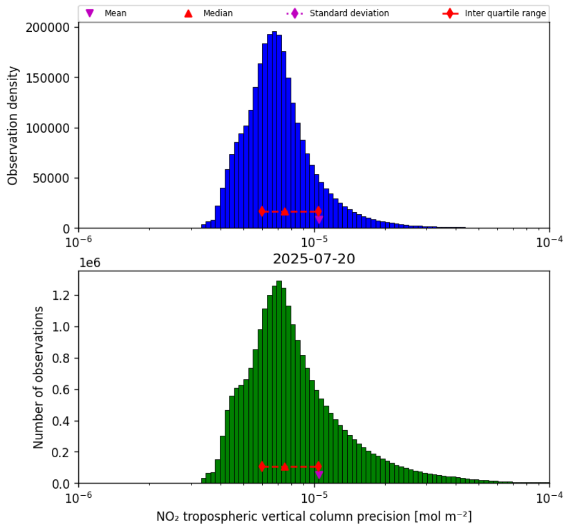
Figure 28: Histogram of “NO 2 tropospheric vertical column precision” for 2025-07-20 to 2025-07-21
