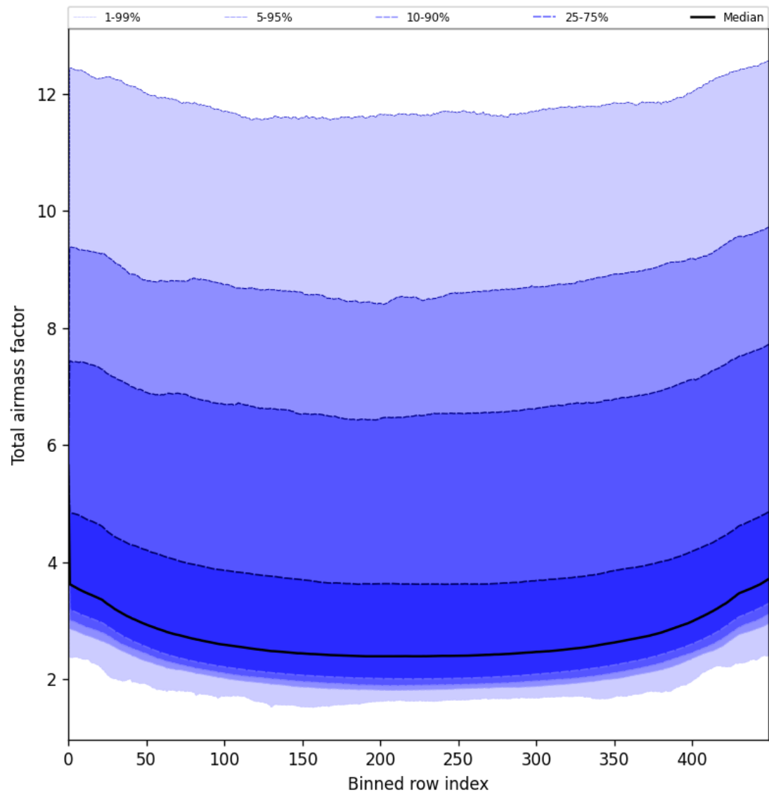
Figure 47: Along track statistics of “Total airmass factor” for 2025-07-21 to 2025-07-22
