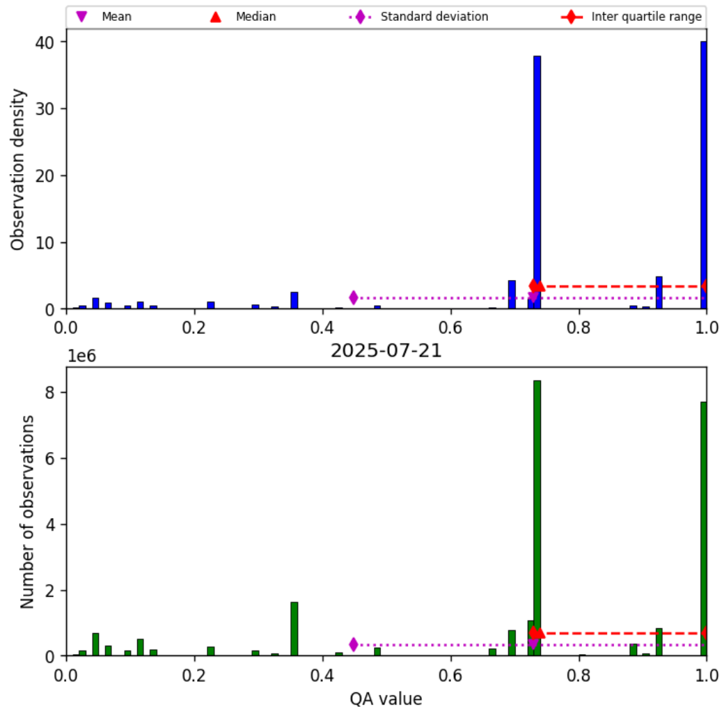
Figure 26: Histogram of “QA value” for 2025-07-21 to 2025-07-22
