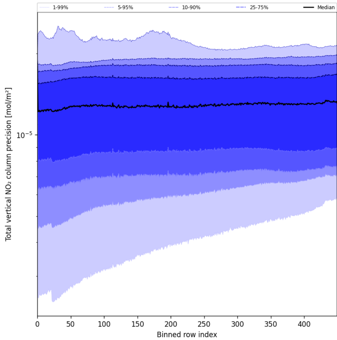
Figure 54: Along track statistics of “Total vertical NO 2 column precision” for 2025-07-21 to 2025-07-22
