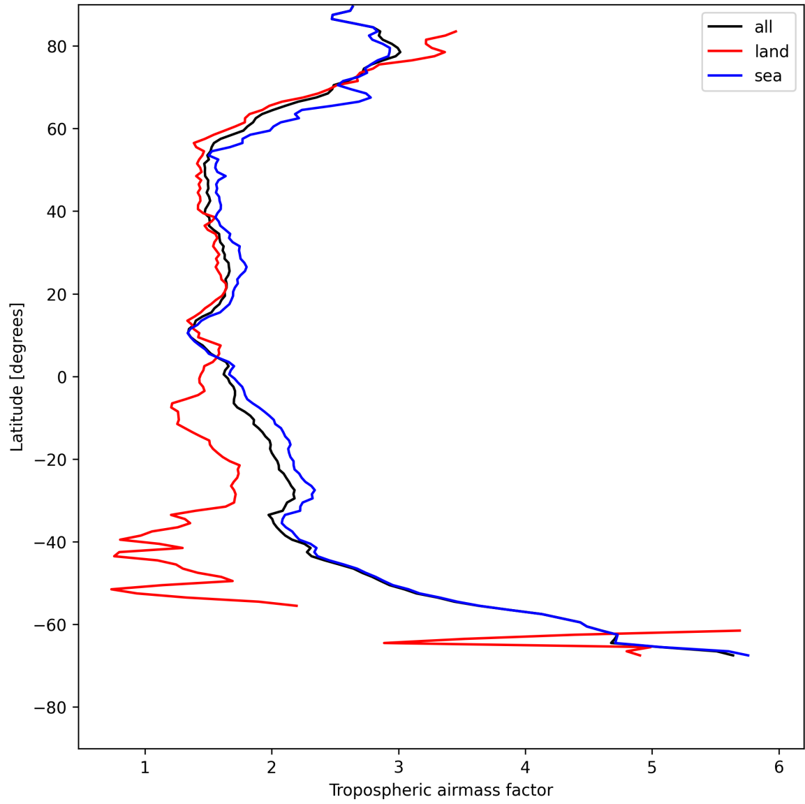
Figure 12: Zonal average of “Tropospheric air mass factor” for 2025-07-21 to 2025-07-22.
