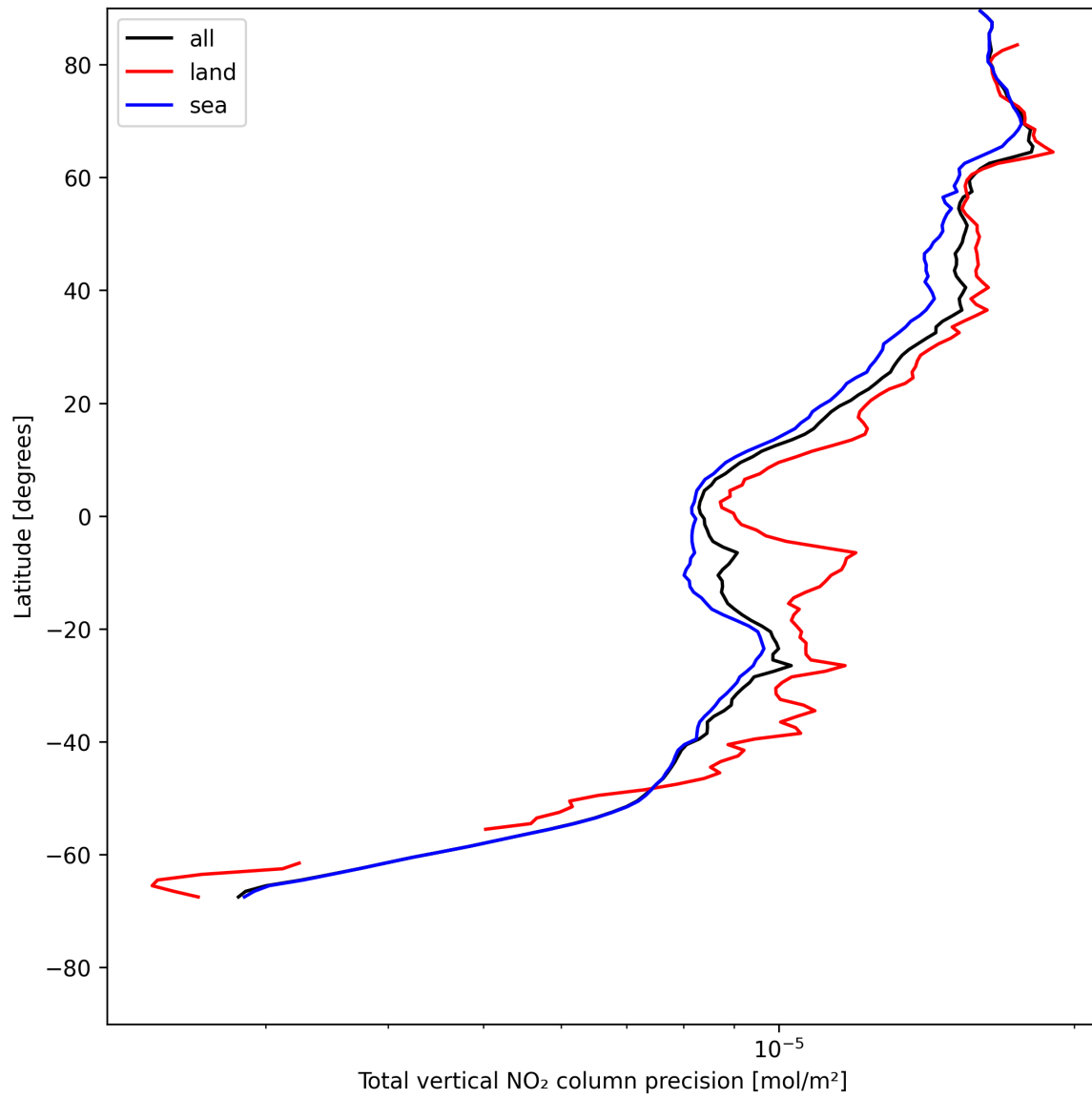
Figure 20: Zonal average of “Total vertical NO 2 column precision” for 2025-07-21 to 2025-07-22.
