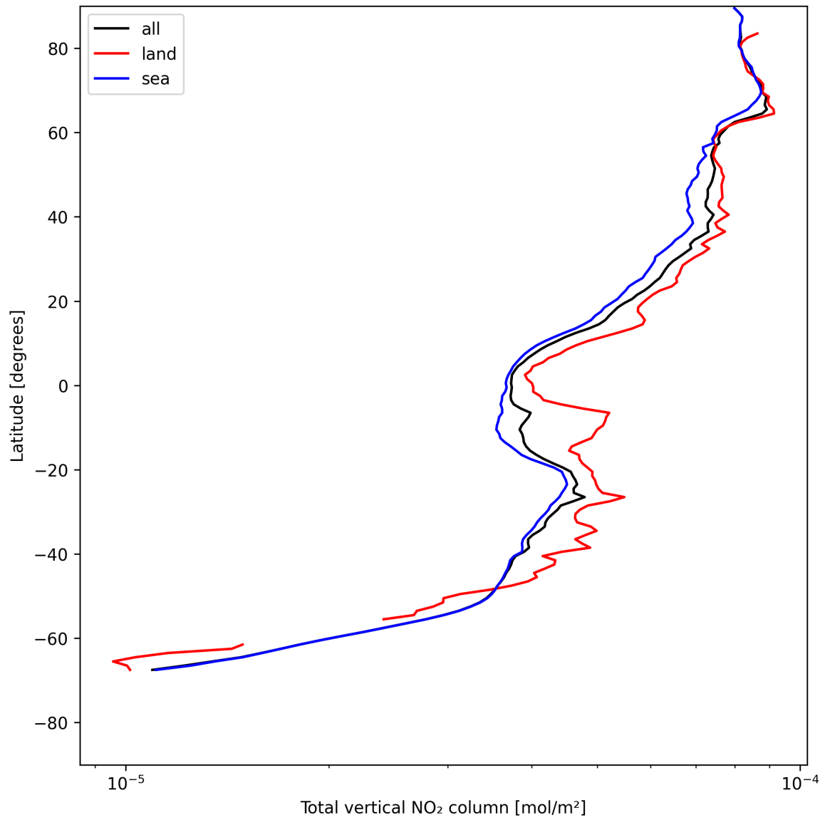
Figure 19: Zonal average of “Total vertical NO 2 column” for 2025-07-21 to 2025-07-22.
