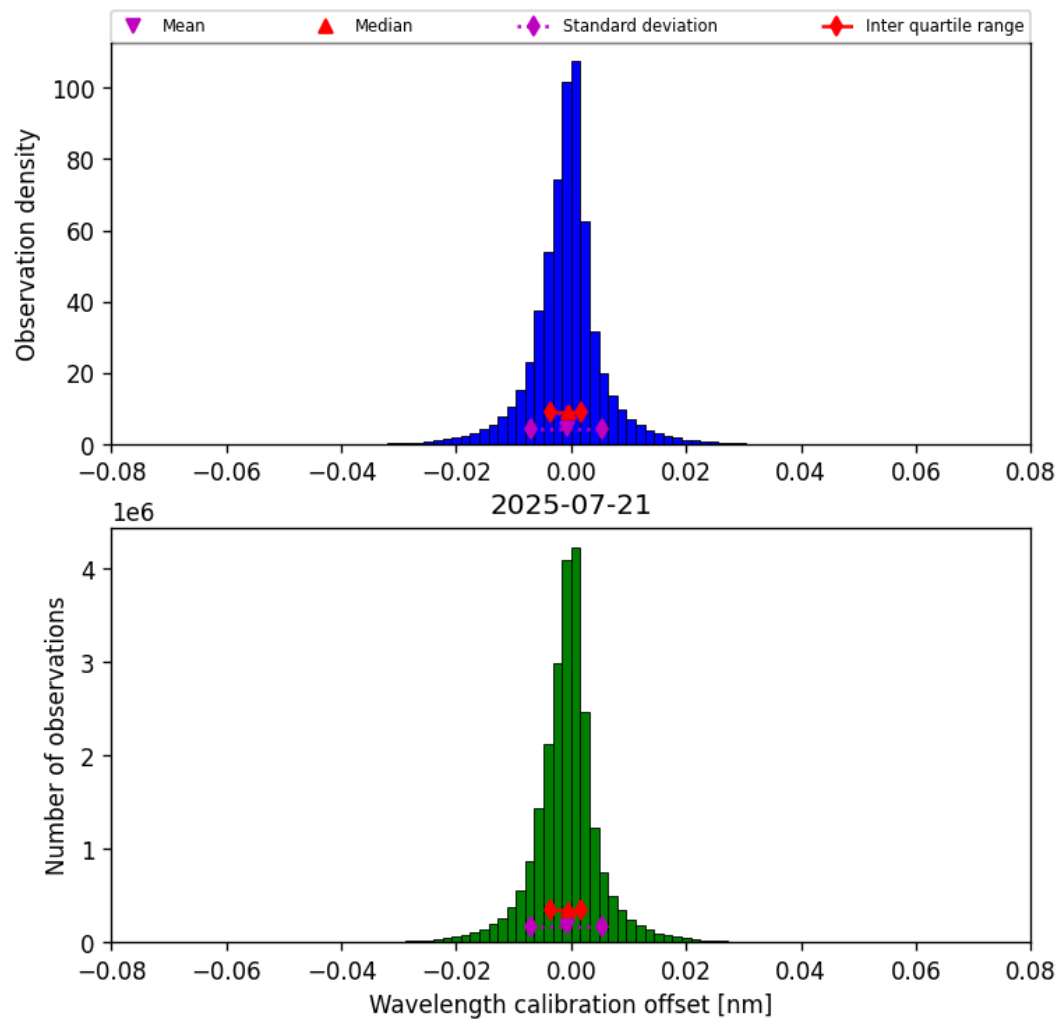
Figure 33: Histogram of “Wavelength calibration offset” for 2025-07-21 to 2025-07-22
