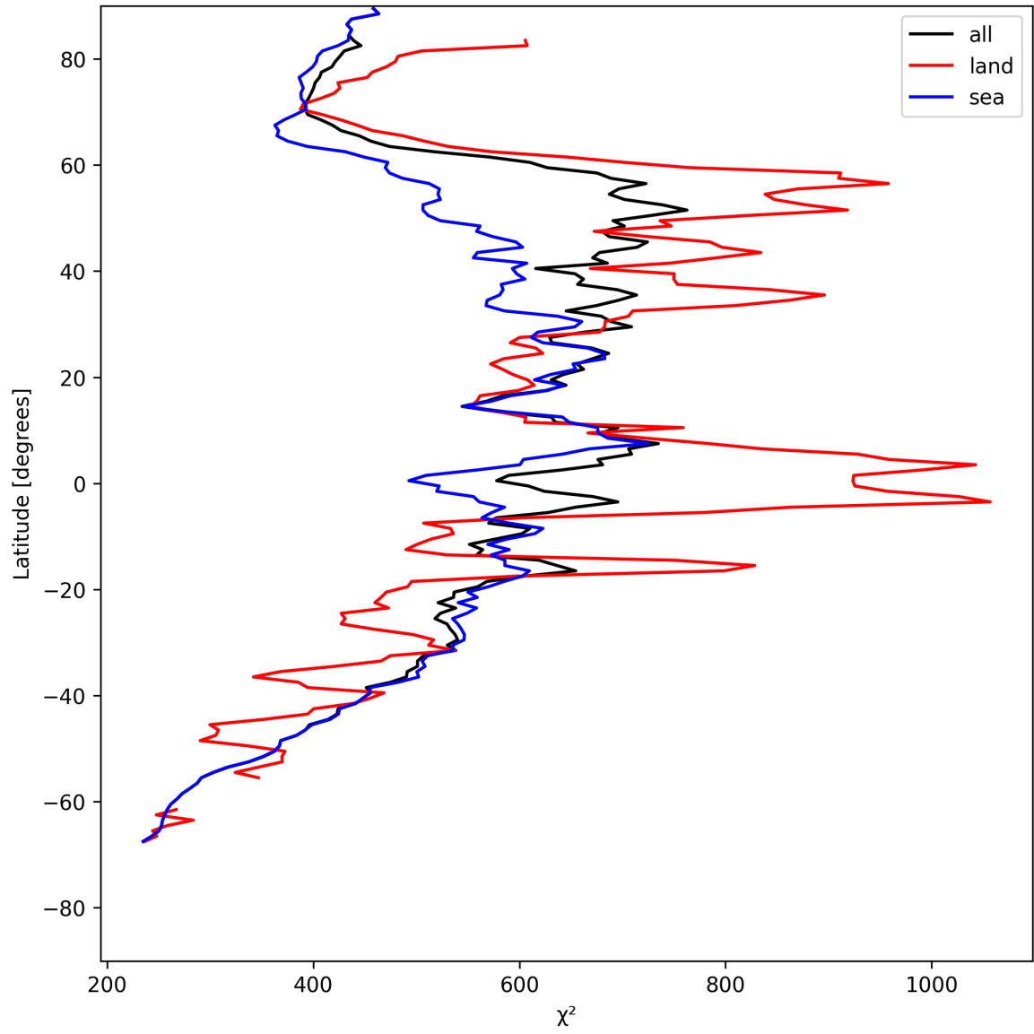
Figure 23: Zonal average of “ \chi^2 ” for 2025-07-21 to 2025-07-22.
