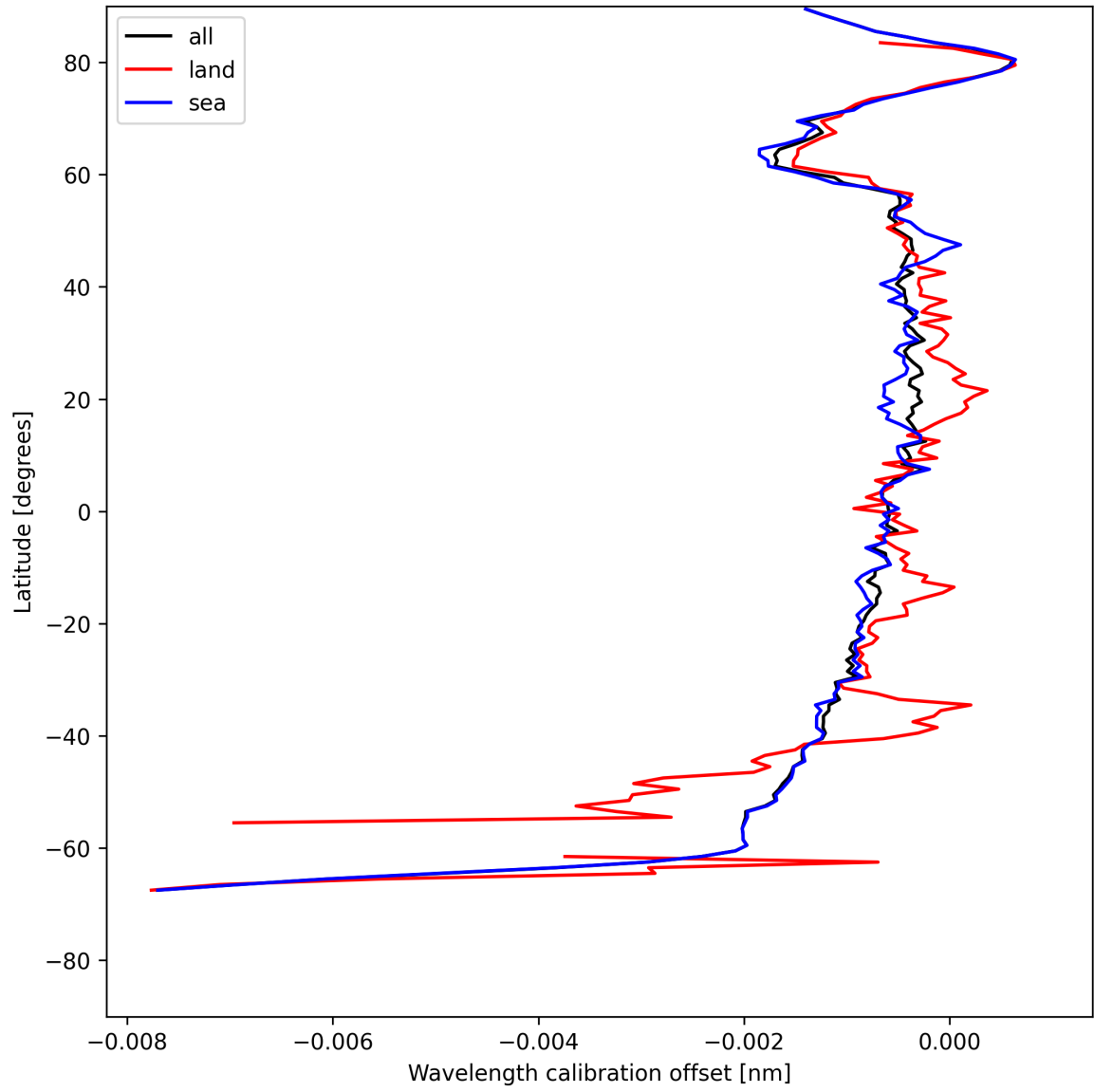
Figure 16: Zonal average of “Wavelength calibration offset” for 2025-07-21 to 2025-07-22.
