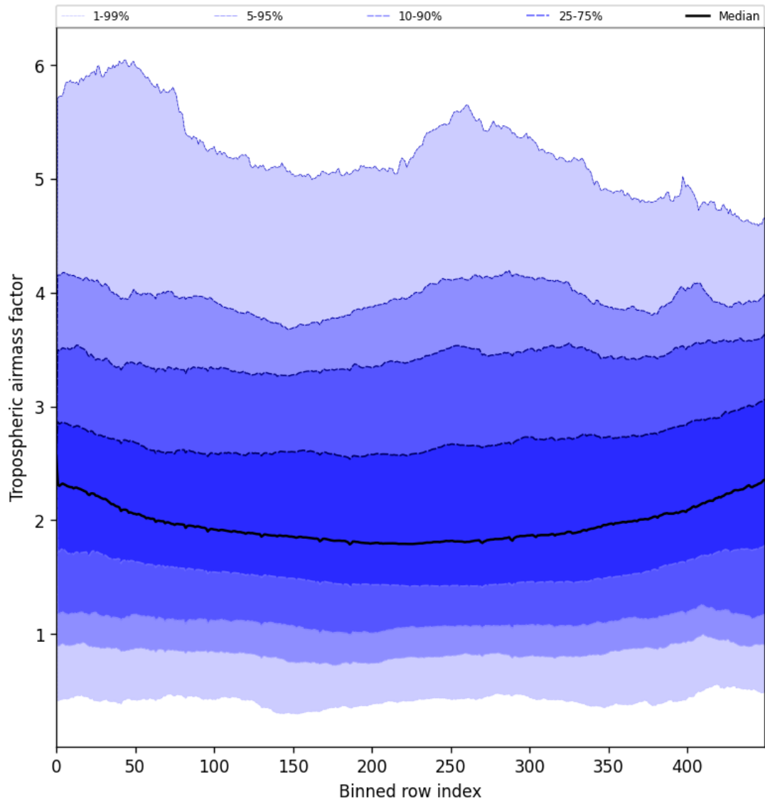
Figure 46: Along track statistics of “Tropospheric airmass factor” for 2025-07-21 to 2025-07-22
