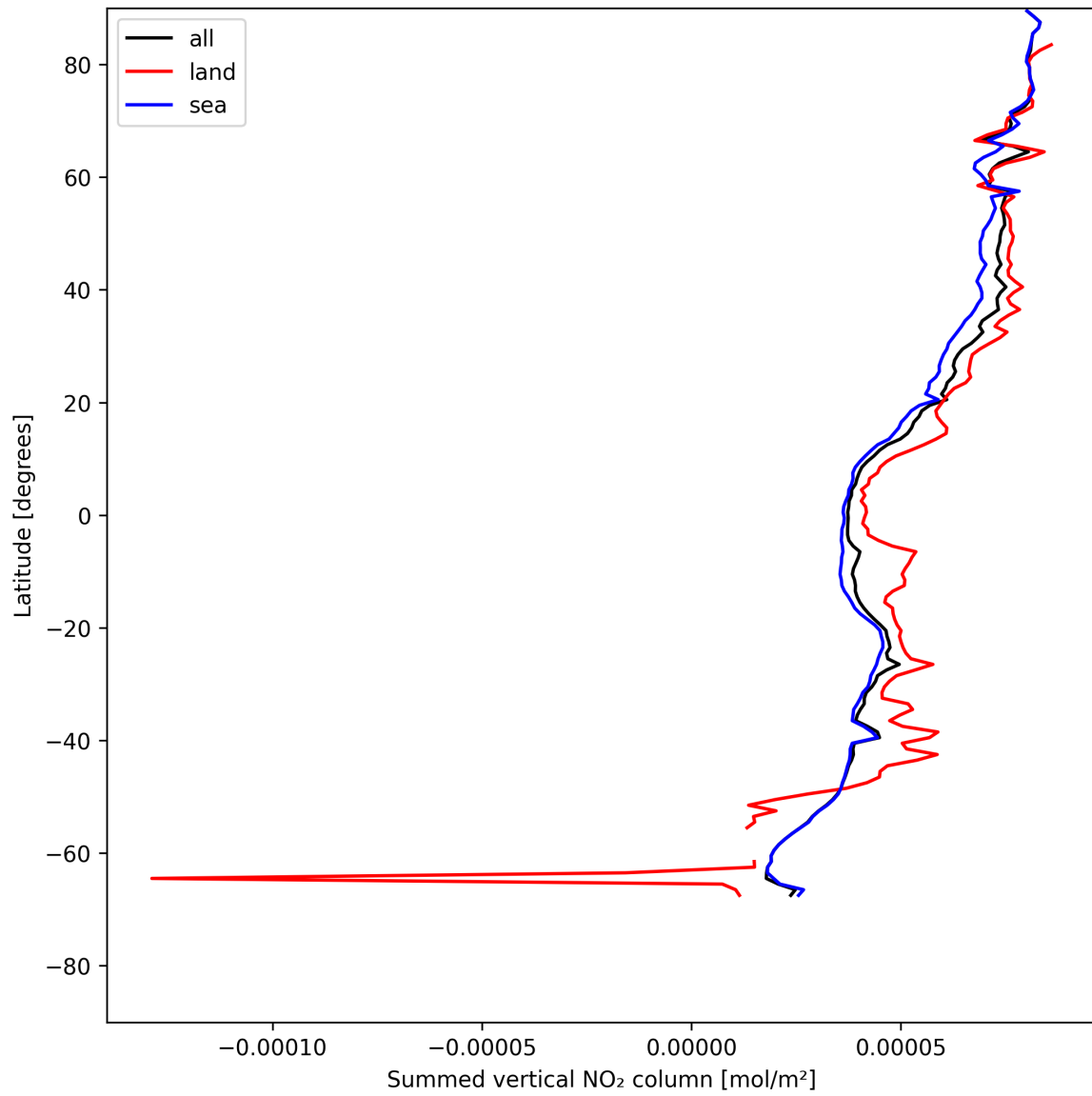
Figure 21: Zonal average of “Summed vertical NO 2 column” for 2025-07-21 to 2025-07-22.
