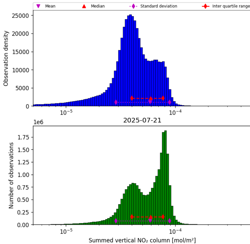
Figure 38: Histogram of “Summed vertical NO 2 column” for 2025-07-21 to 2025-07-22
