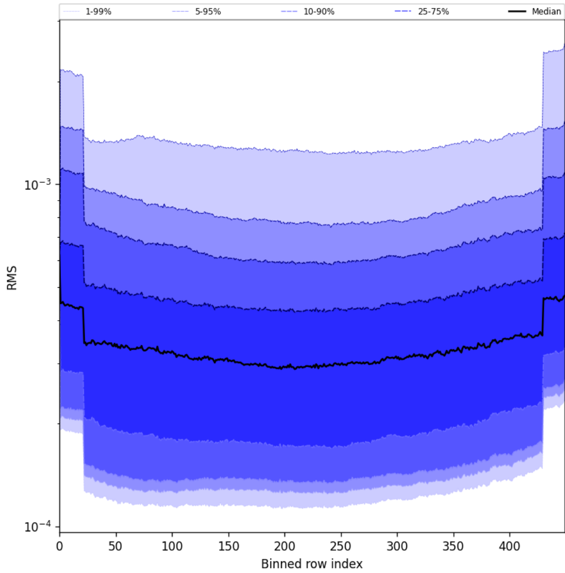
Figure 58: Along track statistics of “RMS” for 2025-07-21 to 2025-07-22
