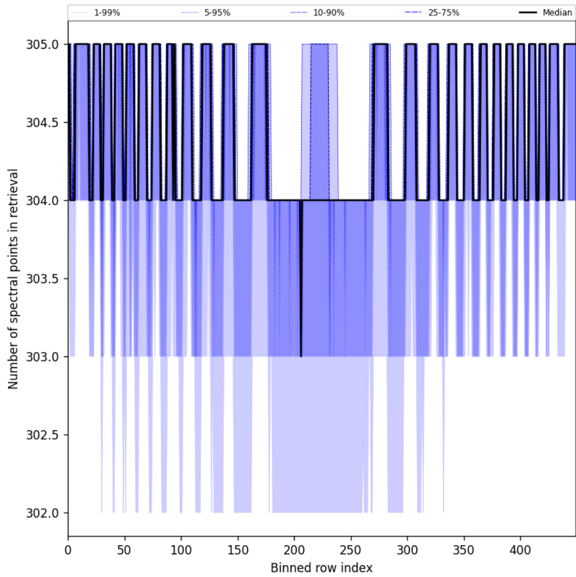
Figure 48: Along track statistics of “Number of spectral points in retrieval” for 2025-07-21 to 2025-07-22
