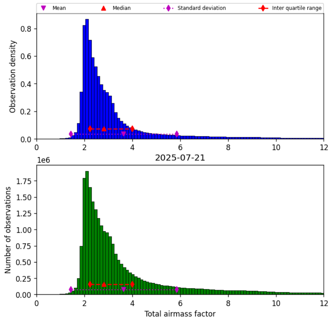
Figure 30: Histogram of “Total airmass factor” for 2025-07-21 to 2025-07-22
