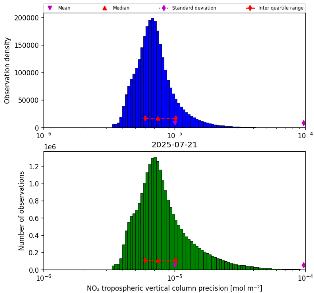
Figure 28: Histogram of “NO 2 tropospheric vertical column precision” for 2025-07-21 to 2025-07-22
