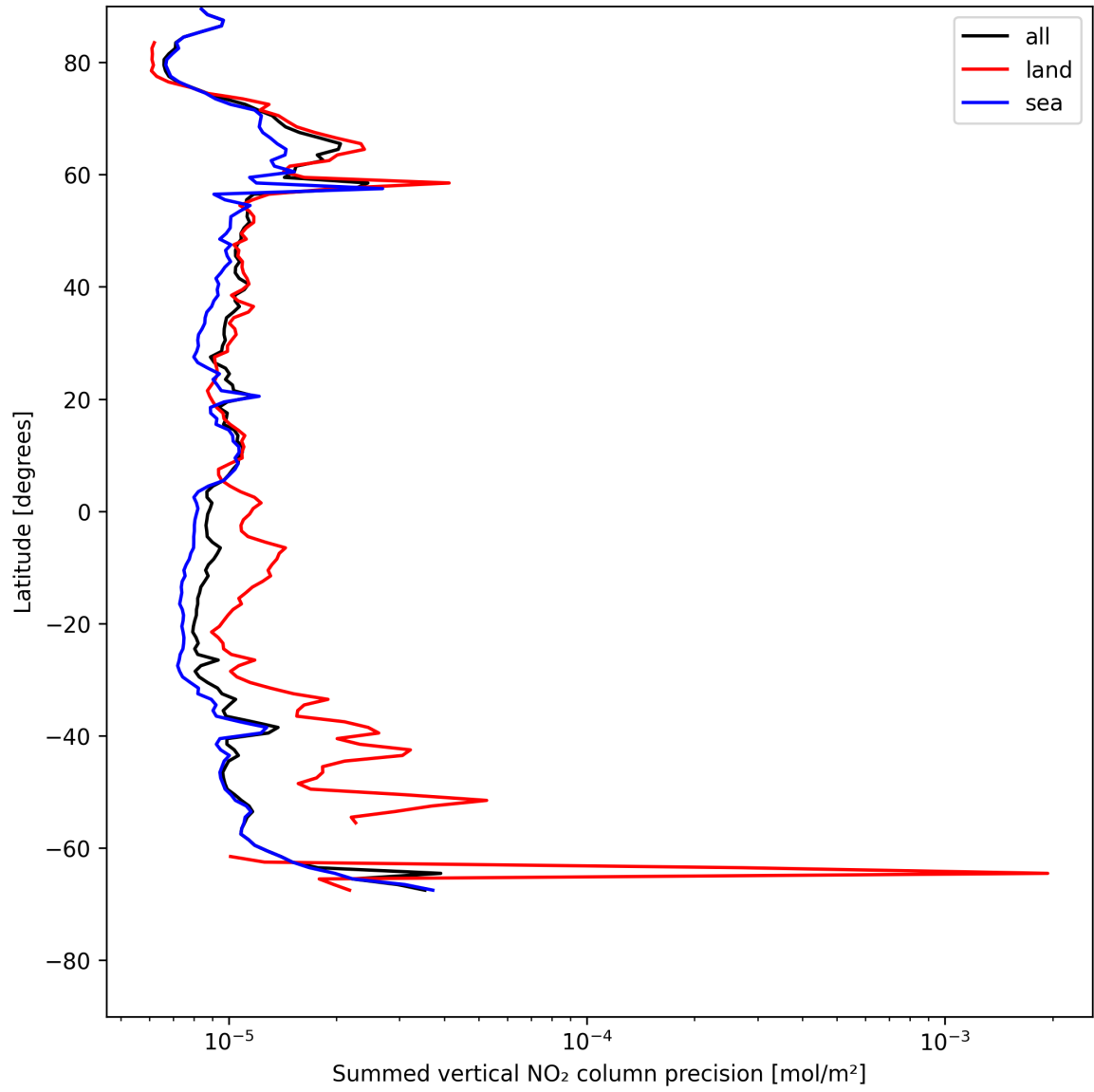
Figure 22: Zonal average of “Summed vertical NO 2 column precision” for 2025-07-21 to 2025-07-22.
