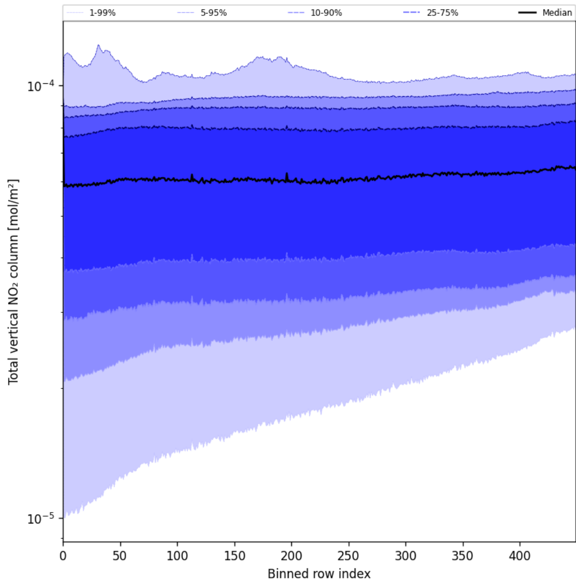
Figure 53: Along track statistics of “Total vertical NO 2 column” for 2025-07-21 to 2025-07-22
