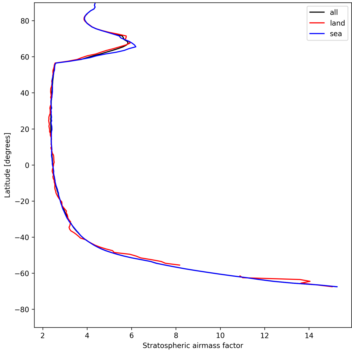
Figure 25: Zonal average of “Stratospheric airmass factor” for 2025-07-21 to 2025-07-22.
