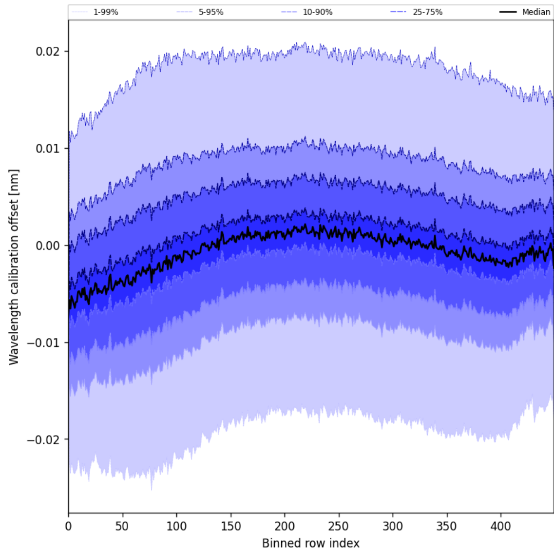
Figure 50: Along track statistics of “Wavelength calibration offset” for 2025-07-21 to 2025-07-22
