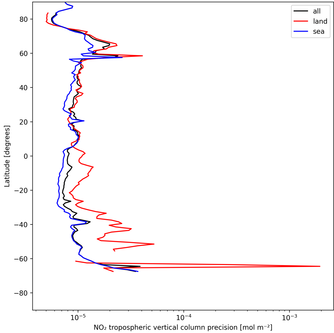
Figure 11: Zonal average of “NO 2 tropospheric vertical column precision” for 2025-07-21 to 2025-07-22.
