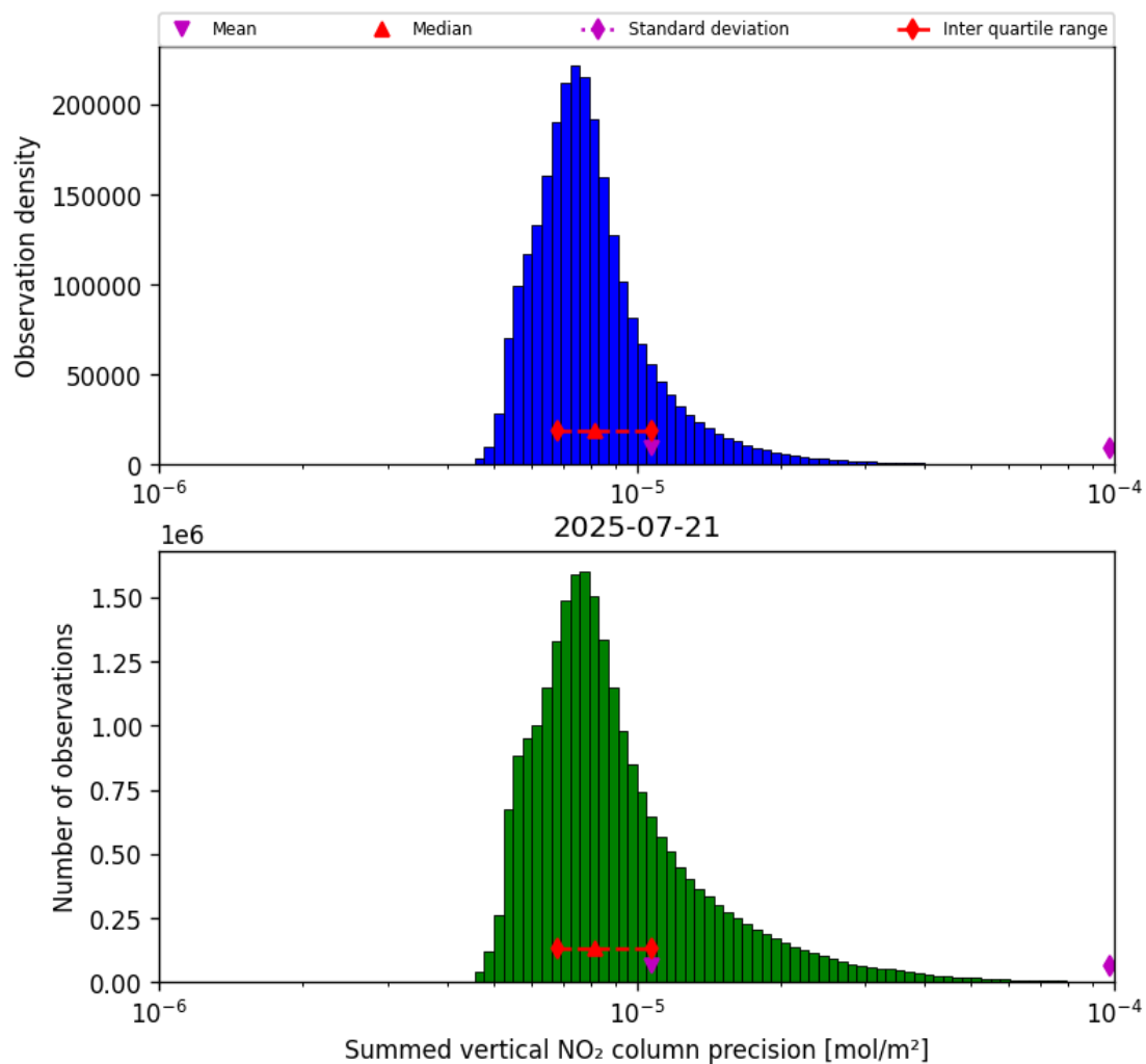
Figure 39: Histogram of “Summed vertical NO 2 column precision” for 2025-07-21 to 2025-07-22
