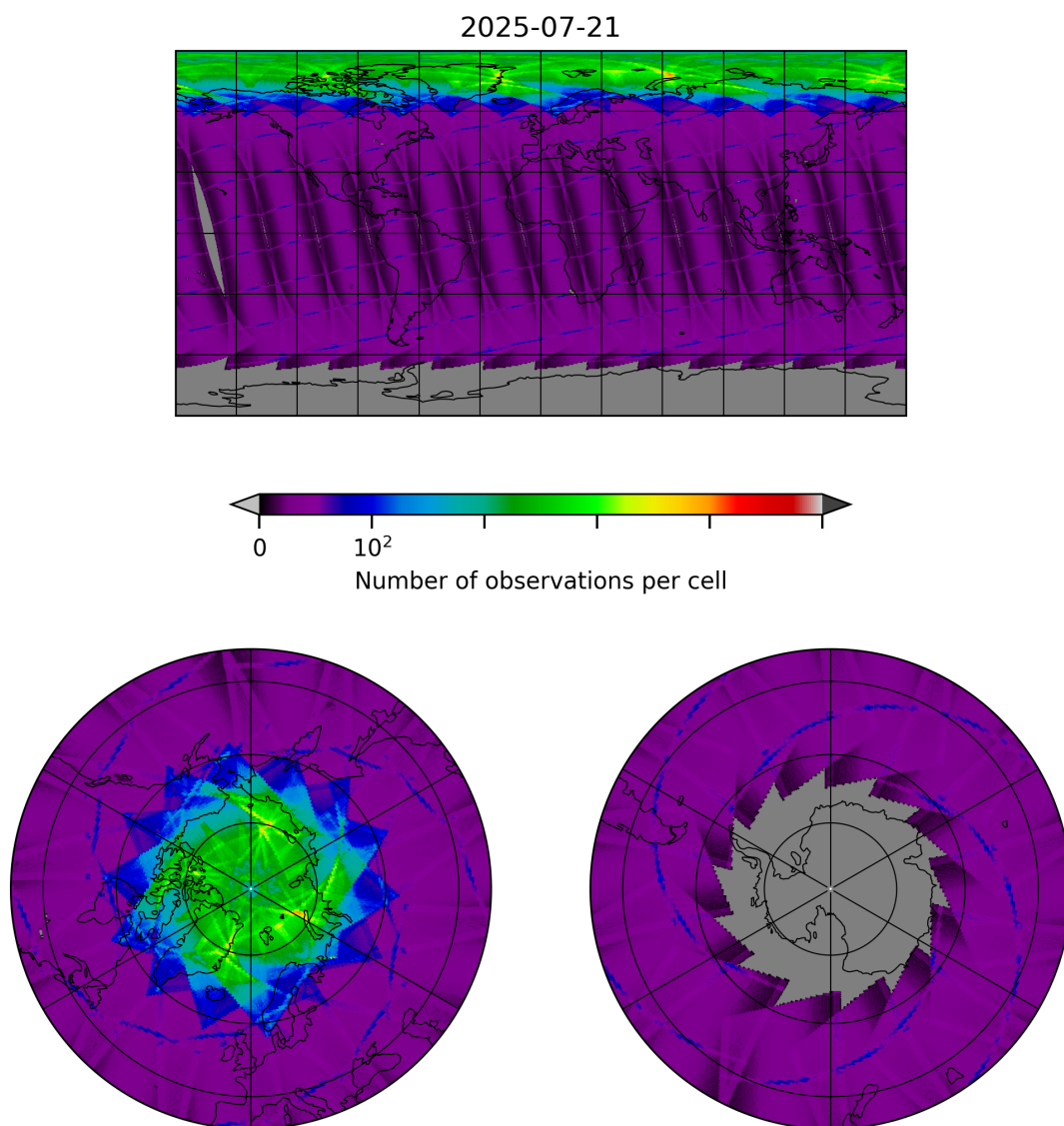
Figure 8: Map of the number of observations for 2025-07-21 to 2025-07-22
