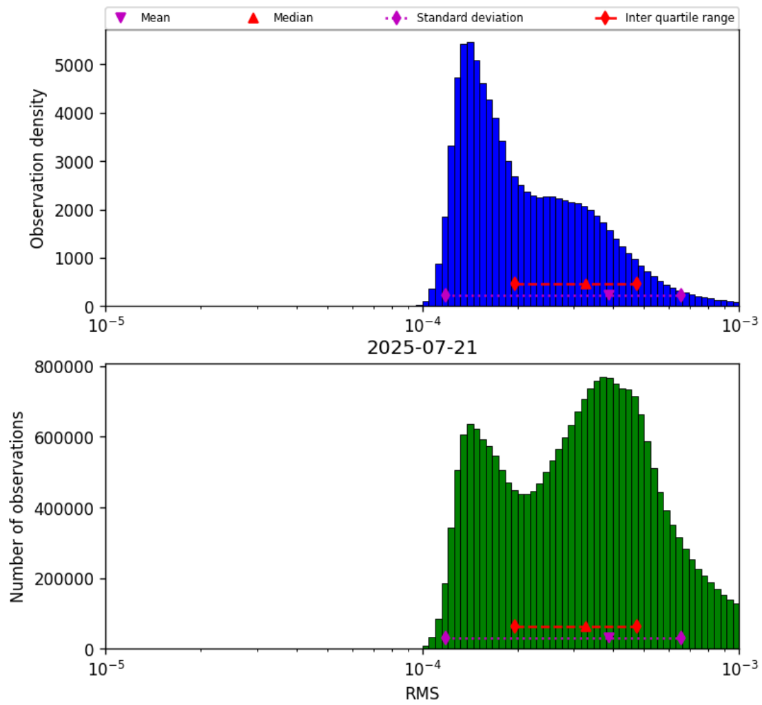
Figure 41: Histogram of “RMS” for 2025-07-21 to 2025-07-22
