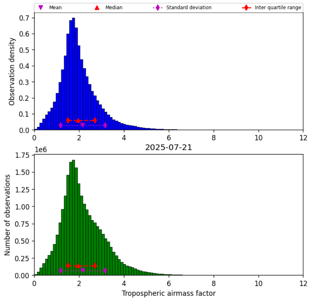
Figure 29: Histogram of “Tropospheric airmass factor” for 2025-07-21 to 2025-07-22
