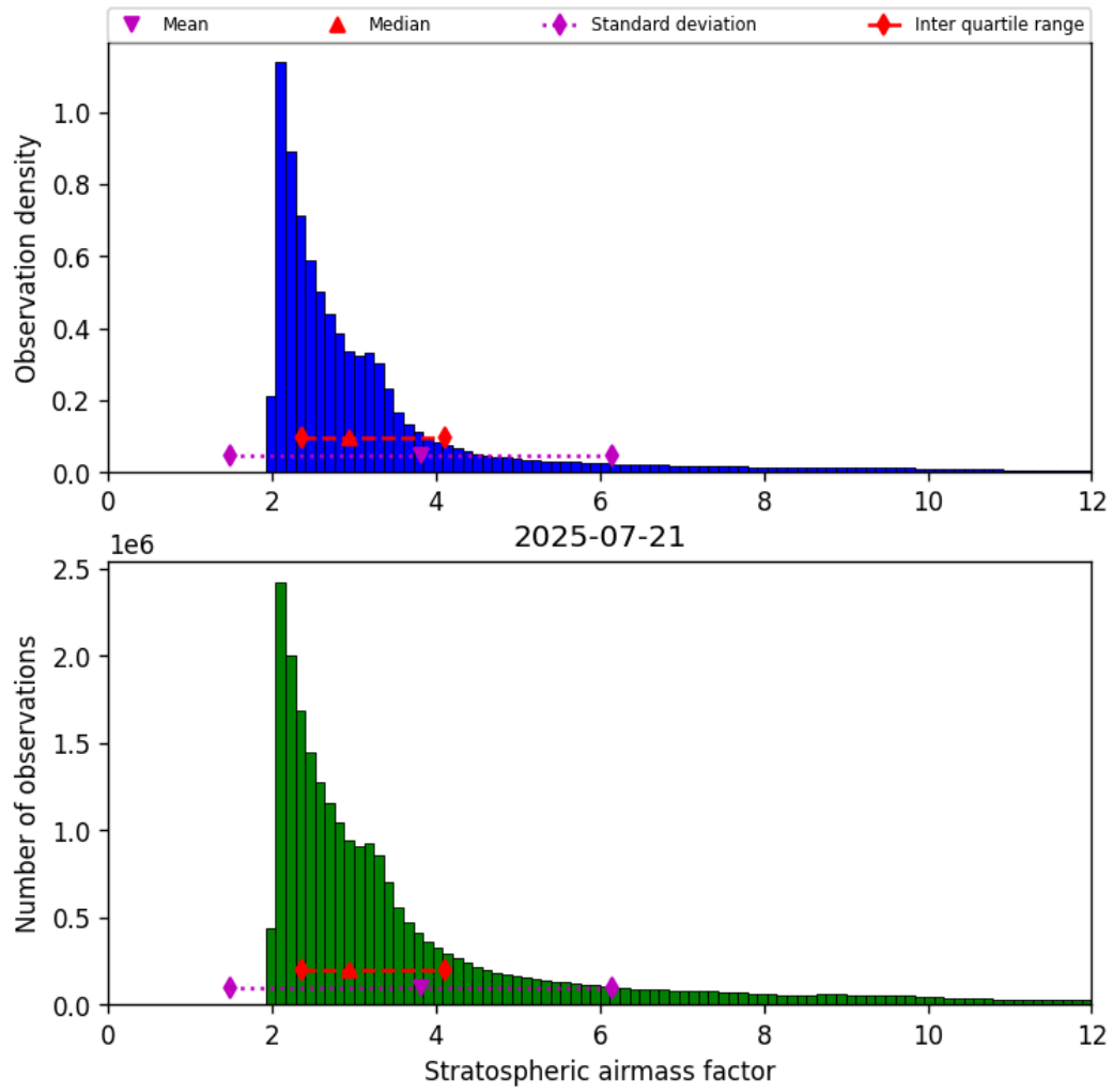
Figure 42: Histogram of “Stratospheric airmass factor” for 2025-07-21 to 2025-07-22
