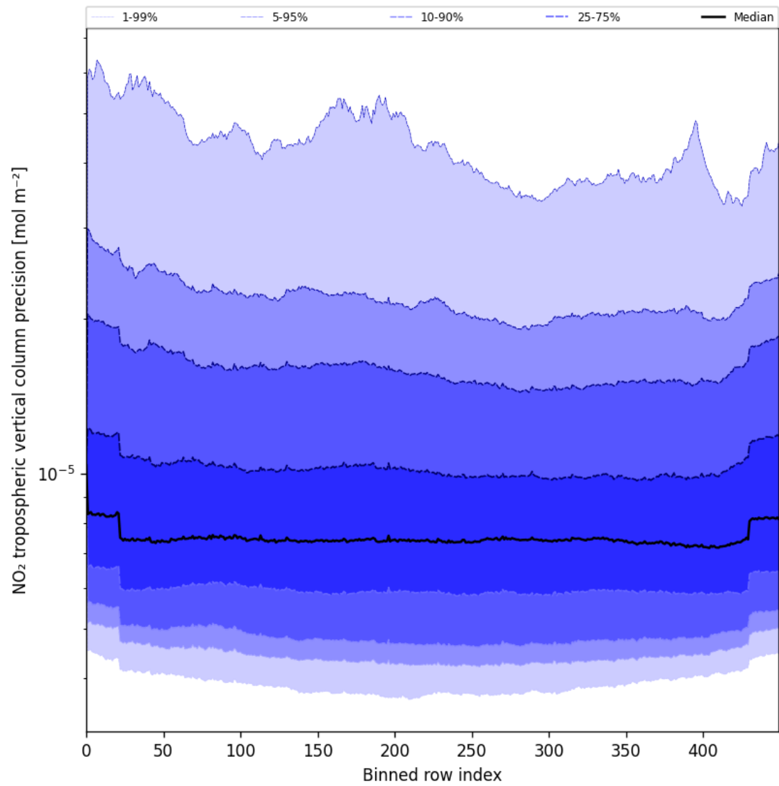
Figure 45: Along track statistics of “NO 2 tropospheric vertical column precision” for 2025-07-21 to 2025-07-22
