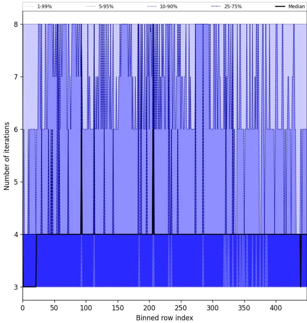
Figure 49: Along track statistics of “Number of iterations” for 2025-07-21 to 2025-07-22
