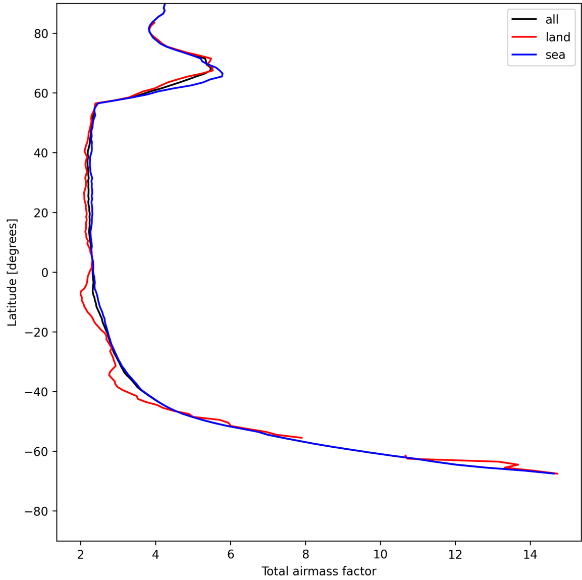
Figure 13: Zonal average of “Total airmass factor” for 2025-07-21 to 2025-07-22.
