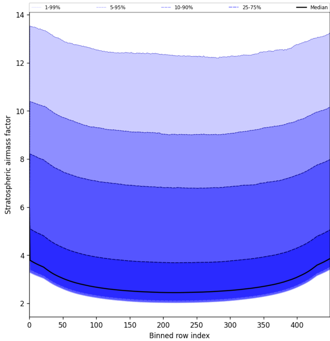
Figure 59: Along track statistics of “Stratospheric airmass factor” for 2025-07-21 to 2025-07-22
