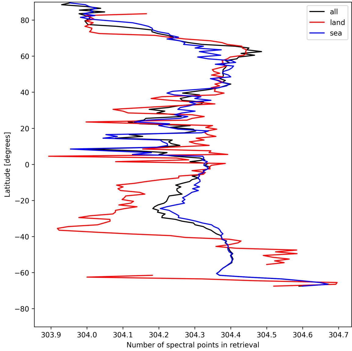
Figure 14: Zonal average of “Number of spectral points in retrieval” for 2025-07-21 to 2025-07-22.
