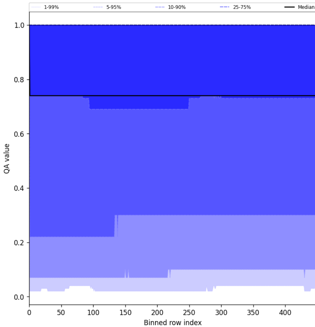
Figure 43: Along track statistics of “QA value” for 2025-07-21 to 2025-07-22
