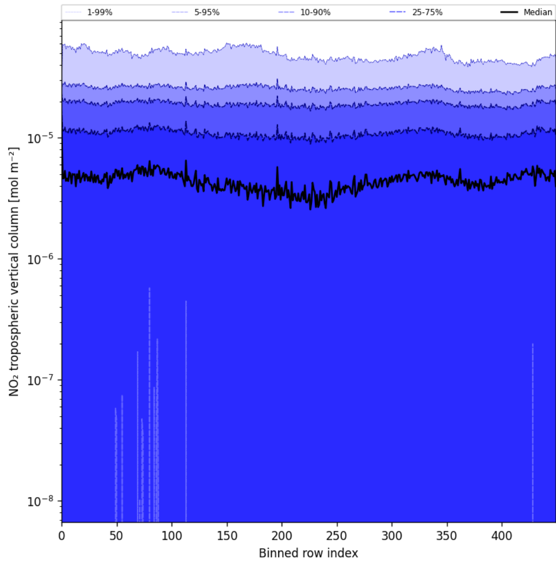
Figure 44: Along track statistics of "NO 2 tropospheric vertical column" for 2025-07-21 to 2025-07-22
