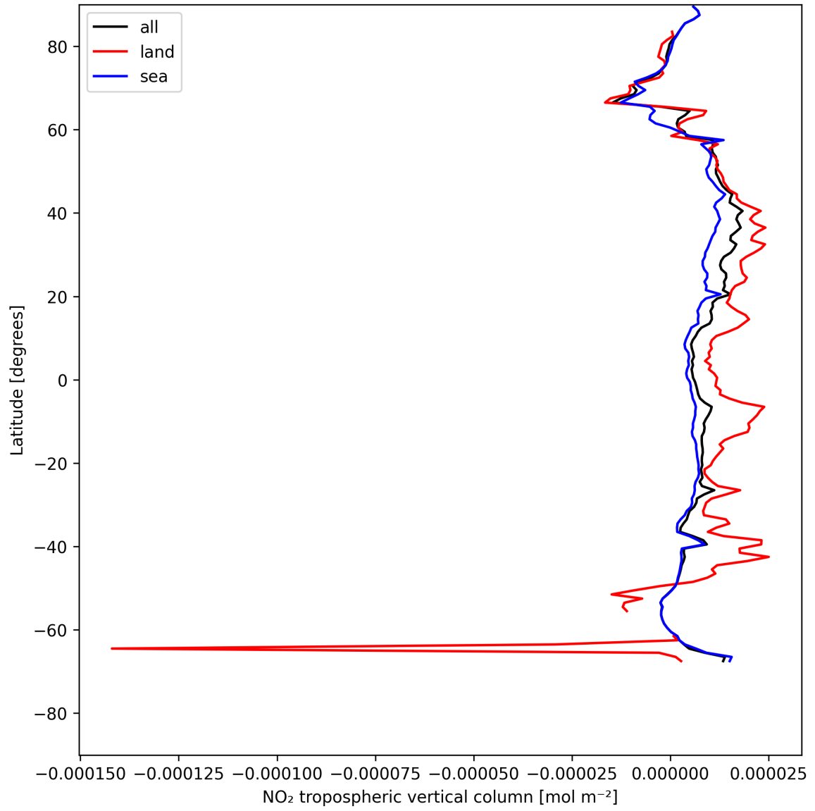
Figure 10: Zonal average of “NO 2 tropospheric vertical column” for 2025-07-21 to 2025-07-22.
