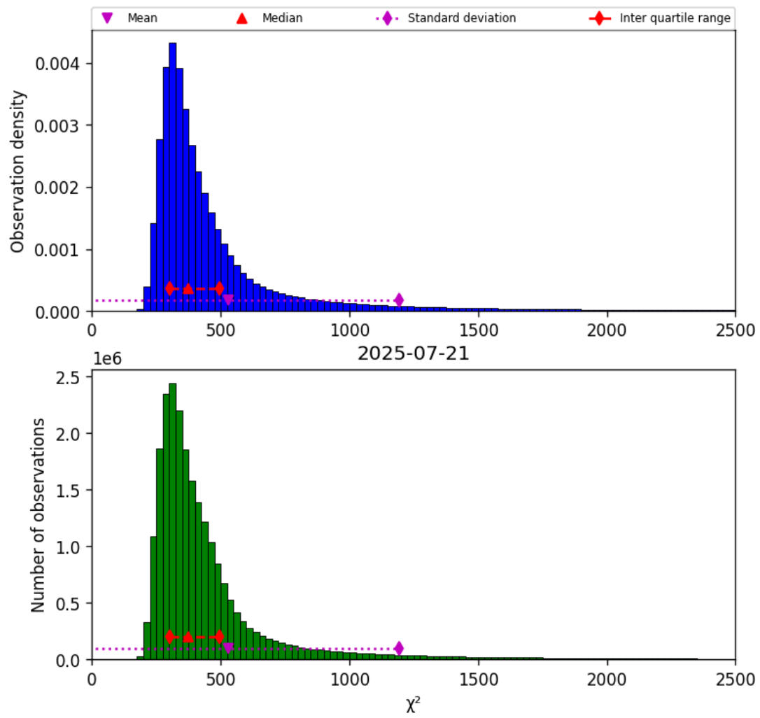
Figure 40: Histogram of “ \chi^2 ” for 2025-07-21 to 2025-07-22
