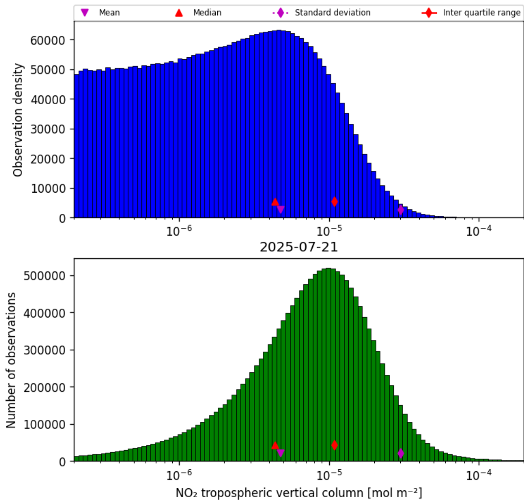
Figure 27: Histogram of “NO 2 tropospheric vertical column” for 2025-07-21 to 2025-07-22
