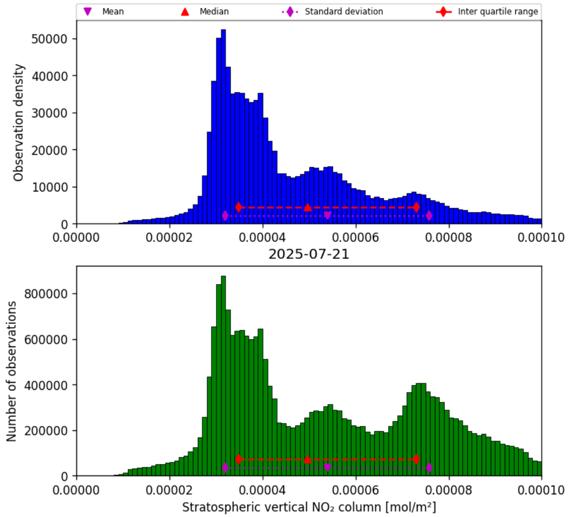
Figure 34: Histogram of “Stratospheric vertical NO 2 column” for 2025-07-21 to 2025-07-22
