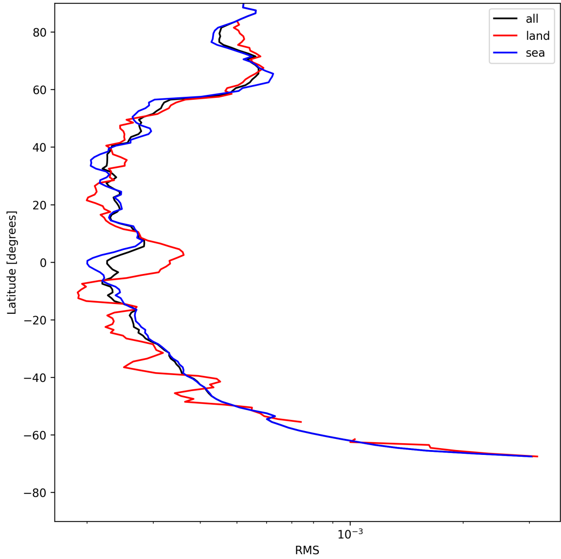
Figure 24: Zonal average of “RMS” for 2025-07-21 to 2025-07-22.
