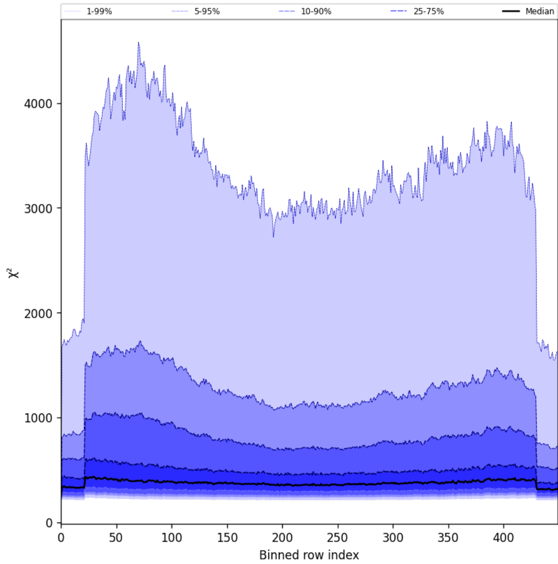
Figure 57: Along track statistics of “ \chi^2 ” for 2025-07-21 to 2025-07-22
