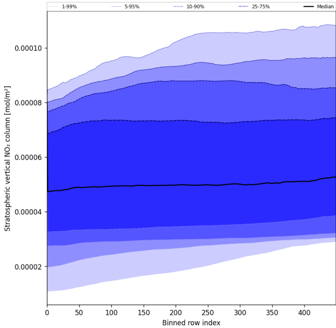
Figure 51: Along track statistics of “Stratospheric vertical NO 2 column” for 2025-07-21 to 2025-07-22
