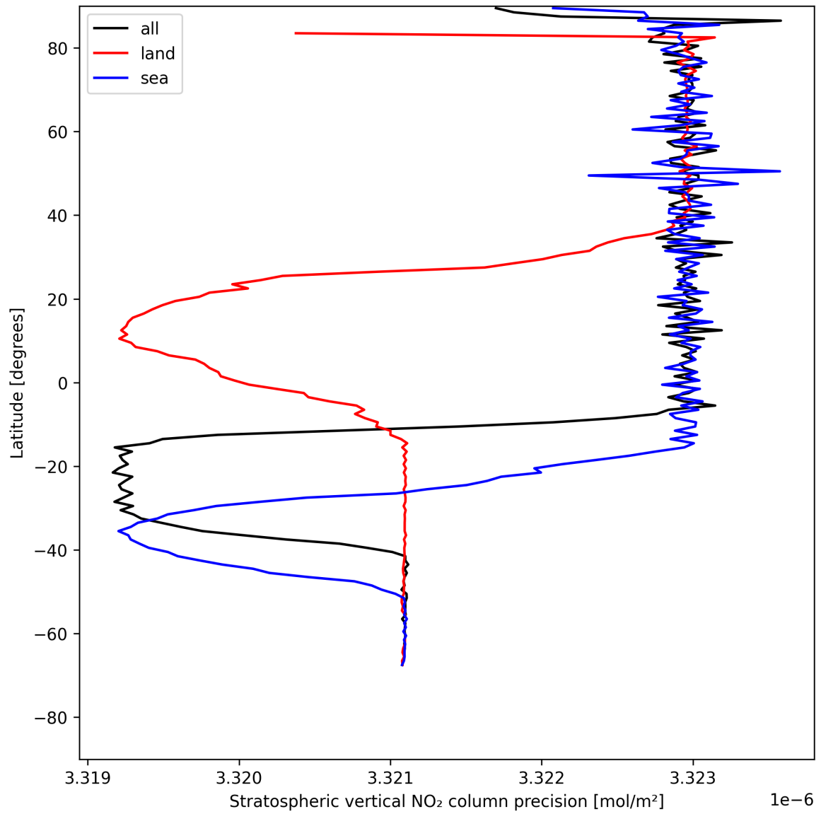
Figure 18: Zonal average of “Stratospheric vertical NO 2 column precision” for 2025-07-21 to 2025-07-22.
