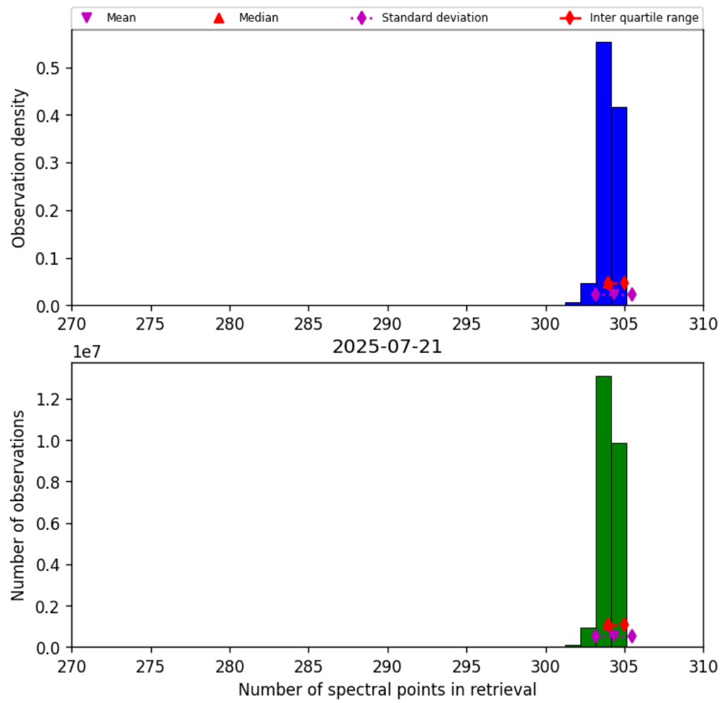
Figure 31: Histogram of “Number of spectral points in retrieval” for 2025-07-21 to 2025-07-22
