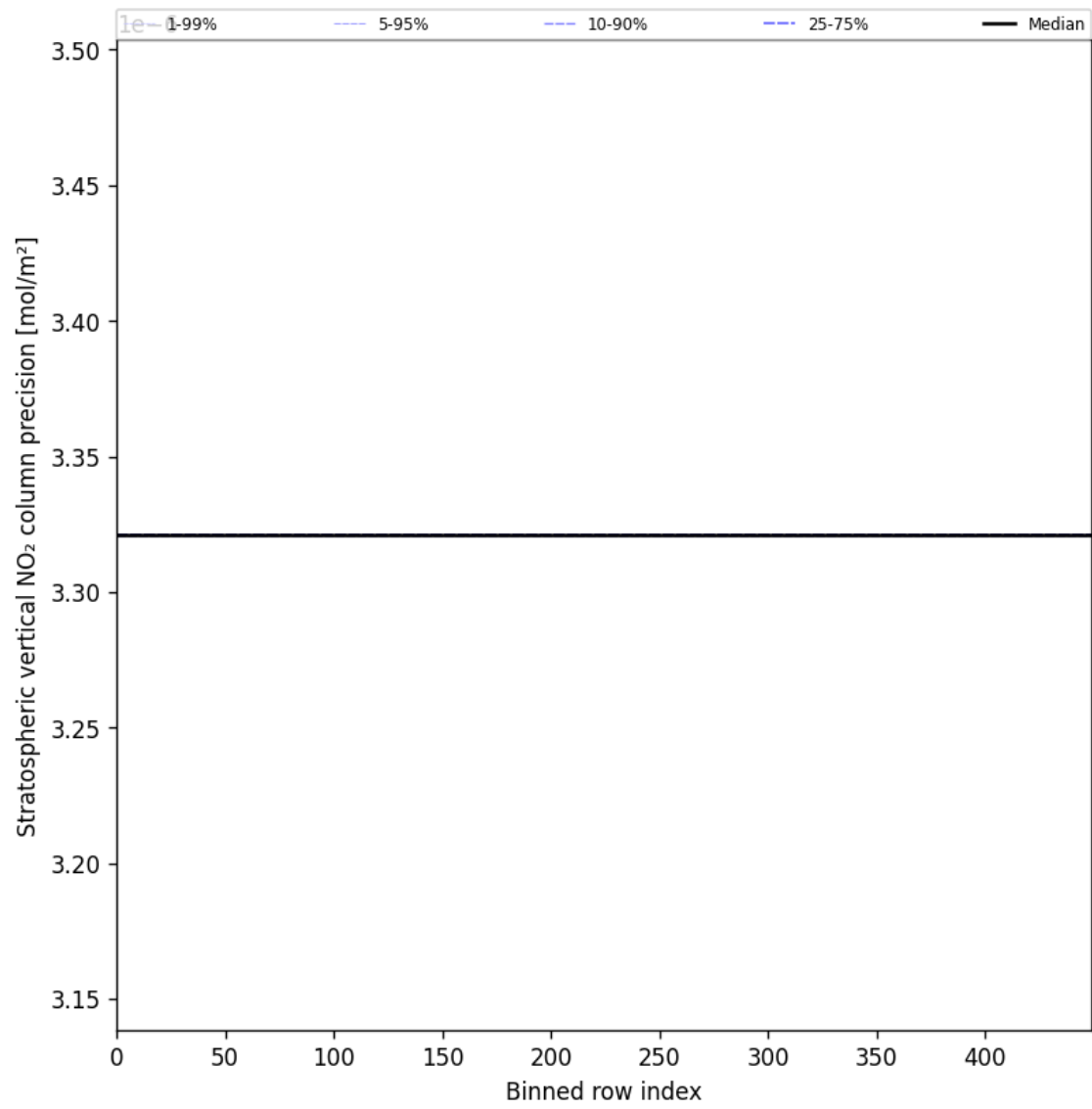
Figure 52: Along track statistics of “Stratospheric vertical NO 2 column precision” for 2025-07-21 to 2025-07-22
