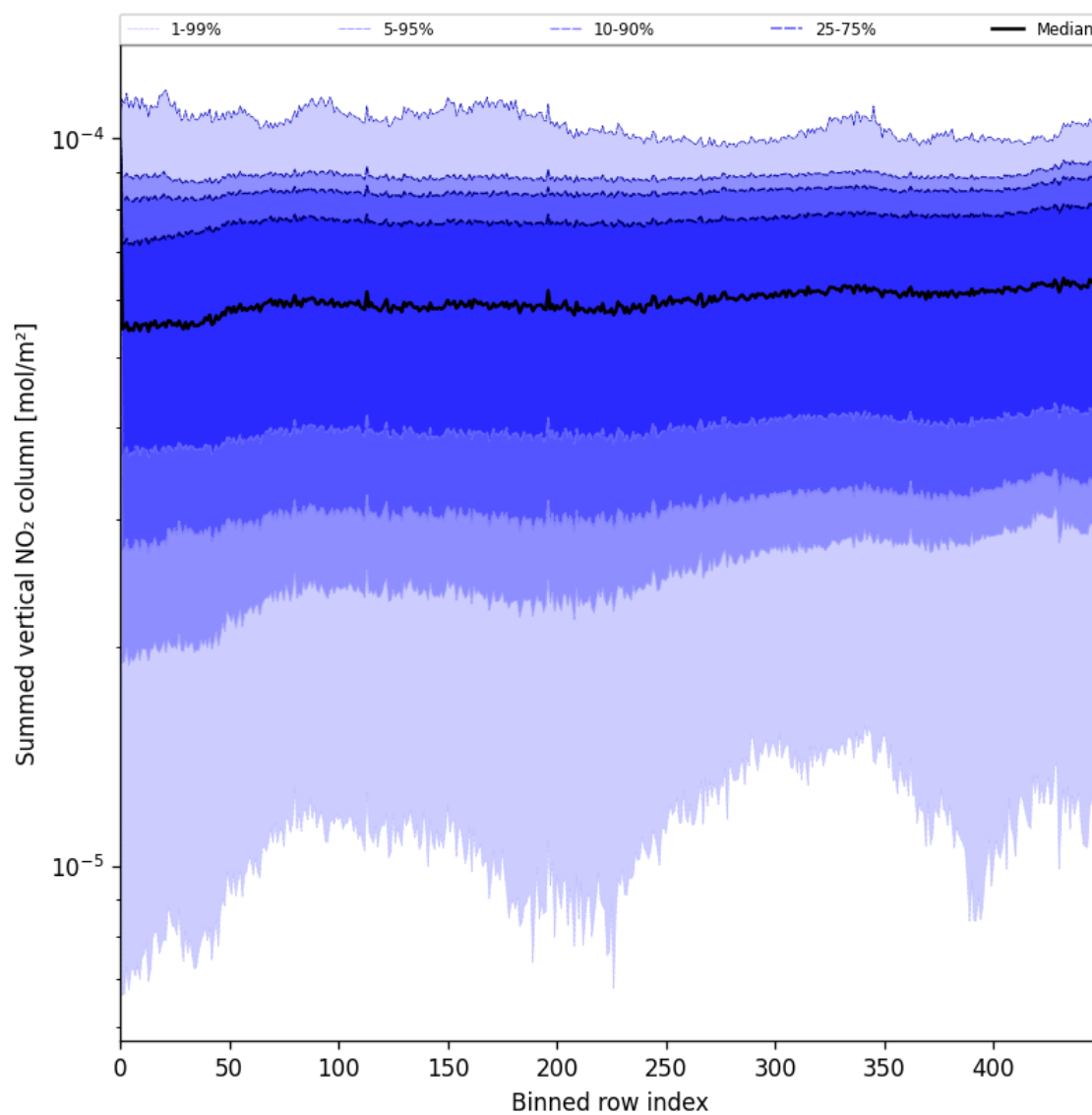
Figure 55: Along track statistics of “Summed vertical NO 2 column” for 2025-07-21 to 2025-07-22
