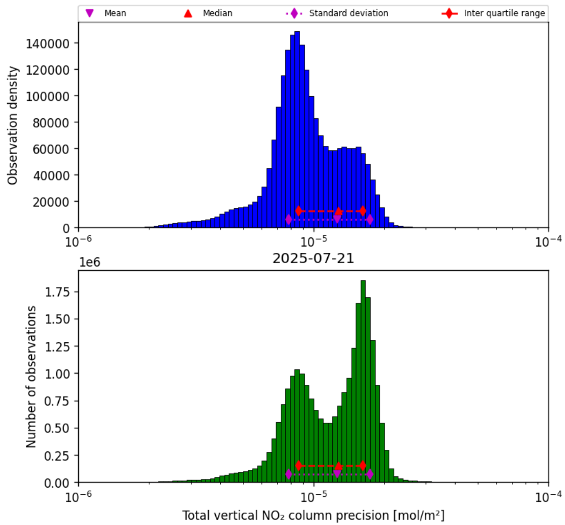
Figure 37: Histogram of “Total vertical NO 2 column precision” for 2025-07-21 to 2025-07-22
