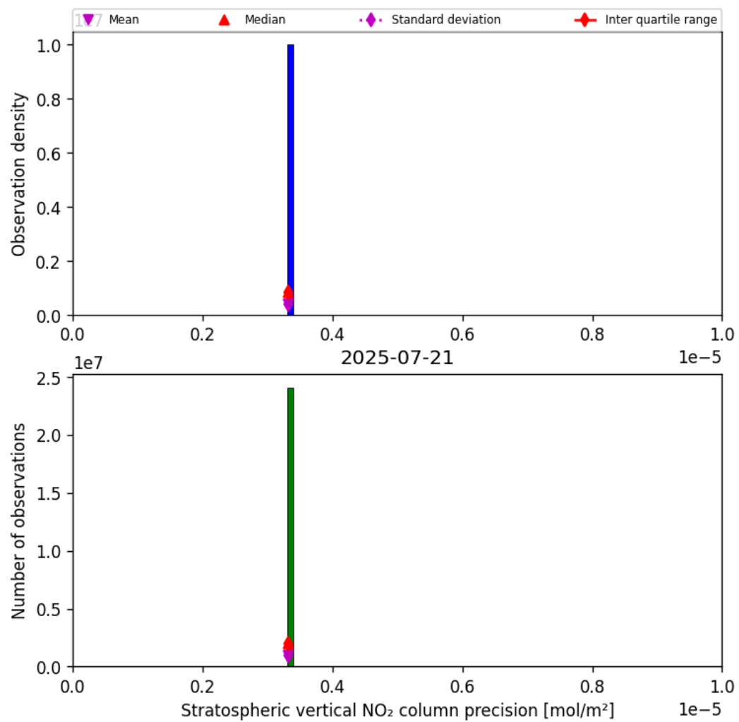
Figure 35: Histogram of “Stratospheric vertical NO 2 column precision” for 2025-07-21 to 2025-07-22
