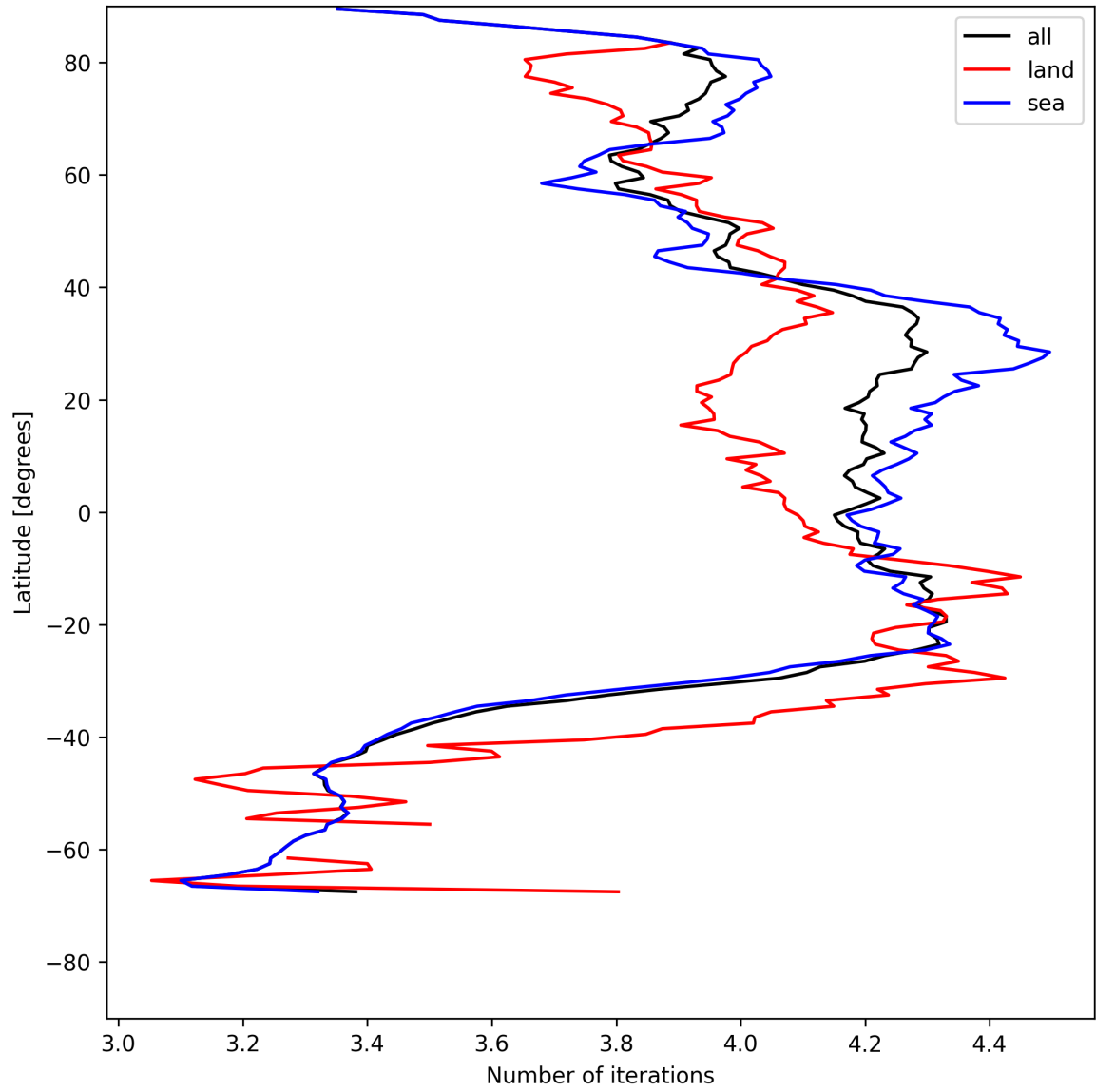
Figure 15: Zonal average of “Number of iterations” for 2025-07-21 to 2025-07-22.
