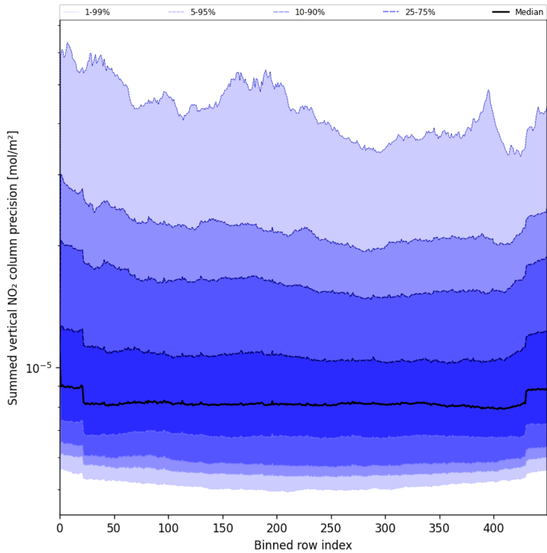
Figure 56: Along track statistics of “Summed vertical NO 2 column precision” for 2025-07-21 to 2025-07-22
