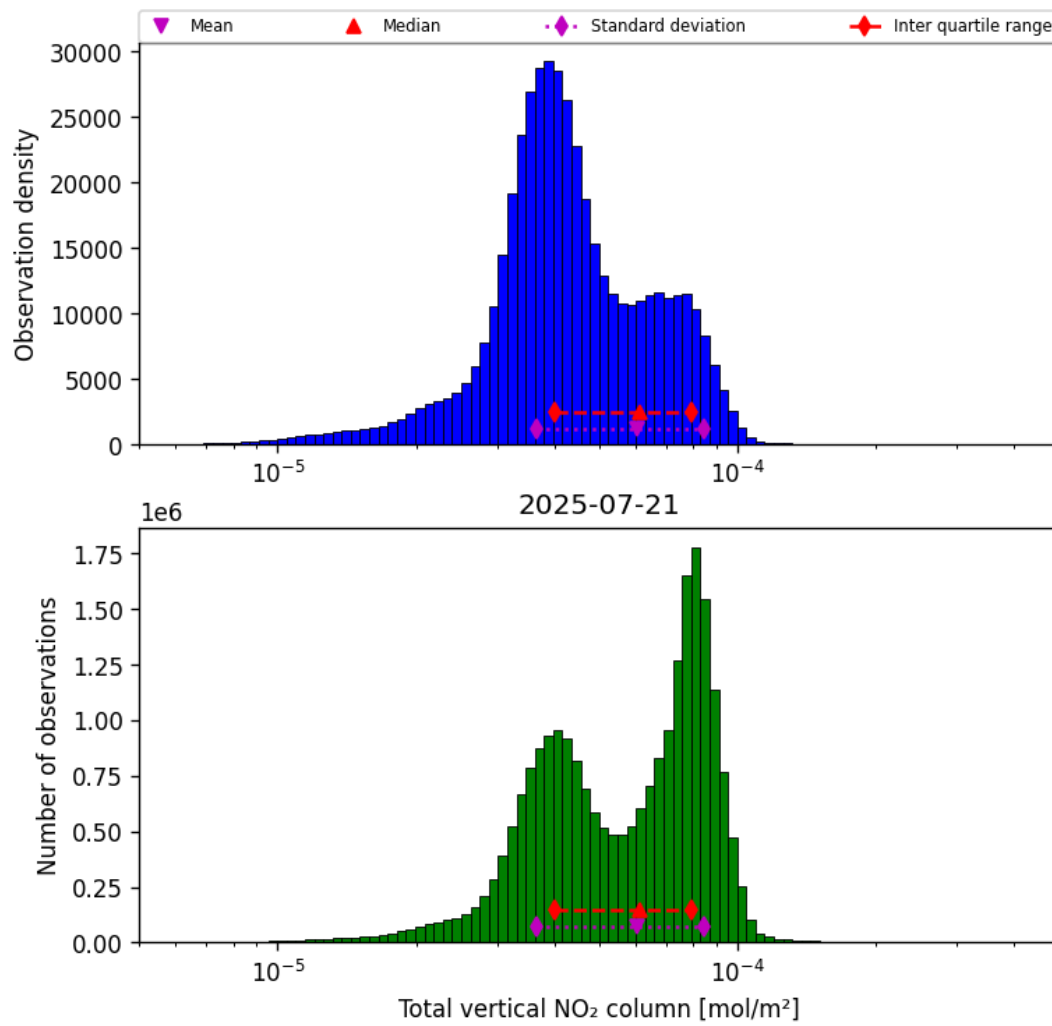
Figure 36: Histogram of “Total vertical NO 2 column” for 2025-07-21 to 2025-07-22
