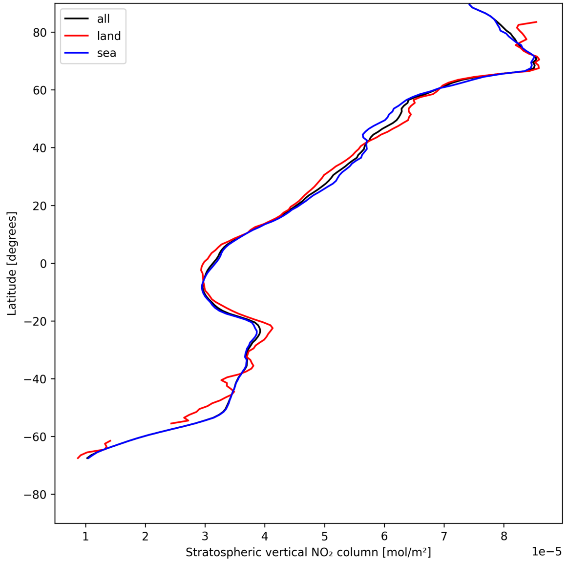
Figure 17: Zonal average of “Stratospheric vertical NO 2 column” for 2025-07-21 to 2025-07-22.
