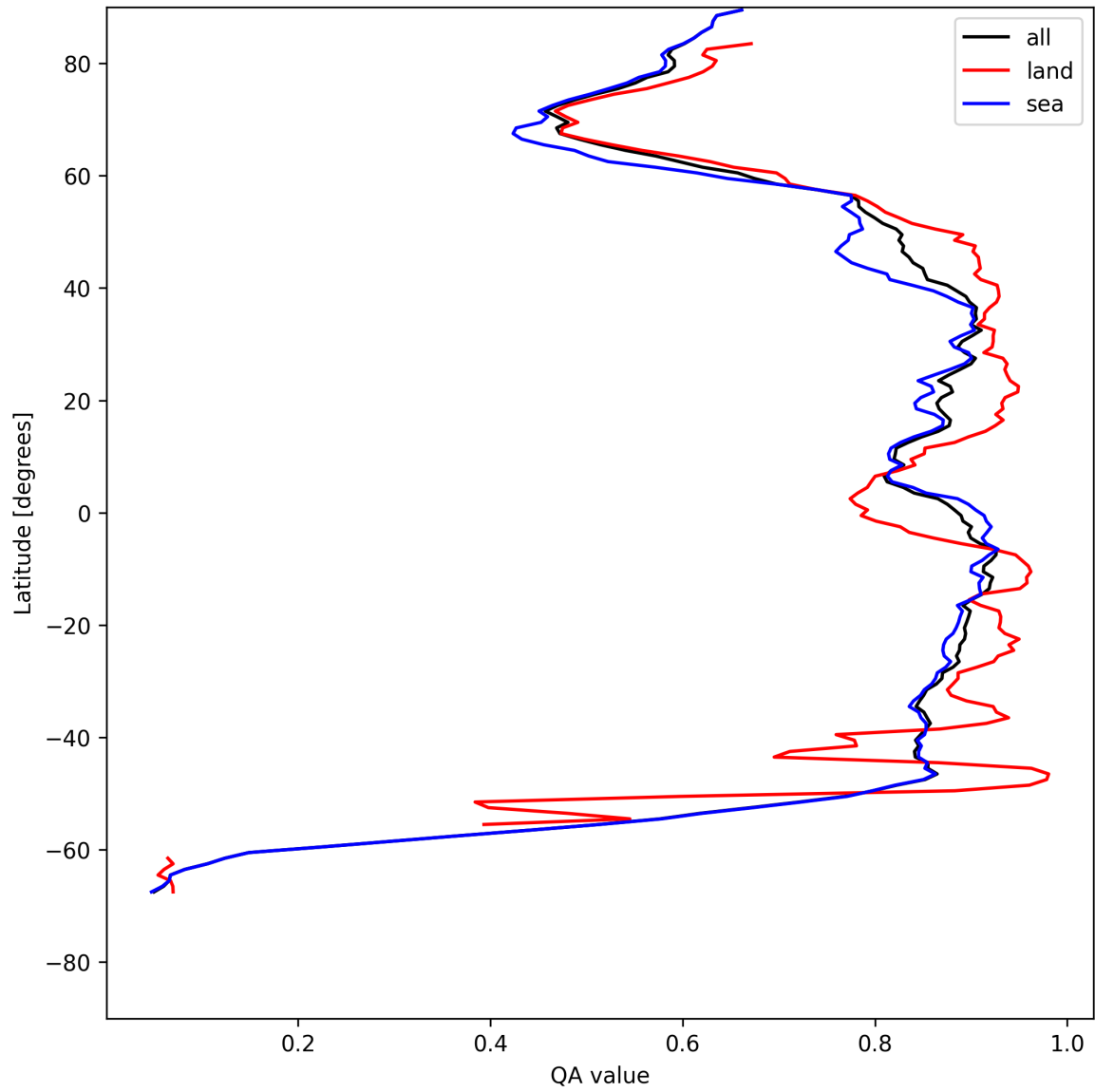
Figure 9: Zonal average of “QA value” for 2025-07-21 to 2025-07-22.
