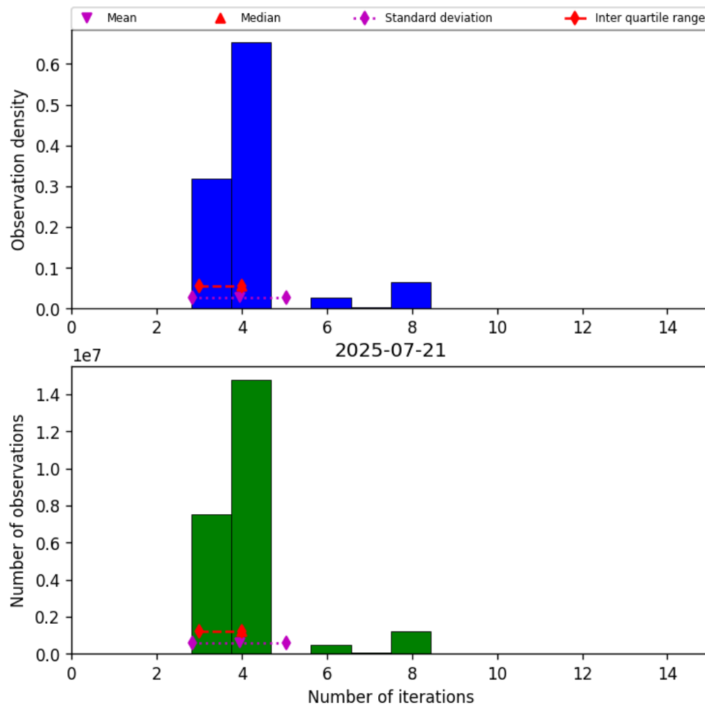
Figure 32: Histogram of “Number of iterations” for 2025-07-21 to 2025-07-22
