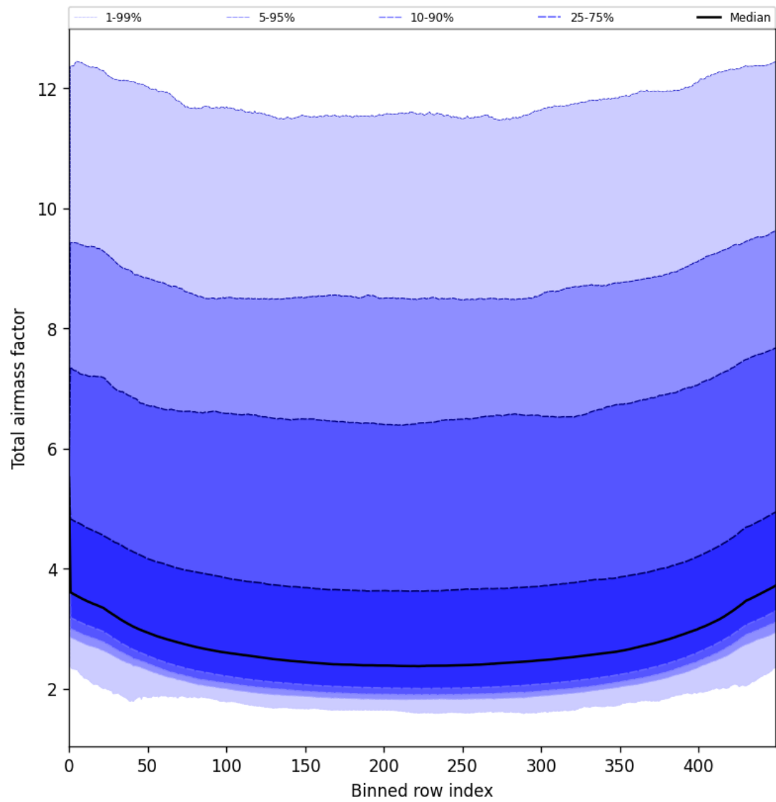
Figure 47: Along track statistics of “Total airmass factor” for 2025-07-22 to 2025-07-22
