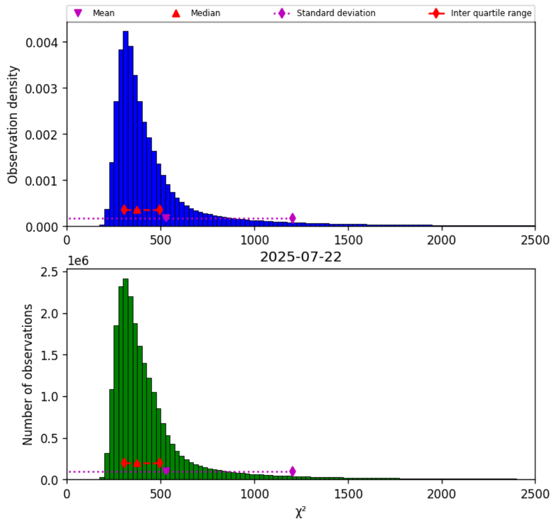
Figure 40: Histogram of “ \chi^2 ” for 2025-07-22 to 2025-07-22
