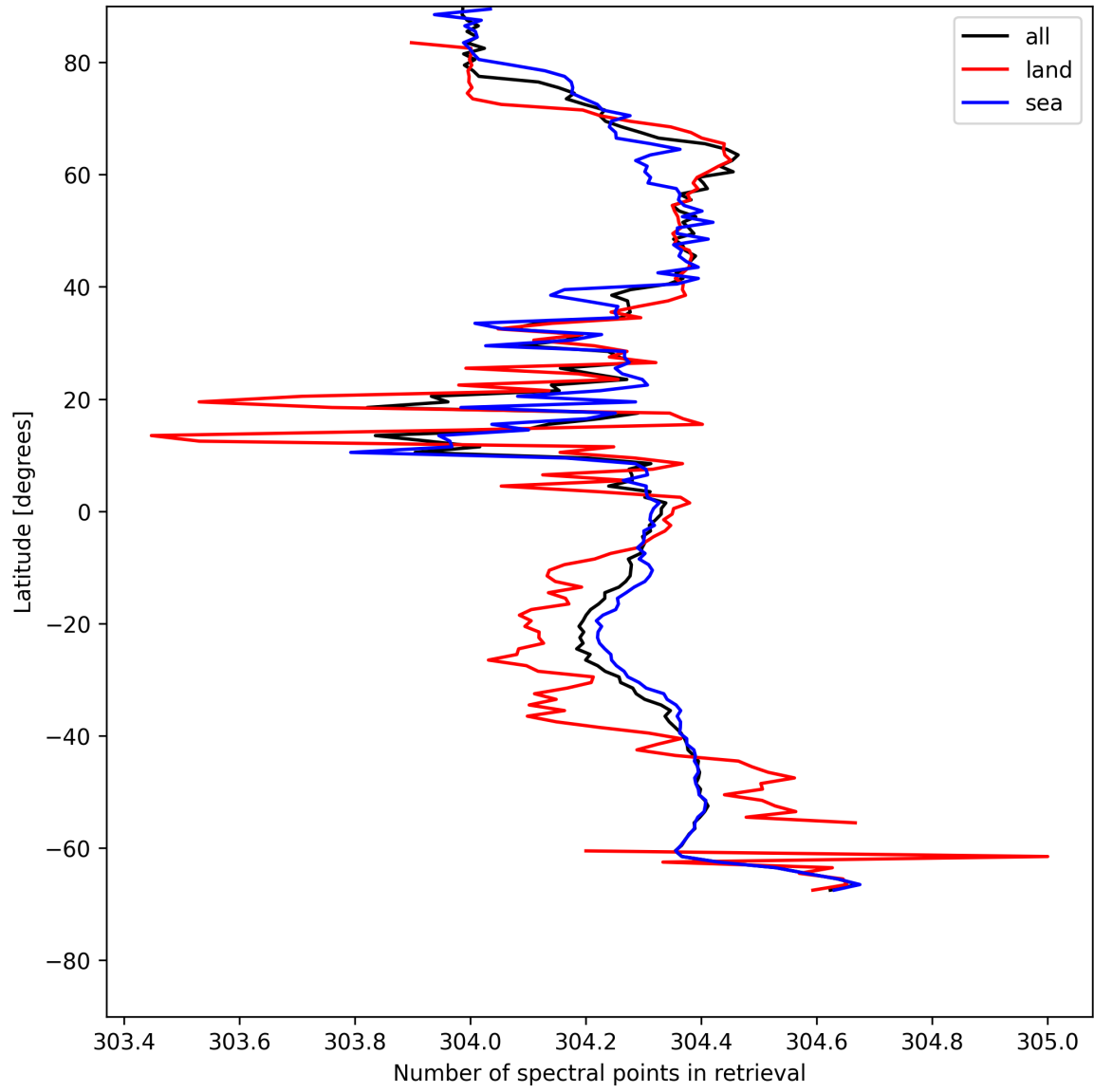
Figure 14: Zonal average of “Number of spectral points in retrieval” for 2025-07-22 to 2025-07-22.
