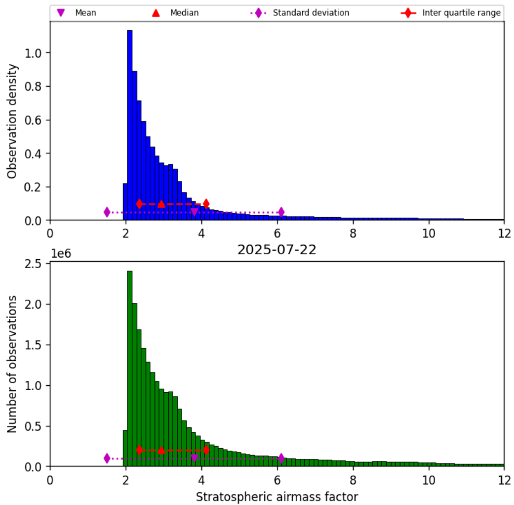
Figure 42: Histogram of “Stratospheric airmass factor” for 2025-07-22 to 2025-07-22
