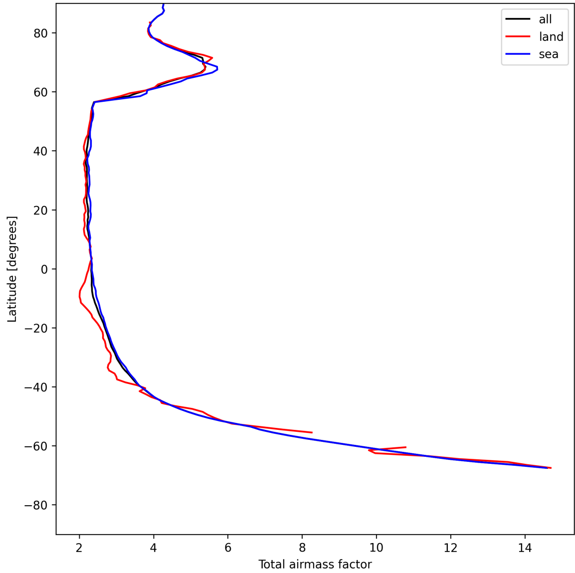
Figure 13: Zonal average of “Total airmass factor” for 2025-07-22 to 2025-07-22.
