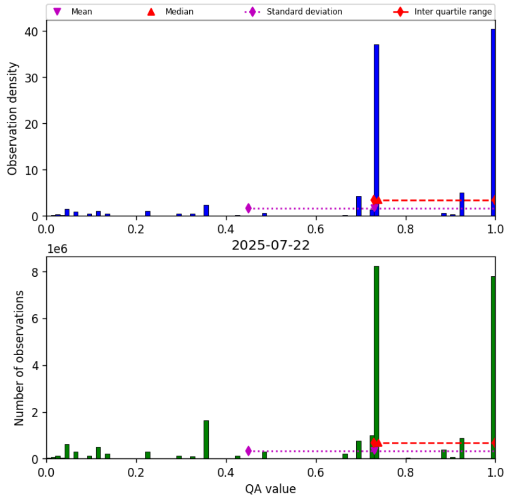
Figure 26: Histogram of “QA value” for 2025-07-22 to 2025-07-22
