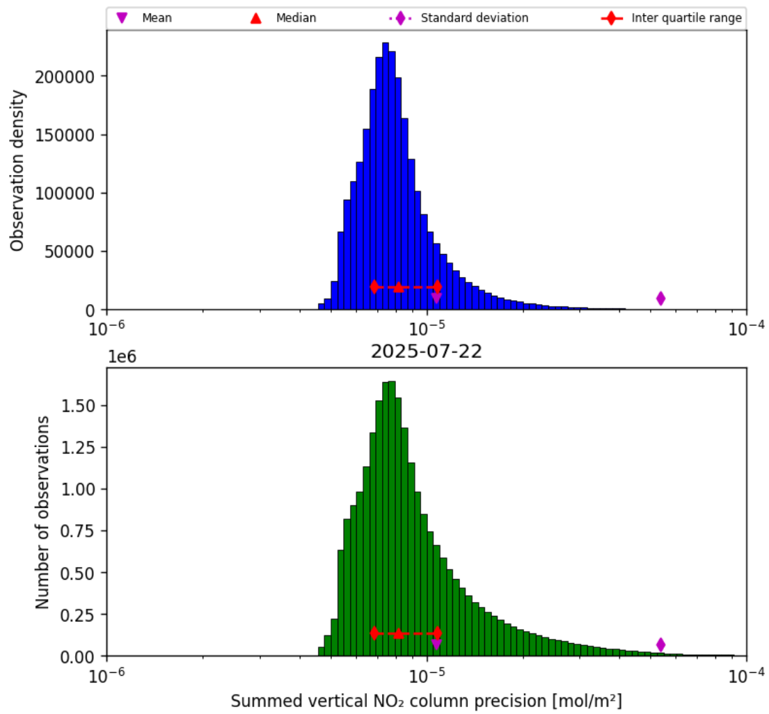
Figure 39: Histogram of "Summed vertical NO 2 column precision" for 2025-07-22 to 2025-07-22
