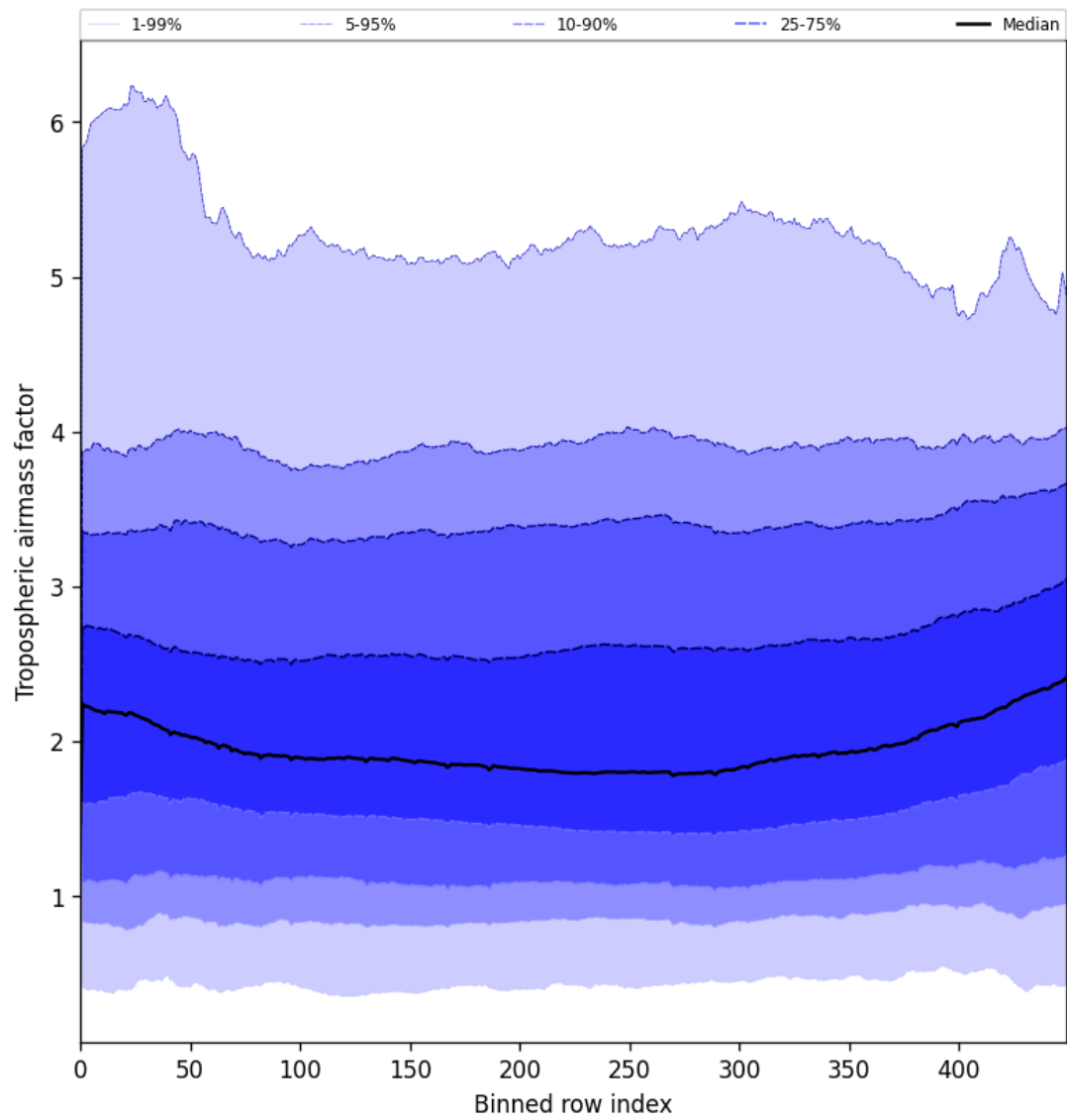
Figure 46: Along track statistics of “Tropospheric airmass factor” for 2025-07-22 to 2025-07-22
