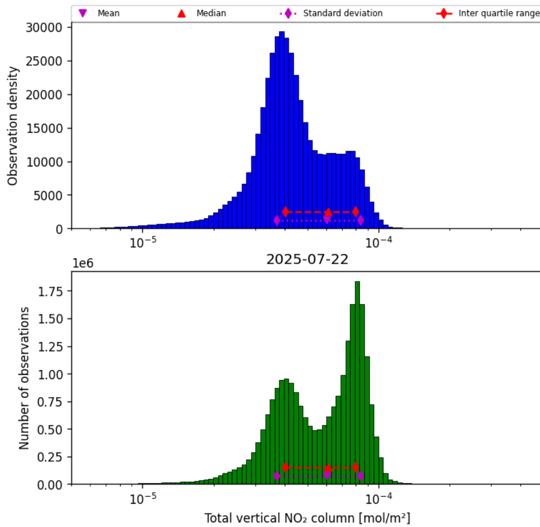
Figure 36: Histogram of "Total vertical NO 2 column" for 2025-07-22 to 2025-07-22
