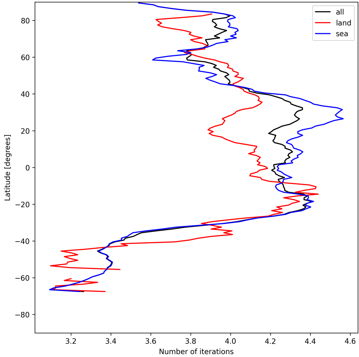
Figure 15: Zonal average of “Number of iterations” for 2025-07-22 to 2025-07-22.
