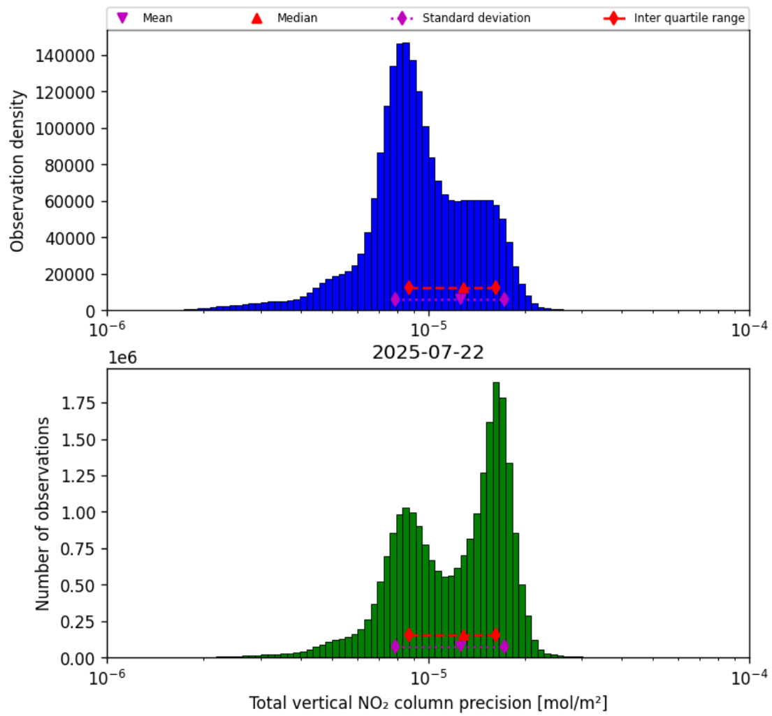
Figure 37: Histogram of "Total vertical NO 2 column precision" for 2025-07-22 to 2025-07-22
