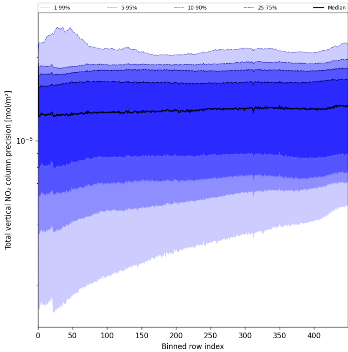
Figure 54: Along track statistics of “Total vertical NO 2 column precision” for 2025-07-22 to 2025-07-22
