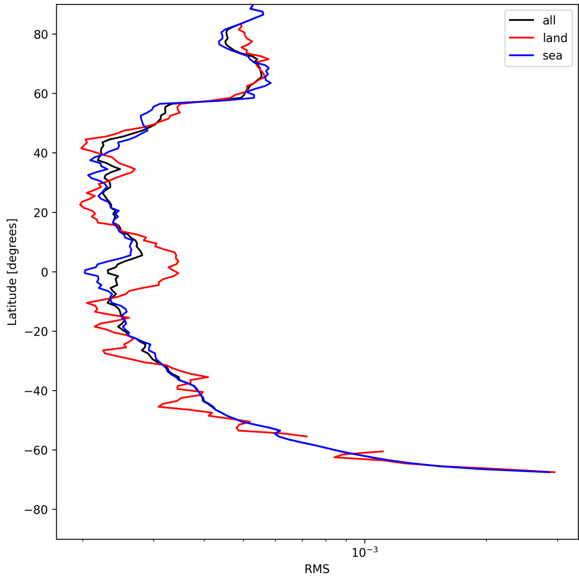
Figure 24: Zonal average of “RMS” for 2025-07-22 to 2025-07-22.
