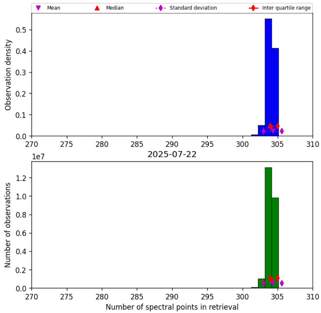
Figure 31: Histogram of “Number of spectral points in retrieval” for 2025-07-22 to 2025-07-22
