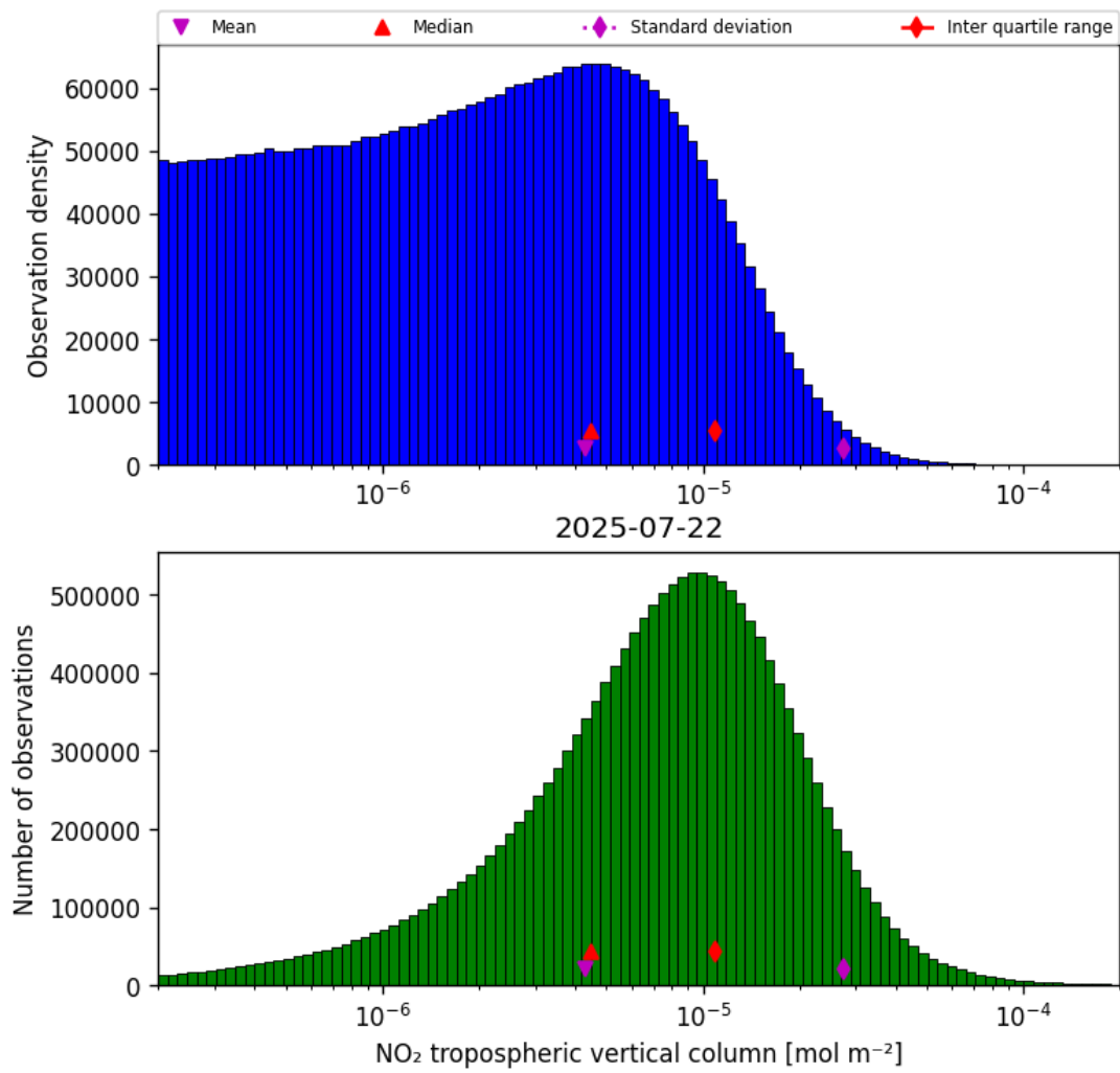
Figure 27: Histogram of “NO 2 tropospheric vertical column” for 2025-07-22 to 2025-07-22
