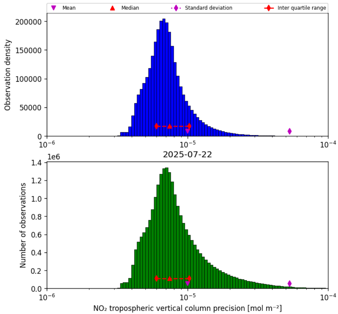
Figure 28: Histogram of “NO 2 tropospheric vertical column precision” for 2025-07-22 to 2025-07-22
