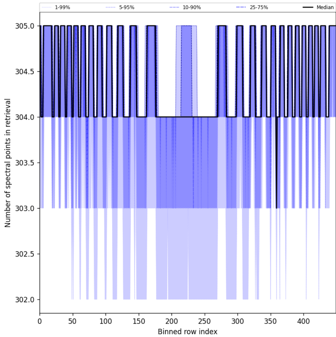
Figure 48: Along track statistics of “Number of spectral points in retrieval” for 2025-07-22 to 2025-07-22
