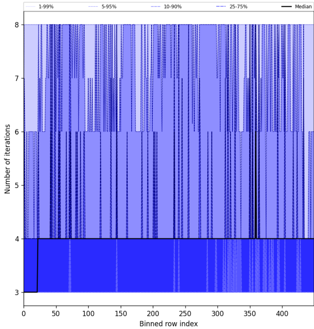
Figure 49: Along track statistics of “Number of iterations” for 2025-07-22 to 2025-07-22
