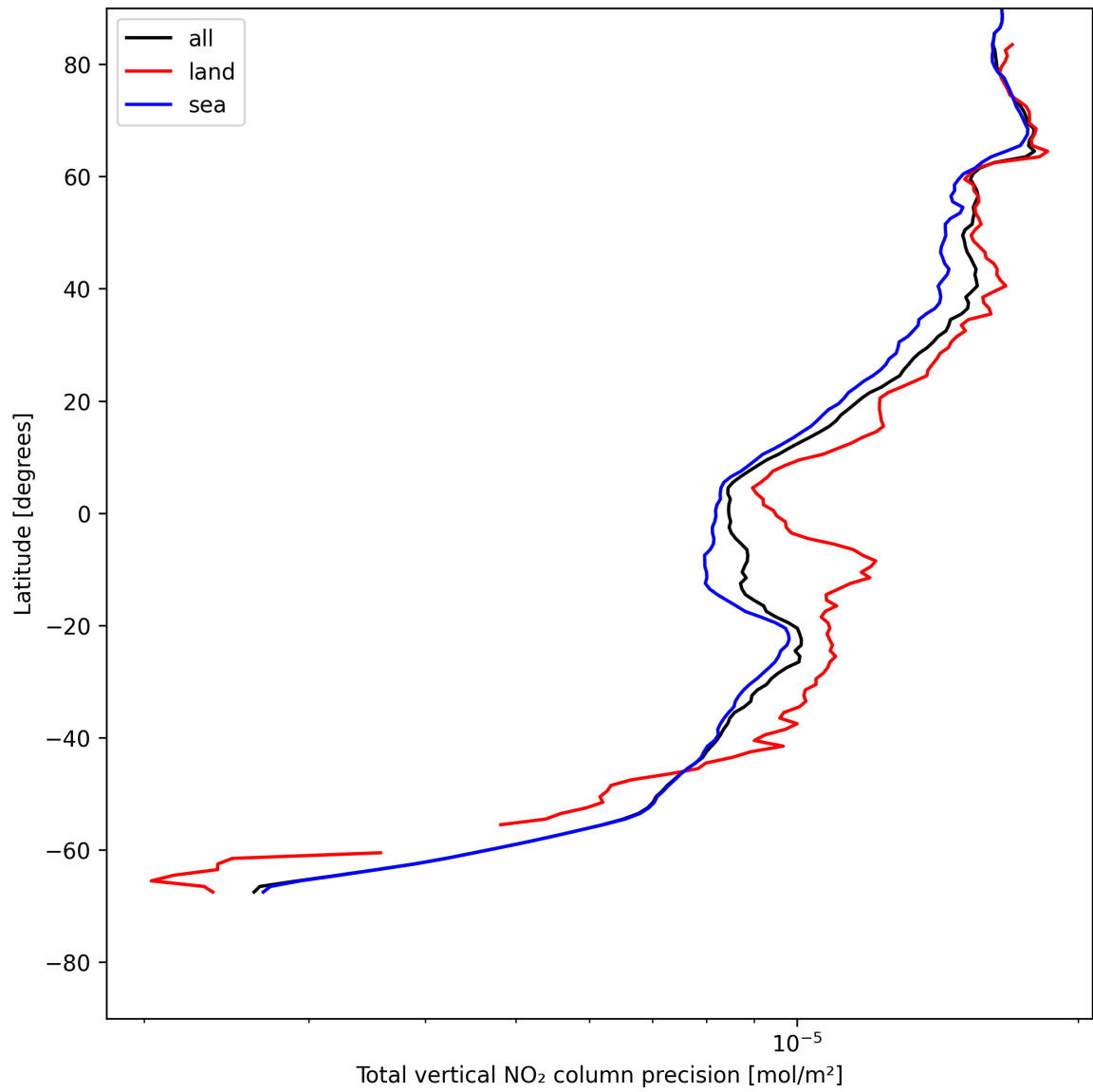
Figure 20: Zonal average of “Total vertical NO 2 column precision” for 2025-07-22 to 2025-07-22.
