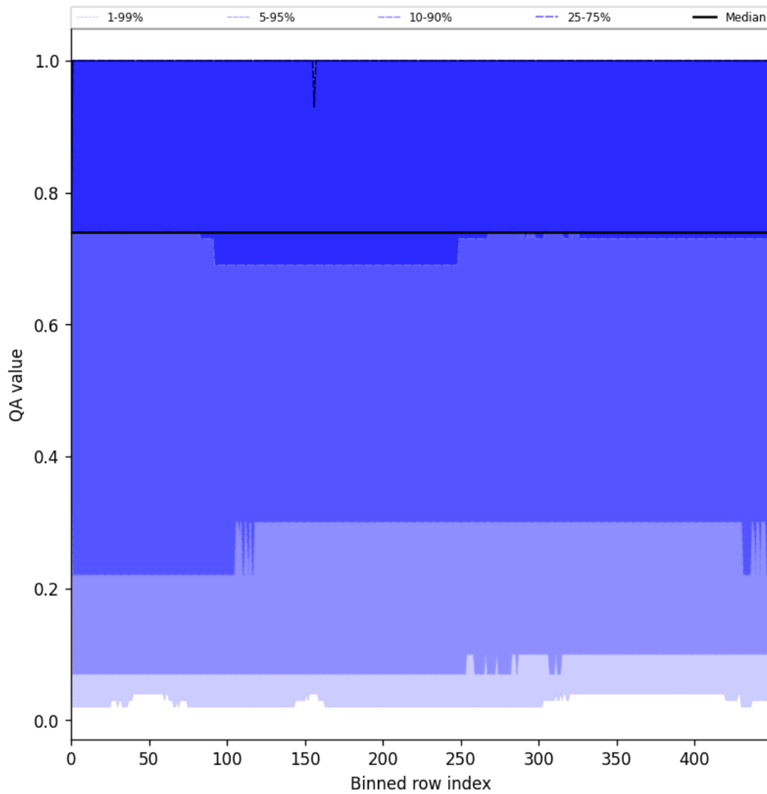
Figure 43: Along track statistics of “QA value” for 2025-07-22 to 2025-07-22
