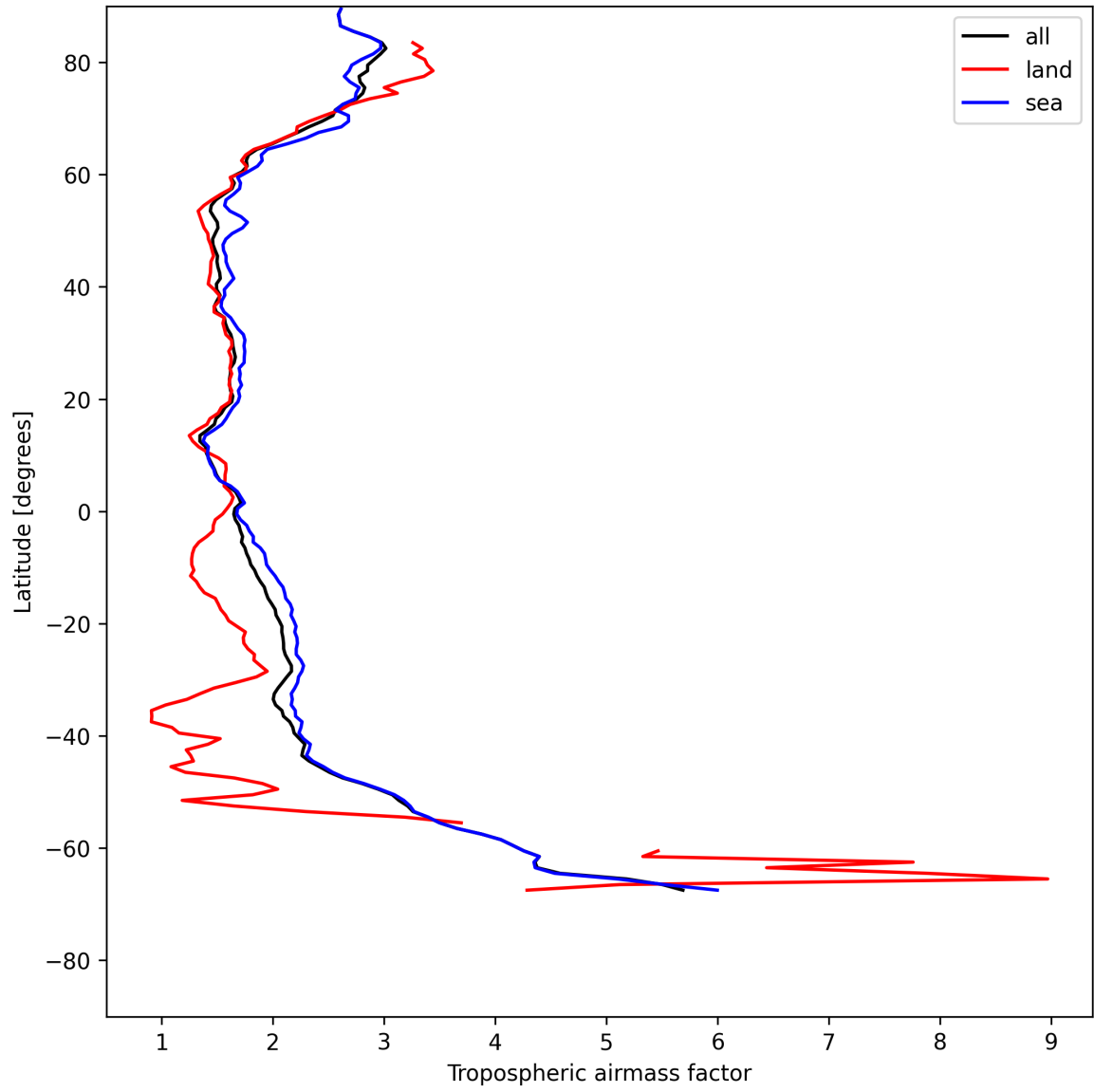
Figure 12: Zonal average of “Tropospheric airmass factor” for 2025-07-22 to 2025-07-22.
