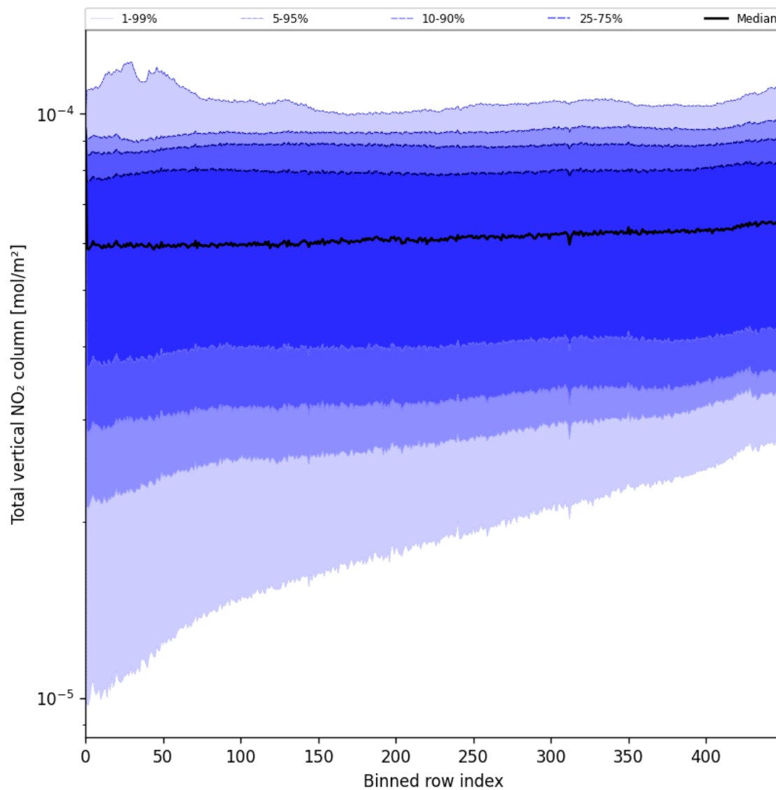
Figure 53: Along track statistics of “Total vertical NO 2 column” for 2025-07-22 to 2025-07-22
