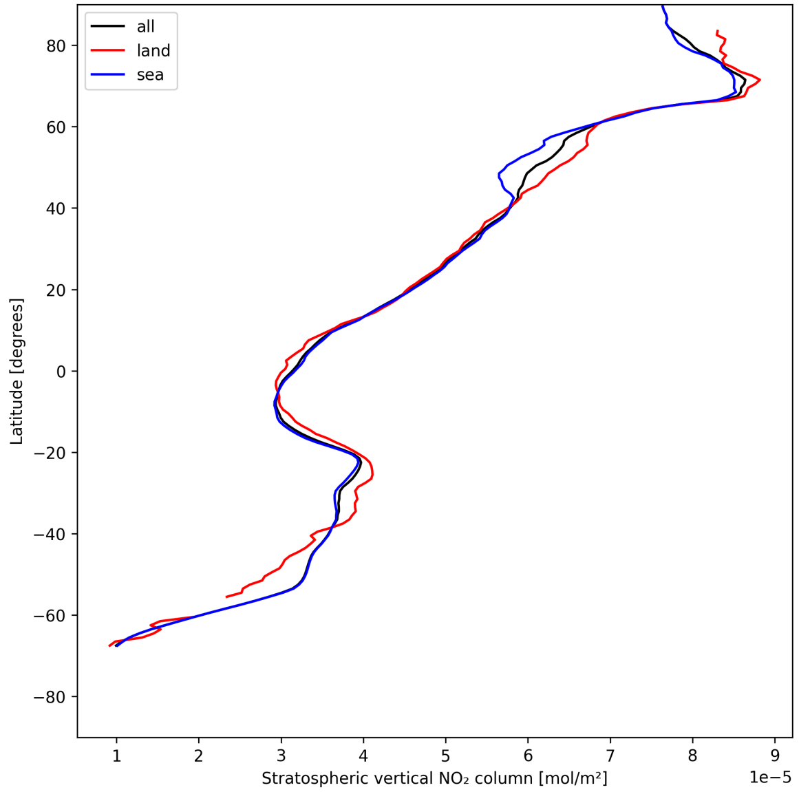
Figure 17: Zonal average of “Stratospheric vertical NO 2 column” for 2025-07-22 to 2025-07-22.
