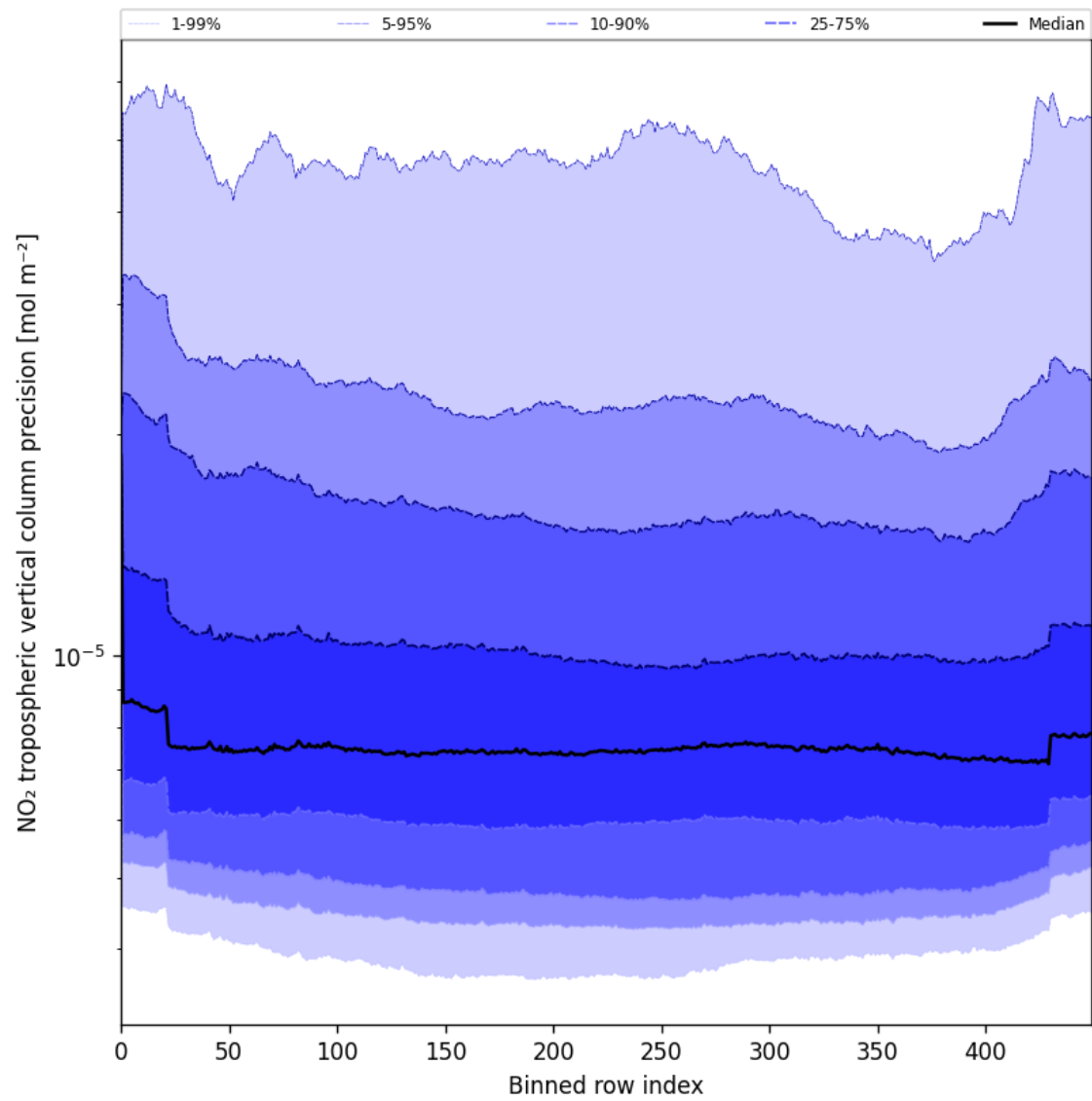
Figure 45: Along track statistics of “NO 2 tropospheric vertical column precision” for 2025-07-22 to 2025-07-22
