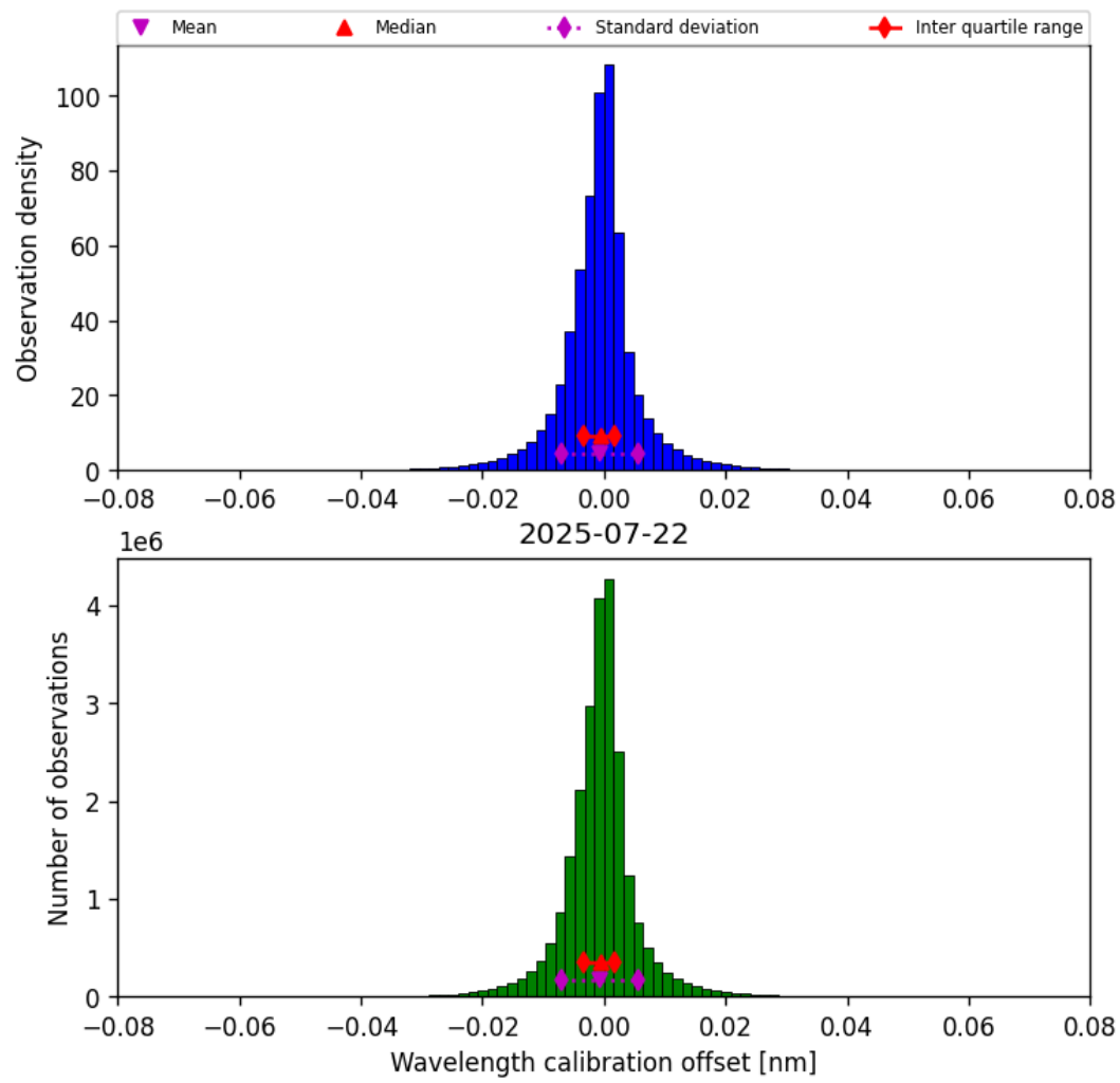
Figure 33: Histogram of “Wavelength calibration offset” for 2025-07-22 to 2025-07-22
