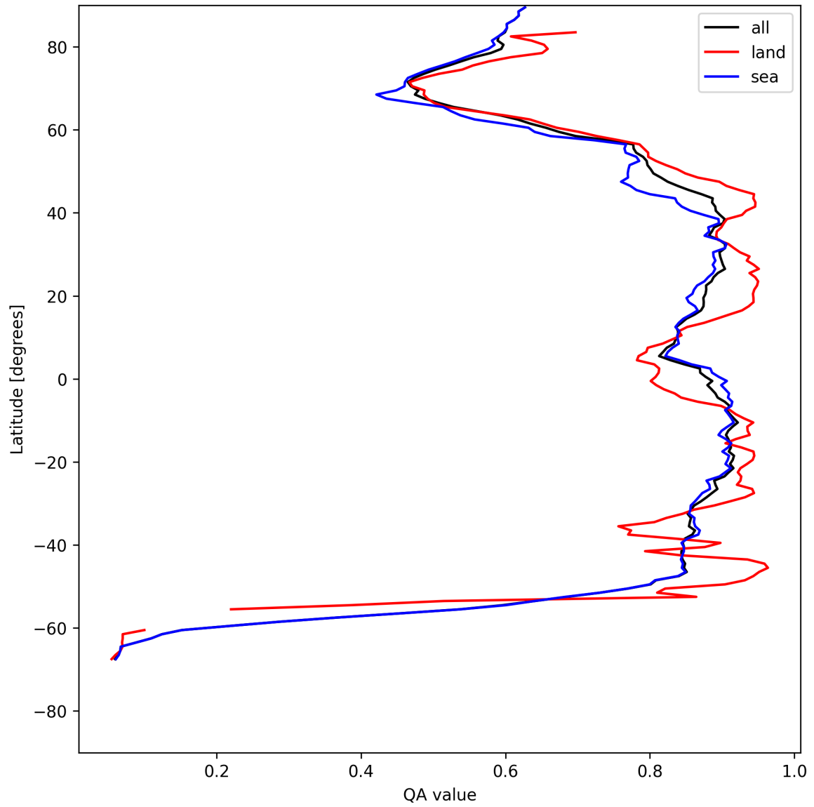
Figure 9: Zonal average of “QA value” for 2025-07-22 to 2025-07-22.
