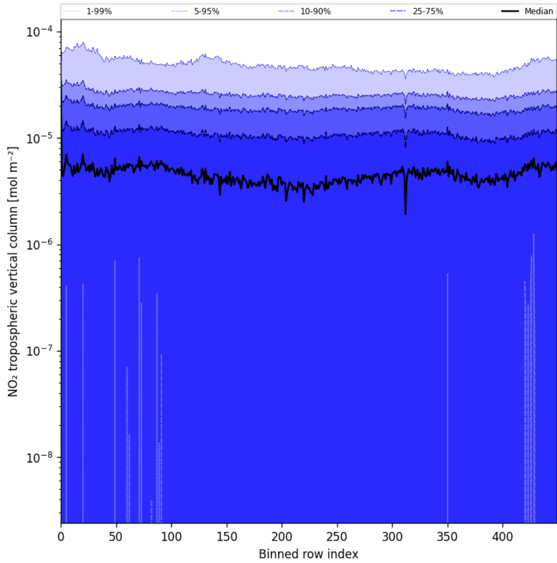
Figure 44: Along track statistics of “NO 2 tropospheric vertical column” for 2025-07-22 to 2025-07-22
