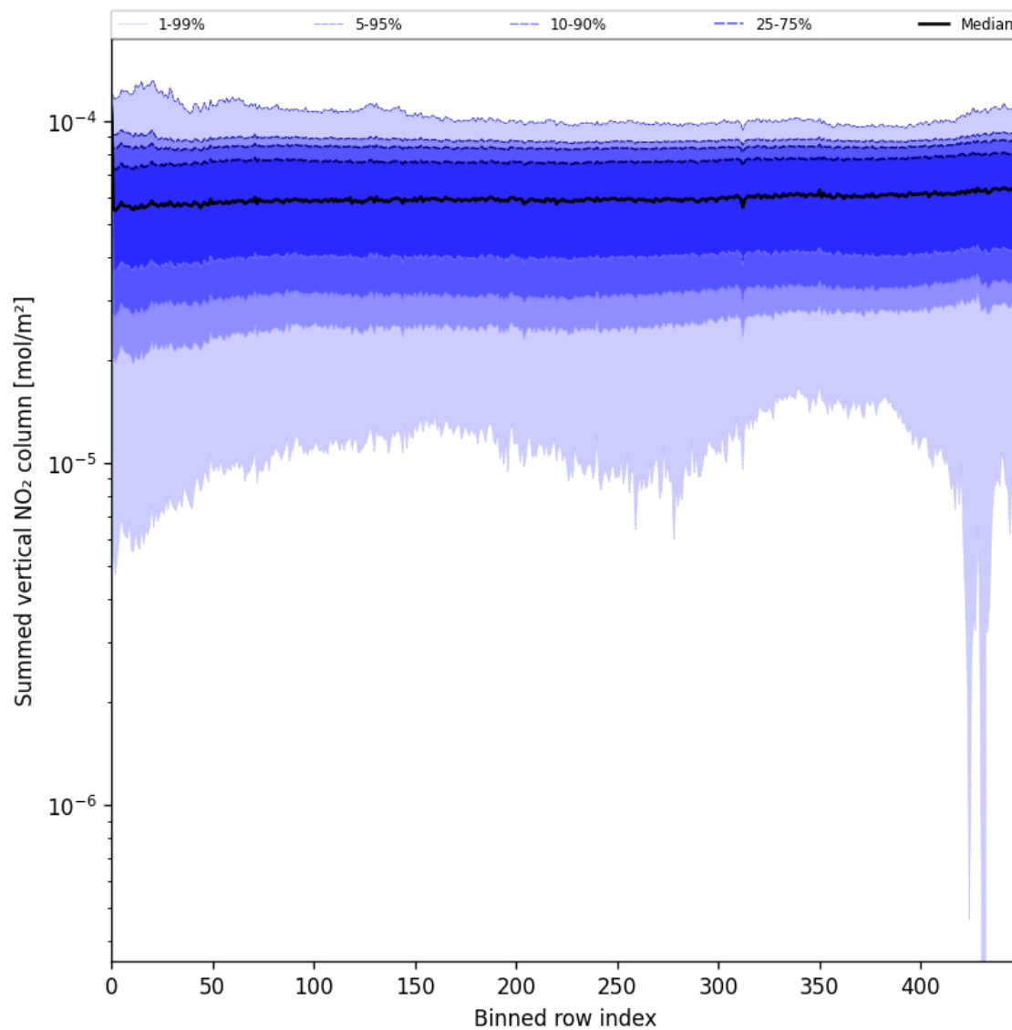
Figure 55: Along track statistics of “Summed vertical NO 2 column” for 2025-07-22 to 2025-07-22
