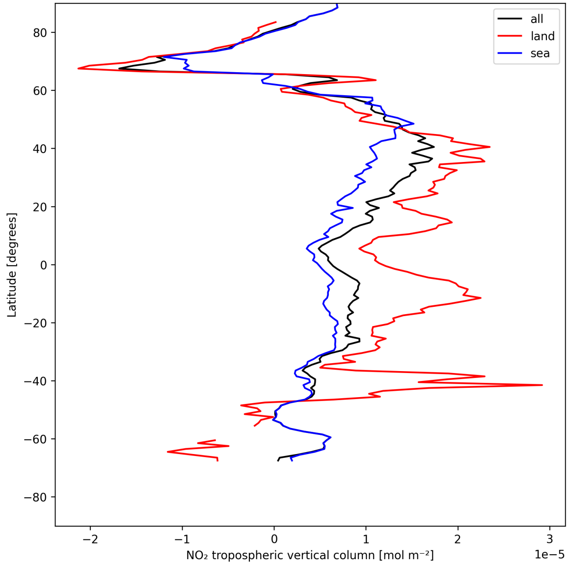
Figure 10: Zonal average of “NO 2 tropospheric vertical column” for 2025-07-22 to 2025-07-22.
