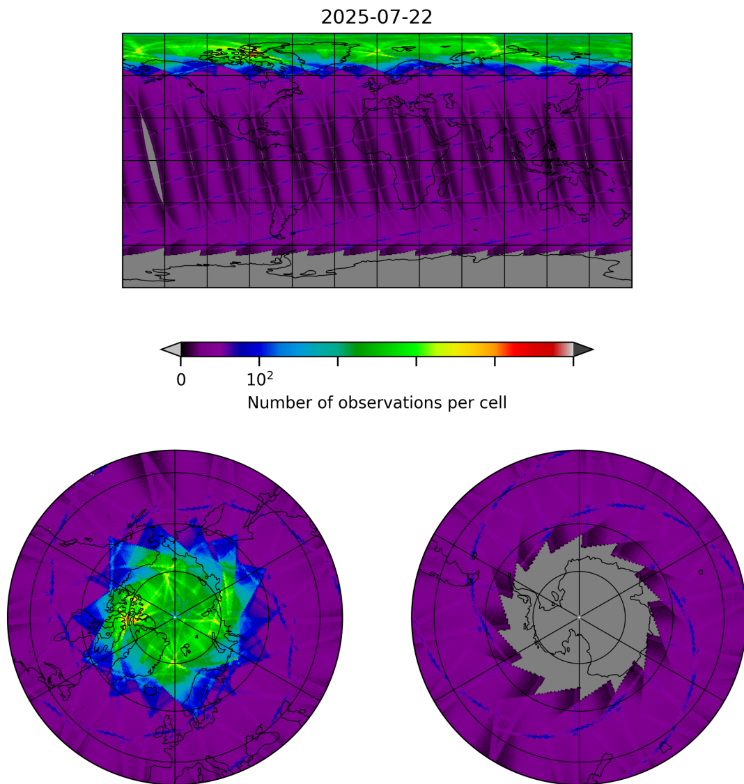
Figure 8: Map of the number of observations for 2025-07-22 to 2025-07-22
