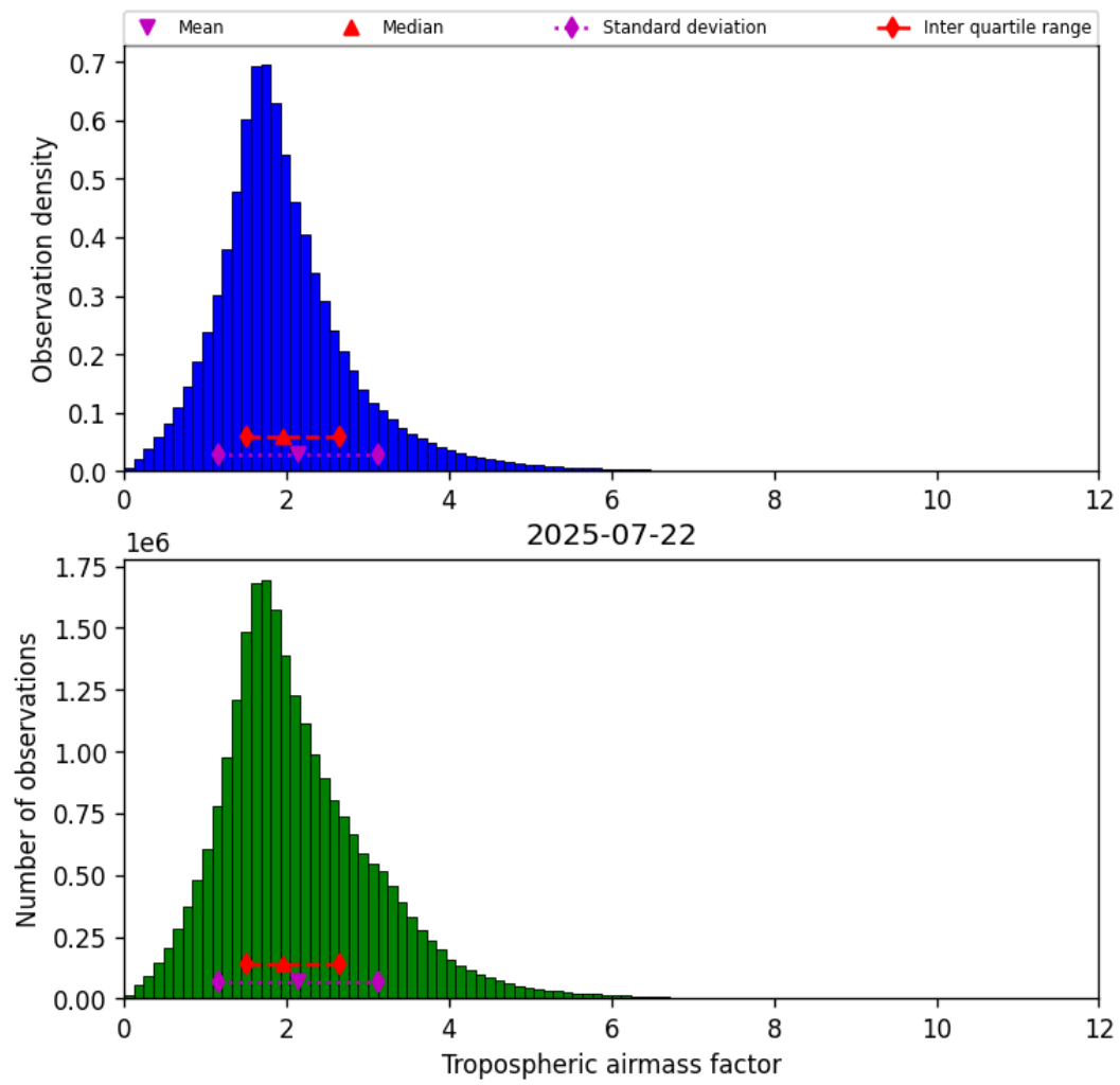
Figure 29: Histogram of “Tropospheric airmass factor” for 2025-07-22 to 2025-07-22
