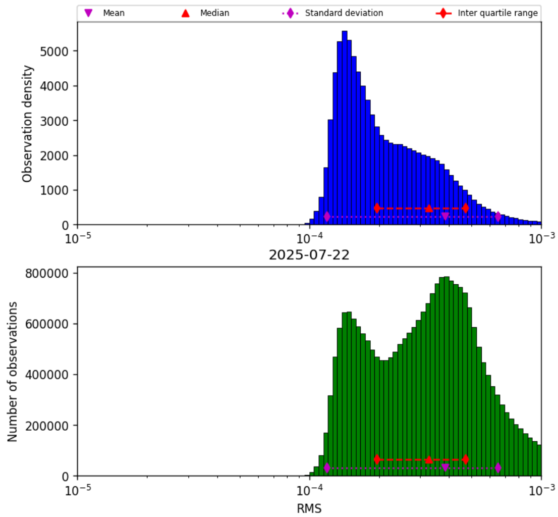
Figure 41: Histogram of “RMS” for 2025-07-22 to 2025-07-22
