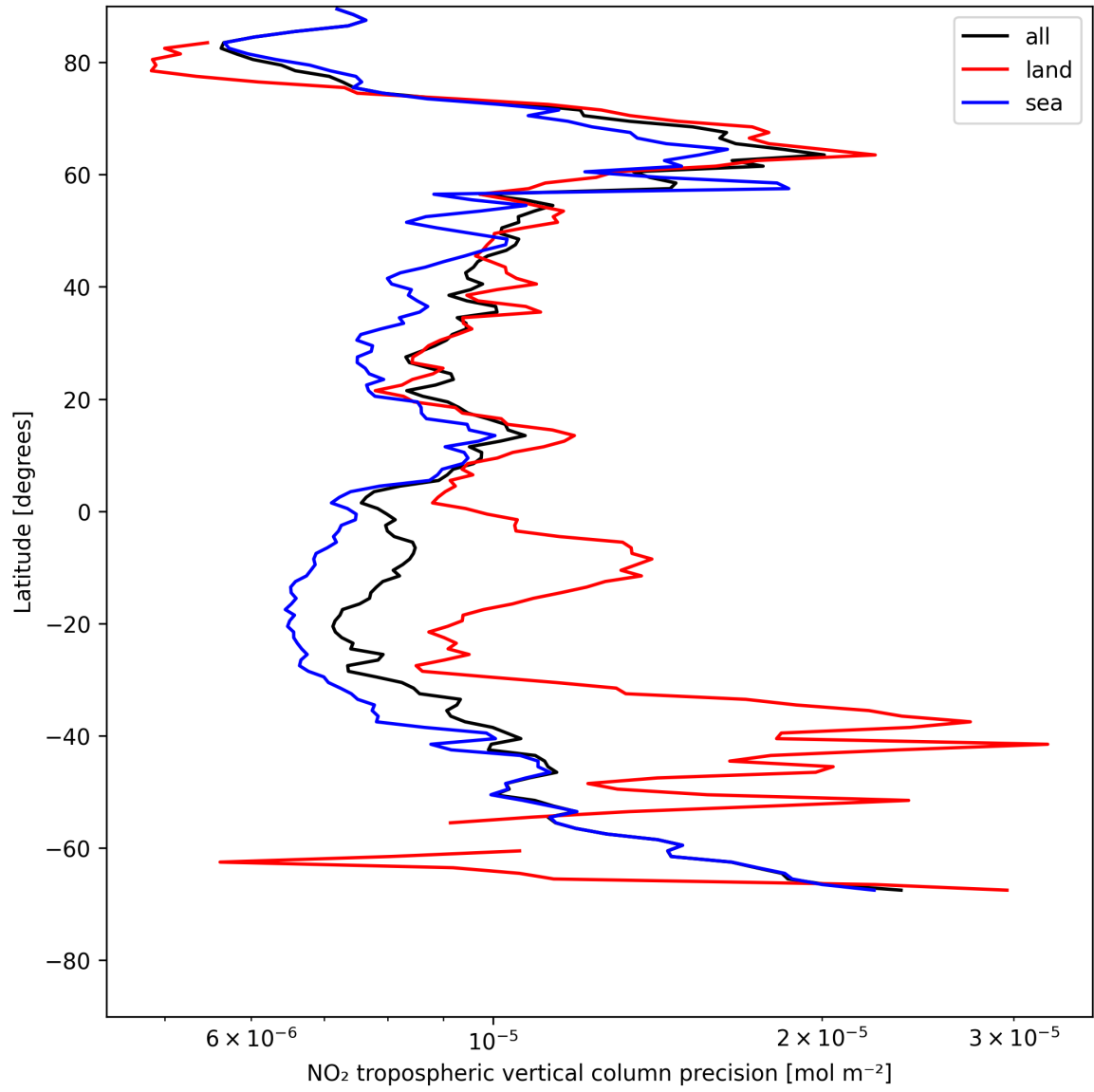
Figure 11: Zonal average of “NO 2 tropospheric vertical column precision” for 2025-07-22 to 2025-07-22.
