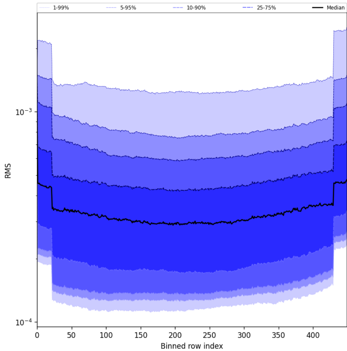
Figure 58: Along track statistics of “RMS” for 2025-07-22 to 2025-07-22
