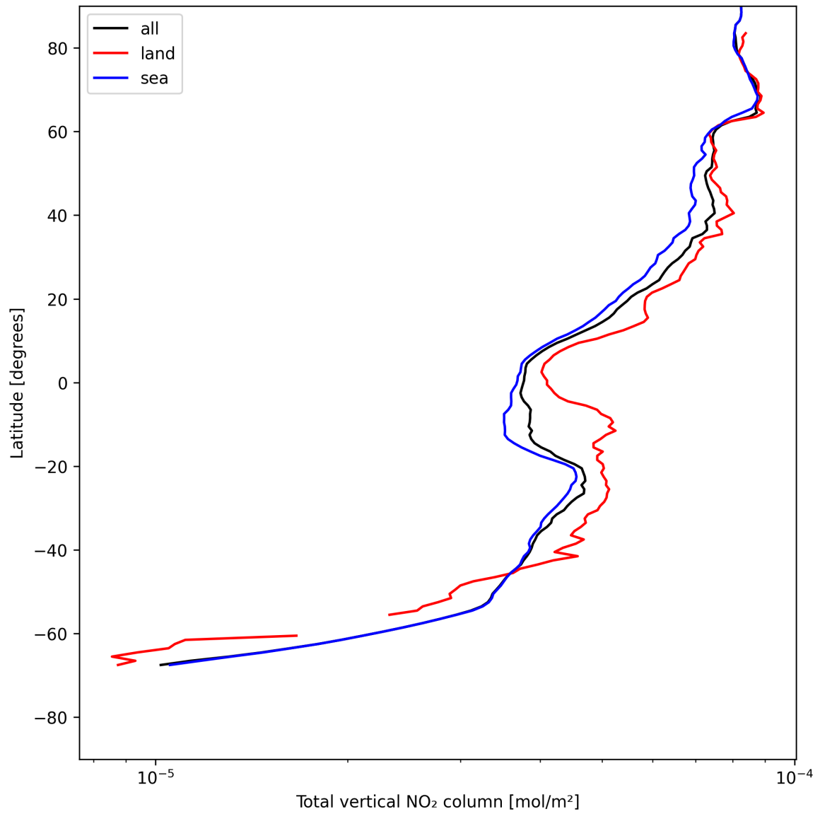
Figure 19: Zonal average of “Total vertical NO 2 column” for 2025-07-22 to 2025-07-22.
