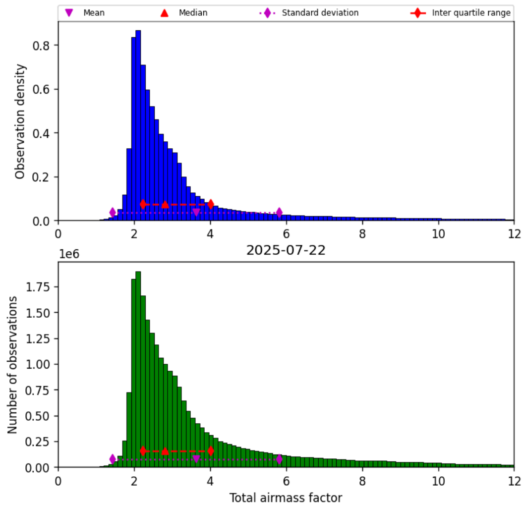
Figure 30: Histogram of “Total airmass factor” for 2025-07-22 to 2025-07-22
