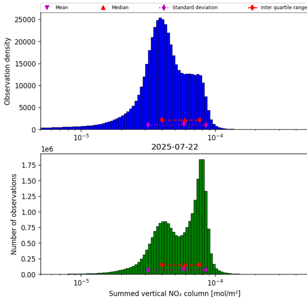
Figure 38: Histogram of "Summed vertical NO 2 column" for 2025-07-22 to 2025-07-22
