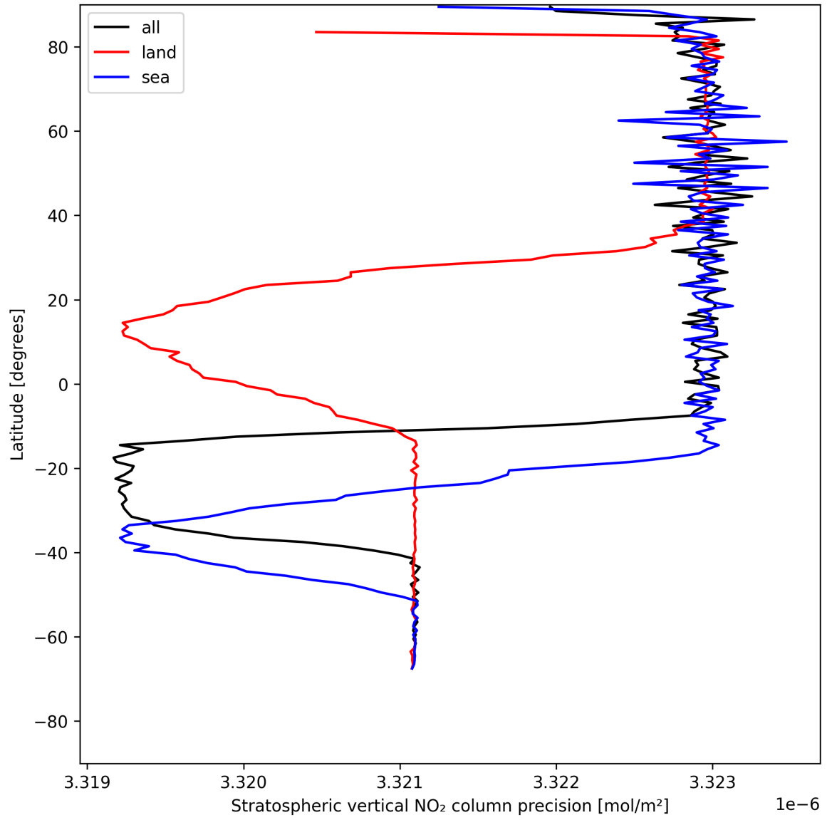
Figure 18: Zonal average of “Stratospheric vertical NO 2 column precision” for 2025-07-22 to 2025-07-22.
