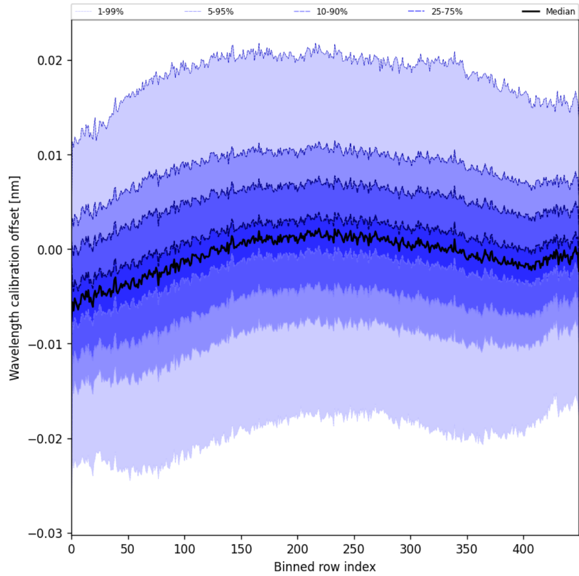
Figure 50: Along track statistics of “Wavelength calibration offset” for 2025-07-22 to 2025-07-22
