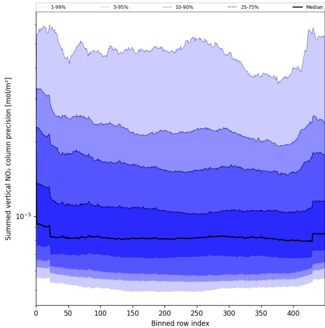
Figure 56: Along track statistics of “Summed vertical NO 2 column precision” for 2025-07-22 to 2025-07-22
