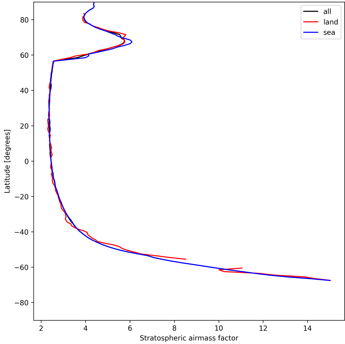
Figure 25: Zonal average of “Stratospheric air mass factor” for 2025-07-22 to 2025-07-22.
