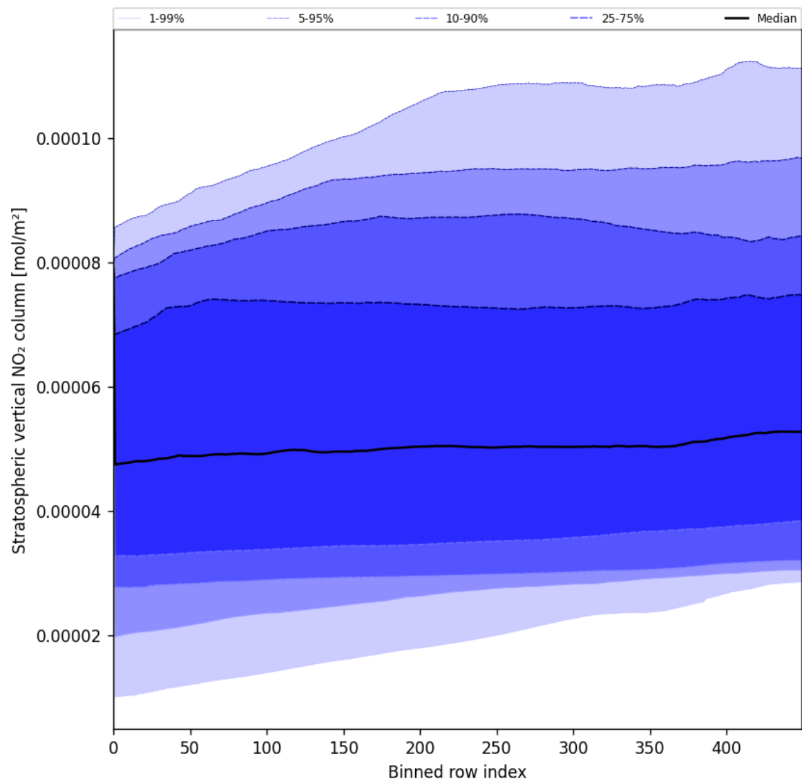
Figure 51: Along track statistics of “Stratospheric vertical NO 2 column” for 2025-07-22 to 2025-07-22
