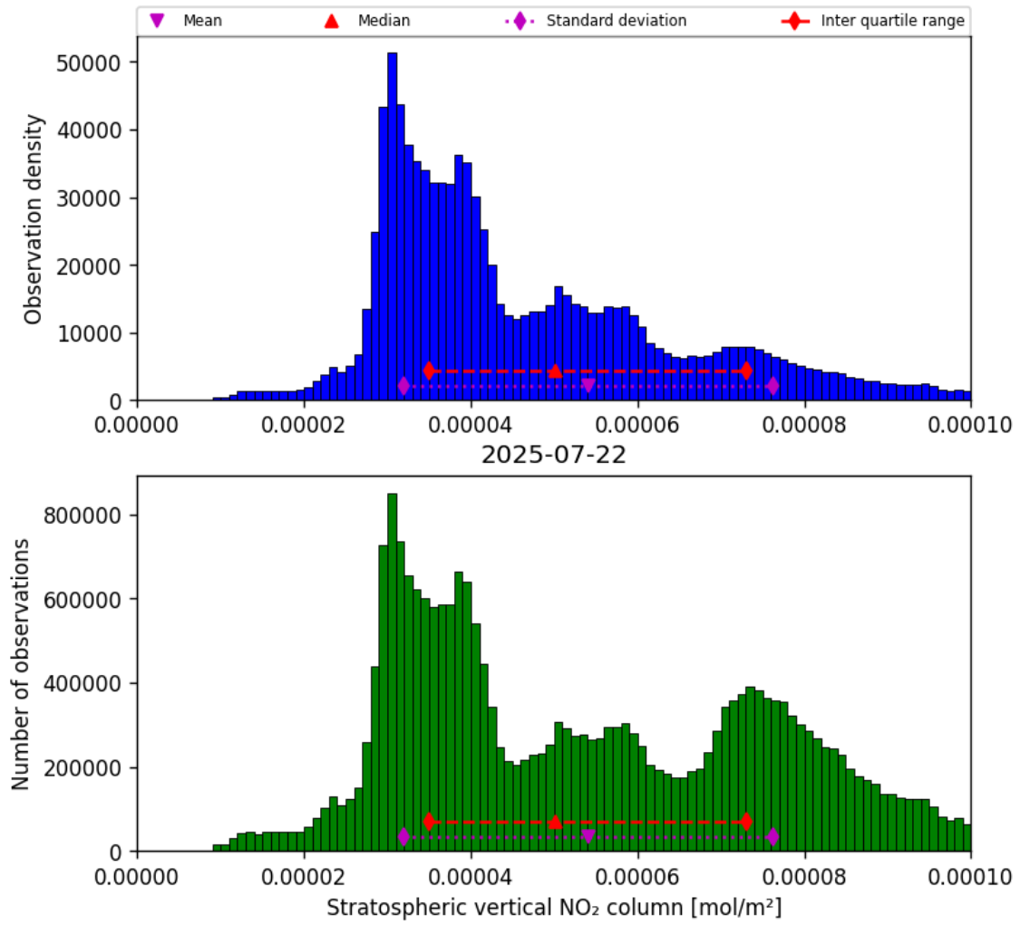
Figure 34: Histogram of “Stratospheric vertical NO 2 column” for 2025-07-22 to 2025-07-22
