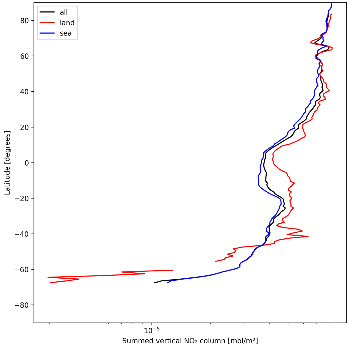
Figure 21: Zonal average of “Summed vertical NO 2 column” for 2025-07-22 to 2025-07-22.
