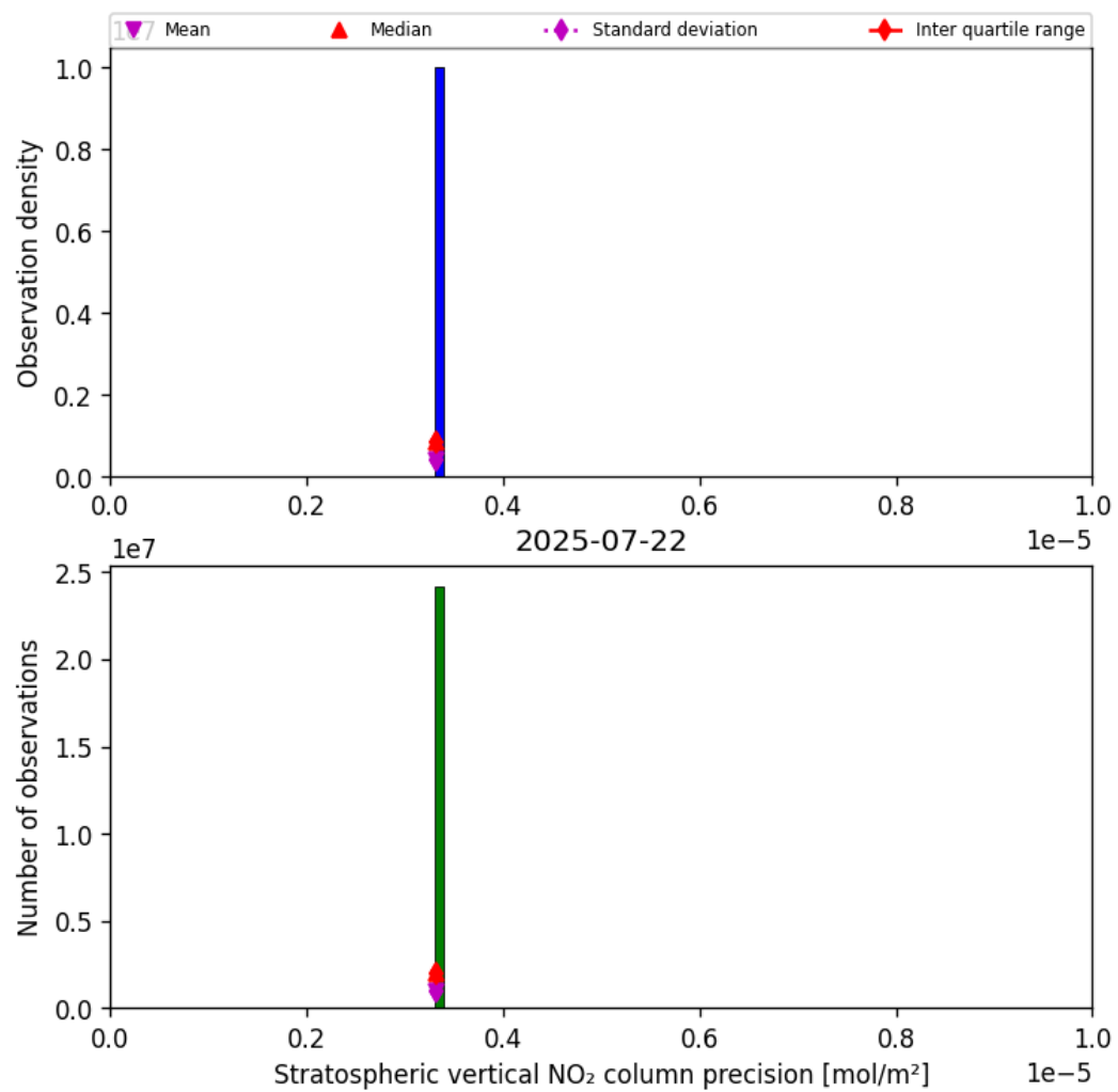
Figure 35: Histogram of “Stratospheric vertical NO 2 column precision” for 2025-07-22 to 2025-07-22
