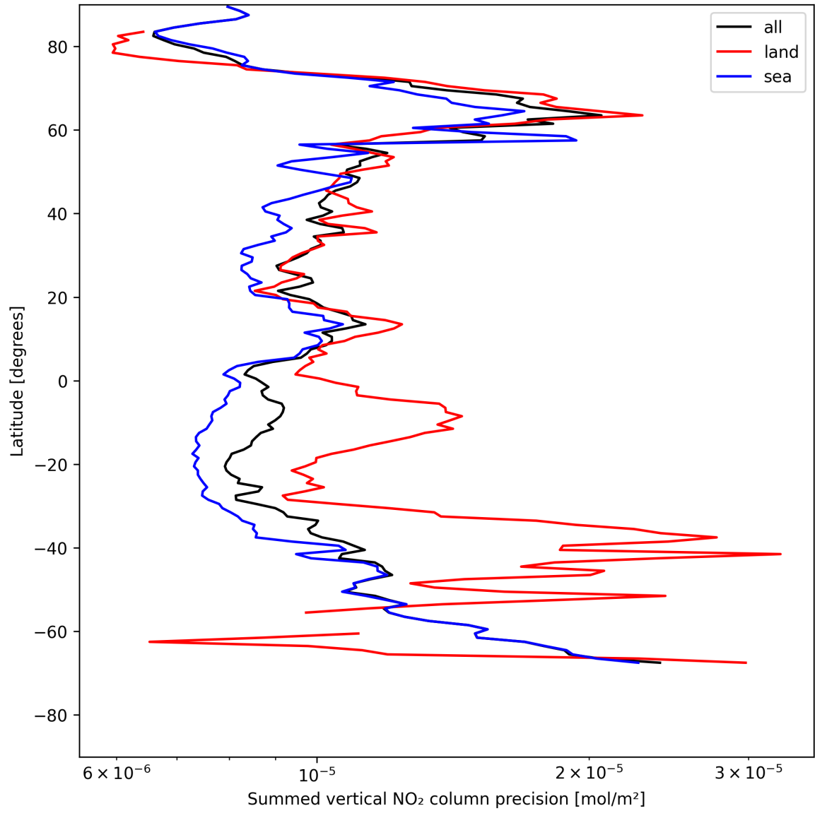
Figure 22: Zonal average of “Summed vertical NO 2 column precision” for 2025-07-22 to 2025-07-22.
