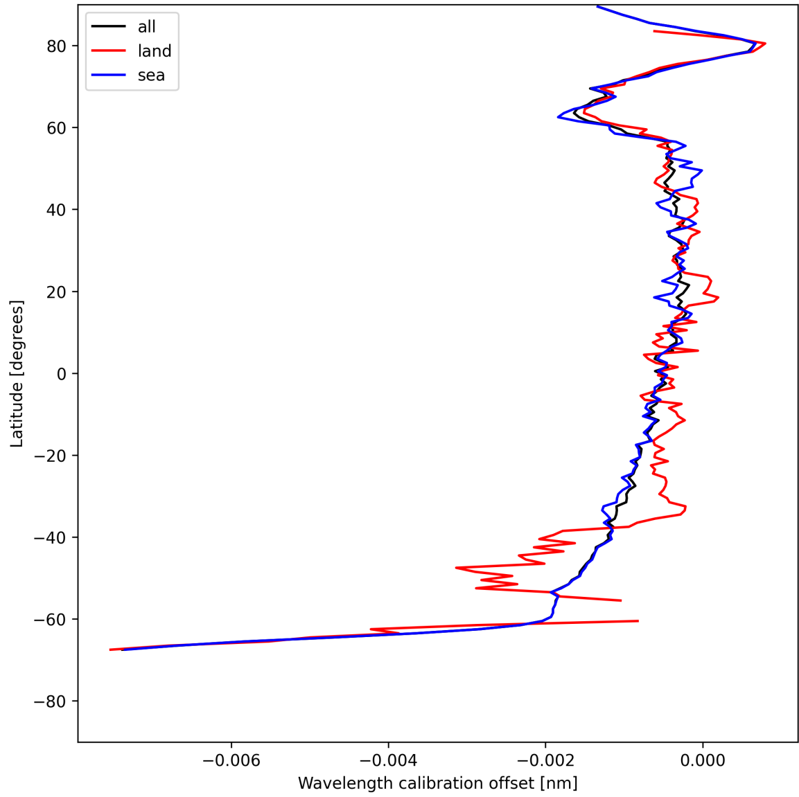
Figure 16: Zonal average of “Wavelength calibration offset” for 2025-07-22 to 2025-07-22.
