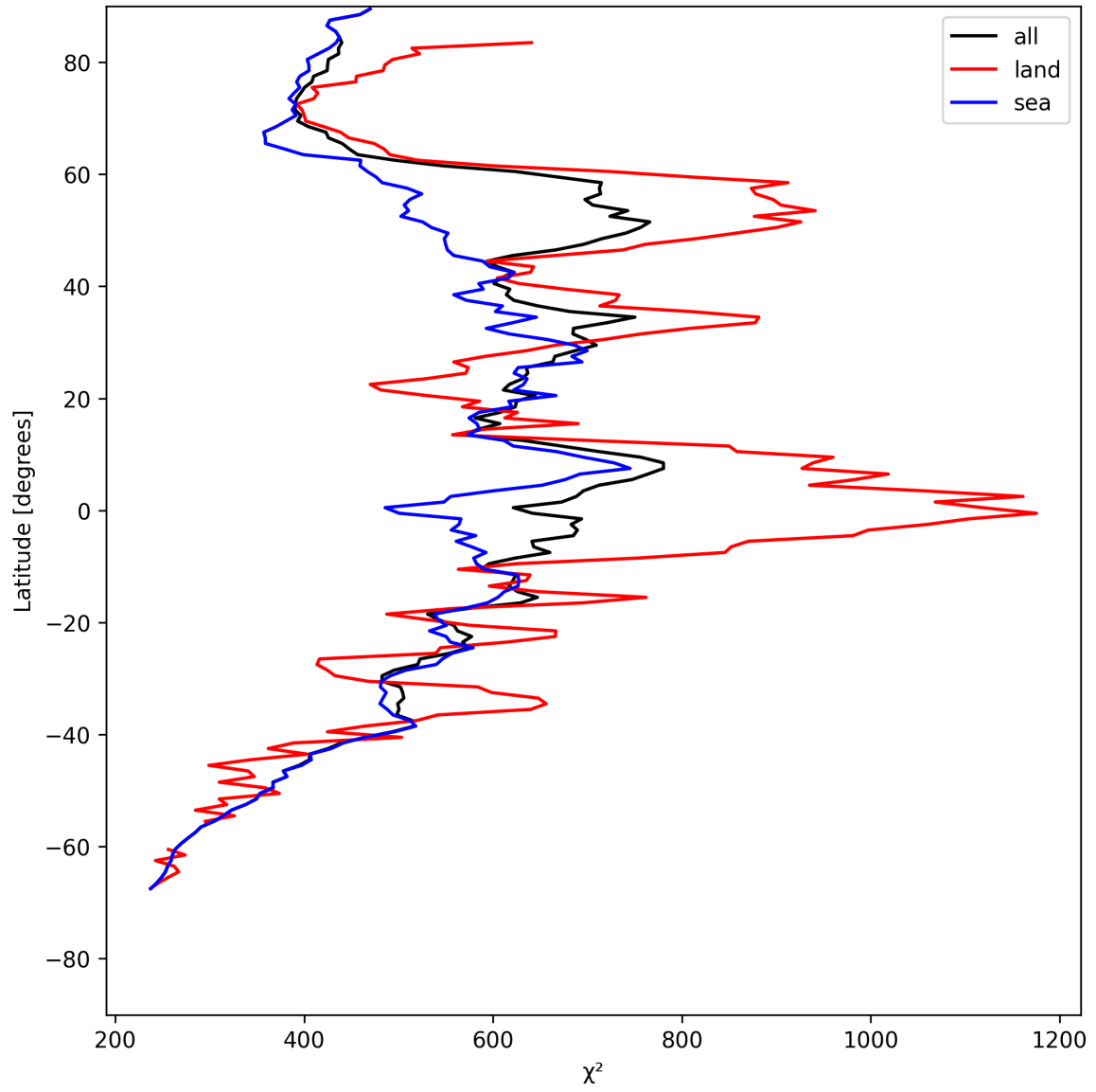
Figure 23: Zonal average of “ \chi^2 ” for 2025-07-22 to 2025-07-22.
