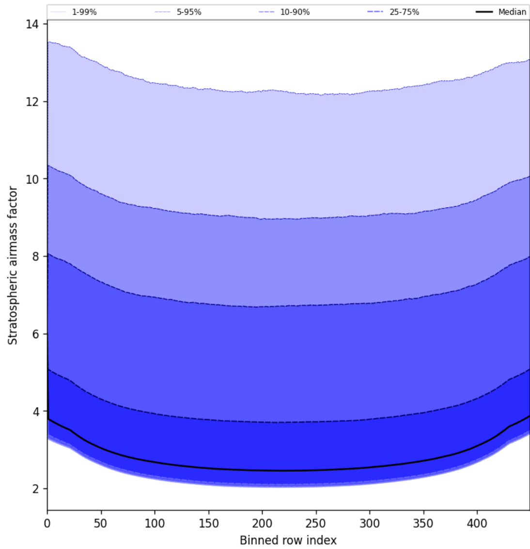
Figure 59: Along track statistics of “Stratospheric airmass factor” for 2025-07-22 to 2025-07-22
