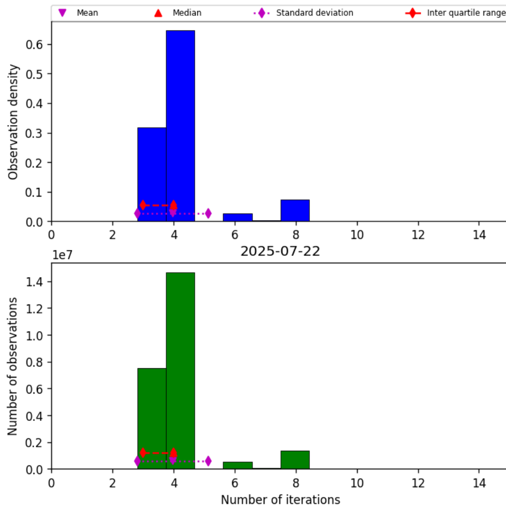
Figure 32: Histogram of “Number of iterations” for 2025-07-22 to 2025-07-22
