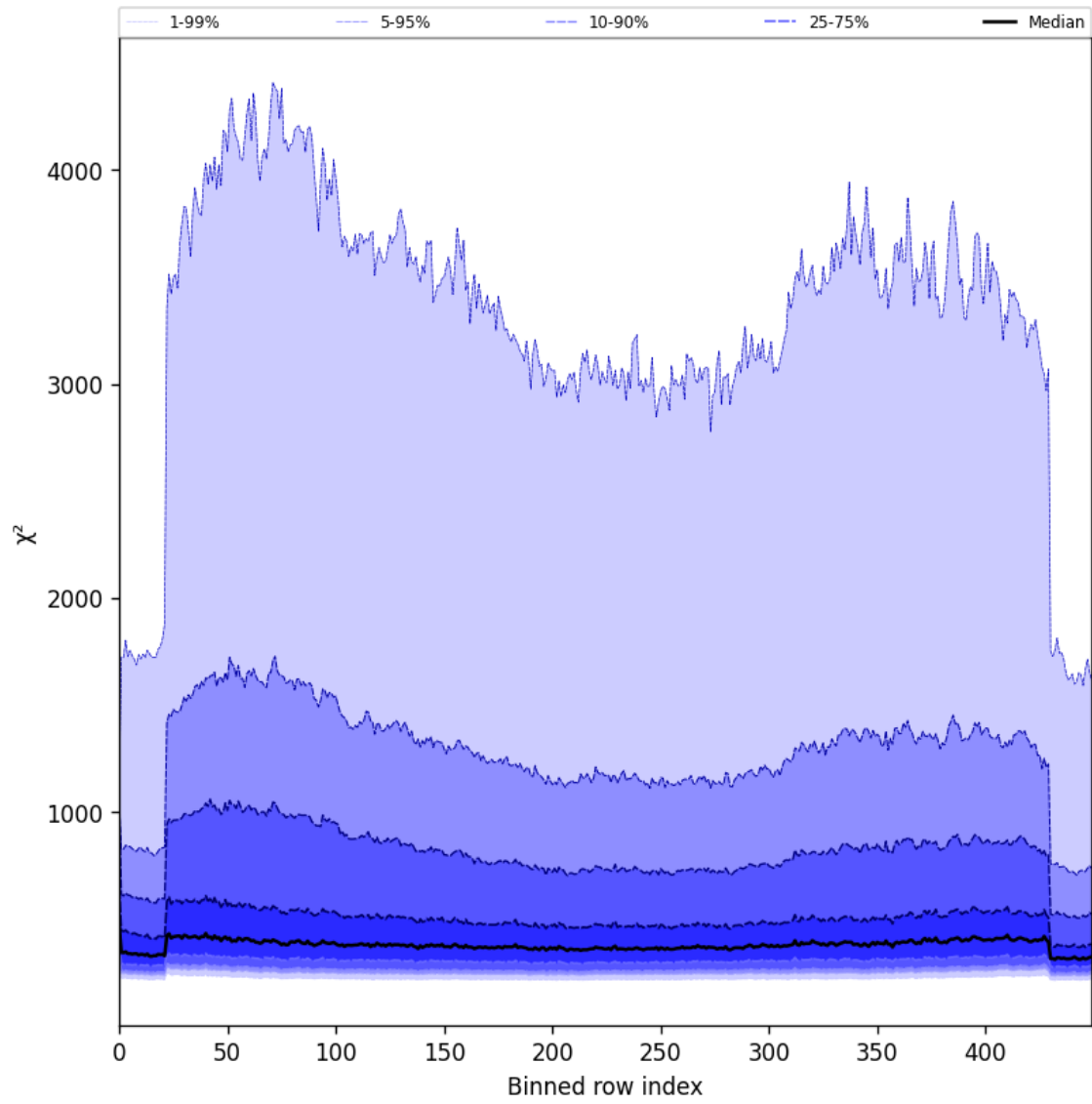
Figure 57: Along track statistics of “ \chi^2 ” for 2025-07-22 to 2025-07-22
