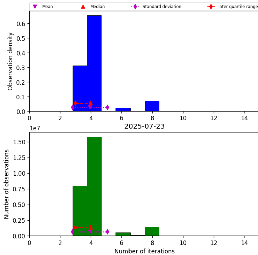
Figure 32: Histogram of “Number of iterations” for 2025-07-23 to 2025-07-24
