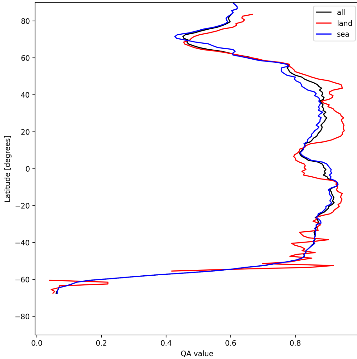
Figure 9: Zonal average of “QA value” for 2025-07-23 to 2025-07-24.
