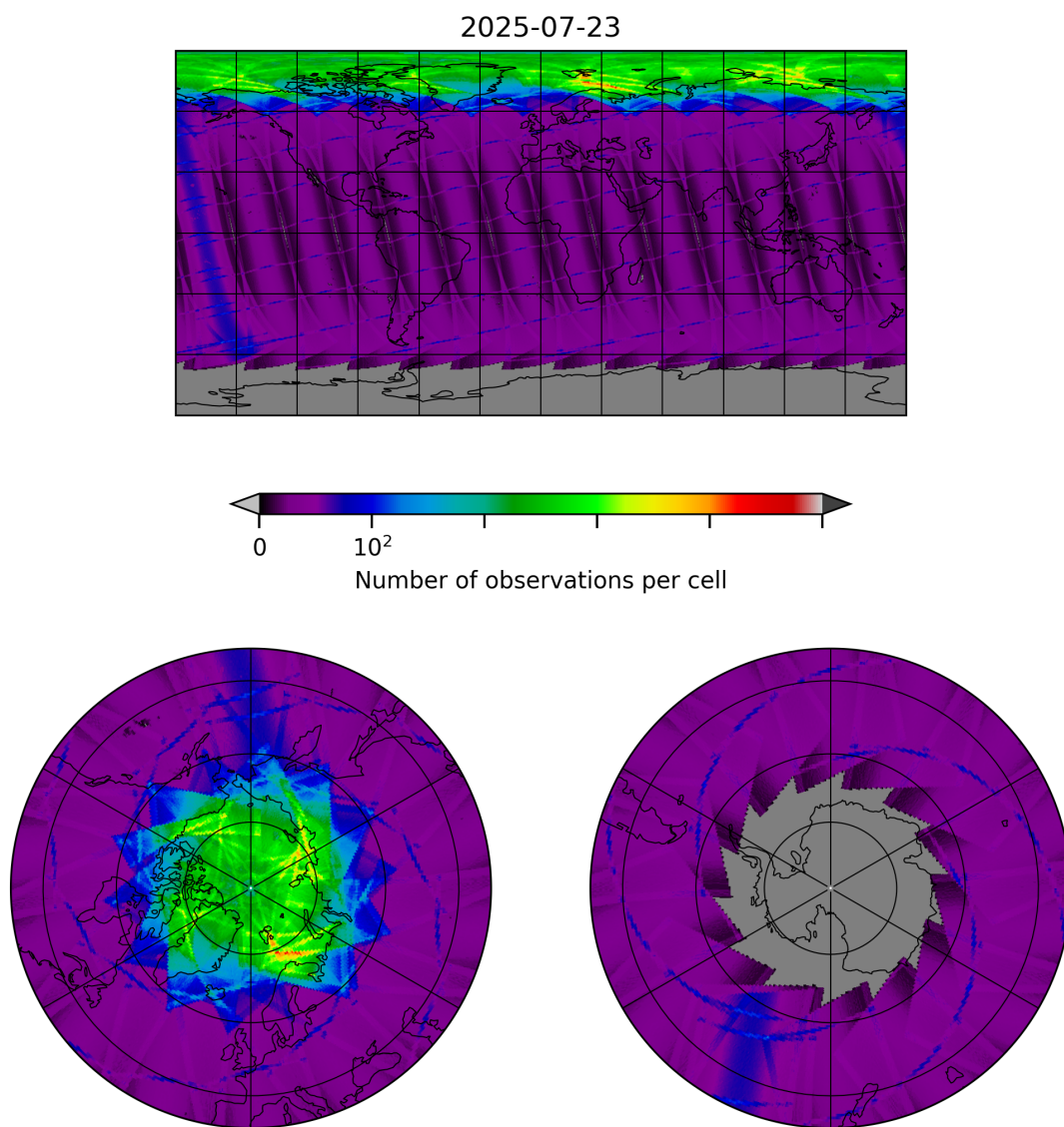
Figure 8: Map of the number of observations for 2025-07-23 to 2025-07-24
