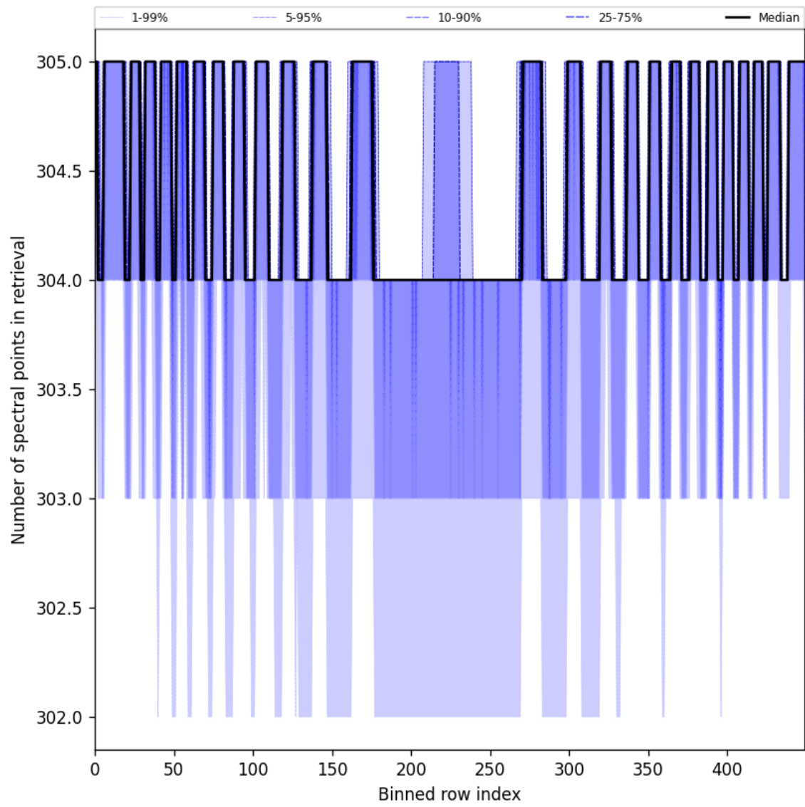
Figure 48: Along track statistics of “Number of spectral points in retrieval” for 2025-07-23 to 2025-07-24
