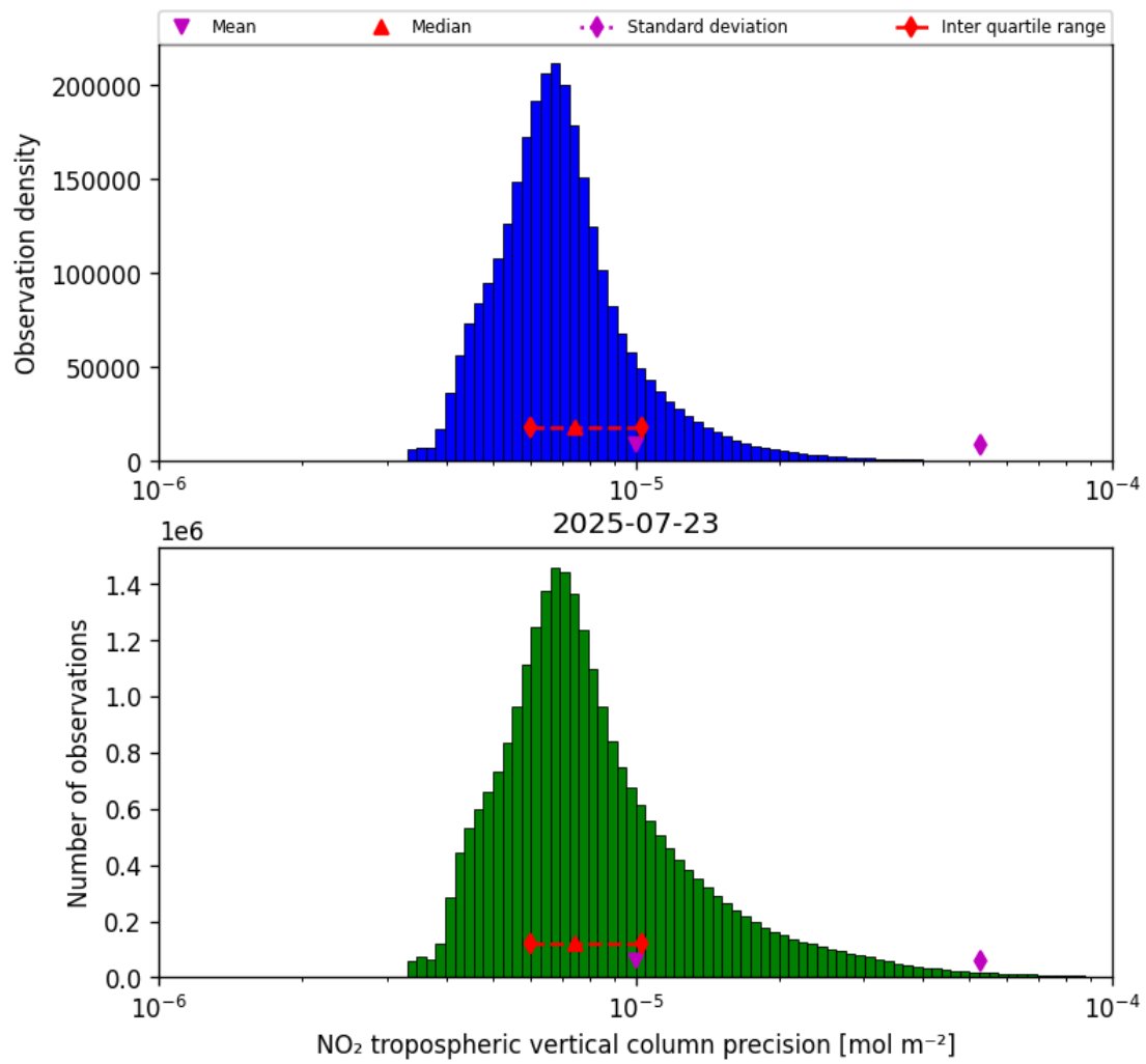
Figure 28: Histogram of “NO 2 tropospheric vertical column precision” for 2025-07-23 to 2025-07-24
