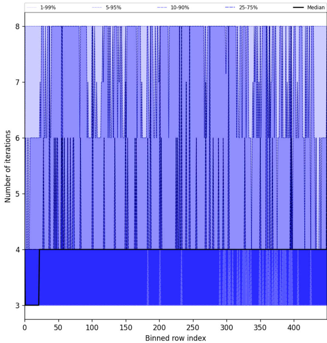
Figure 49: Along track statistics of “Number of iterations” for 2025-07-23 to 2025-07-24
