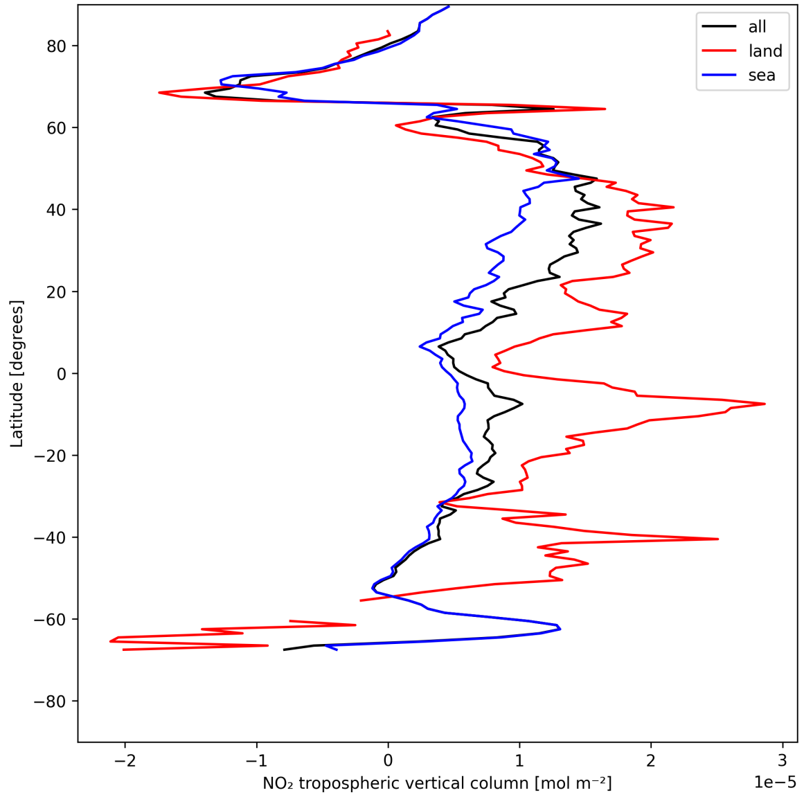
Figure 10: Zonal average of “NO 2 tropospheric vertical column” for 2025-07-23 to 2025-07-24.
