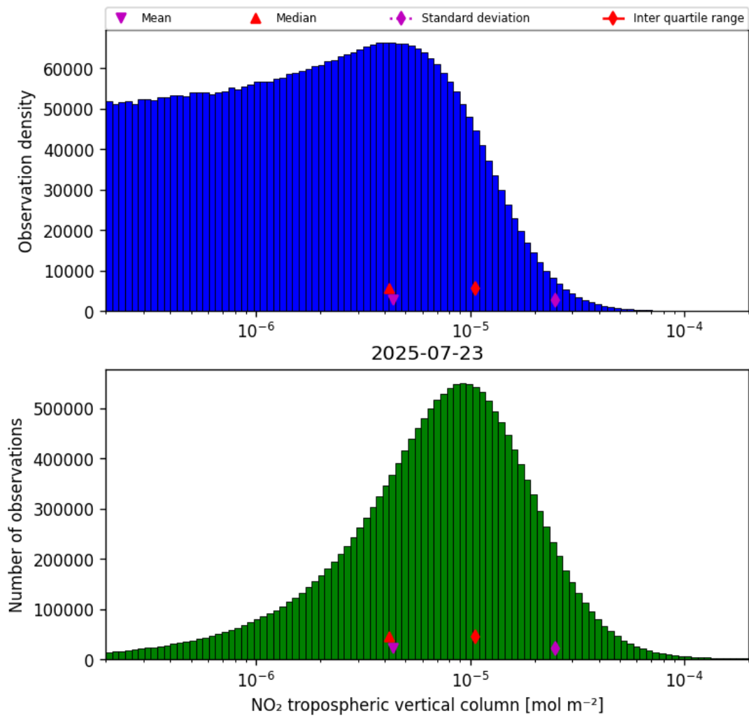
Figure 27: Histogram of “NO 2 tropospheric vertical column” for 2025-07-23 to 2025-07-24
