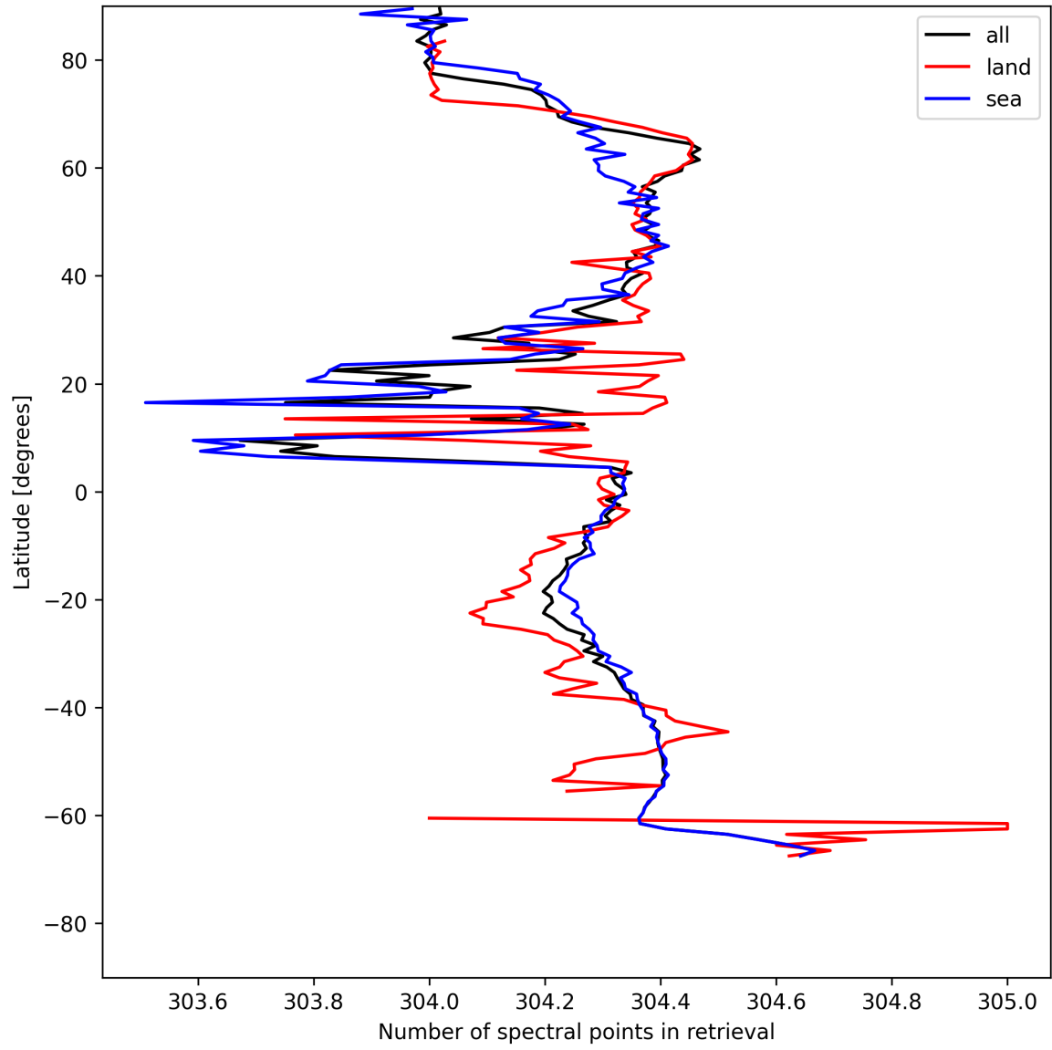
Figure 14: Zonal average of “Number of spectral points in retrieval” for 2025-07-23 to 2025-07-24.
