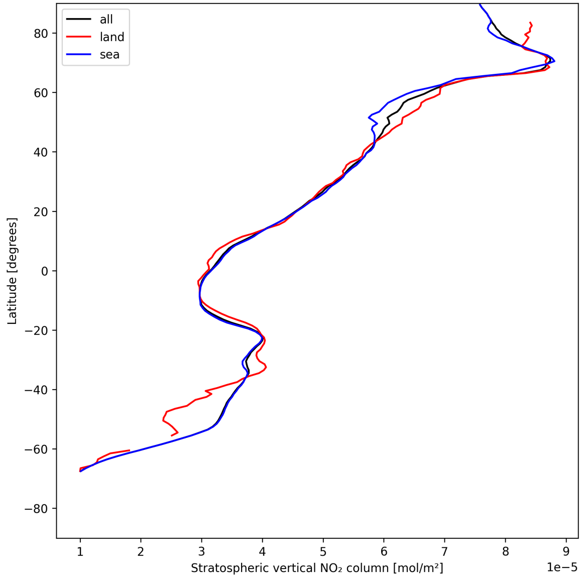
Figure 17: Zonal average of “Stratospheric vertical NO 2 column” for 2025-07-23 to 2025-07-24.
