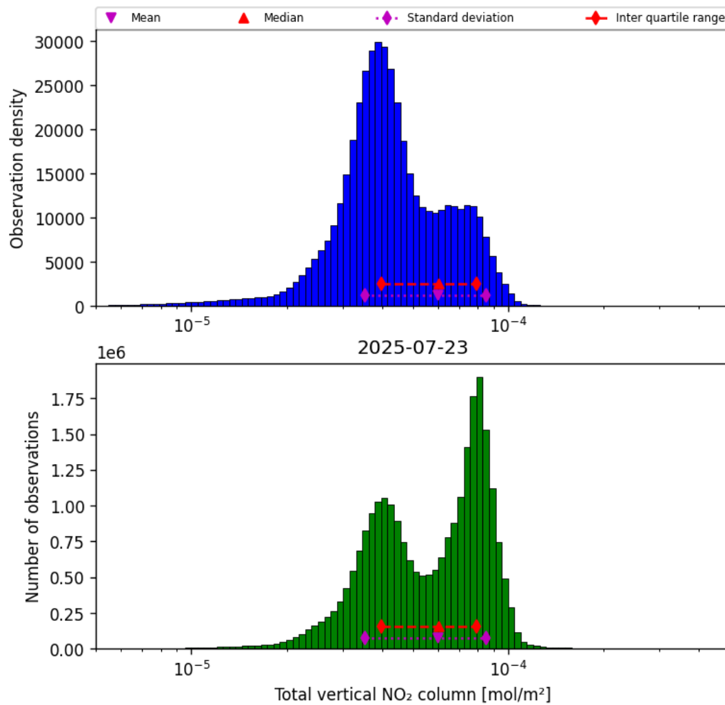
Figure 36: Histogram of "Total vertical NO 2 column" for 2025-07-23 to 2025-07-24
