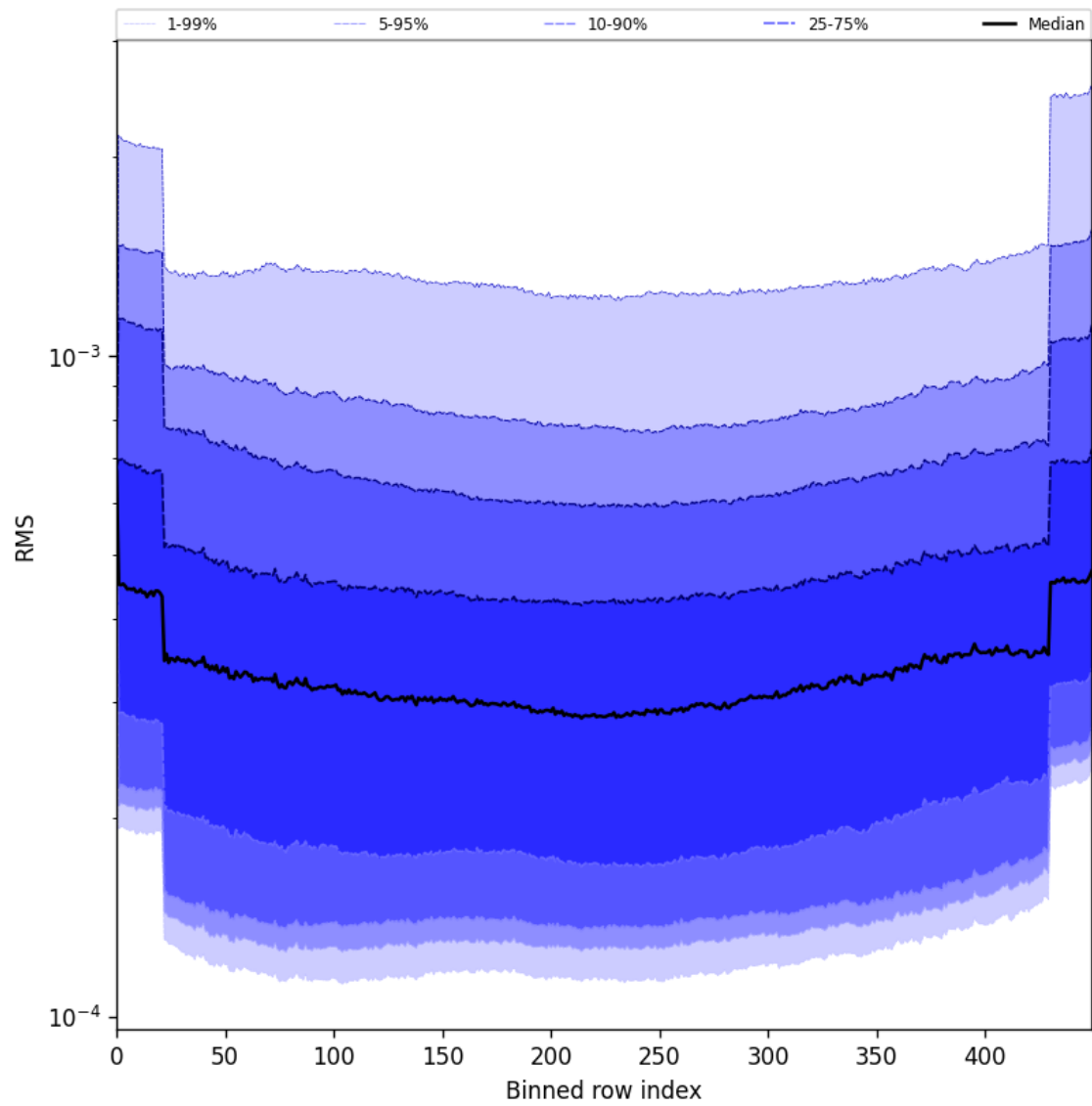
Figure 58: Along track statistics of “RMS” for 2025-07-23 to 2025-07-24
