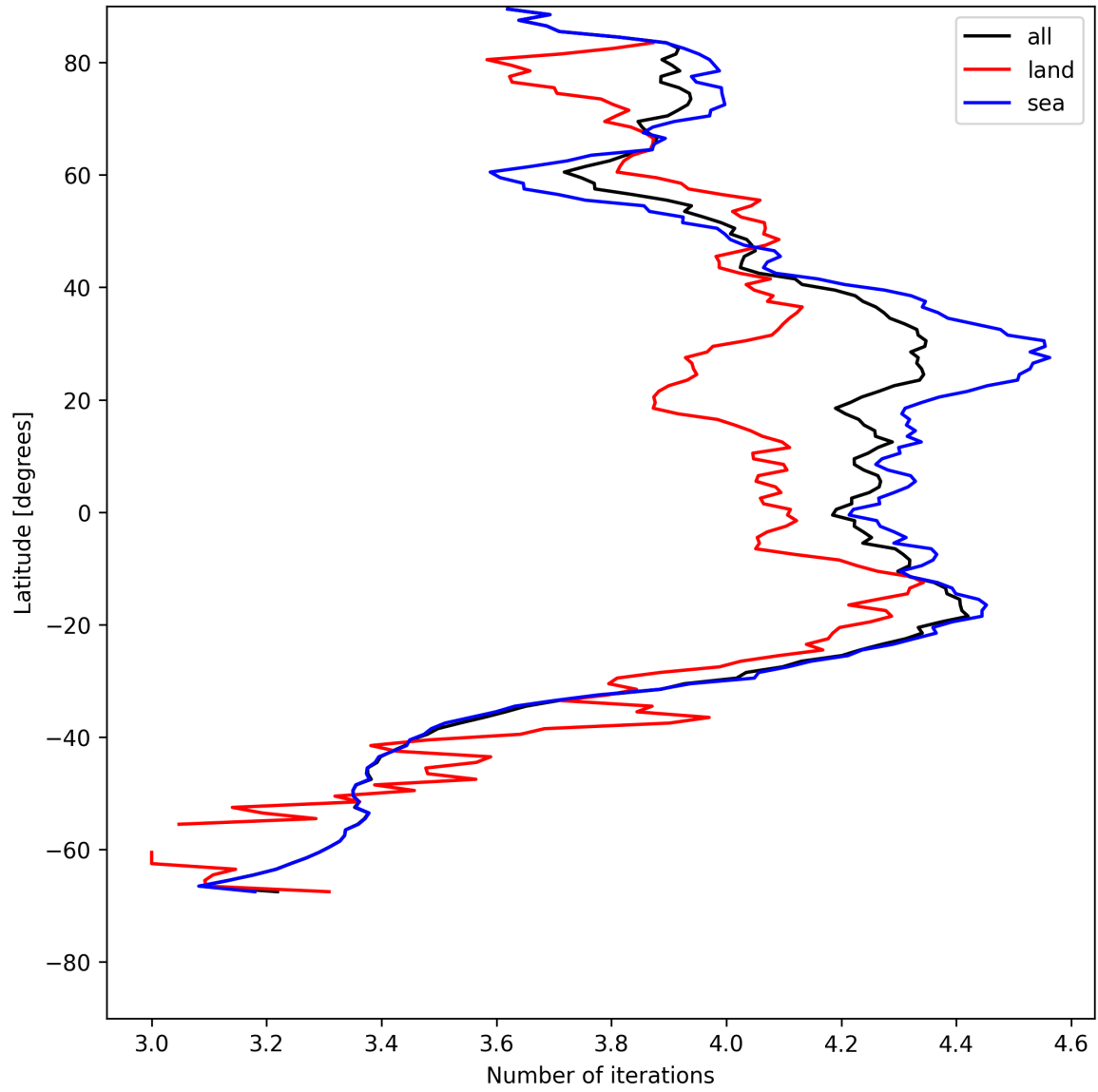
Figure 15: Zonal average of “Number of iterations” for 2025-07-23 to 2025-07-24.
