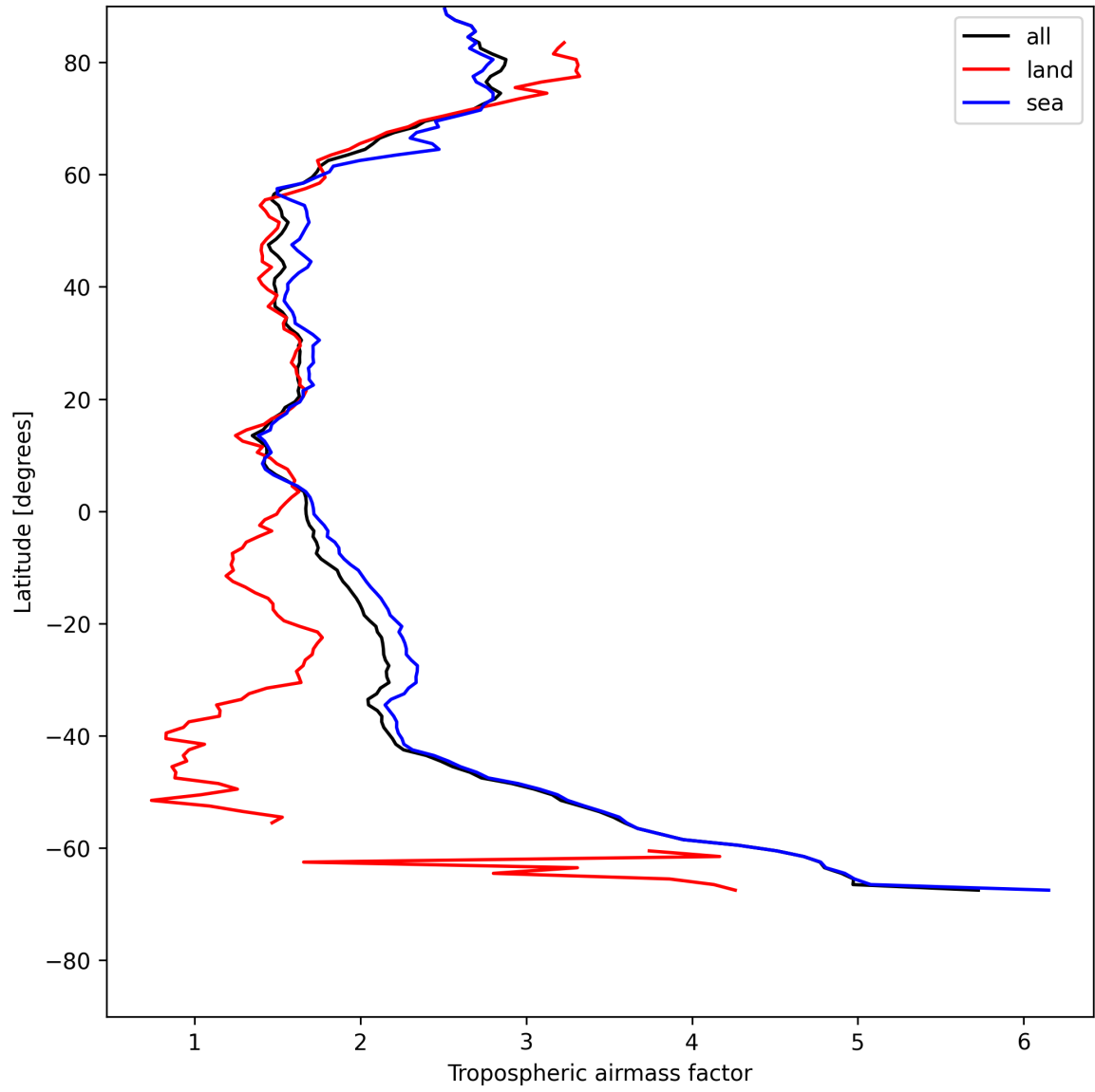
Figure 12: Zonal average of “Tropospheric airmass factor” for 2025-07-23 to 2025-07-24.
