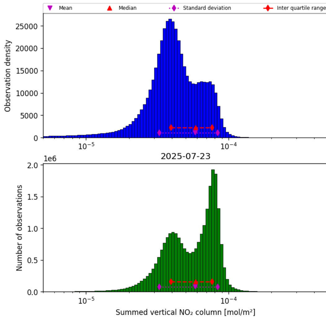
Figure 38: Histogram of “Summed vertical NO 2 column” for 2025-07-23 to 2025-07-24
