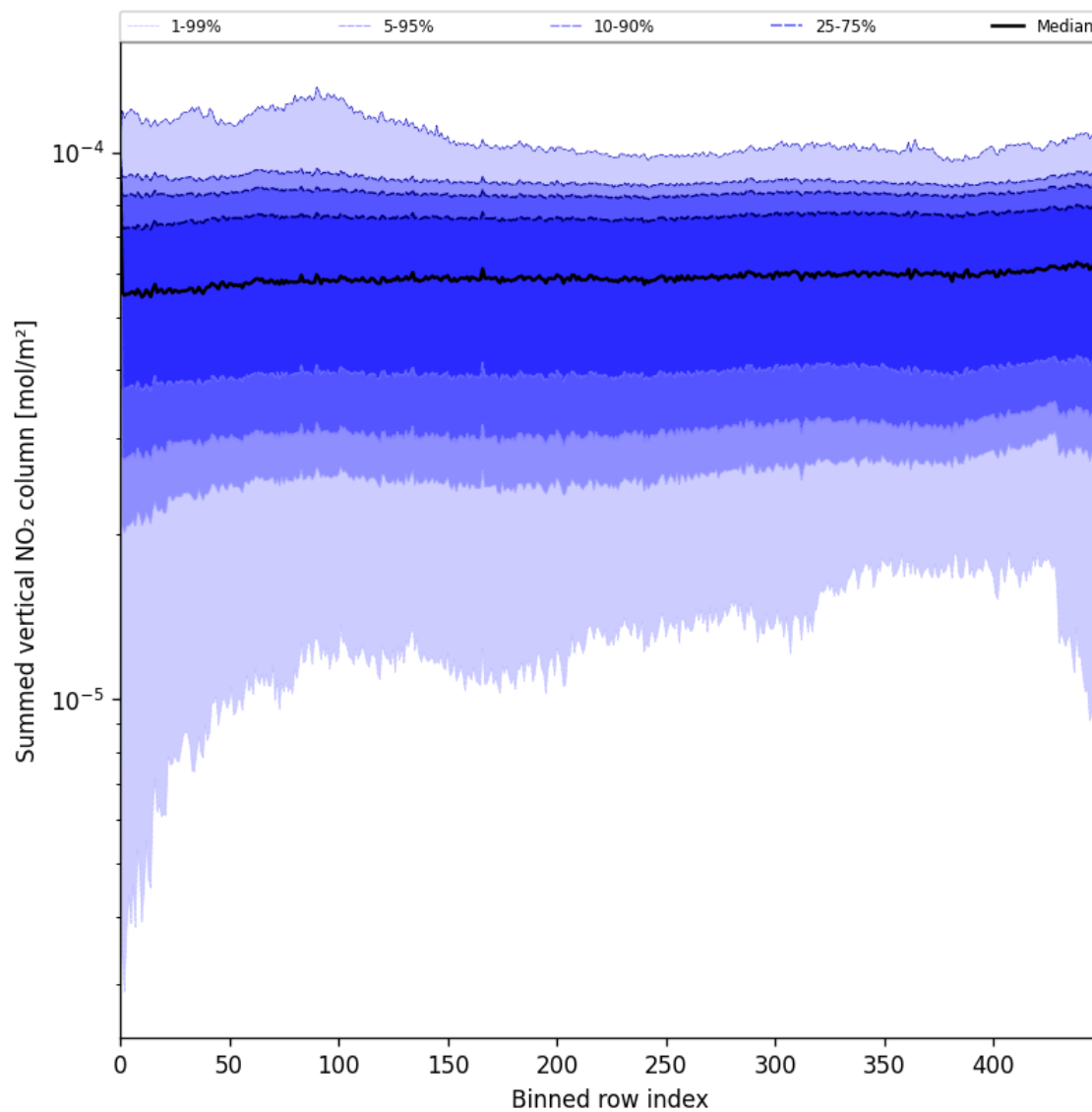
Figure 55: Along track statistics of “Summed vertical NO 2 column” for 2025-07-23 to 2025-07-24
