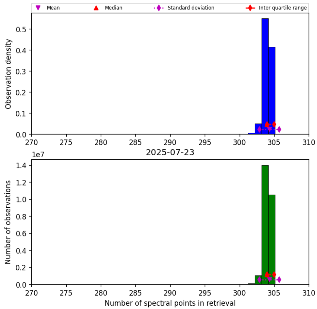
Figure 31: Histogram of “Number of spectral points in retrieval” for 2025-07-23 to 2025-07-24
