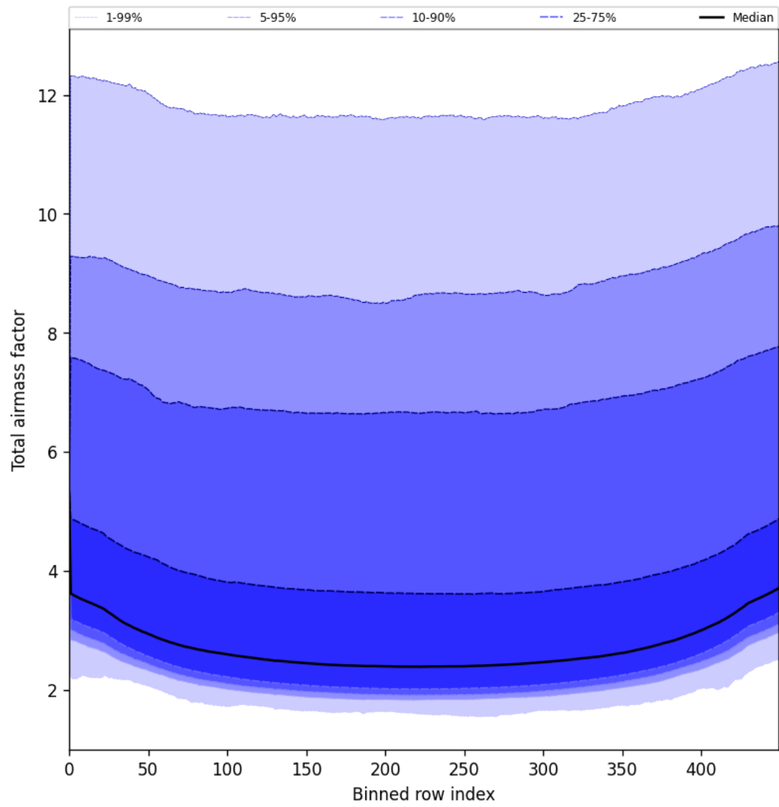
Figure 47: Along track statistics of “Total airmass factor” for 2025-07-23 to 2025-07-24
