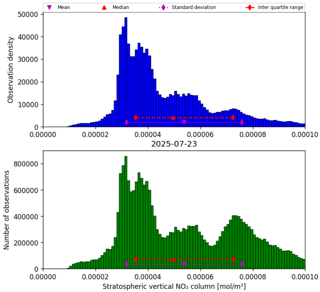
Figure 34: Histogram of “Stratospheric vertical NO 2 column” for 2025-07-23 to 2025-07-24
