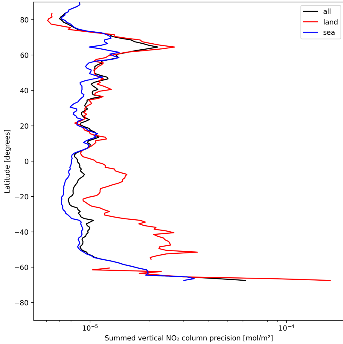
Figure 22: Zonal average of “Summed vertical NO 2 column precision” for 2025-07-23 to 2025-07-24.
