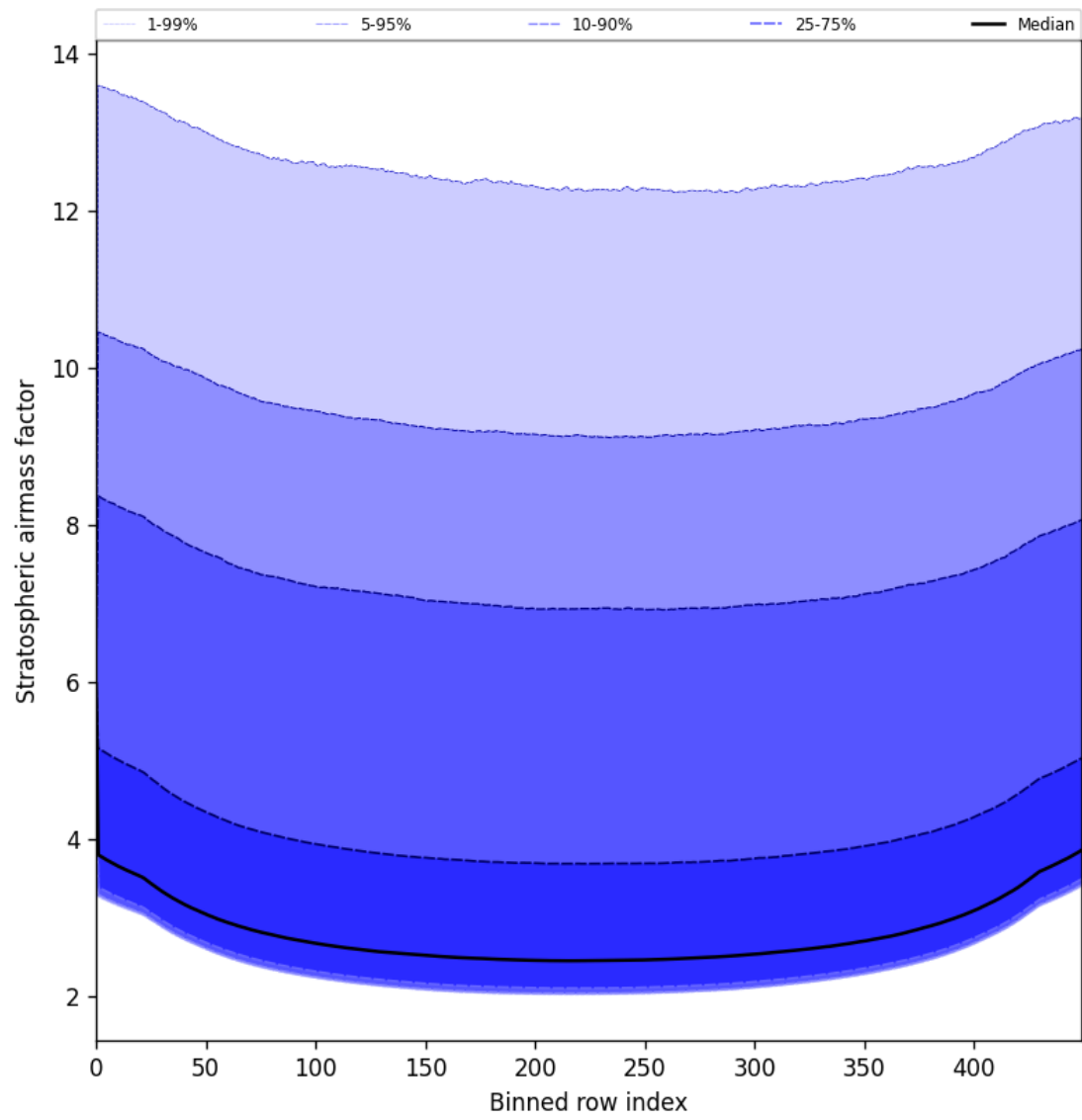
Figure 59: Along track statistics of “Stratospheric airmass factor” for 2025-07-23 to 2025-07-24
