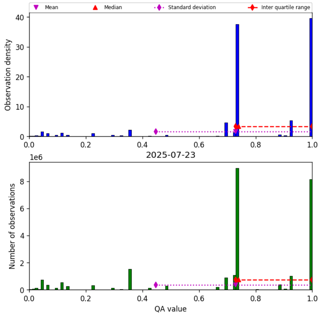
Figure 26: Histogram of “QA value” for 2025-07-23 to 2025-07-24
