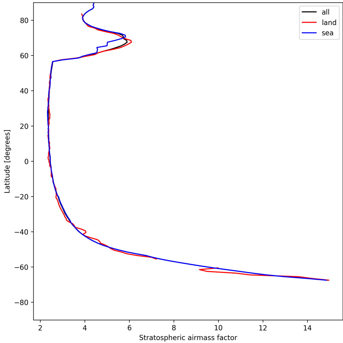
Figure 25: Zonal average of “Stratospheric airmass factor” for 2025-07-23 to 2025-07-24.
