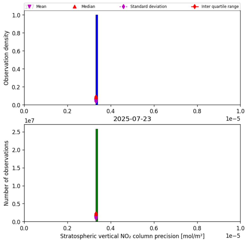
Figure 35: Histogram of “Stratospheric vertical NO 2 column precision” for 2025-07-23 to 2025-07-24
