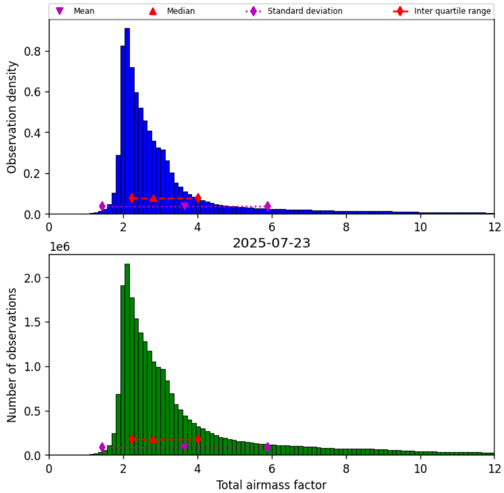
Figure 30: Histogram of “Total airmass factor” for 2025-07-23 to 2025-07-24
