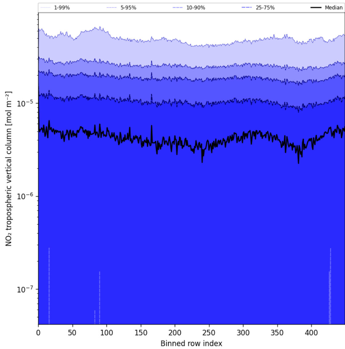
Figure 44: Along track statistics of “NO 2 tropospheric vertical column” for 2025-07-23 to 2025-07-24
