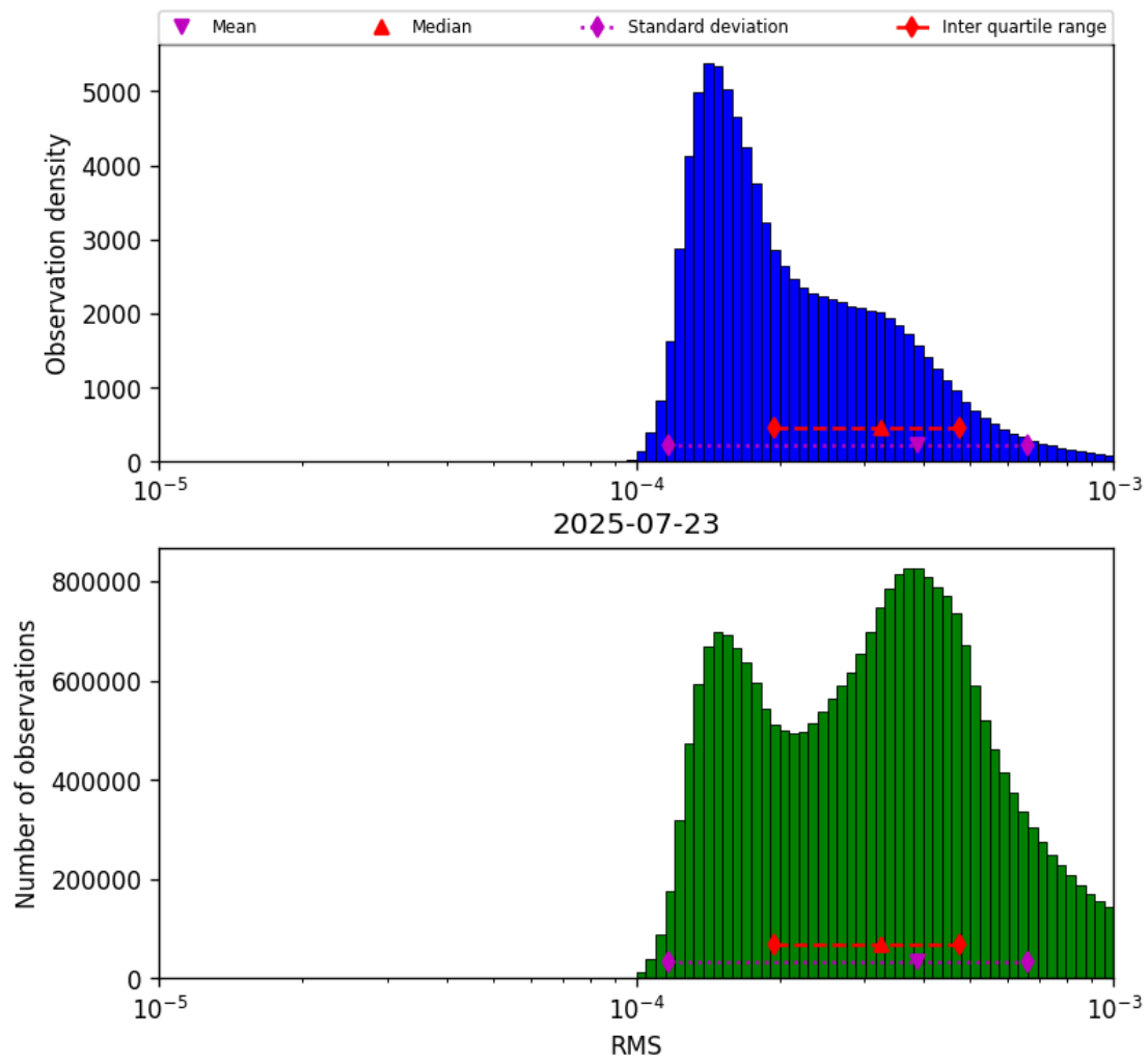
Figure 41: Histogram of “RMS” for 2025-07-23 to 2025-07-24
