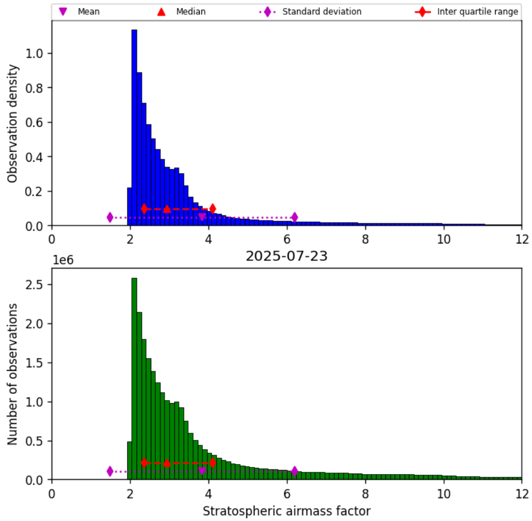
Figure 42: Histogram of “Stratospheric airmass factor” for 2025-07-23 to 2025-07-24
