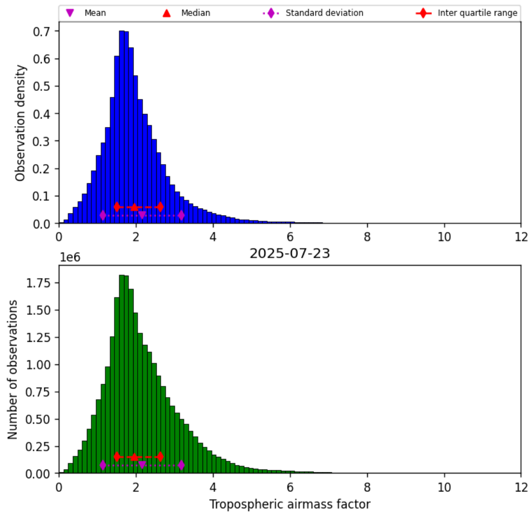
Figure 29: Histogram of “Tropospheric airmass factor” for 2025-07-23 to 2025-07-24
