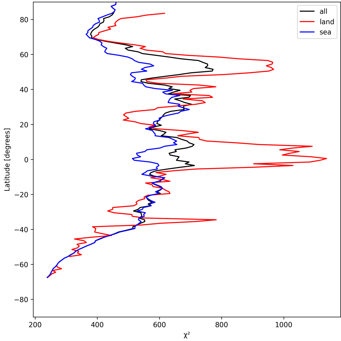
Figure 23: Zonal average of “ \chi^2 ” for 2025-07-23 to 2025-07-24.
