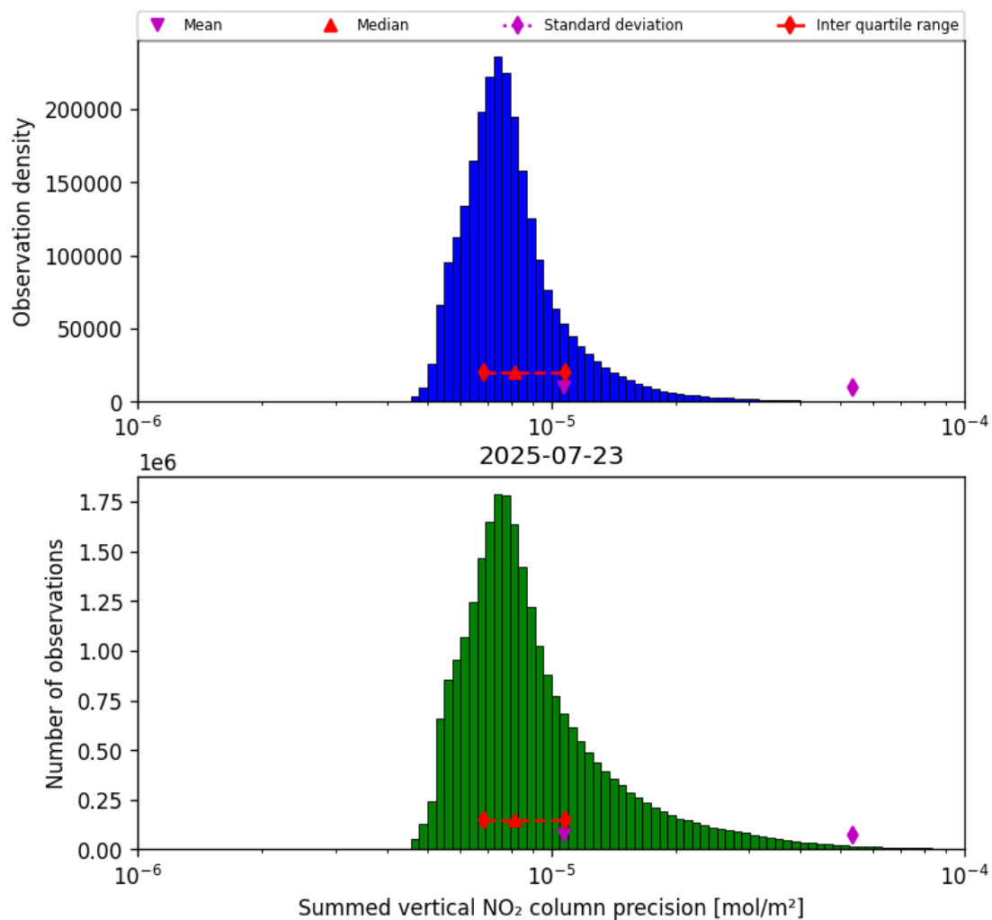
Figure 39: Histogram of “Summed vertical NO 2 column precision” for 2025-07-23 to 2025-07-24
