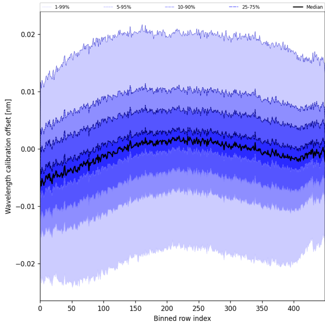
Figure 50: Along track statistics of “Wavelength calibration offset” for 2025-07-23 to 2025-07-24
