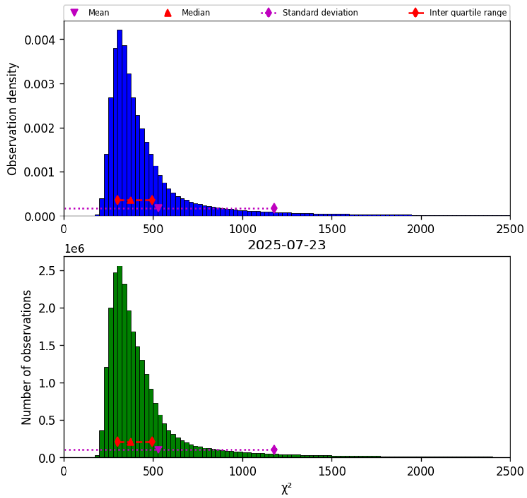
Figure 40: Histogram of “ \chi^2 ” for 2025-07-23 to 2025-07-24
