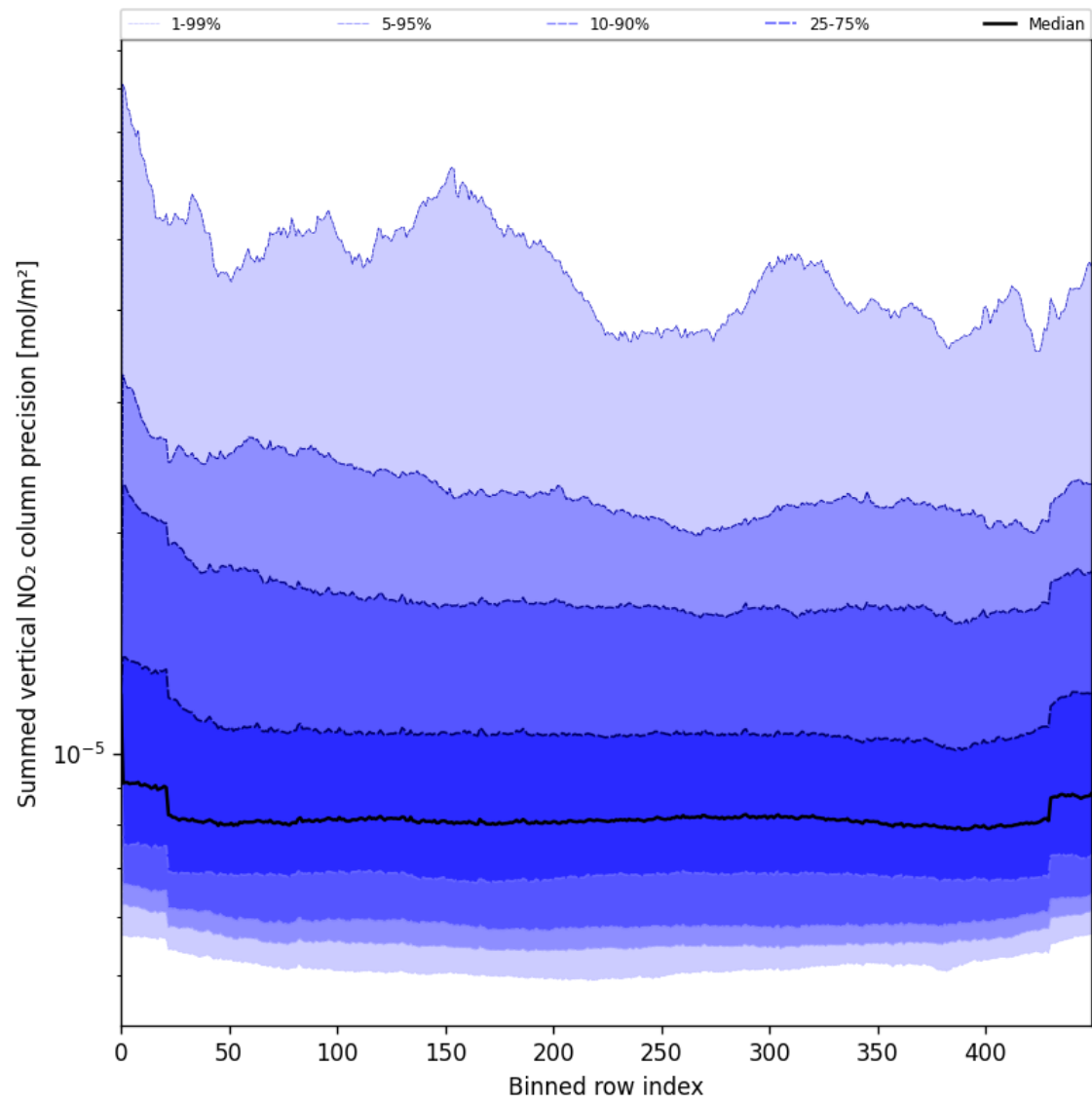
Figure 56: Along track statistics of “Summed vertical NO 2 column precision” for 2025-07-23 to 2025-07-24
