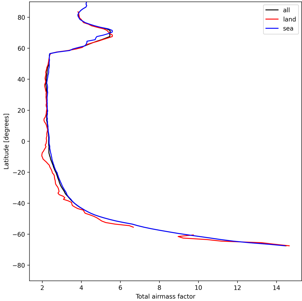
Figure 13: Zonal average of “Total airmass factor” for 2025-07-23 to 2025-07-24.
