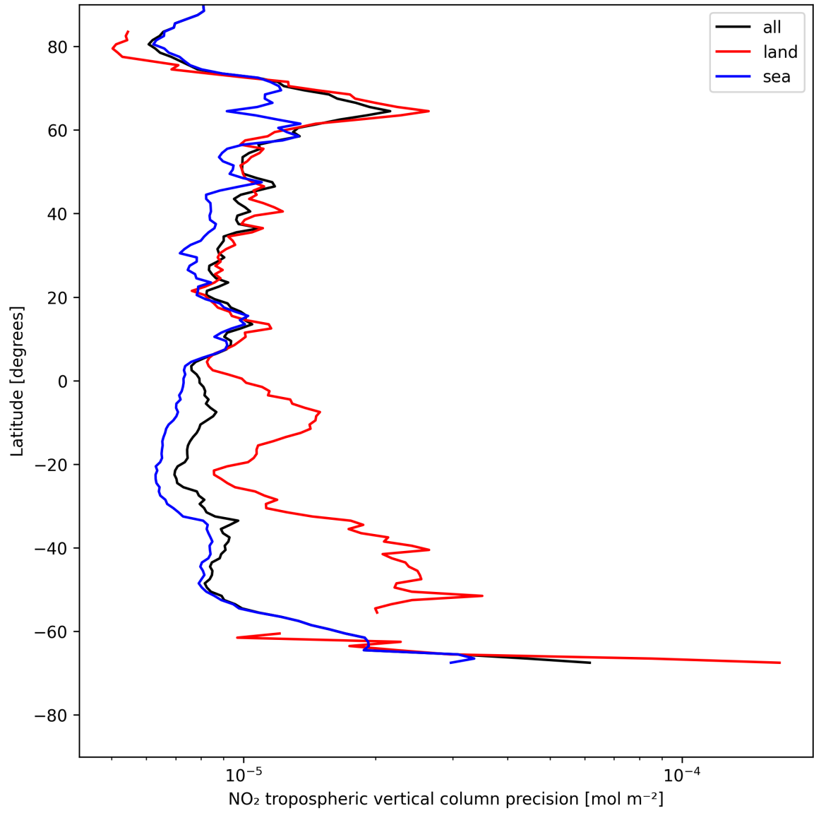
Figure 11: Zonal average of “NO 2 tropospheric vertical column precision” for 2025-07-23 to 2025-07-24.
