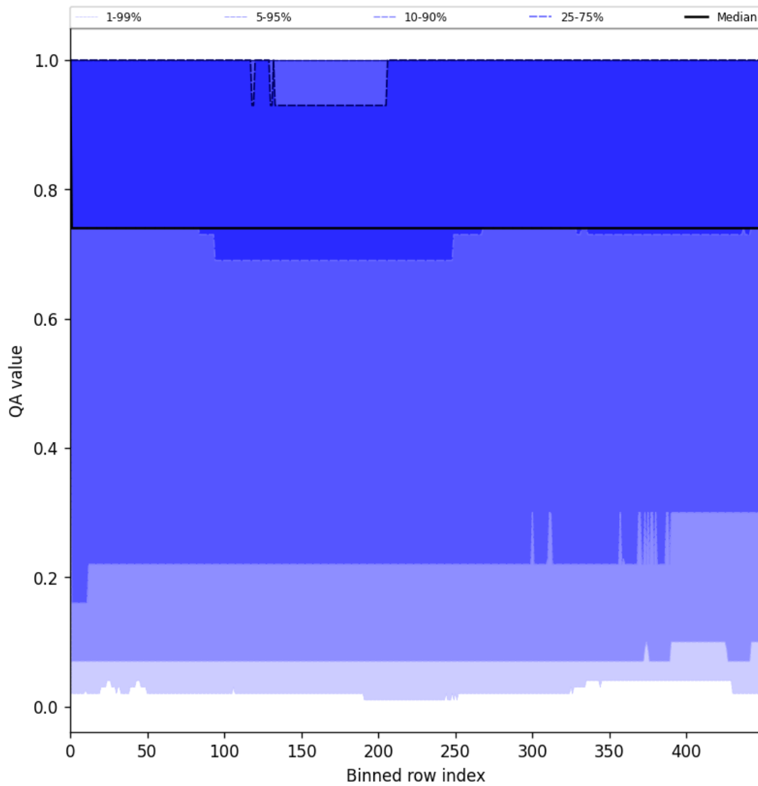
Figure 43: Along track statistics of “QA value” for 2025-07-23 to 2025-07-24
