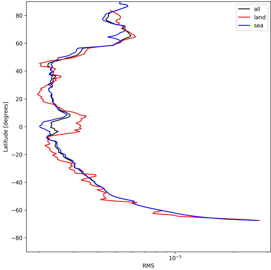
Figure 24: Zonal average of “RMS” for 2025-07-23 to 2025-07-24.
