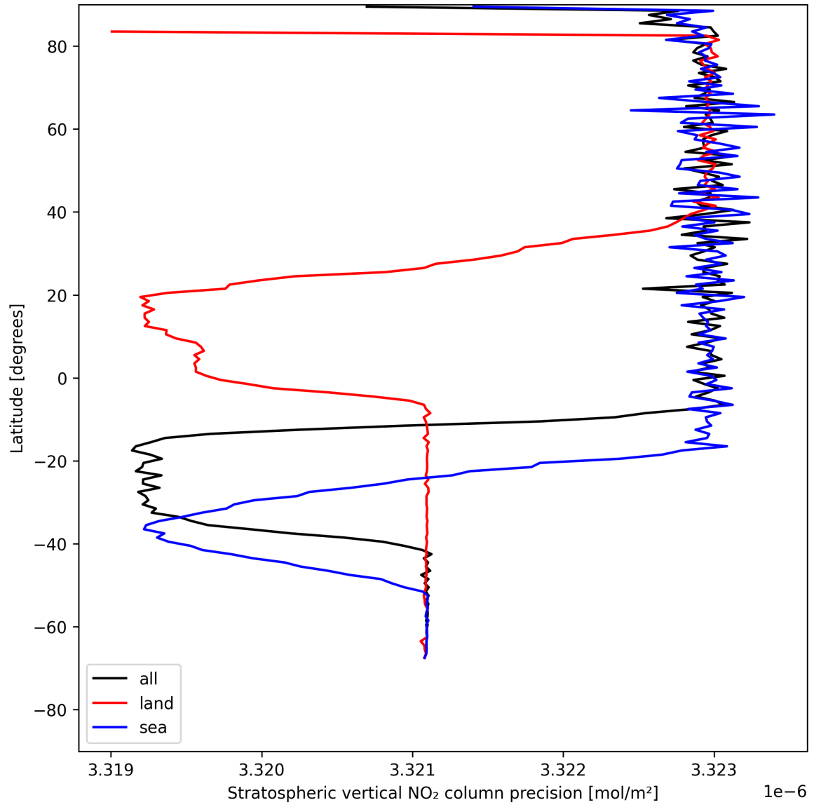
Figure 18: Zonal average of “Stratospheric vertical NO 2 column precision” for 2025-07-23 to 2025-07-24.
