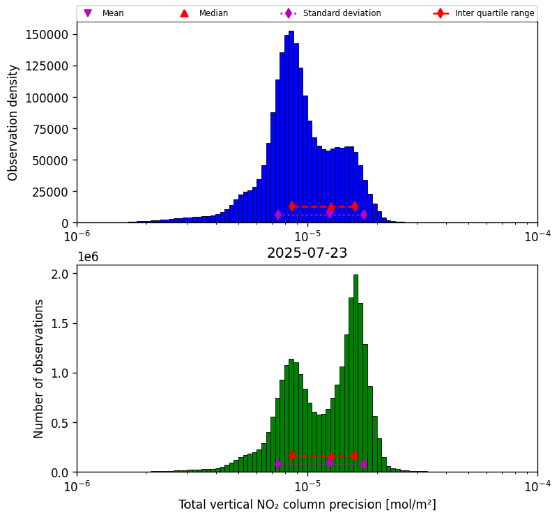
Figure 37: Histogram of “Total vertical NO 2 column precision” for 2025-07-23 to 2025-07-24
