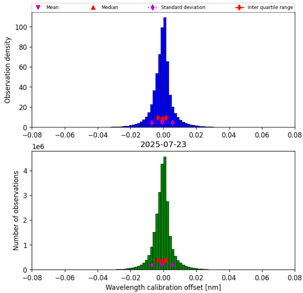
Figure 33: Histogram of “Wavelength calibration offset” for 2025-07-23 to 2025-07-24
