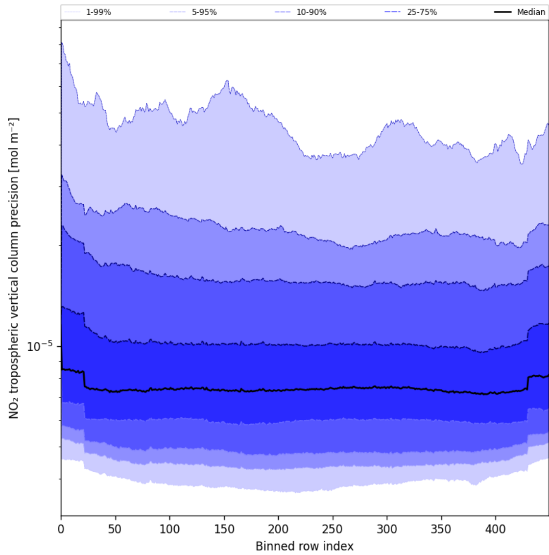
Figure 45: Along track statistics of “NO 2 tropospheric vertical column precision” for 2025-07-23 to 2025-07-24
