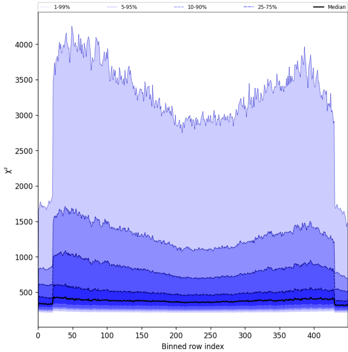
Figure 57: Along track statistics of “ \chi^2 ” for 2025-07-23 to 2025-07-24
