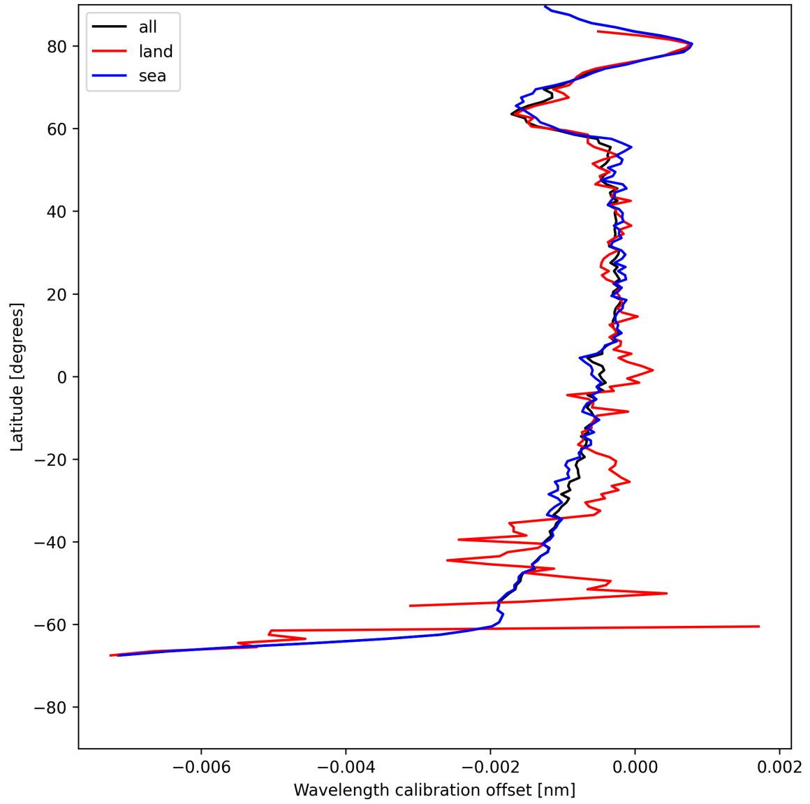
Figure 16: Zonal average of “Wavelength calibration offset” for 2025-07-23 to 2025-07-24.
