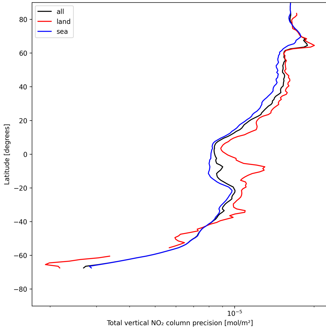
Figure 20: Zonal average of “Total vertical NO 2 column precision” for 2025-07-23 to 2025-07-24.
