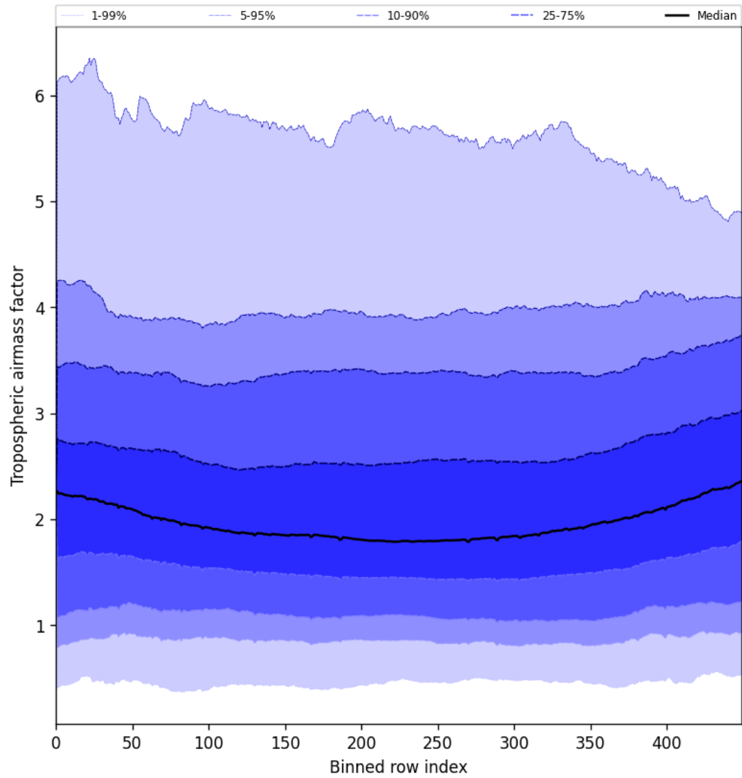
Figure 46: Along track statistics of “Tropospheric airmass factor” for 2025-07-23 to 2025-07-24
