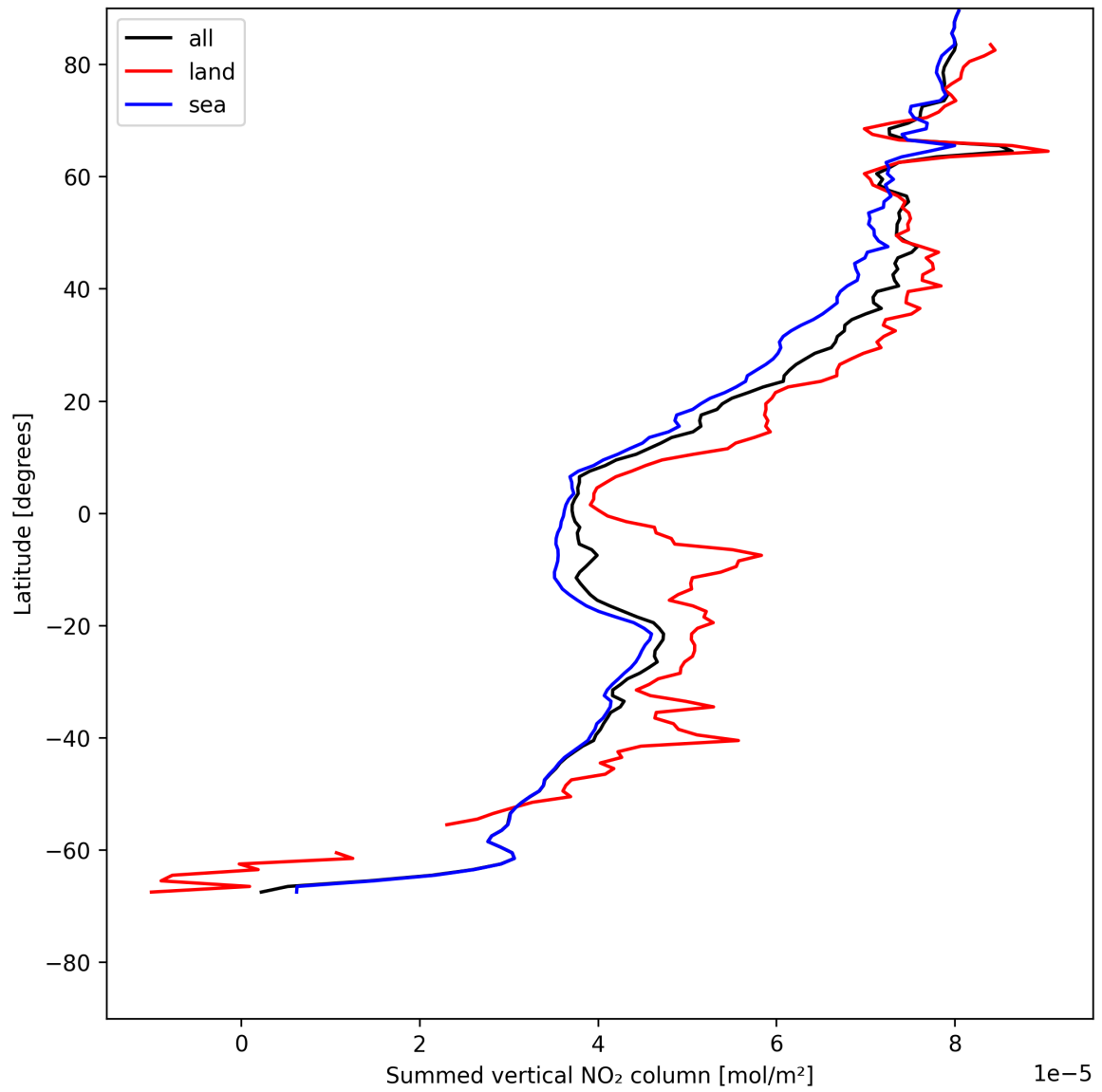
Figure 21: Zonal average of “Summed vertical NO 2 column” for 2025-07-23 to 2025-07-24.
