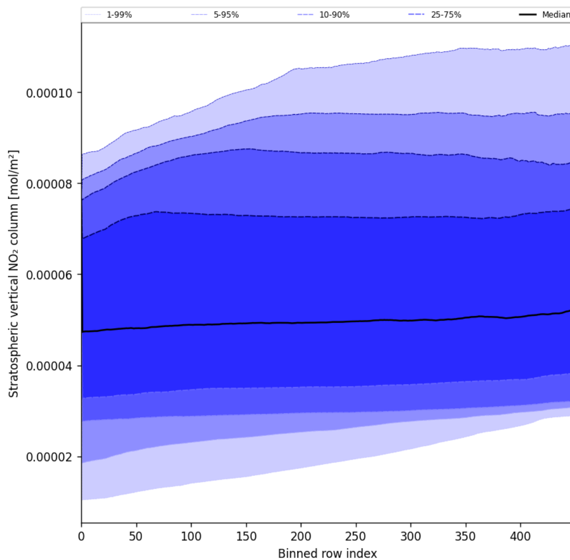
Figure 51: Along track statistics of “Stratospheric vertical NO 2 column” for 2025-07-23 to 2025-07-24
