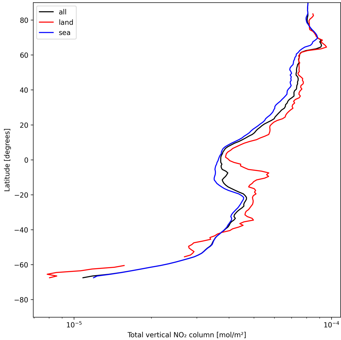
Figure 19: Zonal average of “Total vertical NO 2 column” for 2025-07-23 to 2025-07-24.
