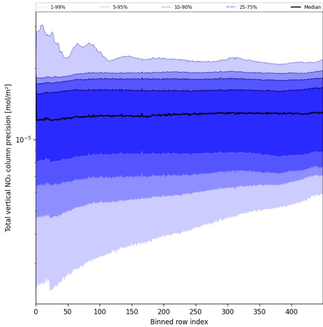
Figure 54: Along track statistics of “Total vertical NO 2 column precision” for 2025-07-23 to 2025-07-24
