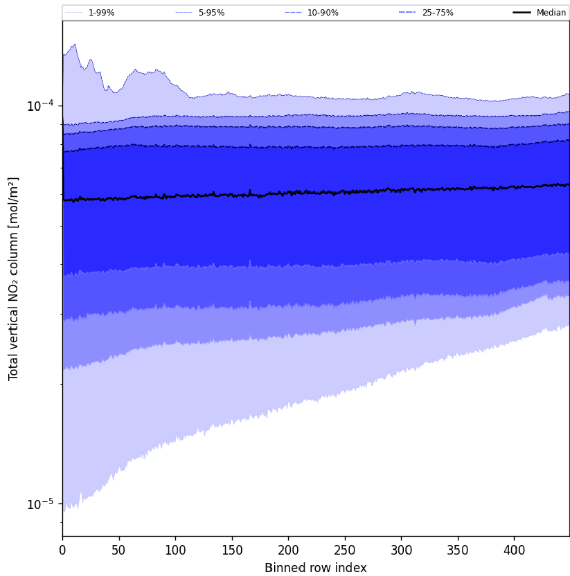
Figure 53: Along track statistics of “Total vertical NO 2 column” for 2025-07-23 to 2025-07-24
