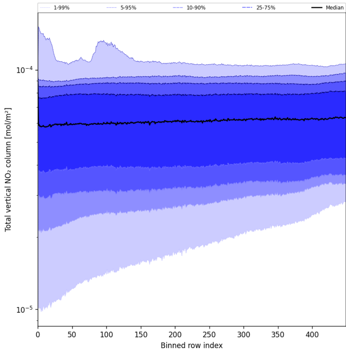
Figure 53: Along track statistics of “Total vertical NO 2 column” for 2025-07-24 to 2025-07-25
