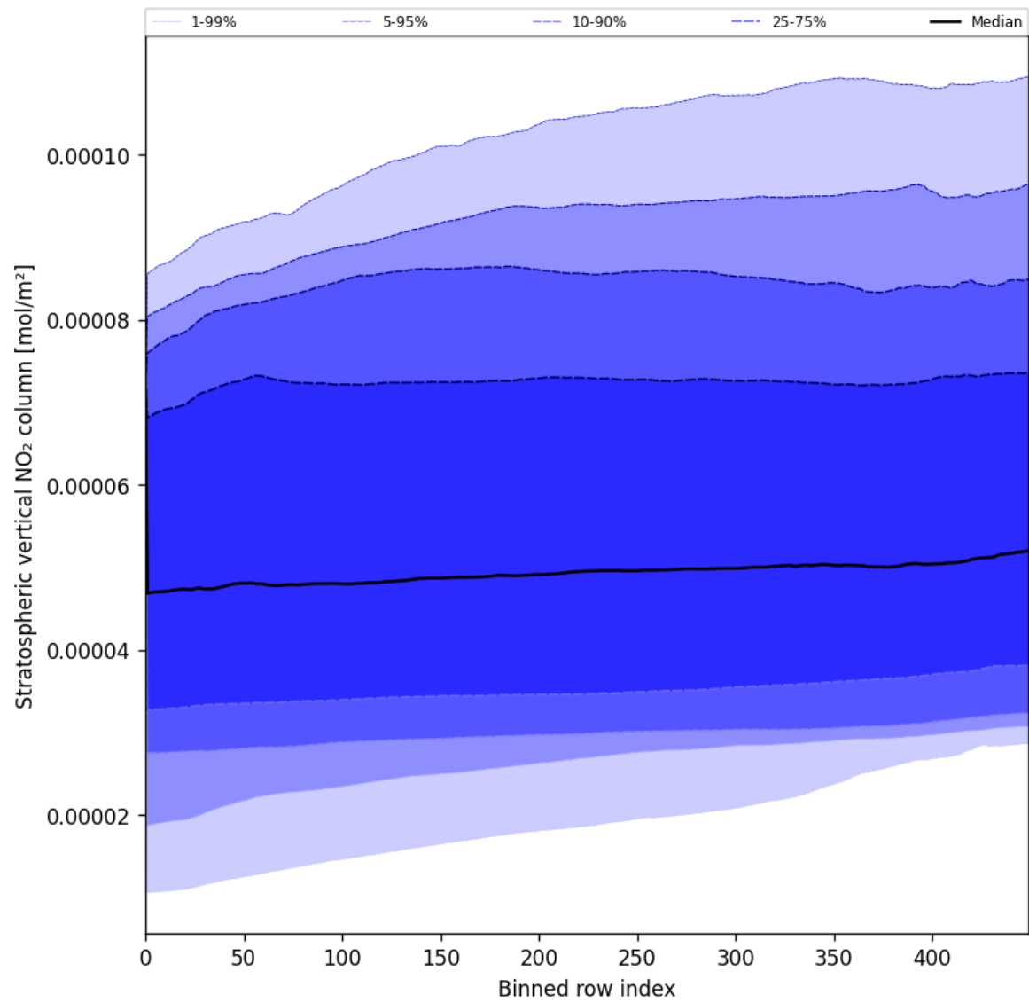
Figure 51: Along track statistics of “Stratospheric vertical NO 2 column” for 2025-07-24 to 2025-07-25
