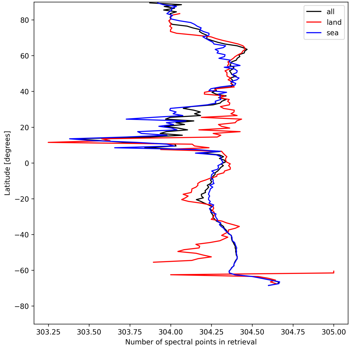
Figure 14: Zonal average of “Number of spectral points in retrieval” for 2025-07-24 to 2025-07-25.
