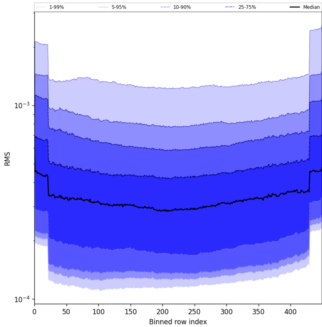
Figure 58: Along track statistics of “RMS” for 2025-07-24 to 2025-07-25
