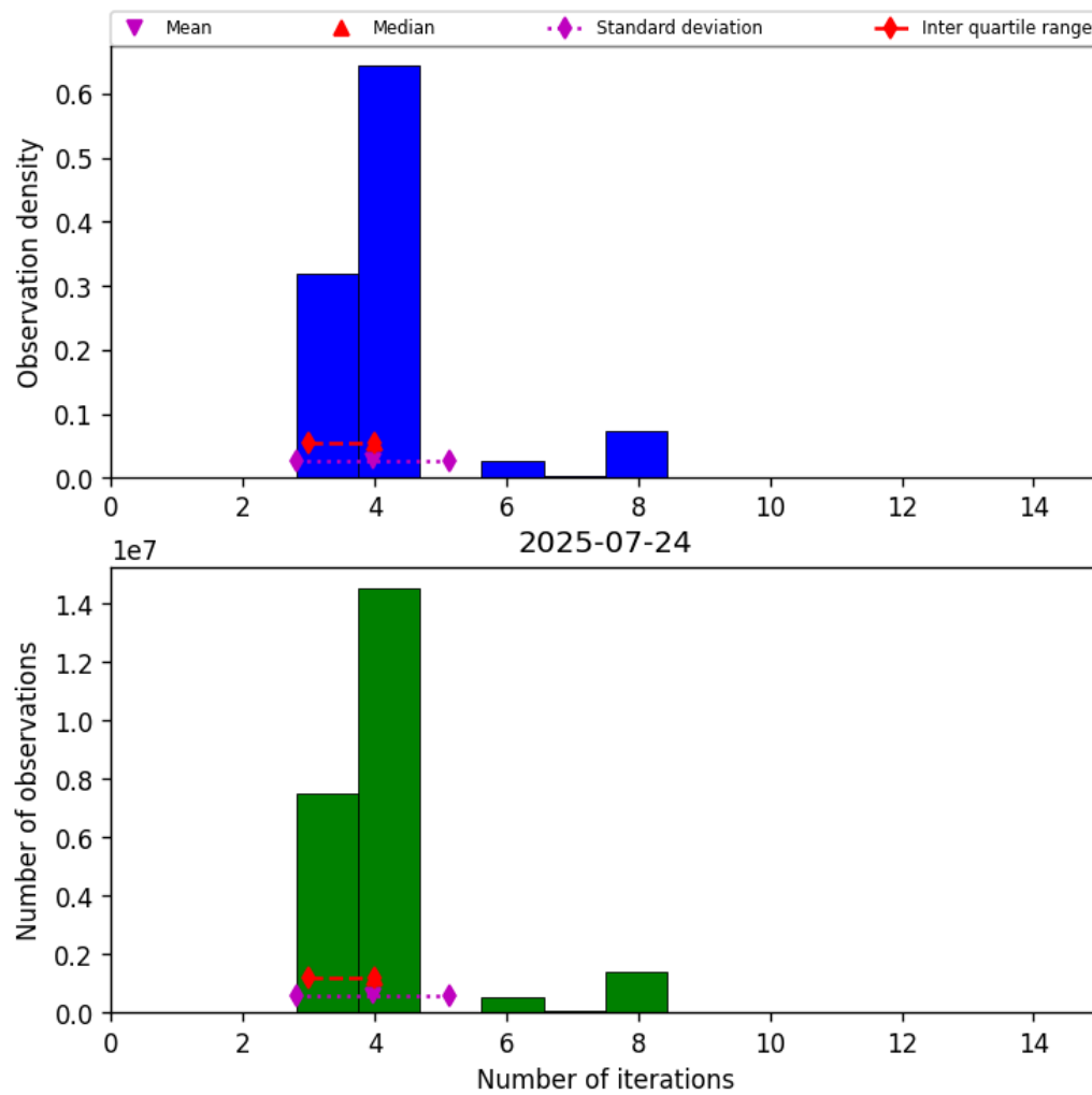
Figure 32: Histogram of “Number of iterations” for 2025-07-24 to 2025-07-25
