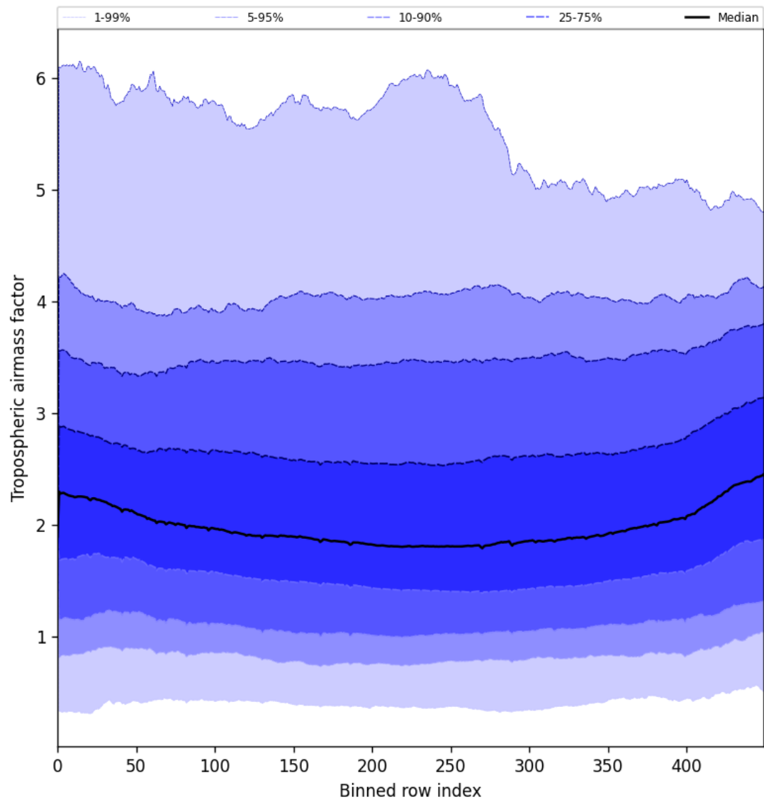
Figure 46: Along track statistics of “Tropospheric airmass factor” for 2025-07-24 to 2025-07-25
