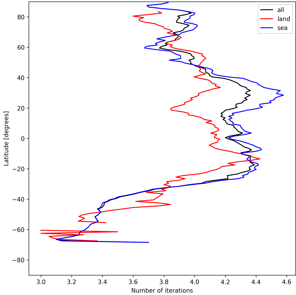
Figure 15: Zonal average of “Number of iterations” for 2025-07-24 to 2025-07-25.
