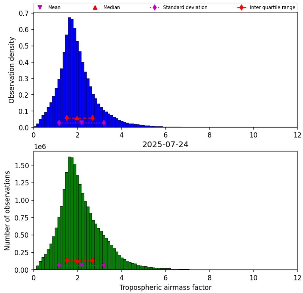
Figure 29: Histogram of “Tropospheric airmass factor” for 2025-07-24 to 2025-07-25
