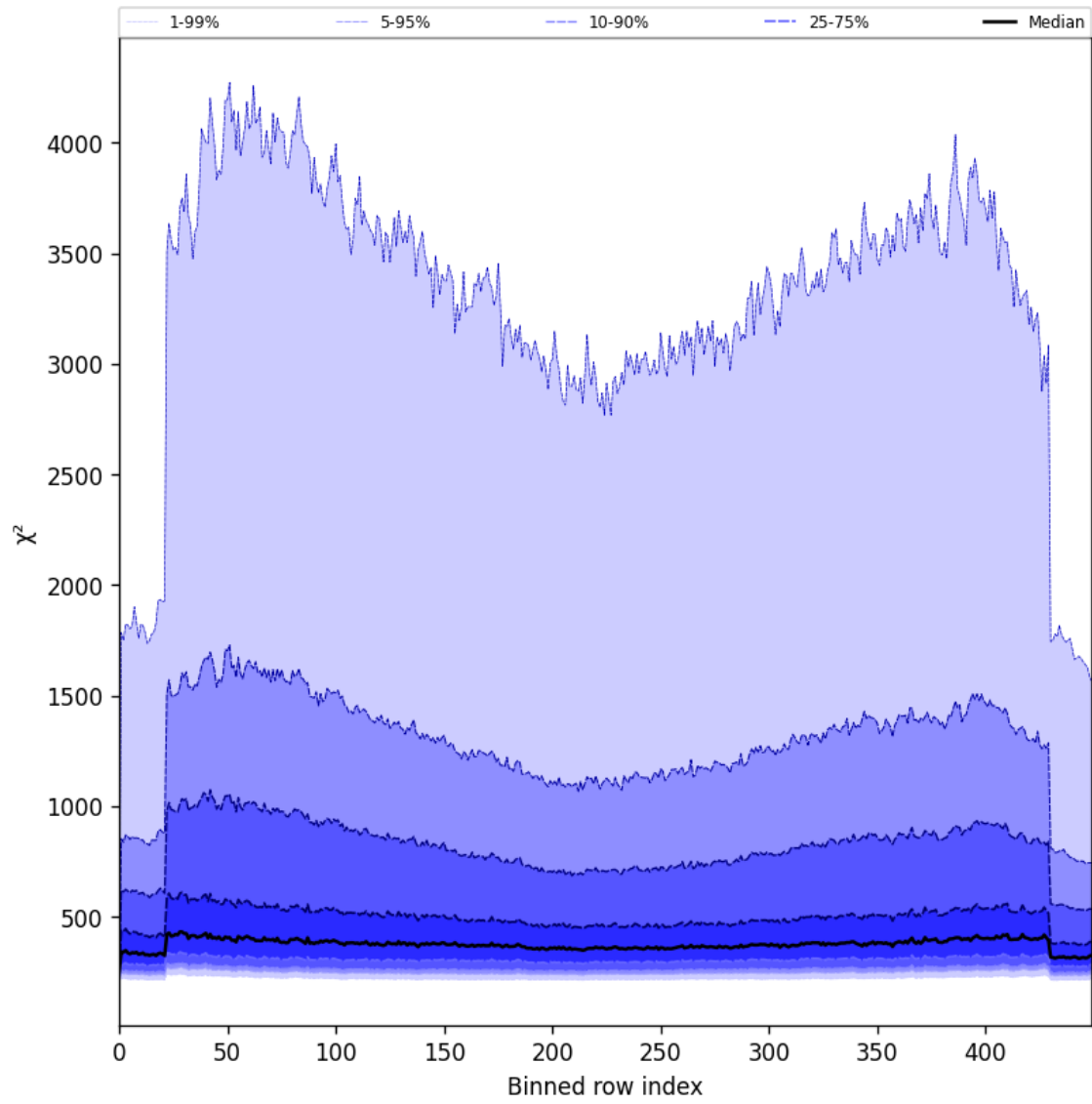
Figure 57: Along track statistics of “ \chi^2 ” for 2025-07-24 to 2025-07-25
