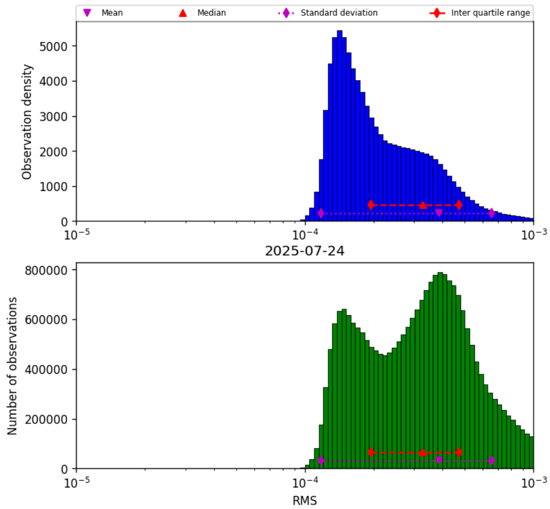
Figure 41: Histogram of “RMS” for 2025-07-24 to 2025-07-25
