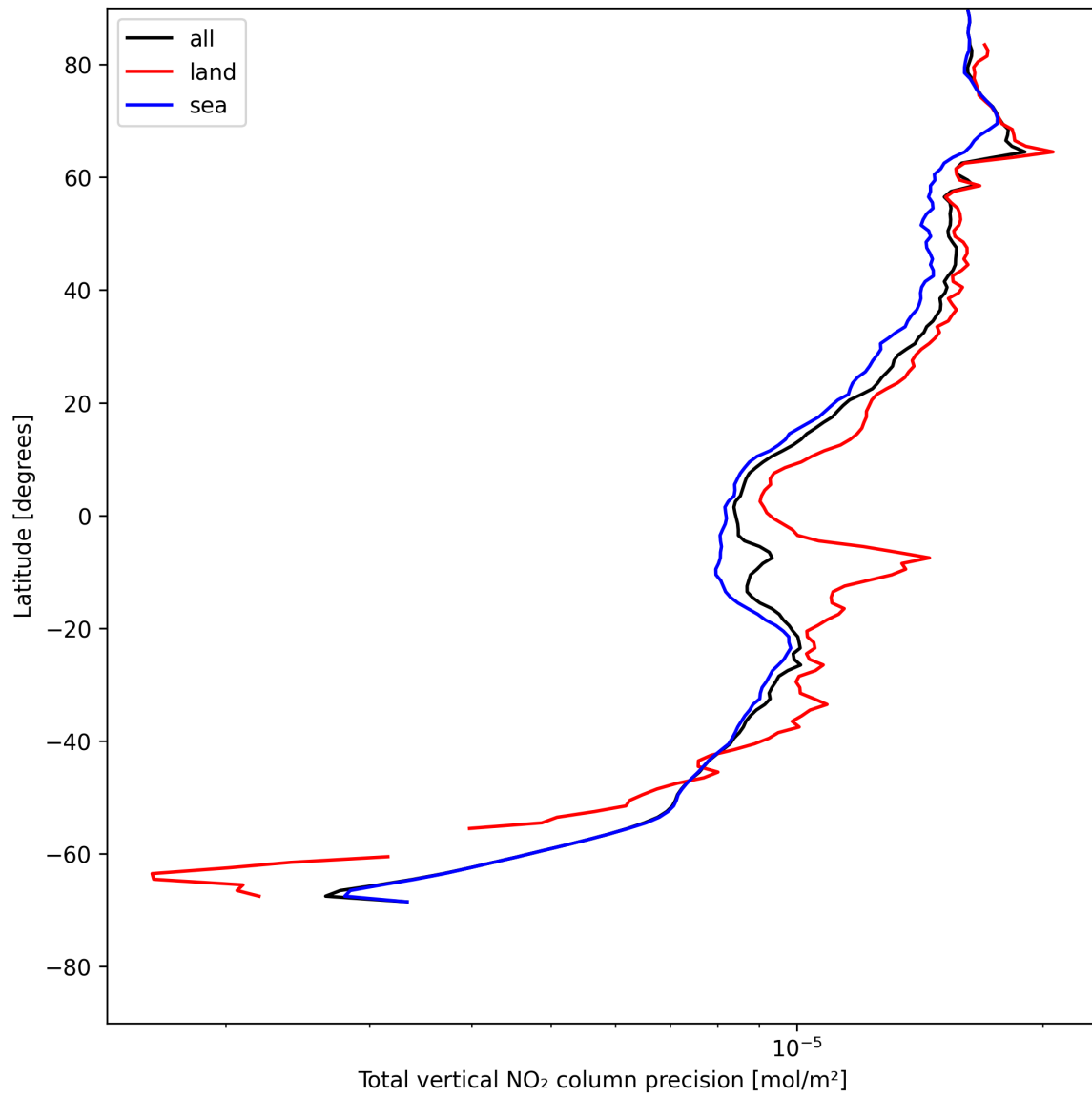
Figure 20: Zonal average of “Total vertical NO 2 column precision” for 2025-07-24 to 2025-07-25.
