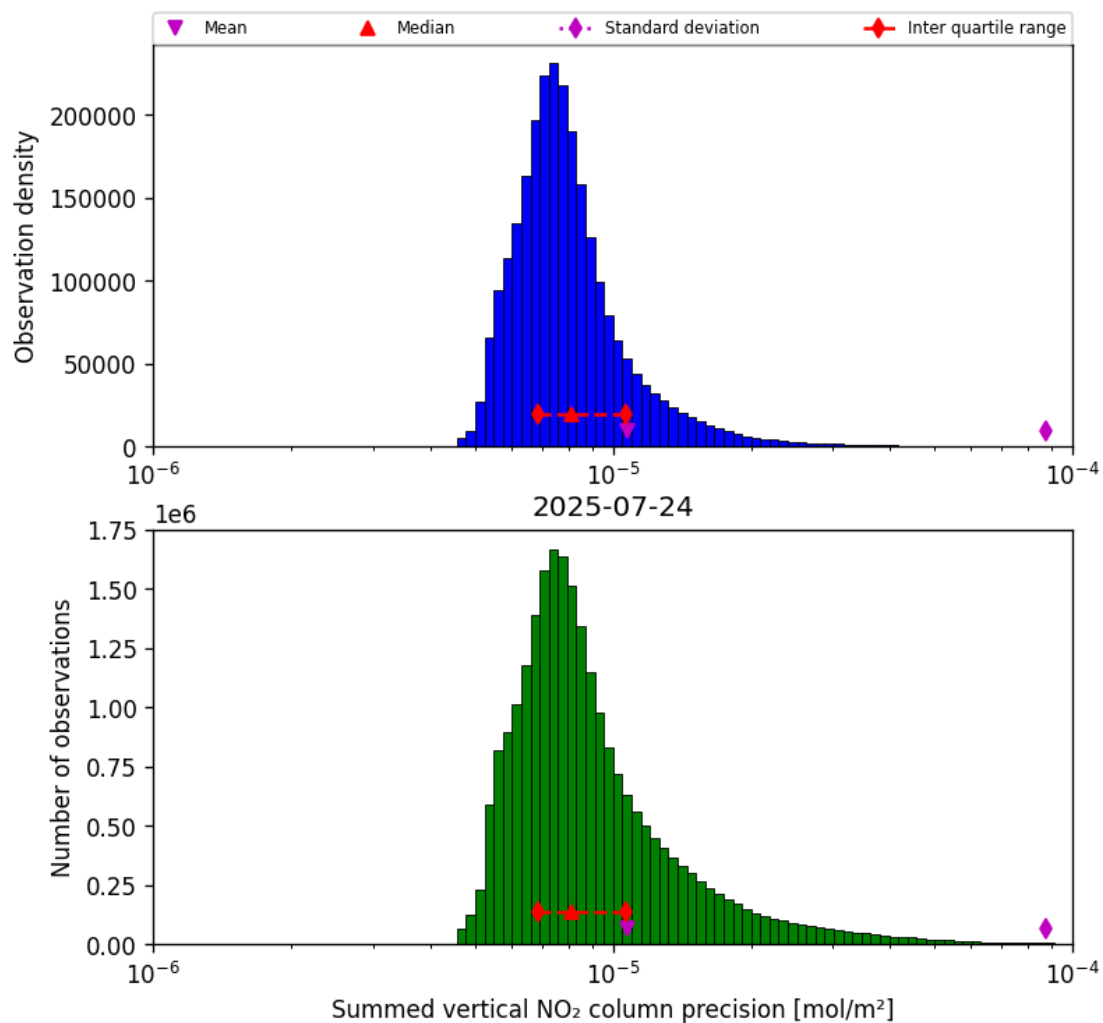
Figure 39: Histogram of “Summed vertical NO 2 column precision” for 2025-07-24 to 2025-07-25
