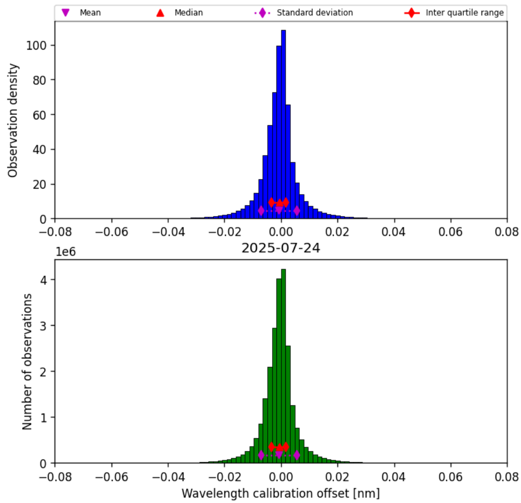
Figure 33: Histogram of “Wavelength calibration offset” for 2025-07-24 to 2025-07-25
