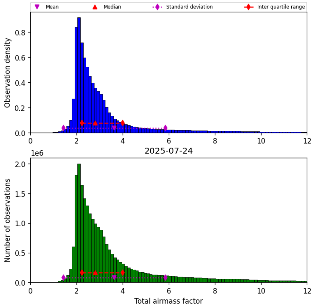
Figure 30: Histogram of “Total airmass factor” for 2025-07-24 to 2025-07-25
