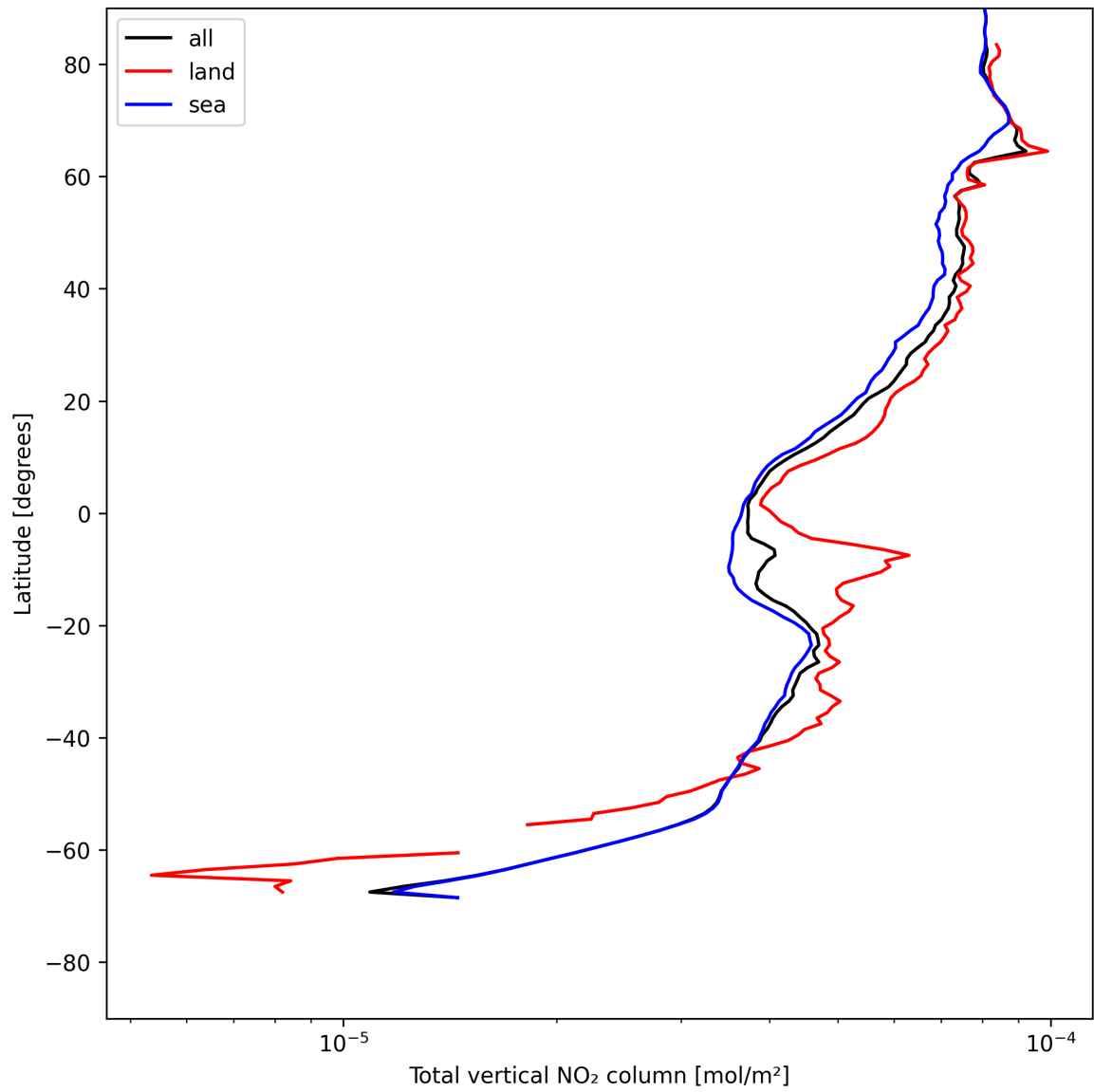
Figure 19: Zonal average of “Total vertical NO 2 column” for 2025-07-24 to 2025-07-25.
