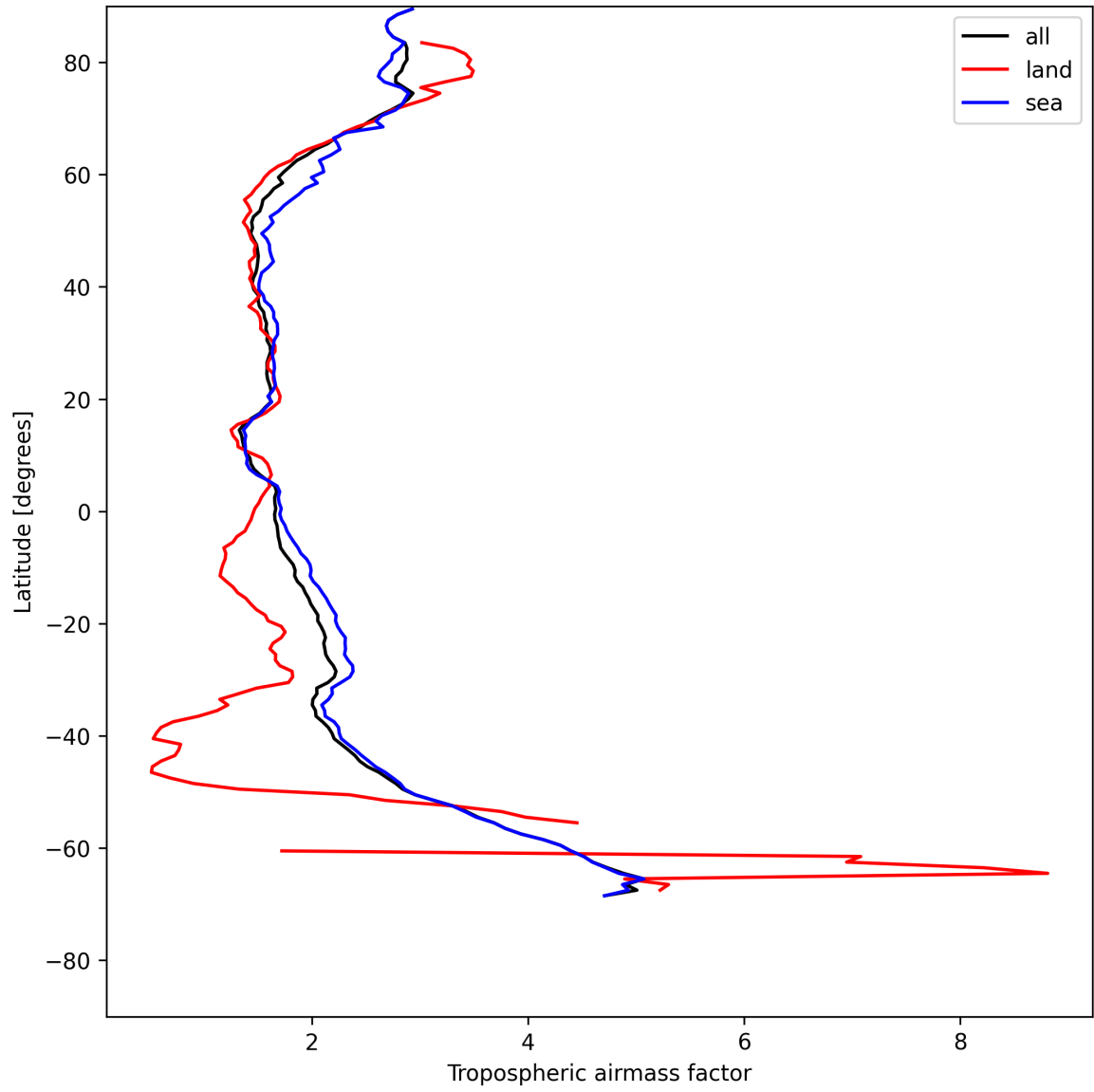
Figure 12: Zonal average of “Tropospheric air mass factor” for 2025-07-24 to 2025-07-25.
