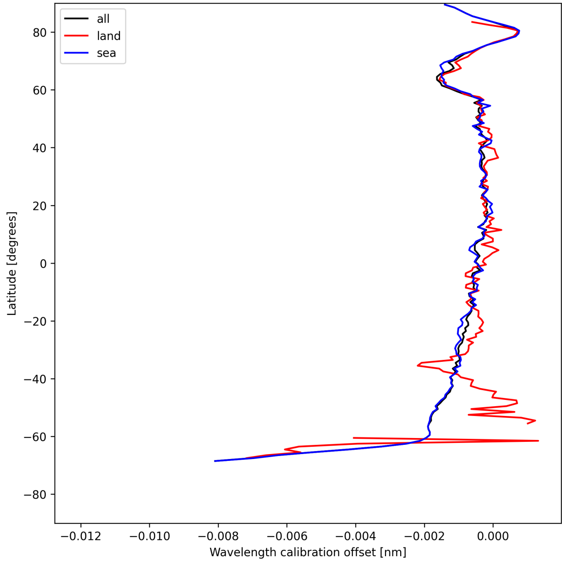
Figure 16: Zonal average of “Wavelength calibration offset” for 2025-07-24 to 2025-07-25.
