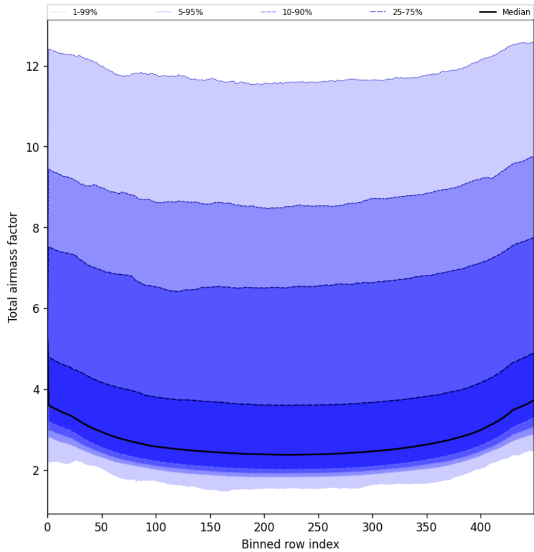
Figure 47: Along track statistics of “Total airmass factor” for 2025-07-24 to 2025-07-25
