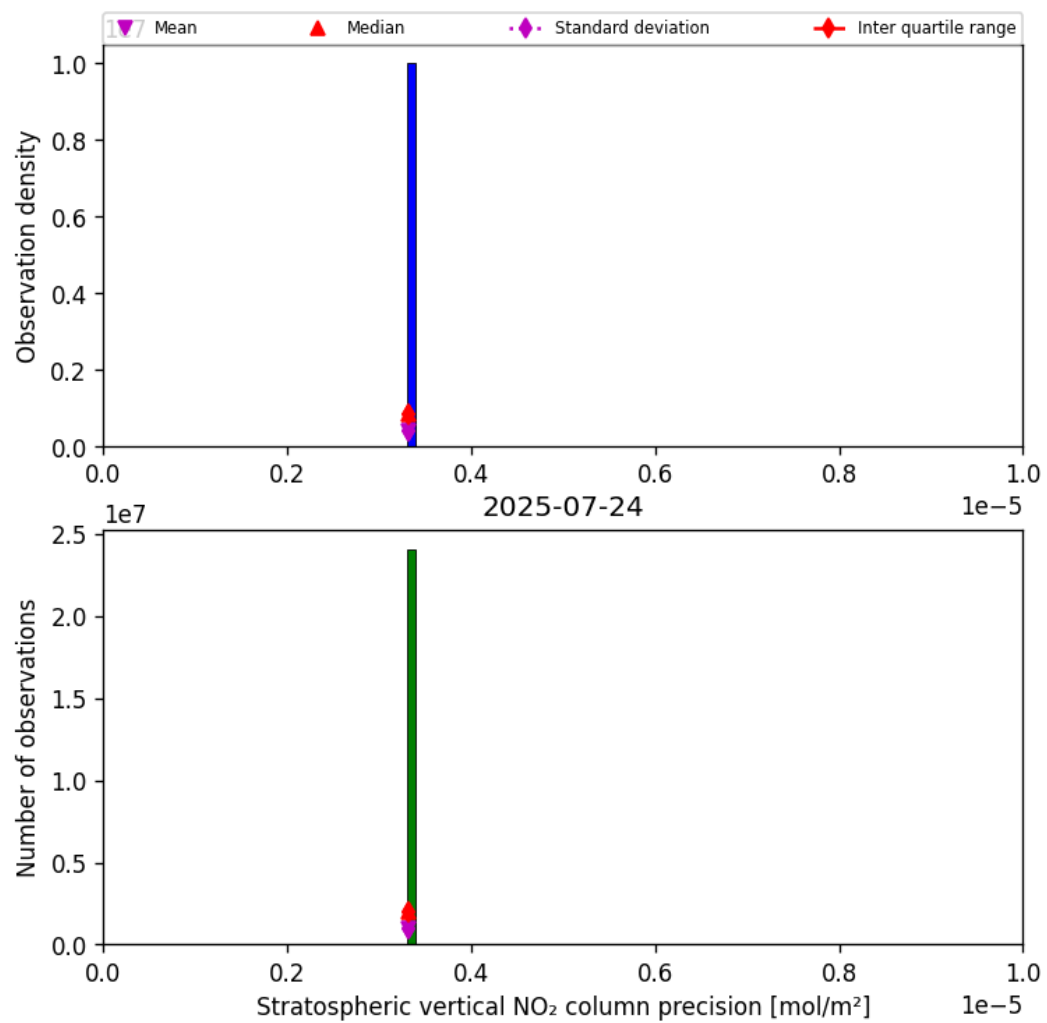
Figure 35: Histogram of “Stratospheric vertical NO 2 column precision” for 2025-07-24 to 2025-07-25
