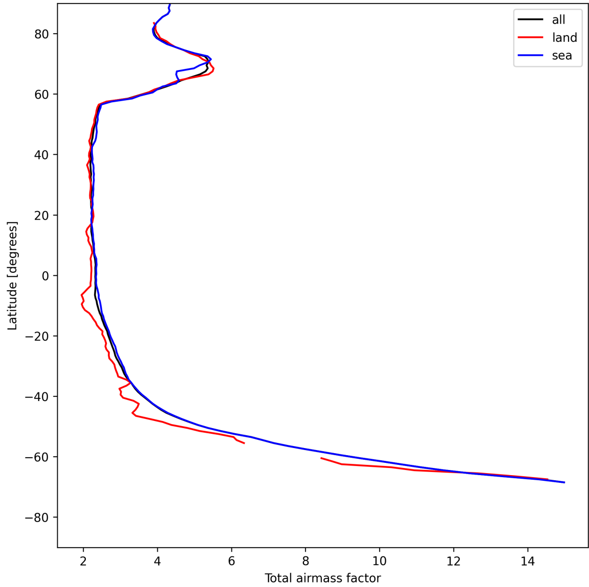
Figure 13: Zonal average of “Total airmass factor” for 2025-07-24 to 2025-07-25.
