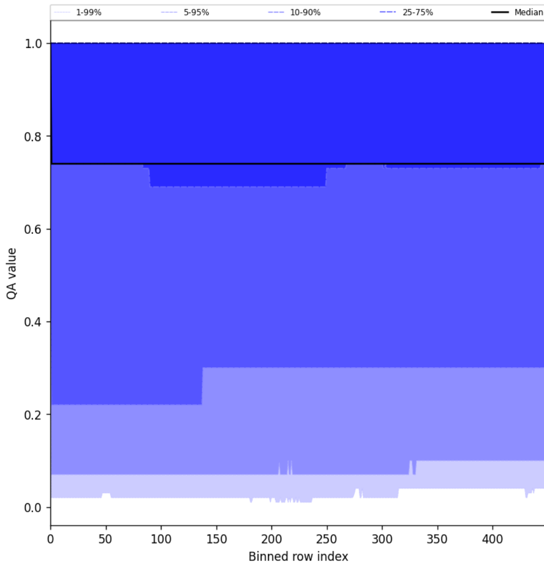
Figure 43: Along track statistics of “QA value” for 2025-07-24 to 2025-07-25
