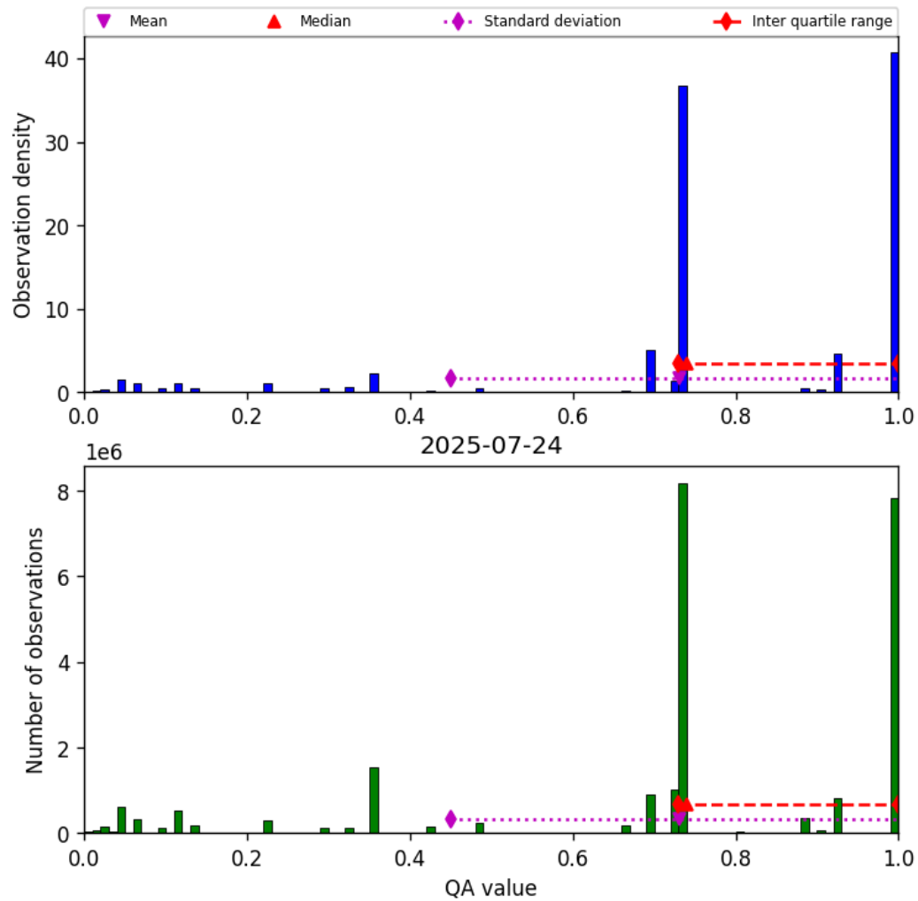
Figure 26: Histogram of “QA value” for 2025-07-24 to 2025-07-25
