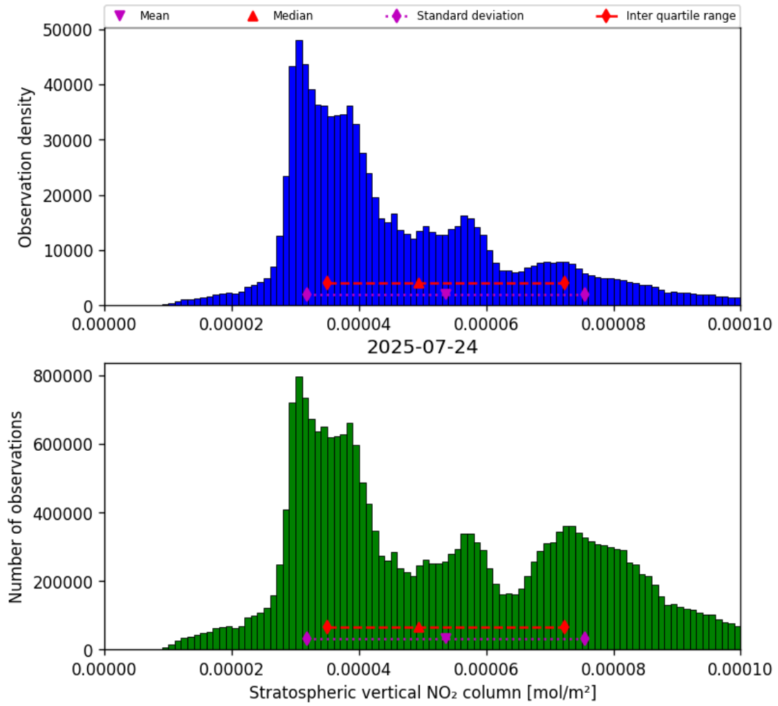
Figure 34: Histogram of “Stratospheric vertical NO 2 column” for 2025-07-24 to 2025-07-25
