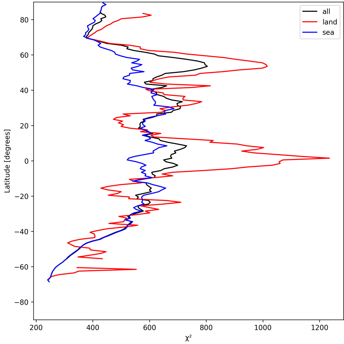
Figure 23: Zonal average of “ \chi^2 ” for 2025-07-24 to 2025-07-25.
