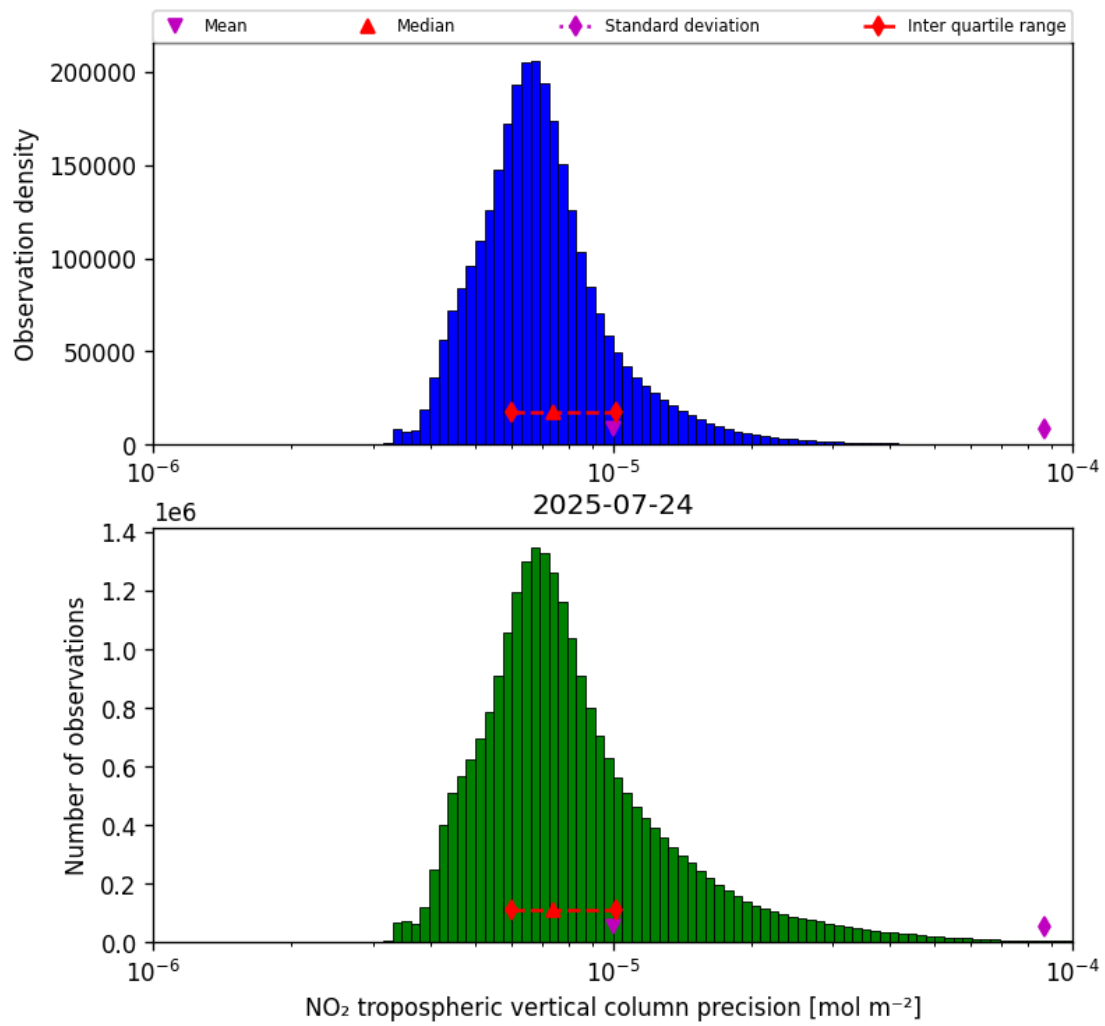
Figure 28: Histogram of “NO 2 tropospheric vertical column precision” for 2025-07-24 to 2025-07-25
