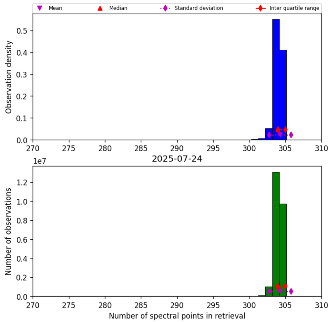
Figure 31: Histogram of “Number of spectral points in retrieval” for 2025-07-24 to 2025-07-25
