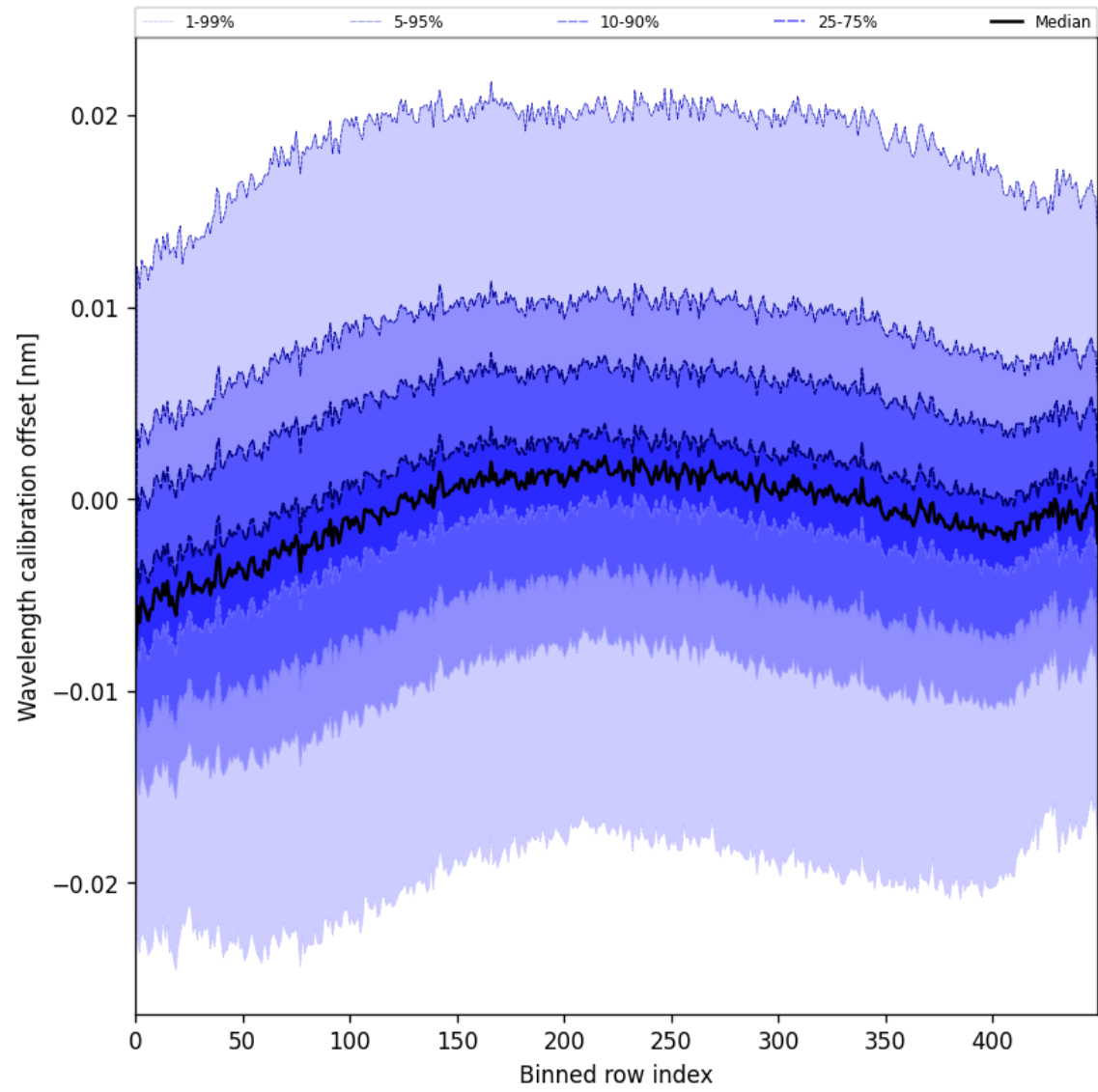
Figure 50: Along track statistics of “Wavelength calibration offset” for 2025-07-24 to 2025-07-25
