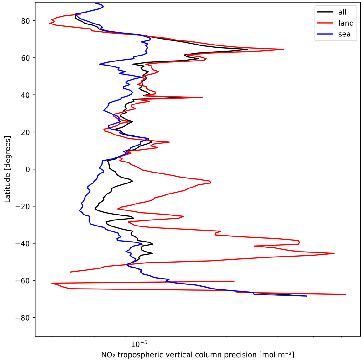
Figure 11: Zonal average of “NO 2 tropospheric vertical column precision” for 2025-07-24 to 2025-07-25.
