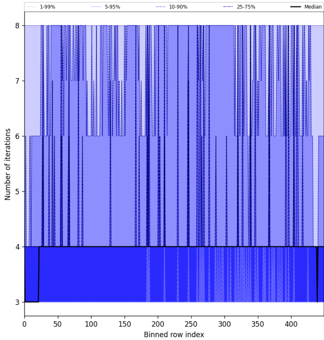
Figure 49: Along track statistics of “Number of iterations” for 2025-07-24 to 2025-07-25
