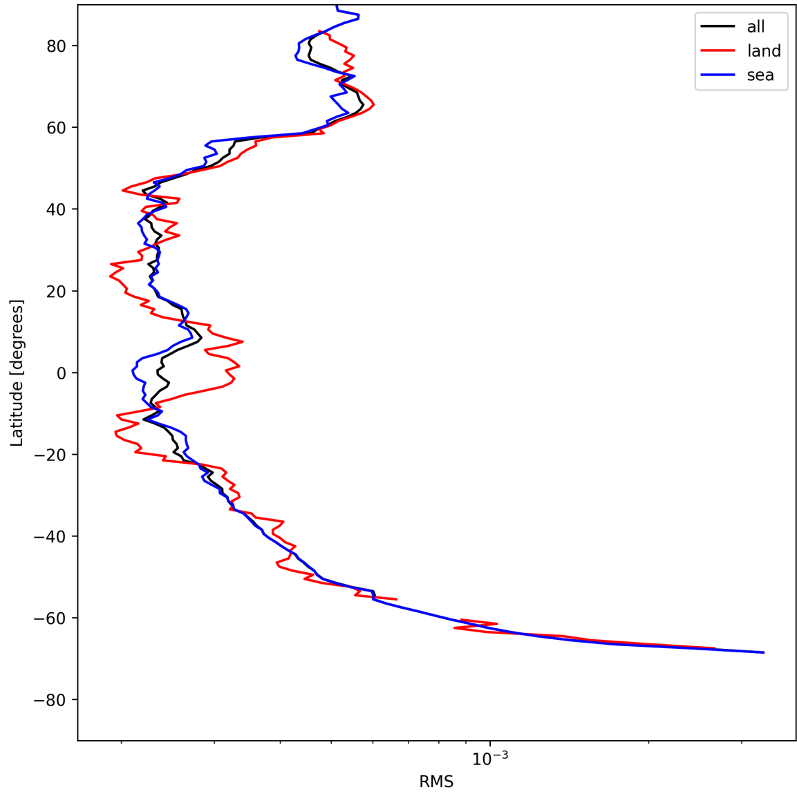
Figure 24: Zonal average of “RMS” for 2025-07-24 to 2025-07-25.
