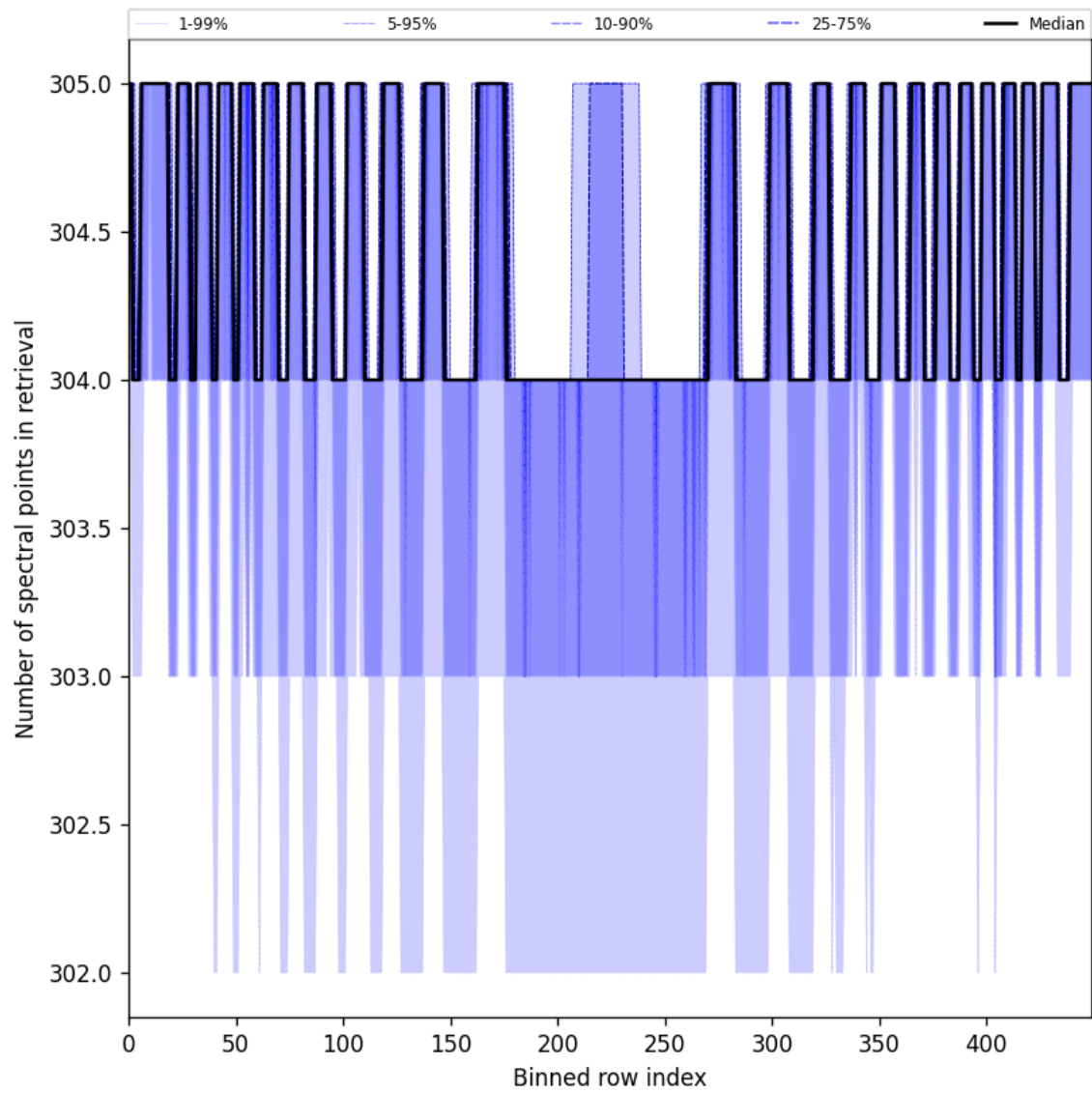
Figure 48: Along track statistics of “Number of spectral points in retrieval” for 2025-07-24 to 2025-07-25
