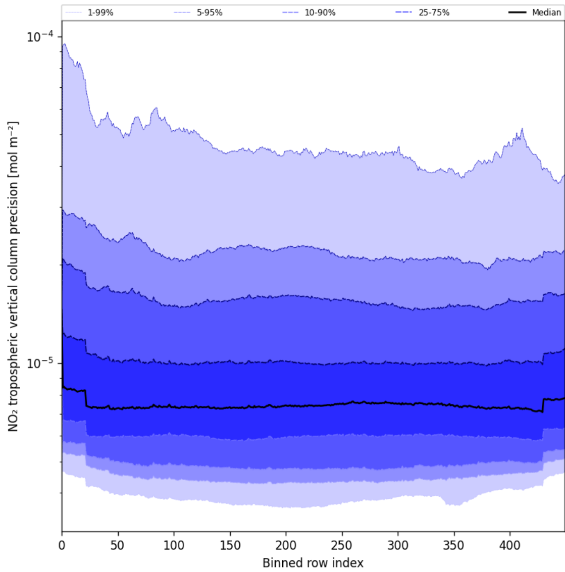
Figure 45: Along track statistics of “NO 2 tropospheric vertical column precision” for 2025-07-24 to 2025-07-25
