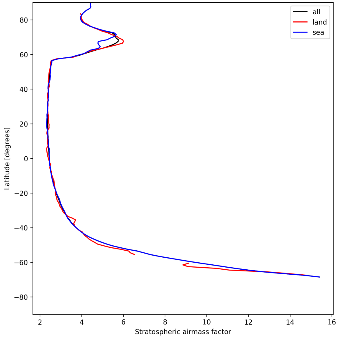
Figure 25: Zonal average of “Stratospheric airmass factor” for 2025-07-24 to 2025-07-25.
