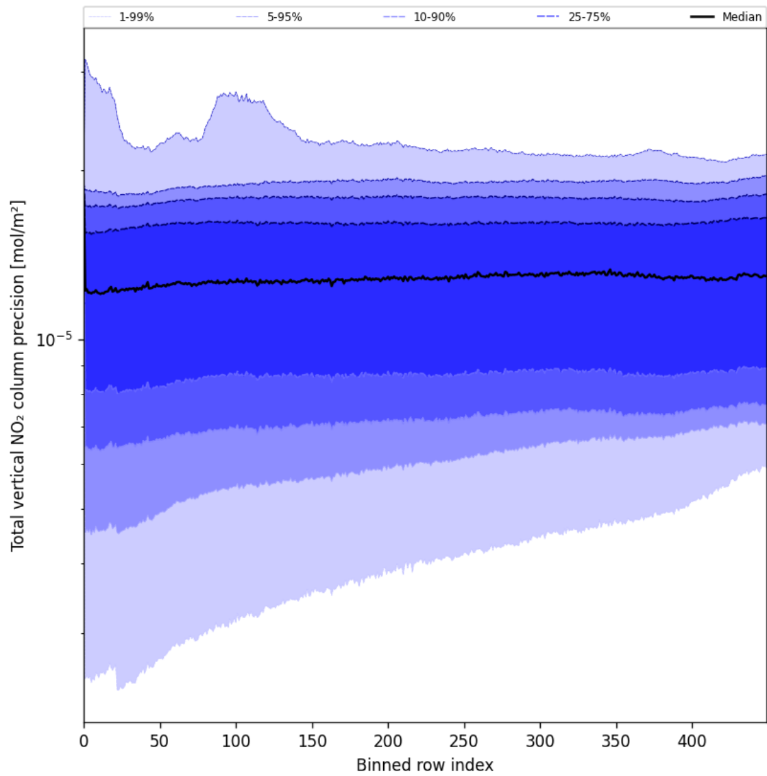
Figure 54: Along track statistics of “Total vertical NO 2 column precision” for 2025-07-24 to 2025-07-25
