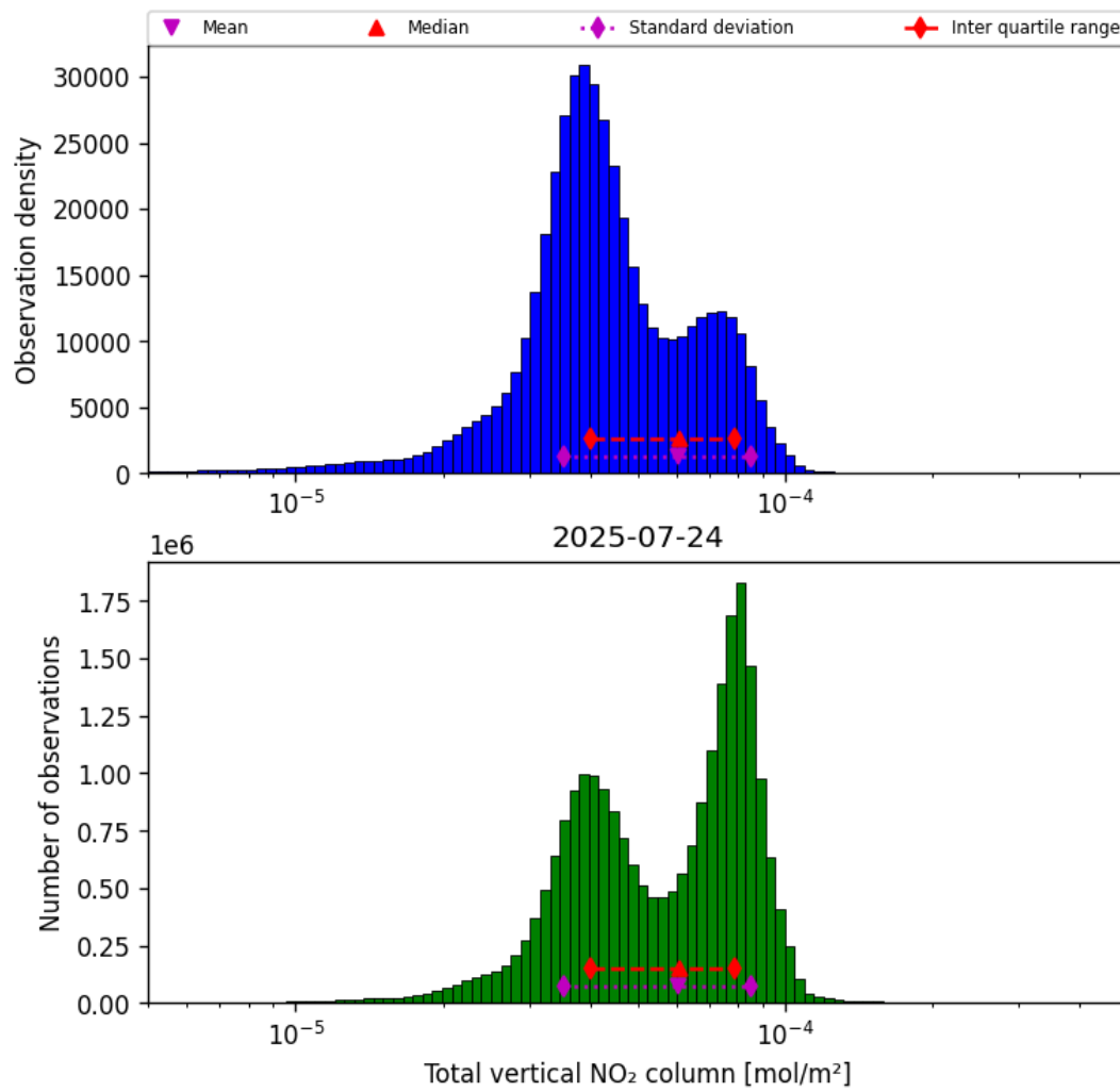
Figure 36: Histogram of “Total vertical NO 2 column” for 2025-07-24 to 2025-07-25
