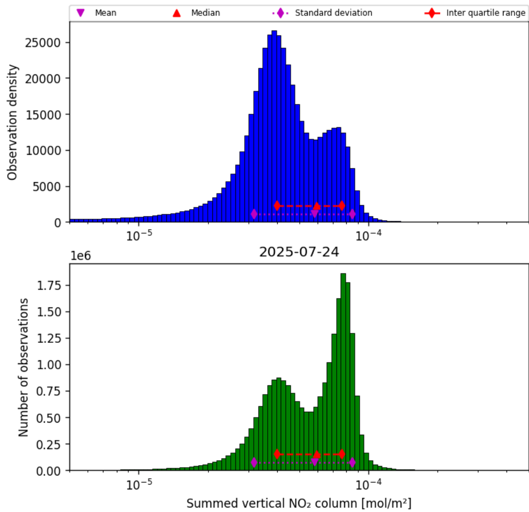
Figure 38: Histogram of “Summed vertical NO 2 column” for 2025-07-24 to 2025-07-25
