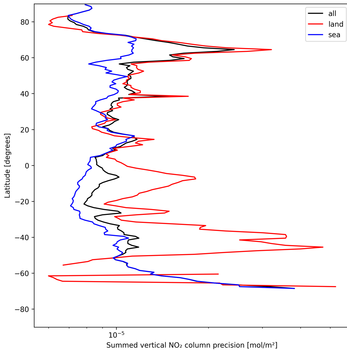
Figure 22: Zonal average of “Summed vertical NO 2 column precision” for 2025-07-24 to 2025-07-25.
