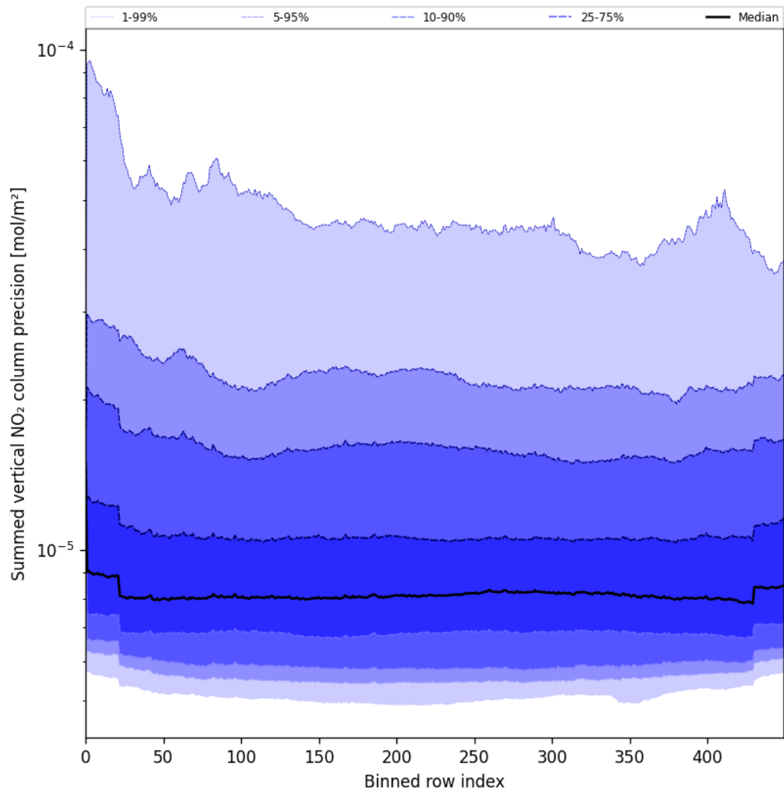
Figure 56: Along track statistics of “Summed vertical NO 2 column precision” for 2025-07-24 to 2025-07-25
