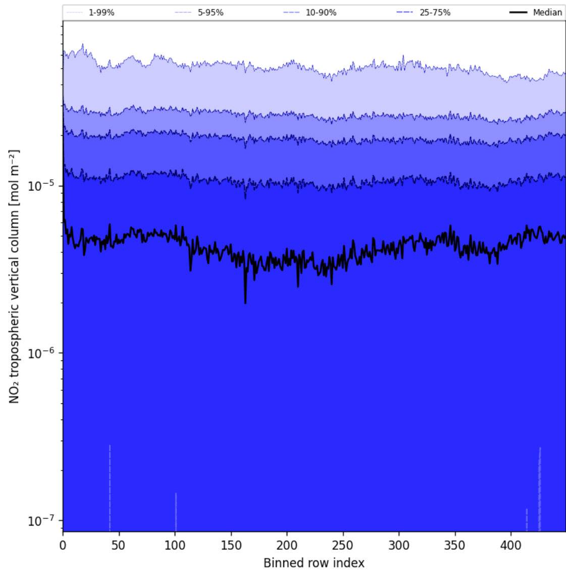
Figure 44: Along track statistics of “NO 2 tropospheric vertical column” for 2025-07-24 to 2025-07-25
