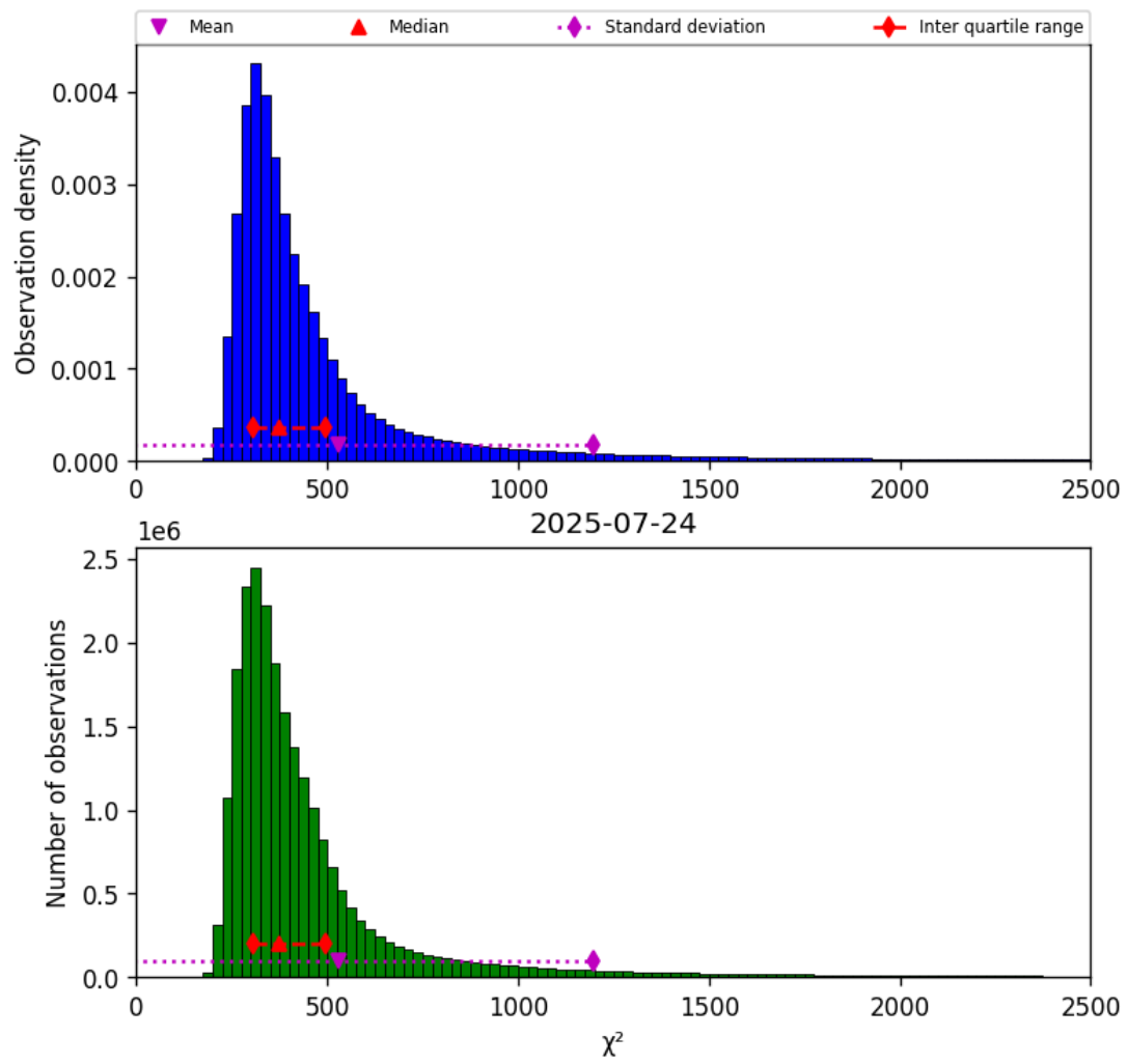
Figure 40: Histogram of “ \chi^2 ” for 2025-07-24 to 2025-07-25
