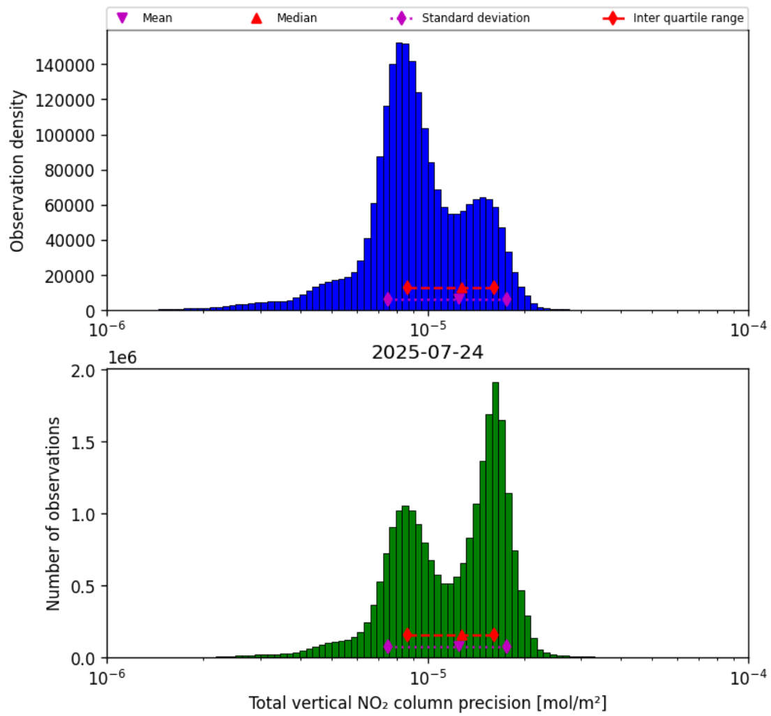
Figure 37: Histogram of “Total vertical NO 2 column precision” for 2025-07-24 to 2025-07-25
