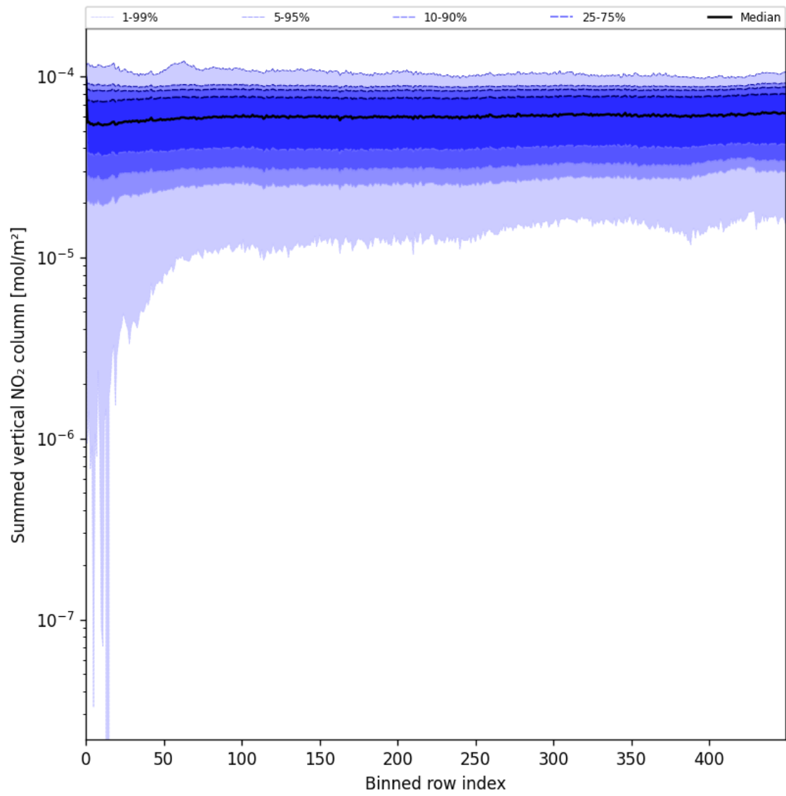
Figure 55: Along track statistics of “Summed vertical NO 2 column” for 2025-07-24 to 2025-07-25
