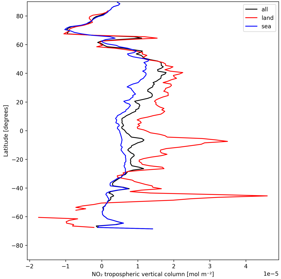
Figure 10: Zonal average of “NO 2 tropospheric vertical column” for 2025-07-24 to 2025-07-25.
