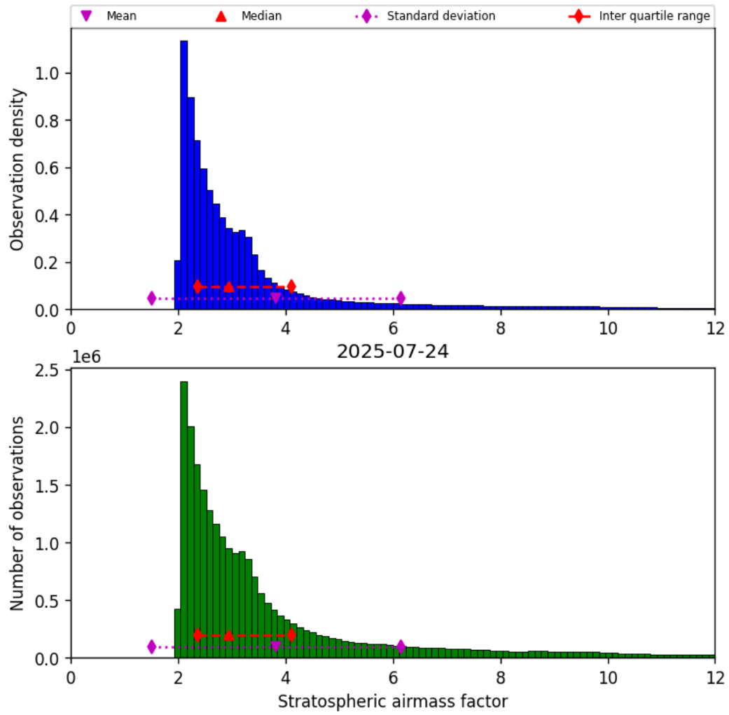
Figure 42: Histogram of “Stratospheric airmass factor” for 2025-07-24 to 2025-07-25
