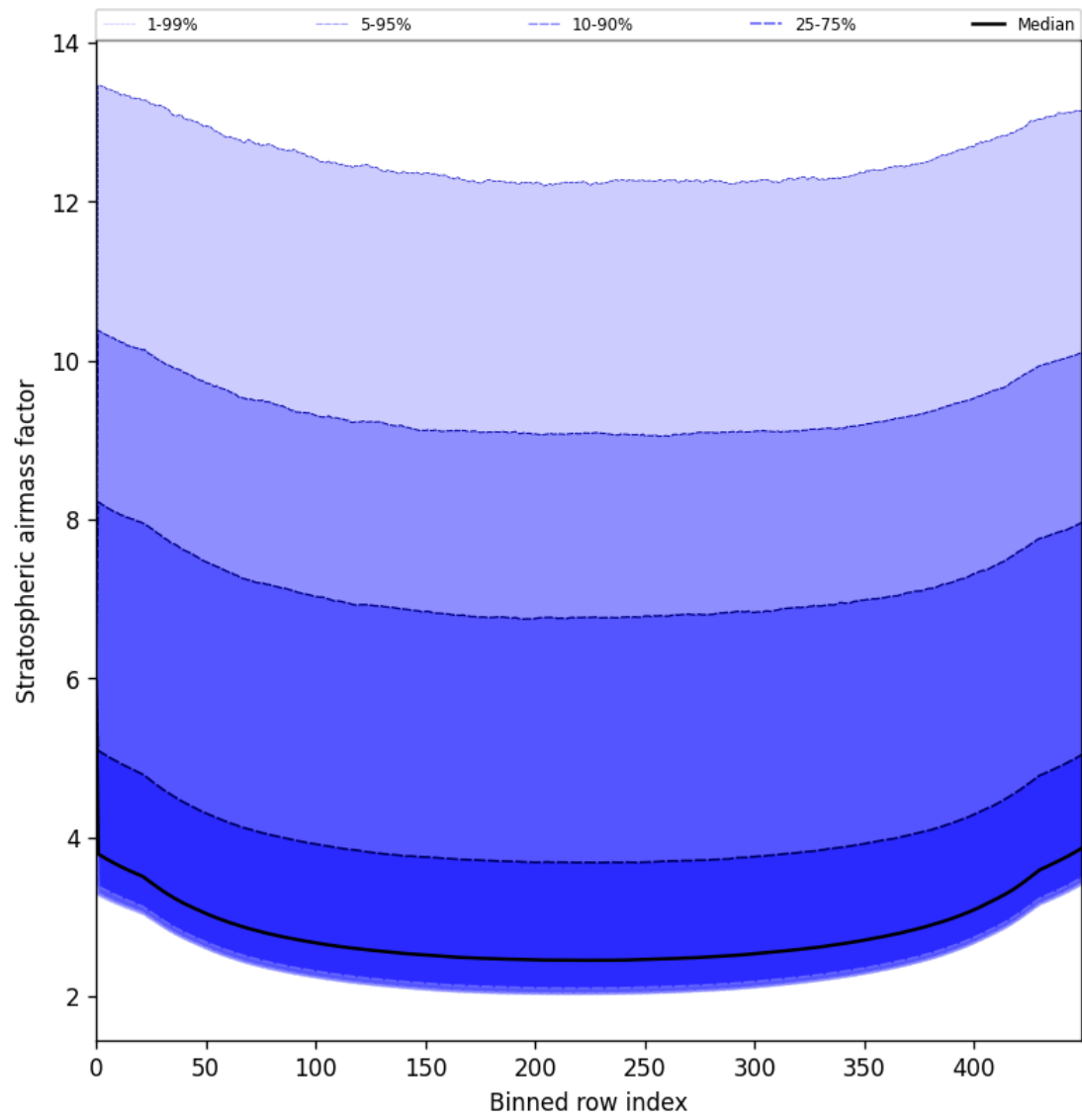
Figure 59: Along track statistics of “Stratospheric airmass factor” for 2025-07-24 to 2025-07-25
