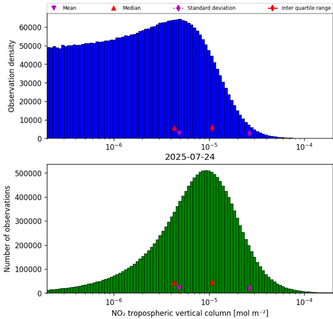
Figure 27: Histogram of “NO 2 tropospheric vertical column” for 2025-07-24 to 2025-07-25
