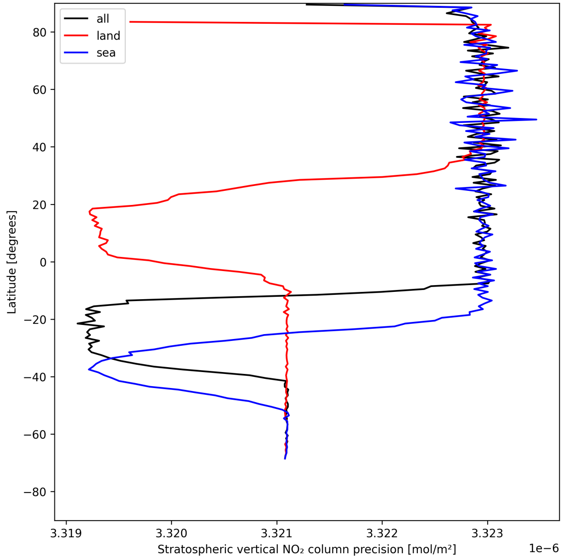
Figure 18: Zonal average of “Stratospheric vertical NO 2 column precision” for 2025-07-24 to 2025-07-25.
