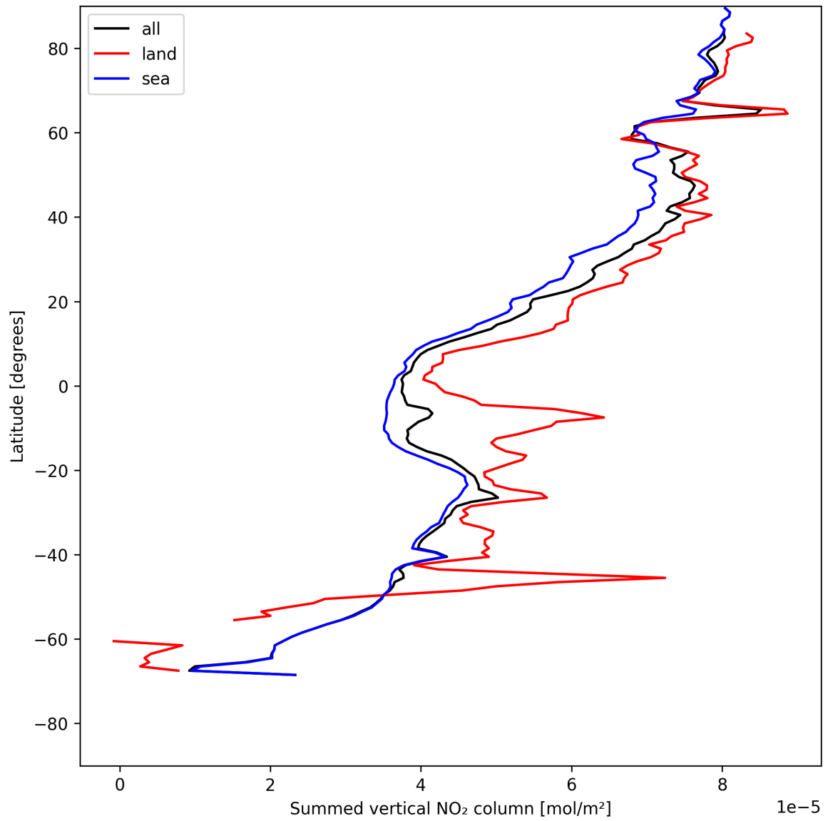
Figure 21: Zonal average of “Summed vertical NO 2 column” for 2025-07-24 to 2025-07-25.
