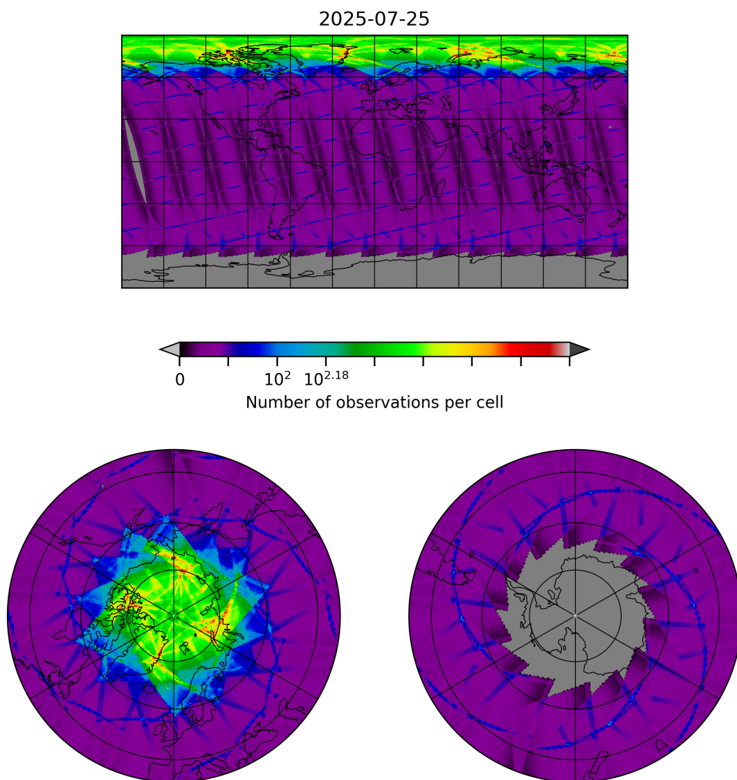
Figure 8: Map of the number of observations for 2025-07-25 to 2025-07-26
