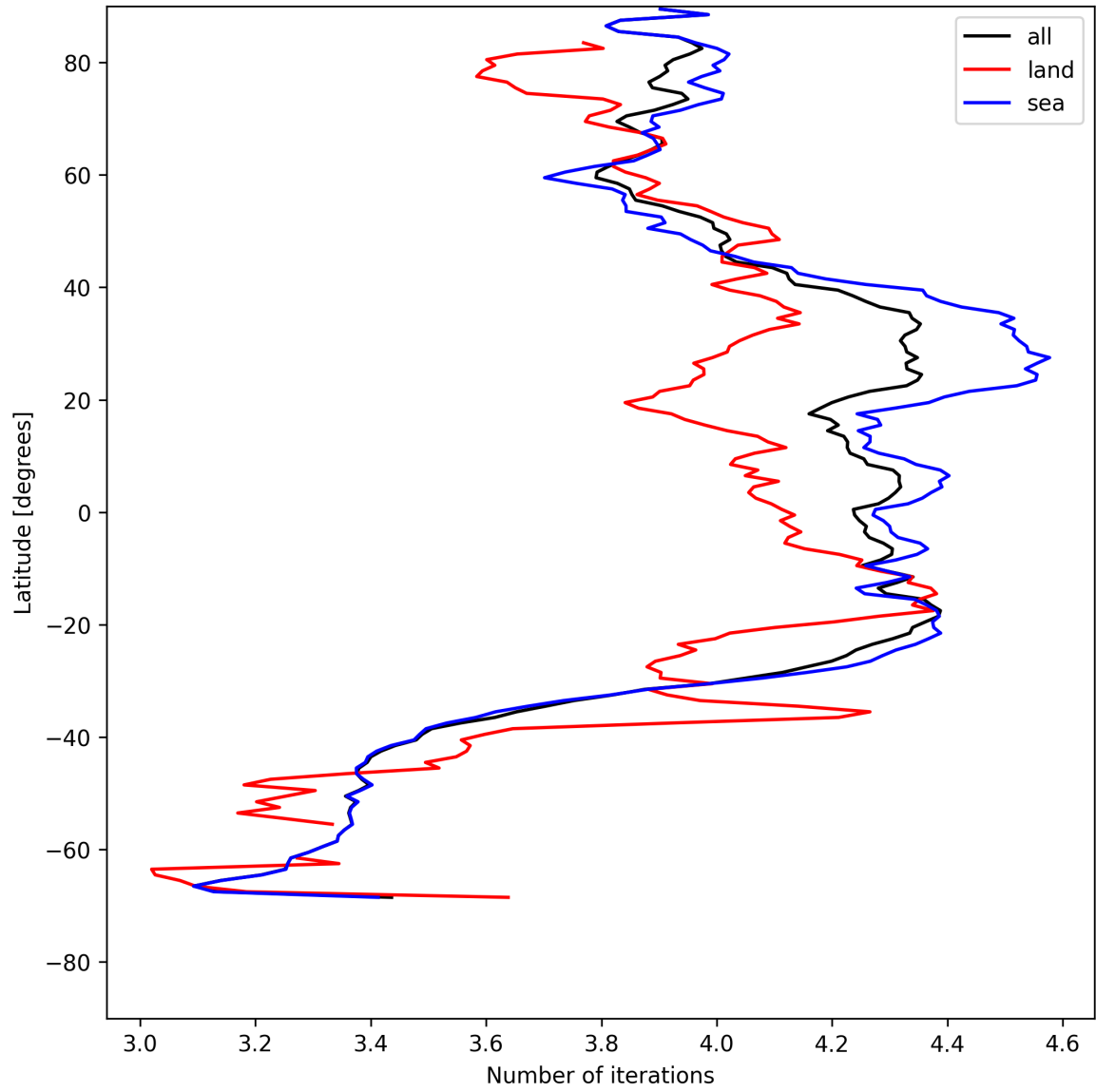
Figure 15: Zonal average of “Number of iterations” for 2025-07-25 to 2025-07-26.
