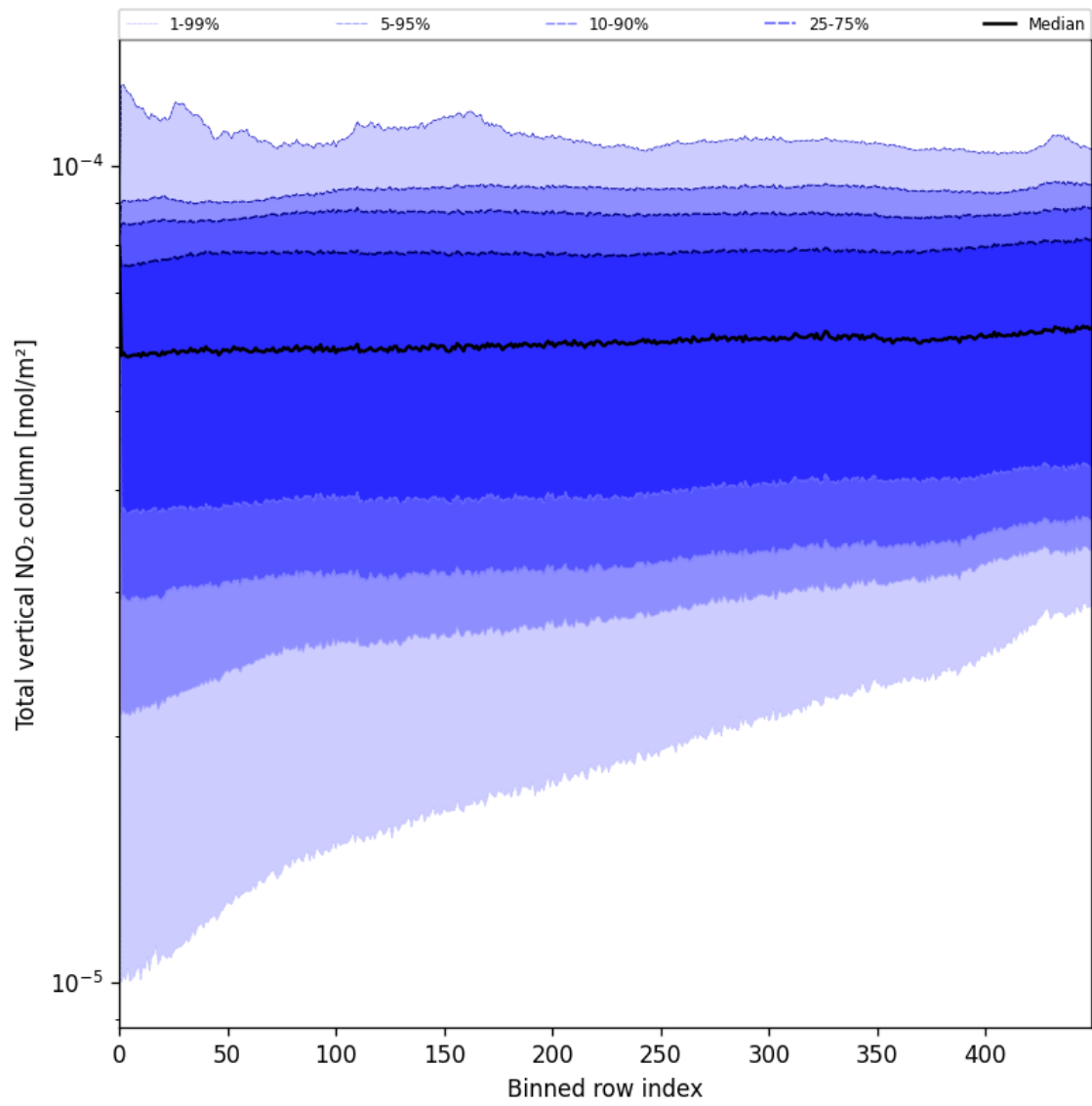
Figure 53: Along track statistics of “Total vertical NO 2 column” for 2025-07-25 to 2025-07-26
