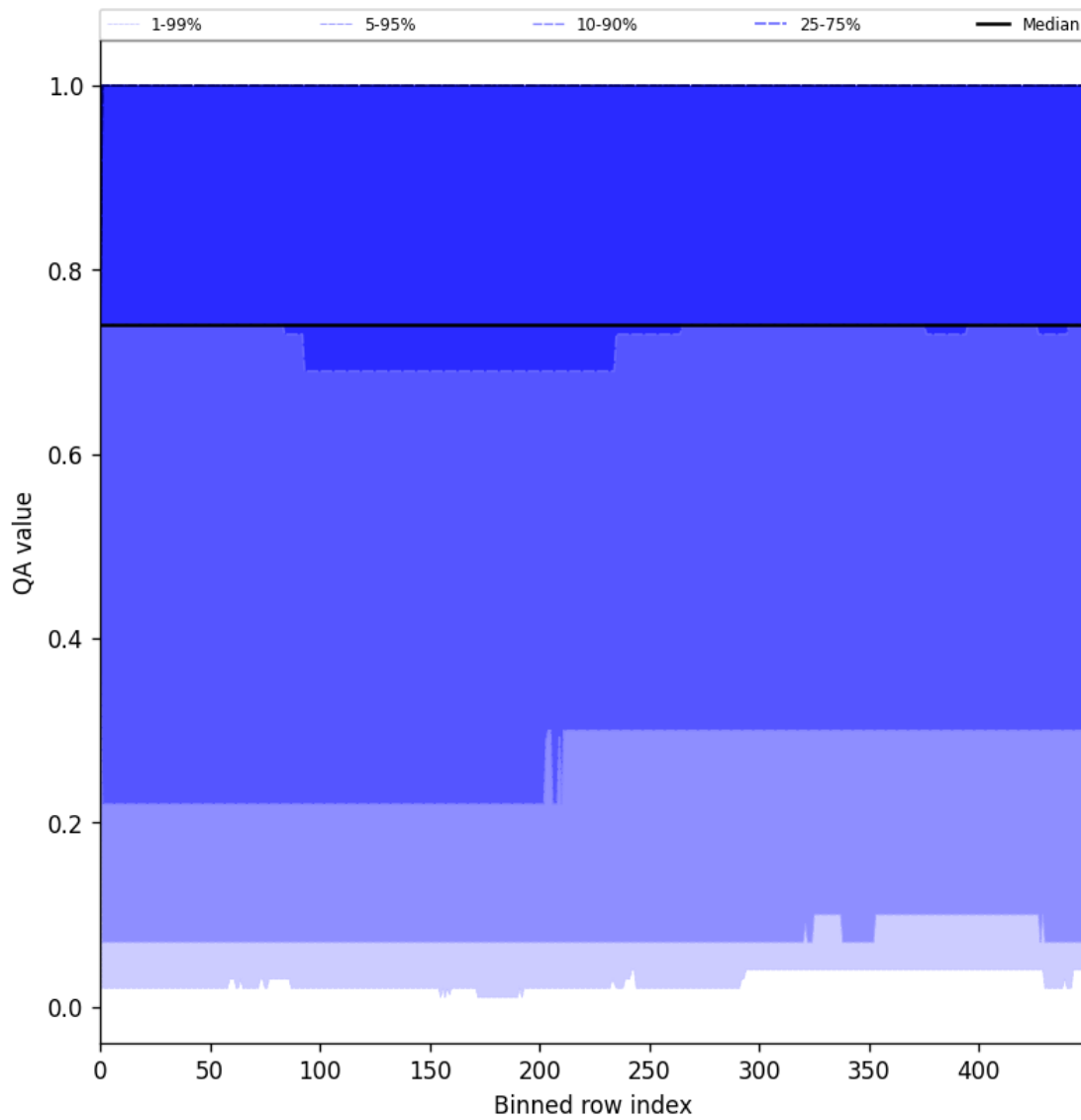
Figure 43: Along track statistics of “QA value” for 2025-07-25 to 2025-07-26
