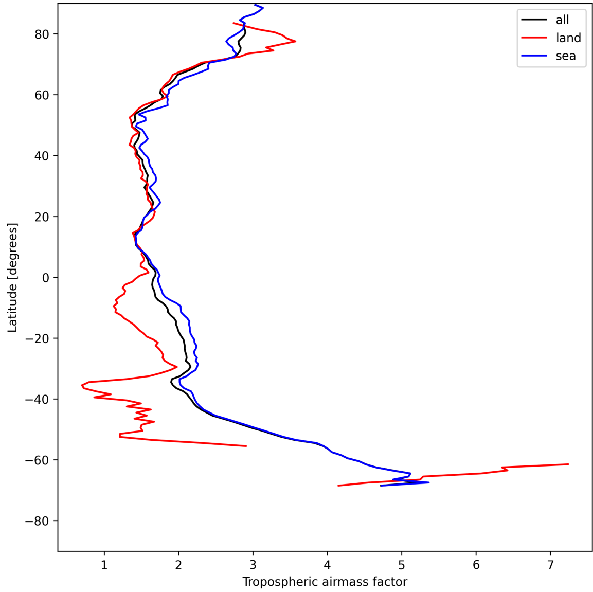
Figure 12: Zonal average of “Tropospheric airmass factor” for 2025-07-25 to 2025-07-26.
