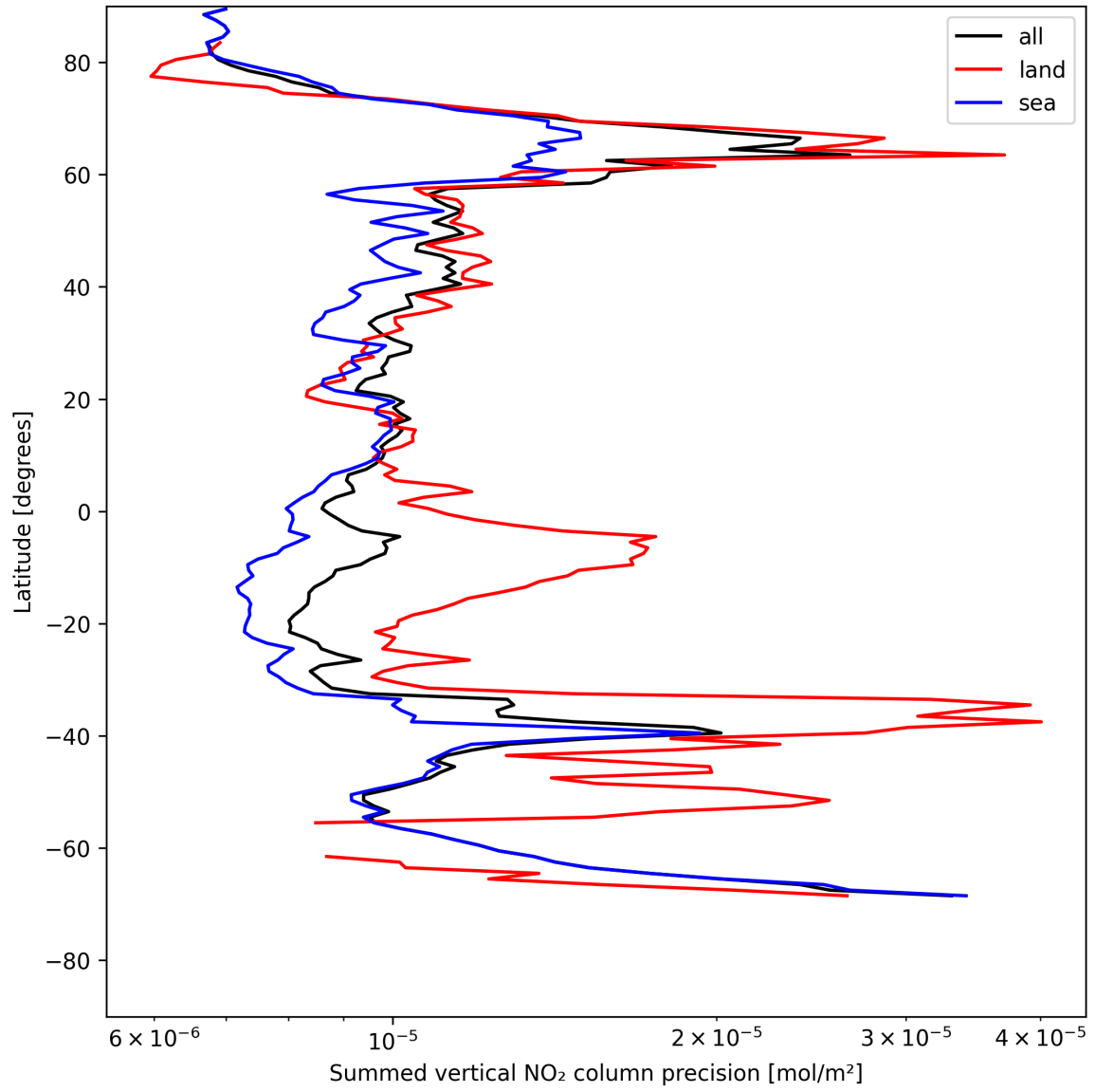
Figure 22: Zonal average of “Summed vertical NO 2 column precision” for 2025-07-25 to 2025-07-26.
