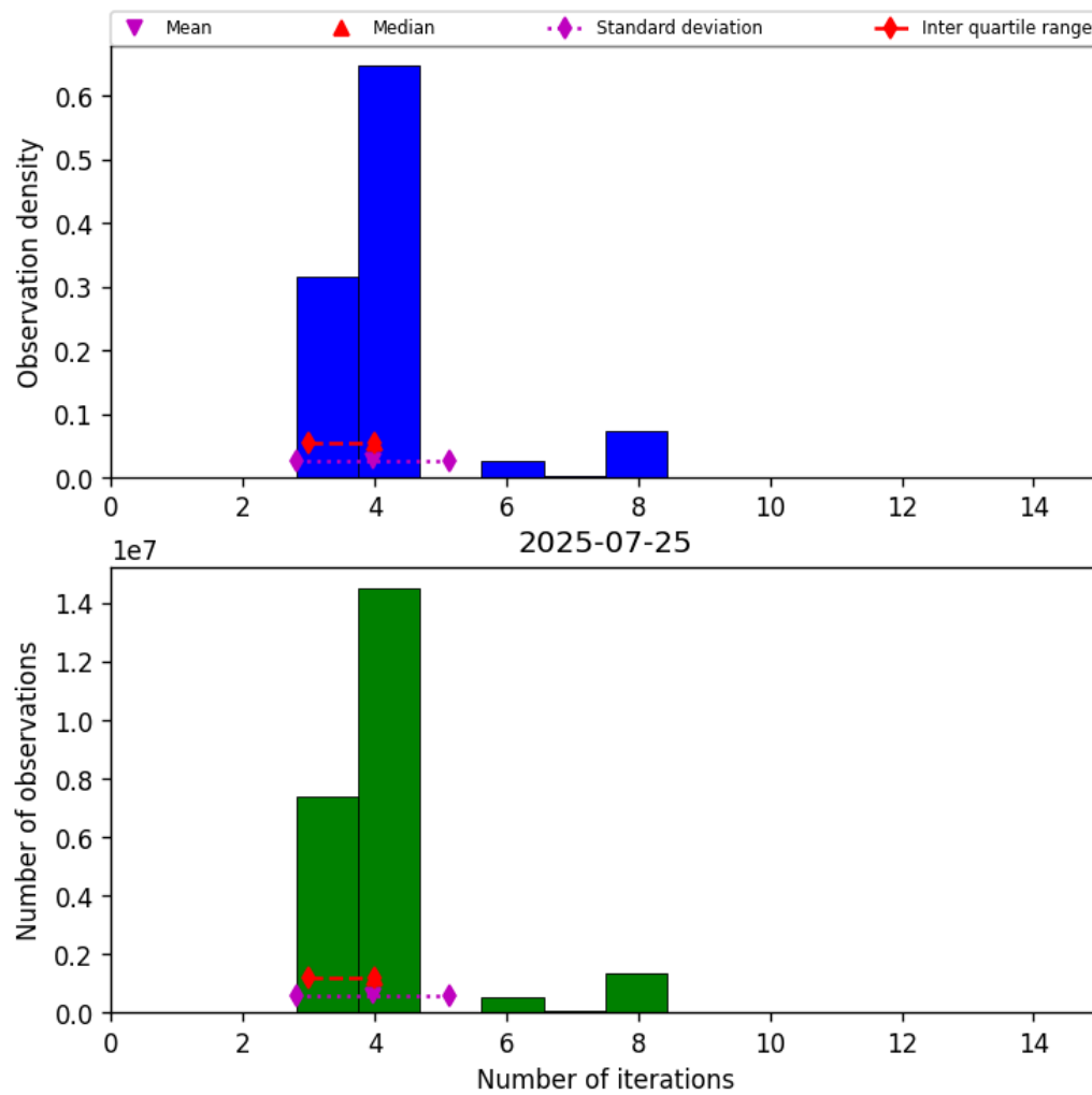
Figure 32: Histogram of “Number of iterations” for 2025-07-25 to 2025-07-26
