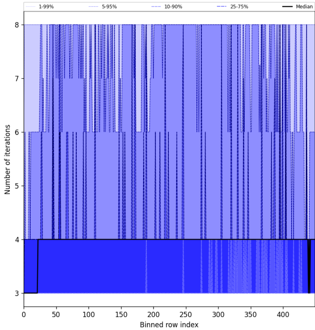
Figure 49: Along track statistics of “Number of iterations” for 2025-07-25 to 2025-07-26
