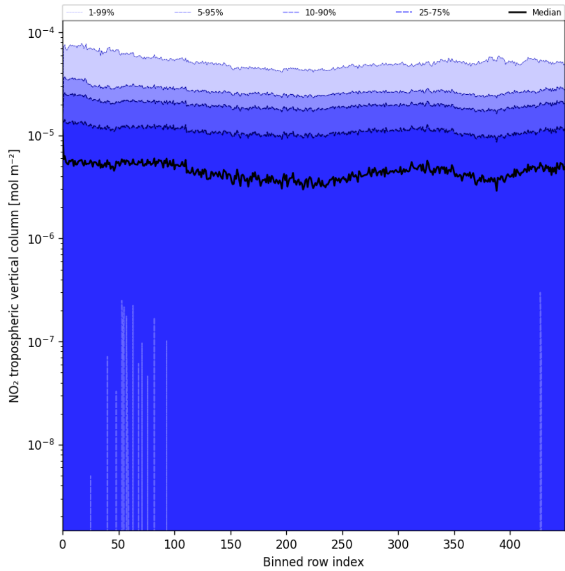
Figure 44: Along track statistics of “NO 2 tropospheric vertical column” for 2025-07-25 to 2025-07-26
