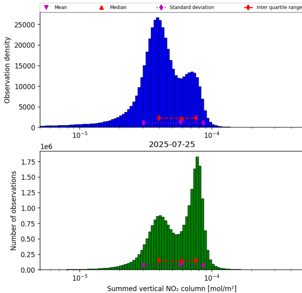
Figure 38: Histogram of “Summed vertical NO 2 column” for 2025-07-25 to 2025-07-26
