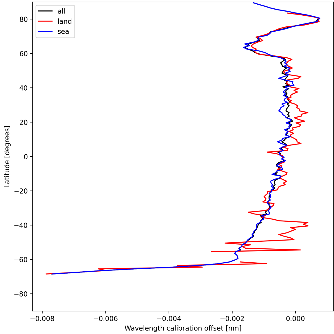
Figure 16: Zonal average of “Wavelength calibration offset” for 2025-07-25 to 2025-07-26.
