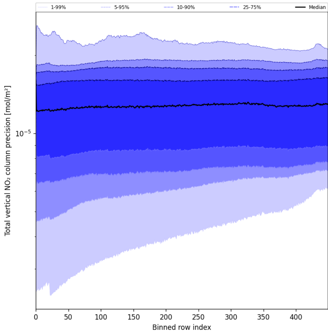
Figure 54: Along track statistics of “Total vertical NO 2 column precision” for 2025-07-25 to 2025-07-26
