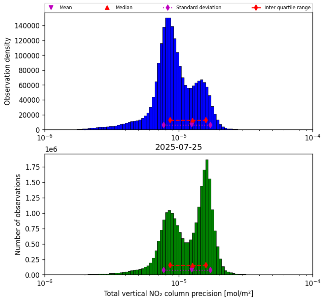
Figure 37: Histogram of “Total vertical NO 2 column precision” for 2025-07-25 to 2025-07-26
