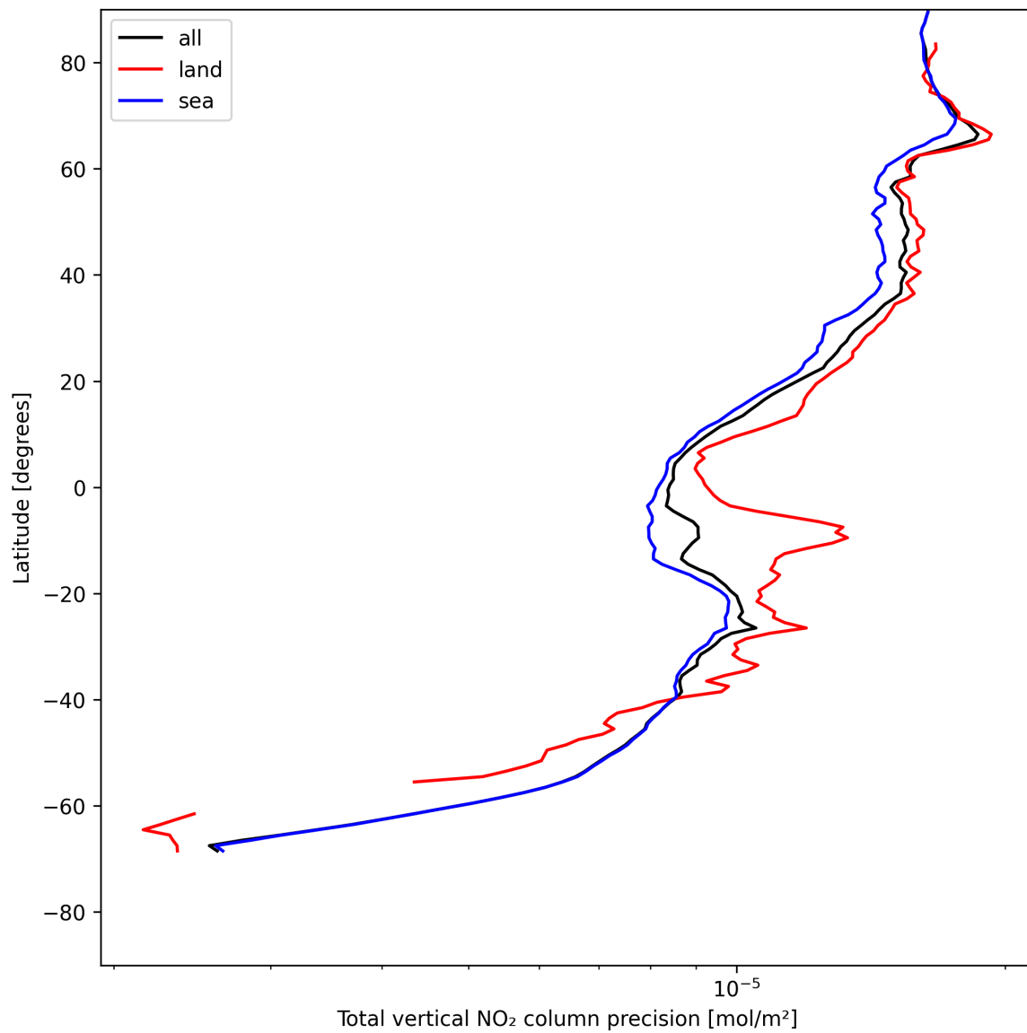
Figure 20: Zonal average of “Total vertical NO 2 column precision” for 2025-07-25 to 2025-07-26.
