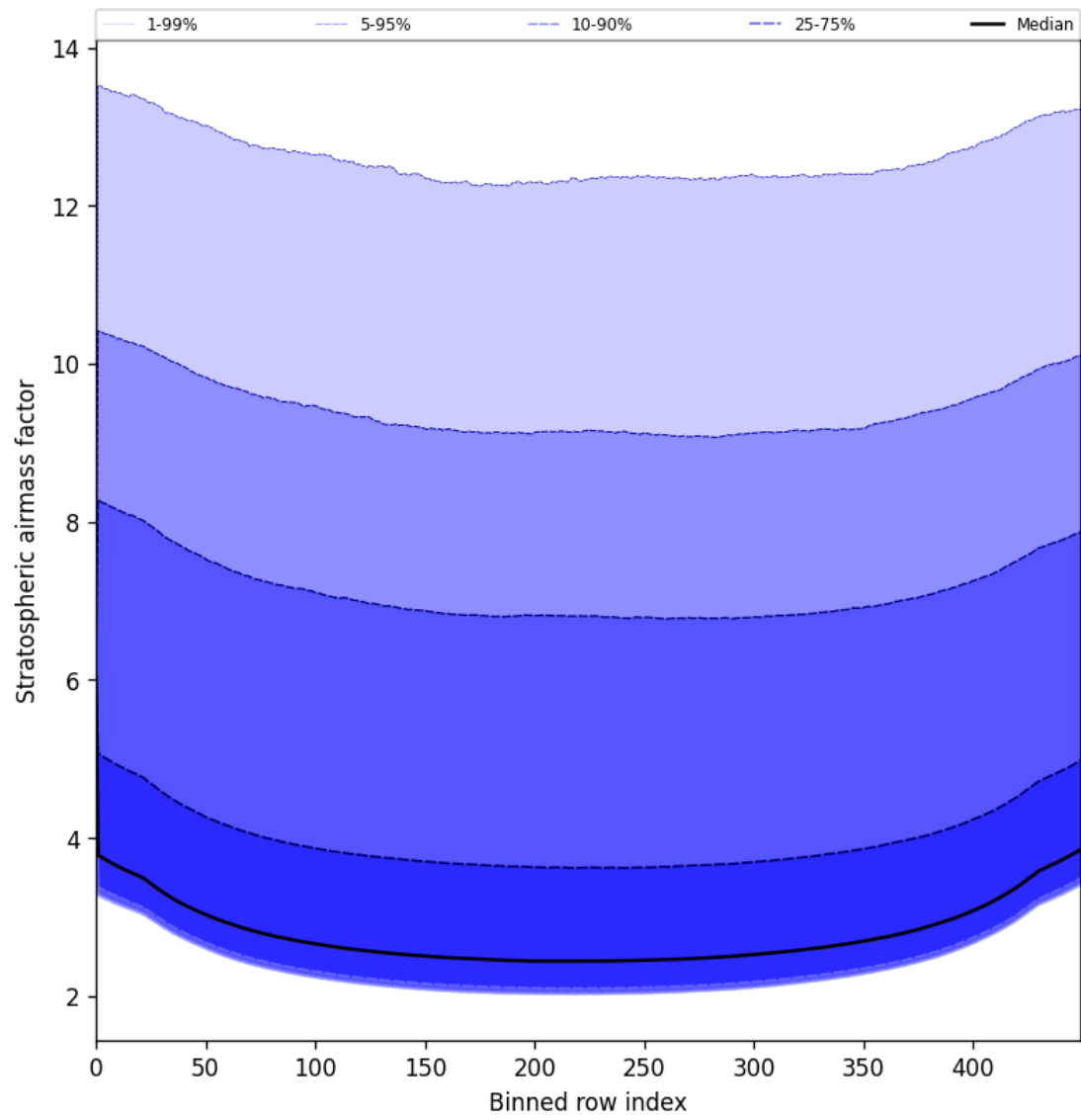
Figure 59: Along track statistics of “Stratospheric airmass factor” for 2025-07-25 to 2025-07-26
