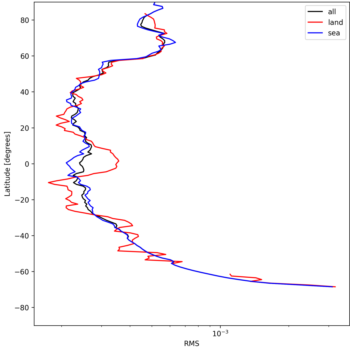
Figure 24: Zonal average of “RMS” for 2025-07-25 to 2025-07-26.
