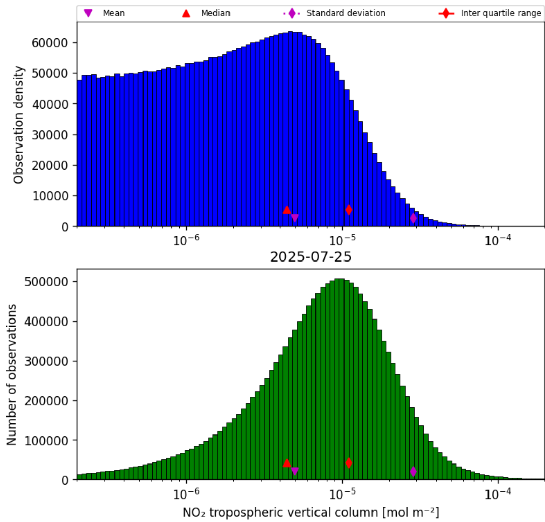
Figure 27: Histogram of “NO 2 tropospheric vertical column” for 2025-07-25 to 2025-07-26
