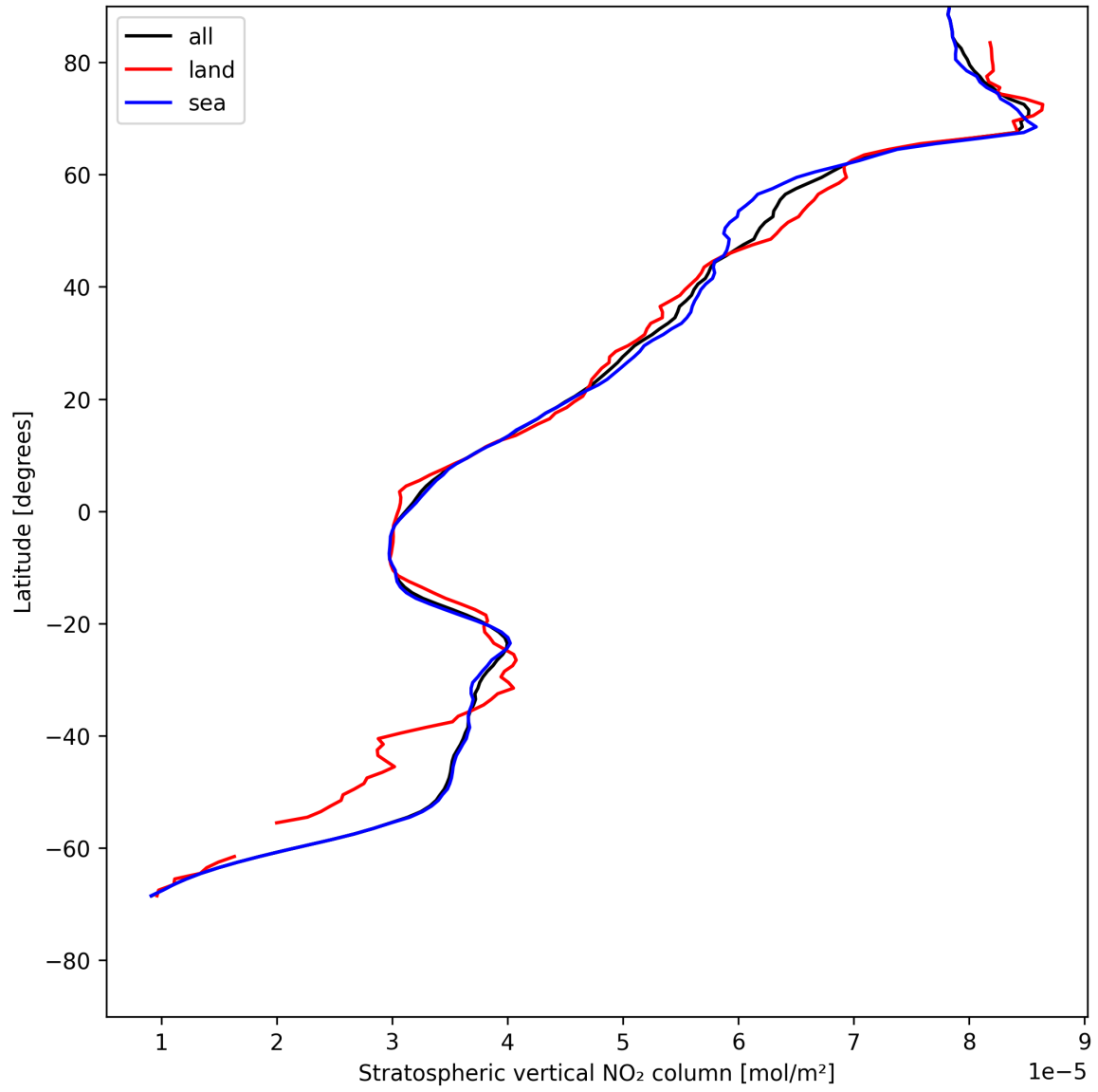
Figure 17: Zonal average of “Stratospheric vertical NO 2 column” for 2025-07-25 to 2025-07-26.
