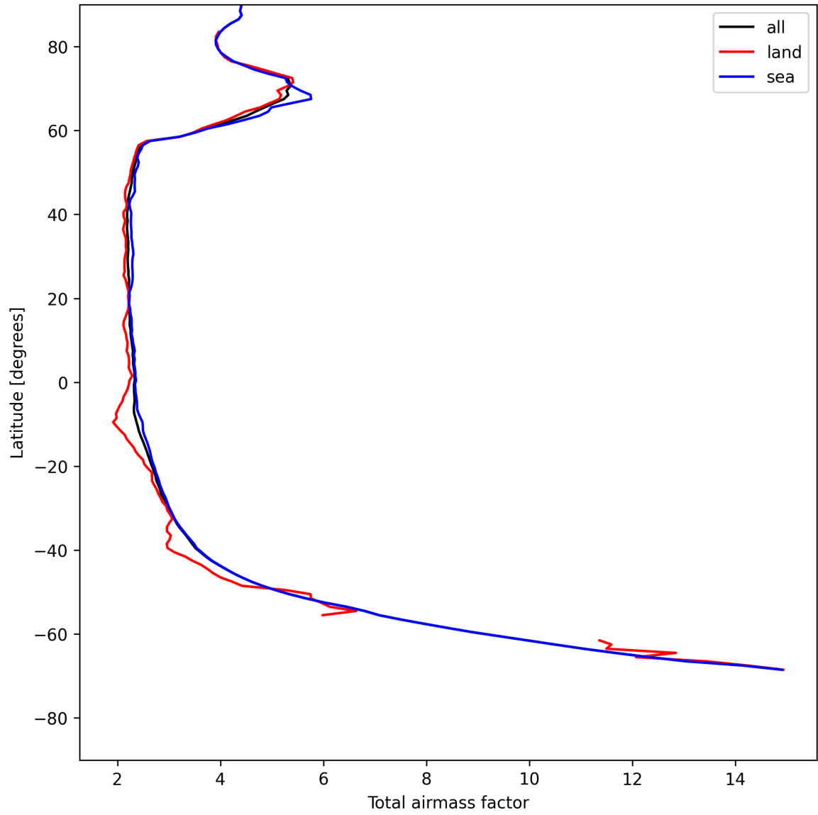
Figure 13: Zonal average of “Total airmass factor” for 2025-07-25 to 2025-07-26.
