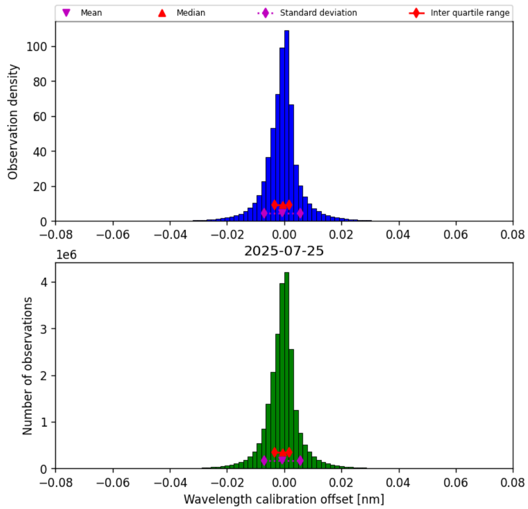
Figure 33: Histogram of “Wavelength calibration offset” for 2025-07-25 to 2025-07-26
