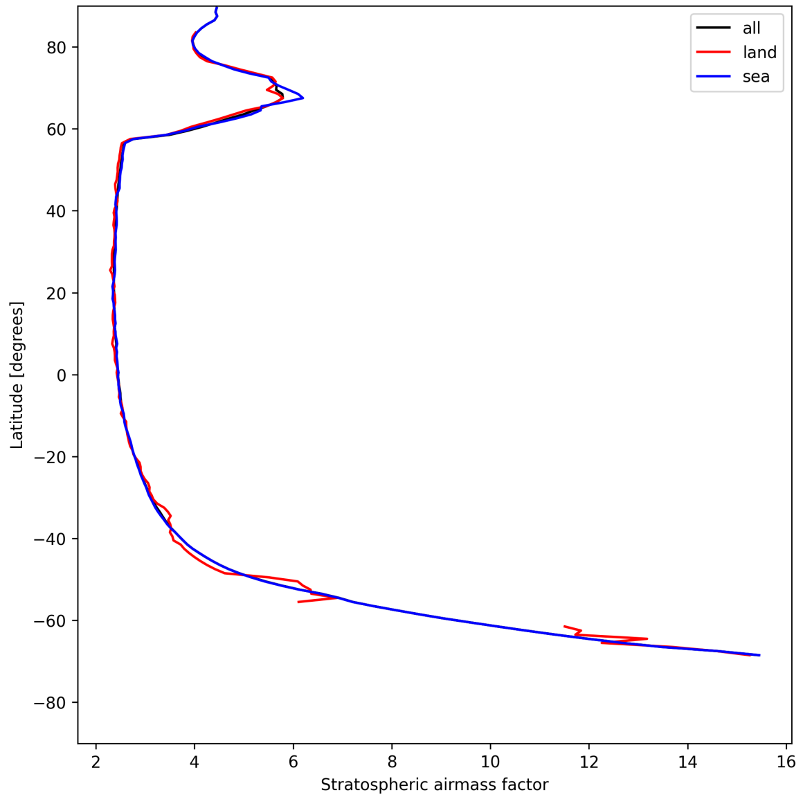
Figure 25: Zonal average of “Stratospheric airmass factor” for 2025-07-25 to 2025-07-26.
