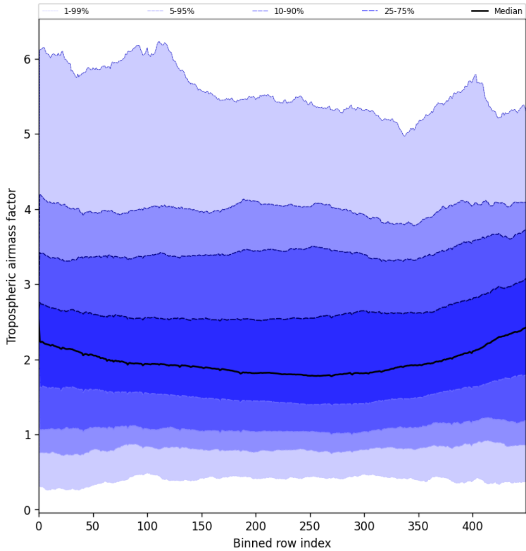
Figure 46: Along track statistics of “Tropospheric airmass factor” for 2025-07-25 to 2025-07-26
