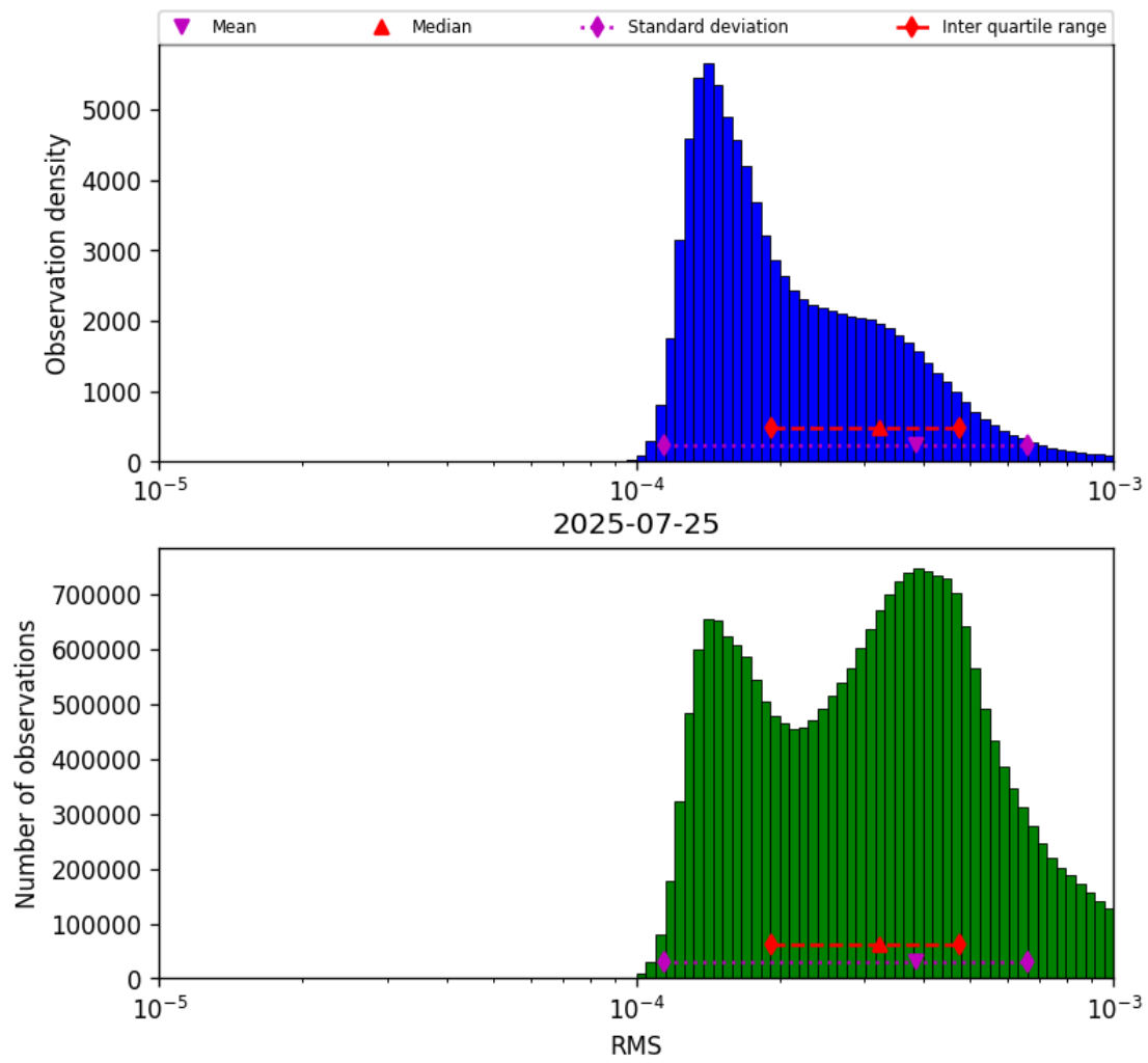
Figure 41: Histogram of “RMS” for 2025-07-25 to 2025-07-26
