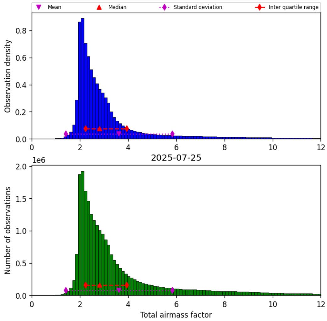
Figure 30: Histogram of “Total airmass factor” for 2025-07-25 to 2025-07-26
