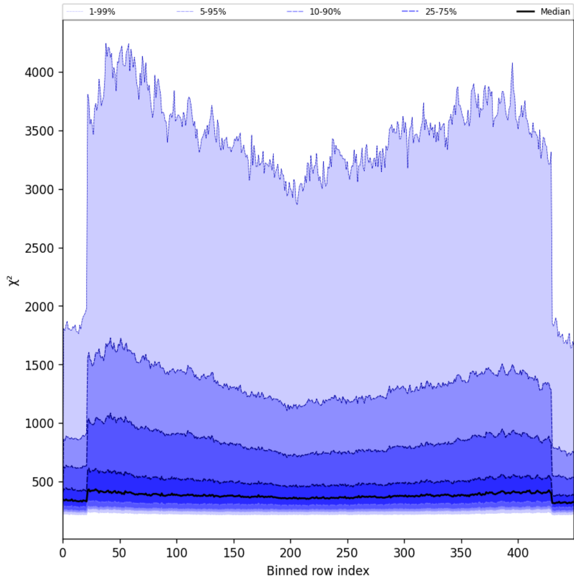
Figure 57: Along track statistics of “ \chi^2 ” for 2025-07-25 to 2025-07-26
