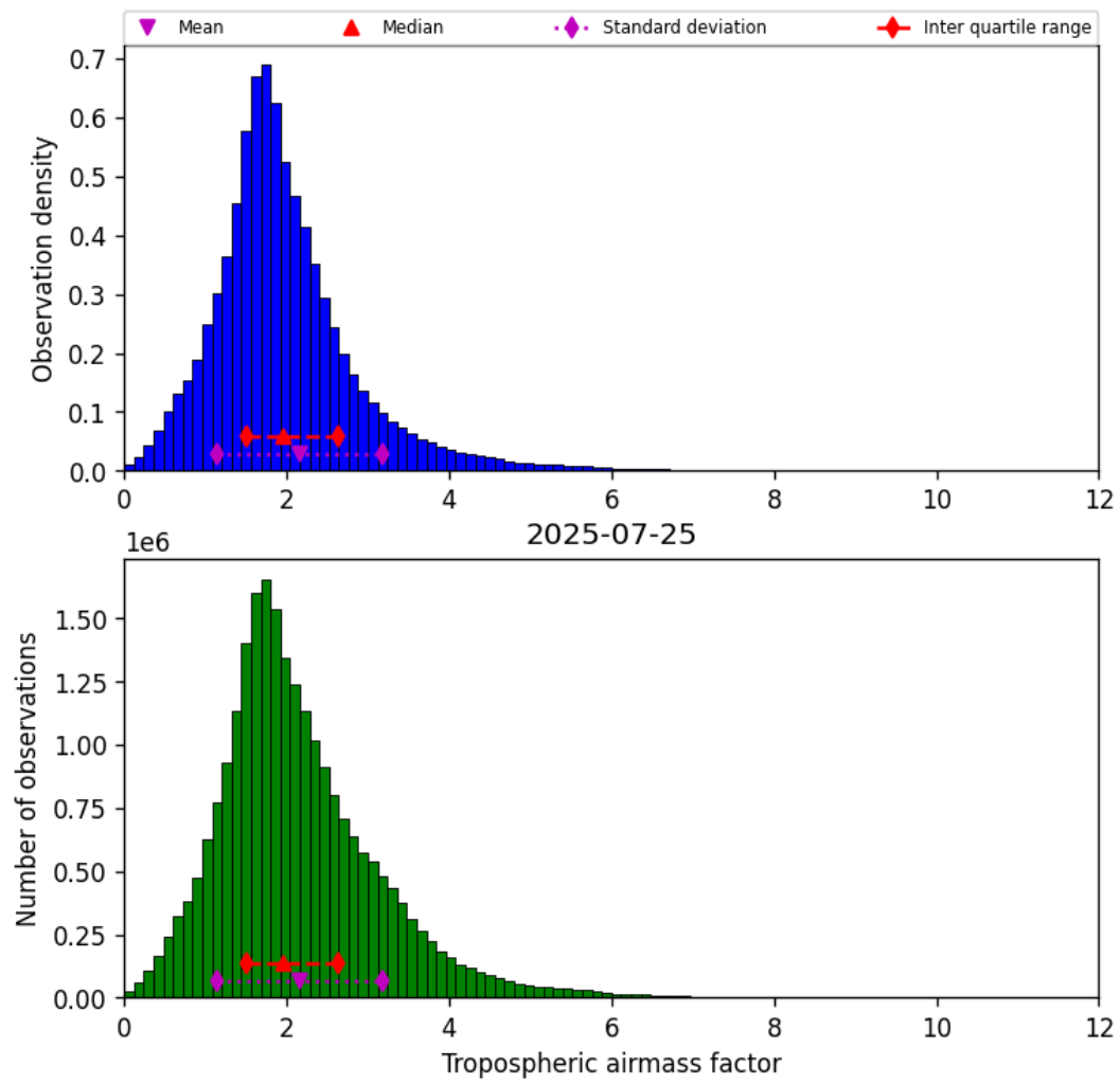
Figure 29: Histogram of “Tropospheric airmass factor” for 2025-07-25 to 2025-07-26
