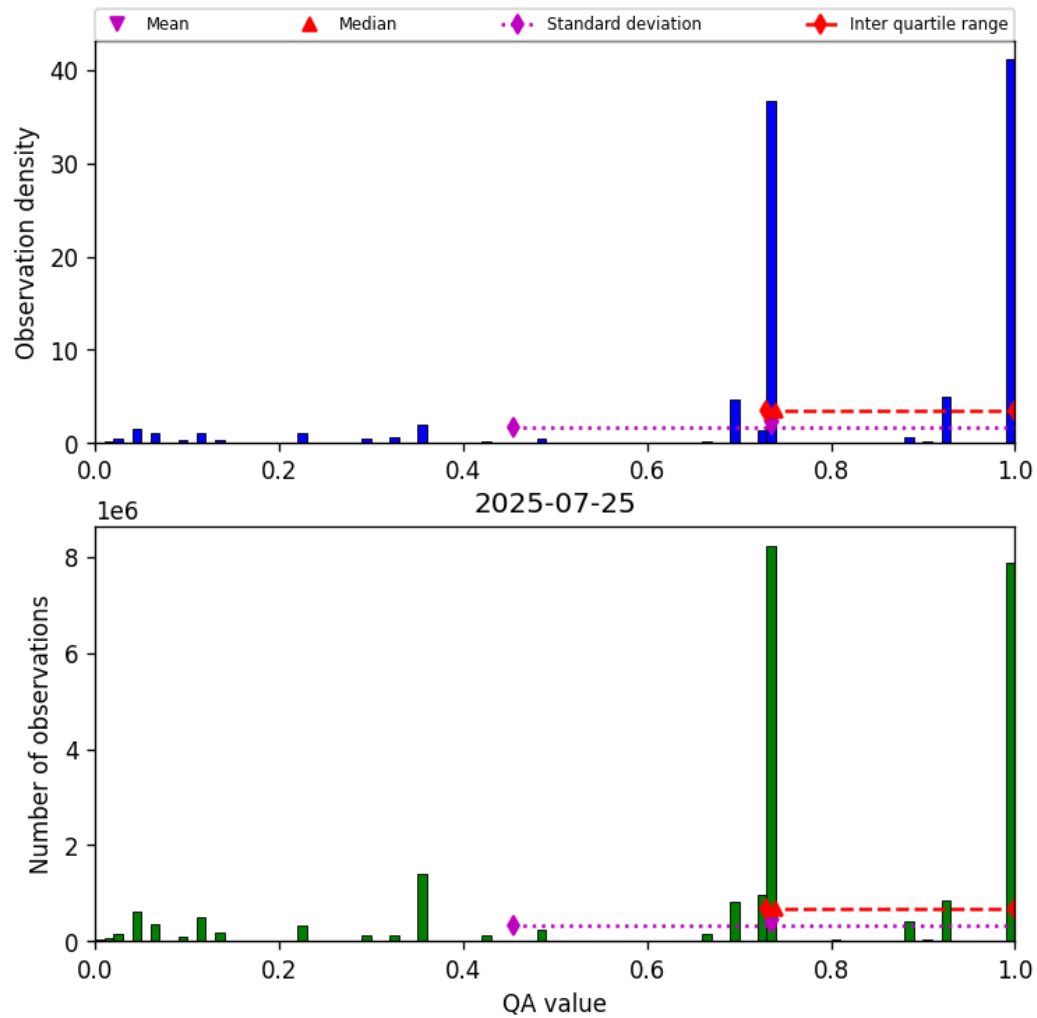
Figure 26: Histogram of “QA value” for 2025-07-25 to 2025-07-26
