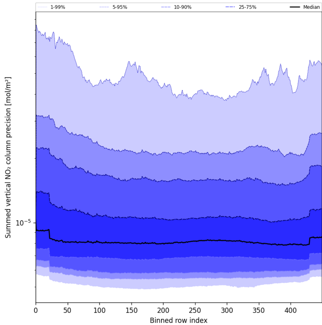
Figure 56: Along track statistics of “Summed vertical NO 2 column precision” for 2025-07-25 to 2025-07-26
