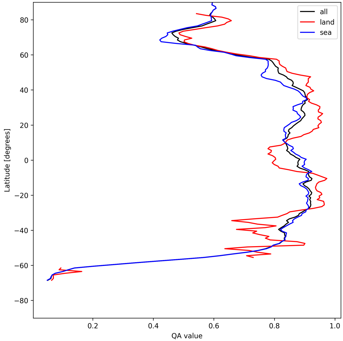
Figure 9: Zonal average of “QA value” for 2025-07-25 to 2025-07-26.
