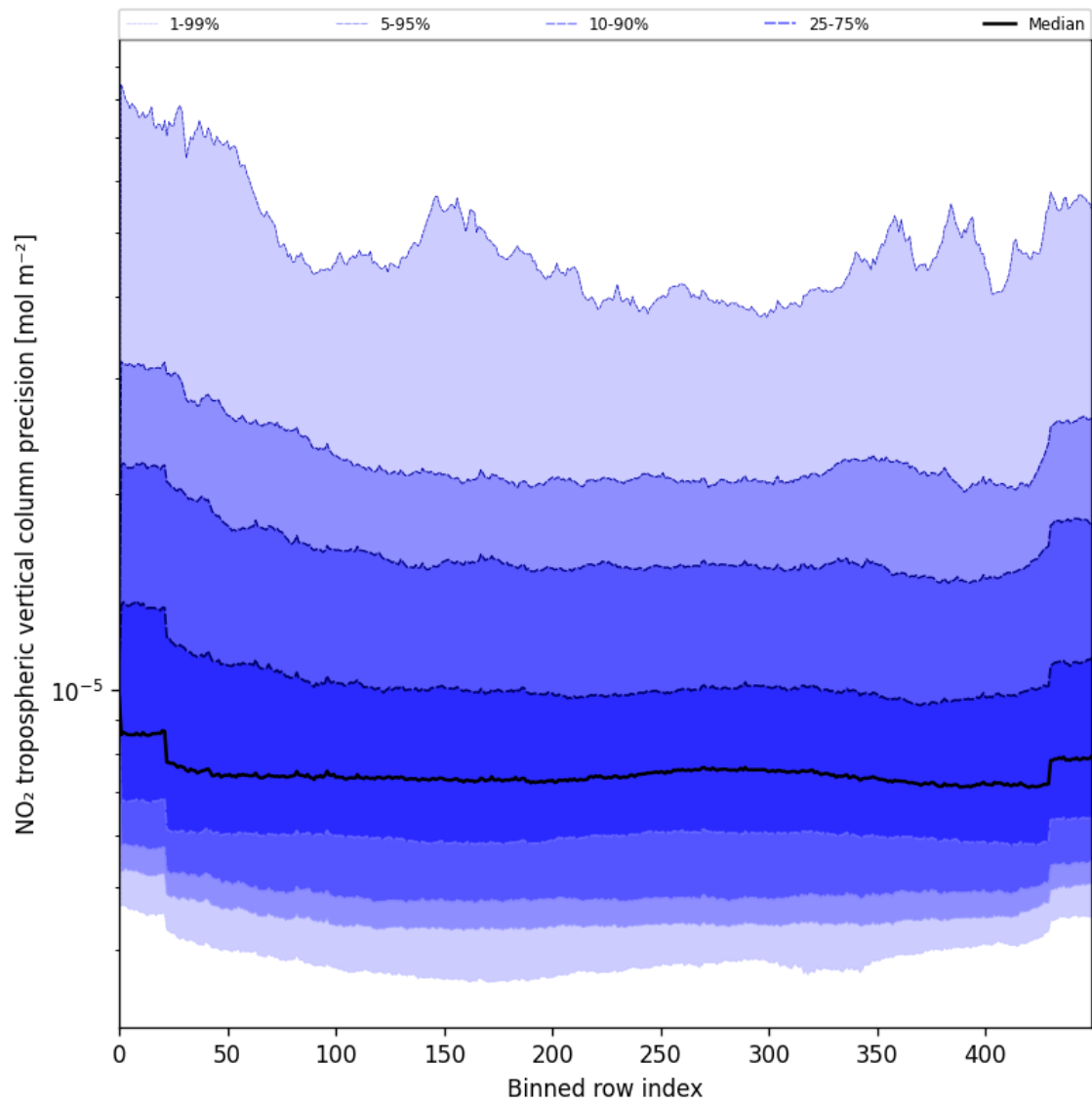
Figure 45: Along track statistics of “NO 2 tropospheric vertical column precision” for 2025-07-25 to 2025-07-26
