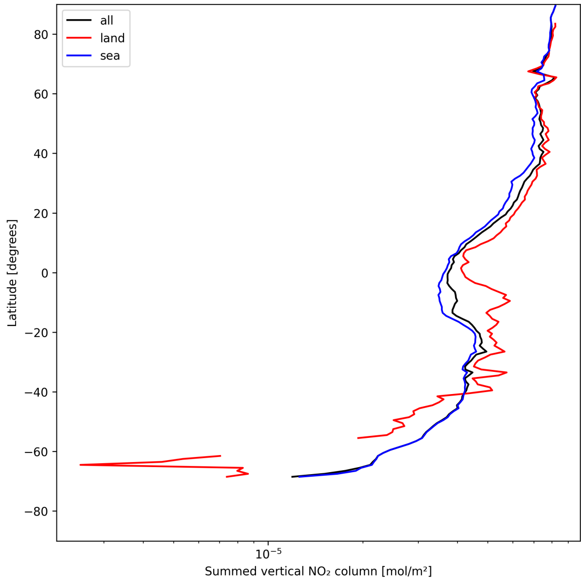
Figure 21: Zonal average of “Summed vertical NO 2 column” for 2025-07-25 to 2025-07-26.
