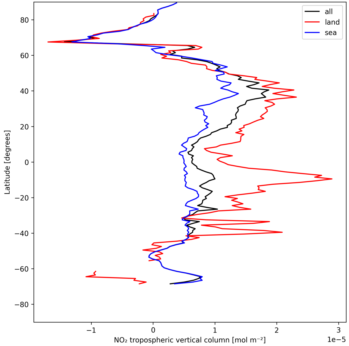
Figure 10: Zonal average of “NO 2 tropospheric vertical column” for 2025-07-25 to 2025-07-26.
