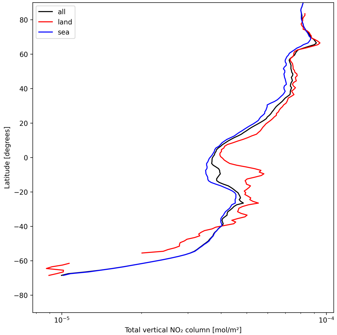
Figure 19: Zonal average of “Total vertical NO 2 column” for 2025-07-25 to 2025-07-26.
