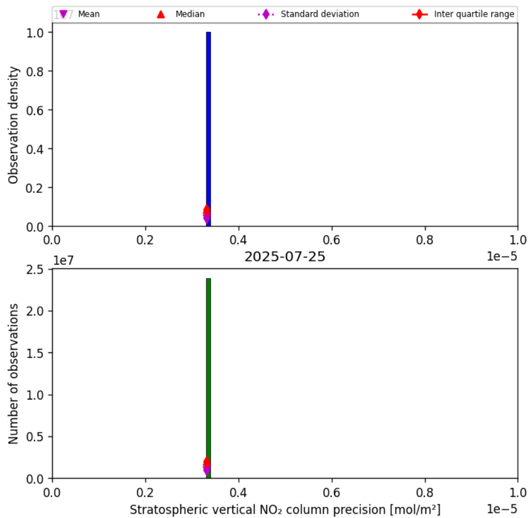
Figure 35: Histogram of “Stratospheric vertical NO 2 column precision” for 2025-07-25 to 2025-07-26
