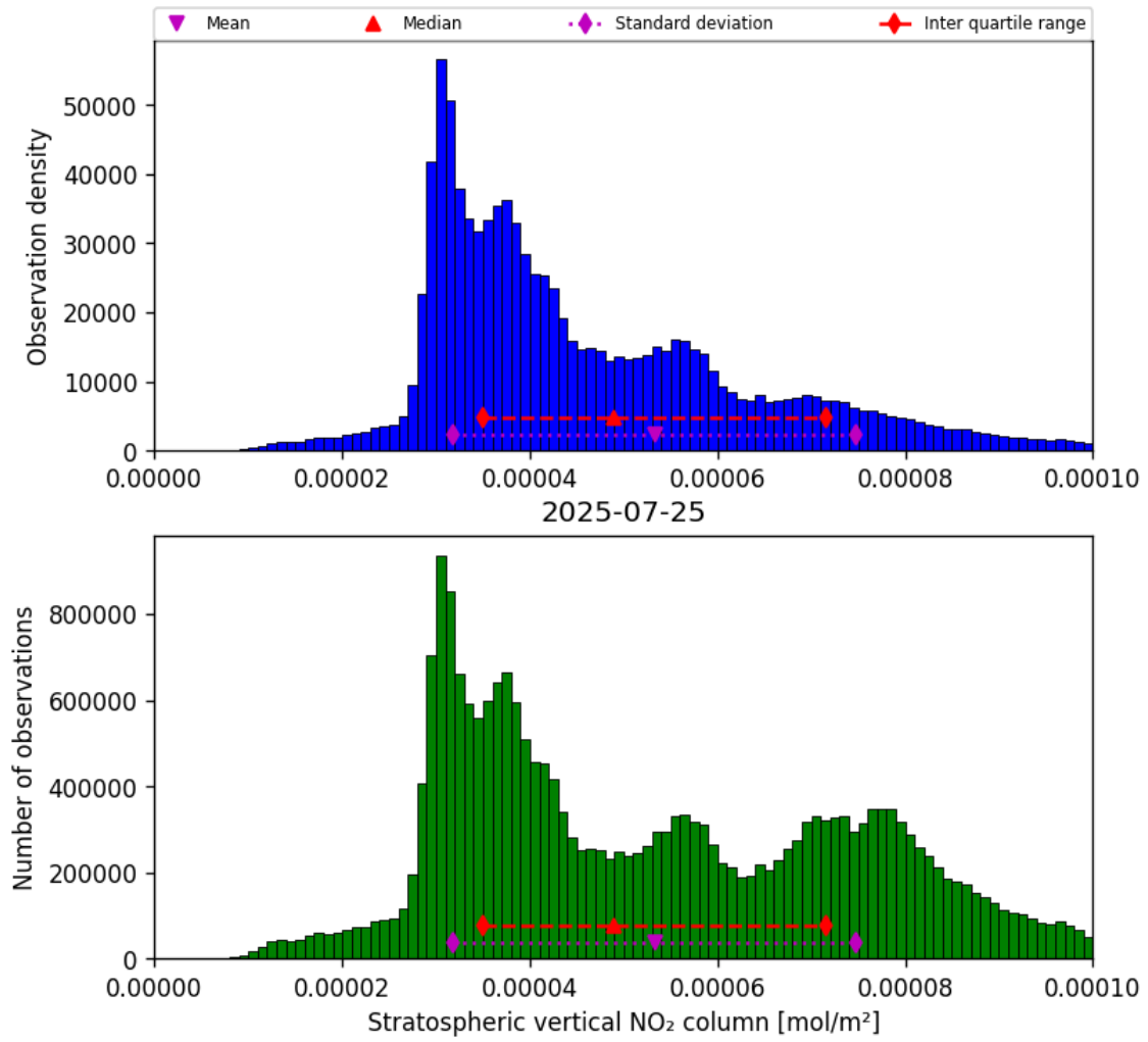
Figure 34: Histogram of “Stratospheric vertical NO 2 column” for 2025-07-25 to 2025-07-26
