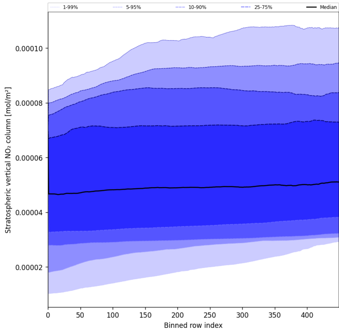
Figure 51: Along track statistics of “Stratospheric vertical NO 2 column” for 2025-07-25 to 2025-07-26
