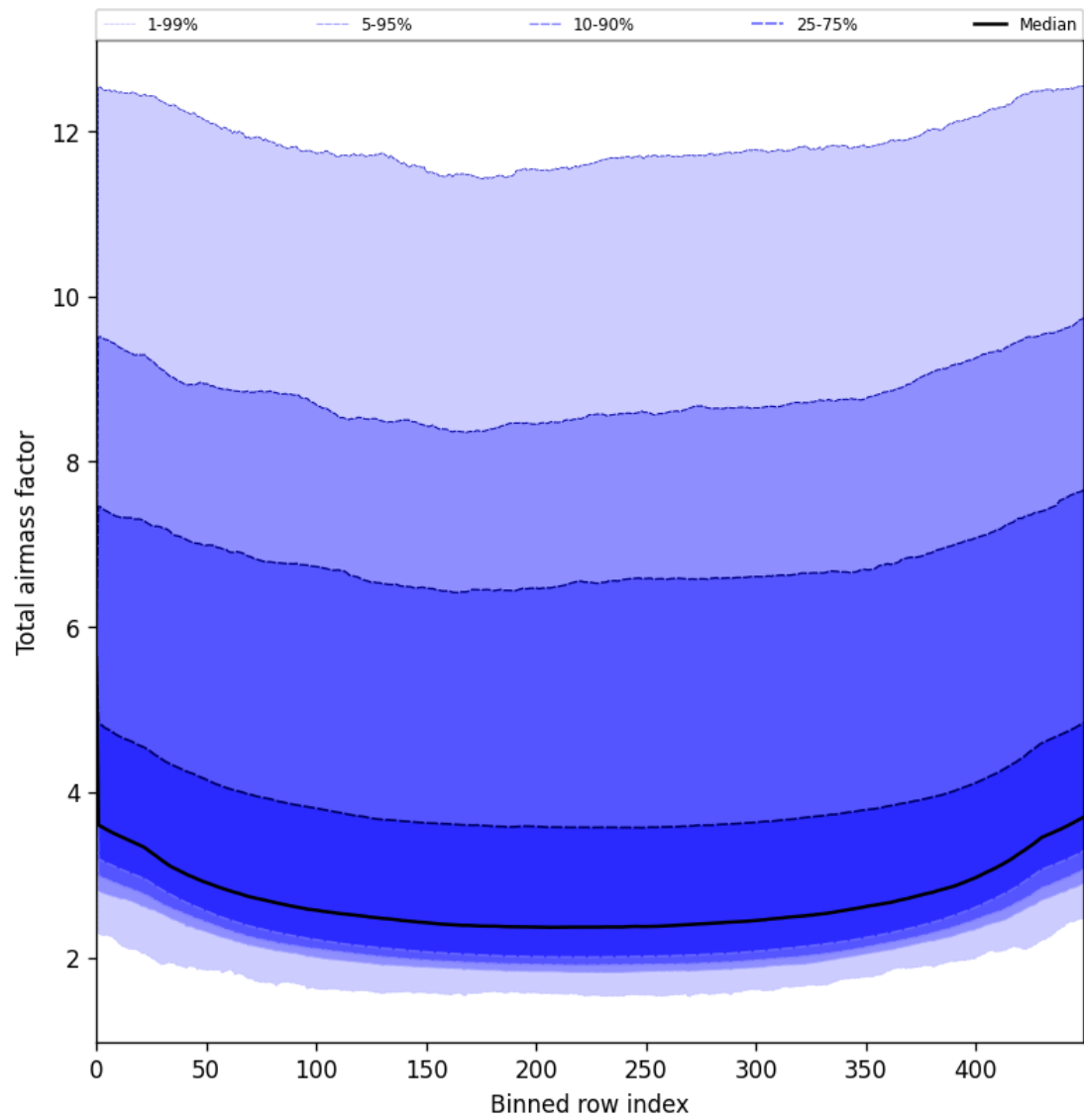
Figure 47: Along track statistics of “Total airmass factor” for 2025-07-25 to 2025-07-26
