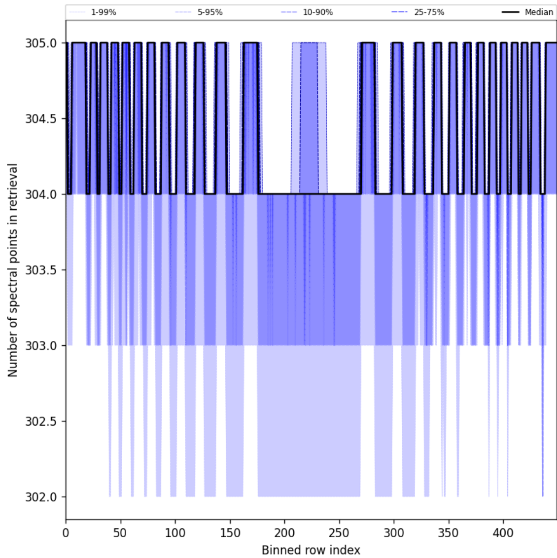
Figure 48: Along track statistics of “Number of spectral points in retrieval” for 2025-07-25 to 2025-07-26
