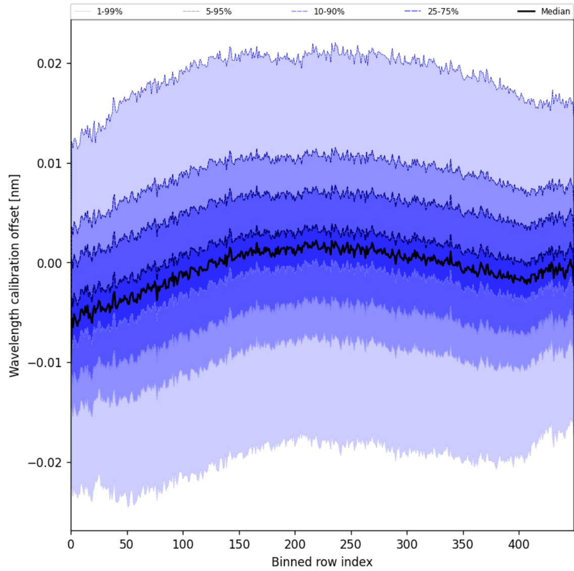
Figure 50: Along track statistics of “Wavelength calibration offset” for 2025-07-25 to 2025-07-26
