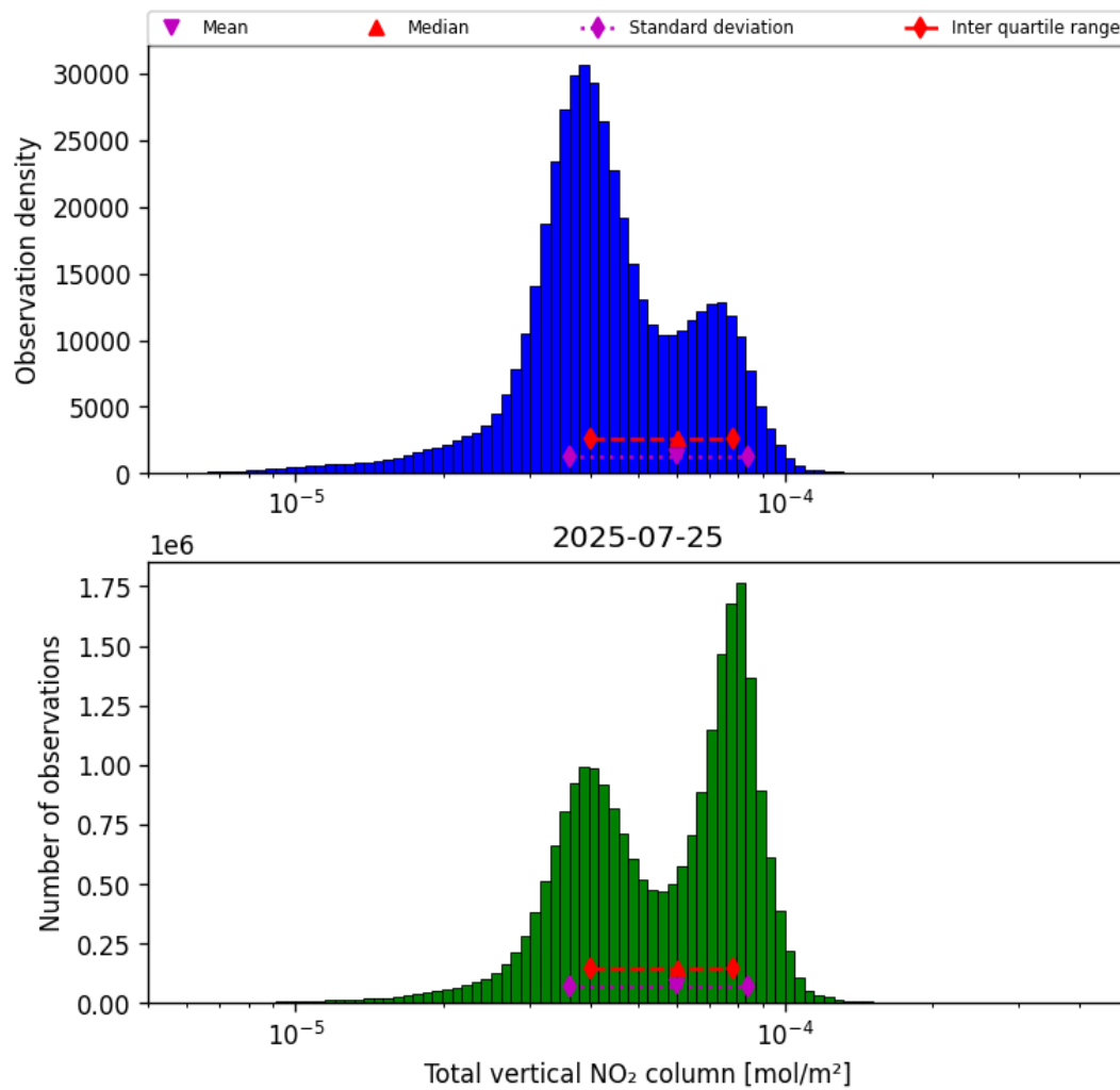
Figure 36: Histogram of “Total vertical NO 2 column” for 2025-07-25 to 2025-07-26
