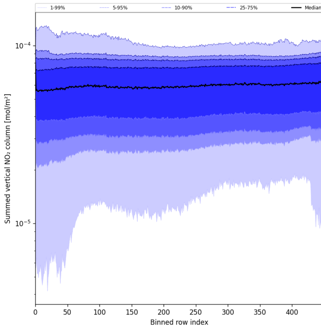
Figure 55: Along track statistics of “Summed vertical NO 2 column” for 2025-07-25 to 2025-07-26
