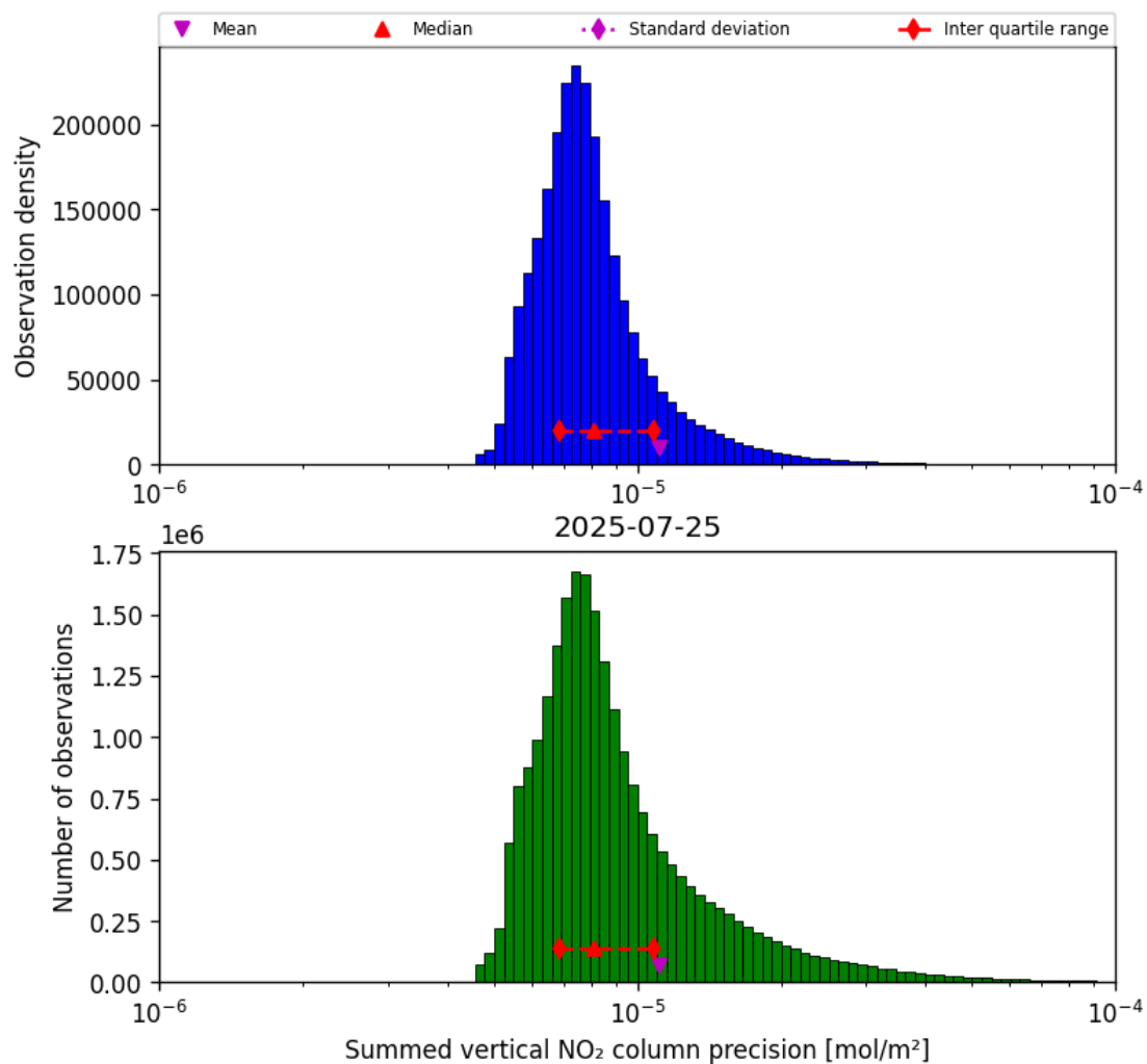
Figure 39: Histogram of "Summed vertical NO 2 column precision" for 2025-07-25 to 2025-07-26
