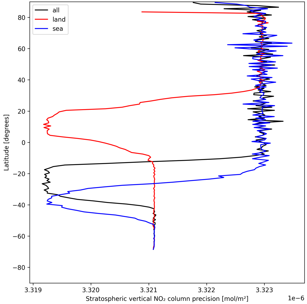
Figure 18: Zonal average of “Stratospheric vertical NO 2 column precision” for 2025-07-25 to 2025-07-26.
