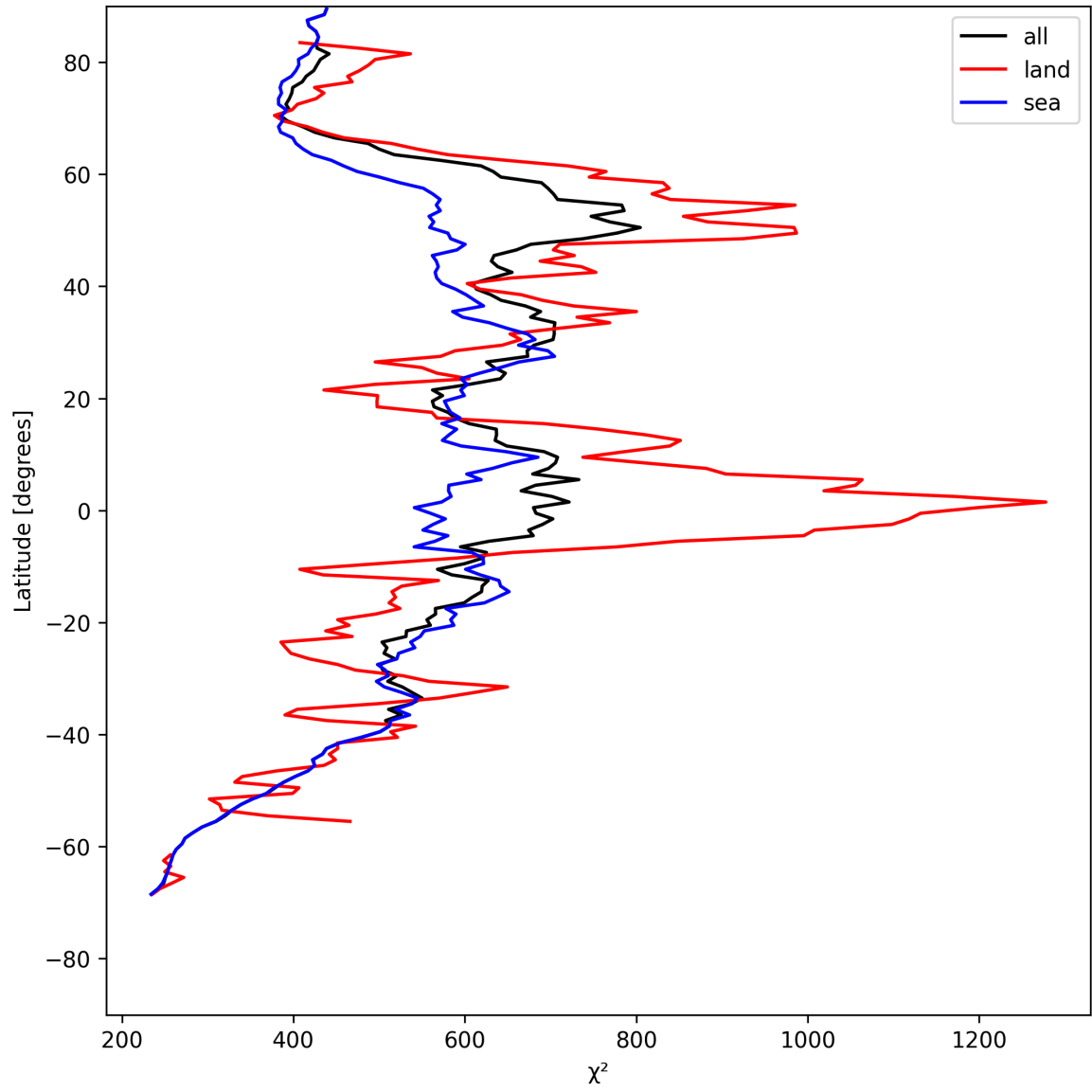
Figure 23: Zonal average of “ \chi^2 ” for 2025-07-25 to 2025-07-26.
