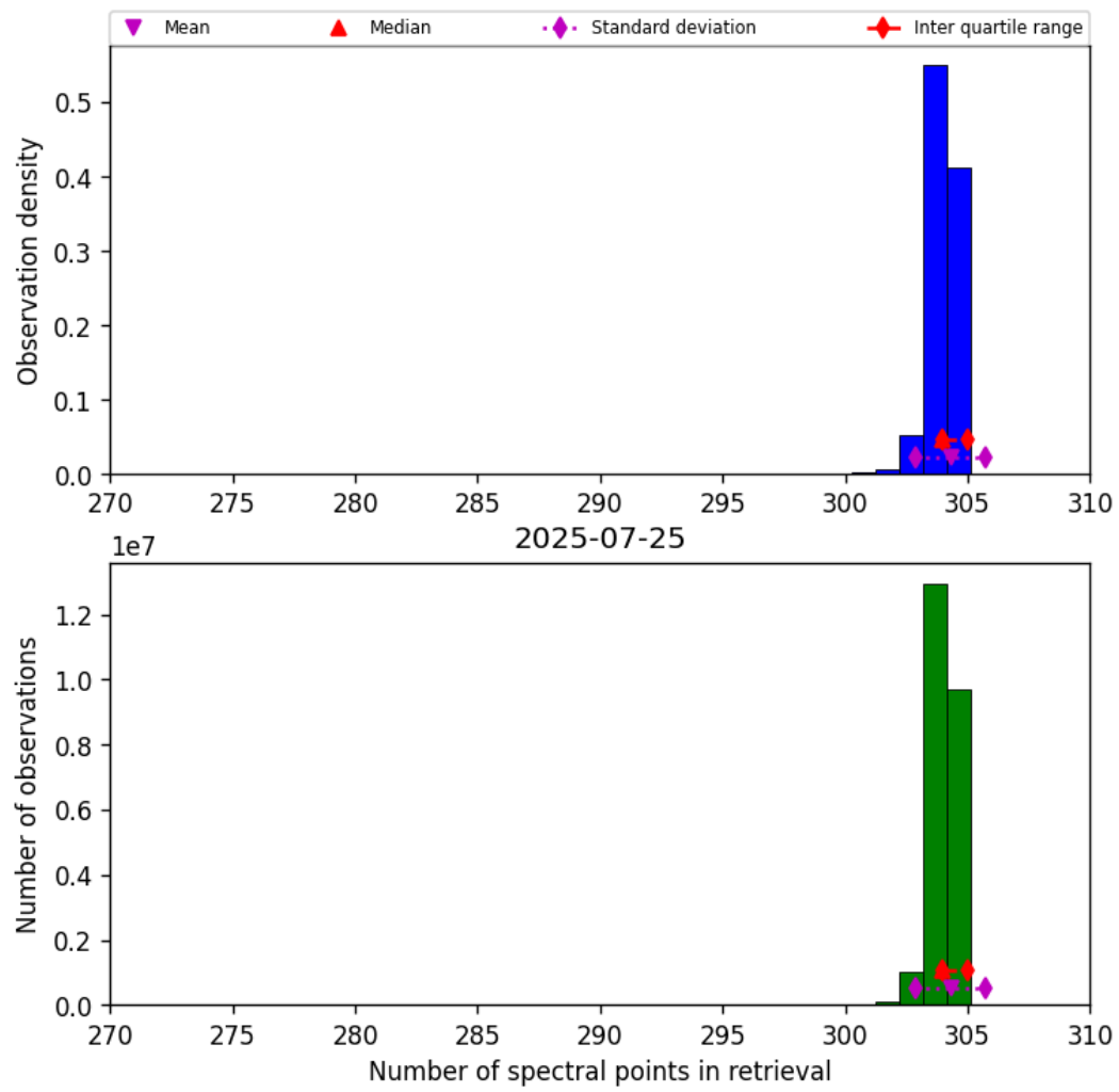
Figure 31: Histogram of “Number of spectral points in retrieval” for 2025-07-25 to 2025-07-26
