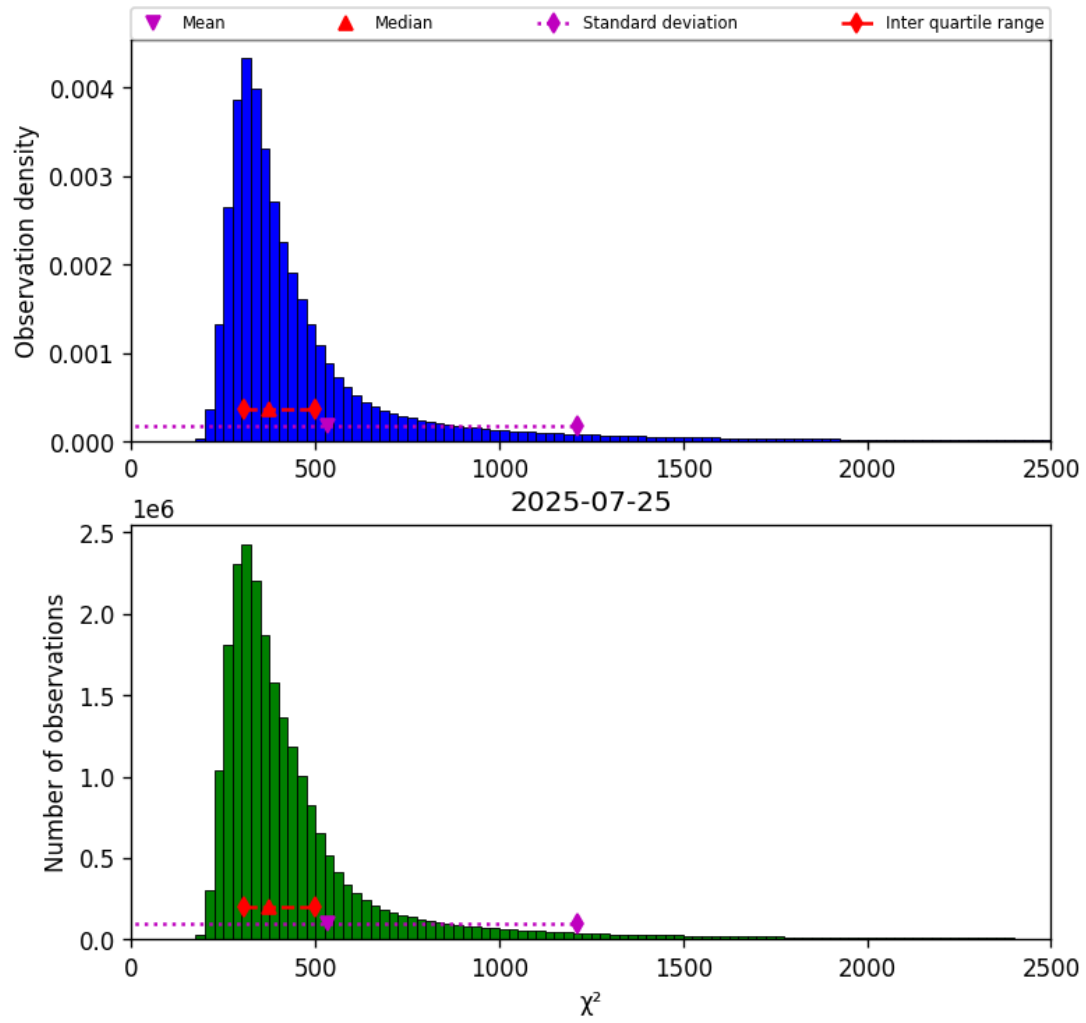
Figure 40: Histogram of “ \chi^2 ” for 2025-07-25 to 2025-07-26
