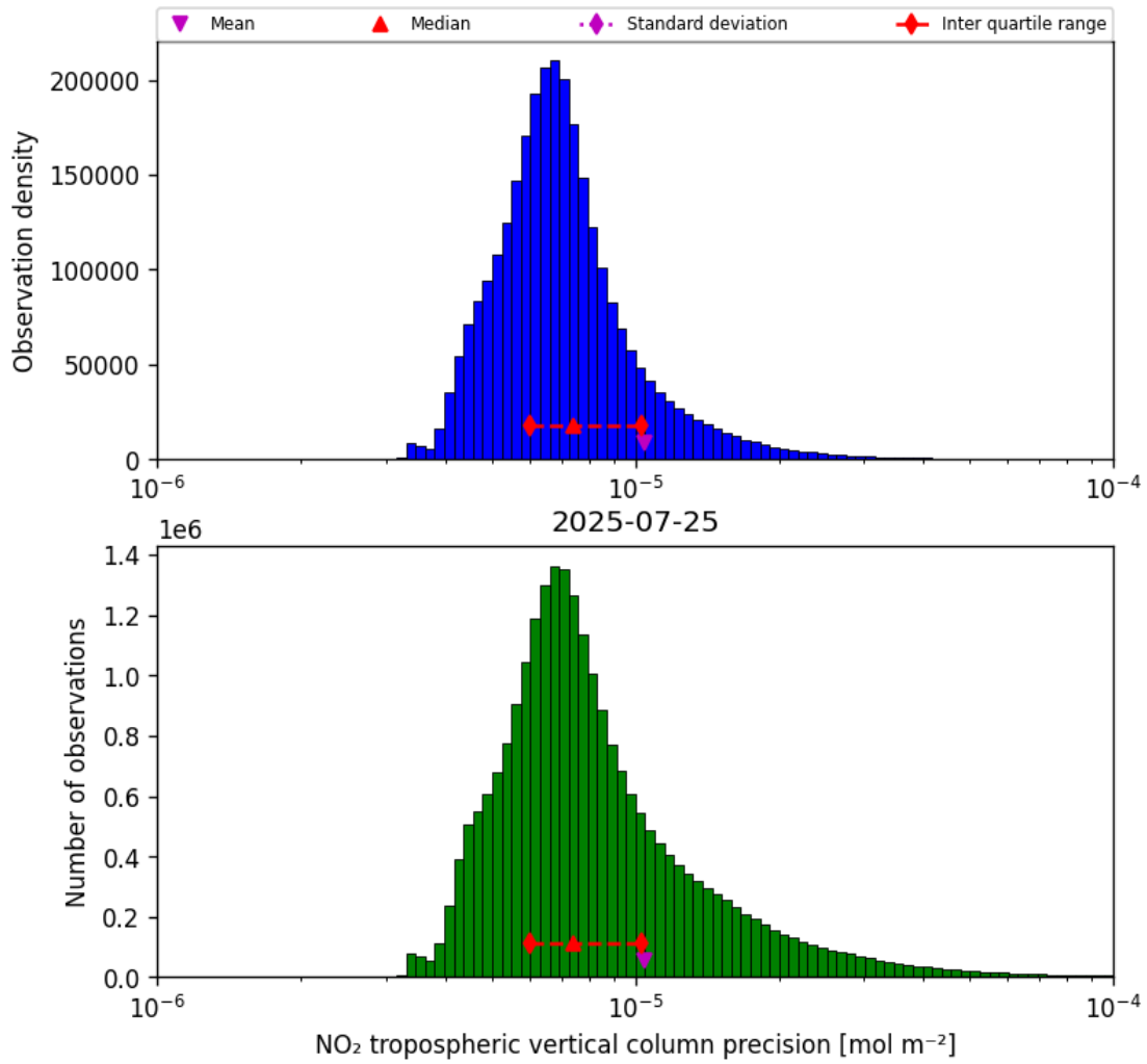
Figure 28: Histogram of “NO 2 tropospheric vertical column precision” for 2025-07-25 to 2025-07-26
