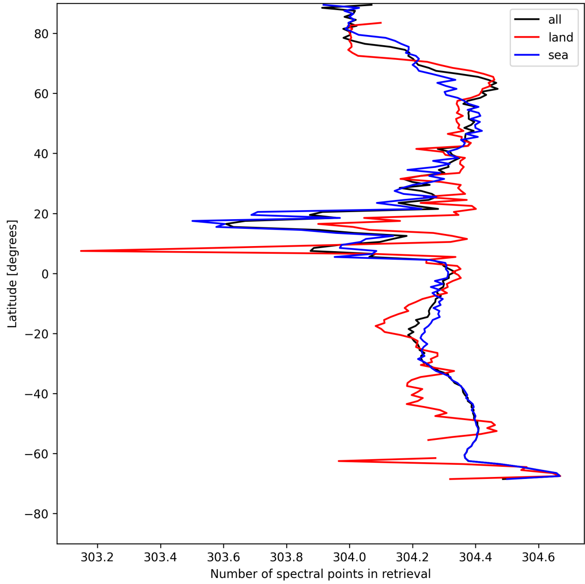
Figure 14: Zonal average of “Number of spectral points in retrieval” for 2025-07-25 to 2025-07-26.
