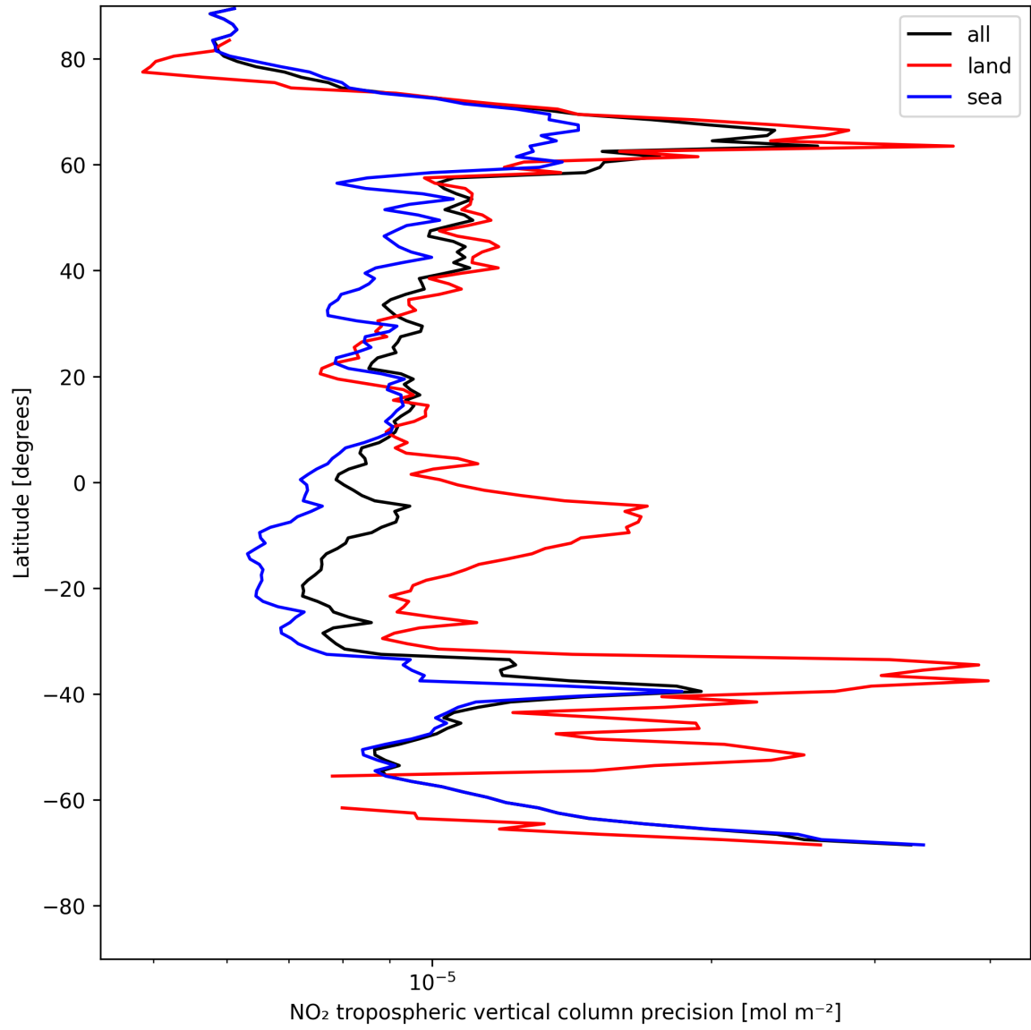
Figure 11: Zonal average of “NO 2 tropospheric vertical column precision” for 2025-07-25 to 2025-07-26.
