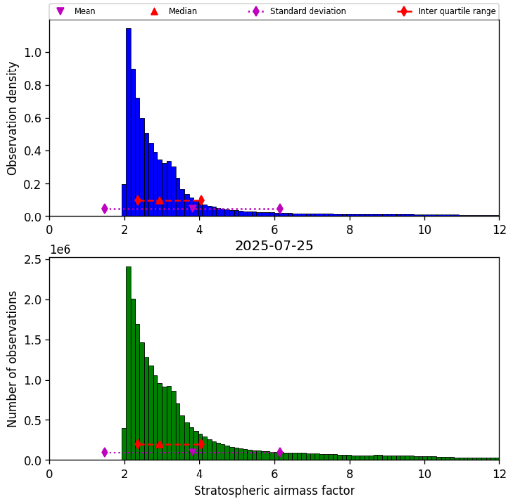
Figure 42: Histogram of “Stratospheric airmass factor” for 2025-07-25 to 2025-07-26
