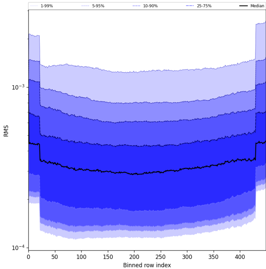
Figure 58: Along track statistics of “RMS” for 2025-07-25 to 2025-07-26
